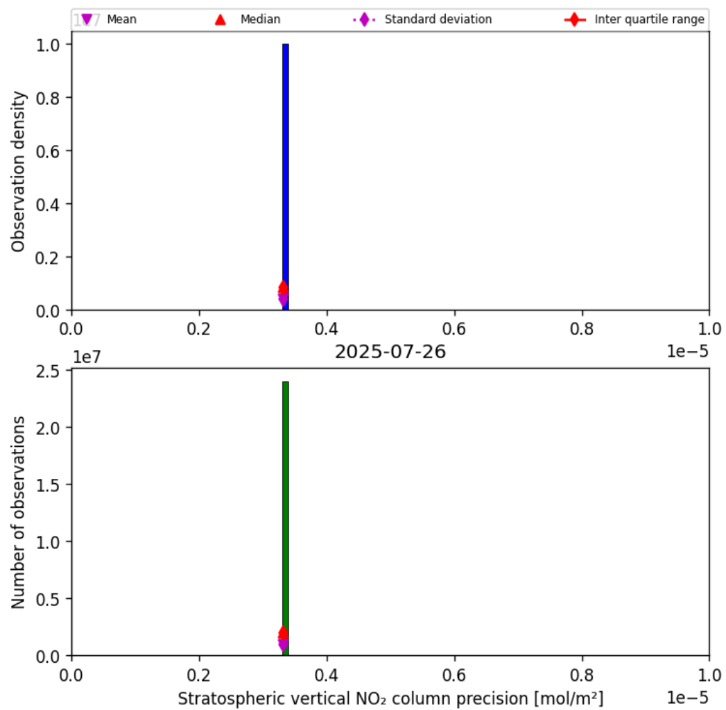
Figure 35: Histogram of “Stratospheric vertical NO 2 column precision” for 2025-07-26 to 2025-07-27
