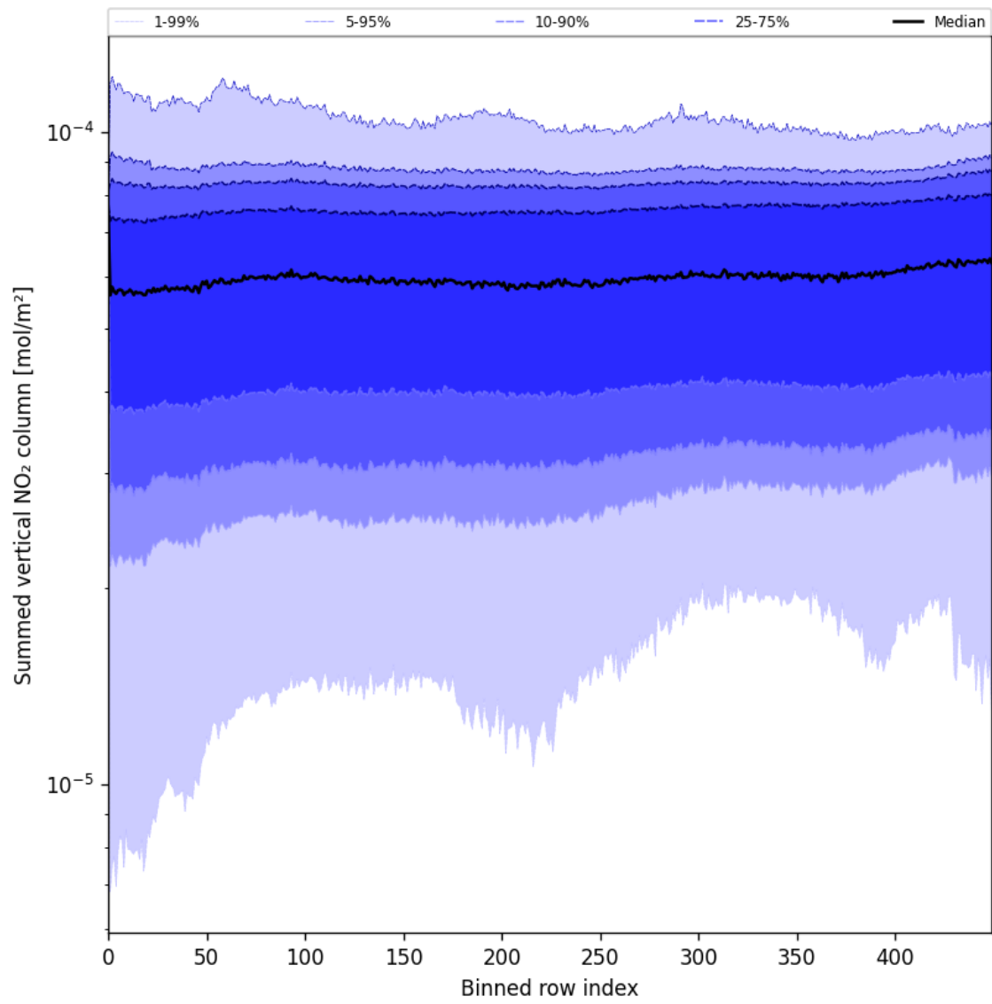
Figure 55: Along track statistics of “Summed vertical NO 2 column” for 2025-07-26 to 2025-07-27
