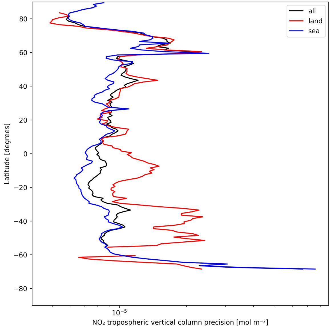
Figure 11: Zonal average of “NO 2 tropospheric vertical column precision” for 2025-07-26 to 2025-07-27.
