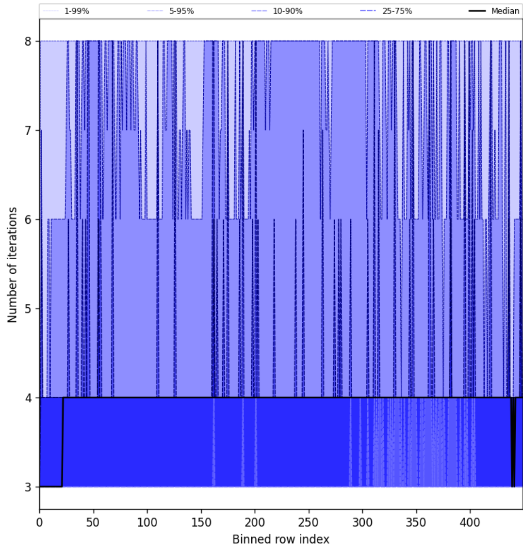
Figure 49: Along track statistics of “Number of iterations” for 2025-07-26 to 2025-07-27
