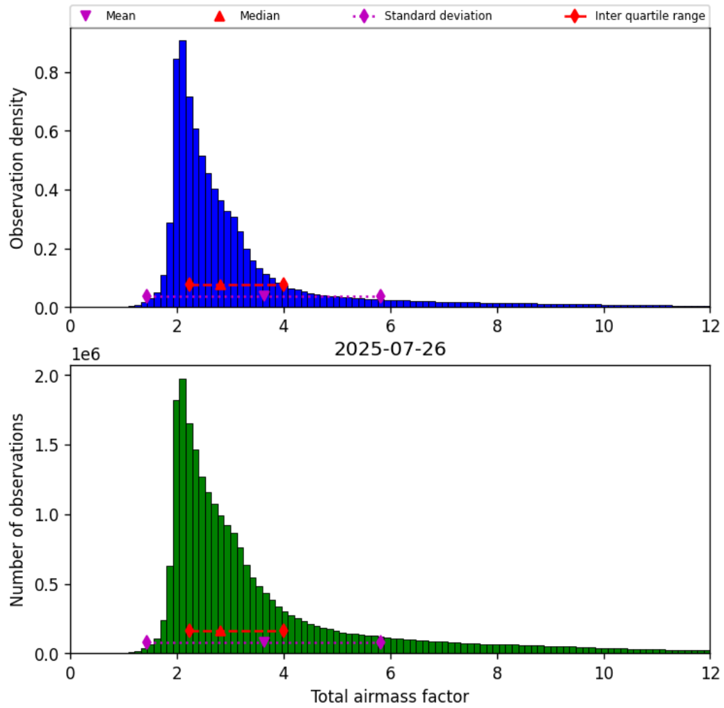
Figure 30: Histogram of “Total airmass factor” for 2025-07-26 to 2025-07-27
