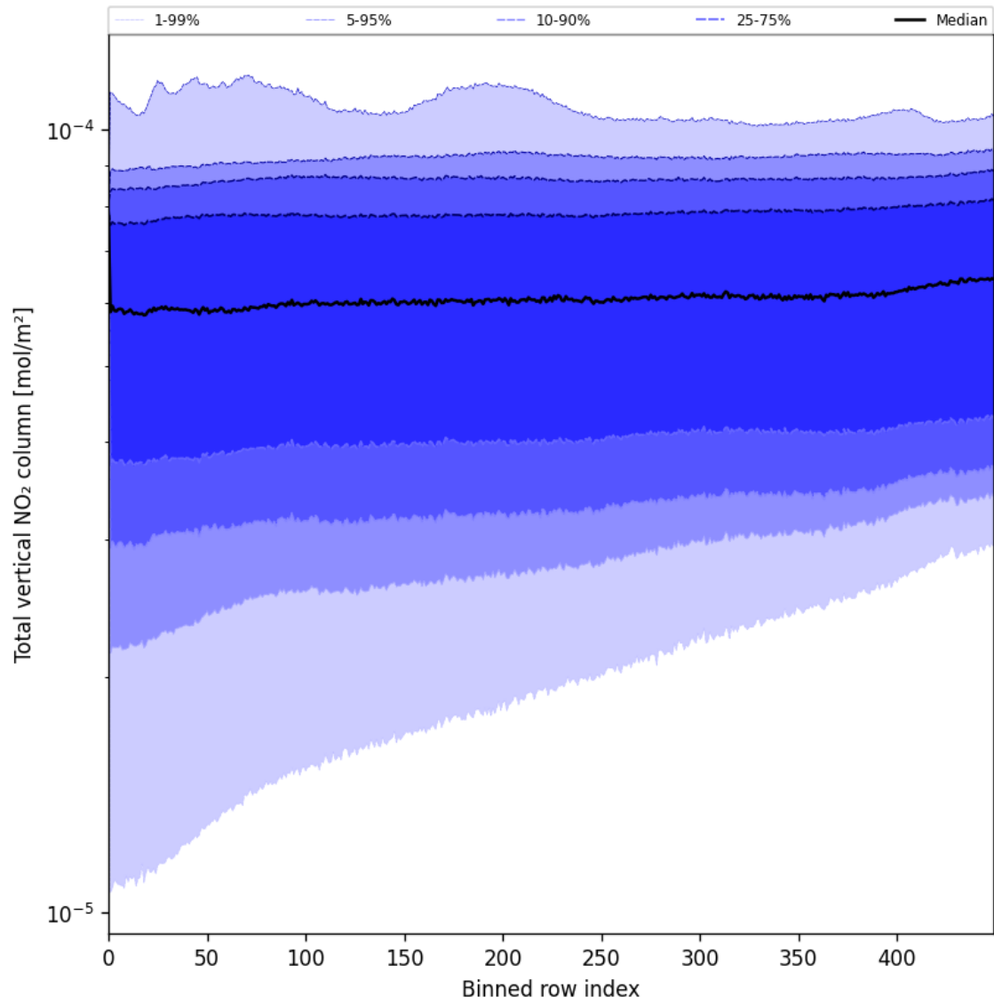
Figure 53: Along track statistics of “Total vertical NO 2 column” for 2025-07-26 to 2025-07-27
