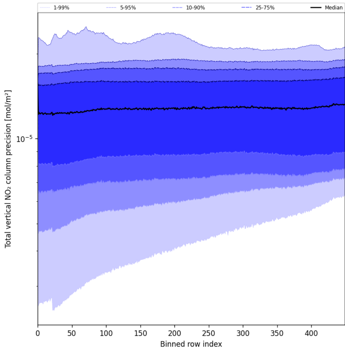
Figure 54: Along track statistics of “Total vertical NO 2 column precision” for 2025-07-26 to 2025-07-27
