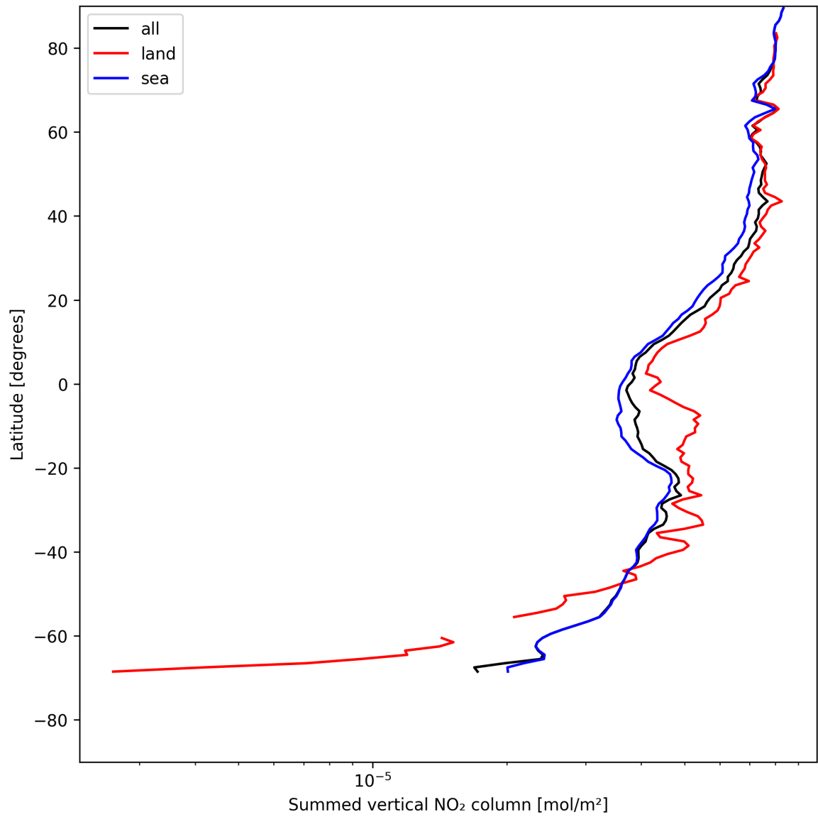
Figure 21: Zonal average of “Summed vertical NO 2 column” for 2025-07-26 to 2025-07-27.
