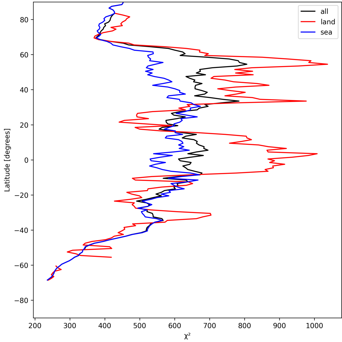
Figure 23: Zonal average of “ \chi^2 ” for 2025-07-26 to 2025-07-27.
