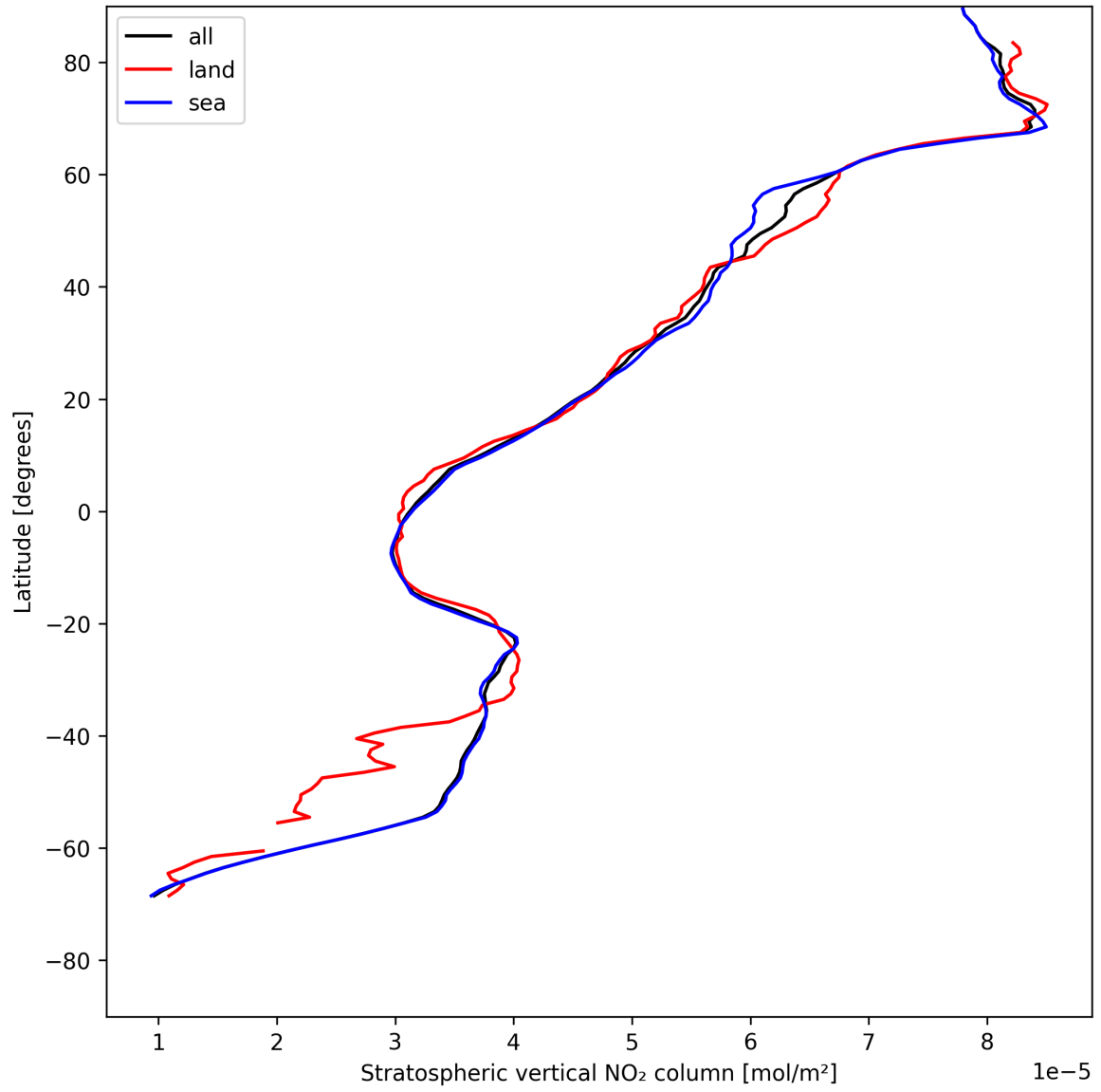
Figure 17: Zonal average of “Stratospheric vertical NO 2 column” for 2025-07-26 to 2025-07-27.
