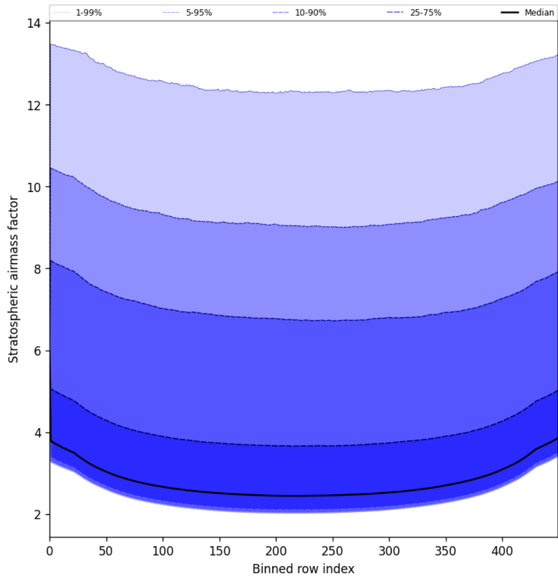
Figure 59: Along track statistics of “Stratospheric airmass factor” for 2025-07-26 to 2025-07-27
