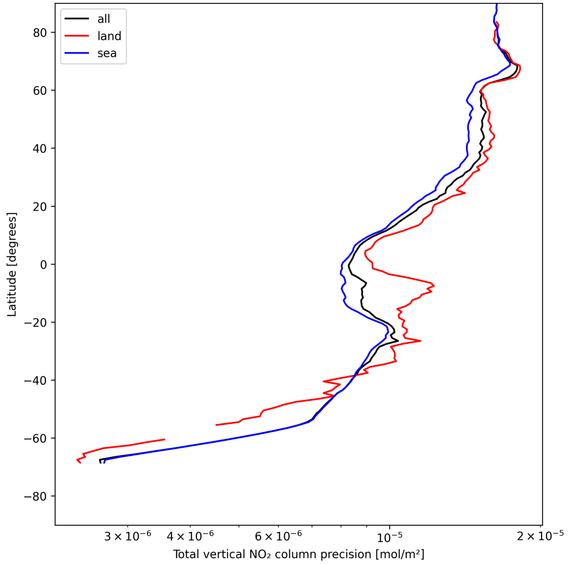
Figure 20: Zonal average of “Total vertical NO 2 column precision” for 2025-07-26 to 2025-07-27.
