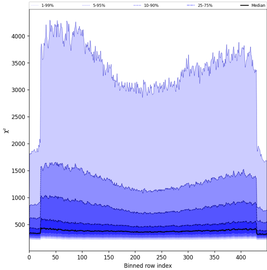
Figure 57: Along track statistics of “ \chi^2 ” for 2025-07-26 to 2025-07-27
