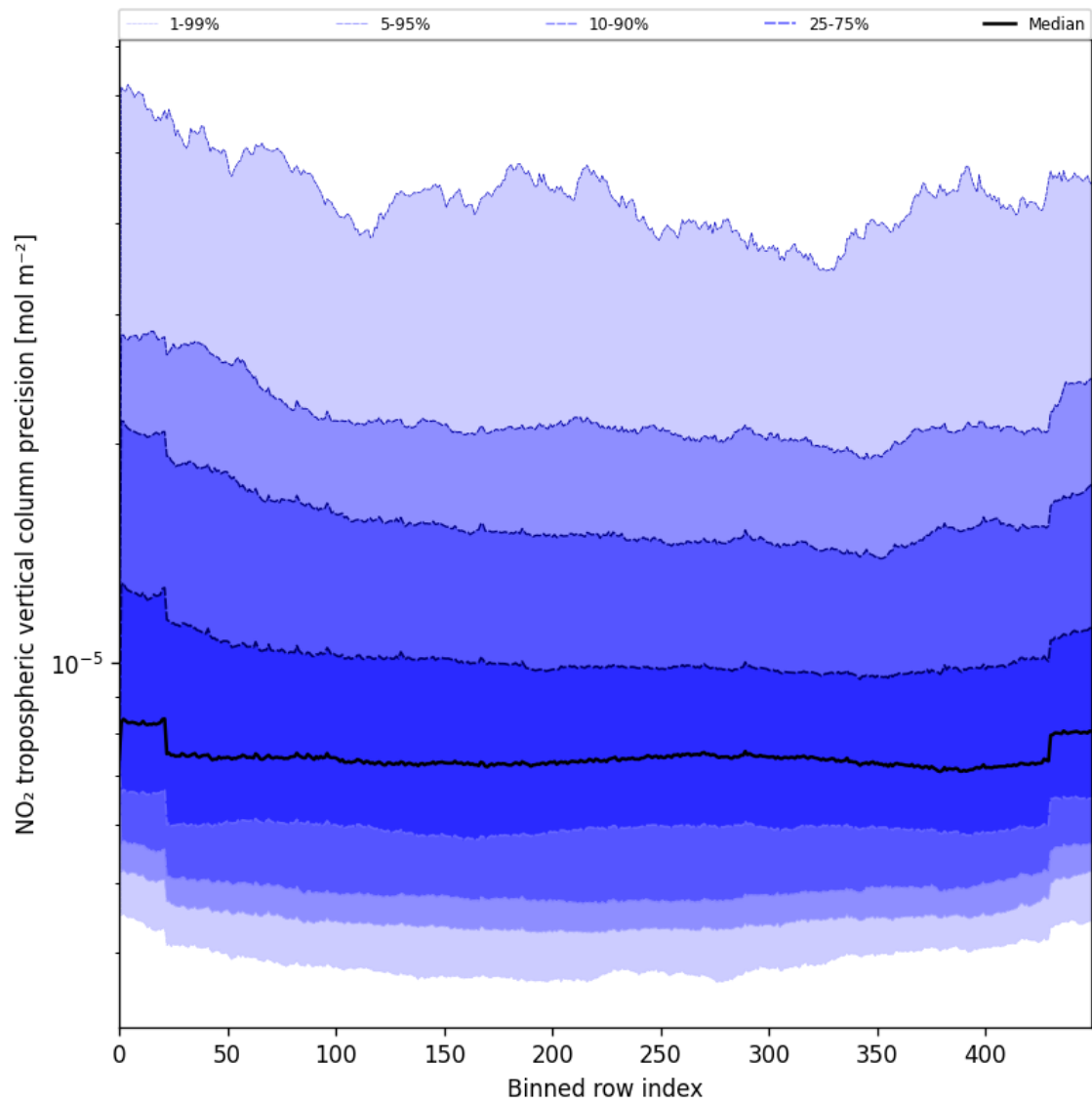
Figure 45: Along track statistics of “NO 2 tropospheric vertical column precision” for 2025-07-26 to 2025-07-27
