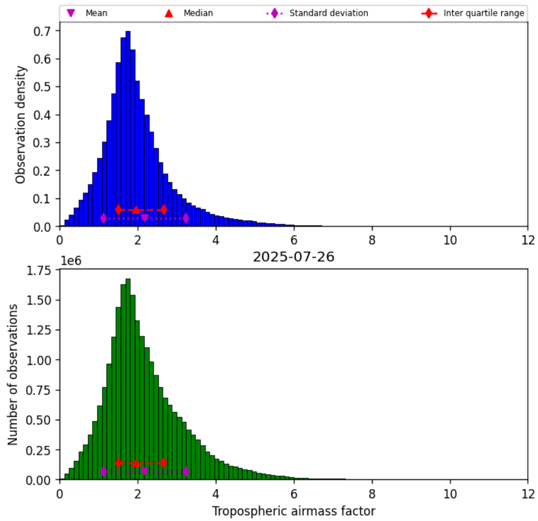
Figure 29: Histogram of “Tropospheric airmass factor” for 2025-07-26 to 2025-07-27
