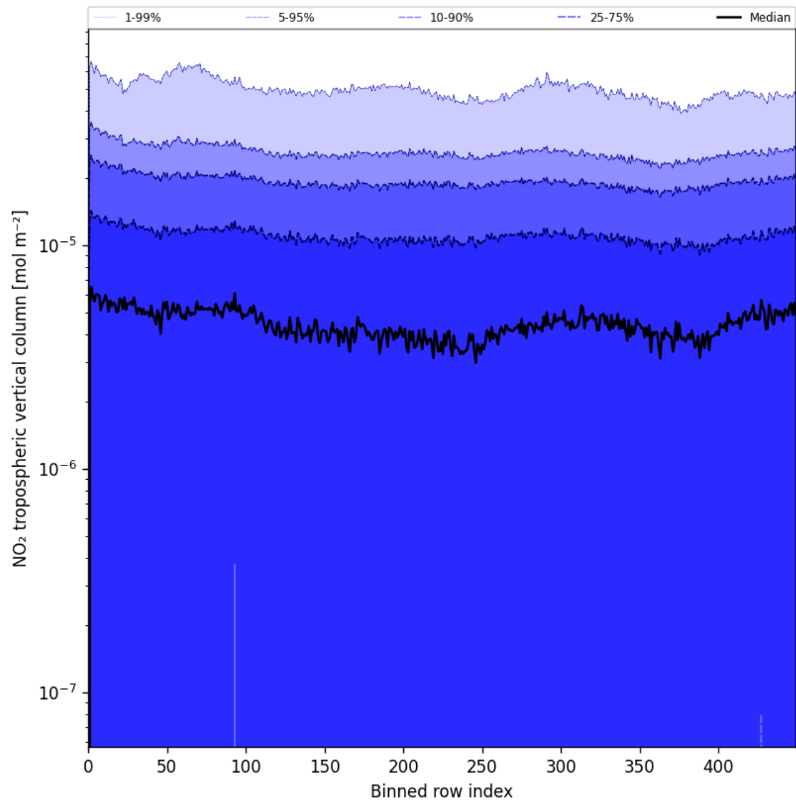
Figure 44: Along track statistics of “NO 2 tropospheric vertical column” for 2025-07-26 to 2025-07-27
