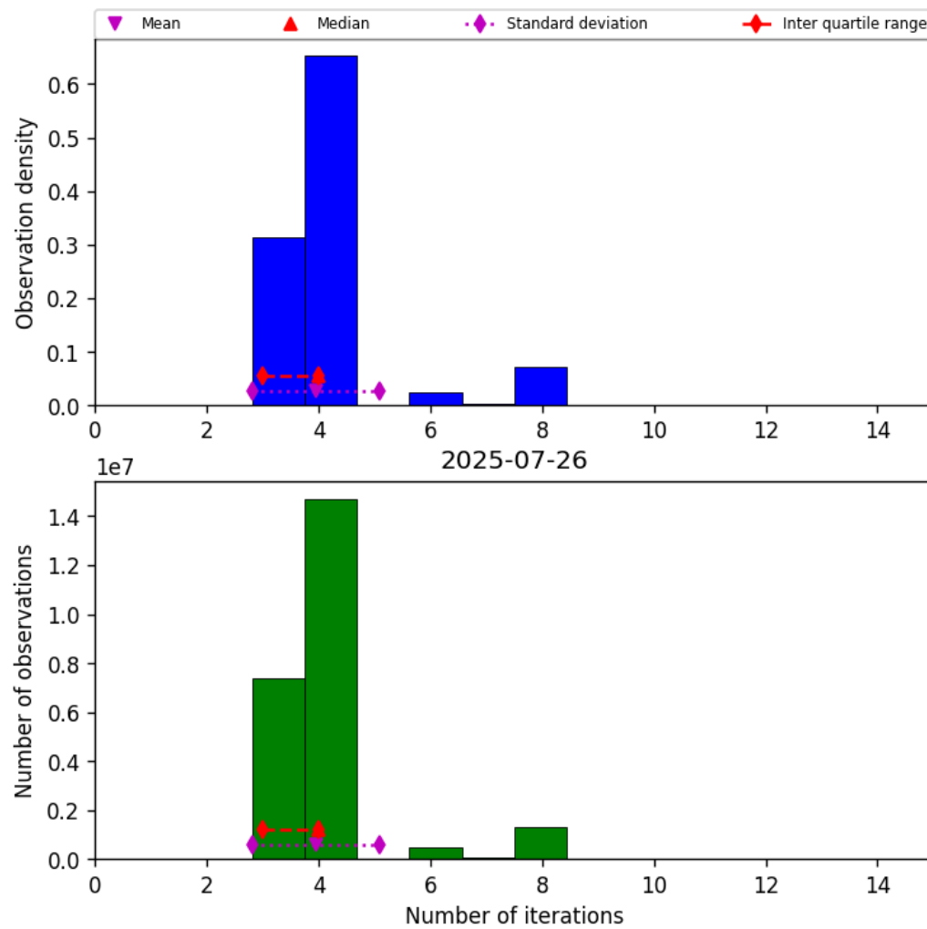
Figure 32: Histogram of “Number of iterations” for 2025-07-26 to 2025-07-27
