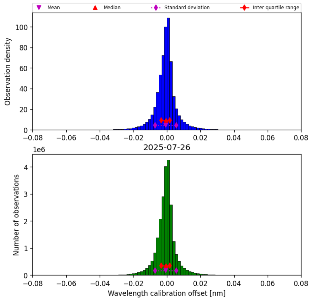
Figure 33: Histogram of “Wavelength calibration offset” for 2025-07-26 to 2025-07-27
