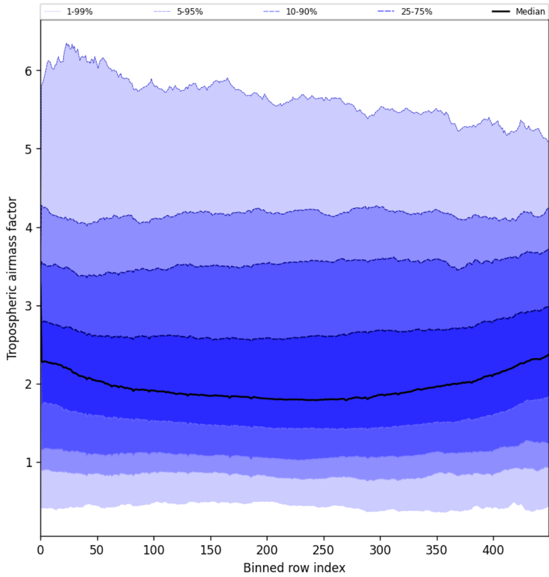
Figure 46: Along track statistics of “Tropospheric airmass factor” for 2025-07-26 to 2025-07-27
