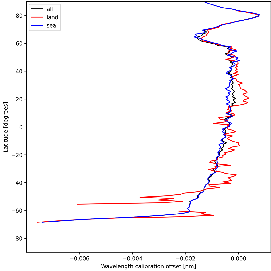
Figure 16: Zonal average of “Wavelength calibration offset” for 2025-07-26 to 2025-07-27.
