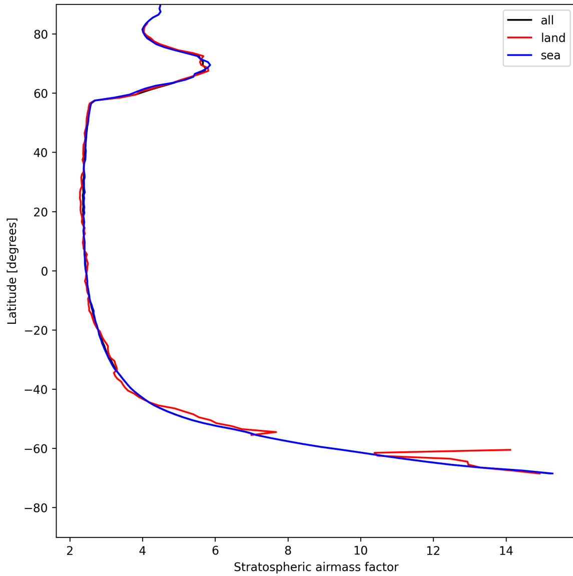
Figure 25: Zonal average of “Stratospheric airmass factor” for 2025-07-26 to 2025-07-27.
