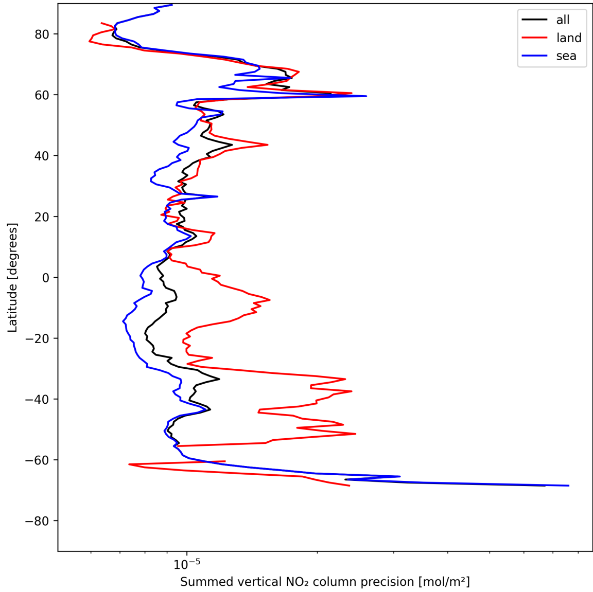
Figure 22: Zonal average of “Summed vertical NO 2 column precision” for 2025-07-26 to 2025-07-27.
