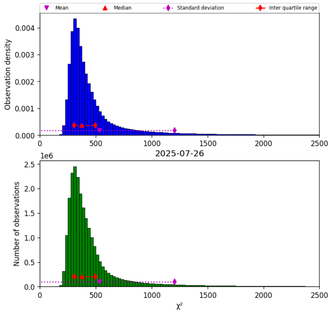
Figure 40: Histogram of “ \chi^2 ” for 2025-07-26 to 2025-07-27
