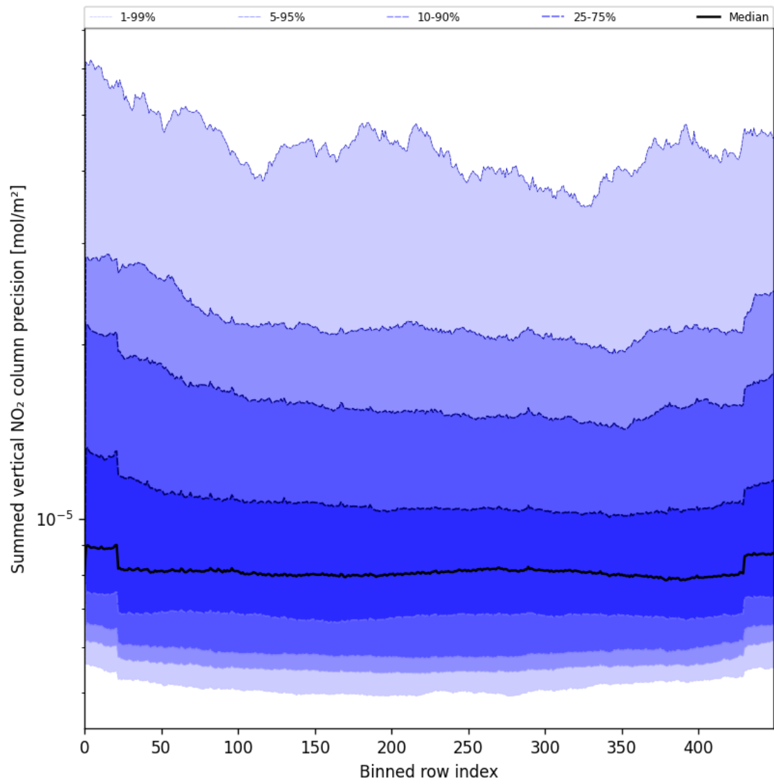
Figure 56: Along track statistics of “Summed vertical NO 2 column precision” for 2025-07-26 to 2025-07-27
