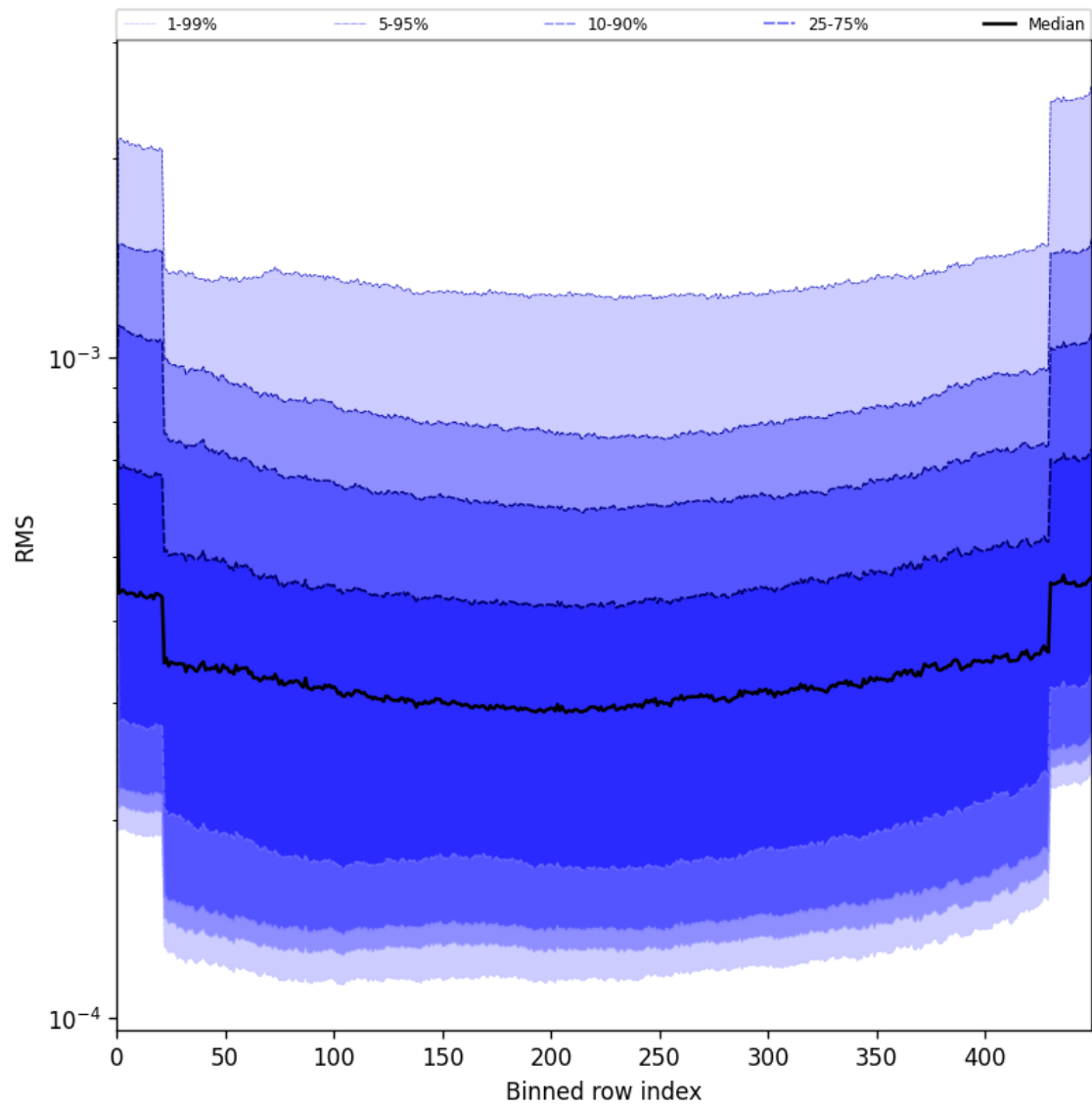
Figure 58: Along track statistics of “RMS” for 2025-07-26 to 2025-07-27
