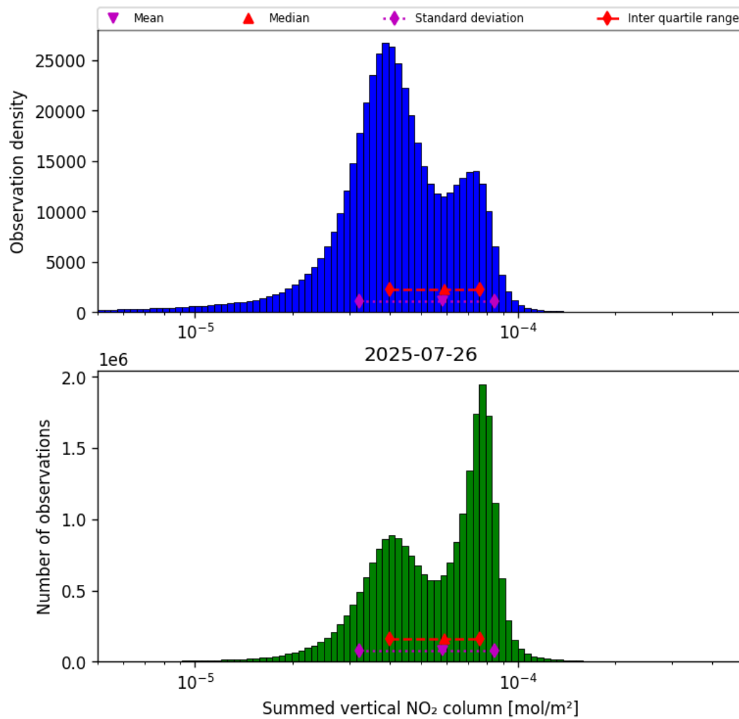
Figure 38: Histogram of “Summed vertical NO 2 column” for 2025-07-26 to 2025-07-27
