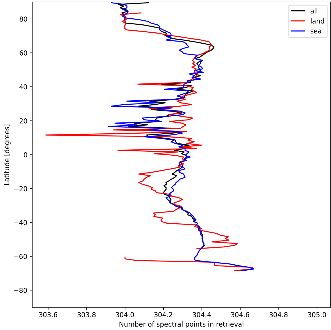
Figure 14: Zonal average of “Number of spectral points in retrieval” for 2025-07-26 to 2025-07-27.
