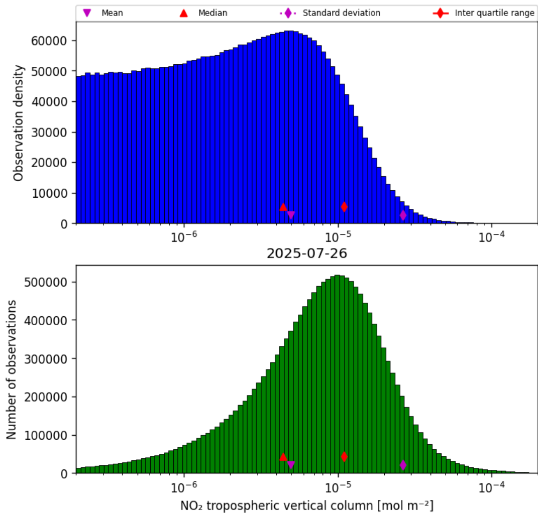
Figure 27: Histogram of “NO 2 tropospheric vertical column” for 2025-07-26 to 2025-07-27
