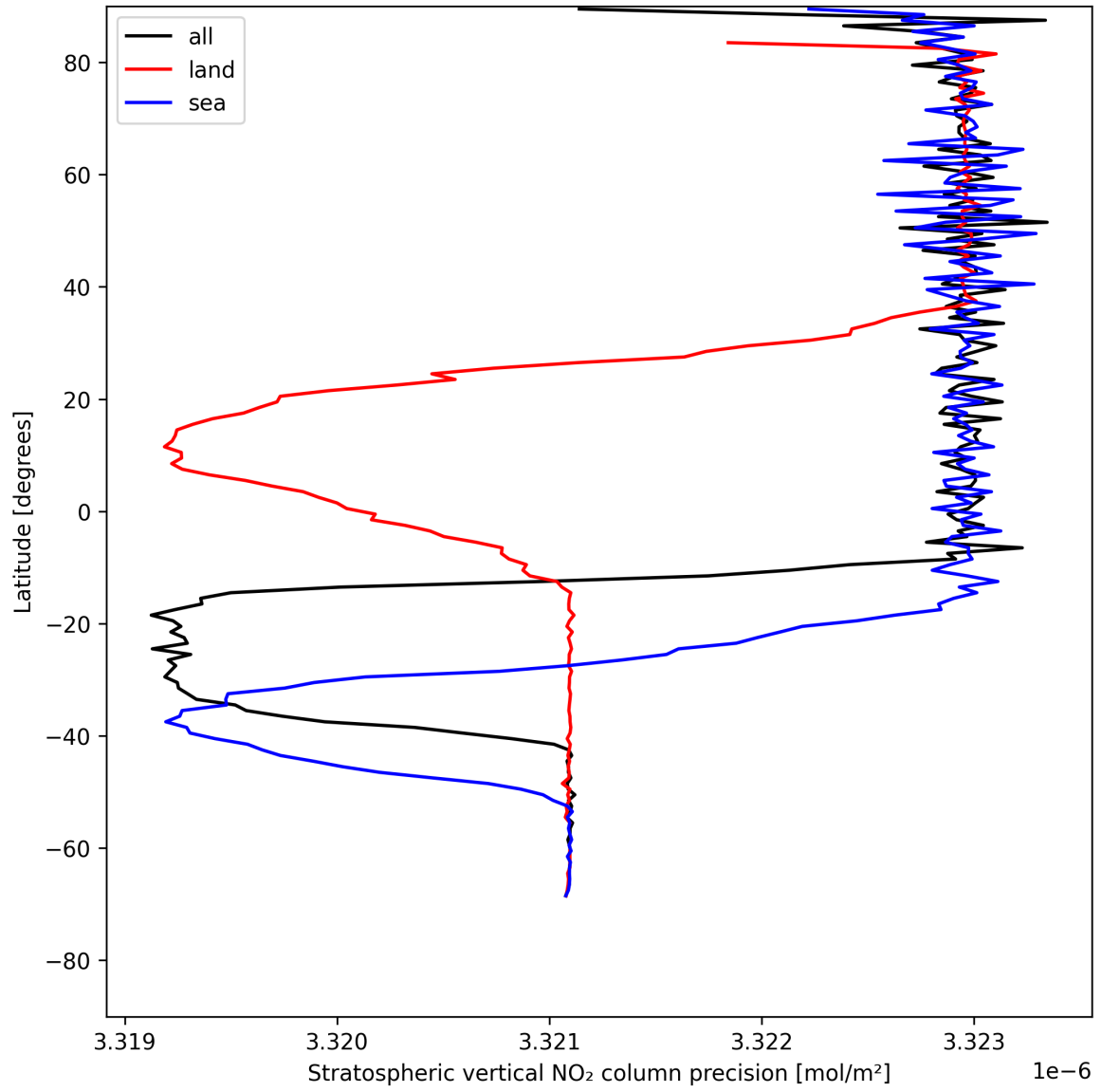
Figure 18: Zonal average of “Stratospheric vertical NO 2 column precision” for 2025-07-26 to 2025-07-27.
