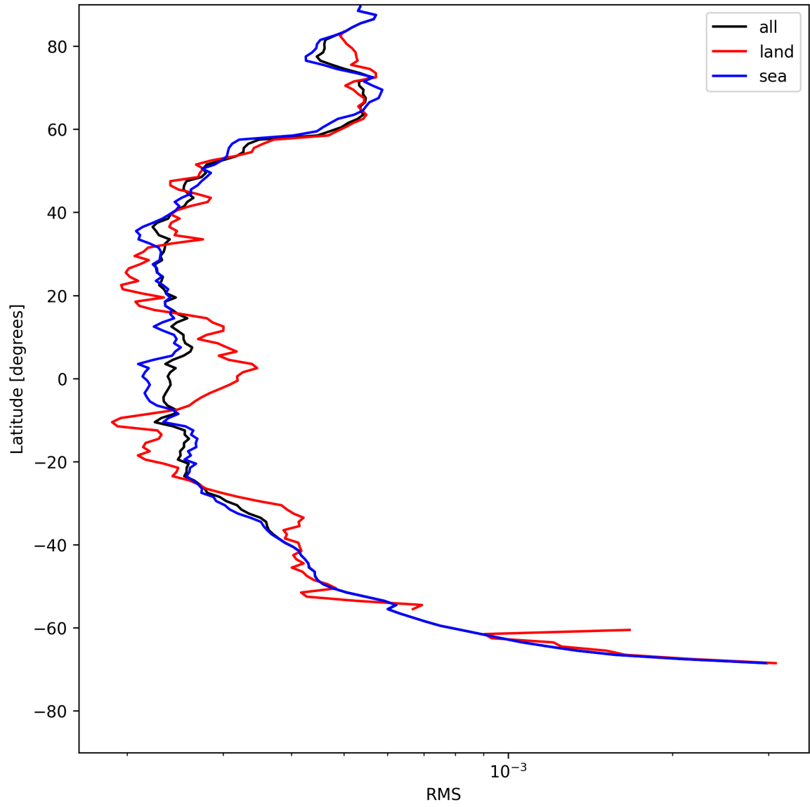
Figure 24: Zonal average of “RMS” for 2025-07-26 to 2025-07-27.
