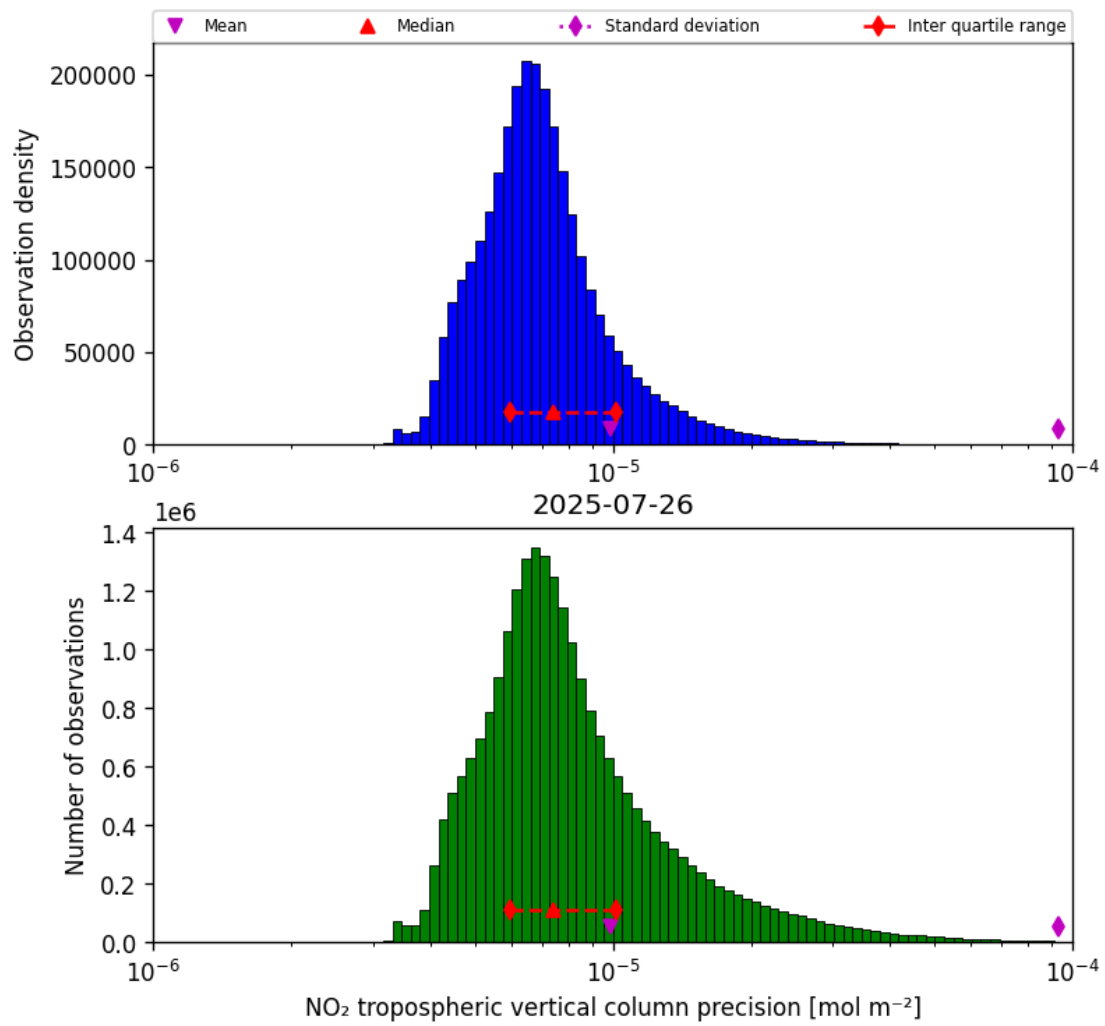
Figure 28: Histogram of “NO 2 tropospheric vertical column precision” for 2025-07-26 to 2025-07-27
