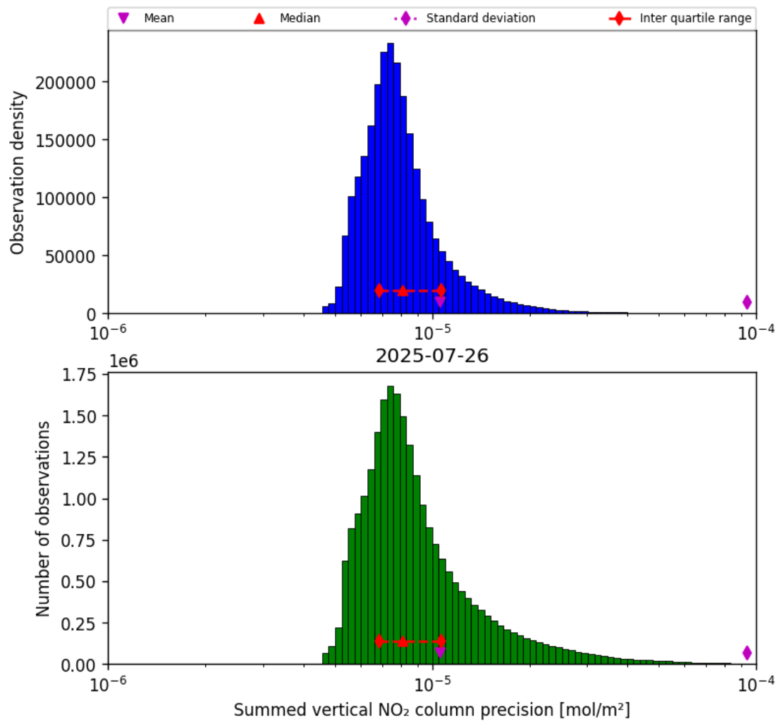
Figure 39: Histogram of “Summed vertical NO 2 column precision” for 2025-07-26 to 2025-07-27
