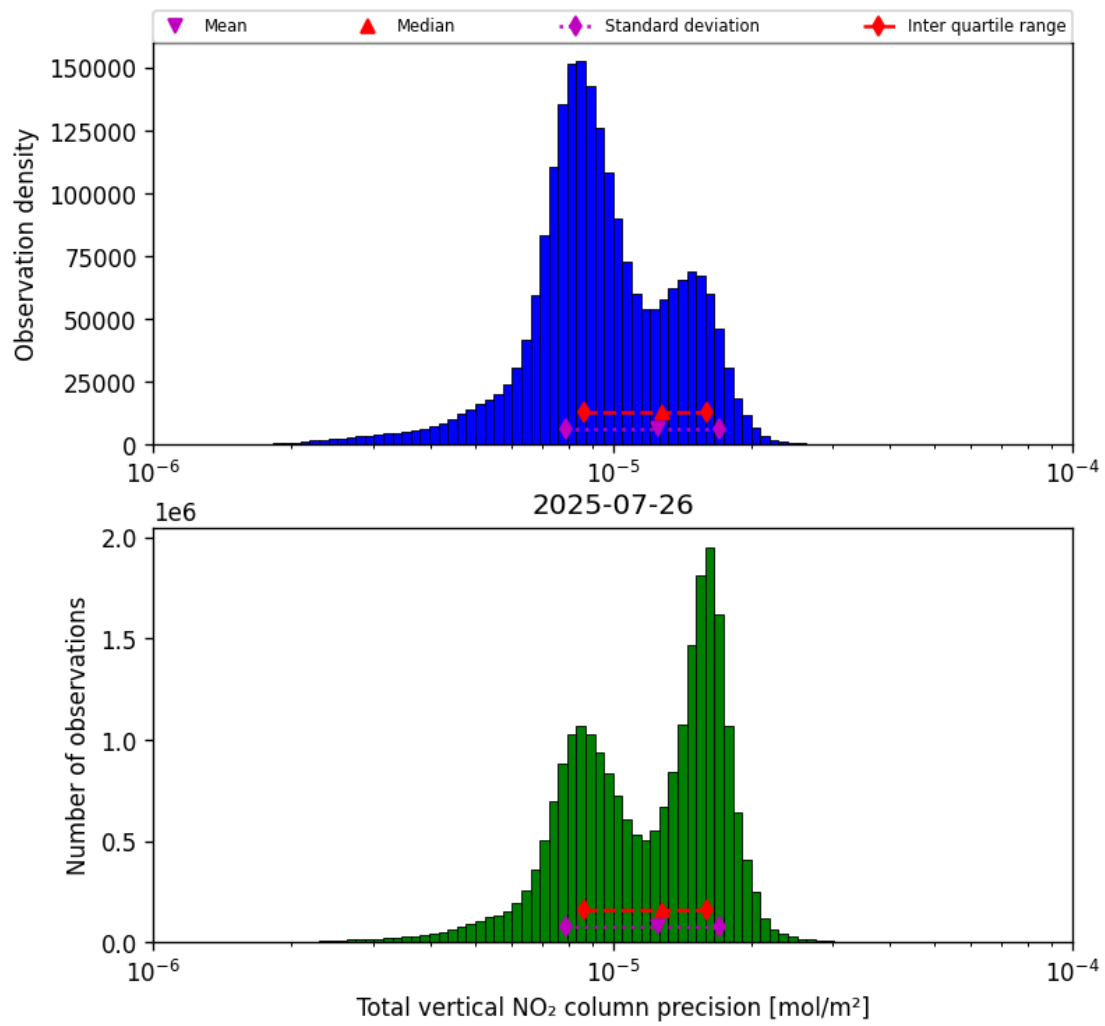
Figure 37: Histogram of “Total vertical NO 2 column precision” for 2025-07-26 to 2025-07-27
