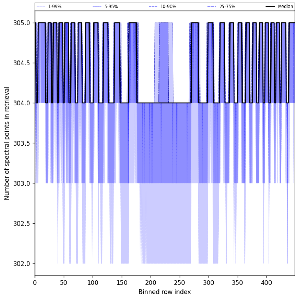
Figure 48: Along track statistics of “Number of spectral points in retrieval” for 2025-07-26 to 2025-07-27
