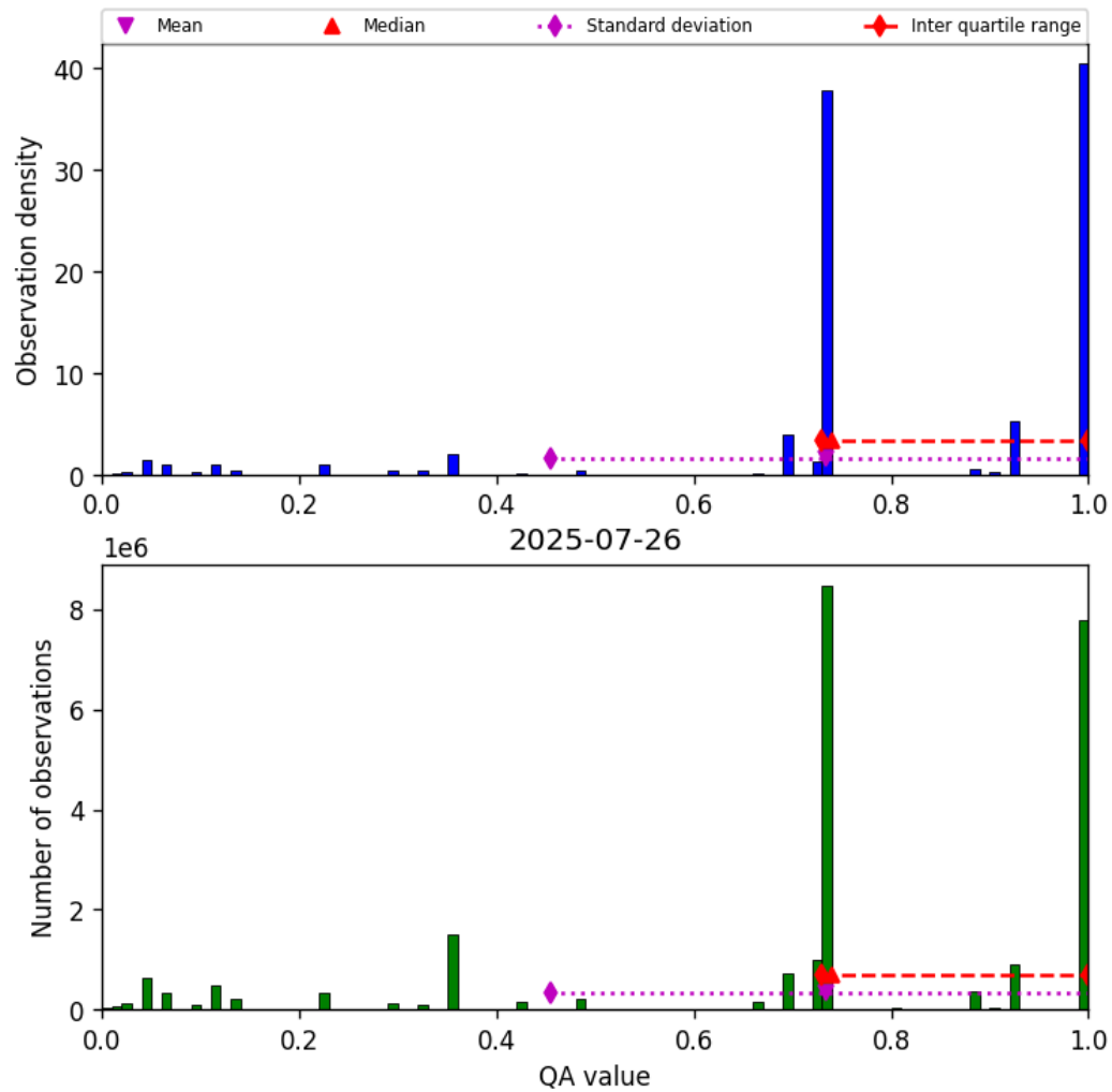
Figure 26: Histogram of “QA value” for 2025-07-26 to 2025-07-27
