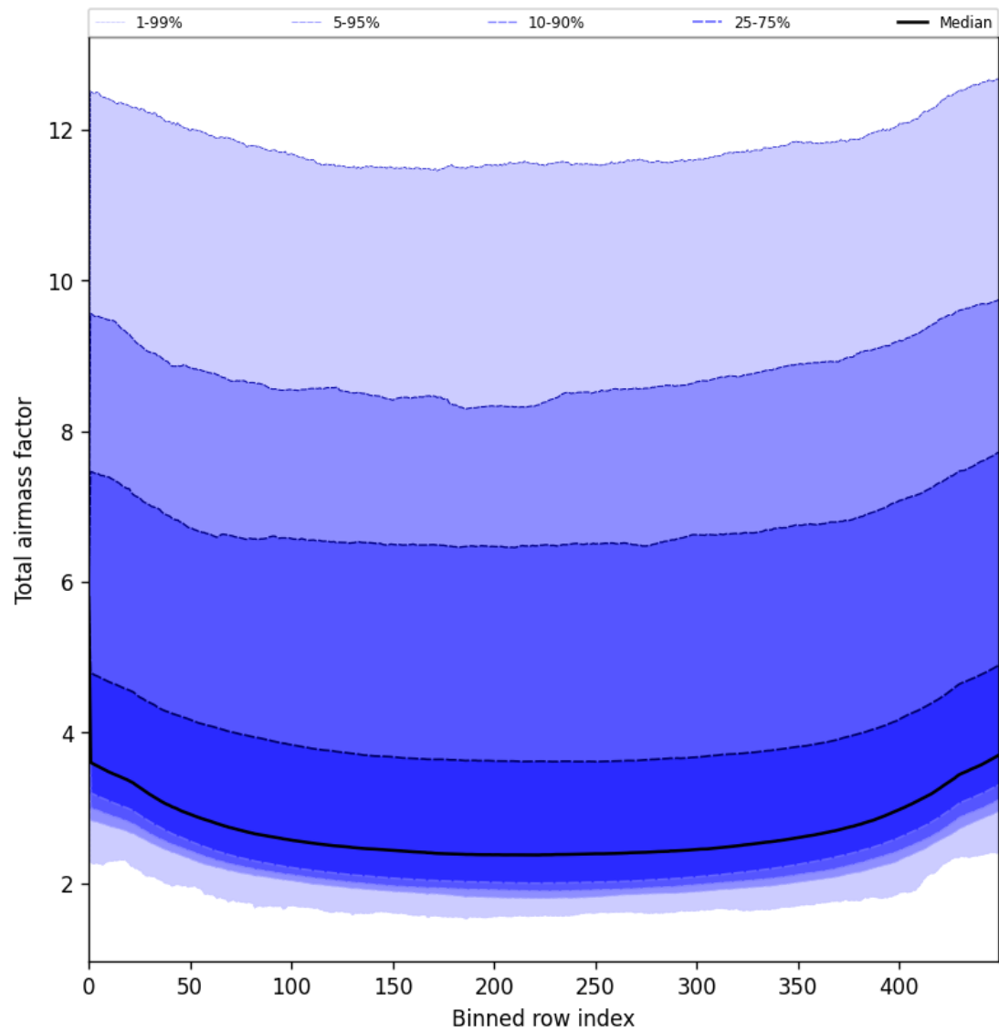
Figure 47: Along track statistics of “Total airmass factor” for 2025-07-26 to 2025-07-27
