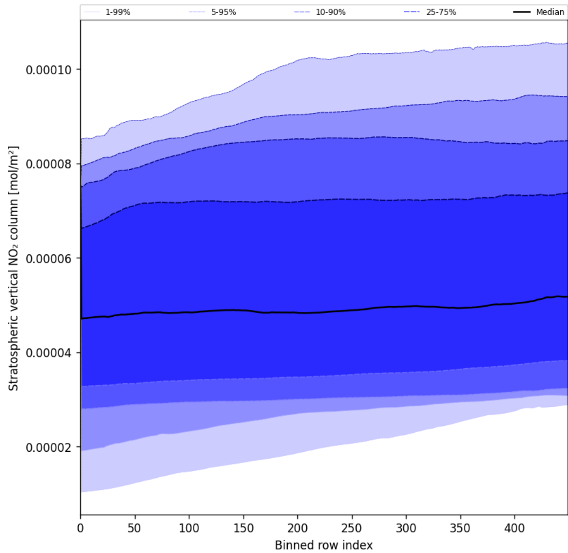
Figure 51: Along track statistics of “Stratospheric vertical NO 2 column” for 2025-07-26 to 2025-07-27
