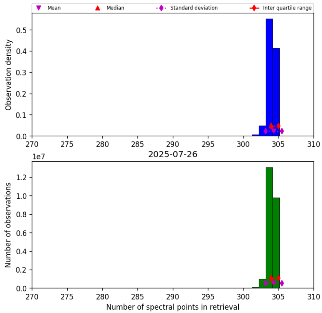
Figure 31: Histogram of “Number of spectral points in retrieval” for 2025-07-26 to 2025-07-27
