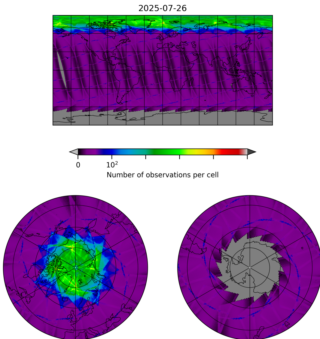
Figure 8: Map of the number of observations for 2025-07-26 to 2025-07-27
