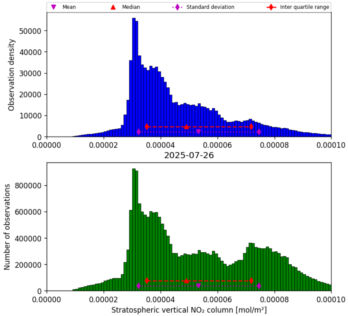
Figure 34: Histogram of “Stratospheric vertical NO 2 column” for 2025-07-26 to 2025-07-27
