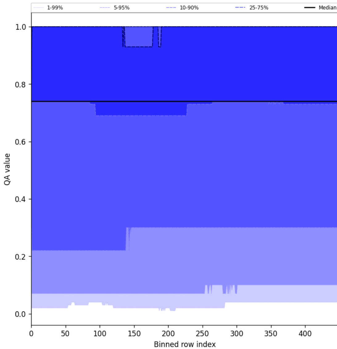
Figure 43: Along track statistics of “QA value” for 2025-07-26 to 2025-07-27
