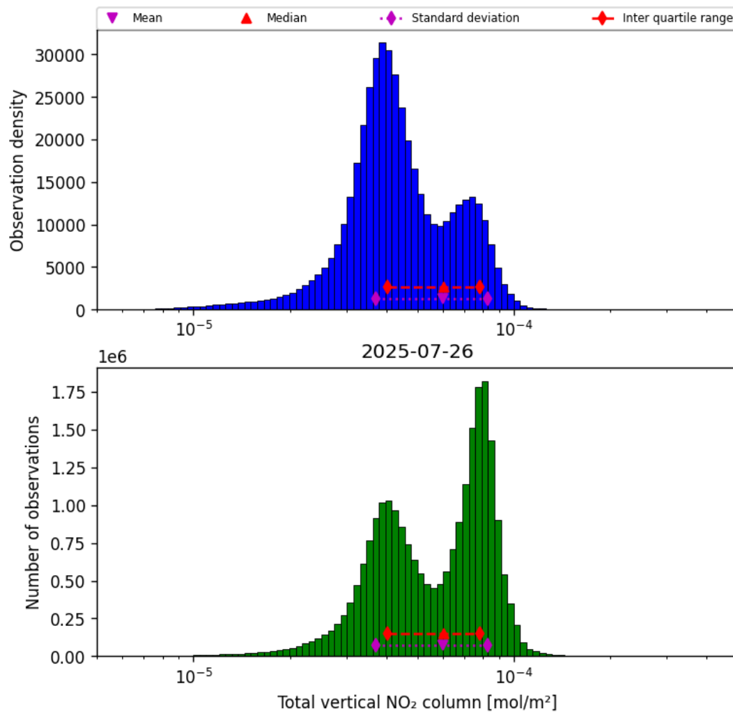
Figure 36: Histogram of “Total vertical NO 2 column” for 2025-07-26 to 2025-07-27
