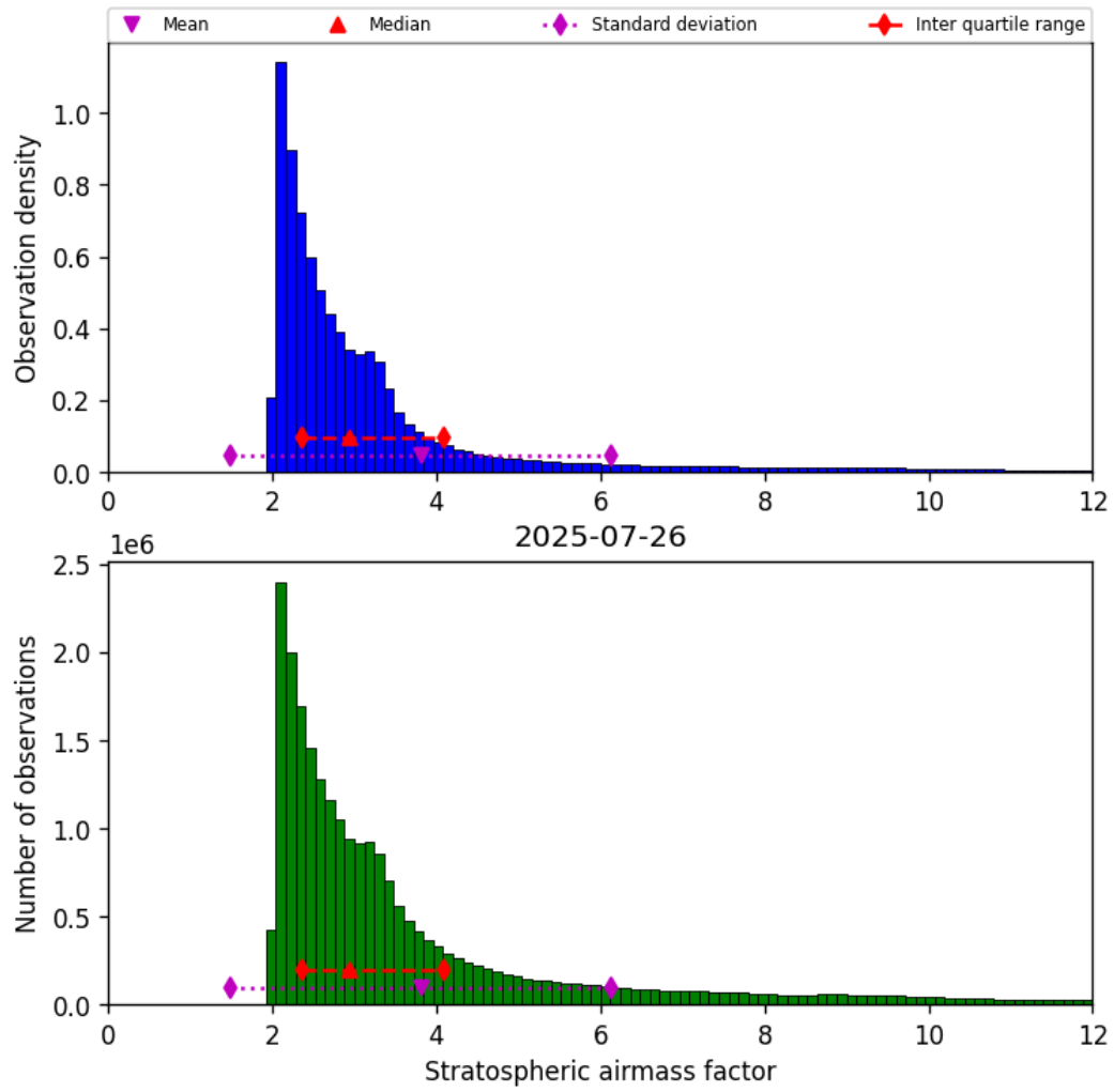
Figure 42: Histogram of “Stratospheric airmass factor” for 2025-07-26 to 2025-07-27
