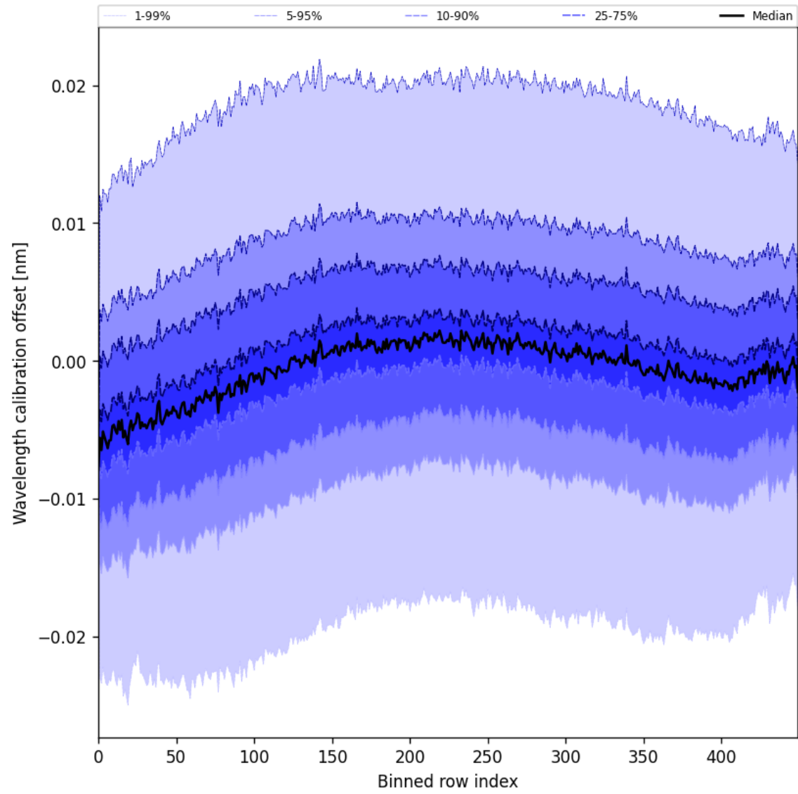
Figure 50: Along track statistics of “Wavelength calibration offset” for 2025-07-26 to 2025-07-27
