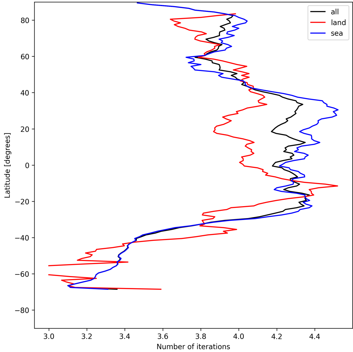
Figure 15: Zonal average of “Number of iterations” for 2025-07-26 to 2025-07-27.
