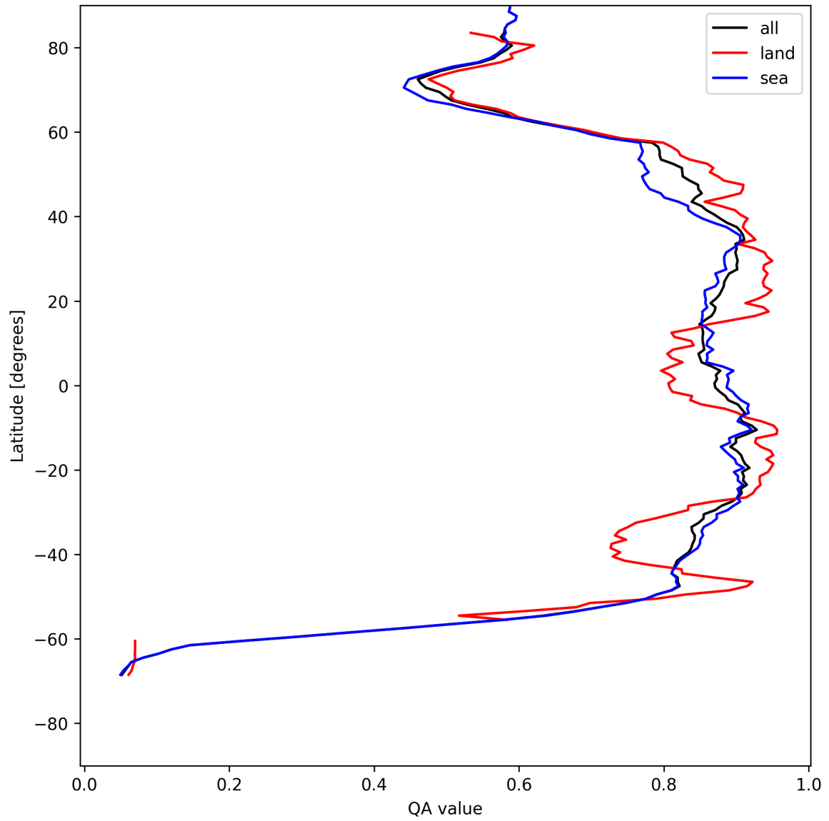
Figure 9: Zonal average of “QA value” for 2025-07-26 to 2025-07-27.
