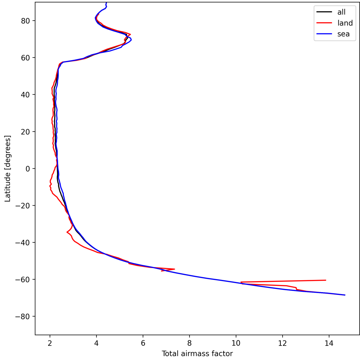
Figure 13: Zonal average of “Total airmass factor” for 2025-07-26 to 2025-07-27.
