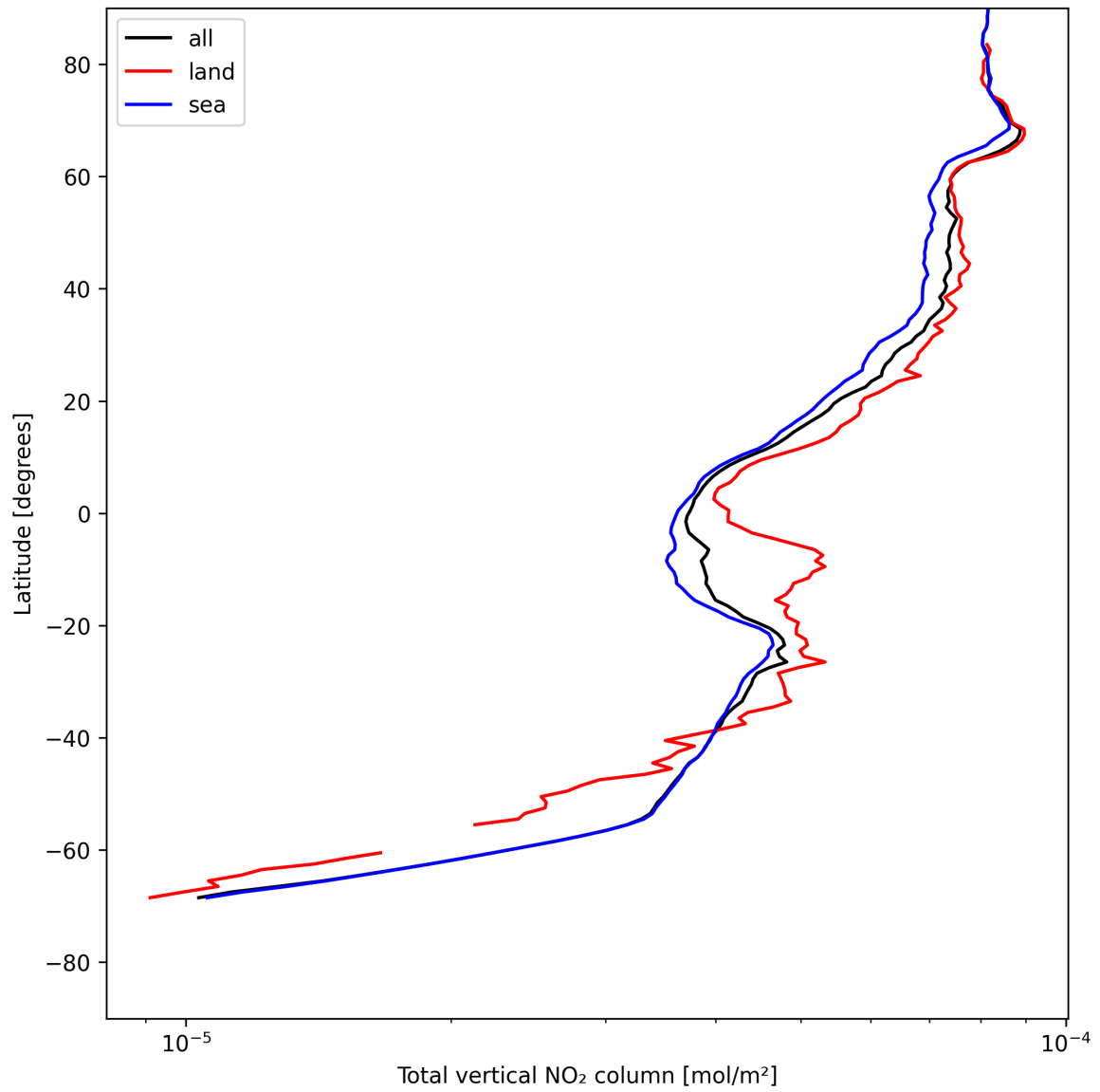
Figure 19: Zonal average of “Total vertical NO 2 column” for 2025-07-26 to 2025-07-27.
