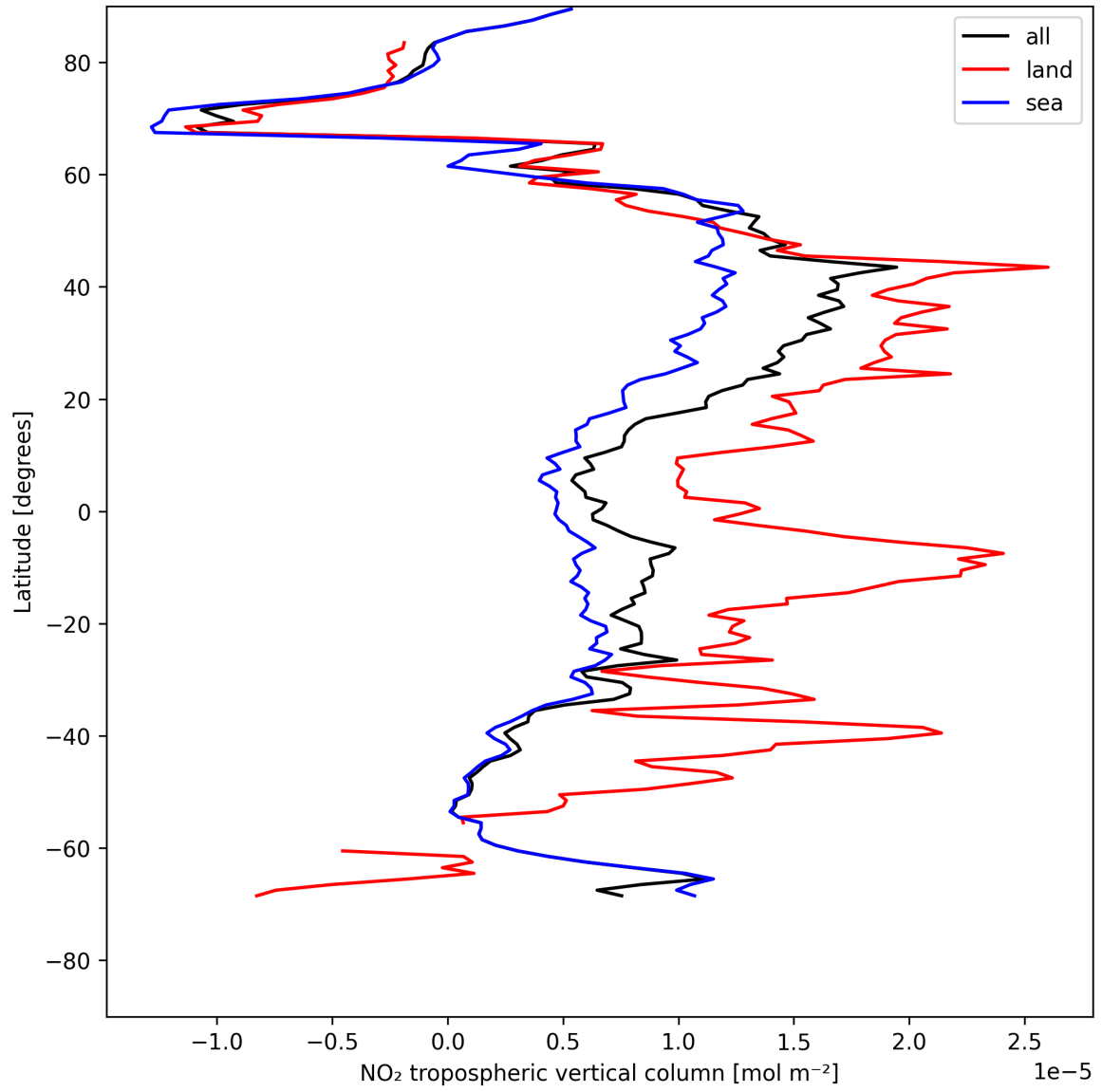
Figure 10: Zonal average of “NO 2 tropospheric vertical column” for 2025-07-26 to 2025-07-27.
