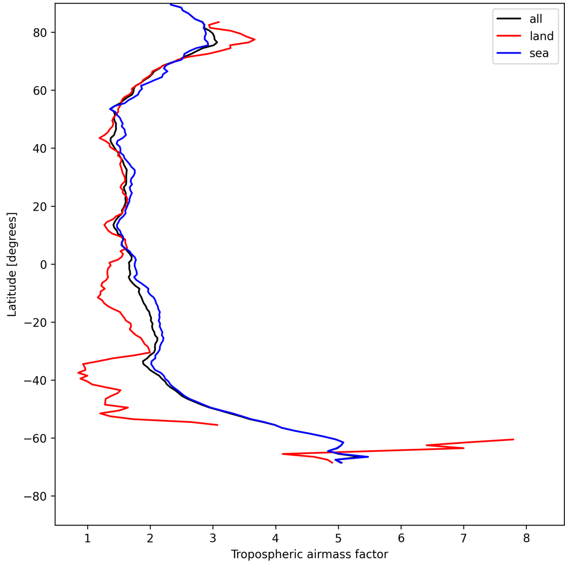
Figure 12: Zonal average of “Tropospheric air mass factor” for 2025-07-26 to 2025-07-27.
