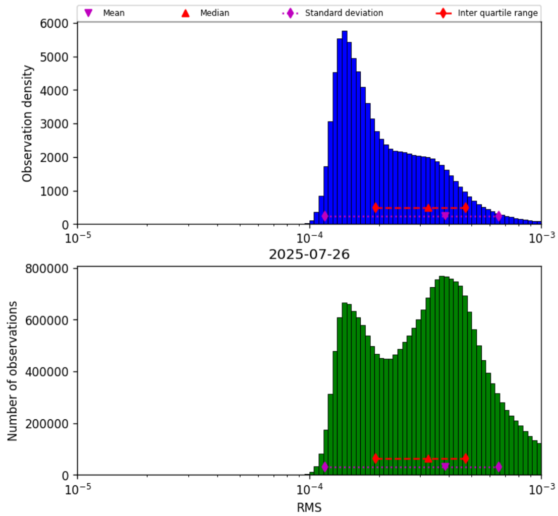
Figure 41: Histogram of “RMS” for 2025-07-26 to 2025-07-27
