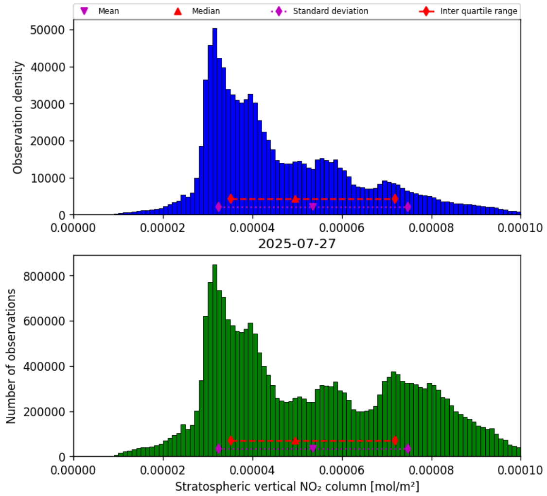
Figure 34: Histogram of “Stratospheric vertical NO 2 column” for 2025-07-27 to 2025-07-27
