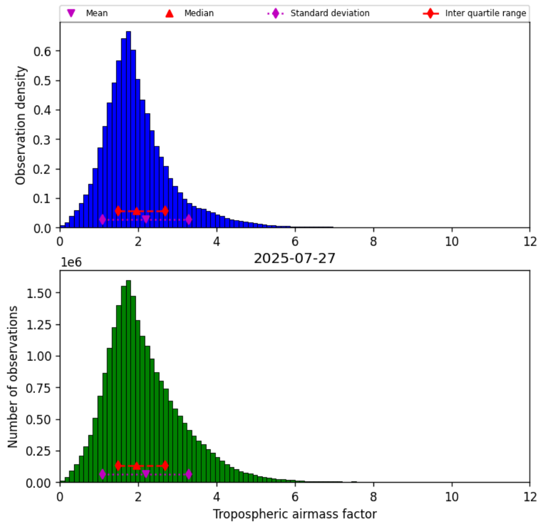
Figure 29: Histogram of “Tropospheric airmass factor” for 2025-07-27 to 2025-07-27
