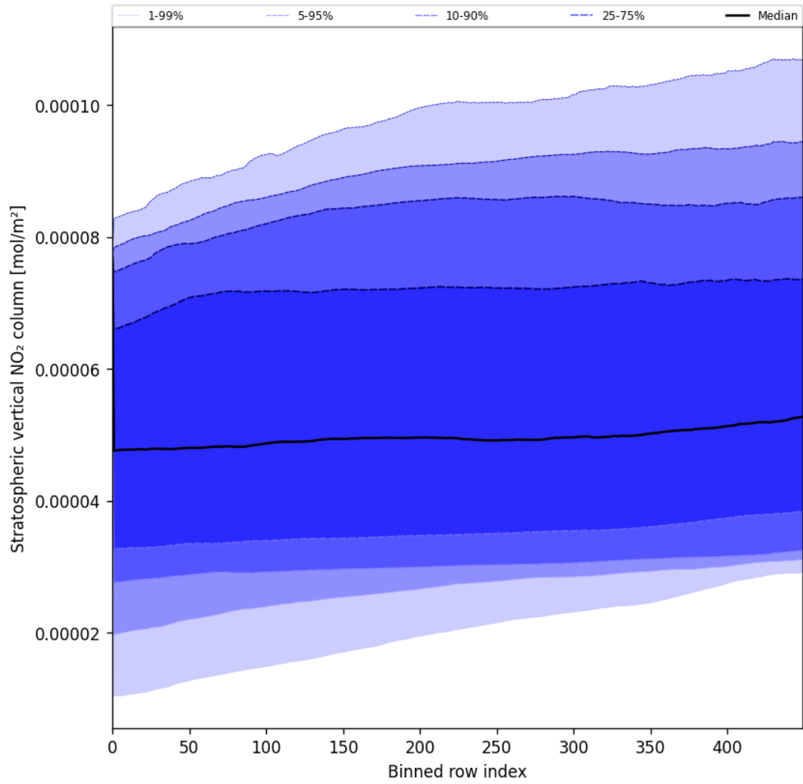
Figure 51: Along track statistics of “Stratospheric vertical NO 2 column” for 2025-07-27 to 2025-07-27
