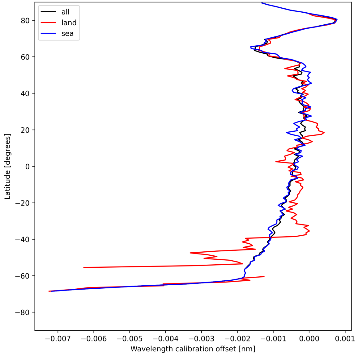
Figure 16: Zonal average of “Wavelength calibration offset” for 2025-07-27 to 2025-07-27.
