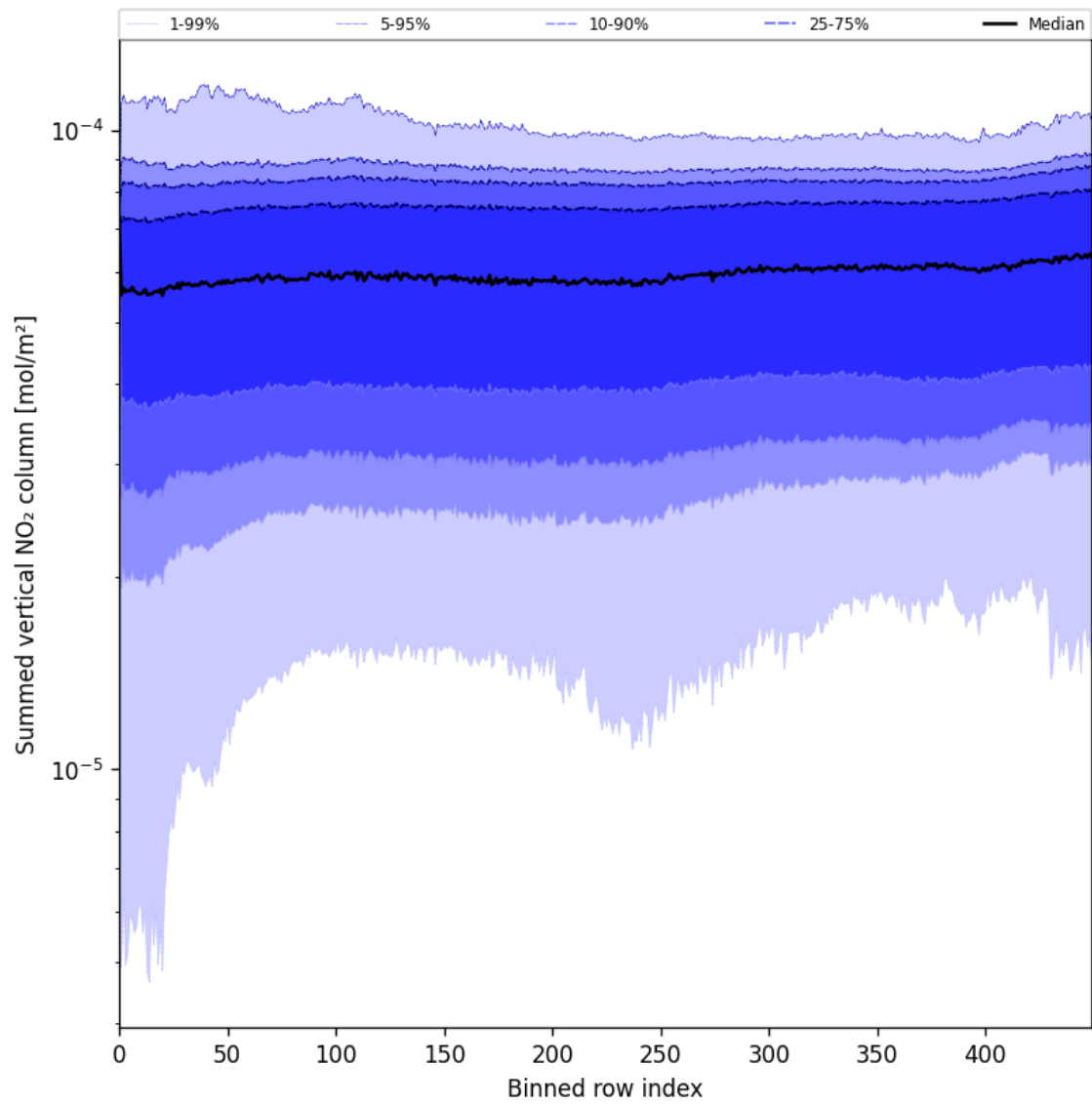
Figure 55: Along track statistics of “Summed vertical NO 2 column” for 2025-07-27 to 2025-07-27
