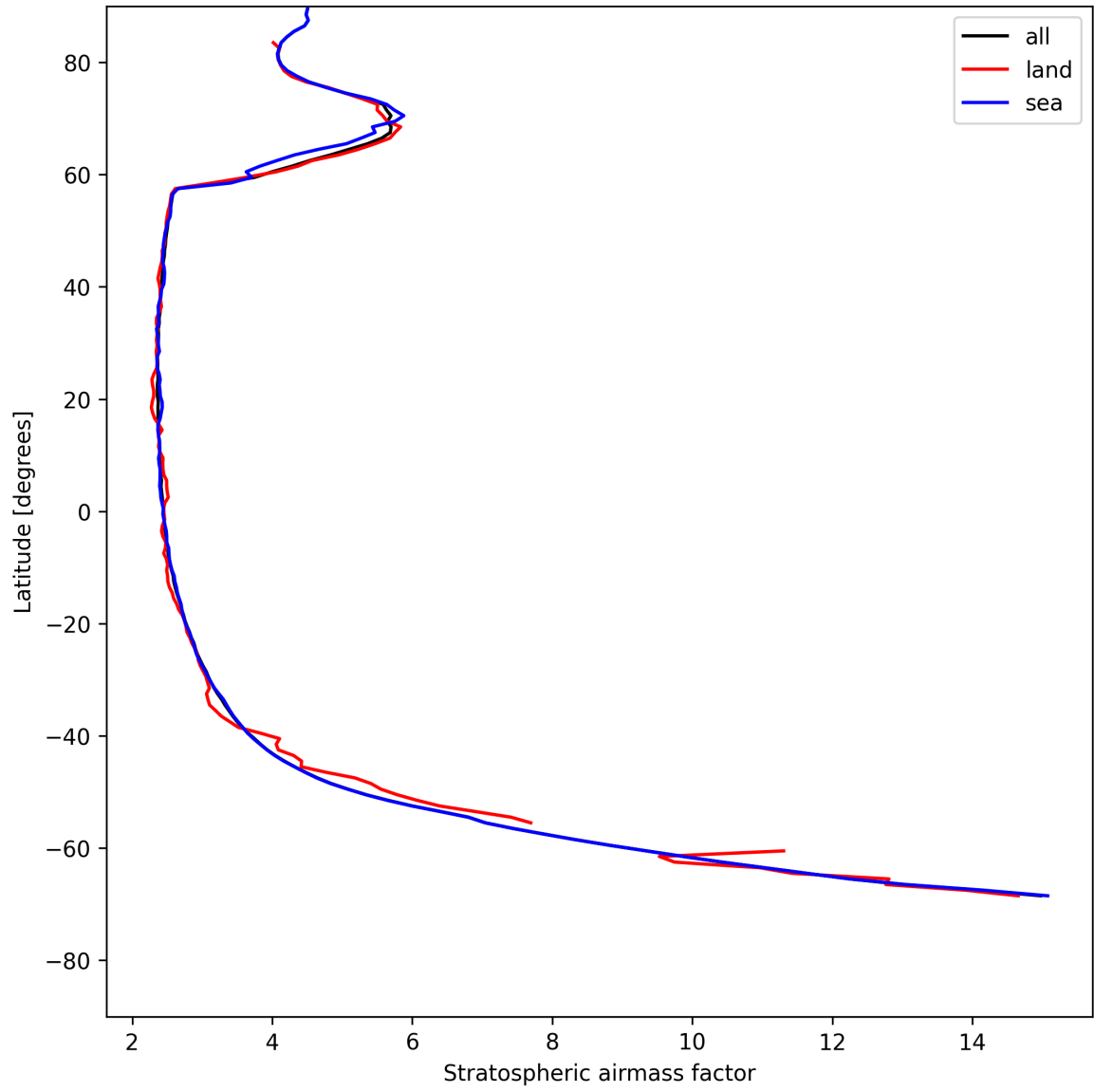
Figure 25: Zonal average of “Stratospheric air mass factor” for 2025-07-27 to 2025-07-27.
