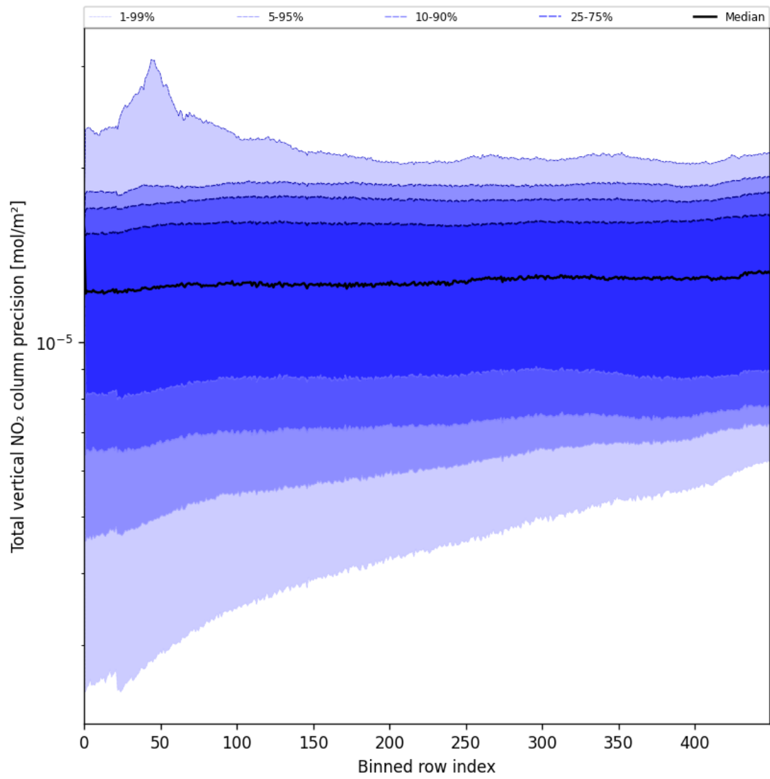
Figure 54: Along track statistics of “Total vertical NO 2 column precision” for 2025-07-27 to 2025-07-27
