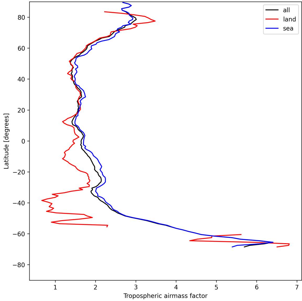
Figure 12: Zonal average of “Tropospheric air mass factor” for 2025-07-27 to 2025-07-27.
