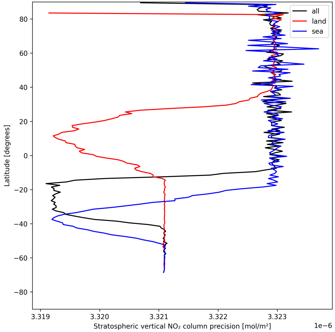
Figure 18: Zonal average of “Stratospheric vertical NO 2 column precision” for 2025-07-27 to 2025-07-27.
