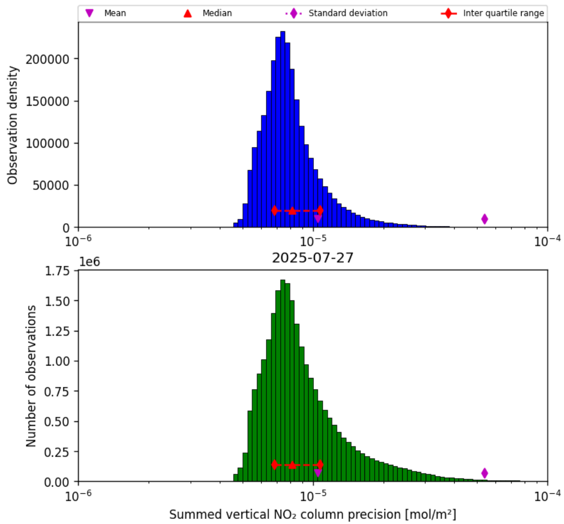
Figure 39: Histogram of "Summed vertical NO 2 column precision" for 2025-07-27 to 2025-07-27
