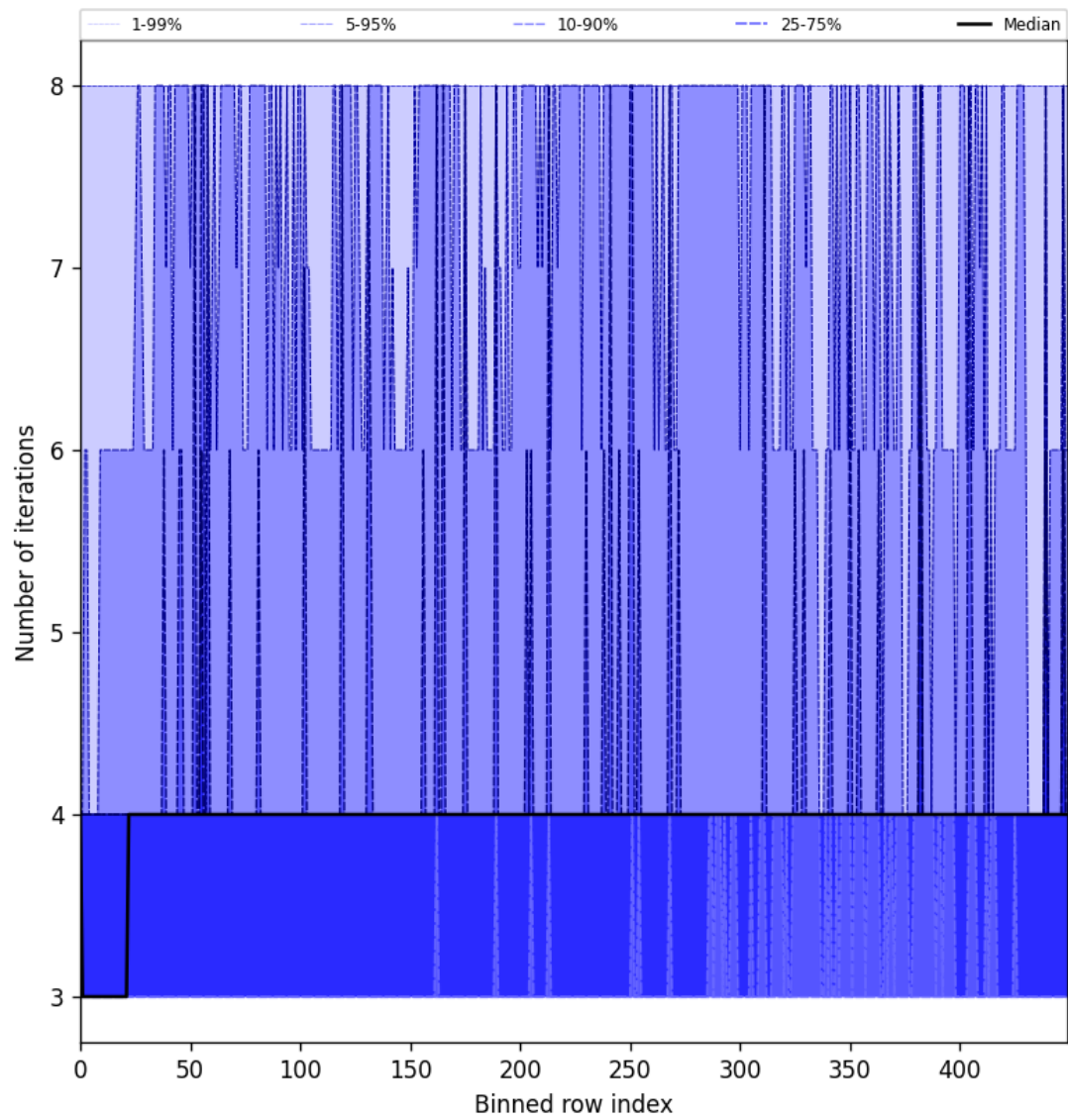
Figure 49: Along track statistics of “Number of iterations” for 2025-07-27 to 2025-07-27
