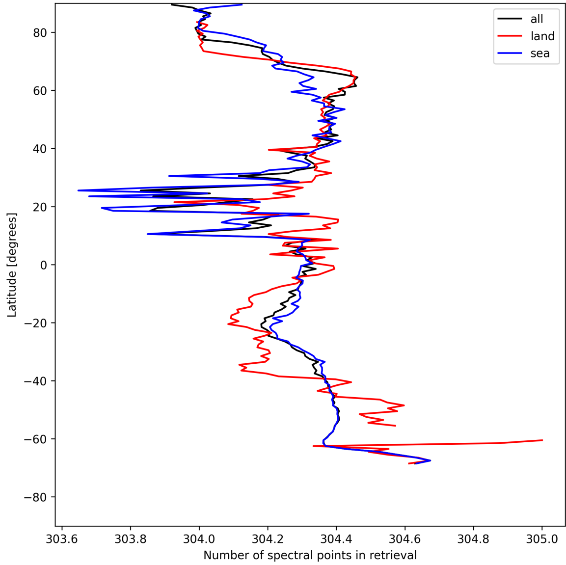
Figure 14: Zonal average of “Number of spectral points in retrieval” for 2025-07-27 to 2025-07-27.
