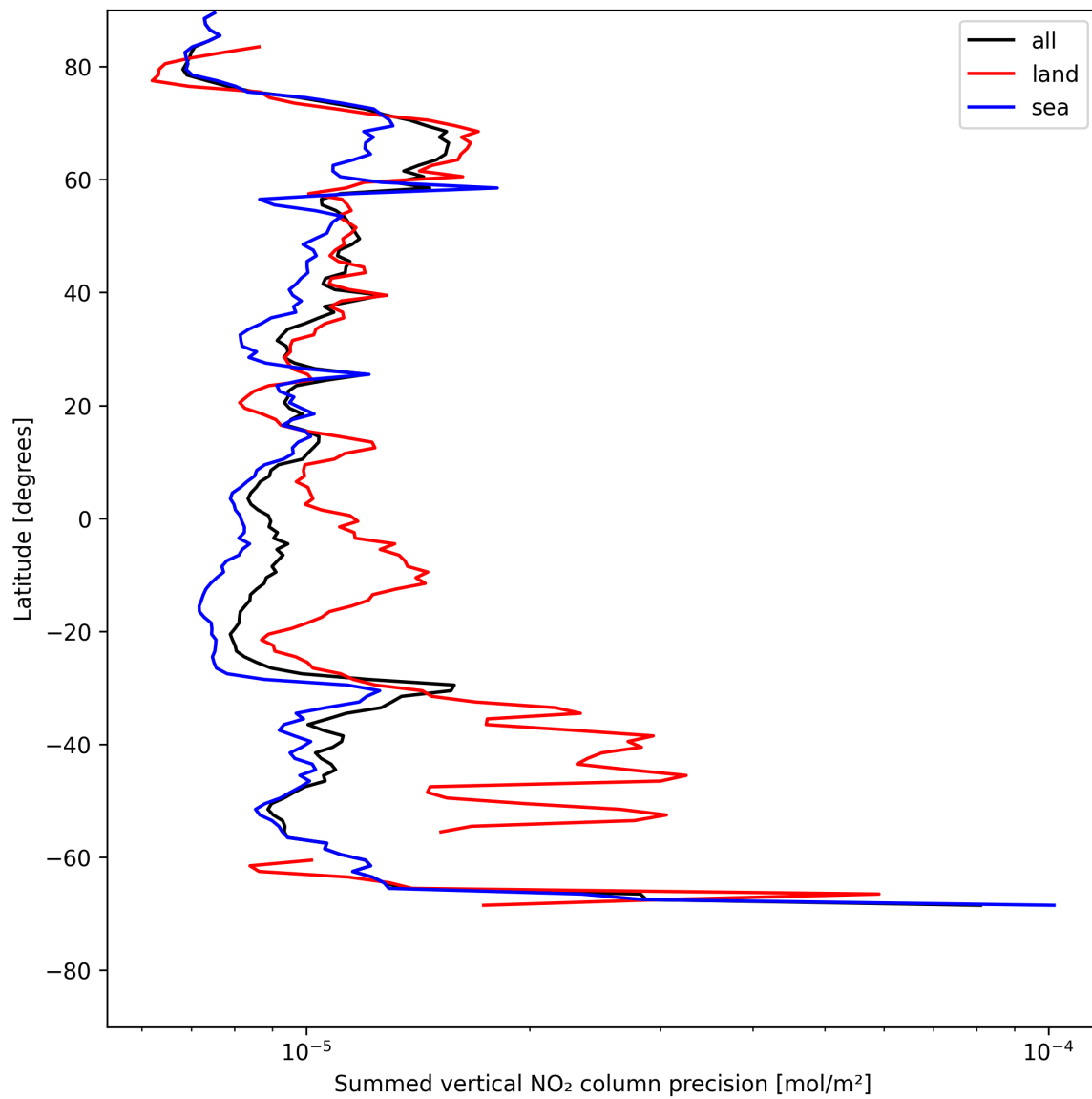
Figure 22: Zonal average of “Summed vertical NO 2 column precision” for 2025-07-27 to 2025-07-27.
