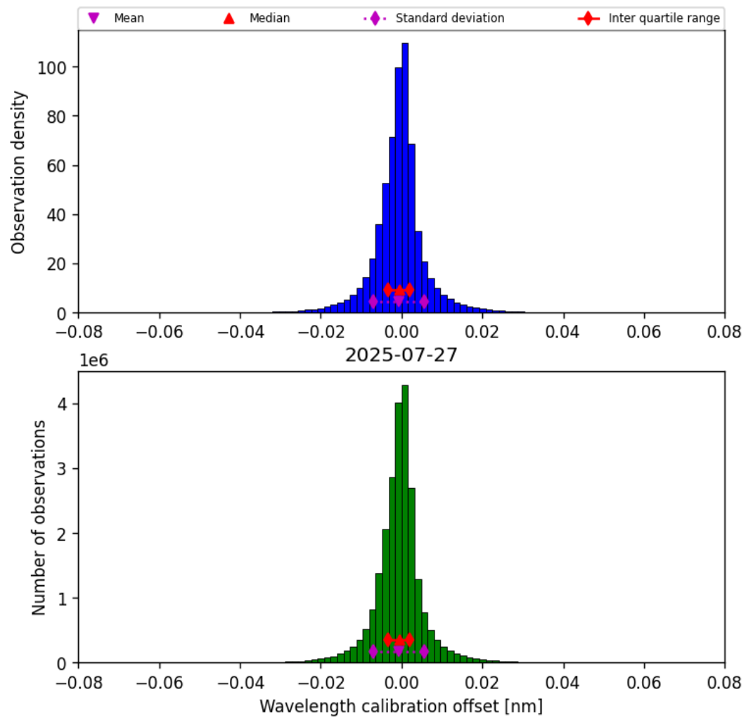
Figure 33: Histogram of “Wavelength calibration offset” for 2025-07-27 to 2025-07-27
