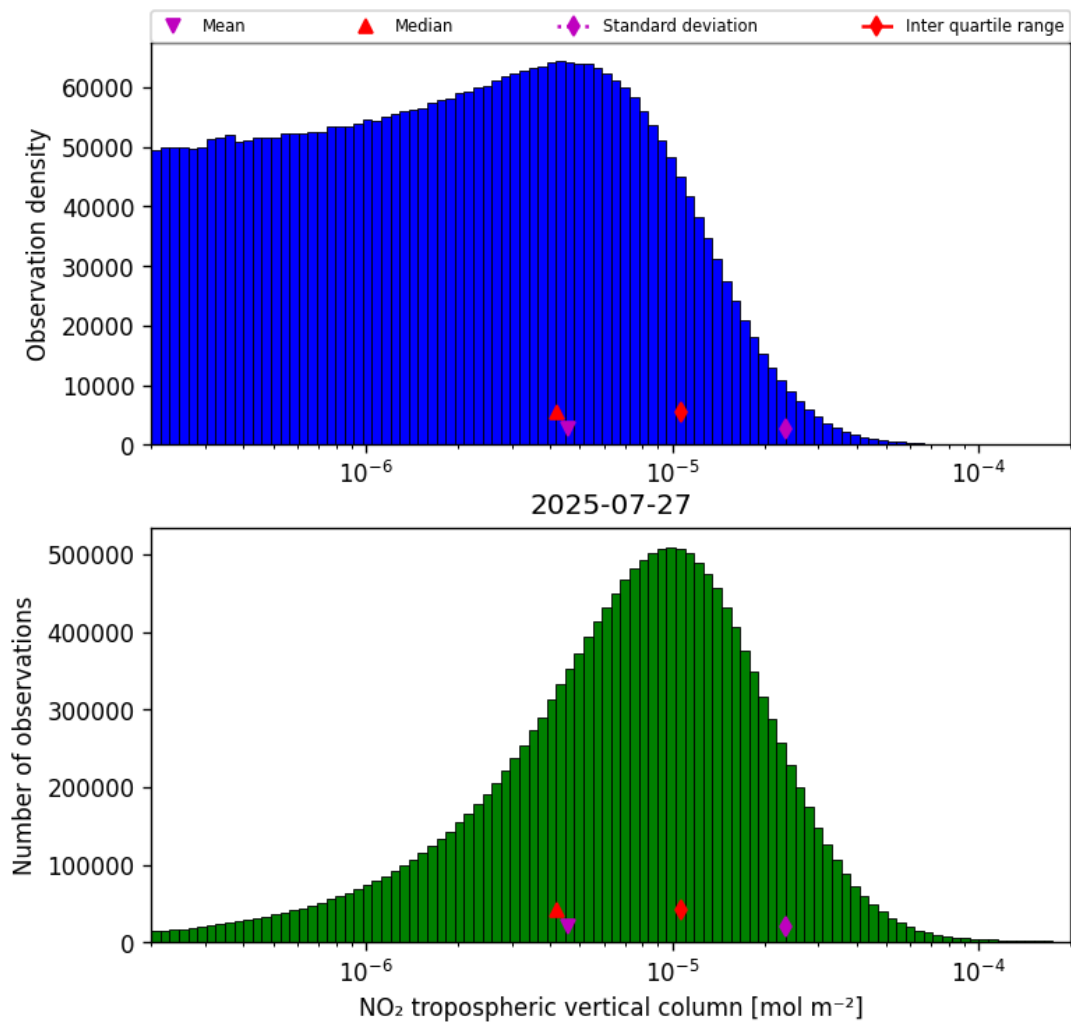
Figure 27: Histogram of “NO 2 tropospheric vertical column” for 2025-07-27 to 2025-07-27
