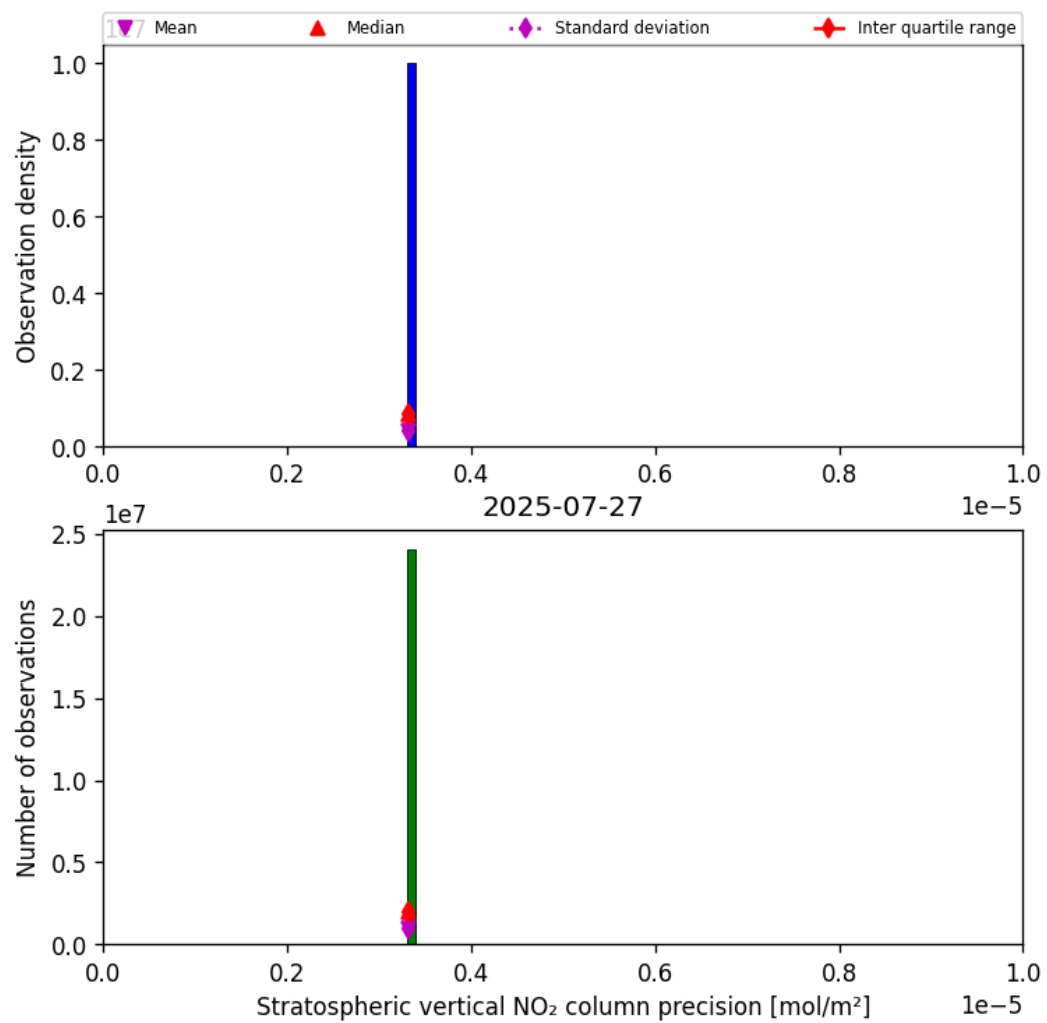
Figure 35: Histogram of “Stratospheric vertical NO 2 column precision” for 2025-07-27 to 2025-07-27
