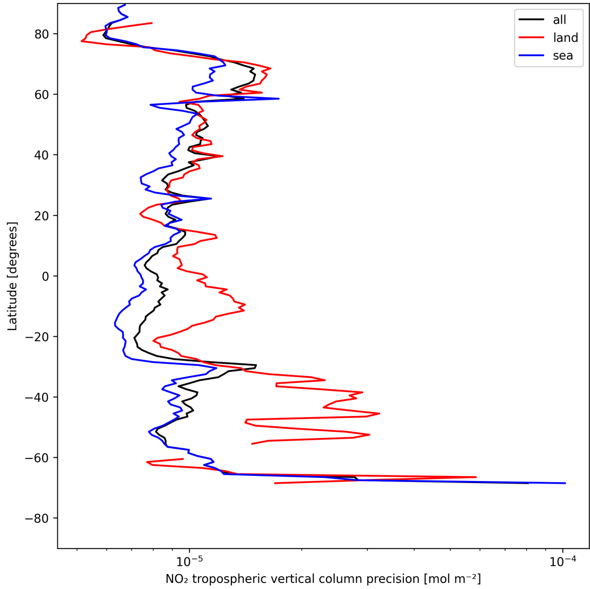
Figure 11: Zonal average of “NO 2 tropospheric vertical column precision” for 2025-07-27 to 2025-07-27.
