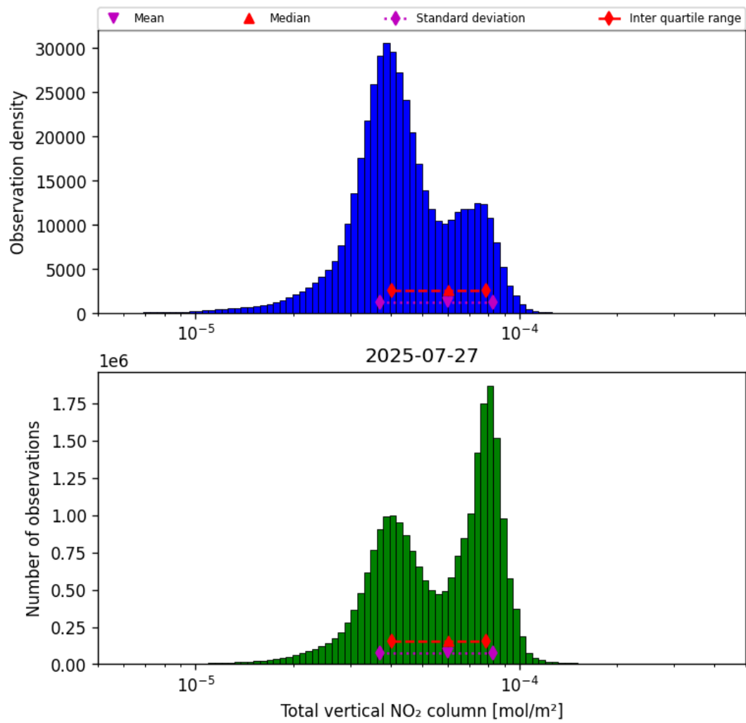
Figure 36: Histogram of "Total vertical NO 2 column" for 2025-07-27 to 2025-07-27
