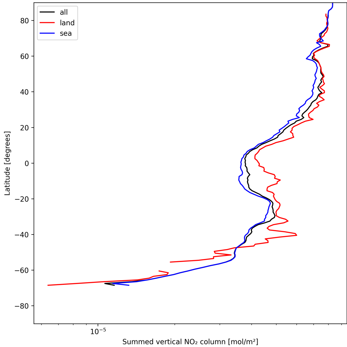
Figure 21: Zonal average of “Summed vertical NO 2 column” for 2025-07-27 to 2025-07-27.
