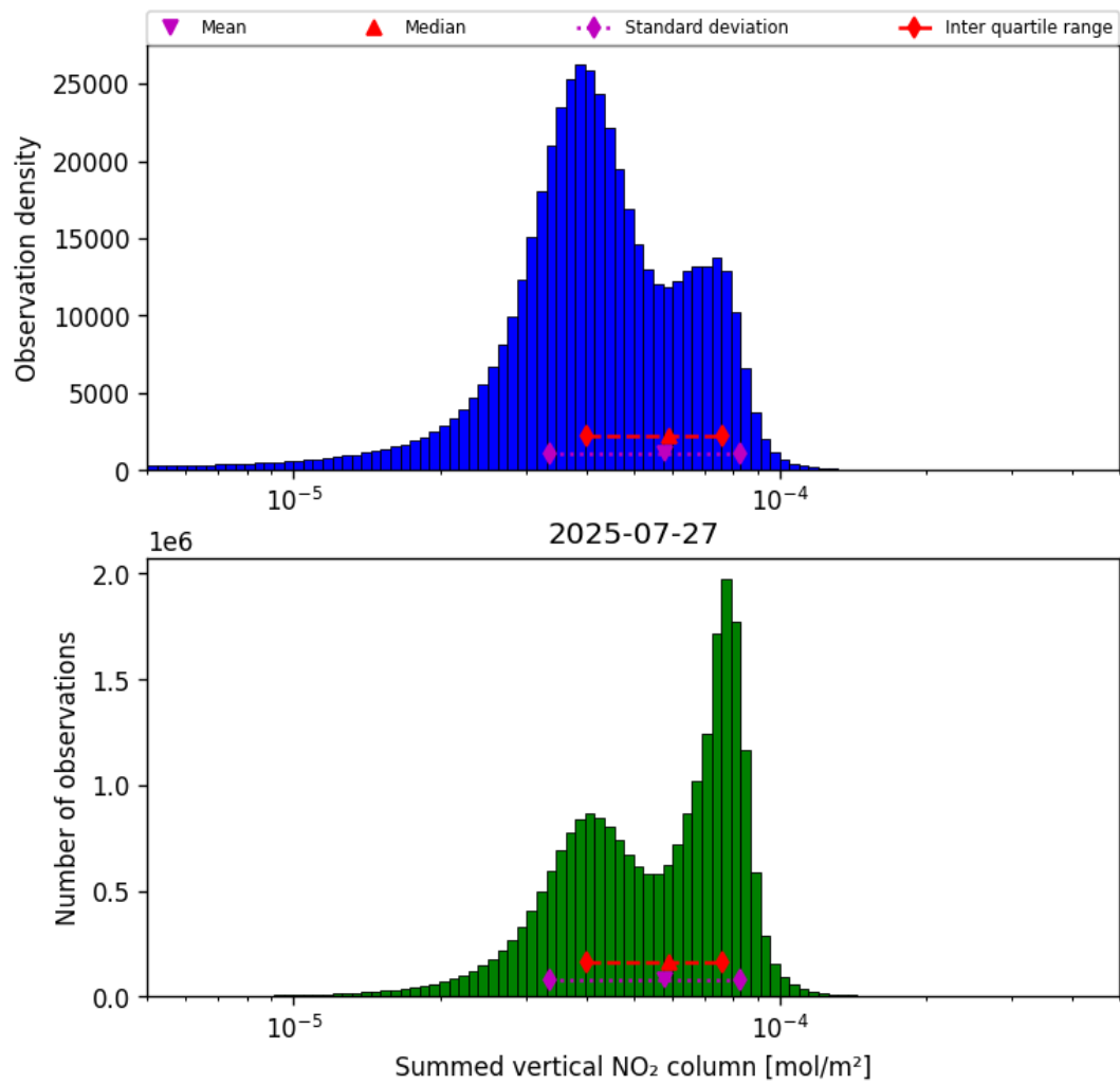
Figure 38: Histogram of “Summed vertical NO 2 column” for 2025-07-27 to 2025-07-27
