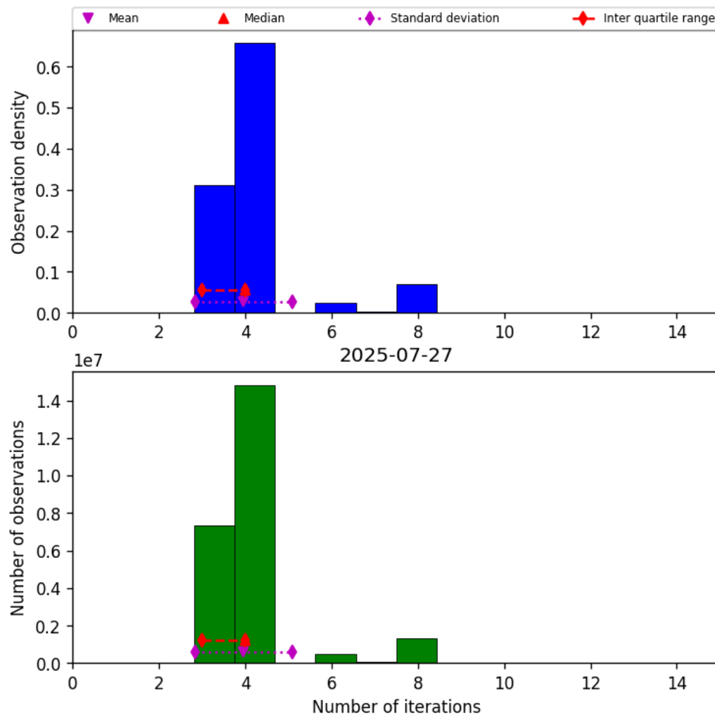
Figure 32: Histogram of “Number of iterations” for 2025-07-27 to 2025-07-27
