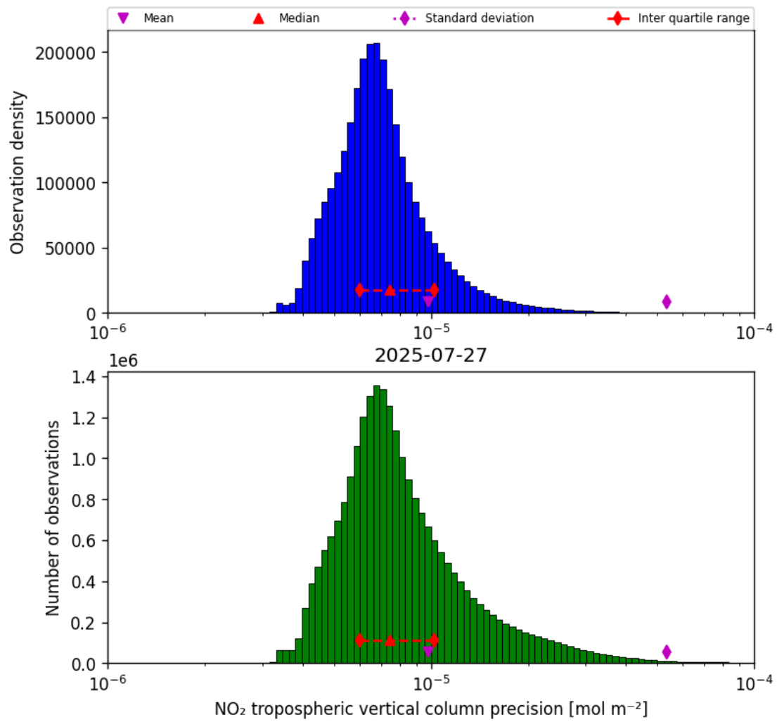
Figure 28: Histogram of “NO 2 tropospheric vertical column precision” for 2025-07-27 to 2025-07-27
