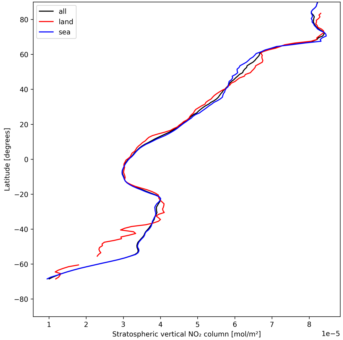
Figure 17: Zonal average of “Stratospheric vertical NO 2 column” for 2025-07-27 to 2025-07-27.
