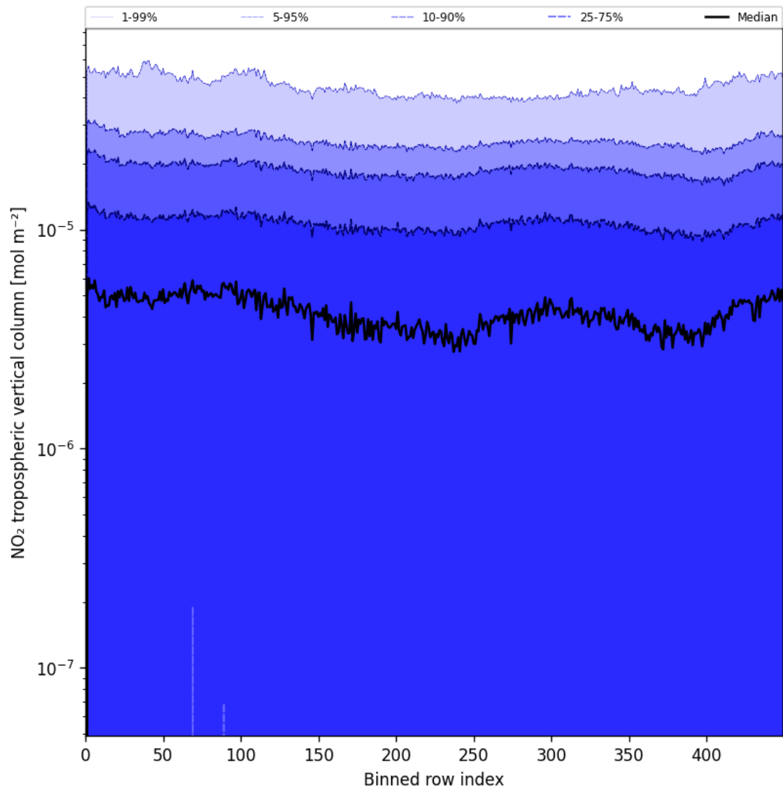
Figure 44: Along track statistics of “NO 2 tropospheric vertical column” for 2025-07-27 to 2025-07-27
