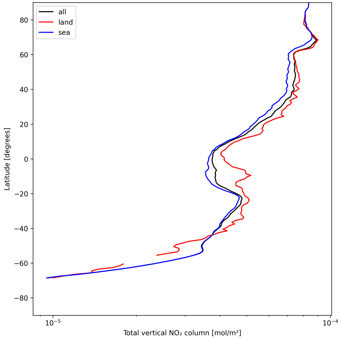
Figure 19: Zonal average of “Total vertical NO 2 column” for 2025-07-27 to 2025-07-27.
