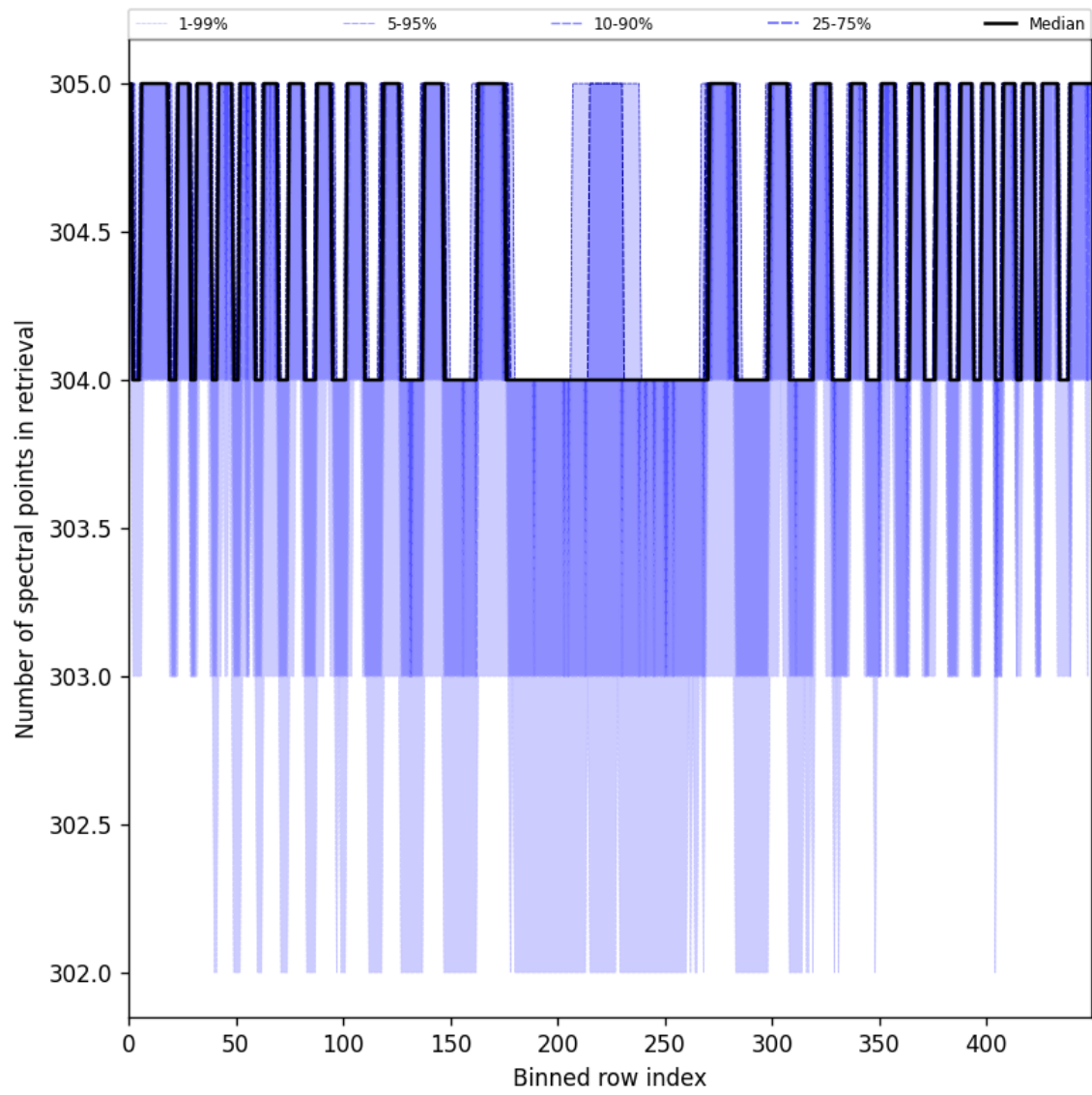
Figure 48: Along track statistics of “Number of spectral points in retrieval” for 2025-07-27 to 2025-07-27
