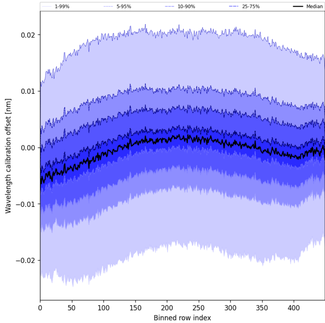
Figure 50: Along track statistics of “Wavelength calibration offset” for 2025-07-27 to 2025-07-27
