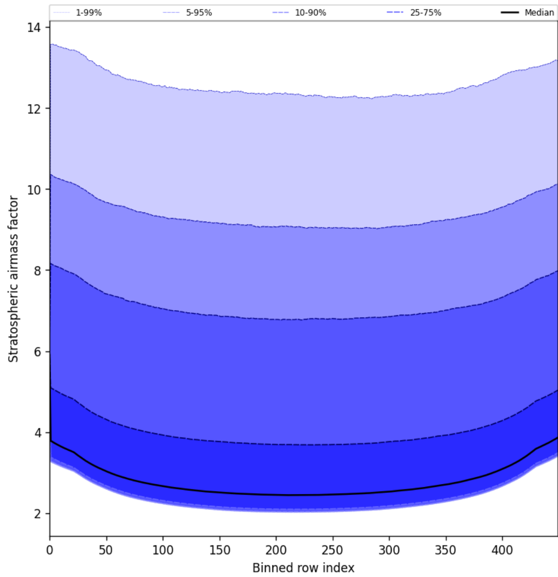
Figure 59: Along track statistics of “Stratospheric airmass factor” for 2025-07-27 to 2025-07-27
