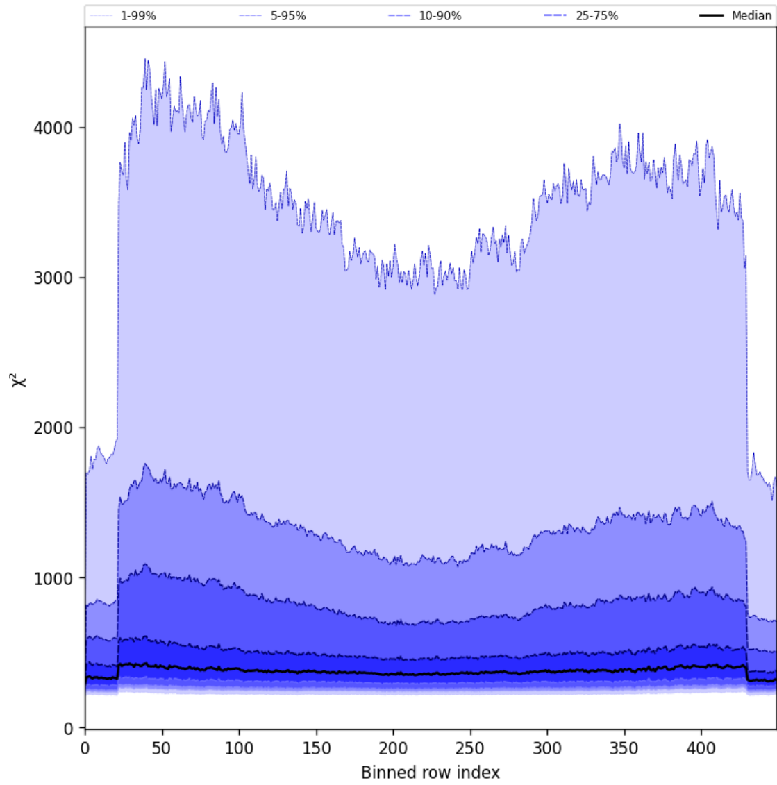
Figure 57: Along track statistics of “ \chi^2 ” for 2025-07-27 to 2025-07-27
