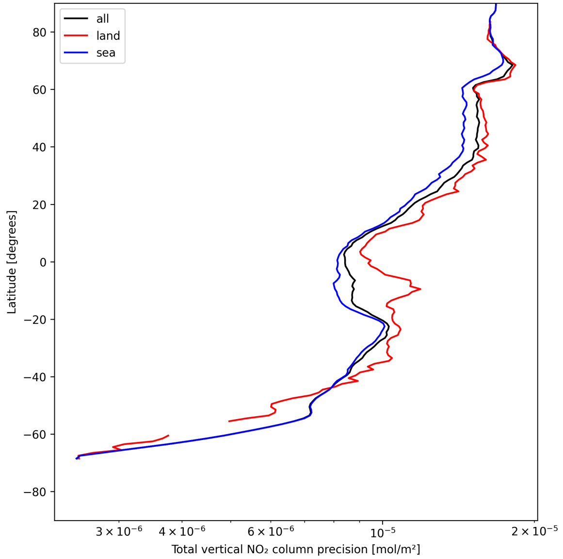
Figure 20: Zonal average of “Total vertical NO 2 column precision” for 2025-07-27 to 2025-07-27.
