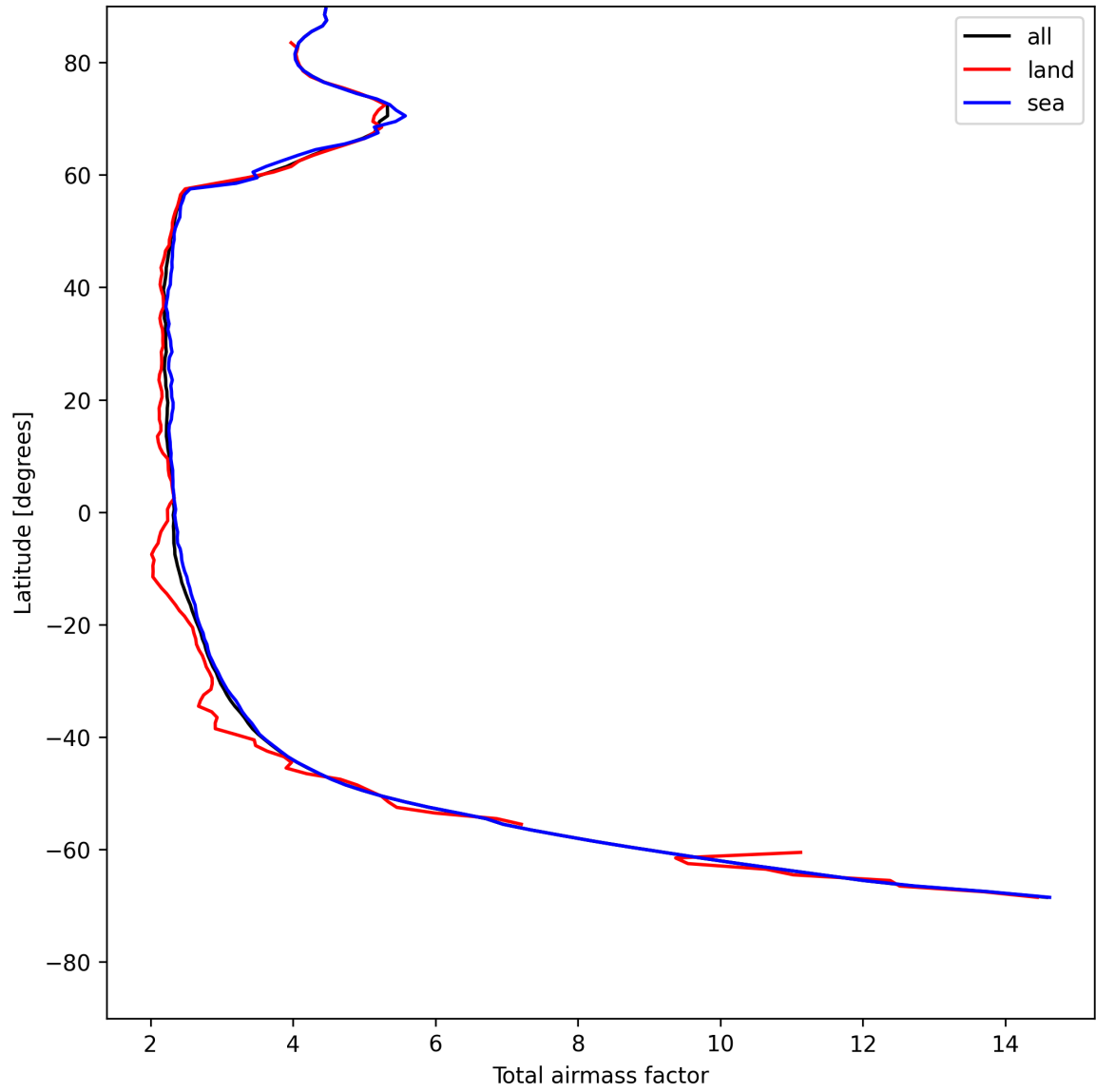
Figure 13: Zonal average of “Total airmass factor” for 2025-07-27 to 2025-07-27.
