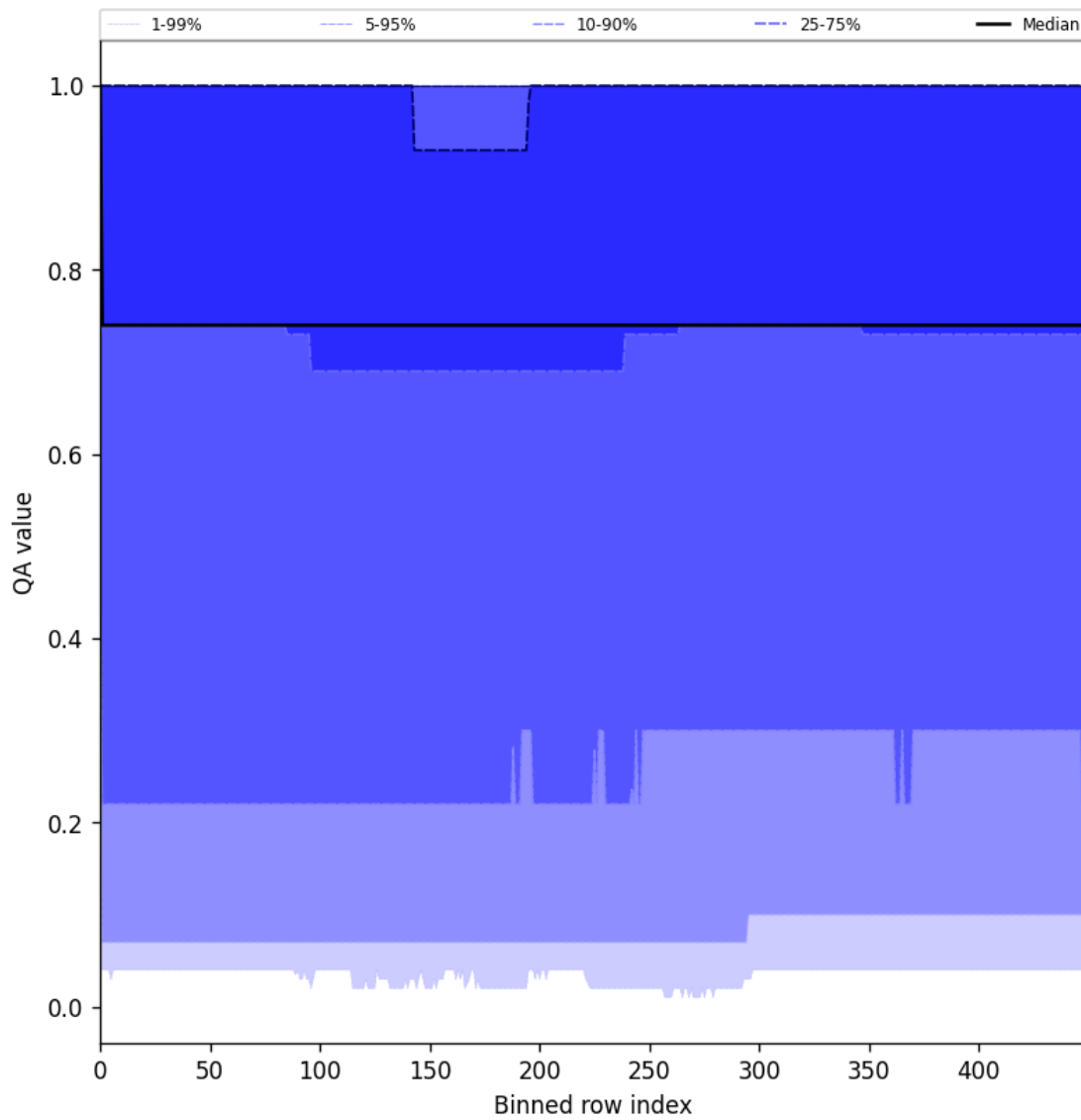
Figure 43: Along track statistics of “QA value” for 2025-07-27 to 2025-07-27
