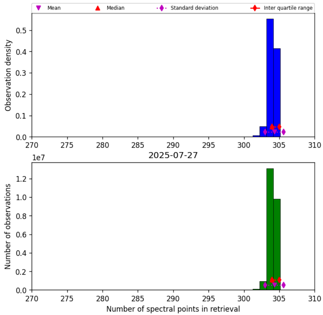
Figure 31: Histogram of “Number of spectral points in retrieval” for 2025-07-27 to 2025-07-27
