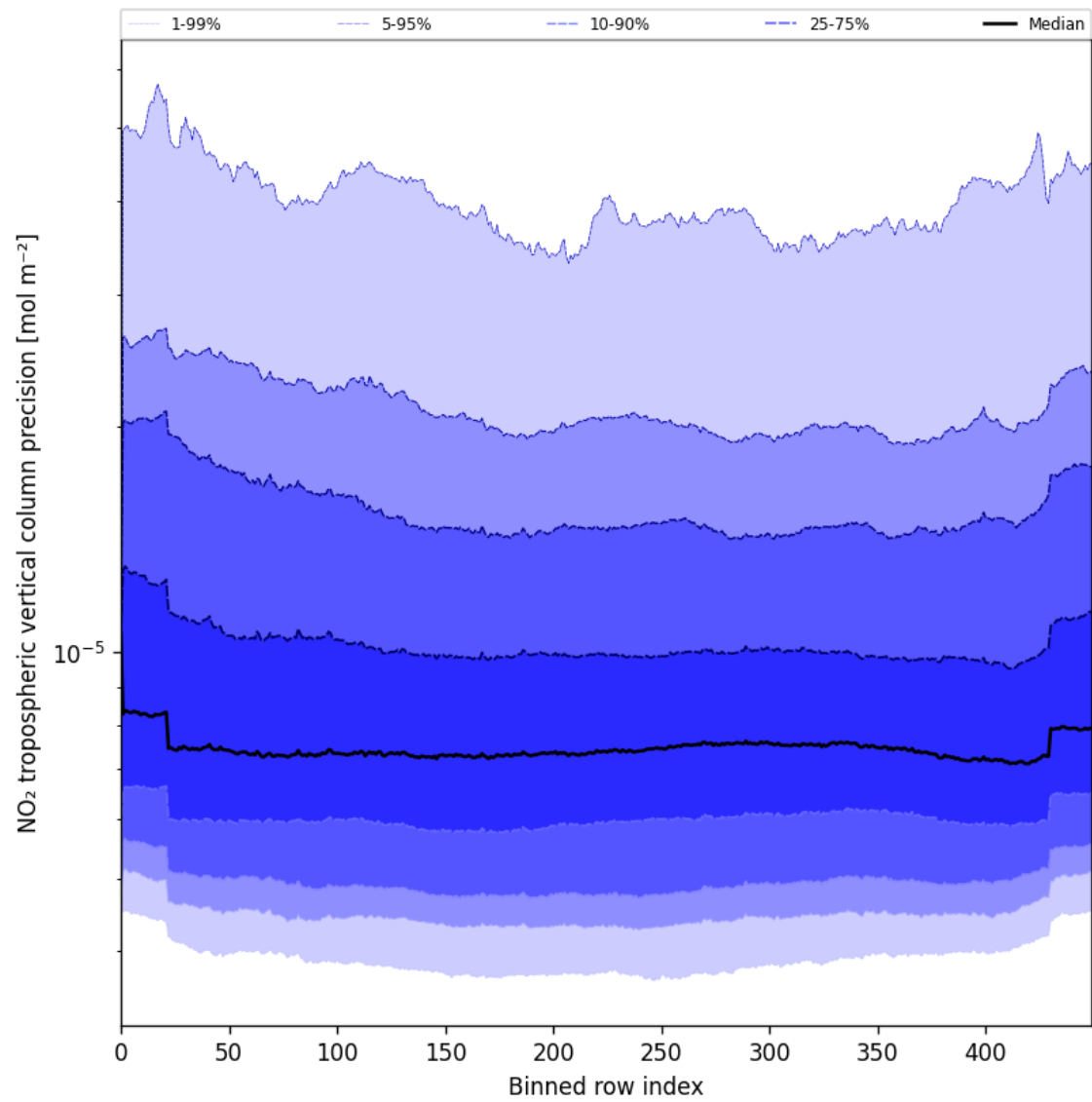
Figure 45: Along track statistics of “NO 2 tropospheric vertical column precision” for 2025-07-27 to 2025-07-27
