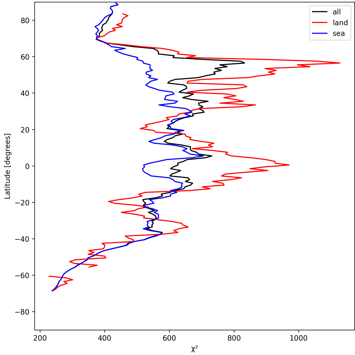
Figure 23: Zonal average of “ \chi^2 ” for 2025-07-27 to 2025-07-27.
