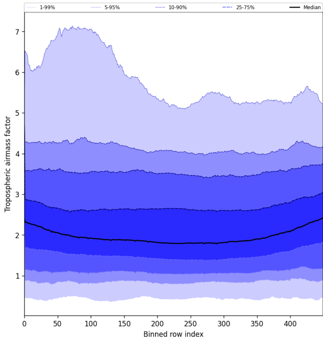
Figure 46: Along track statistics of “Tropospheric airmass factor” for 2025-07-27 to 2025-07-27
