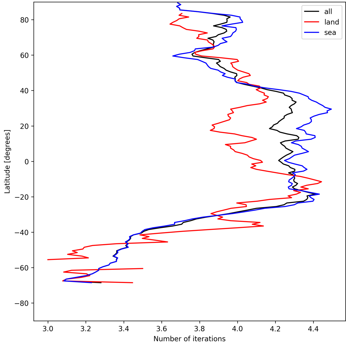
Figure 15: Zonal average of “Number of iterations” for 2025-07-27 to 2025-07-27.
