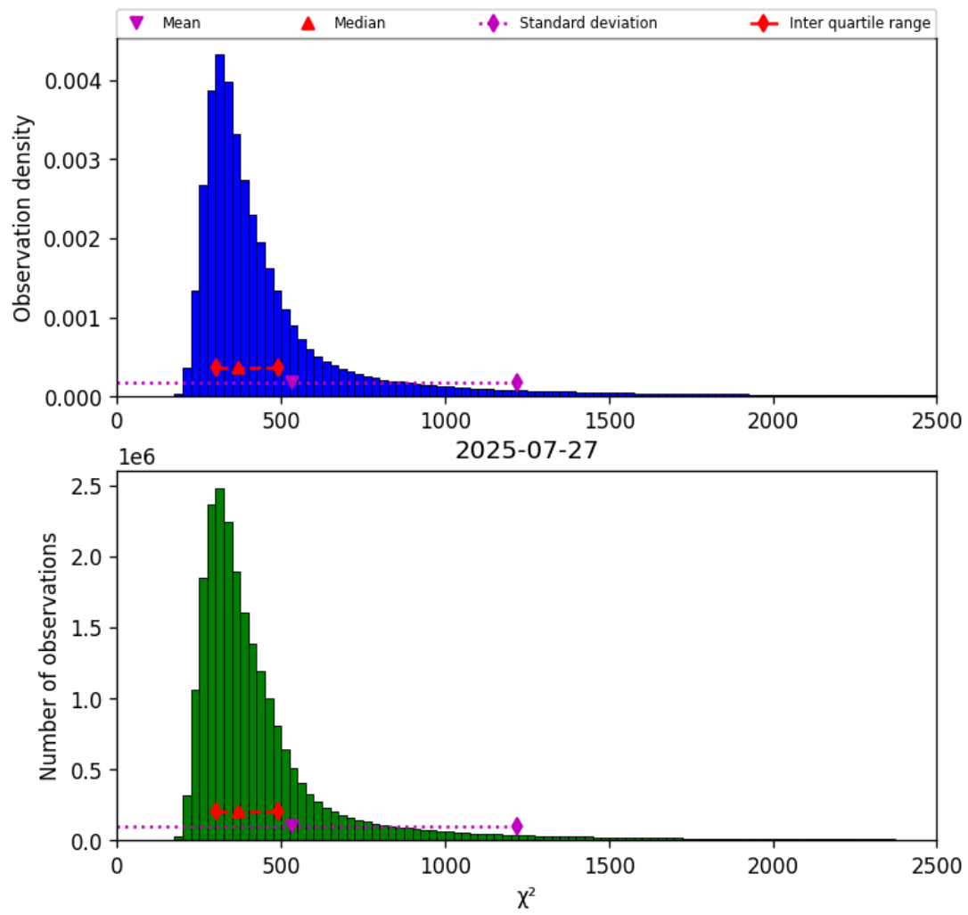
Figure 40: Histogram of “ \chi^2 ” for 2025-07-27 to 2025-07-27
