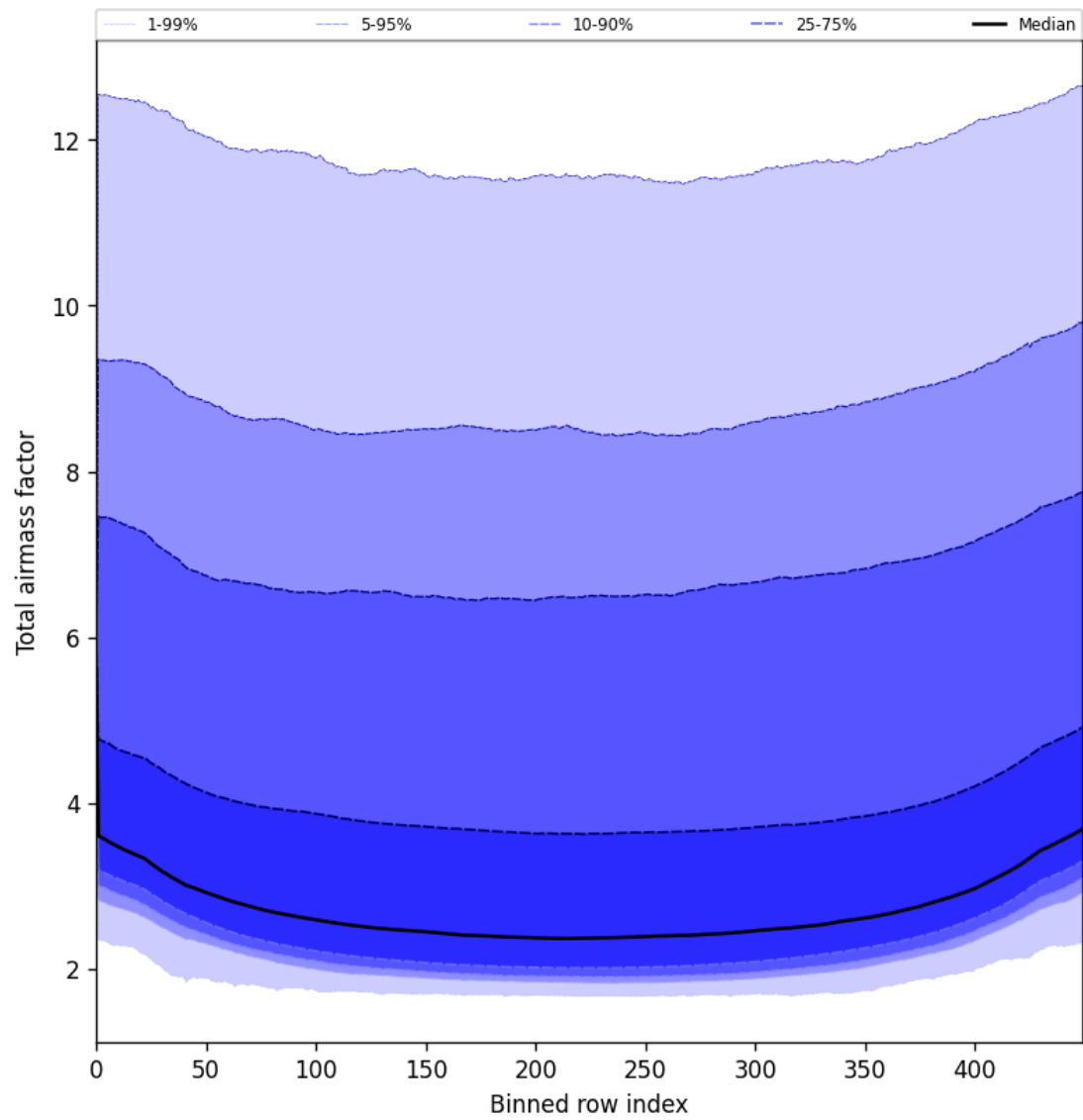
Figure 47: Along track statistics of “Total airmass factor” for 2025-07-27 to 2025-07-27
