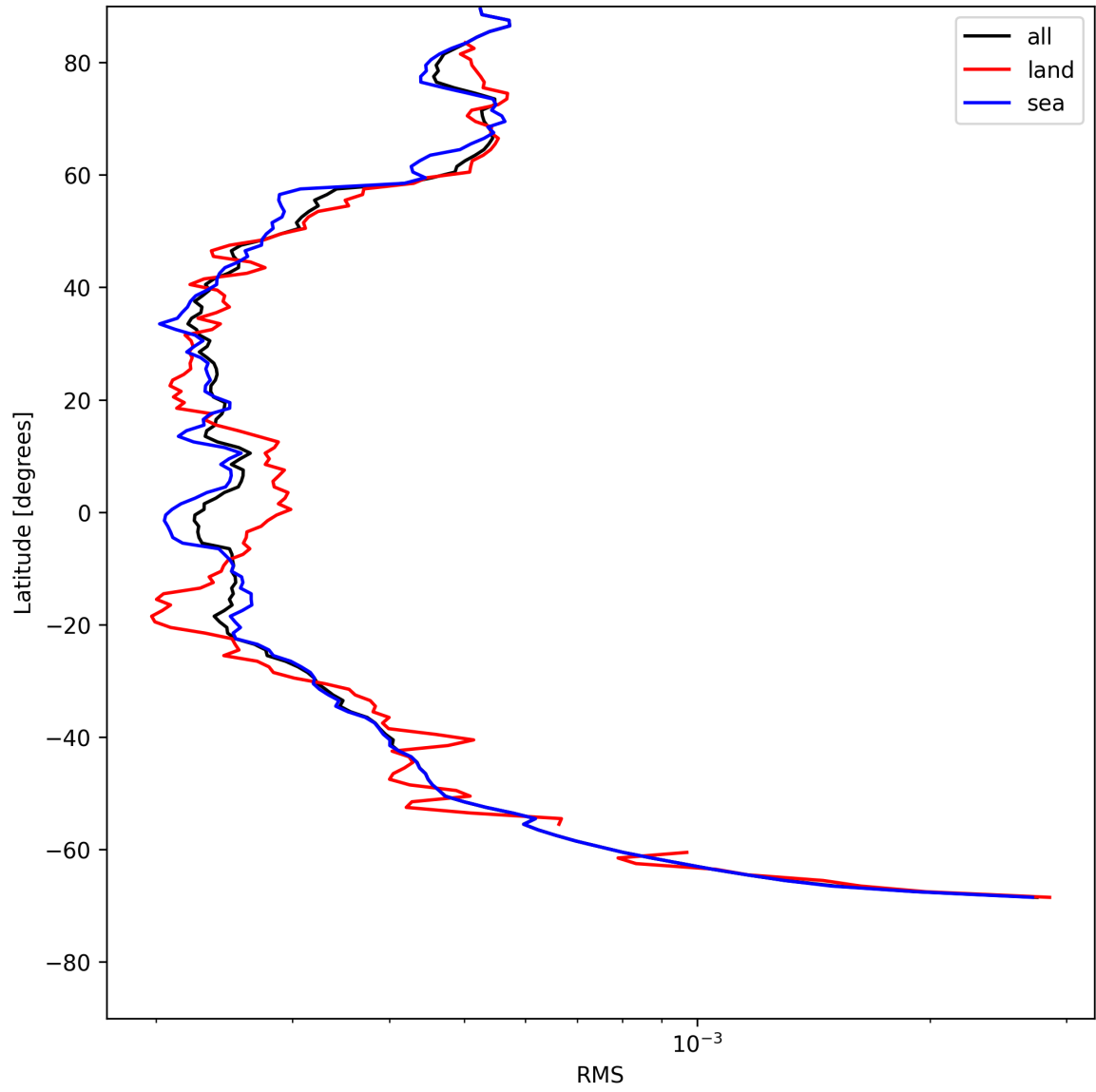
Figure 24: Zonal average of “RMS” for 2025-07-27 to 2025-07-27.
