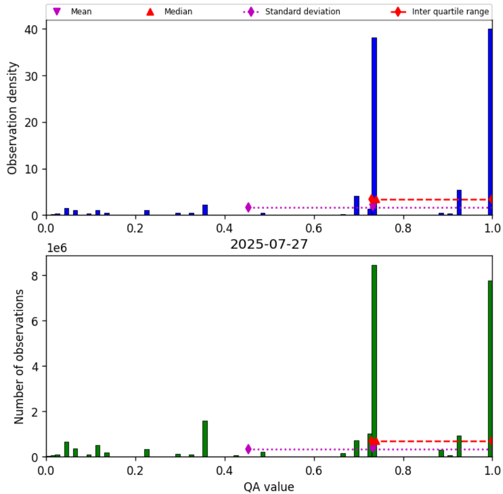
Figure 26: Histogram of “QA value” for 2025-07-27 to 2025-07-27
