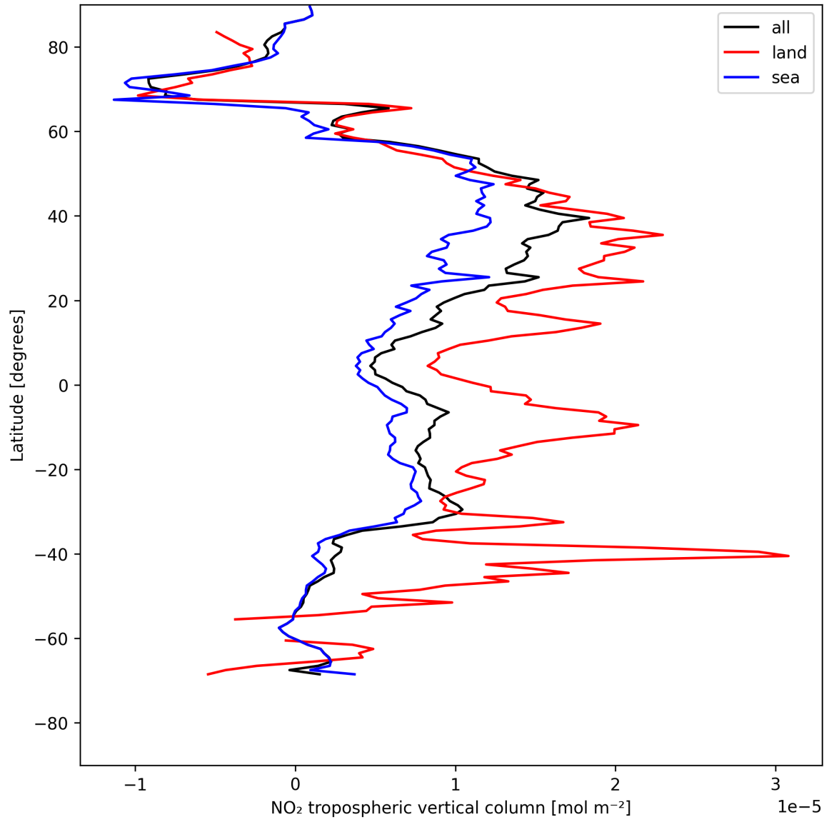
Figure 10: Zonal average of “NO 2 tropospheric vertical column” for 2025-07-27 to 2025-07-27.
