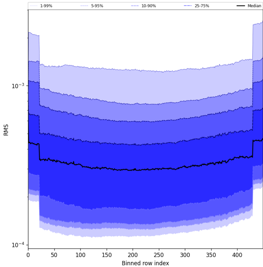
Figure 58: Along track statistics of “RMS” for 2025-07-27 to 2025-07-27
