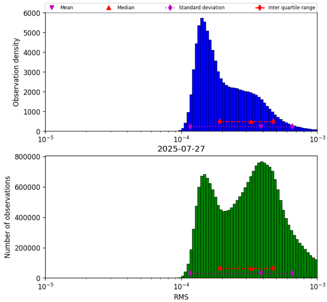
Figure 41: Histogram of “RMS” for 2025-07-27 to 2025-07-27
