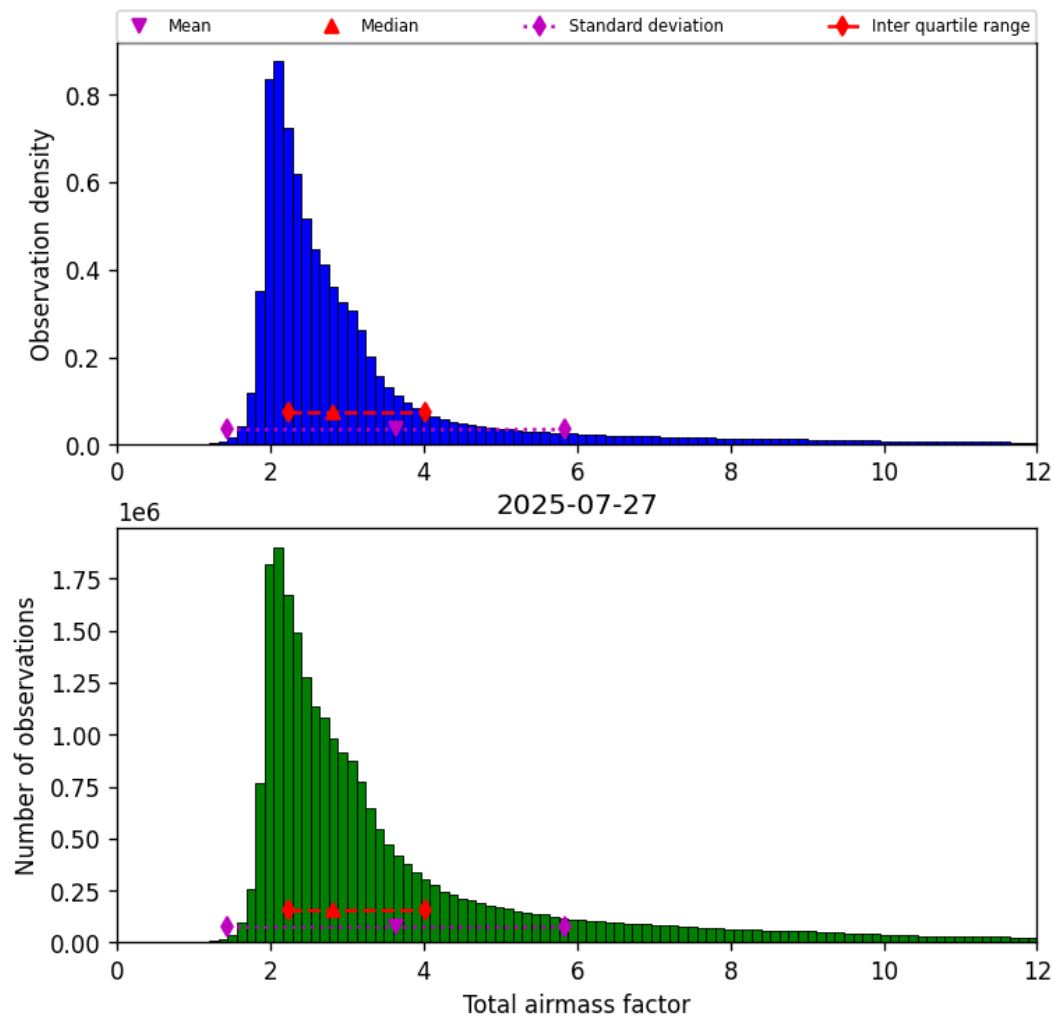
Figure 30: Histogram of “Total airmass factor” for 2025-07-27 to 2025-07-27
