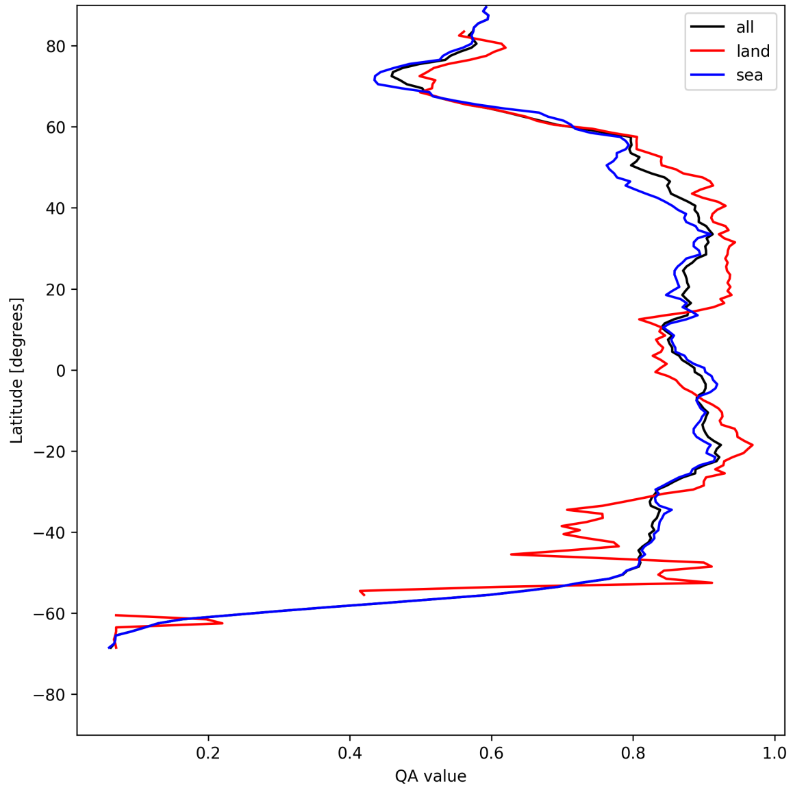
Figure 9: Zonal average of “QA value” for 2025-07-27 to 2025-07-27.
