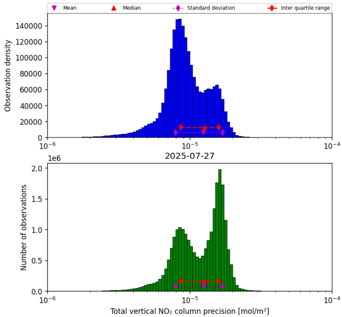
Figure 37: Histogram of "Total vertical NO 2 column precision" for 2025-07-27 to 2025-07-27
