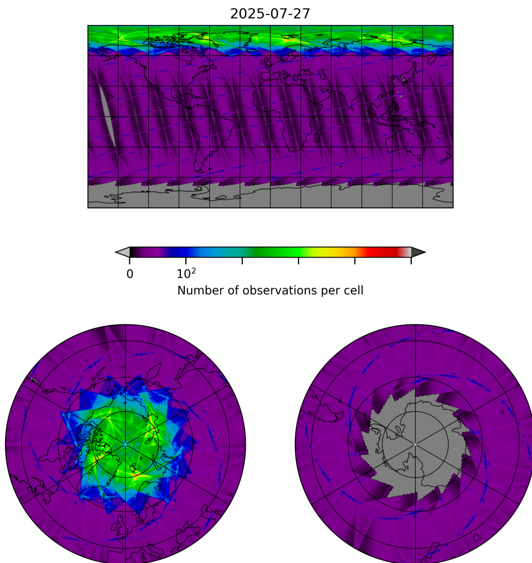
Figure 8: Map of the number of observations for 2025-07-27 to 2025-07-27
