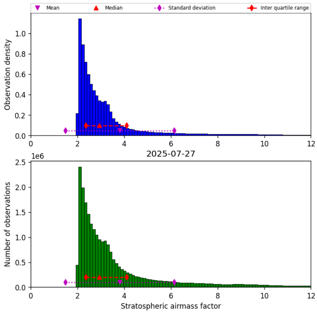
Figure 42: Histogram of “Stratospheric airmass factor” for 2025-07-27 to 2025-07-27
