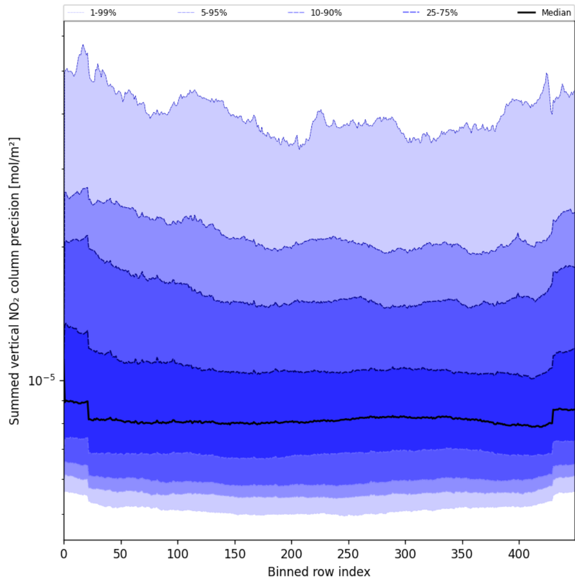
Figure 56: Along track statistics of “Summed vertical NO 2 column precision” for 2025-07-27 to 2025-07-27
