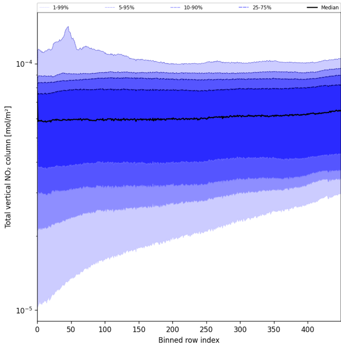
Figure 53: Along track statistics of “Total vertical NO 2 column” for 2025-07-27 to 2025-07-27
