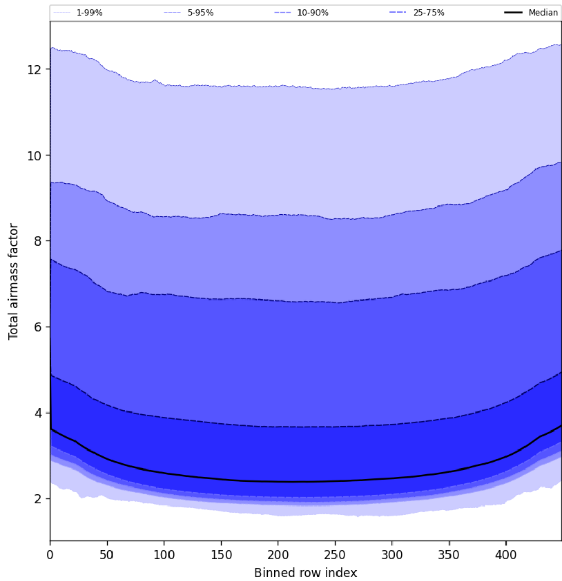
Figure 47: Along track statistics of “Total airmass factor” for 2025-07-28 to 2025-07-29
