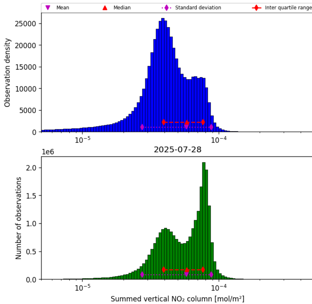
Figure 38: Histogram of “Summed vertical NO 2 column” for 2025-07-28 to 2025-07-29
