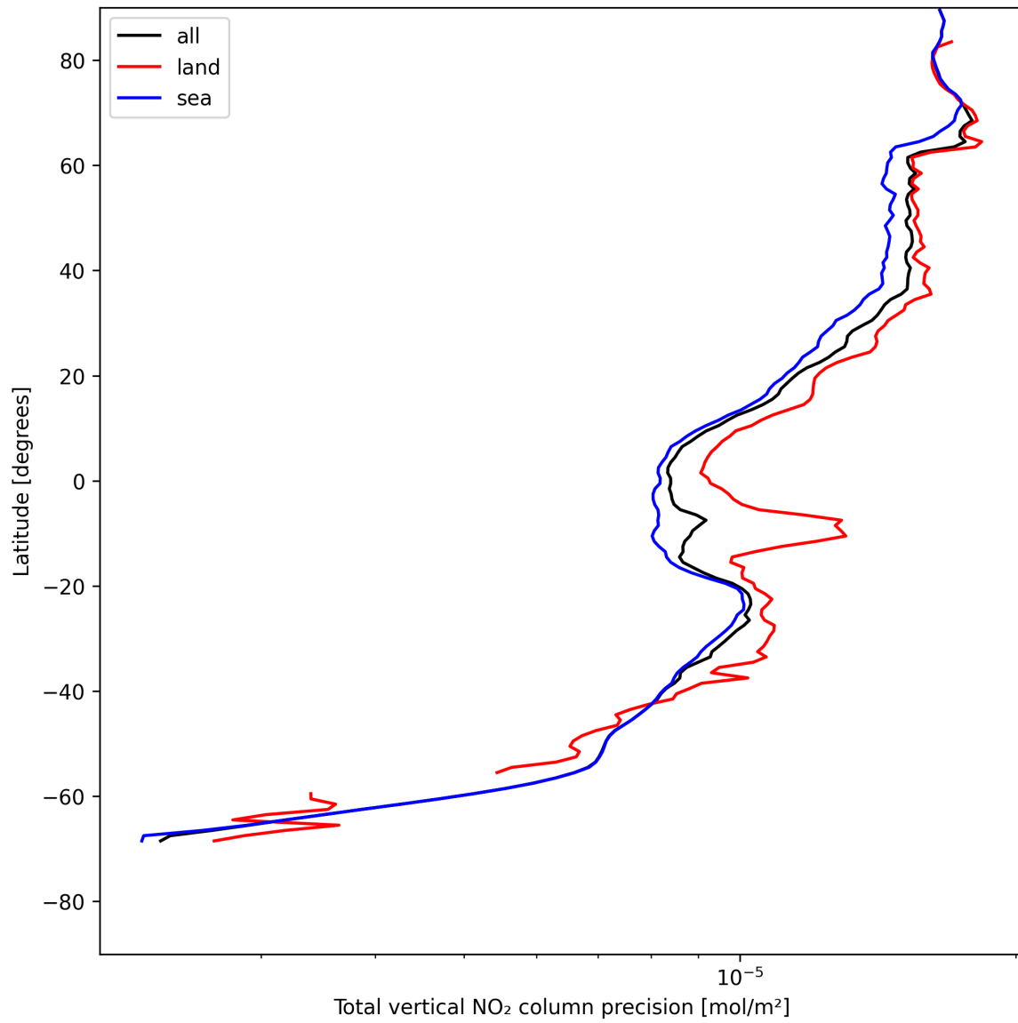
Figure 20: Zonal average of “Total vertical NO 2 column precision” for 2025-07-28 to 2025-07-29.
