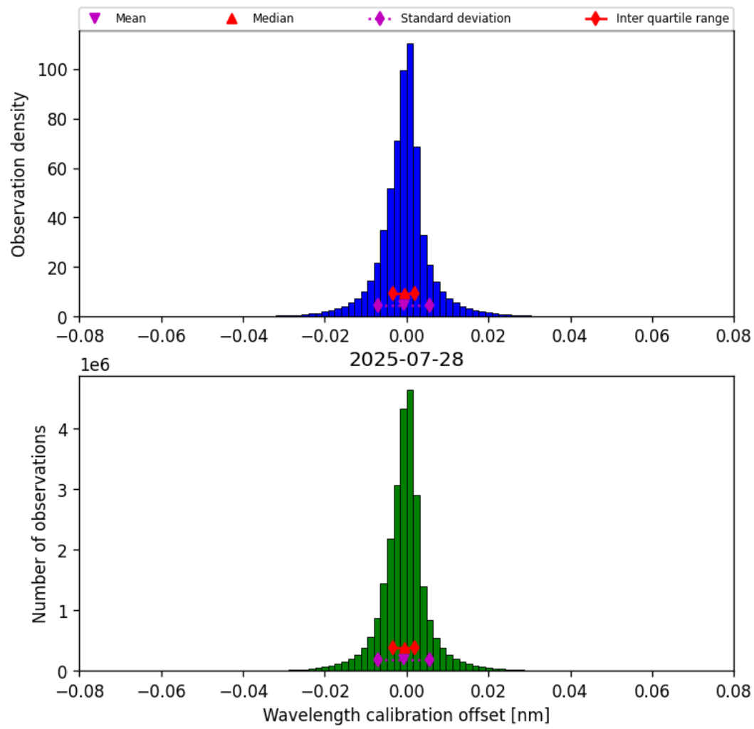
Figure 33: Histogram of “Wavelength calibration offset” for 2025-07-28 to 2025-07-29
