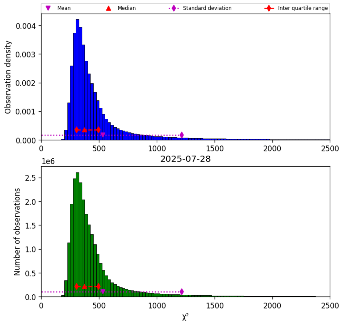
Figure 40: Histogram of “ \chi^2 ” for 2025-07-28 to 2025-07-29
