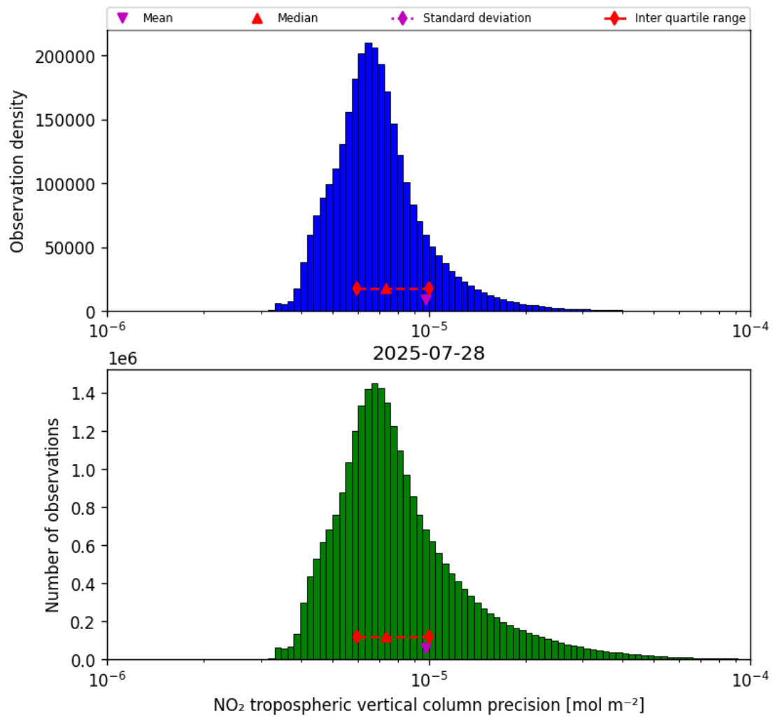
Figure 28: Histogram of “NO 2 tropospheric vertical column precision” for 2025-07-28 to 2025-07-29
