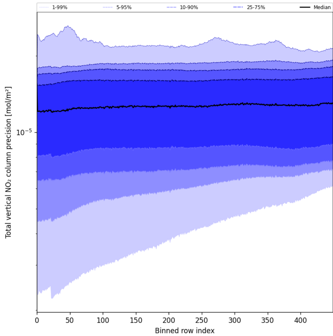
Figure 54: Along track statistics of “Total vertical NO 2 column precision” for 2025-07-28 to 2025-07-29
