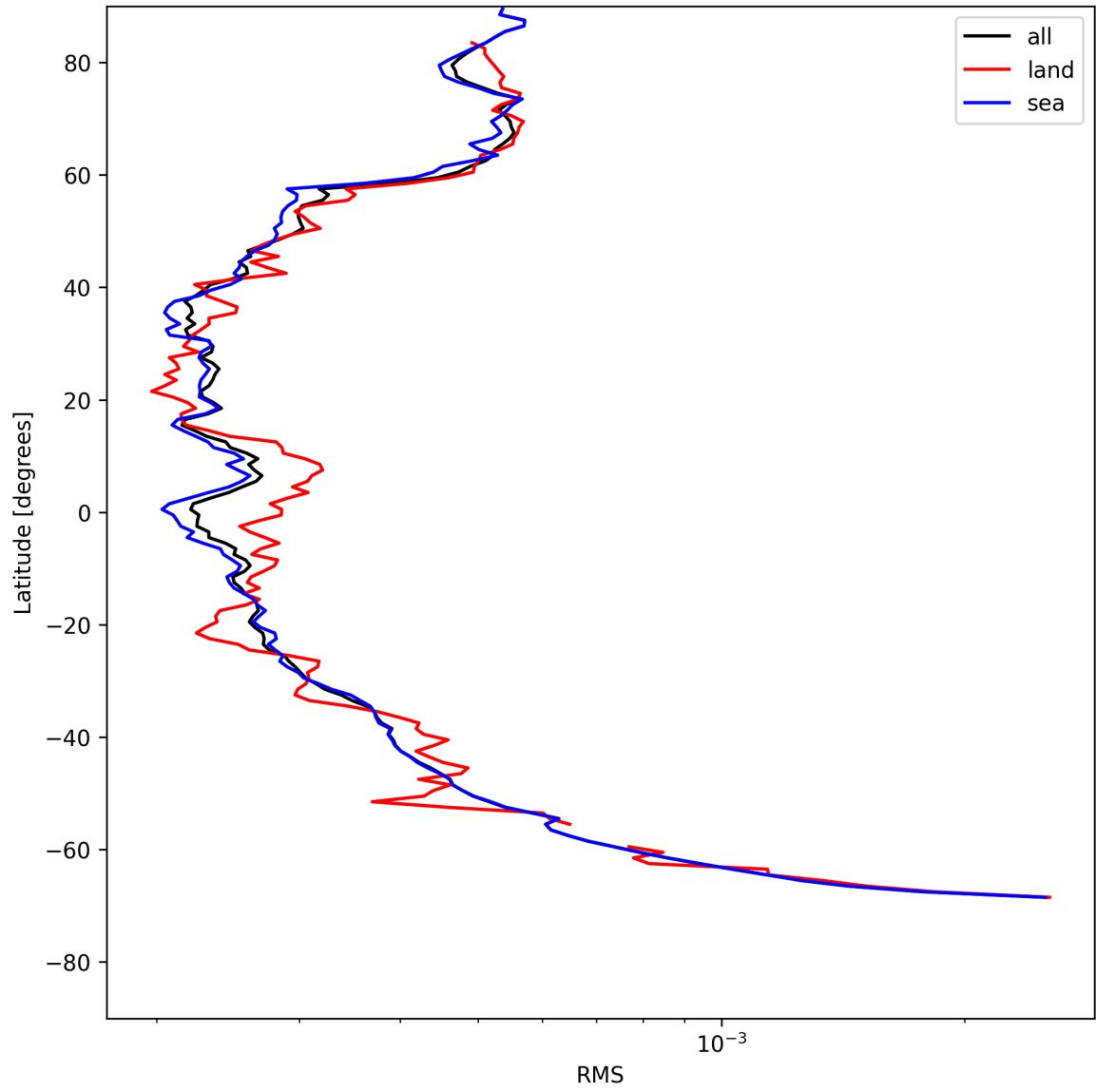
Figure 24: Zonal average of “RMS” for 2025-07-28 to 2025-07-29.
