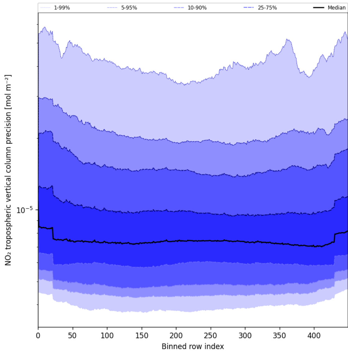
Figure 45: Along track statistics of “NO 2 tropospheric vertical column precision” for 2025-07-28 to 2025-07-29
