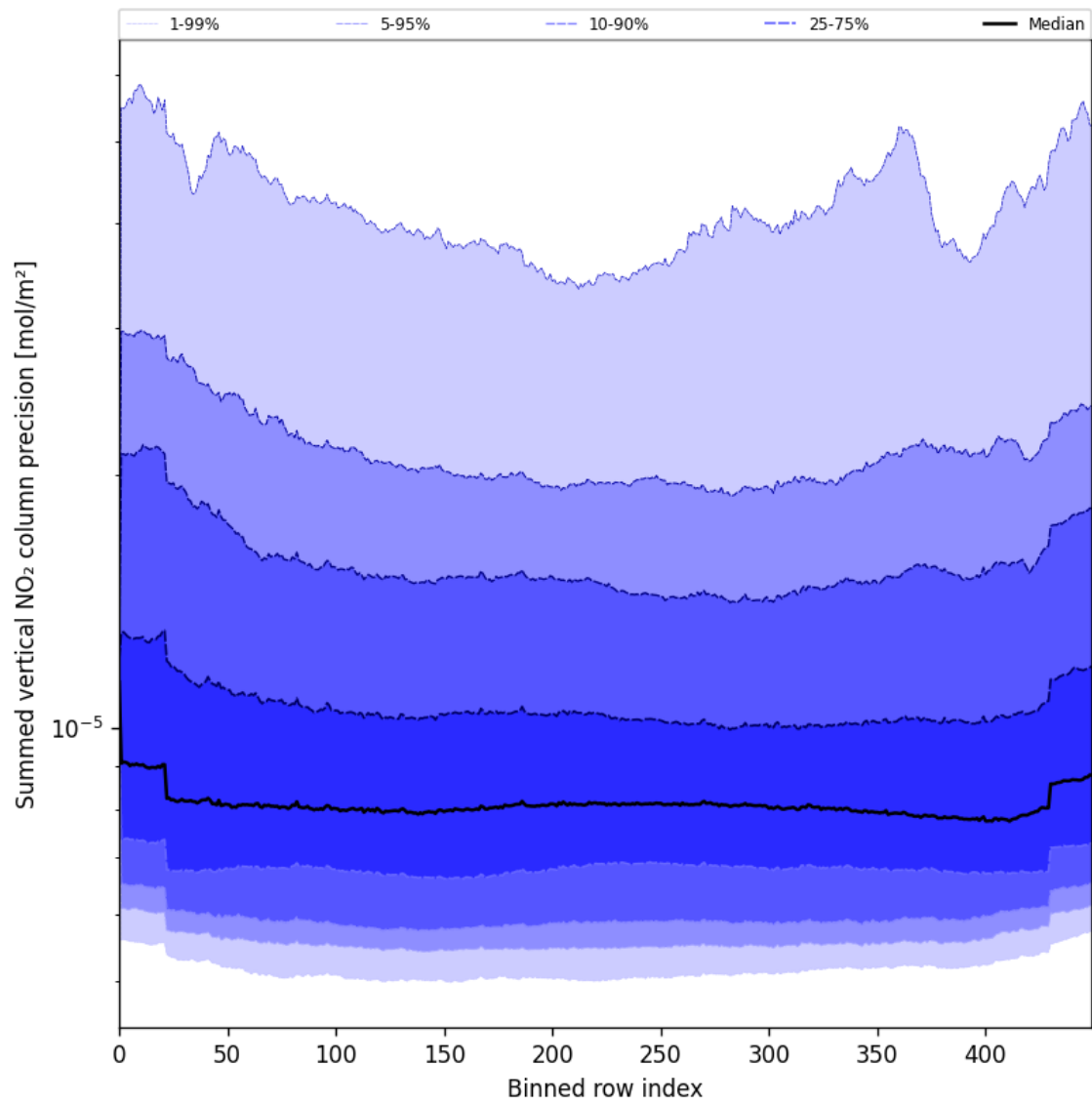
Figure 56: Along track statistics of “Summed vertical NO 2 column precision” for 2025-07-28 to 2025-07-29
