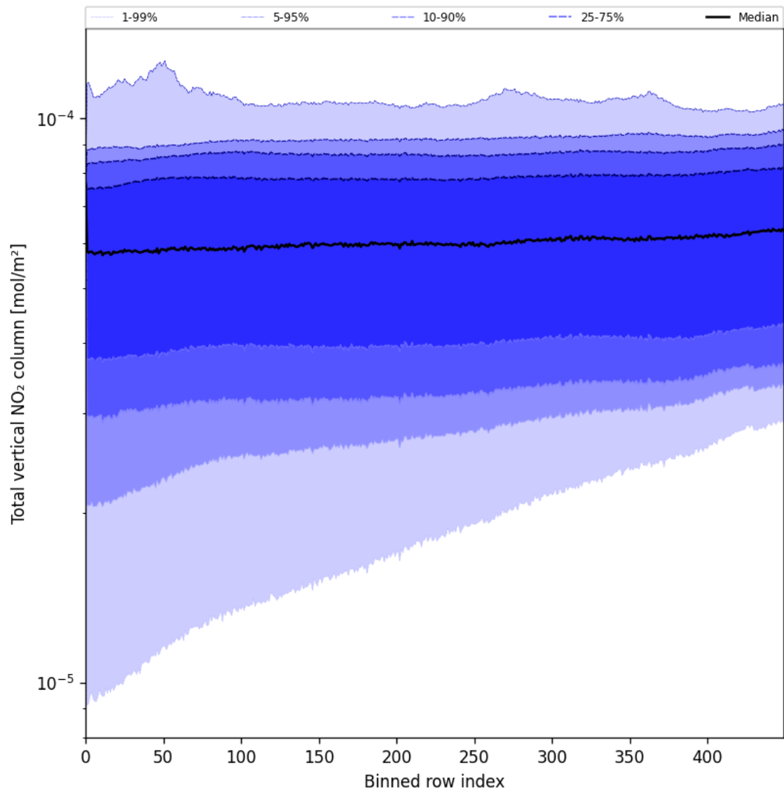
Figure 53: Along track statistics of “Total vertical NO 2 column” for 2025-07-28 to 2025-07-29
