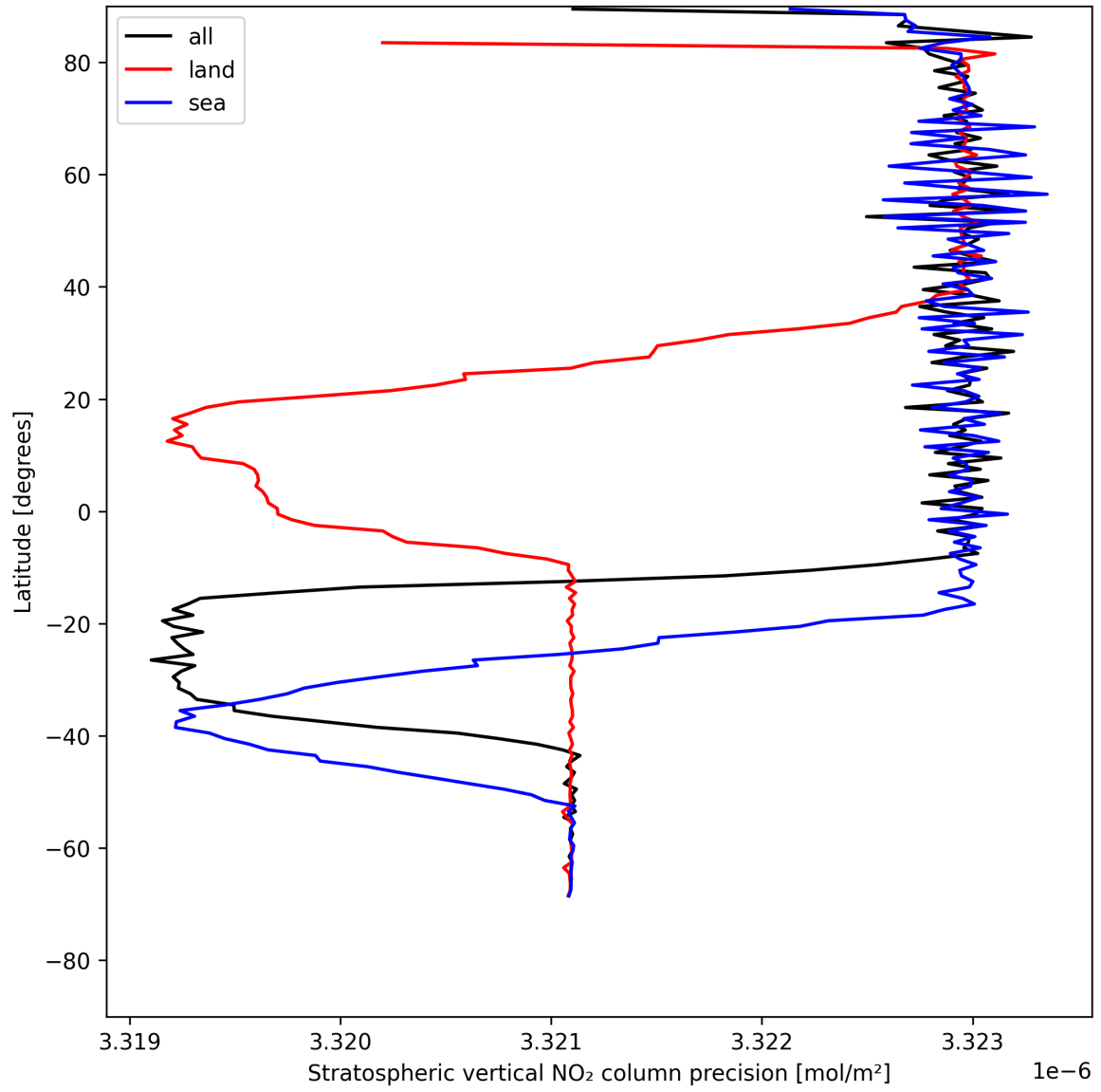
Figure 18: Zonal average of “Stratospheric vertical NO 2 column precision” for 2025-07-28 to 2025-07-29.
