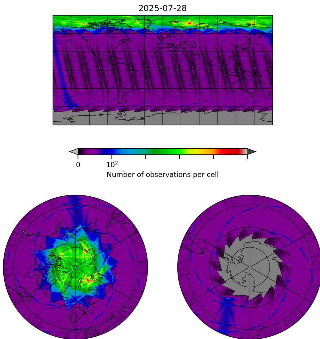
Figure 8: Map of the number of observations for 2025-07-28 to 2025-07-29
