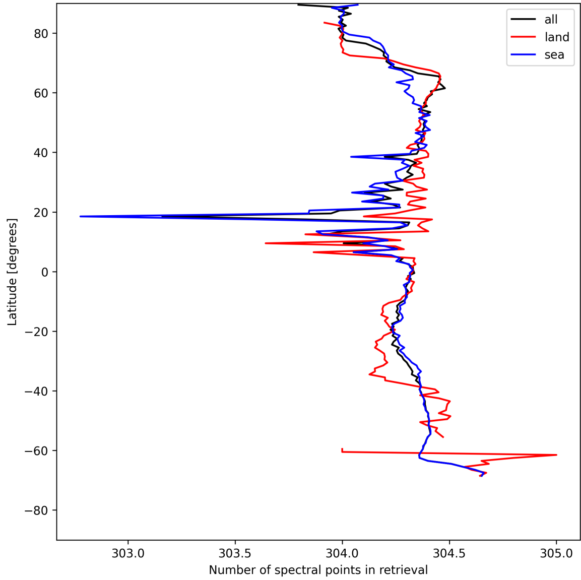
Figure 14: Zonal average of “Number of spectral points in retrieval” for 2025-07-28 to 2025-07-29.
