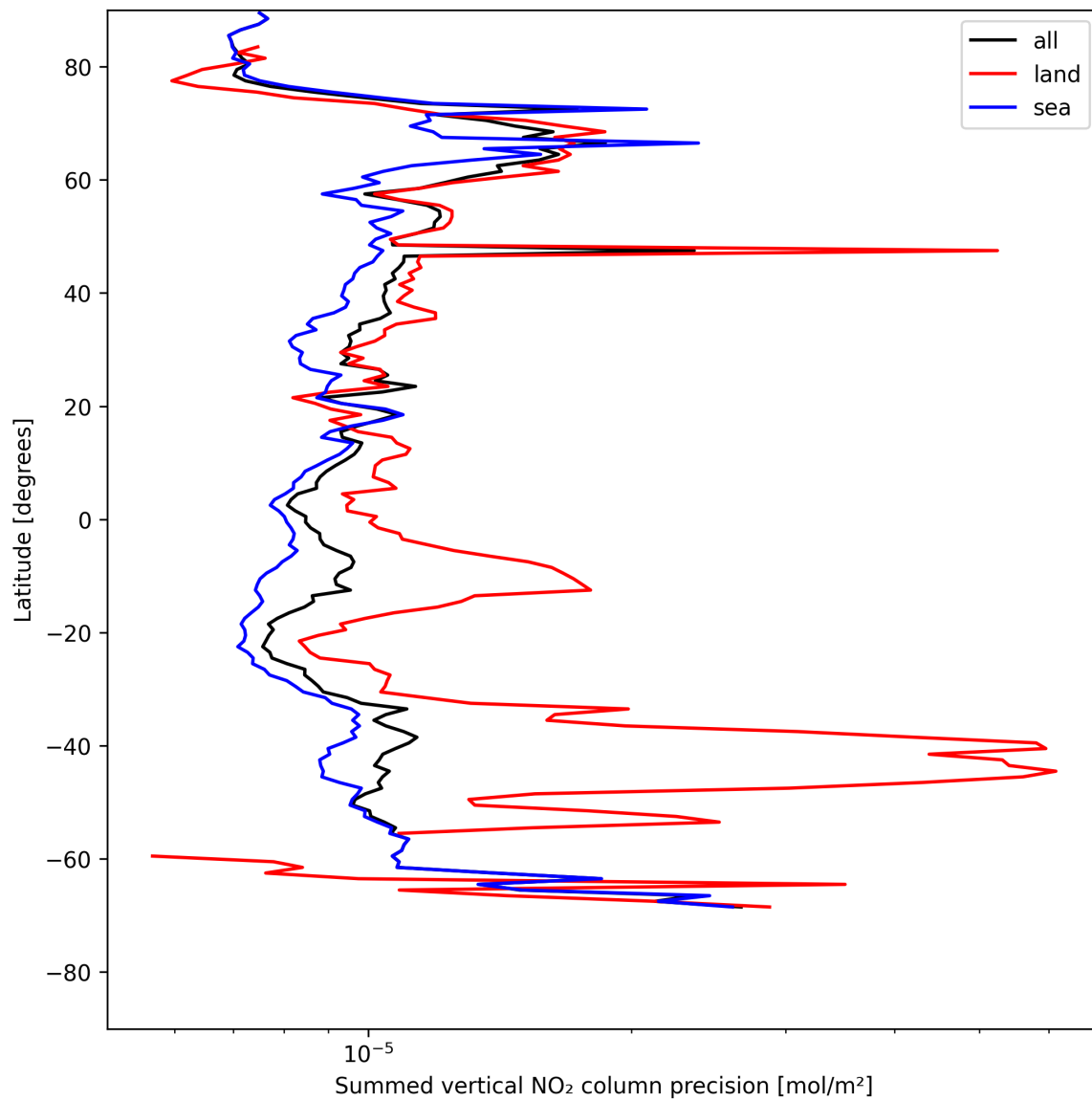
Figure 22: Zonal average of “Summed vertical NO 2 column precision” for 2025-07-28 to 2025-07-29.
