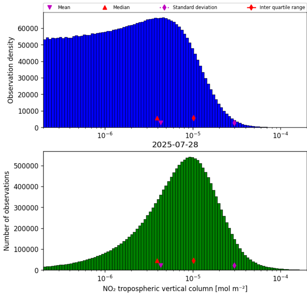
Figure 27: Histogram of “NO 2 tropospheric vertical column” for 2025-07-28 to 2025-07-29
