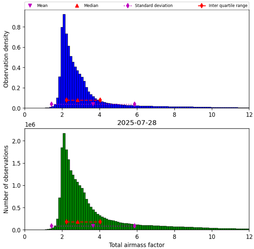
Figure 30: Histogram of “Total airmass factor” for 2025-07-28 to 2025-07-29
