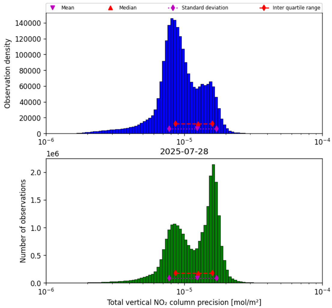
Figure 37: Histogram of “Total vertical NO 2 column precision” for 2025-07-28 to 2025-07-29
