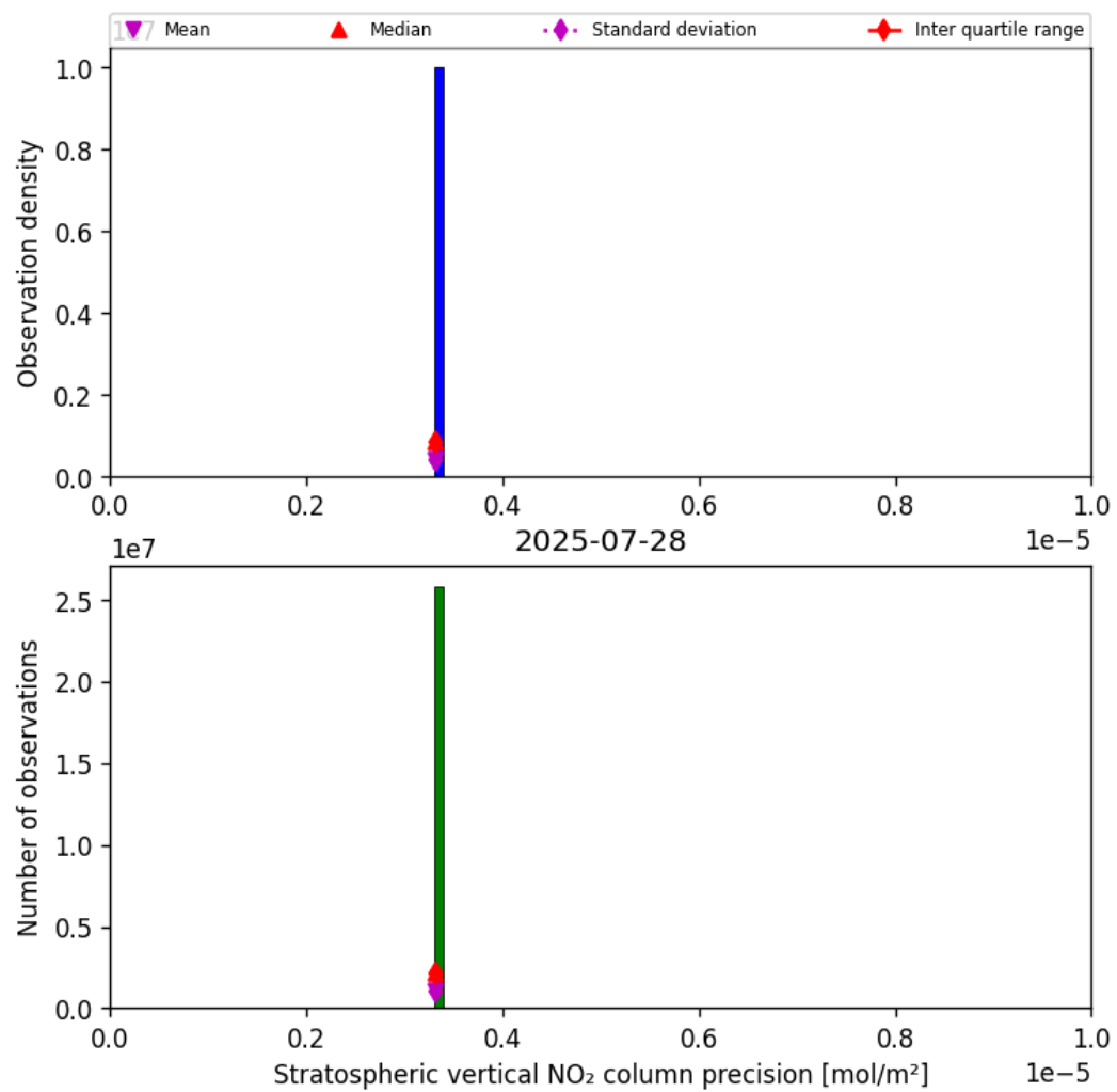
Figure 35: Histogram of “Stratospheric vertical NO 2 column precision” for 2025-07-28 to 2025-07-29
