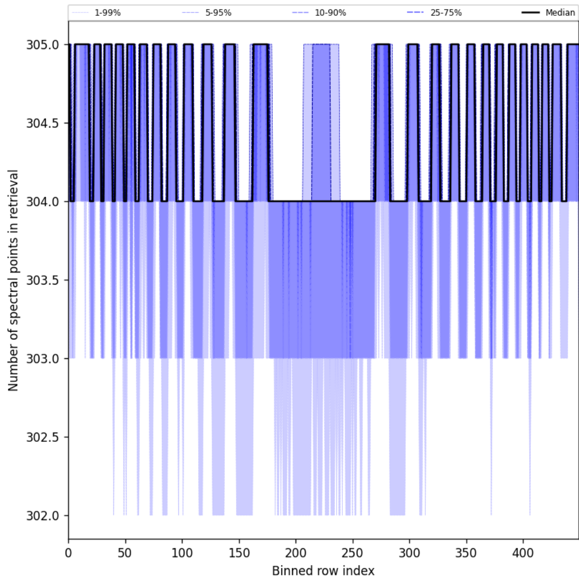
Figure 48: Along track statistics of “Number of spectral points in retrieval” for 2025-07-28 to 2025-07-29
