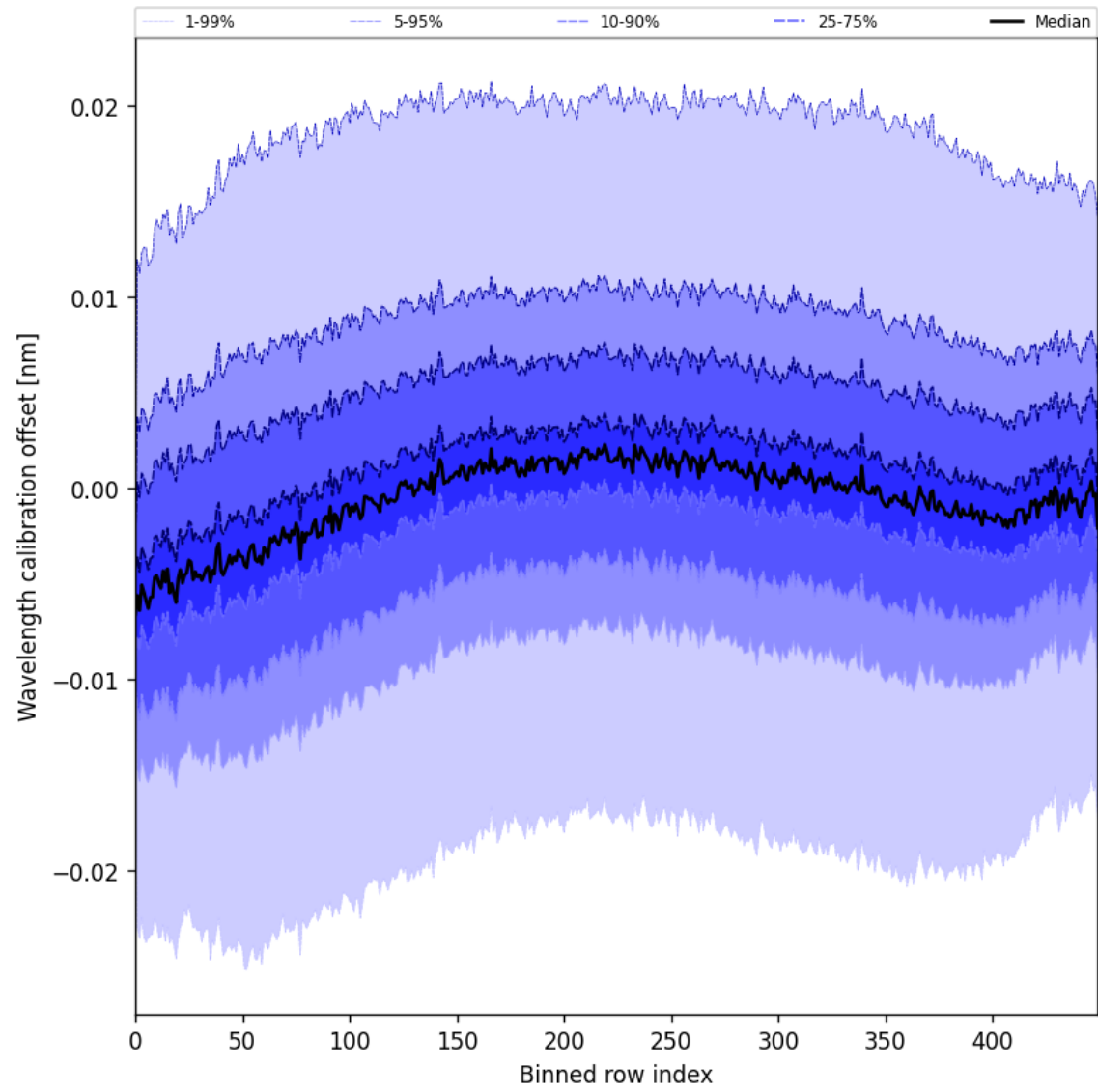
Figure 50: Along track statistics of “Wavelength calibration offset” for 2025-07-28 to 2025-07-29
