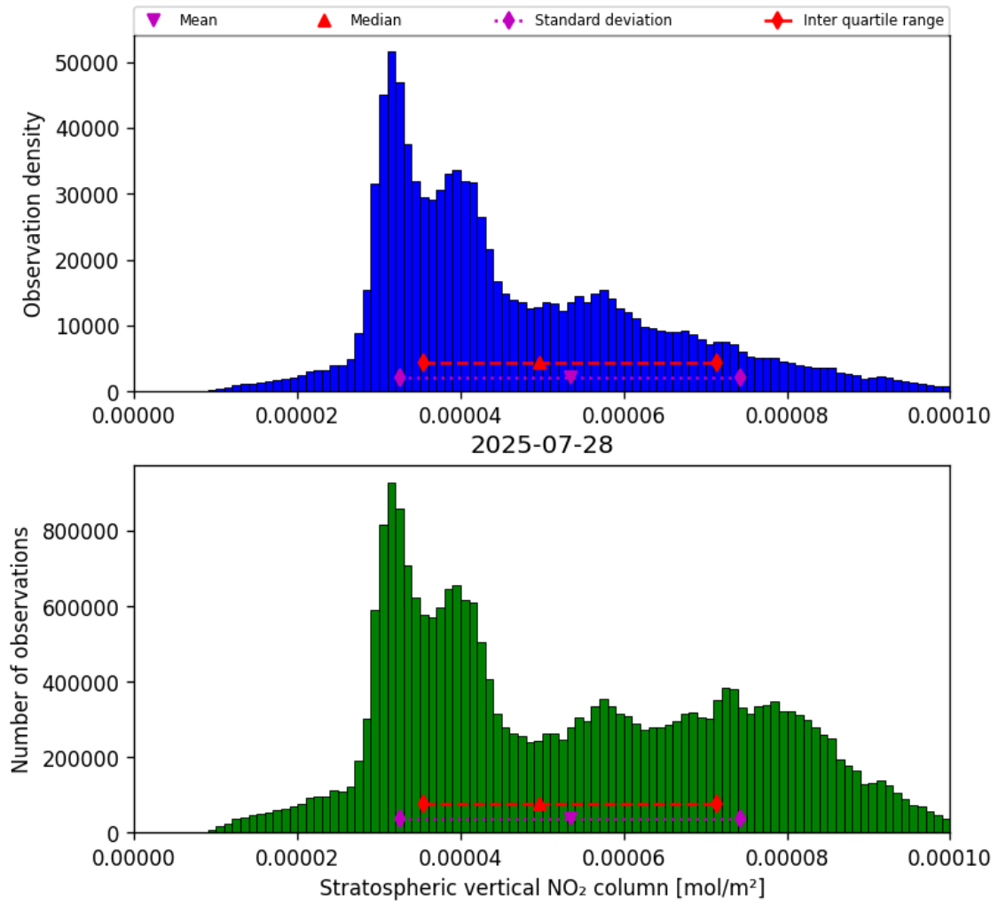
Figure 34: Histogram of “Stratospheric vertical NO 2 column” for 2025-07-28 to 2025-07-29
