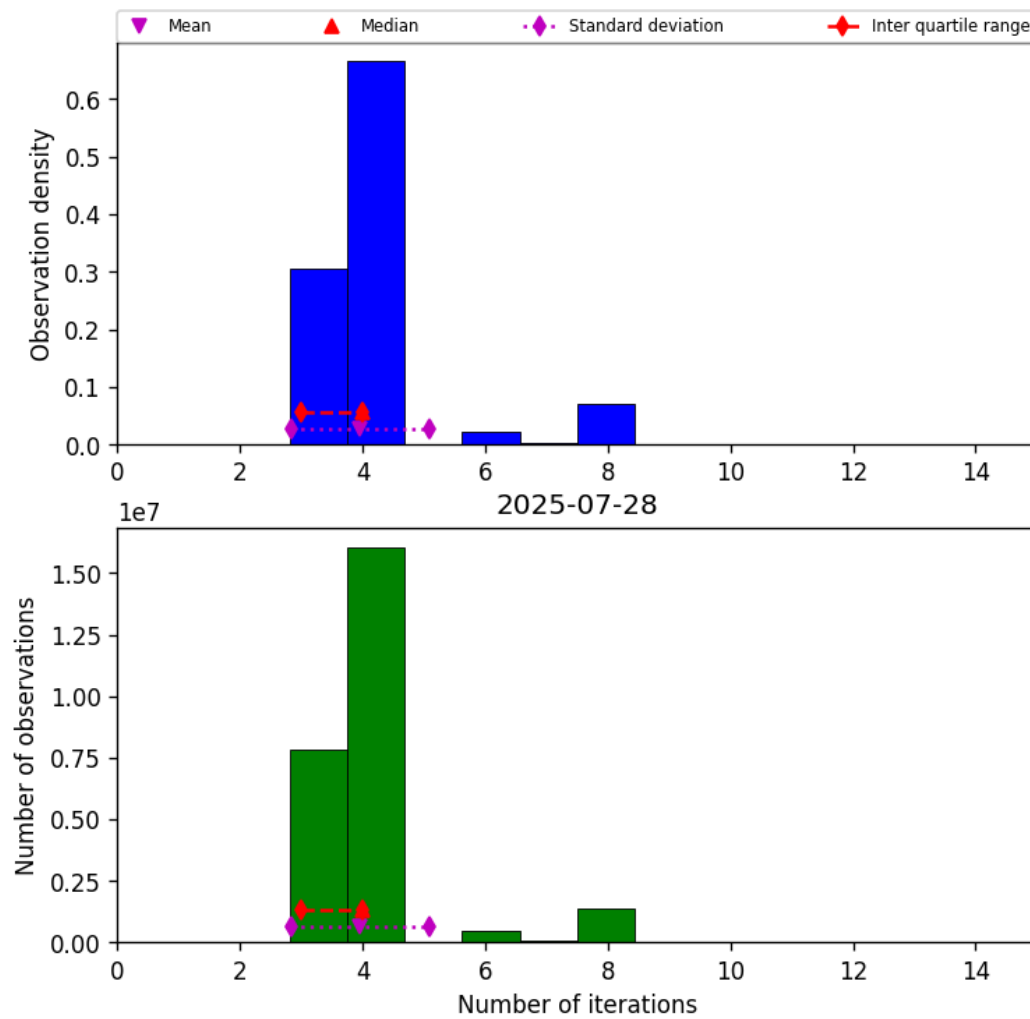
Figure 32: Histogram of “Number of iterations” for 2025-07-28 to 2025-07-29
