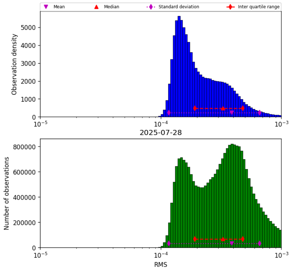
Figure 41: Histogram of “RMS” for 2025-07-28 to 2025-07-29
