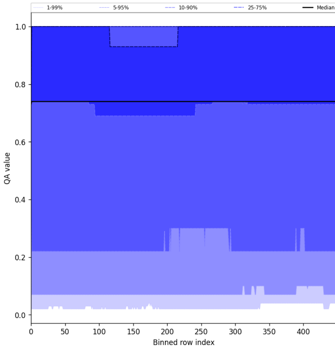
Figure 43: Along track statistics of “QA value” for 2025-07-28 to 2025-07-29
