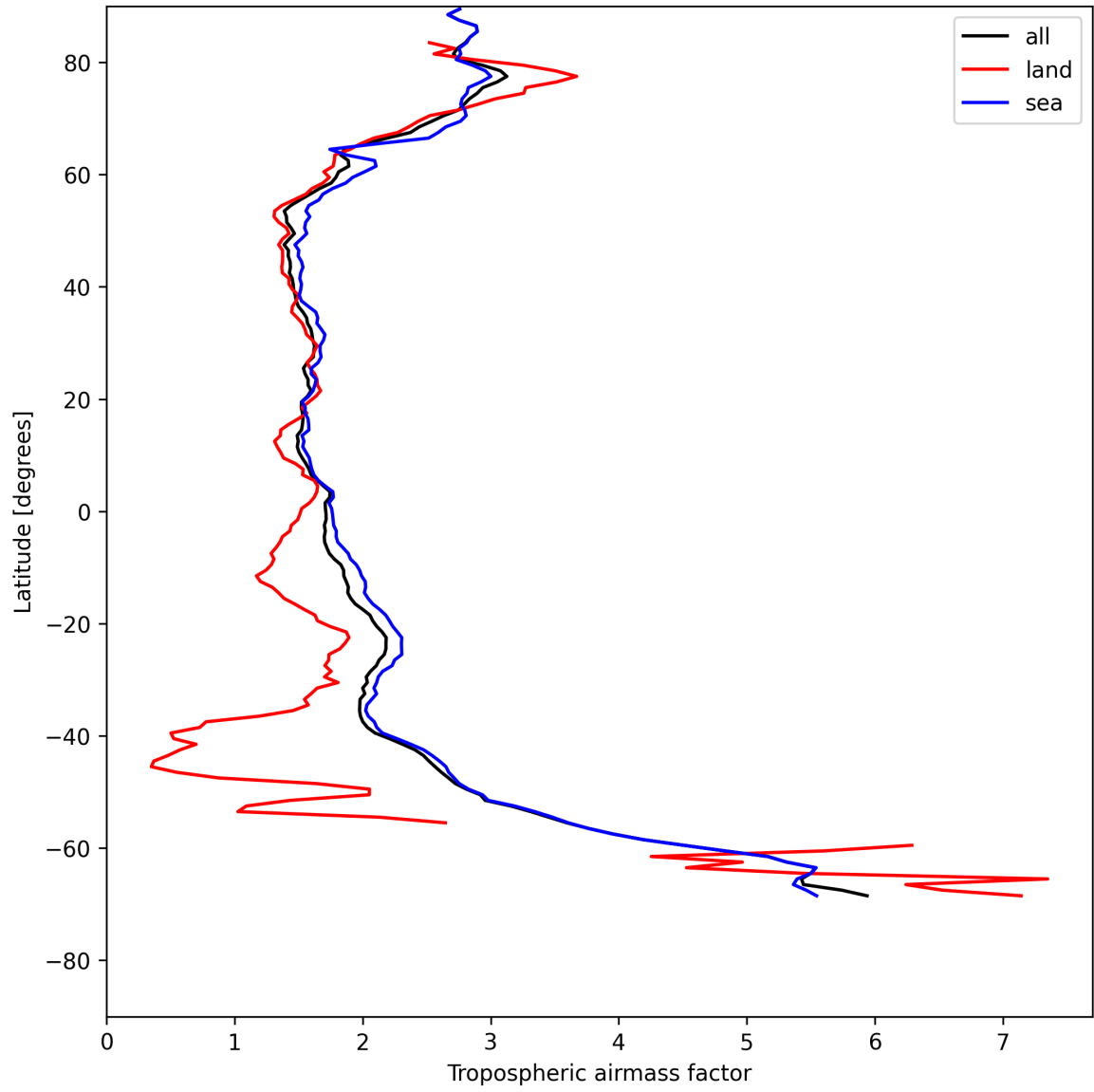
Figure 12: Zonal average of “Tropospheric airmass factor” for 2025-07-28 to 2025-07-29.
