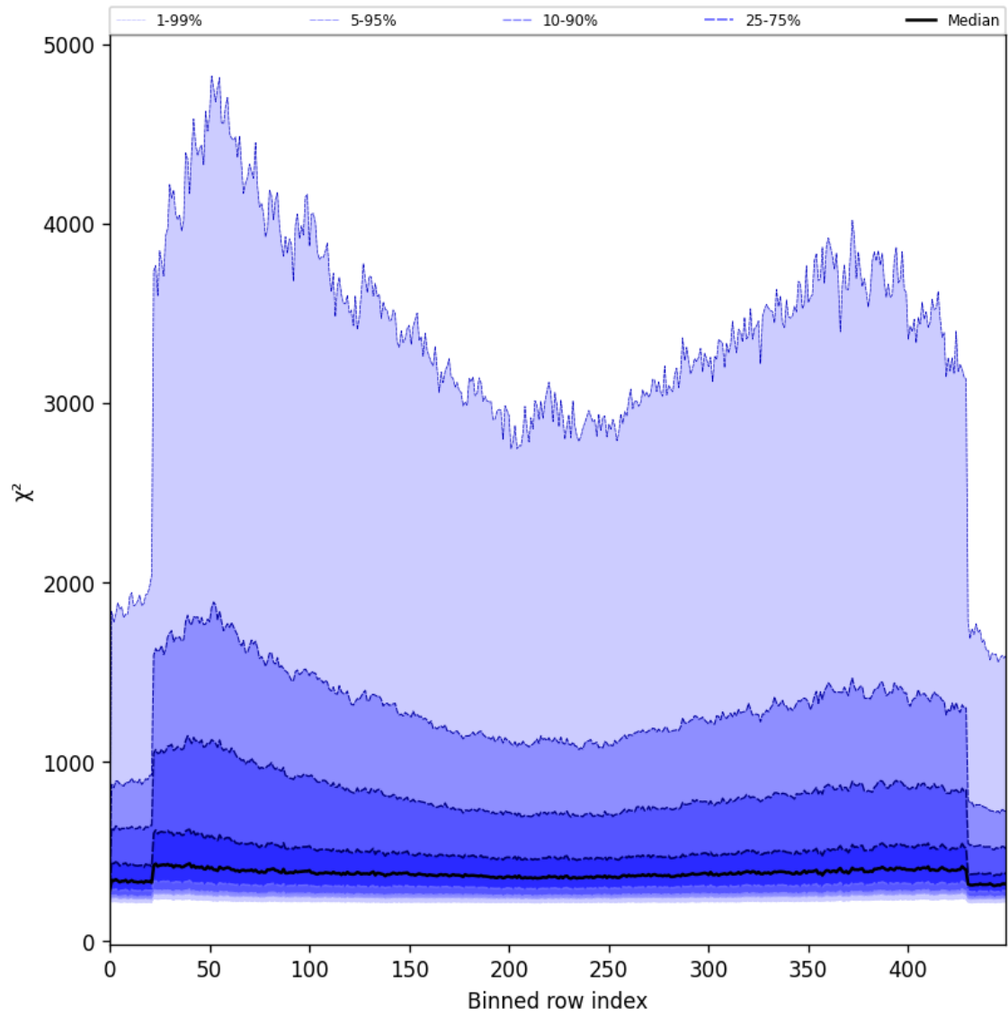
Figure 57: Along track statistics of “ \chi^2 ” for 2025-07-28 to 2025-07-29
