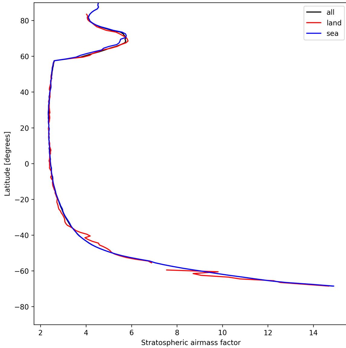
Figure 25: Zonal average of “Stratospheric air mass factor” for 2025-07-28 to 2025-07-29.
