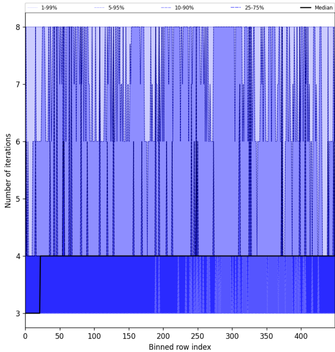
Figure 49: Along track statistics of “Number of iterations” for 2025-07-28 to 2025-07-29
