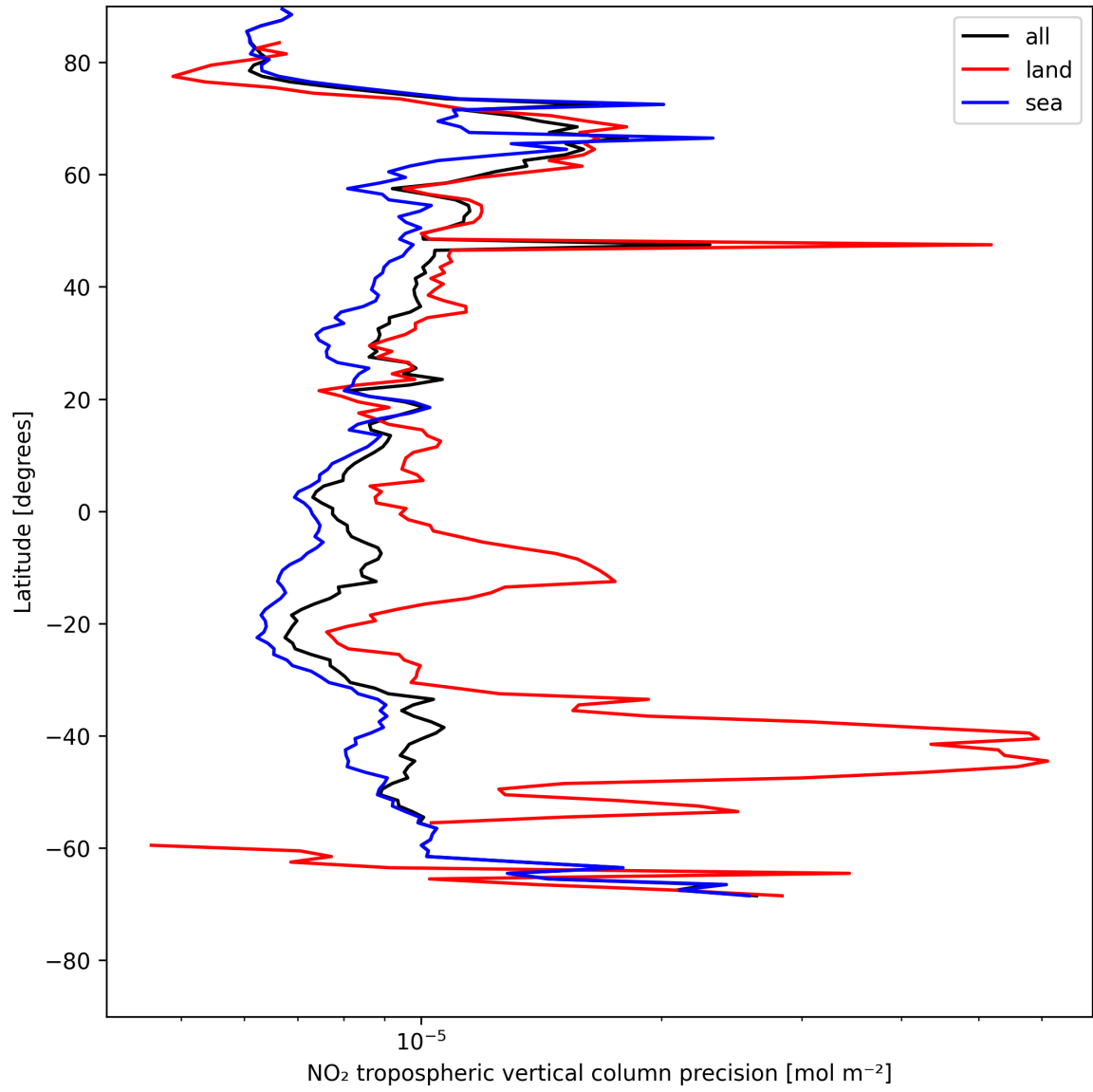
Figure 11: Zonal average of “NO 2 tropospheric vertical column precision” for 2025-07-28 to 2025-07-29.
