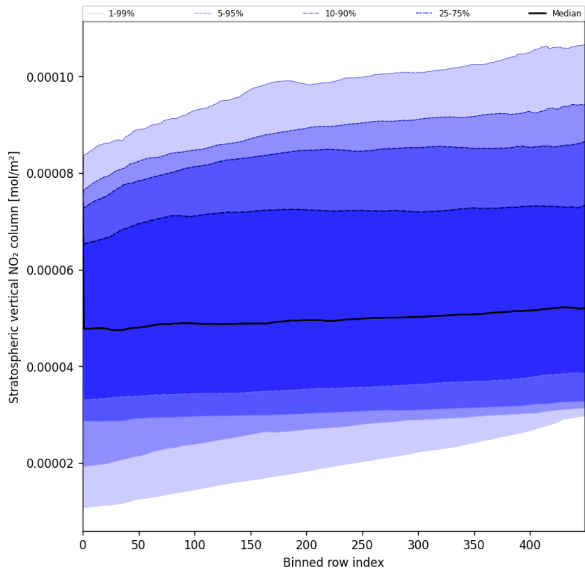
Figure 51: Along track statistics of “Stratospheric vertical NO 2 column” for 2025-07-28 to 2025-07-29
