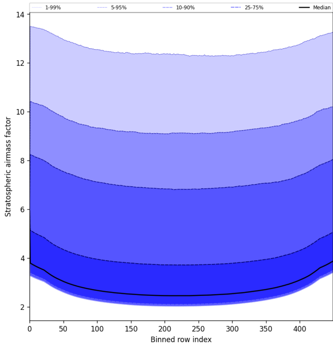
Figure 59: Along track statistics of “Stratospheric airmass factor” for 2025-07-28 to 2025-07-29
