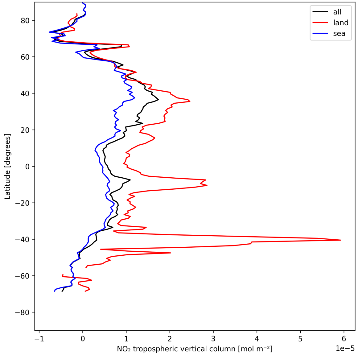
Figure 10: Zonal average of “NO 2 tropospheric vertical column” for 2025-07-28 to 2025-07-29.
