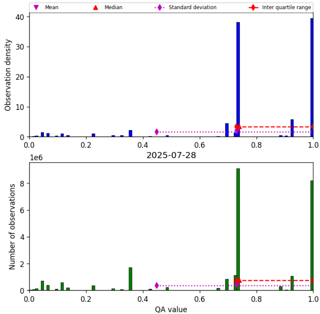
Figure 26: Histogram of “QA value” for 2025-07-28 to 2025-07-29
