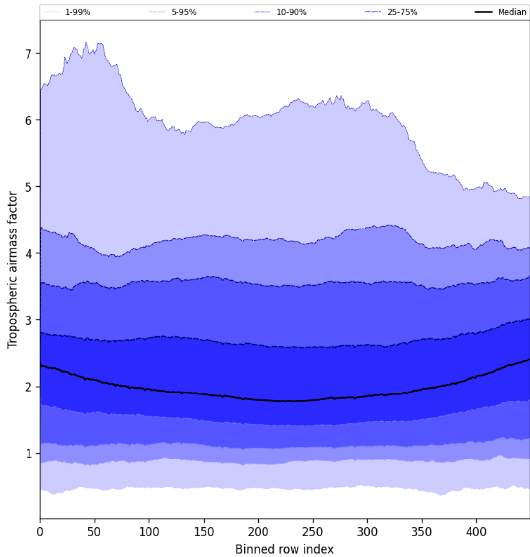
Figure 46: Along track statistics of “Tropospheric airmass factor” for 2025-07-28 to 2025-07-29
