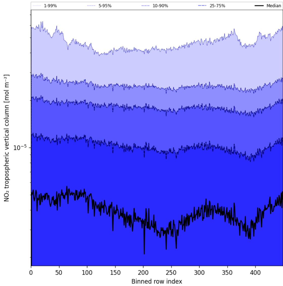
Figure 44: Along track statistics of “NO 2 tropospheric vertical column” for 2025-07-28 to 2025-07-29
