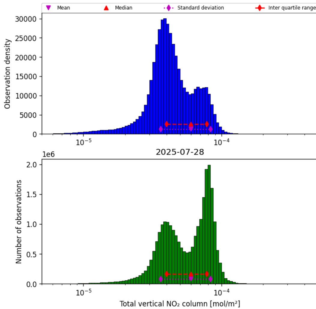
Figure 36: Histogram of "Total vertical NO 2 column" for 2025-07-28 to 2025-07-29
