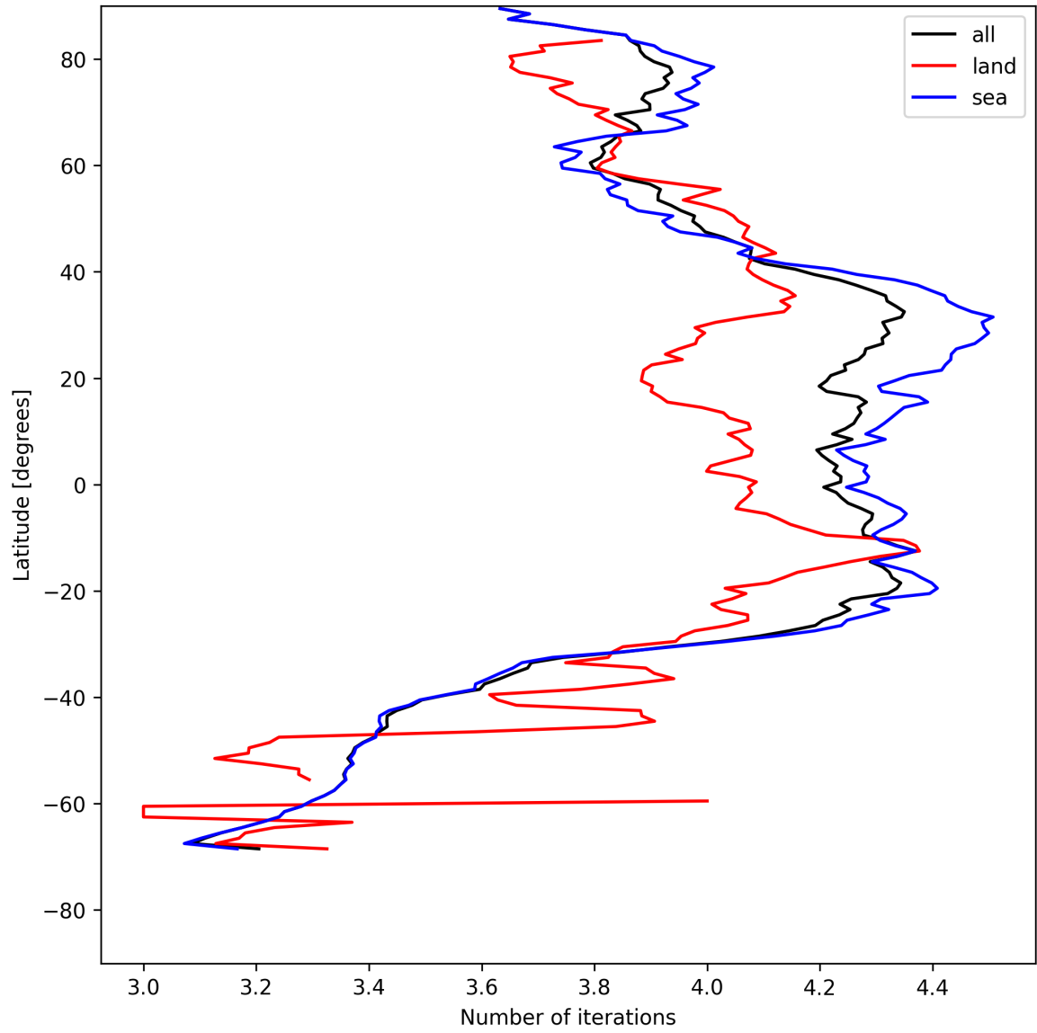
Figure 15: Zonal average of “Number of iterations” for 2025-07-28 to 2025-07-29.
