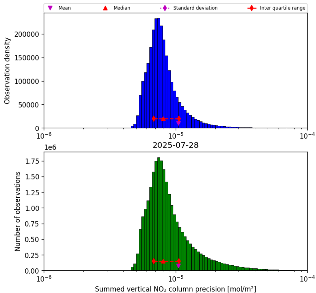
Figure 39: Histogram of "Summed vertical NO 2 column precision" for 2025-07-28 to 2025-07-29
