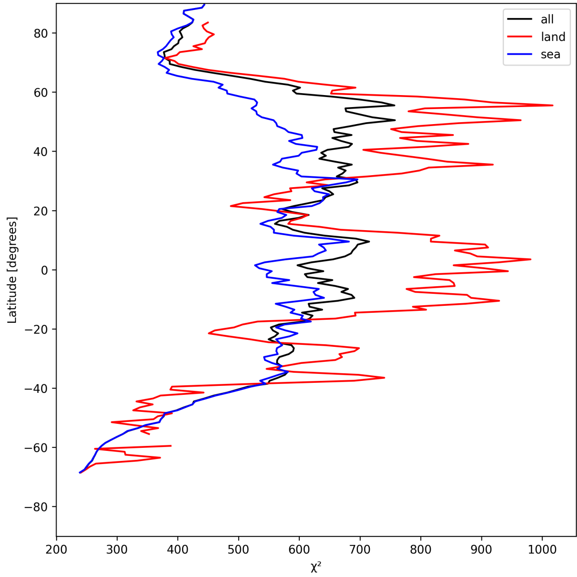
Figure 23: Zonal average of “ \chi^2 ” for 2025-07-28 to 2025-07-29.
