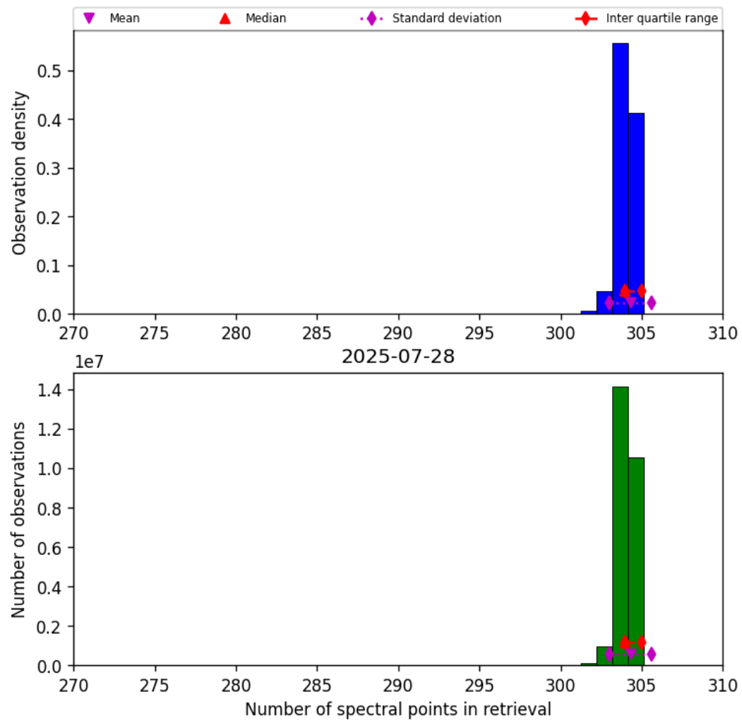
Figure 31: Histogram of “Number of spectral points in retrieval” for 2025-07-28 to 2025-07-29
