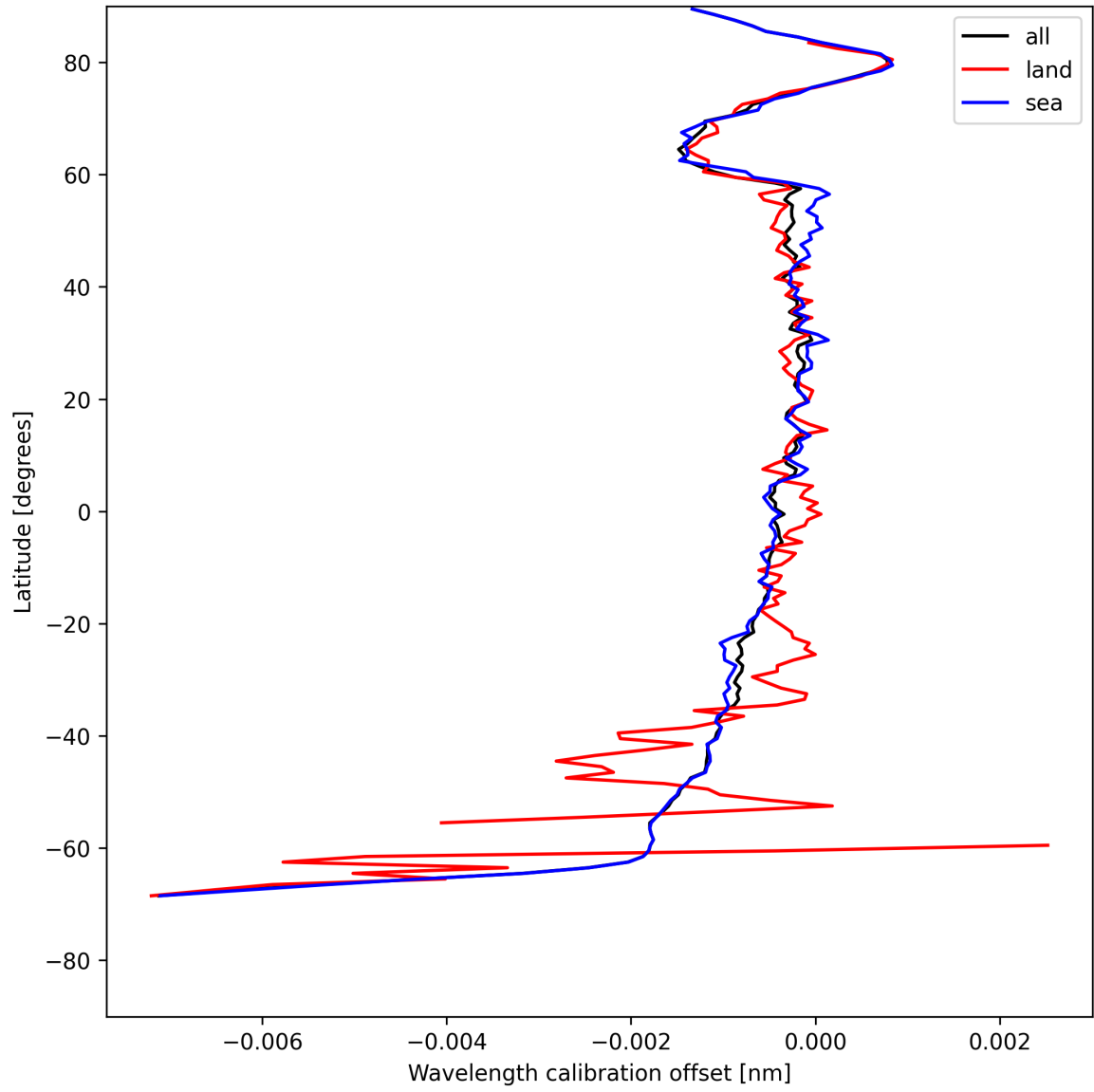
Figure 16: Zonal average of “Wavelength calibration offset” for 2025-07-28 to 2025-07-29.
