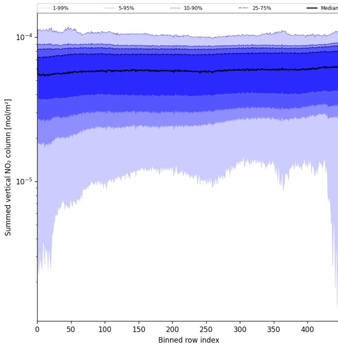
Figure 55: Along track statistics of “Summed vertical NO 2 column” for 2025-07-28 to 2025-07-29
