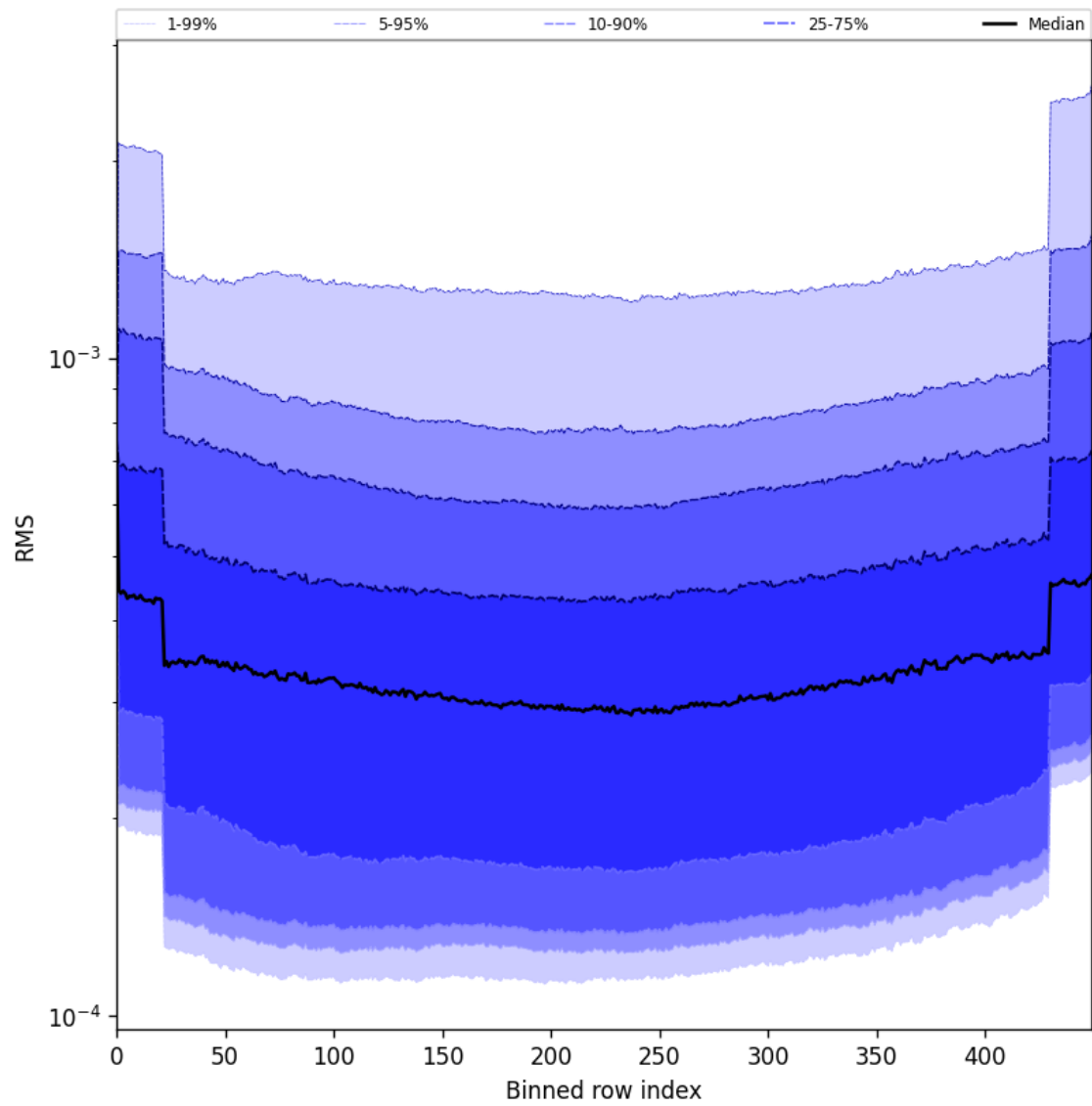
Figure 58: Along track statistics of “RMS” for 2025-07-28 to 2025-07-29
