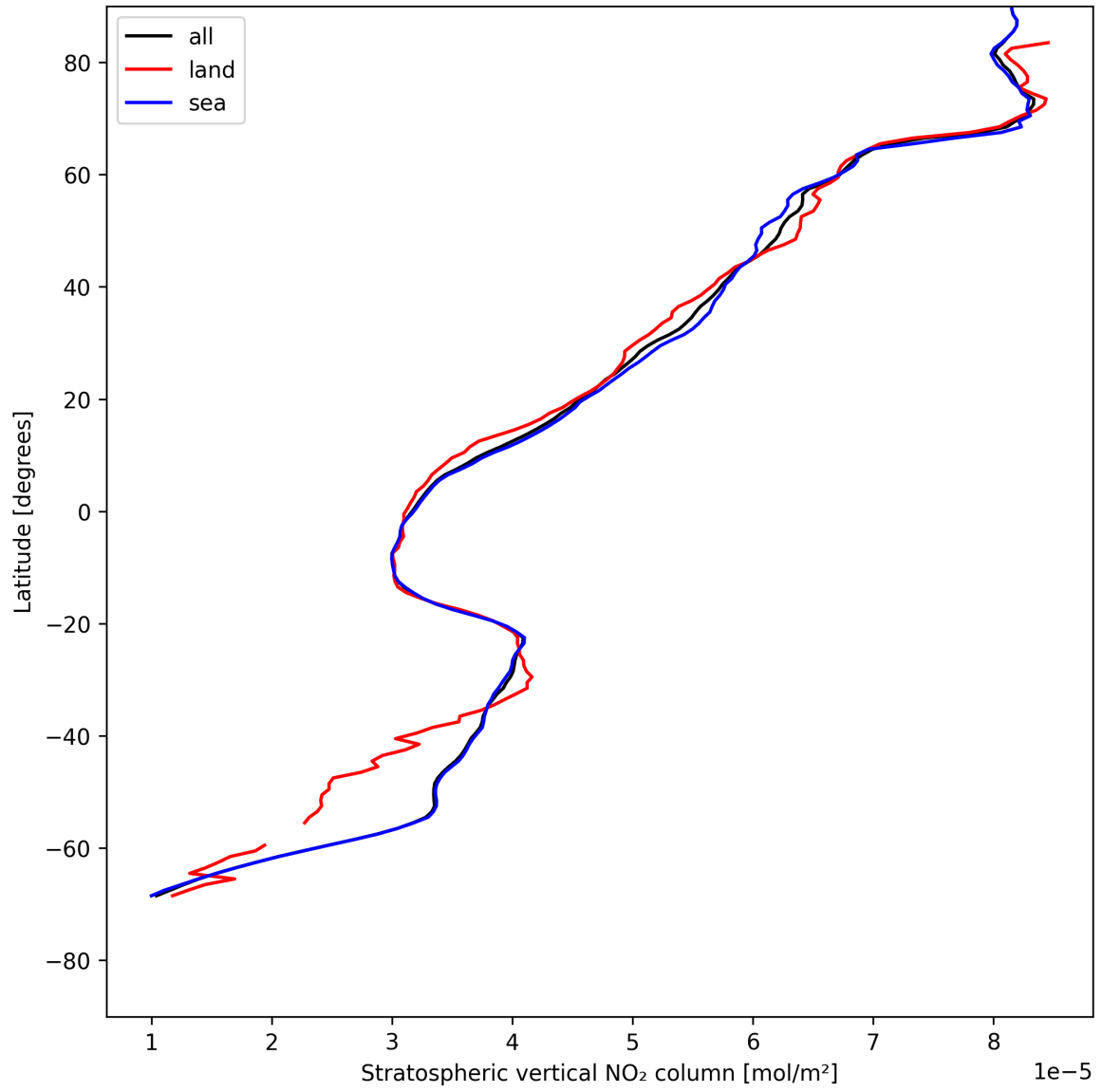
Figure 17: Zonal average of “Stratospheric vertical NO 2 column” for 2025-07-28 to 2025-07-29.
