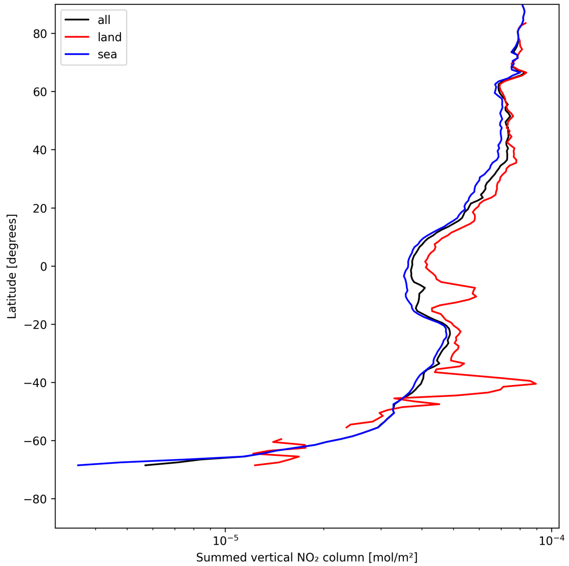
Figure 21: Zonal average of “Summed vertical NO 2 column” for 2025-07-28 to 2025-07-29.
