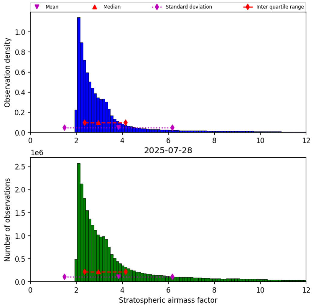
Figure 42: Histogram of “Stratospheric airmass factor” for 2025-07-28 to 2025-07-29
