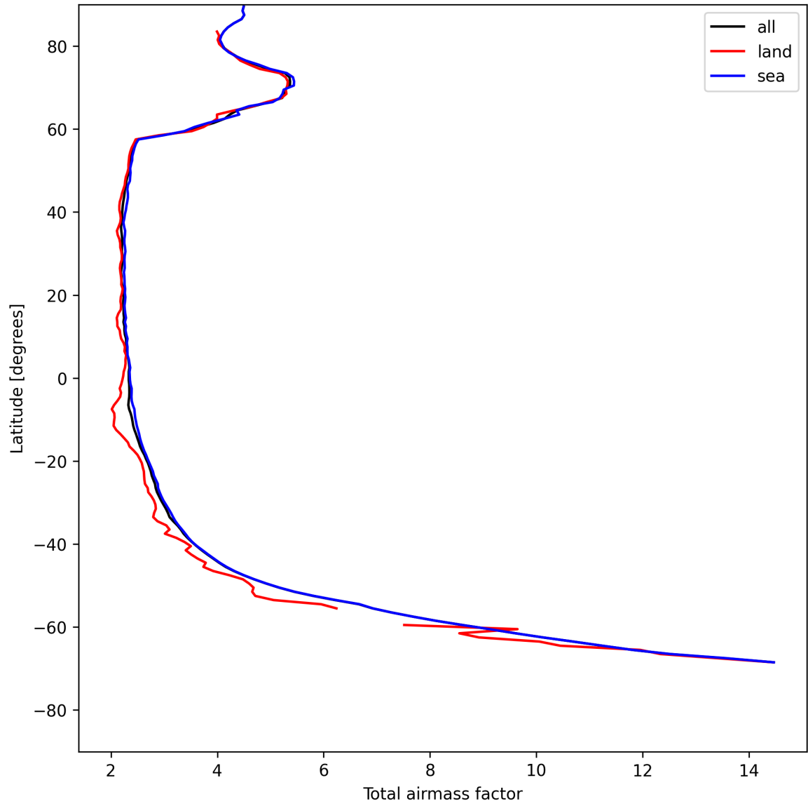
Figure 13: Zonal average of “Total airmass factor” for 2025-07-28 to 2025-07-29.
