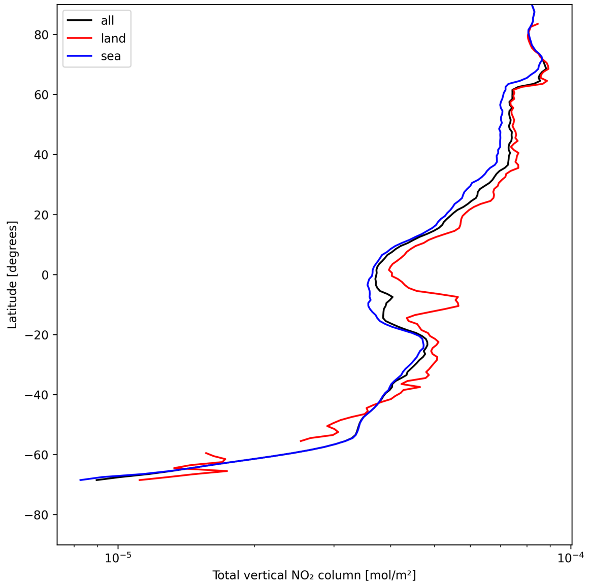
Figure 19: Zonal average of “Total vertical NO 2 column” for 2025-07-28 to 2025-07-29.
