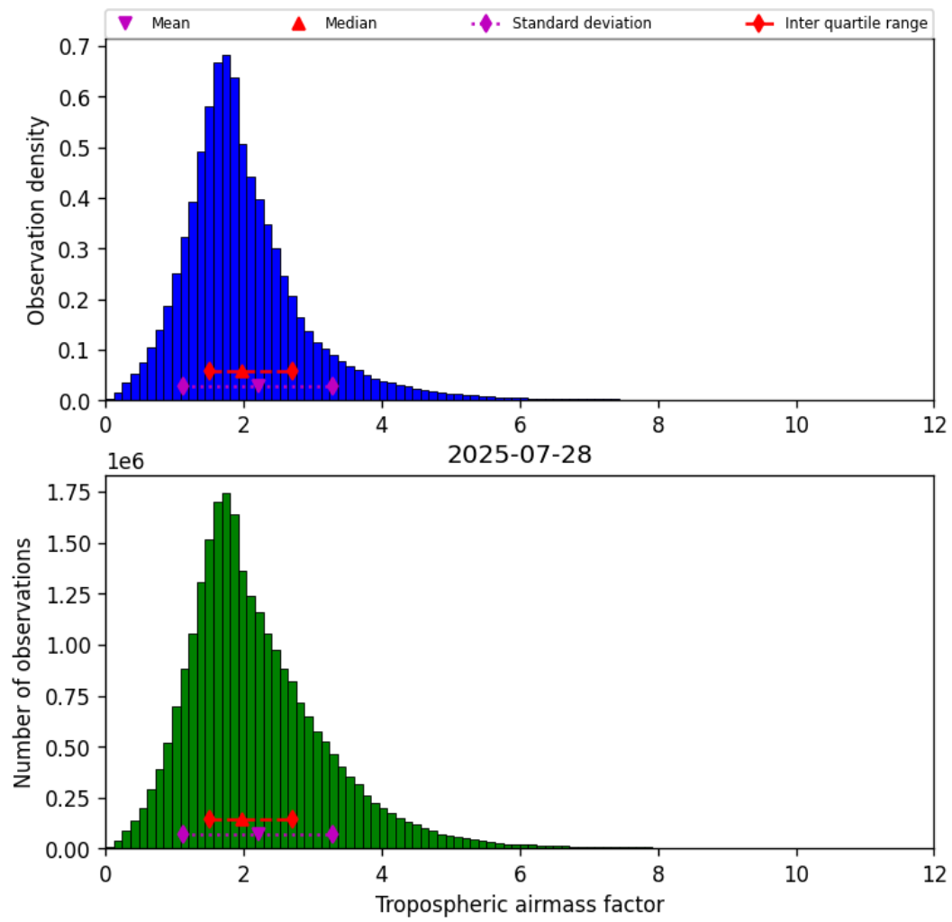
Figure 29: Histogram of “Tropospheric airmass factor” for 2025-07-28 to 2025-07-29
