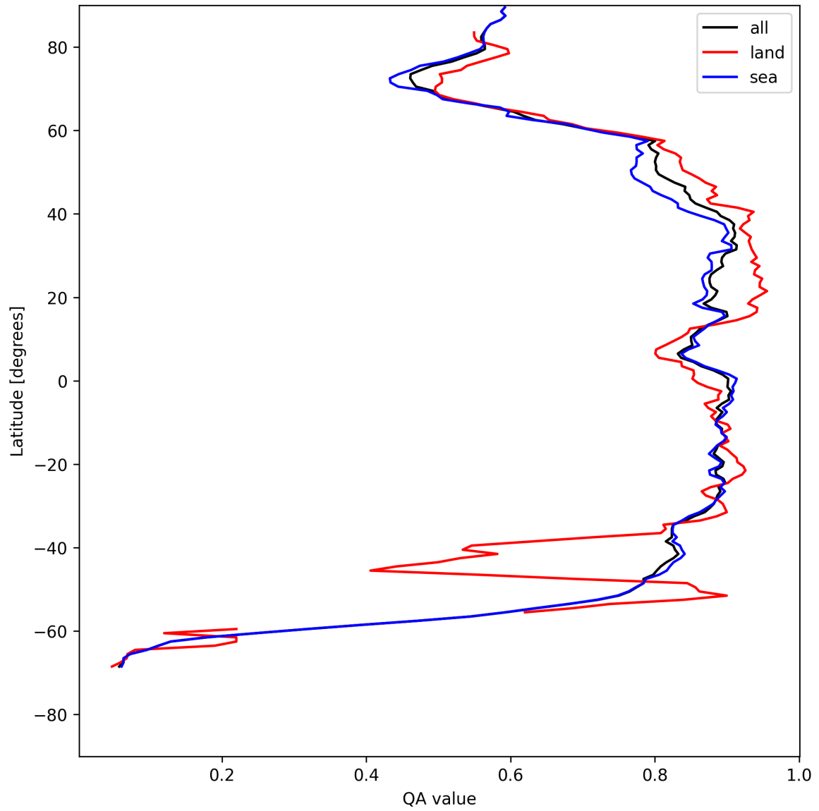
Figure 9: Zonal average of “QA value” for 2025-07-28 to 2025-07-29.
