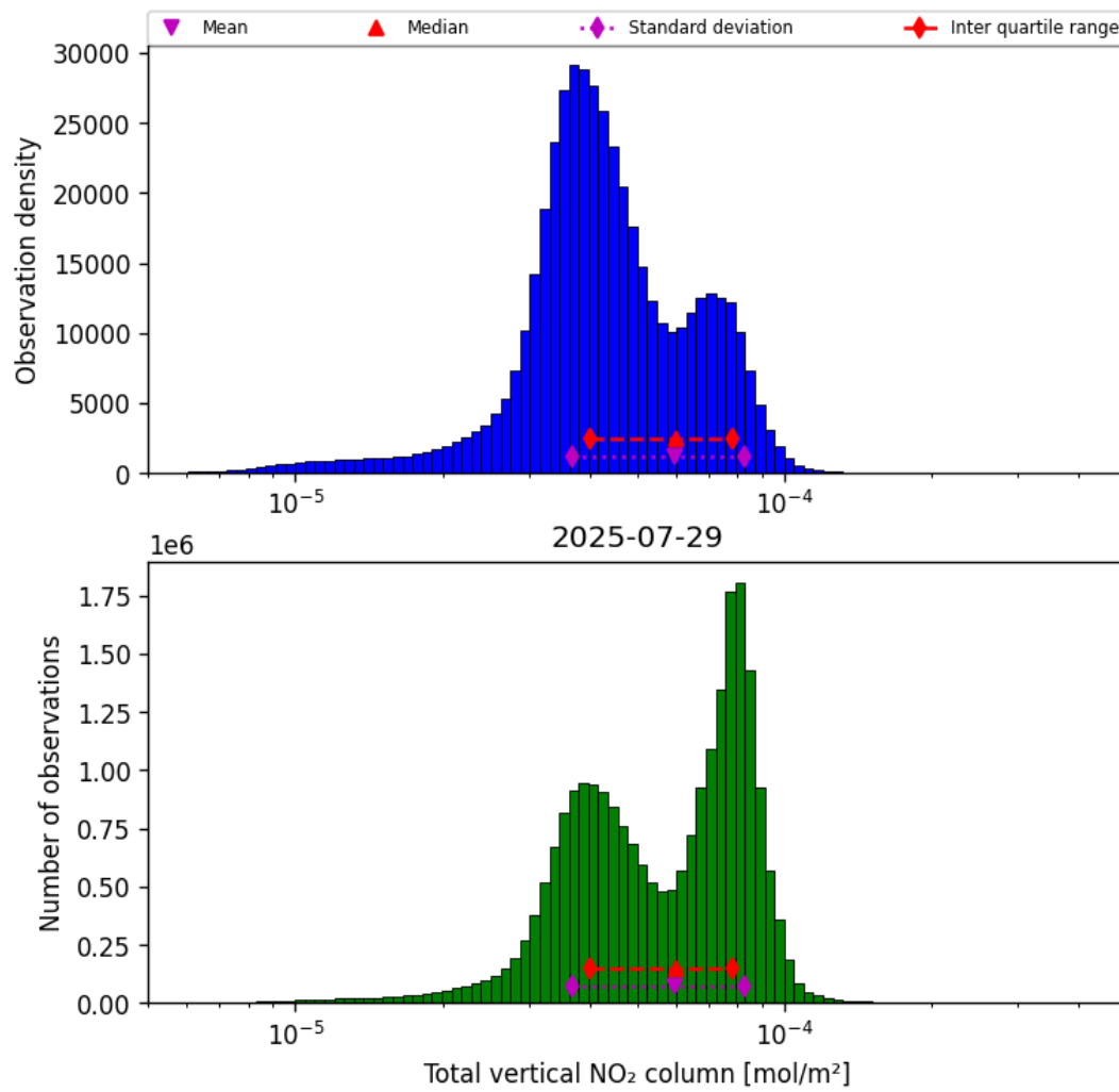
Figure 36: Histogram of “Total vertical NO 2 column” for 2025-07-29 to 2025-07-30
