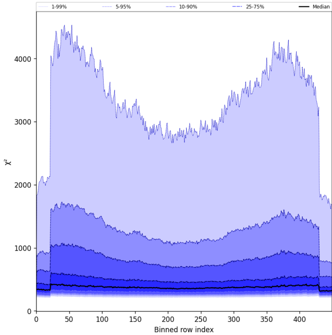
Figure 57: Along track statistics of “ \chi^2 ” for 2025-07-29 to 2025-07-30
