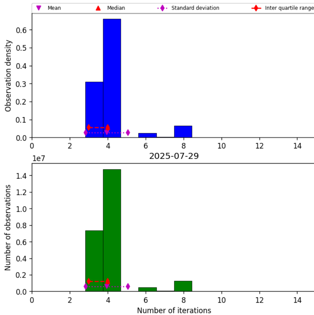
Figure 32: Histogram of “Number of iterations” for 2025-07-29 to 2025-07-30
