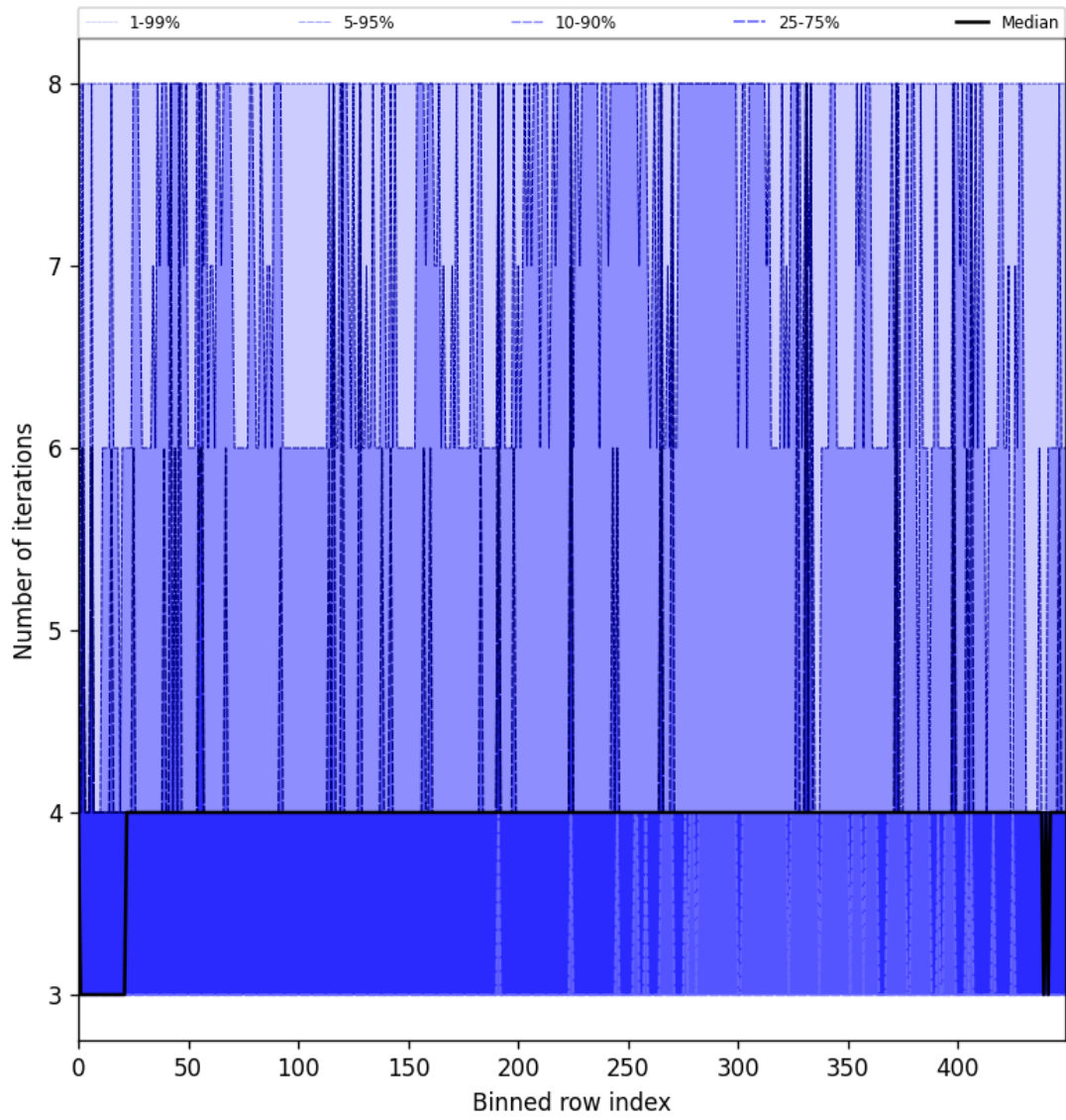
Figure 49: Along track statistics of “Number of iterations” for 2025-07-29 to 2025-07-30
