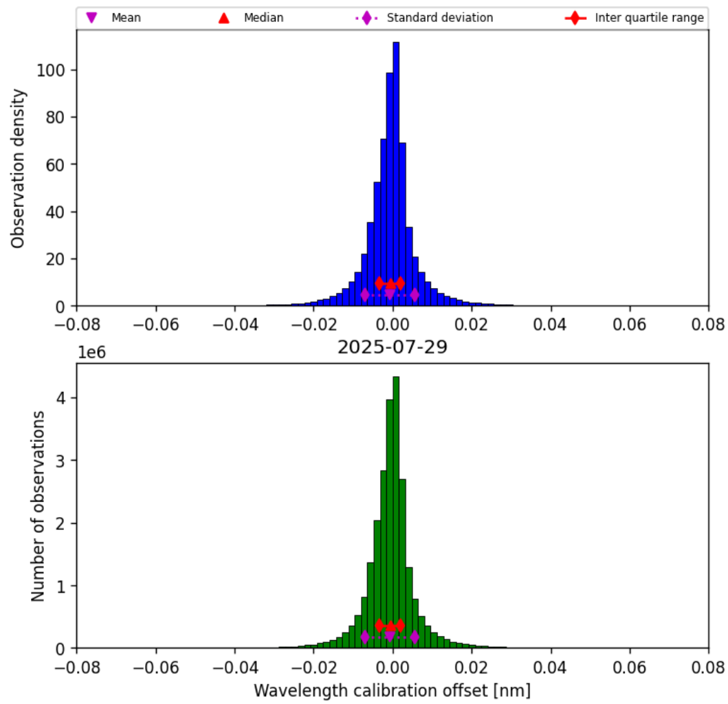
Figure 33: Histogram of “Wavelength calibration offset” for 2025-07-29 to 2025-07-30
