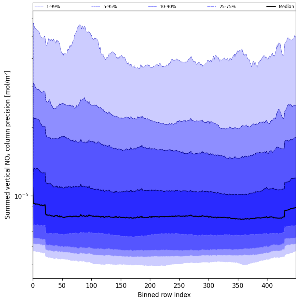
Figure 56: Along track statistics of “Summed vertical NO 2 column precision” for 2025-07-29 to 2025-07-30
