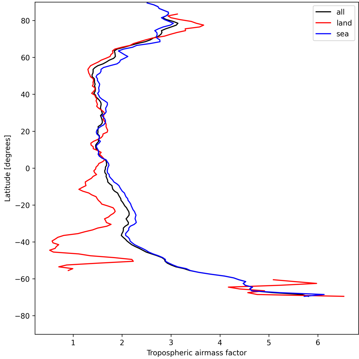
Figure 12: Zonal average of “Tropospheric air mass factor” for 2025-07-29 to 2025-07-30.
