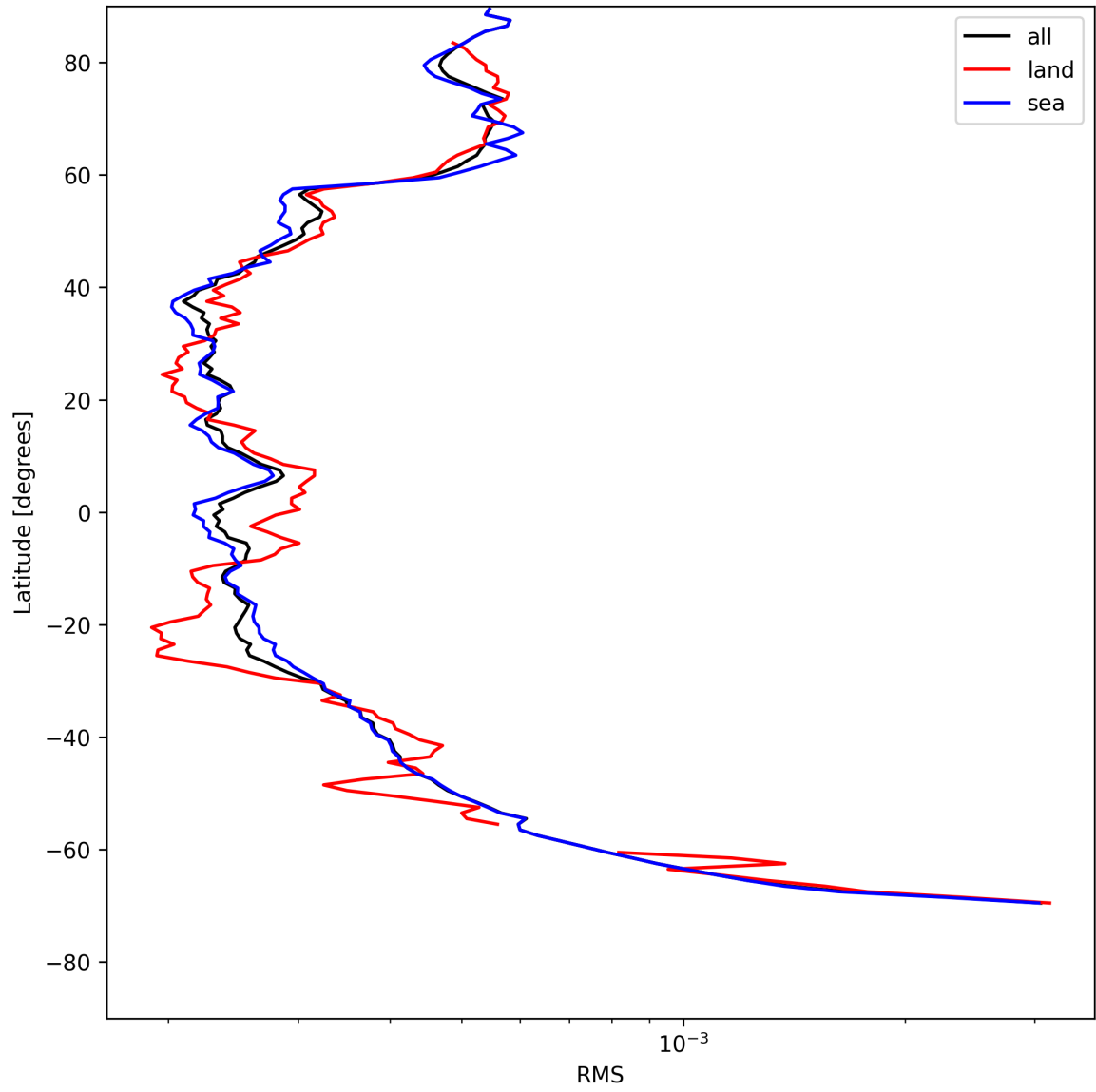
Figure 24: Zonal average of “RMS” for 2025-07-29 to 2025-07-30.
