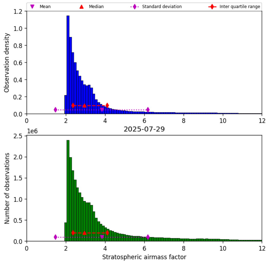
Figure 42: Histogram of “Stratospheric airmass factor” for 2025-07-29 to 2025-07-30
