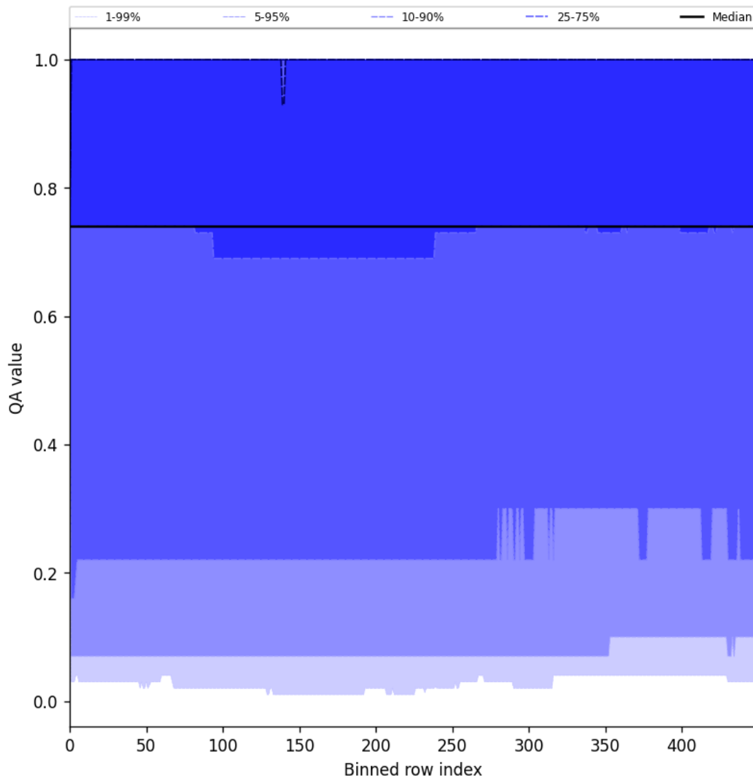
Figure 43: Along track statistics of “QA value” for 2025-07-29 to 2025-07-30
