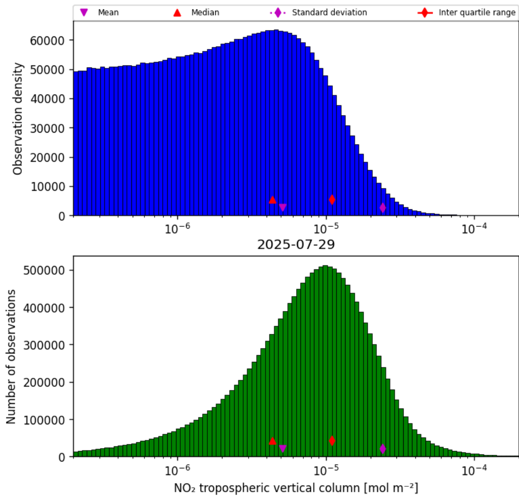
Figure 27: Histogram of “NO 2 tropospheric vertical column” for 2025-07-29 to 2025-07-30
