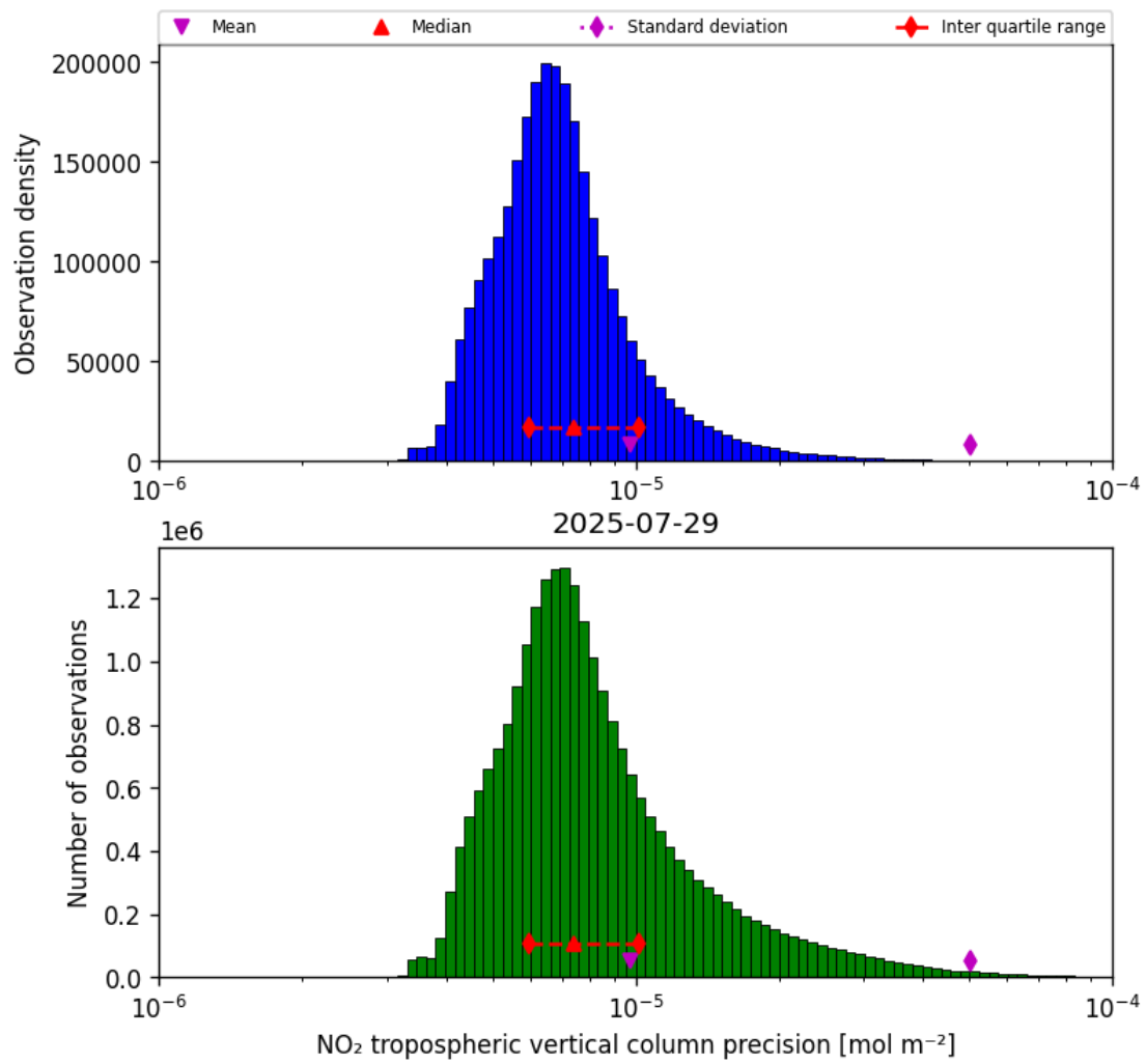
Figure 28: Histogram of “NO 2 tropospheric vertical column precision” for 2025-07-29 to 2025-07-30
