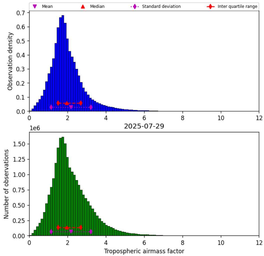
Figure 29: Histogram of “Tropospheric airmass factor” for 2025-07-29 to 2025-07-30
