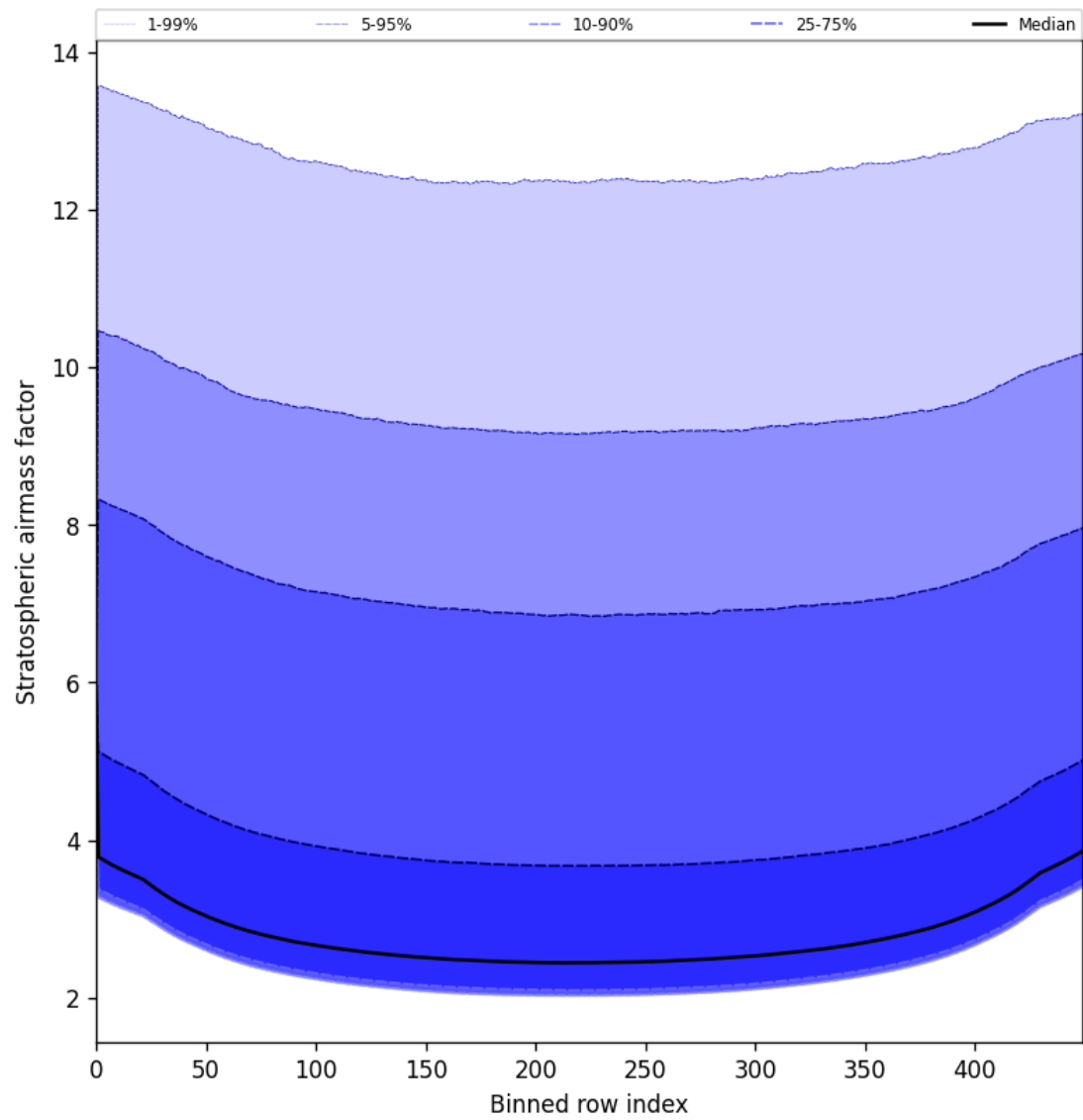
Figure 59: Along track statistics of “Stratospheric airmass factor” for 2025-07-29 to 2025-07-30
