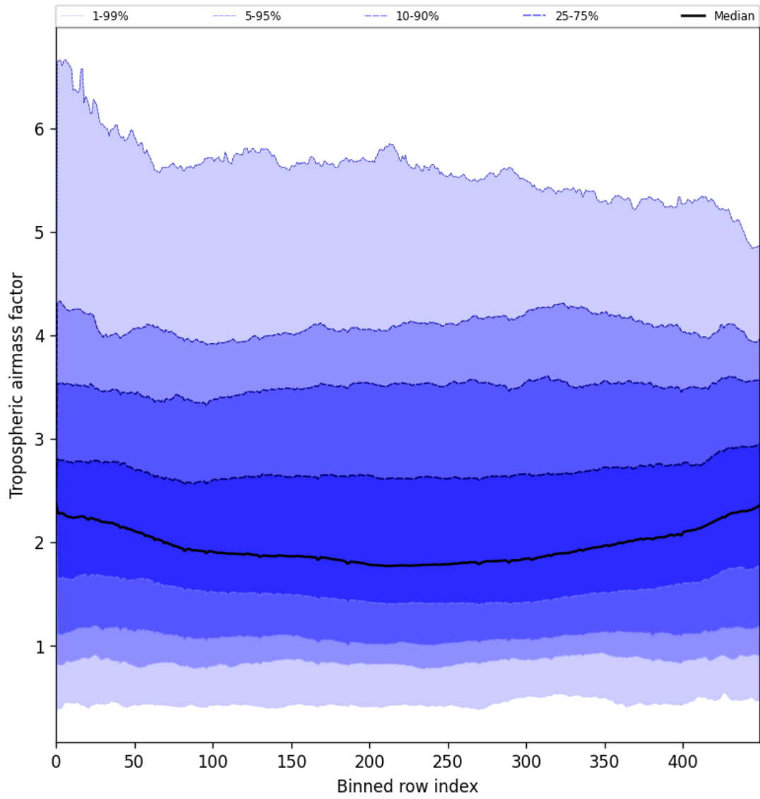
Figure 46: Along track statistics of “Tropospheric air mass factor” for 2025-07-29 to 2025-07-30
