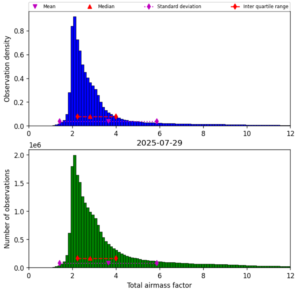
Figure 30: Histogram of “Total airmass factor” for 2025-07-29 to 2025-07-30
