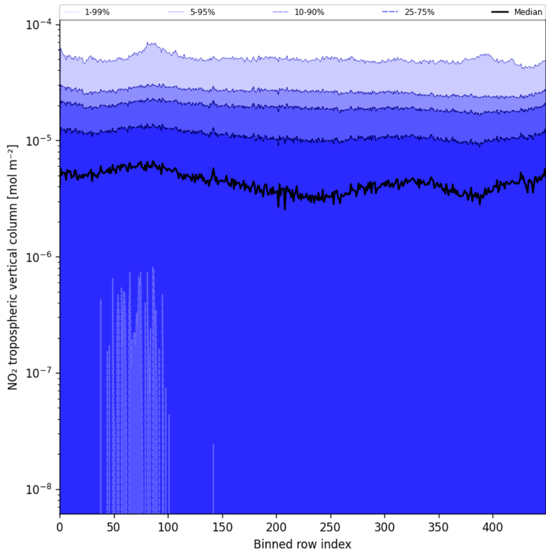
Figure 44: Along track statistics of “NO 2 tropospheric vertical column” for 2025-07-29 to 2025-07-30
