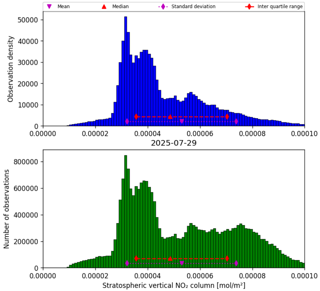
Figure 34: Histogram of “Stratospheric vertical NO 2 column” for 2025-07-29 to 2025-07-30
