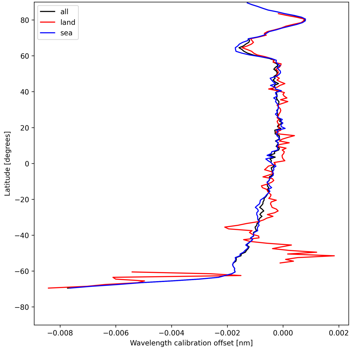
Figure 16: Zonal average of “Wavelength calibration offset” for 2025-07-29 to 2025-07-30.
