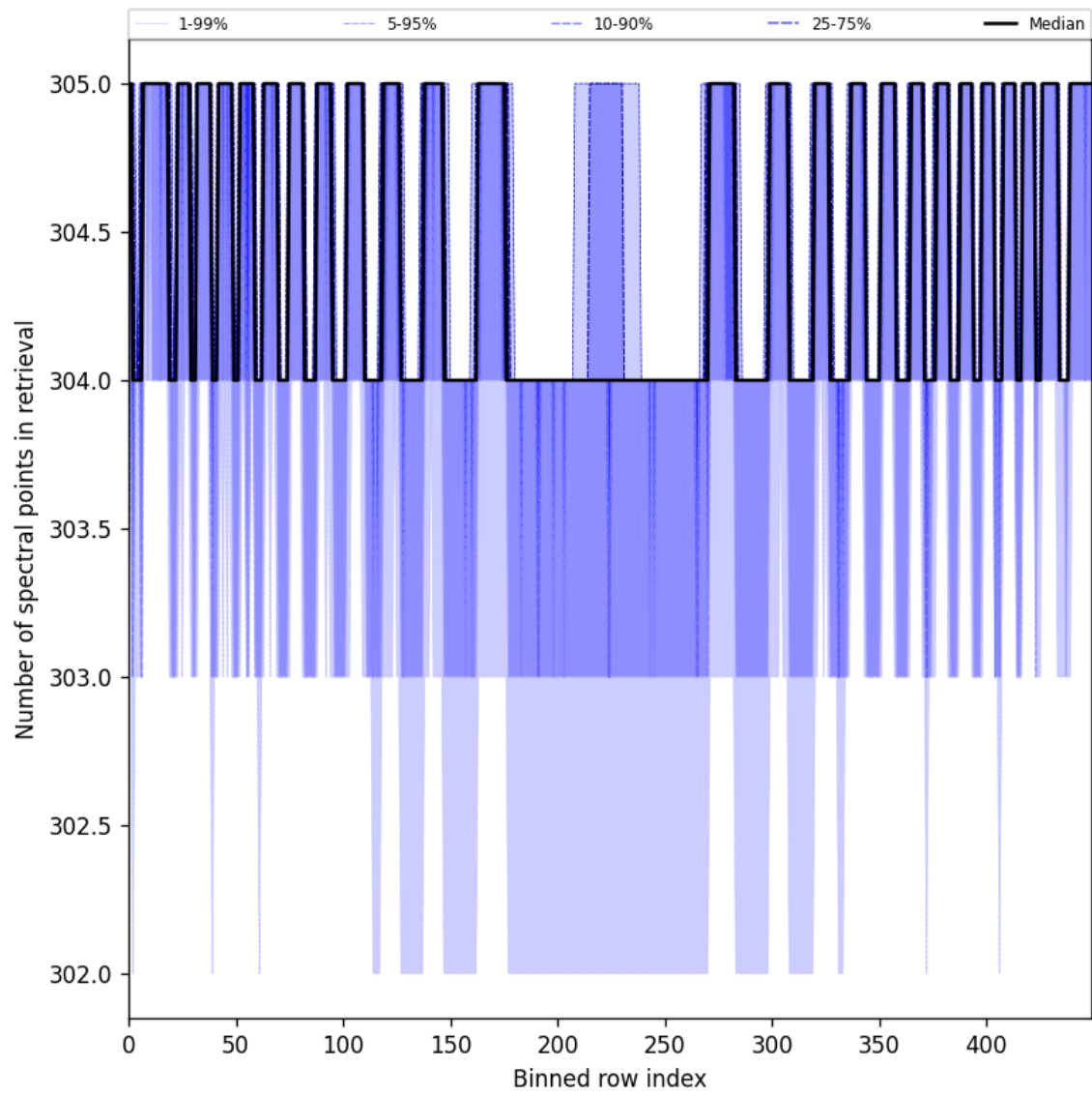
Figure 48: Along track statistics of “Number of spectral points in retrieval” for 2025-07-29 to 2025-07-30
