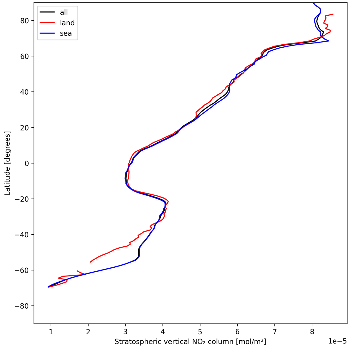
Figure 17: Zonal average of “Stratospheric vertical NO 2 column” for 2025-07-29 to 2025-07-30.
