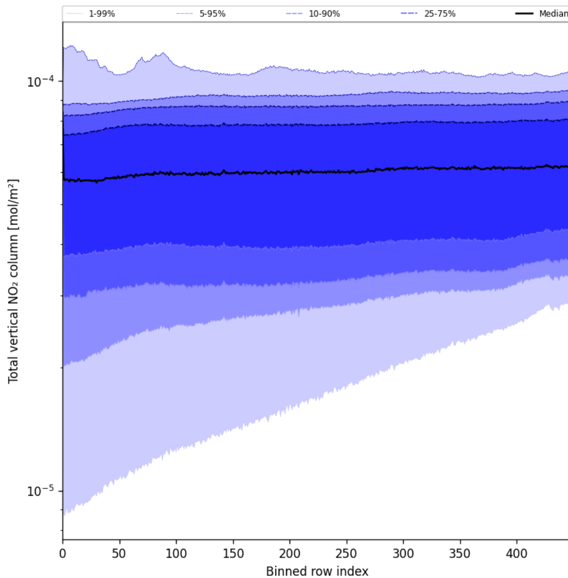
Figure 53: Along track statistics of “Total vertical NO 2 column” for 2025-07-29 to 2025-07-30
