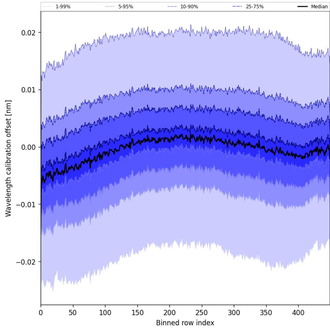
Figure 50: Along track statistics of “Wavelength calibration offset” for 2025-07-29 to 2025-07-30
