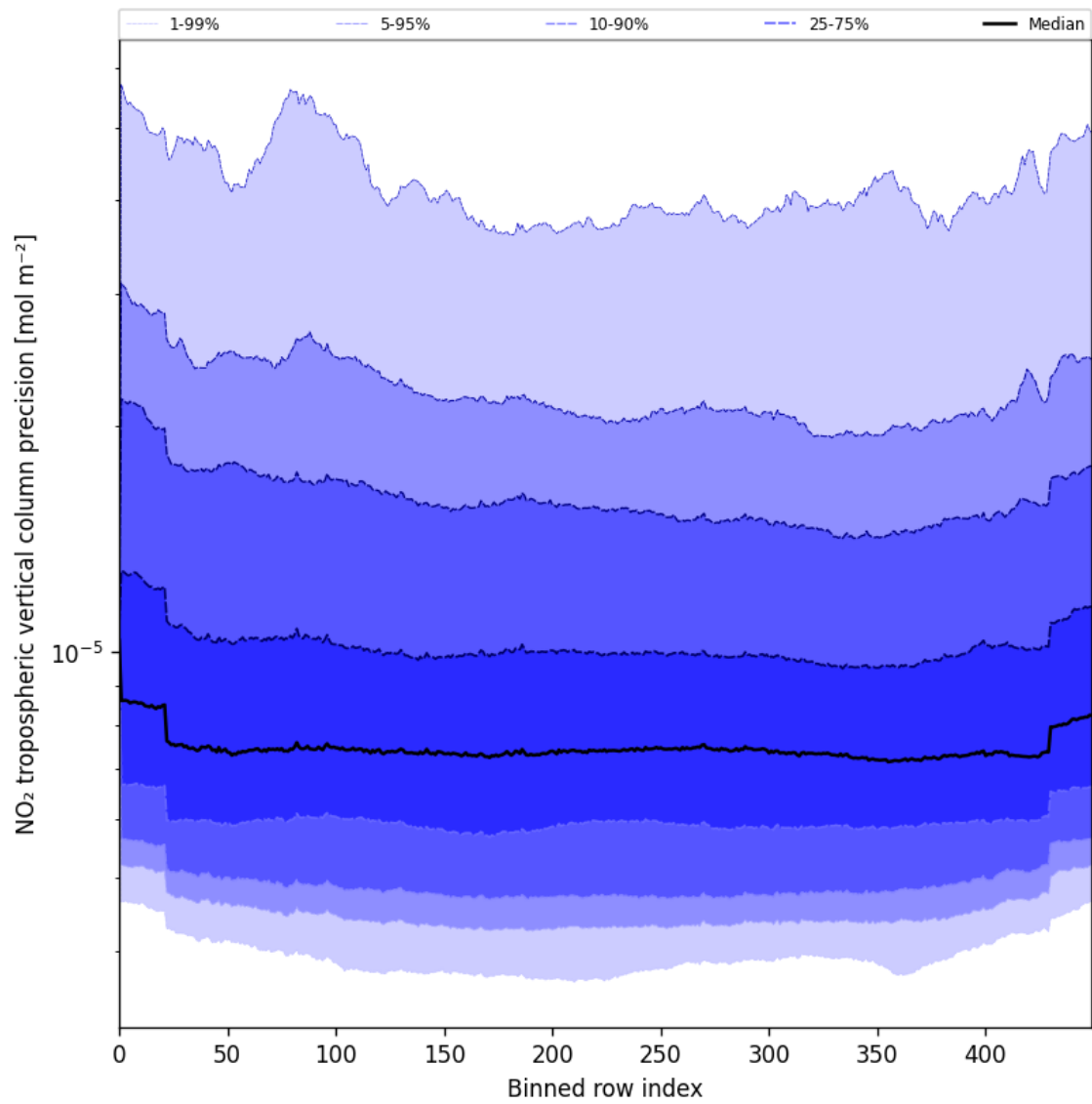
Figure 45: Along track statistics of “NO 2 tropospheric vertical column precision” for 2025-07-29 to 2025-07-30
