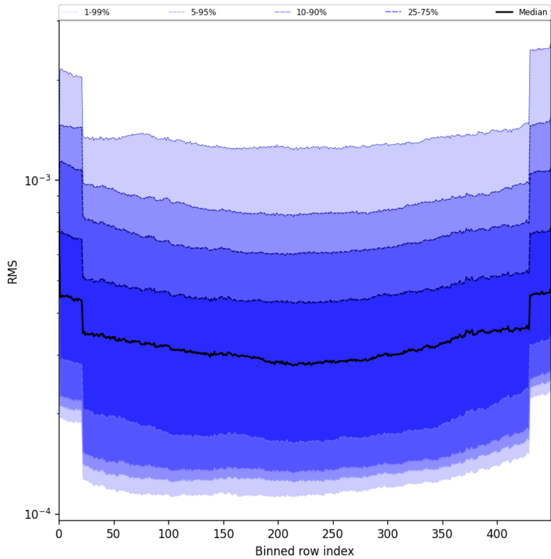
Figure 58: Along track statistics of “RMS” for 2025-07-29 to 2025-07-30
