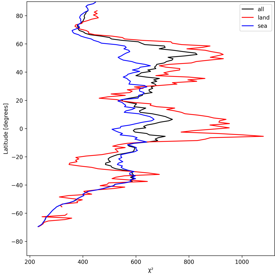
Figure 23: Zonal average of “ \chi^2 ” for 2025-07-29 to 2025-07-30.
