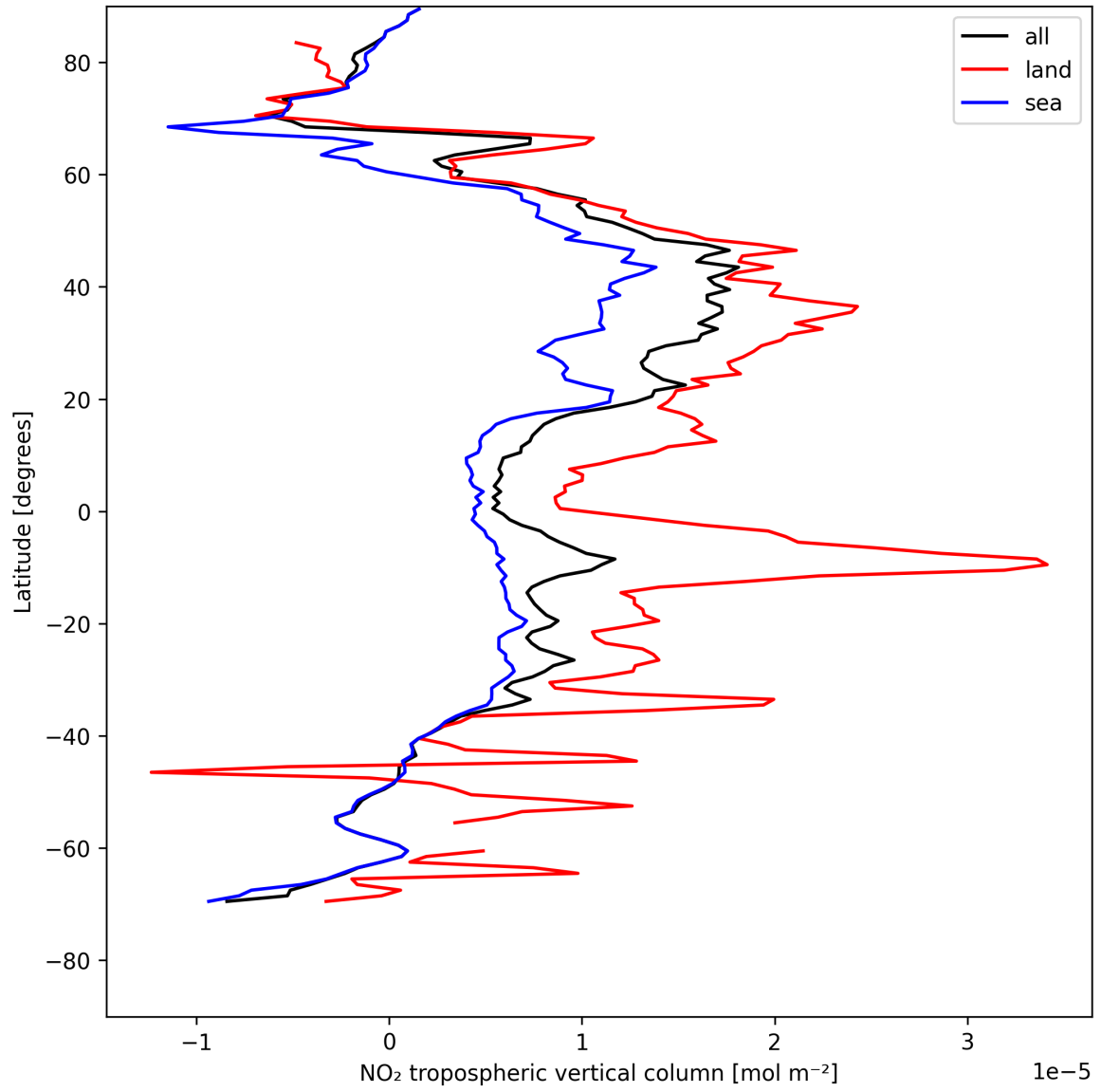
Figure 10: Zonal average of “NO 2 tropospheric vertical column” for 2025-07-29 to 2025-07-30.
