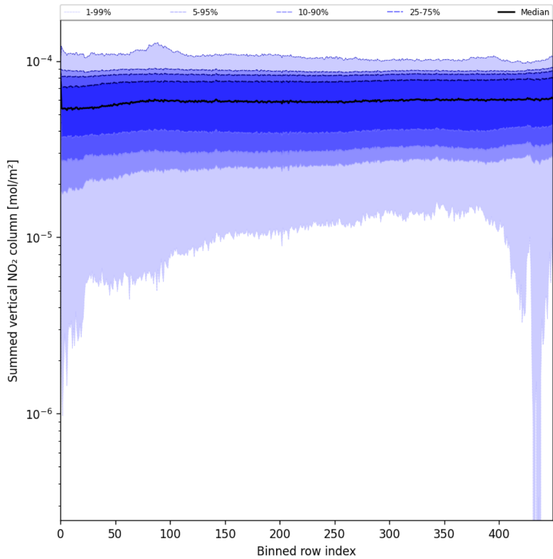
Figure 55: Along track statistics of “Summed vertical NO 2 column” for 2025-07-29 to 2025-07-30
