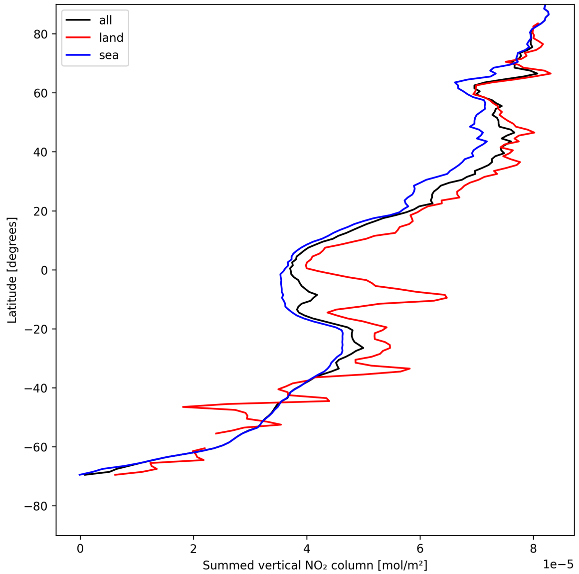
Figure 21: Zonal average of “Summed vertical NO 2 column” for 2025-07-29 to 2025-07-30.
