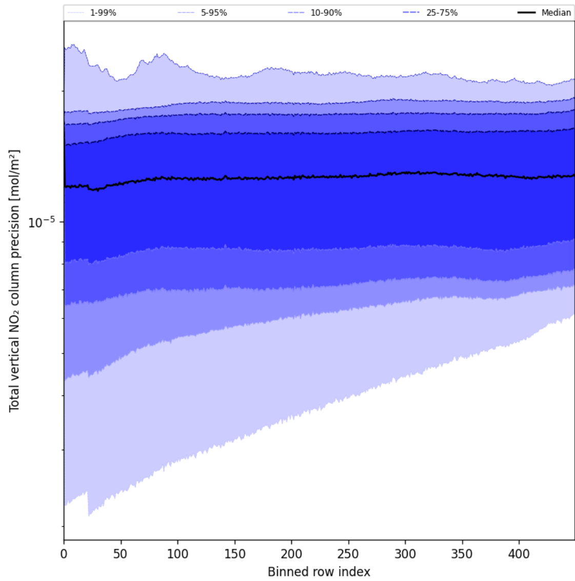
Figure 54: Along track statistics of “Total vertical NO 2 column precision” for 2025-07-29 to 2025-07-30
