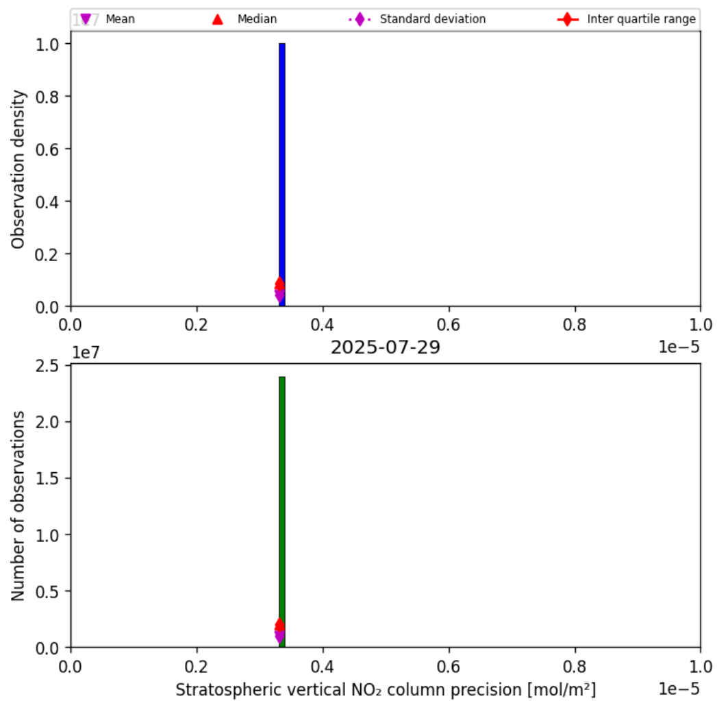
Figure 35: Histogram of “Stratospheric vertical NO 2 column precision” for 2025-07-29 to 2025-07-30
