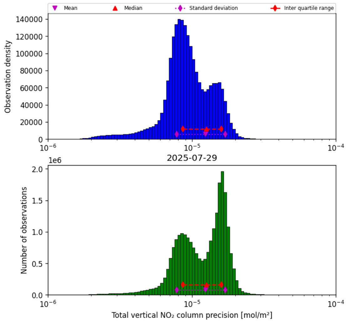
Figure 37: Histogram of “Total vertical NO 2 column precision” for 2025-07-29 to 2025-07-30
