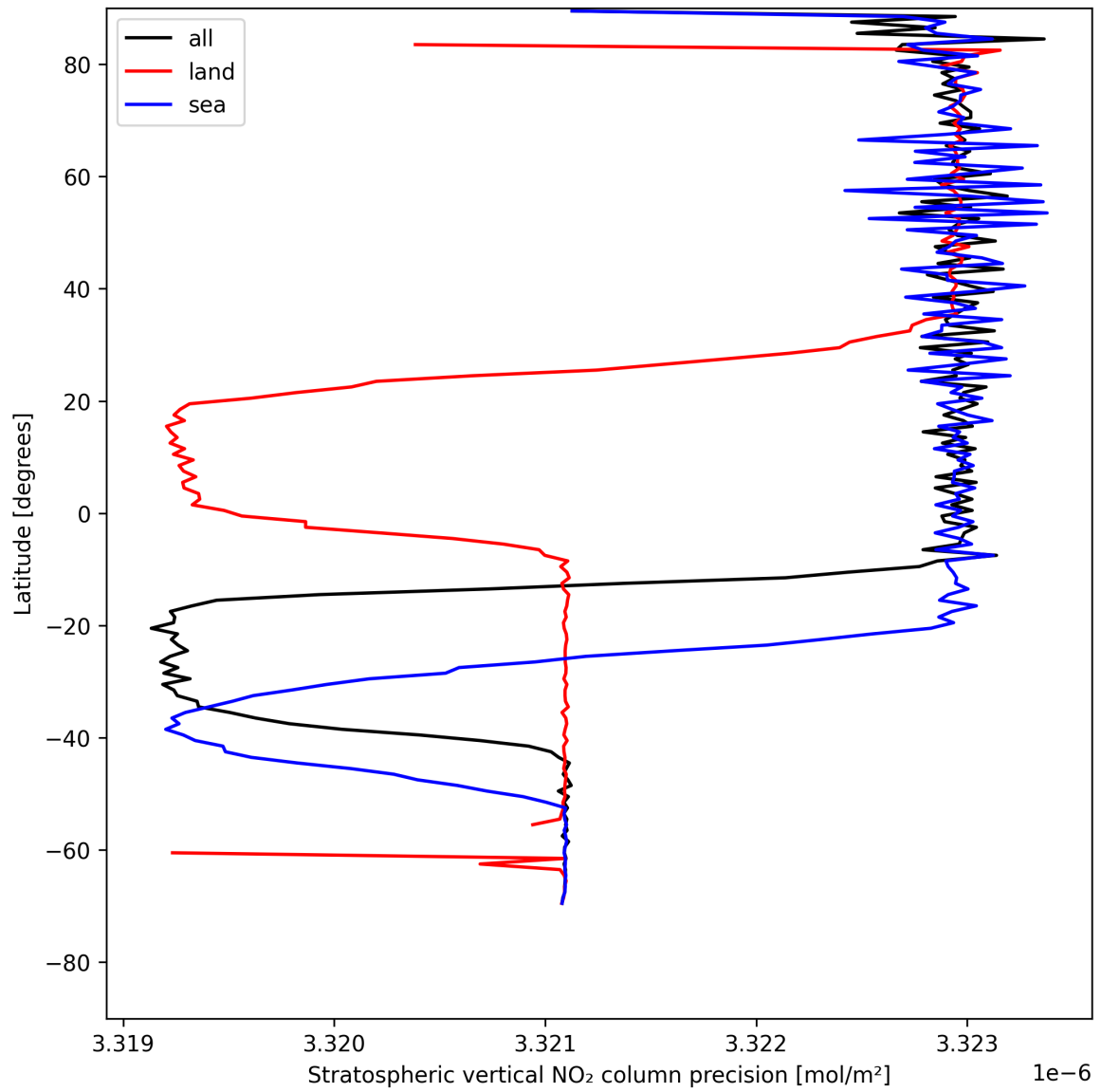
Figure 18: Zonal average of “Stratospheric vertical NO 2 column precision” for 2025-07-29 to 2025-07-30.
