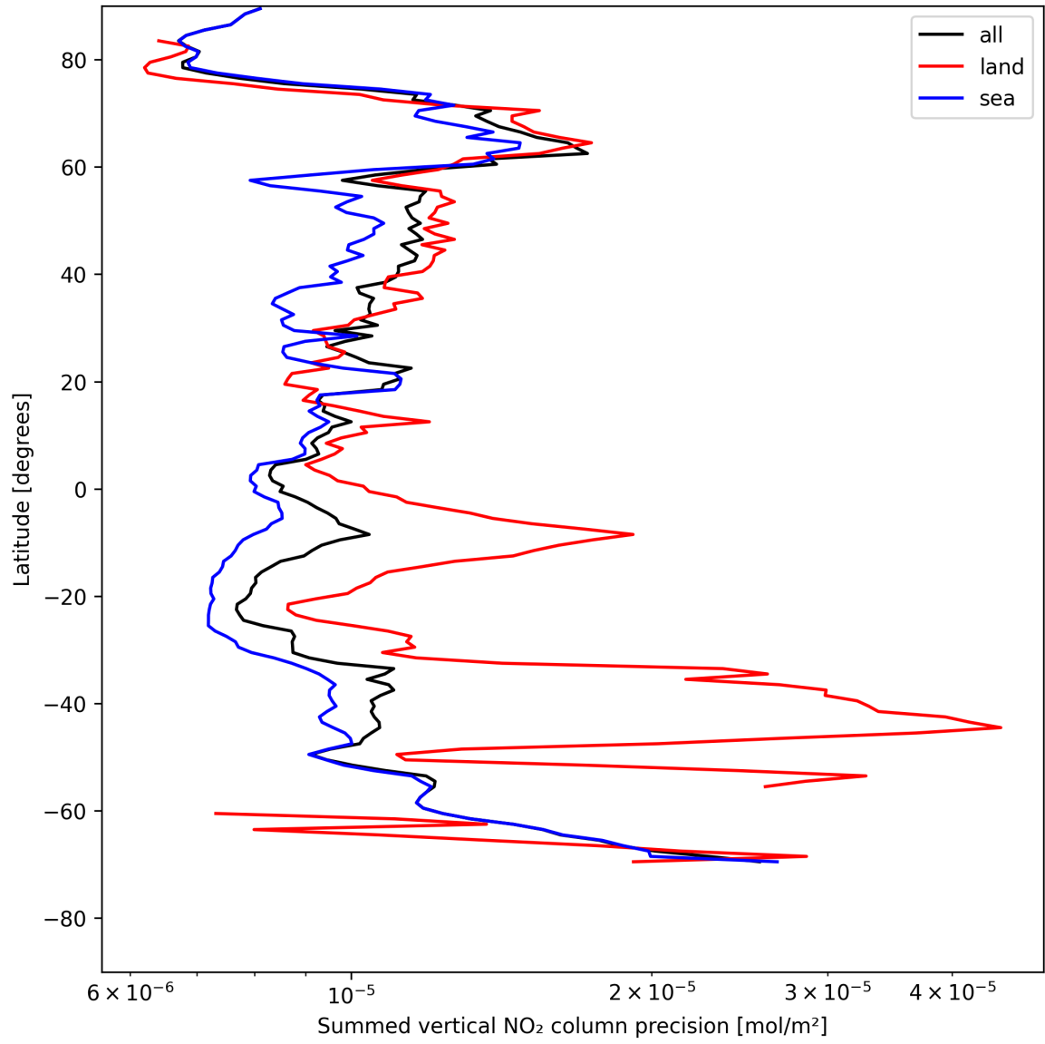
Figure 22: Zonal average of “Summed vertical NO 2 column precision” for 2025-07-29 to 2025-07-30.
