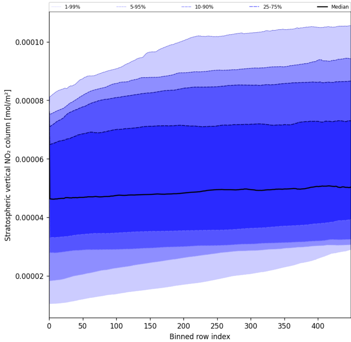
Figure 51: Along track statistics of “Stratospheric vertical NO 2 column” for 2025-07-29 to 2025-07-30
