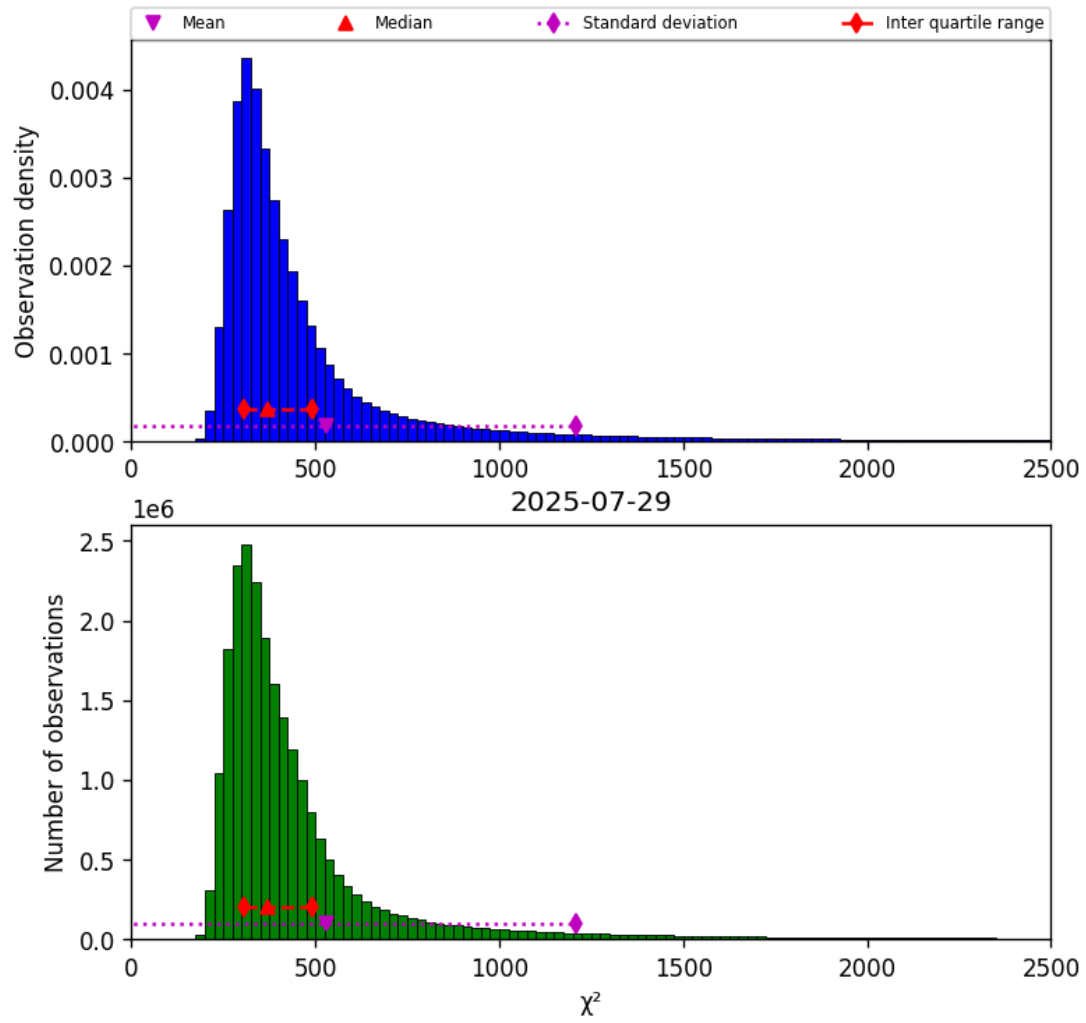
Figure 40: Histogram of “ \chi^2 ” for 2025-07-29 to 2025-07-30
