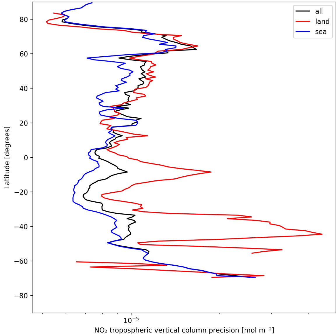
Figure 11: Zonal average of “NO 2 tropospheric vertical column precision” for 2025-07-29 to 2025-07-30.
