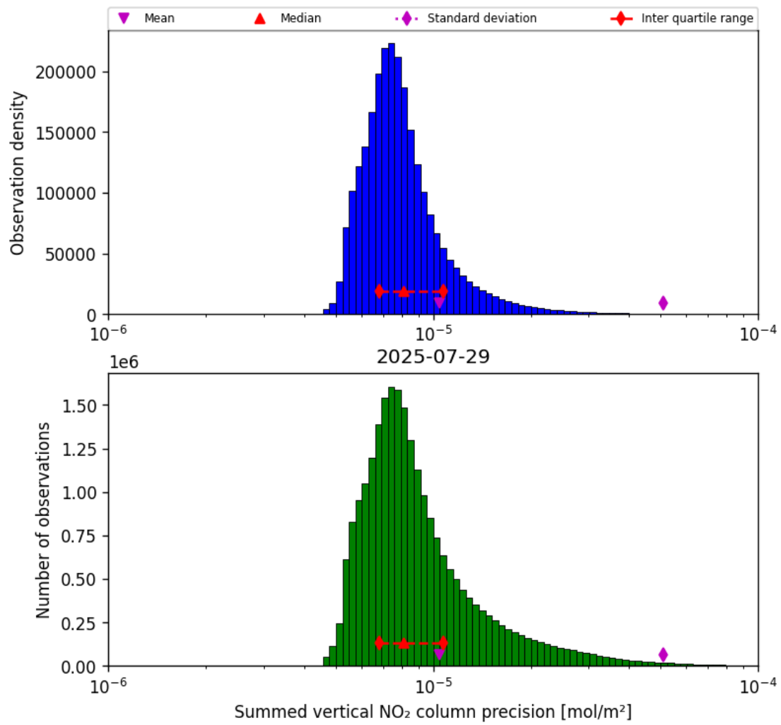
Figure 39: Histogram of “Summed vertical NO 2 column precision” for 2025-07-29 to 2025-07-30
