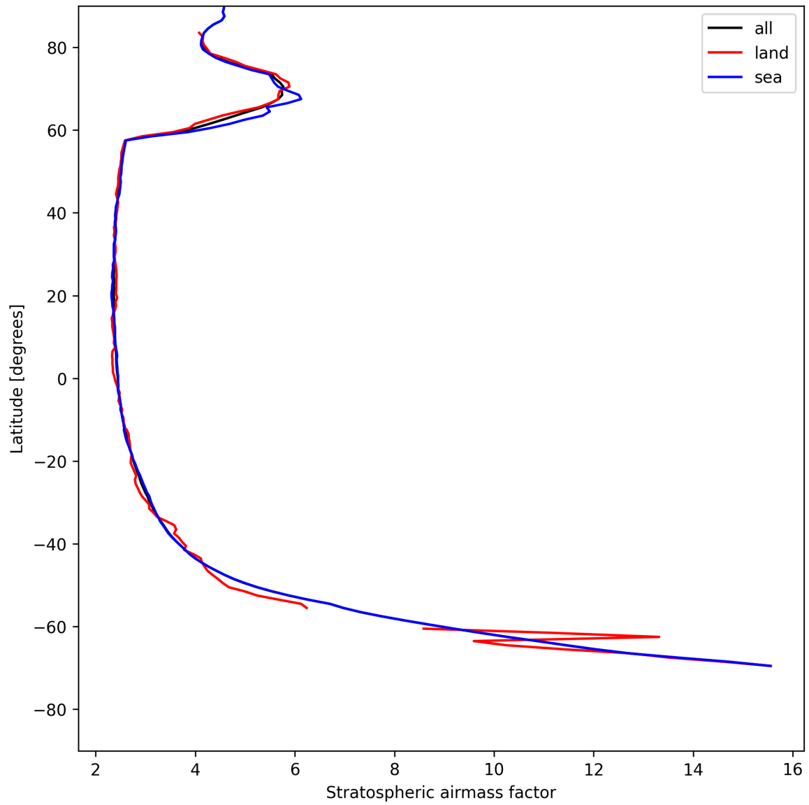
Figure 25: Zonal average of “Stratospheric airmass factor” for 2025-07-29 to 2025-07-30.
