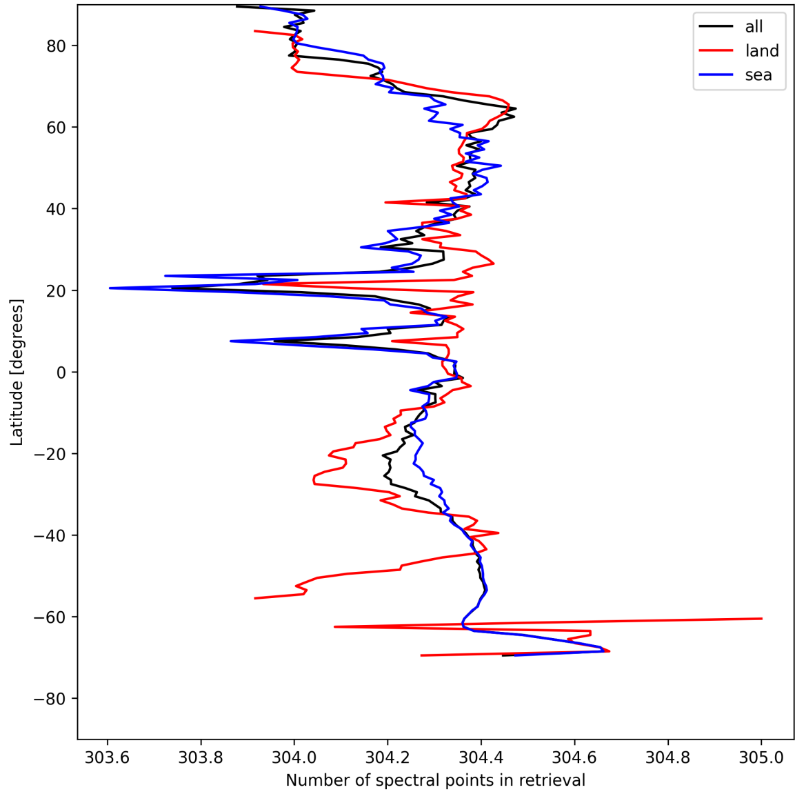
Figure 14: Zonal average of “Number of spectral points in retrieval” for 2025-07-29 to 2025-07-30.
