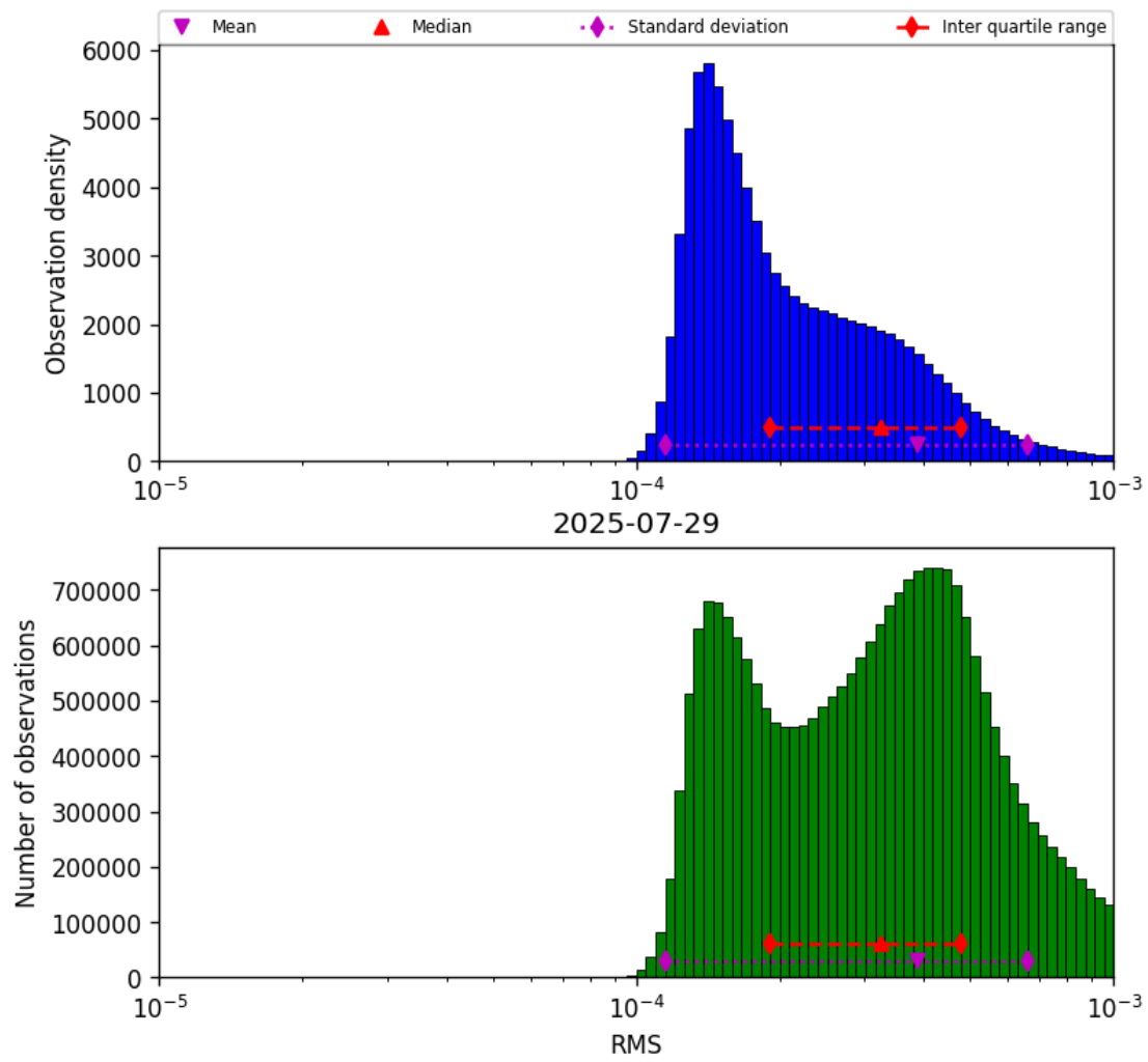
Figure 41: Histogram of “RMS” for 2025-07-29 to 2025-07-30
