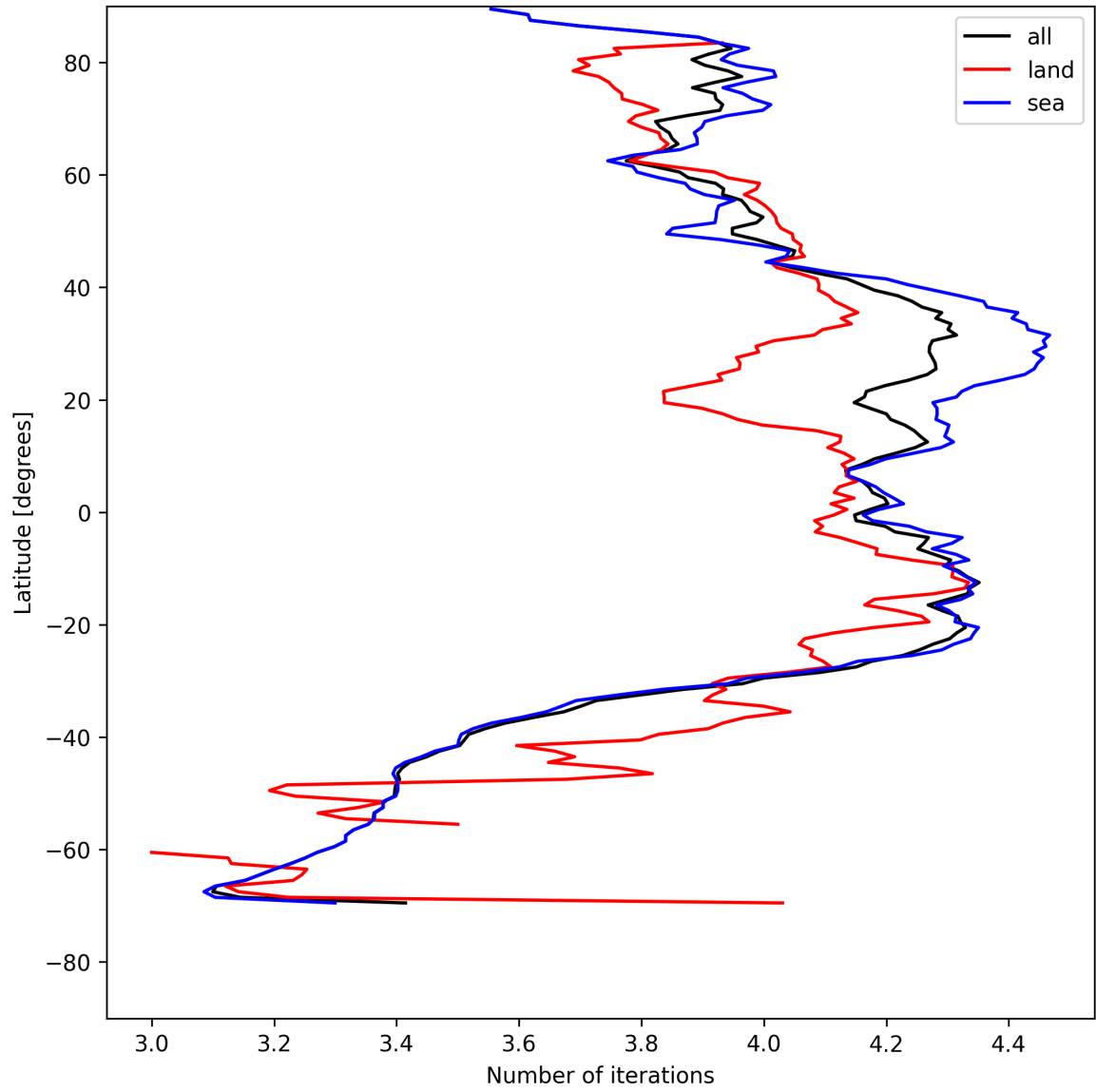
Figure 15: Zonal average of “Number of iterations” for 2025-07-29 to 2025-07-30.
