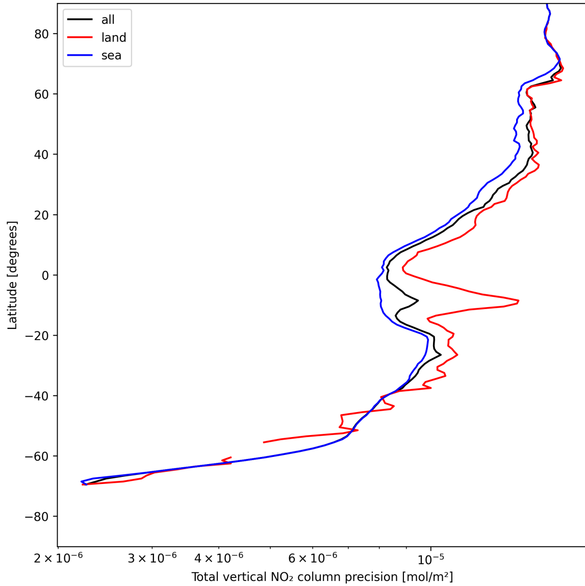
Figure 20: Zonal average of “Total vertical NO 2 column precision” for 2025-07-29 to 2025-07-30.
