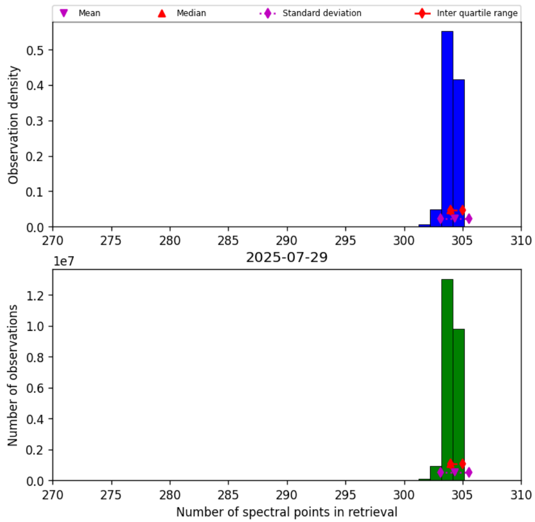
Figure 31: Histogram of “Number of spectral points in retrieval” for 2025-07-29 to 2025-07-30
