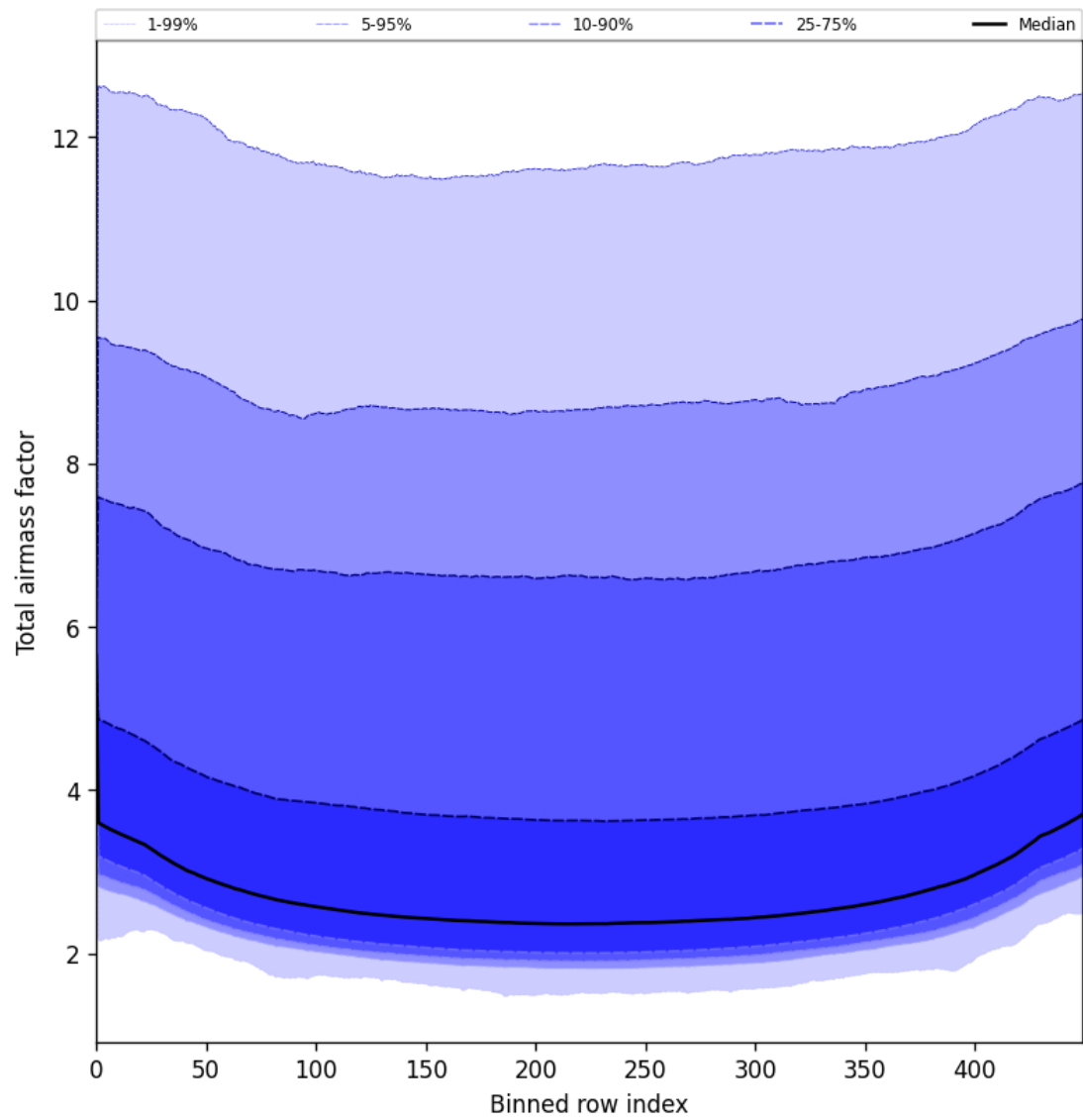
Figure 47: Along track statistics of “Total airmass factor” for 2025-07-29 to 2025-07-30
