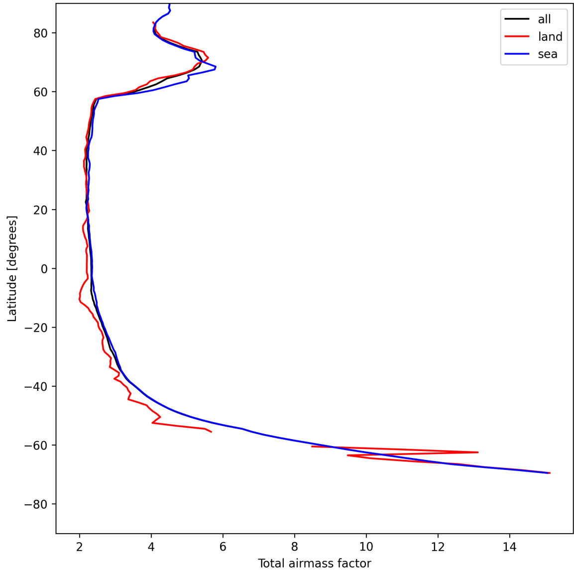
Figure 13: Zonal average of “Total airmass factor” for 2025-07-29 to 2025-07-30.
