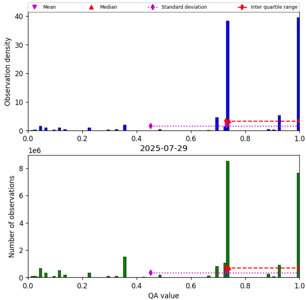
Figure 26: Histogram of “QA value” for 2025-07-29 to 2025-07-30
