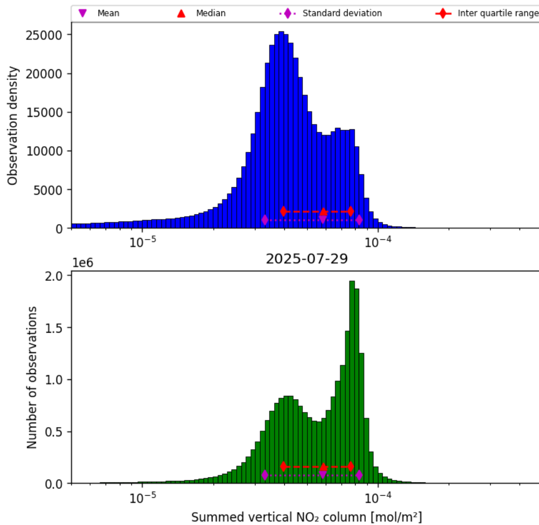
Figure 38: Histogram of “Summed vertical NO 2 column” for 2025-07-29 to 2025-07-30
