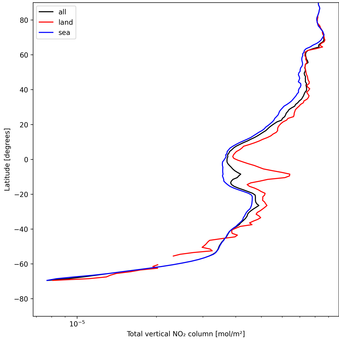
Figure 19: Zonal average of “Total vertical NO 2 column” for 2025-07-29 to 2025-07-30.
