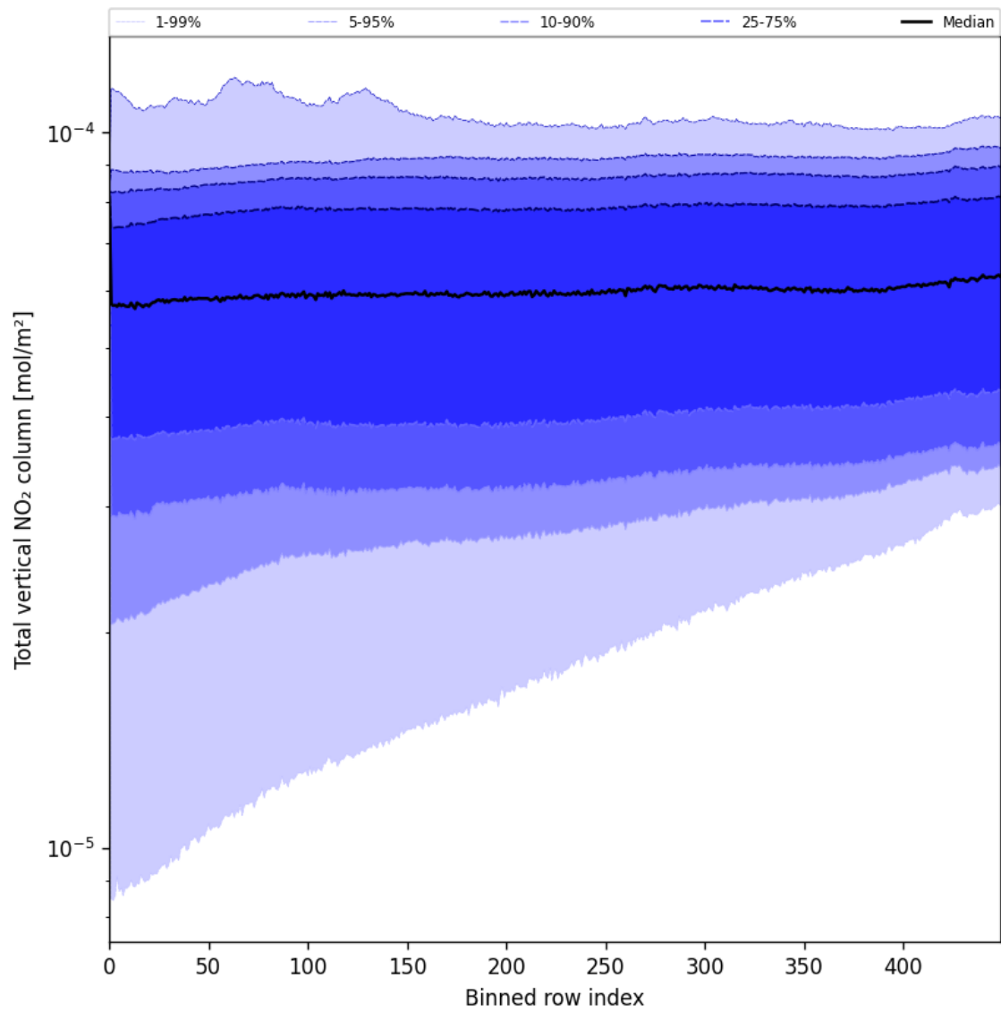
Figure 53: Along track statistics of “Total vertical NO 2 column” for 2025-07-30 to 2025-07-31
