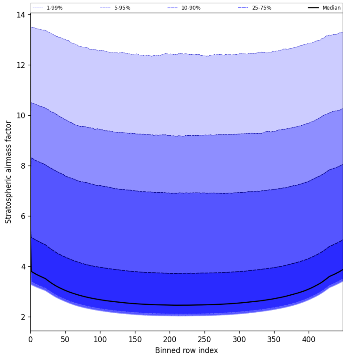
Figure 59: Along track statistics of “Stratospheric airmass factor” for 2025-07-30 to 2025-07-31
