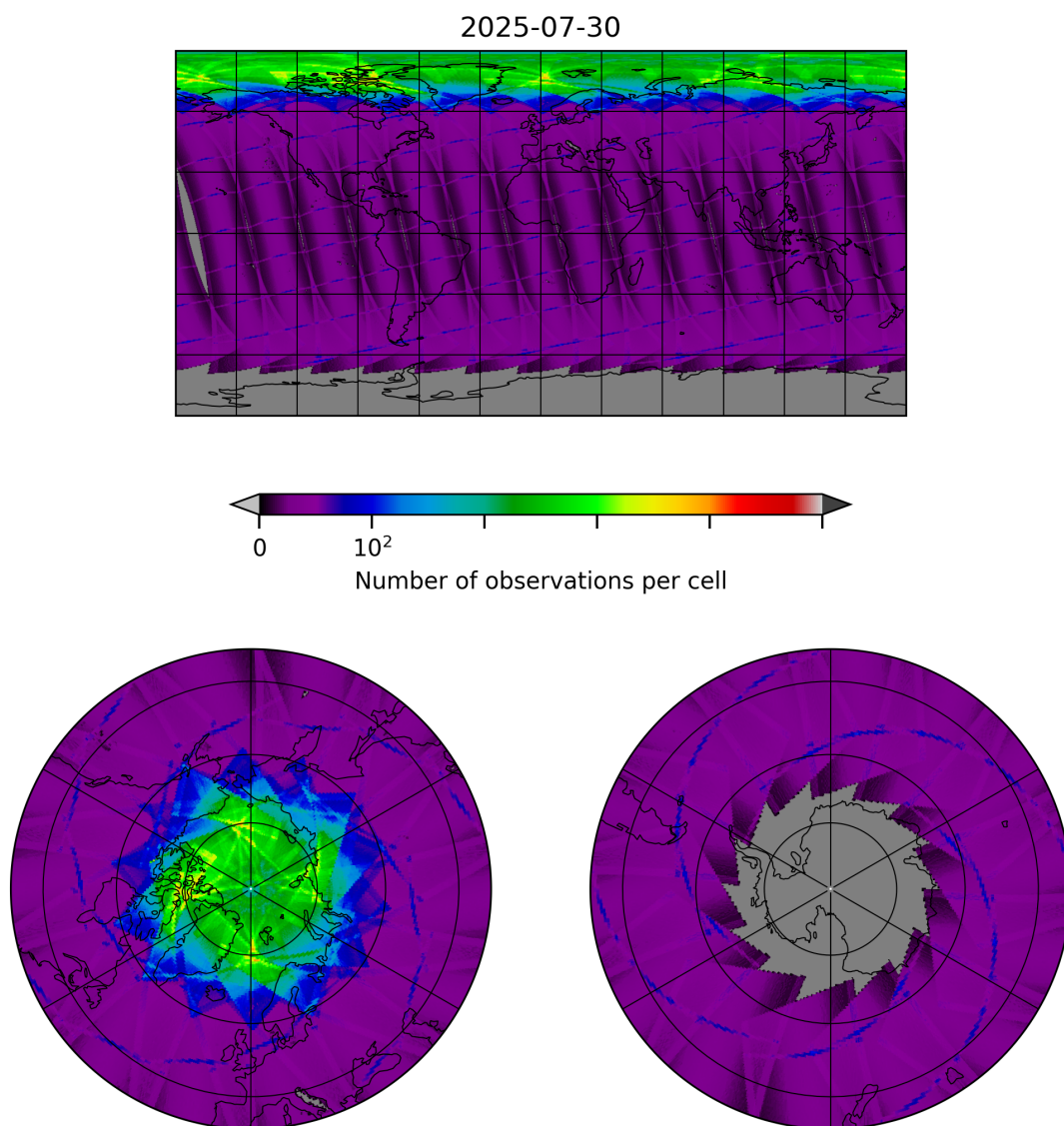
Figure 8: Map of the number of observations for 2025-07-30 to 2025-07-31
