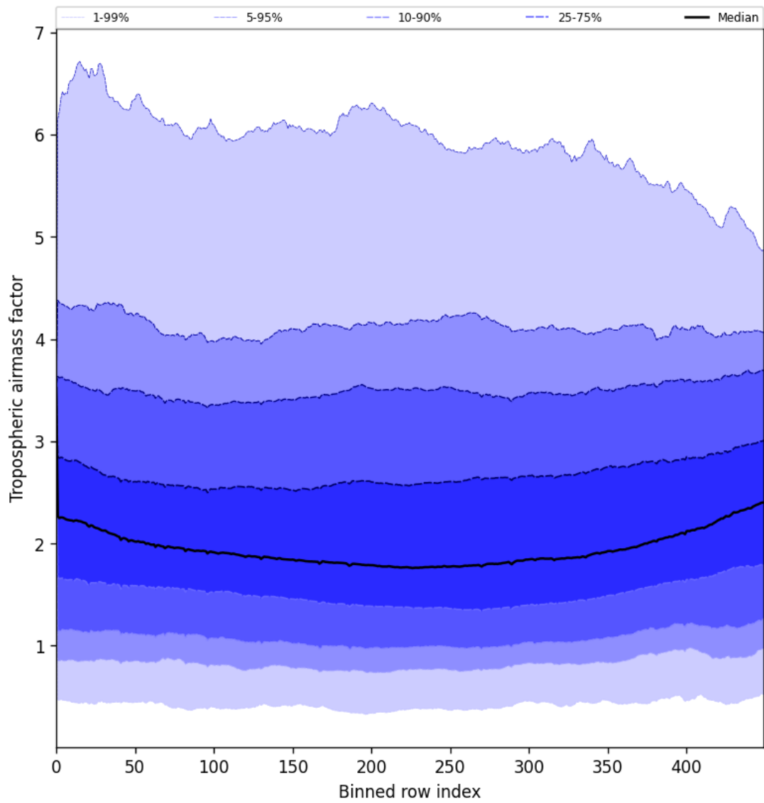
Figure 46: Along track statistics of “Tropospheric airmass factor” for 2025-07-30 to 2025-07-31
