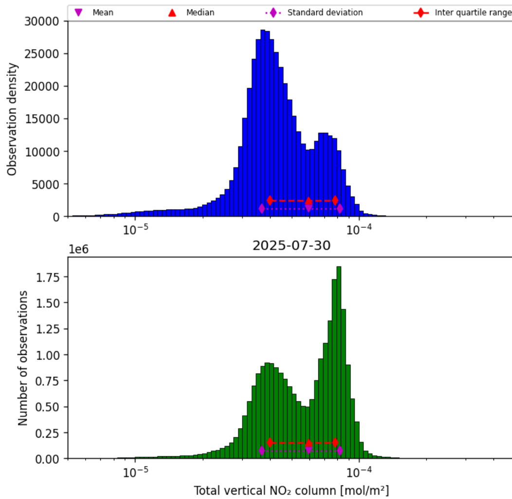
Figure 36: Histogram of “Total vertical NO 2 column” for 2025-07-30 to 2025-07-31
