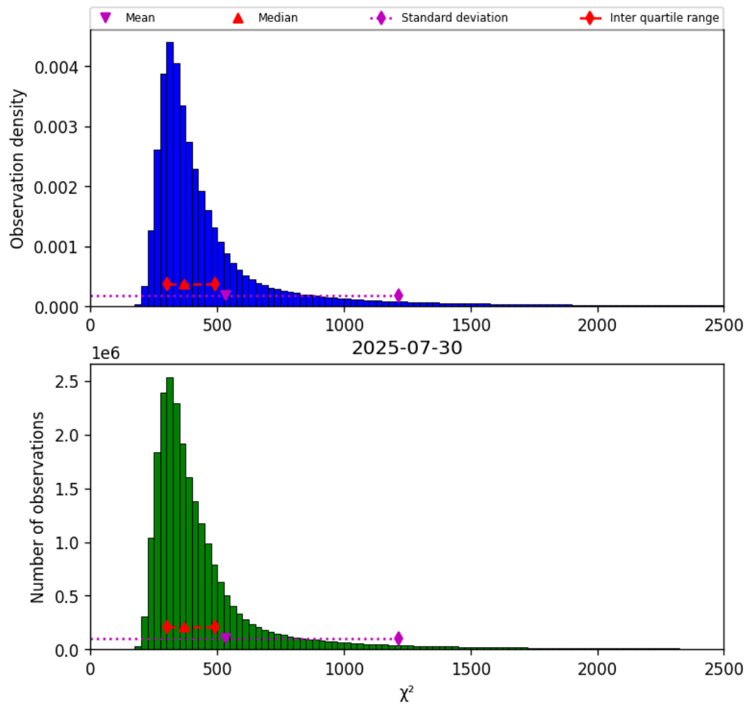
Figure 40: Histogram of “ \chi^2 ” for 2025-07-30 to 2025-07-31
