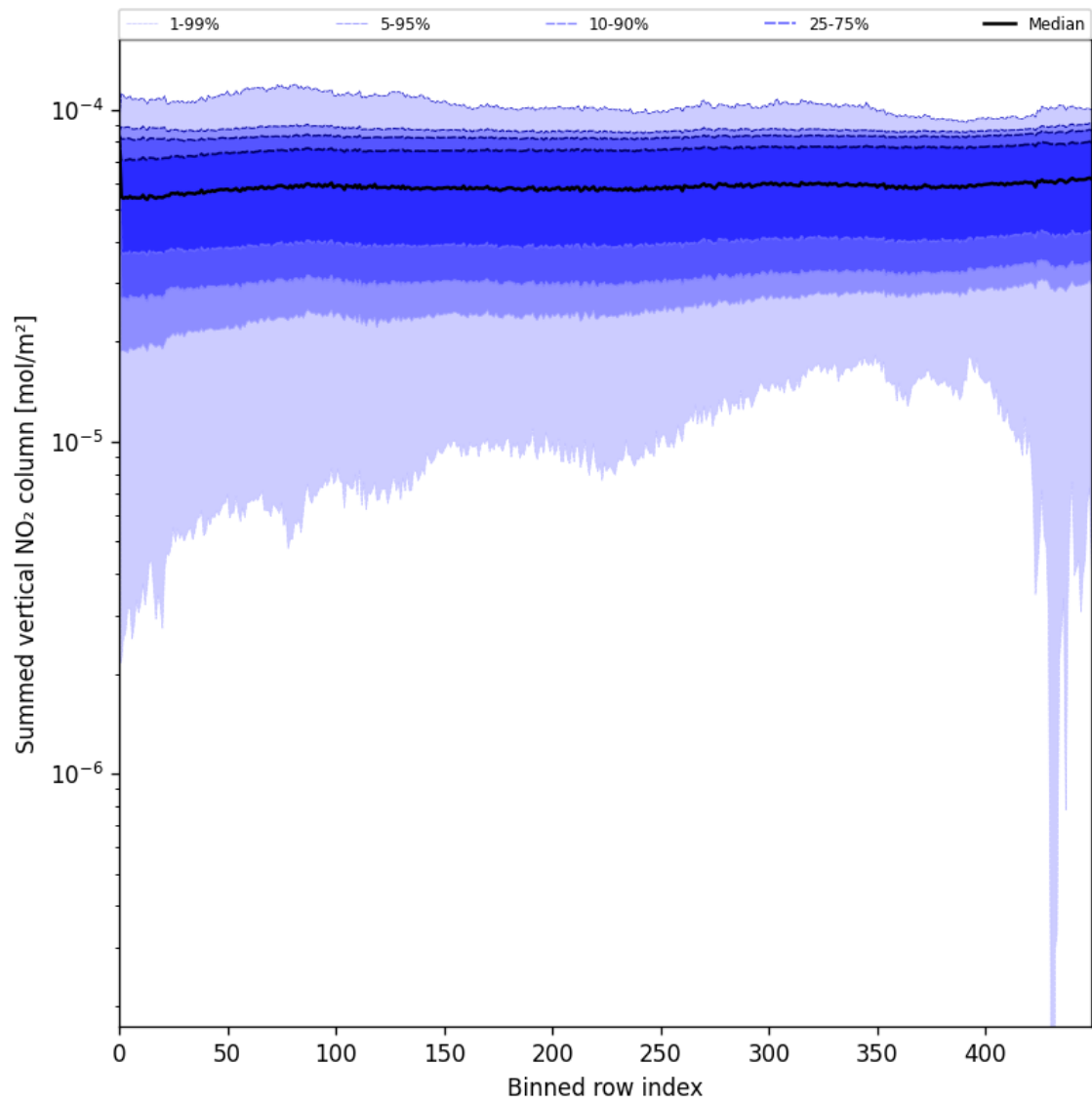
Figure 55: Along track statistics of “Summed vertical NO 2 column” for 2025-07-30 to 2025-07-31
