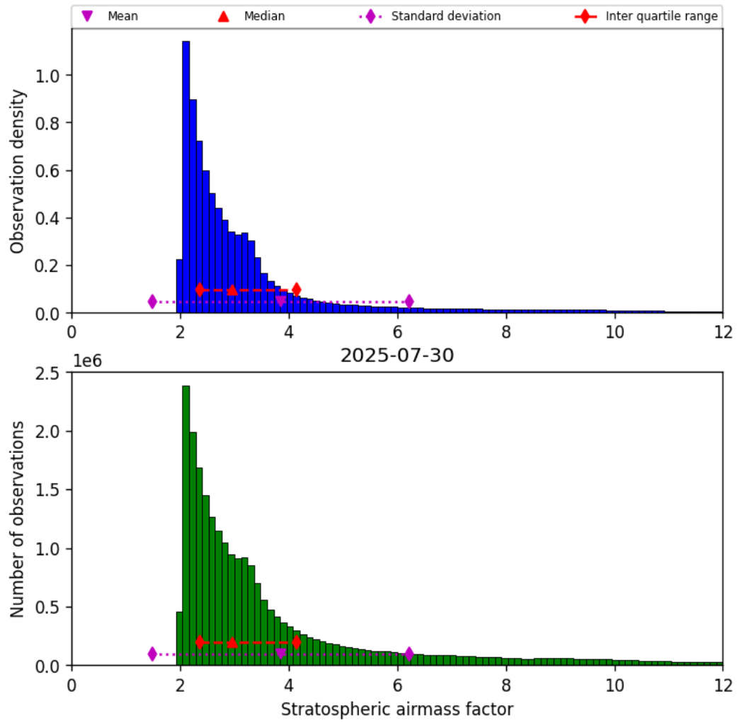
Figure 42: Histogram of “Stratospheric airmass factor” for 2025-07-30 to 2025-07-31
