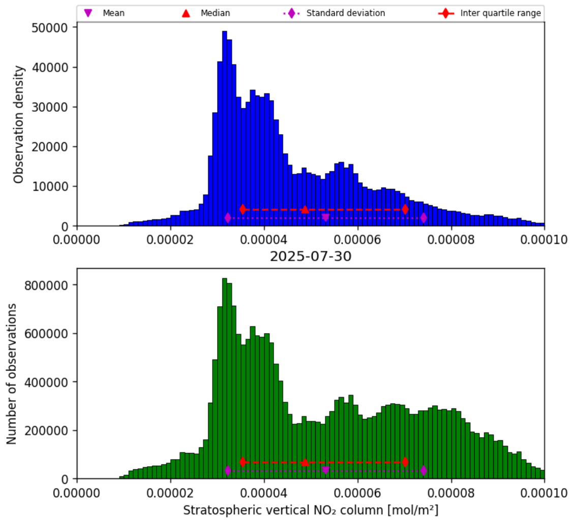
Figure 34: Histogram of “Stratospheric vertical NO 2 column” for 2025-07-30 to 2025-07-31
