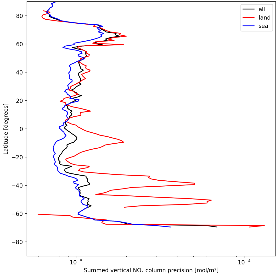
Figure 22: Zonal average of “Summed vertical NO 2 column precision” for 2025-07-30 to 2025-07-31.
