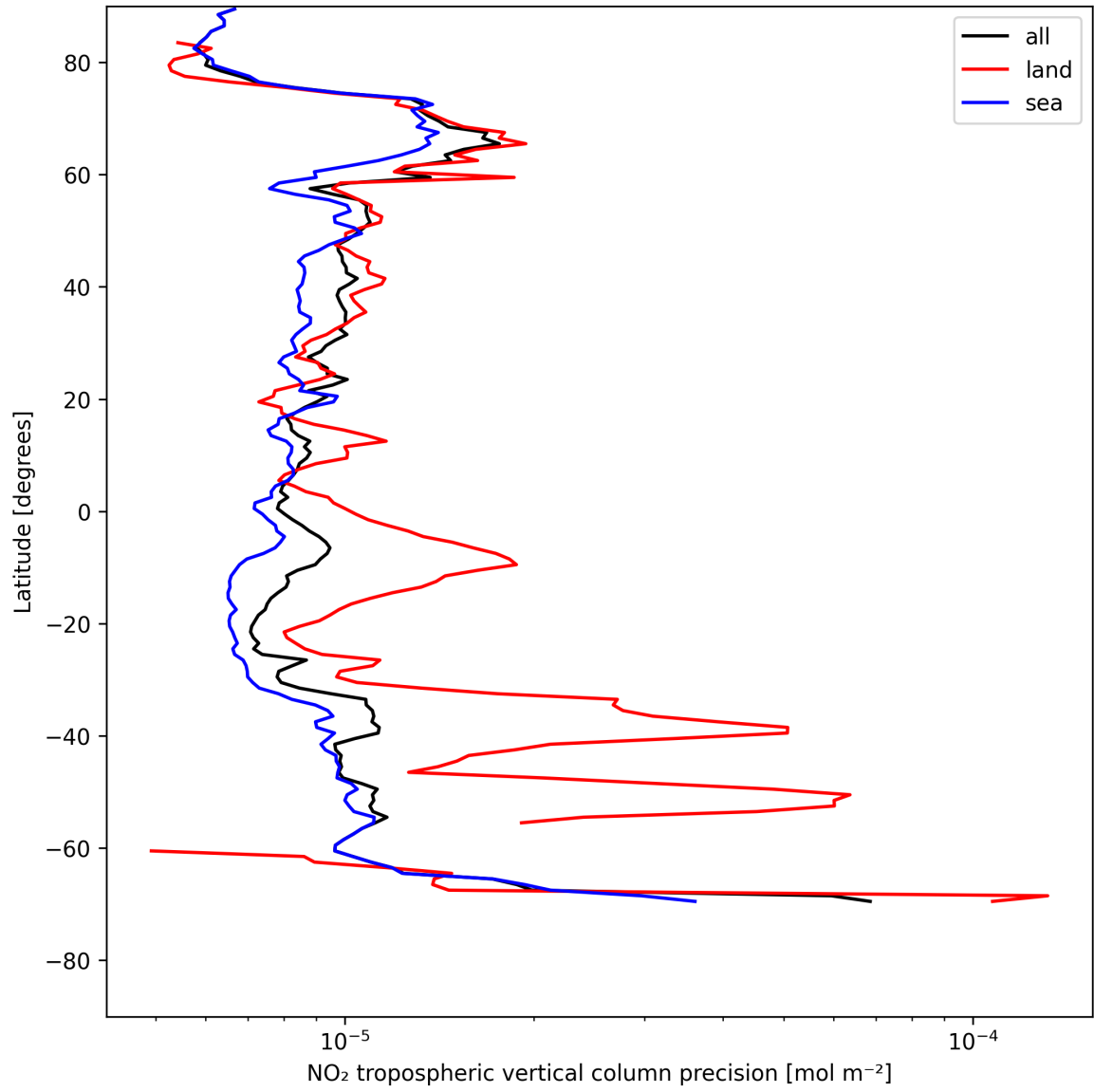
Figure 11: Zonal average of “NO 2 tropospheric vertical column precision” for 2025-07-30 to 2025-07-31.
