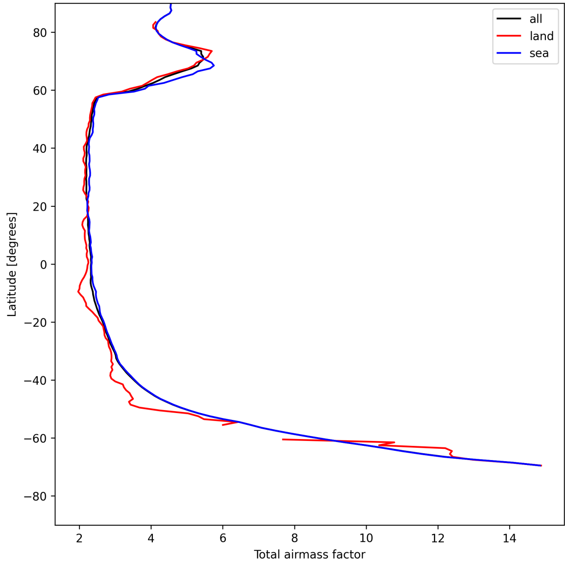
Figure 13: Zonal average of “Total airmass factor” for 2025-07-30 to 2025-07-31.
