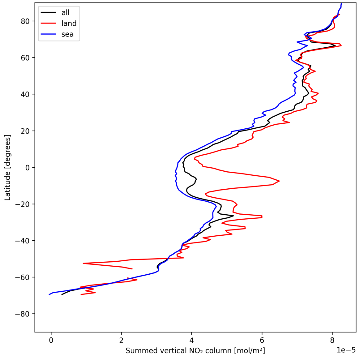
Figure 21: Zonal average of “Summed vertical NO 2 column” for 2025-07-30 to 2025-07-31.
