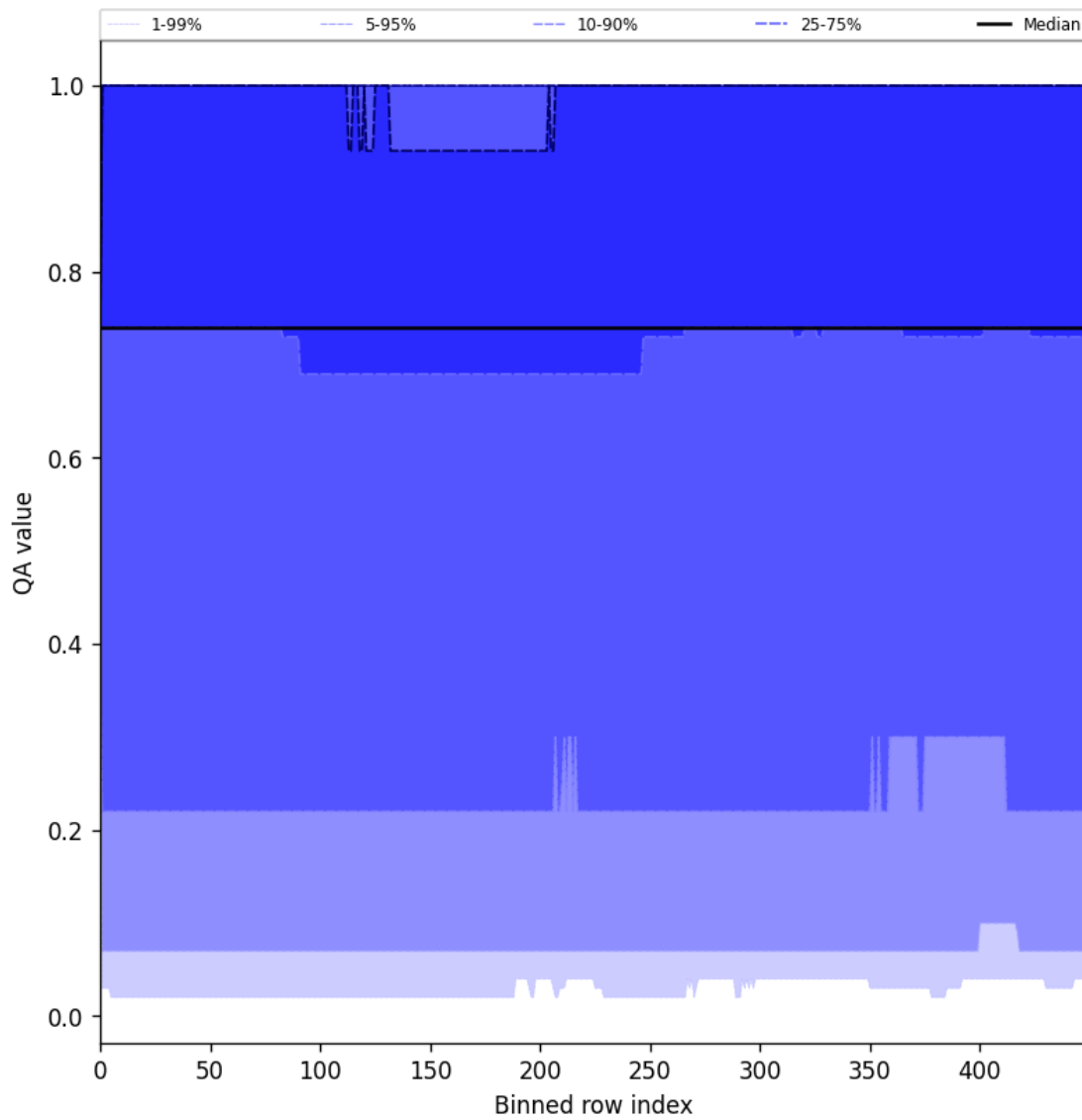
Figure 43: Along track statistics of “QA value” for 2025-07-30 to 2025-07-31
