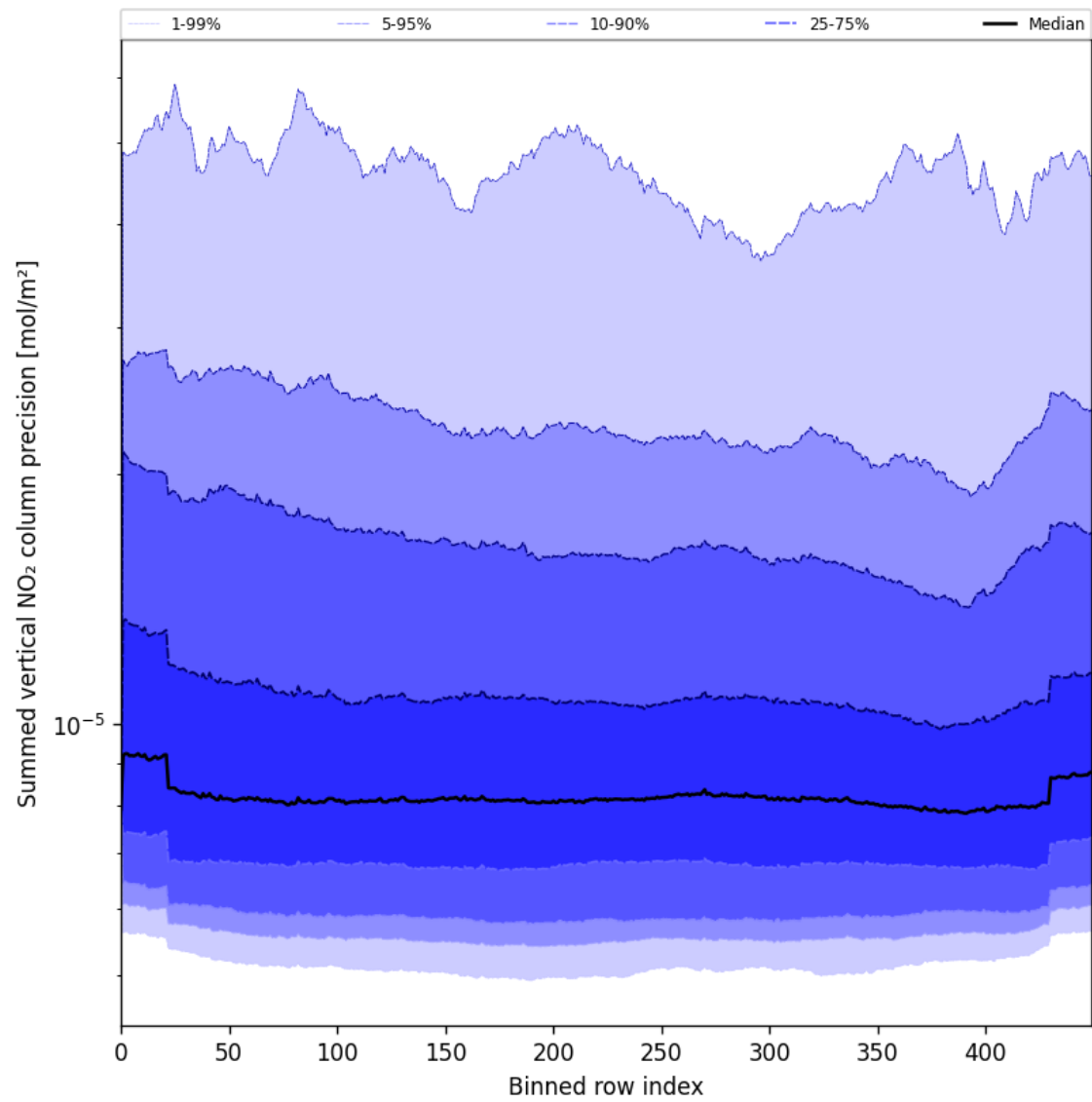
Figure 56: Along track statistics of “Summed vertical NO 2 column precision” for 2025-07-30 to 2025-07-31
