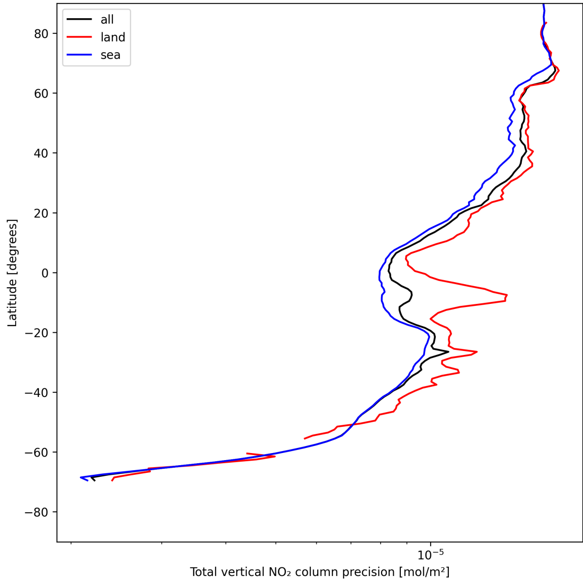
Figure 20: Zonal average of “Total vertical NO 2 column precision” for 2025-07-30 to 2025-07-31.
