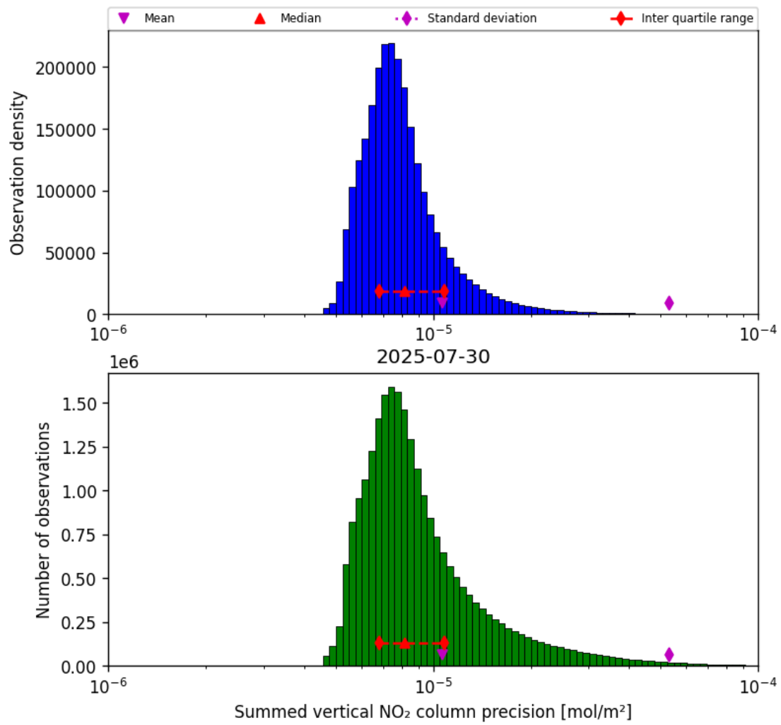
Figure 39: Histogram of “Summed vertical NO 2 column precision” for 2025-07-30 to 2025-07-31
