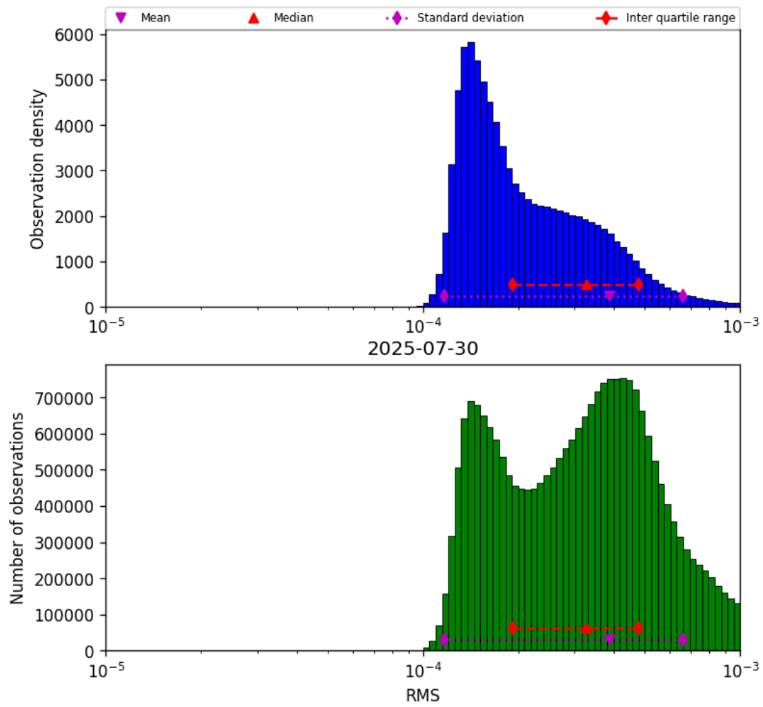
Figure 41: Histogram of “RMS” for 2025-07-30 to 2025-07-31
