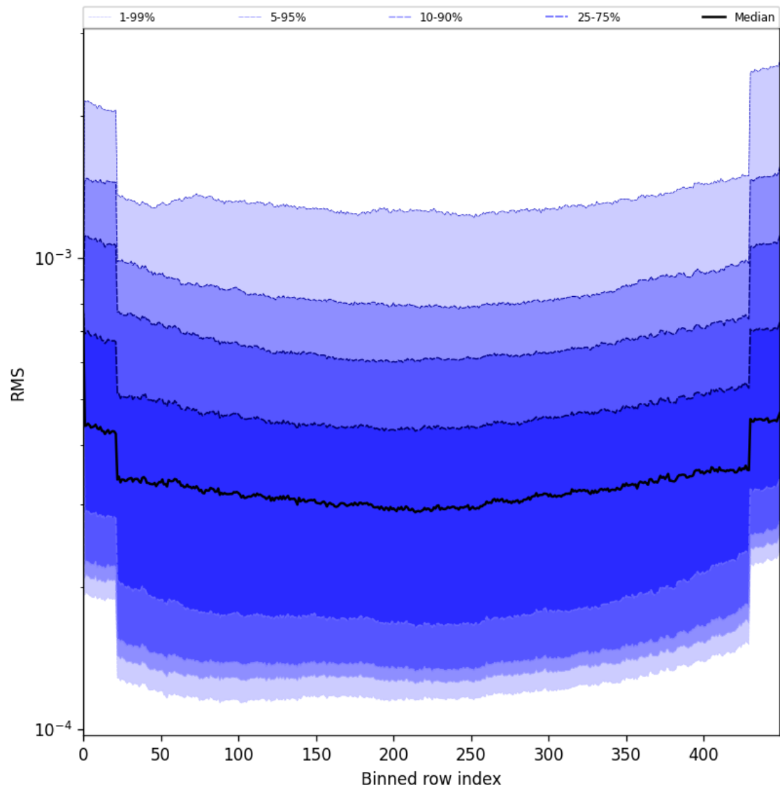
Figure 58: Along track statistics of “RMS” for 2025-07-30 to 2025-07-31
