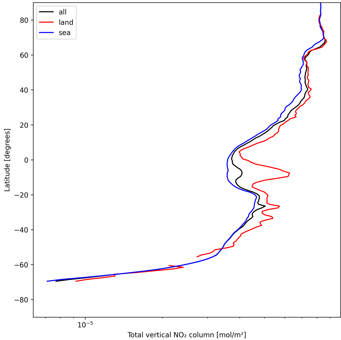
Figure 19: Zonal average of “Total vertical NO 2 column” for 2025-07-30 to 2025-07-31.
