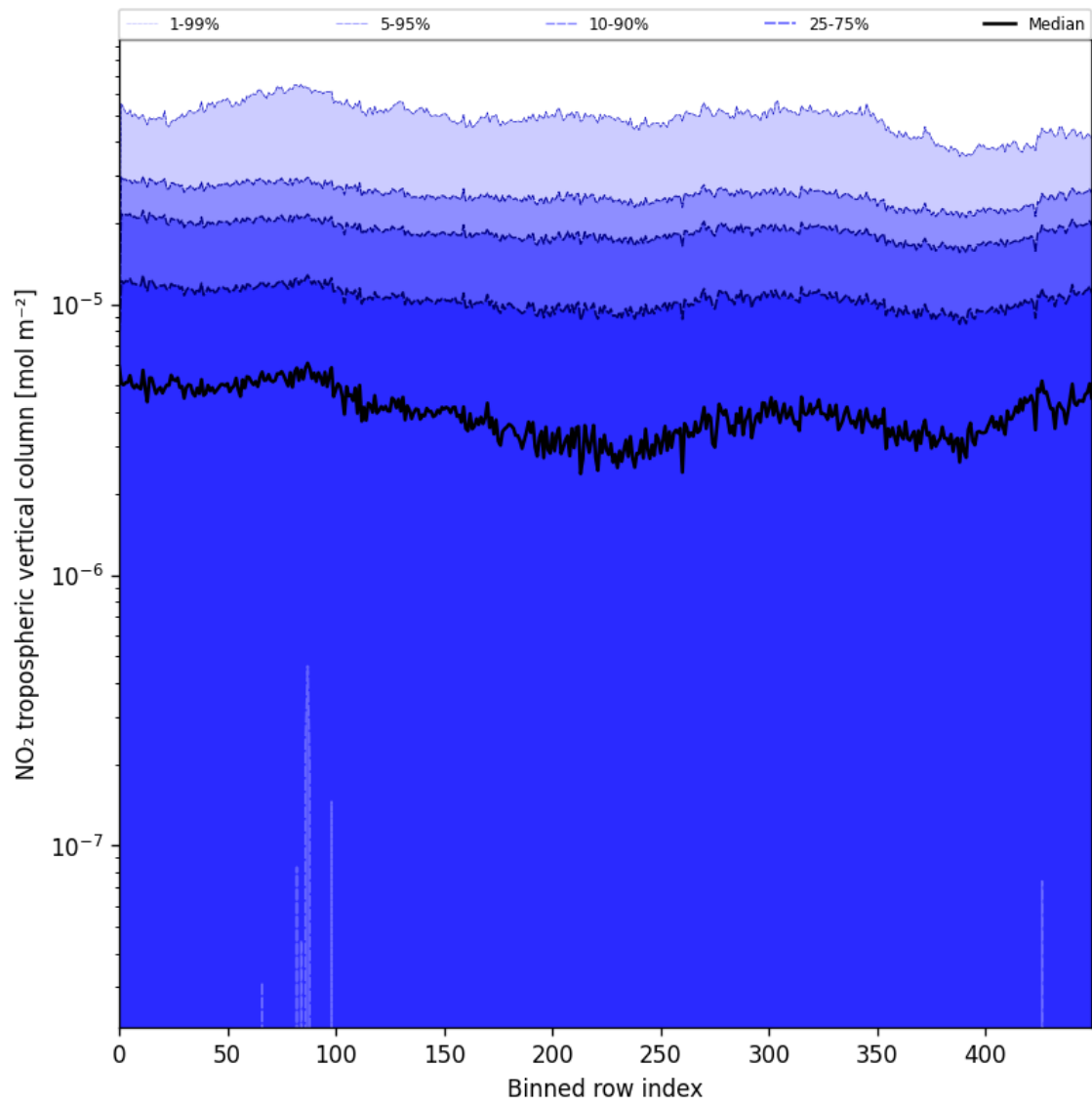
Figure 44: Along track statistics of “NO 2 tropospheric vertical column” for 2025-07-30 to 2025-07-31
