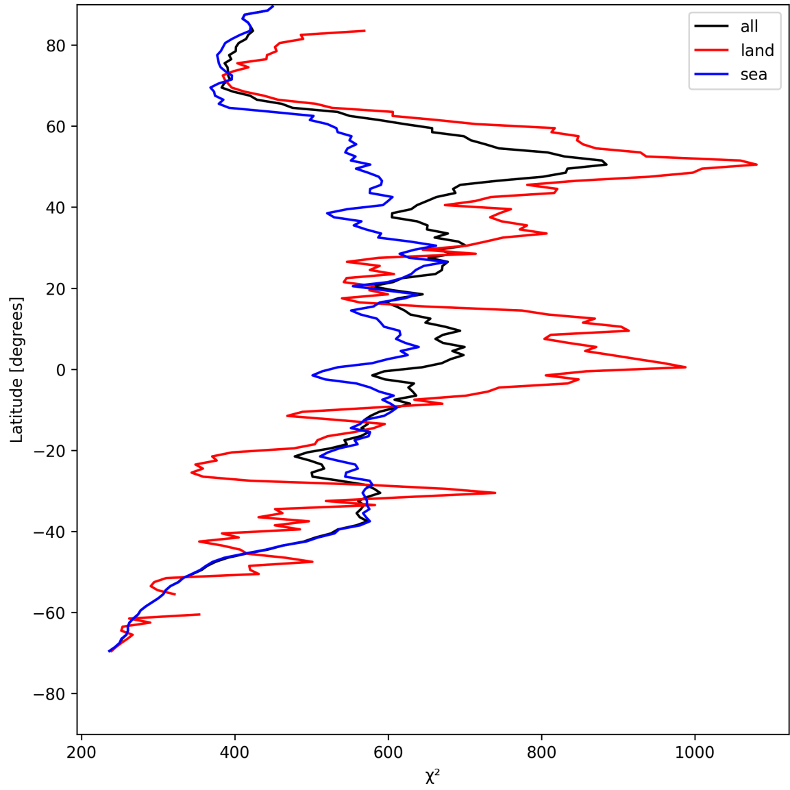
Figure 23: Zonal average of “ \chi^2 ” for 2025-07-30 to 2025-07-31.
