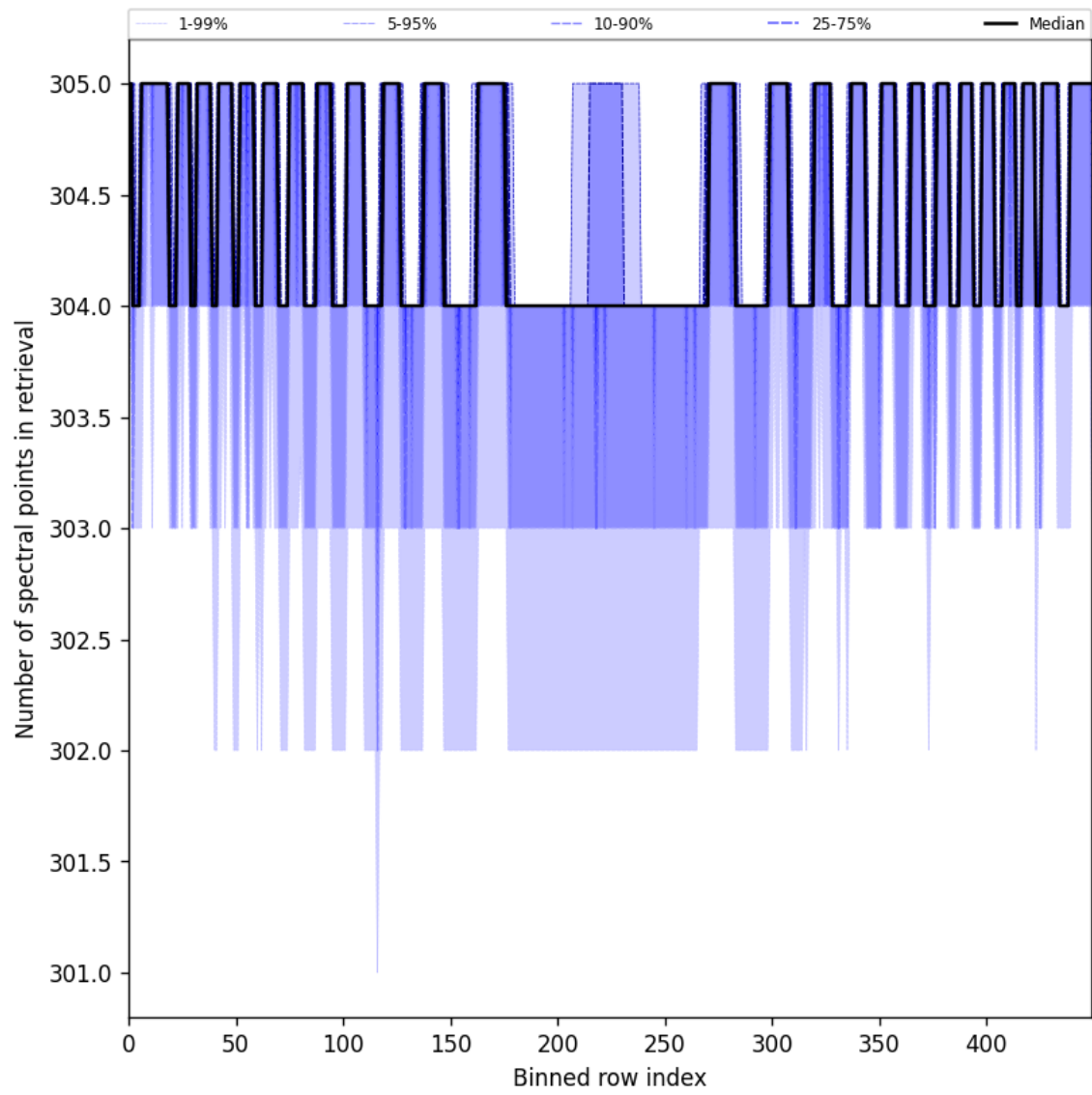
Figure 48: Along track statistics of “Number of spectral points in retrieval” for 2025-07-30 to 2025-07-31
