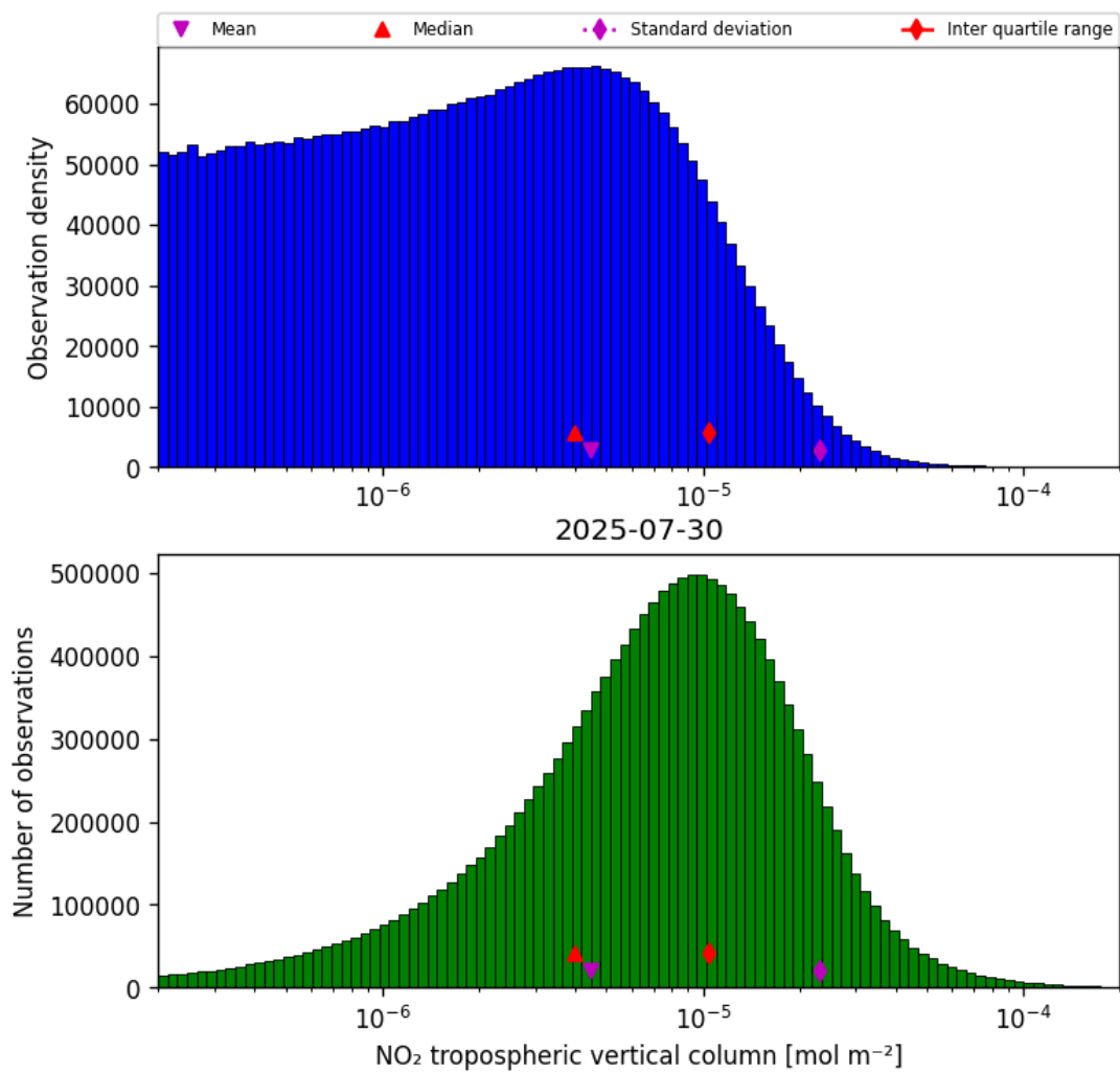
Figure 27: Histogram of “NO 2 tropospheric vertical column” for 2025-07-30 to 2025-07-31
