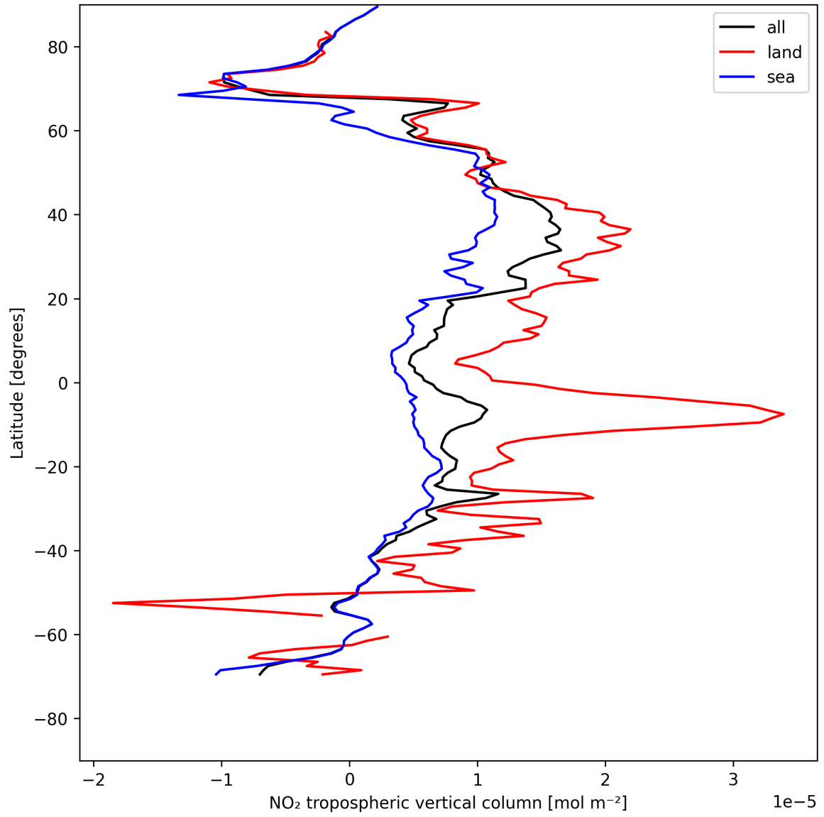
Figure 10: Zonal average of “NO 2 tropospheric vertical column” for 2025-07-30 to 2025-07-31.
