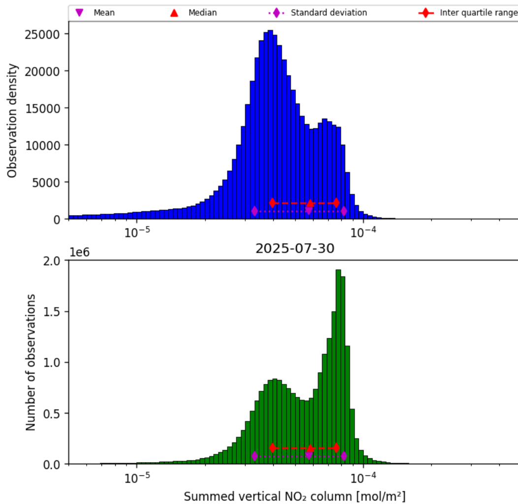
Figure 38: Histogram of “Summed vertical NO 2 column” for 2025-07-30 to 2025-07-31
