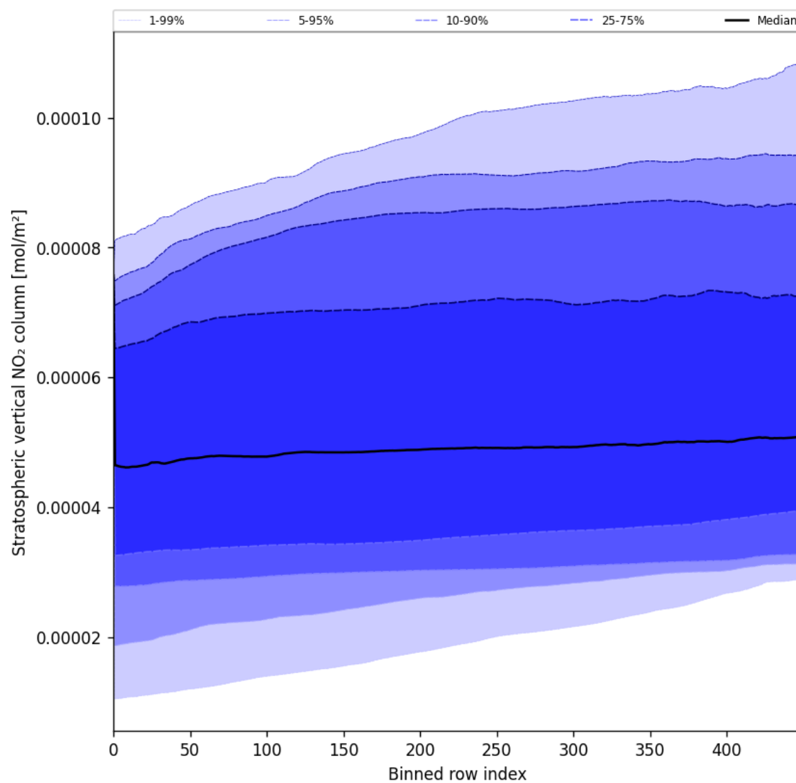
Figure 51: Along track statistics of “Stratospheric vertical NO 2 column” for 2025-07-30 to 2025-07-31
