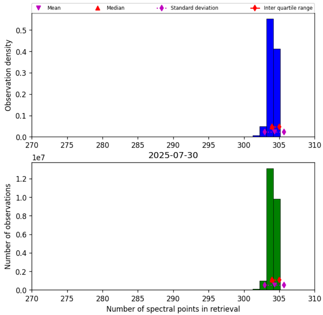
Figure 31: Histogram of “Number of spectral points in retrieval” for 2025-07-30 to 2025-07-31
