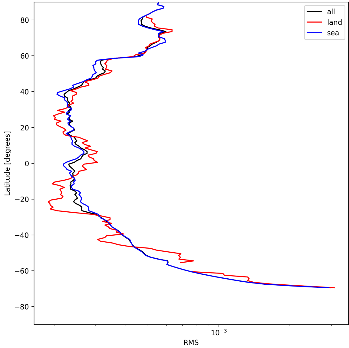
Figure 24: Zonal average of “RMS” for 2025-07-30 to 2025-07-31.
