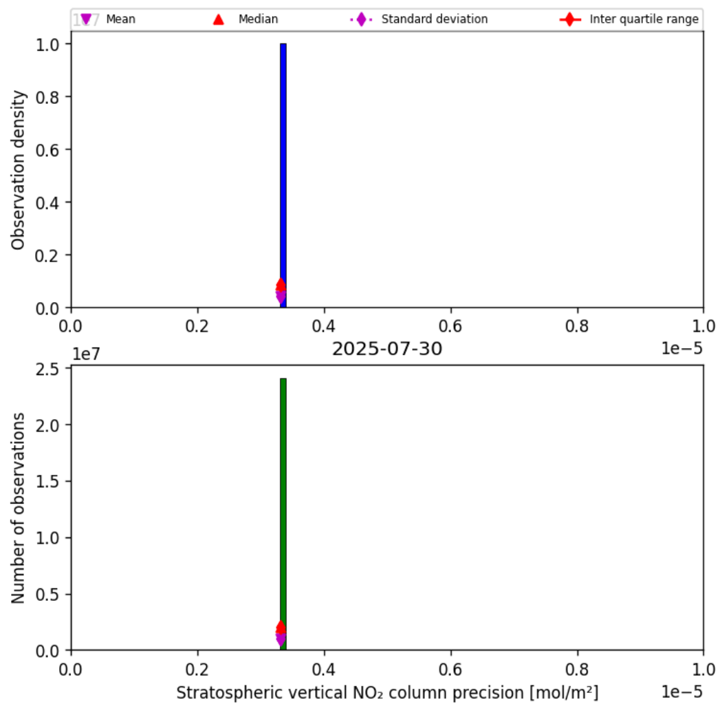
Figure 35: Histogram of “Stratospheric vertical NO 2 column precision” for 2025-07-30 to 2025-07-31
