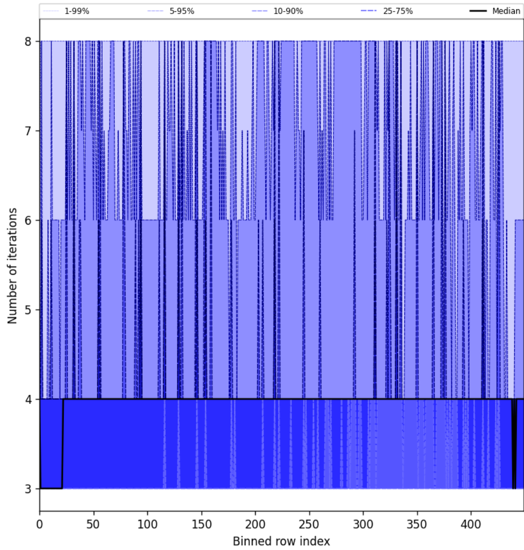
Figure 49: Along track statistics of “Number of iterations” for 2025-07-30 to 2025-07-31
