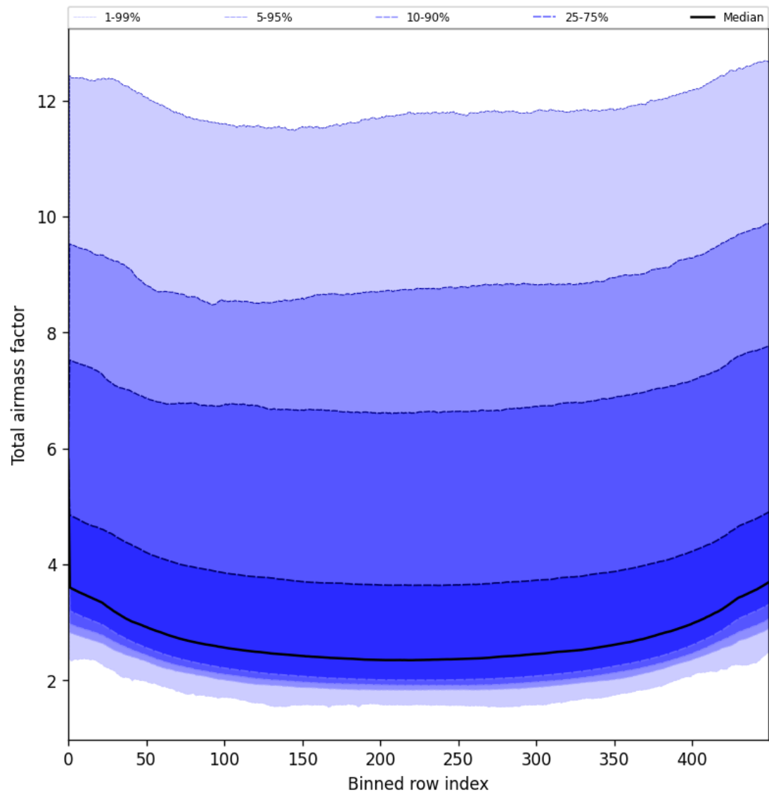
Figure 47: Along track statistics of “Total airmass factor” for 2025-07-30 to 2025-07-31
