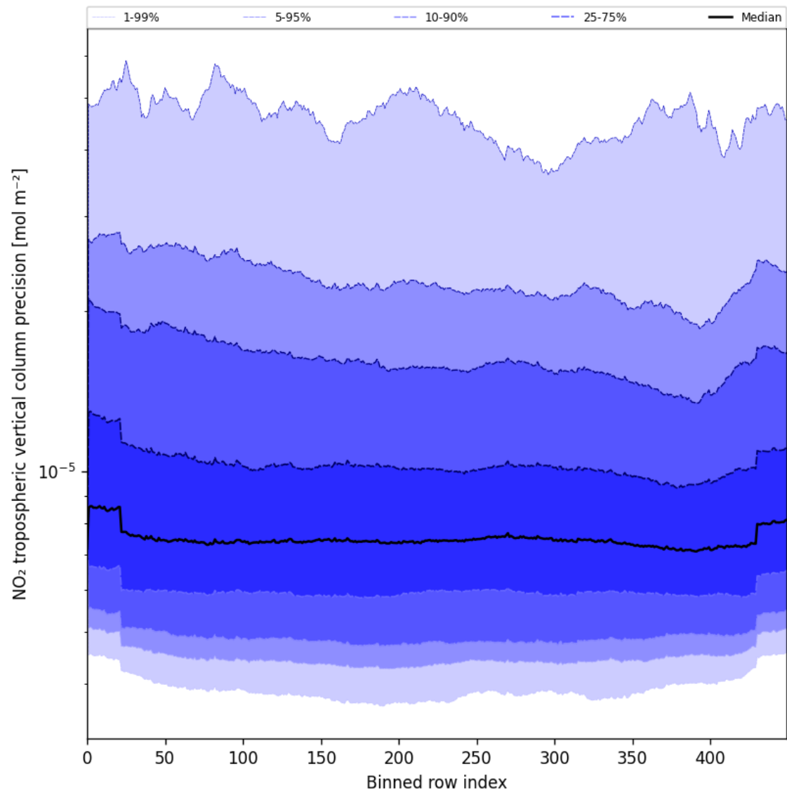
Figure 45: Along track statistics of “NO 2 tropospheric vertical column precision” for 2025-07-30 to 2025-07-31
