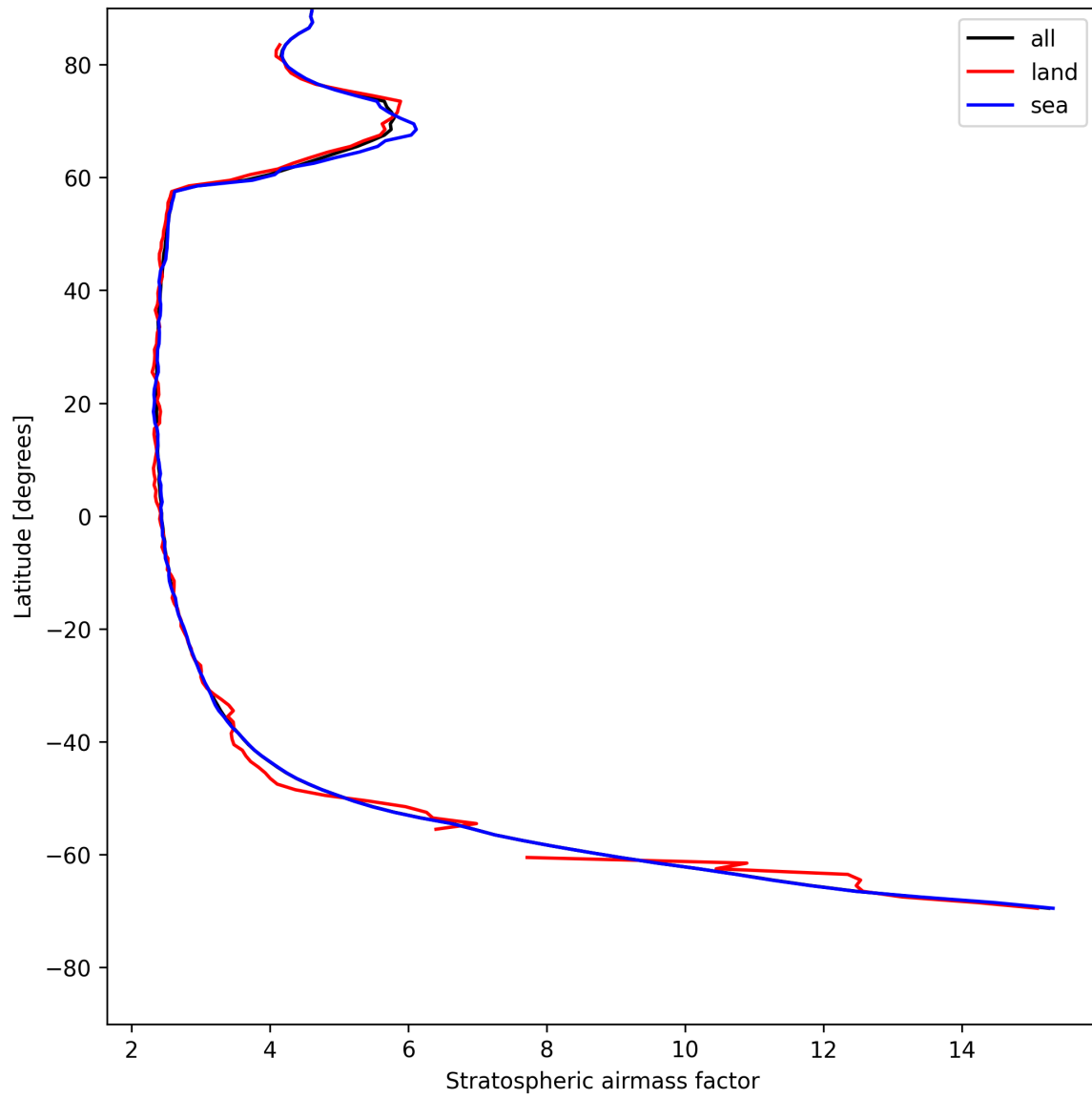
Figure 25: Zonal average of “Stratospheric airmass factor” for 2025-07-30 to 2025-07-31.
