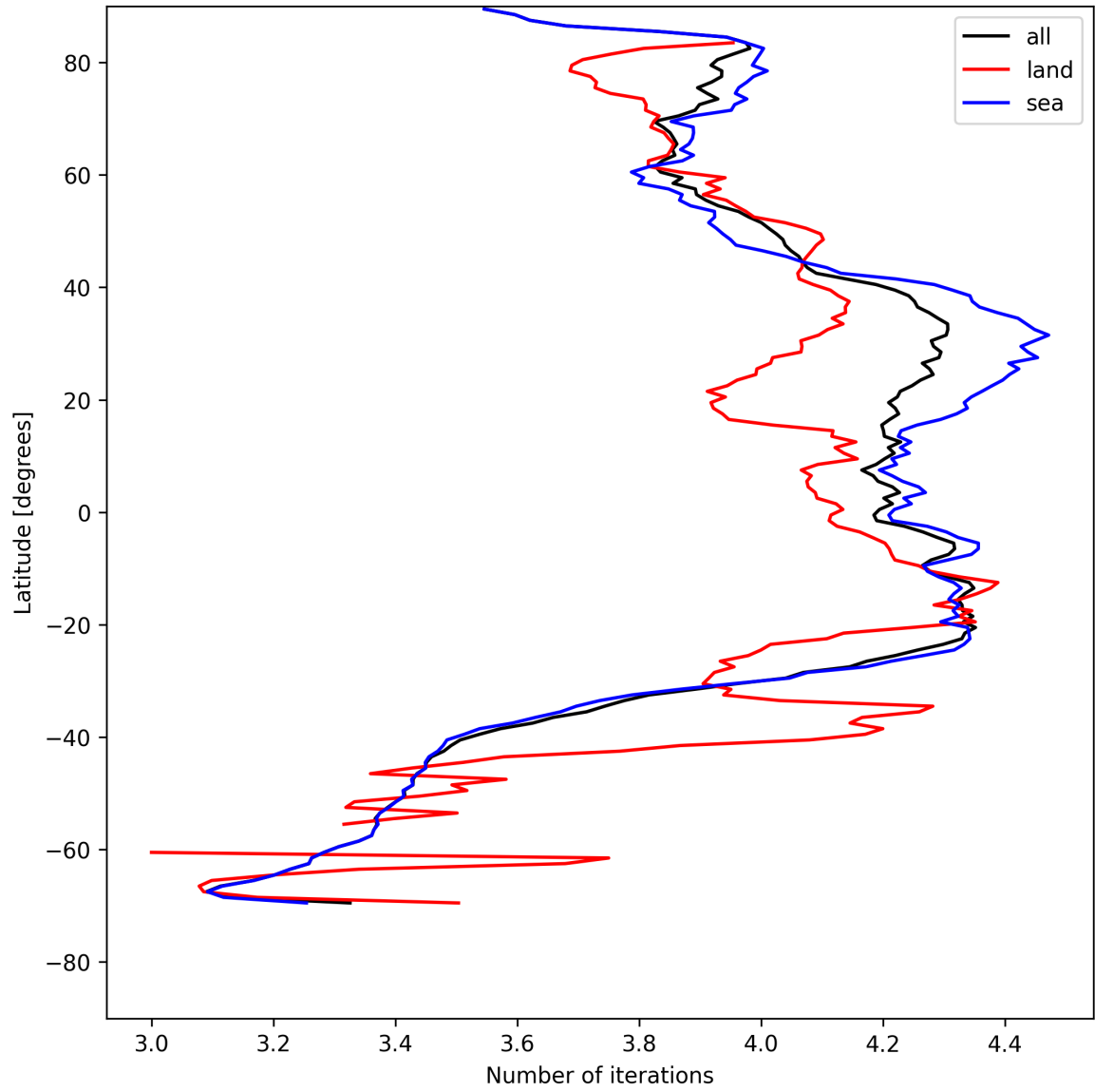
Figure 15: Zonal average of “Number of iterations” for 2025-07-30 to 2025-07-31.
