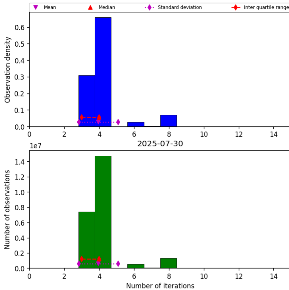
Figure 32: Histogram of “Number of iterations” for 2025-07-30 to 2025-07-31
