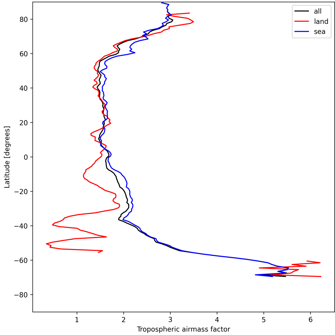
Figure 12: Zonal average of “Tropospheric airmass factor” for 2025-07-30 to 2025-07-31.
