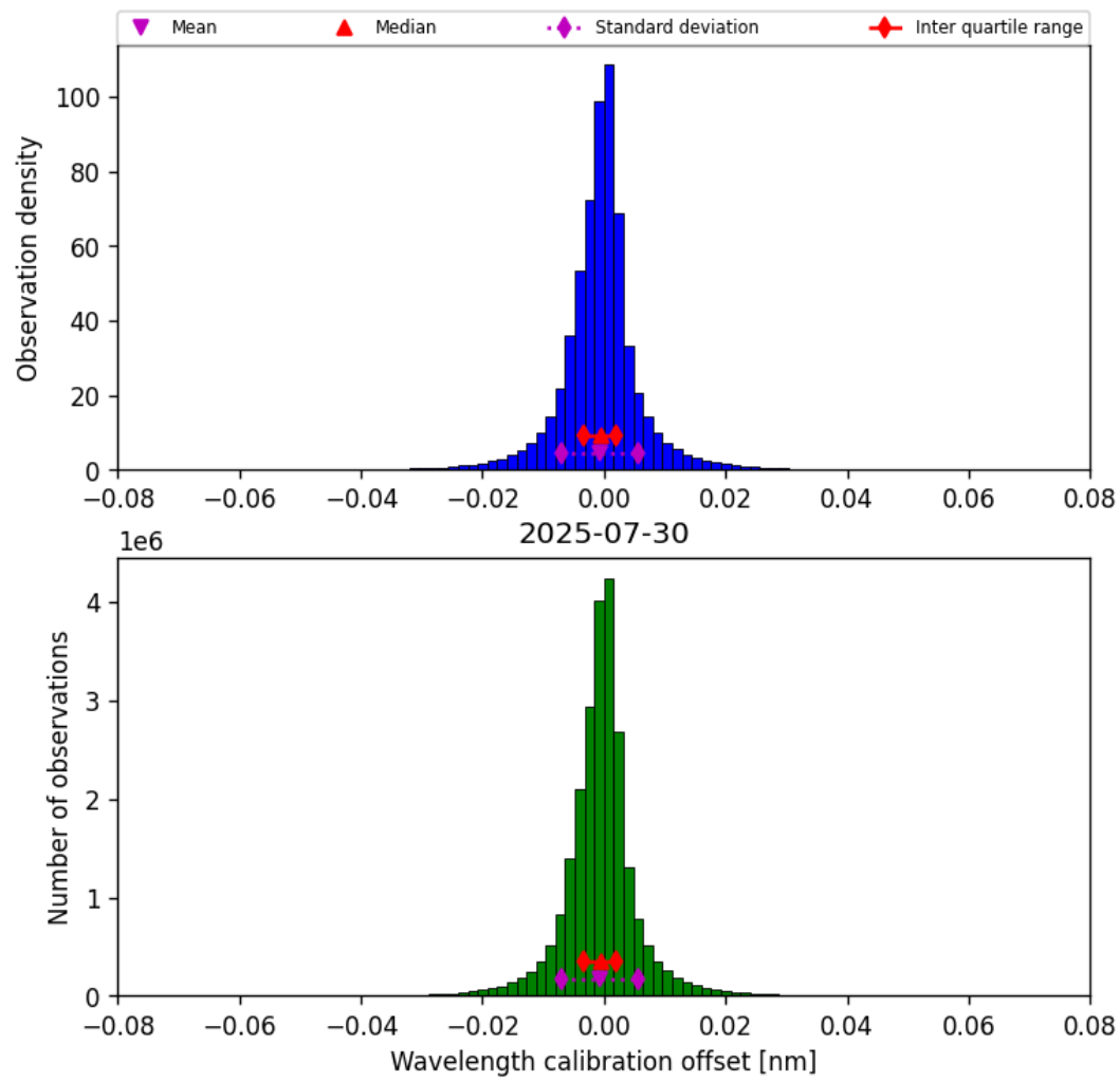
Figure 33: Histogram of “Wavelength calibration offset” for 2025-07-30 to 2025-07-31
