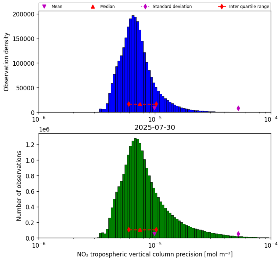
Figure 28: Histogram of “NO 2 tropospheric vertical column precision” for 2025-07-30 to 2025-07-31
