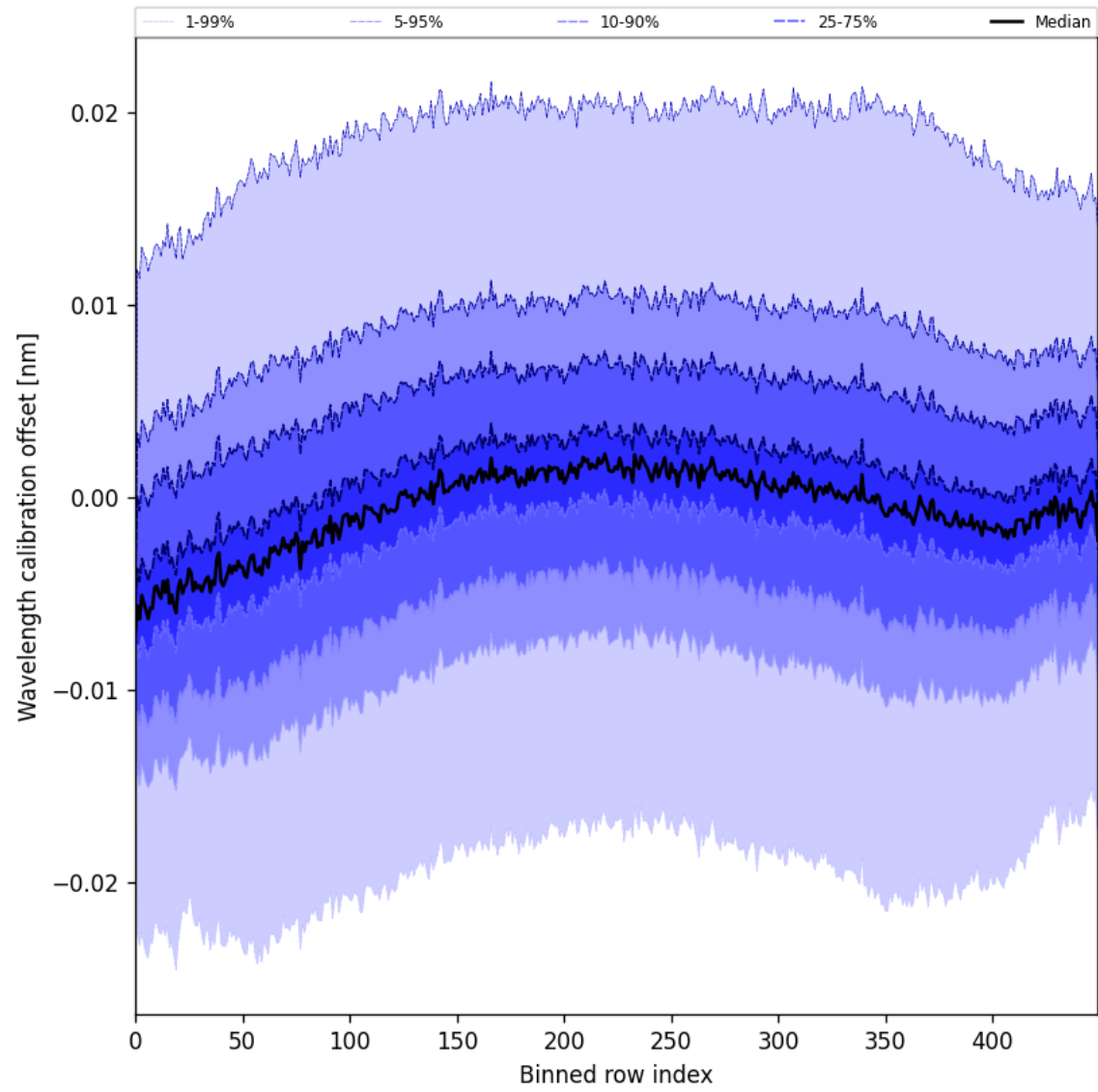
Figure 50: Along track statistics of “Wavelength calibration offset” for 2025-07-30 to 2025-07-31
