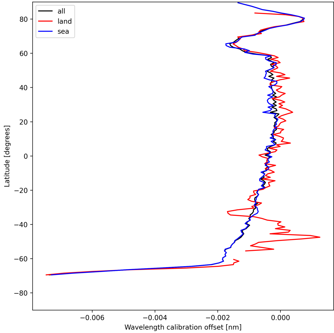
Figure 16: Zonal average of “Wavelength calibration offset” for 2025-07-30 to 2025-07-31.
