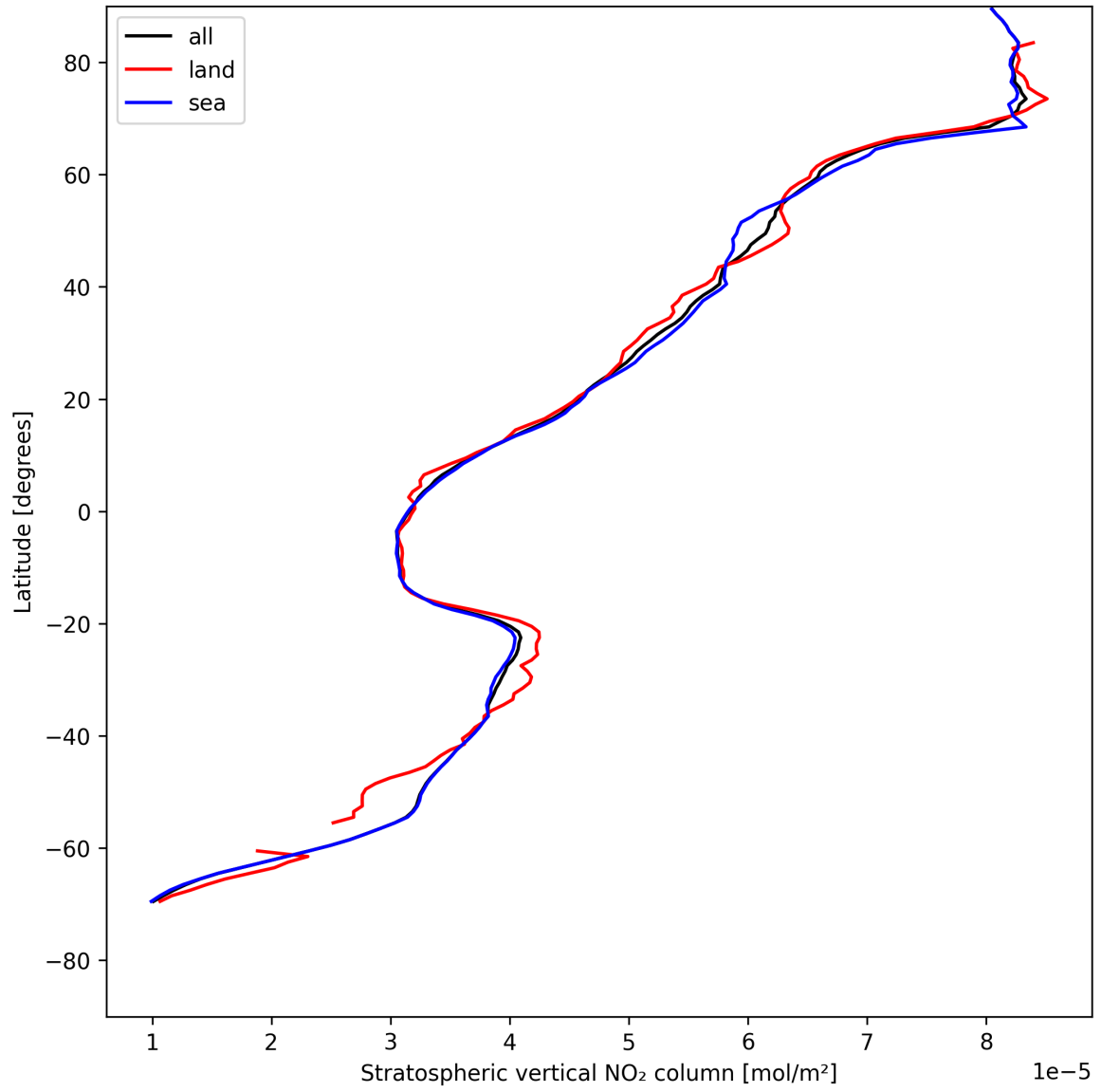
Figure 17: Zonal average of “Stratospheric vertical NO 2 column” for 2025-07-30 to 2025-07-31.
