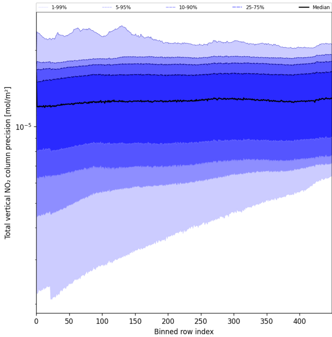
Figure 54: Along track statistics of “Total vertical NO 2 column precision” for 2025-07-30 to 2025-07-31
