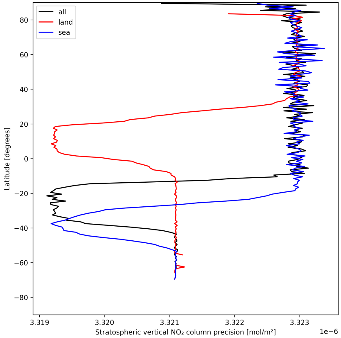
Figure 18: Zonal average of “Stratospheric vertical NO 2 column precision” for 2025-07-30 to 2025-07-31.
