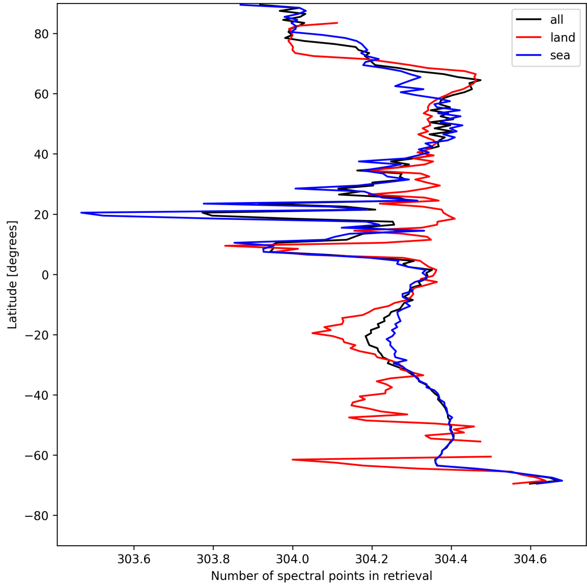
Figure 14: Zonal average of “Number of spectral points in retrieval” for 2025-07-30 to 2025-07-31.
