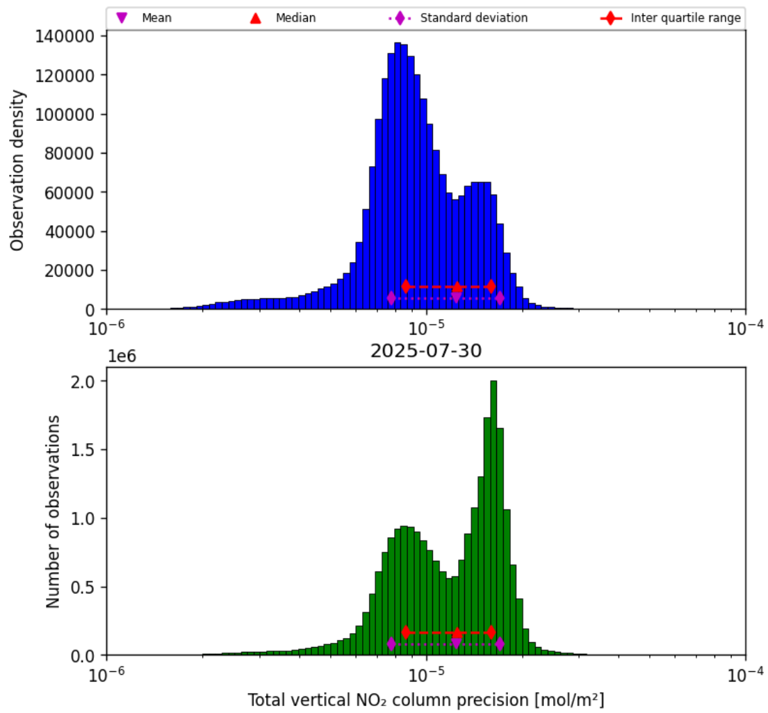
Figure 37: Histogram of “Total vertical NO 2 column precision” for 2025-07-30 to 2025-07-31
