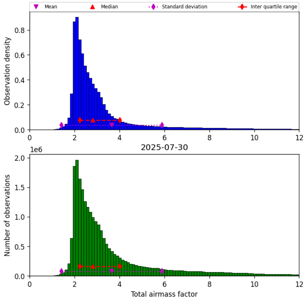
Figure 30: Histogram of “Total airmass factor” for 2025-07-30 to 2025-07-31
