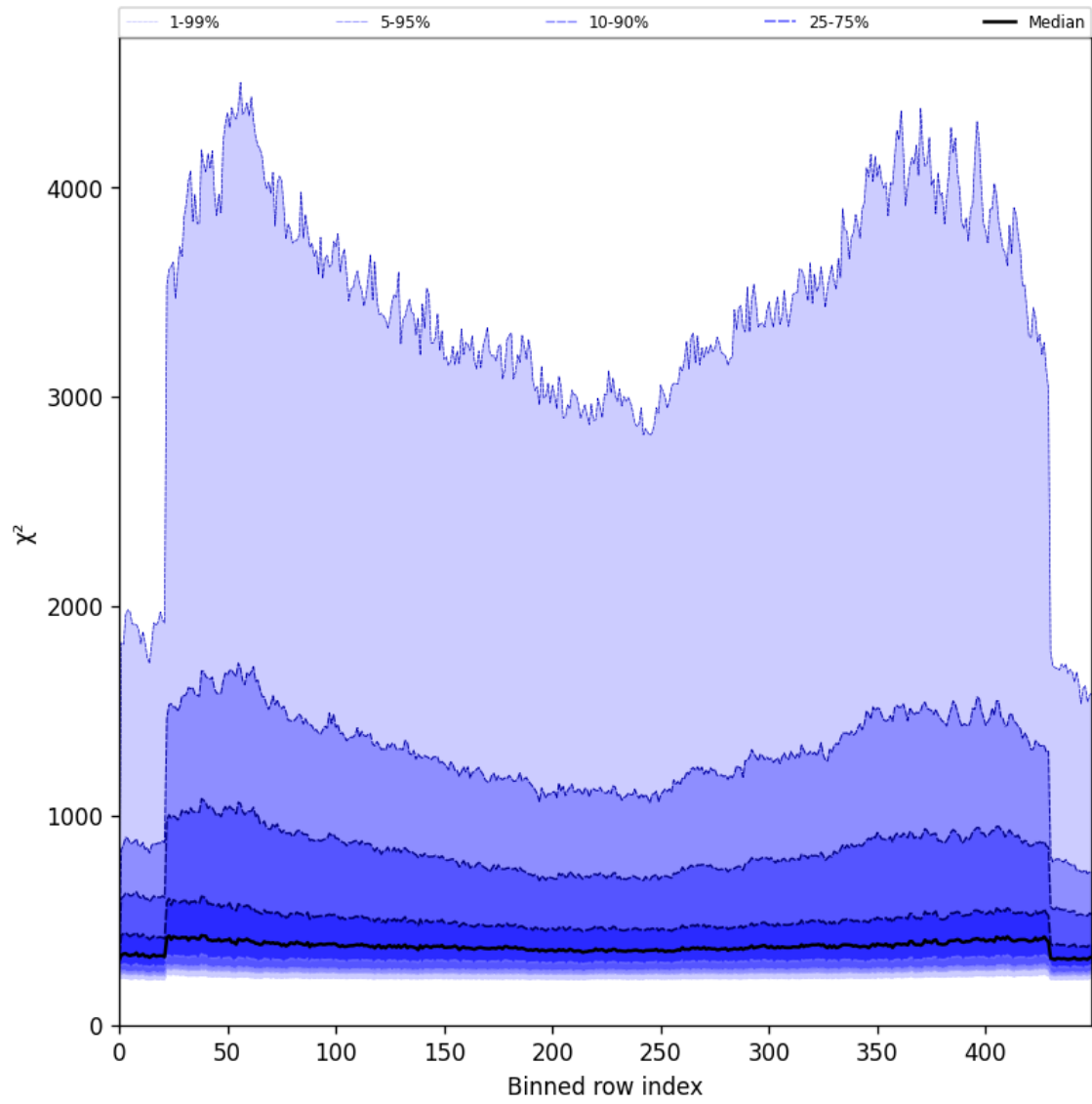
Figure 57: Along track statistics of “ \chi^2 ” for 2025-07-30 to 2025-07-31
