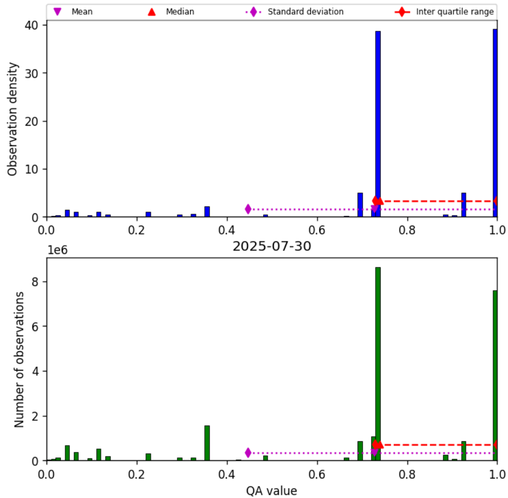
Figure 26: Histogram of “QA value” for 2025-07-30 to 2025-07-31
