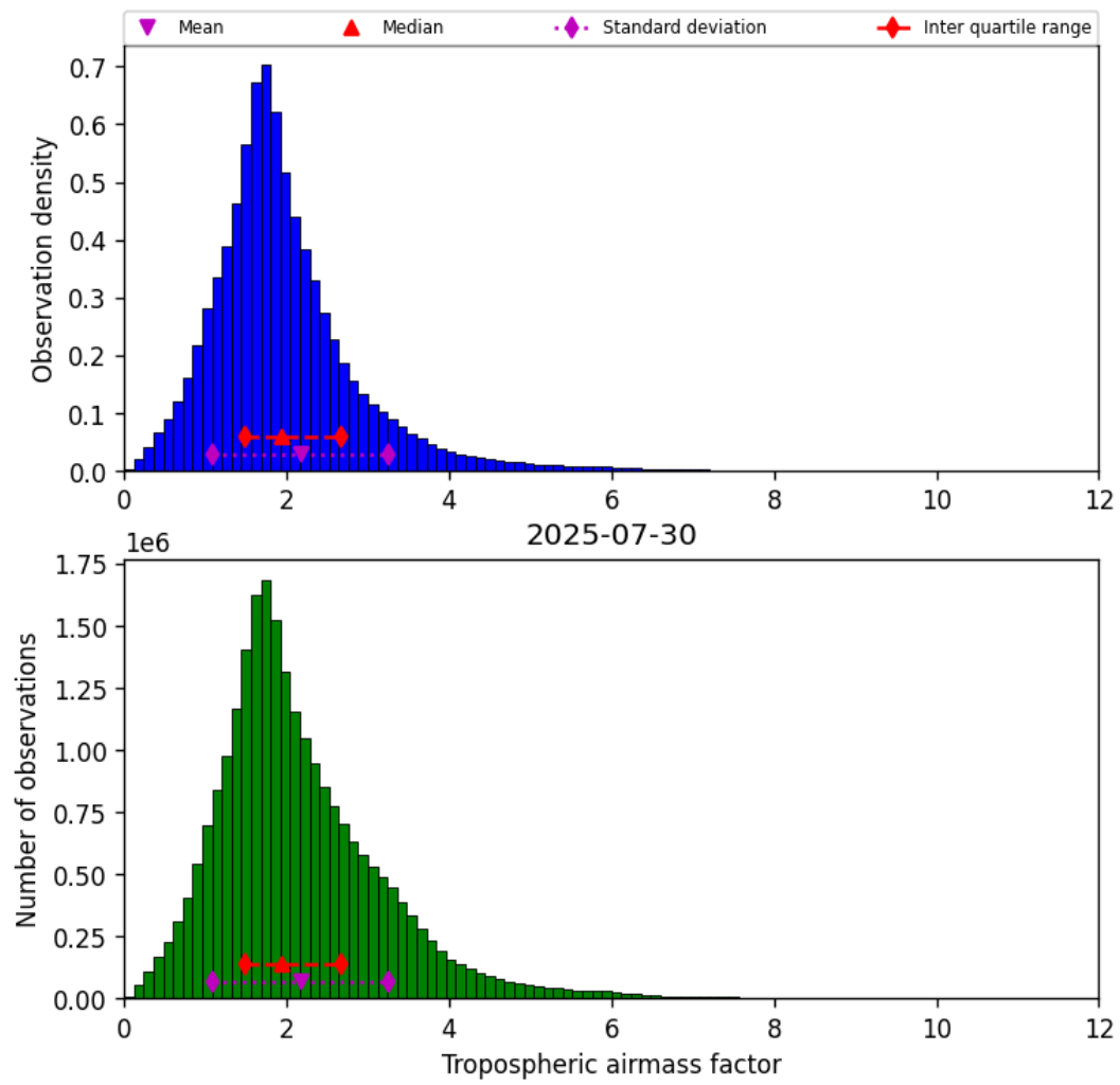
Figure 29: Histogram of “Tropospheric airmass factor” for 2025-07-30 to 2025-07-31
