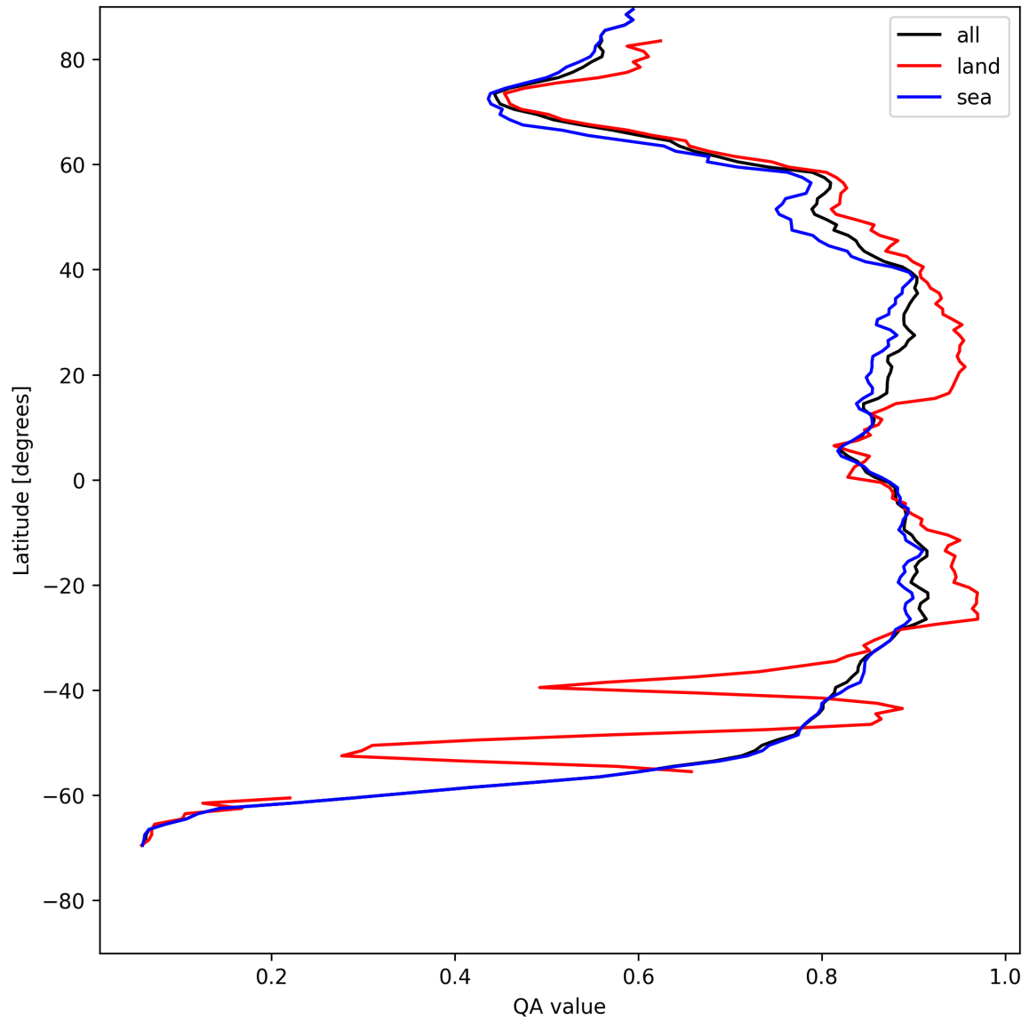
Figure 9: Zonal average of “QA value” for 2025-07-30 to 2025-07-31.
