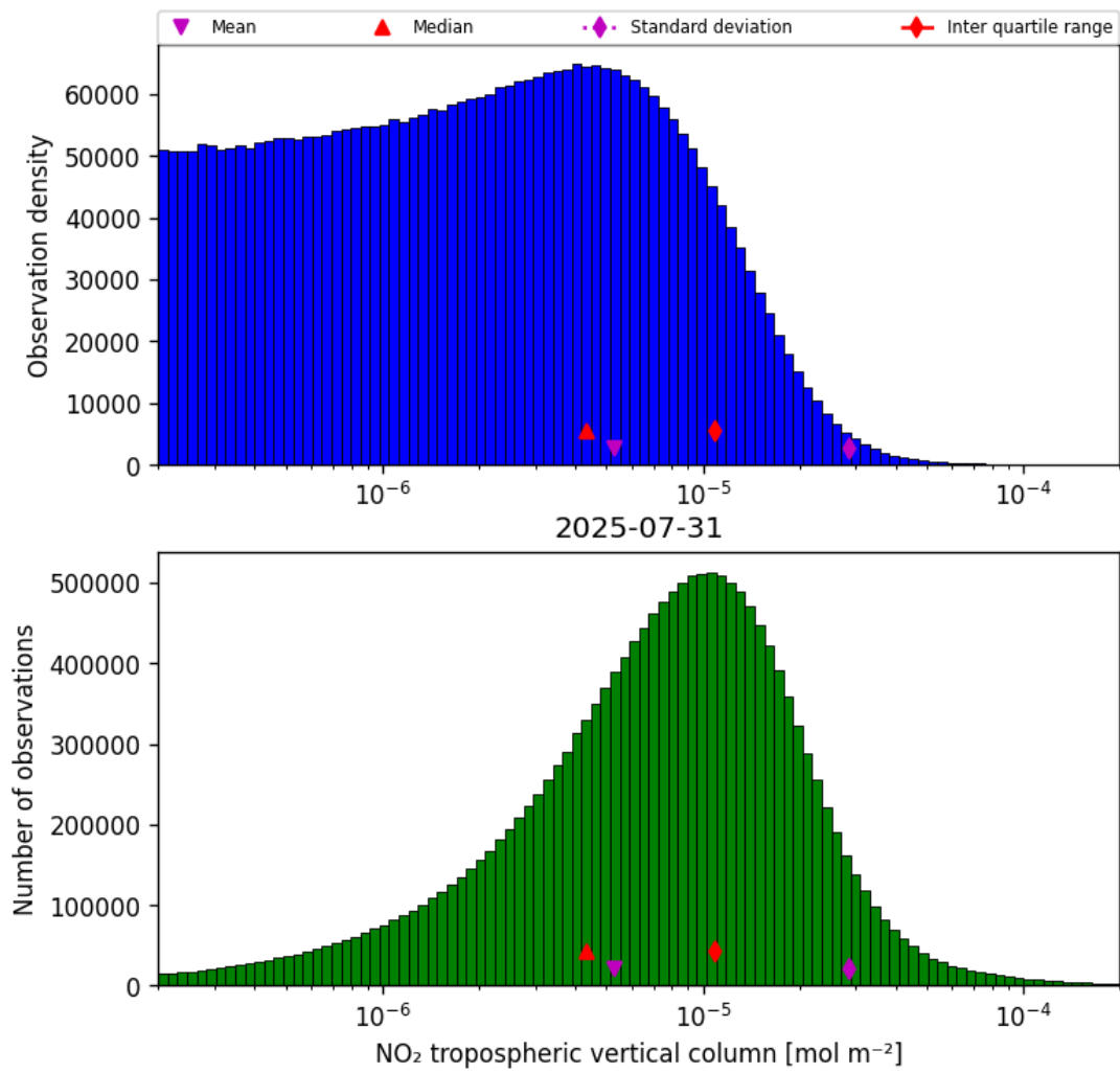
Figure 27: Histogram of “NO 2 tropospheric vertical column” for 2025-07-31 to 2025-08-01
