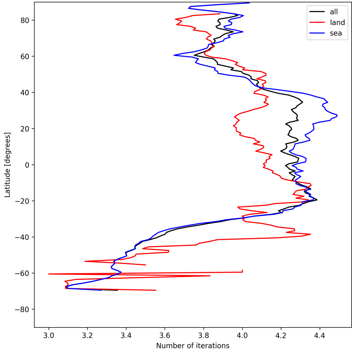
Figure 15: Zonal average of “Number of iterations” for 2025-07-31 to 2025-08-01.
