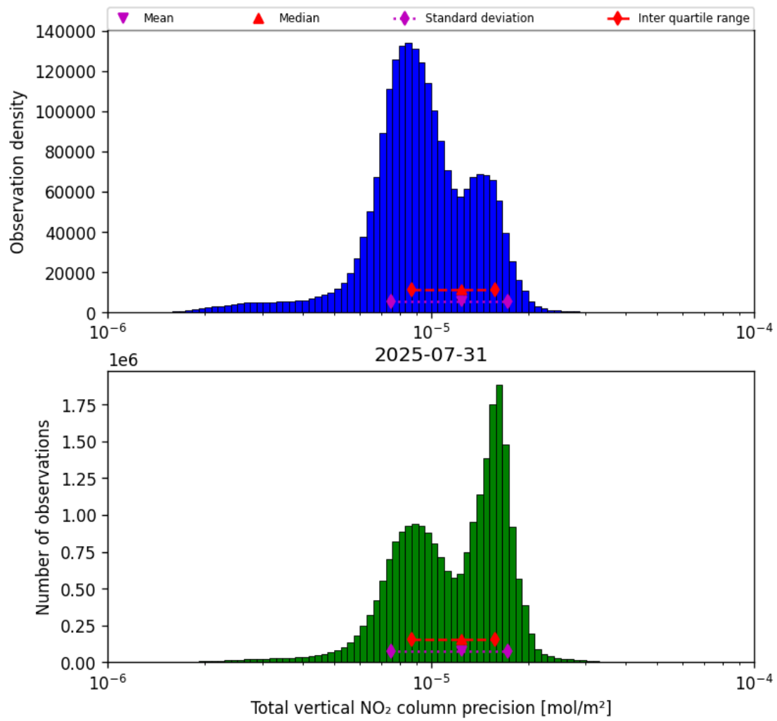
Figure 37: Histogram of “Total vertical NO 2 column precision” for 2025-07-31 to 2025-08-01
