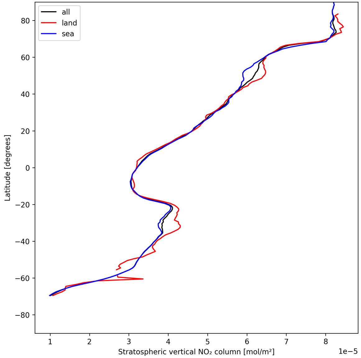
Figure 17: Zonal average of “Stratospheric vertical NO 2 column” for 2025-07-31 to 2025-08-01.
