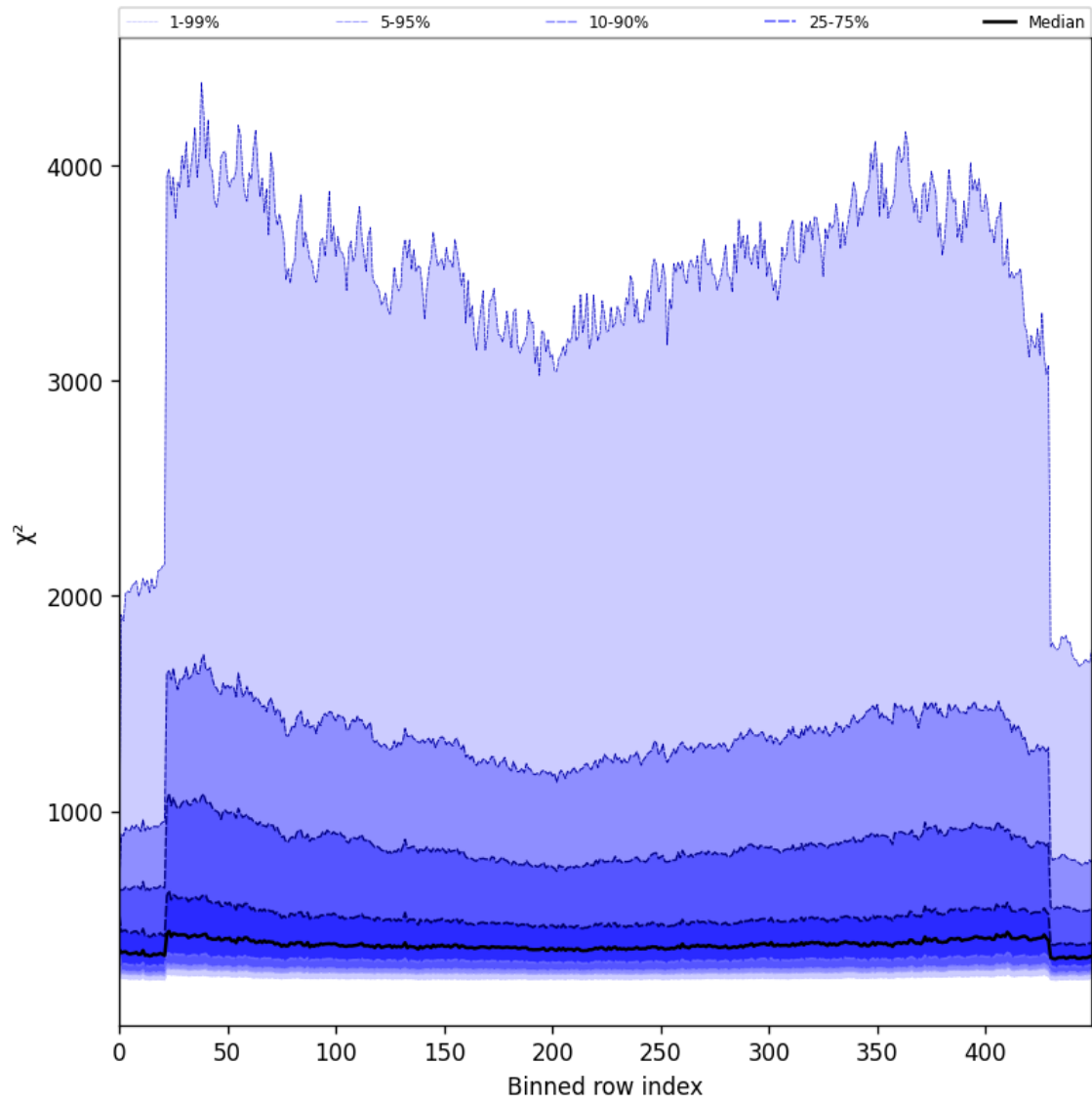
Figure 57: Along track statistics of “ \chi^2 ” for 2025-07-31 to 2025-08-01
