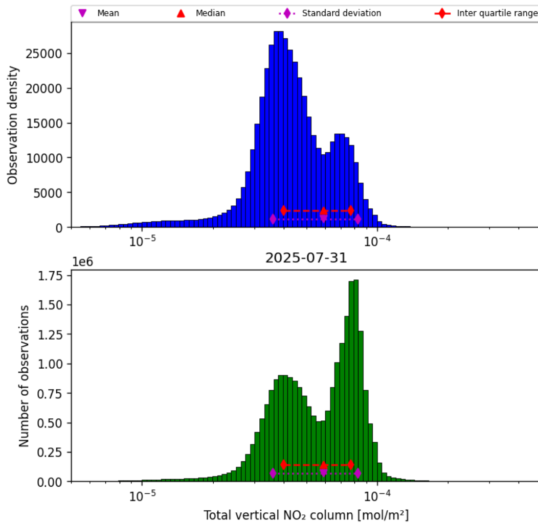
Figure 36: Histogram of “Total vertical NO 2 column” for 2025-07-31 to 2025-08-01
