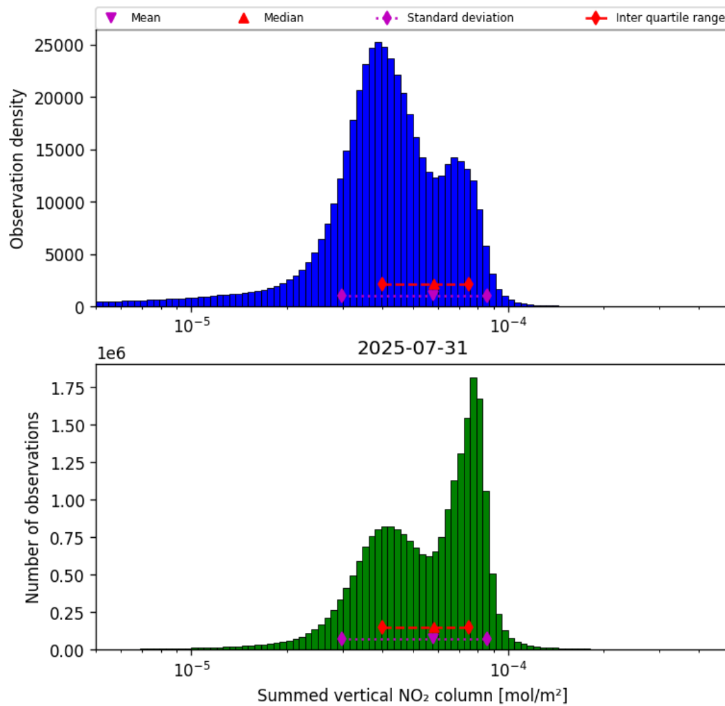
Figure 38: Histogram of “Summed vertical NO 2 column” for 2025-07-31 to 2025-08-01
