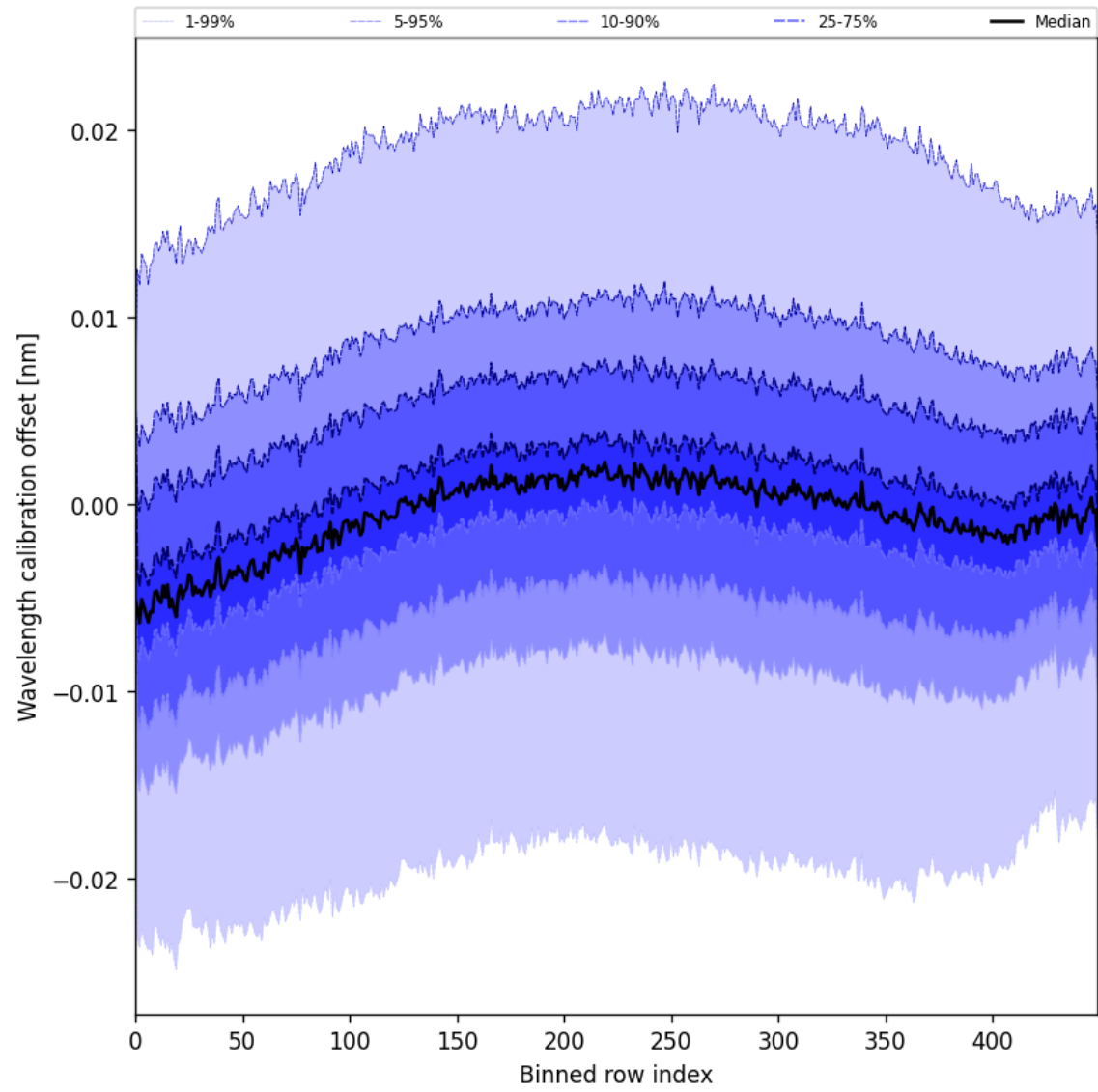
Figure 50: Along track statistics of “Wavelength calibration offset” for 2025-07-31 to 2025-08-01
