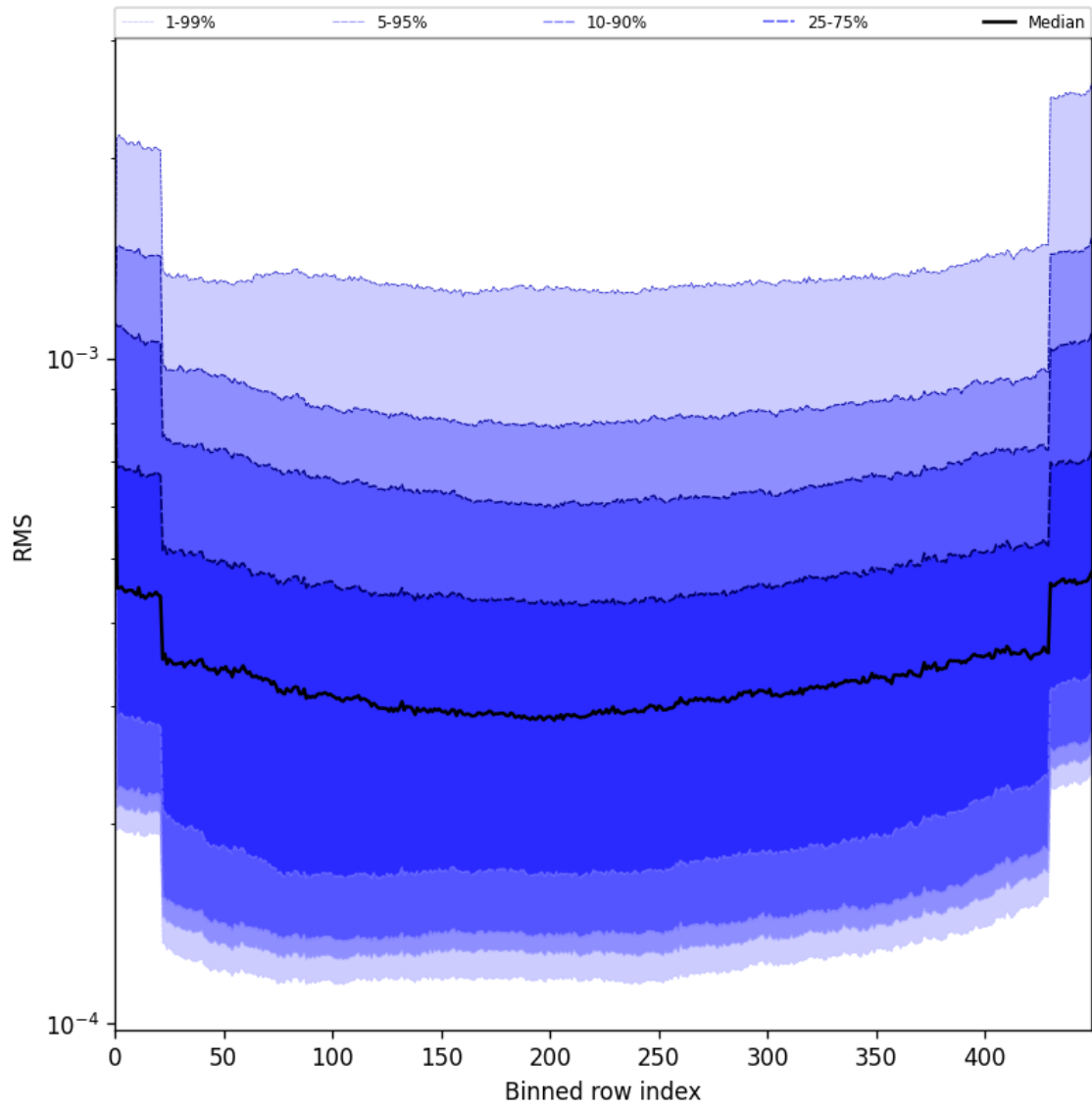
Figure 58: Along track statistics of “RMS” for 2025-07-31 to 2025-08-01
