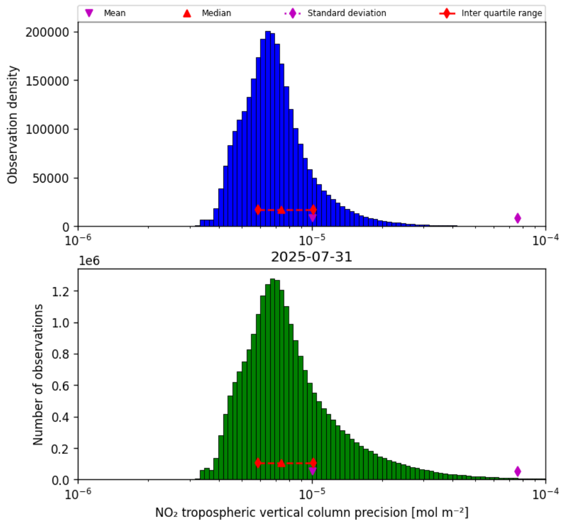
Figure 28: Histogram of “NO 2 tropospheric vertical column precision” for 2025-07-31 to 2025-08-01
