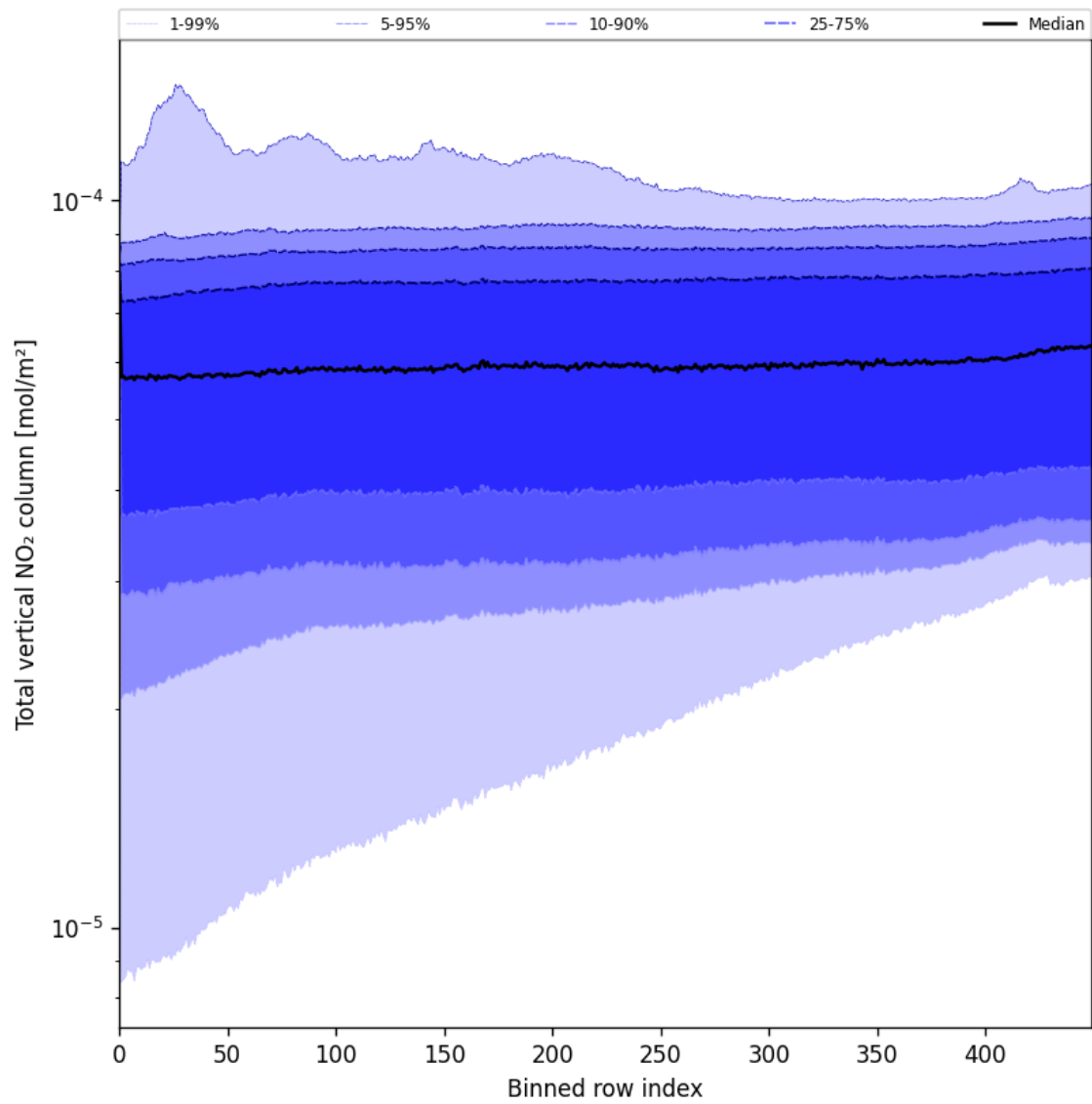
Figure 53: Along track statistics of “Total vertical NO 2 column” for 2025-07-31 to 2025-08-01
