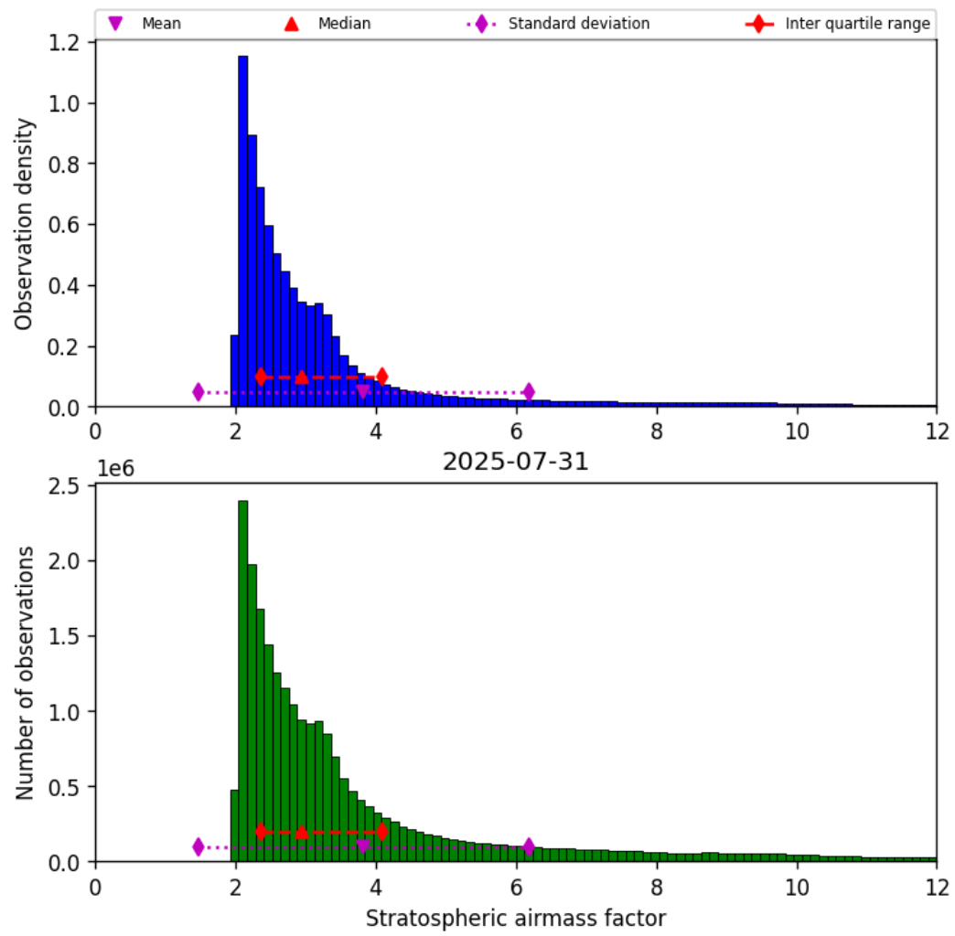
Figure 42: Histogram of “Stratospheric airmass factor” for 2025-07-31 to 2025-08-01
