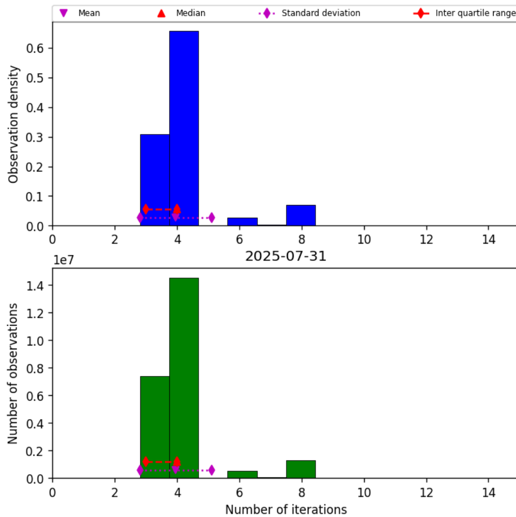
Figure 32: Histogram of “Number of iterations” for 2025-07-31 to 2025-08-01
