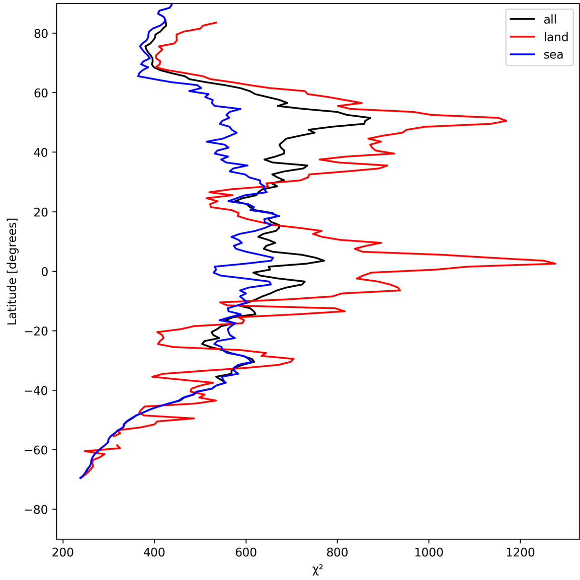
Figure 23: Zonal average of “ \chi^2 ” for 2025-07-31 to 2025-08-01.
