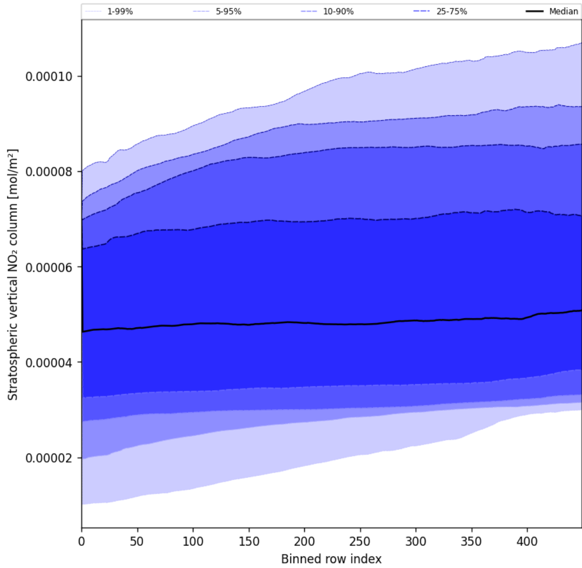
Figure 51: Along track statistics of “Stratospheric vertical NO 2 column” for 2025-07-31 to 2025-08-01
