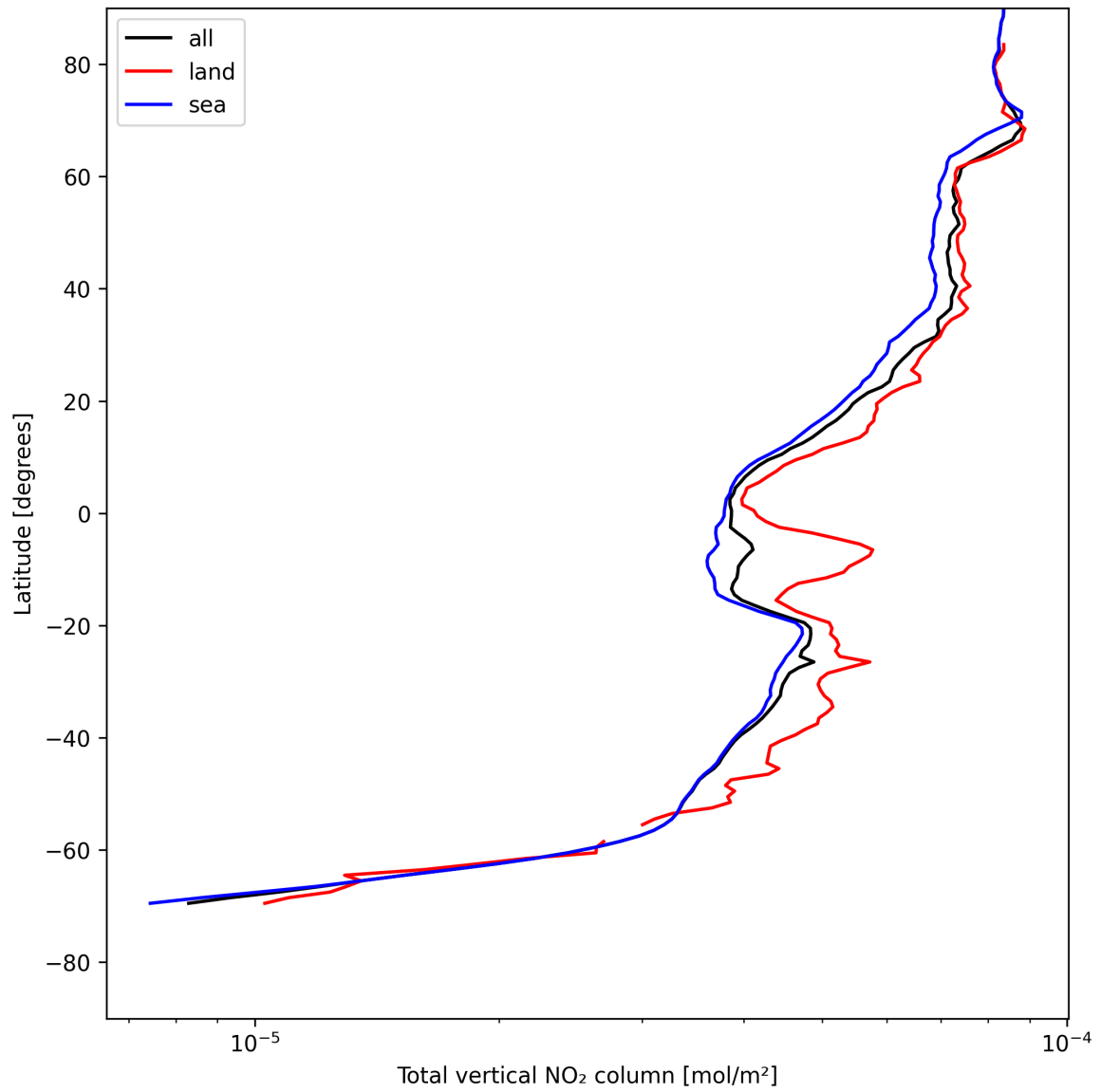
Figure 19: Zonal average of “Total vertical NO 2 column” for 2025-07-31 to 2025-08-01.
