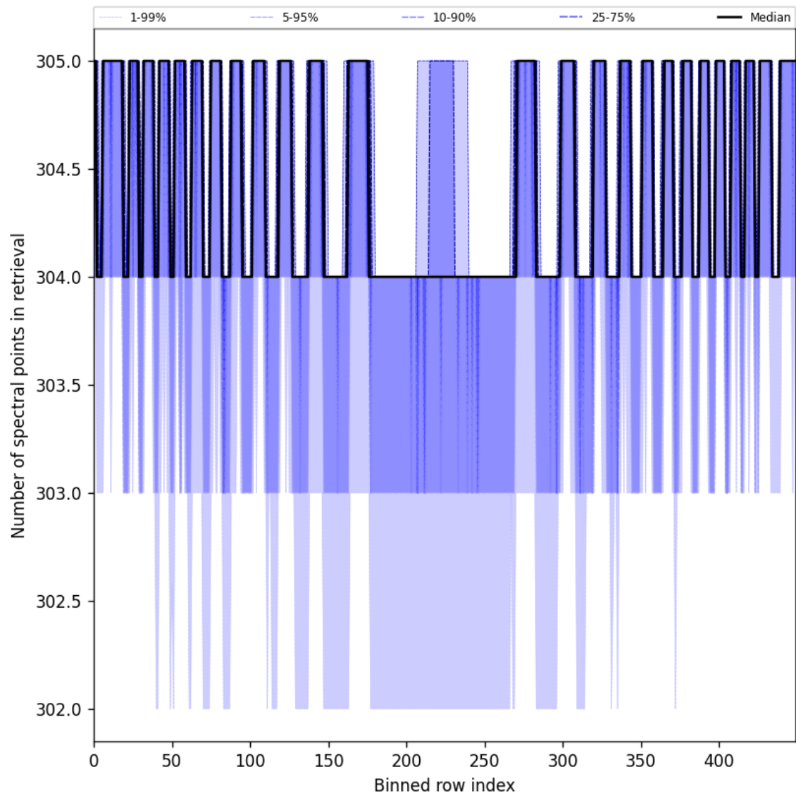
Figure 48: Along track statistics of “Number of spectral points in retrieval” for 2025-07-31 to 2025-08-01
