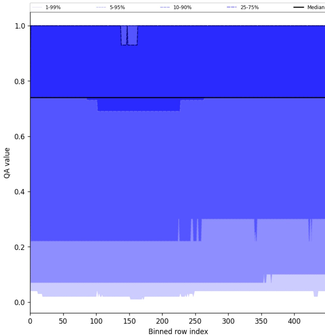
Figure 43: Along track statistics of “QA value” for 2025-07-31 to 2025-08-01
