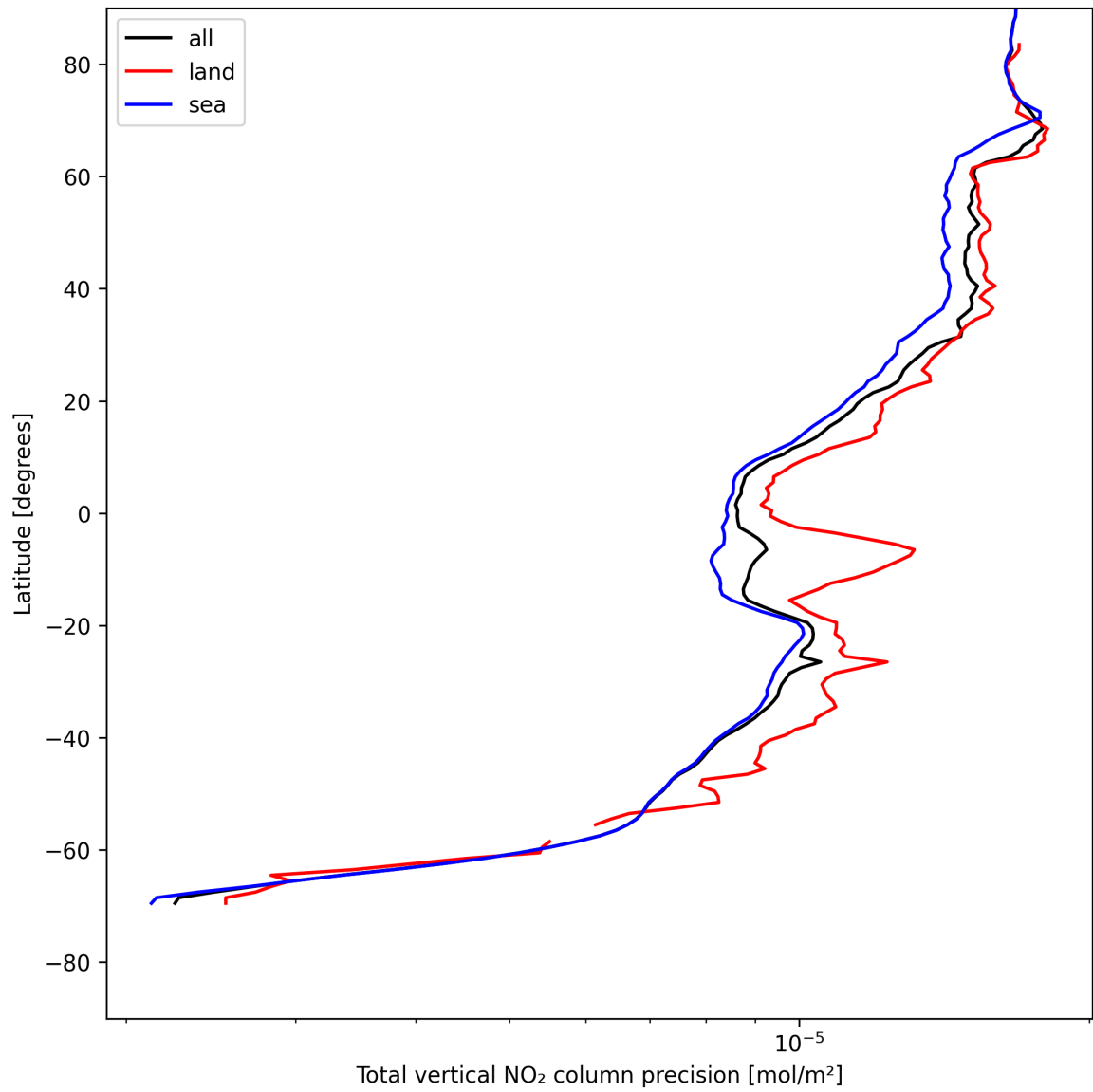
Figure 20: Zonal average of “Total vertical NO 2 column precision” for 2025-07-31 to 2025-08-01.
