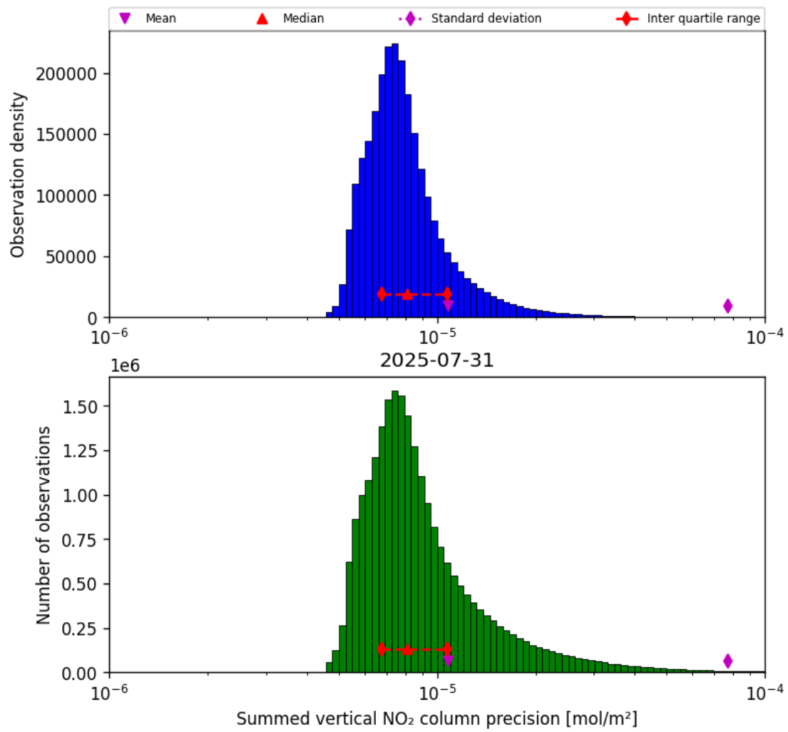
Figure 39: Histogram of “Summed vertical NO 2 column precision” for 2025-07-31 to 2025-08-01
