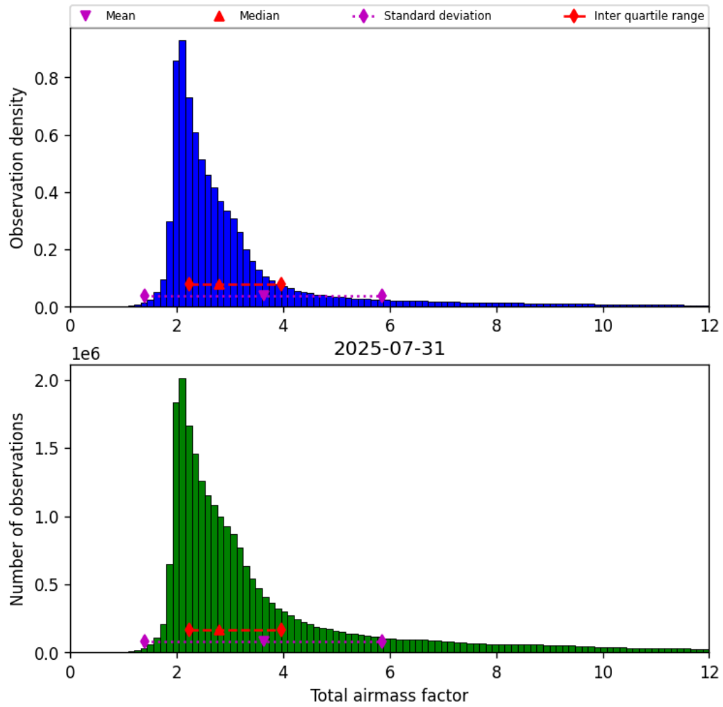
Figure 30: Histogram of “Total airmass factor” for 2025-07-31 to 2025-08-01
