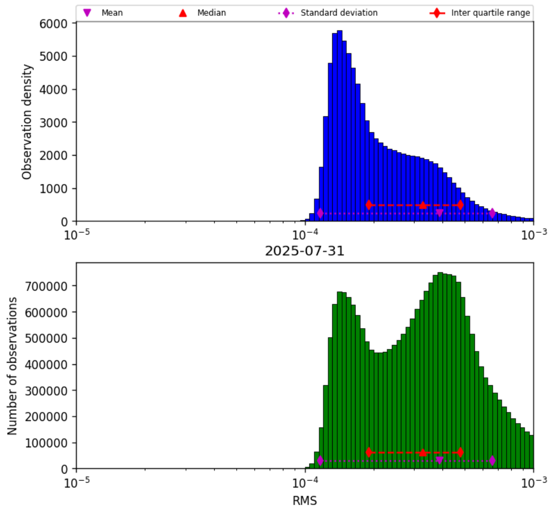
Figure 41: Histogram of “RMS” for 2025-07-31 to 2025-08-01
