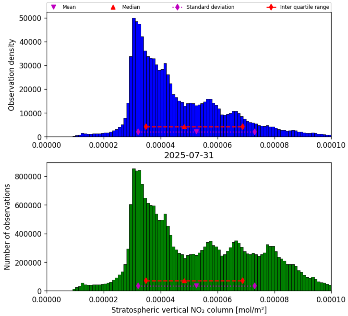
Figure 34: Histogram of “Stratospheric vertical NO 2 column” for 2025-07-31 to 2025-08-01
