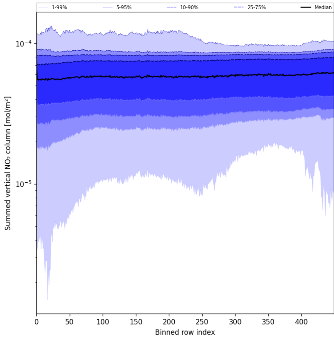
Figure 55: Along track statistics of “Summed vertical NO 2 column” for 2025-07-31 to 2025-08-01
