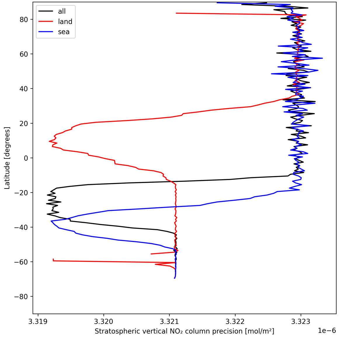
Figure 18: Zonal average of “Stratospheric vertical NO 2 column precision” for 2025-07-31 to 2025-08-01.
