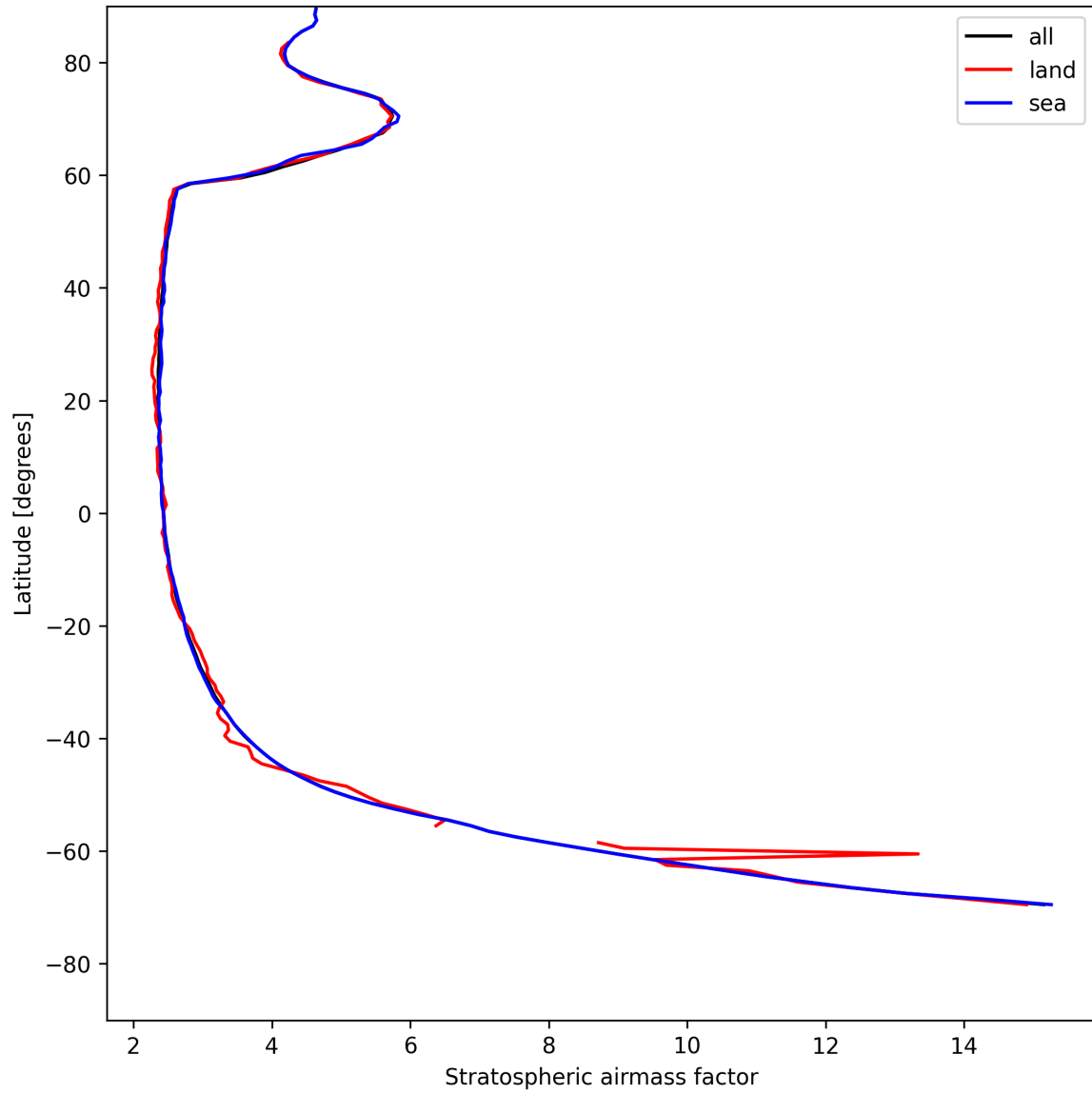
Figure 25: Zonal average of “Stratospheric air mass factor” for 2025-07-31 to 2025-08-01.
