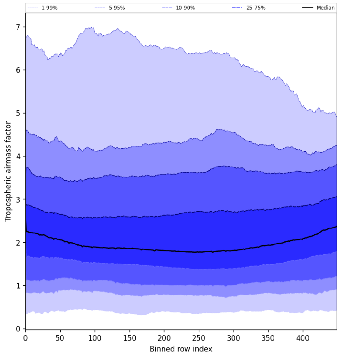
Figure 46: Along track statistics of “Tropospheric air mass factor” for 2025-07-31 to 2025-08-01
