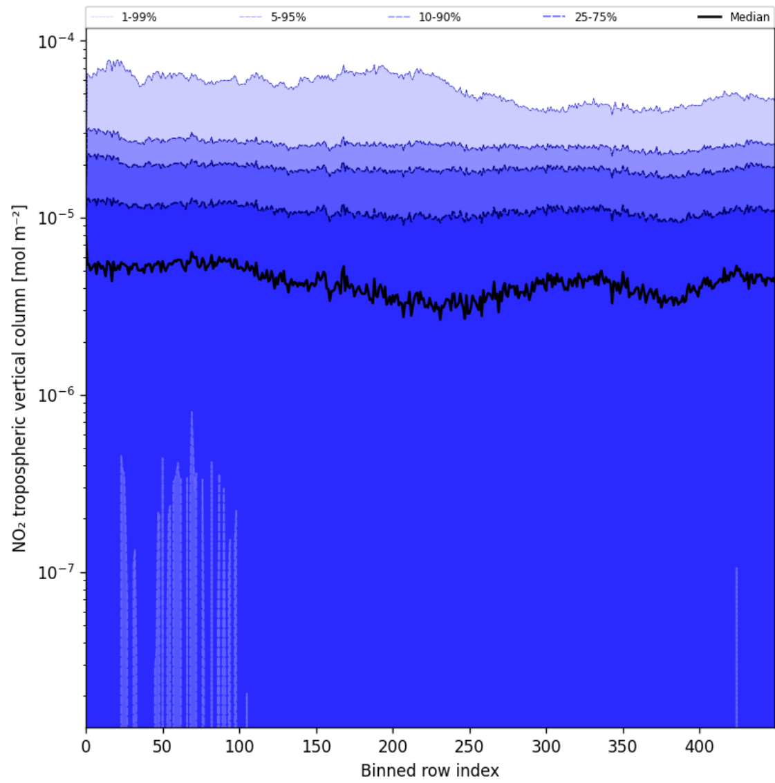
Figure 44: Along track statistics of “NO 2 tropospheric vertical column” for 2025-07-31 to 2025-08-01
