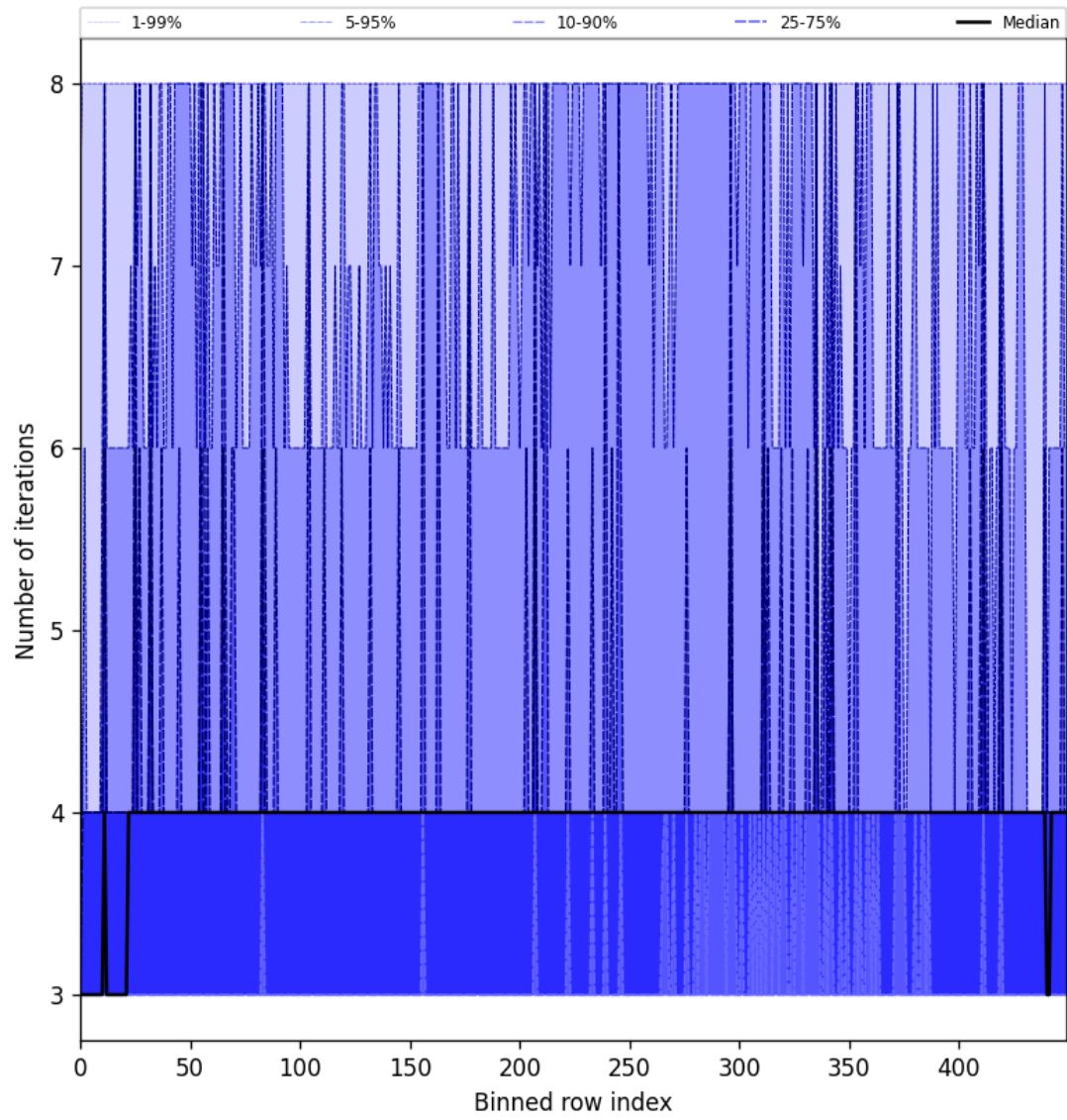
Figure 49: Along track statistics of “Number of iterations” for 2025-07-31 to 2025-08-01
