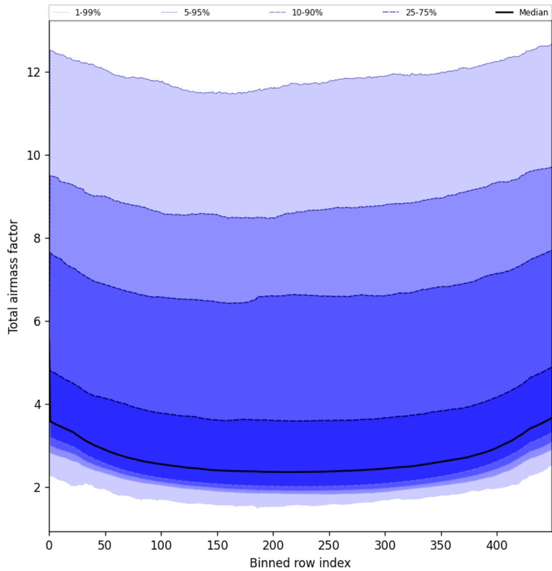
Figure 47: Along track statistics of “Total airmass factor” for 2025-07-31 to 2025-08-01
