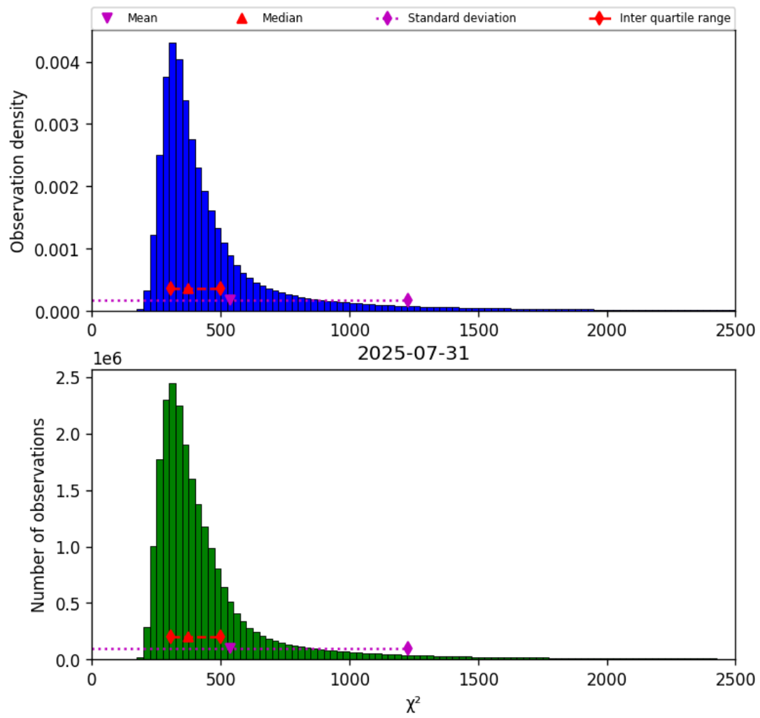
Figure 40: Histogram of “ \chi^2 ” for 2025-07-31 to 2025-08-01
