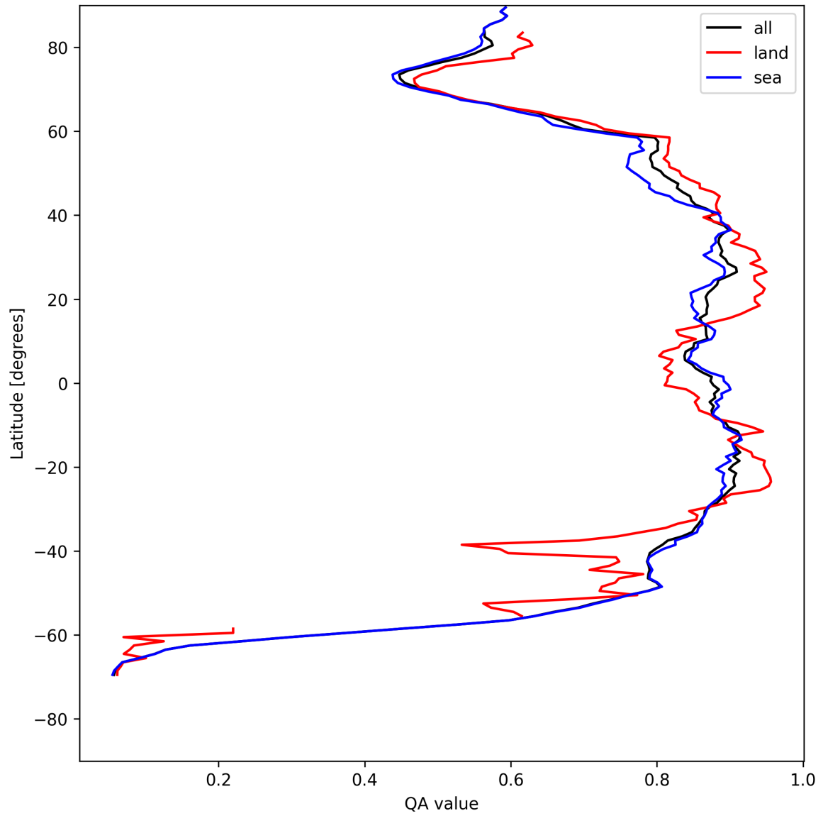
Figure 9: Zonal average of “QA value” for 2025-07-31 to 2025-08-01.
