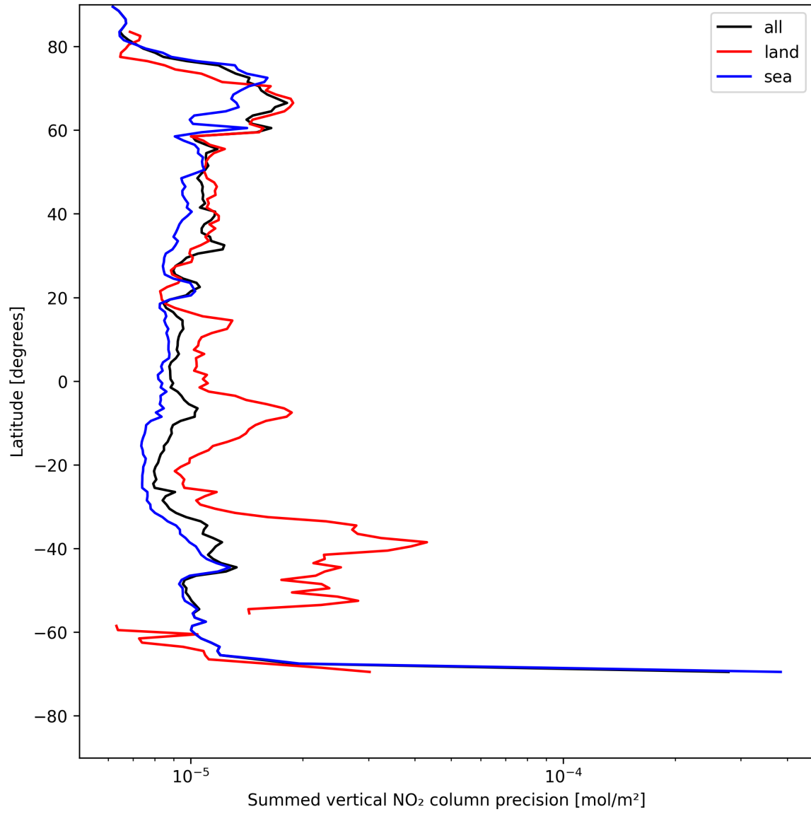
Figure 22: Zonal average of “Summed vertical NO 2 column precision” for 2025-07-31 to 2025-08-01.
