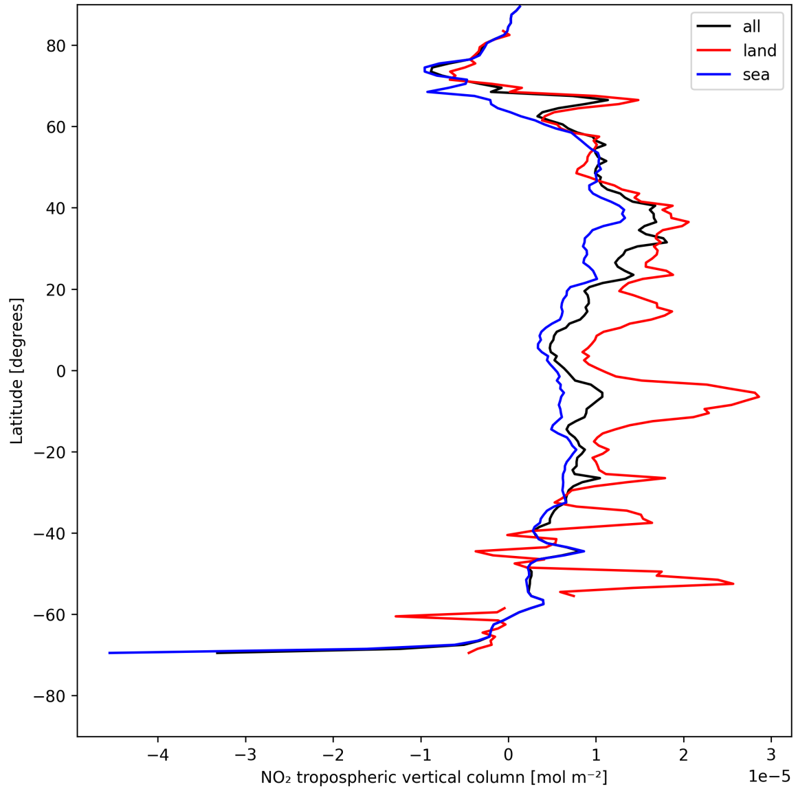
Figure 10: Zonal average of “NO 2 tropospheric vertical column” for 2025-07-31 to 2025-08-01.
