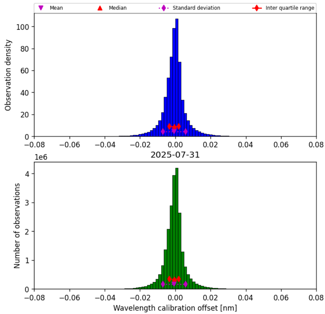
Figure 33: Histogram of “Wavelength calibration offset” for 2025-07-31 to 2025-08-01
