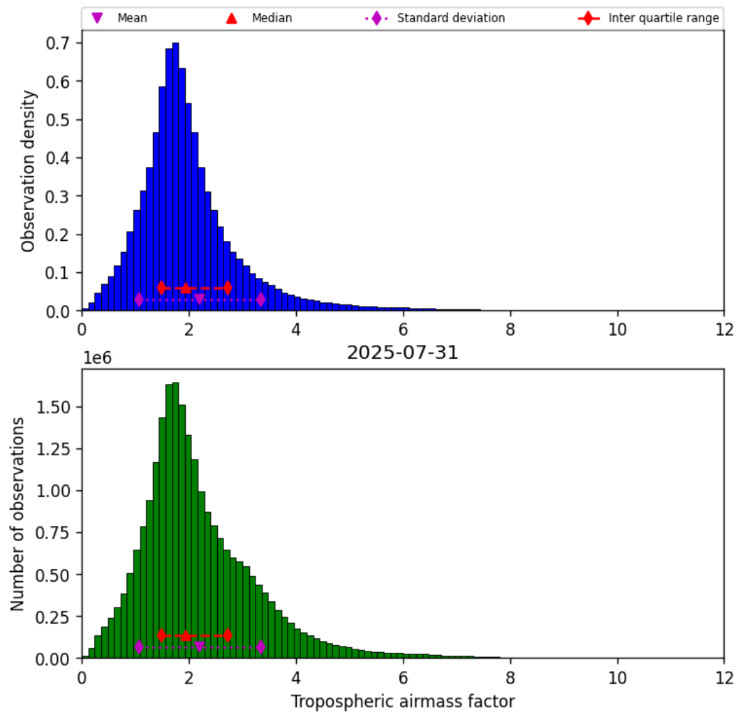
Figure 29: Histogram of “Tropospheric airmass factor” for 2025-07-31 to 2025-08-01
