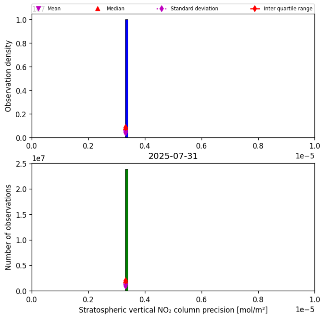
Figure 35: Histogram of “Stratospheric vertical NO 2 column precision” for 2025-07-31 to 2025-08-01
