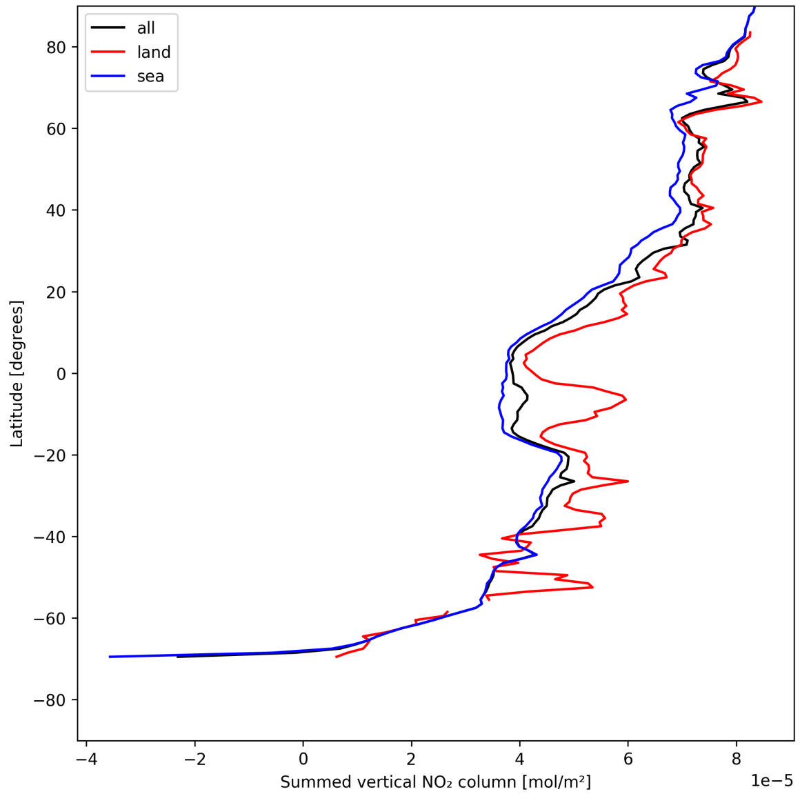
Figure 21: Zonal average of “Summed vertical NO 2 column” for 2025-07-31 to 2025-08-01.
