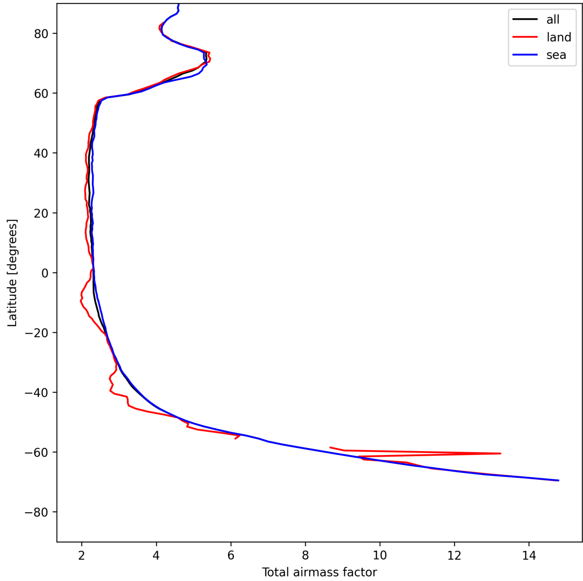
Figure 13: Zonal average of “Total airmass factor” for 2025-07-31 to 2025-08-01.
