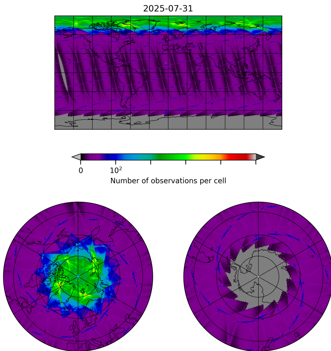
Figure 8: Map of the number of observations for 2025-07-31 to 2025-08-01
