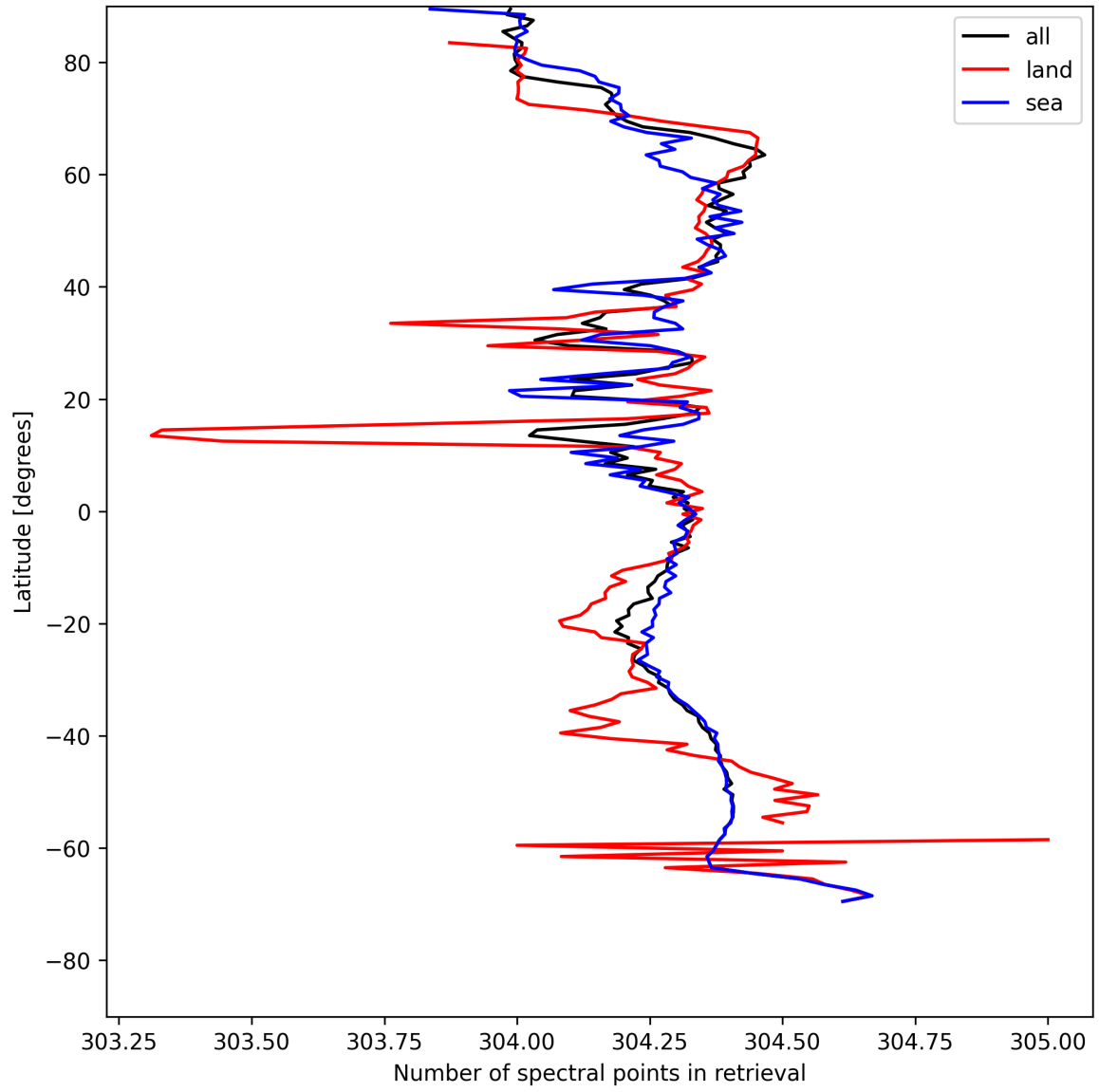
Figure 14: Zonal average of “Number of spectral points in retrieval” for 2025-07-31 to 2025-08-01.
