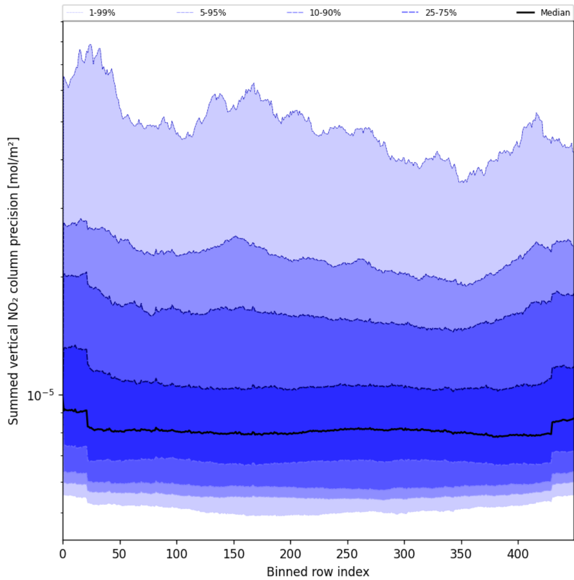
Figure 56: Along track statistics of “Summed vertical NO 2 column precision” for 2025-07-31 to 2025-08-01
