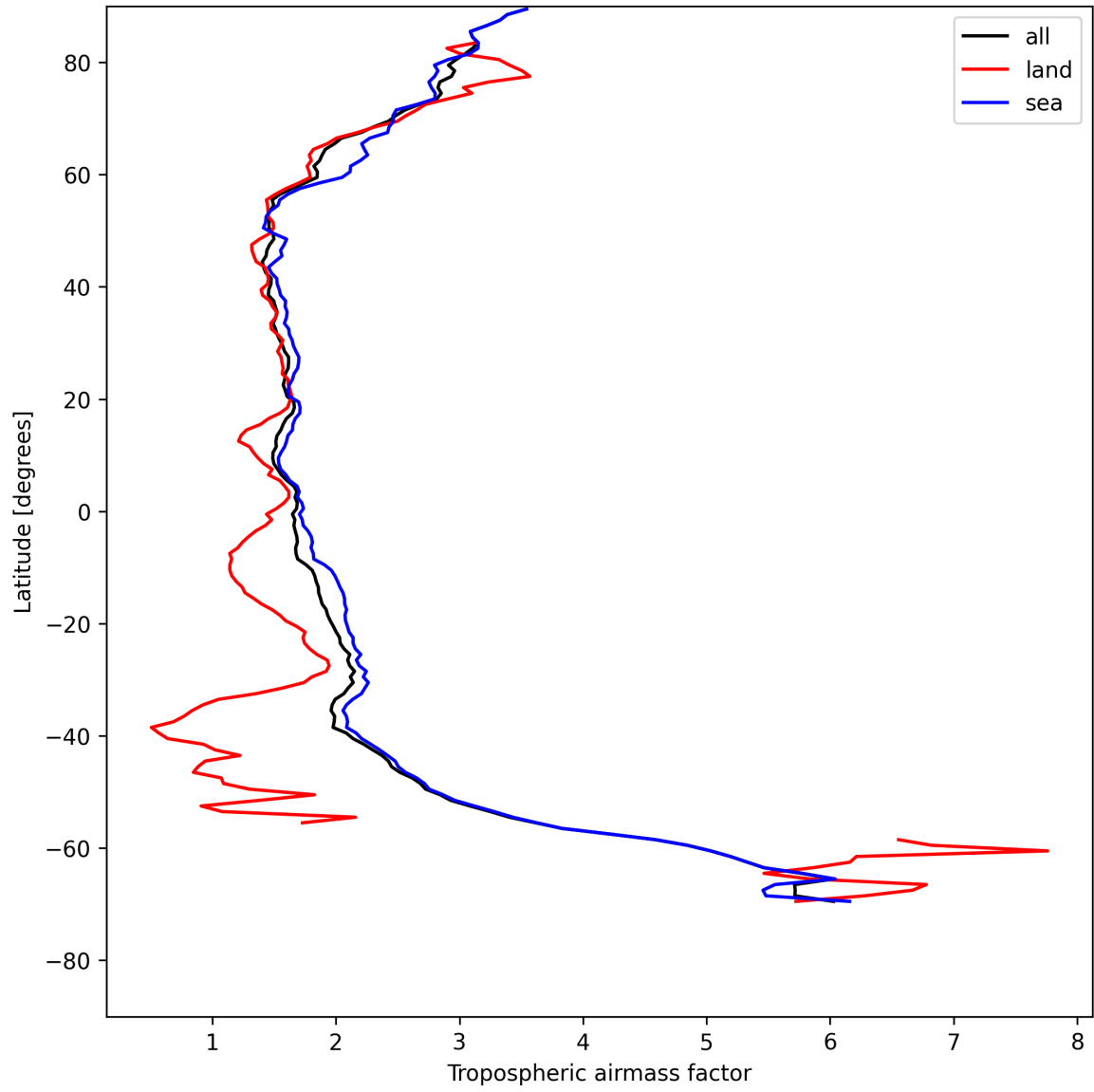
Figure 12: Zonal average of “Tropospheric airmass factor” for 2025-07-31 to 2025-08-01.
