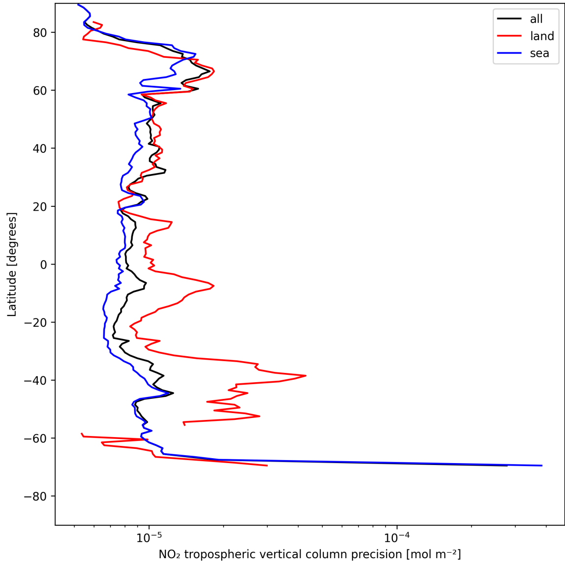
Figure 11: Zonal average of “NO 2 tropospheric vertical column precision” for 2025-07-31 to 2025-08-01.
