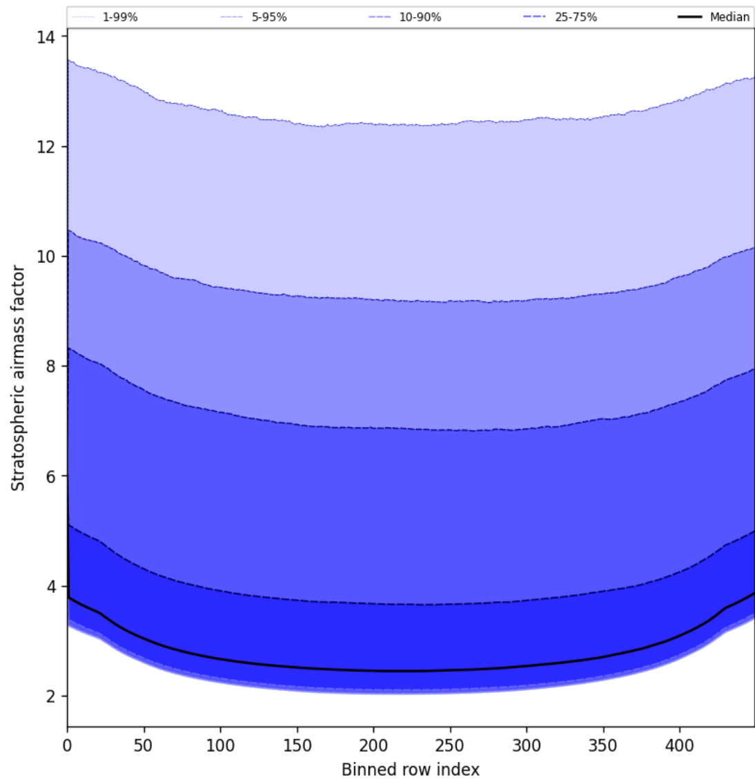
Figure 59: Along track statistics of “Stratospheric airmass factor” for 2025-07-31 to 2025-08-01
