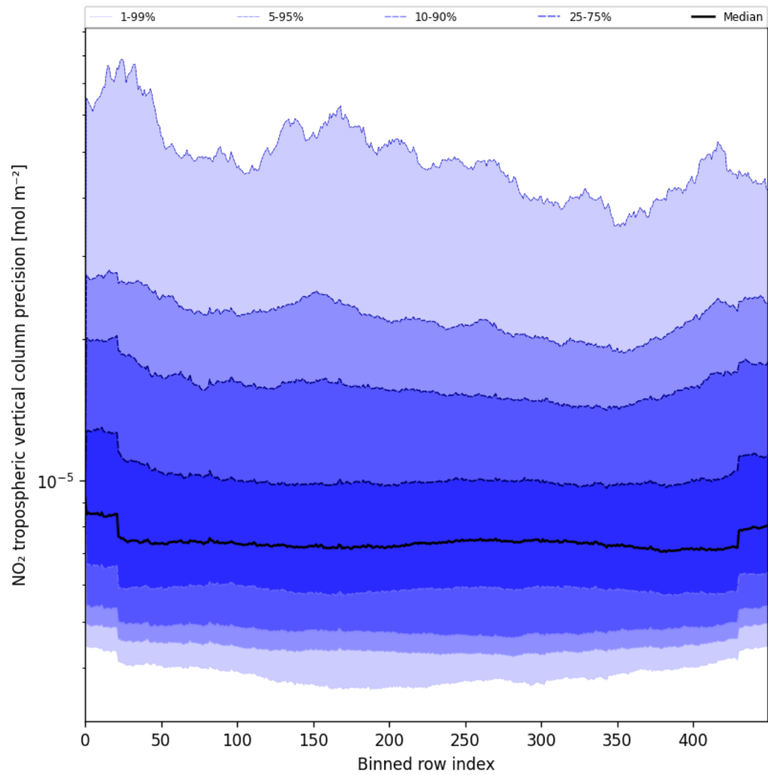
Figure 45: Along track statistics of “NO 2 tropospheric vertical column precision” for 2025-07-31 to 2025-08-01
