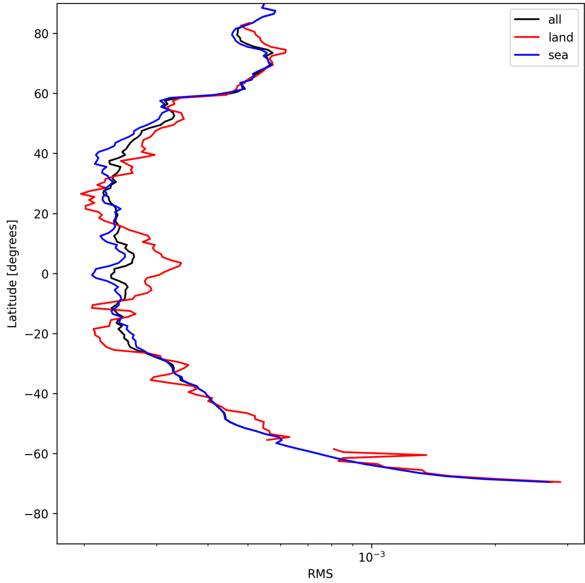
Figure 24: Zonal average of “RMS” for 2025-07-31 to 2025-08-01.
