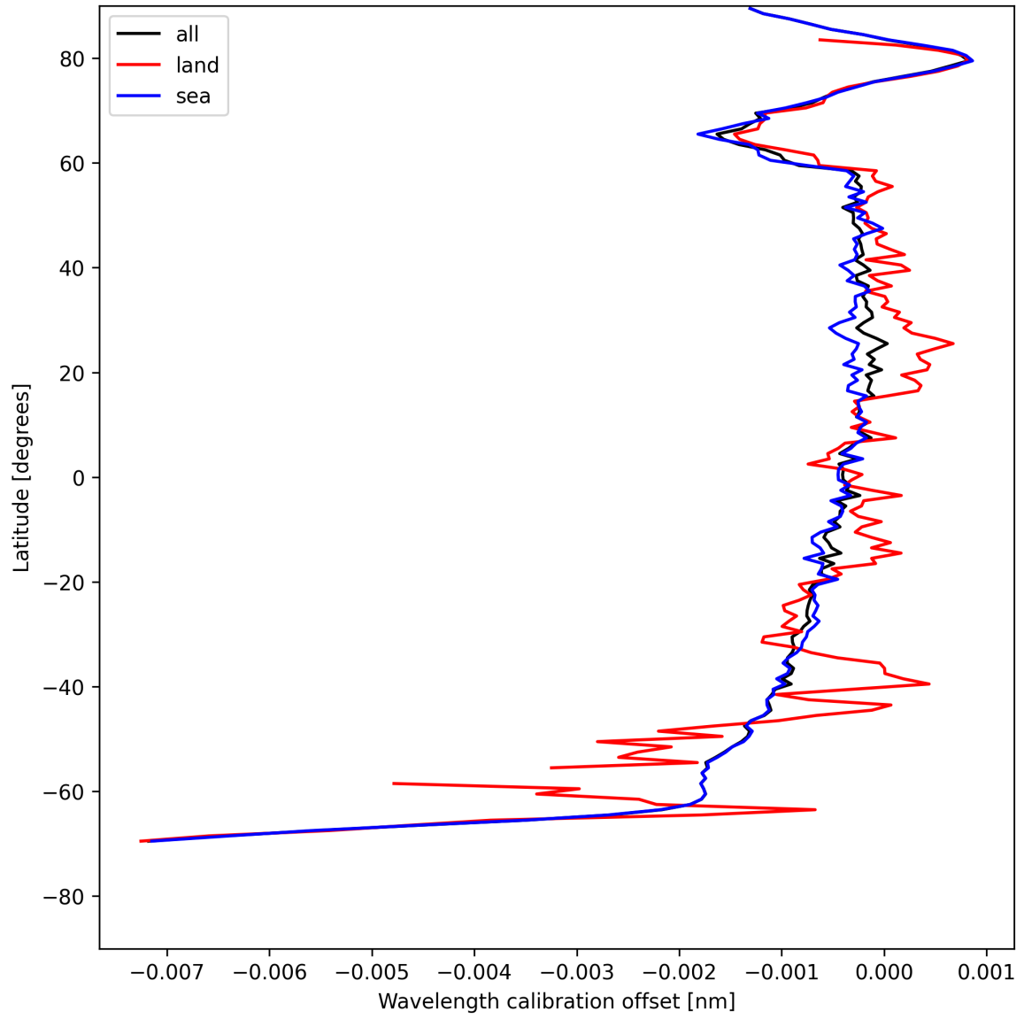
Figure 16: Zonal average of “Wavelength calibration offset” for 2025-07-31 to 2025-08-01.
