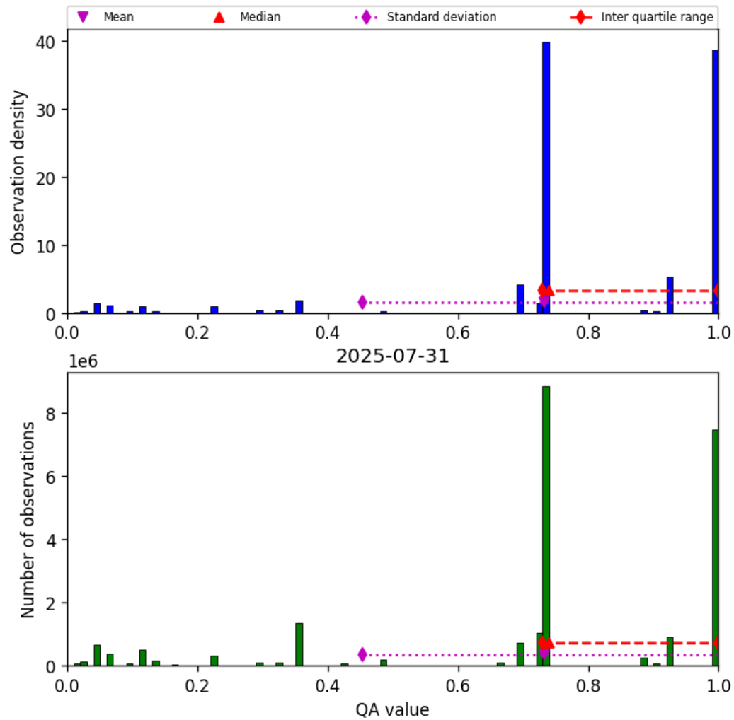
Figure 26: Histogram of “QA value” for 2025-07-31 to 2025-08-01
