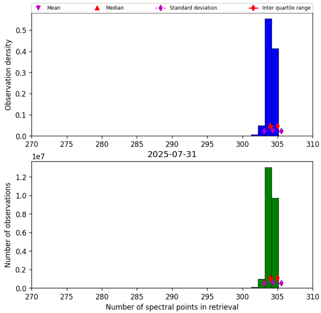
Figure 31: Histogram of “Number of spectral points in retrieval” for 2025-07-31 to 2025-08-01
