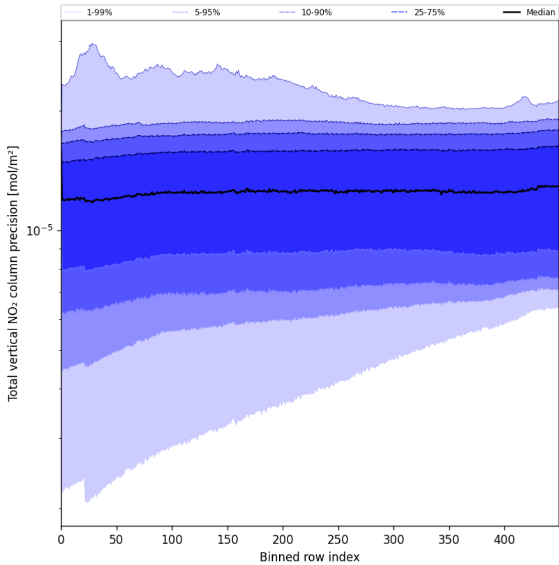
Figure 54: Along track statistics of “Total vertical NO 2 column precision” for 2025-07-31 to 2025-08-01
