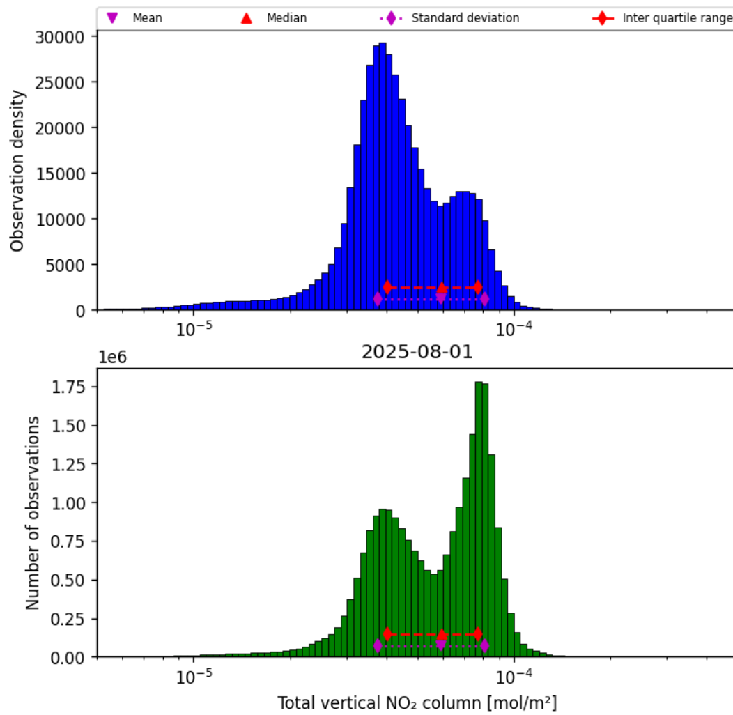
Figure 36: Histogram of "Total vertical NO 2 column" for 2025-08-01 to 2025-08-01
