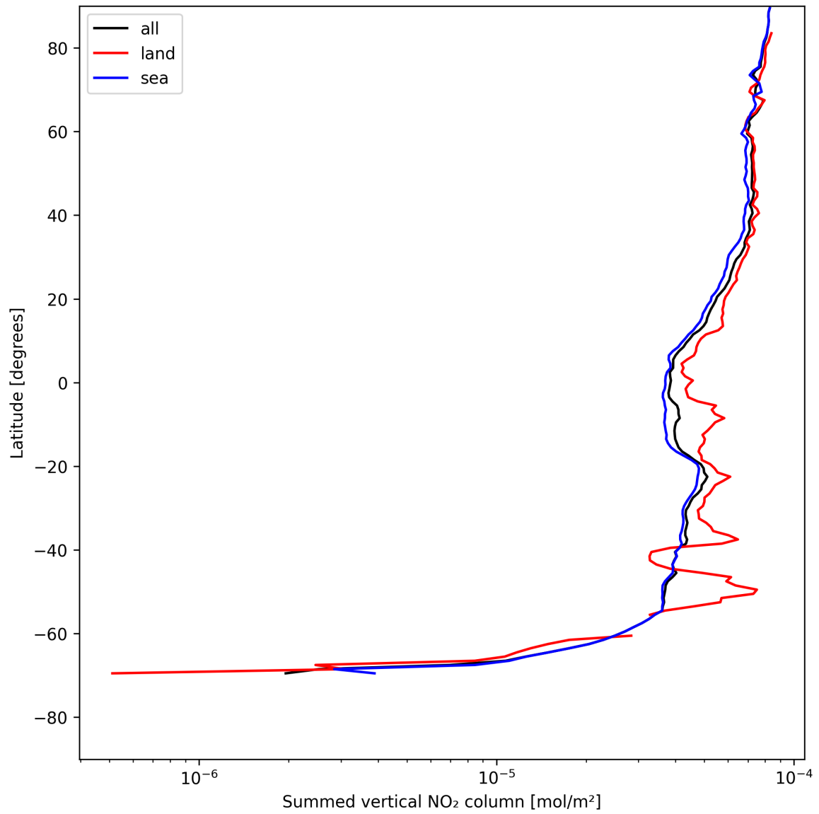
Figure 21: Zonal average of “Summed vertical NO 2 column” for 2025-08-01 to 2025-08-01.
