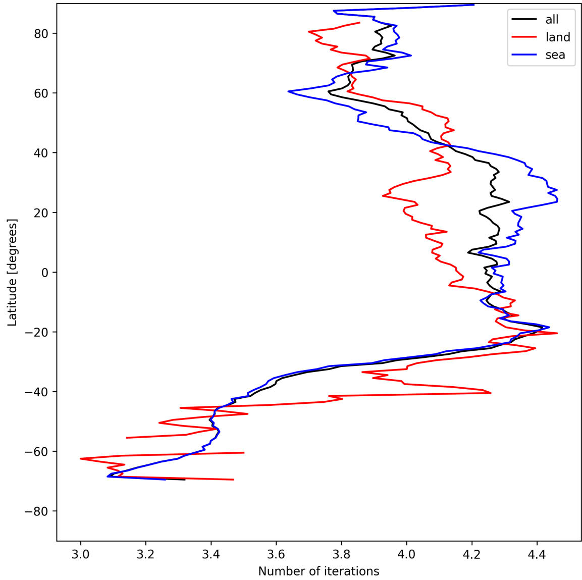
Figure 15: Zonal average of “Number of iterations” for 2025-08-01 to 2025-08-01.
