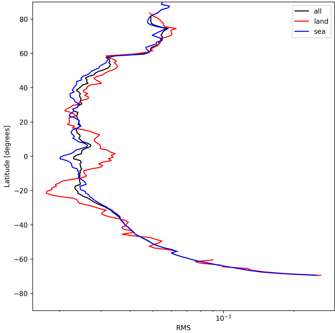
Figure 24: Zonal average of “RMS” for 2025-08-01 to 2025-08-01.
