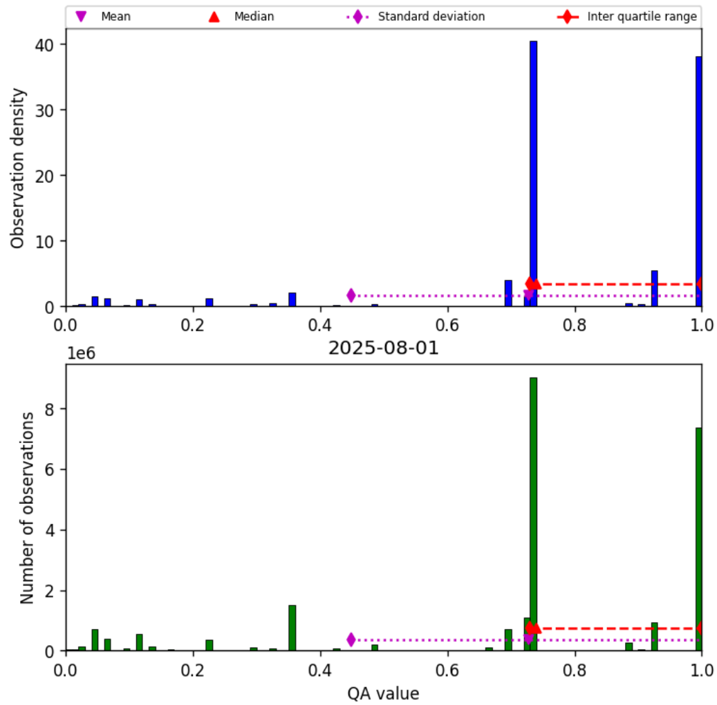
Figure 26: Histogram of “QA value” for 2025-08-01 to 2025-08-01
