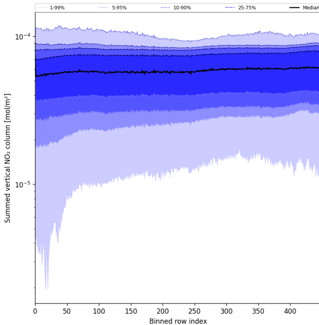
Figure 55: Along track statistics of “Summed vertical NO 2 column” for 2025-08-01 to 2025-08-01
