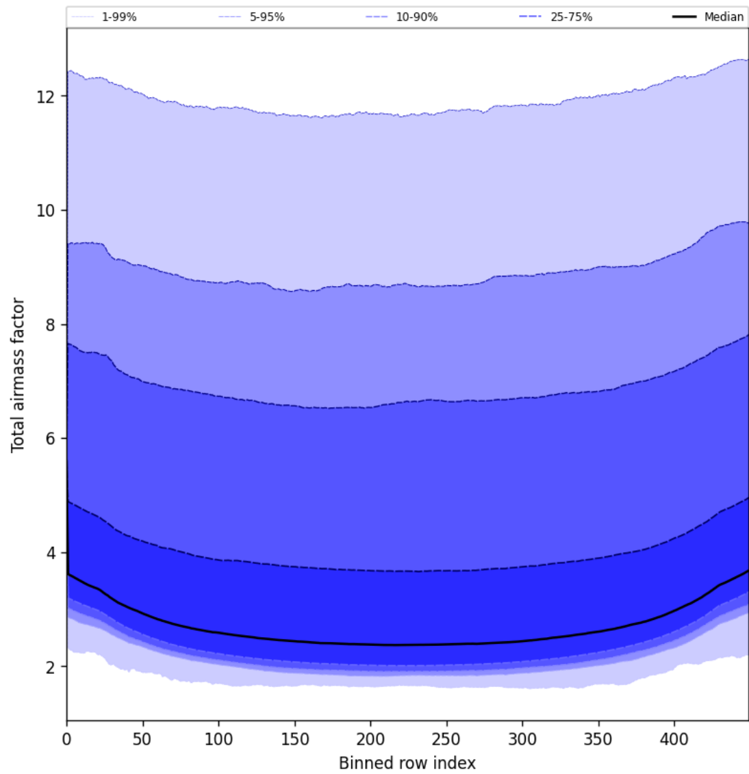
Figure 47: Along track statistics of “Total airmass factor” for 2025-08-01 to 2025-08-01
