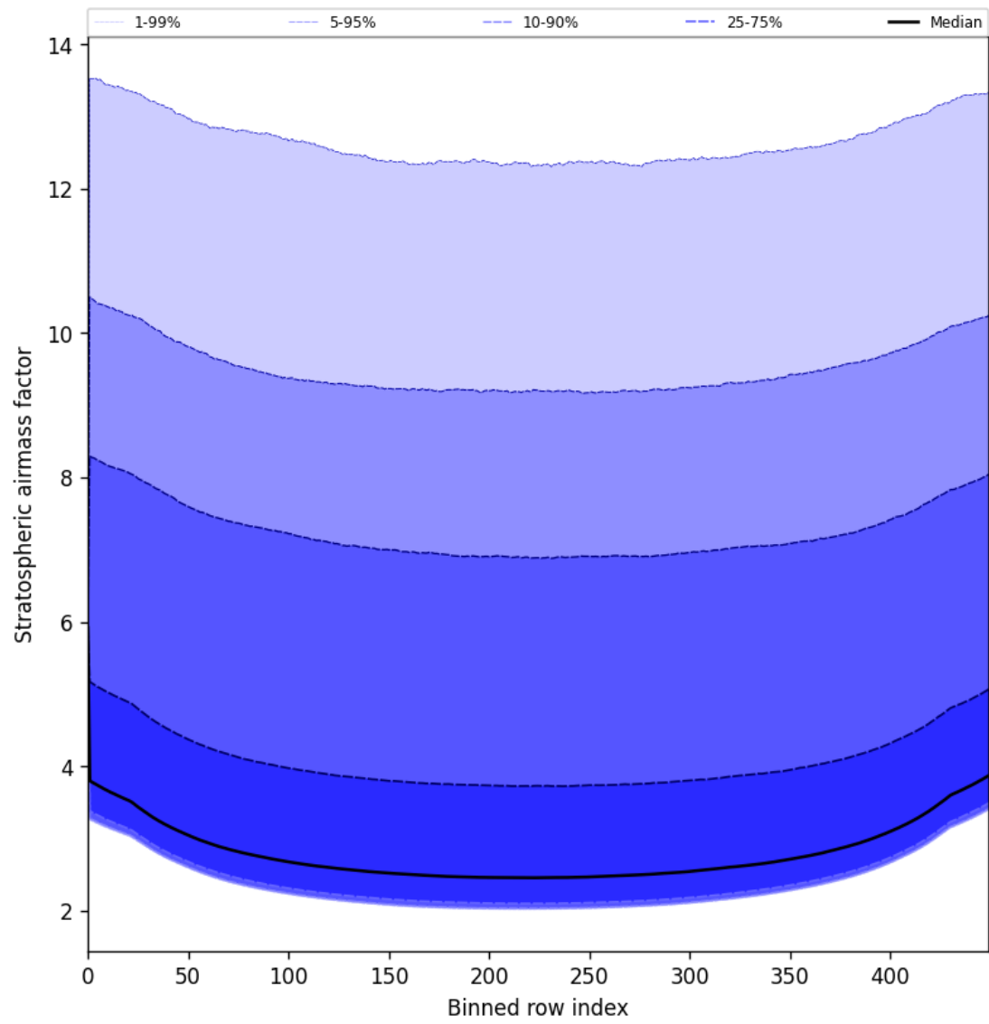
Figure 59: Along track statistics of “Stratospheric airmass factor” for 2025-08-01 to 2025-08-01
