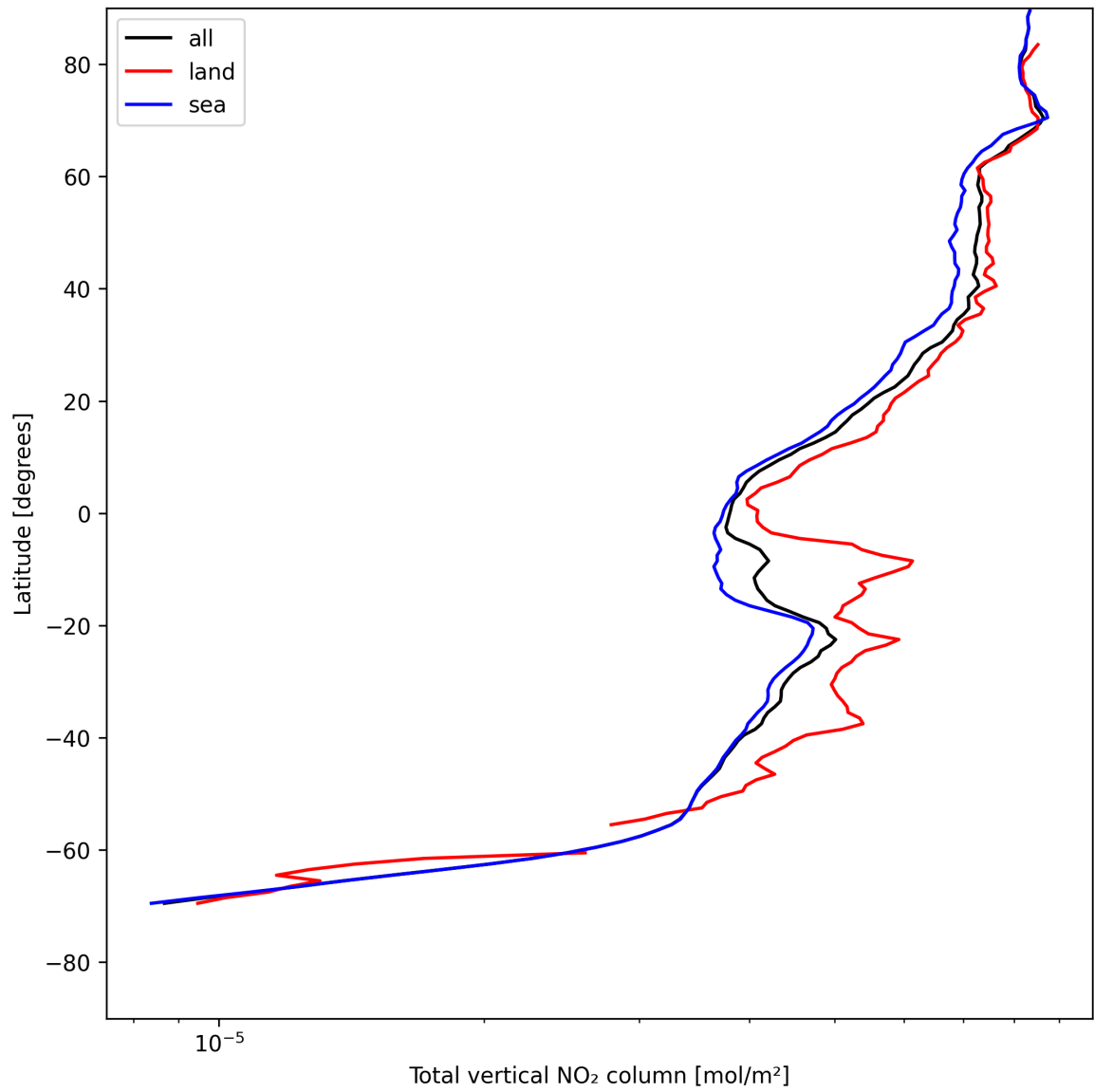
Figure 19: Zonal average of “Total vertical NO 2 column” for 2025-08-01 to 2025-08-01.
