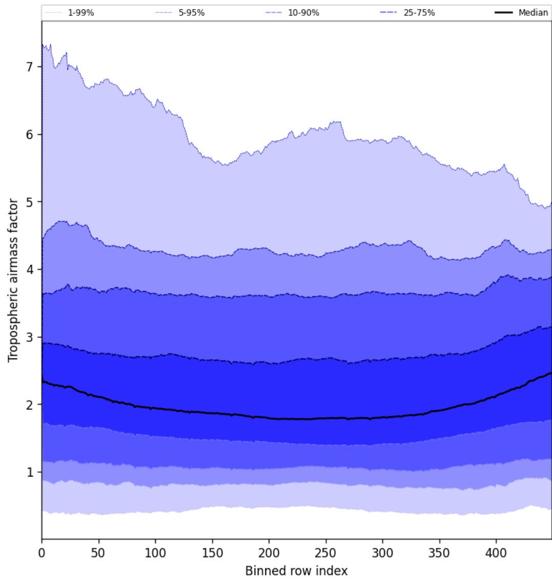
Figure 46: Along track statistics of “Tropospheric airmass factor” for 2025-08-01 to 2025-08-01
