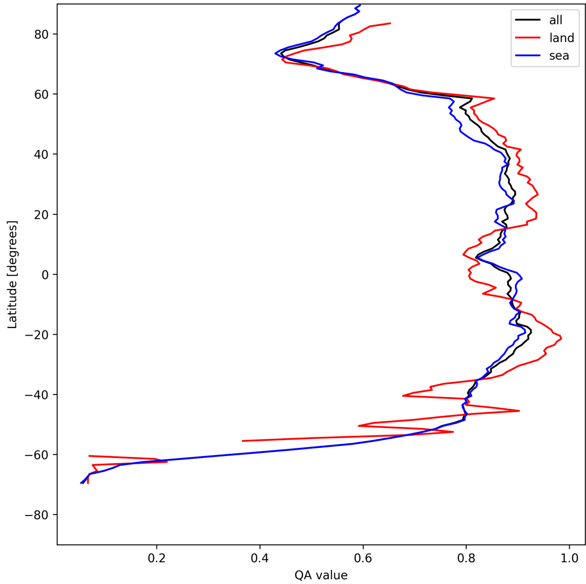
Figure 9: Zonal average of “QA value” for 2025-08-01 to 2025-08-01.
