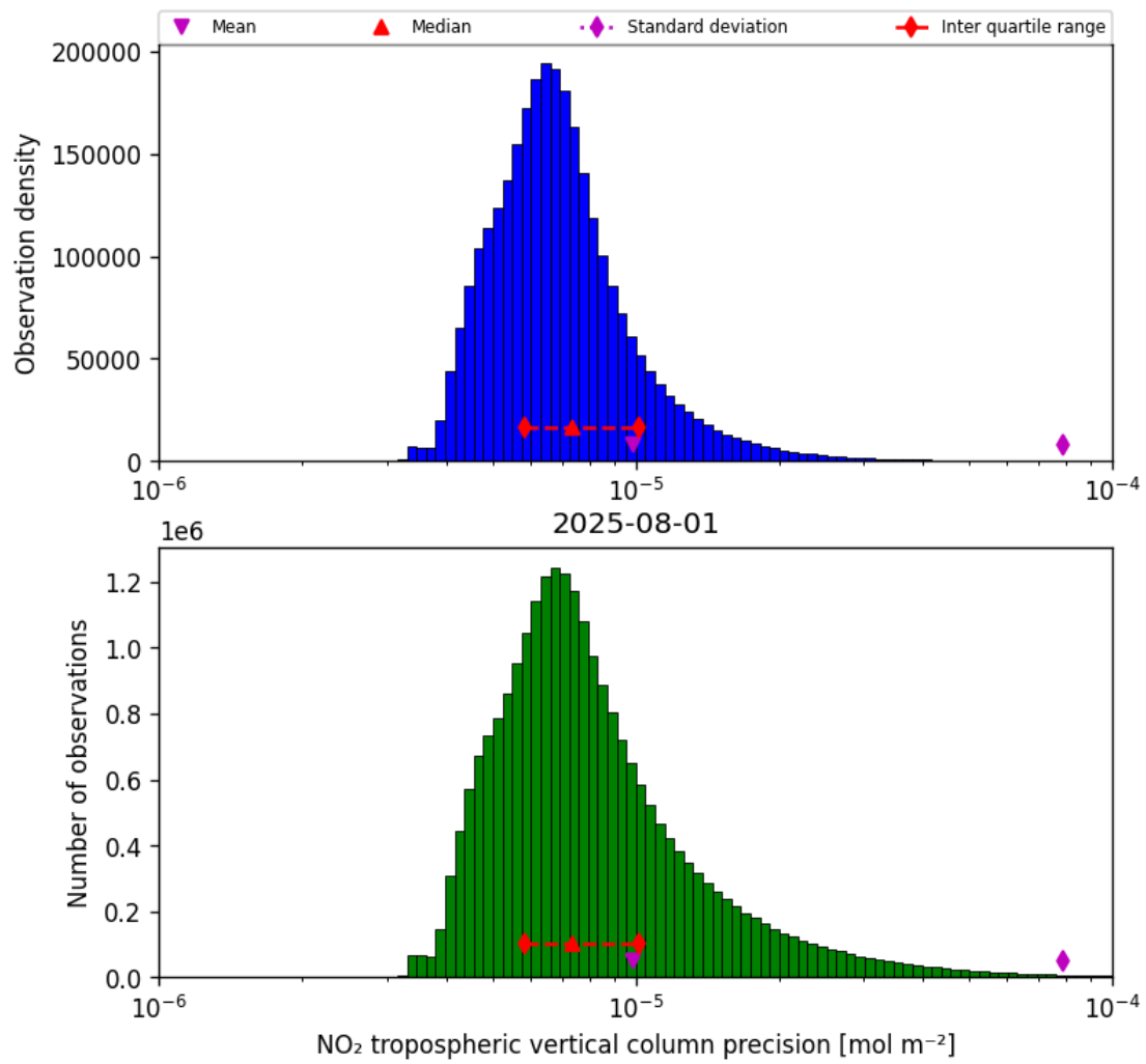
Figure 28: Histogram of “NO 2 tropospheric vertical column precision” for 2025-08-01 to 2025-08-01
