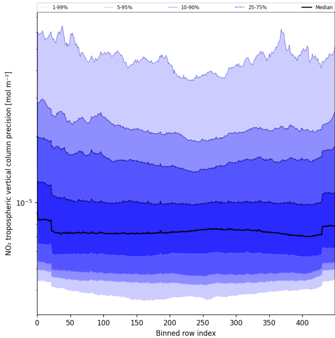
Figure 45: Along track statistics of “NO 2 tropospheric vertical column precision” for 2025-08-01 to 2025-08-01
