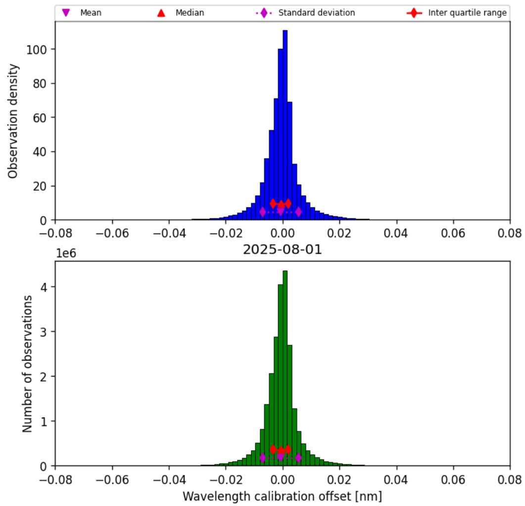
Figure 33: Histogram of “Wavelength calibration offset” for 2025-08-01 to 2025-08-01
