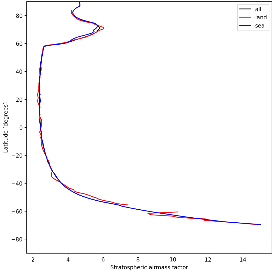
Figure 25: Zonal average of “Stratospheric airmass factor” for 2025-08-01 to 2025-08-01.
