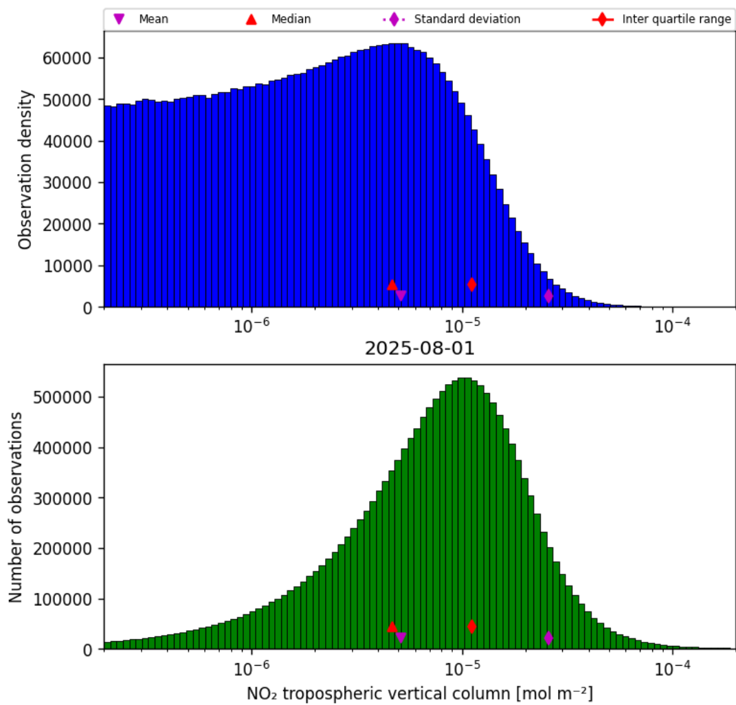
Figure 27: Histogram of “NO 2 tropospheric vertical column” for 2025-08-01 to 2025-08-01
