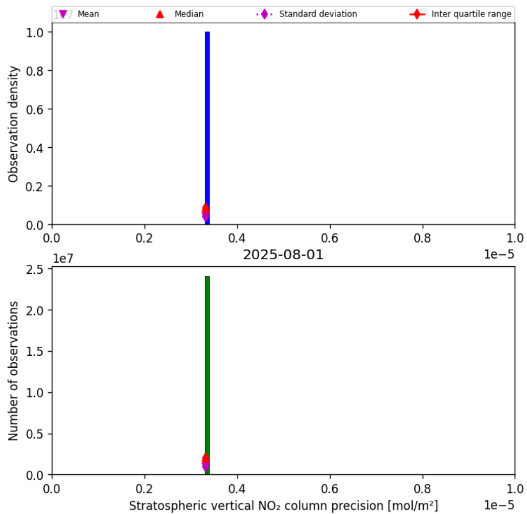
Figure 35: Histogram of “Stratospheric vertical NO 2 column precision” for 2025-08-01 to 2025-08-01
