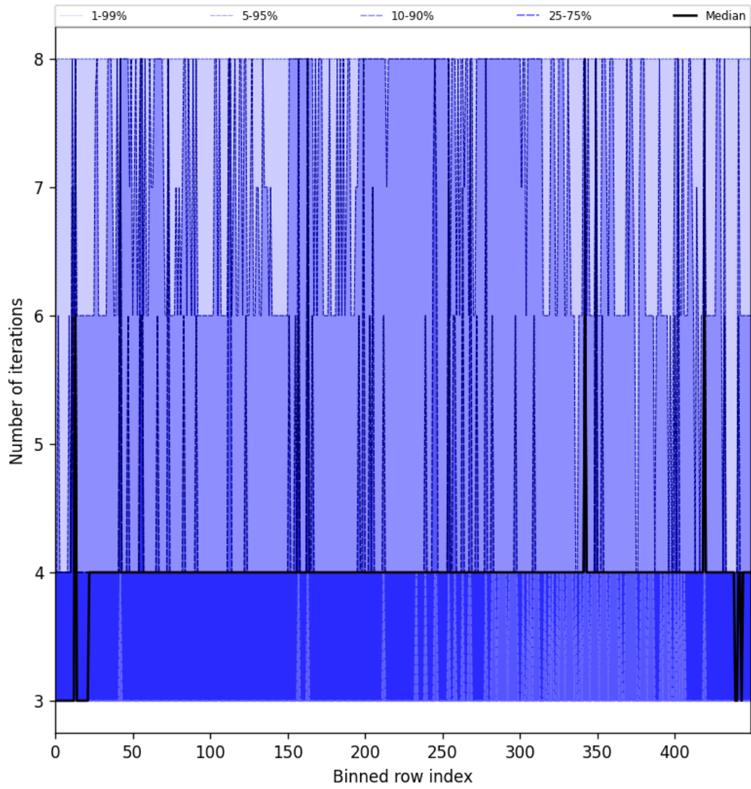
Figure 49: Along track statistics of “Number of iterations” for 2025-08-01 to 2025-08-01
