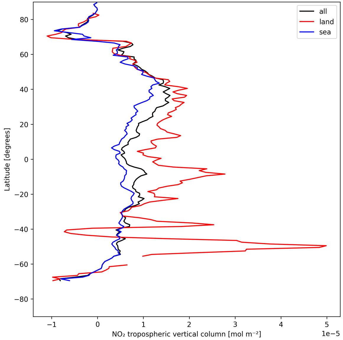
Figure 10: Zonal average of “NO 2 tropospheric vertical column” for 2025-08-01 to 2025-08-01.
