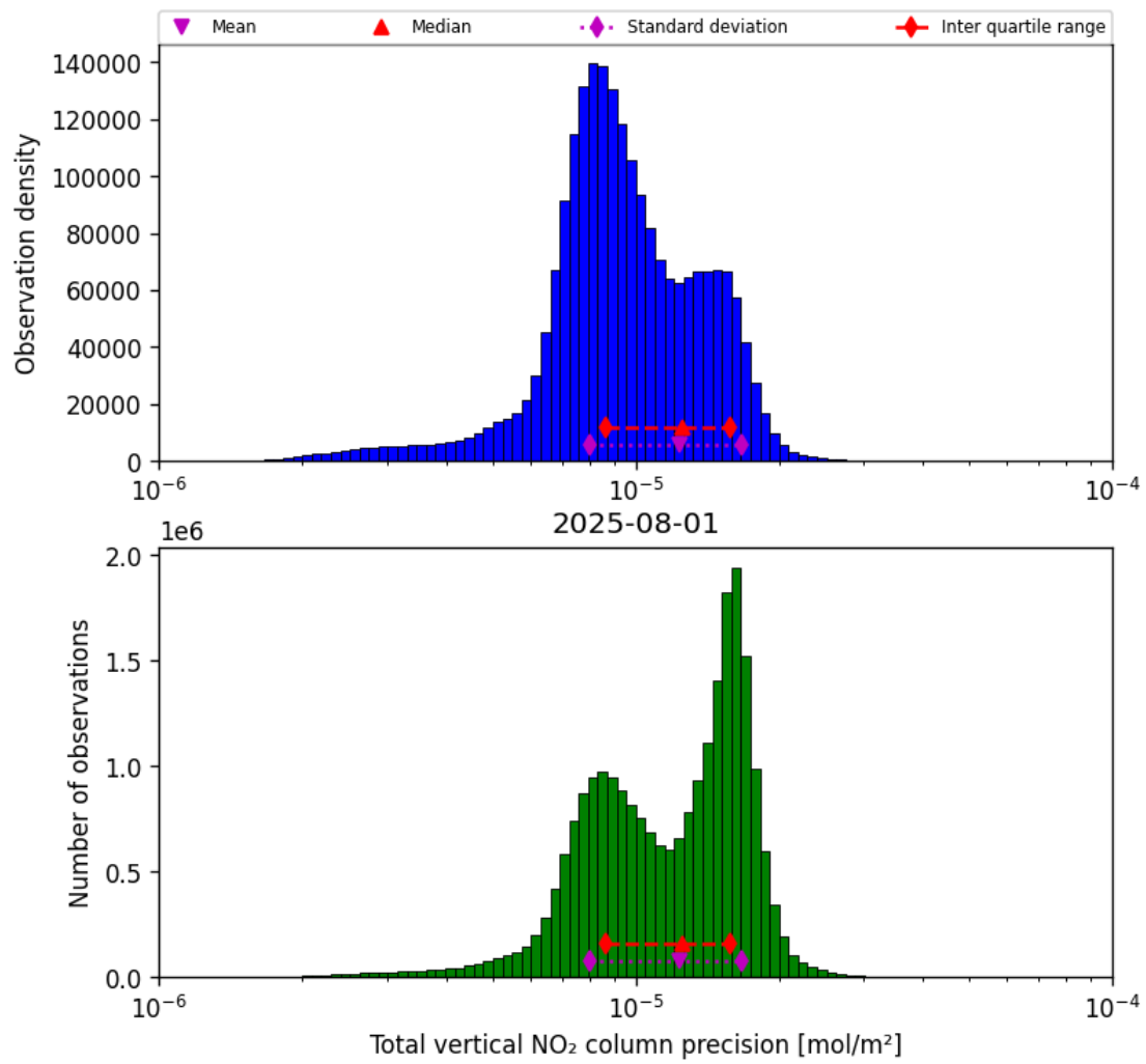
Figure 37: Histogram of “Total vertical NO 2 column precision” for 2025-08-01 to 2025-08-01
