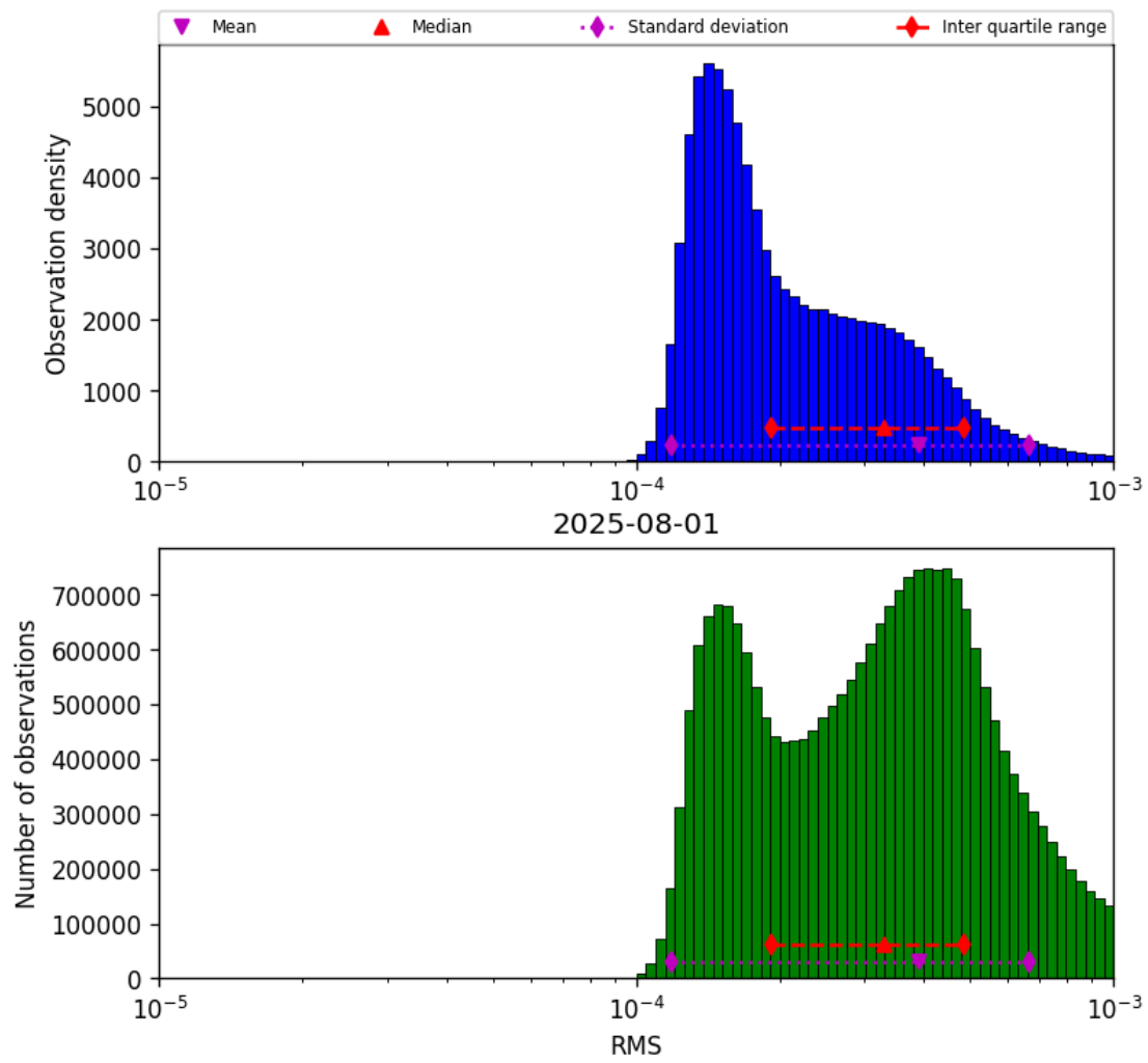
Figure 41: Histogram of “RMS” for 2025-08-01 to 2025-08-01
