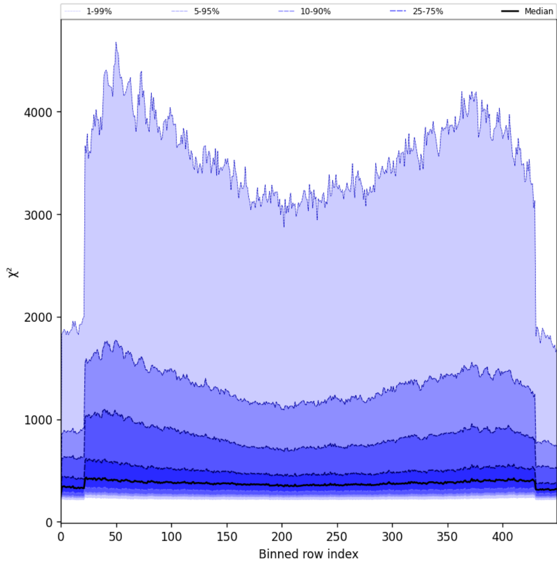
Figure 57: Along track statistics of “ \chi^2 ” for 2025-08-01 to 2025-08-01
