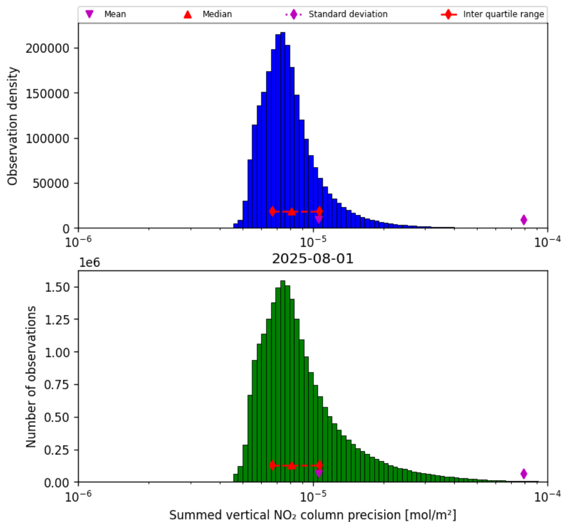
Figure 39: Histogram of "Summed vertical NO 2 column precision" for 2025-08-01 to 2025-08-01
