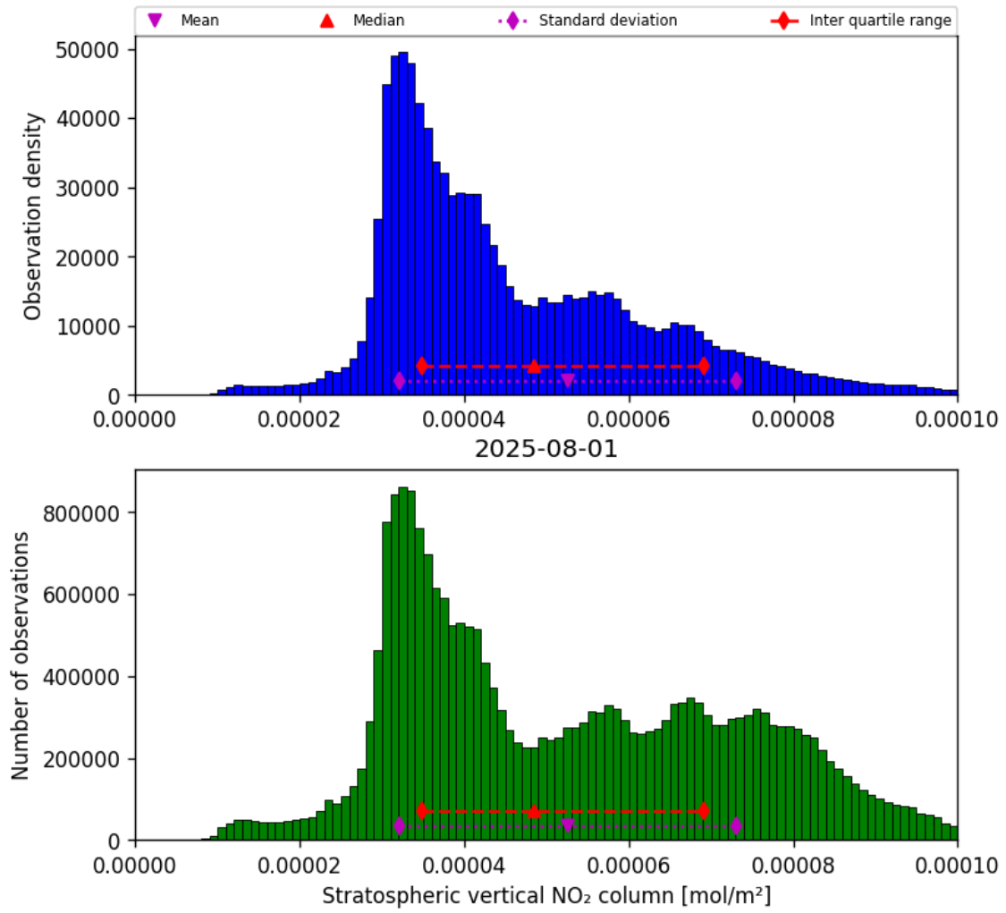
Figure 34: Histogram of “Stratospheric vertical NO 2 column” for 2025-08-01 to 2025-08-01
