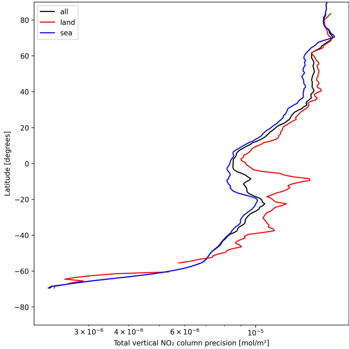
Figure 20: Zonal average of “Total vertical NO 2 column precision” for 2025-08-01 to 2025-08-01.
