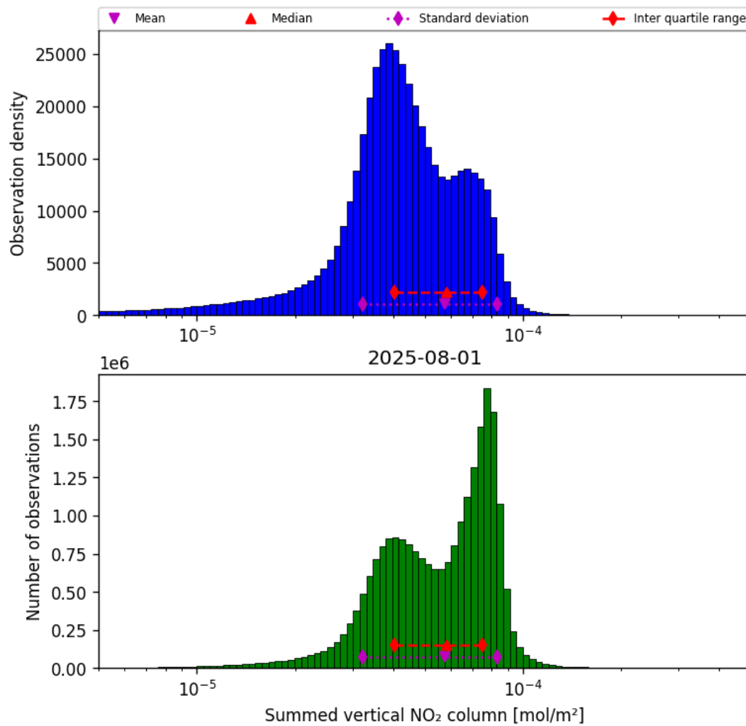
Figure 38: Histogram of "Summed vertical NO 2 column" for 2025-08-01 to 2025-08-01
