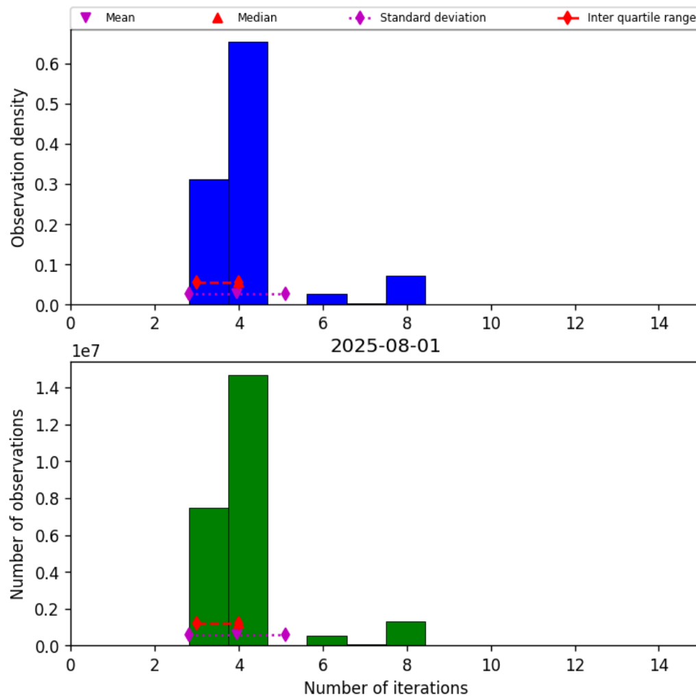
Figure 32: Histogram of “Number of iterations” for 2025-08-01 to 2025-08-01
