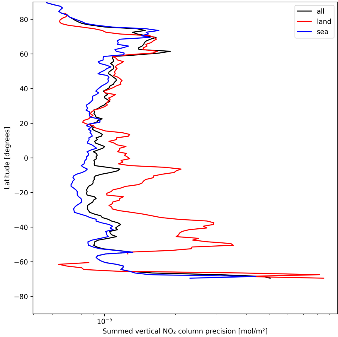
Figure 22: Zonal average of “Summed vertical NO 2 column precision” for 2025-08-01 to 2025-08-01.
