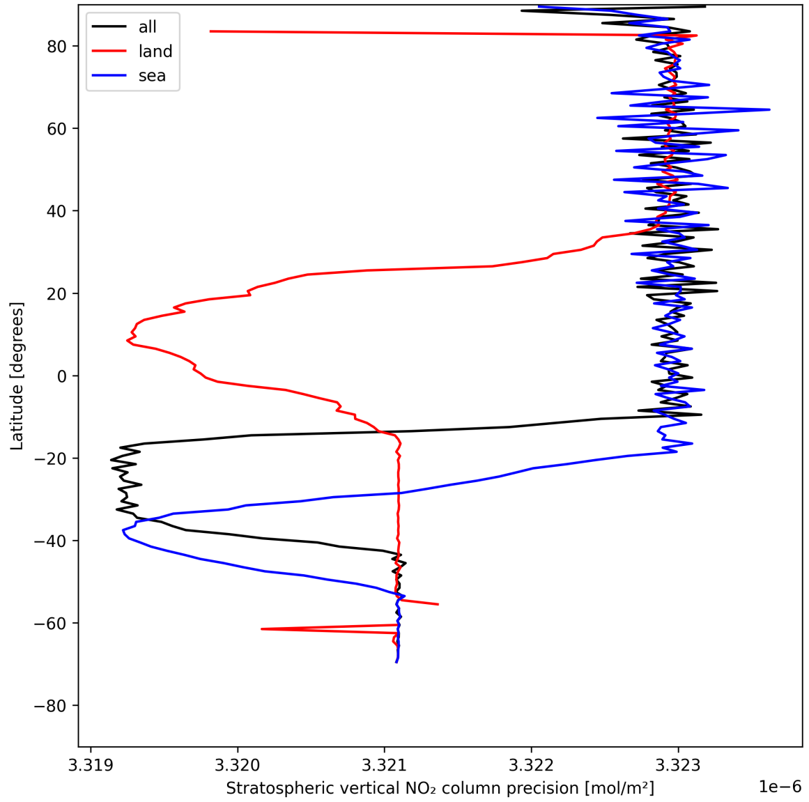
Figure 18: Zonal average of “Stratospheric vertical NO 2 column precision” for 2025-08-01 to 2025-08-01.
