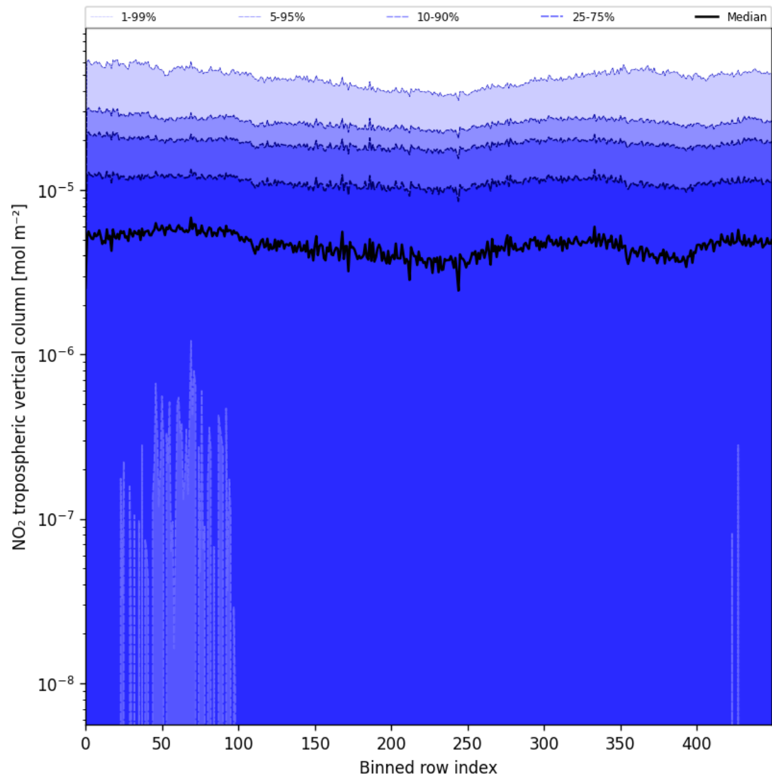
Figure 44: Along track statistics of “NO 2 tropospheric vertical column” for 2025-08-01 to 2025-08-01
