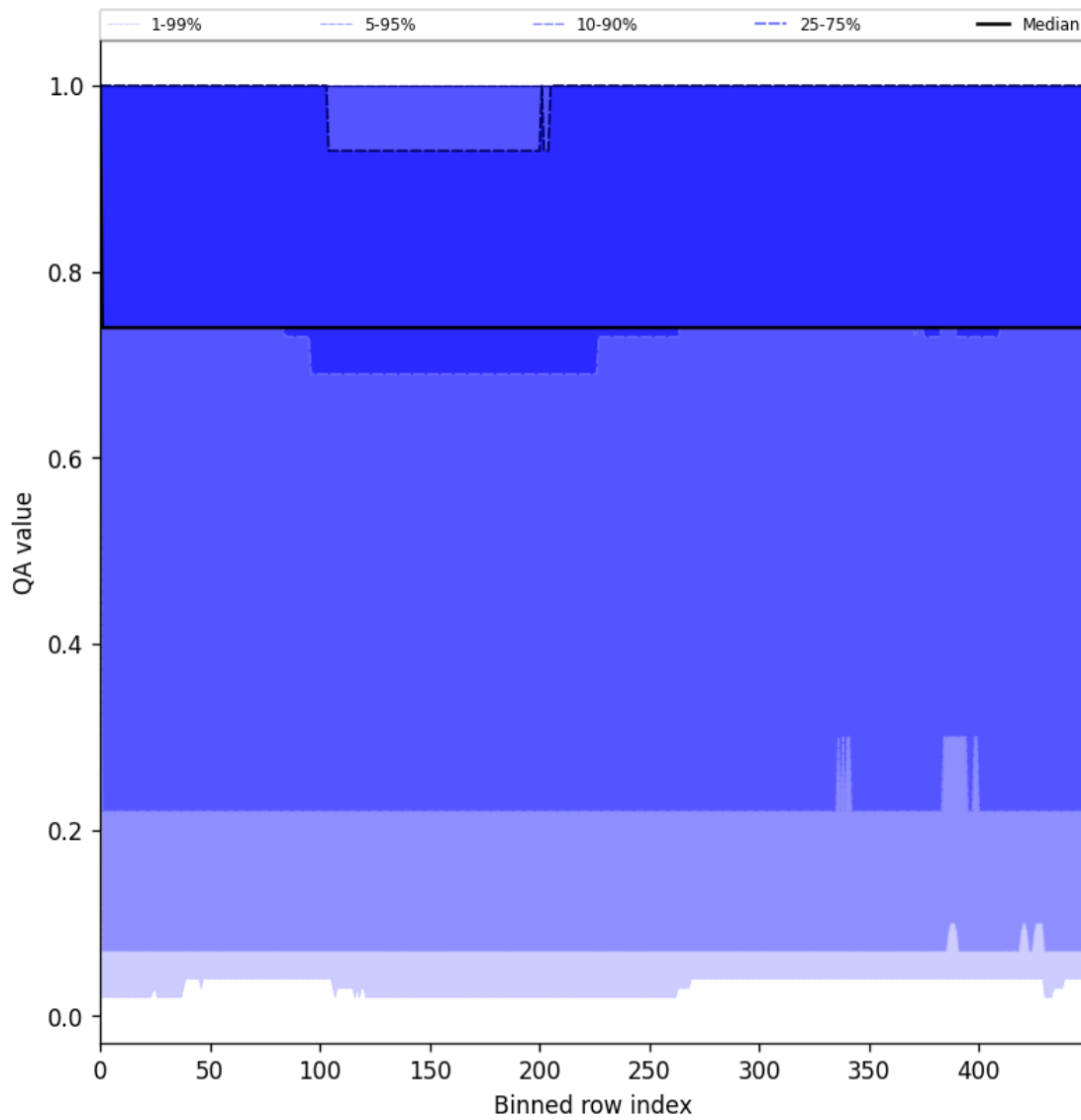
Figure 43: Along track statistics of “QA value” for 2025-08-01 to 2025-08-01
