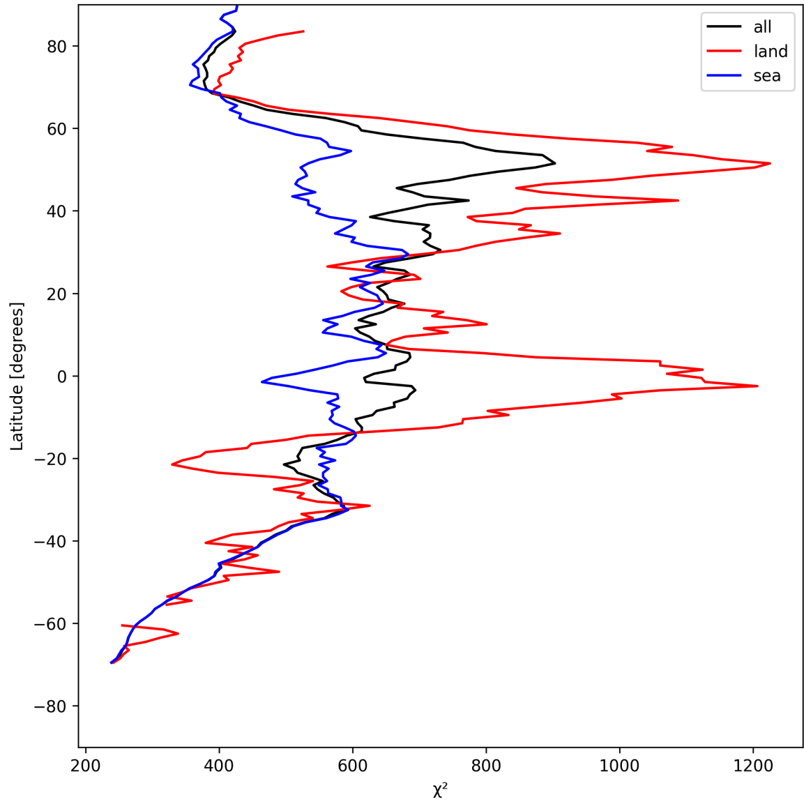
Figure 23: Zonal average of “ \chi^2 ” for 2025-08-01 to 2025-08-01.
