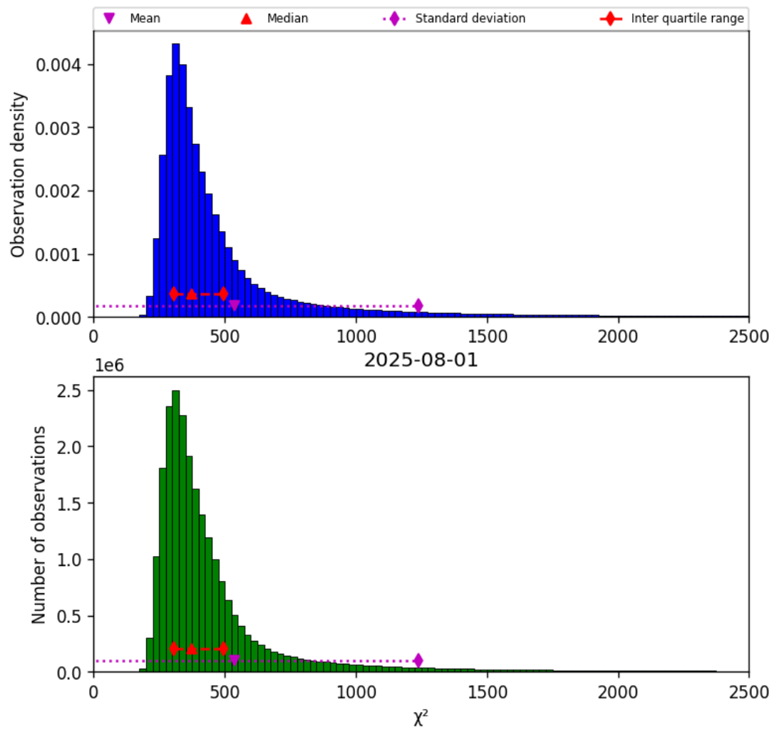
Figure 40: Histogram of “ \chi^2 ” for 2025-08-01 to 2025-08-01
