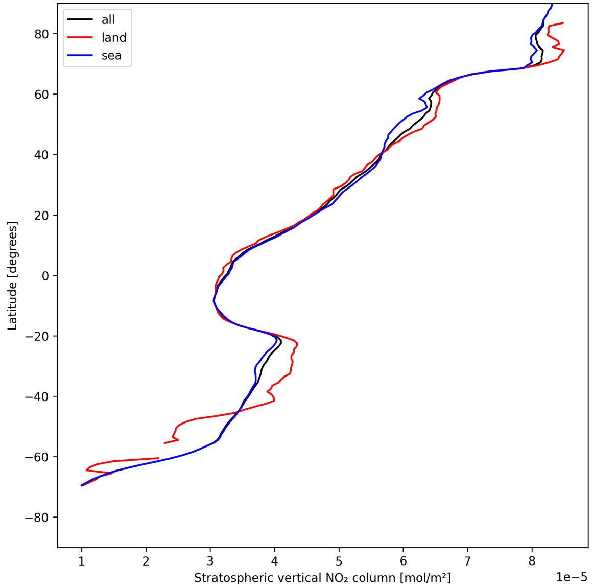
Figure 17: Zonal average of “Stratospheric vertical NO 2 column” for 2025-08-01 to 2025-08-01.
