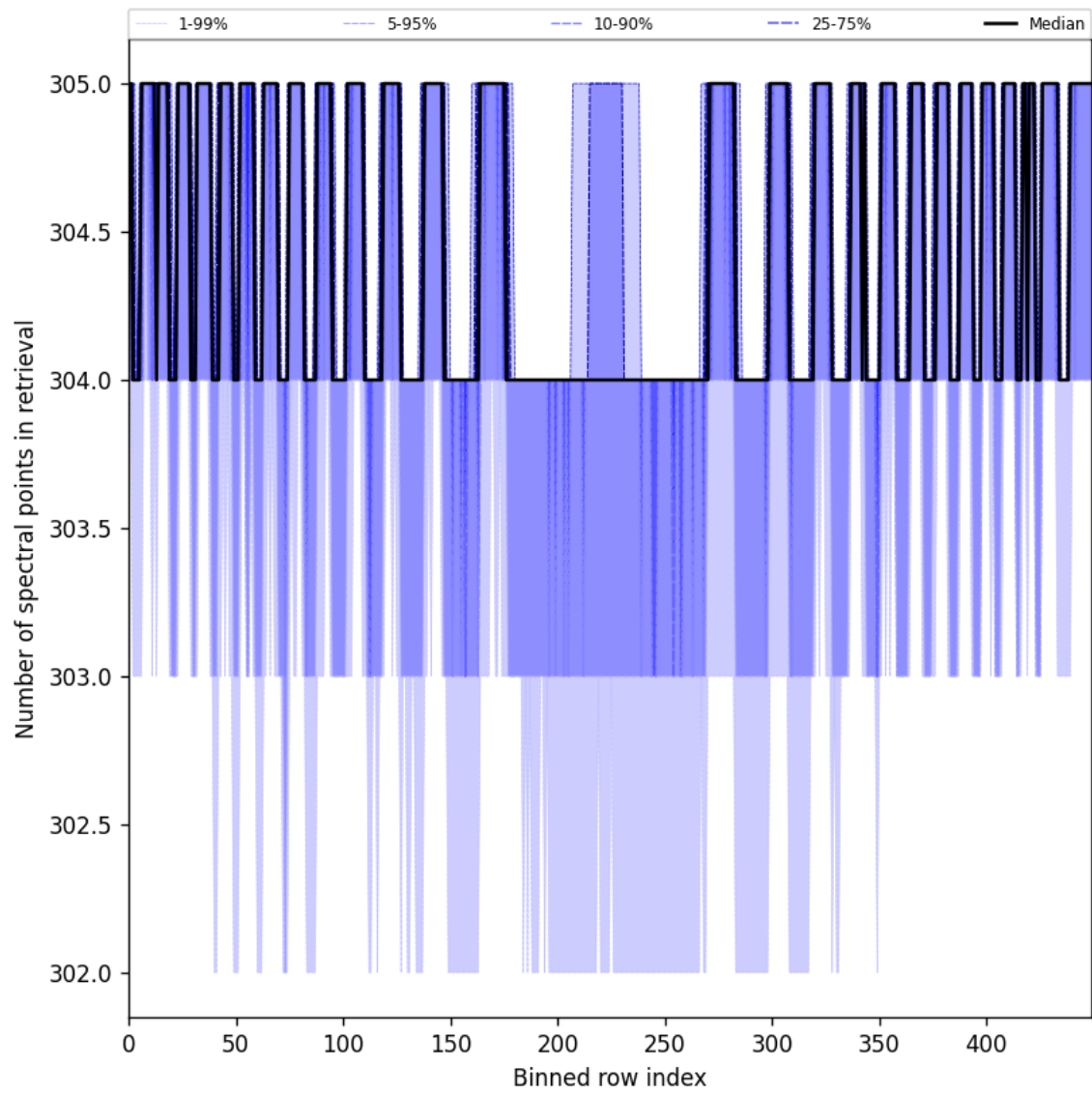
Figure 48: Along track statistics of “Number of spectral points in retrieval” for 2025-08-01 to 2025-08-01
