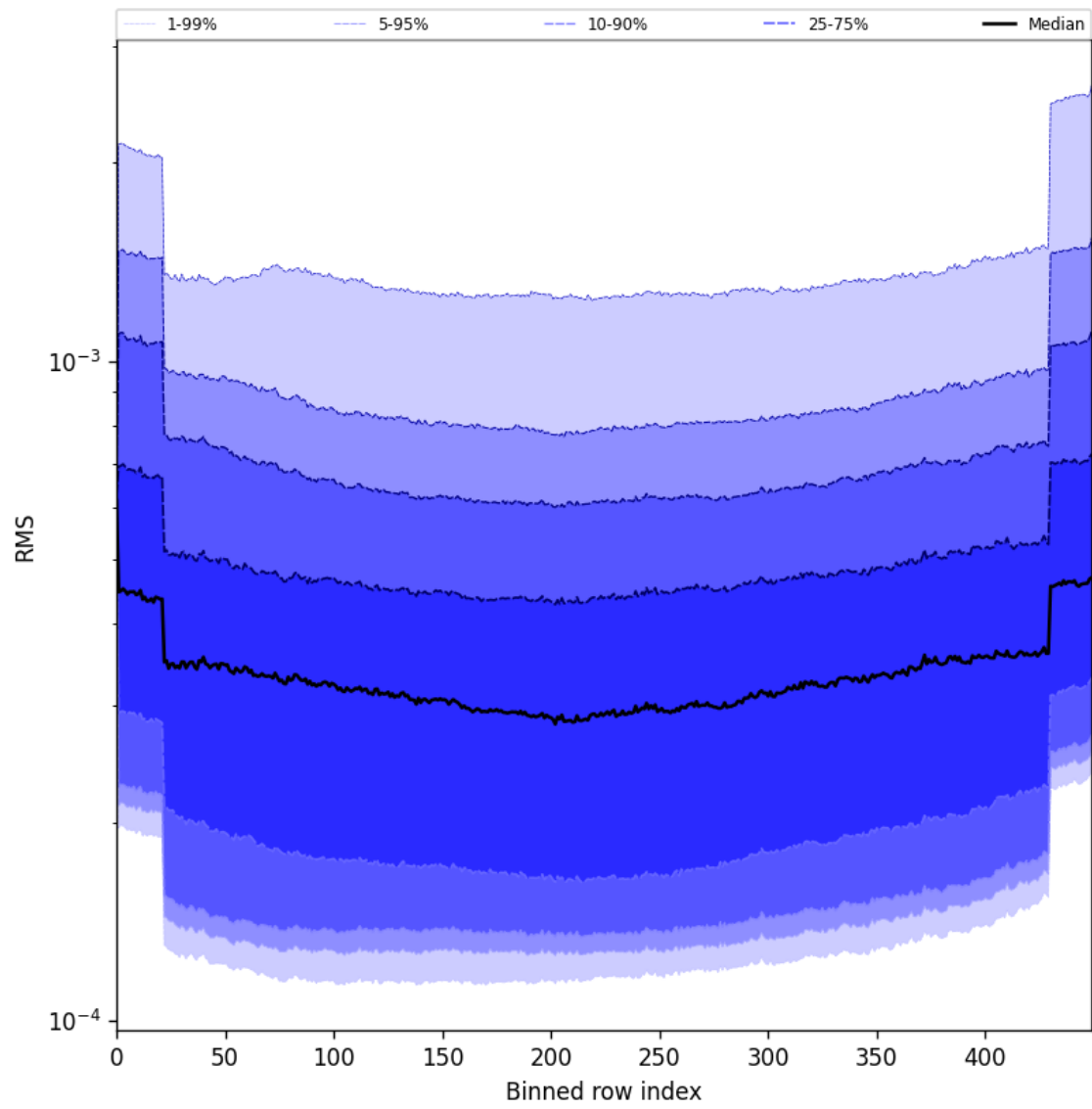
Figure 58: Along track statistics of “RMS” for 2025-08-01 to 2025-08-01
