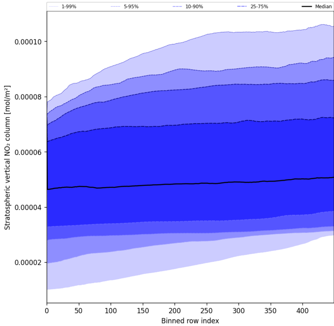
Figure 51: Along track statistics of “Stratospheric vertical NO 2 column” for 2025-08-01 to 2025-08-01
