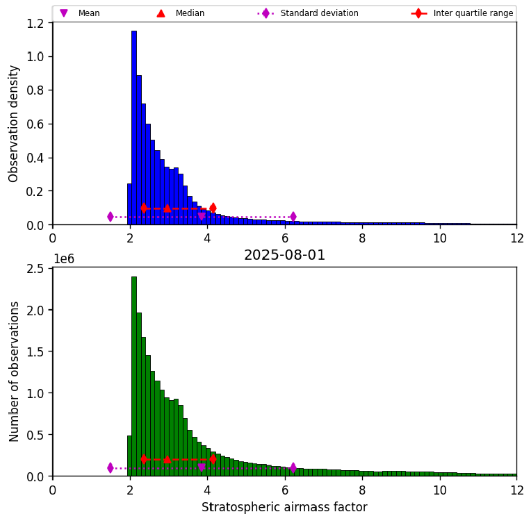
Figure 42: Histogram of “Stratospheric airmass factor” for 2025-08-01 to 2025-08-01
