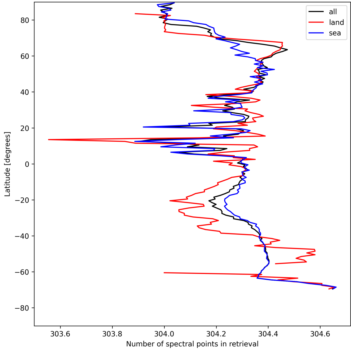
Figure 14: Zonal average of “Number of spectral points in retrieval” for 2025-08-01 to 2025-08-01.
