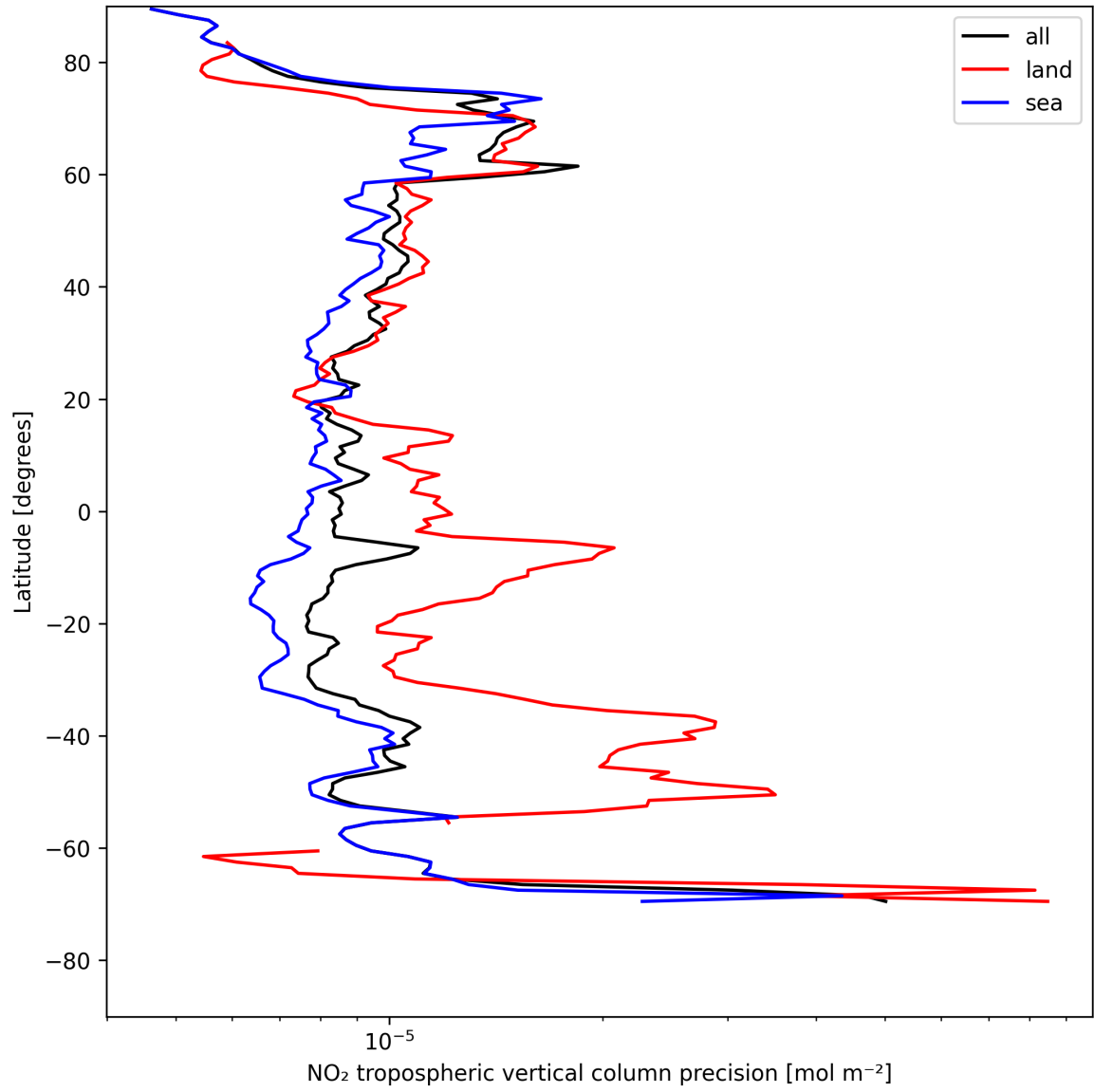
Figure 11: Zonal average of “NO 2 tropospheric vertical column precision” for 2025-08-01 to 2025-08-01.
