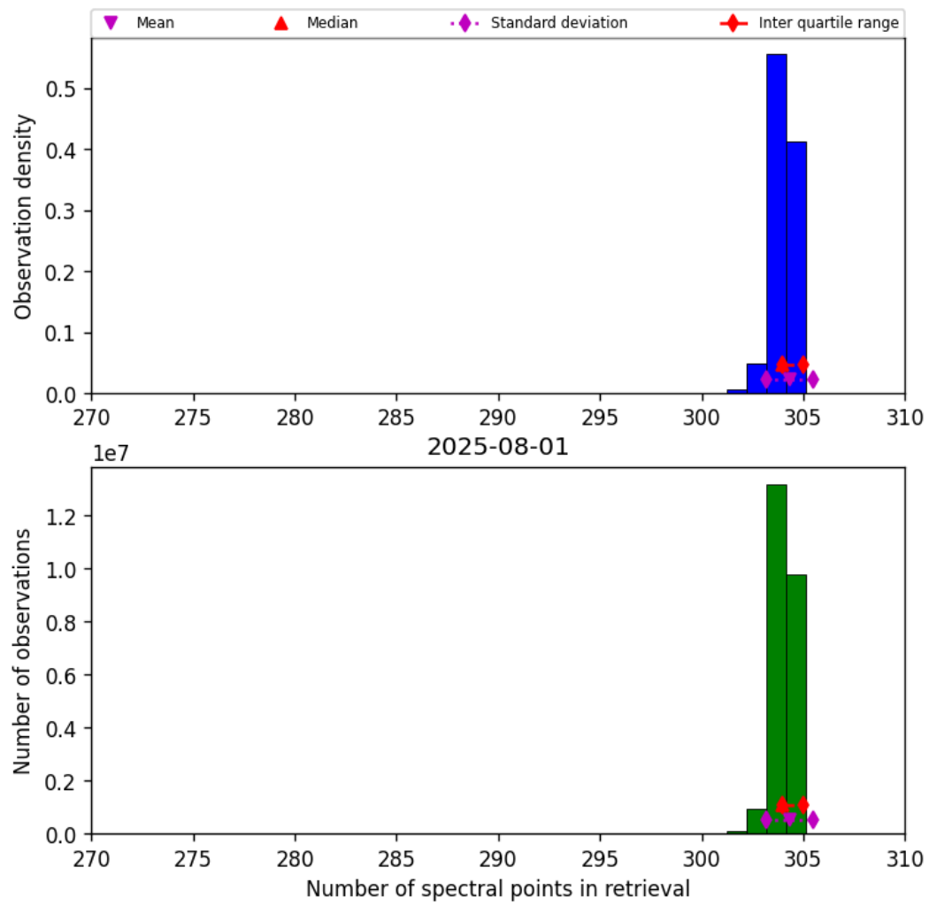
Figure 31: Histogram of “Number of spectral points in retrieval” for 2025-08-01 to 2025-08-01
