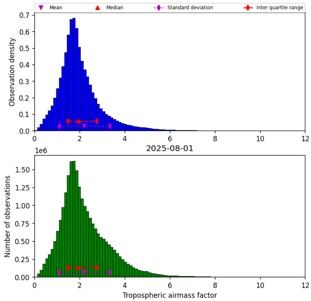
Figure 29: Histogram of “Tropospheric airmass factor” for 2025-08-01 to 2025-08-01
