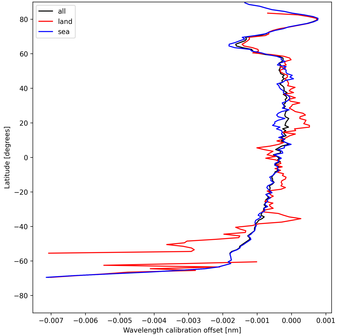
Figure 16: Zonal average of “Wavelength calibration offset” for 2025-08-01 to 2025-08-01.
