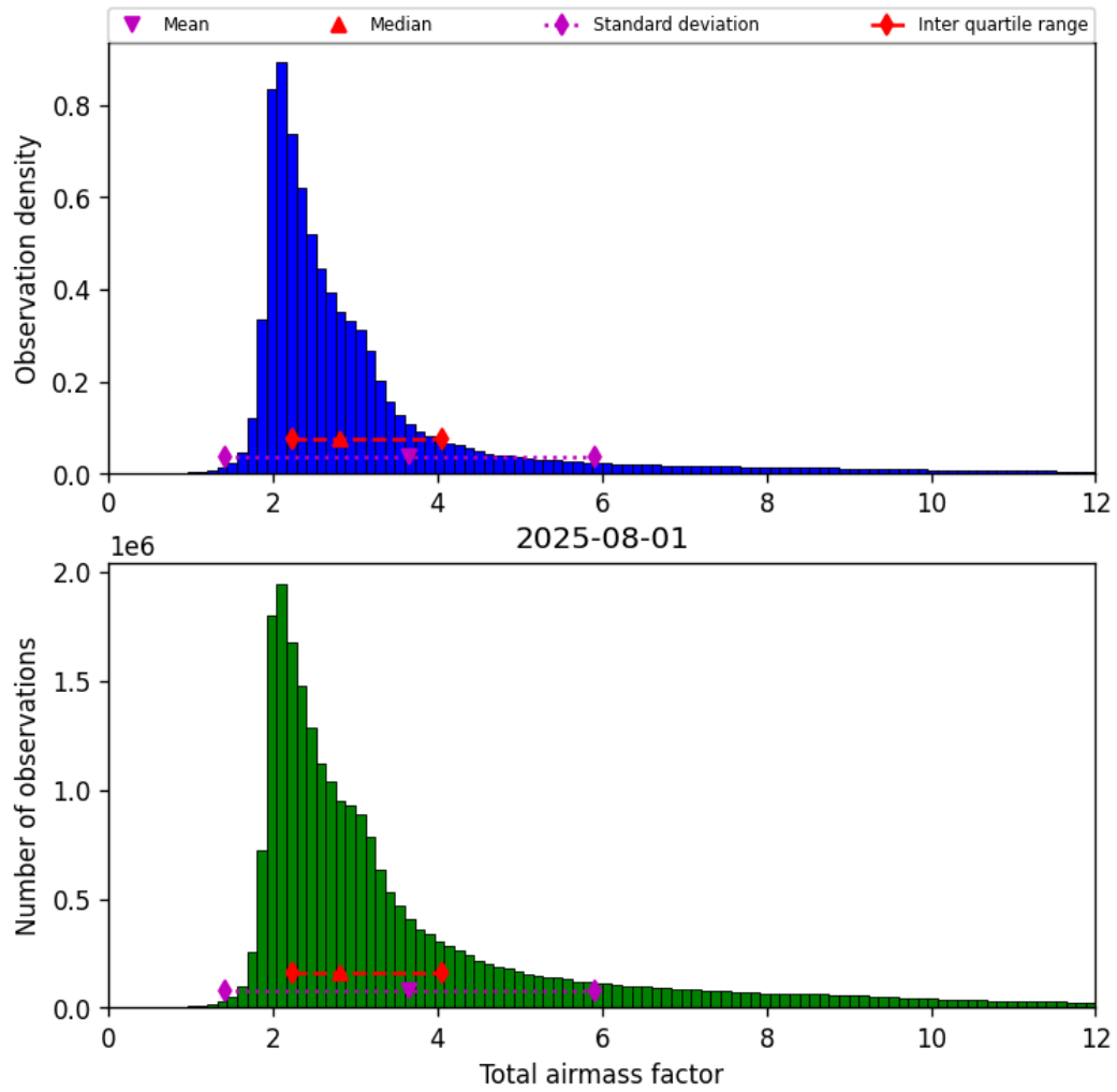
Figure 30: Histogram of “Total airmass factor” for 2025-08-01 to 2025-08-01
