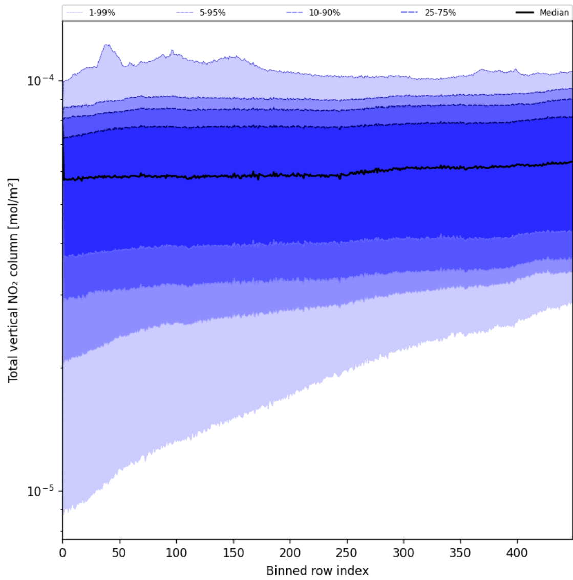
Figure 53: Along track statistics of “Total vertical NO 2 column” for 2025-08-01 to 2025-08-01
