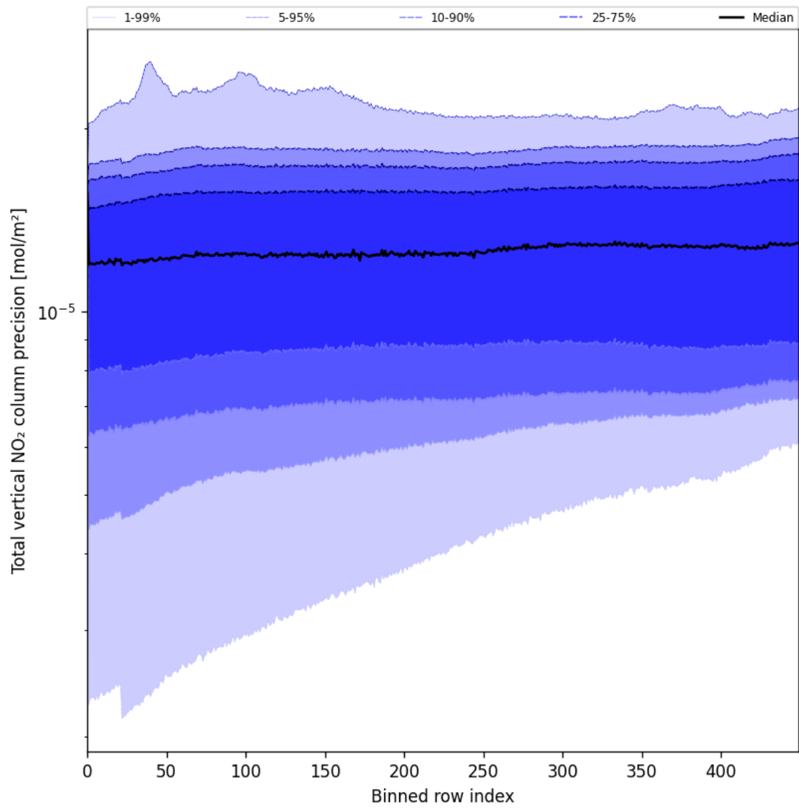
Figure 54: Along track statistics of “Total vertical NO 2 column precision” for 2025-08-01 to 2025-08-01
