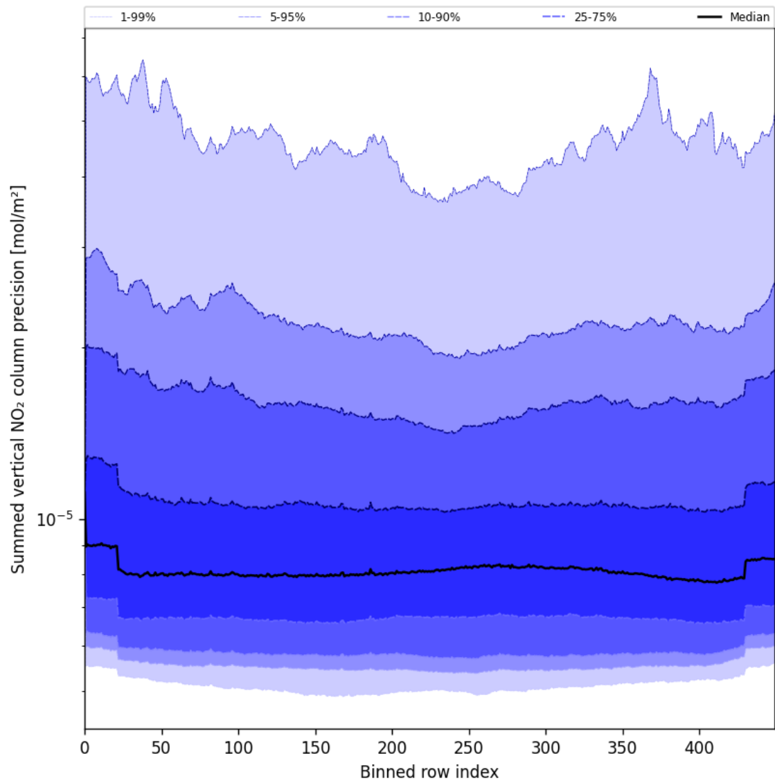
Figure 56: Along track statistics of “Summed vertical NO 2 column precision” for 2025-08-01 to 2025-08-01
