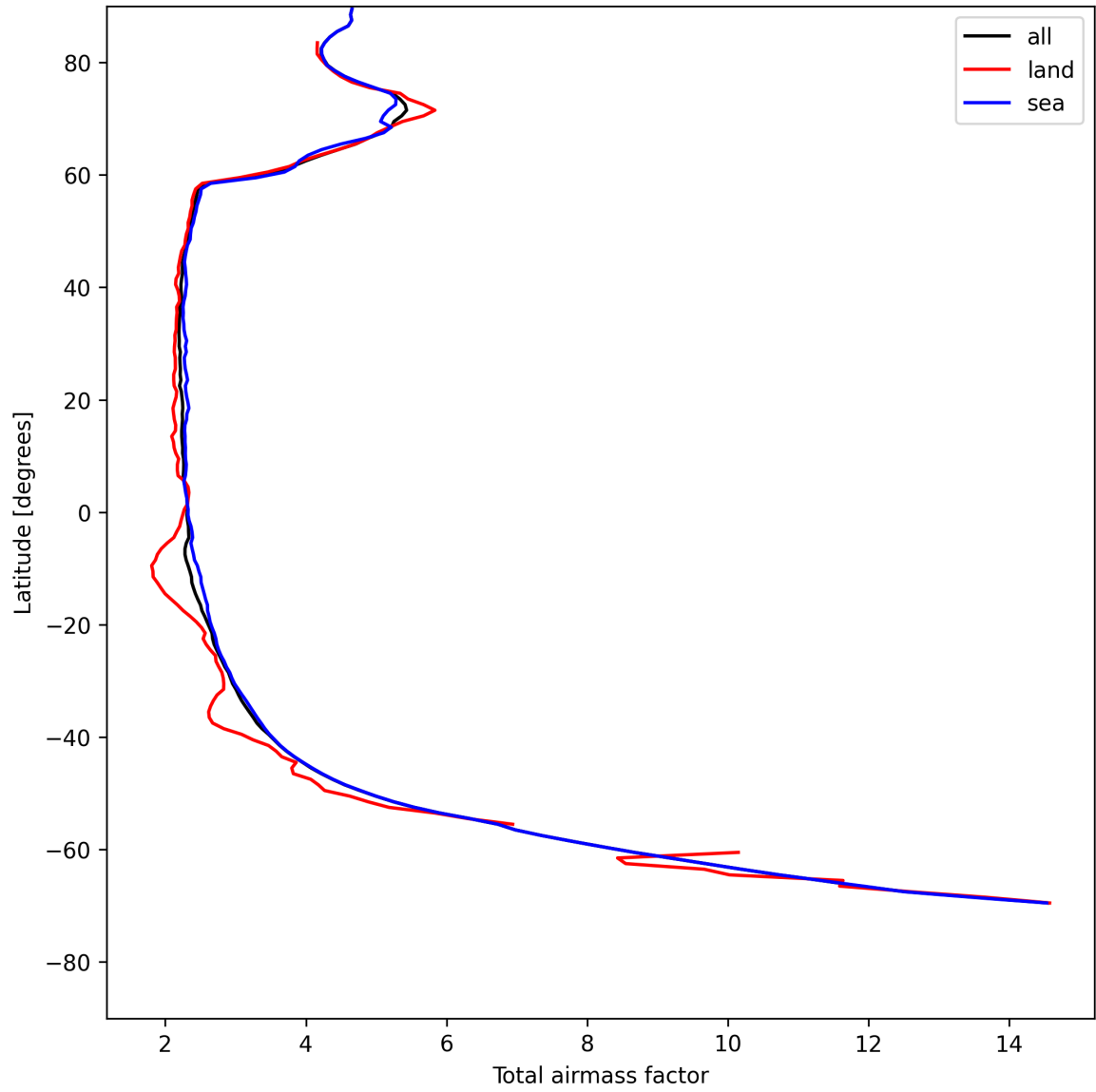
Figure 13: Zonal average of “Total airmass factor” for 2025-08-01 to 2025-08-01.
