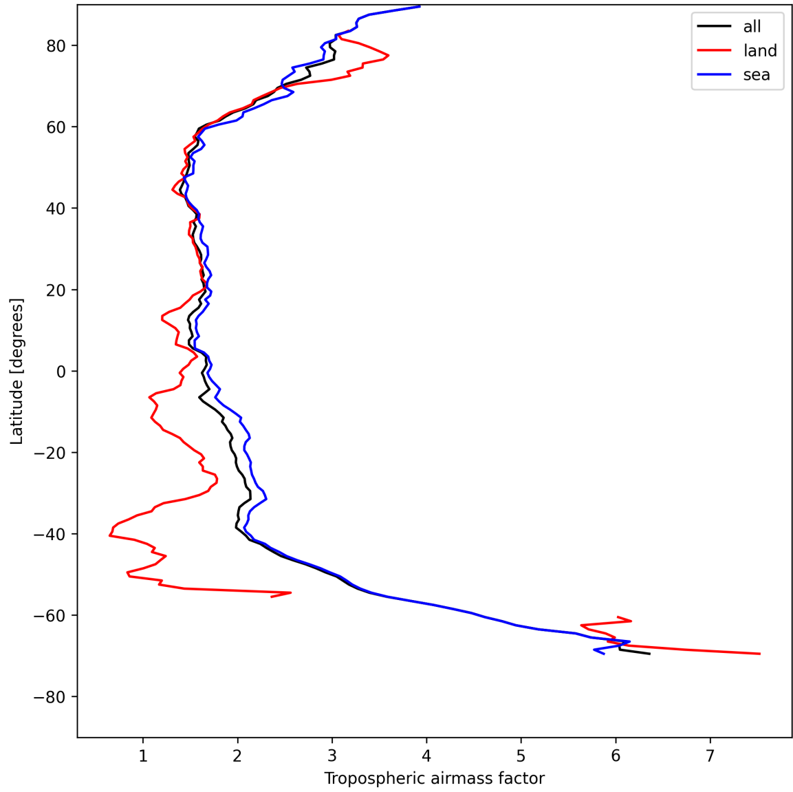
Figure 12: Zonal average of “Tropospheric airmass factor” for 2025-08-01 to 2025-08-01.
