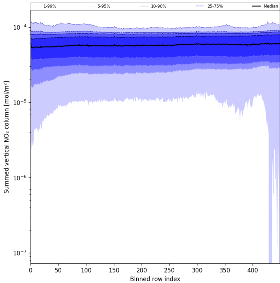
Figure 55: Along track statistics of “Summed vertical NO 2 column” for 2025-08-02 to 2025-08-03
