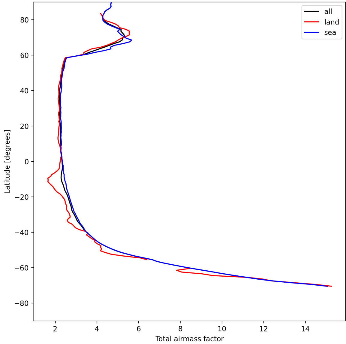
Figure 13: Zonal average of “Total airmass factor” for 2025-08-02 to 2025-08-03.
