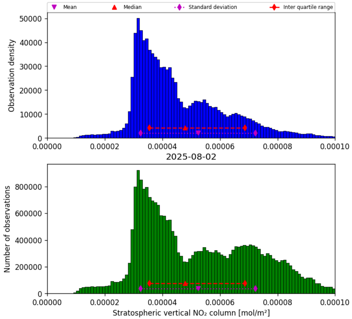
Figure 34: Histogram of “Stratospheric vertical NO 2 column” for 2025-08-02 to 2025-08-03
