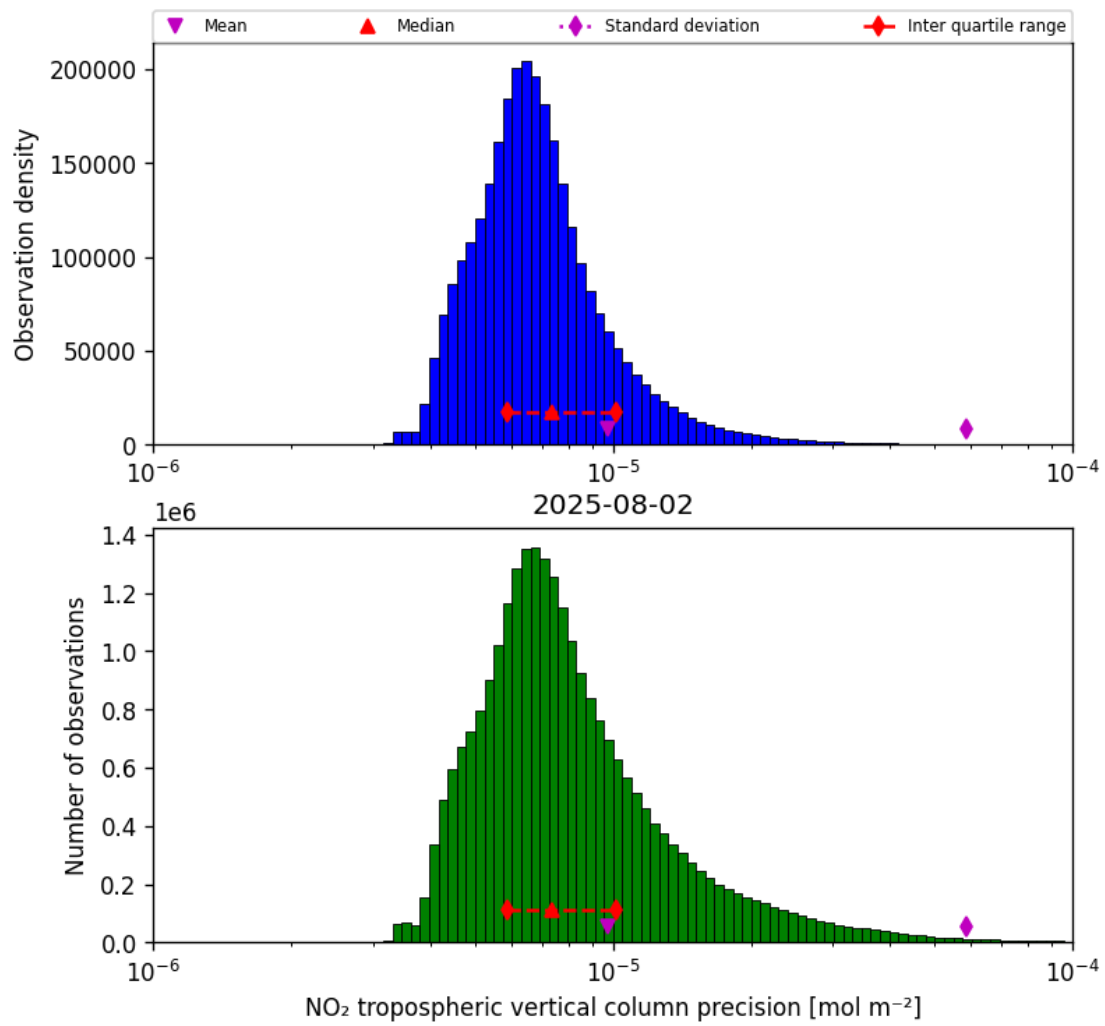
Figure 28: Histogram of “NO 2 tropospheric vertical column precision” for 2025-08-02 to 2025-08-03
