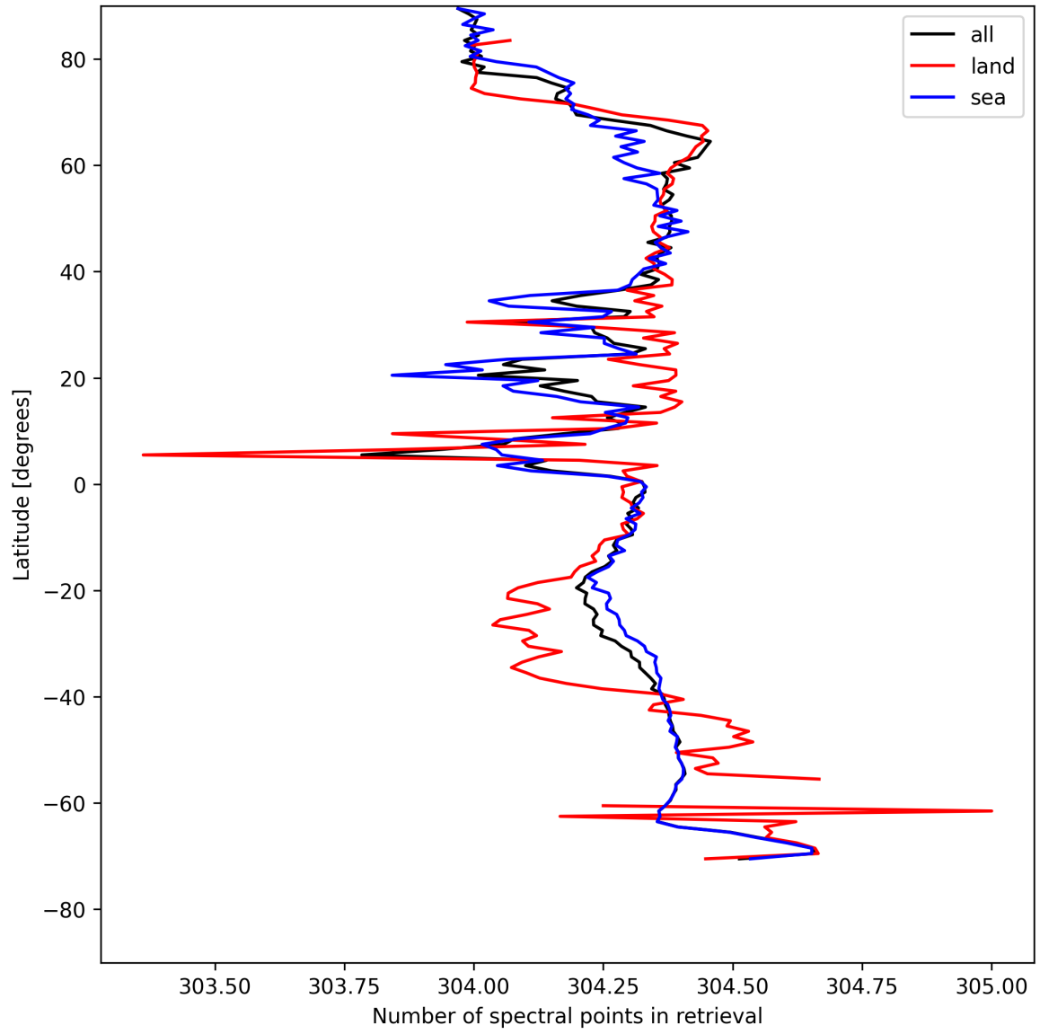
Figure 14: Zonal average of “Number of spectral points in retrieval” for 2025-08-02 to 2025-08-03.
