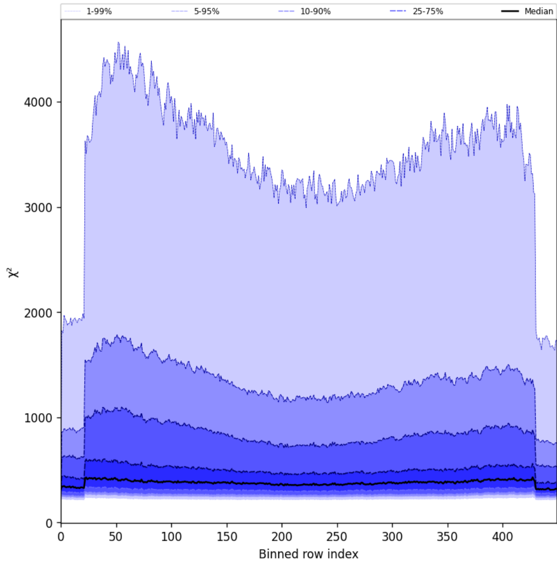
Figure 57: Along track statistics of “ \chi^2 ” for 2025-08-02 to 2025-08-03
