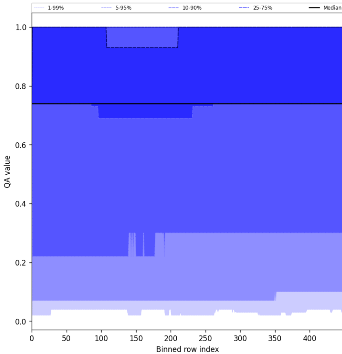
Figure 43: Along track statistics of “QA value” for 2025-08-02 to 2025-08-03
