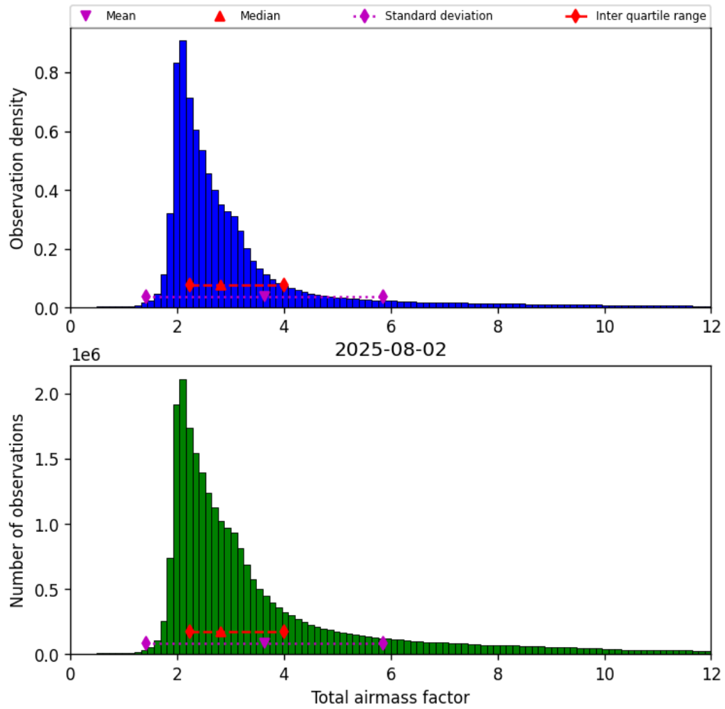
Figure 30: Histogram of “Total airmass factor” for 2025-08-02 to 2025-08-03
