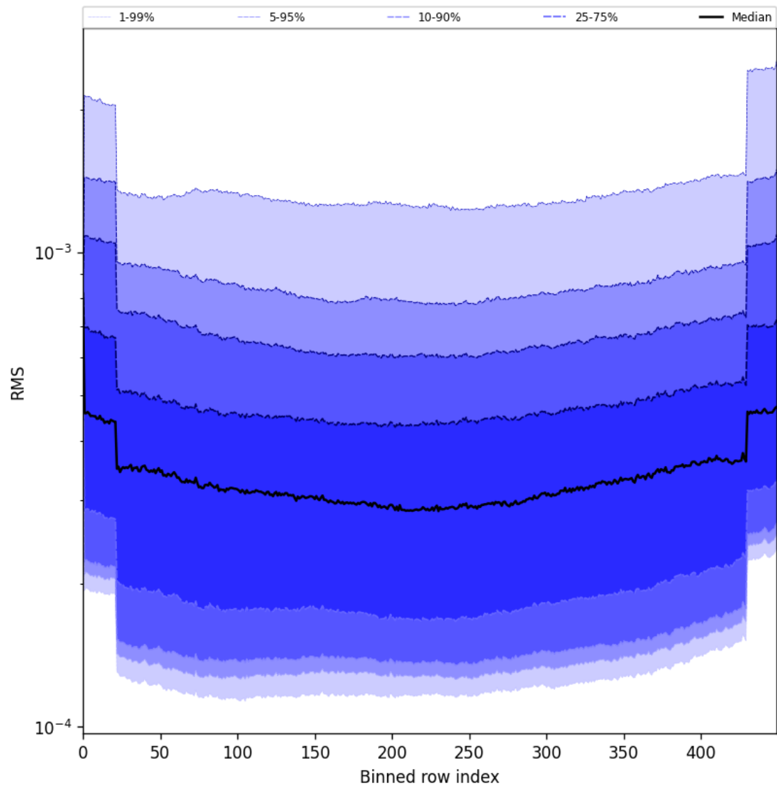
Figure 58: Along track statistics of “RMS” for 2025-08-02 to 2025-08-03
