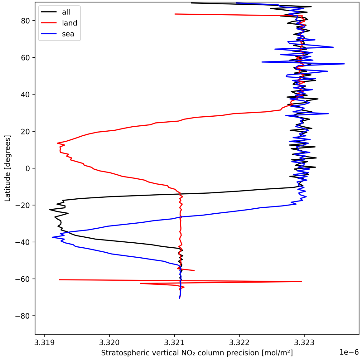
Figure 18: Zonal average of “Stratospheric vertical NO 2 column precision” for 2025-08-02 to 2025-08-03.
