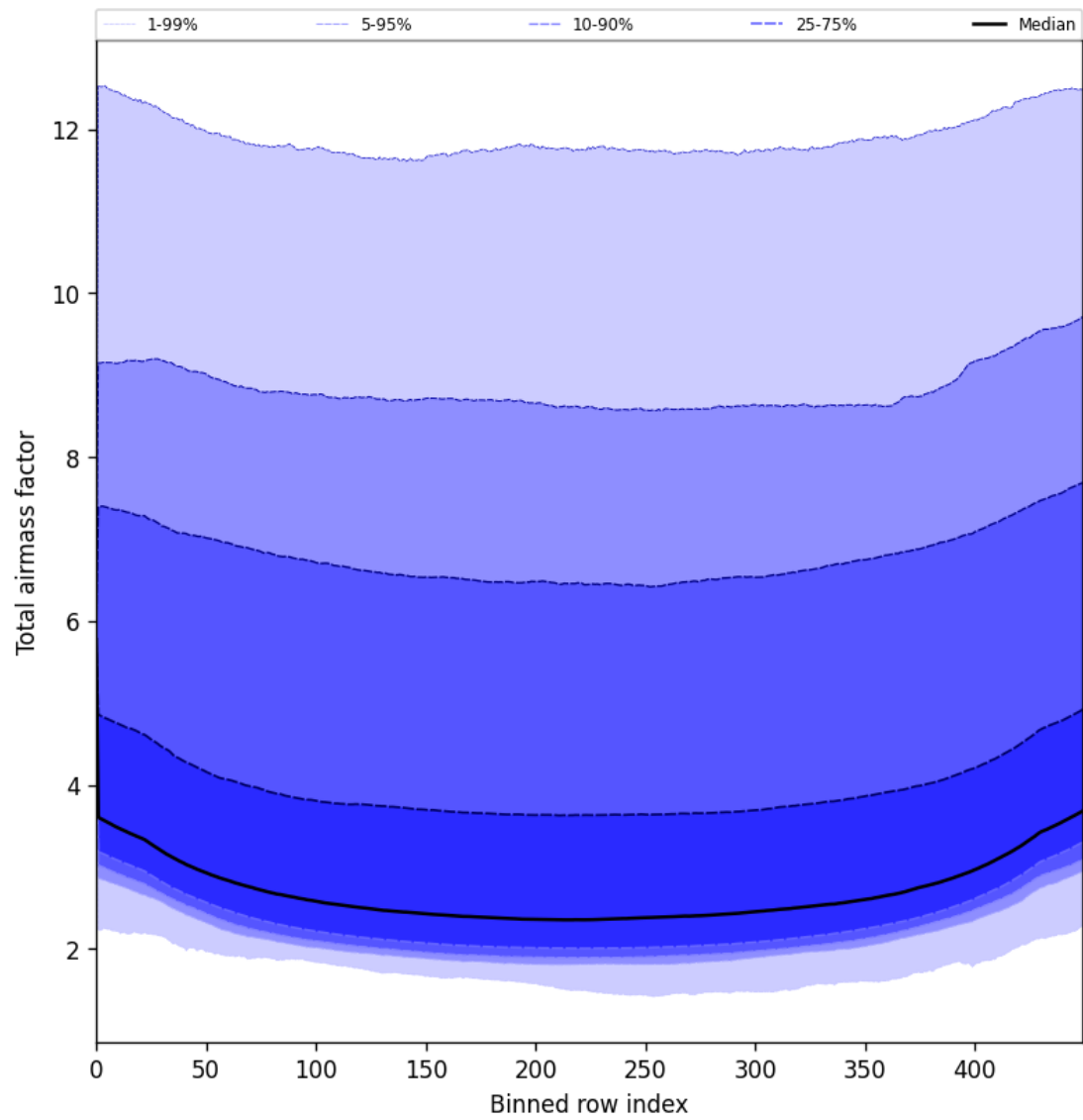
Figure 47: Along track statistics of “Total airmass factor” for 2025-08-02 to 2025-08-03
