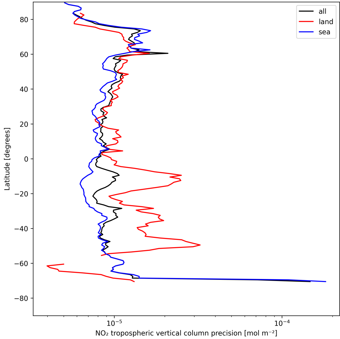
Figure 11: Zonal average of “NO 2 tropospheric vertical column precision” for 2025-08-02 to 2025-08-03.
