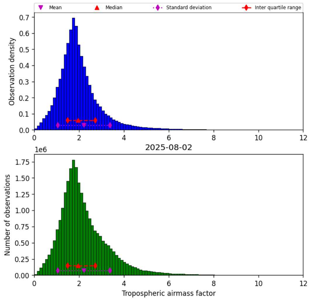
Figure 29: Histogram of “Tropospheric airmass factor” for 2025-08-02 to 2025-08-03
