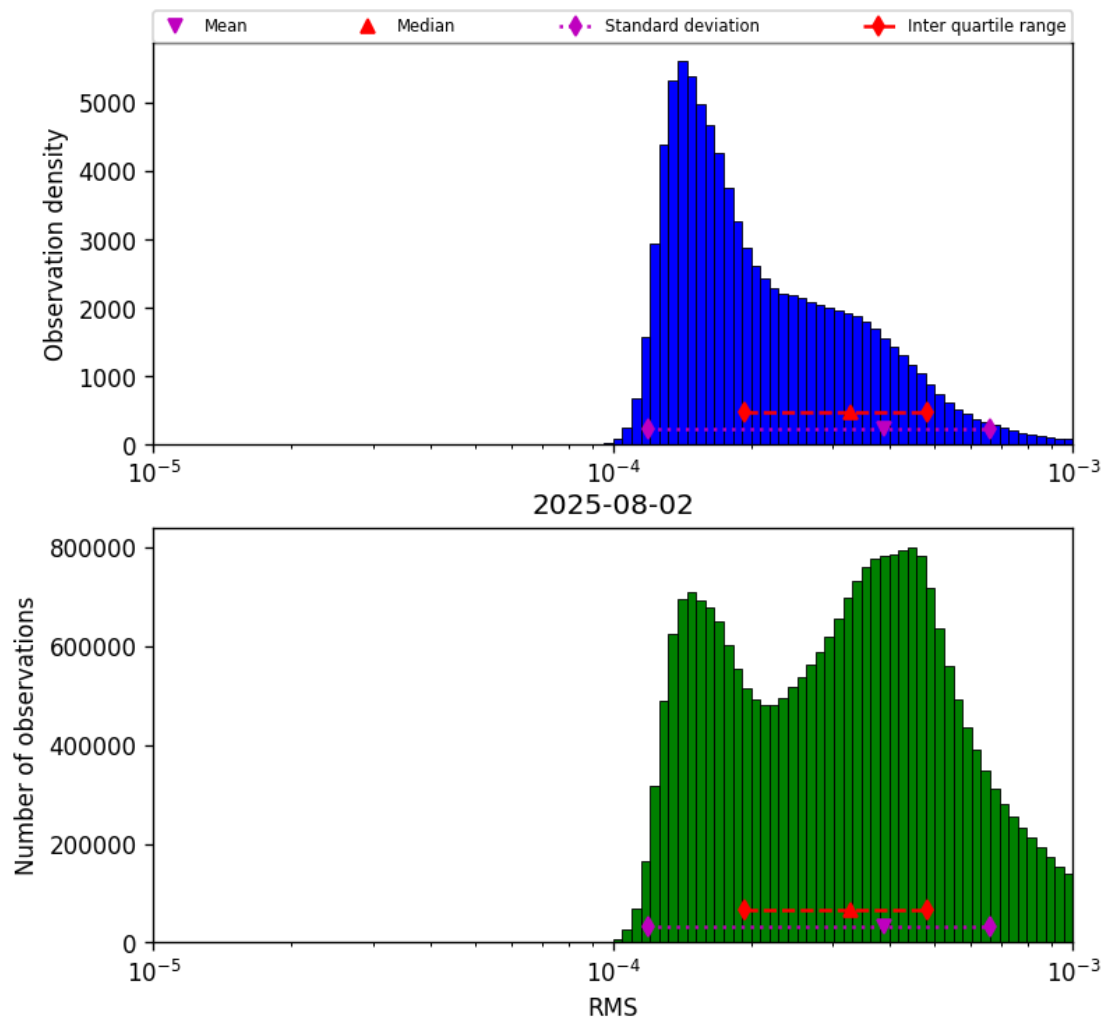
Figure 41: Histogram of “RMS” for 2025-08-02 to 2025-08-03
