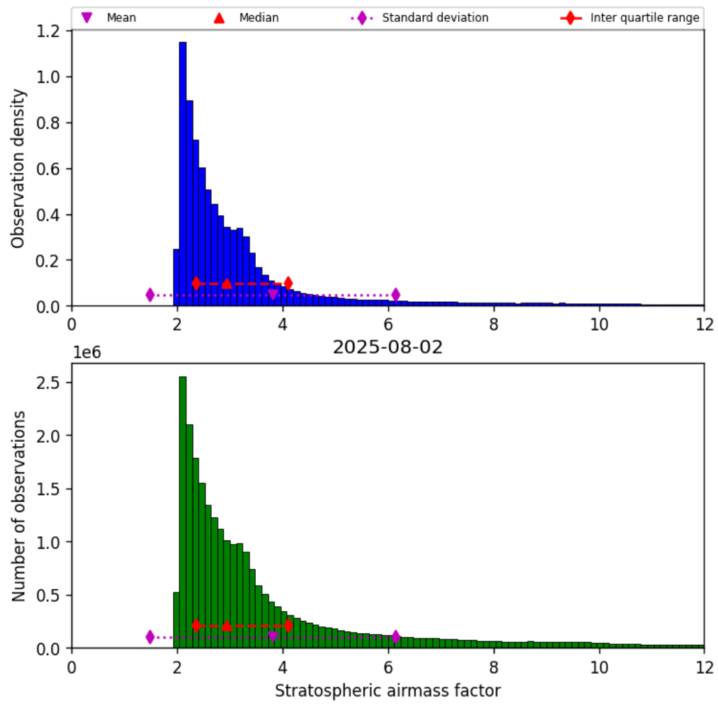
Figure 42: Histogram of “Stratospheric airmass factor” for 2025-08-02 to 2025-08-03
