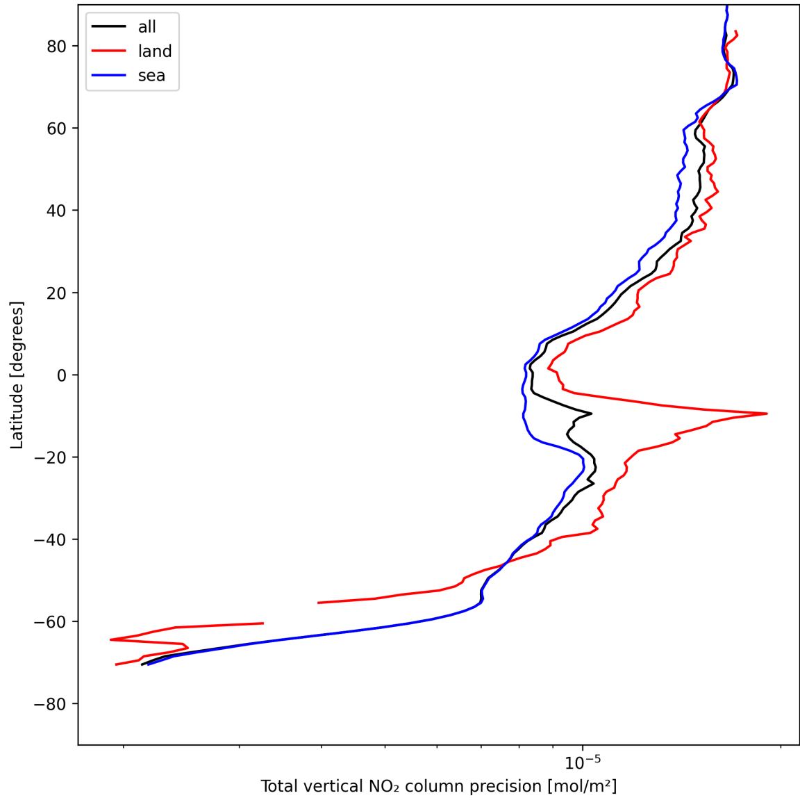
Figure 20: Zonal average of “Total vertical NO 2 column precision” for 2025-08-02 to 2025-08-03.
