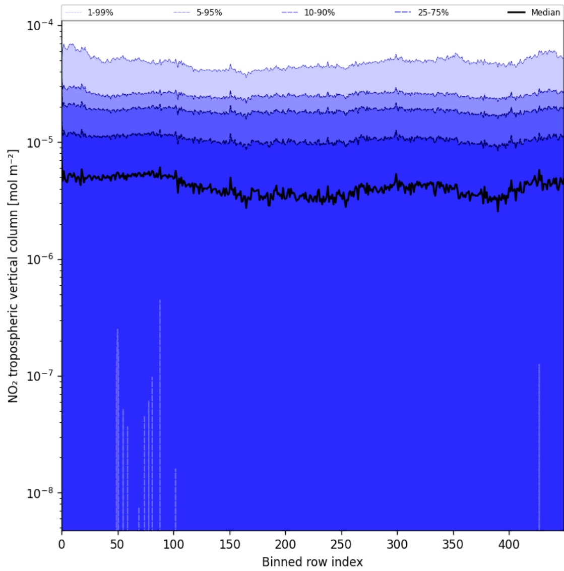
Figure 44: Along track statistics of “NO 2 tropospheric vertical column” for 2025-08-02 to 2025-08-03
