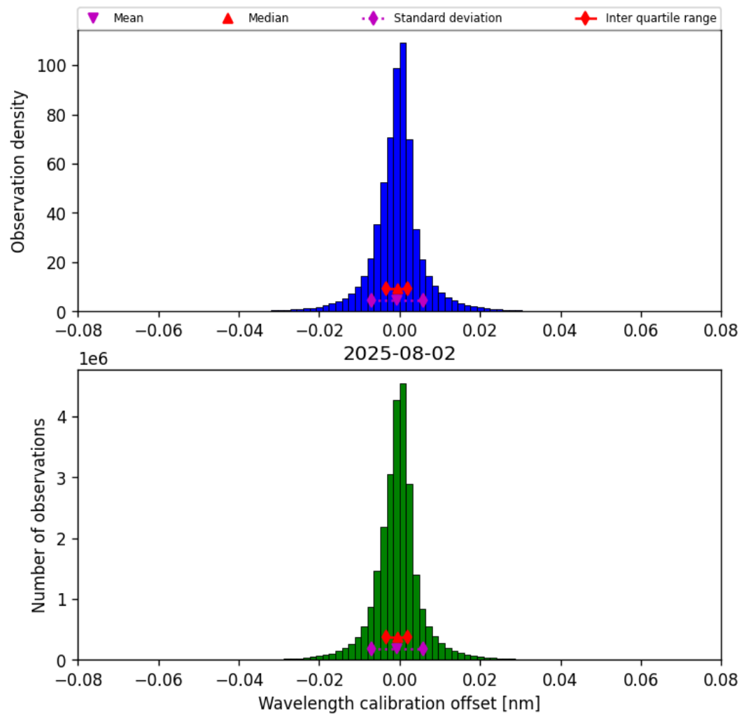
Figure 33: Histogram of “Wavelength calibration offset” for 2025-08-02 to 2025-08-03
