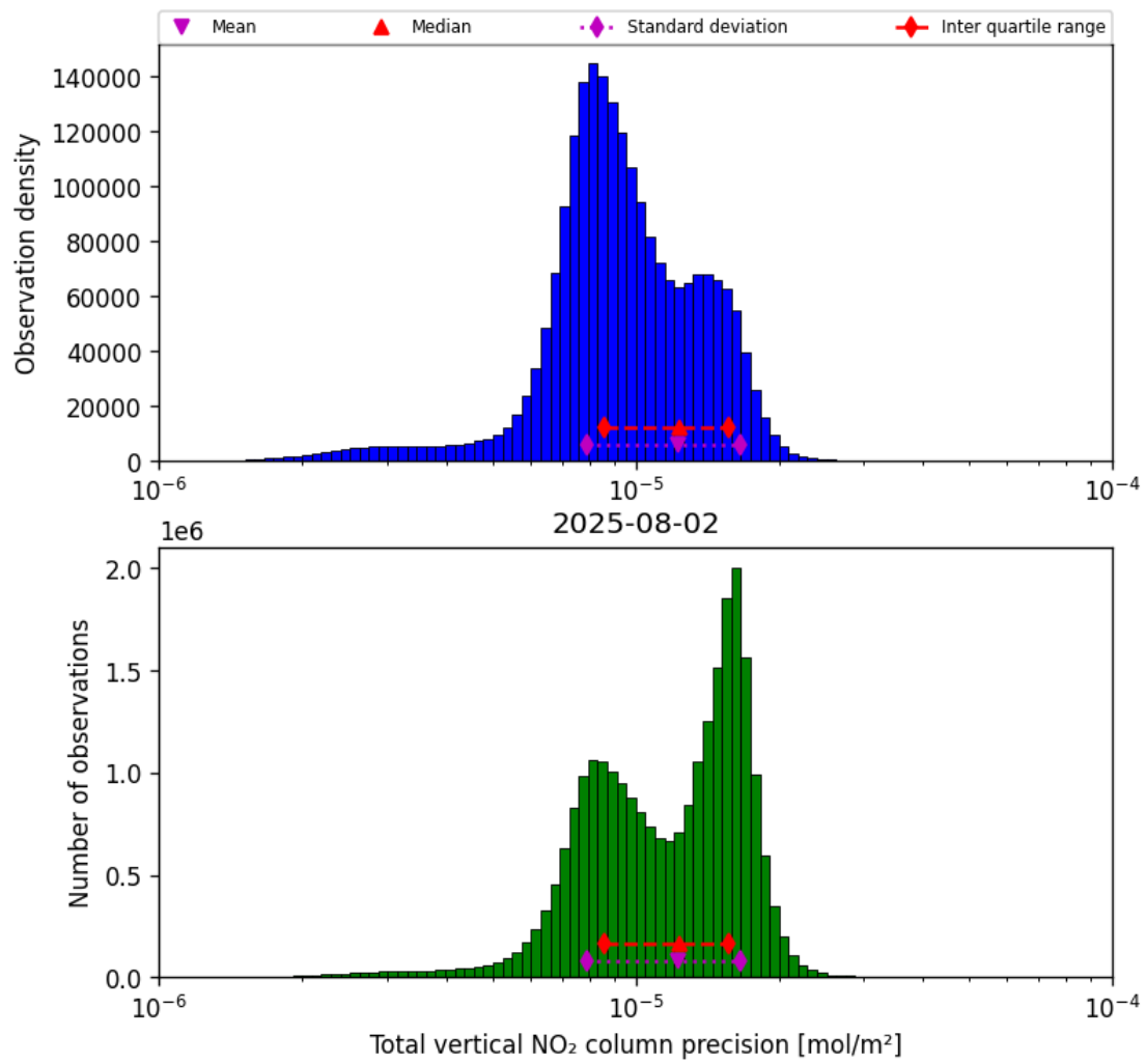
Figure 37: Histogram of “Total vertical NO 2 column precision” for 2025-08-02 to 2025-08-03
