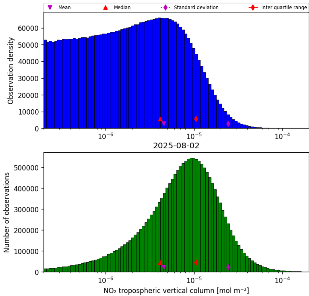
Figure 27: Histogram of “NO 2 tropospheric vertical column” for 2025-08-02 to 2025-08-03
