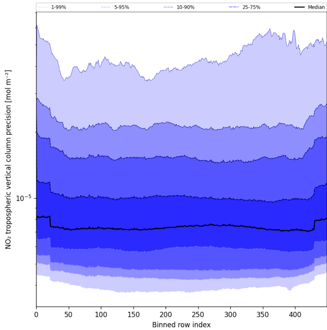
Figure 45: Along track statistics of “NO 2 tropospheric vertical column precision” for 2025-08-02 to 2025-08-03
