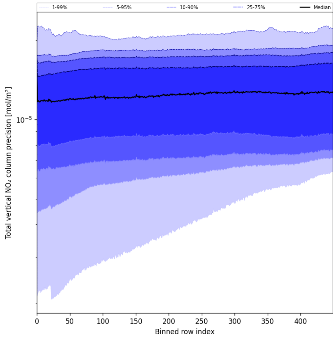
Figure 54: Along track statistics of “Total vertical NO 2 column precision” for 2025-08-02 to 2025-08-03
