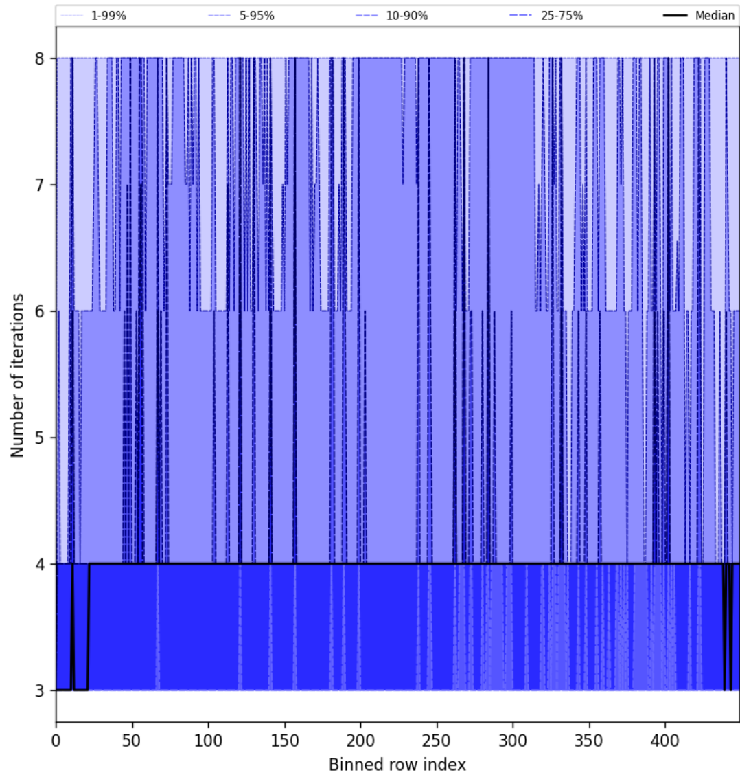
Figure 49: Along track statistics of “Number of iterations” for 2025-08-02 to 2025-08-03
