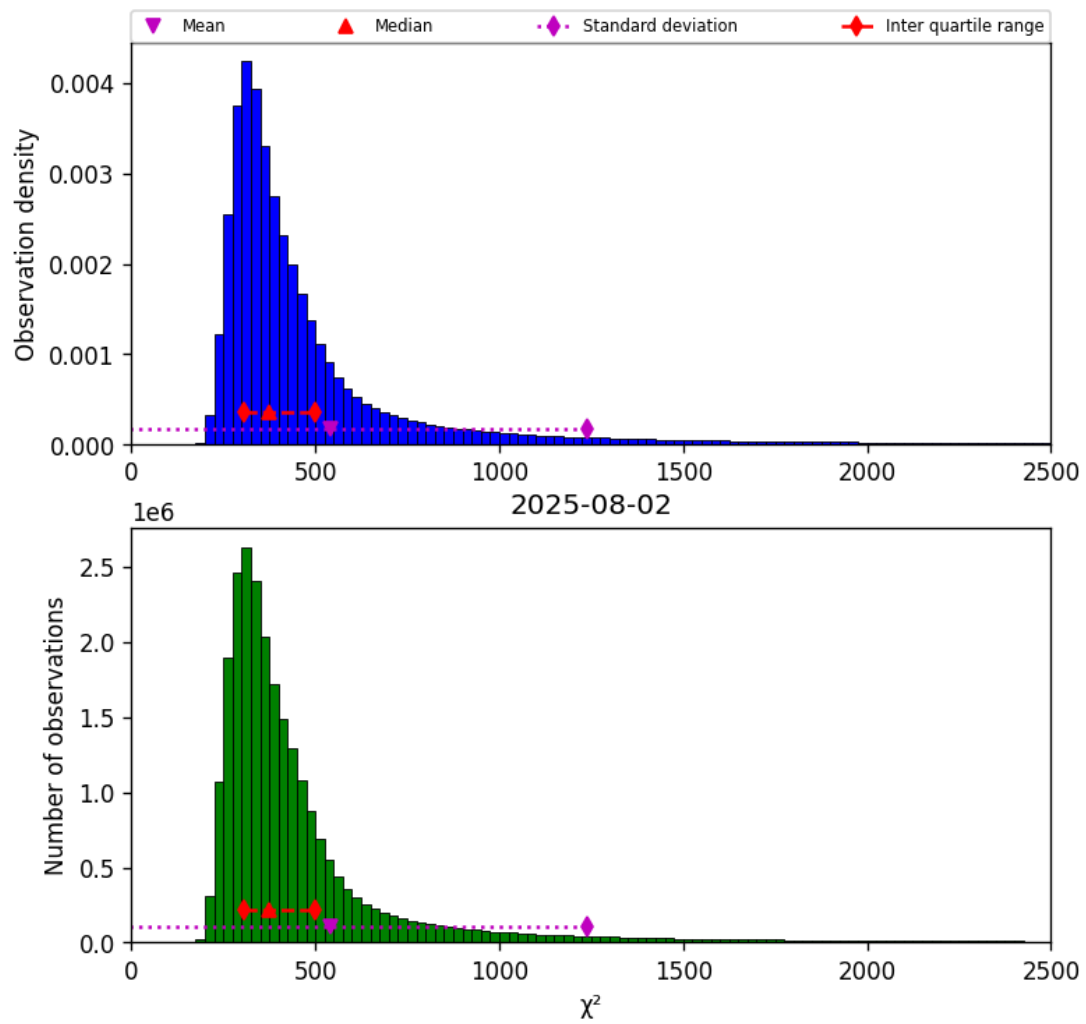
Figure 40: Histogram of “ \chi^2 ” for 2025-08-02 to 2025-08-03
