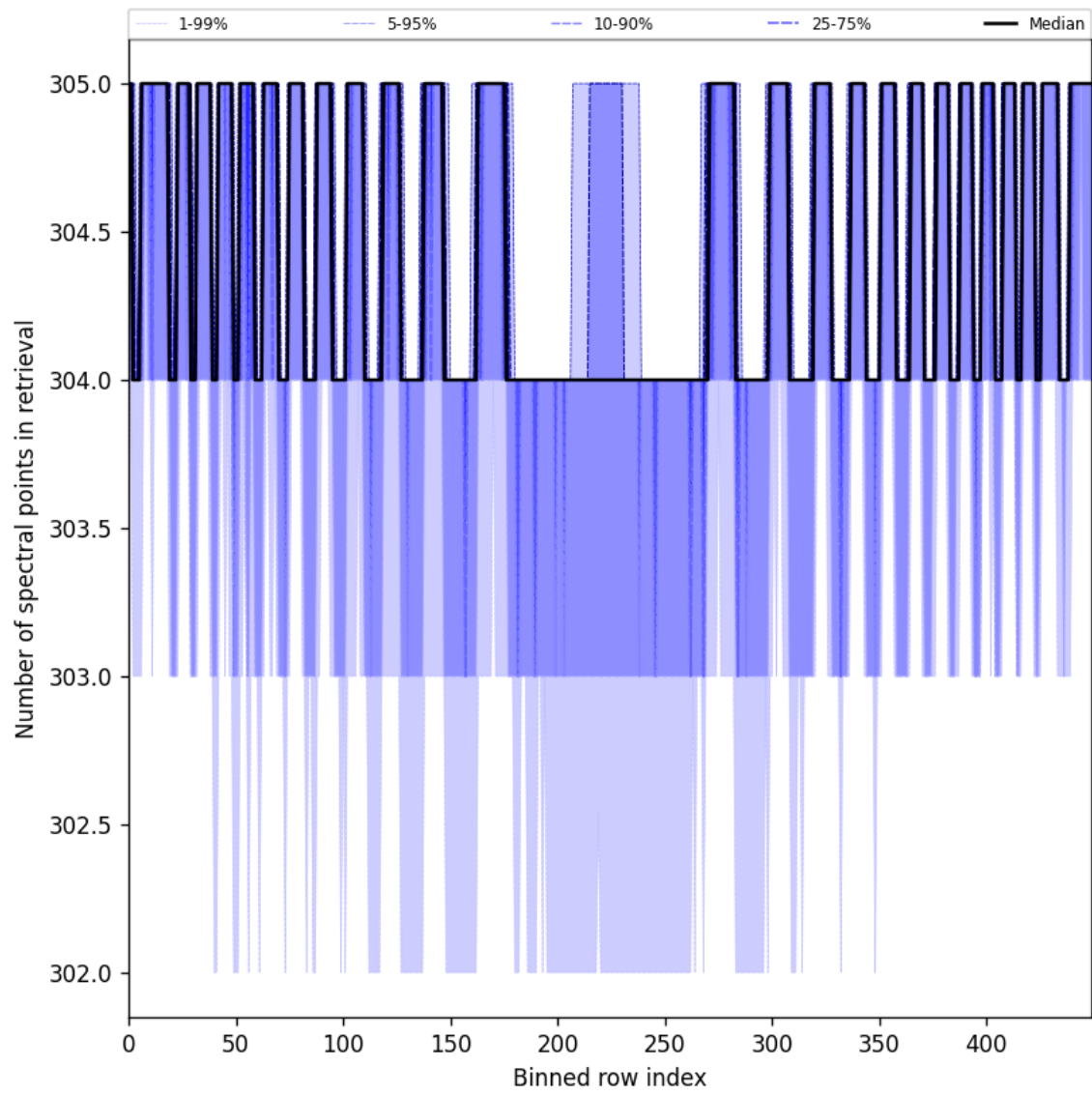
Figure 48: Along track statistics of “Number of spectral points in retrieval” for 2025-08-02 to 2025-08-03
