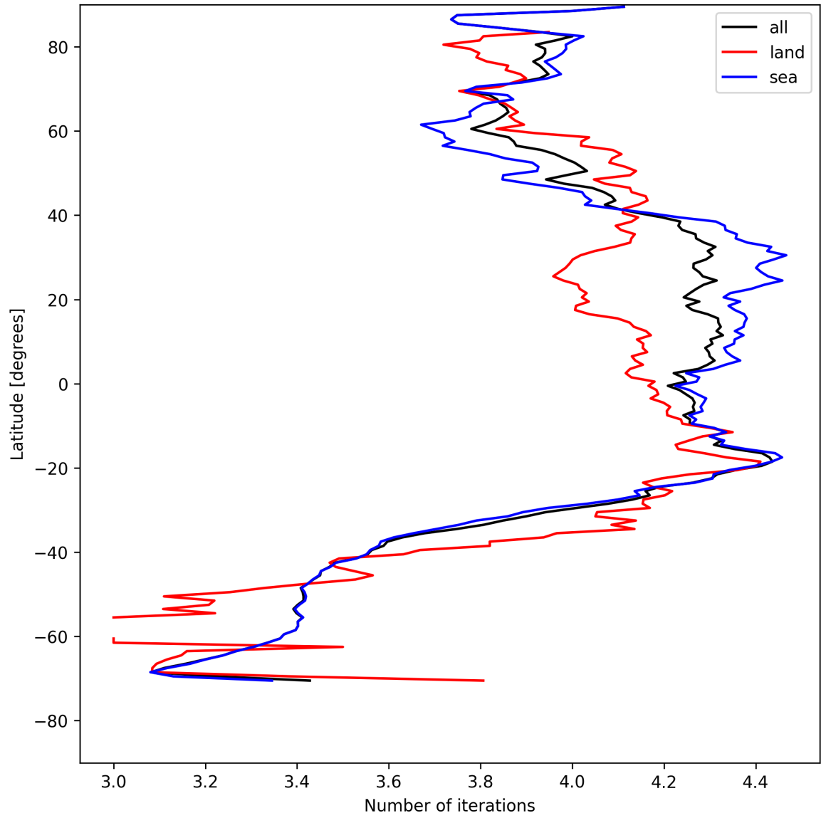
Figure 15: Zonal average of “Number of iterations” for 2025-08-02 to 2025-08-03.
