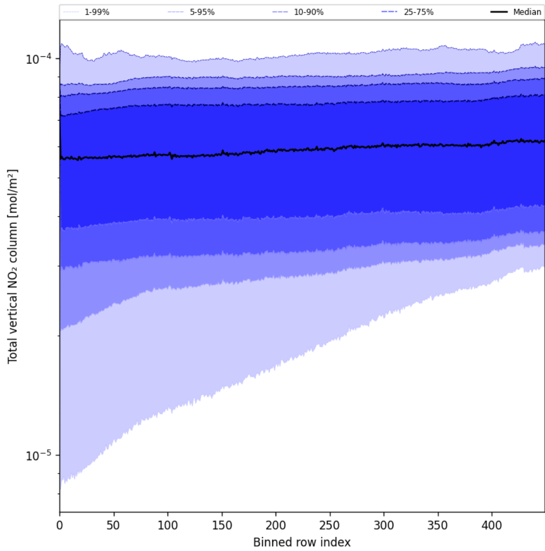
Figure 53: Along track statistics of “Total vertical NO 2 column” for 2025-08-02 to 2025-08-03
