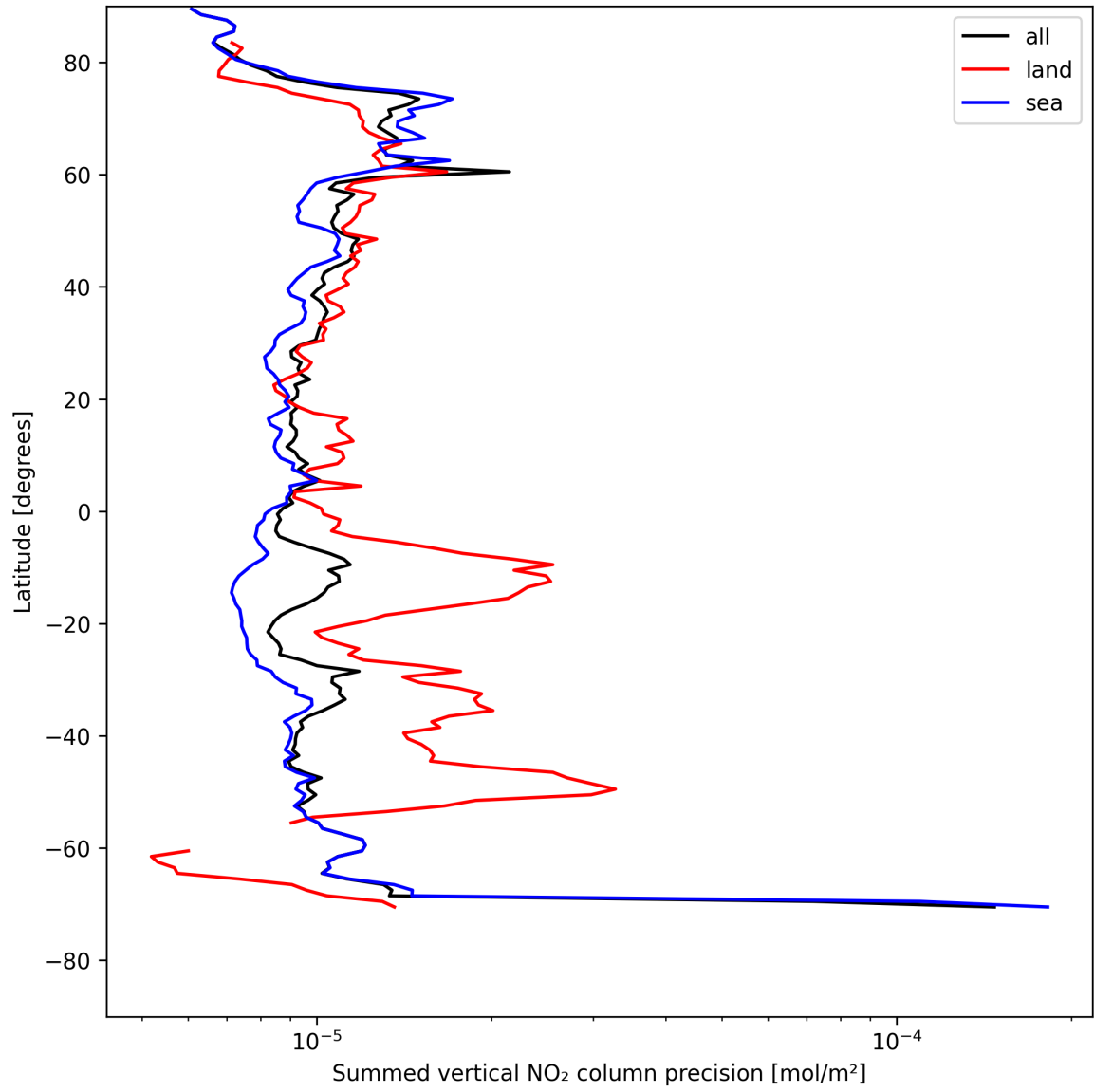
Figure 22: Zonal average of “Summed vertical NO 2 column precision” for 2025-08-02 to 2025-08-03.
