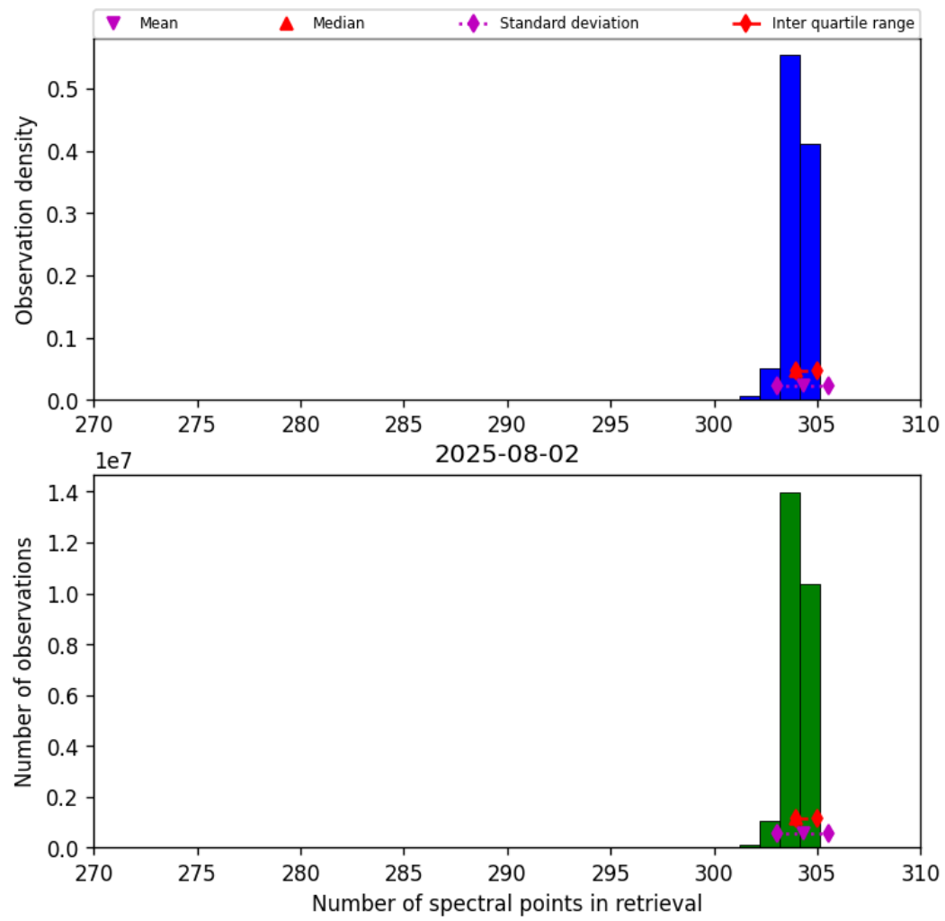
Figure 31: Histogram of “Number of spectral points in retrieval” for 2025-08-02 to 2025-08-03
