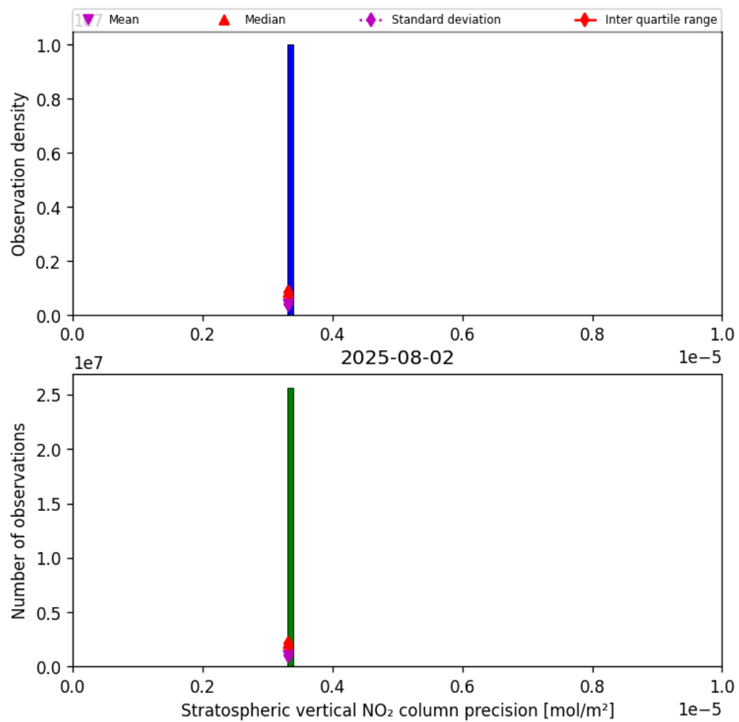
Figure 35: Histogram of “Stratospheric vertical NO 2 column precision” for 2025-08-02 to 2025-08-03
