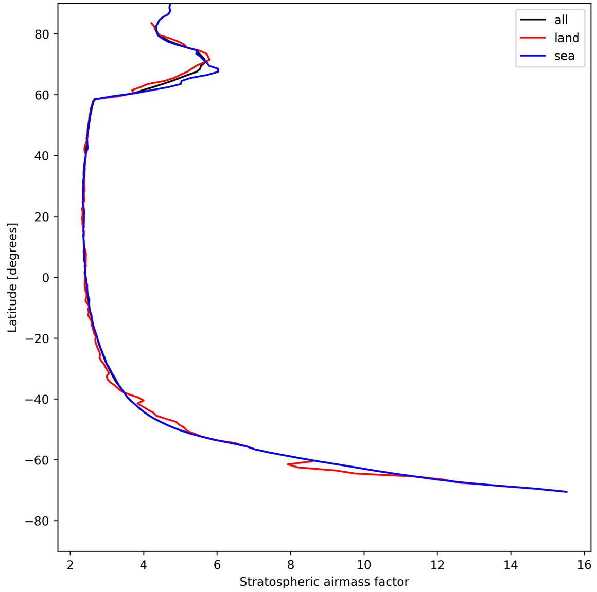
Figure 25: Zonal average of “Stratospheric air mass factor” for 2025-08-02 to 2025-08-03.
