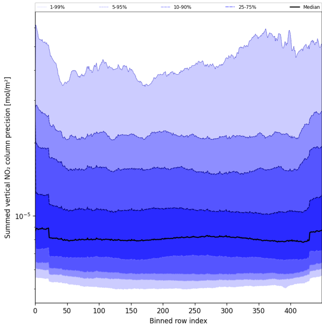
Figure 56: Along track statistics of “Summed vertical NO 2 column precision” for 2025-08-02 to 2025-08-03
