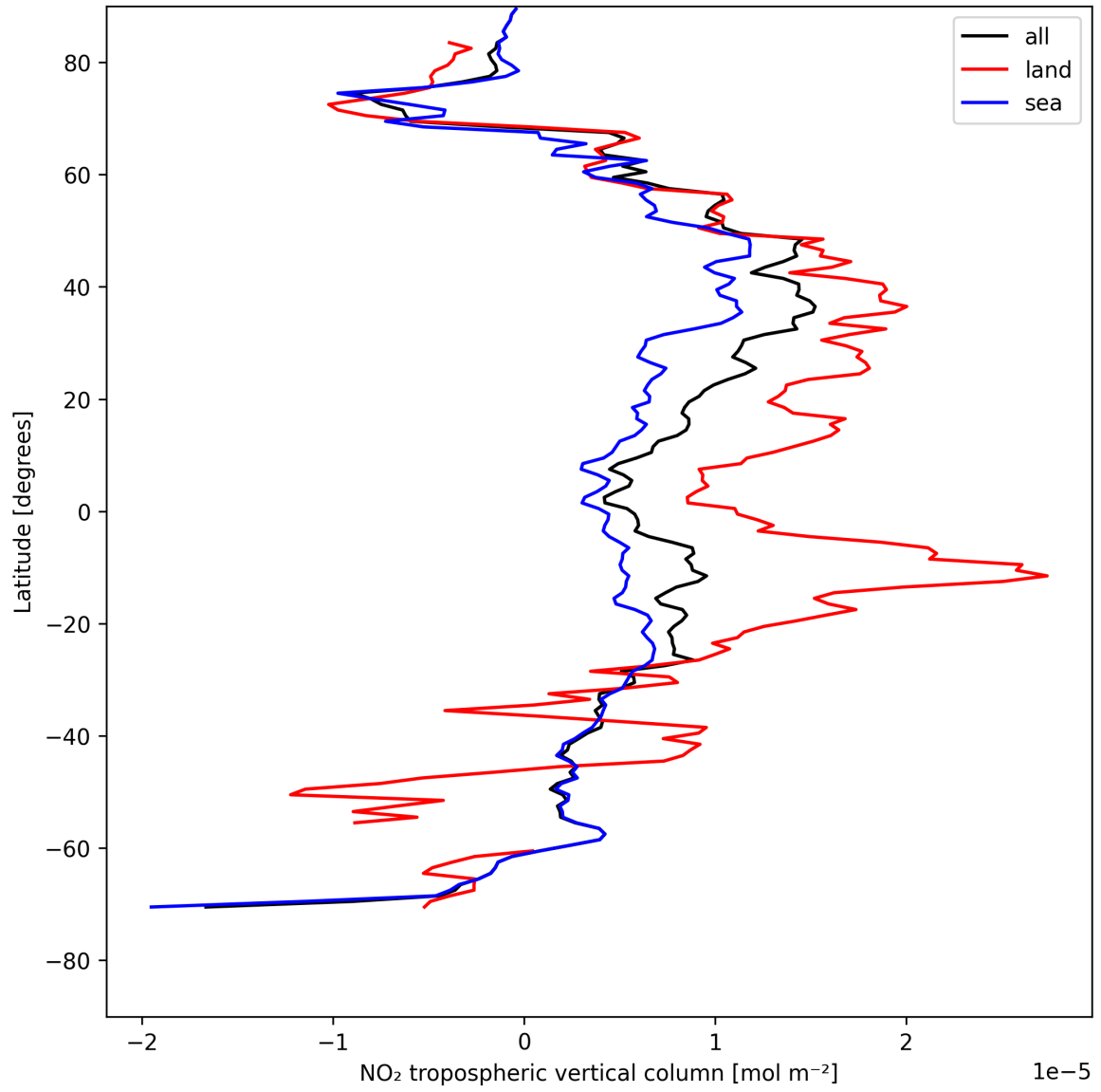
Figure 10: Zonal average of “NO 2 tropospheric vertical column” for 2025-08-02 to 2025-08-03.
