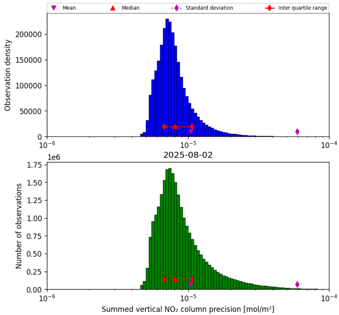
Figure 39: Histogram of “Summed vertical NO 2 column precision” for 2025-08-02 to 2025-08-03
