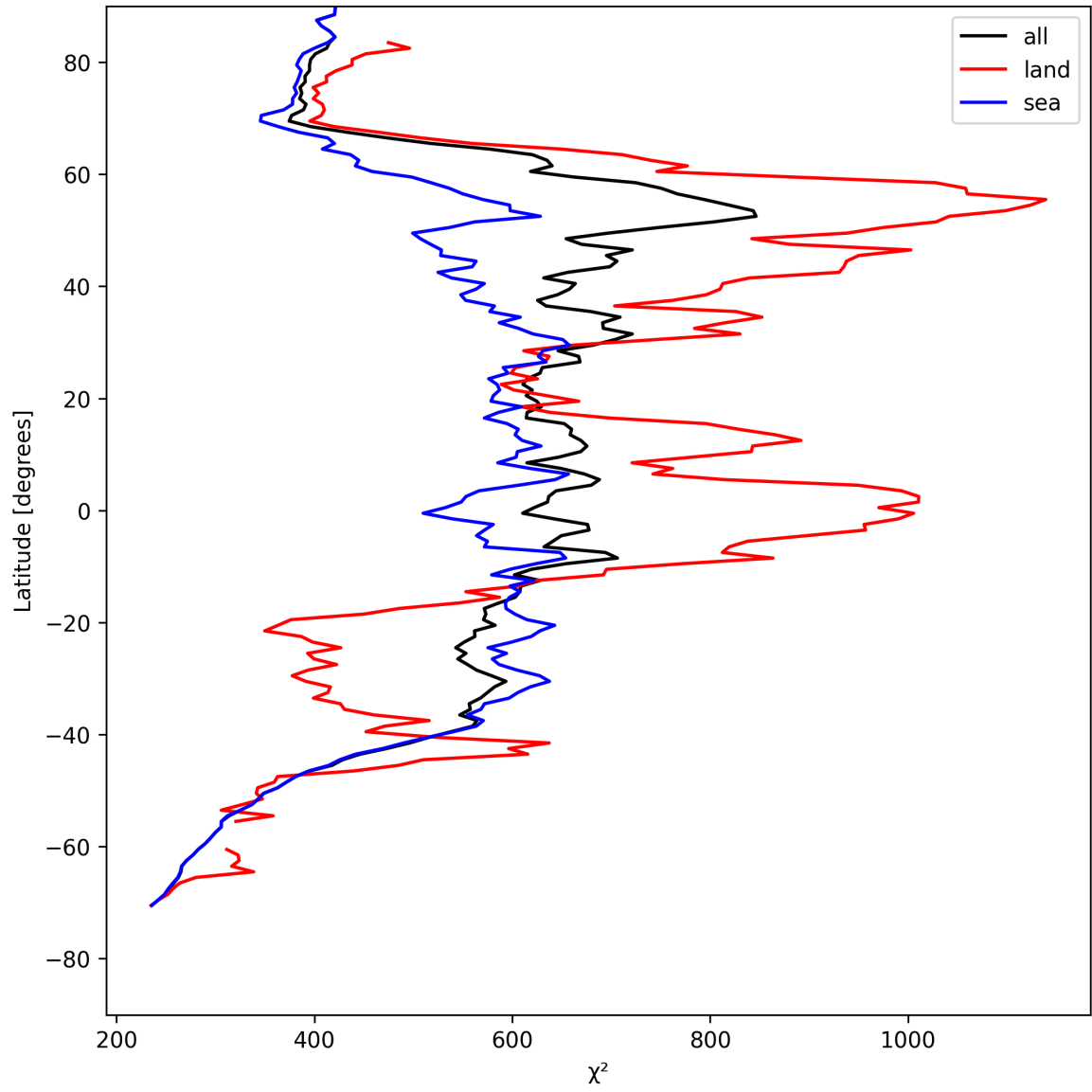
Figure 23: Zonal average of “ \chi^2 ” for 2025-08-02 to 2025-08-03.
