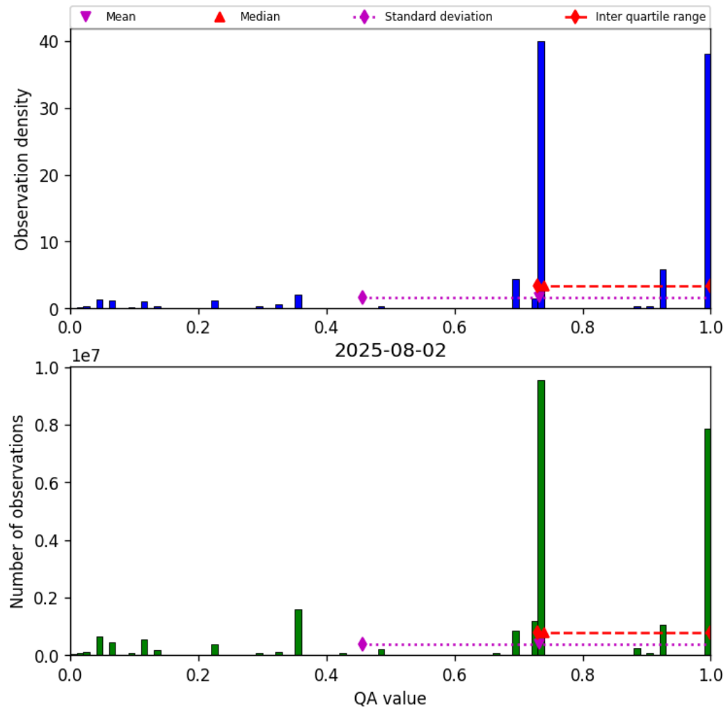
Figure 26: Histogram of “QA value” for 2025-08-02 to 2025-08-03
