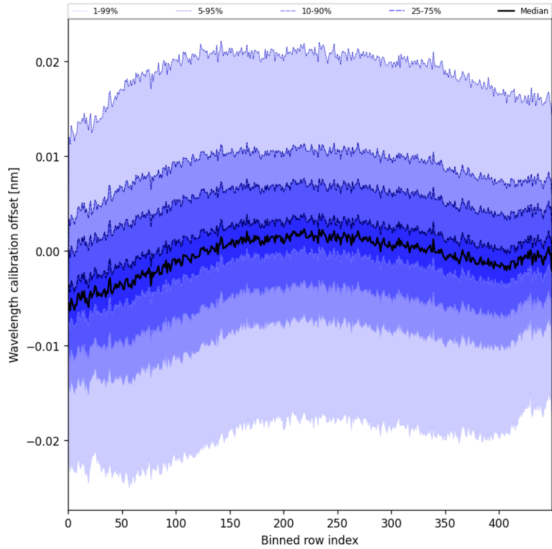
Figure 50: Along track statistics of “Wavelength calibration offset” for 2025-08-02 to 2025-08-03
