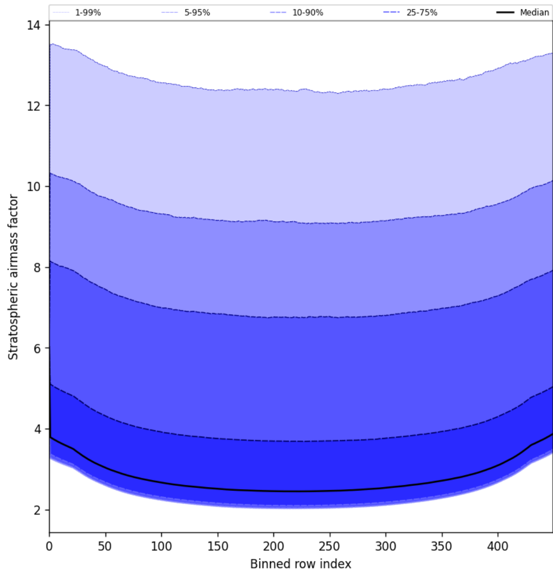
Figure 59: Along track statistics of “Stratospheric airmass factor” for 2025-08-02 to 2025-08-03
