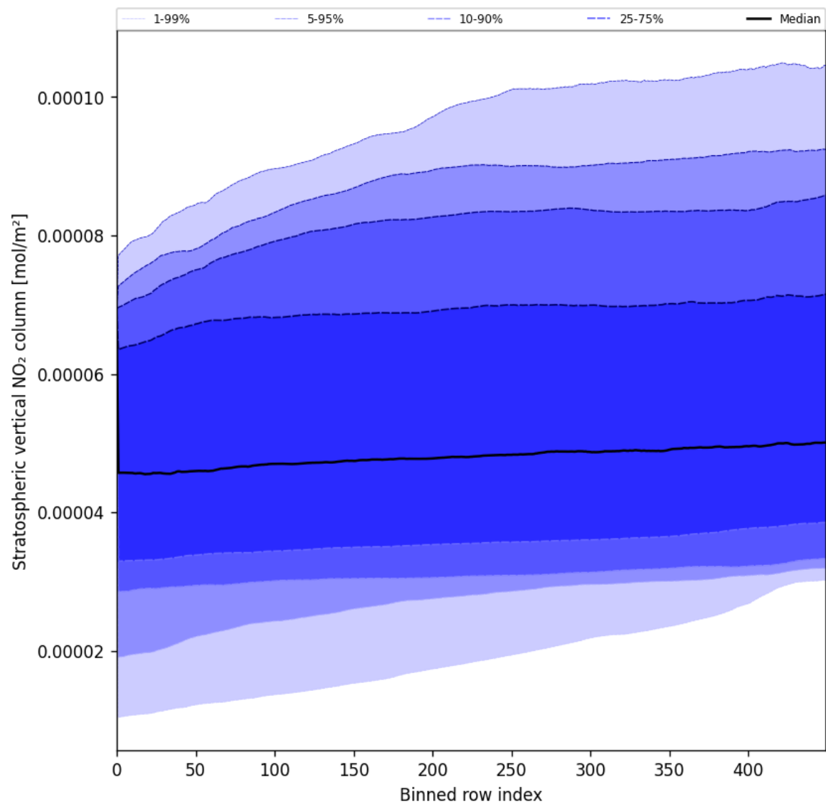
Figure 51: Along track statistics of “Stratospheric vertical NO 2 column” for 2025-08-02 to 2025-08-03
