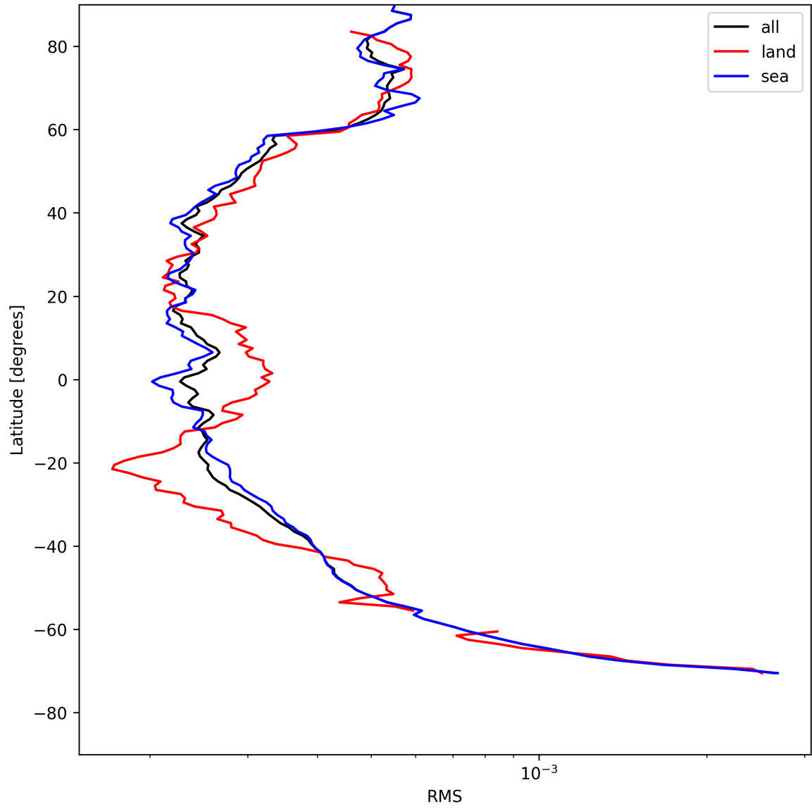
Figure 24: Zonal average of “RMS” for 2025-08-02 to 2025-08-03.
