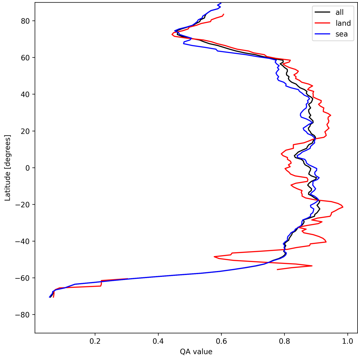
Figure 9: Zonal average of “QA value” for 2025-08-02 to 2025-08-03.
