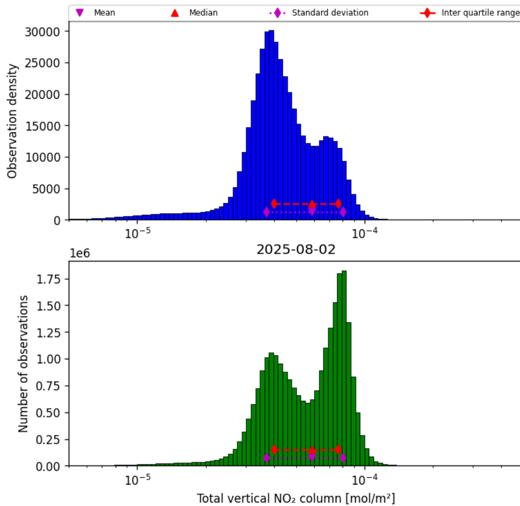
Figure 36: Histogram of “Total vertical NO 2 column” for 2025-08-02 to 2025-08-03
