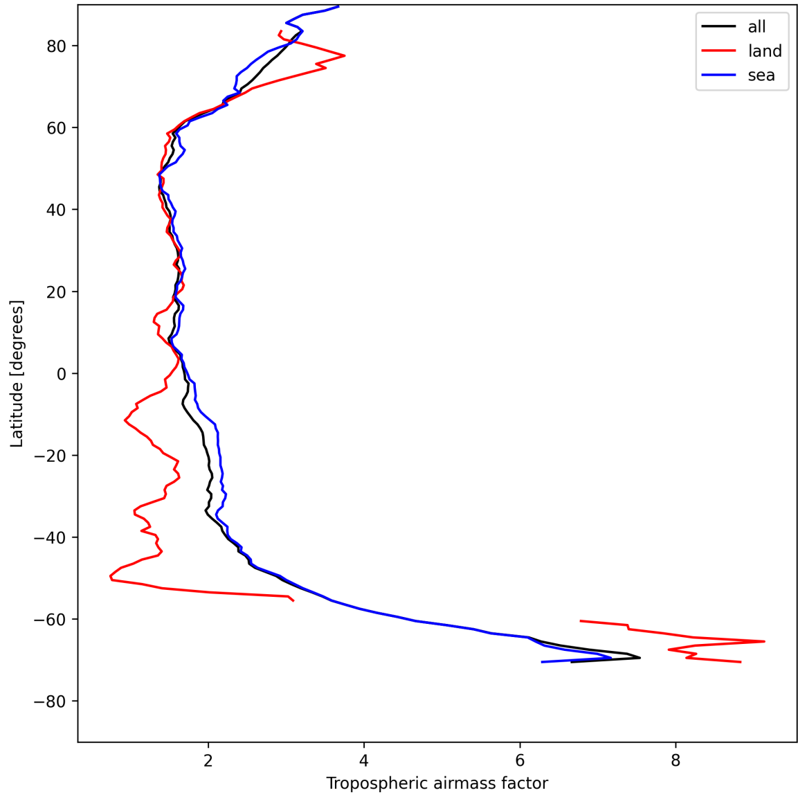
Figure 12: Zonal average of “Tropospheric airmass factor” for 2025-08-02 to 2025-08-03.
