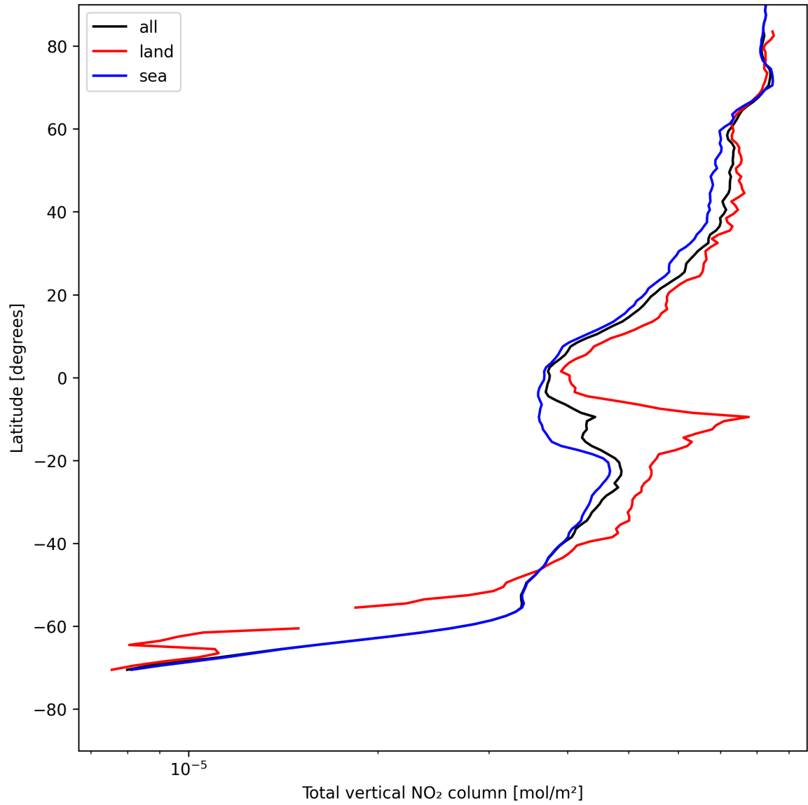
Figure 19: Zonal average of “Total vertical NO 2 column” for 2025-08-02 to 2025-08-03.
