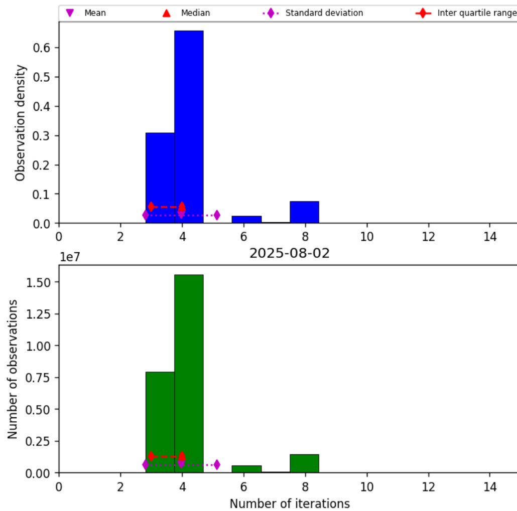
Figure 32: Histogram of “Number of iterations” for 2025-08-02 to 2025-08-03
