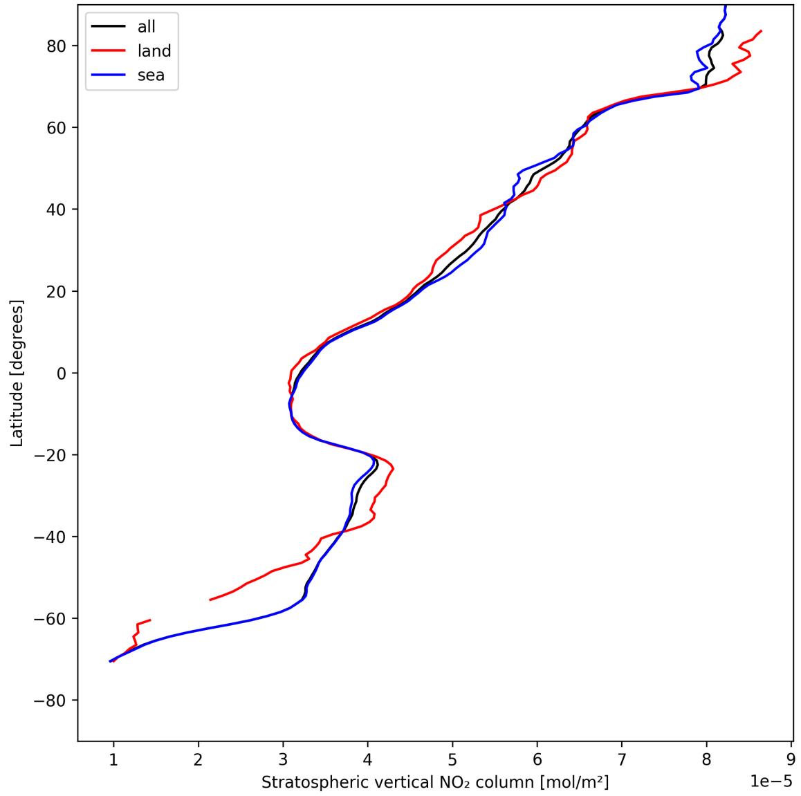
Figure 17: Zonal average of “Stratospheric vertical NO 2 column” for 2025-08-02 to 2025-08-03.
