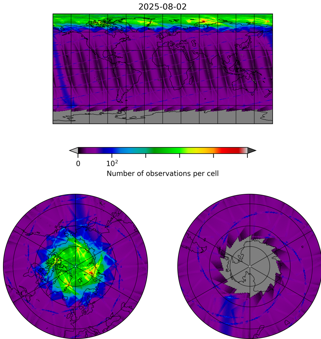
Figure 8: Map of the number of observations for 2025-08-02 to 2025-08-03
