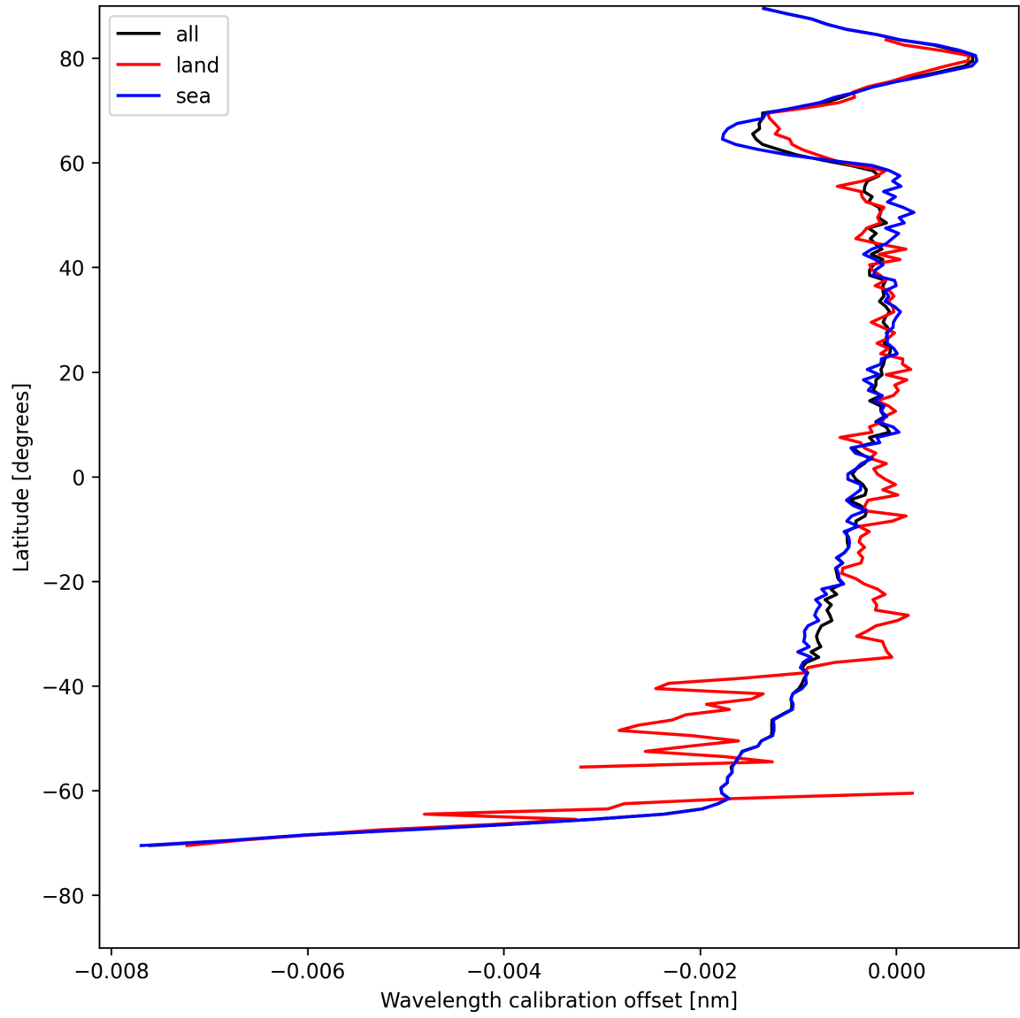
Figure 16: Zonal average of “Wavelength calibration offset” for 2025-08-02 to 2025-08-03.
