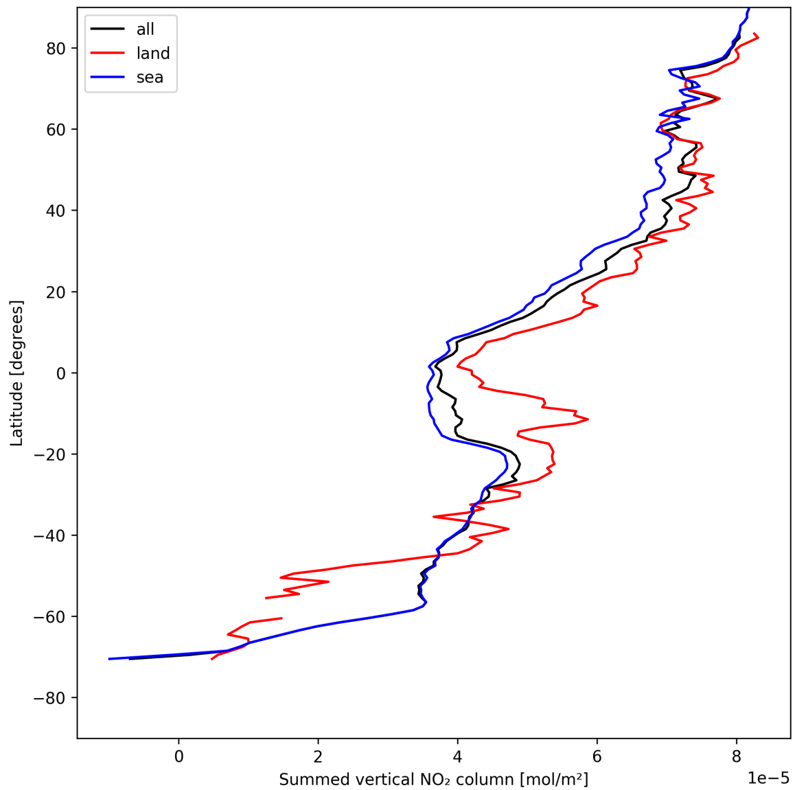
Figure 21: Zonal average of “Summed vertical NO 2 column” for 2025-08-02 to 2025-08-03.
