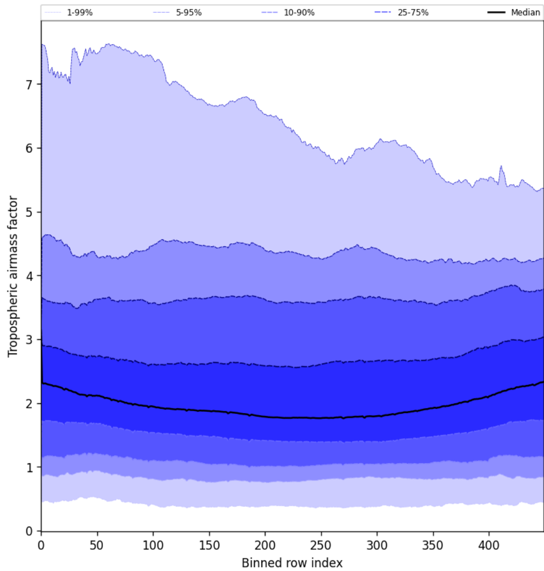
Figure 46: Along track statistics of “Tropospheric airmass factor” for 2025-08-02 to 2025-08-03
