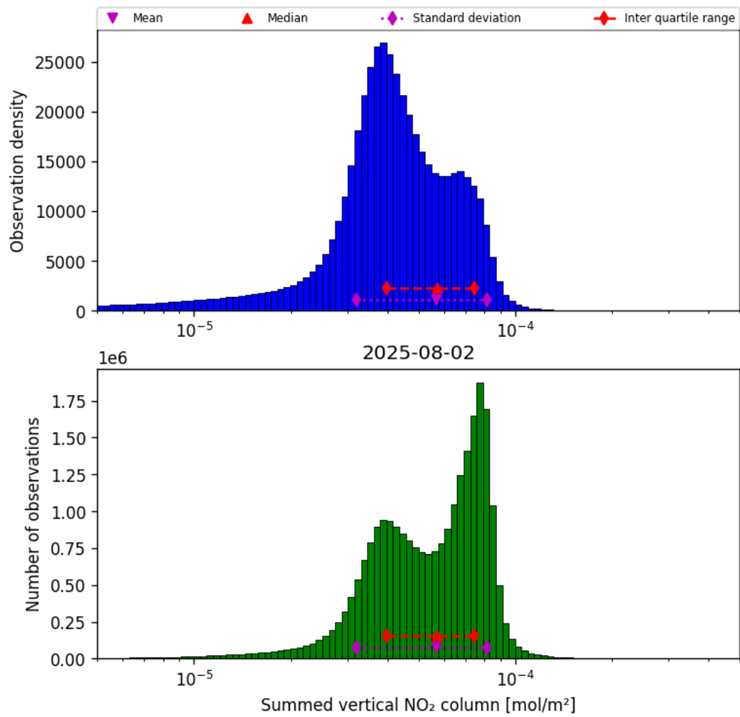
Figure 38: Histogram of “Summed vertical NO 2 column” for 2025-08-02 to 2025-08-03
