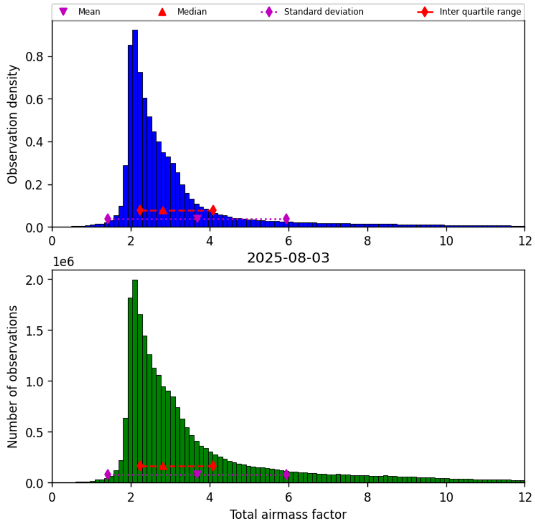
Figure 30: Histogram of “Total airmass factor” for 2025-08-03 to 2025-08-04
