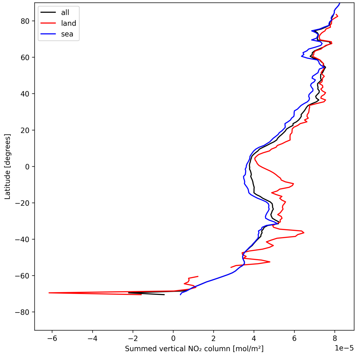
Figure 21: Zonal average of “Summed vertical NO 2 column” for 2025-08-03 to 2025-08-04.
