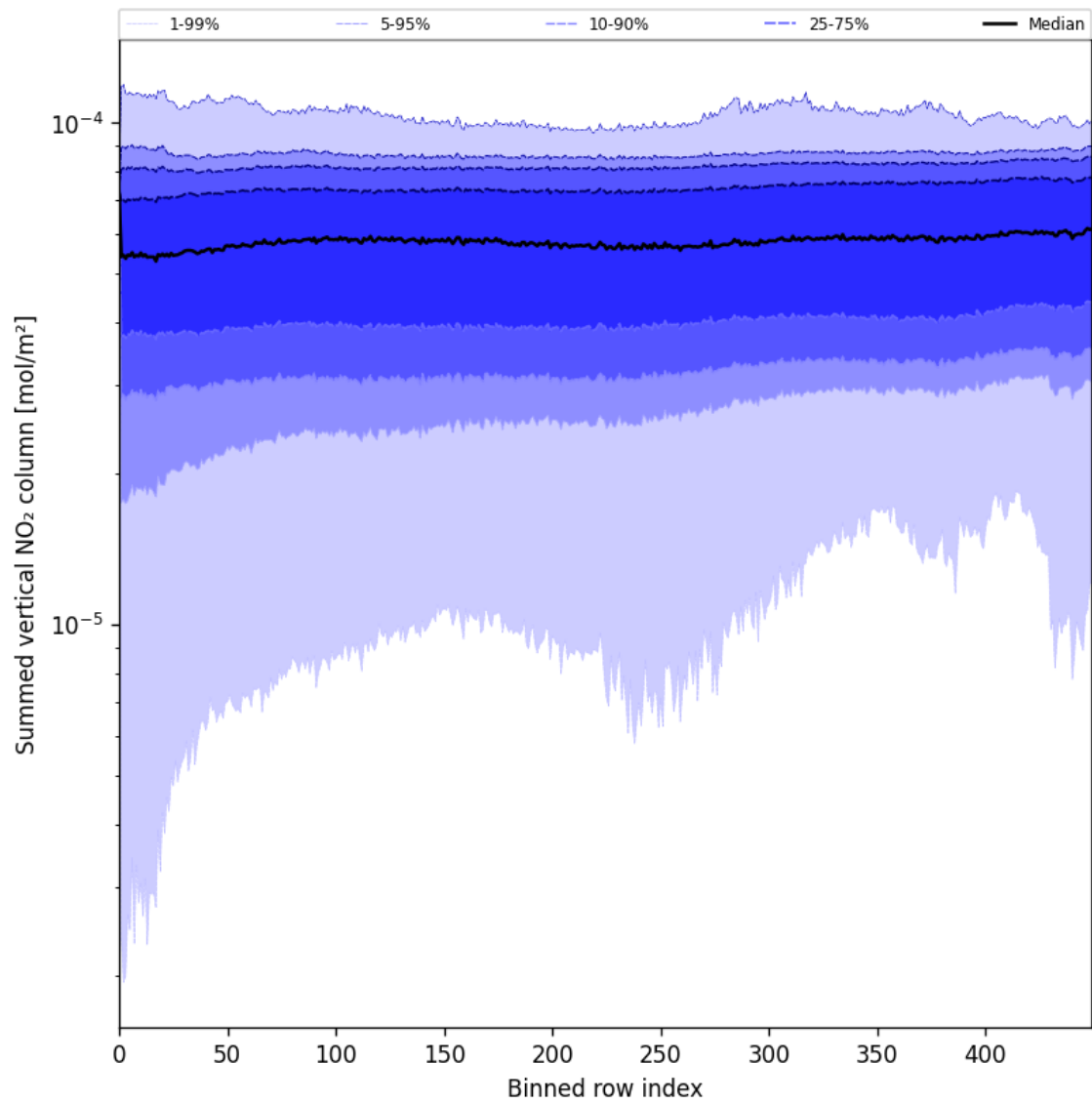
Figure 55: Along track statistics of “Summed vertical NO 2 column” for 2025-08-03 to 2025-08-04
