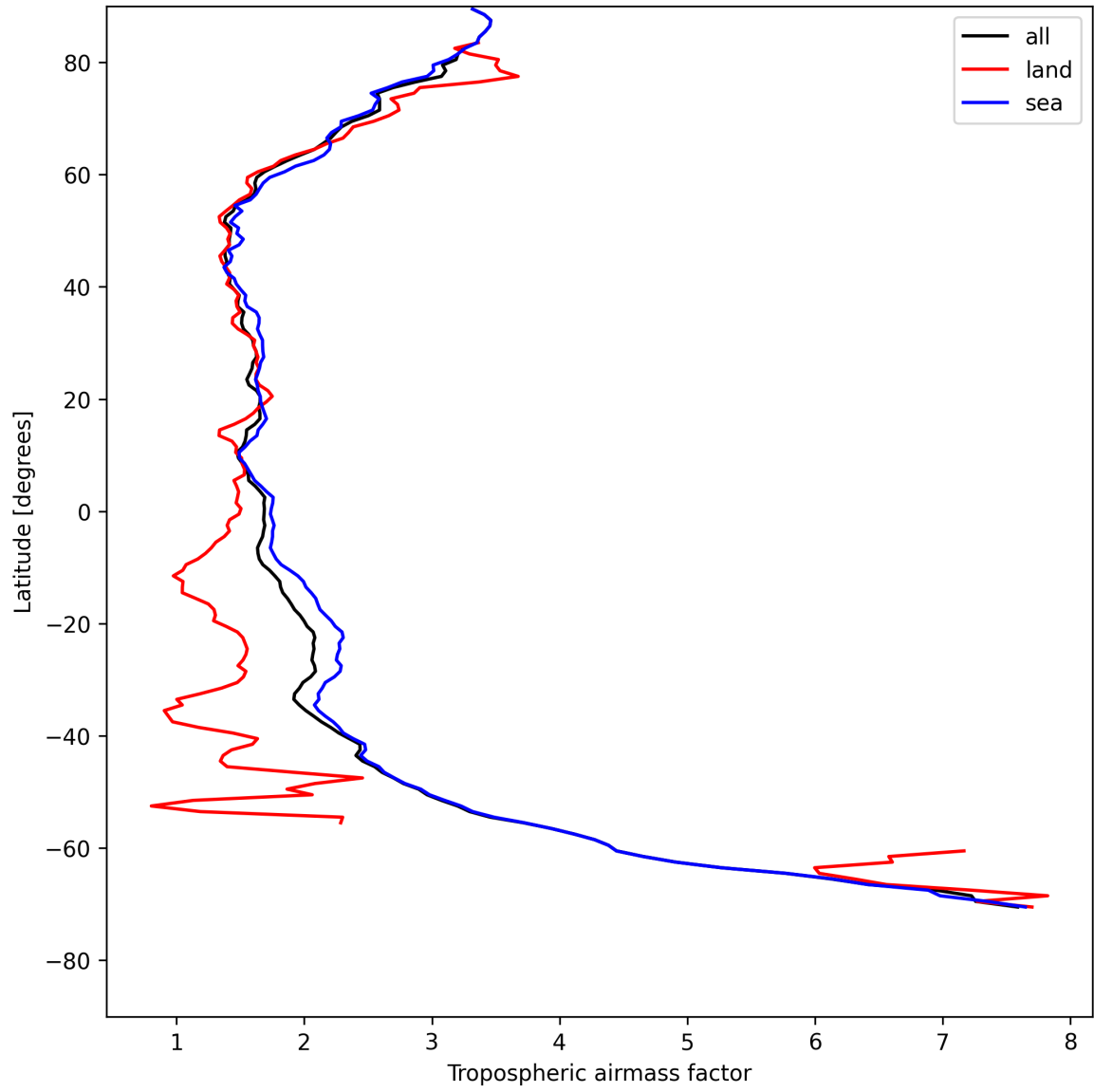
Figure 12: Zonal average of “Tropospheric airmass factor” for 2025-08-03 to 2025-08-04.
