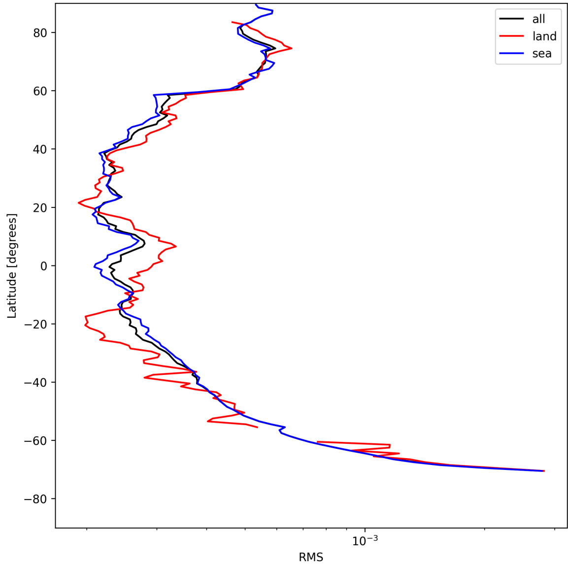
Figure 24: Zonal average of “RMS” for 2025-08-03 to 2025-08-04.
