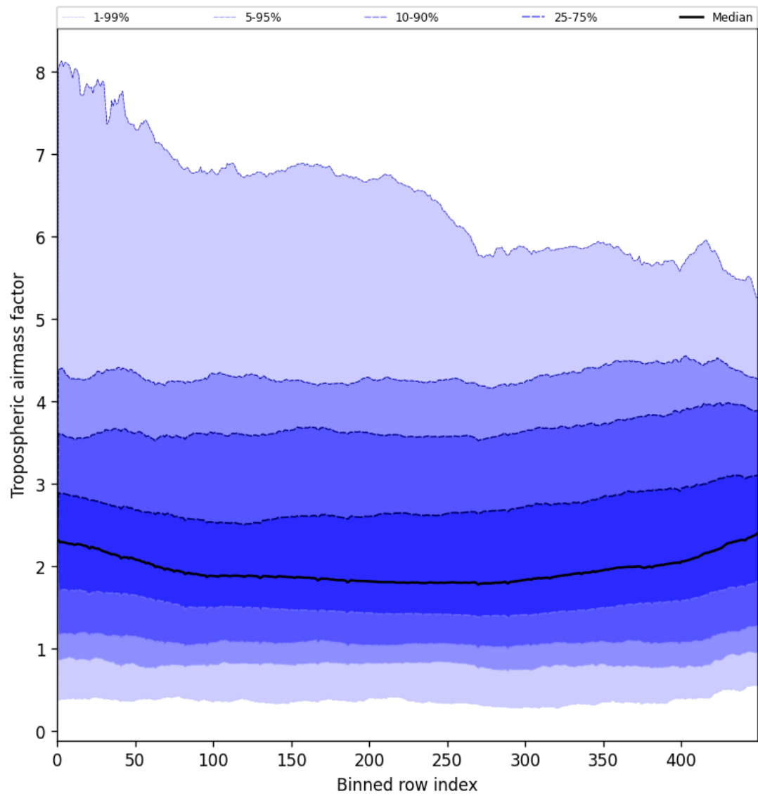
Figure 46: Along track statistics of “Tropospheric air mass factor” for 2025-08-03 to 2025-08-04
