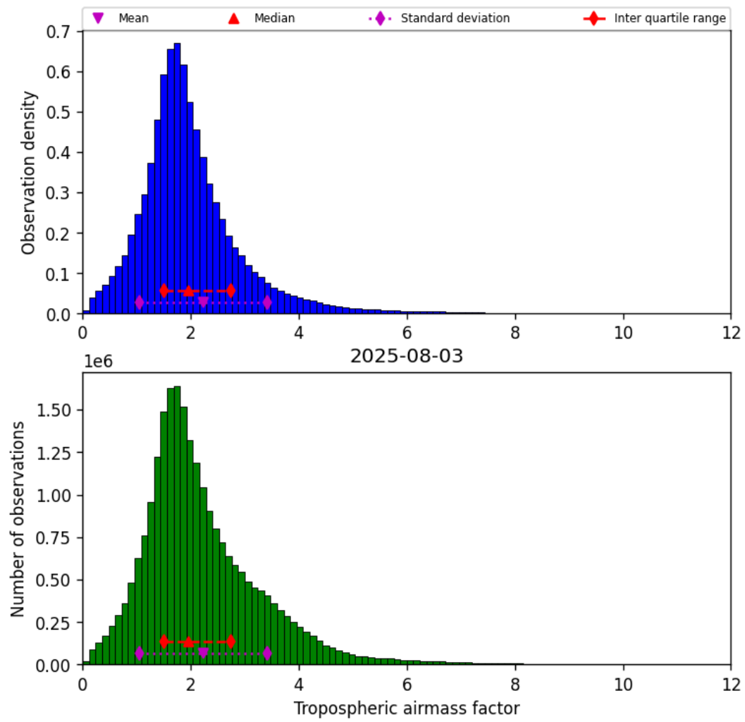
Figure 29: Histogram of “Tropospheric airmass factor” for 2025-08-03 to 2025-08-04
