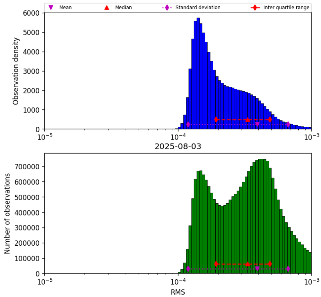
Figure 41: Histogram of “RMS” for 2025-08-03 to 2025-08-04
