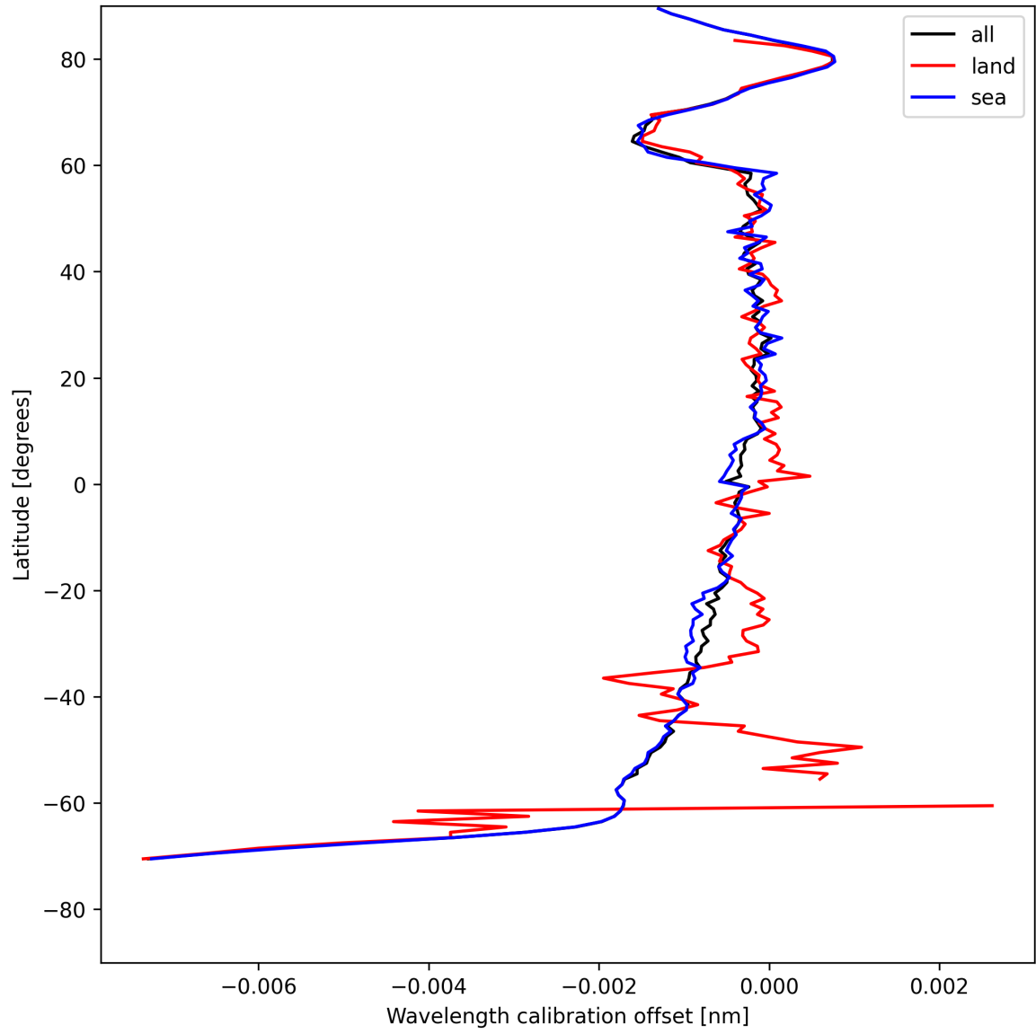
Figure 16: Zonal average of “Wavelength calibration offset” for 2025-08-03 to 2025-08-04.
