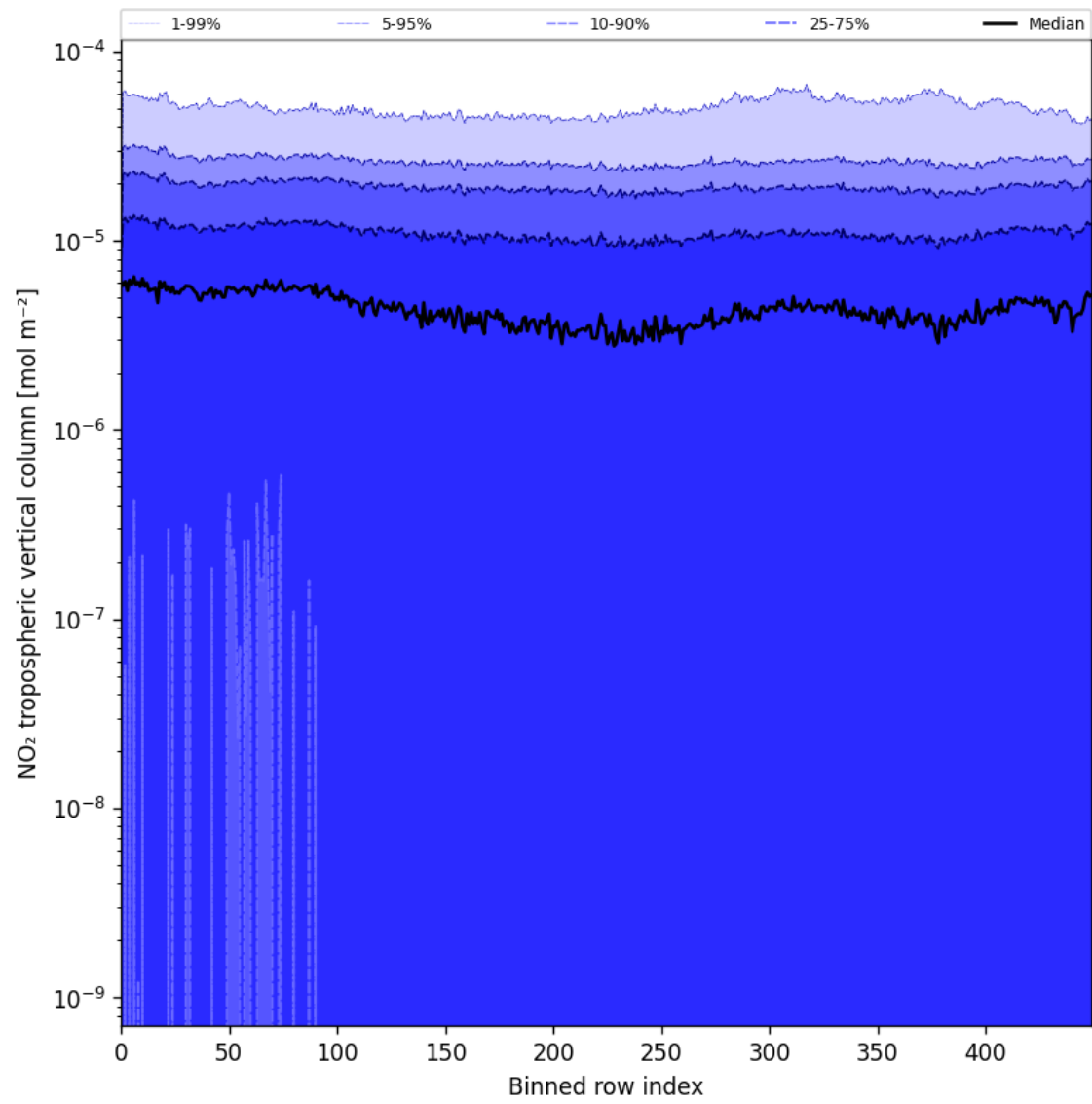
Figure 44: Along track statistics of “NO 2 tropospheric vertical column” for 2025-08-03 to 2025-08-04
