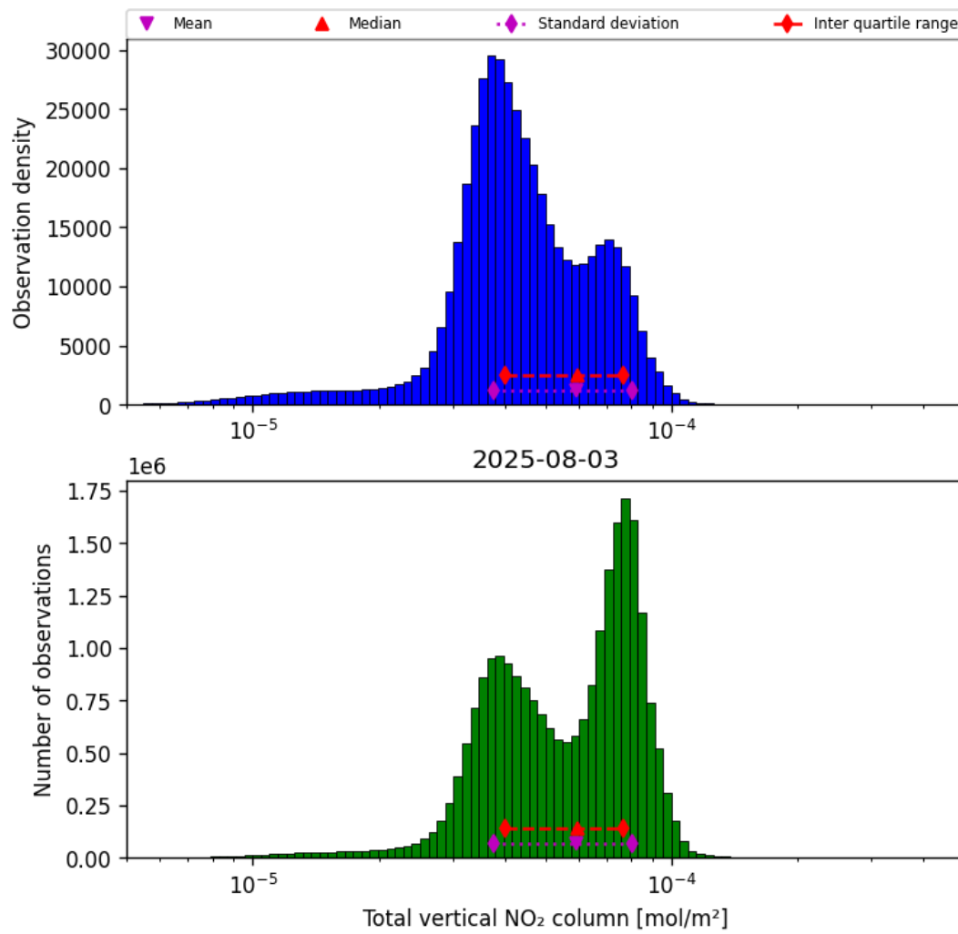
Figure 36: Histogram of “Total vertical NO 2 column” for 2025-08-03 to 2025-08-04
