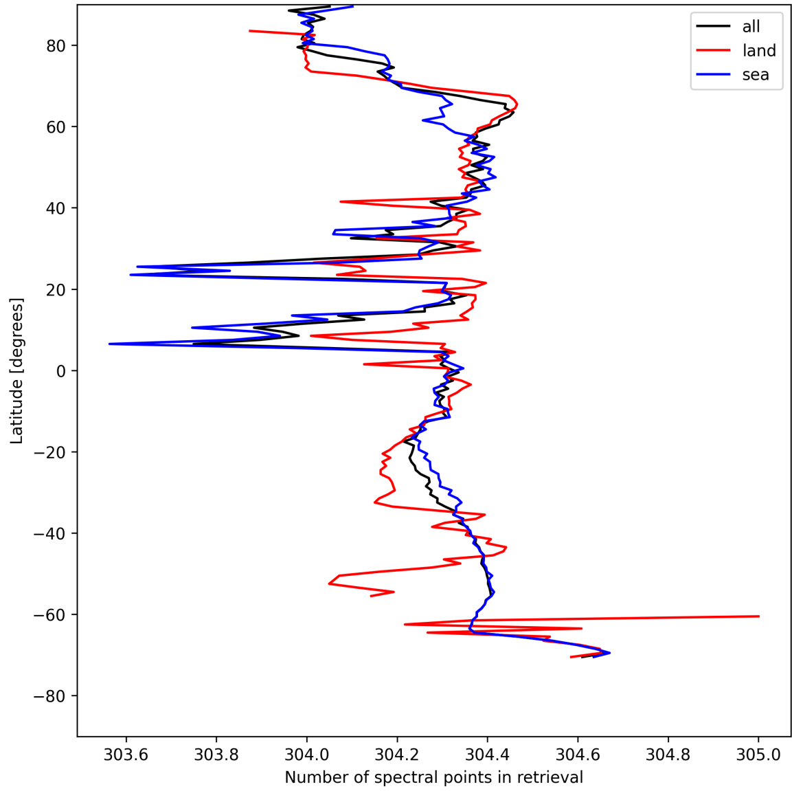
Figure 14: Zonal average of “Number of spectral points in retrieval” for 2025-08-03 to 2025-08-04.
