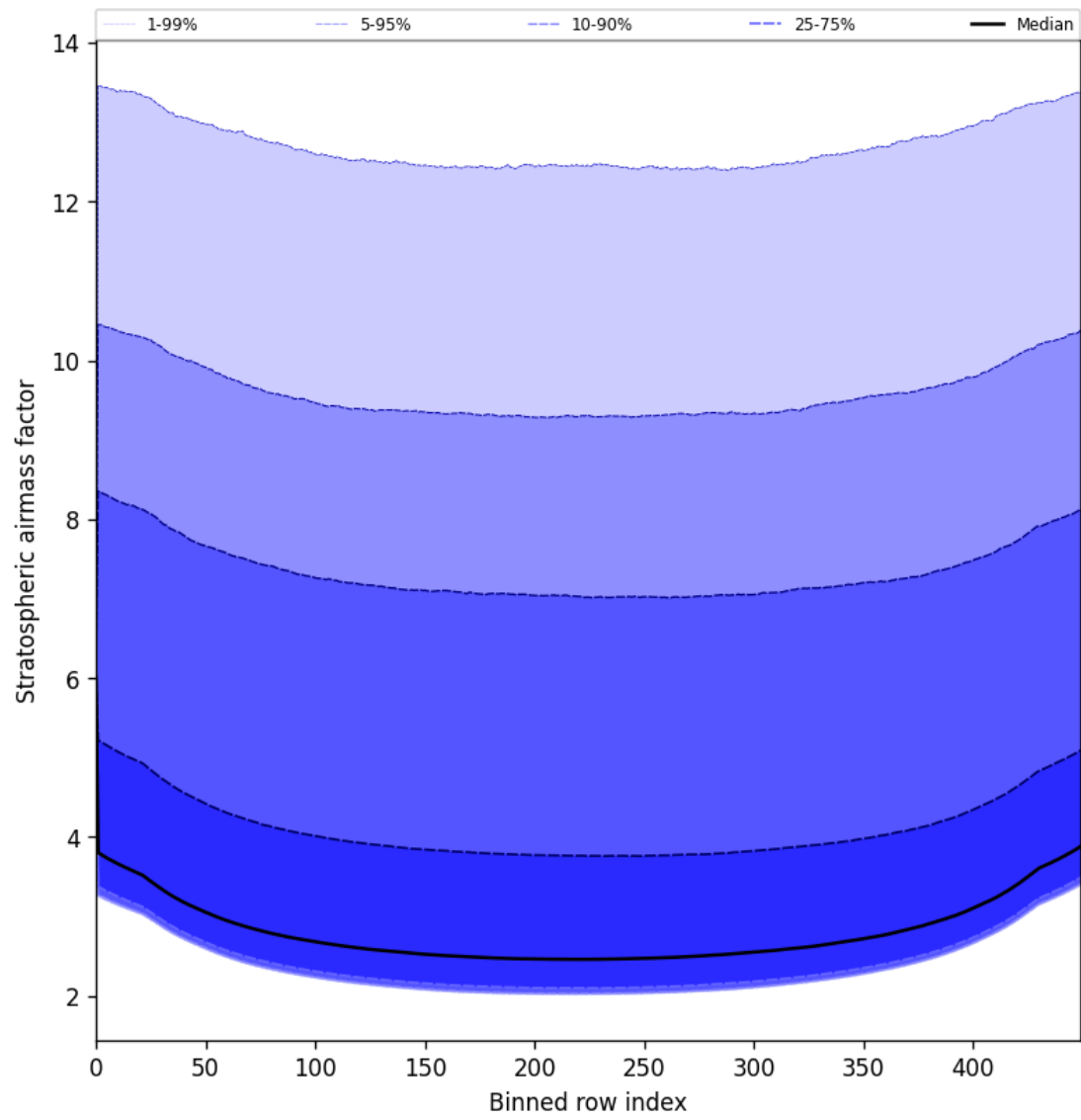
Figure 59: Along track statistics of “Stratospheric airmass factor” for 2025-08-03 to 2025-08-04
