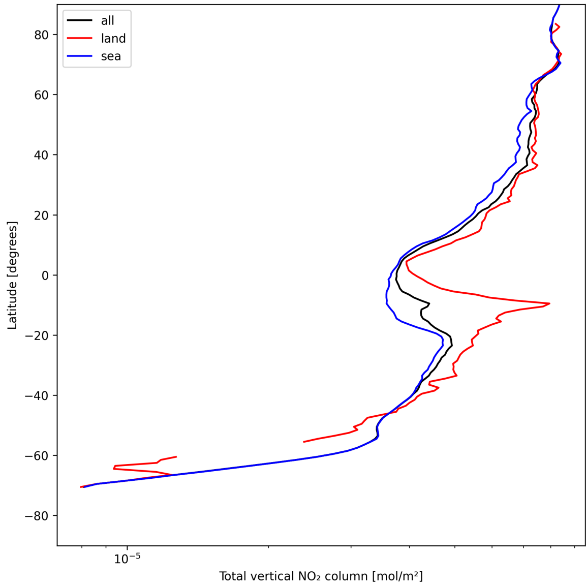
Figure 19: Zonal average of “Total vertical NO 2 column” for 2025-08-03 to 2025-08-04.
