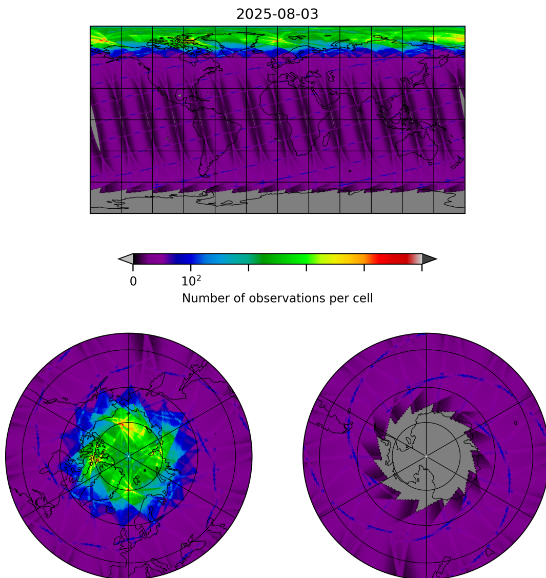
Figure 8: Map of the number of observations for 2025-08-03 to 2025-08-04
