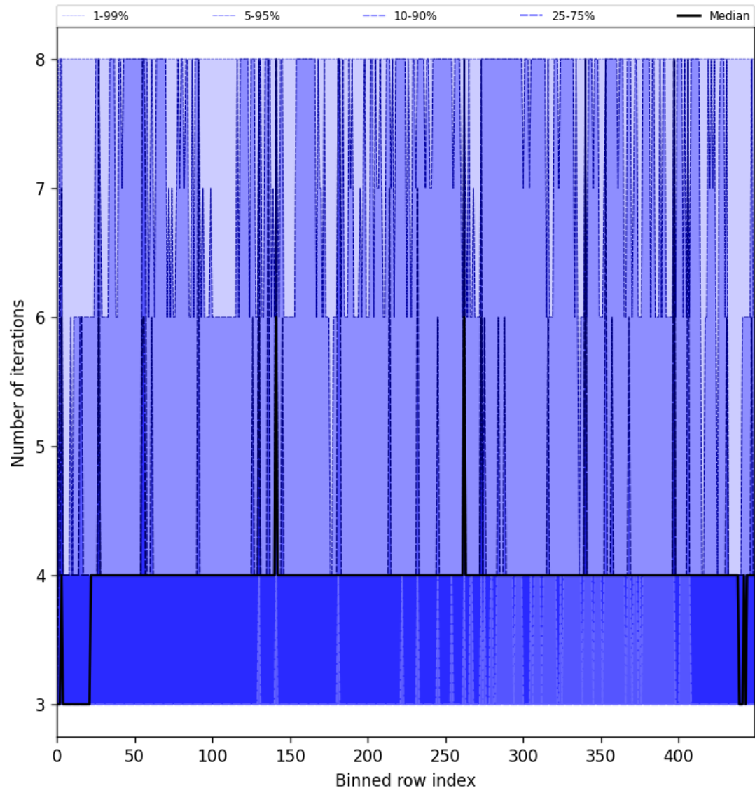
Figure 49: Along track statistics of “Number of iterations” for 2025-08-03 to 2025-08-04
