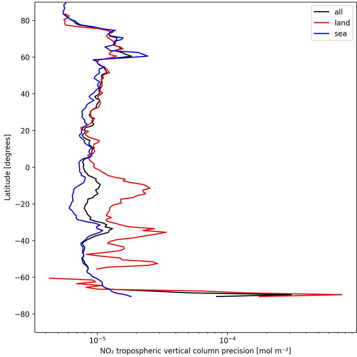
Figure 11: Zonal average of “NO 2 tropospheric vertical column precision” for 2025-08-03 to 2025-08-04.
