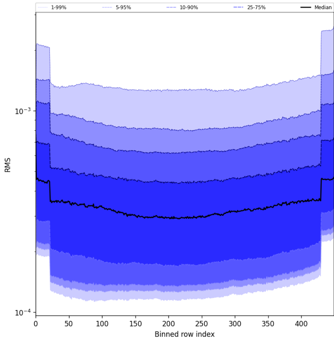
Figure 58: Along track statistics of “RMS” for 2025-08-03 to 2025-08-04
