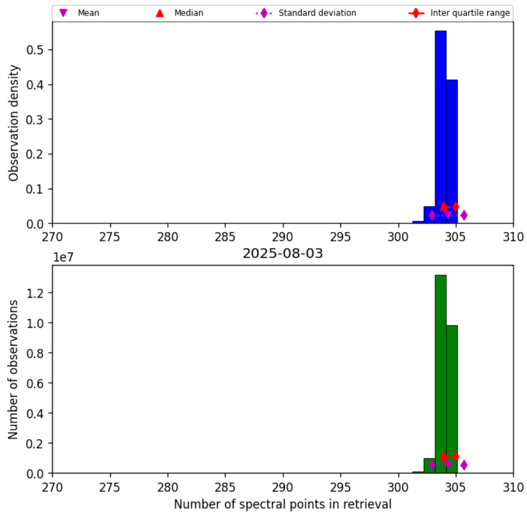
Figure 31: Histogram of “Number of spectral points in retrieval” for 2025-08-03 to 2025-08-04
