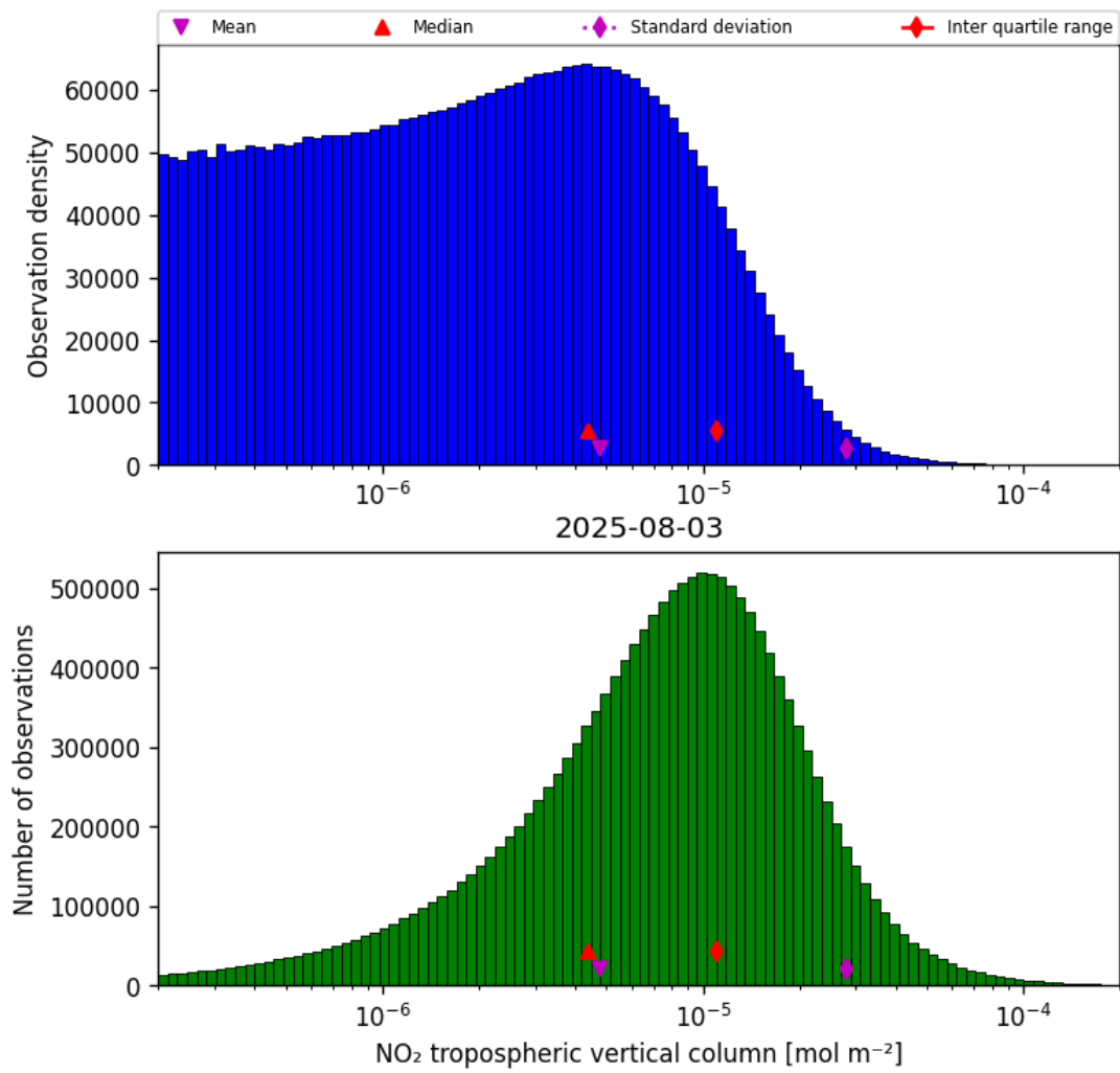
Figure 27: Histogram of “NO 2 tropospheric vertical column” for 2025-08-03 to 2025-08-04
