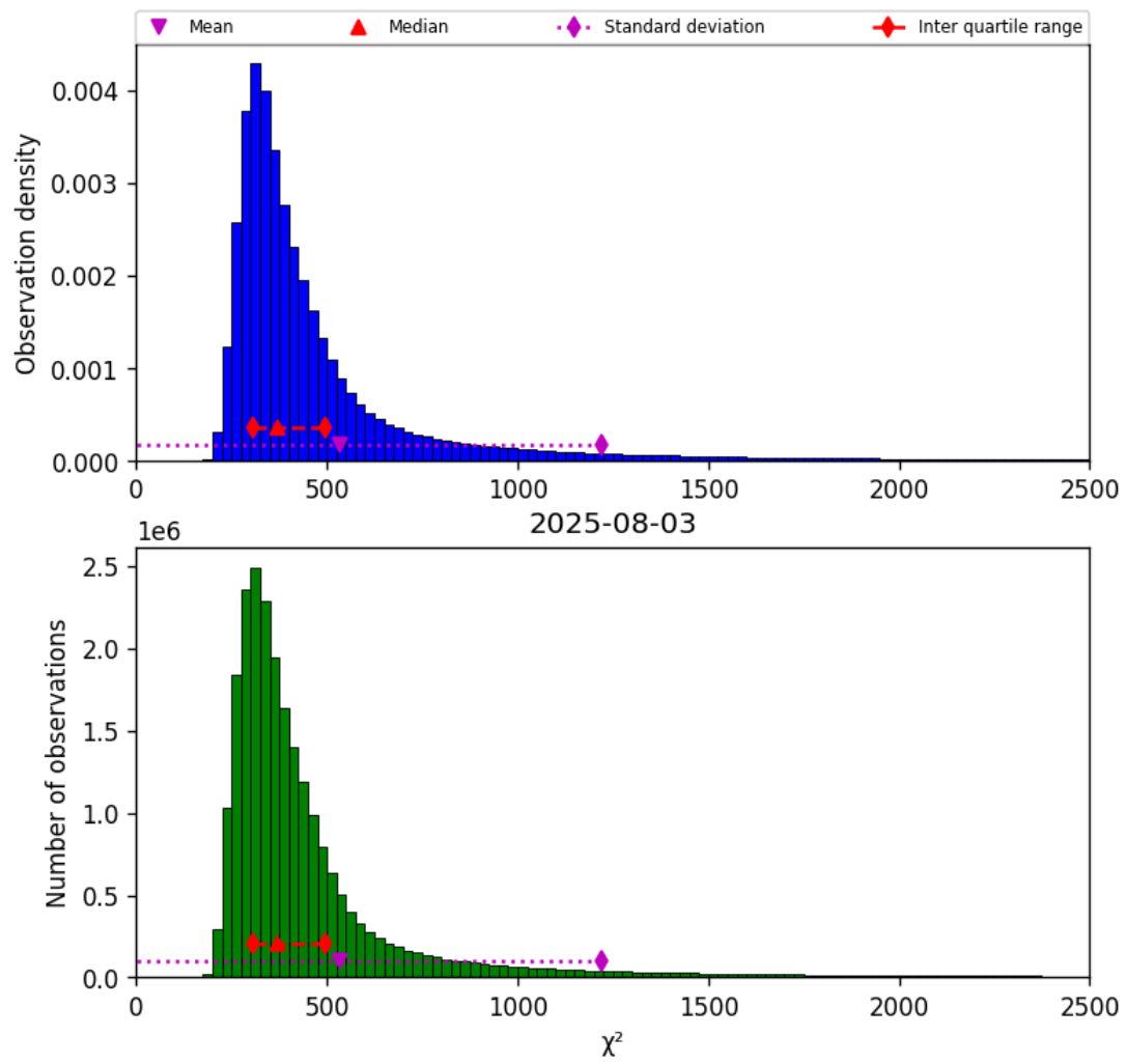
Figure 40: Histogram of “ \chi^2 ” for 2025-08-03 to 2025-08-04
