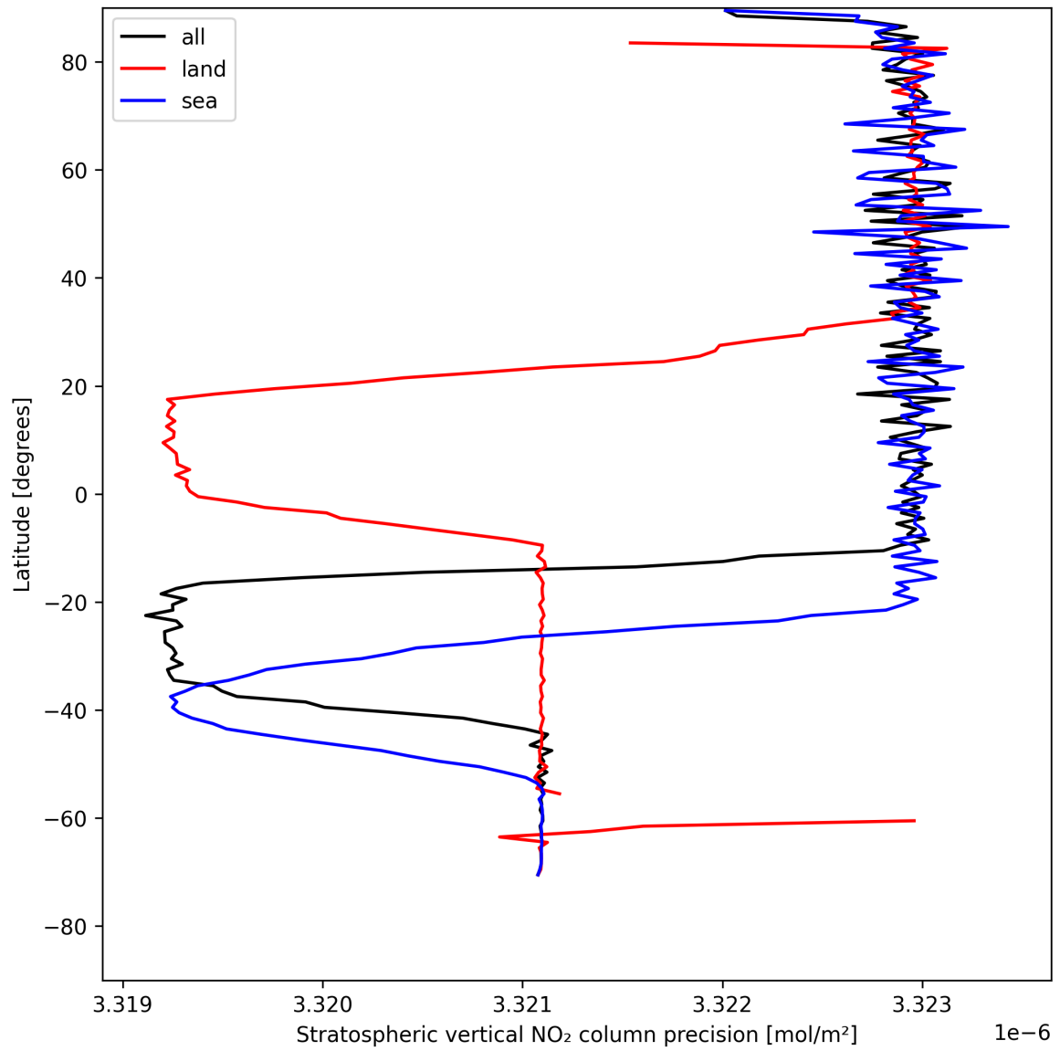
Figure 18: Zonal average of “Stratospheric vertical NO 2 column precision” for 2025-08-03 to 2025-08-04.
