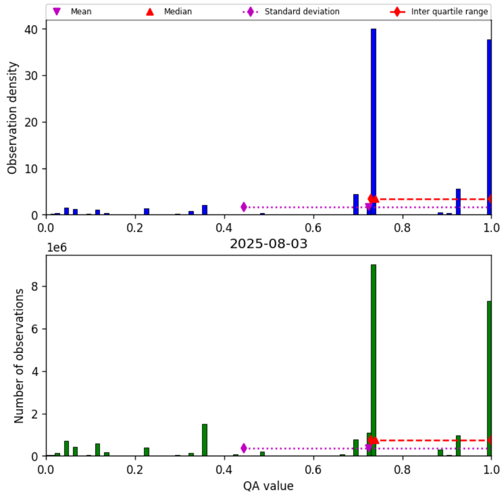
Figure 26: Histogram of “QA value” for 2025-08-03 to 2025-08-04
