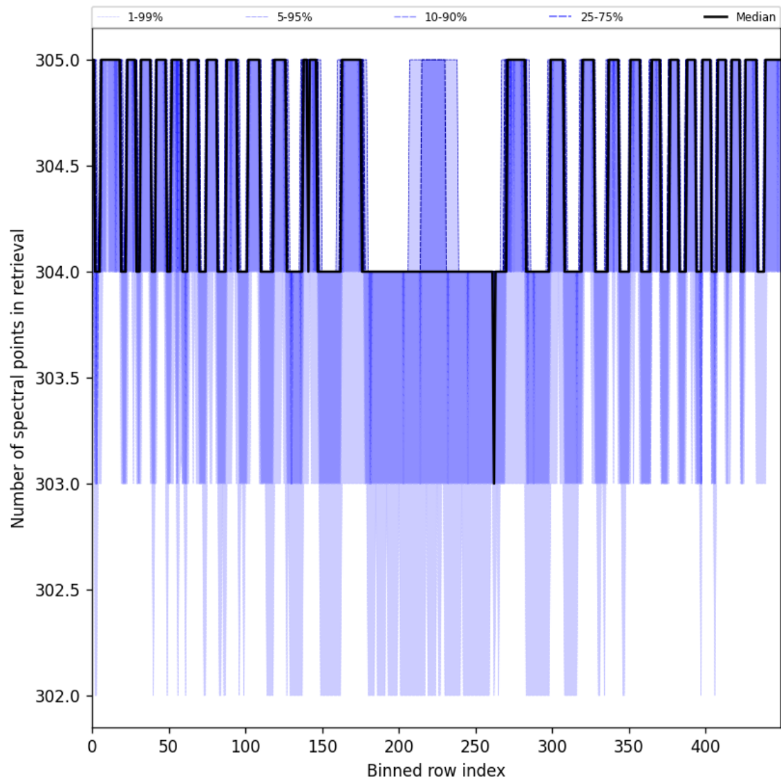
Figure 48: Along track statistics of “Number of spectral points in retrieval” for 2025-08-03 to 2025-08-04
