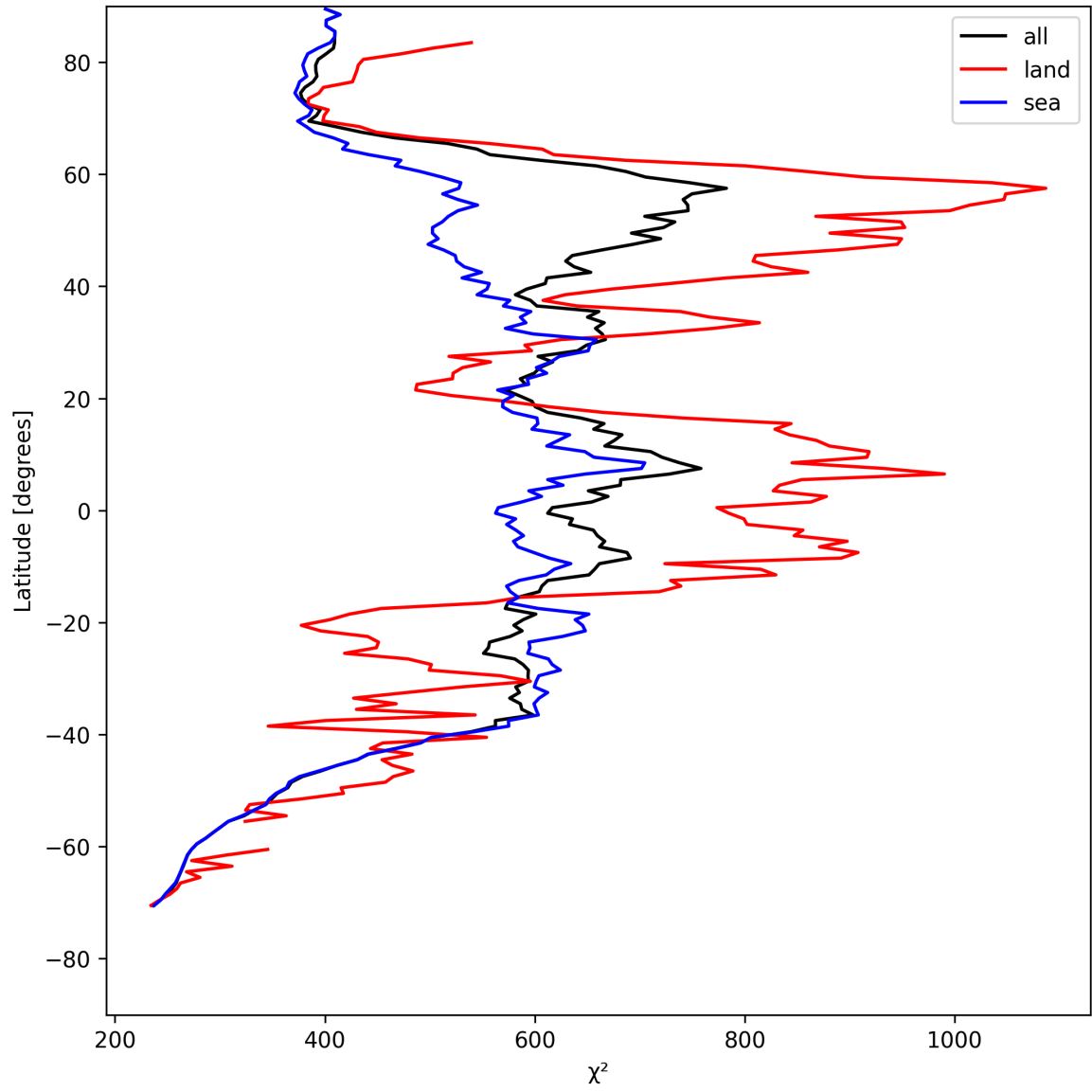
Figure 23: Zonal average of “ \chi^2 ” for 2025-08-03 to 2025-08-04.
