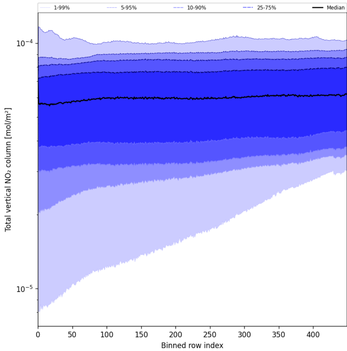
Figure 53: Along track statistics of “Total vertical NO 2 column” for 2025-08-03 to 2025-08-04
