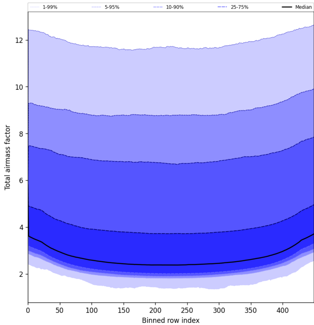
Figure 47: Along track statistics of “Total airmass factor” for 2025-08-03 to 2025-08-04
