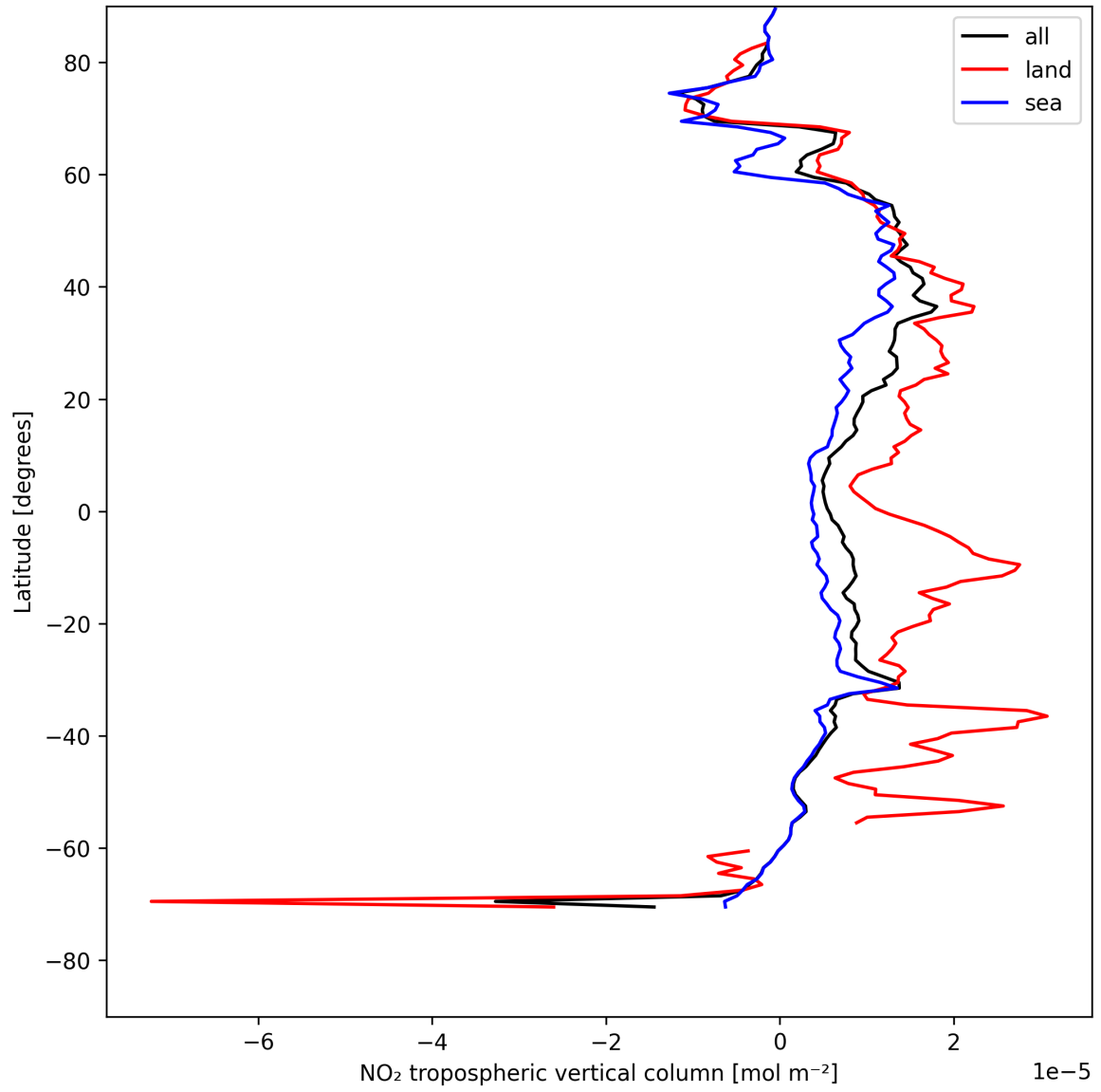
Figure 10: Zonal average of “NO 2 tropospheric vertical column” for 2025-08-03 to 2025-08-04.
