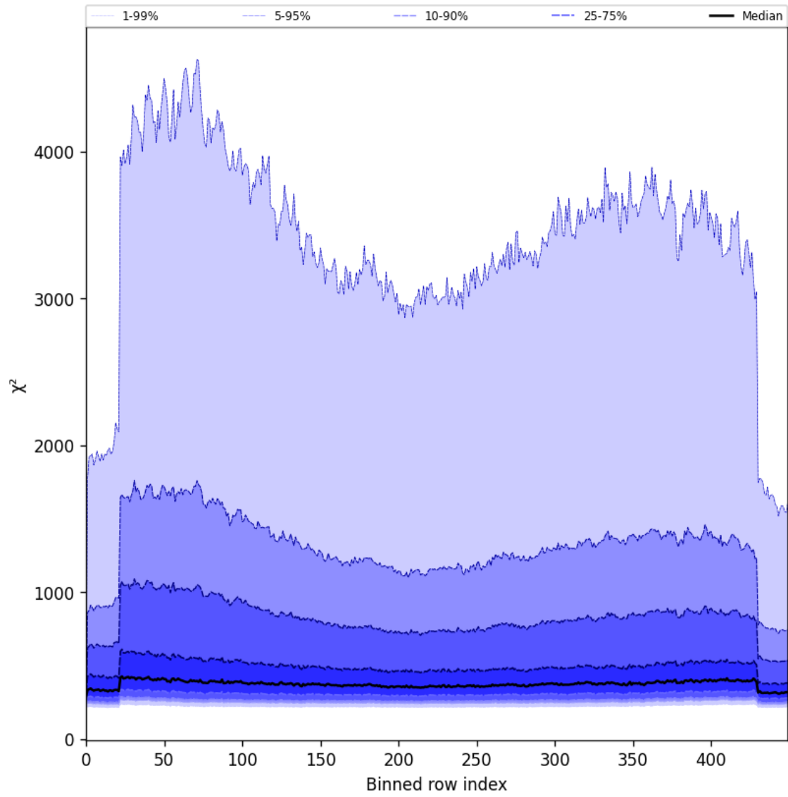
Figure 57: Along track statistics of “ \chi^2 ” for 2025-08-03 to 2025-08-04
