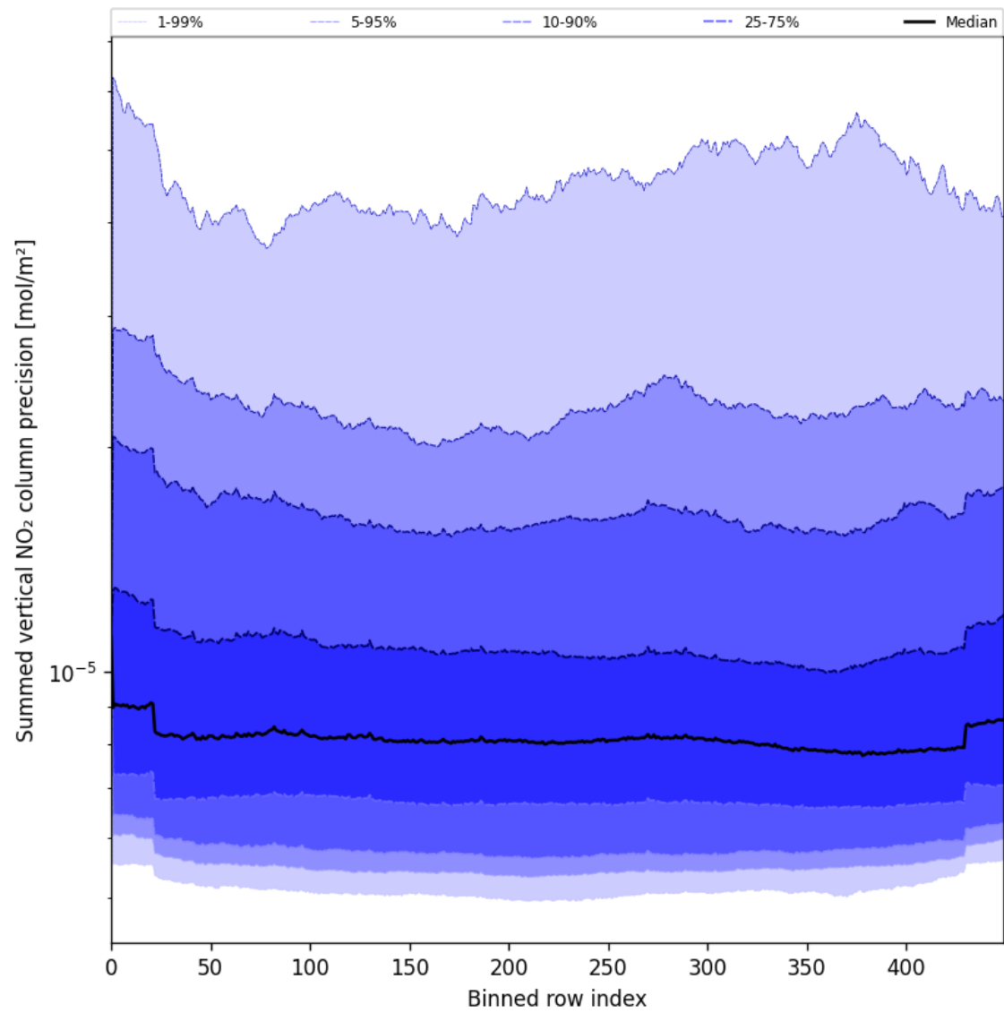
Figure 56: Along track statistics of “Summed vertical NO 2 column precision” for 2025-08-03 to 2025-08-04
