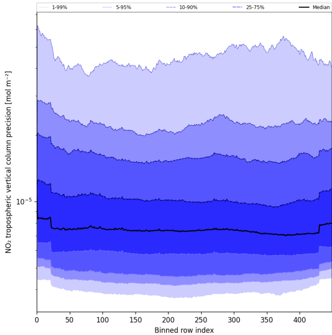
Figure 45: Along track statistics of “NO 2 tropospheric vertical column precision” for 2025-08-03 to 2025-08-04
