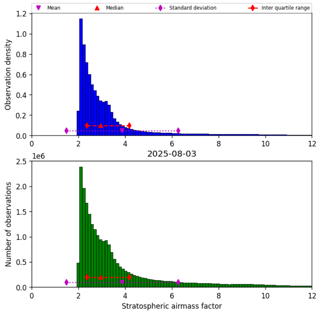
Figure 42: Histogram of “Stratospheric airmass factor” for 2025-08-03 to 2025-08-04
