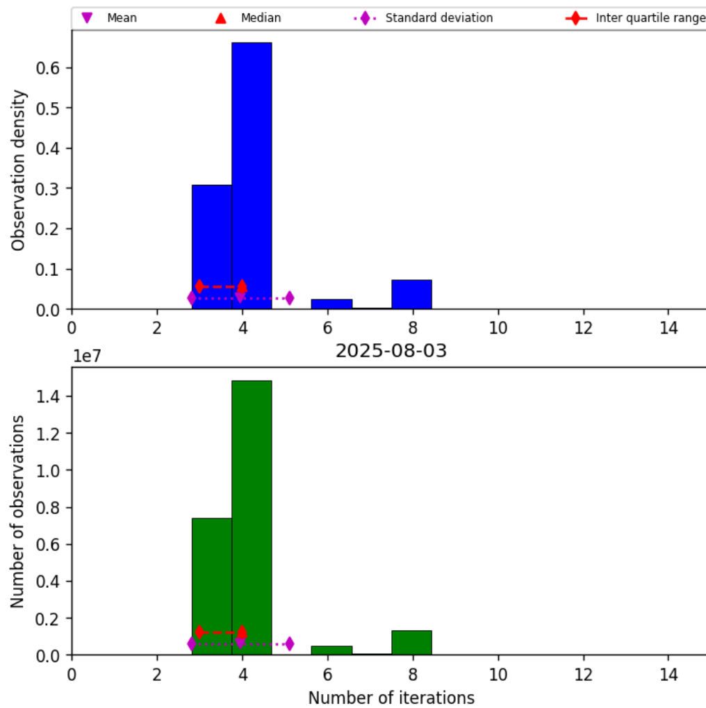
Figure 32: Histogram of “Number of iterations” for 2025-08-03 to 2025-08-04
