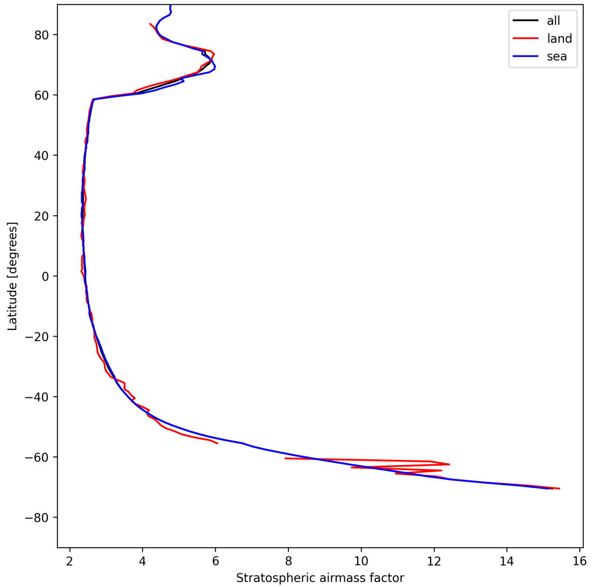
Figure 25: Zonal average of “Stratospheric airmass factor” for 2025-08-03 to 2025-08-04.
