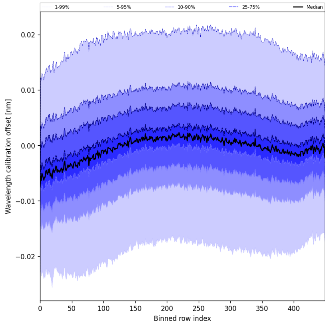
Figure 50: Along track statistics of “Wavelength calibration offset” for 2025-08-03 to 2025-08-04
