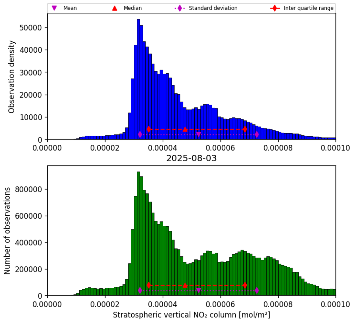
Figure 34: Histogram of “Stratospheric vertical NO 2 column” for 2025-08-03 to 2025-08-04
