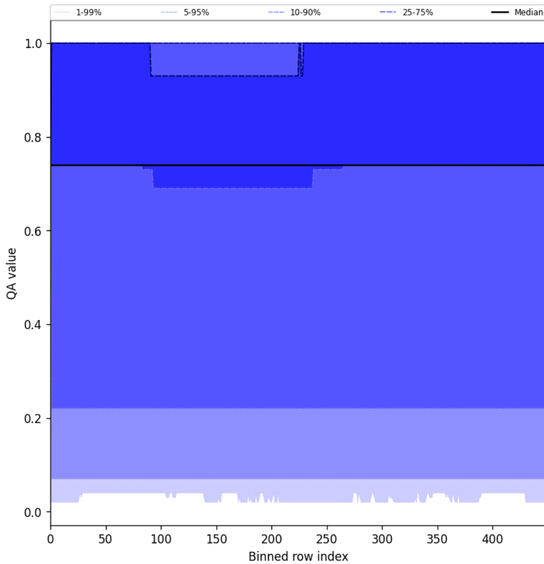
Figure 43: Along track statistics of “QA value” for 2025-08-03 to 2025-08-04
