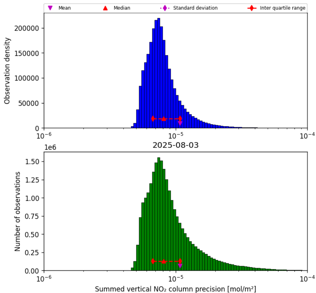
Figure 39: Histogram of “Summed vertical NO 2 column precision” for 2025-08-03 to 2025-08-04
