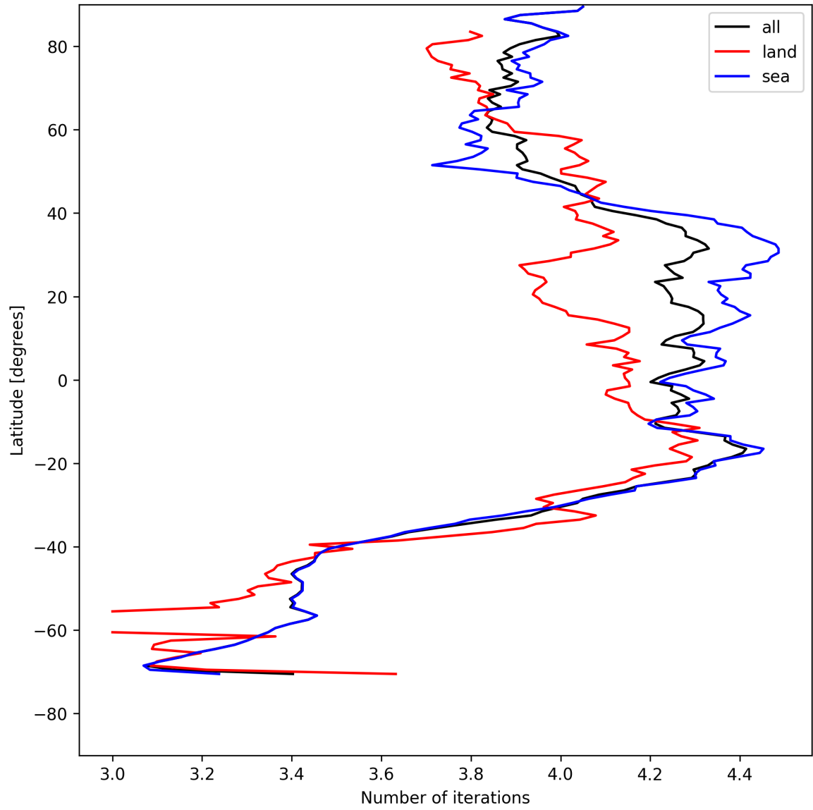
Figure 15: Zonal average of “Number of iterations” for 2025-08-03 to 2025-08-04.
