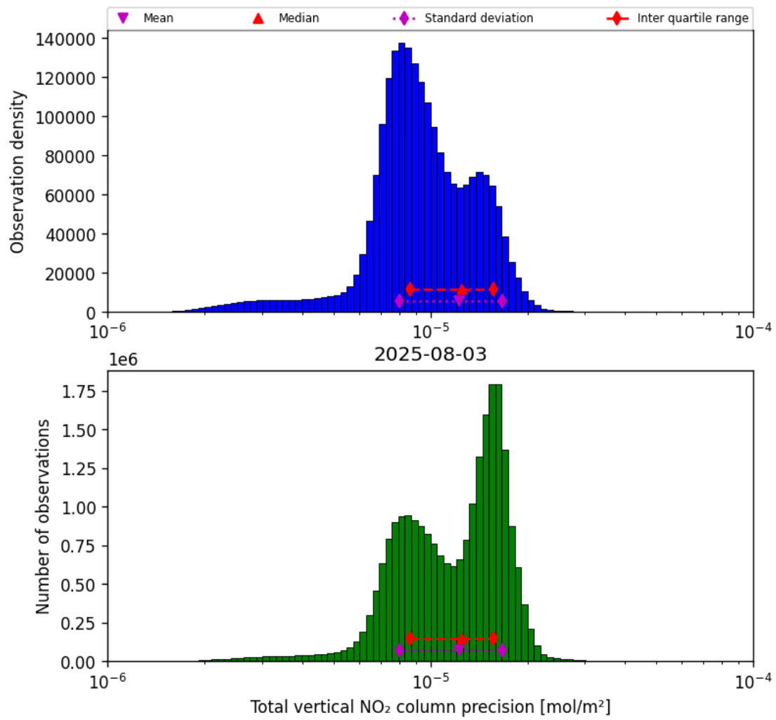
Figure 37: Histogram of “Total vertical NO 2 column precision” for 2025-08-03 to 2025-08-04
