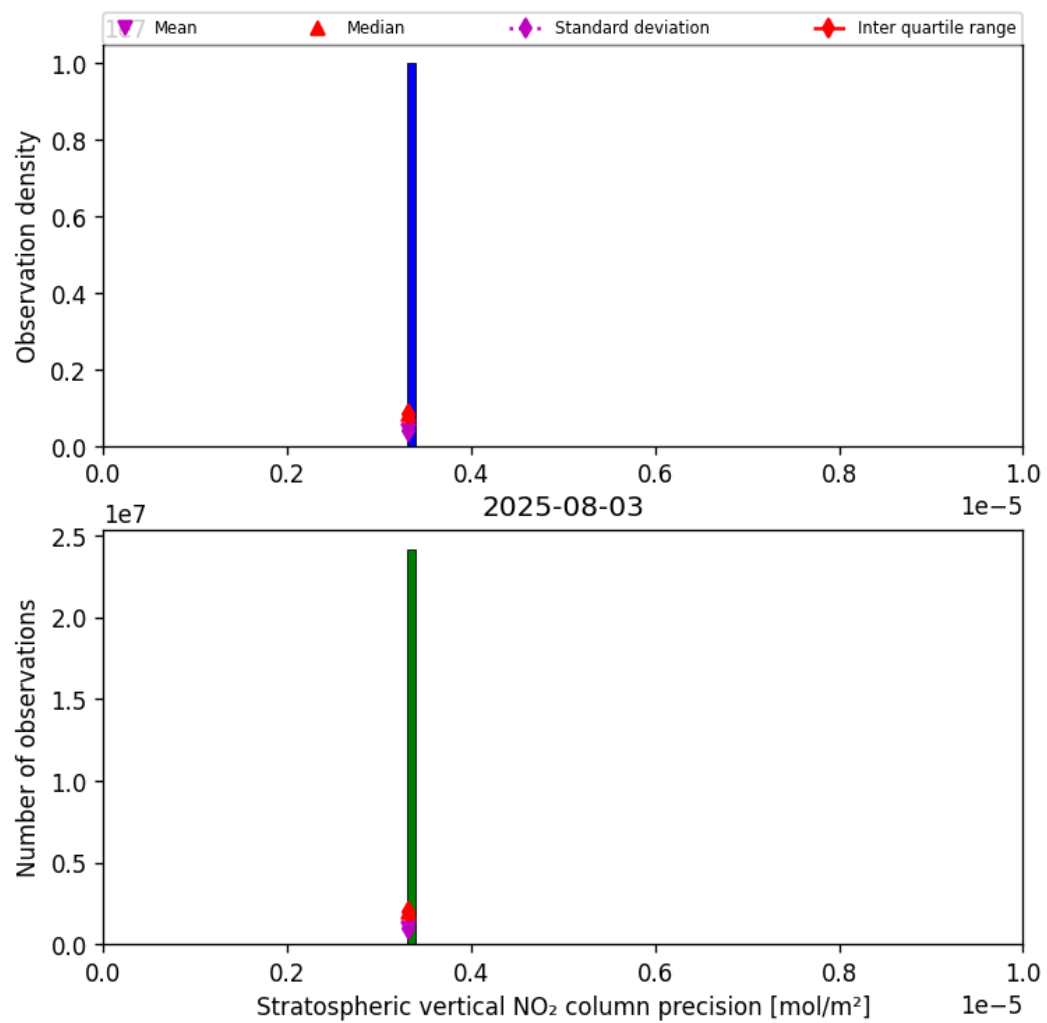
Figure 35: Histogram of “Stratospheric vertical NO 2 column precision” for 2025-08-03 to 2025-08-04
