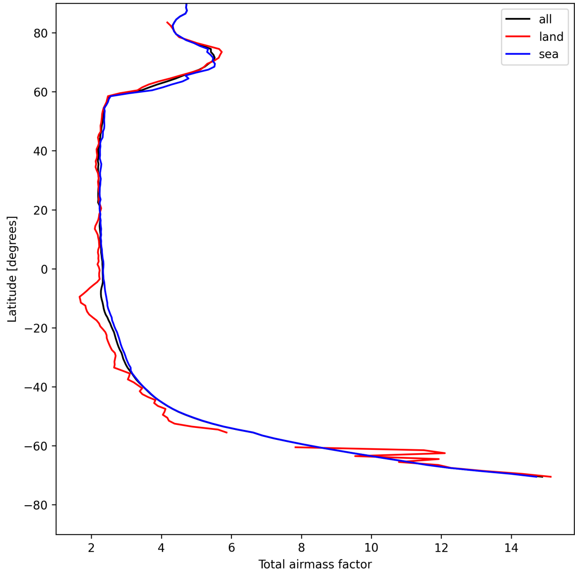
Figure 13: Zonal average of “Total airmass factor” for 2025-08-03 to 2025-08-04.
