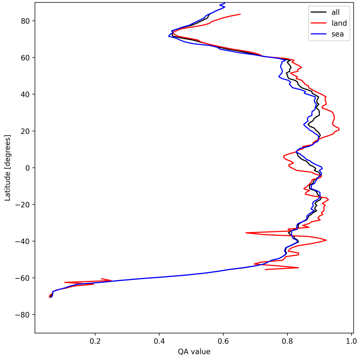
Figure 9: Zonal average of “QA value” for 2025-08-03 to 2025-08-04.
