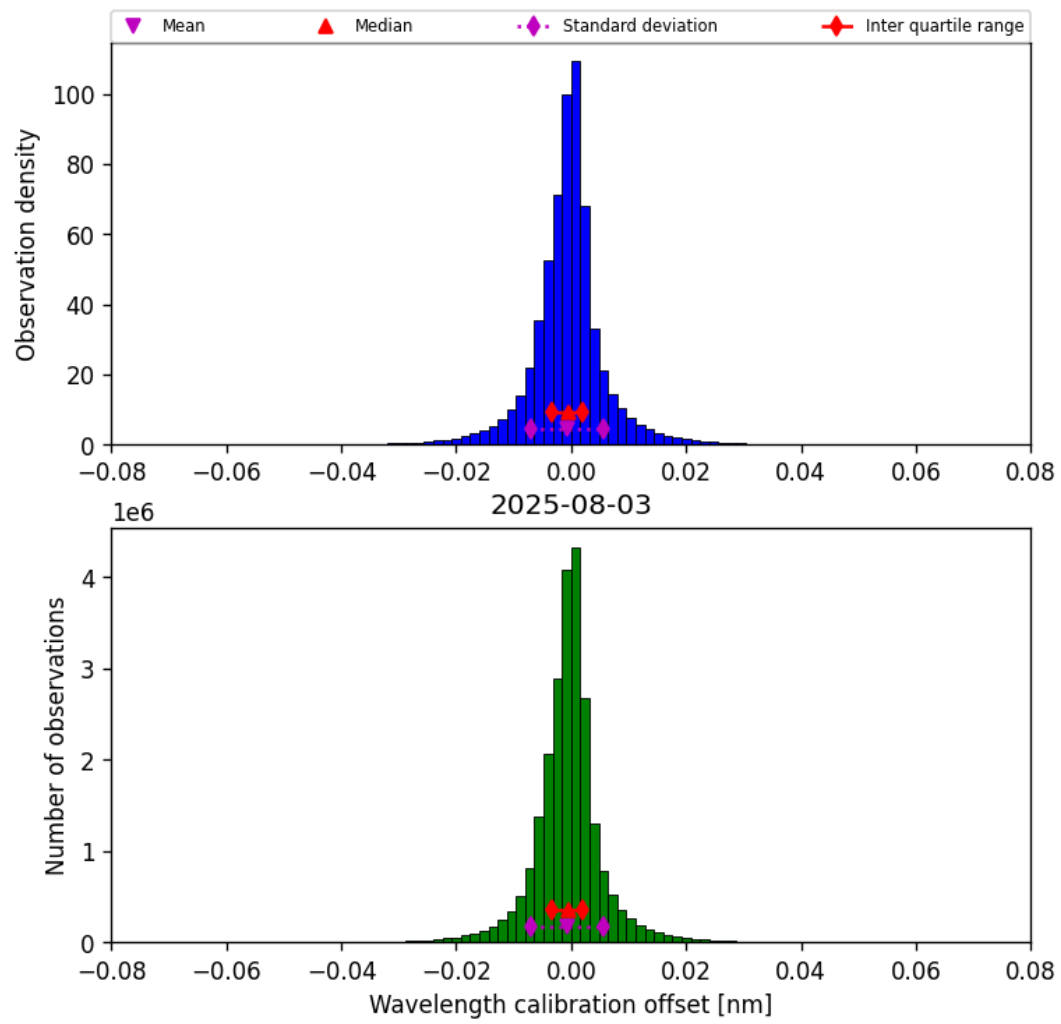
Figure 33: Histogram of “Wavelength calibration offset” for 2025-08-03 to 2025-08-04
