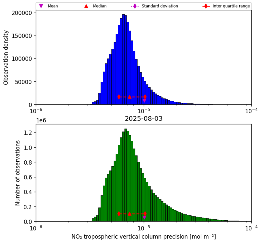
Figure 28: Histogram of “NO 2 tropospheric vertical column precision” for 2025-08-03 to 2025-08-04
