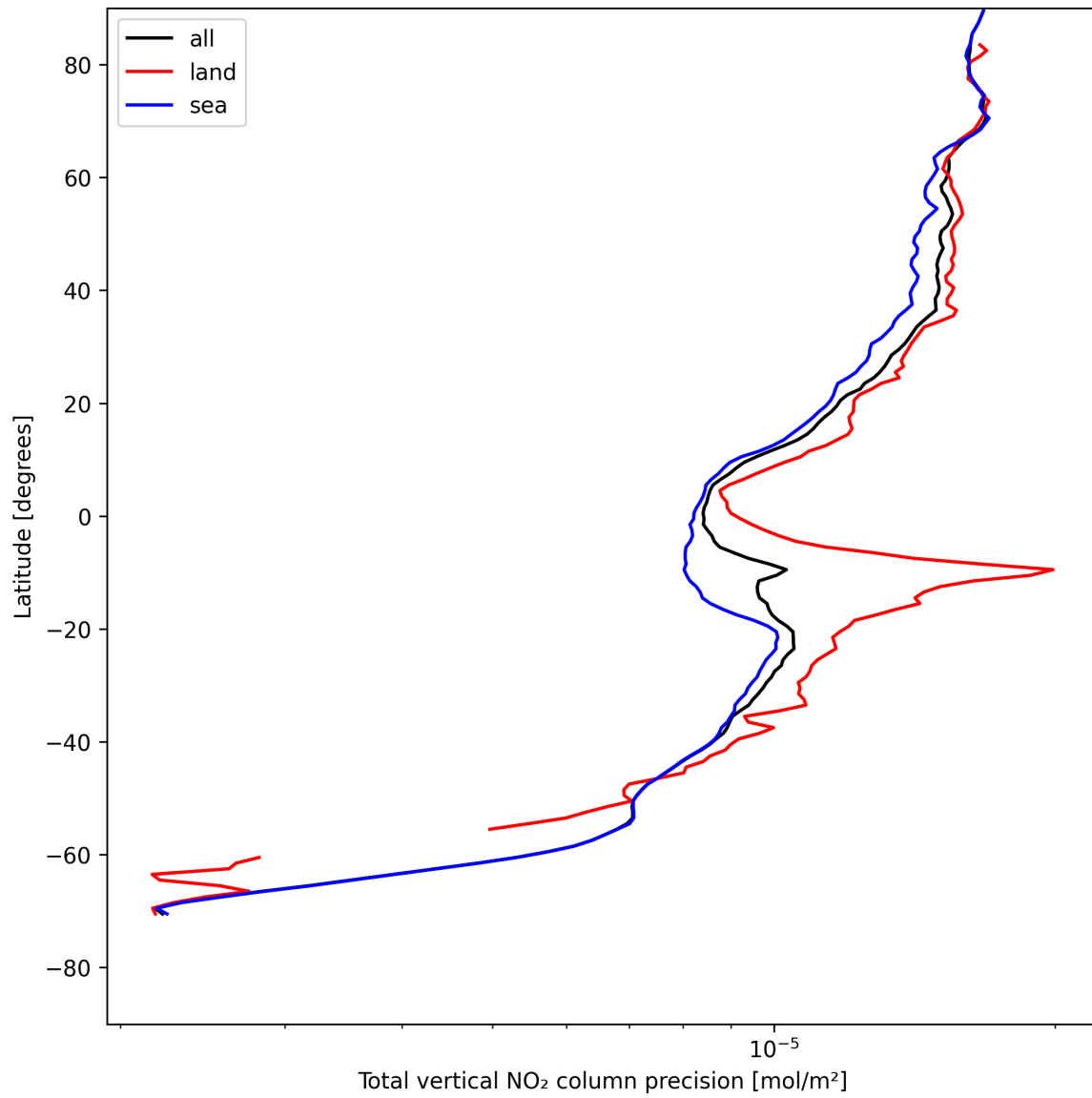
Figure 20: Zonal average of “Total vertical NO 2 column precision” for 2025-08-03 to 2025-08-04.
