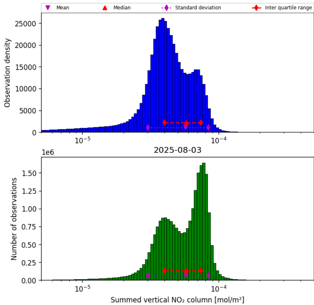
Figure 38: Histogram of “Summed vertical NO 2 column” for 2025-08-03 to 2025-08-04
