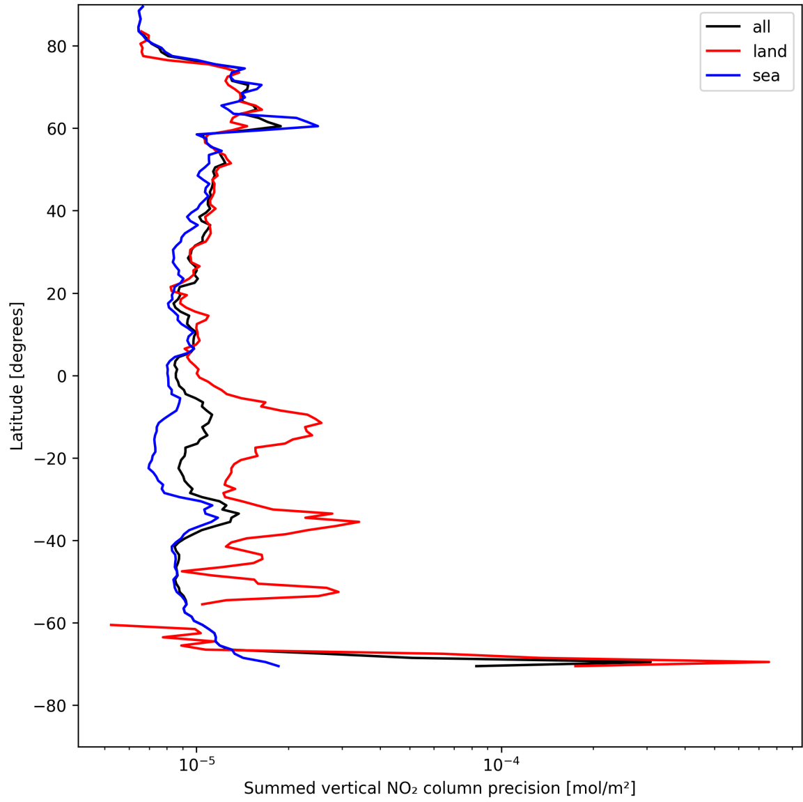
Figure 22: Zonal average of “Summed vertical NO 2 column precision” for 2025-08-03 to 2025-08-04.
