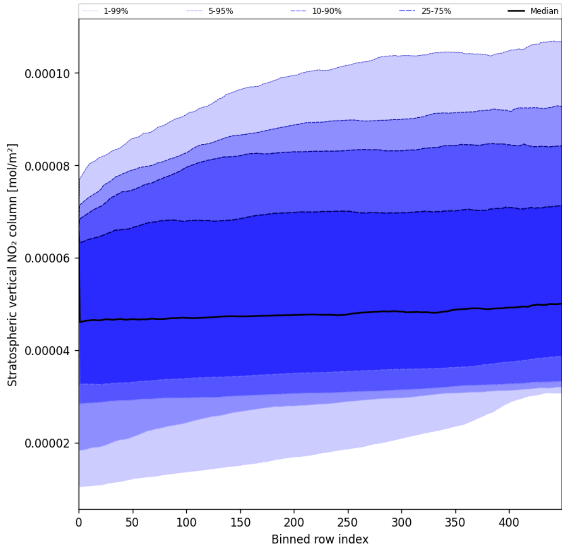
Figure 51: Along track statistics of “Stratospheric vertical NO 2 column” for 2025-08-03 to 2025-08-04
