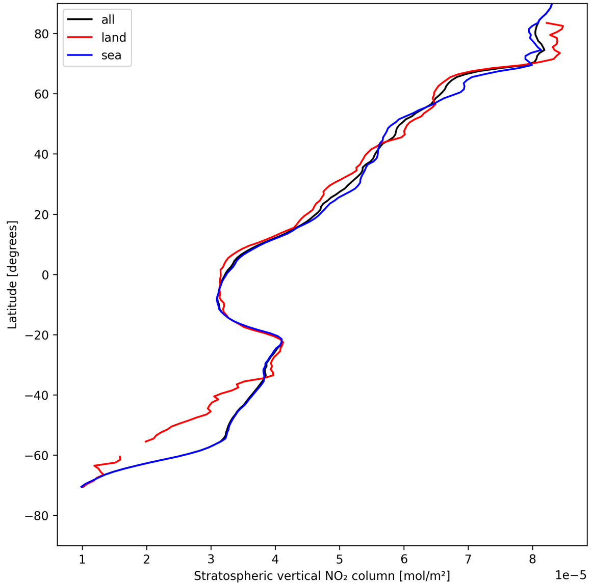
Figure 17: Zonal average of “Stratospheric vertical NO 2 column” for 2025-08-03 to 2025-08-04.
