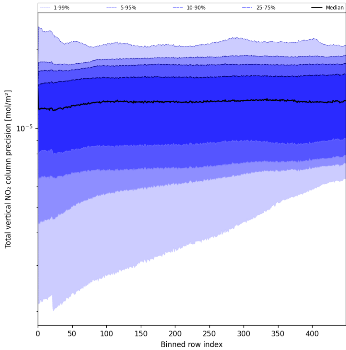
Figure 54: Along track statistics of “Total vertical NO 2 column precision” for 2025-08-03 to 2025-08-04
