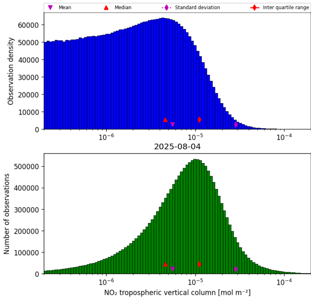
Figure 27: Histogram of “NO 2 tropospheric vertical column” for 2025-08-04 to 2025-08-05
