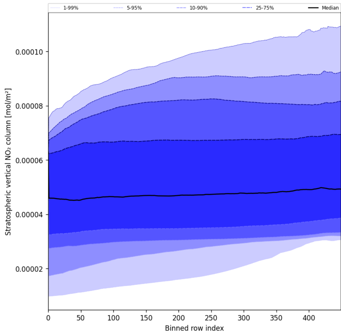
Figure 51: Along track statistics of “Stratospheric vertical NO 2 column” for 2025-08-04 to 2025-08-05
