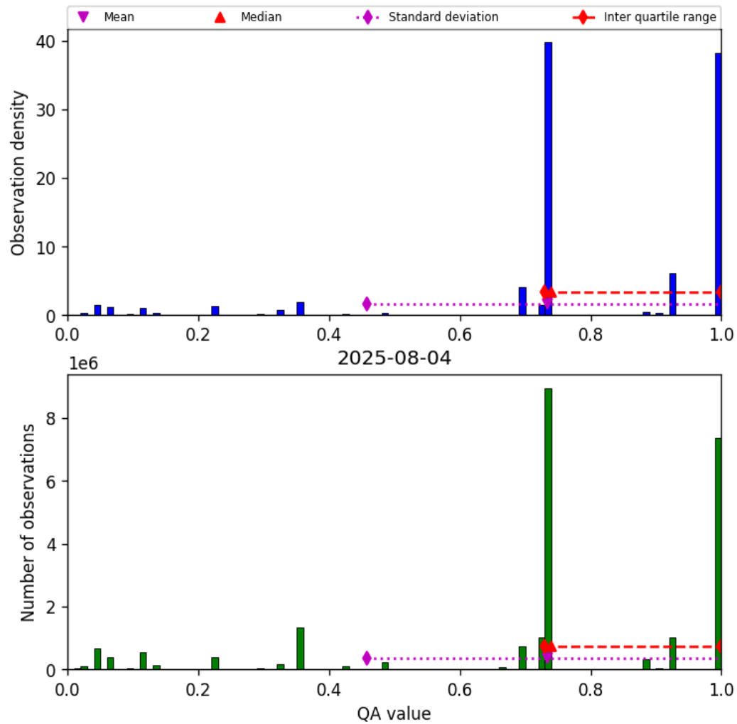
Figure 26: Histogram of “QA value” for 2025-08-04 to 2025-08-05
