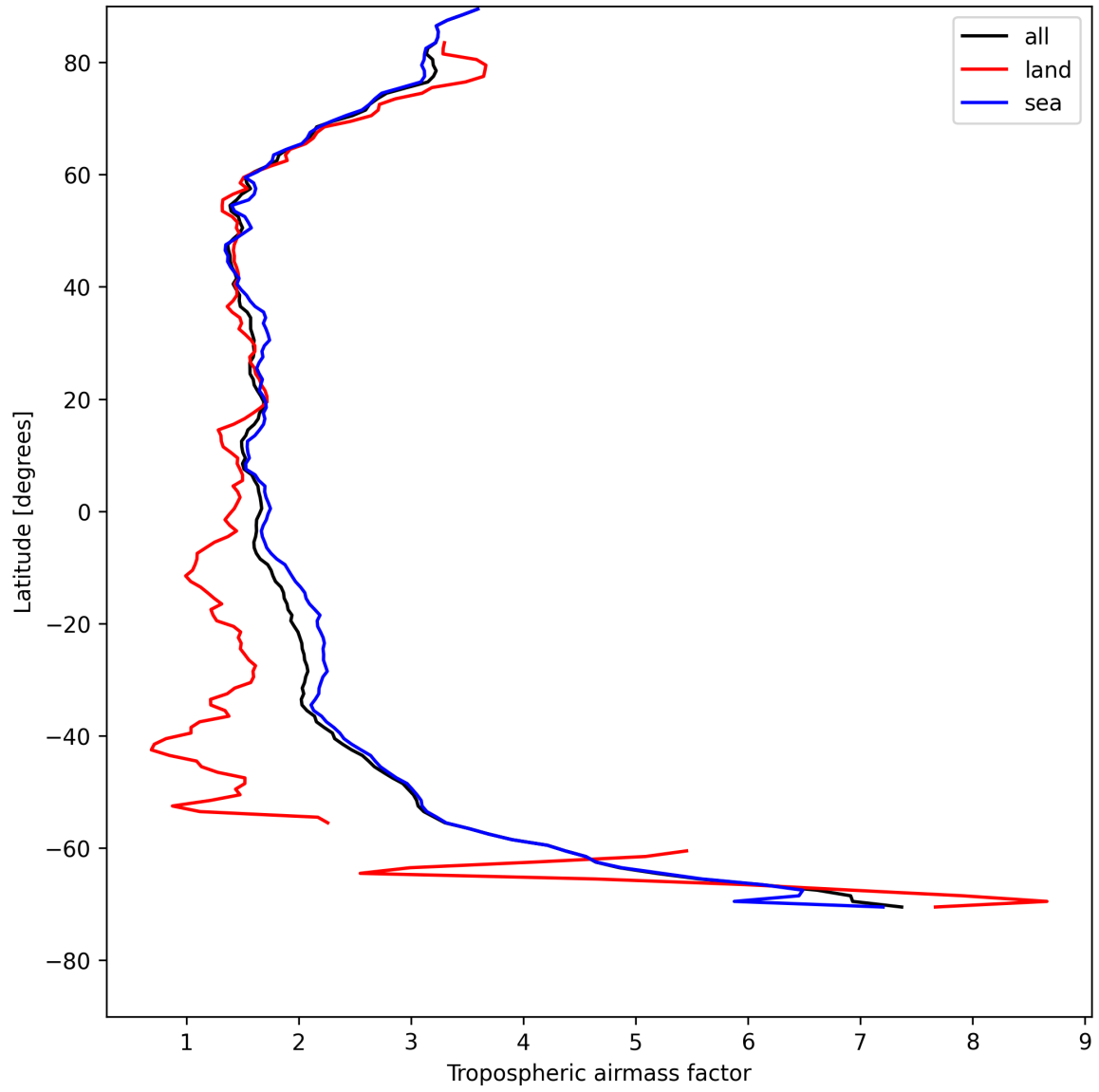
Figure 12: Zonal average of “Tropospheric airmass factor” for 2025-08-04 to 2025-08-05.
