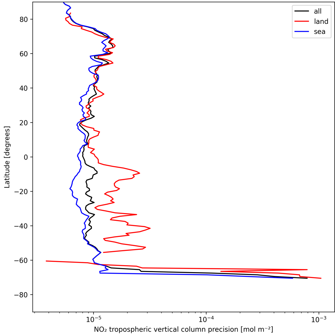
Figure 11: Zonal average of “NO 2 tropospheric vertical column precision” for 2025-08-04 to 2025-08-05.
