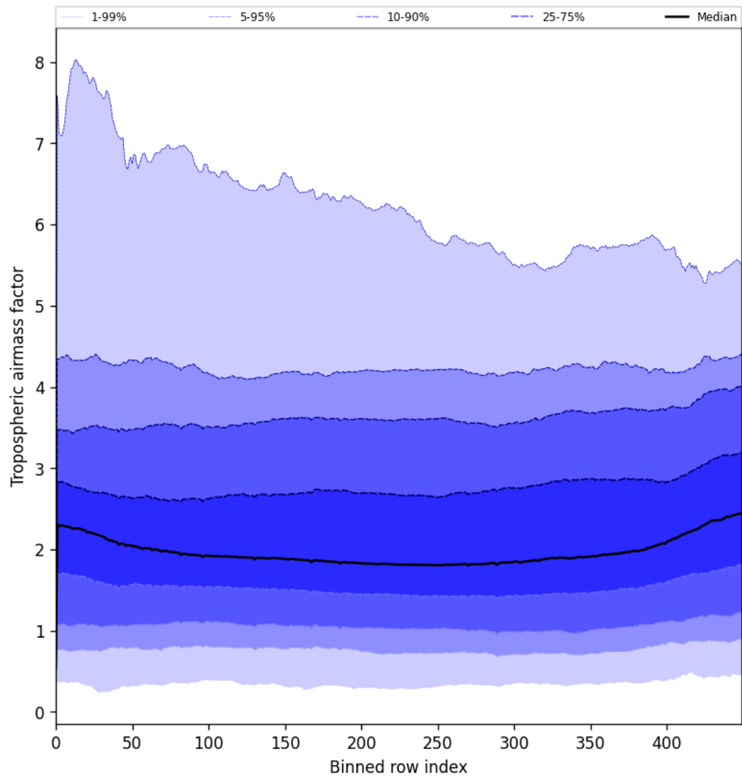
Figure 46: Along track statistics of “Tropospheric airmass factor” for 2025-08-04 to 2025-08-05
