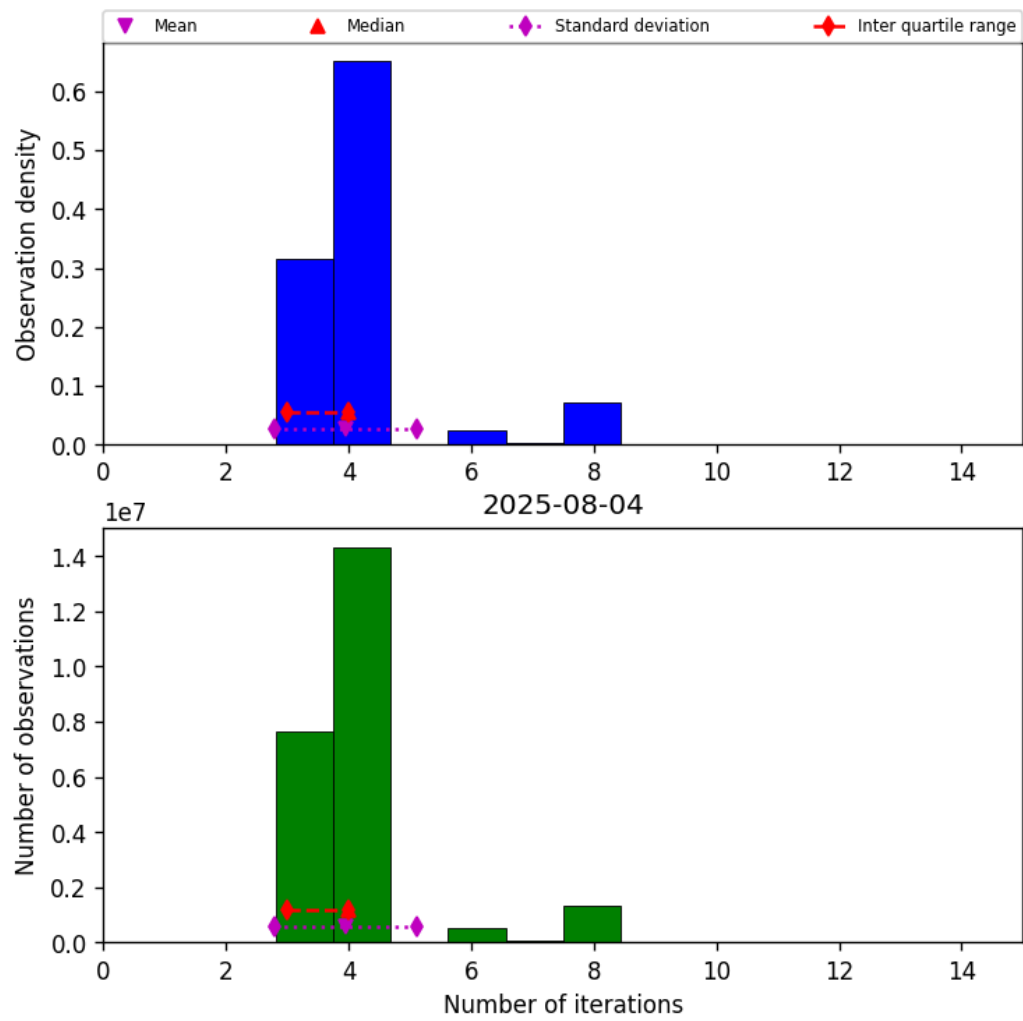
Figure 32: Histogram of “Number of iterations” for 2025-08-04 to 2025-08-05
