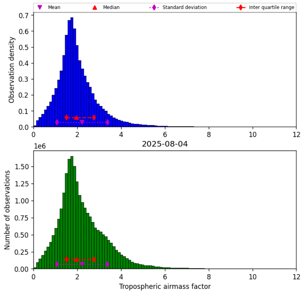
Figure 29: Histogram of “Tropospheric airmass factor” for 2025-08-04 to 2025-08-05
