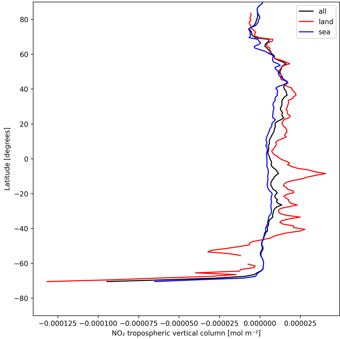
Figure 10: Zonal average of “NO 2 tropospheric vertical column” for 2025-08-04 to 2025-08-05.
