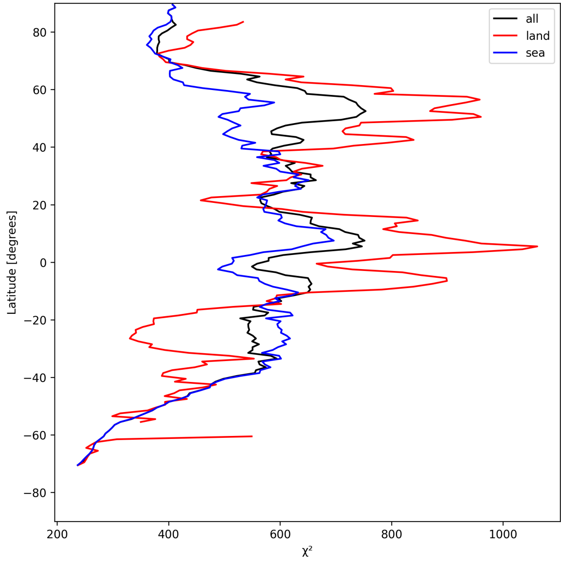
Figure 23: Zonal average of “ \chi^2 ” for 2025-08-04 to 2025-08-05.
