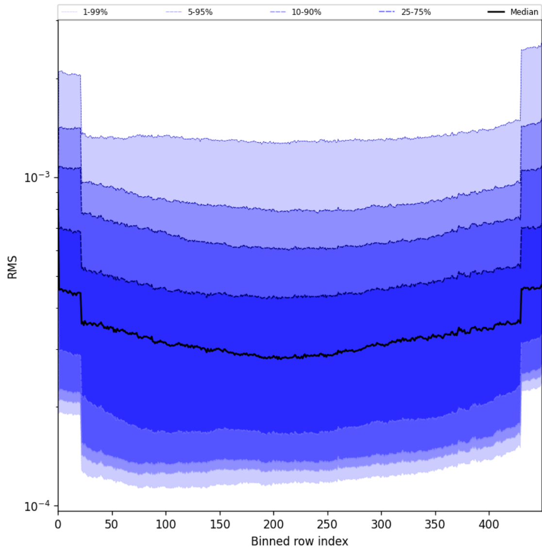
Figure 58: Along track statistics of “RMS” for 2025-08-04 to 2025-08-05
