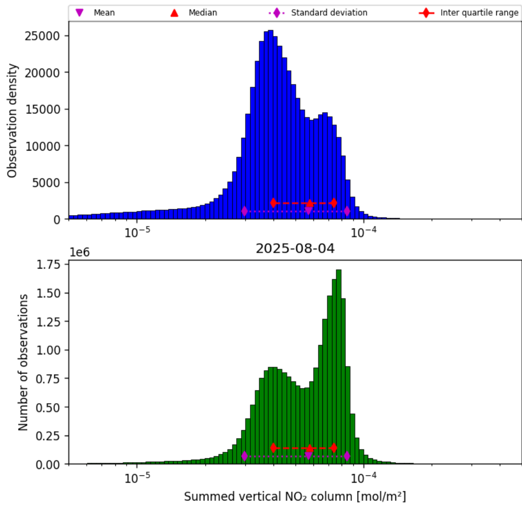
Figure 38: Histogram of “Summed vertical NO 2 column” for 2025-08-04 to 2025-08-05
