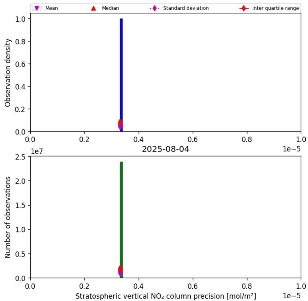
Figure 35: Histogram of “Stratospheric vertical NO 2 column precision” for 2025-08-04 to 2025-08-05
