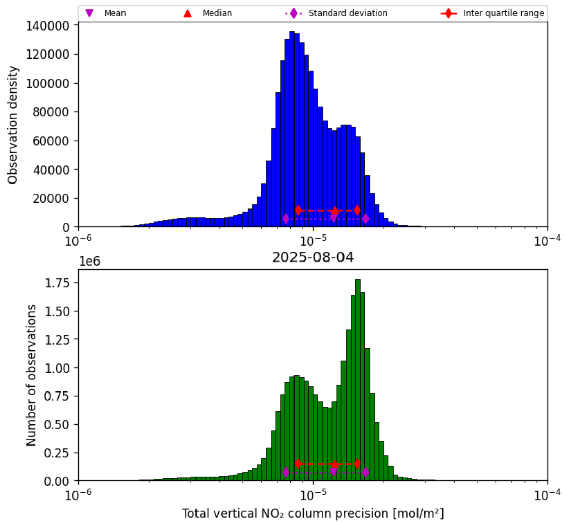
Figure 37: Histogram of “Total vertical NO 2 column precision” for 2025-08-04 to 2025-08-05
