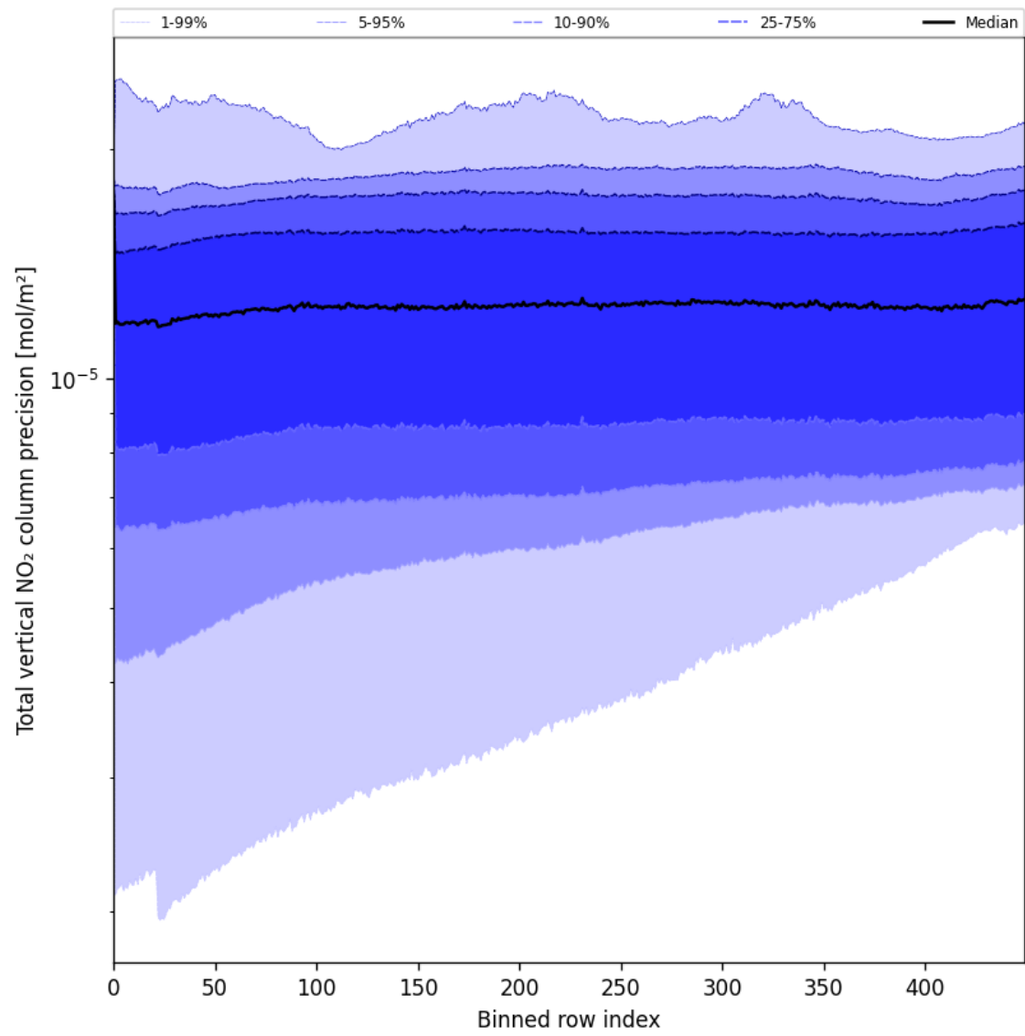
Figure 54: Along track statistics of “Total vertical NO 2 column precision” for 2025-08-04 to 2025-08-05
