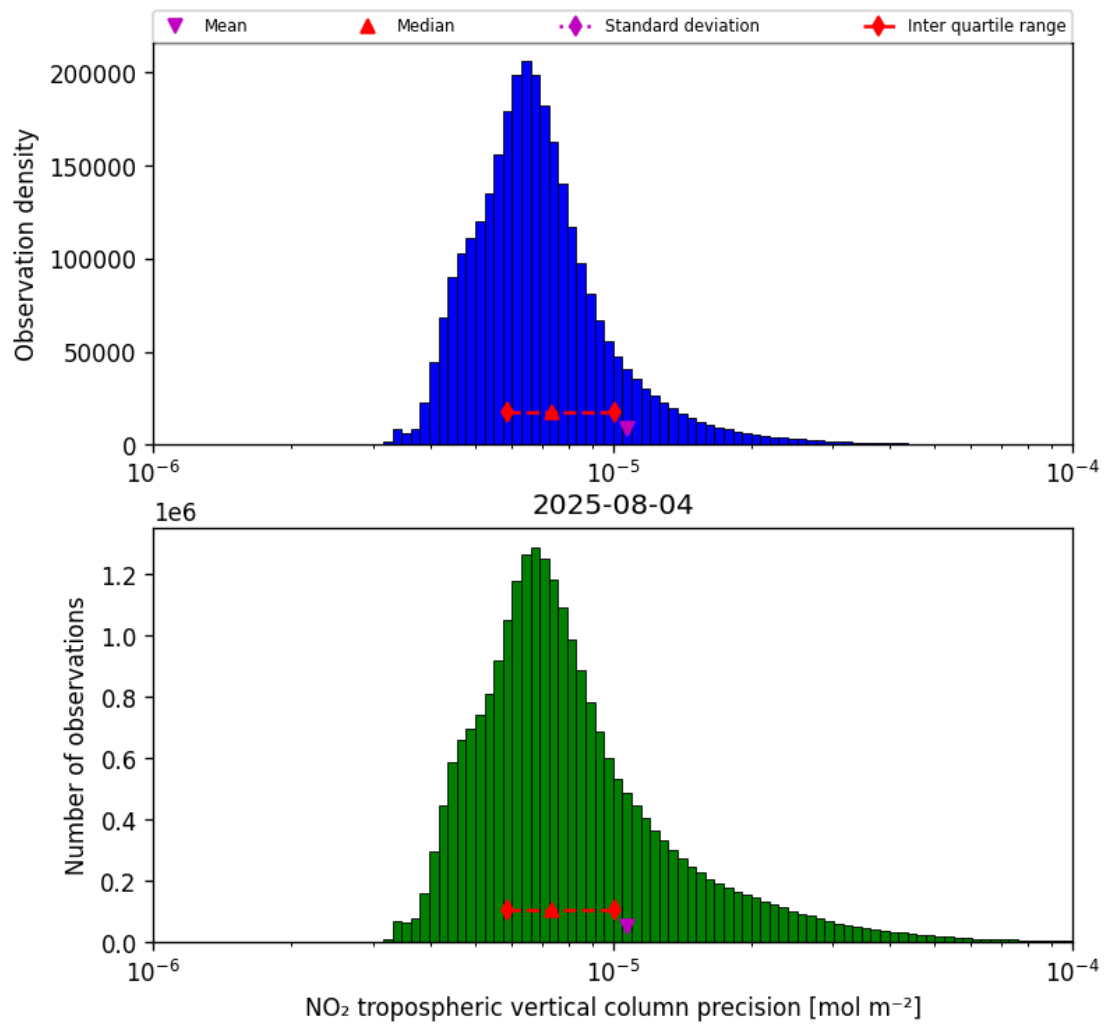
Figure 28: Histogram of “NO 2 tropospheric vertical column precision” for 2025-08-04 to 2025-08-05
