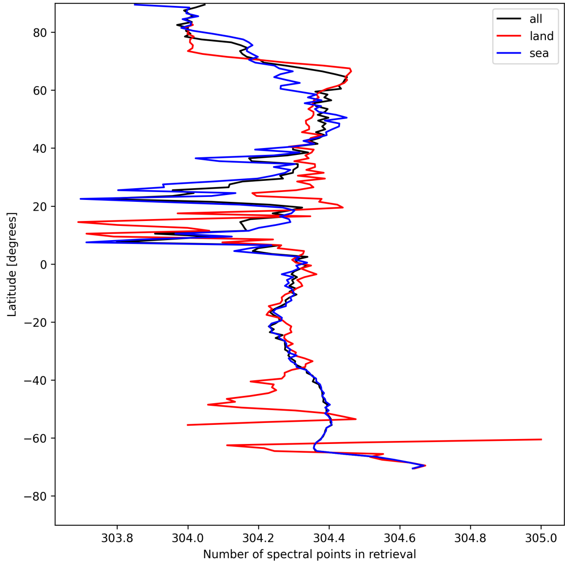
Figure 14: Zonal average of “Number of spectral points in retrieval” for 2025-08-04 to 2025-08-05.
