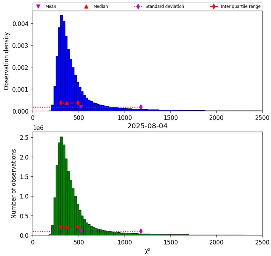
Figure 40: Histogram of “ \chi^2 ” for 2025-08-04 to 2025-08-05
