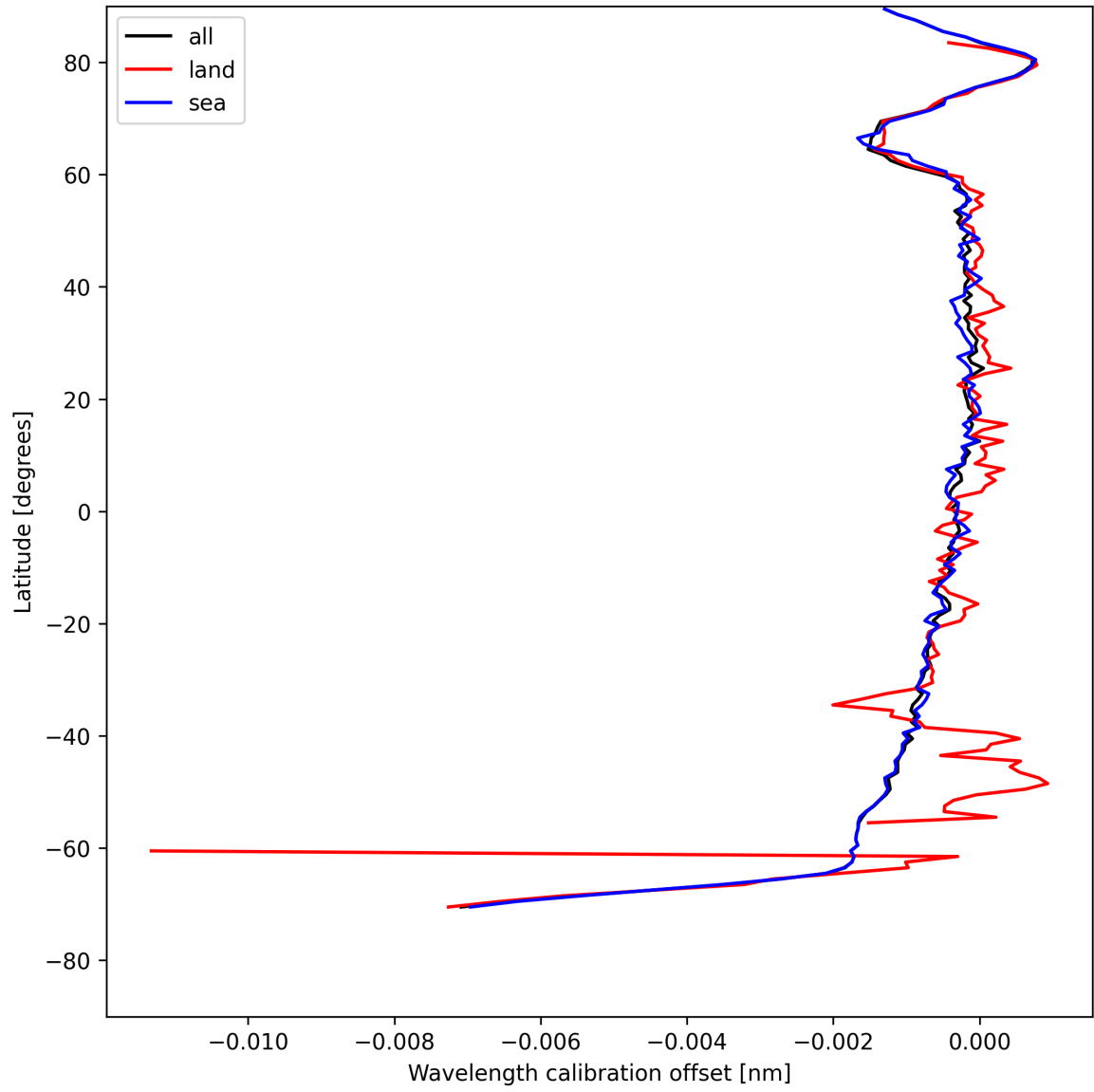
Figure 16: Zonal average of “Wavelength calibration offset” for 2025-08-04 to 2025-08-05.
