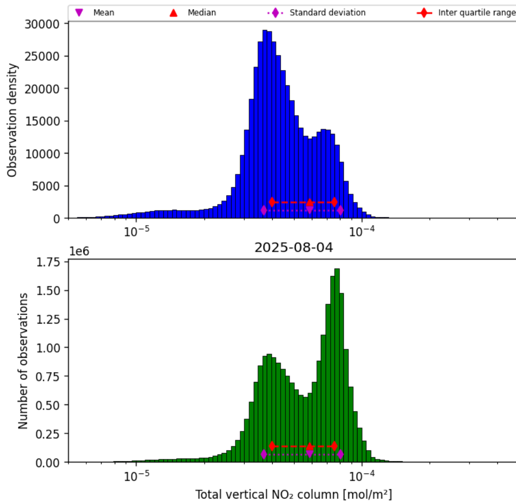
Figure 36: Histogram of “Total vertical NO 2 column” for 2025-08-04 to 2025-08-05
