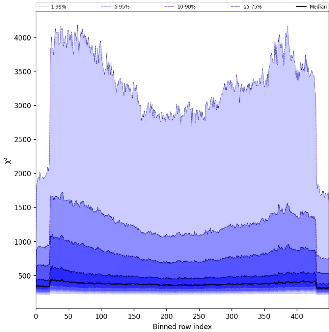
Figure 57: Along track statistics of “ \chi^2 ” for 2025-08-04 to 2025-08-05
