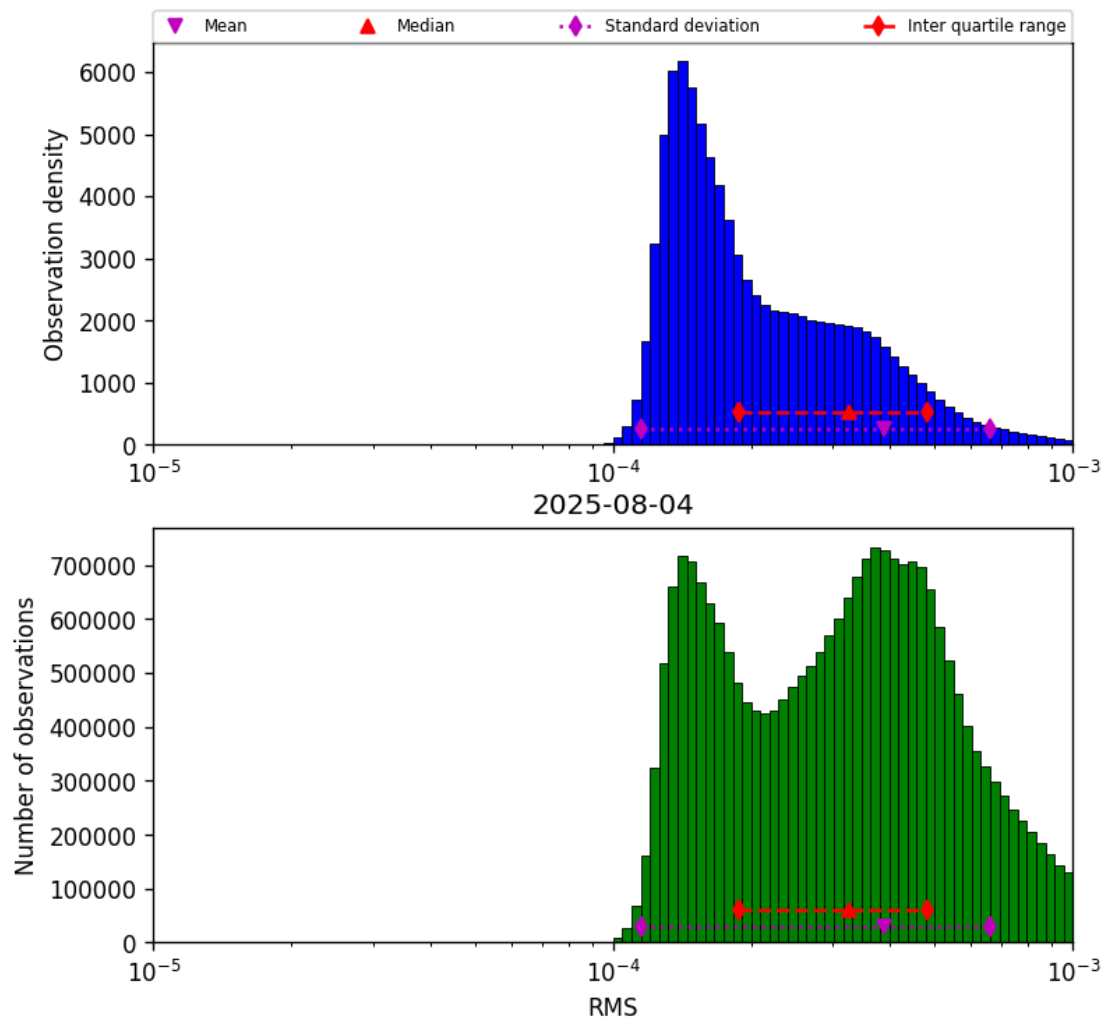
Figure 41: Histogram of “RMS” for 2025-08-04 to 2025-08-05
