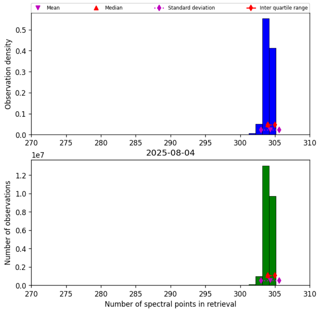
Figure 31: Histogram of “Number of spectral points in retrieval” for 2025-08-04 to 2025-08-05
