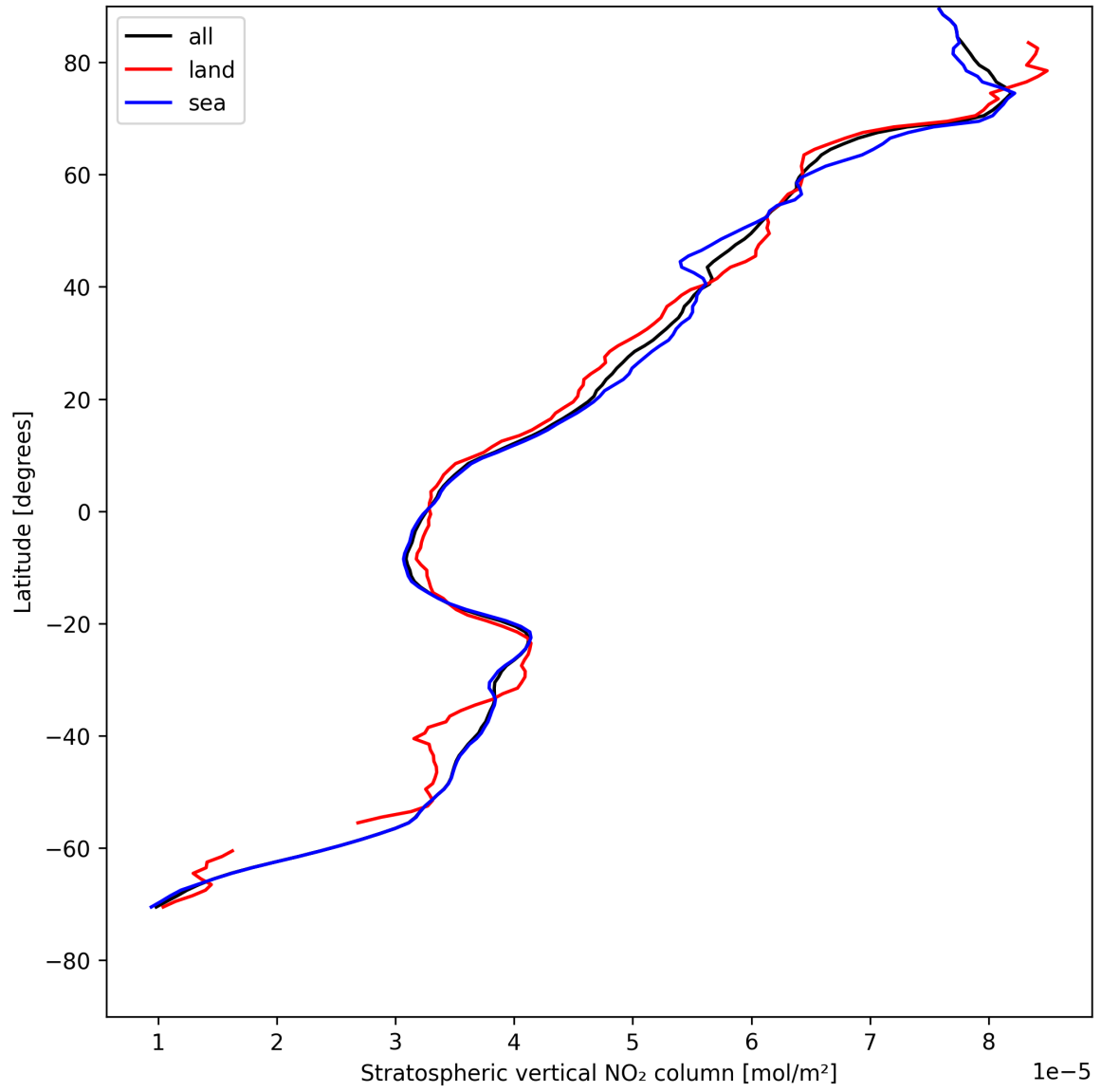
Figure 17: Zonal average of “Stratospheric vertical NO 2 column” for 2025-08-04 to 2025-08-05.
