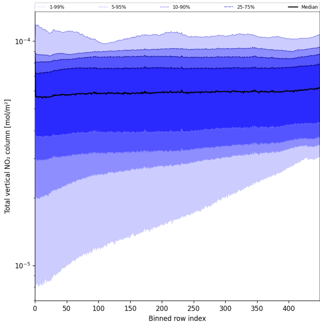
Figure 53: Along track statistics of “Total vertical NO 2 column” for 2025-08-04 to 2025-08-05
