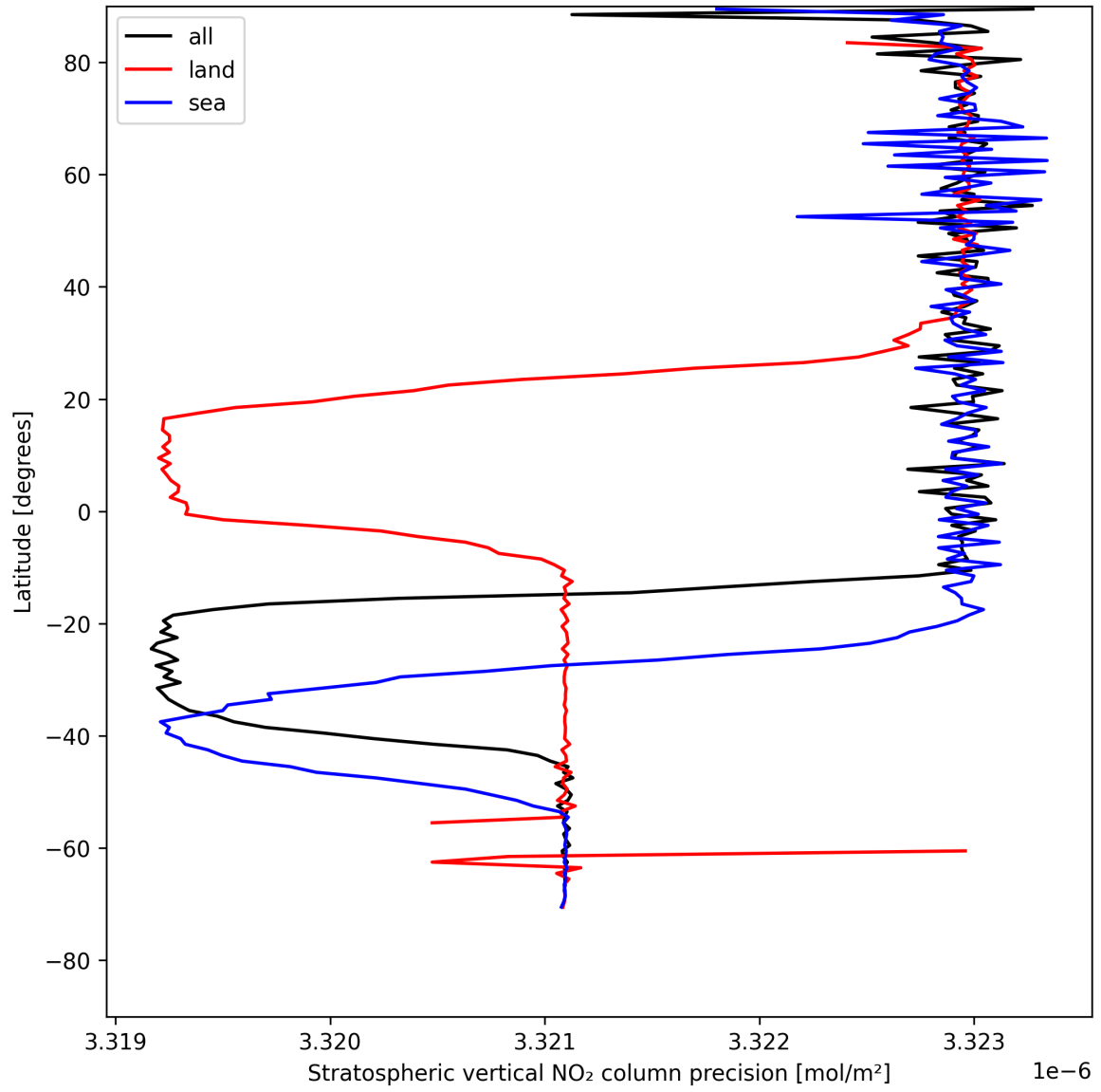
Figure 18: Zonal average of “Stratospheric vertical NO 2 column precision” for 2025-08-04 to 2025-08-05.
