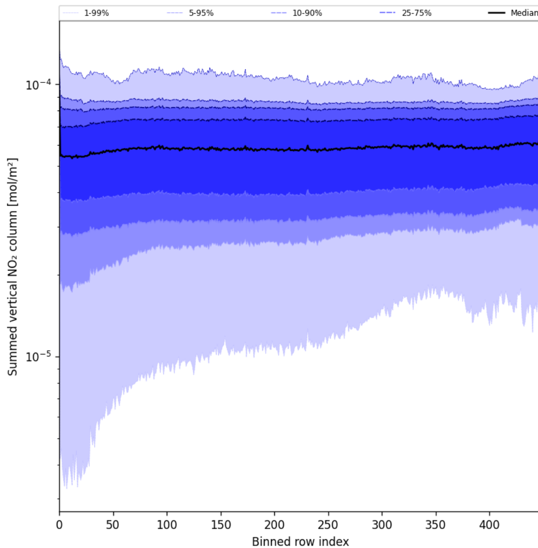
Figure 55: Along track statistics of “Summed vertical NO 2 column” for 2025-08-04 to 2025-08-05
