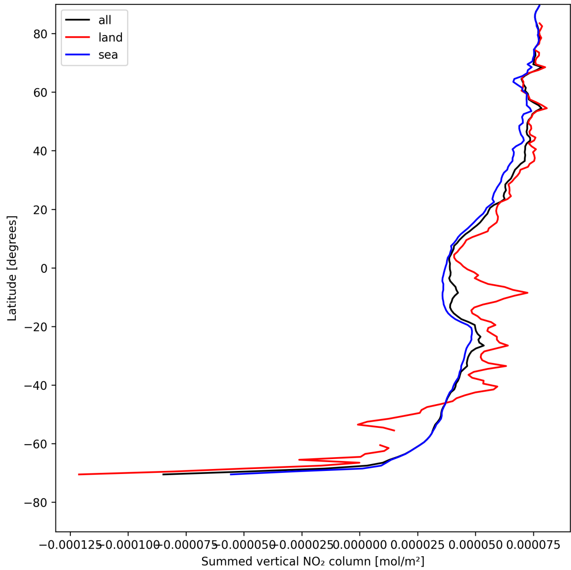
Figure 21: Zonal average of “Summed vertical NO 2 column” for 2025-08-04 to 2025-08-05.
