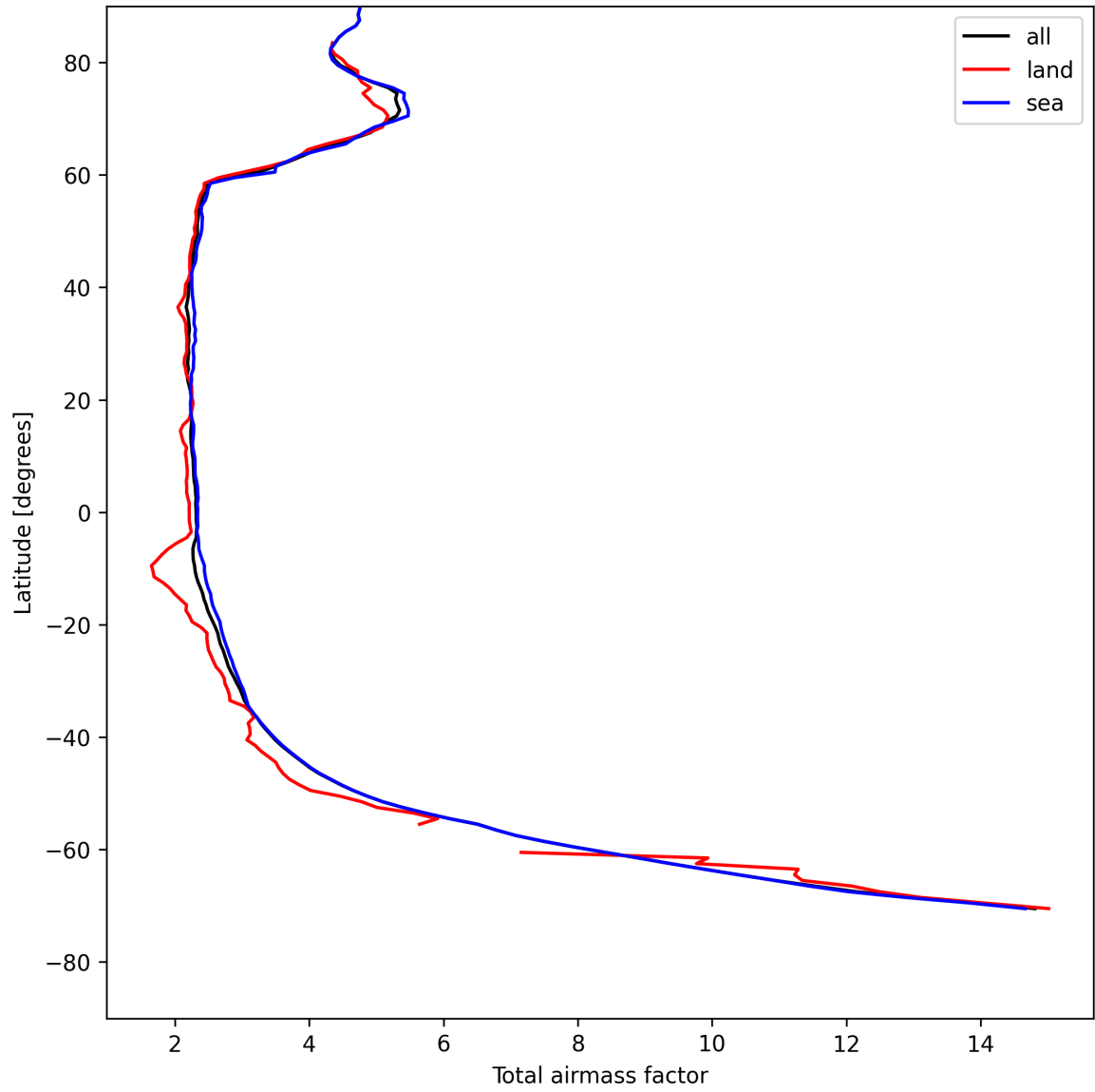
Figure 13: Zonal average of “Total airmass factor” for 2025-08-04 to 2025-08-05.
