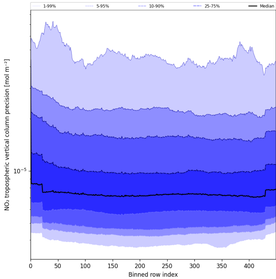
Figure 45: Along track statistics of “NO 2 tropospheric vertical column precision” for 2025-08-04 to 2025-08-05
