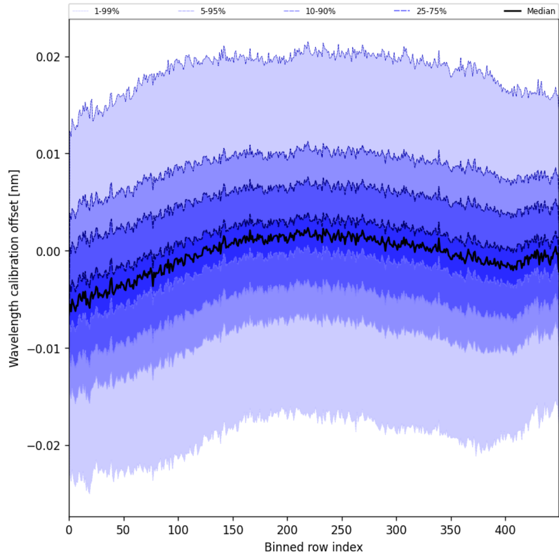
Figure 50: Along track statistics of “Wavelength calibration offset” for 2025-08-04 to 2025-08-05
