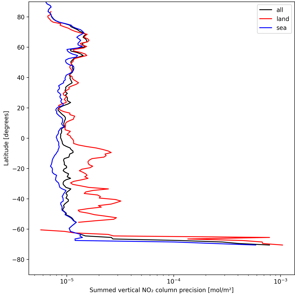
Figure 22: Zonal average of “Summed vertical NO 2 column precision” for 2025-08-04 to 2025-08-05.
