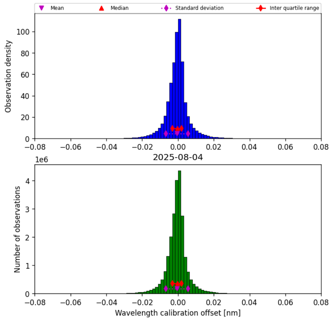
Figure 33: Histogram of “Wavelength calibration offset” for 2025-08-04 to 2025-08-05
