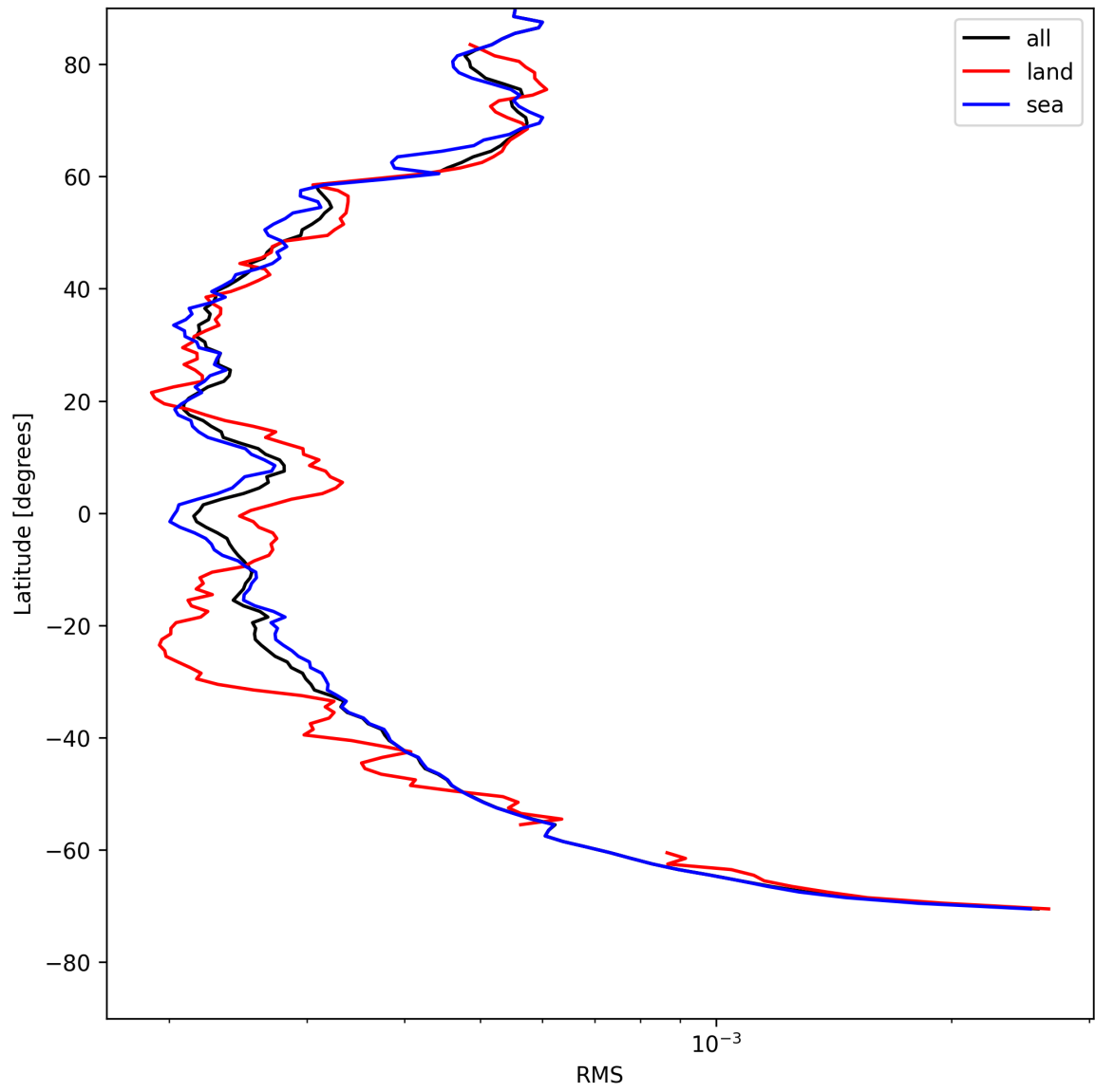
Figure 24: Zonal average of “RMS” for 2025-08-04 to 2025-08-05.
