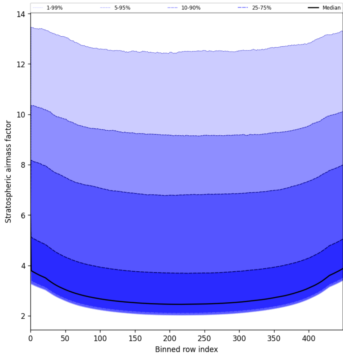
Figure 59: Along track statistics of “Stratospheric airmass factor” for 2025-08-04 to 2025-08-05
