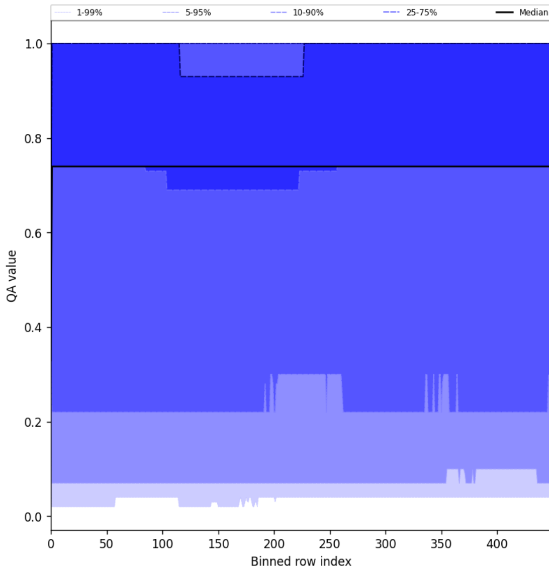
Figure 43: Along track statistics of "QA value" for 2025-08-04 to 2025-08-05
