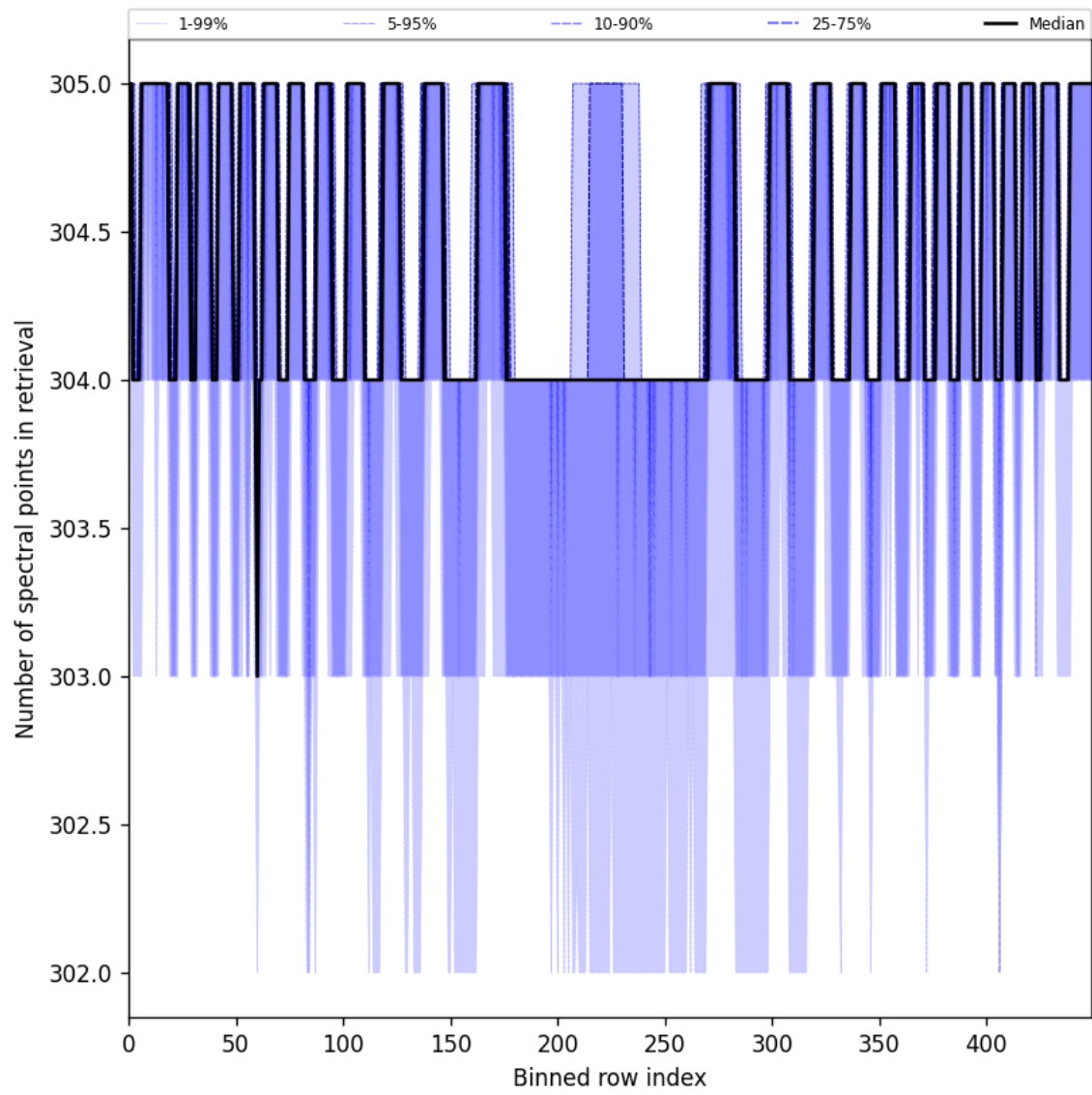
Figure 48: Along track statistics of “Number of spectral points in retrieval” for 2025-08-04 to 2025-08-05
