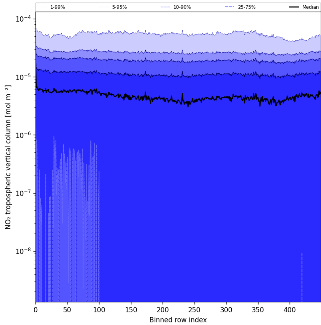
Figure 44: Along track statistics of “NO 2 tropospheric vertical column” for 2025-08-04 to 2025-08-05
