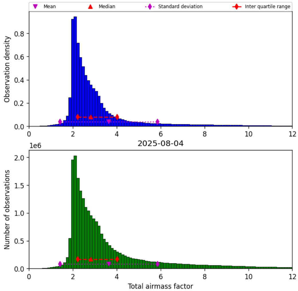
Figure 30: Histogram of “Total airmass factor” for 2025-08-04 to 2025-08-05
