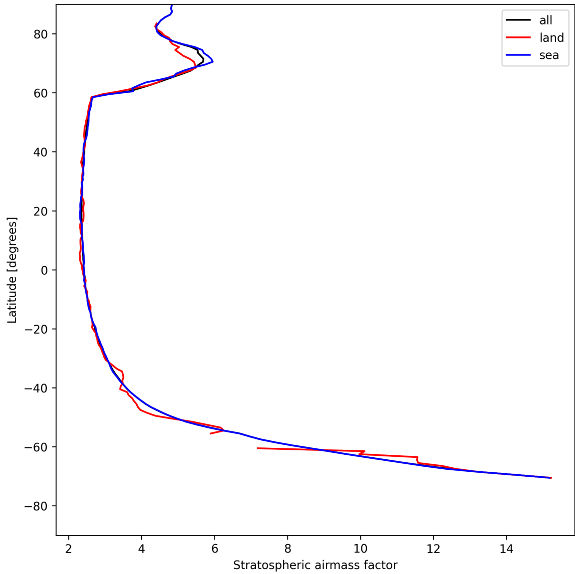
Figure 25: Zonal average of “Stratospheric airmass factor” for 2025-08-04 to 2025-08-05.
