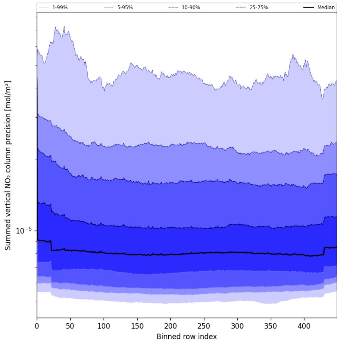
Figure 56: Along track statistics of “Summed vertical NO 2 column precision” for 2025-08-04 to 2025-08-05
