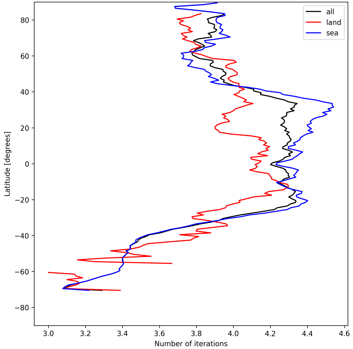
Figure 15: Zonal average of “Number of iterations” for 2025-08-04 to 2025-08-05.
