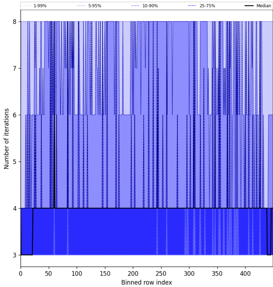
Figure 49: Along track statistics of “Number of iterations” for 2025-08-04 to 2025-08-05
