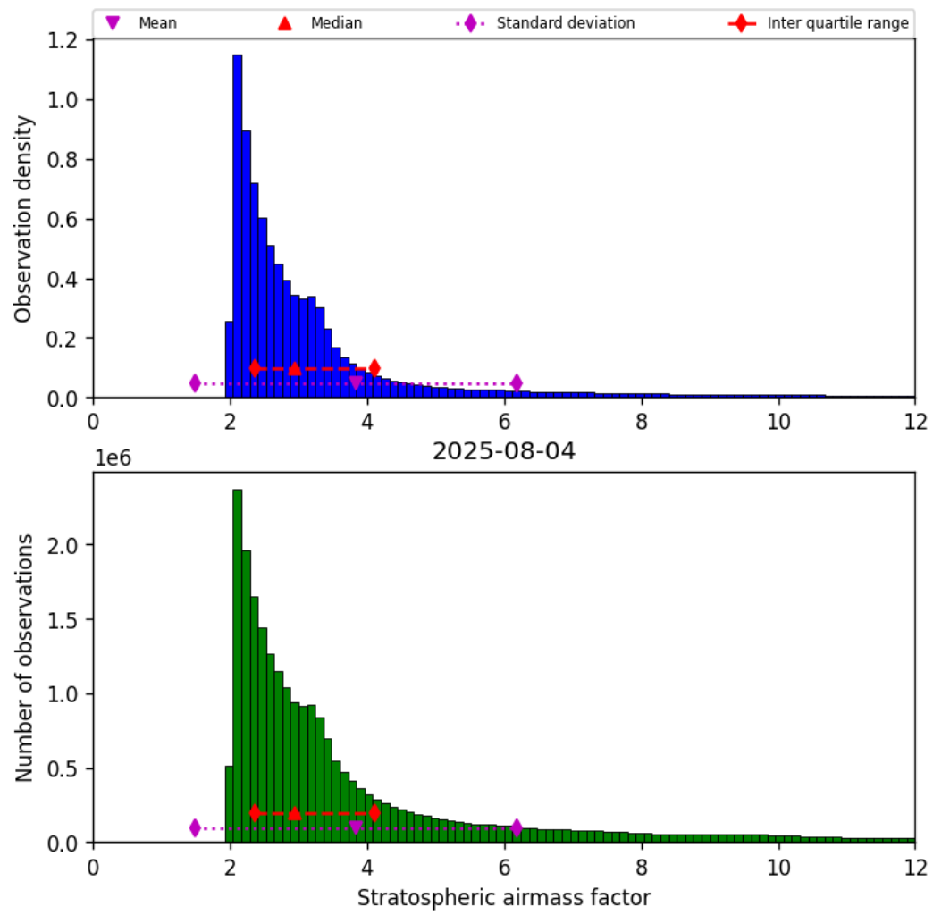
Figure 42: Histogram of “Stratospheric airmass factor” for 2025-08-04 to 2025-08-05
