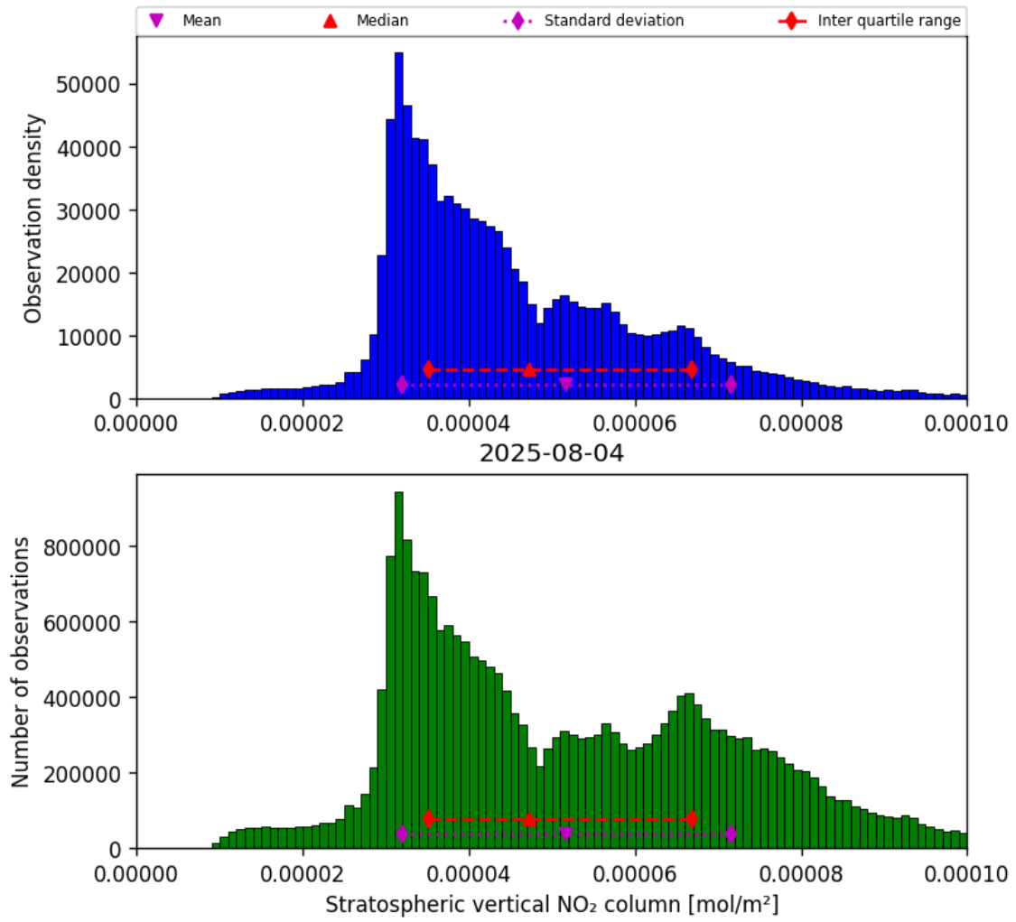
Figure 34: Histogram of “Stratospheric vertical NO 2 column” for 2025-08-04 to 2025-08-05
