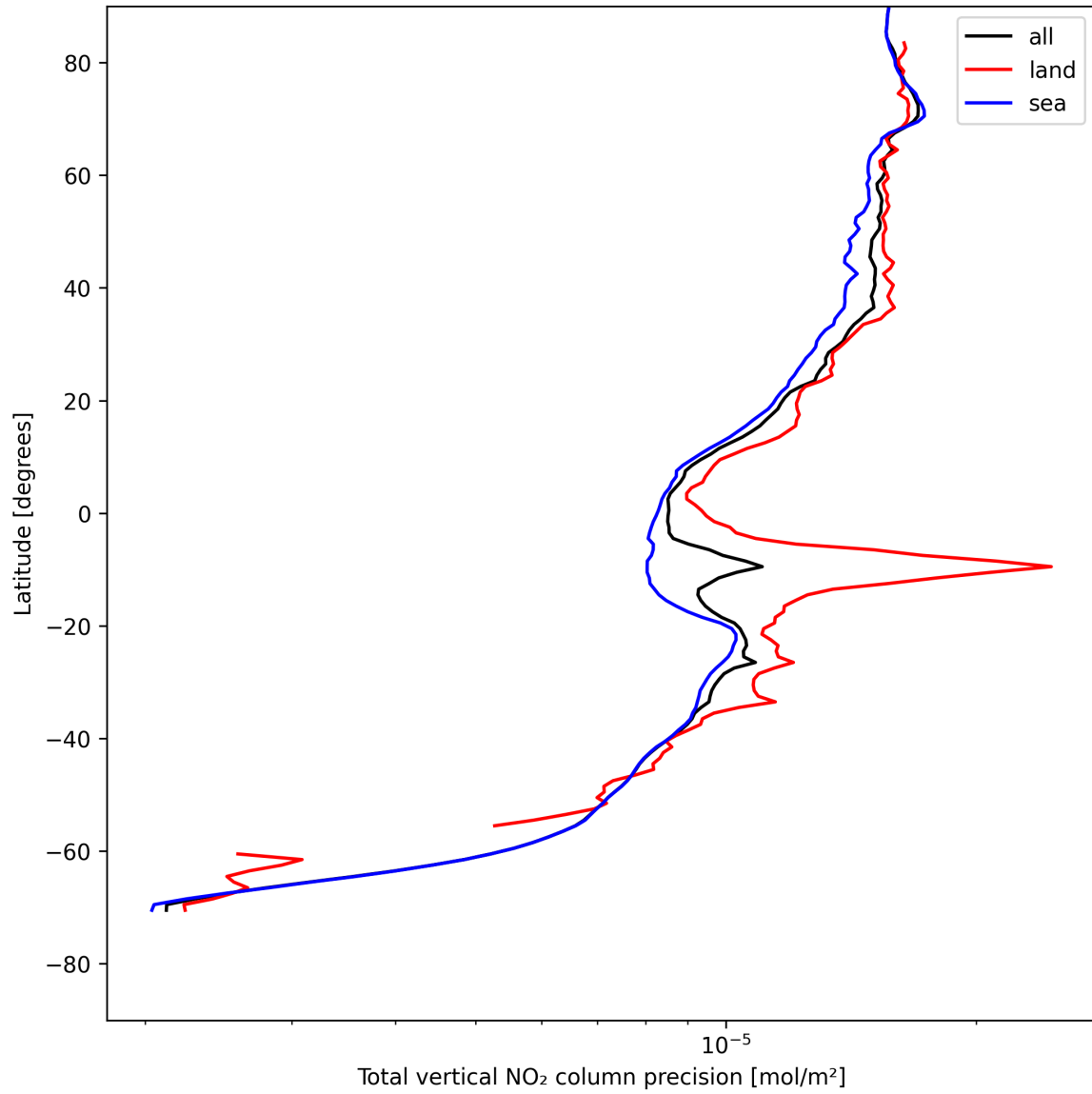
Figure 20: Zonal average of “Total vertical NO 2 column precision” for 2025-08-04 to 2025-08-05.
