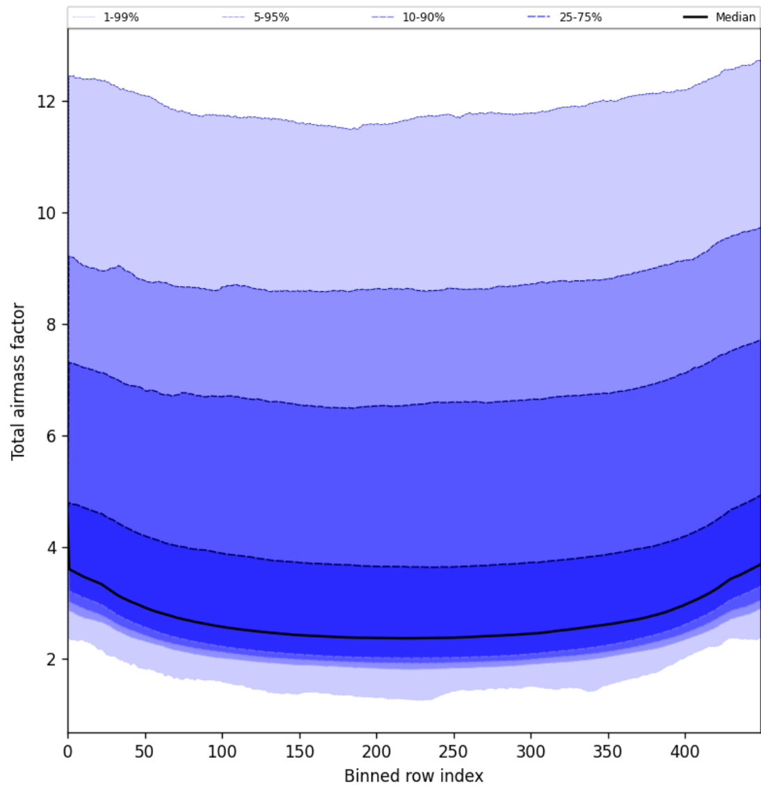
Figure 47: Along track statistics of “Total airmass factor” for 2025-08-04 to 2025-08-05
