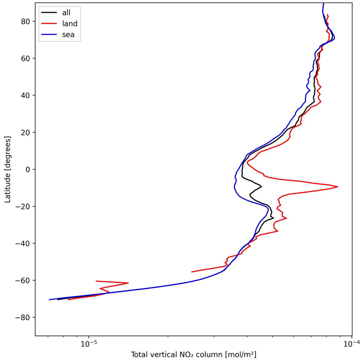
Figure 19: Zonal average of “Total vertical NO 2 column” for 2025-08-04 to 2025-08-05.
