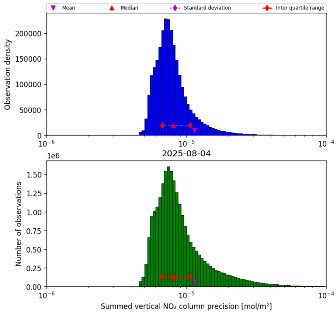
Figure 39: Histogram of “Summed vertical NO 2 column precision” for 2025-08-04 to 2025-08-05
