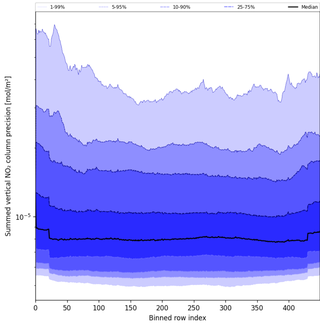
Figure 56: Along track statistics of “Summed vertical NO 2 column precision” for 2025-08-05 to 2025-08-06
