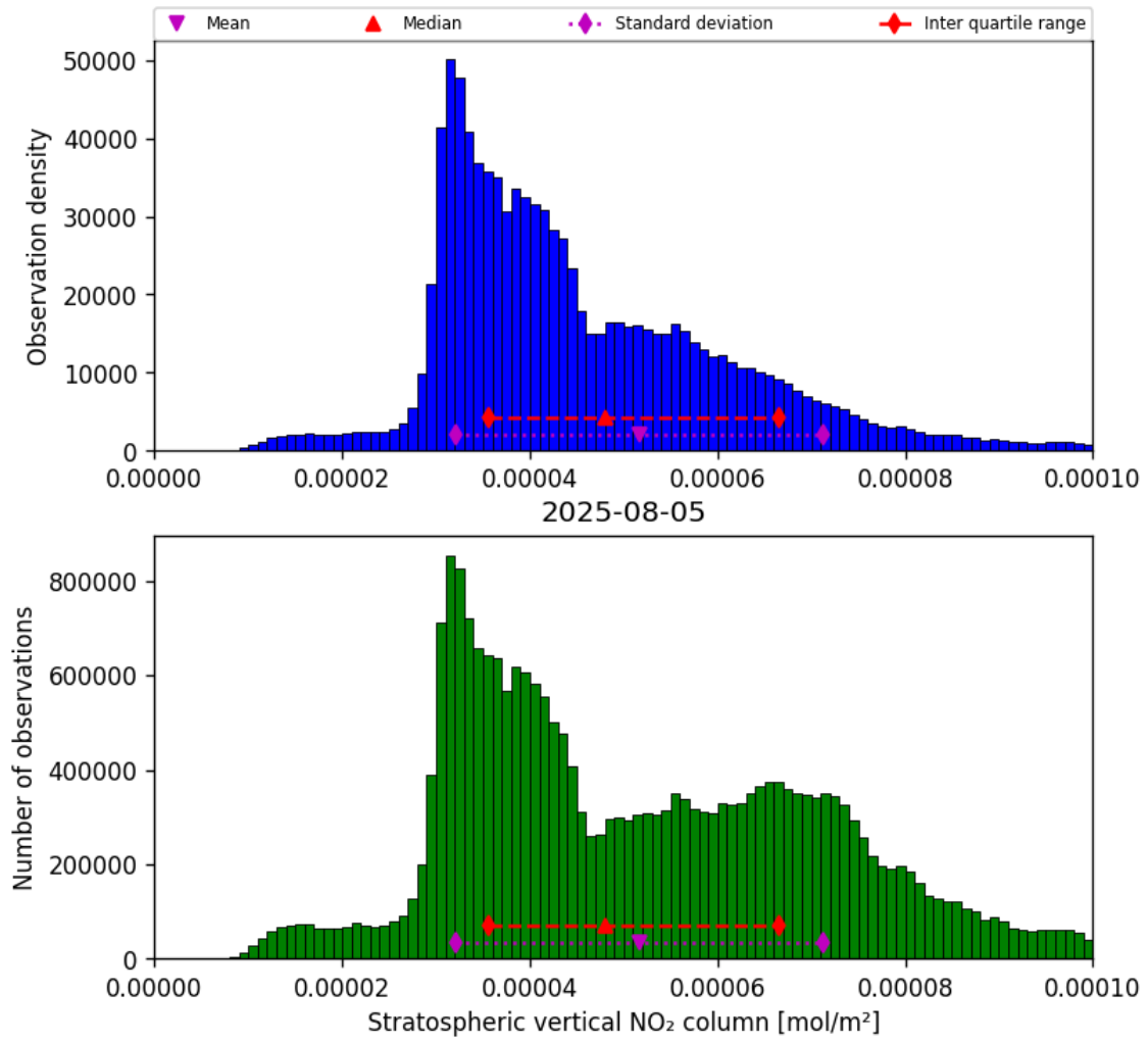
Figure 34: Histogram of “Stratospheric vertical NO 2 column” for 2025-08-05 to 2025-08-06
