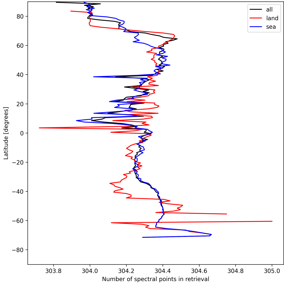
Figure 14: Zonal average of “Number of spectral points in retrieval” for 2025-08-05 to 2025-08-06.
