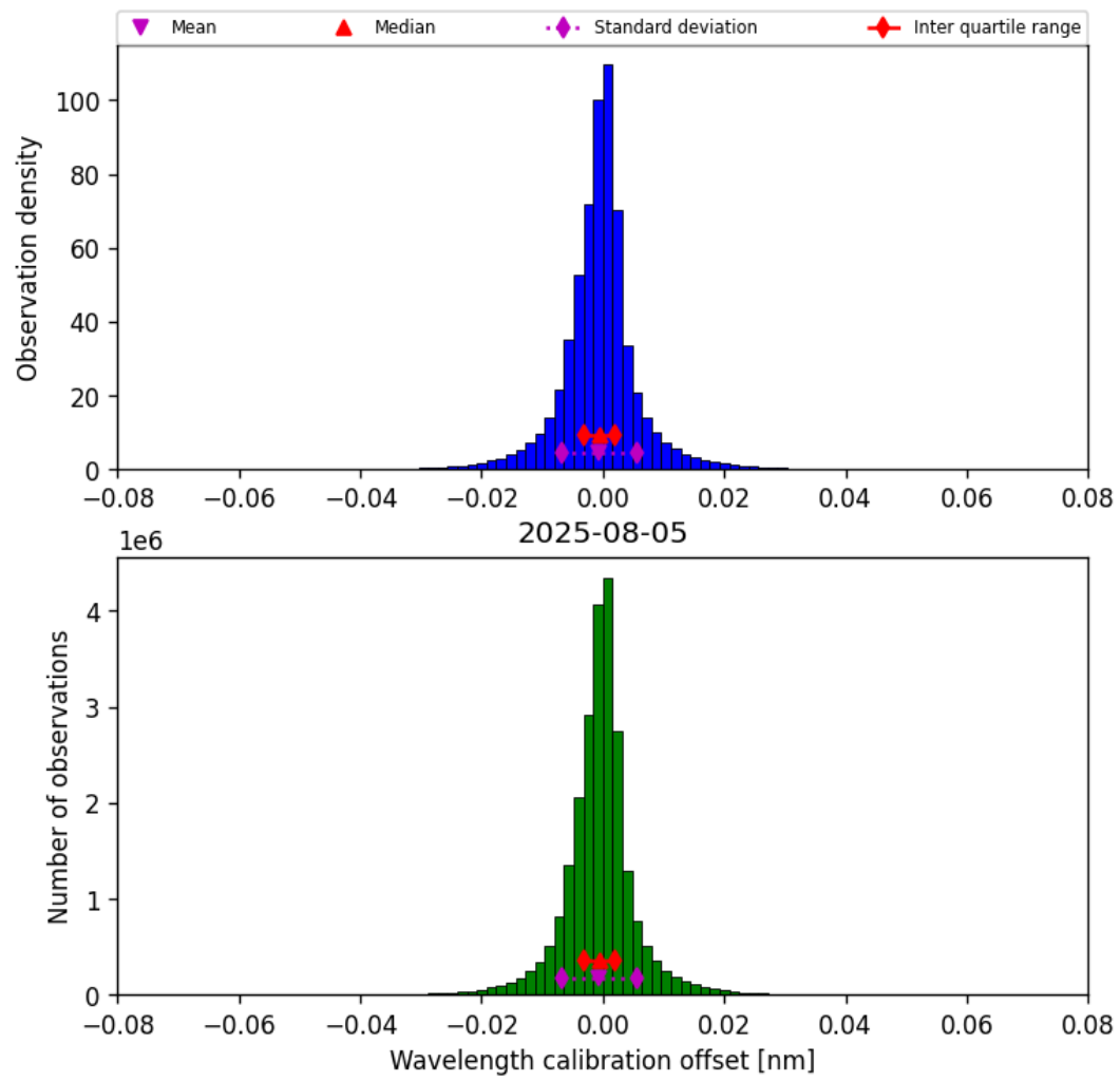
Figure 33: Histogram of “Wavelength calibration offset” for 2025-08-05 to 2025-08-06
