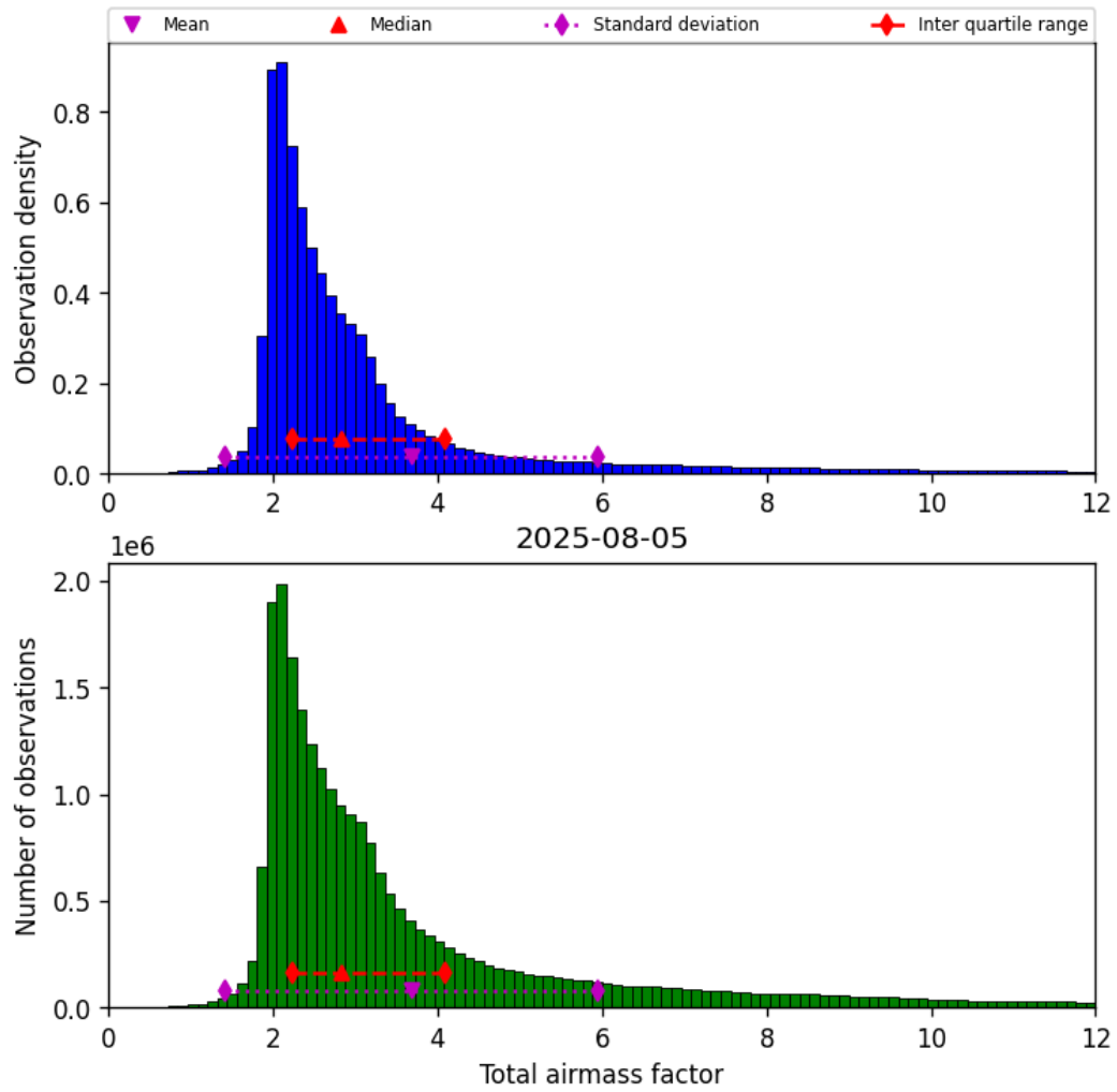
Figure 30: Histogram of “Total airmass factor” for 2025-08-05 to 2025-08-06
