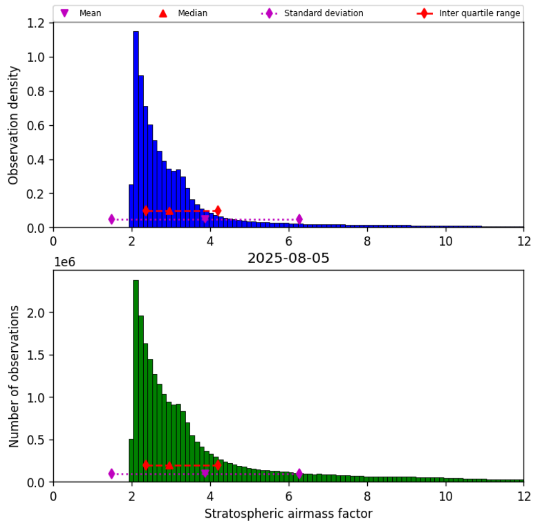
Figure 42: Histogram of “Stratospheric airmass factor” for 2025-08-05 to 2025-08-06
