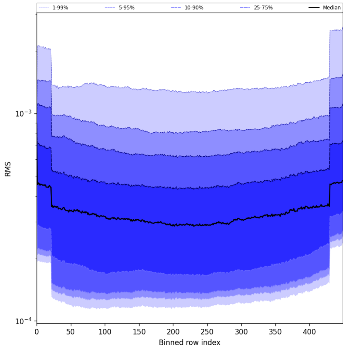
Figure 58: Along track statistics of “RMS” for 2025-08-05 to 2025-08-06
