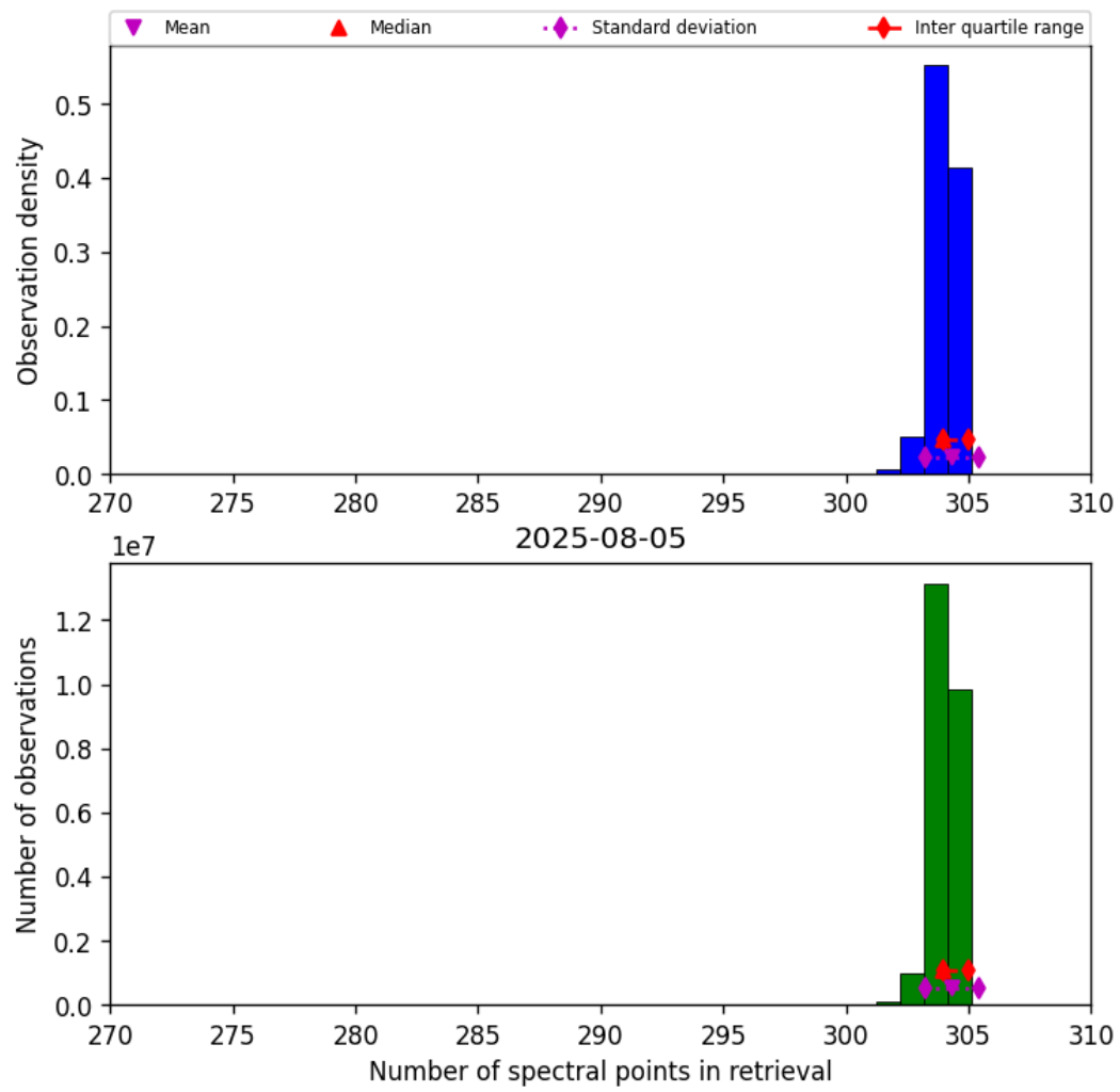
Figure 31: Histogram of “Number of spectral points in retrieval” for 2025-08-05 to 2025-08-06
