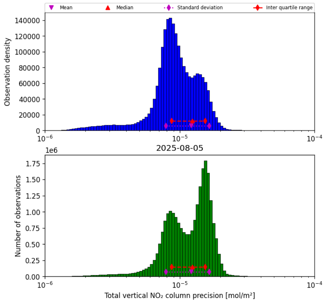
Figure 37: Histogram of “Total vertical NO 2 column precision” for 2025-08-05 to 2025-08-06
