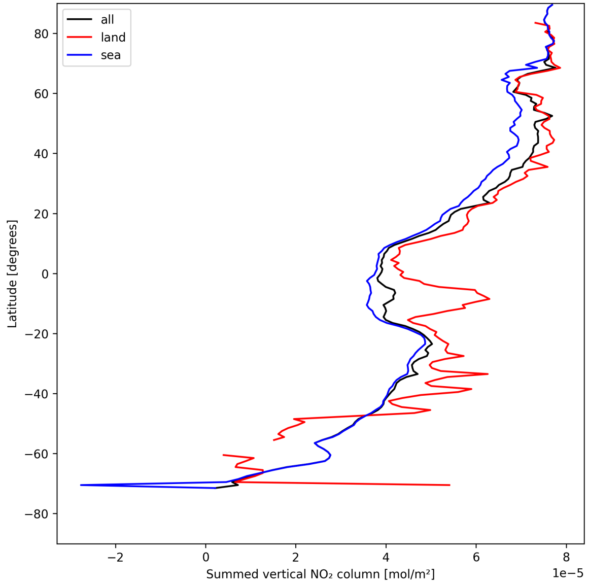
Figure 21: Zonal average of “Summed vertical NO 2 column” for 2025-08-05 to 2025-08-06.
