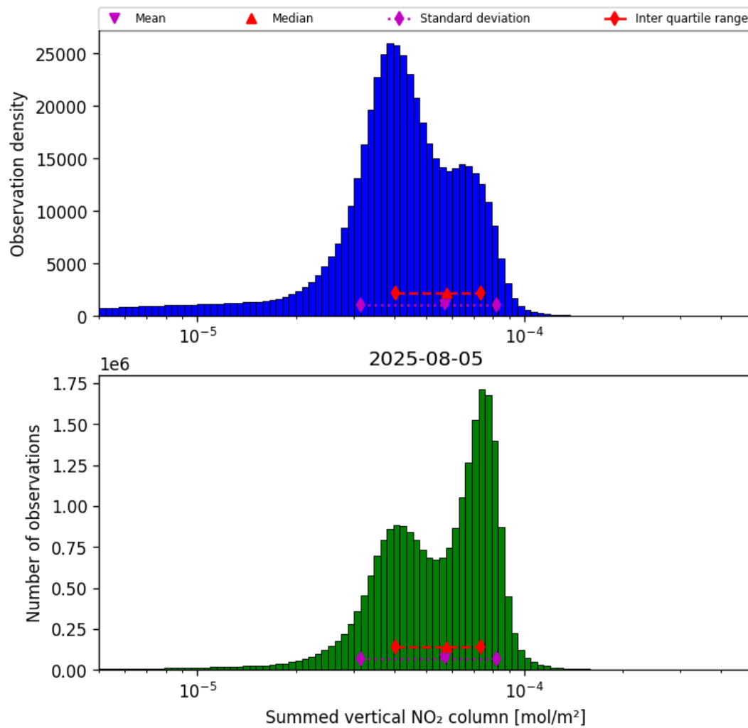
Figure 38: Histogram of “Summed vertical NO 2 column” for 2025-08-05 to 2025-08-06
