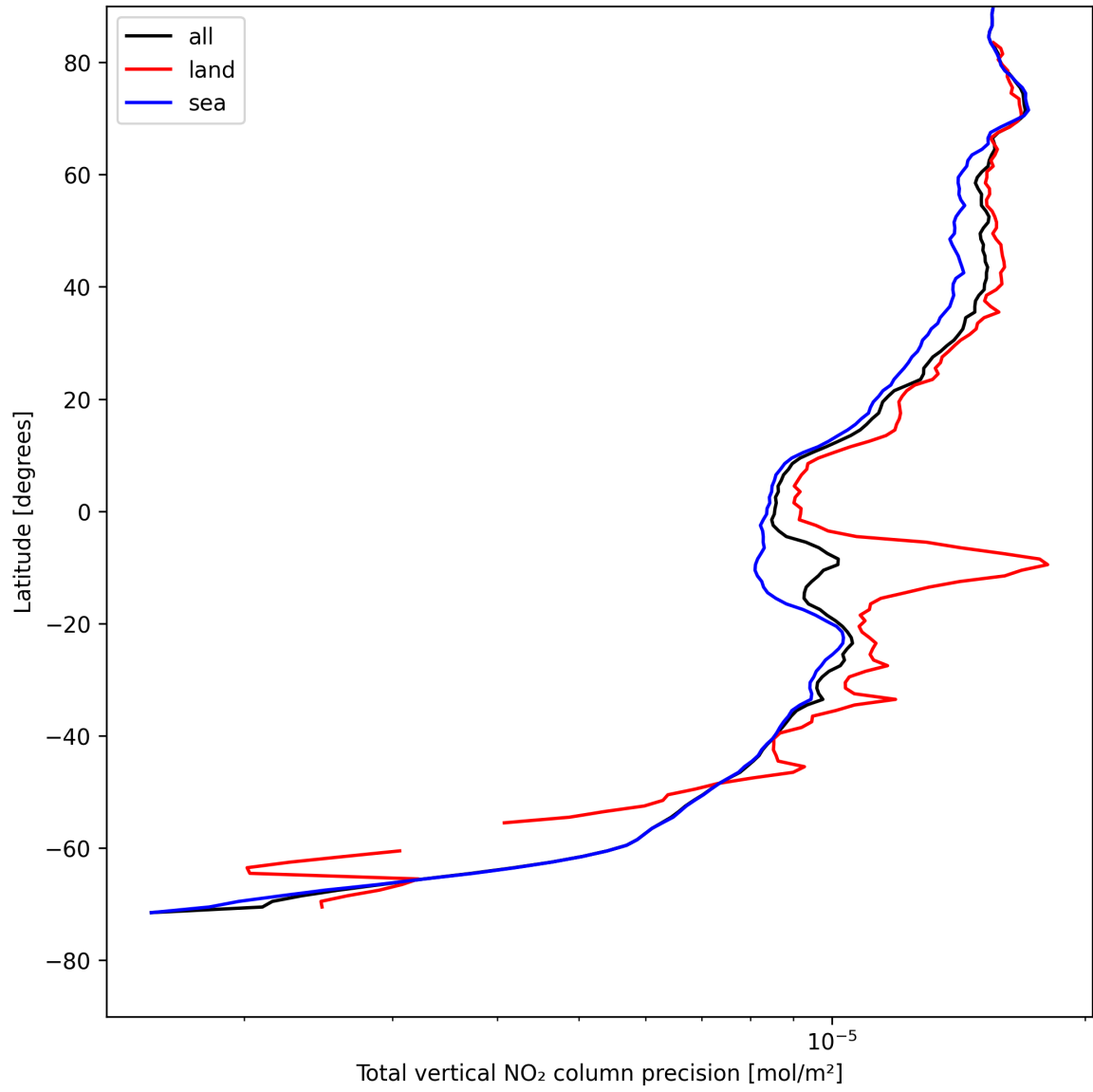
Figure 20: Zonal average of “Total vertical NO 2 column precision” for 2025-08-05 to 2025-08-06.
