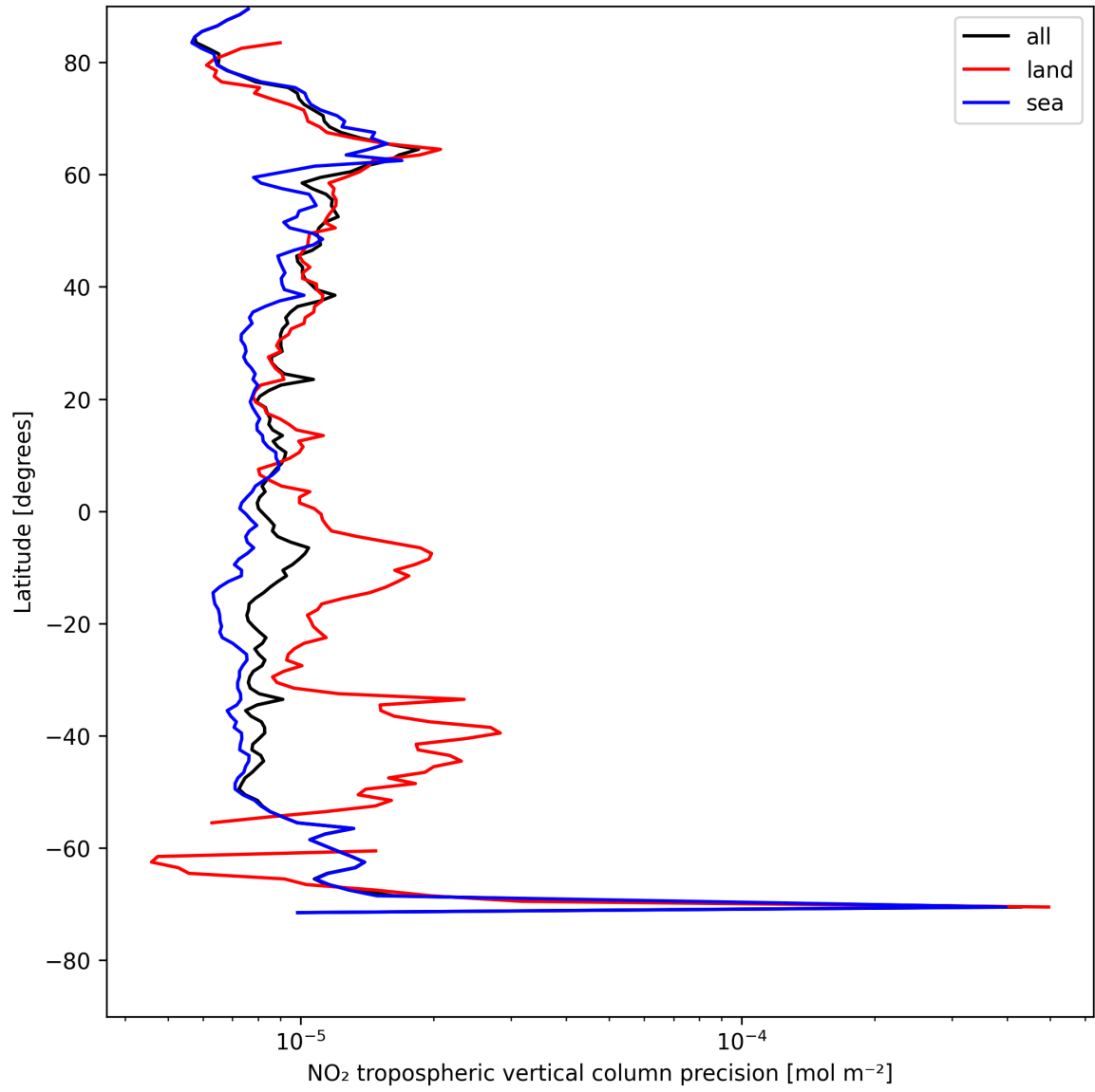
Figure 11: Zonal average of “NO 2 tropospheric vertical column precision” for 2025-08-05 to 2025-08-06.
