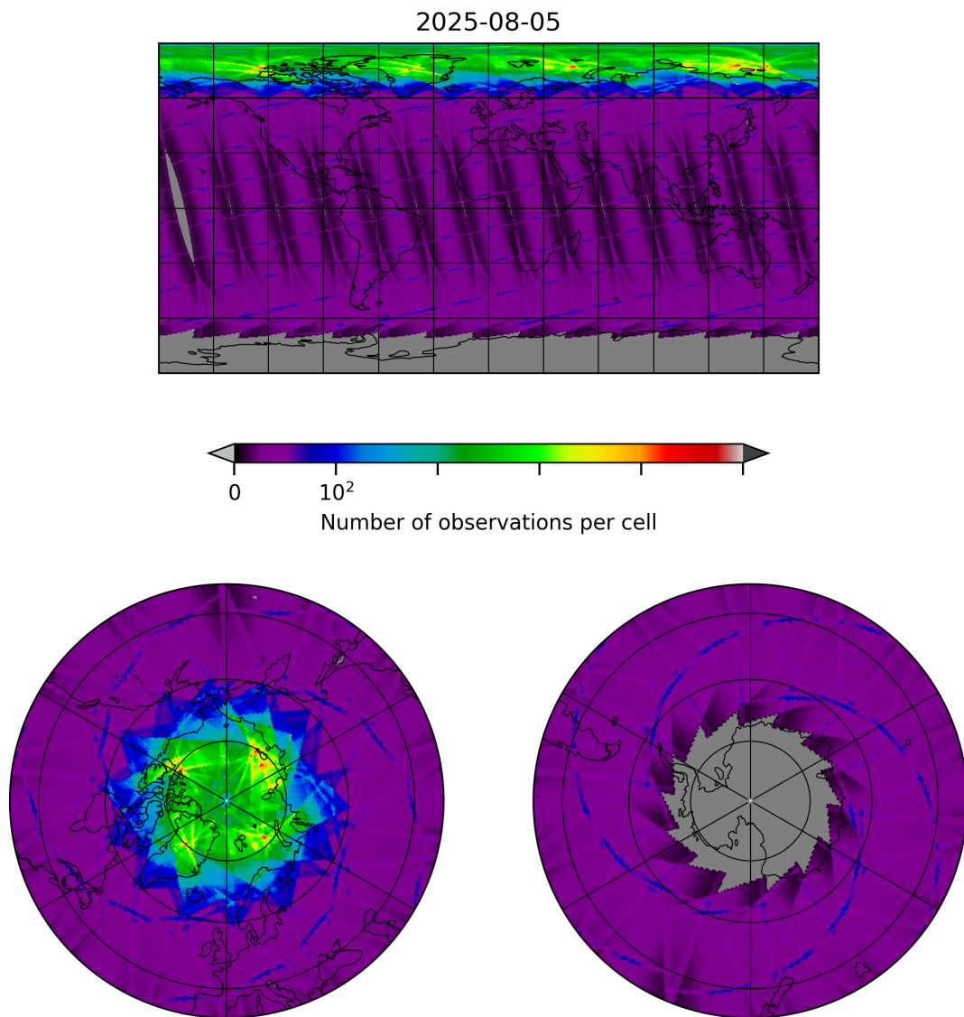
Figure 8: Map of the number of observations for 2025-08-05 to 2025-08-06
