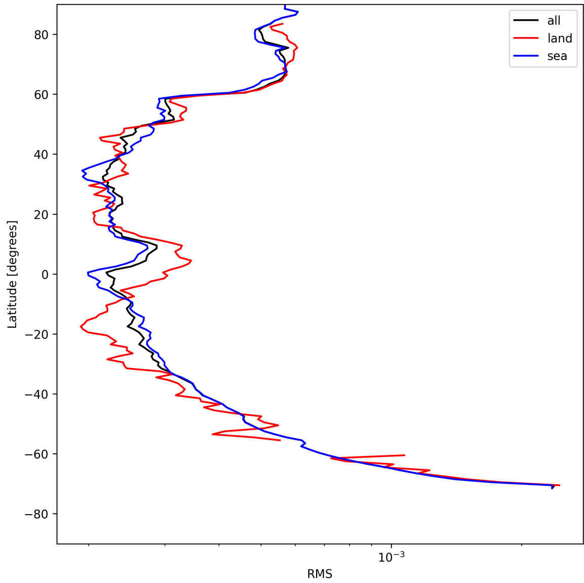
Figure 24: Zonal average of “RMS” for 2025-08-05 to 2025-08-06.
