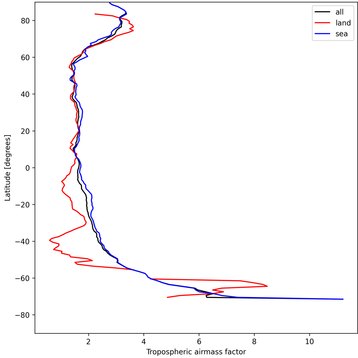
Figure 12: Zonal average of “Tropospheric air mass factor” for 2025-08-05 to 2025-08-06.
