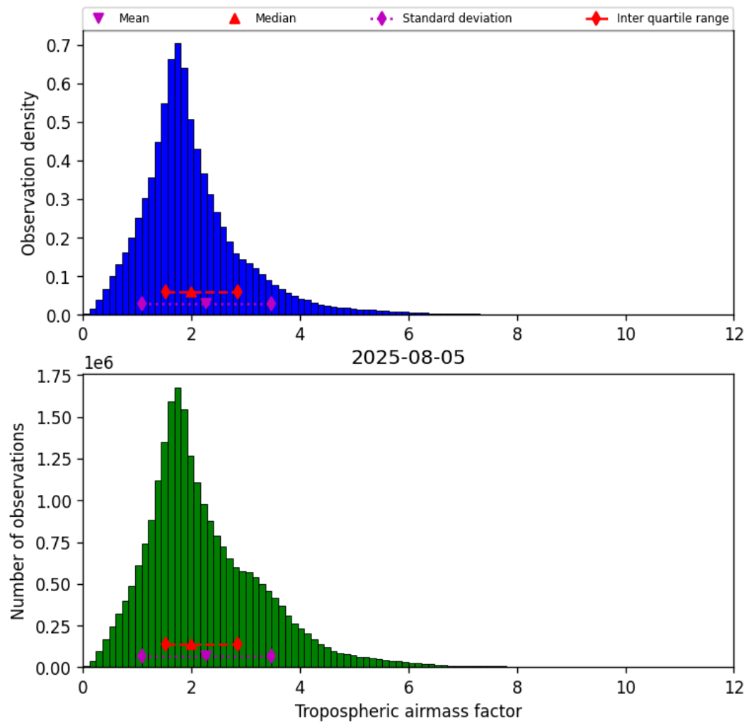
Figure 29: Histogram of “Tropospheric air mass factor” for 2025-08-05 to 2025-08-06
