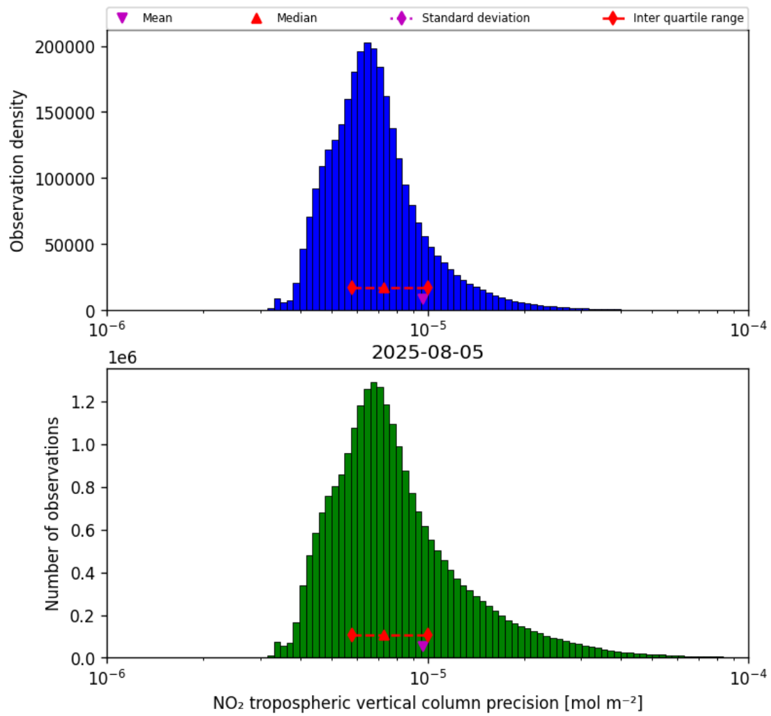
Figure 28: Histogram of “NO 2 tropospheric vertical column precision” for 2025-08-05 to 2025-08-06
