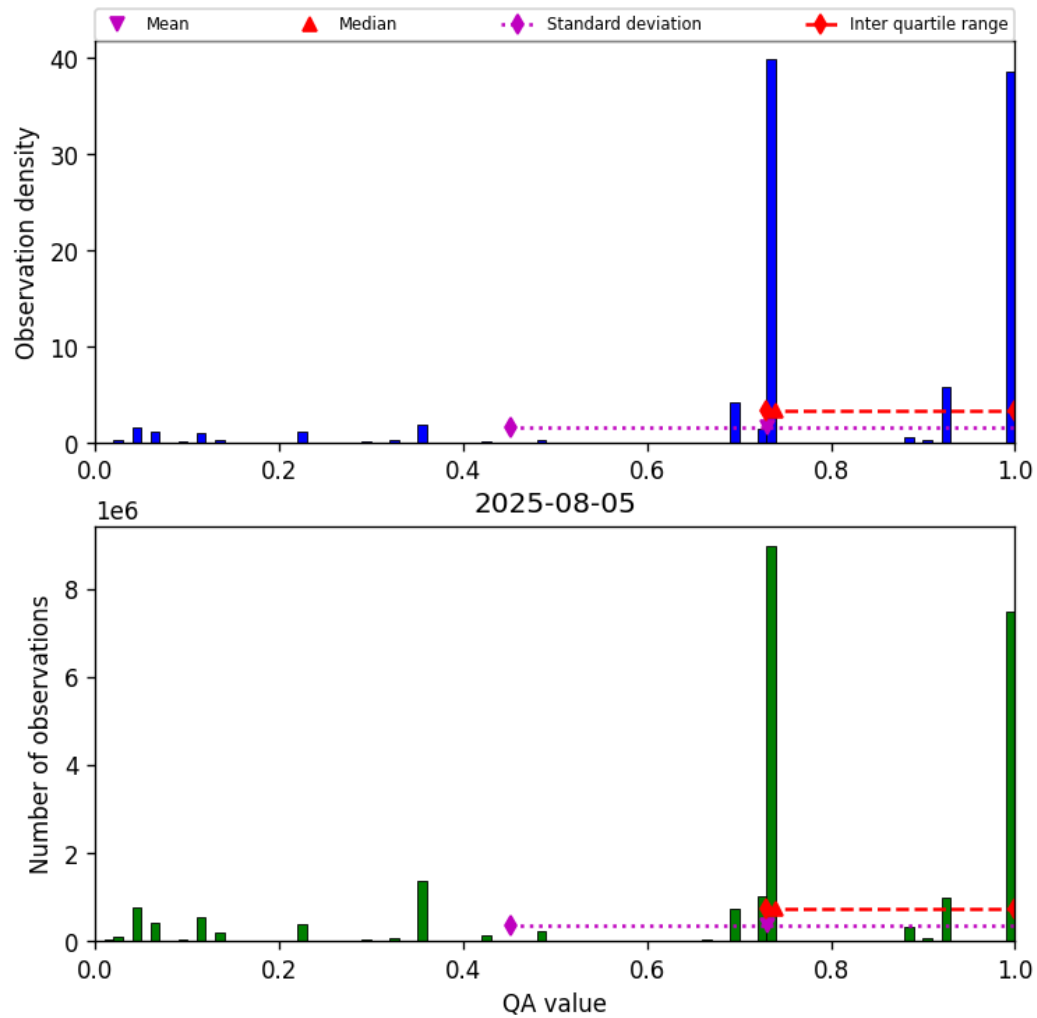
Figure 26: Histogram of “QA value” for 2025-08-05 to 2025-08-06
