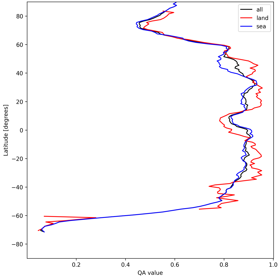
Figure 9: Zonal average of “QA value” for 2025-08-05 to 2025-08-06.
