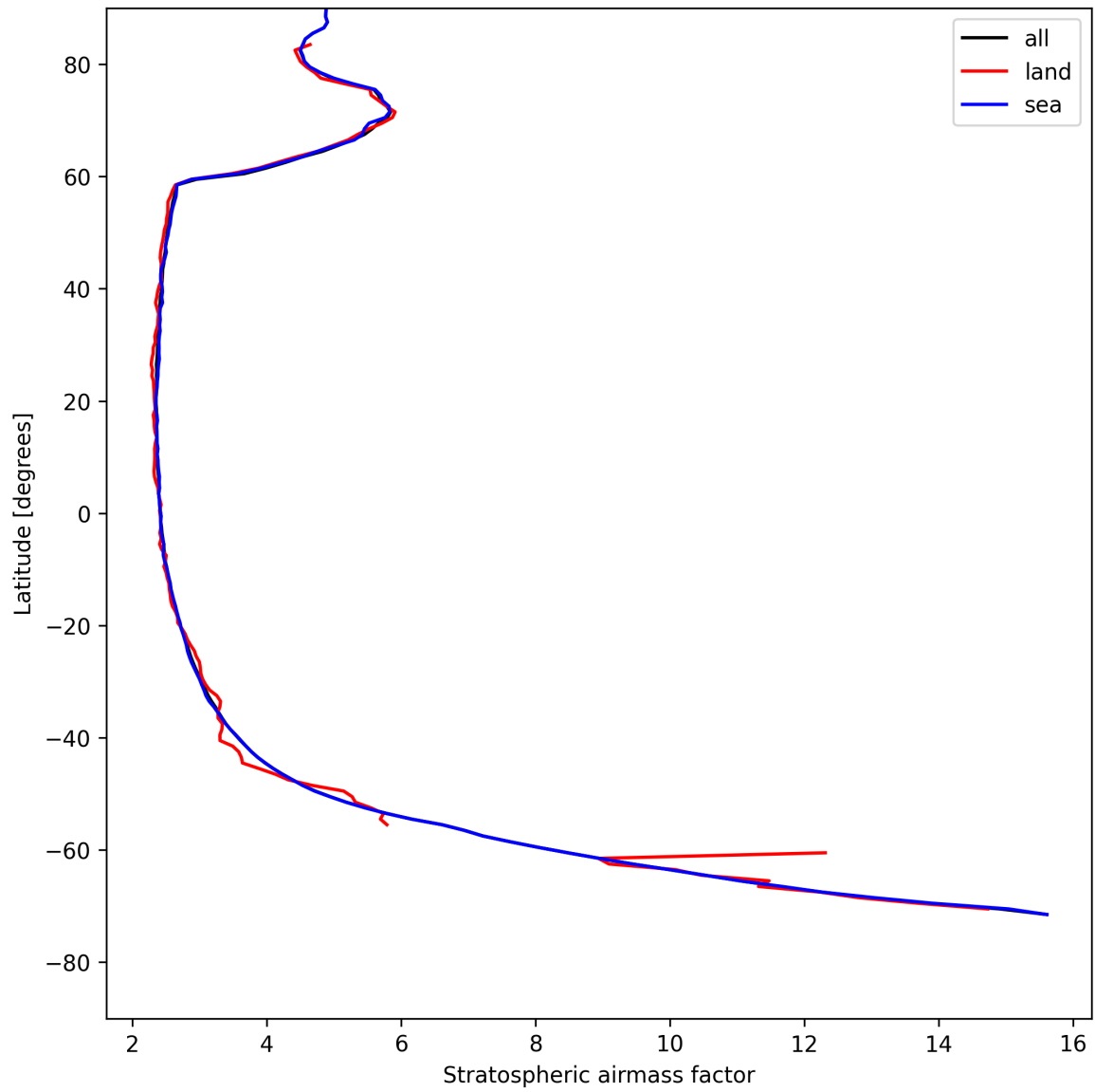
Figure 25: Zonal average of “Stratospheric airmass factor” for 2025-08-05 to 2025-08-06.
