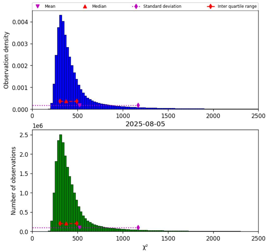
Figure 40: Histogram of “ \chi^2 ” for 2025-08-05 to 2025-08-06
