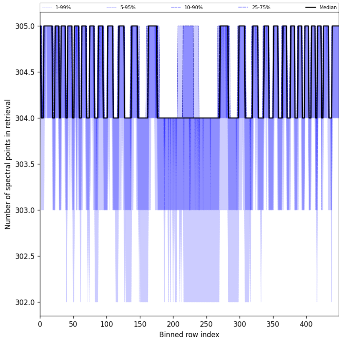
Figure 48: Along track statistics of “Number of spectral points in retrieval” for 2025-08-05 to 2025-08-06
