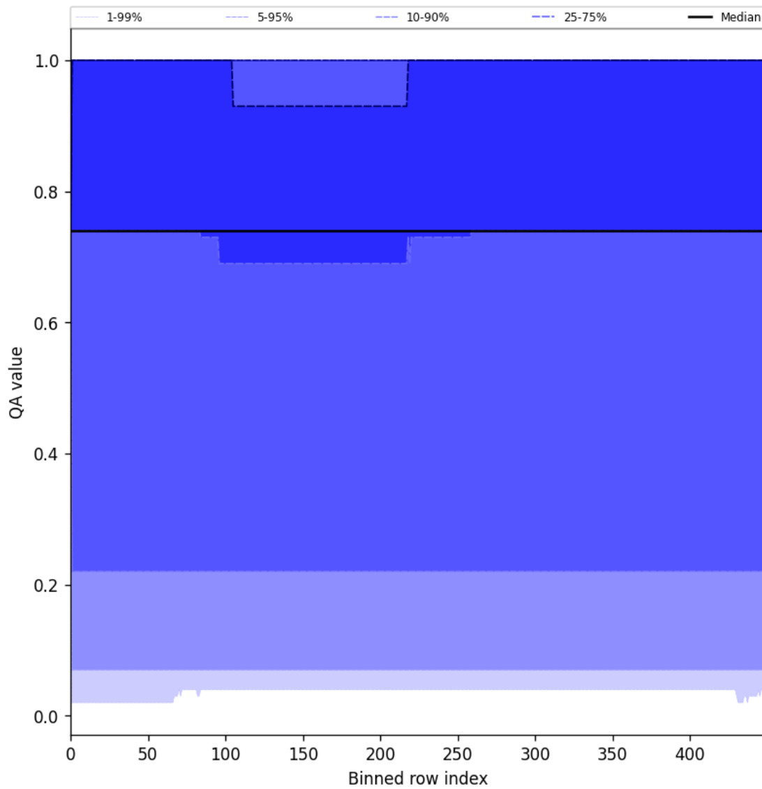
Figure 43: Along track statistics of “QA value” for 2025-08-05 to 2025-08-06
