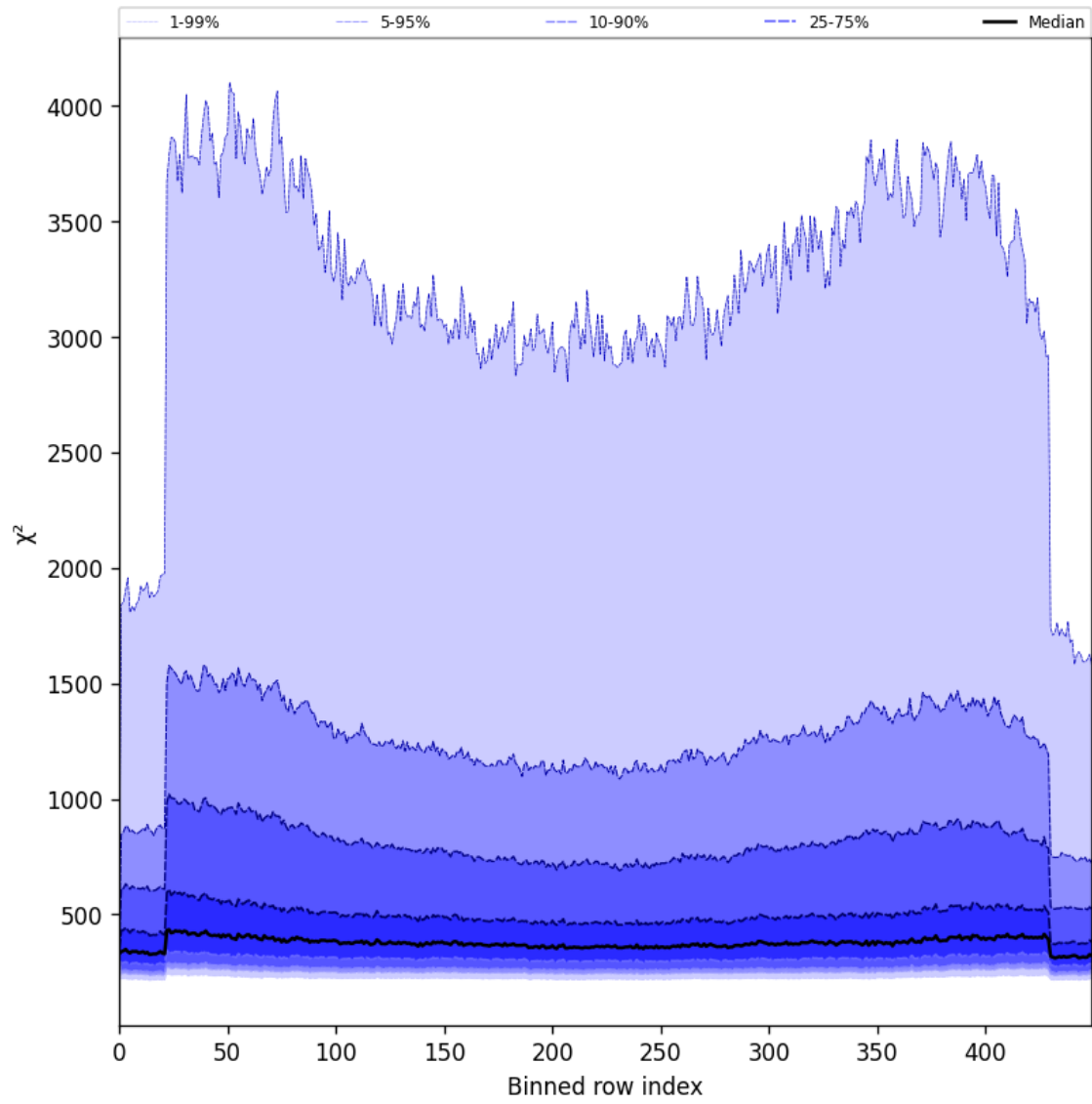
Figure 57: Along track statistics of “ \chi^2 ” for 2025-08-05 to 2025-08-06
