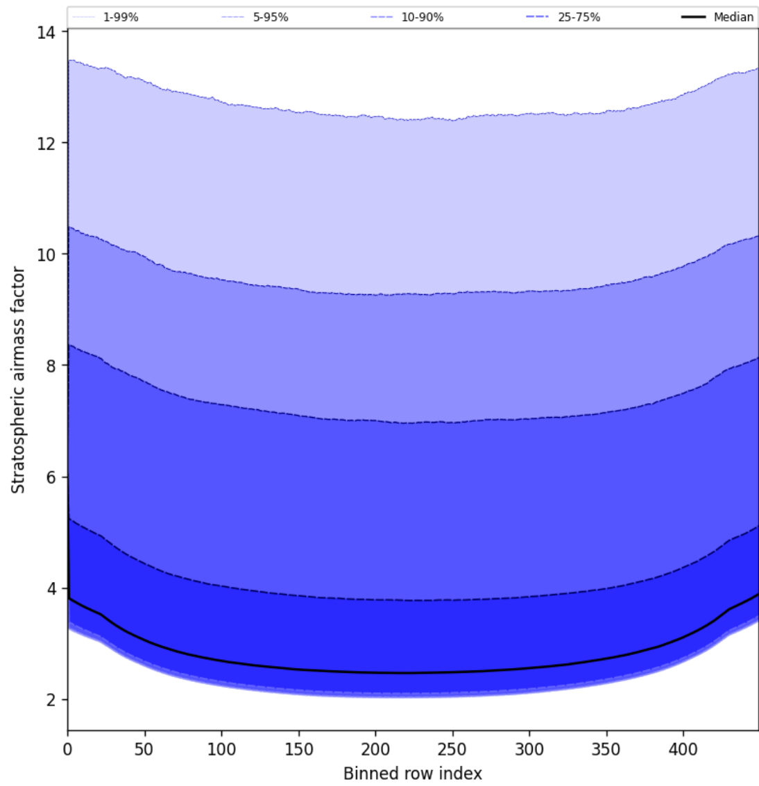
Figure 59: Along track statistics of “Stratospheric airmass factor” for 2025-08-05 to 2025-08-06
