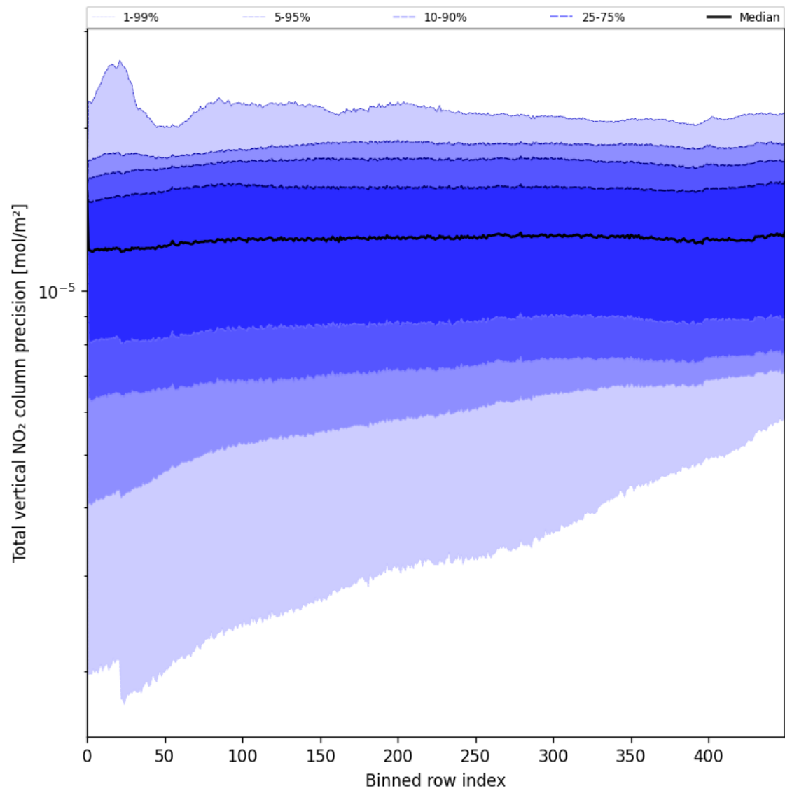
Figure 54: Along track statistics of “Total vertical NO 2 column precision” for 2025-08-05 to 2025-08-06
