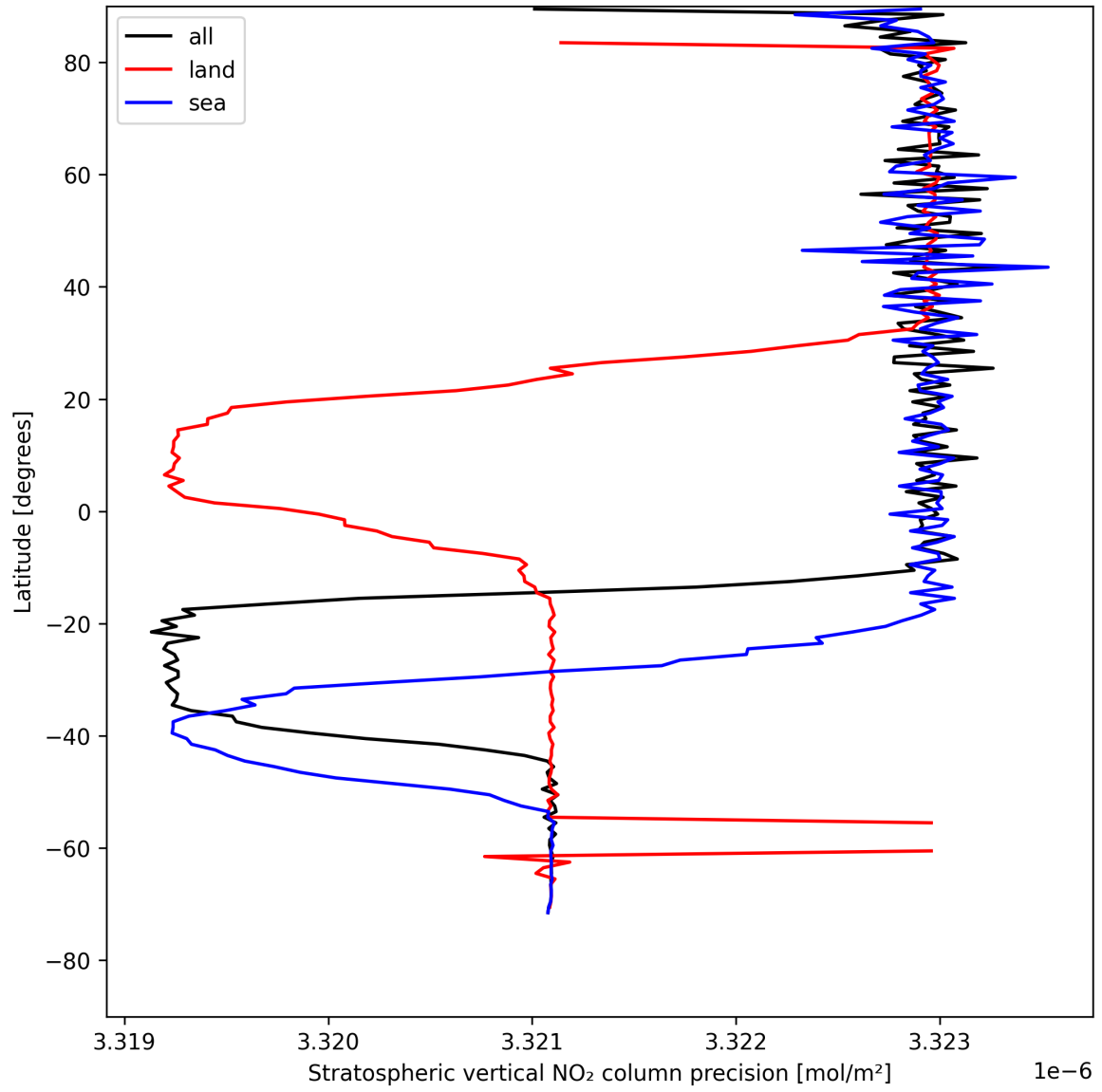
Figure 18: Zonal average of “Stratospheric vertical NO 2 column precision” for 2025-08-05 to 2025-08-06.
