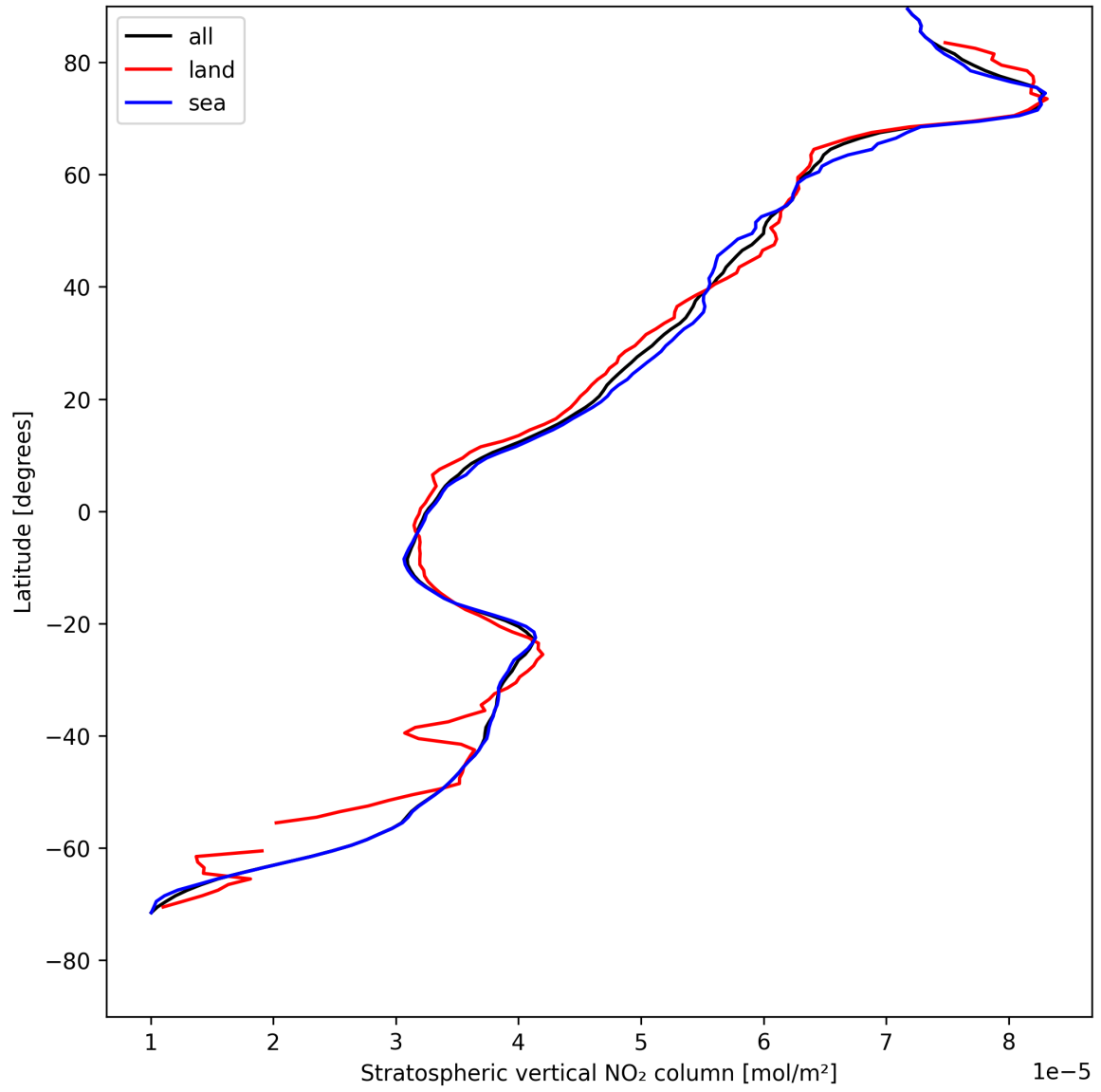
Figure 17: Zonal average of “Stratospheric vertical NO 2 column” for 2025-08-05 to 2025-08-06.
