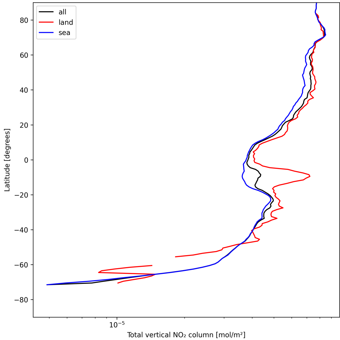
Figure 19: Zonal average of “Total vertical NO 2 column” for 2025-08-05 to 2025-08-06.
