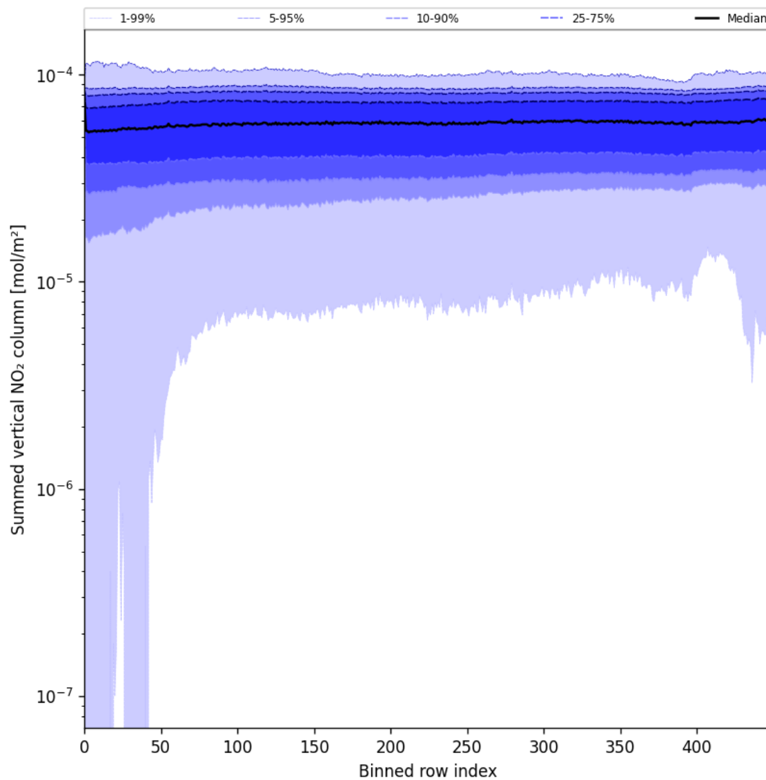
Figure 55: Along track statistics of “Summed vertical NO 2 column” for 2025-08-05 to 2025-08-06
