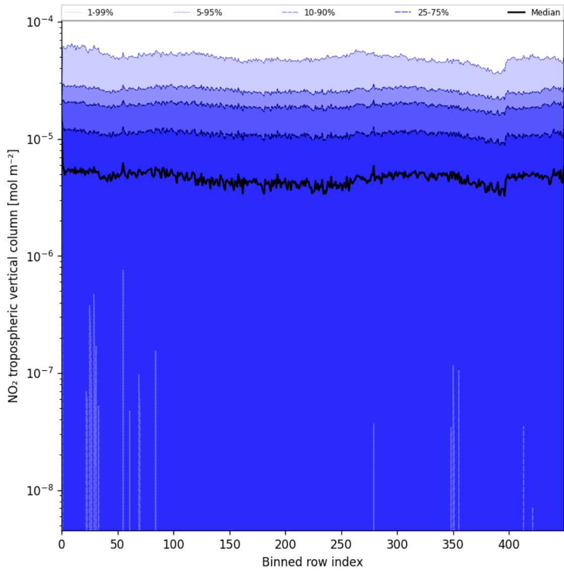
Figure 44: Along track statistics of "NO 2 tropospheric vertical column" for 2025-08-05 to 2025-08-06
