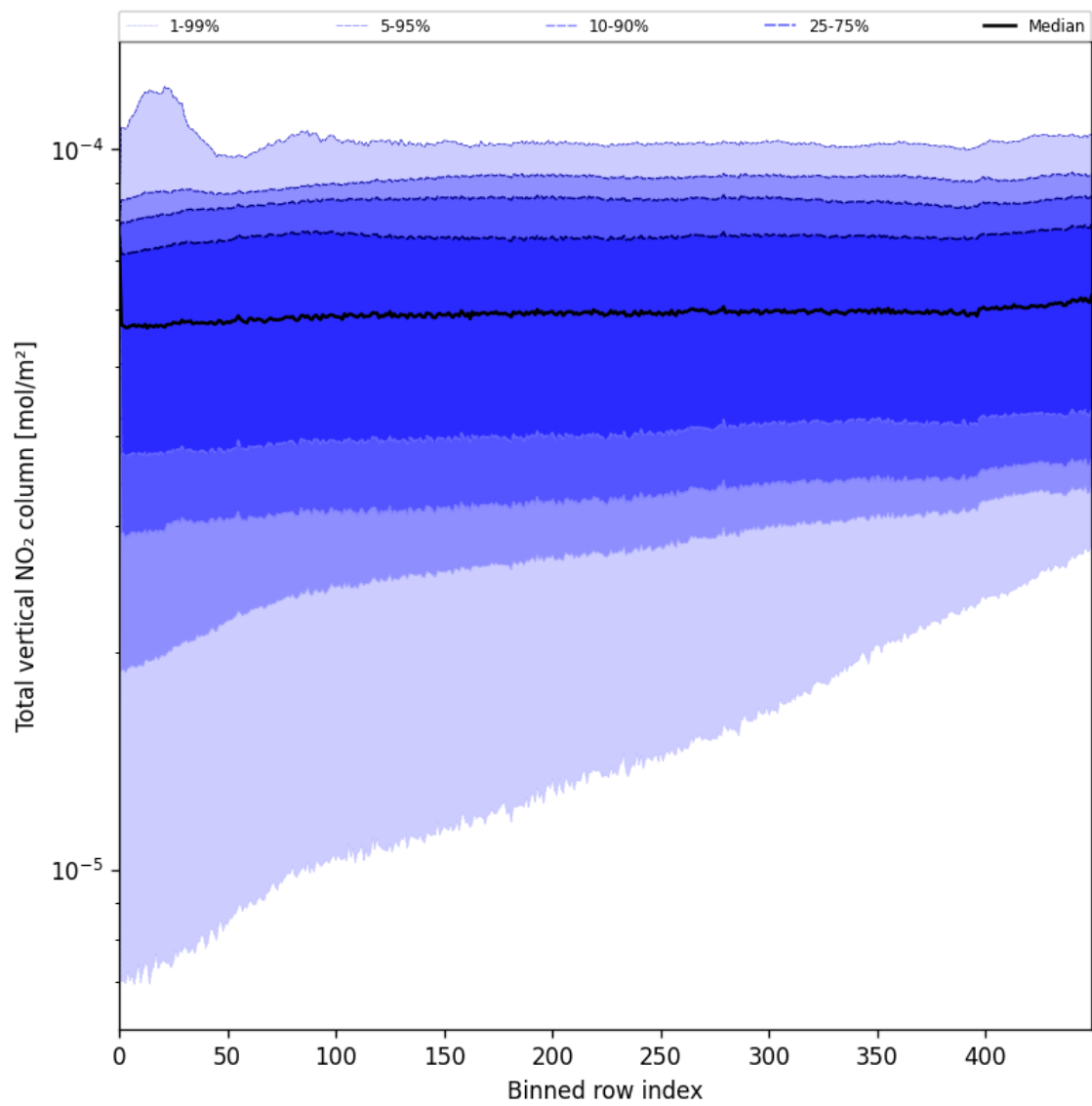
Figure 53: Along track statistics of “Total vertical NO 2 column” for 2025-08-05 to 2025-08-06
