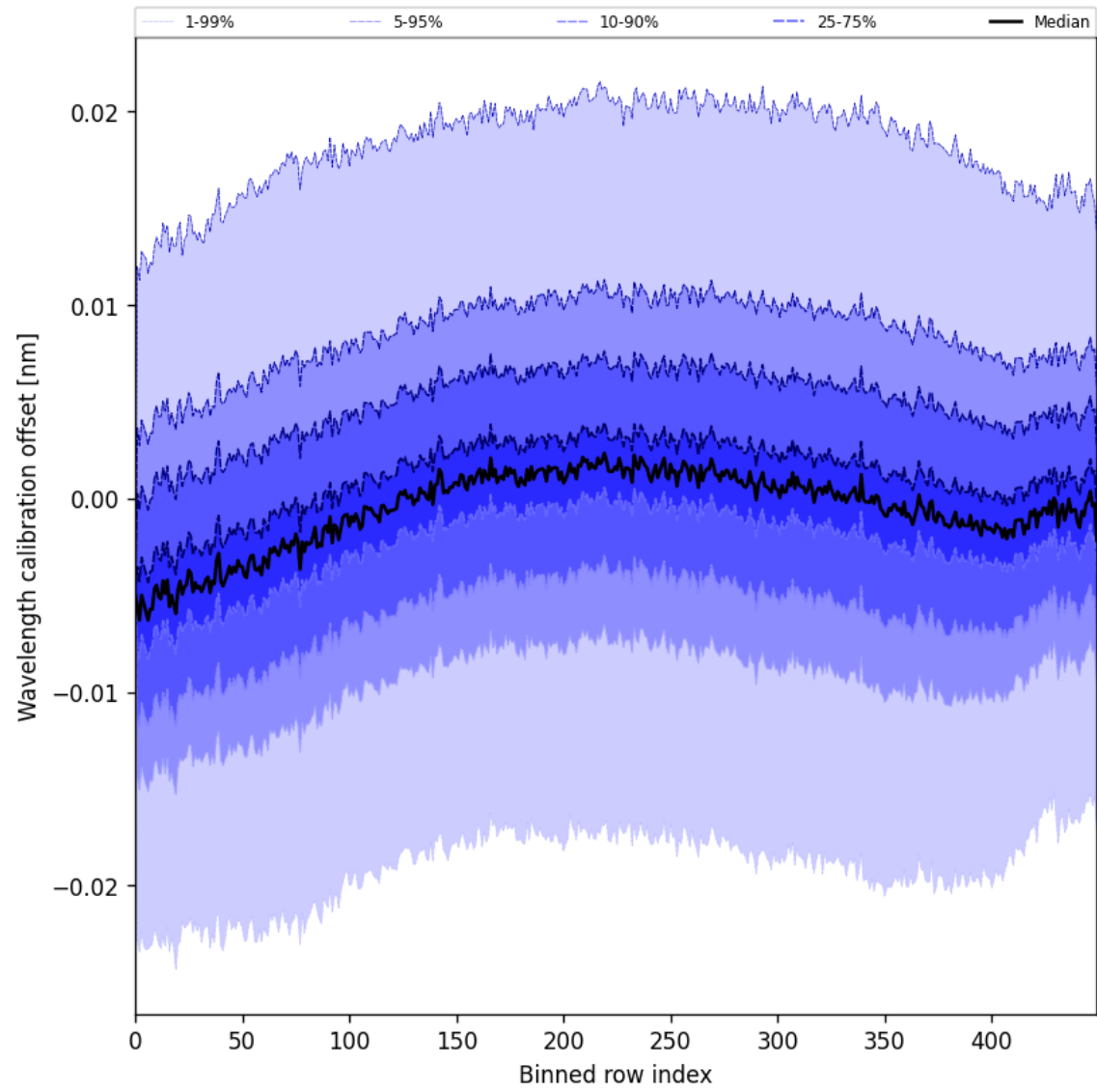
Figure 50: Along track statistics of “Wavelength calibration offset” for 2025-08-05 to 2025-08-06
