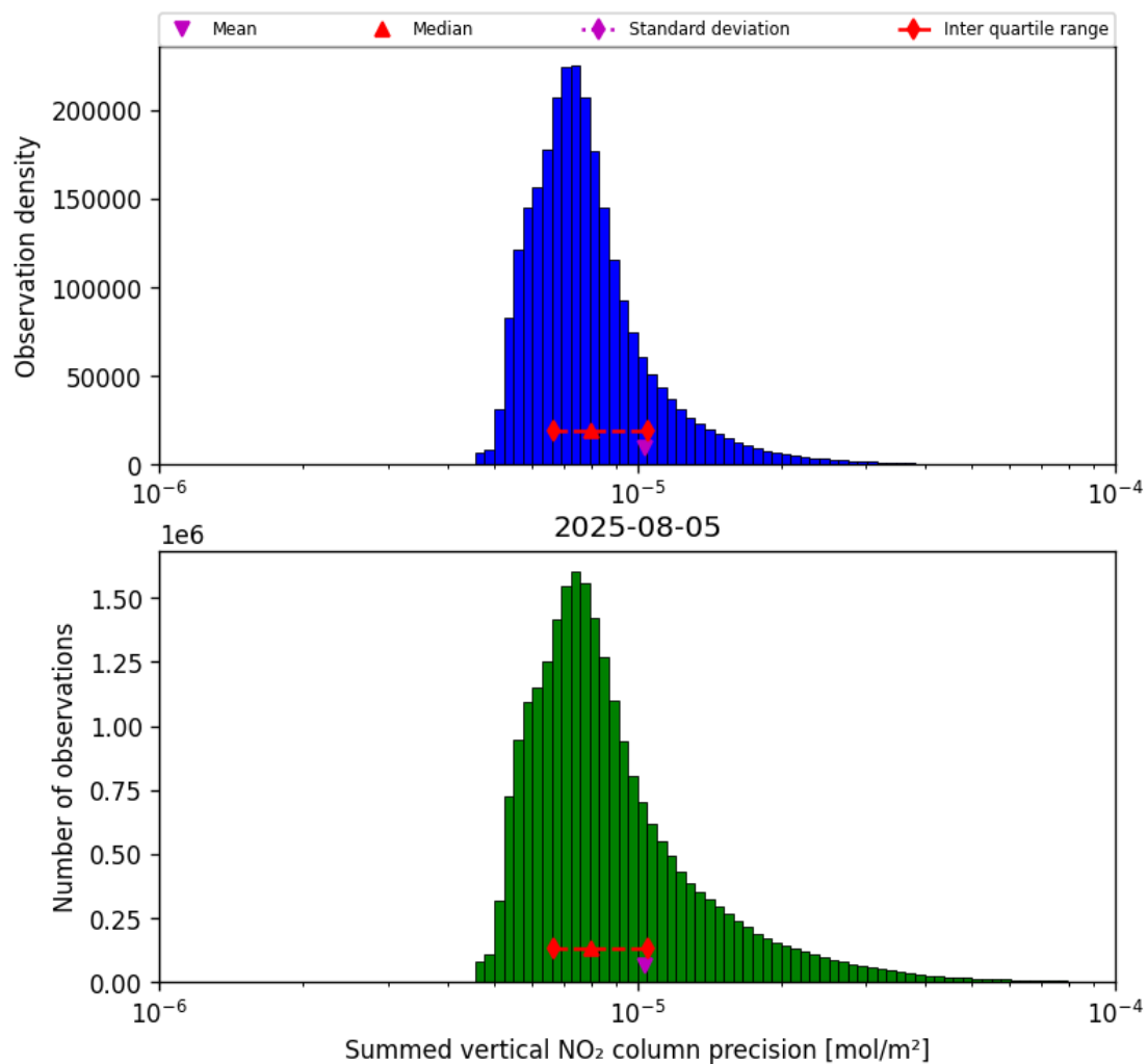
Figure 39: Histogram of “Summed vertical NO 2 column precision” for 2025-08-05 to 2025-08-06
