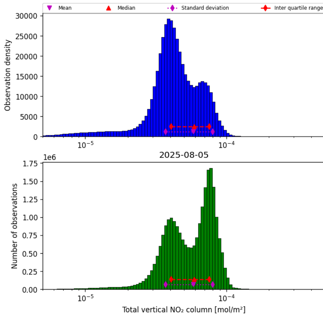
Figure 36: Histogram of “Total vertical NO 2 column” for 2025-08-05 to 2025-08-06
