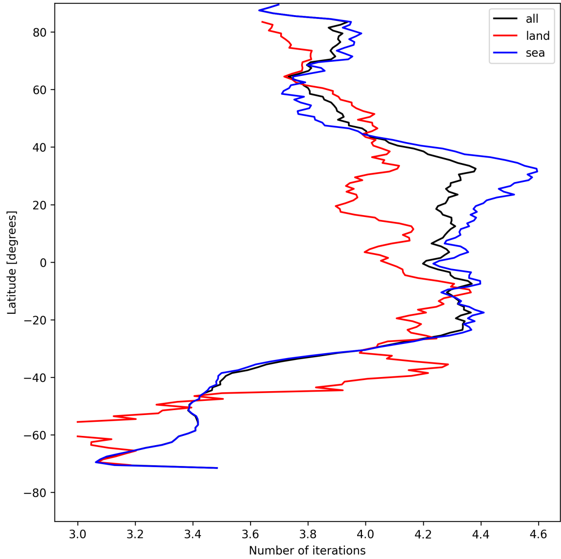
Figure 15: Zonal average of “Number of iterations” for 2025-08-05 to 2025-08-06.
