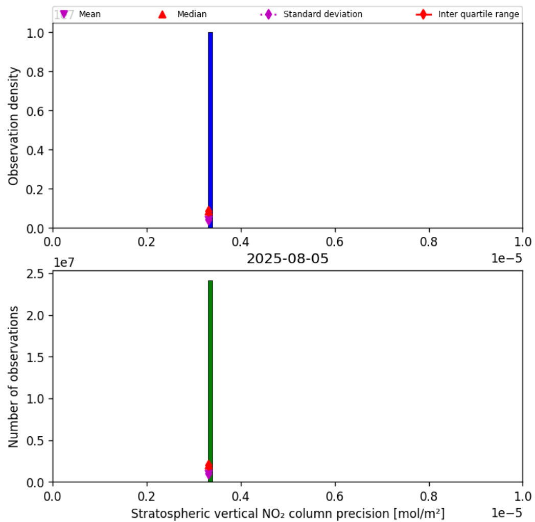
Figure 35: Histogram of “Stratospheric vertical NO 2 column precision” for 2025-08-05 to 2025-08-06
