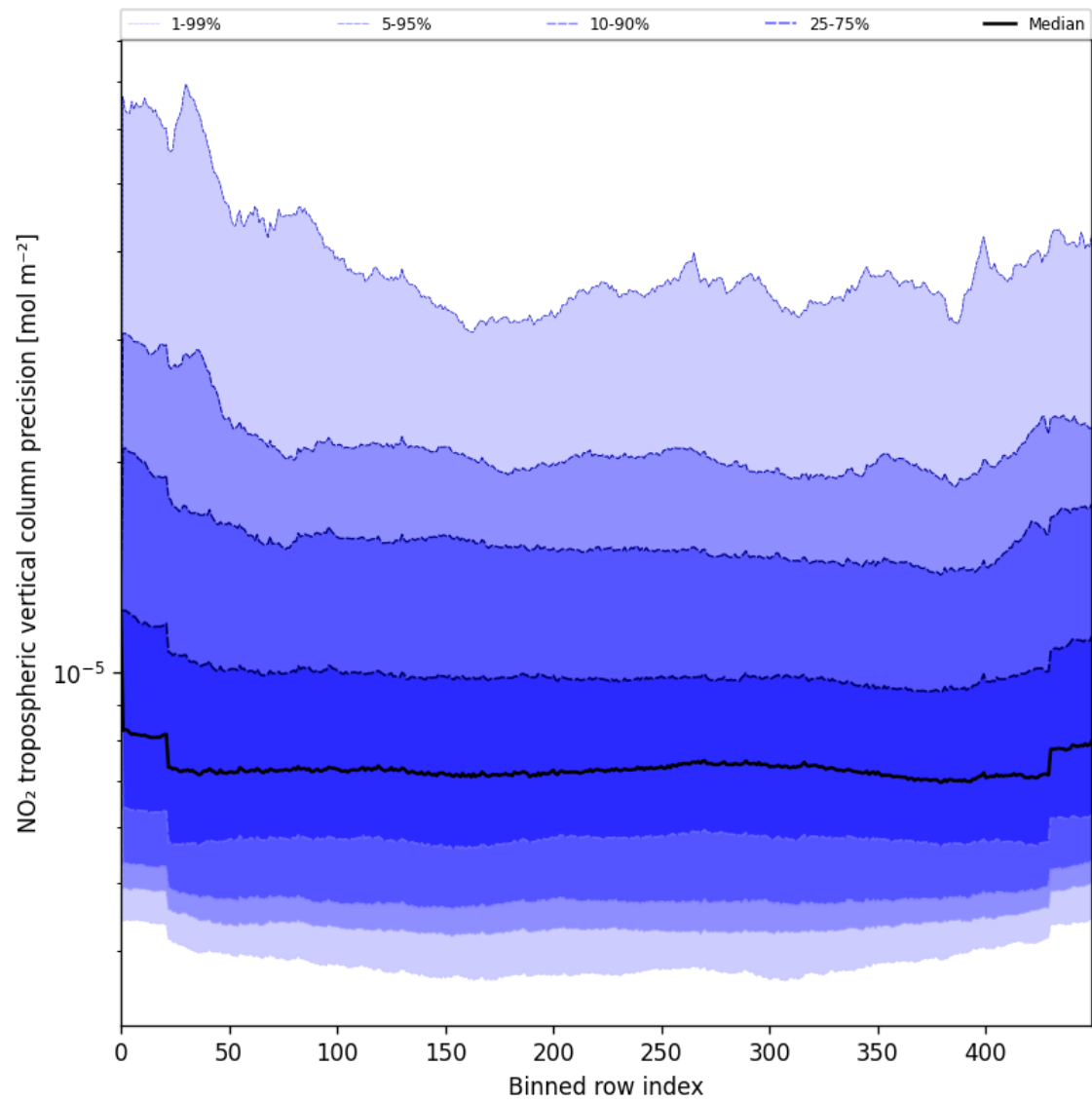
Figure 45: Along track statistics of “NO 2 tropospheric vertical column precision” for 2025-08-05 to 2025-08-06
