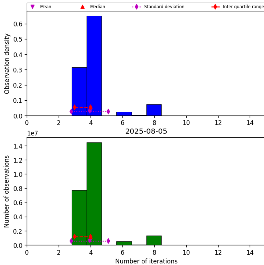
Figure 32: Histogram of “Number of iterations” for 2025-08-05 to 2025-08-06
