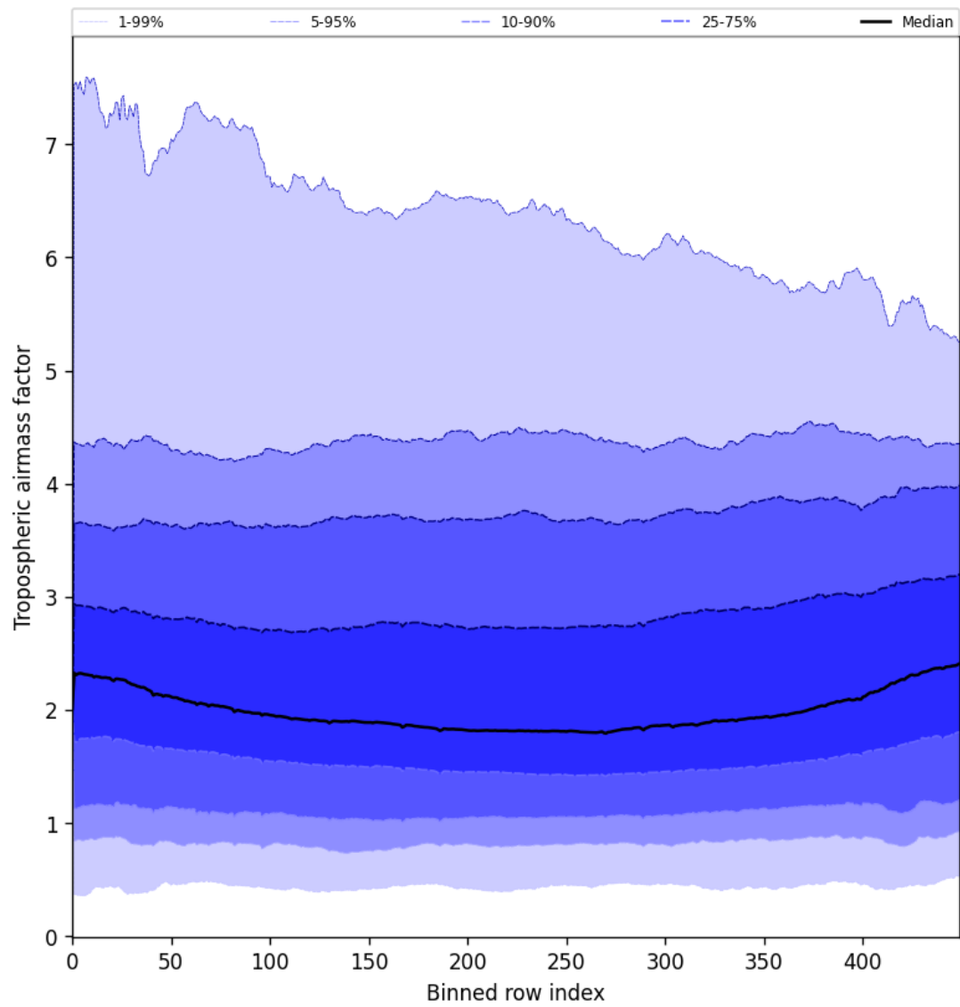
Figure 46: Along track statistics of “Tropospheric airmass factor” for 2025-08-05 to 2025-08-06
