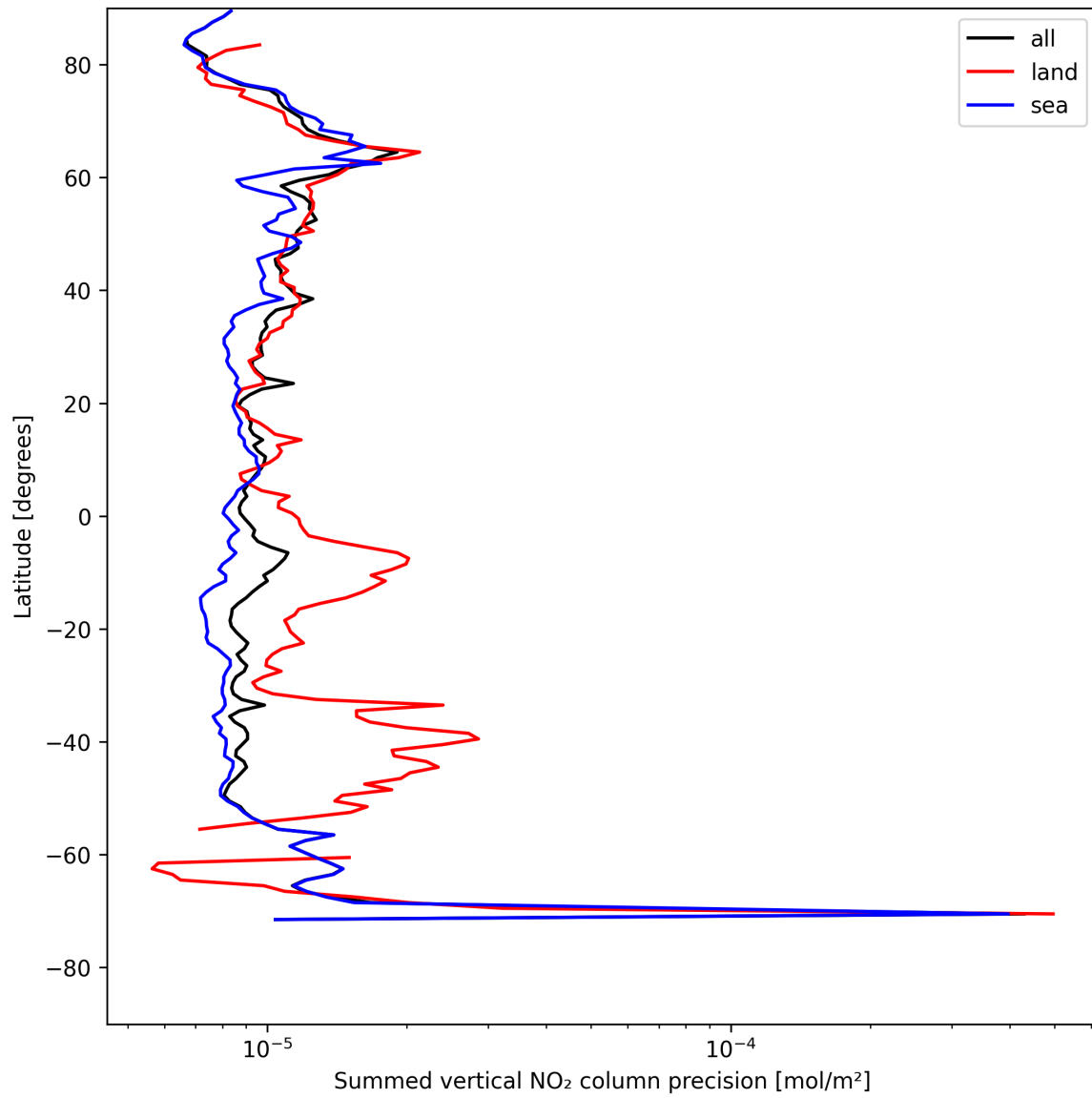
Figure 22: Zonal average of “Summed vertical NO 2 column precision” for 2025-08-05 to 2025-08-06.
