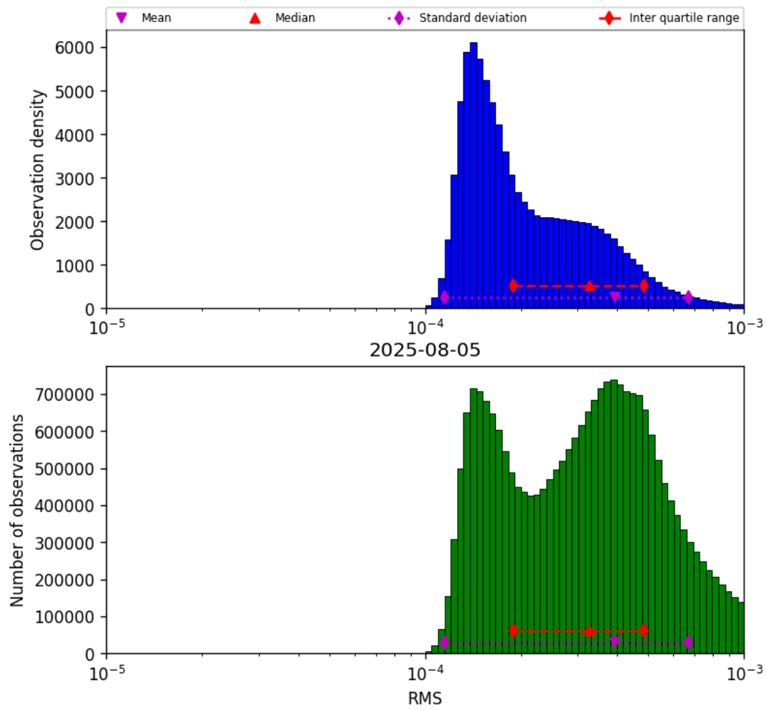
Figure 41: Histogram of “RMS” for 2025-08-05 to 2025-08-06
