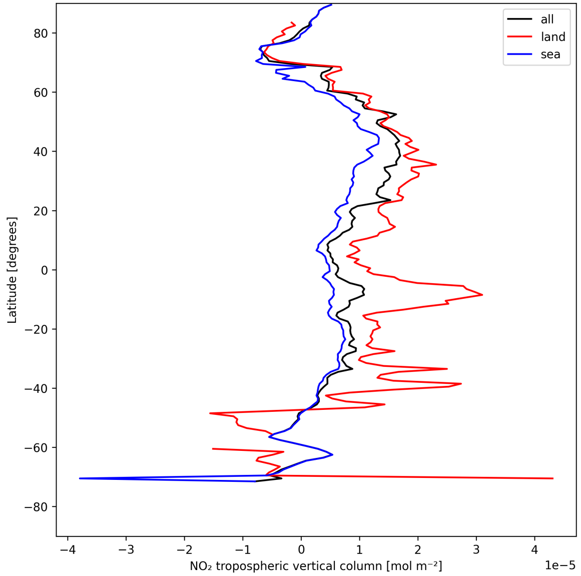
Figure 10: Zonal average of “NO 2 tropospheric vertical column” for 2025-08-05 to 2025-08-06.
