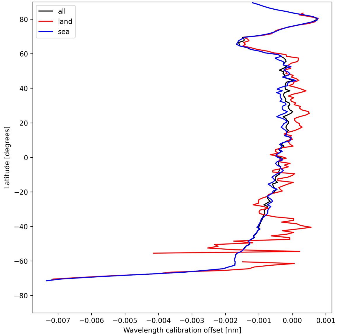
Figure 16: Zonal average of “Wavelength calibration offset” for 2025-08-05 to 2025-08-06.
