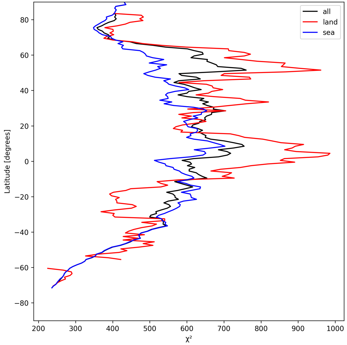
Figure 23: Zonal average of “ \chi^2 ” for 2025-08-05 to 2025-08-06.
