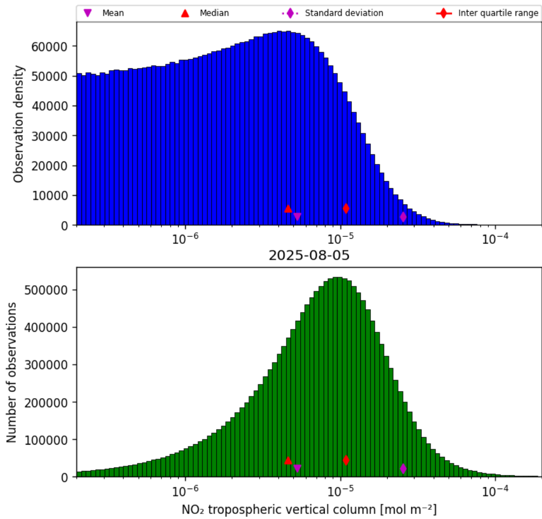
Figure 27: Histogram of “NO 2 tropospheric vertical column” for 2025-08-05 to 2025-08-06
