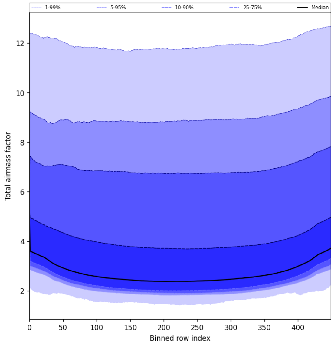
Figure 47: Along track statistics of “Total airmass factor” for 2025-08-05 to 2025-08-06
