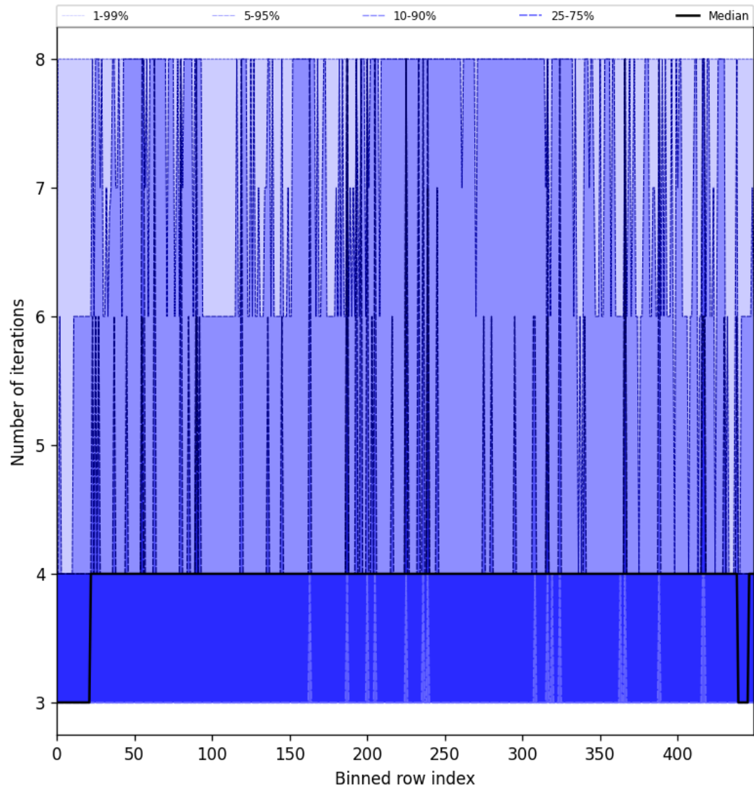
Figure 49: Along track statistics of “Number of iterations” for 2025-08-05 to 2025-08-06
