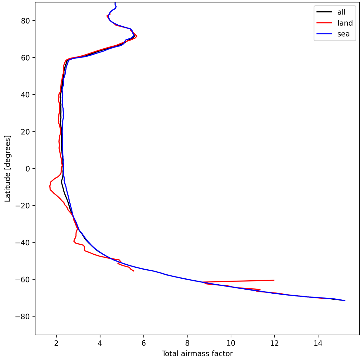
Figure 13: Zonal average of “Total airmass factor” for 2025-08-05 to 2025-08-06.
