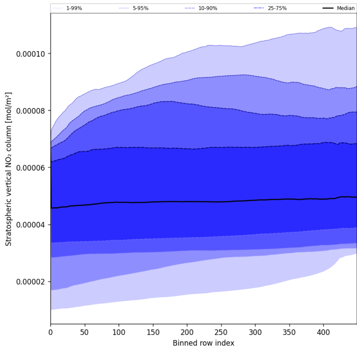
Figure 51: Along track statistics of “Stratospheric vertical NO 2 column” for 2025-08-05 to 2025-08-06
