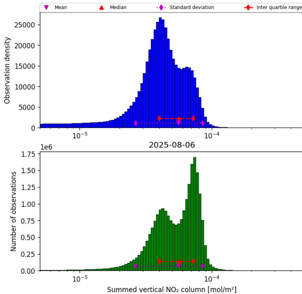
Figure 38: Histogram of “Summed vertical NO 2 column” for 2025-08-06 to 2025-08-07
