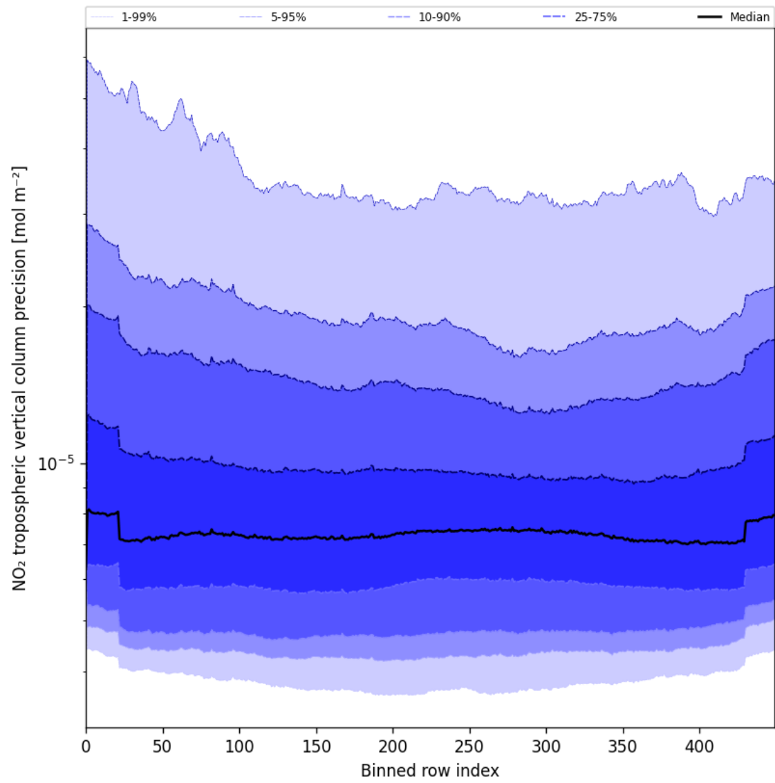
Figure 45: Along track statistics of “NO 2 tropospheric vertical column precision” for 2025-08-06 to 2025-08-07
