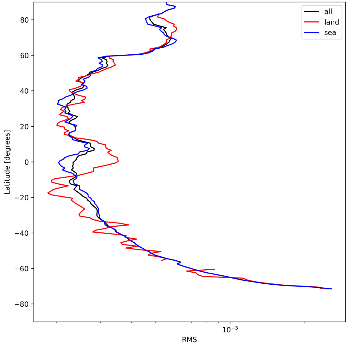
Figure 24: Zonal average of “RMS” for 2025-08-06 to 2025-08-07.
