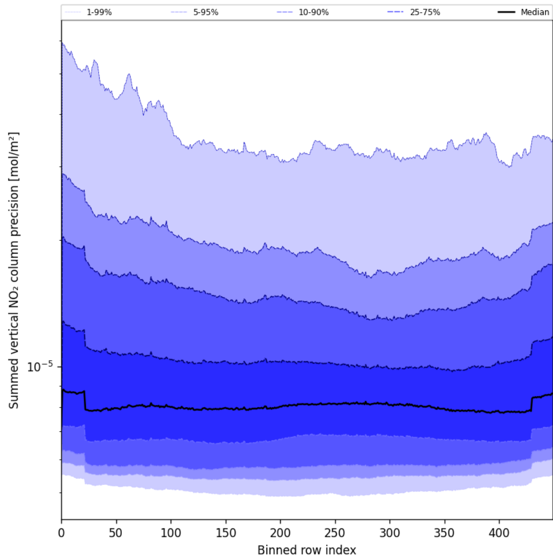
Figure 56: Along track statistics of “Summed vertical NO 2 column precision” for 2025-08-06 to 2025-08-07
