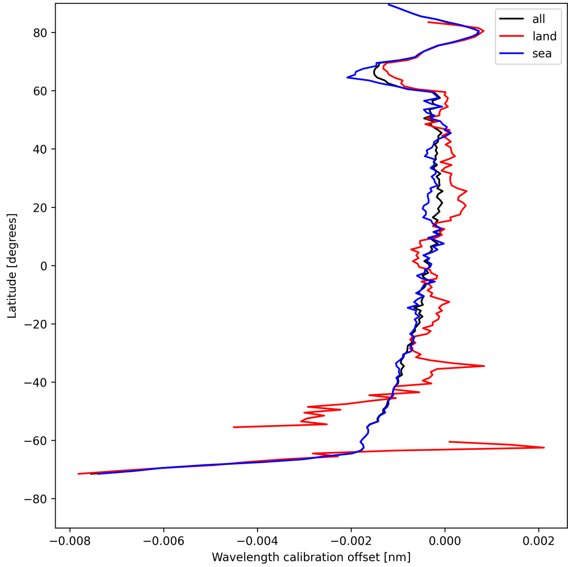
Figure 16: Zonal average of “Wavelength calibration offset” for 2025-08-06 to 2025-08-07.
