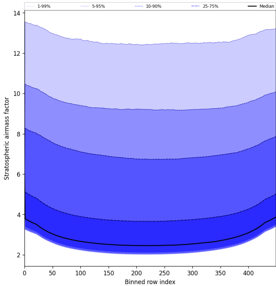
Figure 59: Along track statistics of “Stratospheric airmass factor” for 2025-08-06 to 2025-08-07
