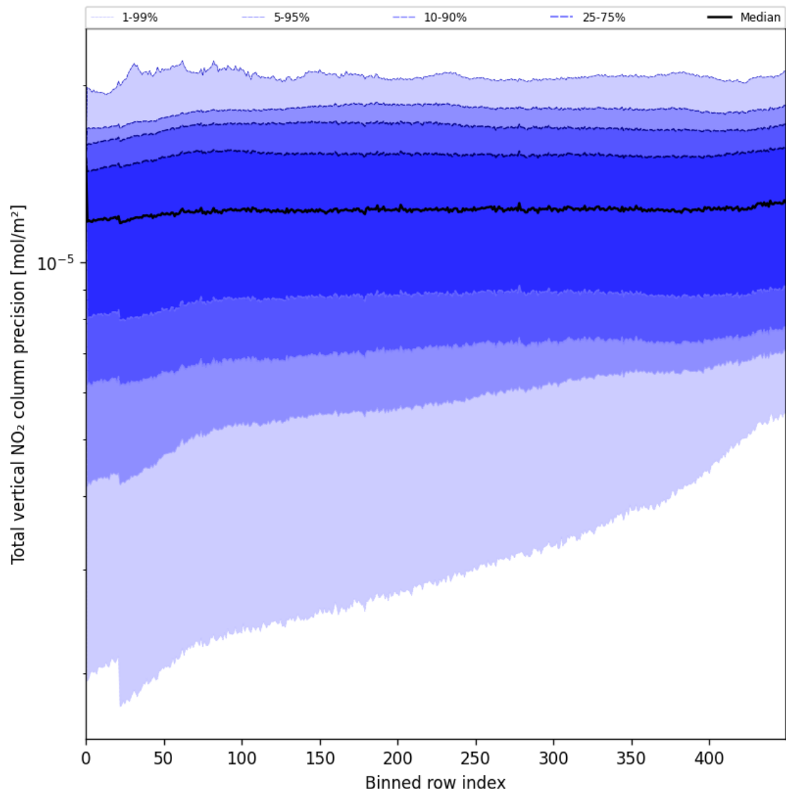
Figure 54: Along track statistics of “Total vertical NO 2 column precision” for 2025-08-06 to 2025-08-07
