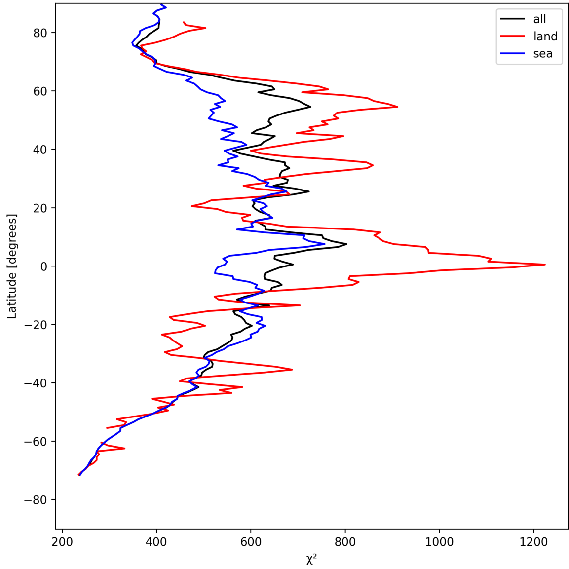
Figure 23: Zonal average of “ \chi^2 ” for 2025-08-06 to 2025-08-07.
