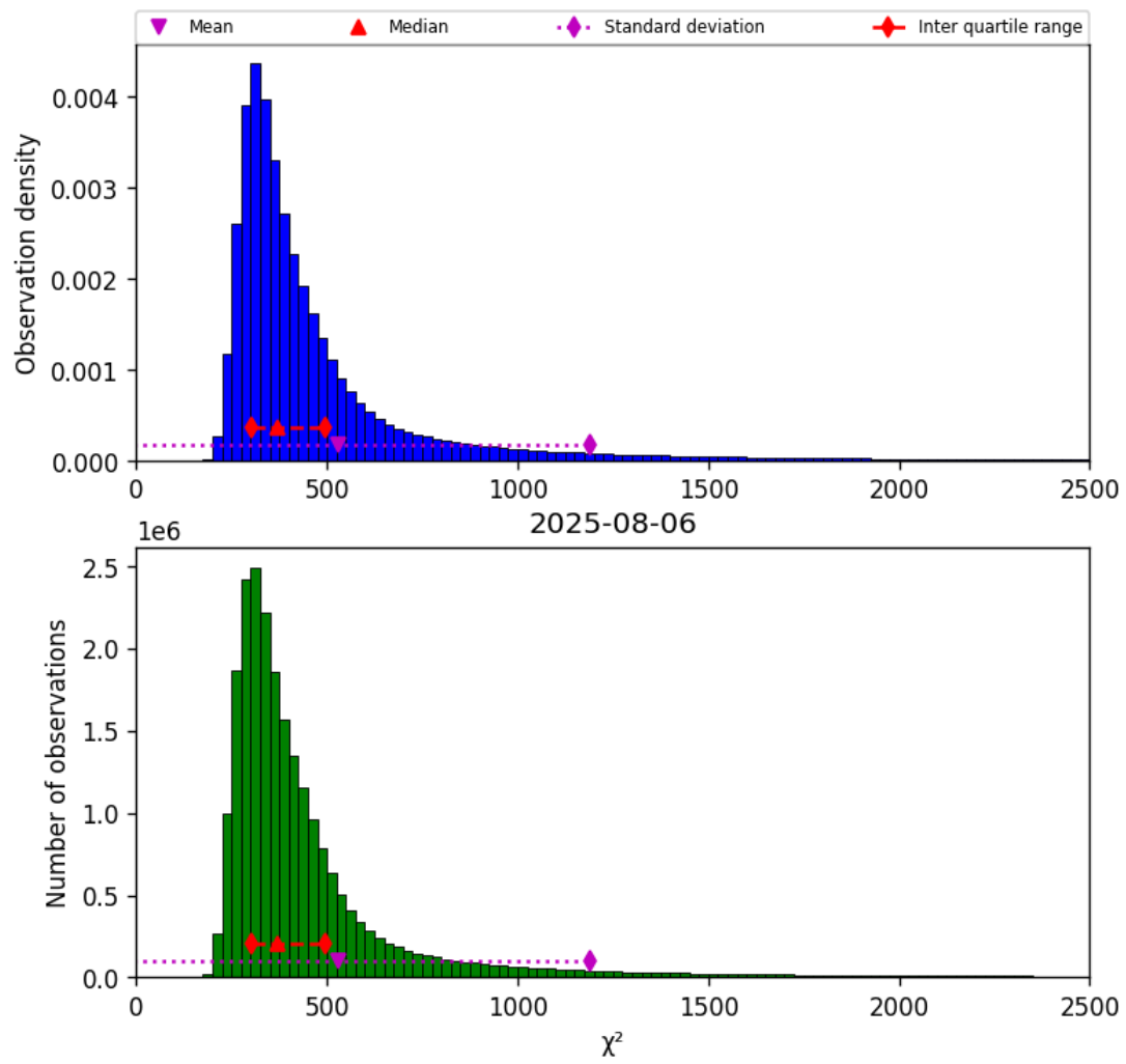
Figure 40: Histogram of “ \chi^2 ” for 2025-08-06 to 2025-08-07
