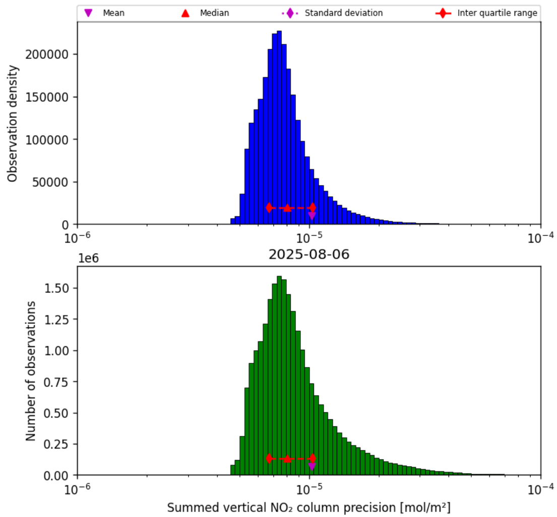
Figure 39: Histogram of “Summed vertical NO 2 column precision” for 2025-08-06 to 2025-08-07
