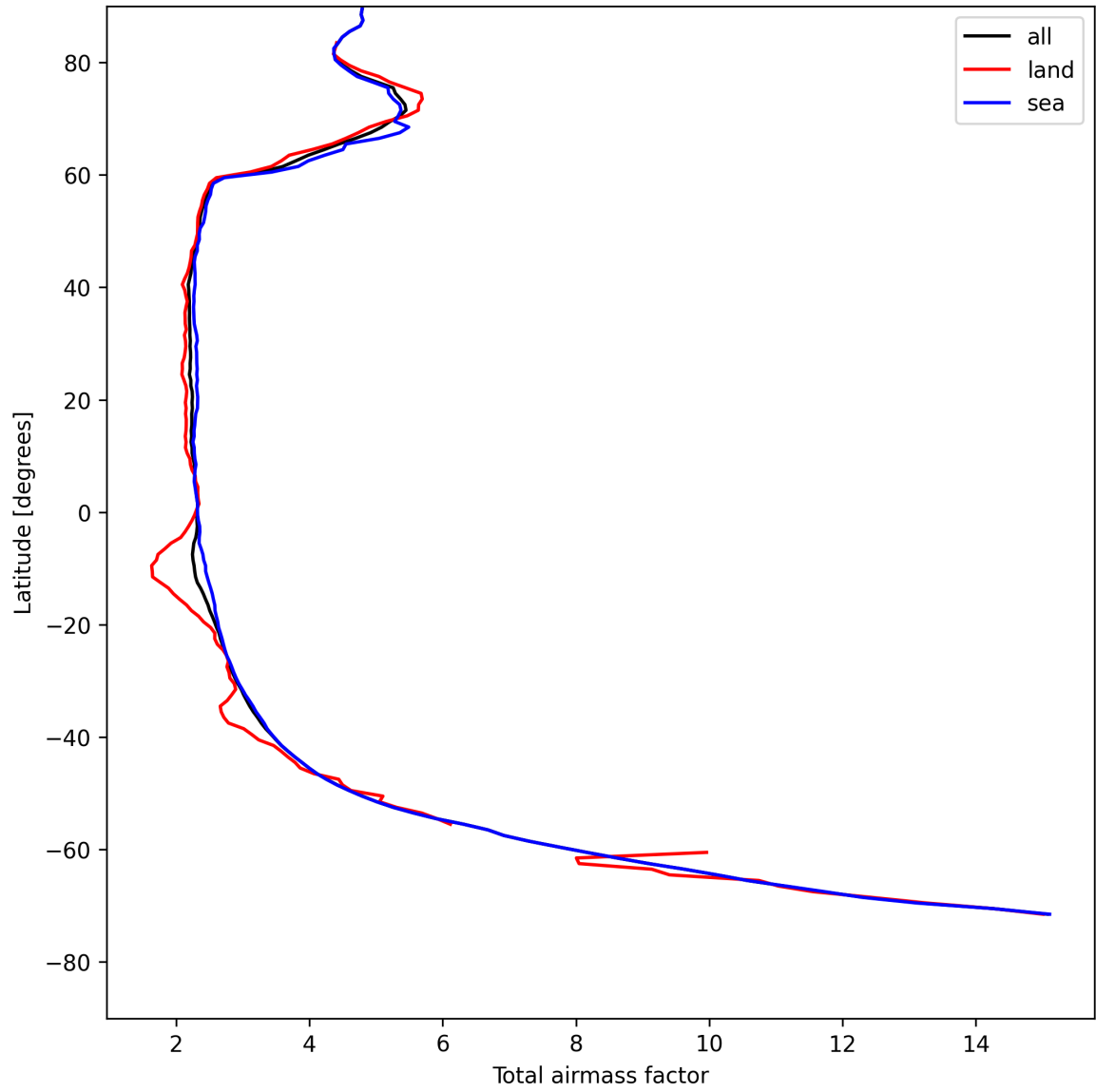
Figure 13: Zonal average of “Total airmass factor” for 2025-08-06 to 2025-08-07.
