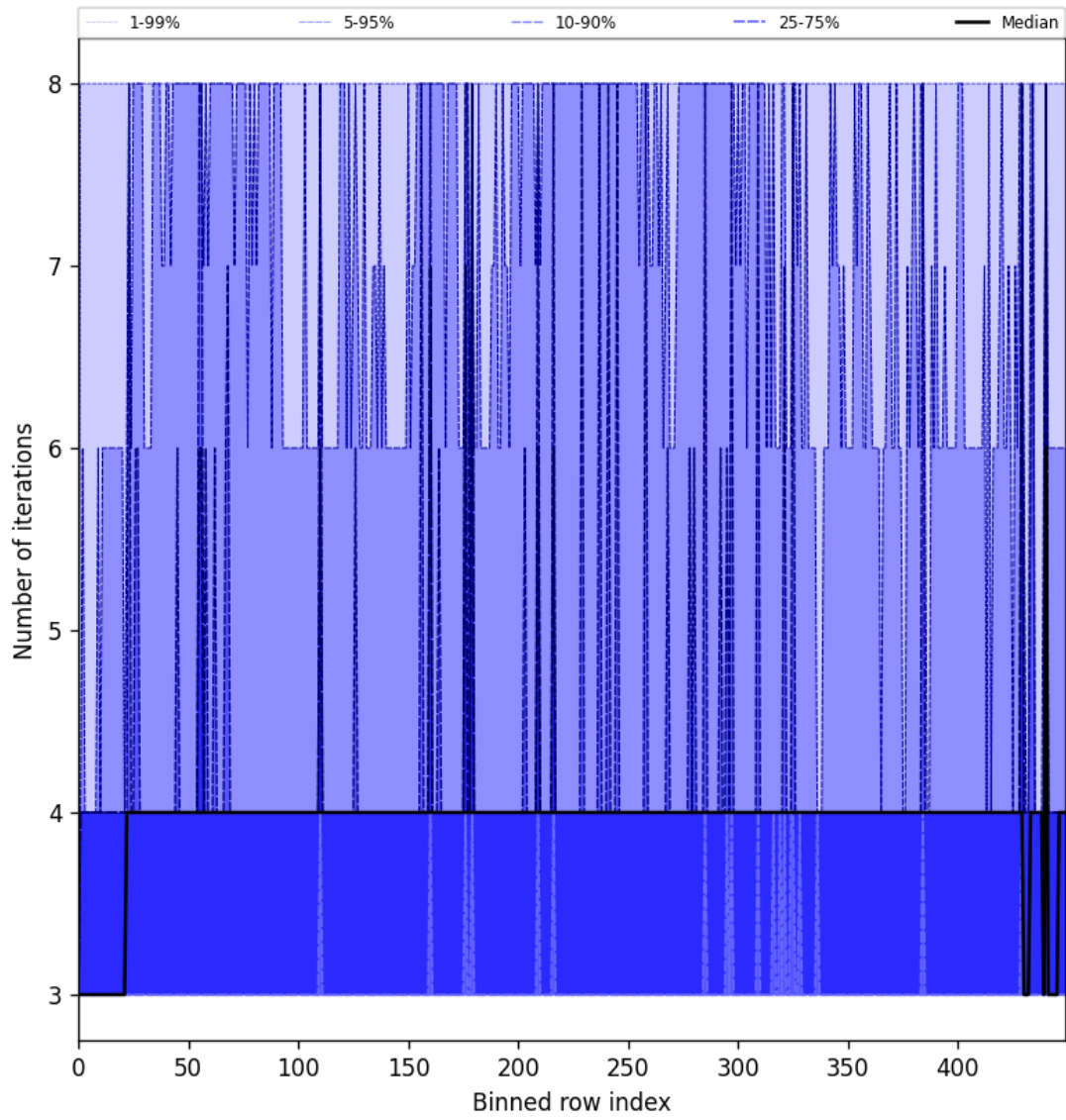
Figure 49: Along track statistics of “Number of iterations” for 2025-08-06 to 2025-08-07
