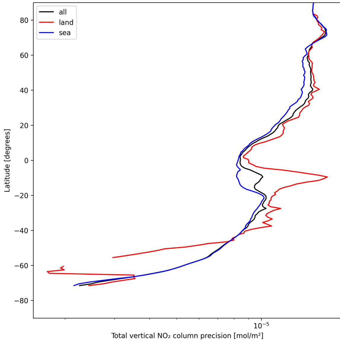
Figure 20: Zonal average of “Total vertical NO 2 column precision” for 2025-08-06 to 2025-08-07.
