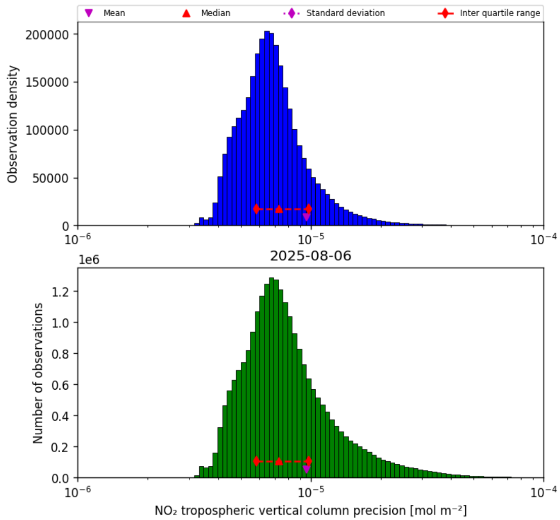
Figure 28: Histogram of “NO 2 tropospheric vertical column precision” for 2025-08-06 to 2025-08-07
