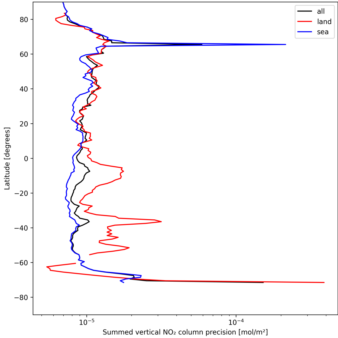
Figure 22: Zonal average of “Summed vertical NO 2 column precision” for 2025-08-06 to 2025-08-07.
