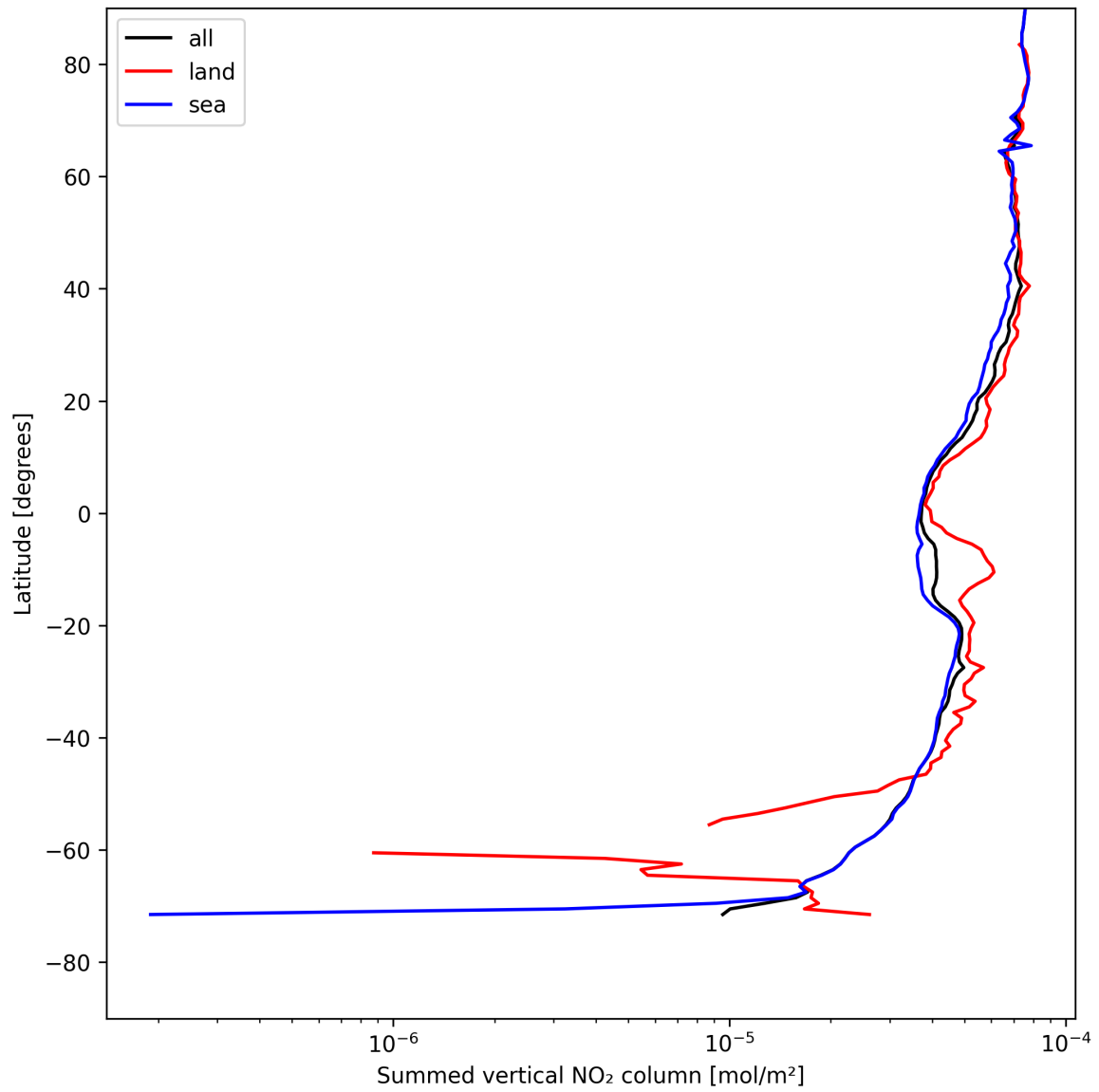
Figure 21: Zonal average of “Summed vertical NO 2 column” for 2025-08-06 to 2025-08-07.
