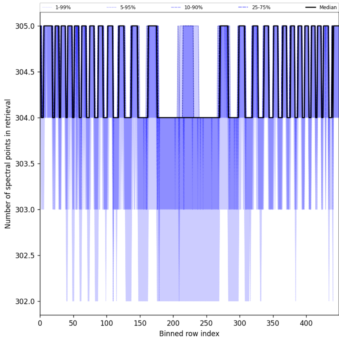
Figure 48: Along track statistics of “Number of spectral points in retrieval” for 2025-08-06 to 2025-08-07
