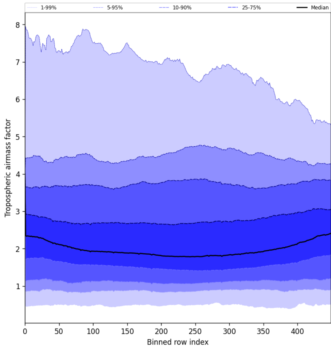
Figure 46: Along track statistics of “Tropospheric airmass factor” for 2025-08-06 to 2025-08-07
