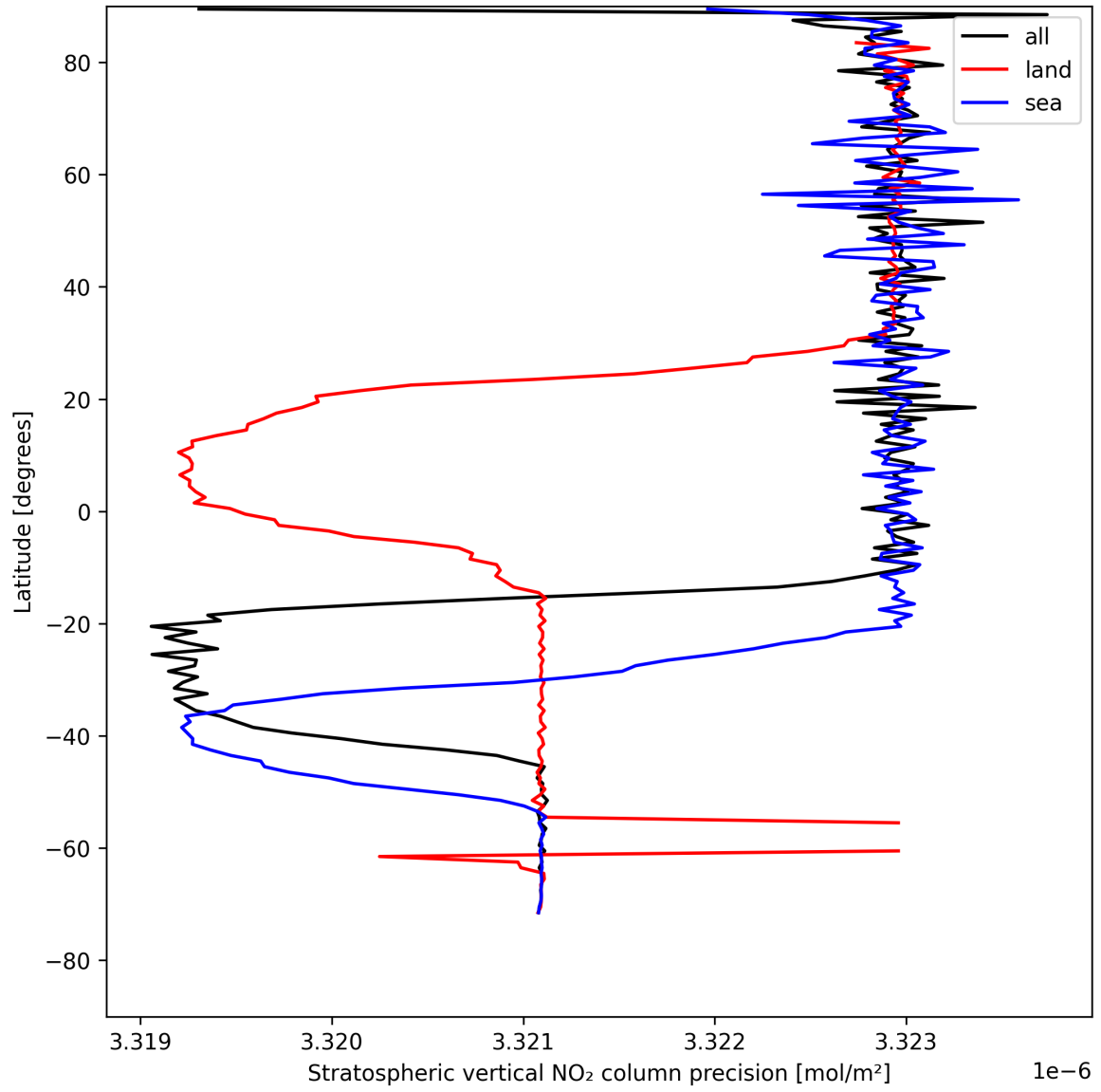
Figure 18: Zonal average of “Stratospheric vertical NO 2 column precision” for 2025-08-06 to 2025-08-07.
