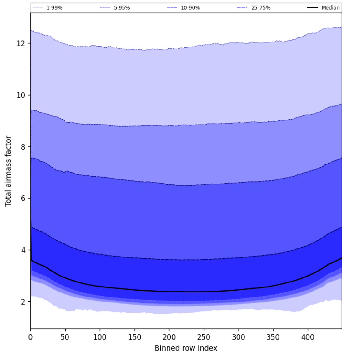
Figure 47: Along track statistics of “Total airmass factor” for 2025-08-06 to 2025-08-07
