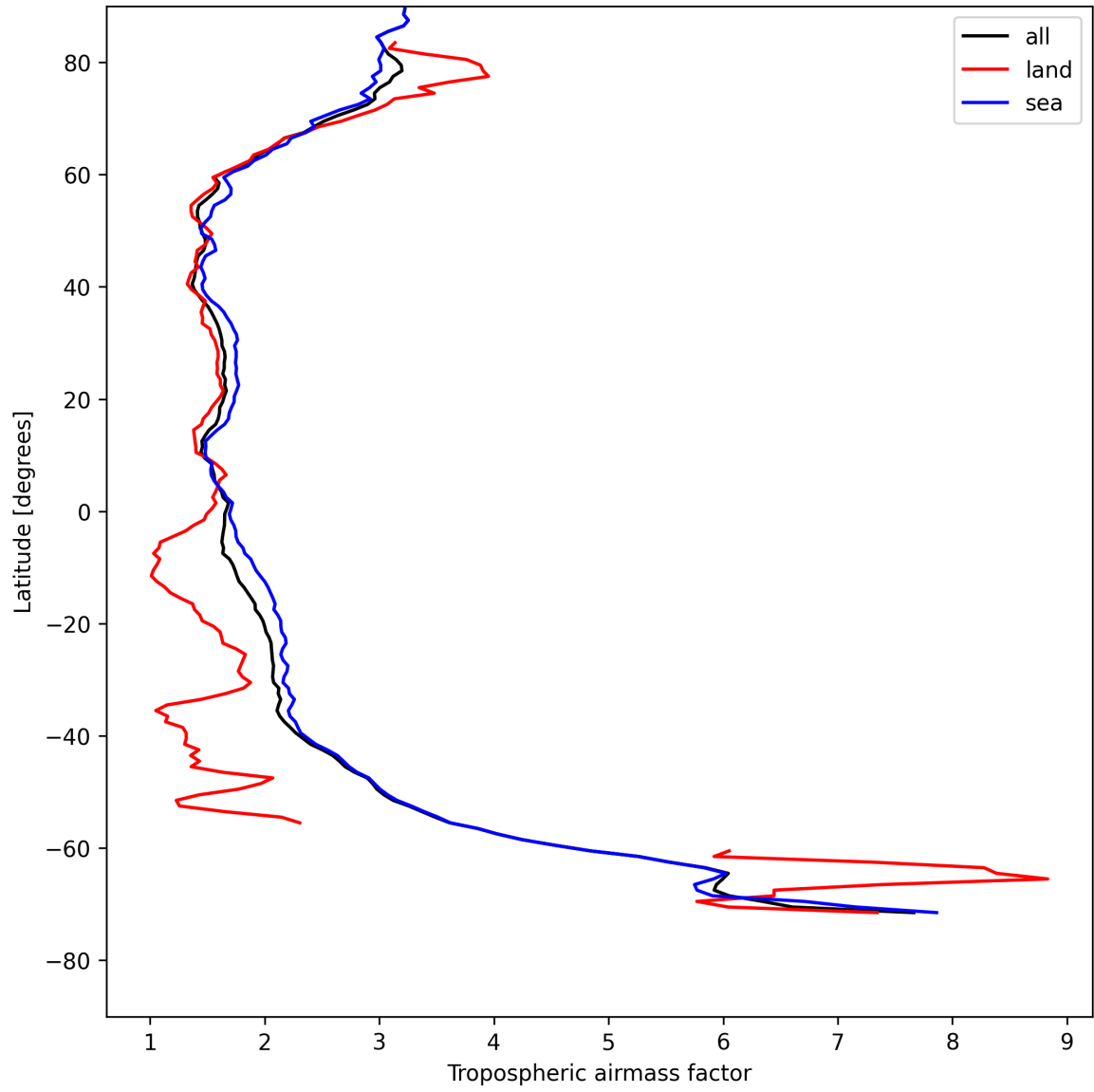
Figure 12: Zonal average of “Tropospheric airmass factor” for 2025-08-06 to 2025-08-07.
