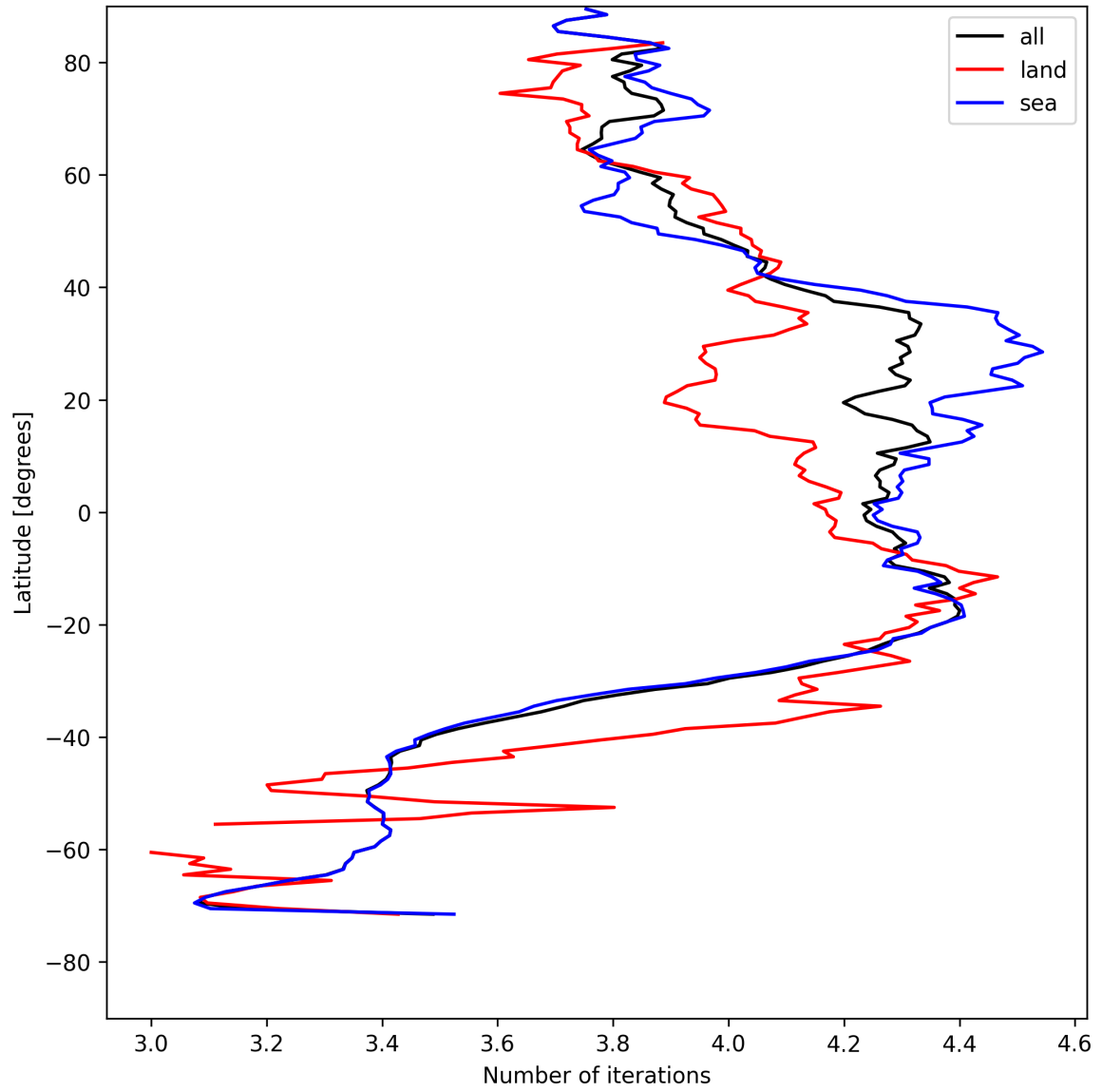
Figure 15: Zonal average of “Number of iterations” for 2025-08-06 to 2025-08-07.
