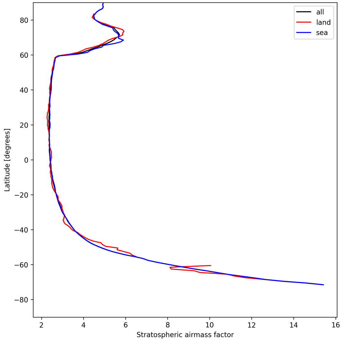
Figure 25: Zonal average of “Stratospheric airmass factor” for 2025-08-06 to 2025-08-07.
