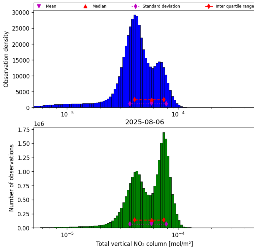
Figure 36: Histogram of “Total vertical NO 2 column” for 2025-08-06 to 2025-08-07
