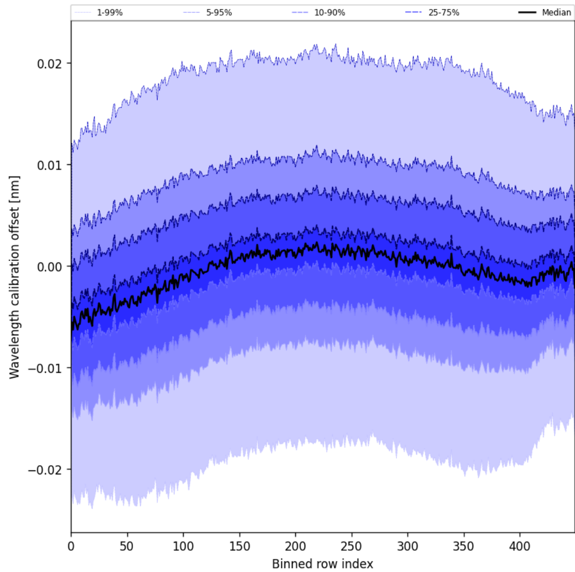
Figure 50: Along track statistics of “Wavelength calibration offset” for 2025-08-06 to 2025-08-07
