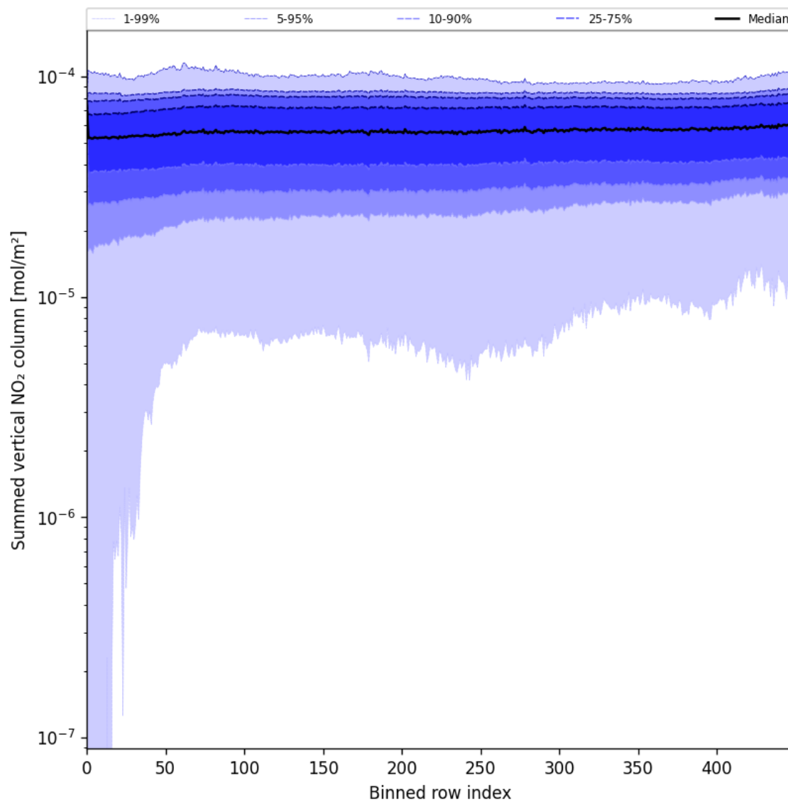
Figure 55: Along track statistics of “Summed vertical NO 2 column” for 2025-08-06 to 2025-08-07
