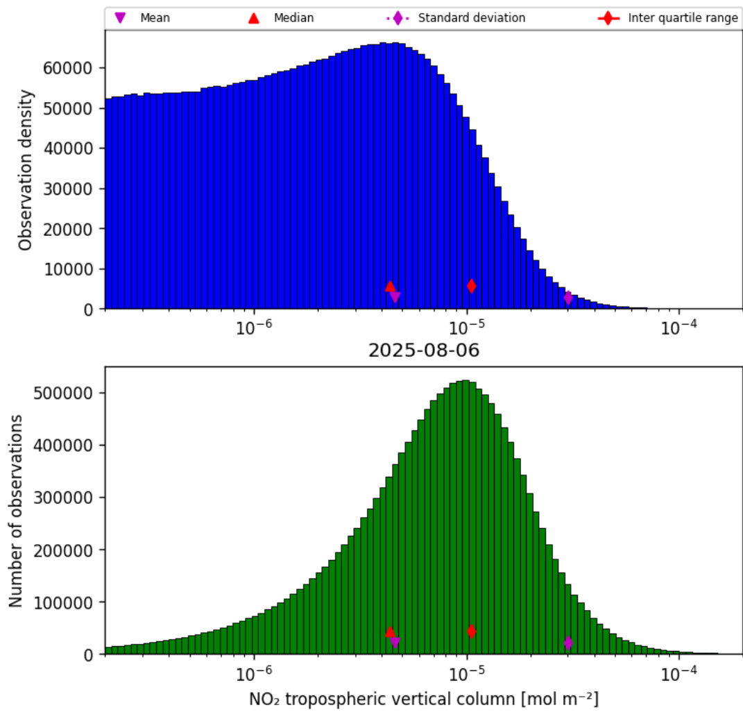
Figure 27: Histogram of “NO 2 tropospheric vertical column” for 2025-08-06 to 2025-08-07
