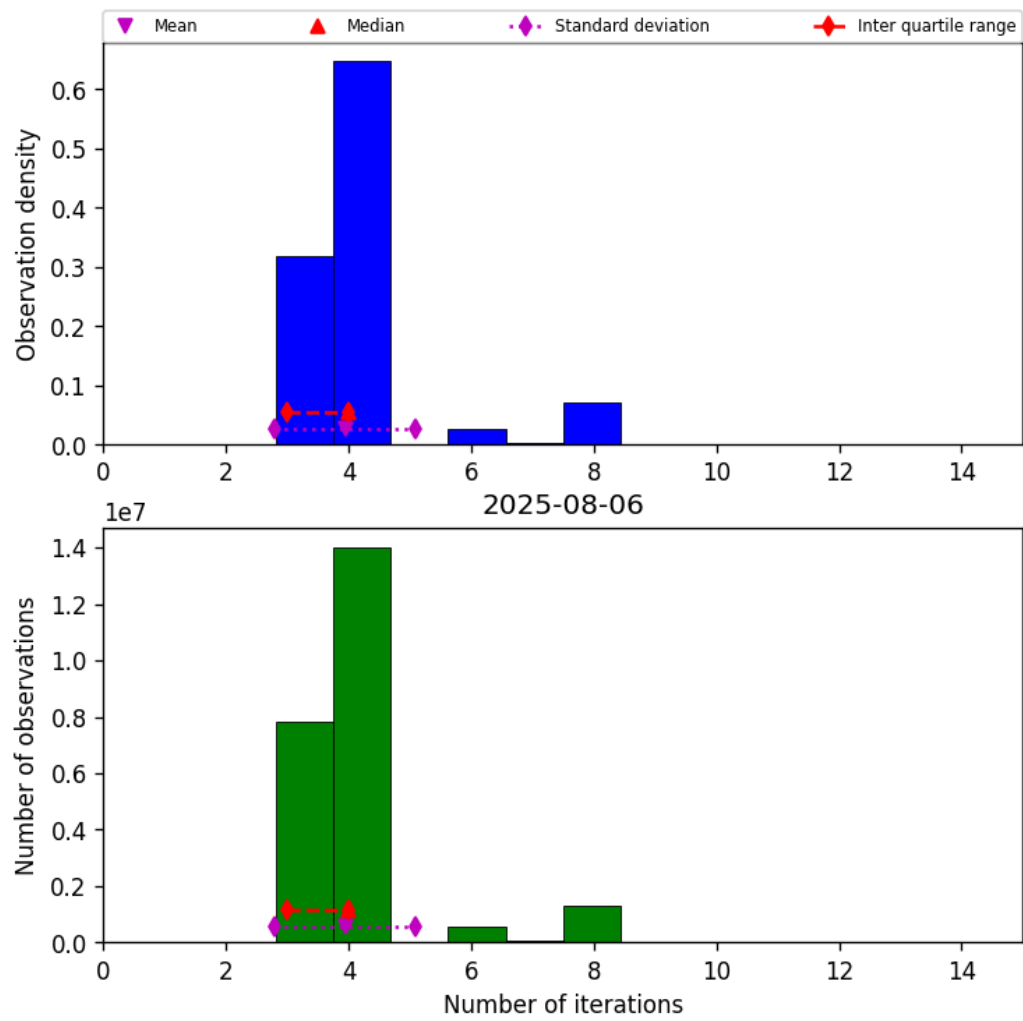
Figure 32: Histogram of “Number of iterations” for 2025-08-06 to 2025-08-07
