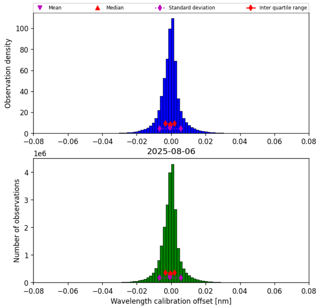
Figure 33: Histogram of “Wavelength calibration offset” for 2025-08-06 to 2025-08-07
