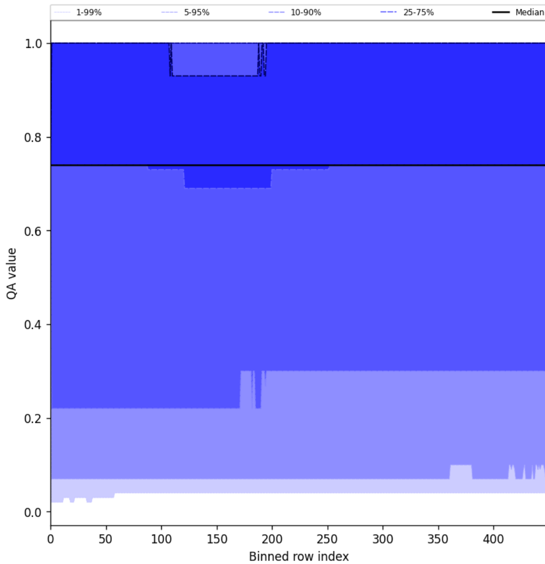
Figure 43: Along track statistics of “QA value” for 2025-08-06 to 2025-08-07
