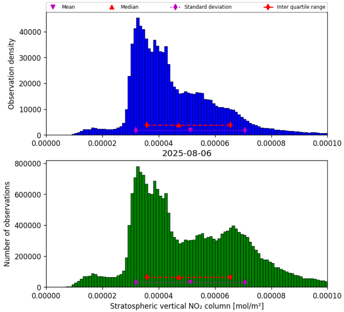
Figure 34: Histogram of “Stratospheric vertical NO 2 column” for 2025-08-06 to 2025-08-07
