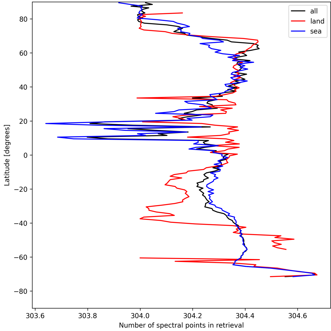
Figure 14: Zonal average of “Number of spectral points in retrieval” for 2025-08-06 to 2025-08-07.
