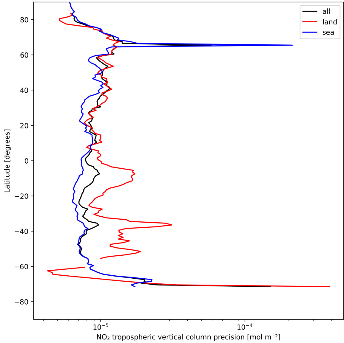
Figure 11: Zonal average of “NO 2 tropospheric vertical column precision” for 2025-08-06 to 2025-08-07.
