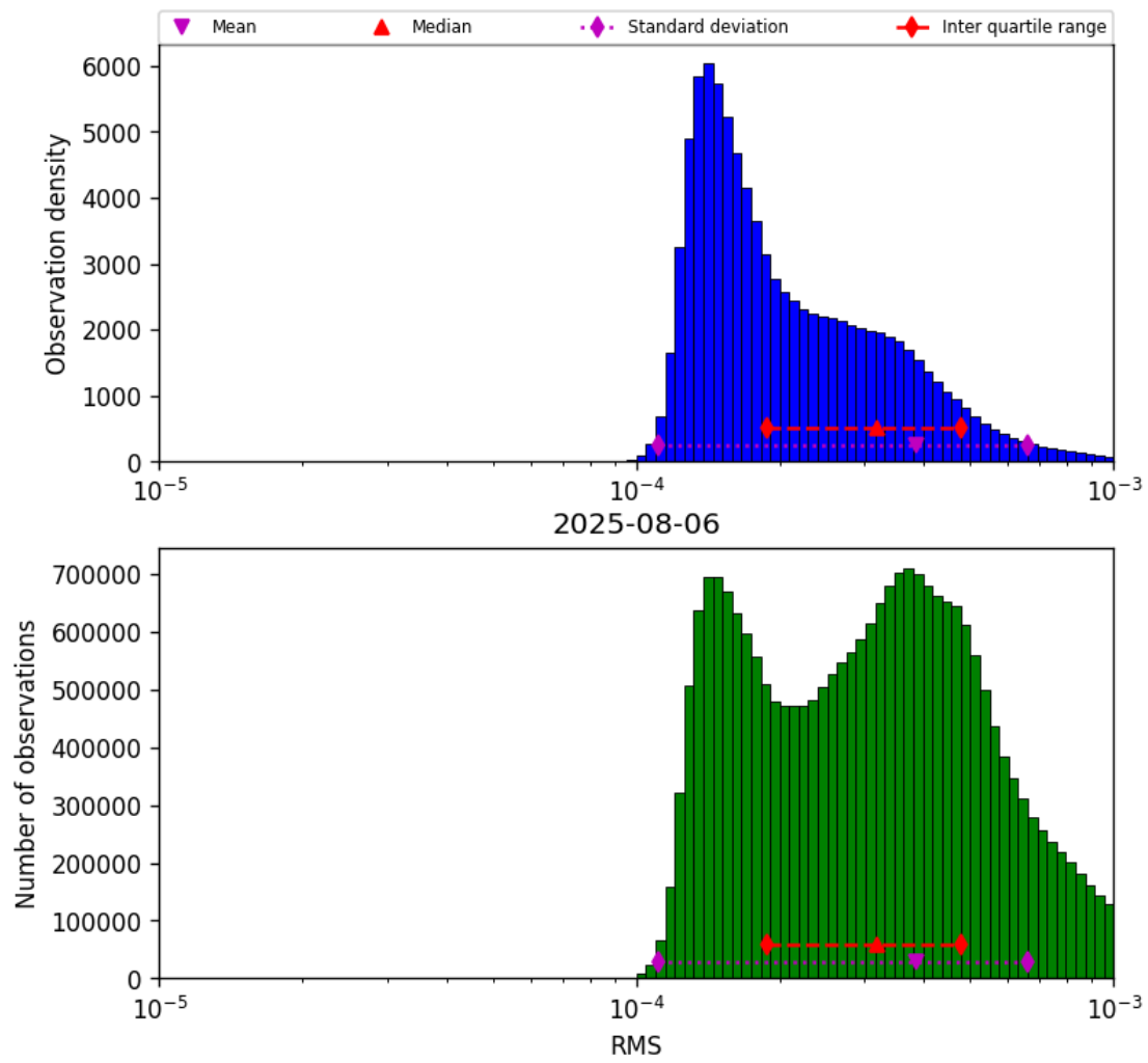
Figure 41: Histogram of “RMS” for 2025-08-06 to 2025-08-07
