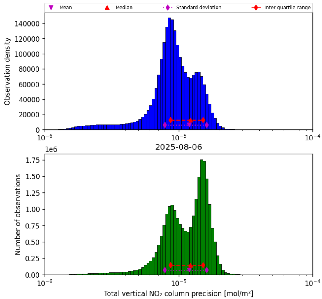
Figure 37: Histogram of “Total vertical NO 2 column precision” for 2025-08-06 to 2025-08-07
