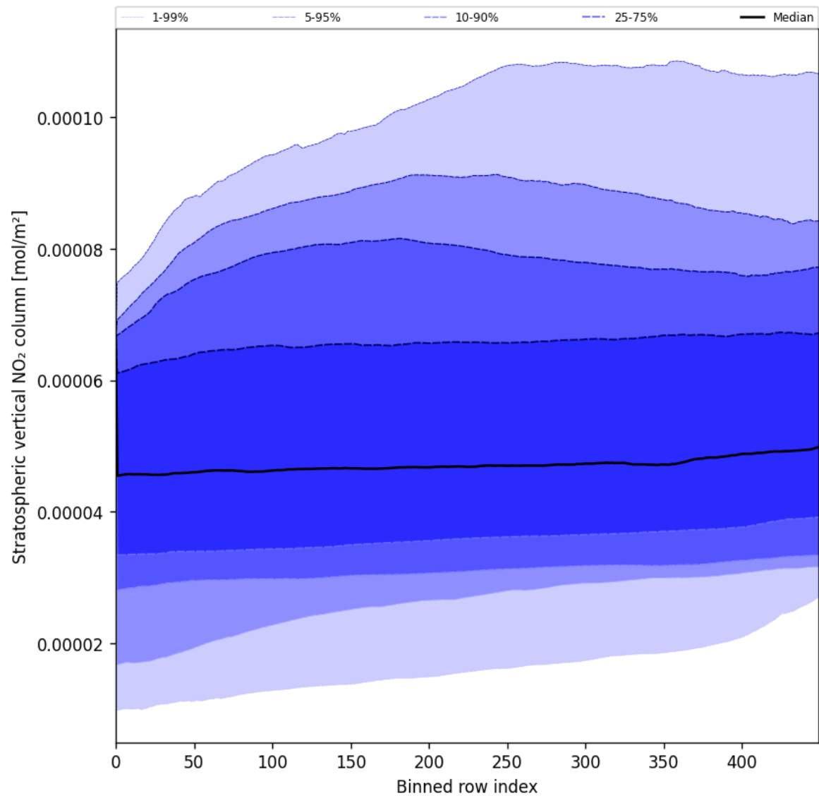
Figure 51: Along track statistics of “Stratospheric vertical NO 2 column” for 2025-08-06 to 2025-08-07
