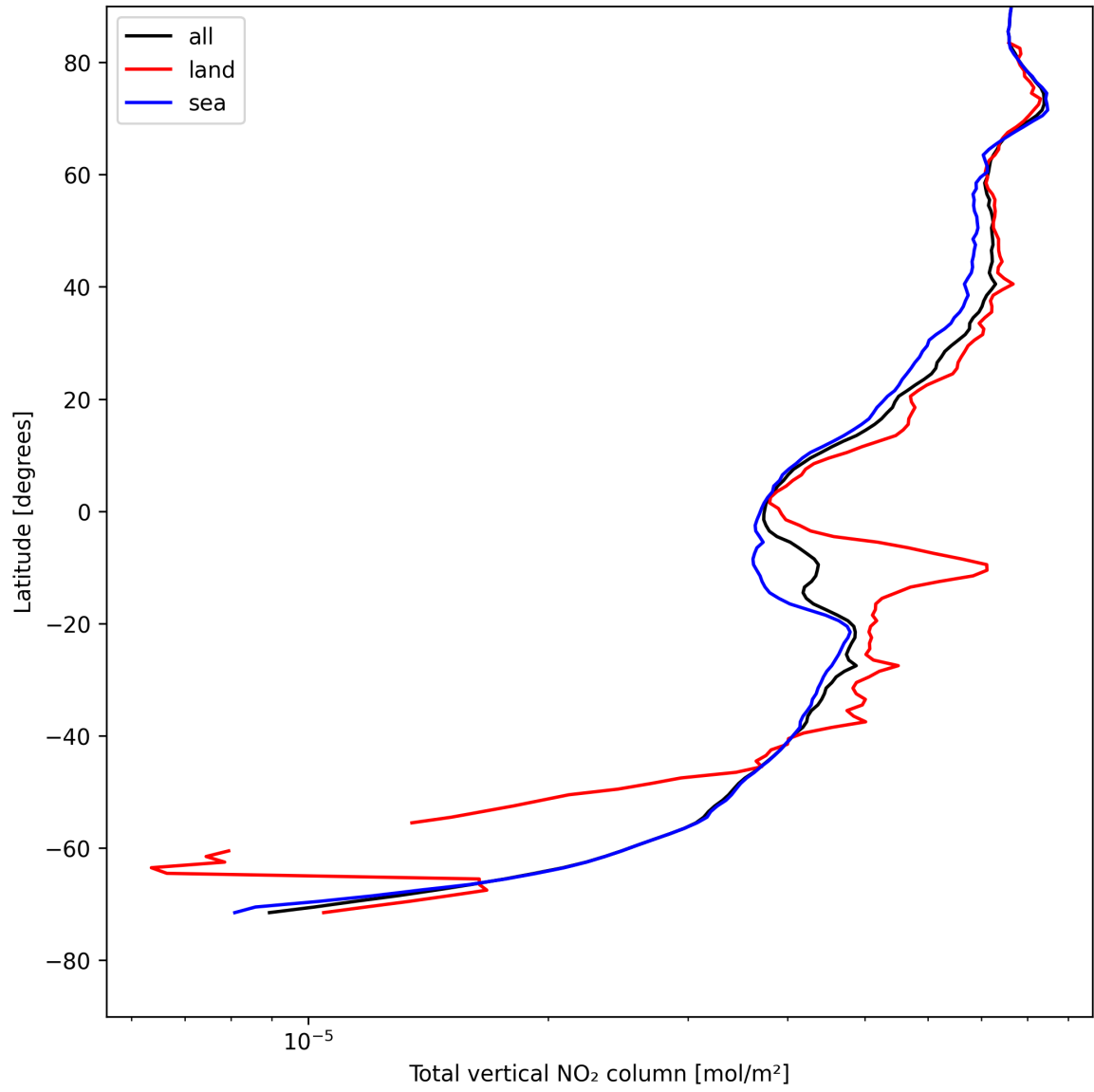
Figure 19: Zonal average of “Total vertical NO 2 column” for 2025-08-06 to 2025-08-07.
