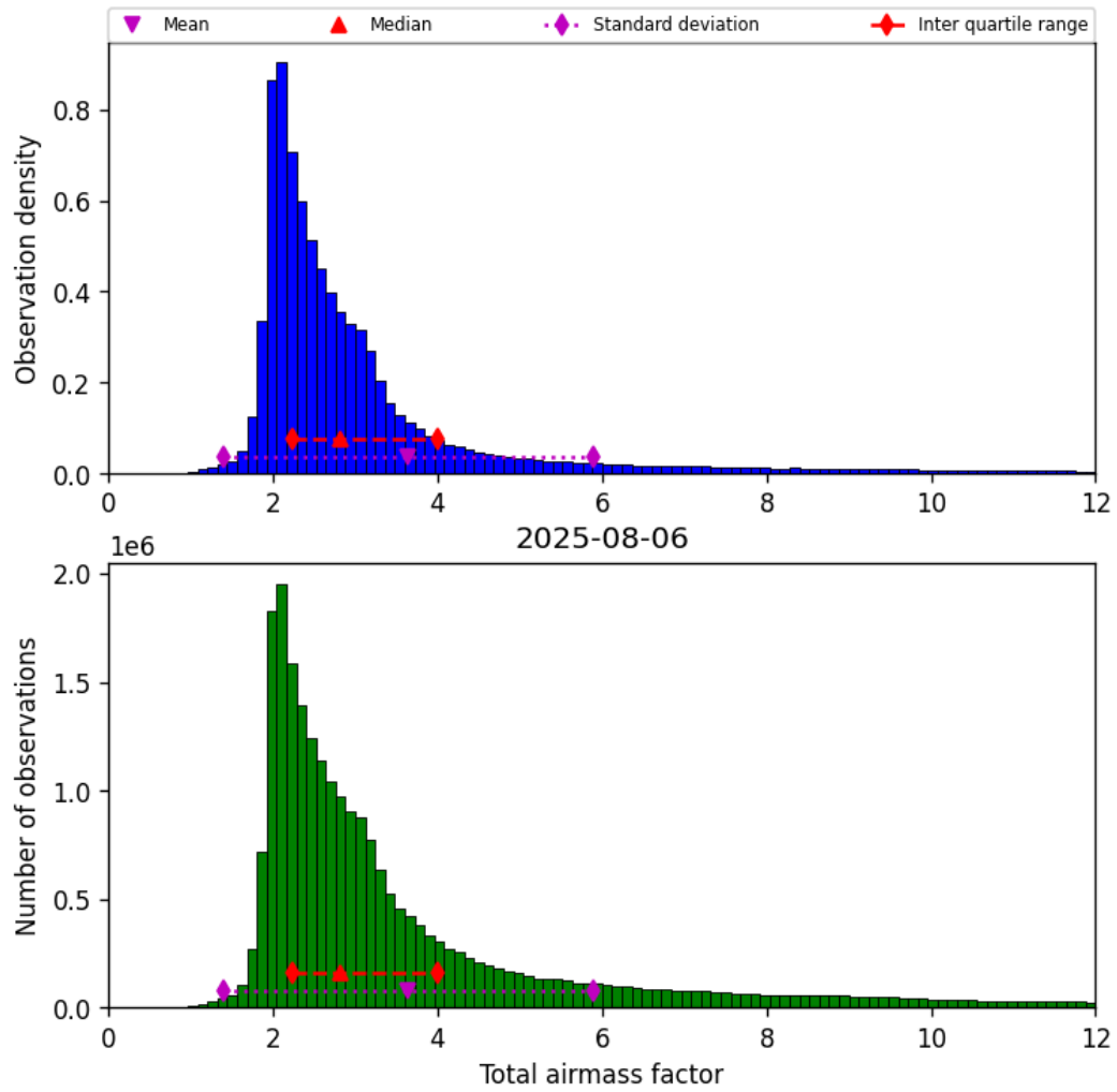
Figure 30: Histogram of “Total airmass factor” for 2025-08-06 to 2025-08-07
