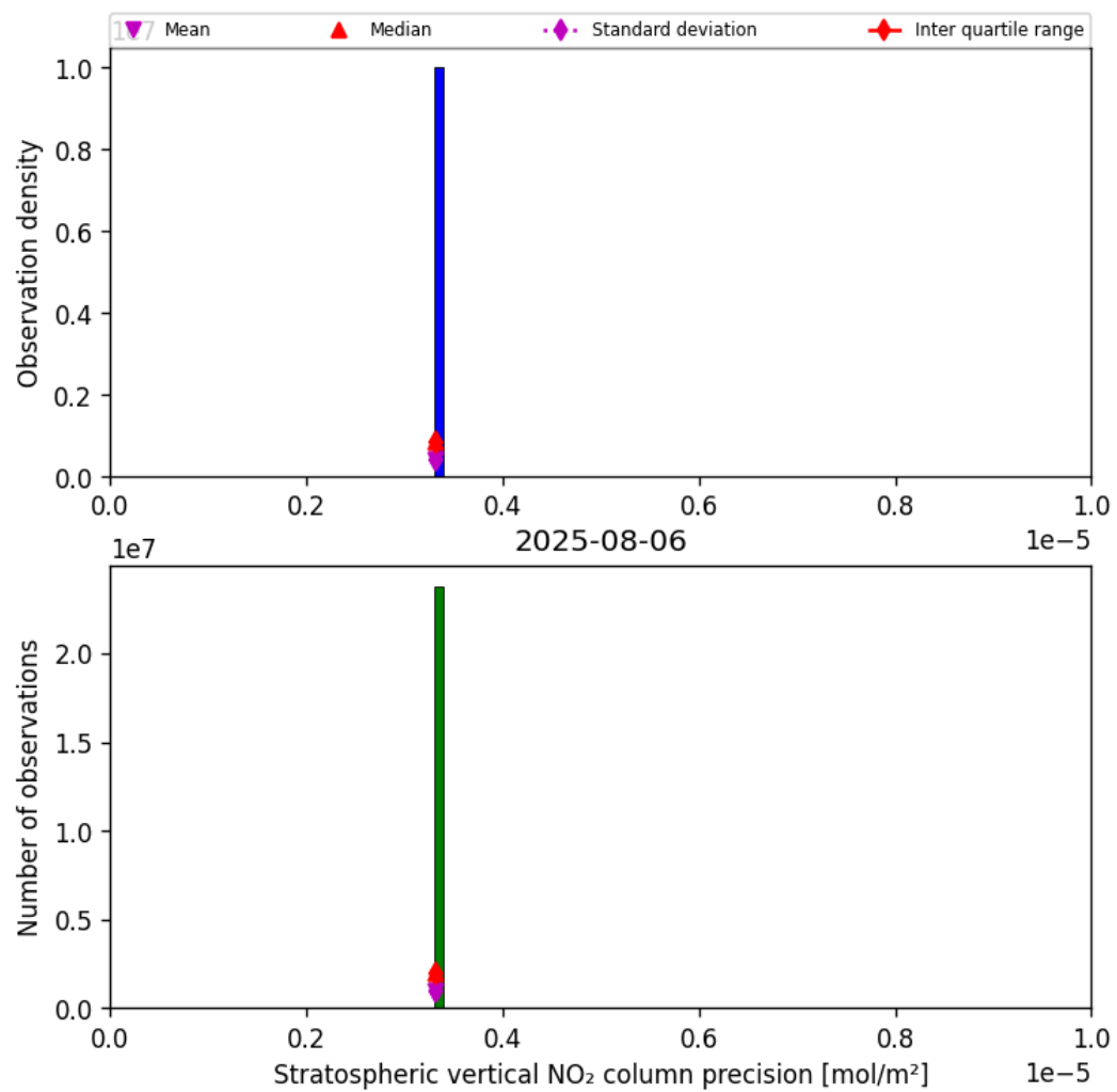
Figure 35: Histogram of “Stratospheric vertical NO 2 column precision” for 2025-08-06 to 2025-08-07
