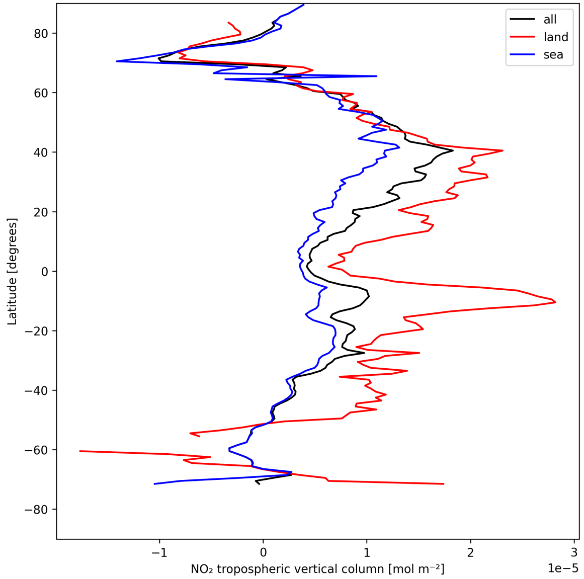
Figure 10: Zonal average of “NO 2 tropospheric vertical column” for 2025-08-06 to 2025-08-07.
