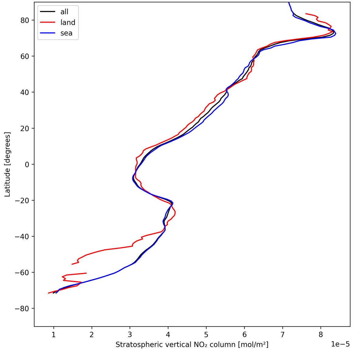
Figure 17: Zonal average of “Stratospheric vertical NO 2 column” for 2025-08-06 to 2025-08-07.
