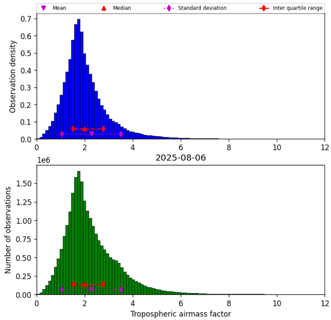
Figure 29: Histogram of “Tropospheric airmass factor” for 2025-08-06 to 2025-08-07
