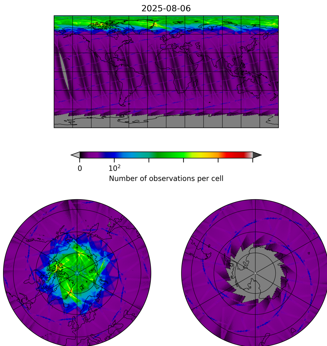
Figure 8: Map of the number of observations for 2025-08-06 to 2025-08-07
