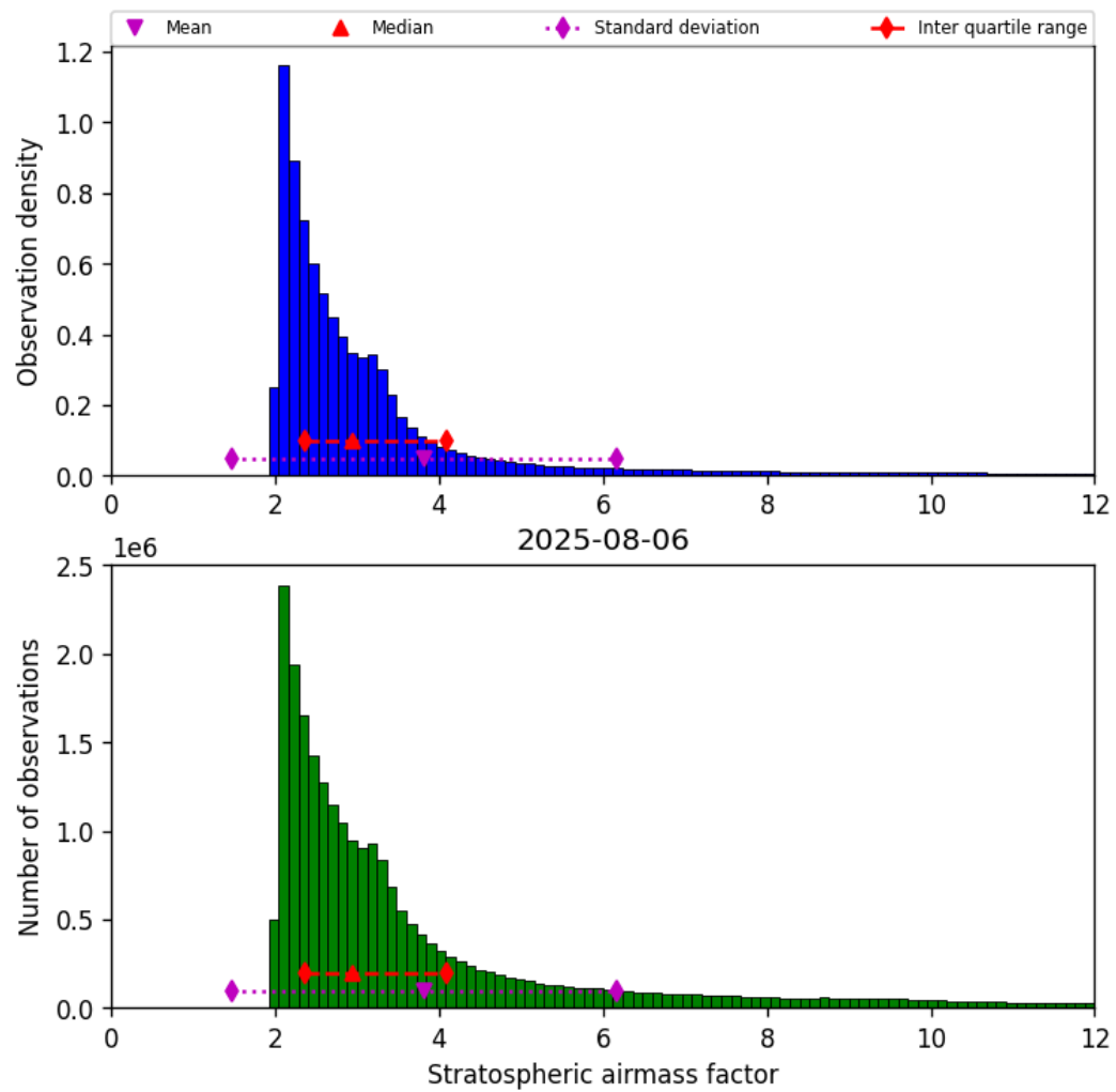
Figure 42: Histogram of “Stratospheric airmass factor” for 2025-08-06 to 2025-08-07
