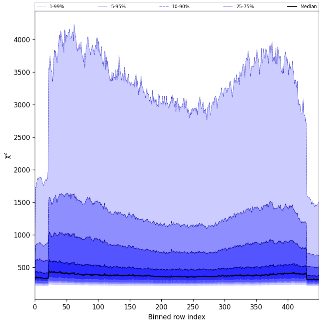
Figure 57: Along track statistics of “ \chi^2 ” for 2025-08-06 to 2025-08-07
