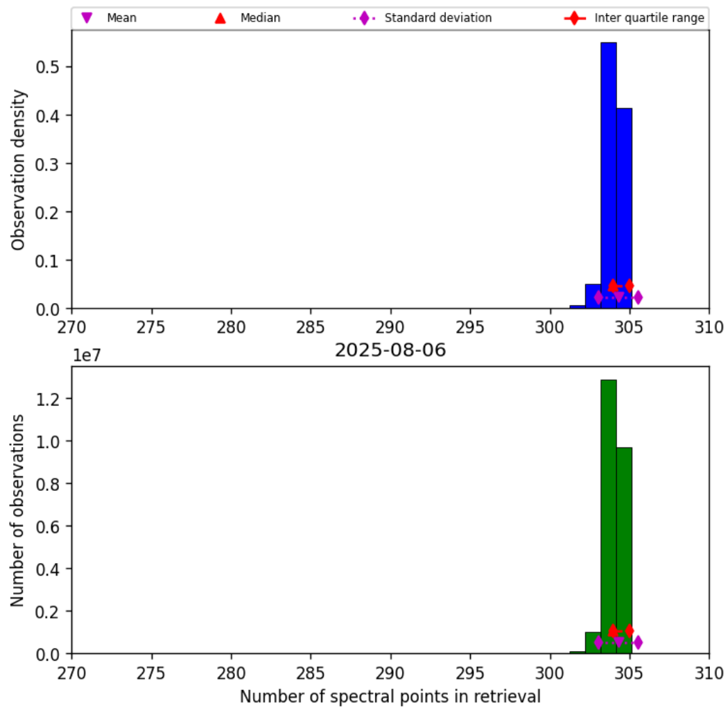
Figure 31: Histogram of “Number of spectral points in retrieval” for 2025-08-06 to 2025-08-07
