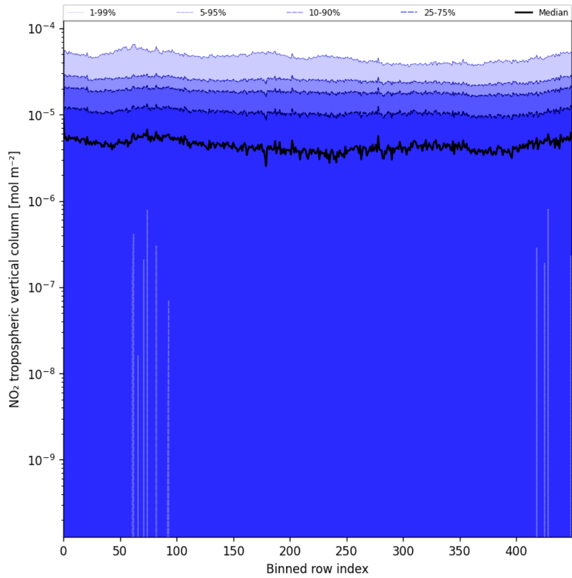
Figure 44: Along track statistics of “NO 2 tropospheric vertical column” for 2025-08-06 to 2025-08-07
