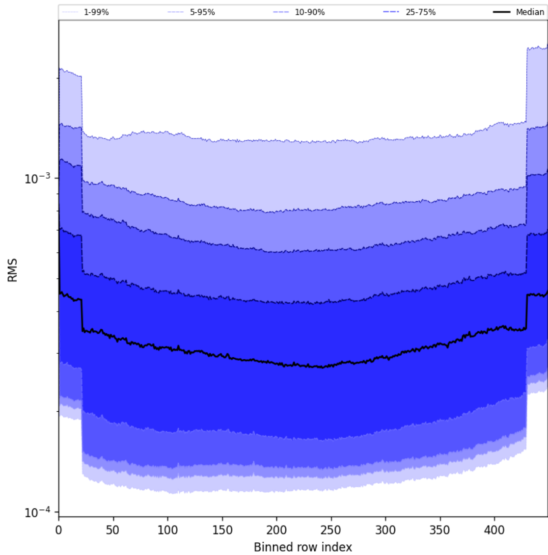
Figure 58: Along track statistics of “RMS” for 2025-08-06 to 2025-08-07
