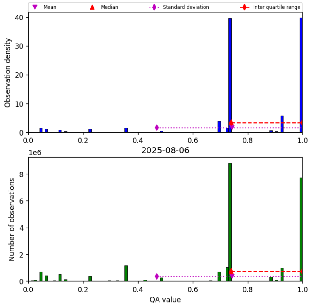
Figure 26: Histogram of “QA value” for 2025-08-06 to 2025-08-07
