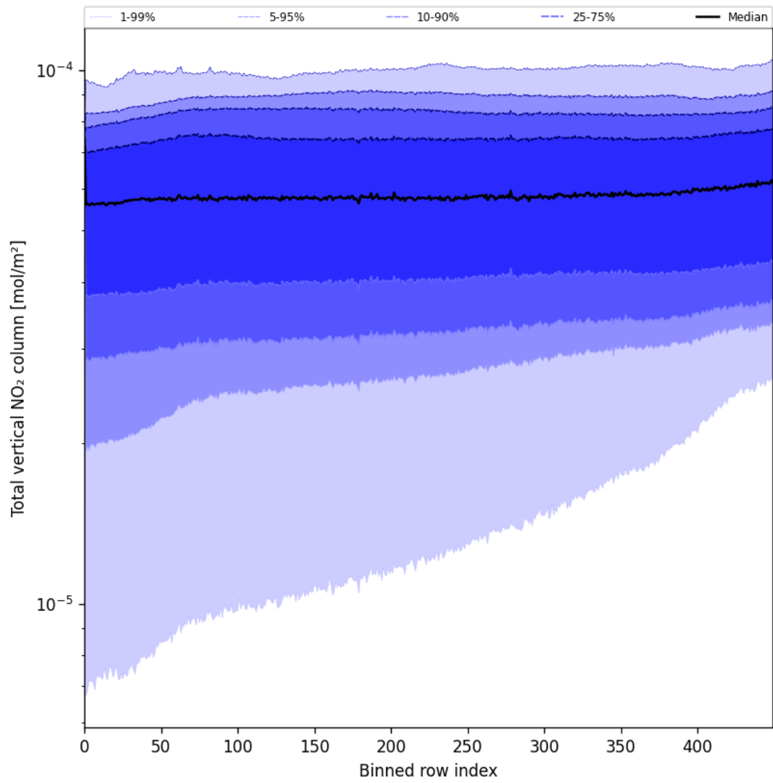
Figure 53: Along track statistics of “Total vertical NO 2 column” for 2025-08-06 to 2025-08-07
