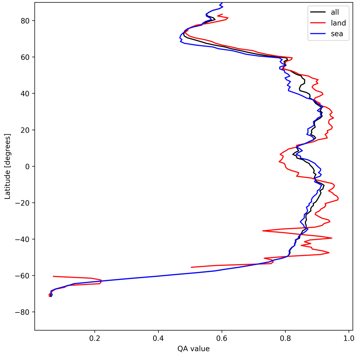
Figure 9: Zonal average of “QA value” for 2025-08-06 to 2025-08-07.
