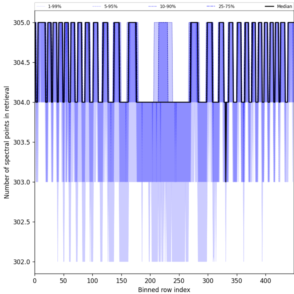
Figure 48: Along track statistics of “Number of spectral points in retrieval” for 2025-08-07 to 2025-08-07
