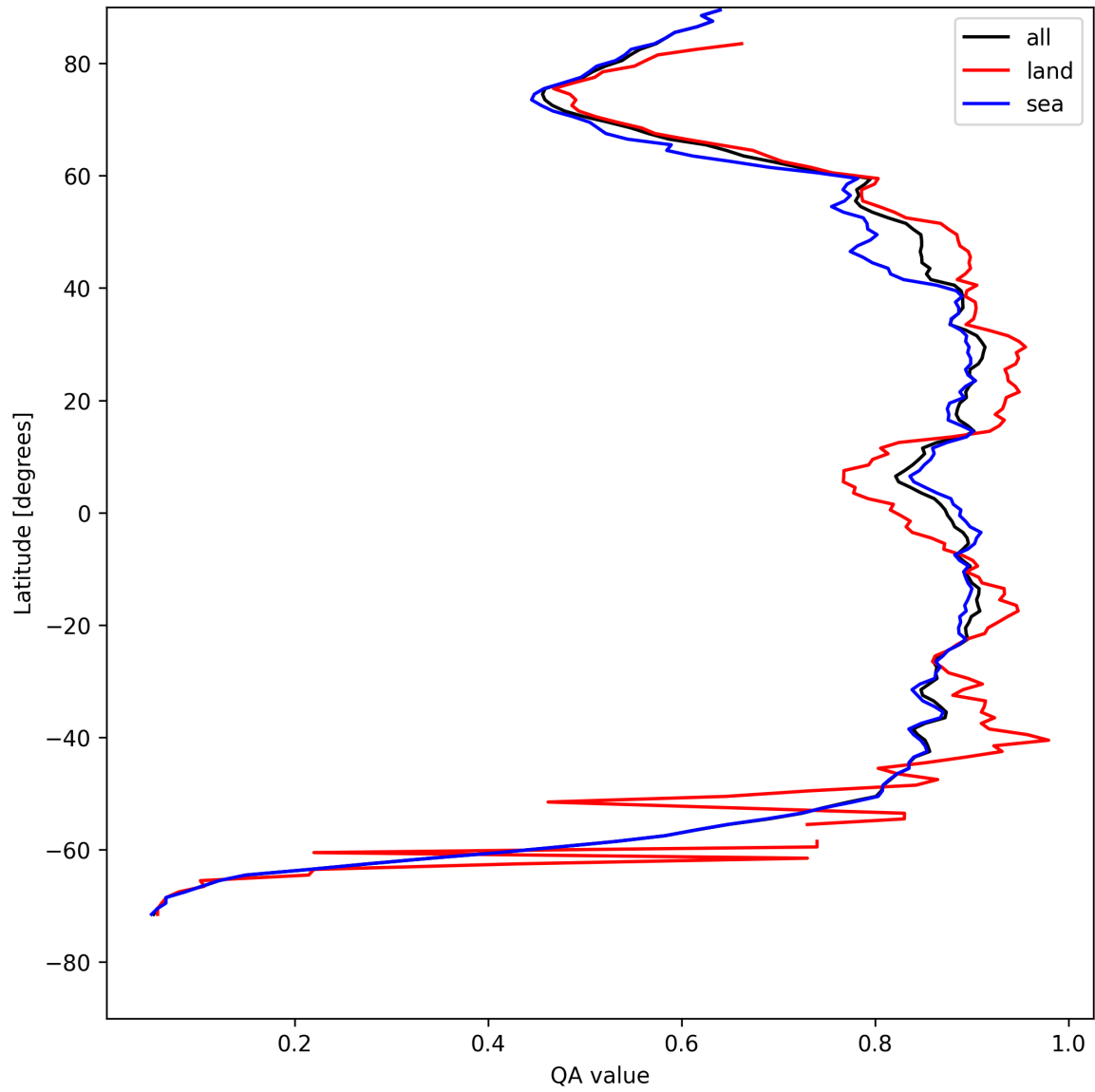
Figure 9: Zonal average of “QA value” for 2025-08-07 to 2025-08-07.
