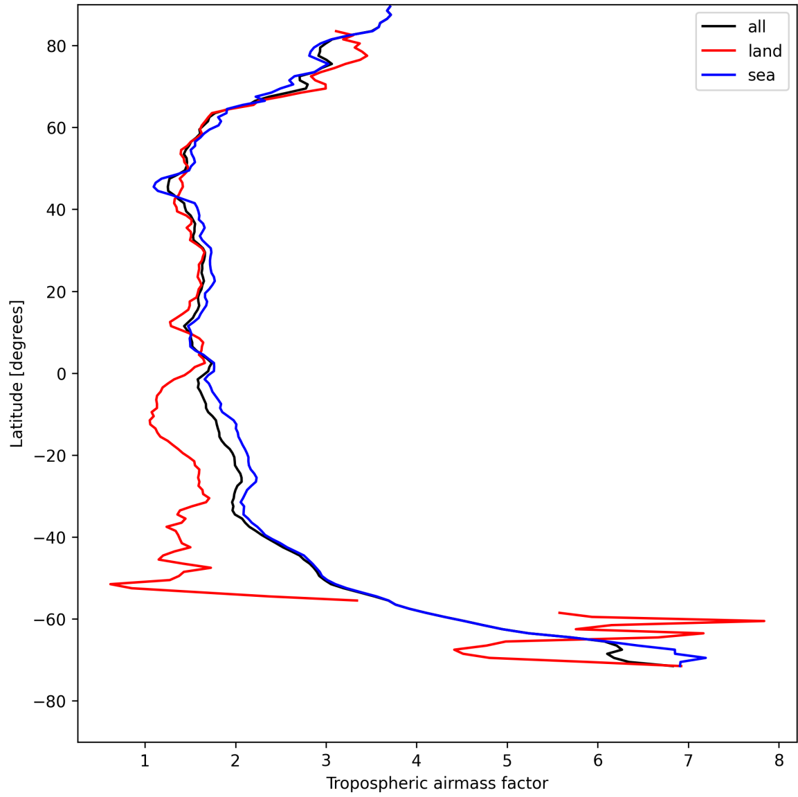
Figure 12: Zonal average of “Tropospheric airmass factor” for 2025-08-07 to 2025-08-07.
