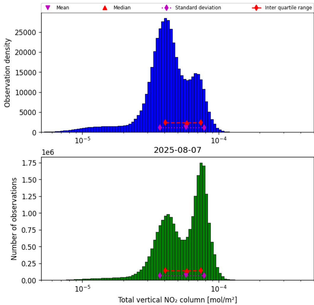
Figure 36: Histogram of “Total vertical NO 2 column” for 2025-08-07 to 2025-08-07
