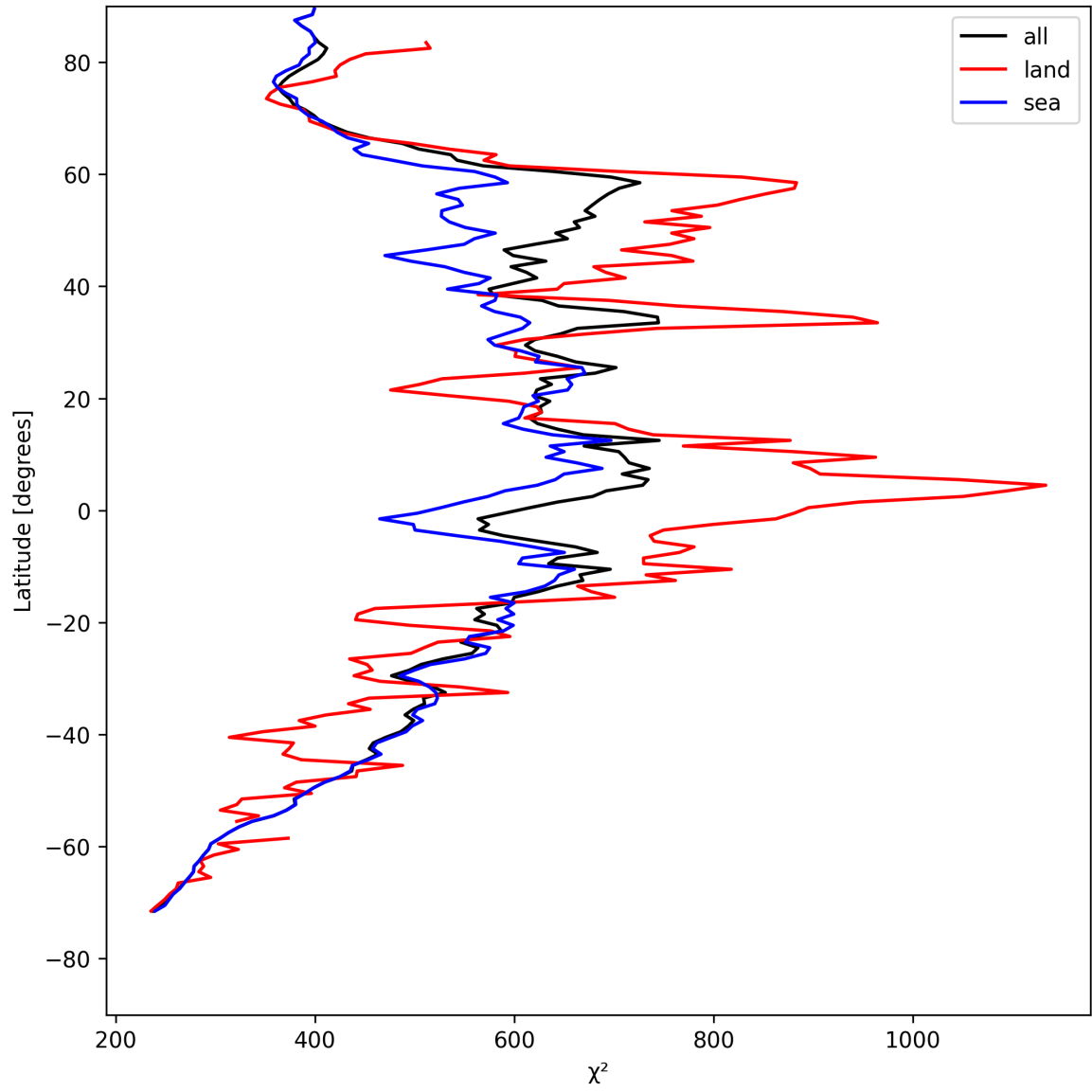
Figure 23: Zonal average of “ \chi^2 ” for 2025-08-07 to 2025-08-07.
