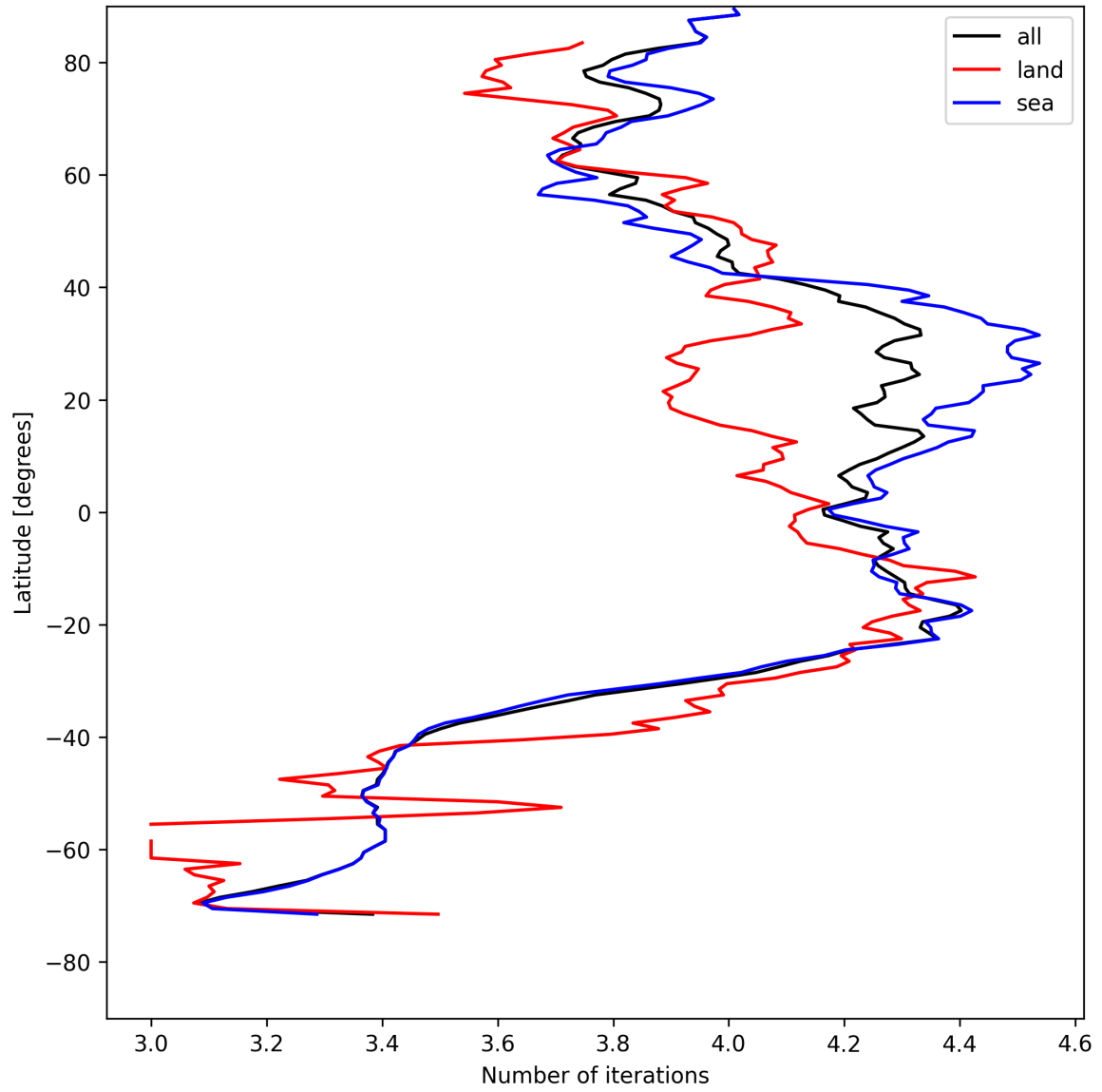
Figure 15: Zonal average of “Number of iterations” for 2025-08-07 to 2025-08-07.
