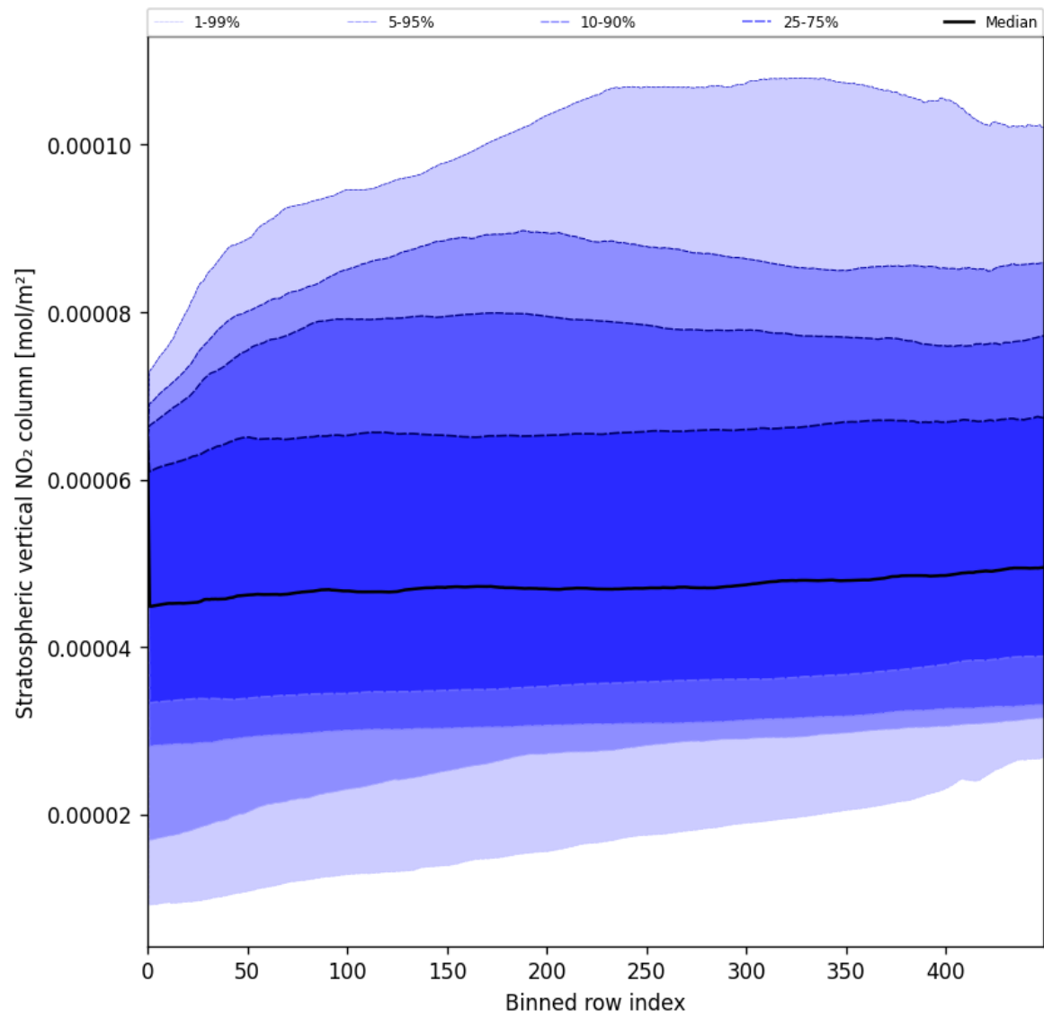
Figure 51: Along track statistics of “Stratospheric vertical NO 2 column” for 2025-08-07 to 2025-08-07
