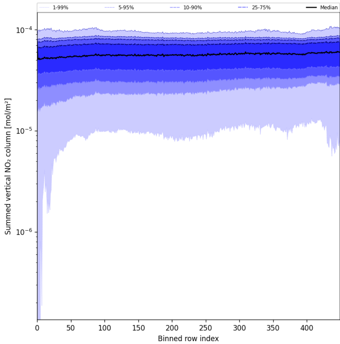
Figure 55: Along track statistics of “Summed vertical NO 2 column” for 2025-08-07 to 2025-08-07
