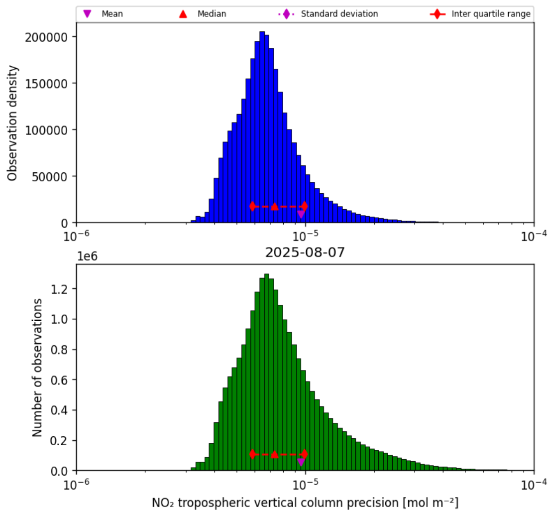
Figure 28: Histogram of “NO 2 tropospheric vertical column precision” for 2025-08-07 to 2025-08-07
