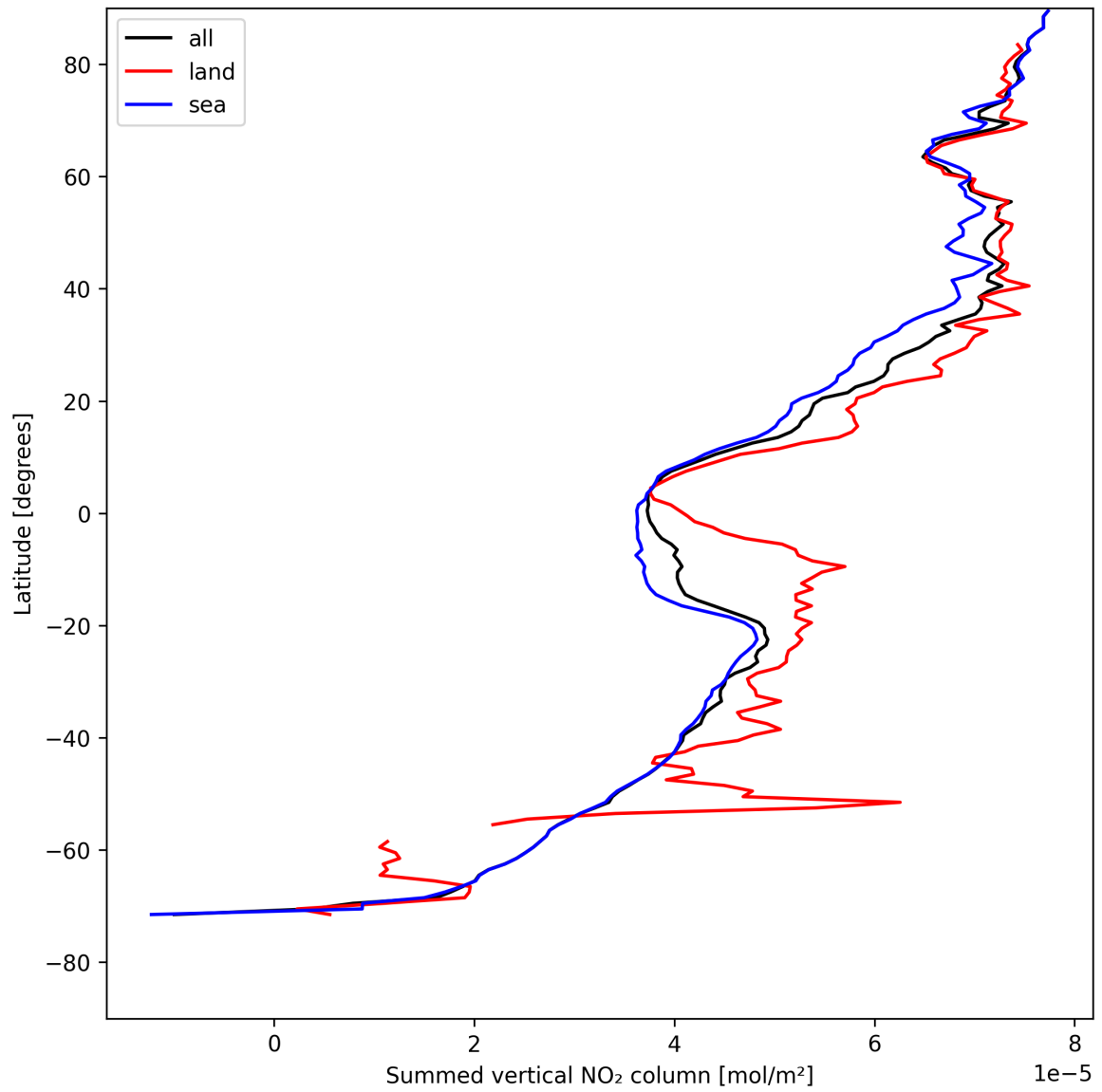
Figure 21: Zonal average of “Summed vertical NO 2 column” for 2025-08-07 to 2025-08-07.
