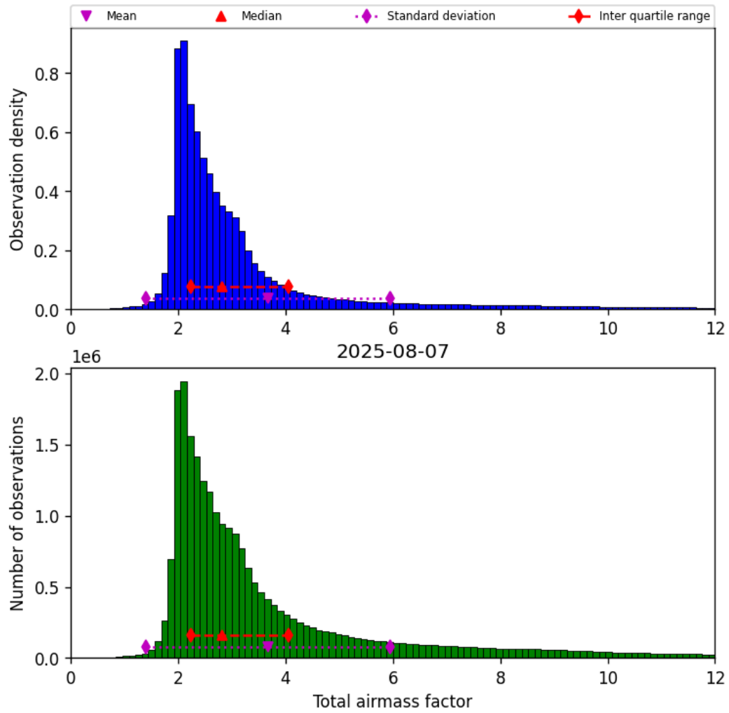
Figure 30: Histogram of “Total airmass factor” for 2025-08-07 to 2025-08-07
