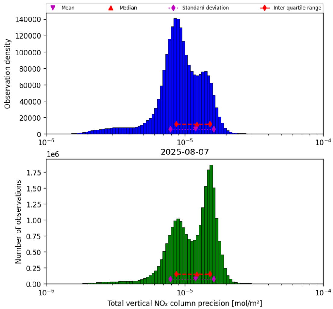
Figure 37: Histogram of “Total vertical NO 2 column precision” for 2025-08-07 to 2025-08-07
