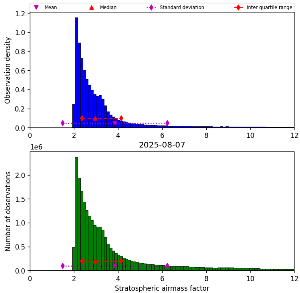
Figure 42: Histogram of “Stratospheric airmass factor” for 2025-08-07 to 2025-08-07
