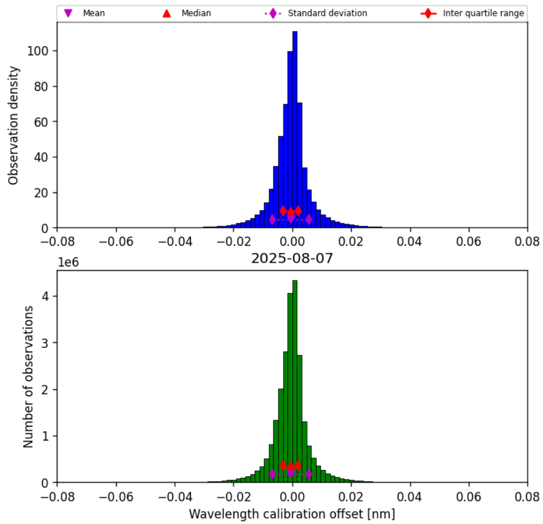
Figure 33: Histogram of “Wavelength calibration offset” for 2025-08-07 to 2025-08-07
