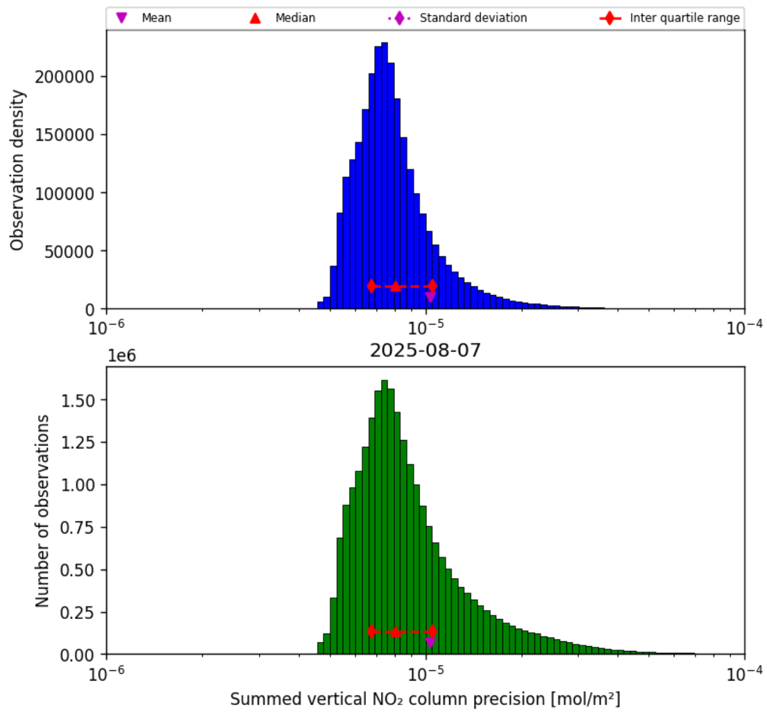
Figure 39: Histogram of "Summed vertical NO 2 column precision" for 2025-08-07 to 2025-08-07
