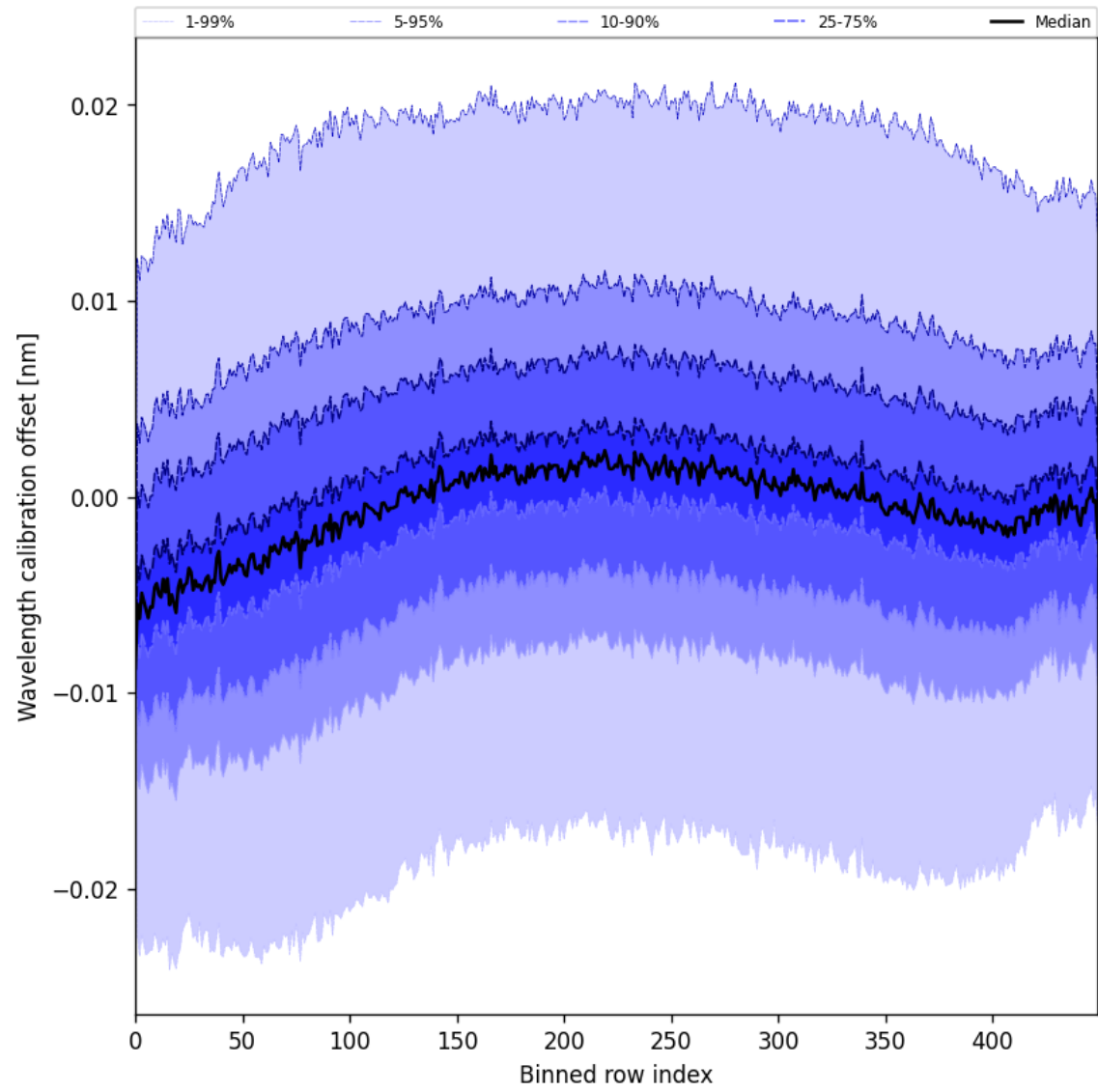
Figure 50: Along track statistics of “Wavelength calibration offset” for 2025-08-07 to 2025-08-07
