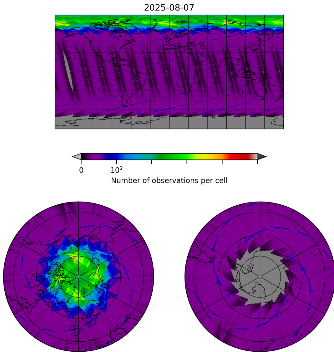
Figure 8: Map of the number of observations for 2025-08-07 to 2025-08-07
