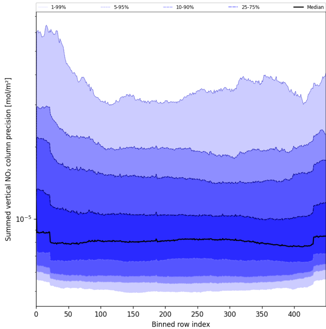
Figure 56: Along track statistics of “Summed vertical NO 2 column precision” for 2025-08-07 to 2025-08-07
