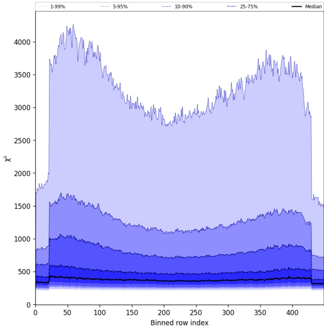
Figure 57: Along track statistics of “ \chi^2 ” for 2025-08-07 to 2025-08-07
