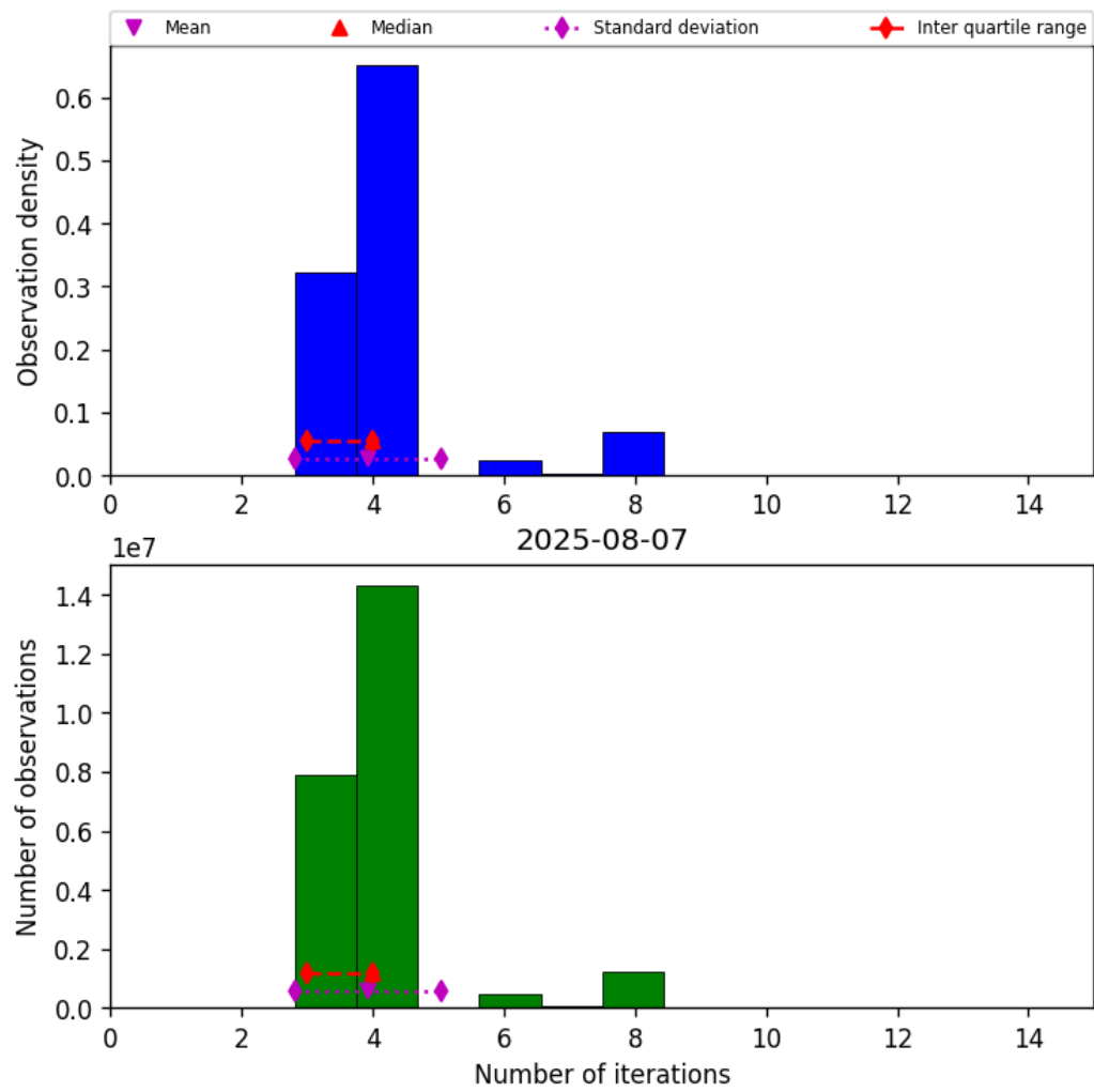
Figure 32: Histogram of “Number of iterations” for 2025-08-07 to 2025-08-07
