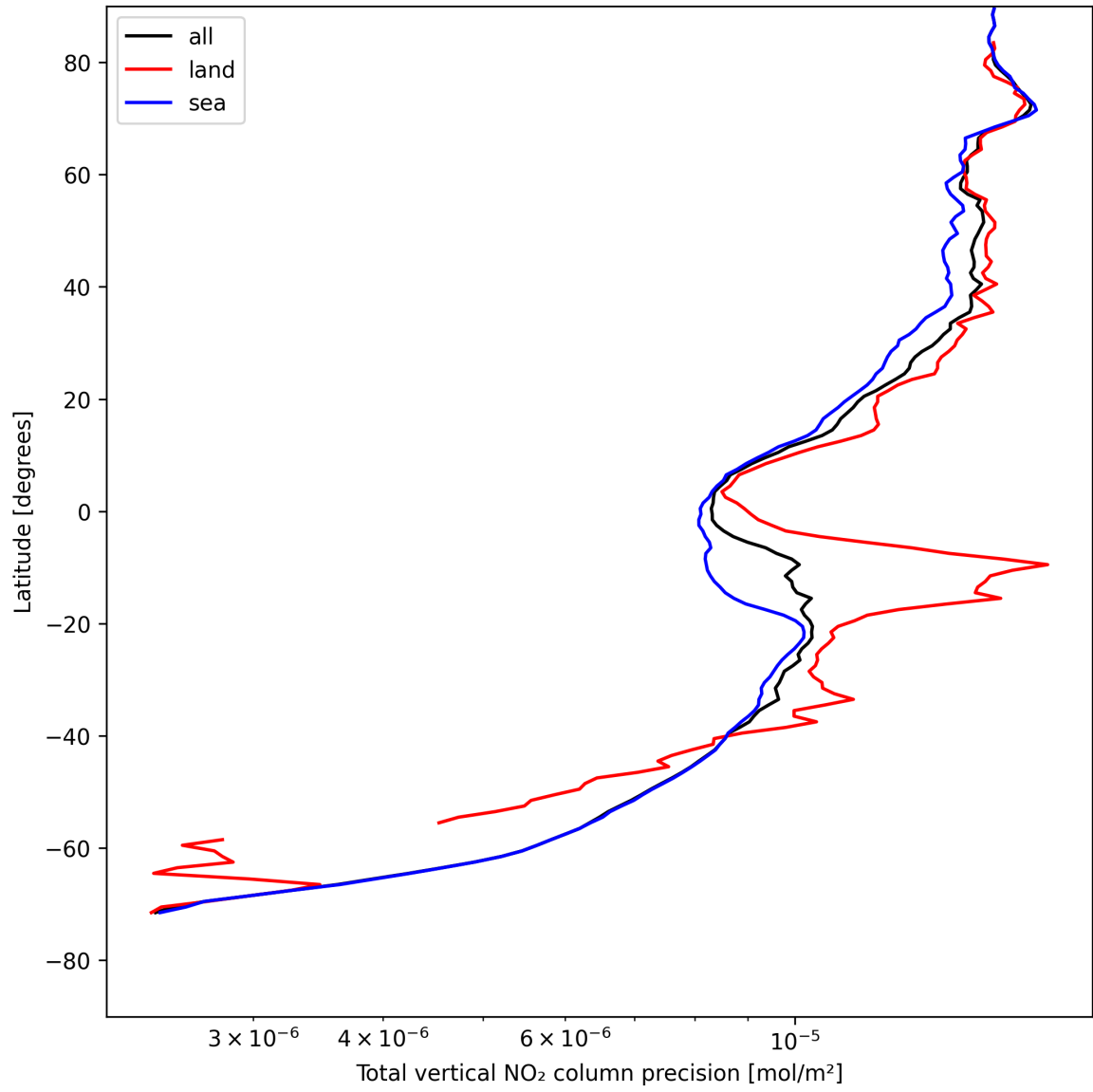
Figure 20: Zonal average of “Total vertical NO 2 column precision” for 2025-08-07 to 2025-08-07.
