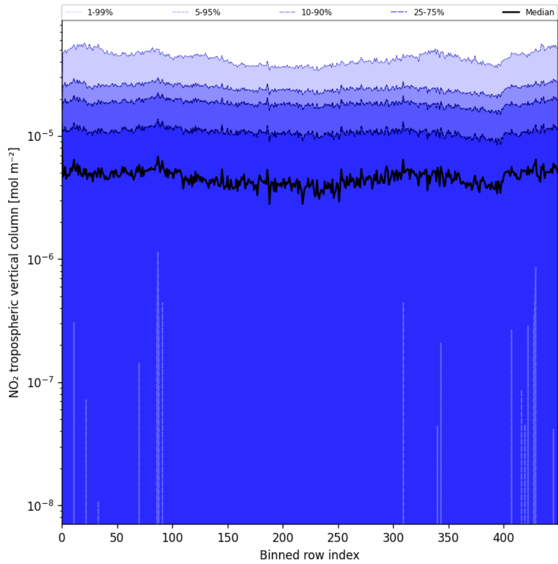
Figure 44: Along track statistics of “NO 2 tropospheric vertical column” for 2025-08-07 to 2025-08-07
