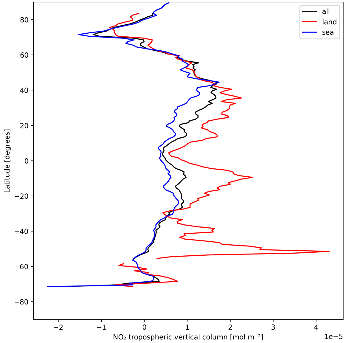
Figure 10: Zonal average of “NO 2 tropospheric vertical column” for 2025-08-07 to 2025-08-07.
