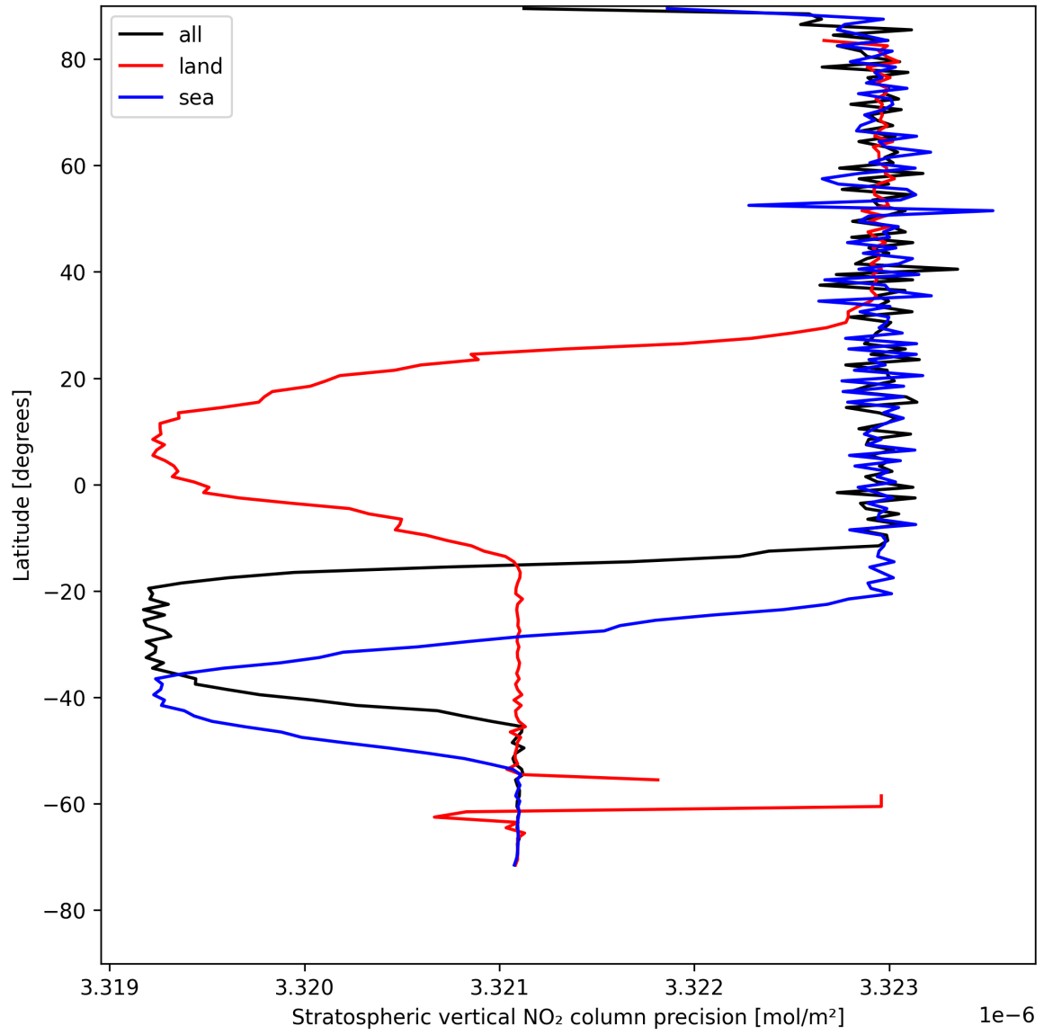
Figure 18: Zonal average of “Stratospheric vertical NO 2 column precision” for 2025-08-07 to 2025-08-07.
