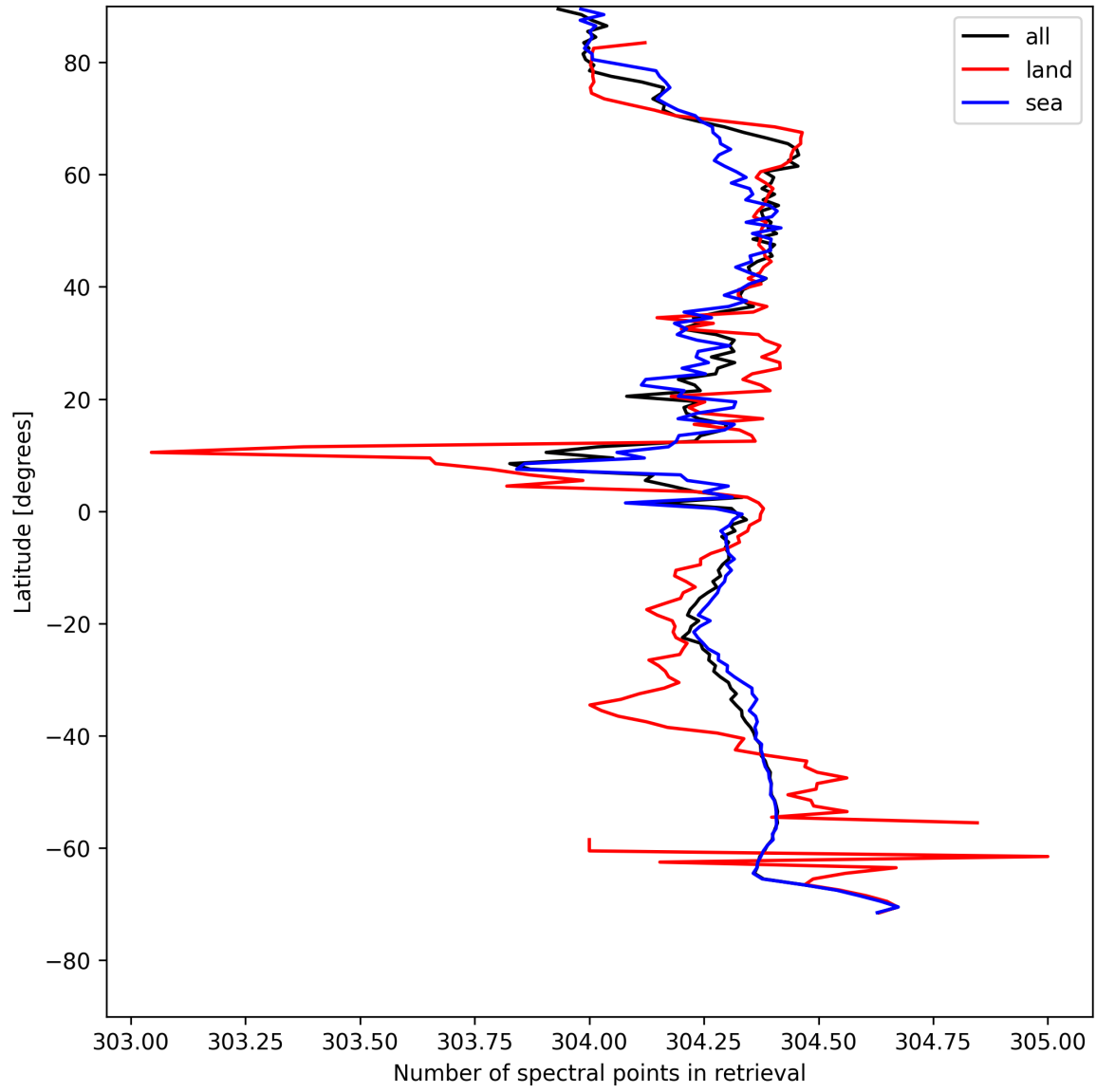
Figure 14: Zonal average of “Number of spectral points in retrieval” for 2025-08-07 to 2025-08-07.
