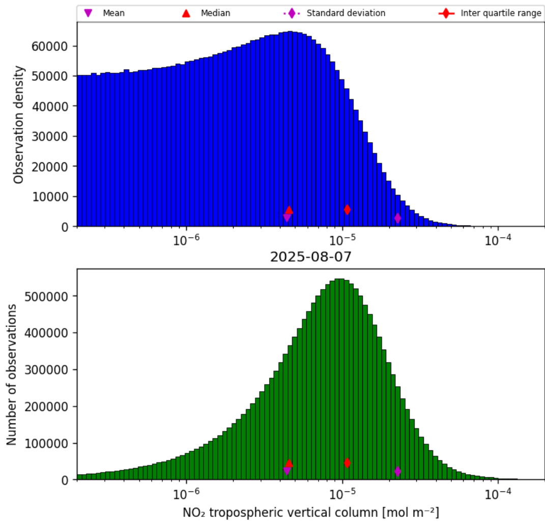
Figure 27: Histogram of “ \text{NO}_2 tropospheric vertical column” for 2025-08-07 to 2025-08-07
