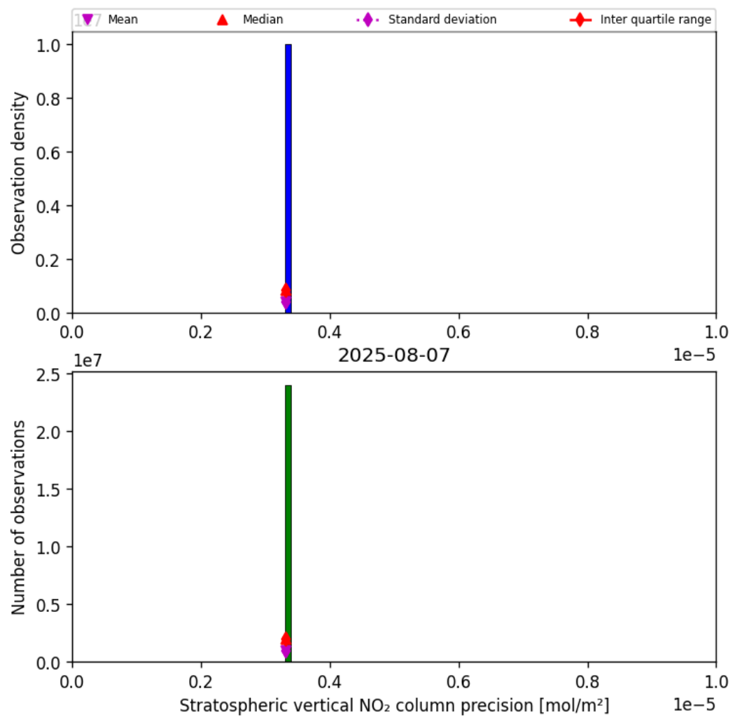
Figure 35: Histogram of “Stratospheric vertical NO 2 column precision” for 2025-08-07 to 2025-08-07
