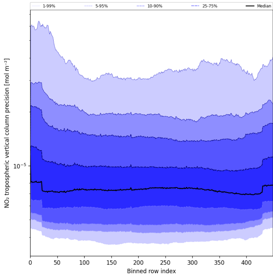
Figure 45: Along track statistics of “NO 2 tropospheric vertical column precision” for 2025-08-07 to 2025-08-07
