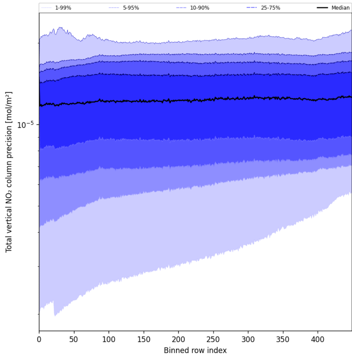
Figure 54: Along track statistics of “Total vertical NO 2 column precision” for 2025-08-07 to 2025-08-07
