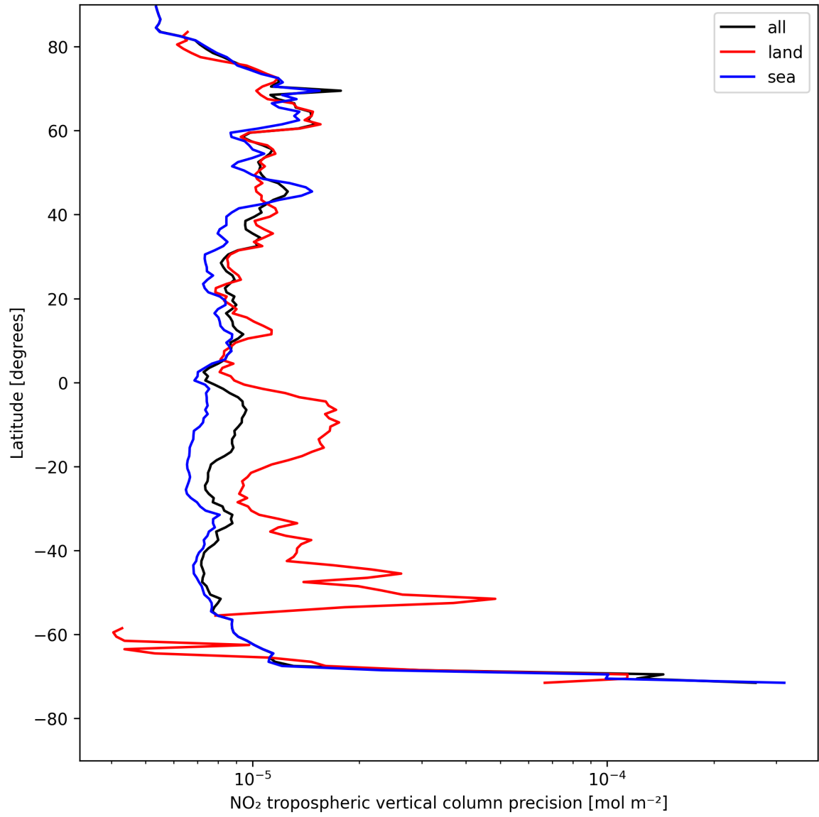
Figure 11: Zonal average of “NO 2 tropospheric vertical column precision” for 2025-08-07 to 2025-08-07.
