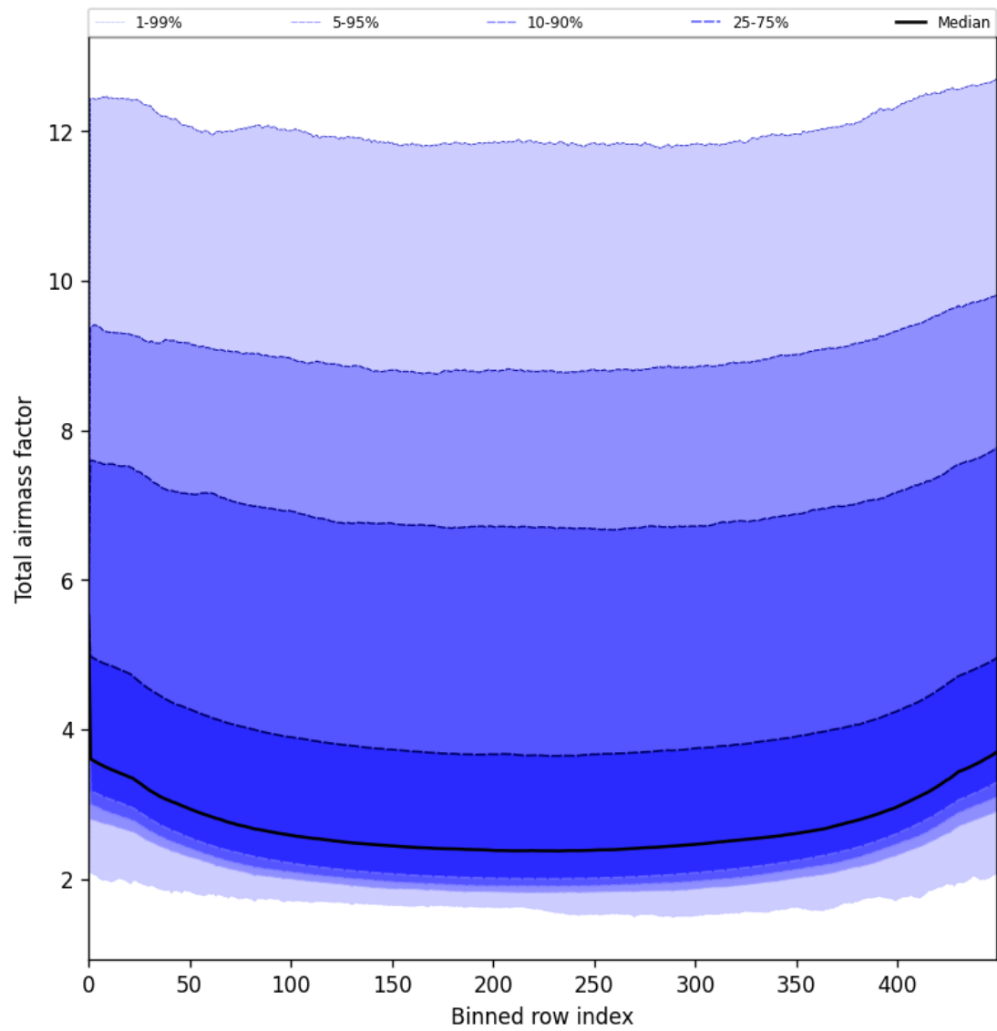
Figure 47: Along track statistics of “Total airmass factor” for 2025-08-07 to 2025-08-07
