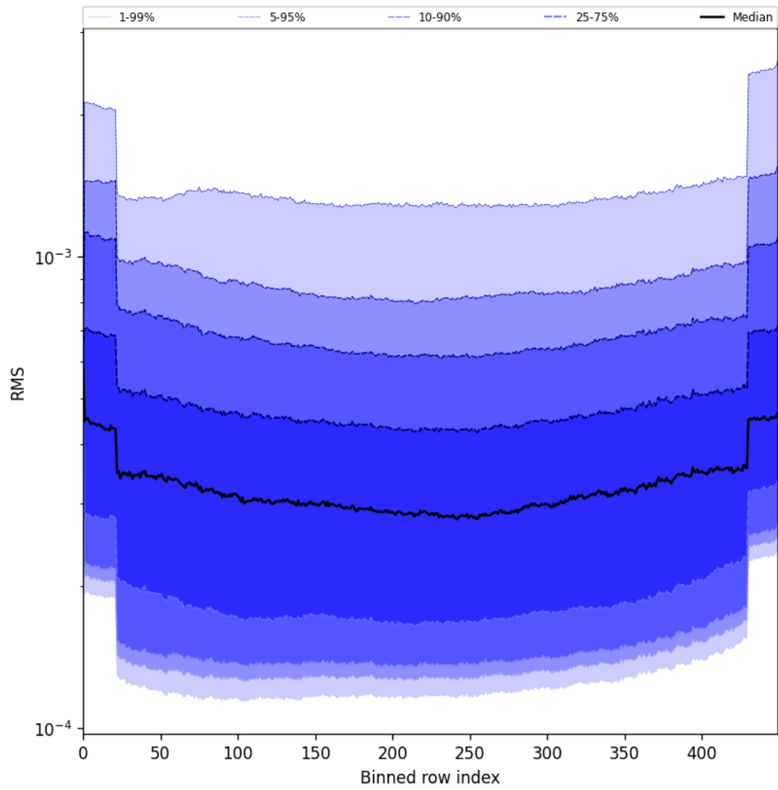
Figure 58: Along track statistics of “RMS” for 2025-08-07 to 2025-08-07
