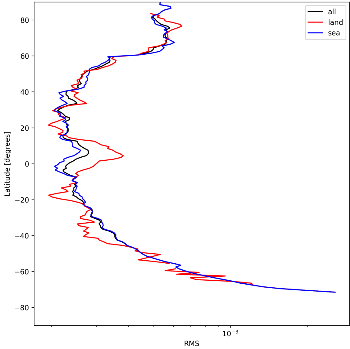
Figure 24: Zonal average of “RMS” for 2025-08-07 to 2025-08-07.
