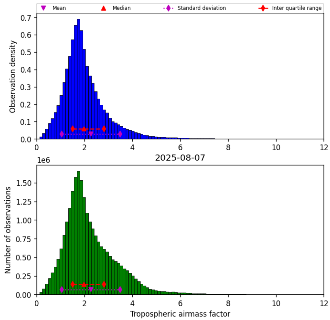
Figure 29: Histogram of “Tropospheric airmass factor” for 2025-08-07 to 2025-08-07
