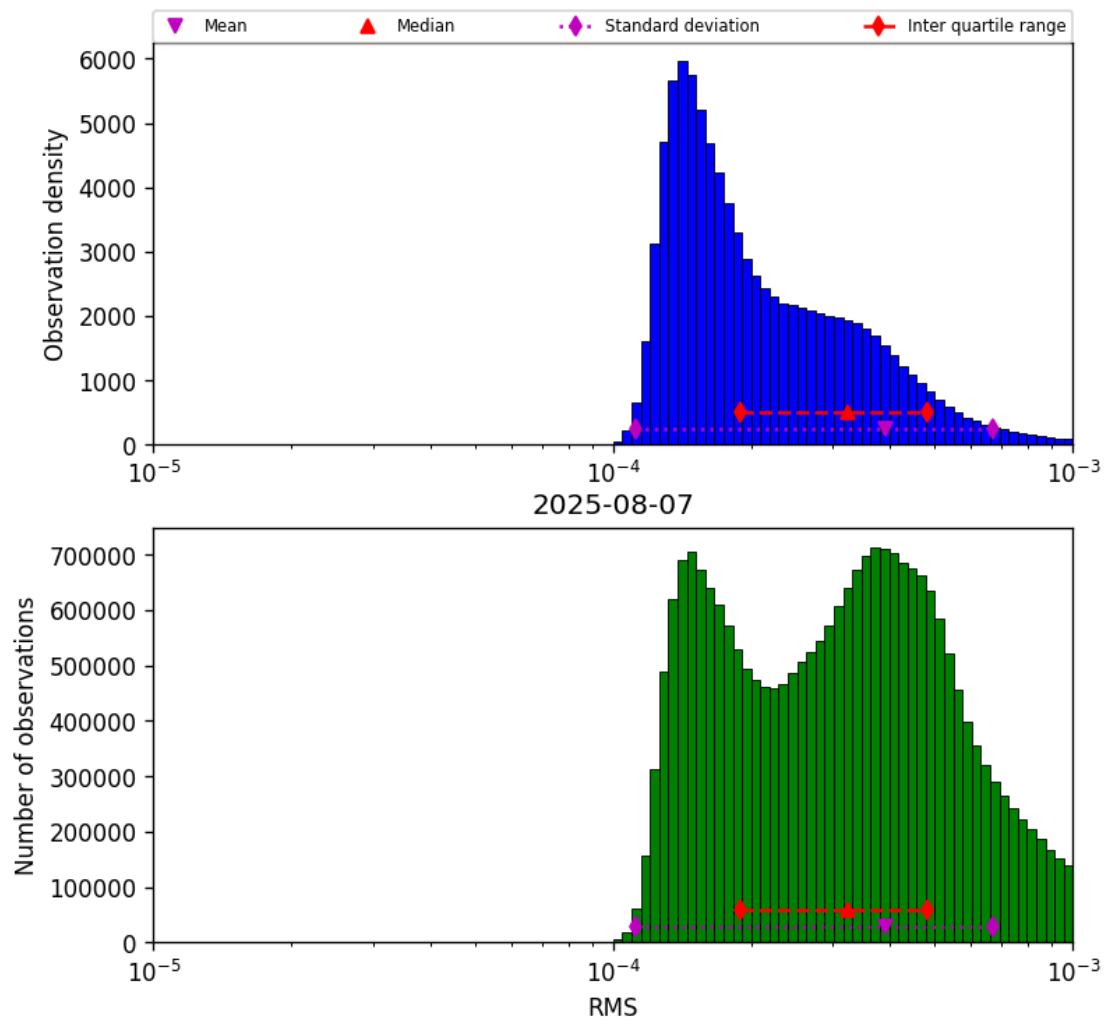
Figure 41: Histogram of “RMS” for 2025-08-07 to 2025-08-07
