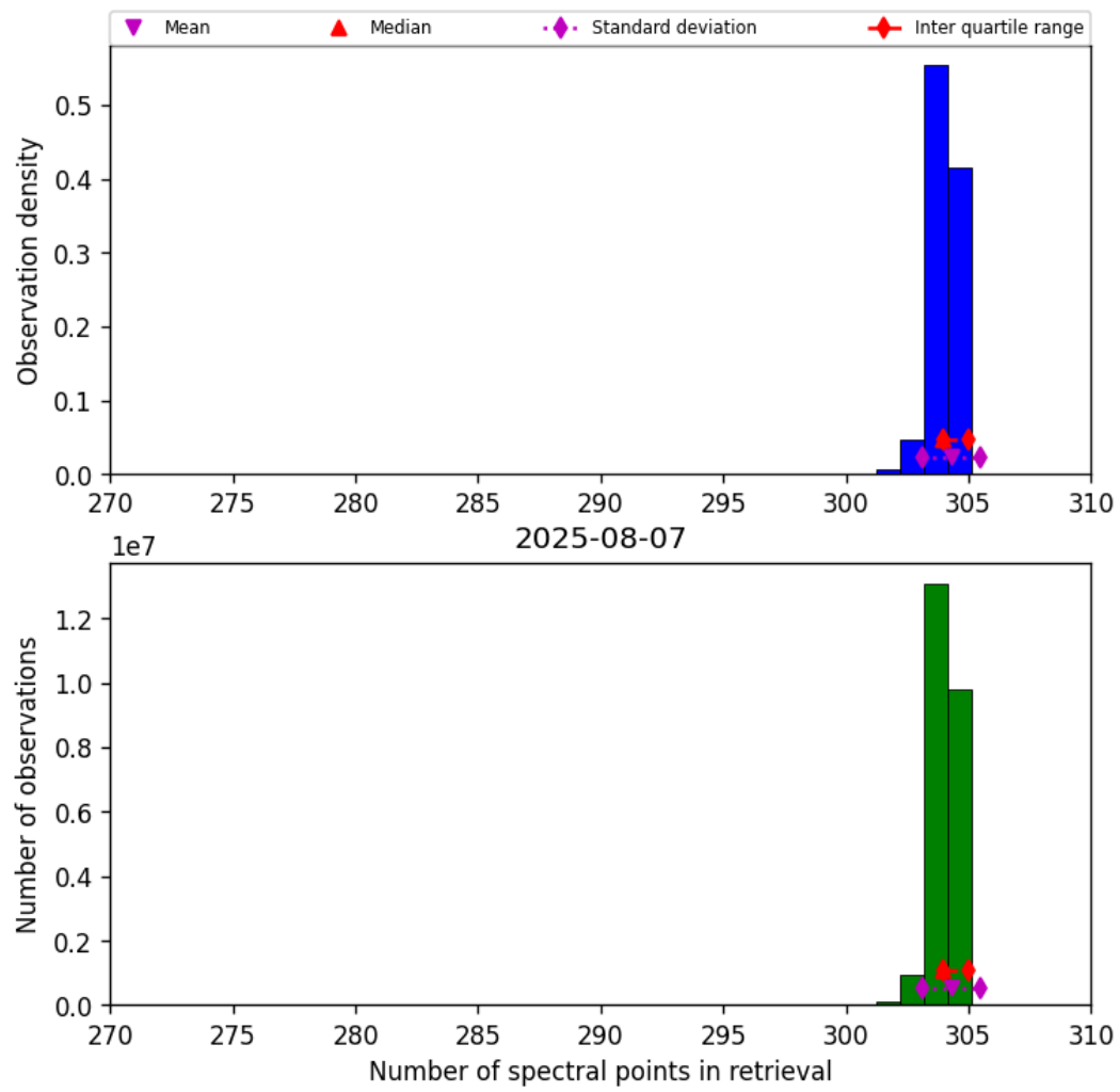
Figure 31: Histogram of “Number of spectral points in retrieval” for 2025-08-07 to 2025-08-07
