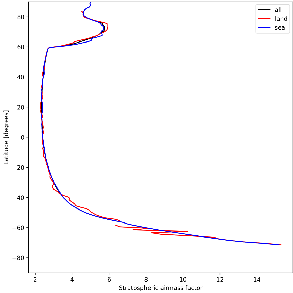
Figure 25: Zonal average of “Stratospheric airmass factor” for 2025-08-07 to 2025-08-07.
