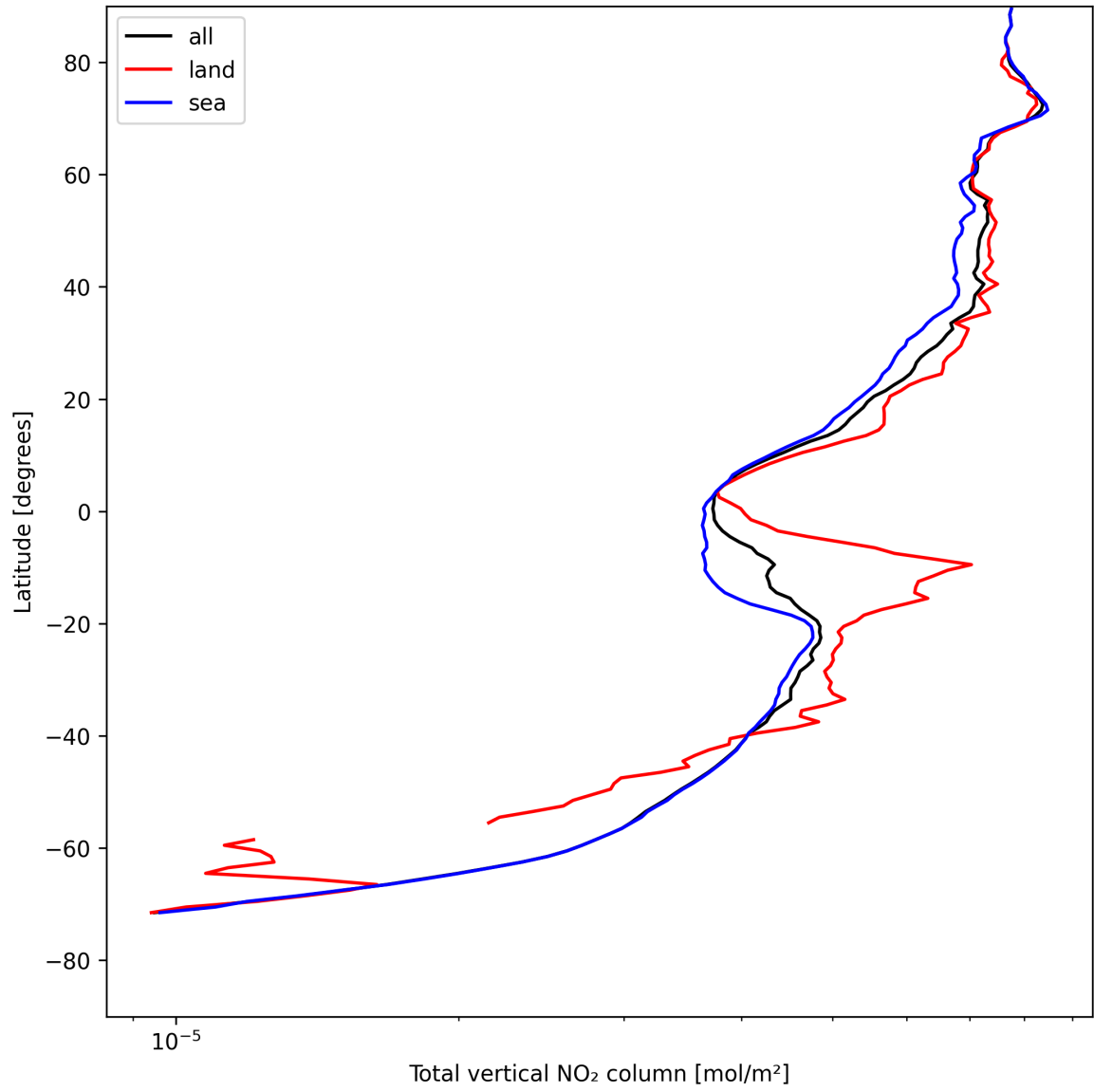
Figure 19: Zonal average of “Total vertical NO 2 column” for 2025-08-07 to 2025-08-07.
