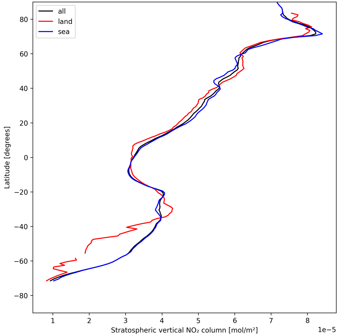
Figure 17: Zonal average of “Stratospheric vertical NO 2 column” for 2025-08-07 to 2025-08-07.
