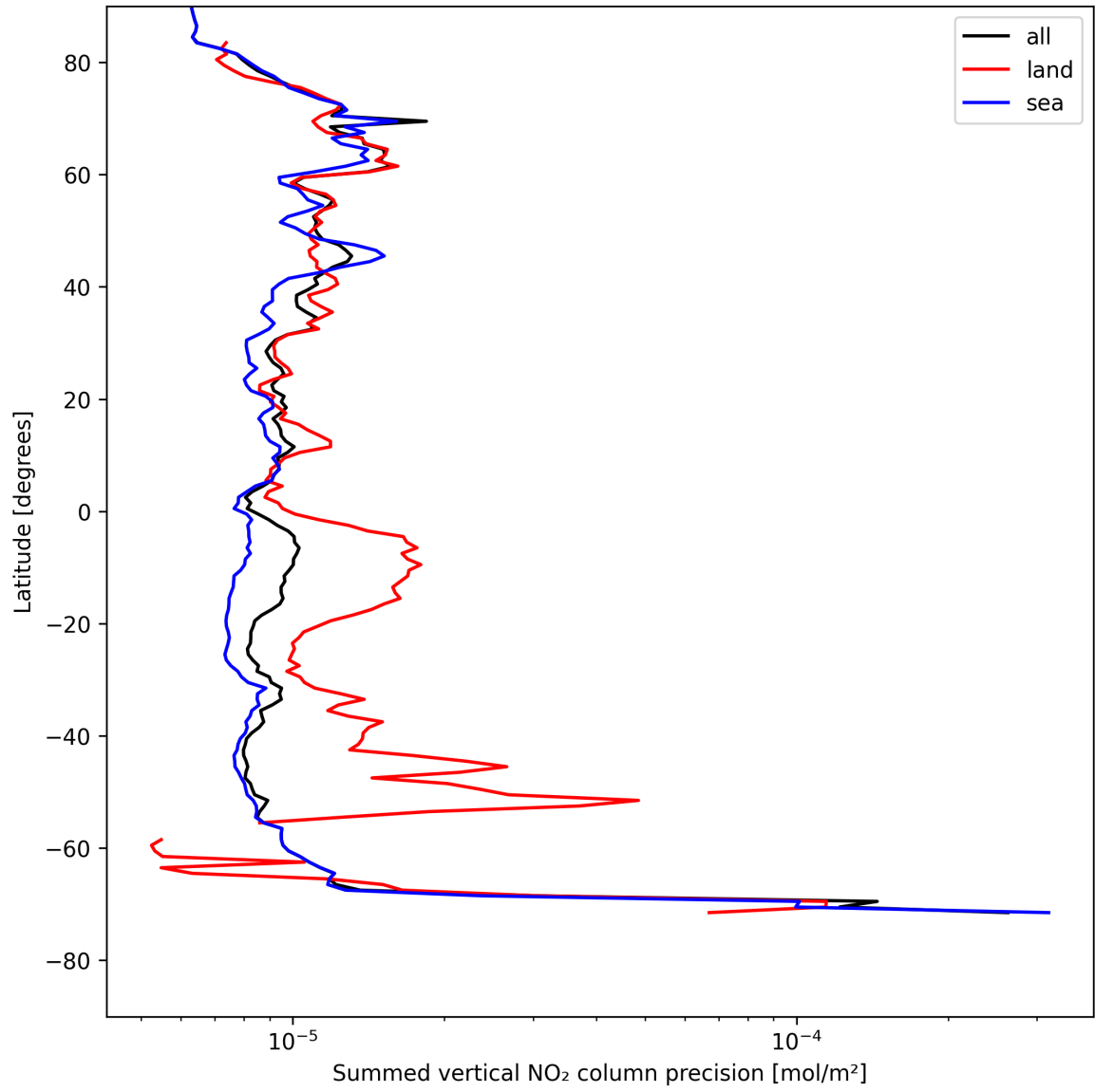
Figure 22: Zonal average of "Summed vertical NO 2 column precision" for 2025-08-07 to 2025-08-07.
