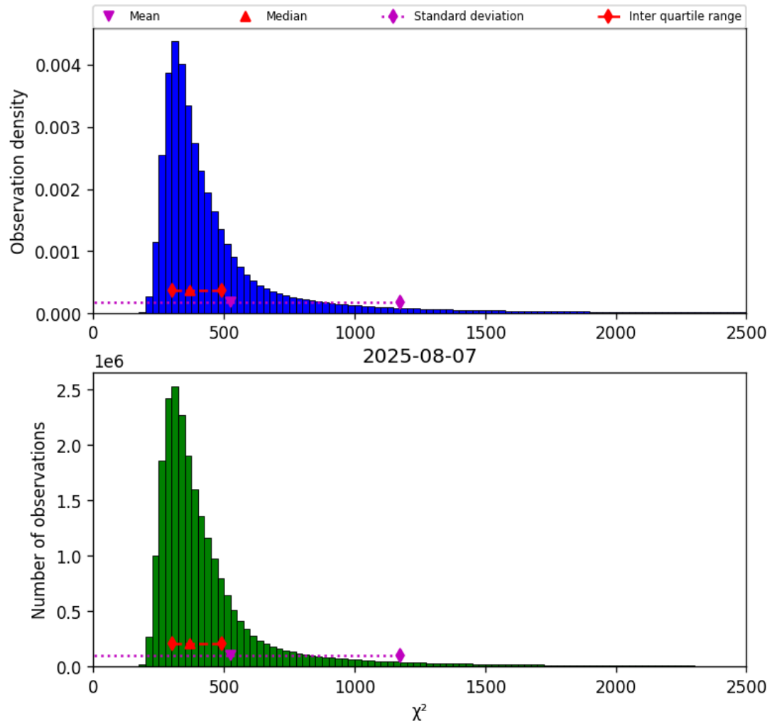
Figure 40: Histogram of “ \chi^2 ” for 2025-08-07 to 2025-08-07
