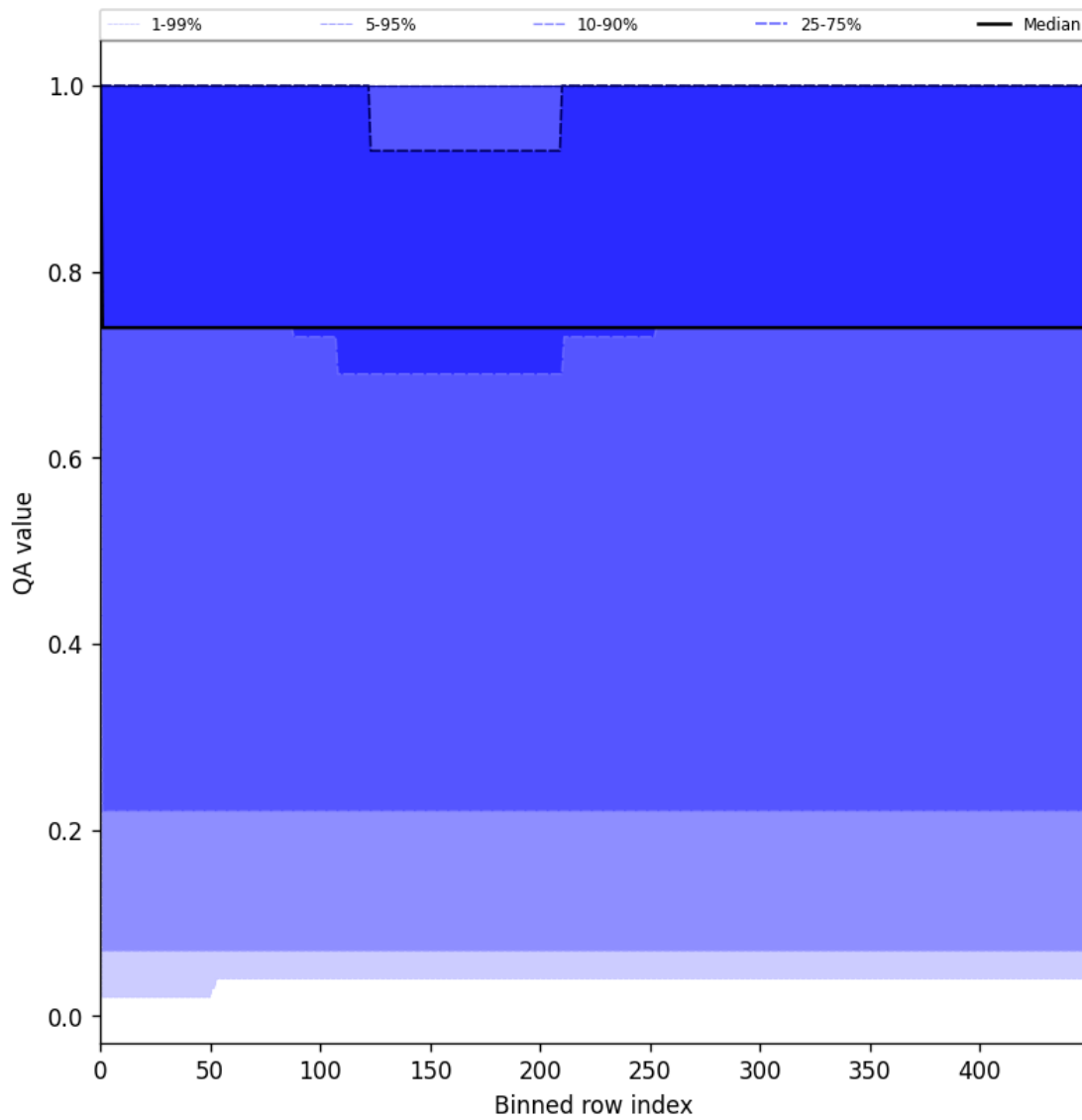
Figure 43: Along track statistics of “QA value” for 2025-08-07 to 2025-08-07
