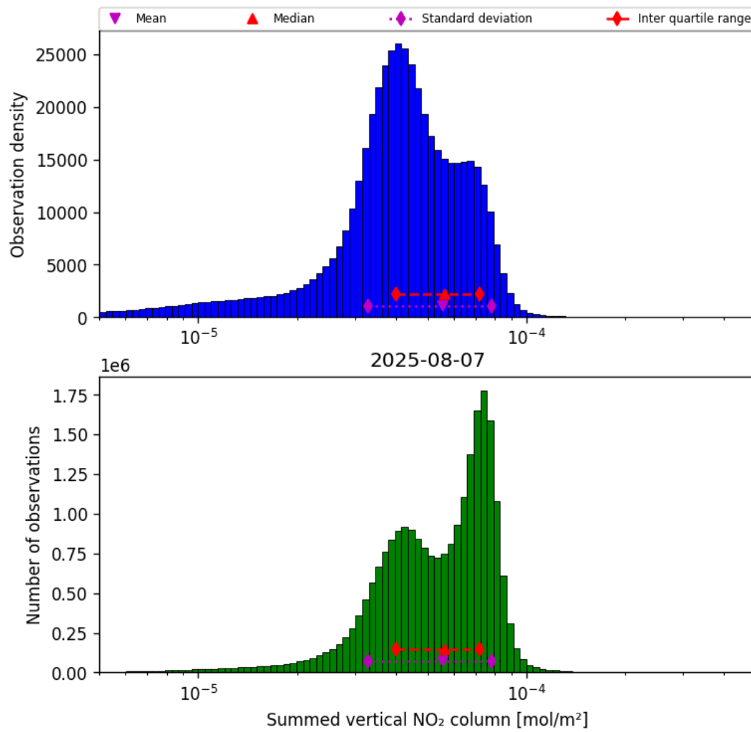
Figure 38: Histogram of “Summed vertical NO 2 column” for 2025-08-07 to 2025-08-07
