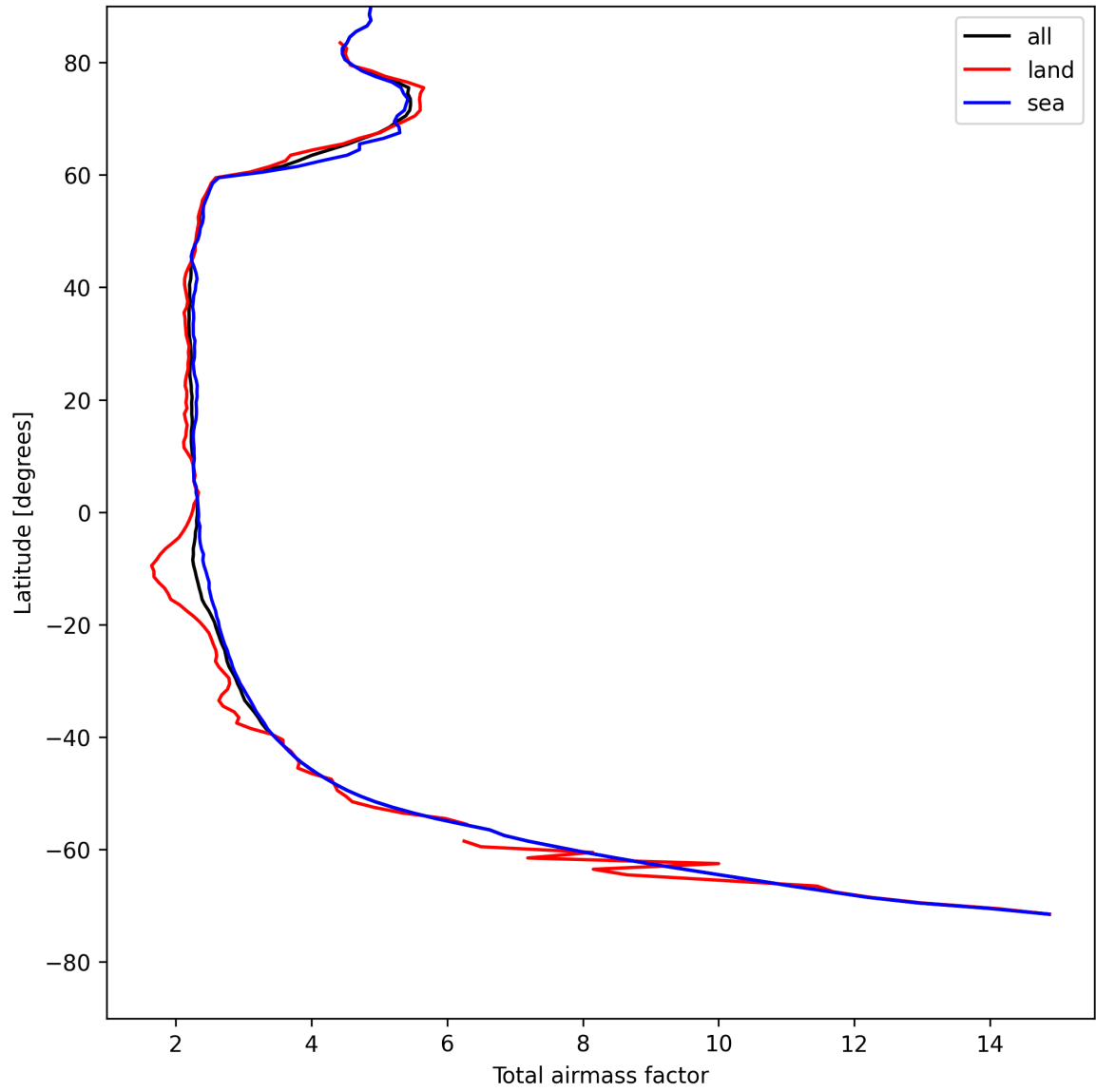
Figure 13: Zonal average of “Total airmass factor” for 2025-08-07 to 2025-08-07.
