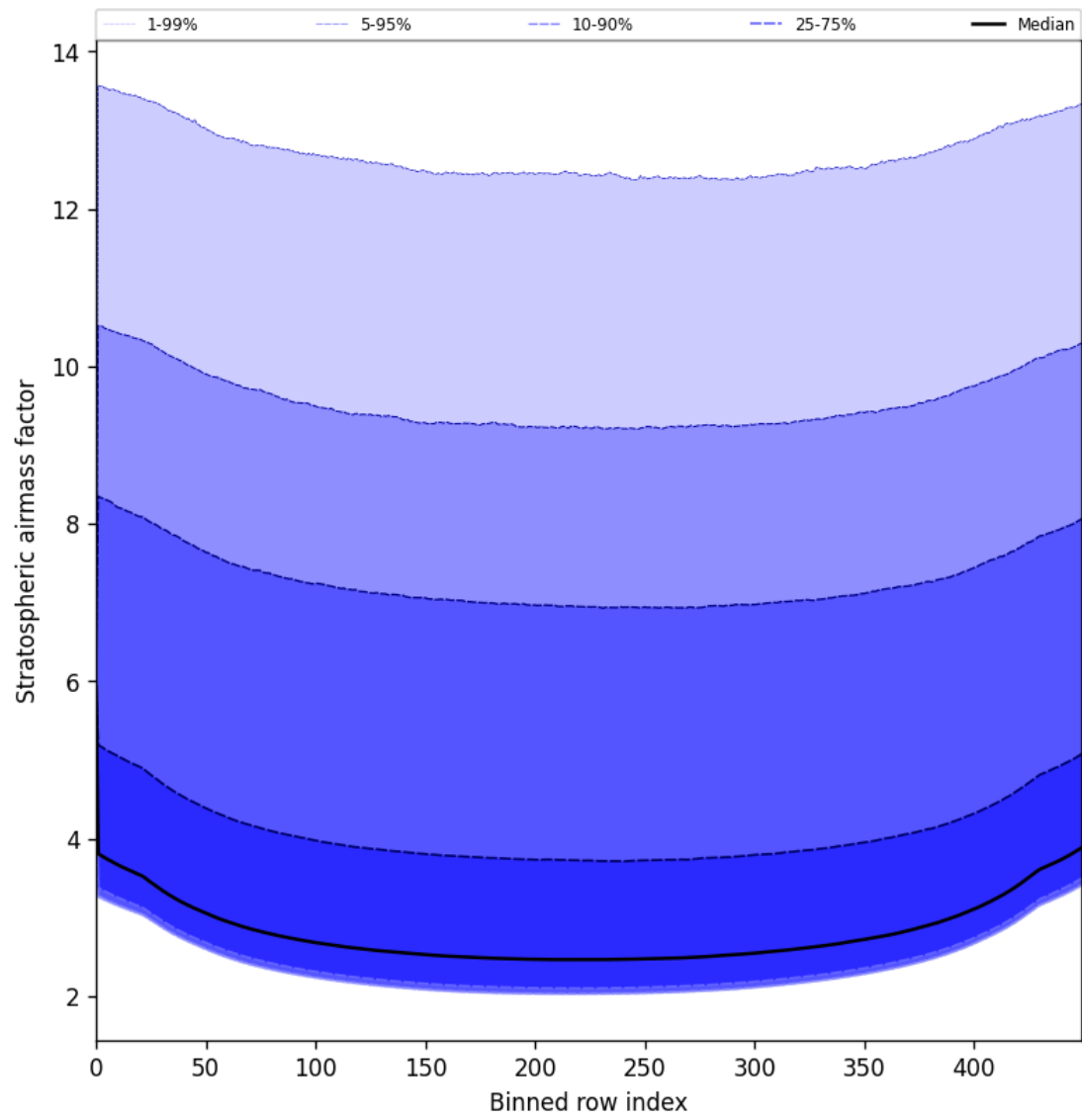
Figure 59: Along track statistics of “Stratospheric airmass factor” for 2025-08-07 to 2025-08-07
