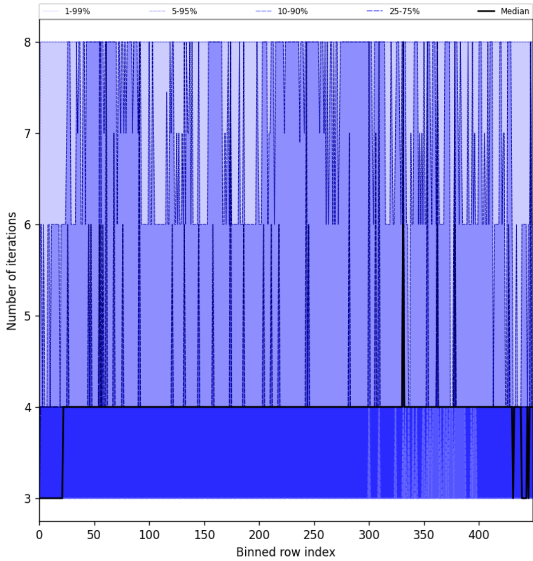
Figure 49: Along track statistics of “Number of iterations” for 2025-08-07 to 2025-08-07
