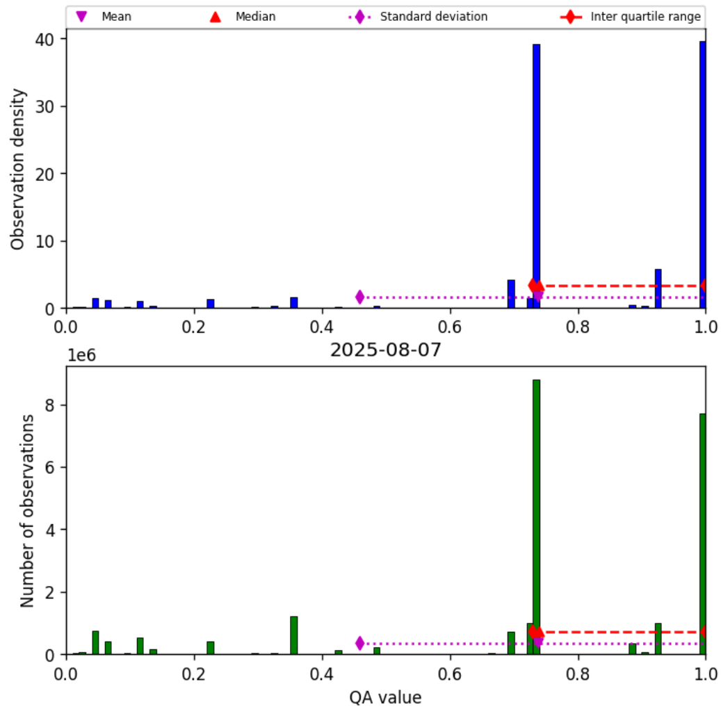
Figure 26: Histogram of “QA value” for 2025-08-07 to 2025-08-07
