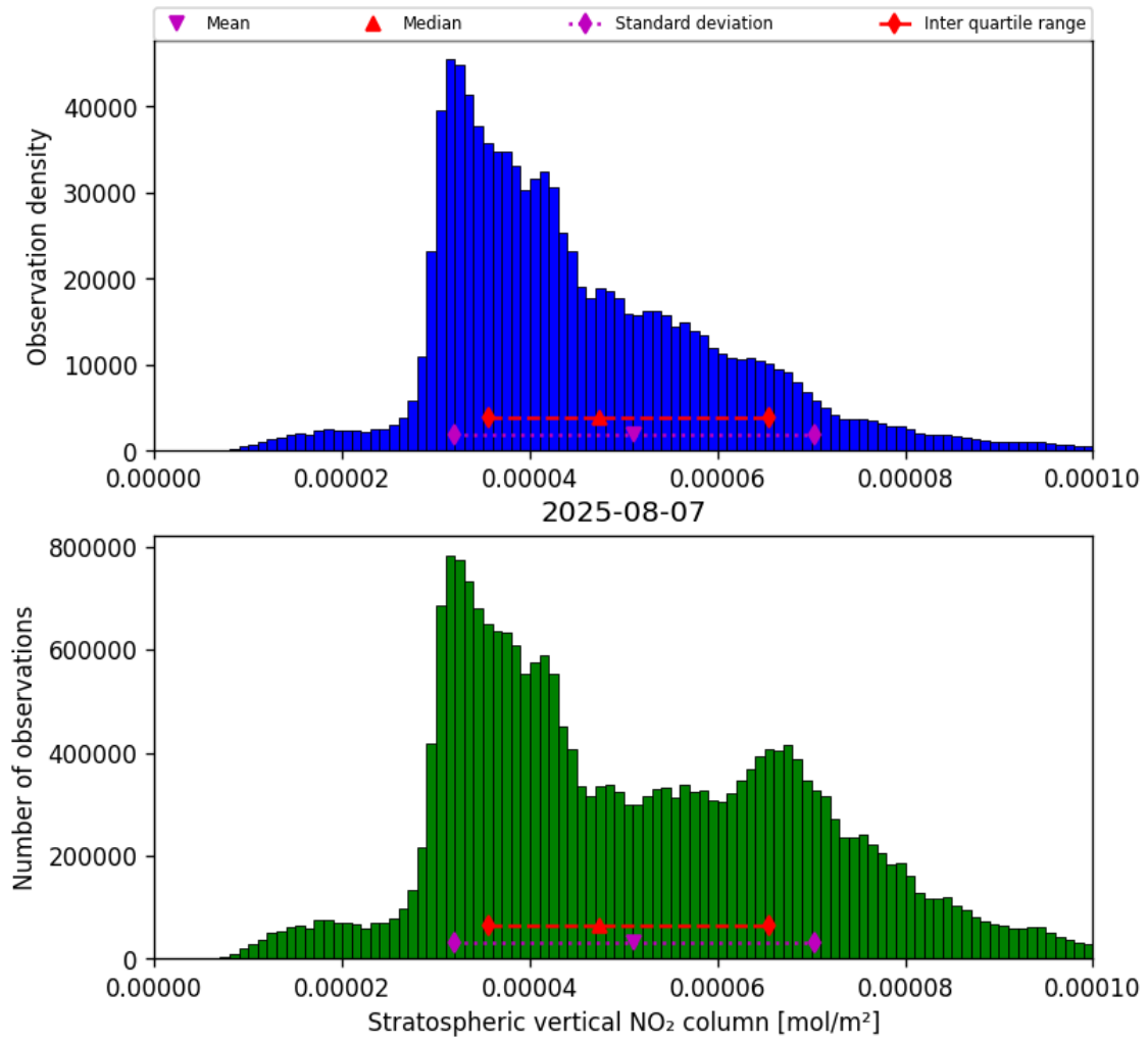
Figure 34: Histogram of “Stratospheric vertical NO 2 column” for 2025-08-07 to 2025-08-07
