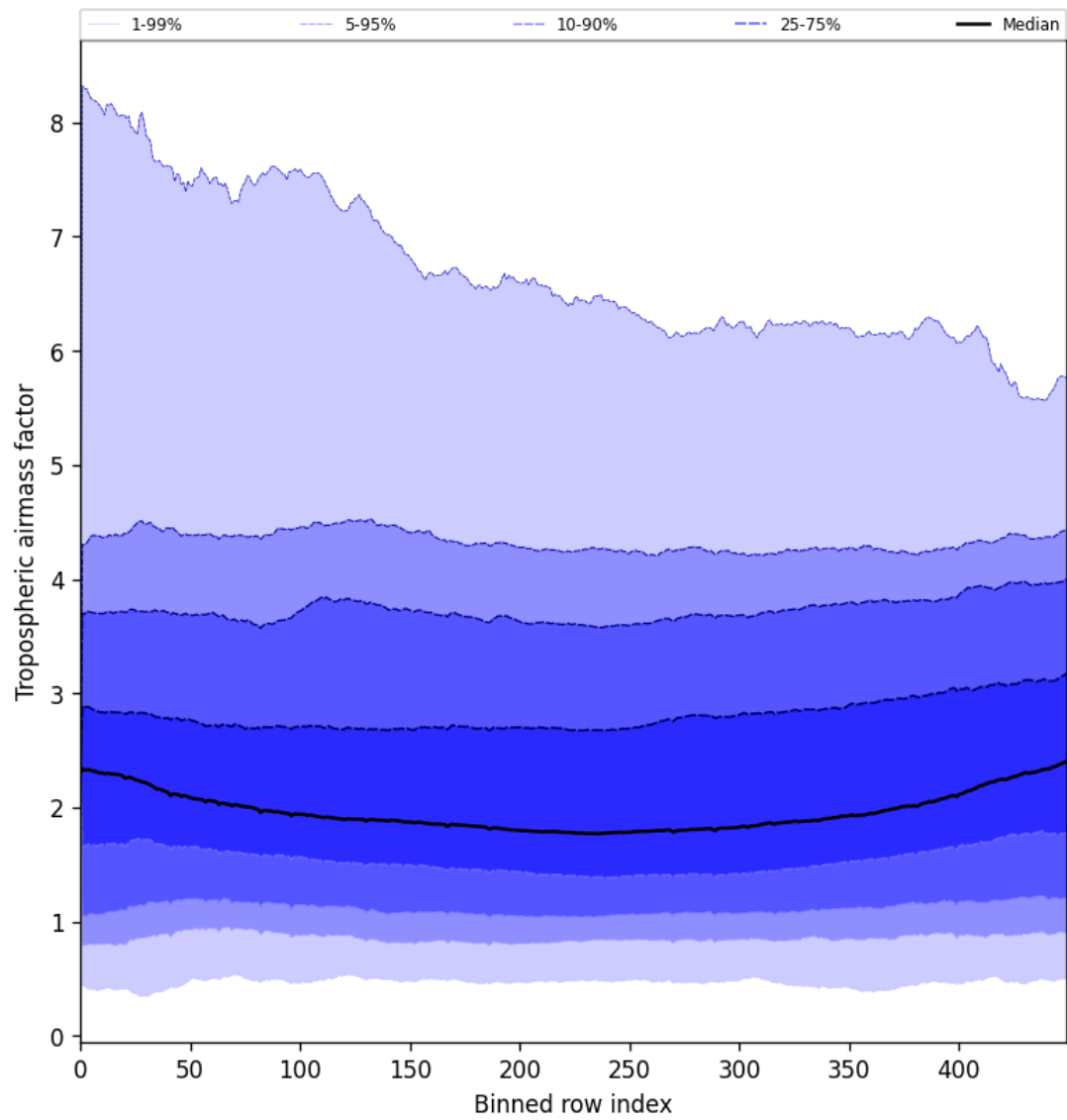
Figure 46: Along track statistics of “Tropospheric air mass factor” for 2025-08-07 to 2025-08-07
