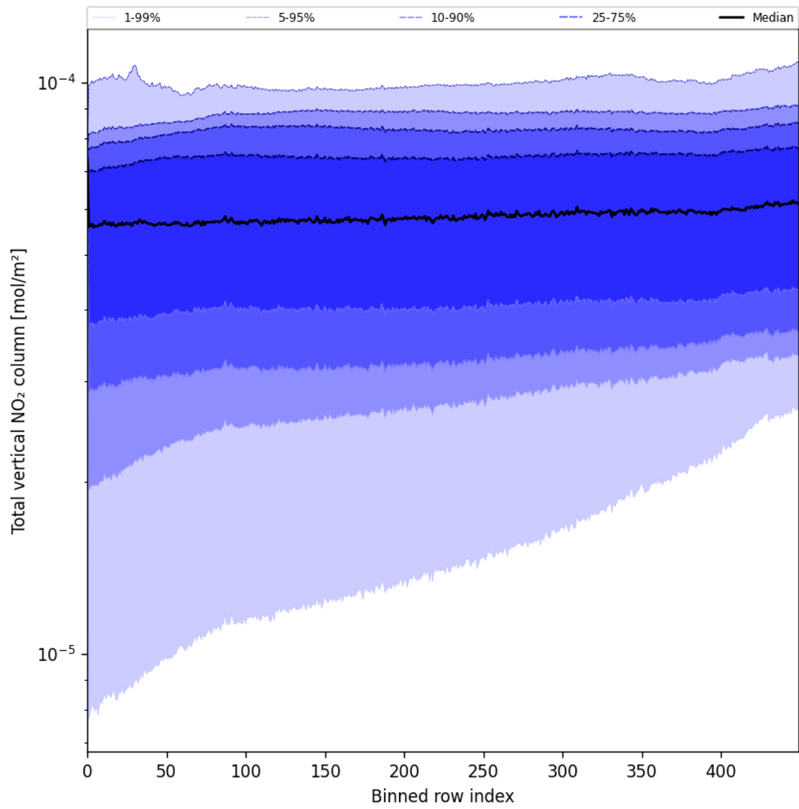
Figure 53: Along track statistics of “Total vertical NO 2 column” for 2025-08-07 to 2025-08-07
