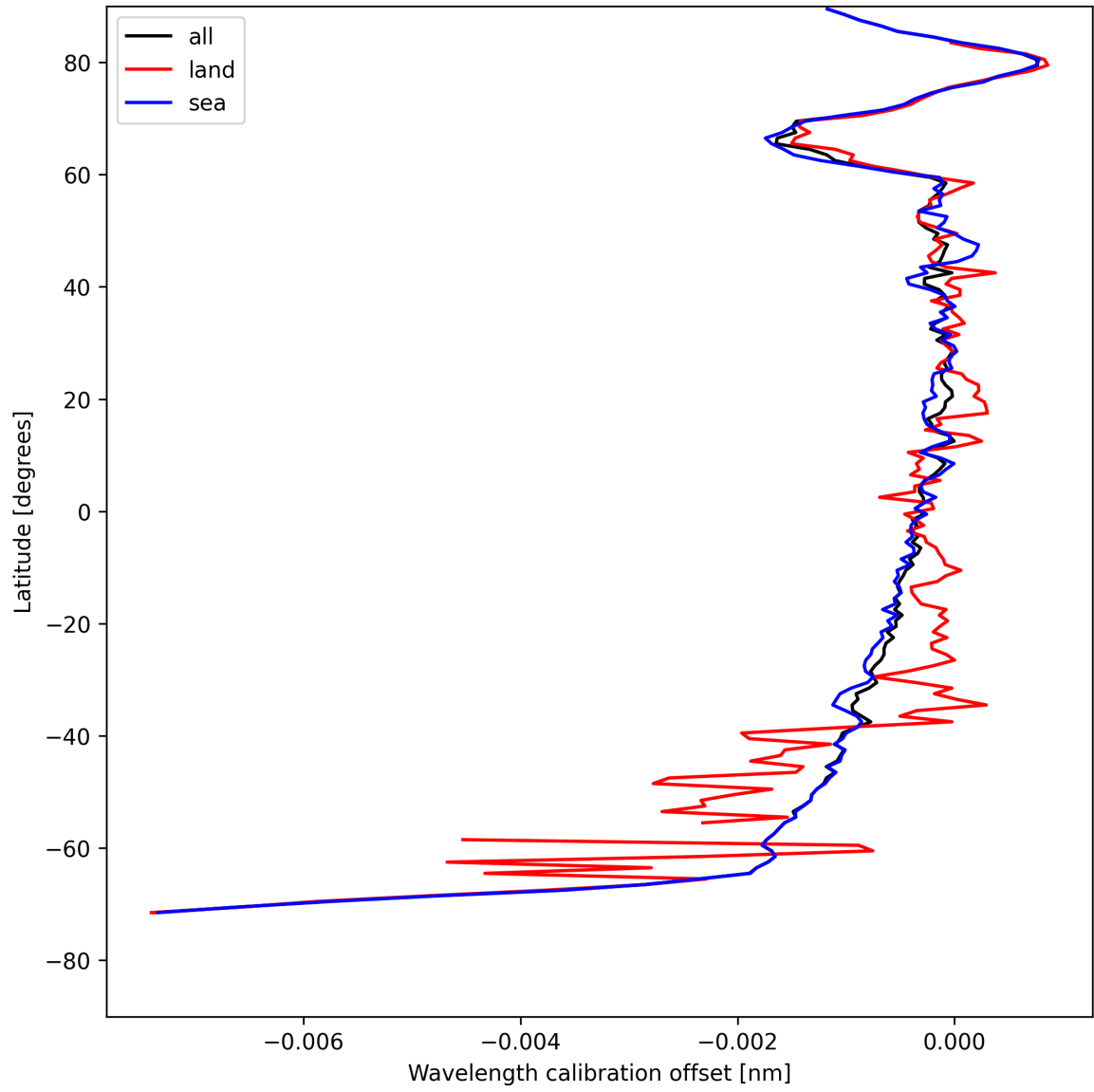
Figure 16: Zonal average of “Wavelength calibration offset” for 2025-08-07 to 2025-08-07.
