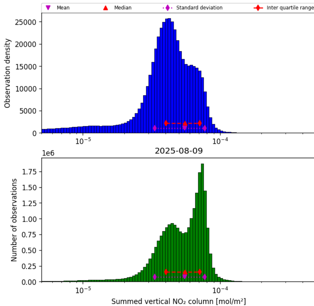
Figure 38: Histogram of “Summed vertical NO 2 column” for 2025-08-09 to 2025-08-10
