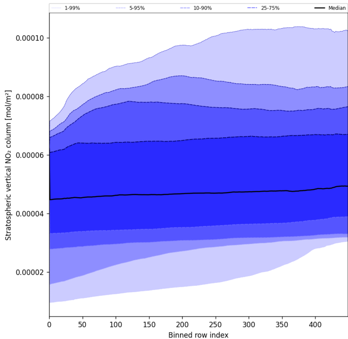
Figure 51: Along track statistics of “Stratospheric vertical NO 2 column” for 2025-08-09 to 2025-08-10
