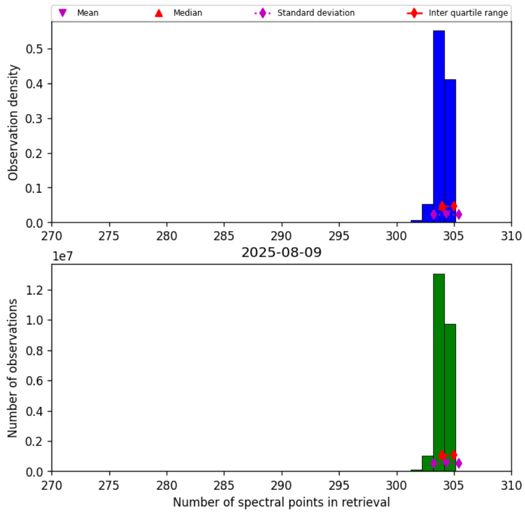
Figure 31: Histogram of “Number of spectral points in retrieval” for 2025-08-09 to 2025-08-10
