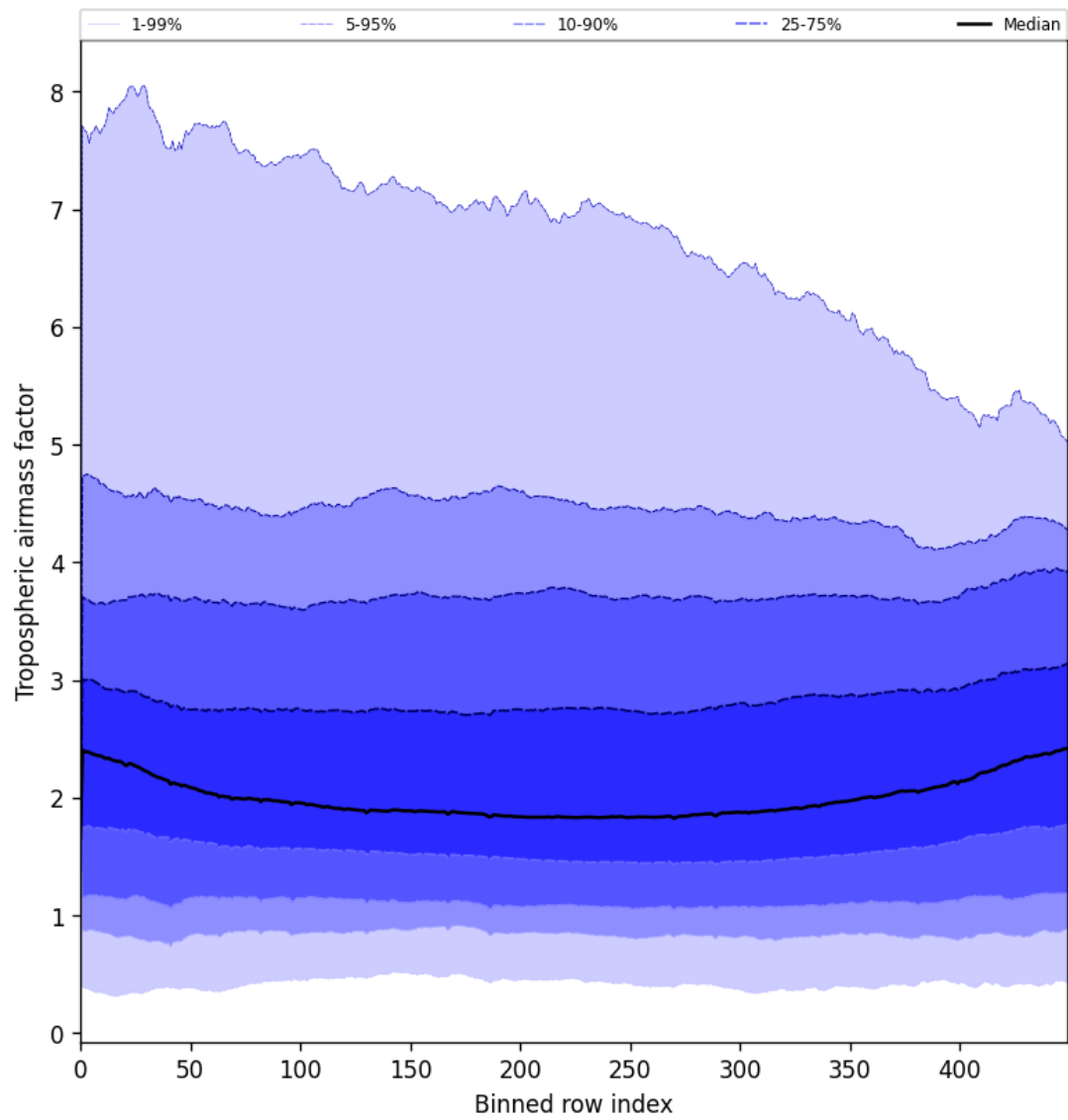
Figure 46: Along track statistics of “Tropospheric airmass factor” for 2025-08-09 to 2025-08-10
