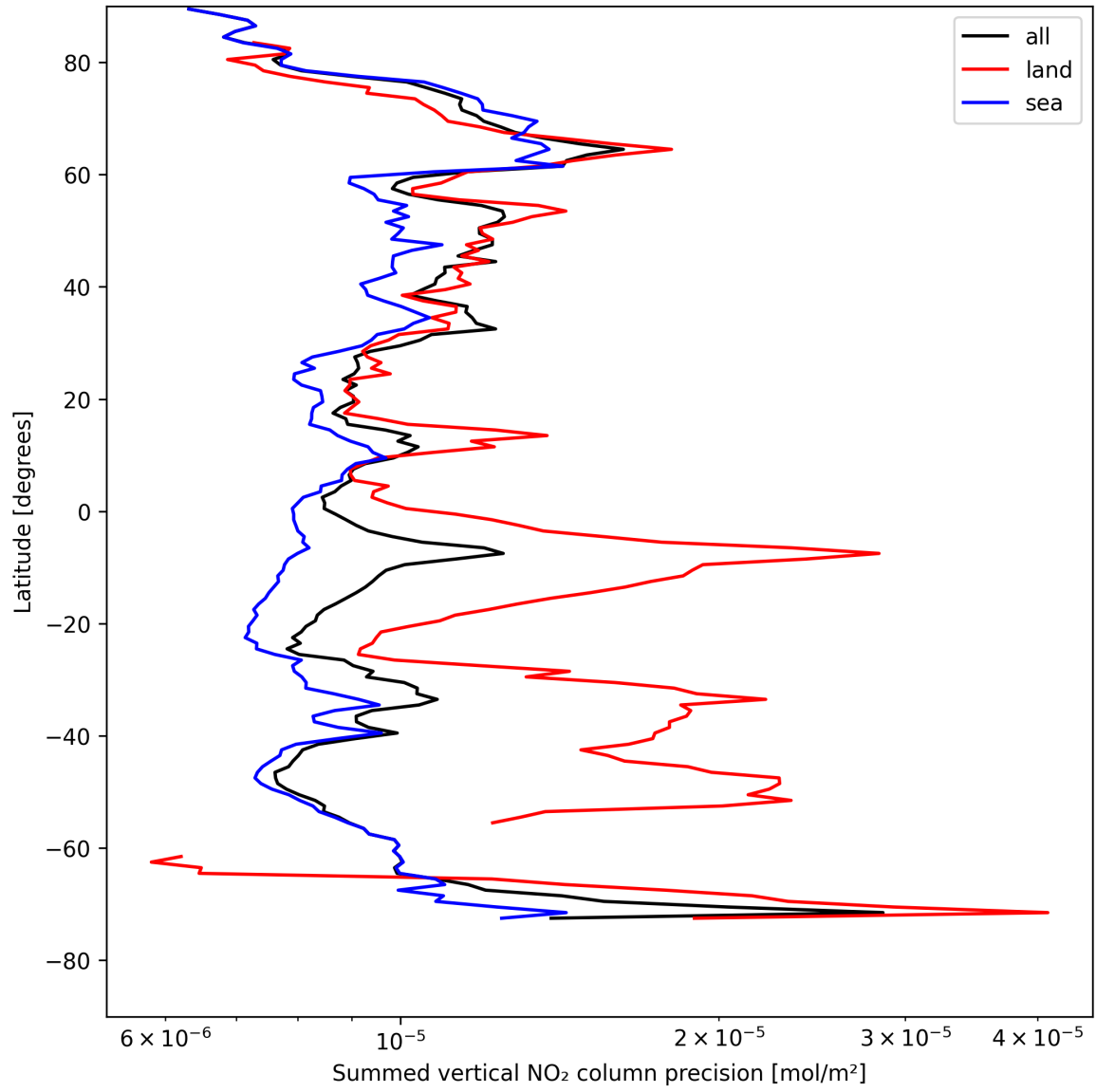
Figure 22: Zonal average of “Summed vertical NO 2 column precision” for 2025-08-09 to 2025-08-10.
