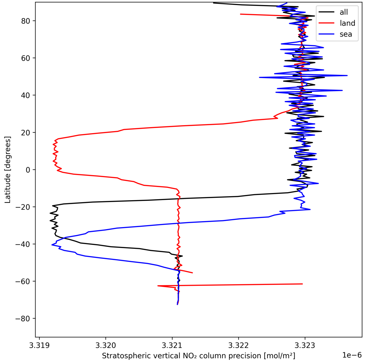
Figure 18: Zonal average of “Stratospheric vertical NO 2 column precision” for 2025-08-09 to 2025-08-10.
