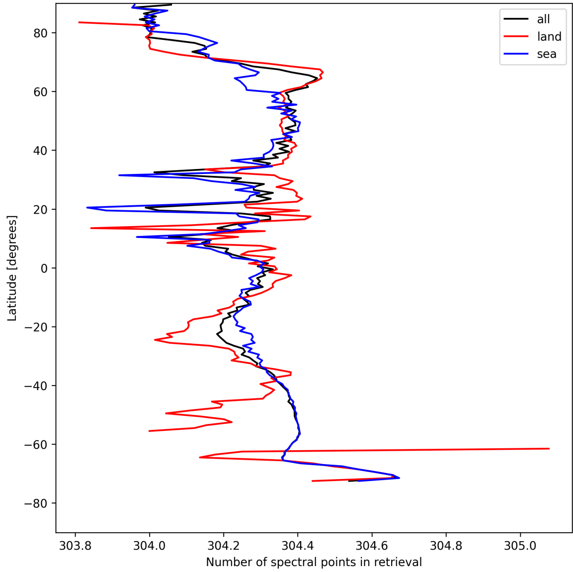
Figure 14: Zonal average of “Number of spectral points in retrieval” for 2025-08-09 to 2025-08-10.
