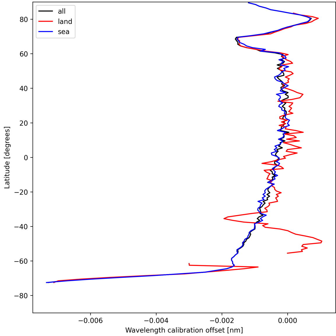
Figure 16: Zonal average of “Wavelength calibration offset” for 2025-08-09 to 2025-08-10.
