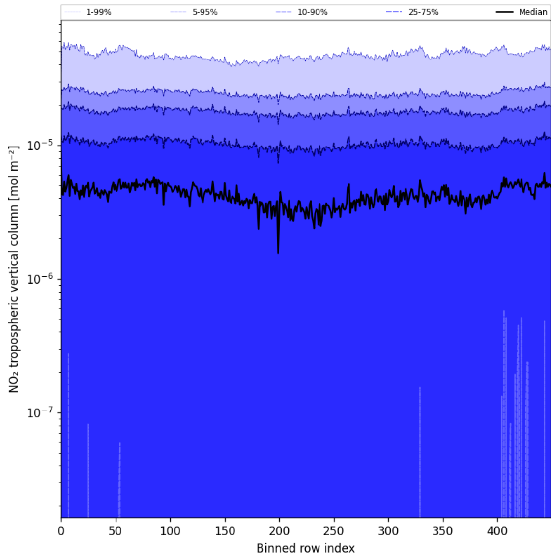
Figure 44: Along track statistics of “NO 2 tropospheric vertical column” for 2025-08-09 to 2025-08-10
