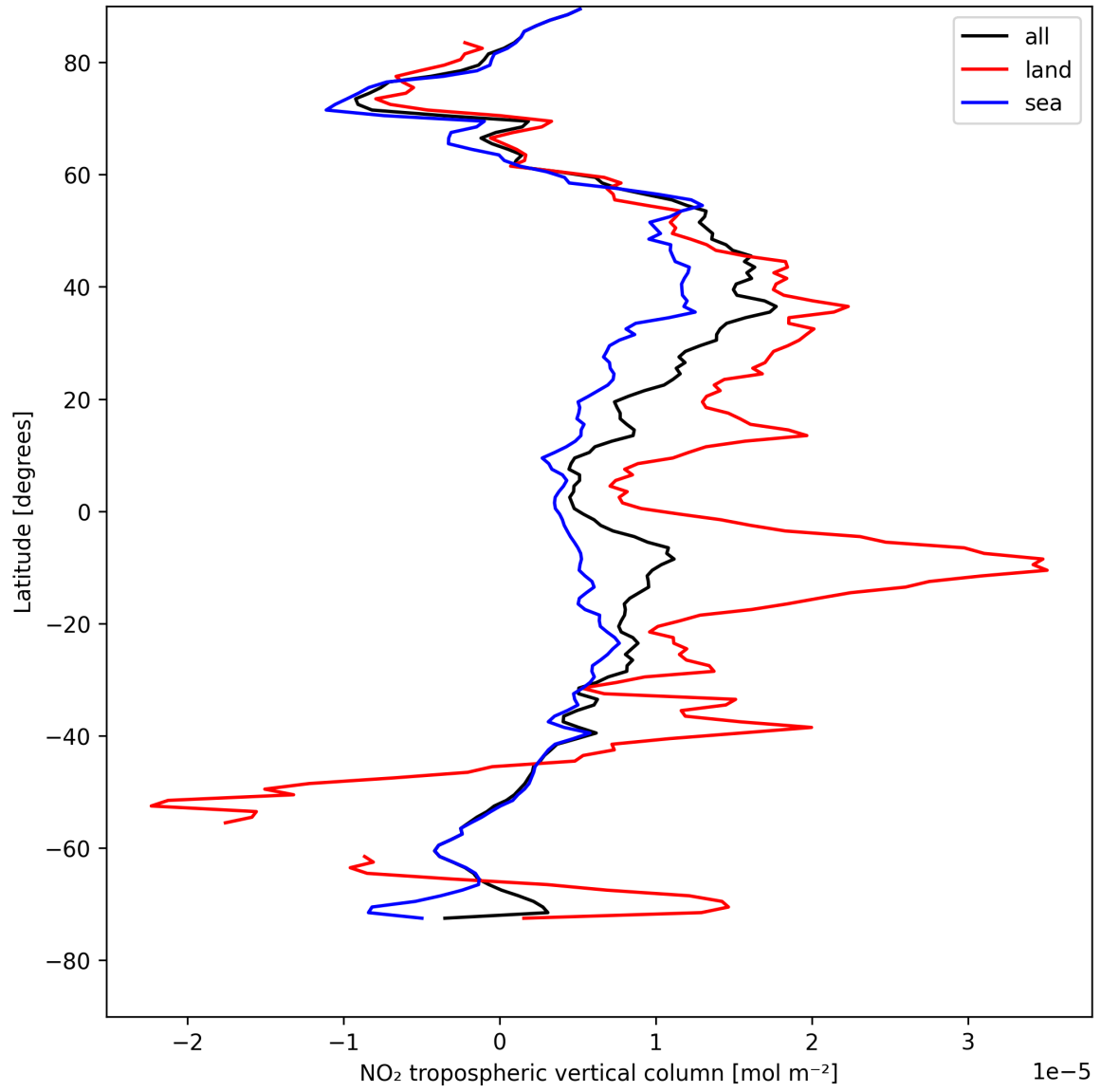
Figure 10: Zonal average of “NO 2 tropospheric vertical column” for 2025-08-09 to 2025-08-10.
