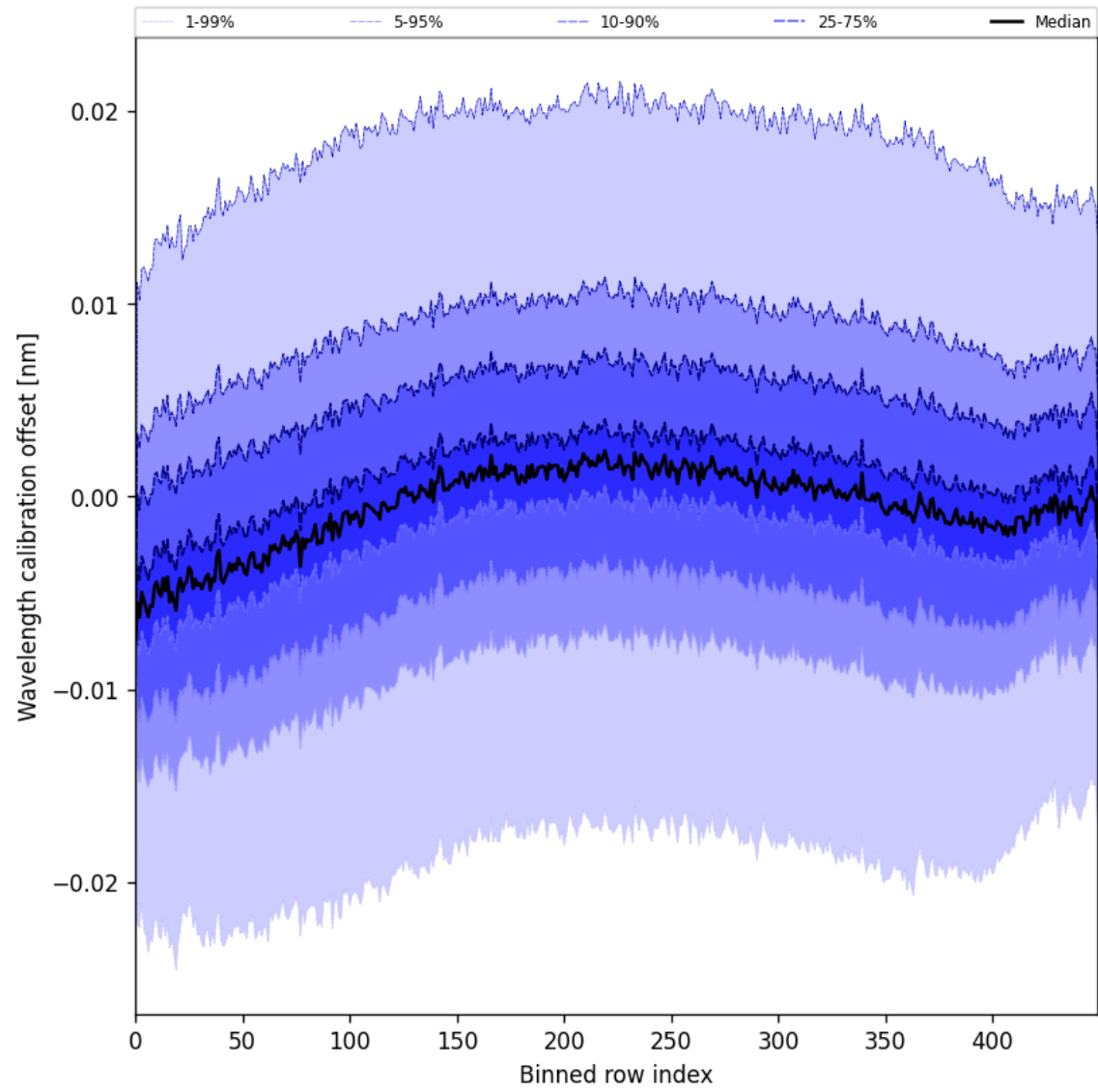
Figure 50: Along track statistics of “Wavelength calibration offset” for 2025-08-09 to 2025-08-10
