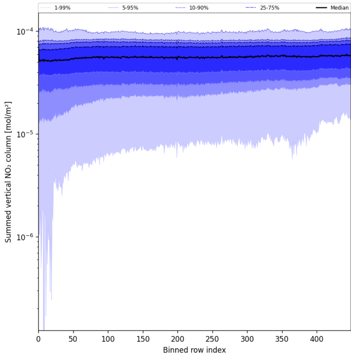
Figure 55: Along track statistics of “Summed vertical NO 2 column” for 2025-08-09 to 2025-08-10
