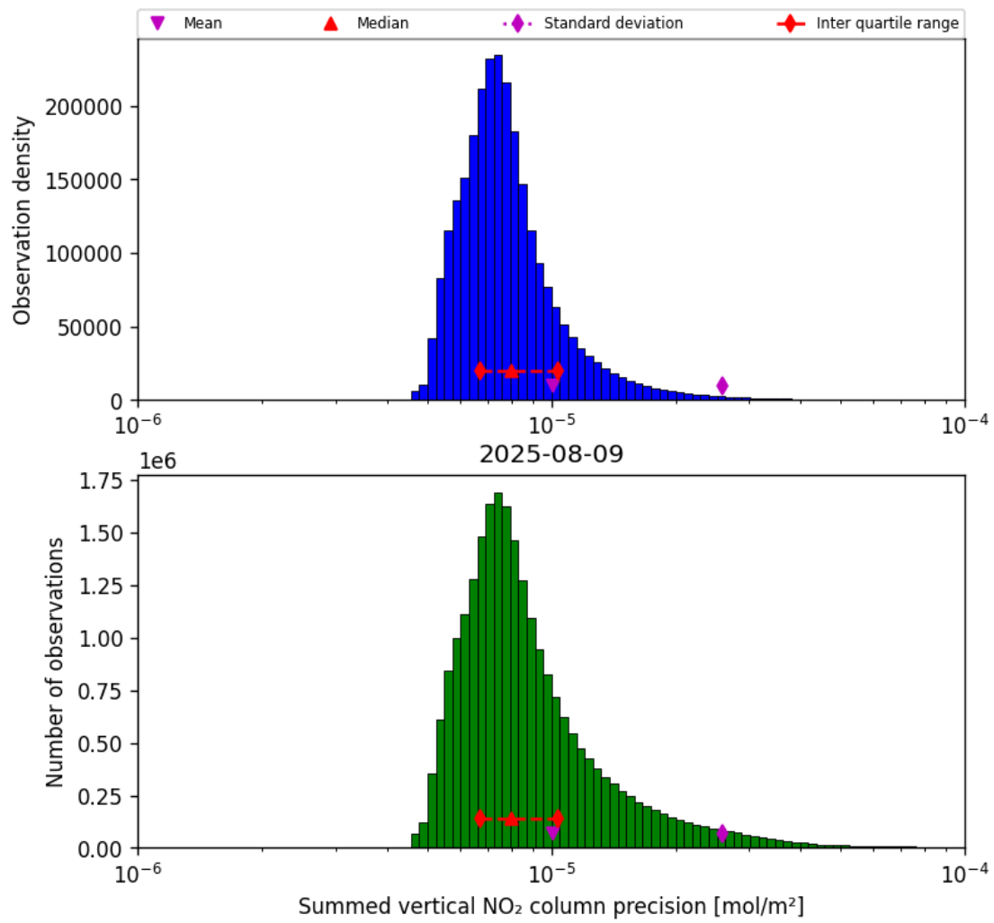
Figure 39: Histogram of “Summed vertical NO 2 column precision” for 2025-08-09 to 2025-08-10
