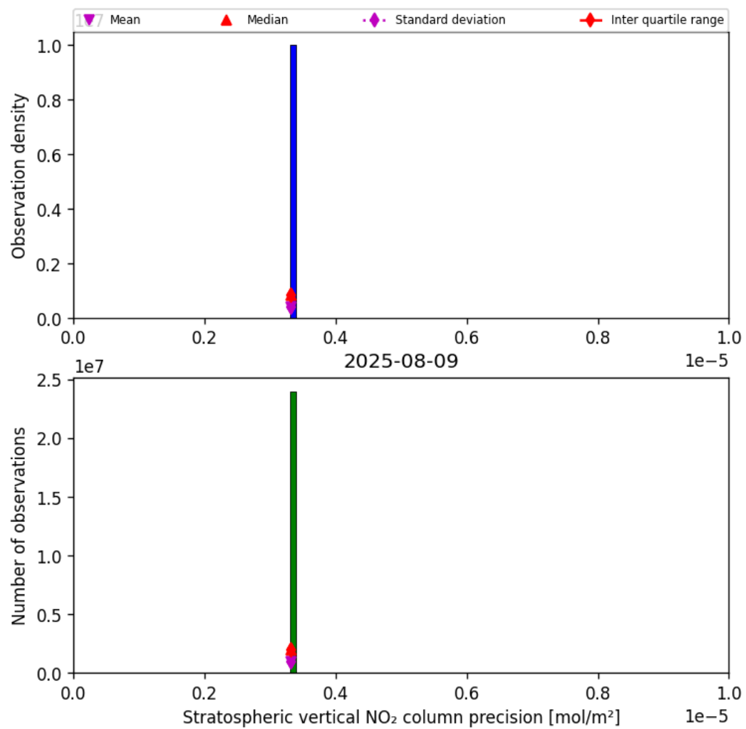
Figure 35: Histogram of “Stratospheric vertical NO 2 column precision” for 2025-08-09 to 2025-08-10
