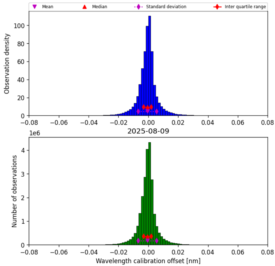
Figure 33: Histogram of “Wavelength calibration offset” for 2025-08-09 to 2025-08-10
