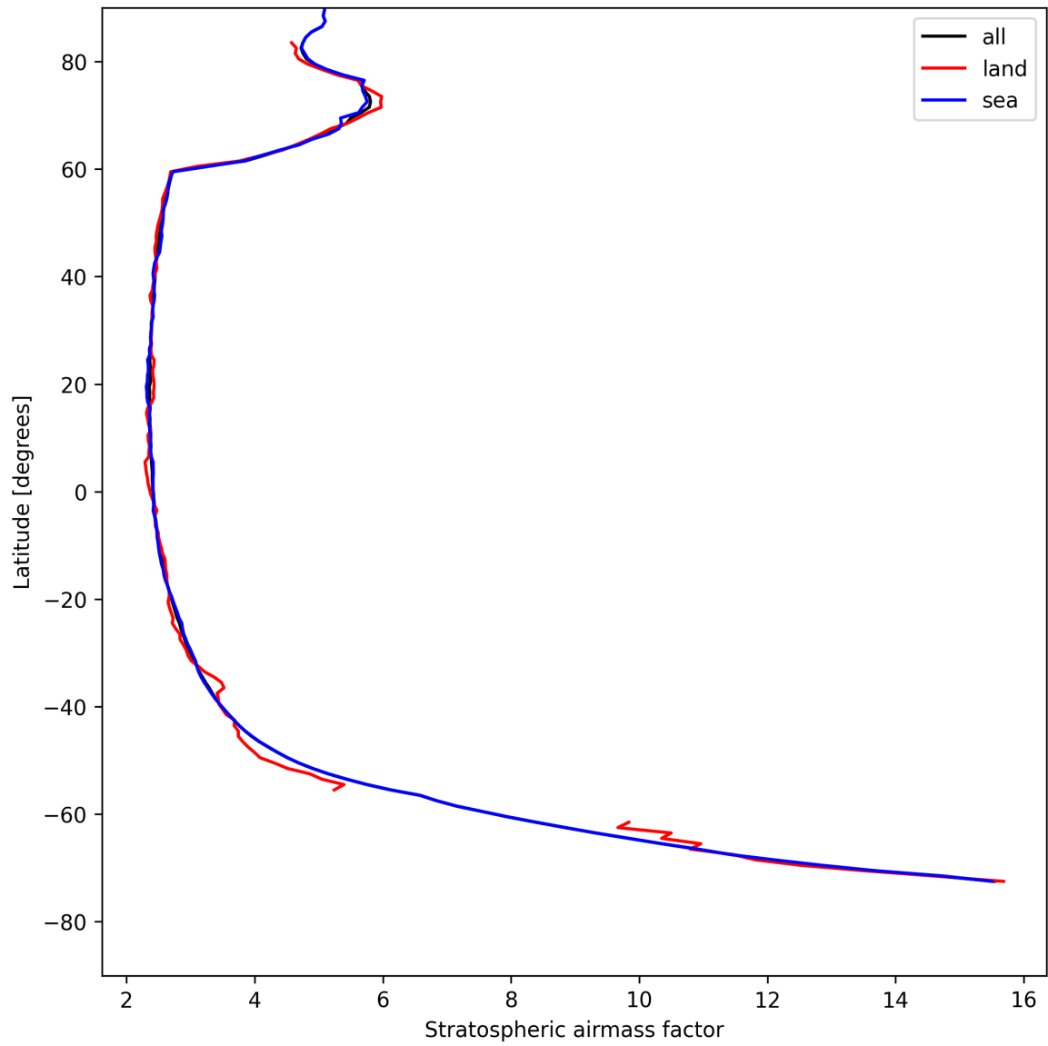
Figure 25: Zonal average of “Stratospheric airmass factor” for 2025-08-09 to 2025-08-10.
