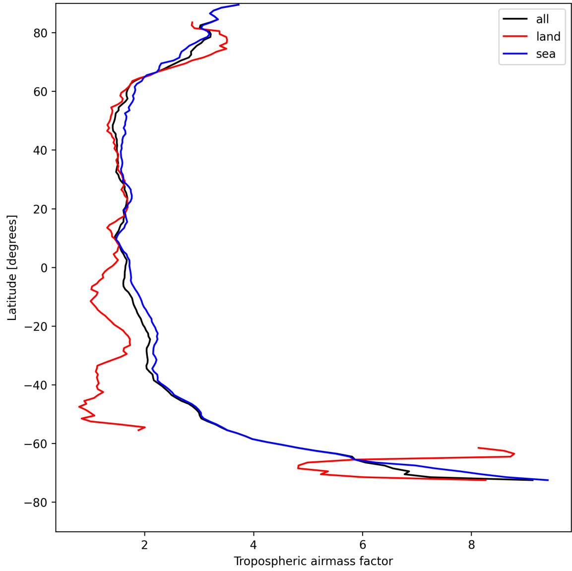
Figure 12: Zonal average of “Tropospheric airmass factor” for 2025-08-09 to 2025-08-10.
