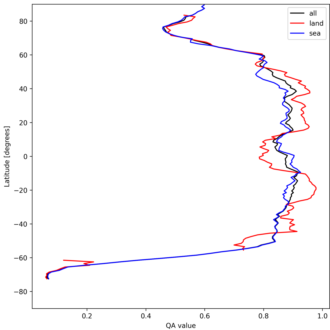
Figure 9: Zonal average of “QA value” for 2025-08-09 to 2025-08-10.
