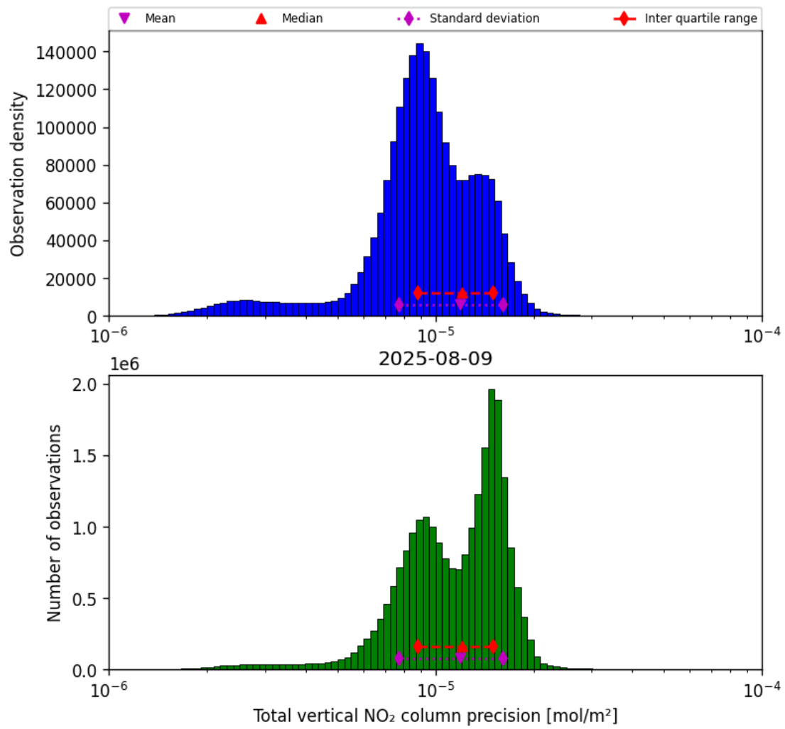
Figure 37: Histogram of “Total vertical NO 2 column precision” for 2025-08-09 to 2025-08-10
