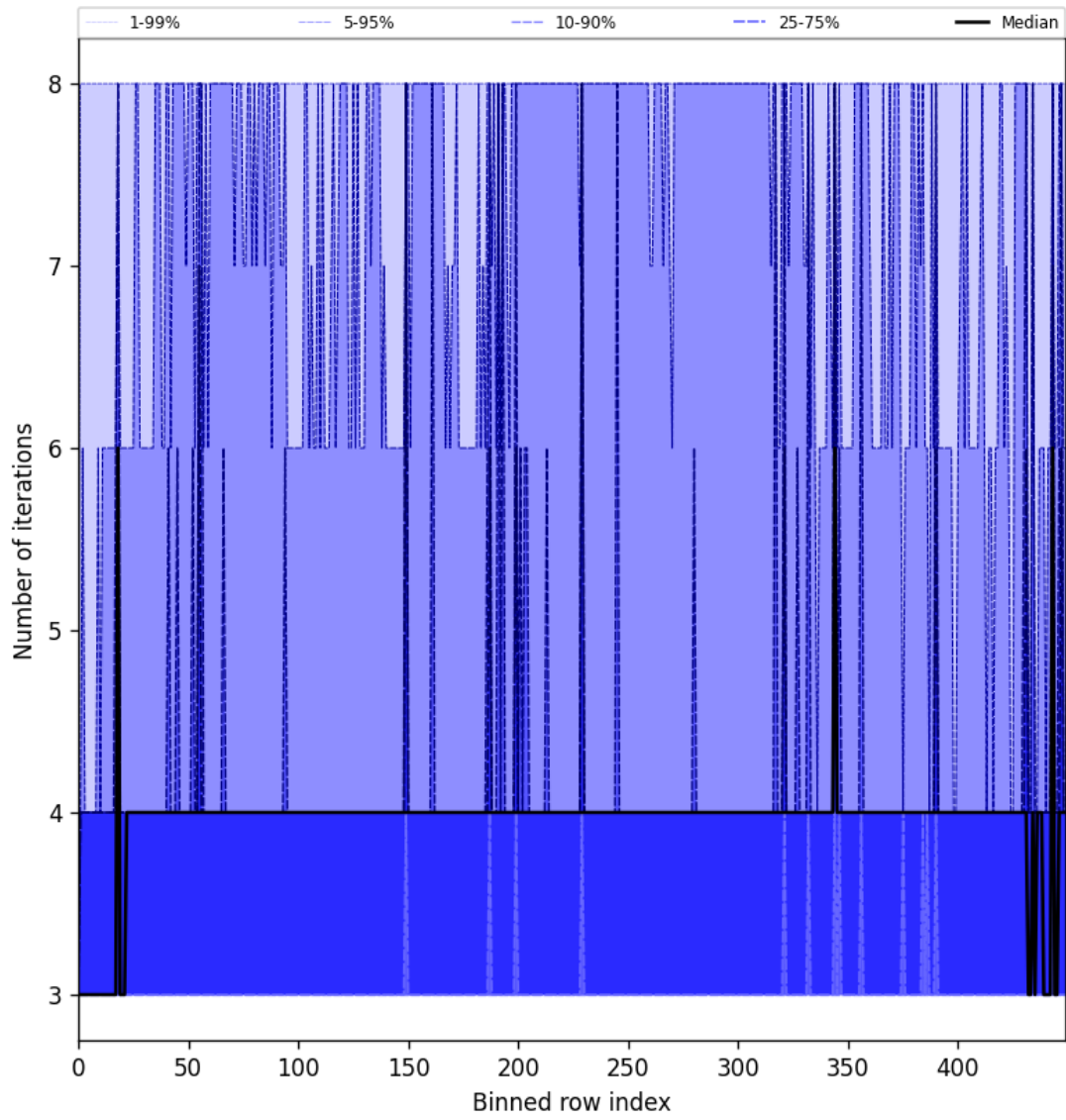
Figure 49: Along track statistics of “Number of iterations” for 2025-08-09 to 2025-08-10
