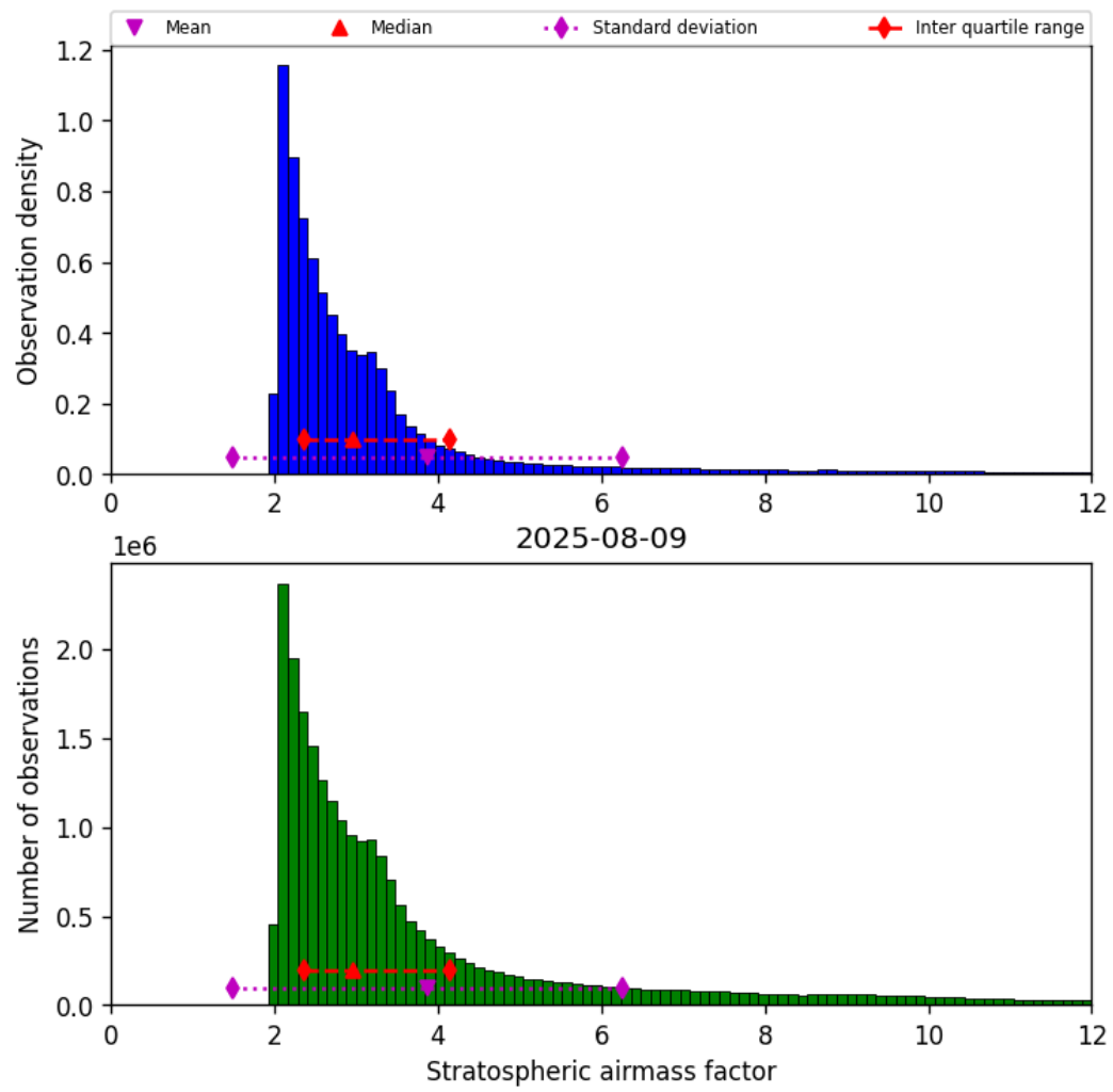
Figure 42: Histogram of “Stratospheric airmass factor” for 2025-08-09 to 2025-08-10
