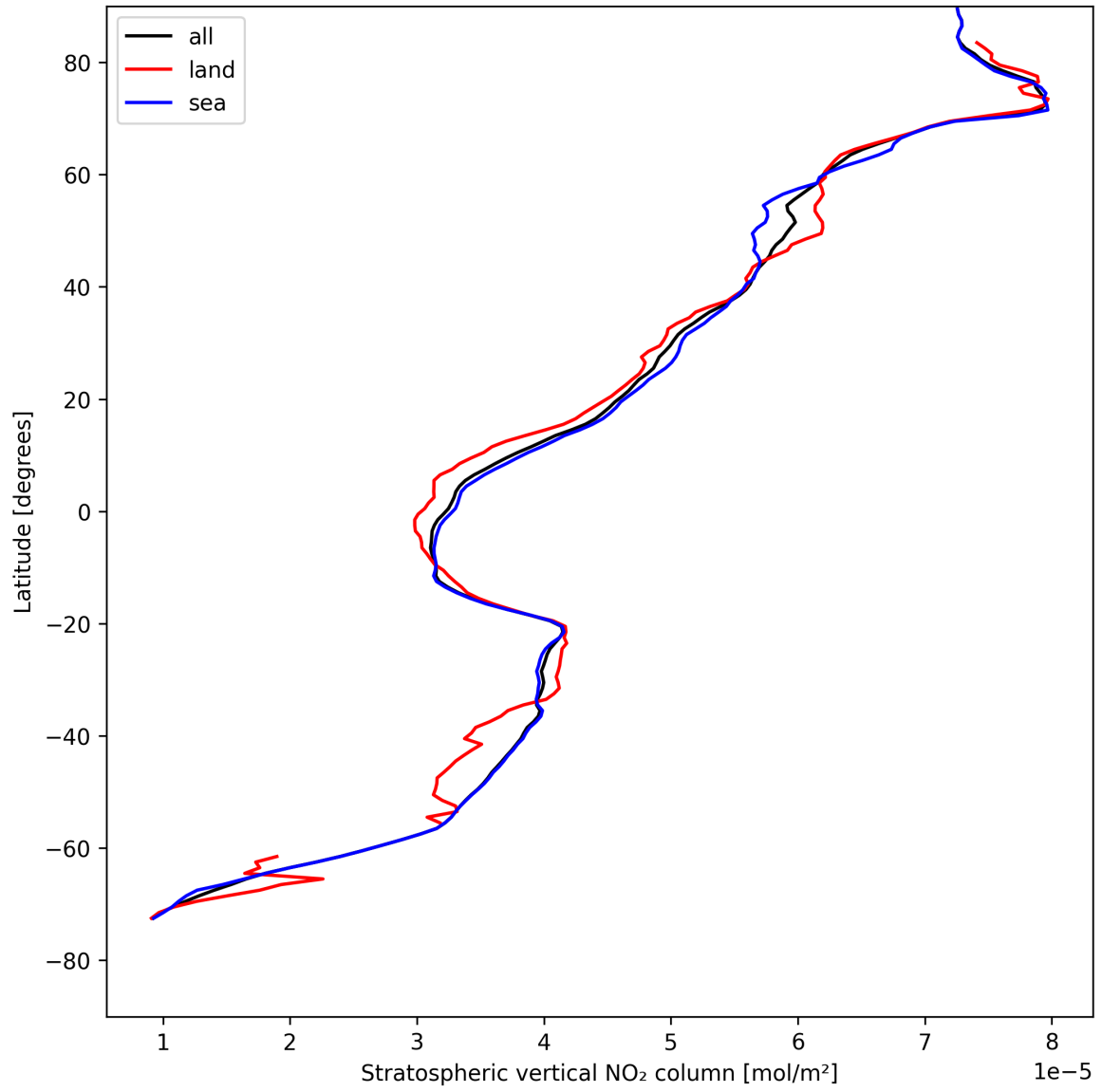
Figure 17: Zonal average of “Stratospheric vertical NO 2 column” for 2025-08-09 to 2025-08-10.
