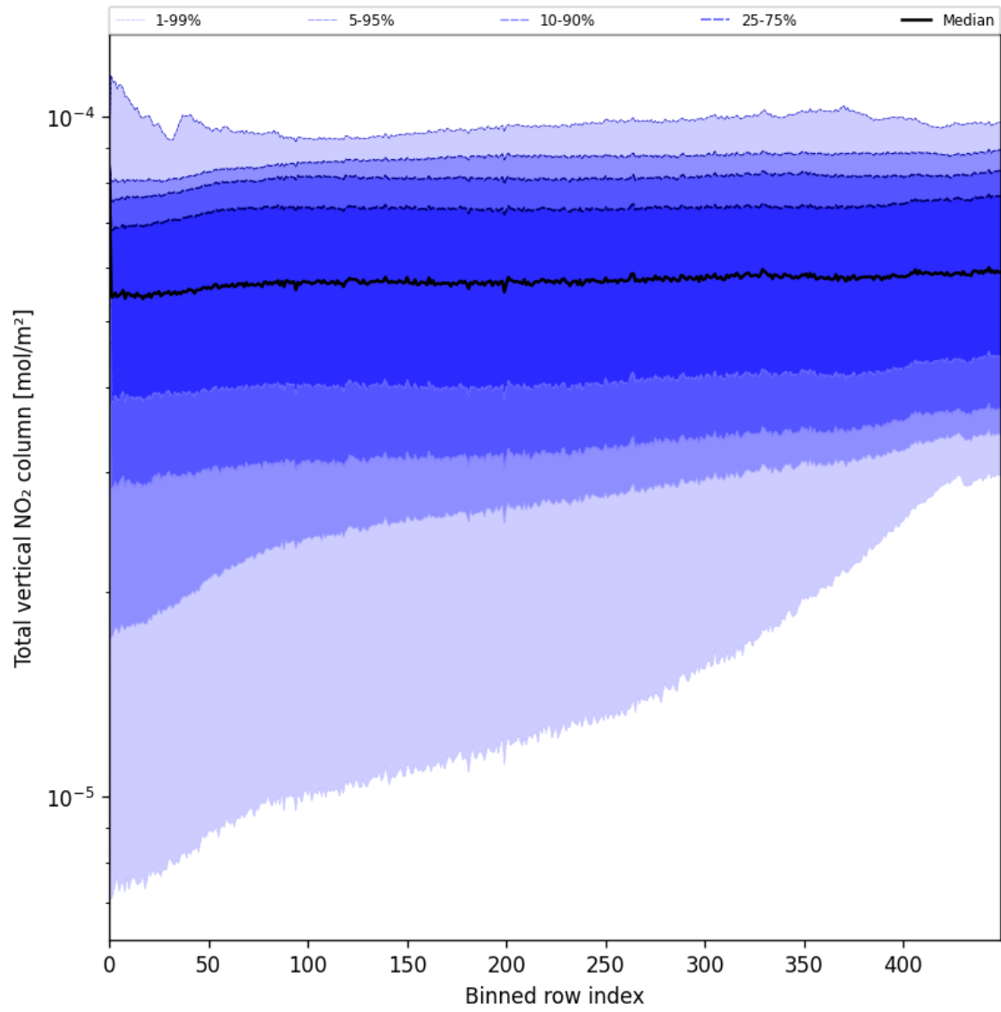
Figure 53: Along track statistics of “Total vertical NO 2 column” for 2025-08-09 to 2025-08-10
