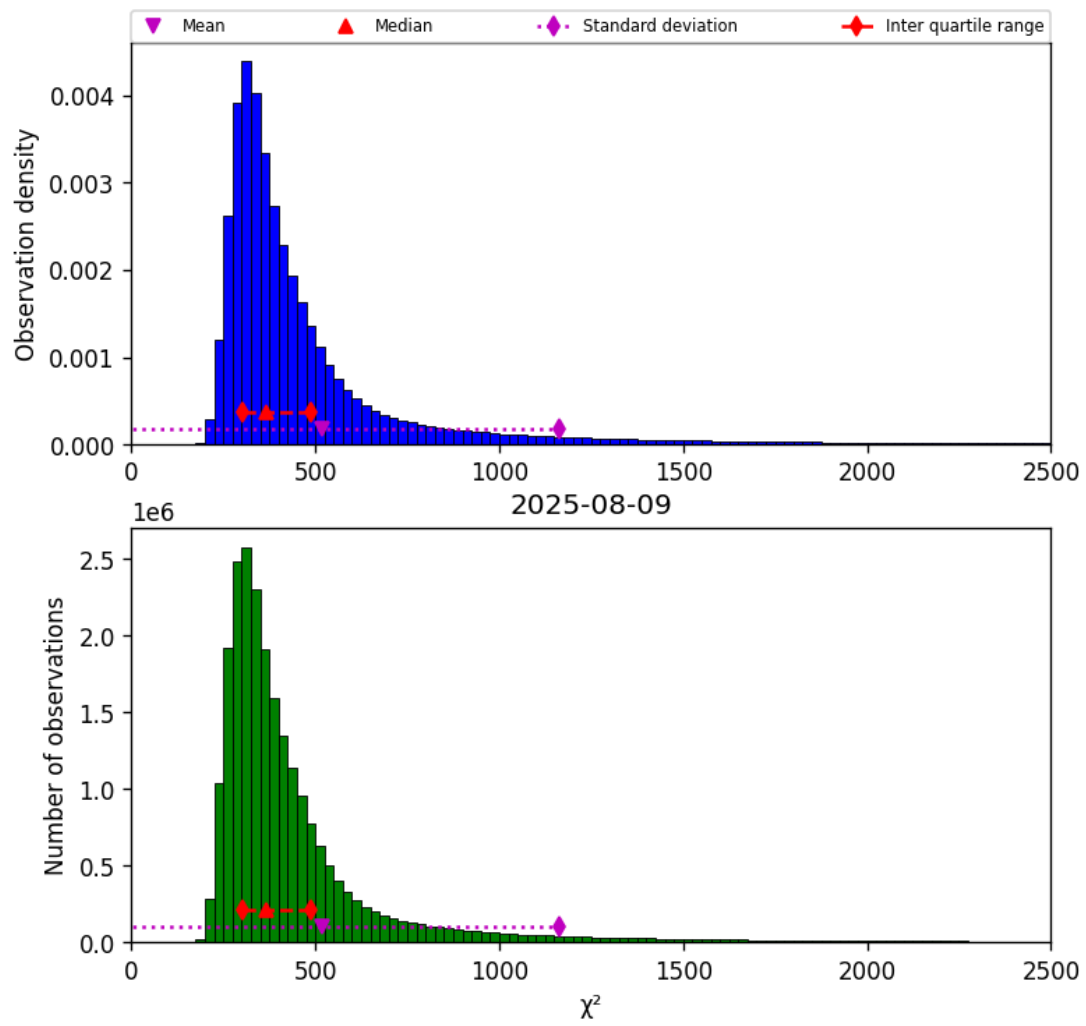
Figure 40: Histogram of “ \chi^2 ” for 2025-08-09 to 2025-08-10
