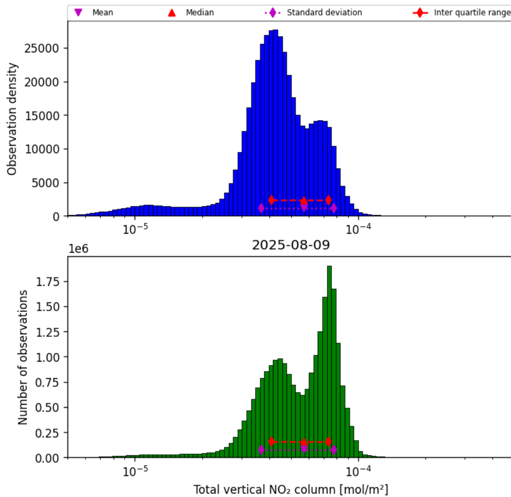
Figure 36: Histogram of “Total vertical NO 2 column” for 2025-08-09 to 2025-08-10
