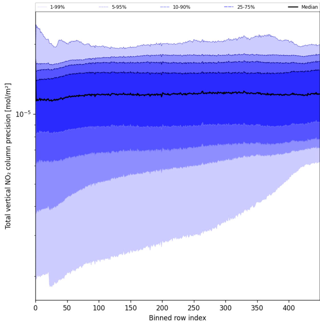
Figure 54: Along track statistics of “Total vertical NO 2 column precision” for 2025-08-09 to 2025-08-10
