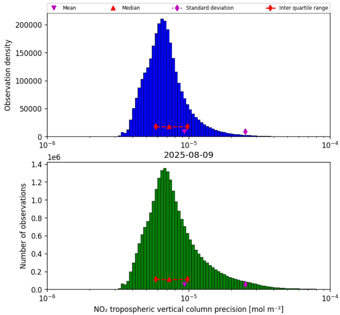
Figure 28: Histogram of “NO 2 tropospheric vertical column precision” for 2025-08-09 to 2025-08-10
