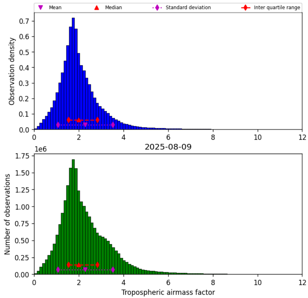
Figure 29: Histogram of “Tropospheric airmass factor” for 2025-08-09 to 2025-08-10
