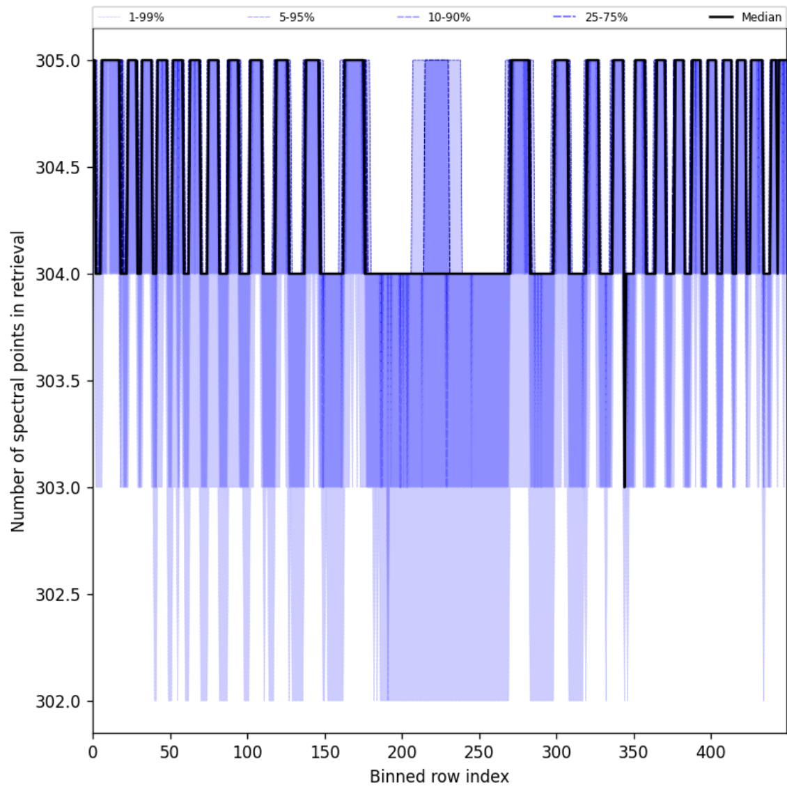
Figure 48: Along track statistics of “Number of spectral points in retrieval” for 2025-08-09 to 2025-08-10
