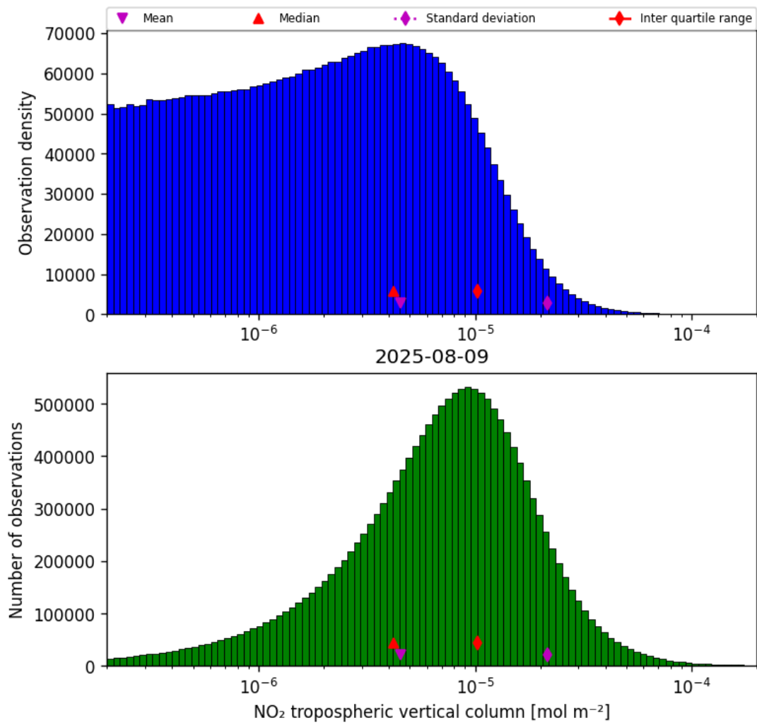
Figure 27: Histogram of “NO 2 tropospheric vertical column” for 2025-08-09 to 2025-08-10
