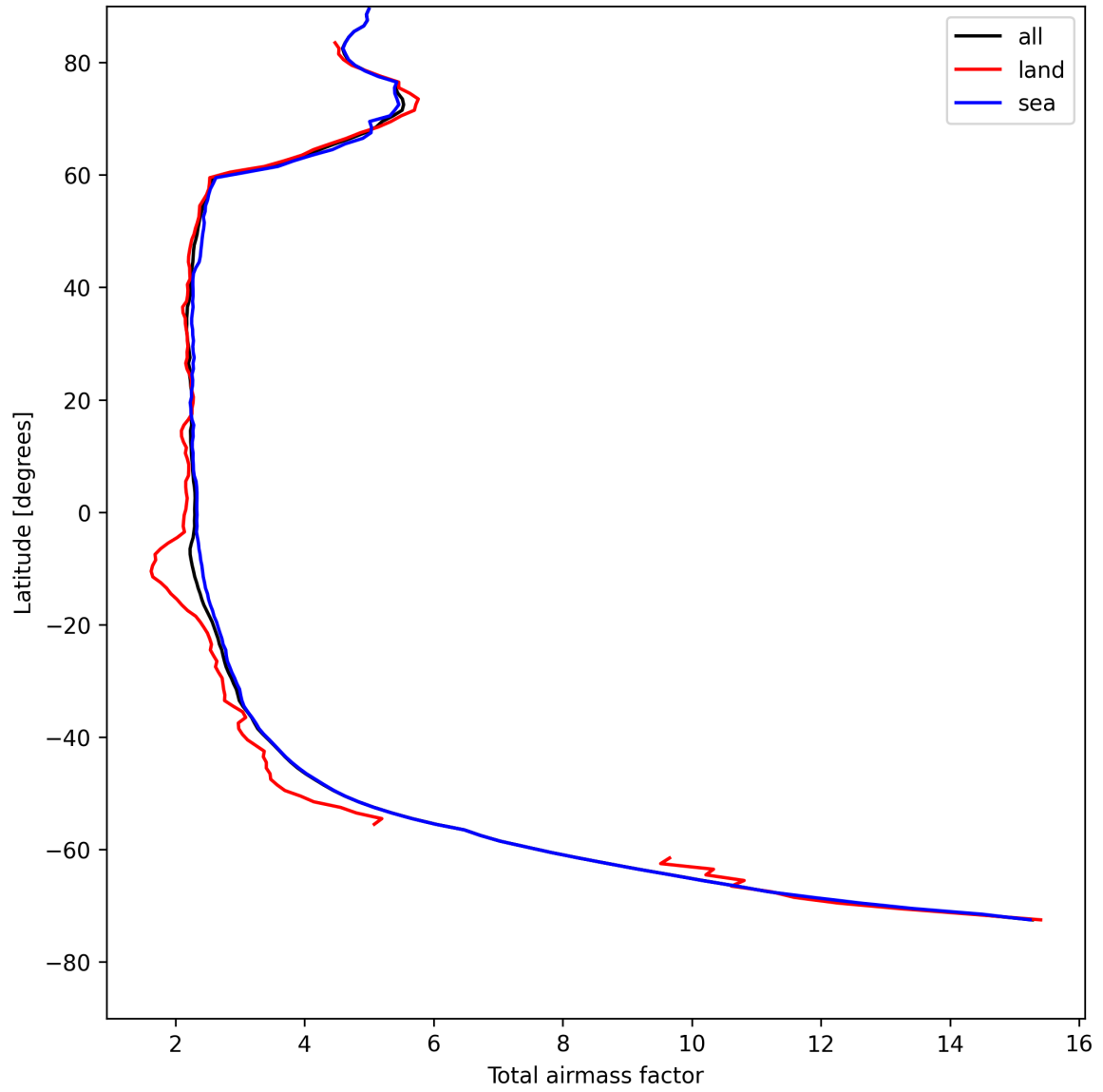
Figure 13: Zonal average of “Total airmass factor” for 2025-08-09 to 2025-08-10.
