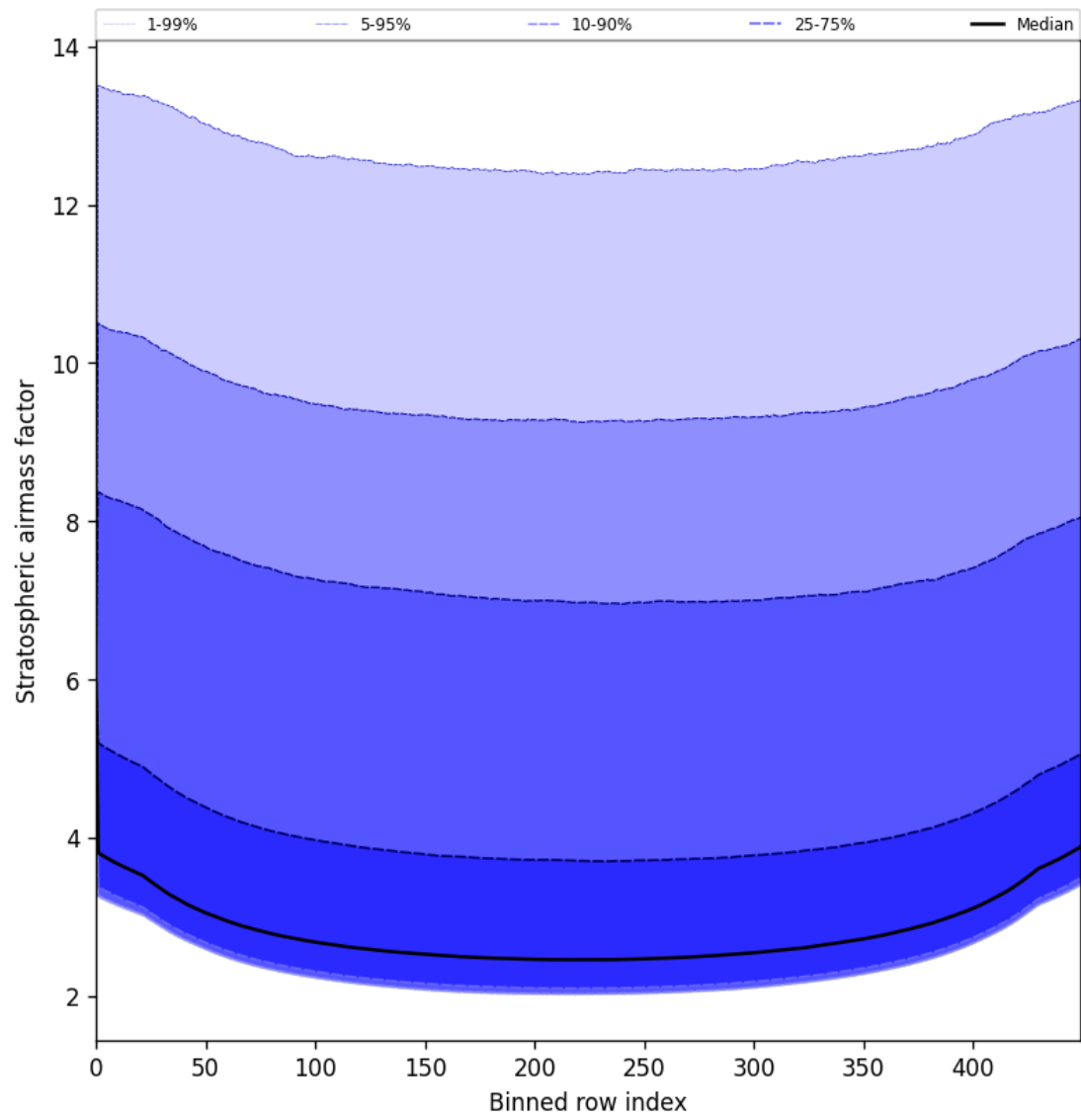
Figure 59: Along track statistics of “Stratospheric airmass factor” for 2025-08-09 to 2025-08-10
