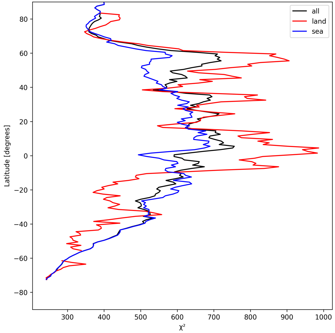
Figure 23: Zonal average of “ \chi^2 ” for 2025-08-09 to 2025-08-10.
