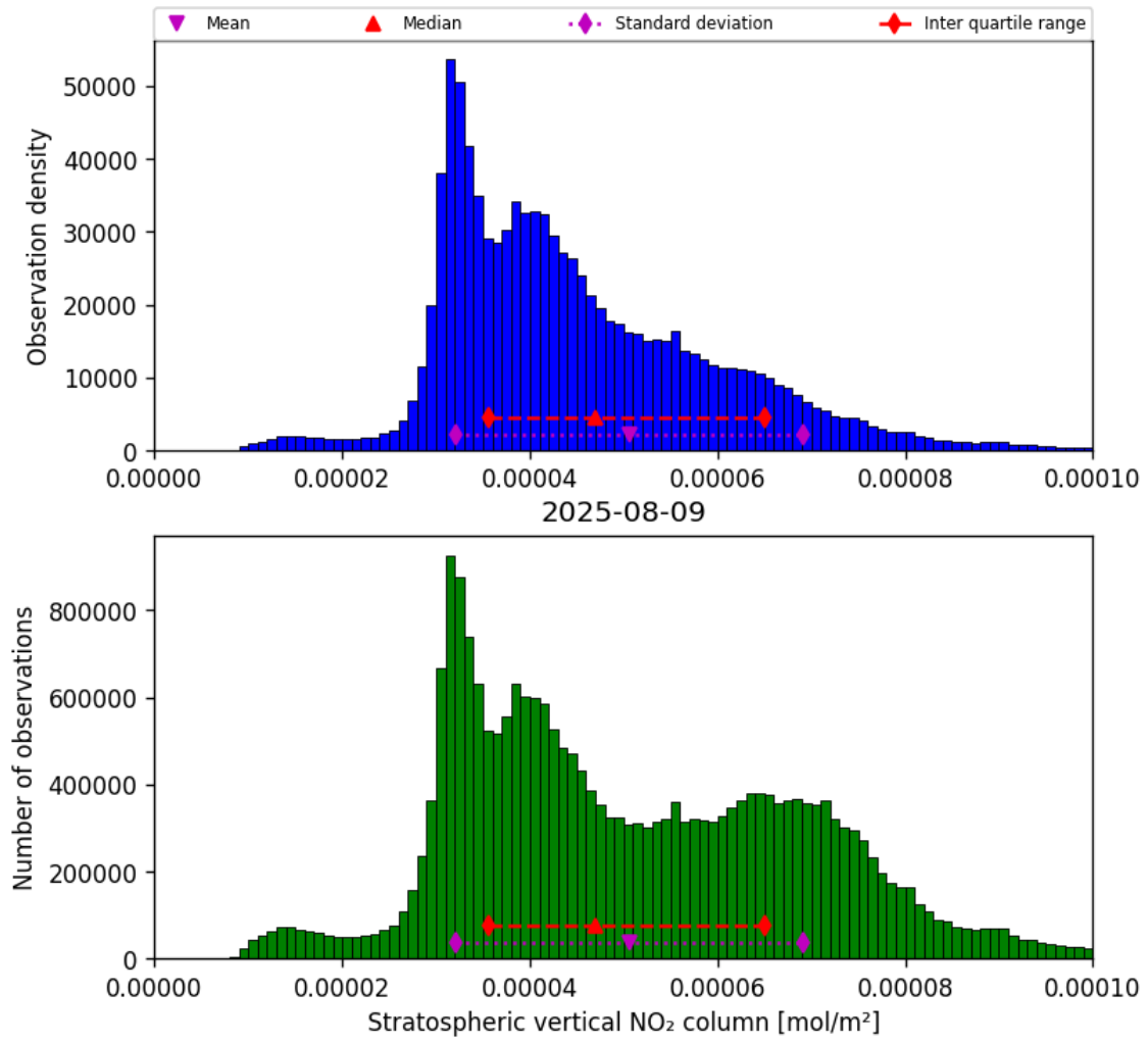
Figure 34: Histogram of “Stratospheric vertical NO 2 column” for 2025-08-09 to 2025-08-10
