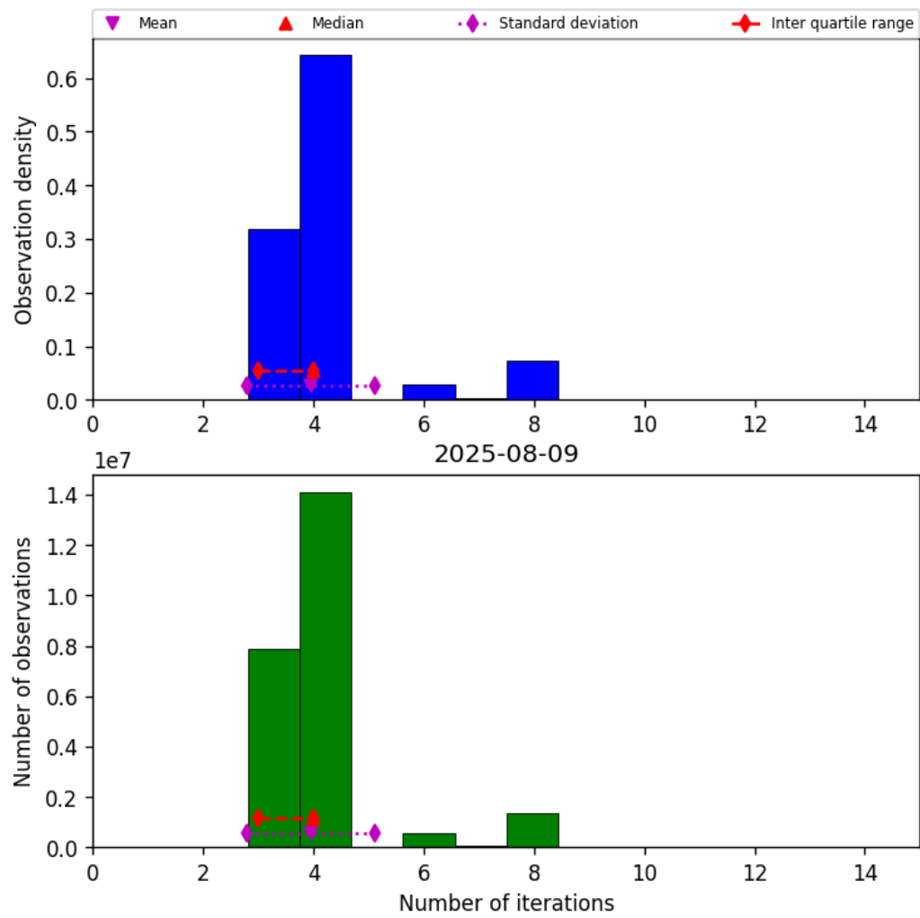
Figure 32: Histogram of “Number of iterations” for 2025-08-09 to 2025-08-10
