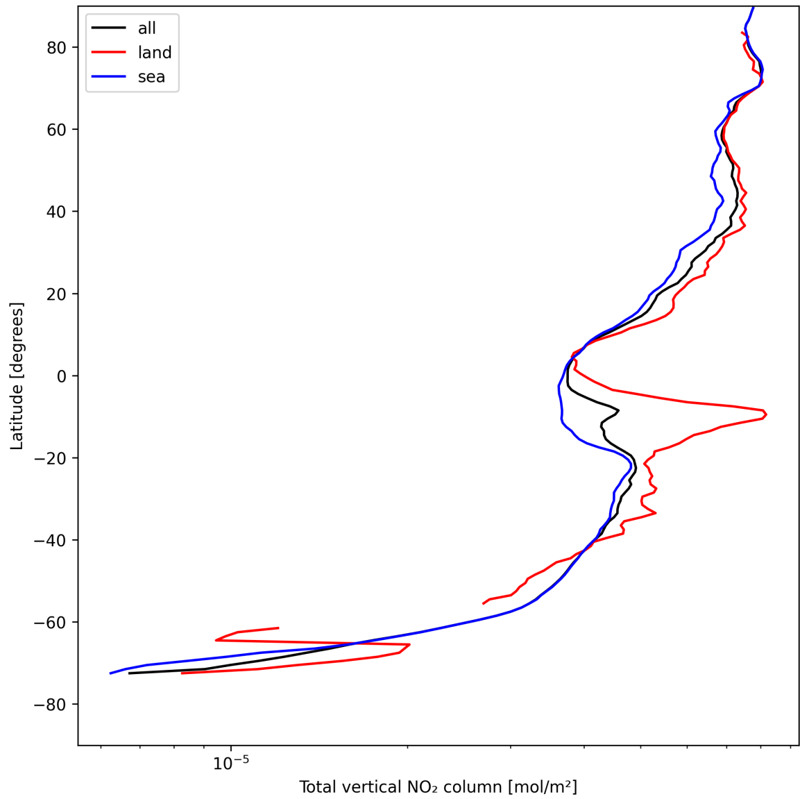
Figure 19: Zonal average of “Total vertical NO 2 column” for 2025-08-09 to 2025-08-10.
