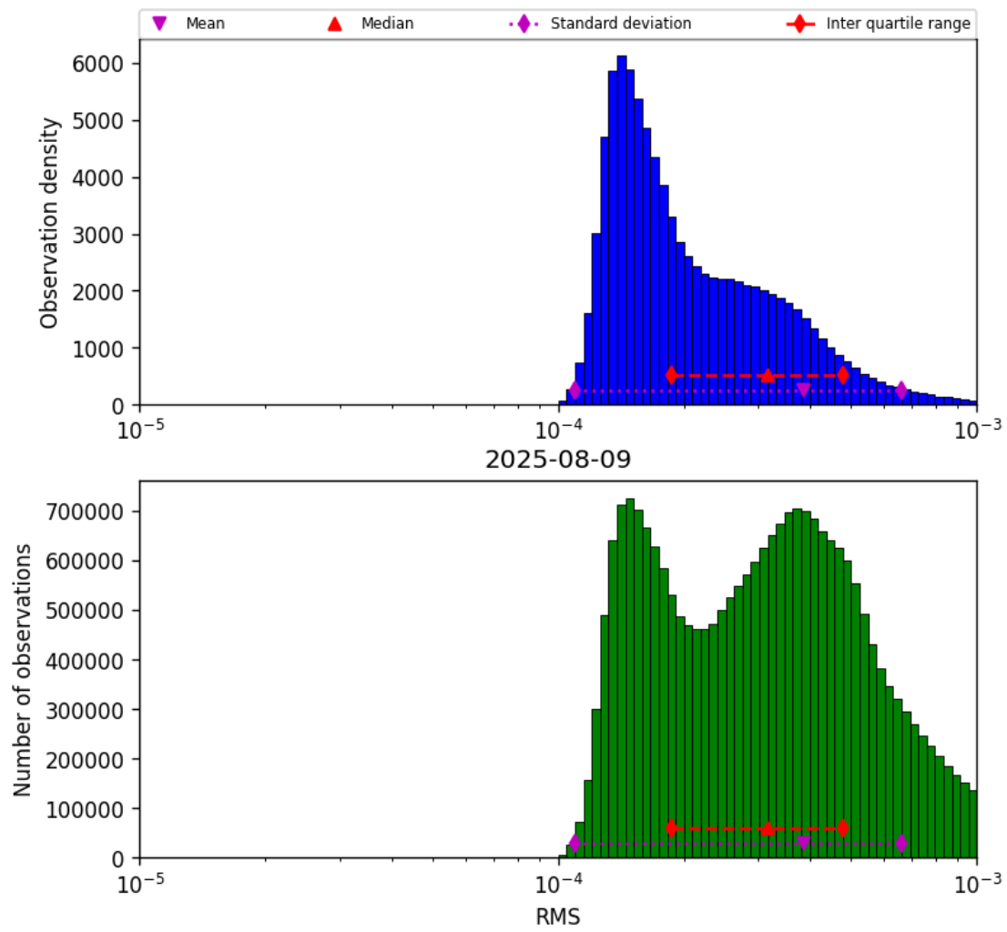
Figure 41: Histogram of “RMS” for 2025-08-09 to 2025-08-10
