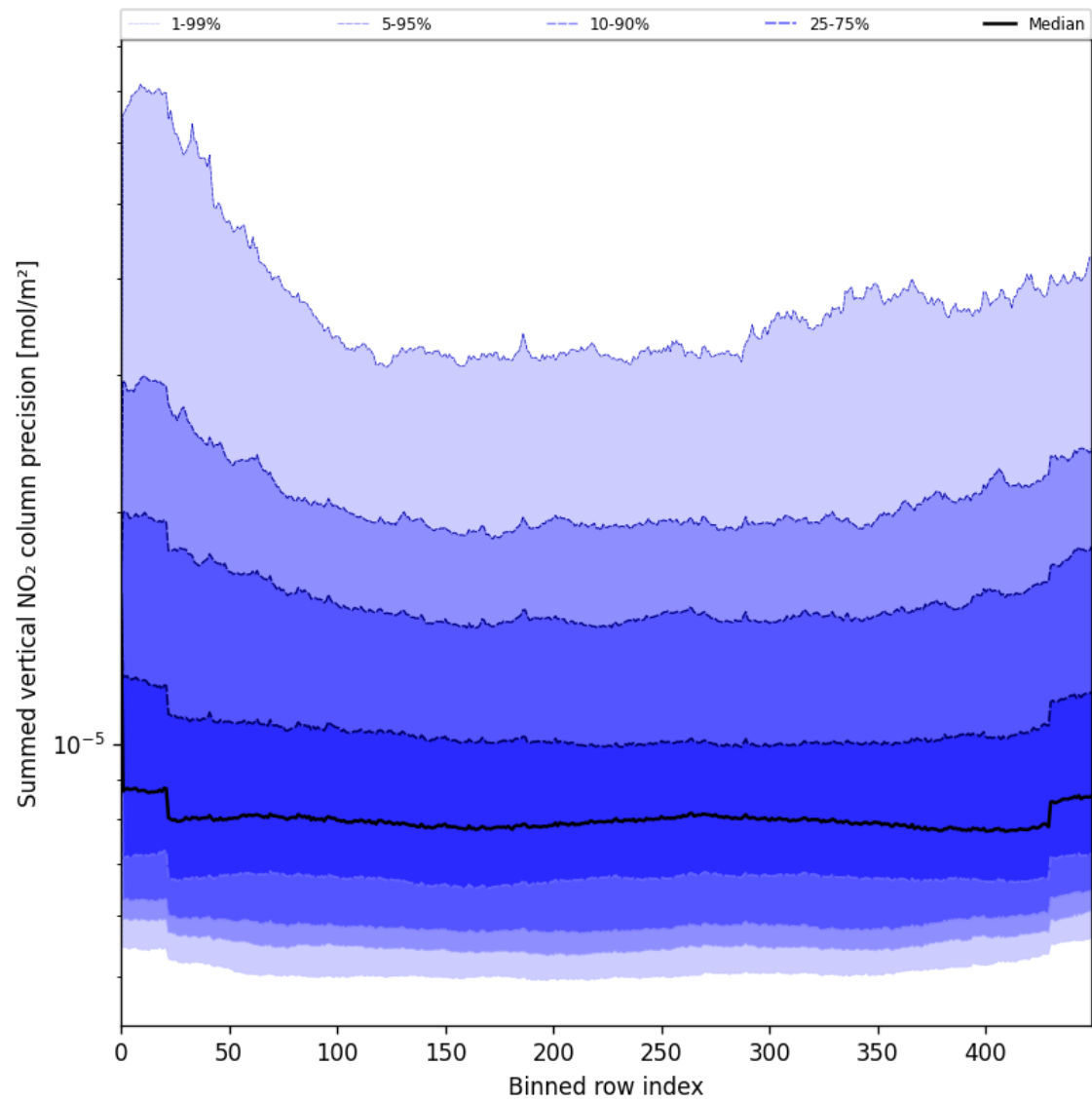
Figure 56: Along track statistics of “Summed vertical NO 2 column precision” for 2025-08-09 to 2025-08-10
