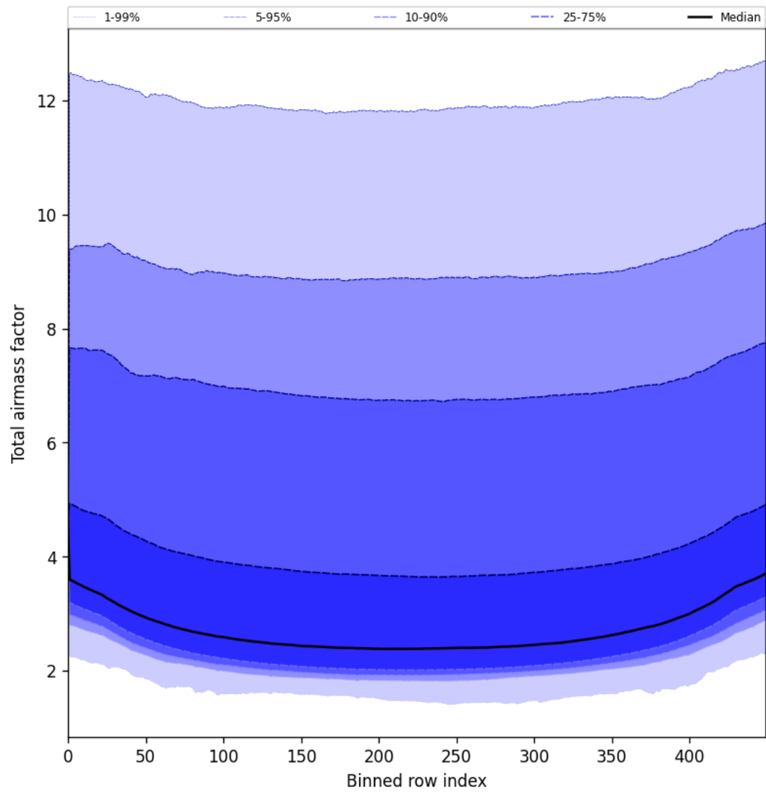
Figure 47: Along track statistics of “Total airmass factor” for 2025-08-09 to 2025-08-10
