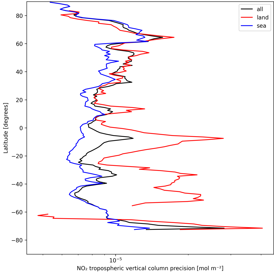
Figure 11: Zonal average of “NO 2 tropospheric vertical column precision” for 2025-08-09 to 2025-08-10.
