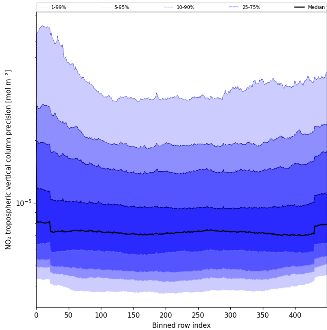
Figure 45: Along track statistics of “NO 2 tropospheric vertical column precision” for 2025-08-09 to 2025-08-10
