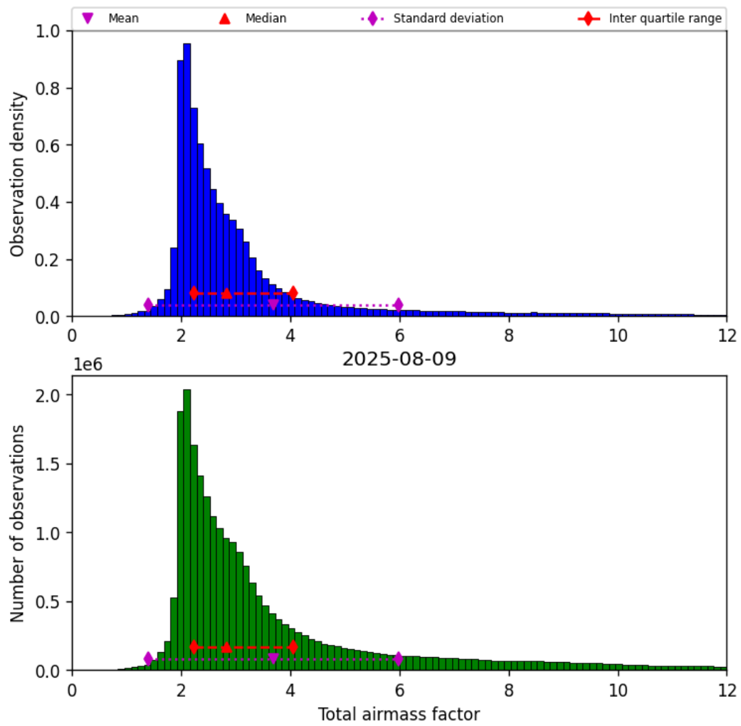
Figure 30: Histogram of “Total airmass factor” for 2025-08-09 to 2025-08-10
