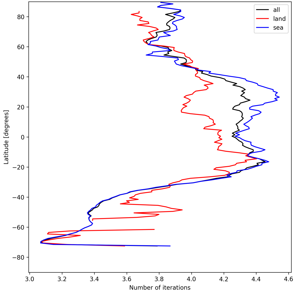
Figure 15: Zonal average of “Number of iterations” for 2025-08-09 to 2025-08-10.
