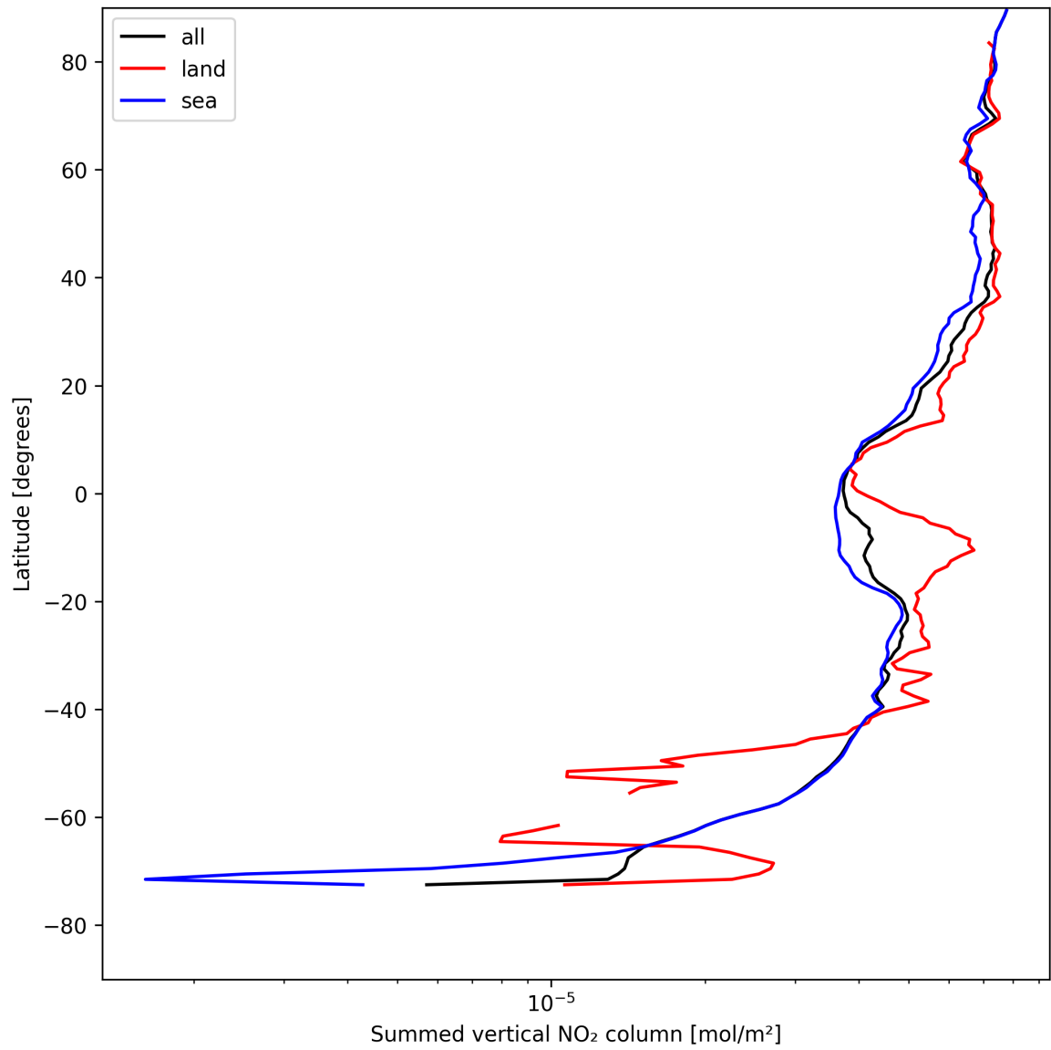
Figure 21: Zonal average of “Summed vertical NO 2 column” for 2025-08-09 to 2025-08-10.
