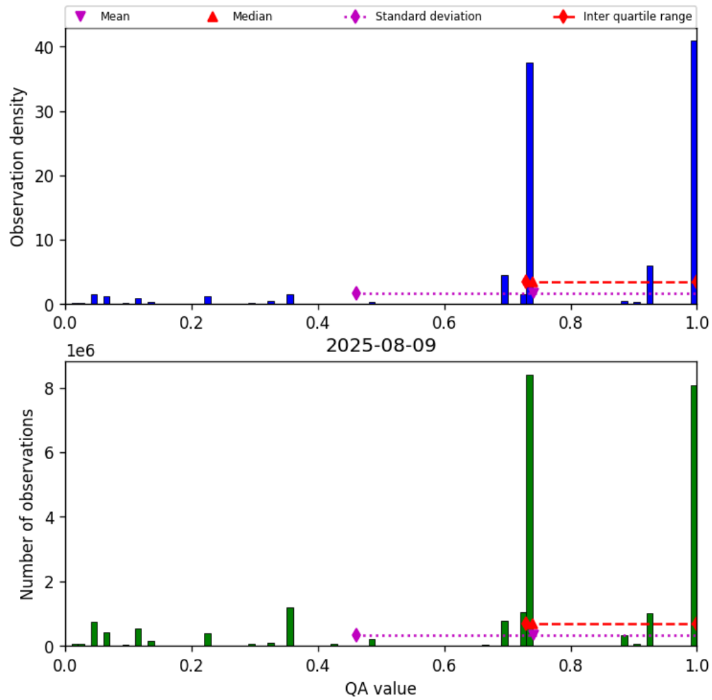
Figure 26: Histogram of “QA value” for 2025-08-09 to 2025-08-10
