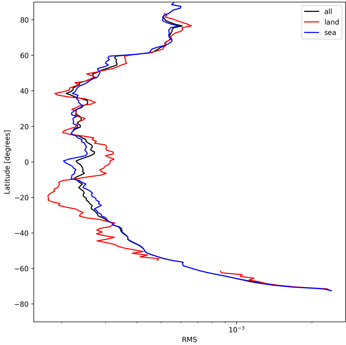
Figure 24: Zonal average of “RMS” for 2025-08-09 to 2025-08-10.
