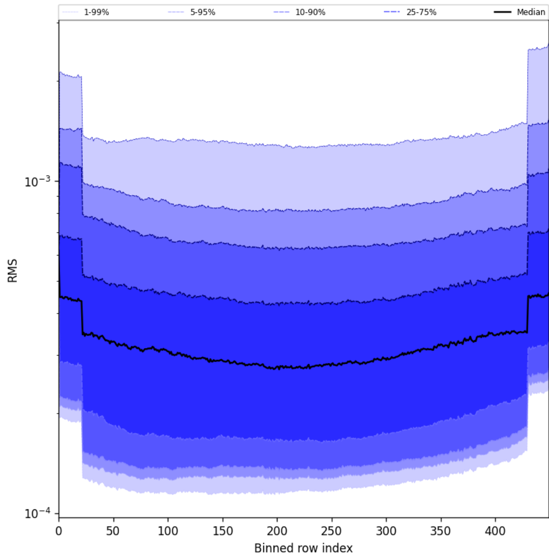
Figure 58: Along track statistics of “RMS” for 2025-08-09 to 2025-08-10
