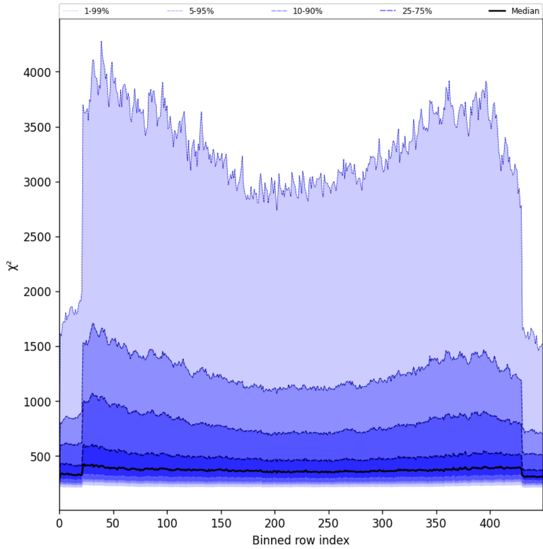
Figure 57: Along track statistics of “ \chi^2 ” for 2025-08-09 to 2025-08-10
