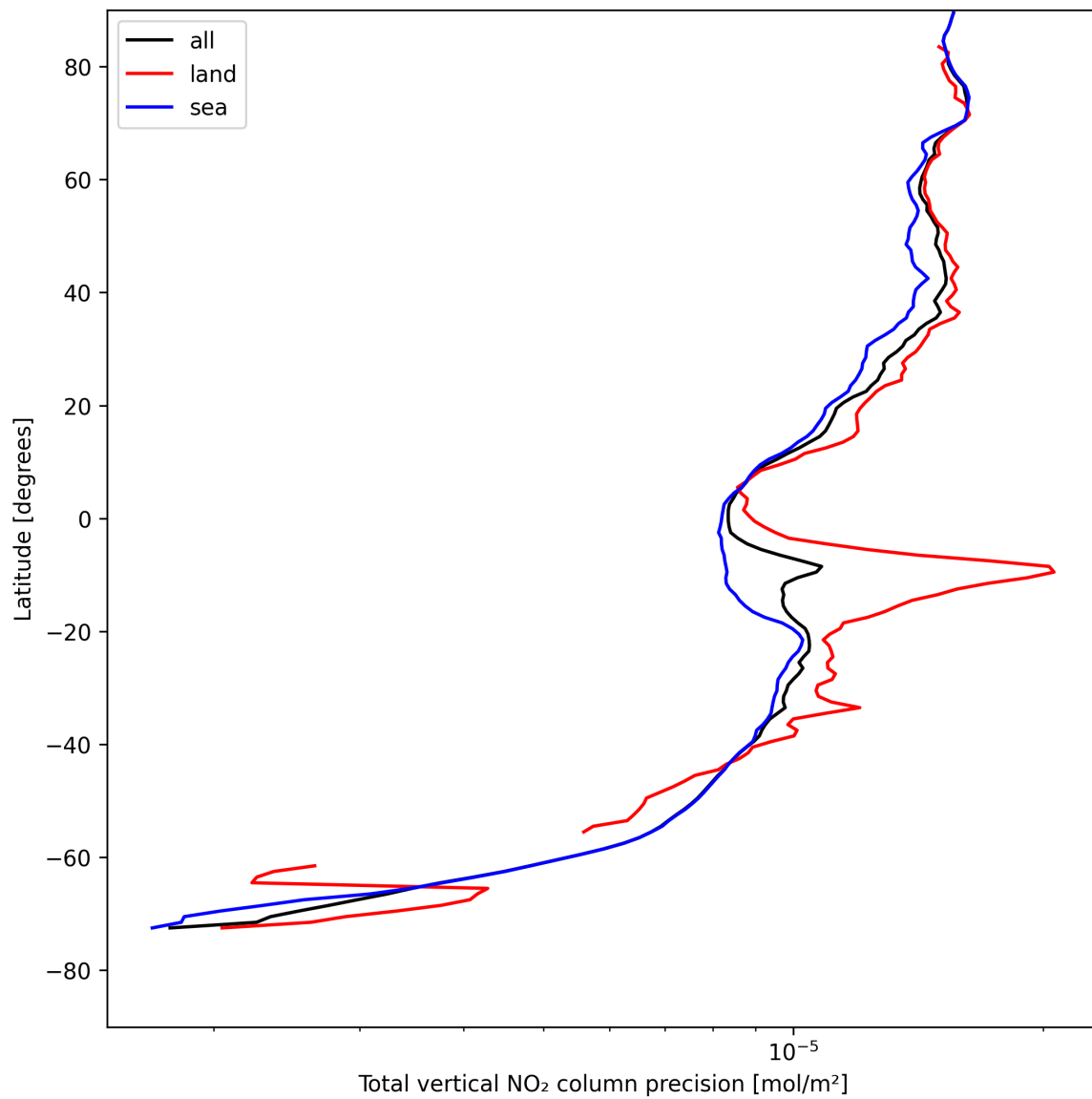
Figure 20: Zonal average of “Total vertical NO 2 column precision” for 2025-08-09 to 2025-08-10.
