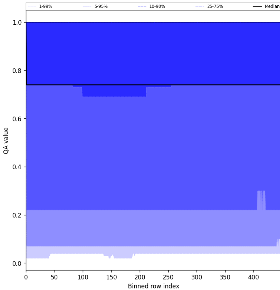
Figure 43: Along track statistics of “QA value” for 2025-08-09 to 2025-08-10
