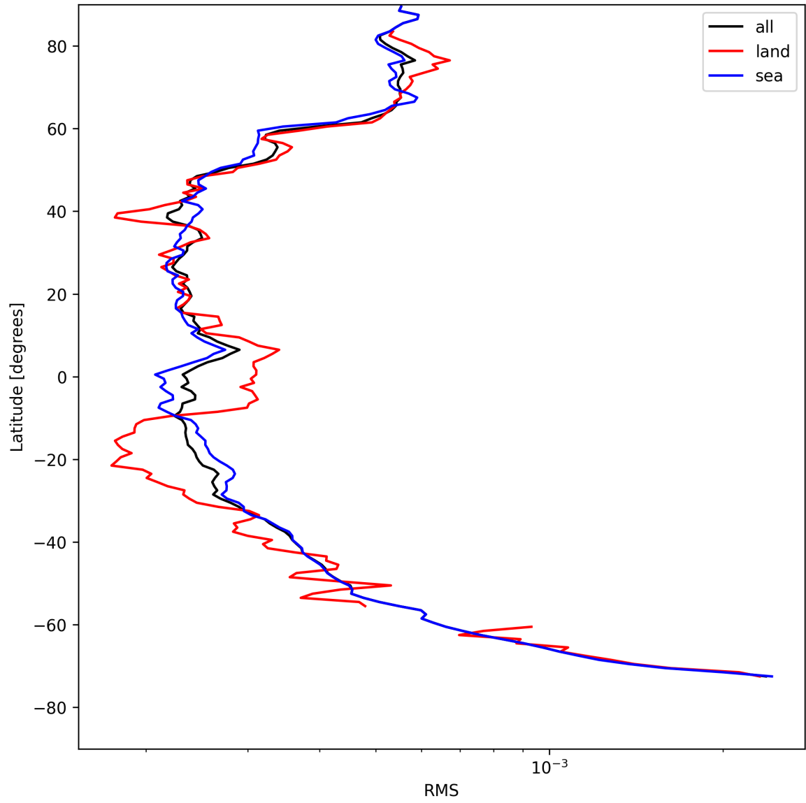
Figure 24: Zonal average of “RMS” for 2025-08-10 to 2025-08-11.
