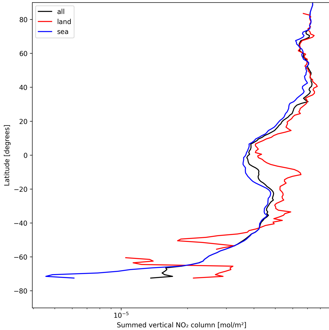
Figure 21: Zonal average of “Summed vertical NO 2 column” for 2025-08-10 to 2025-08-11.
