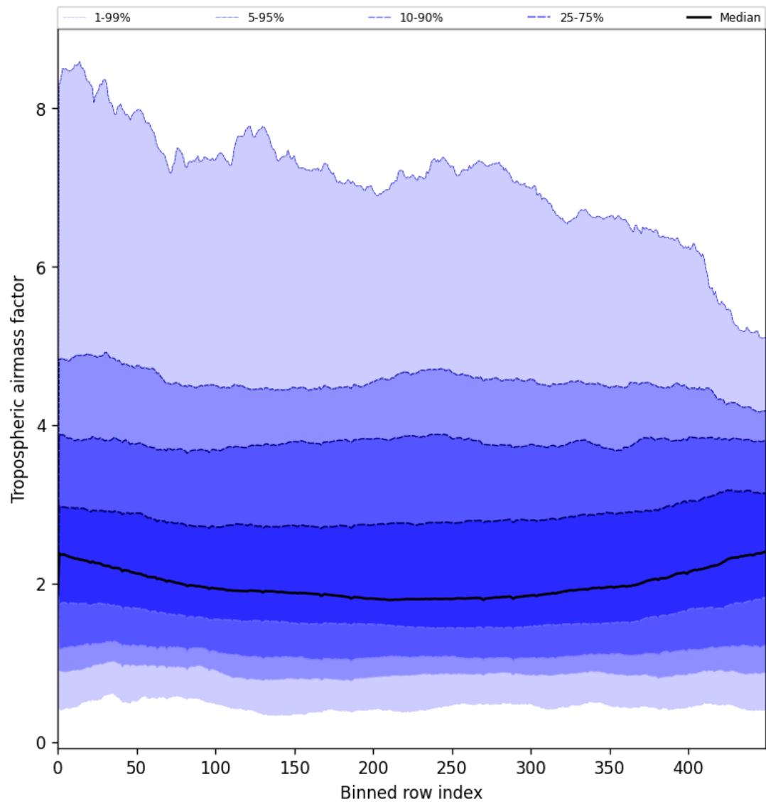
Figure 46: Along track statistics of “Tropospheric airmass factor” for 2025-08-10 to 2025-08-11
