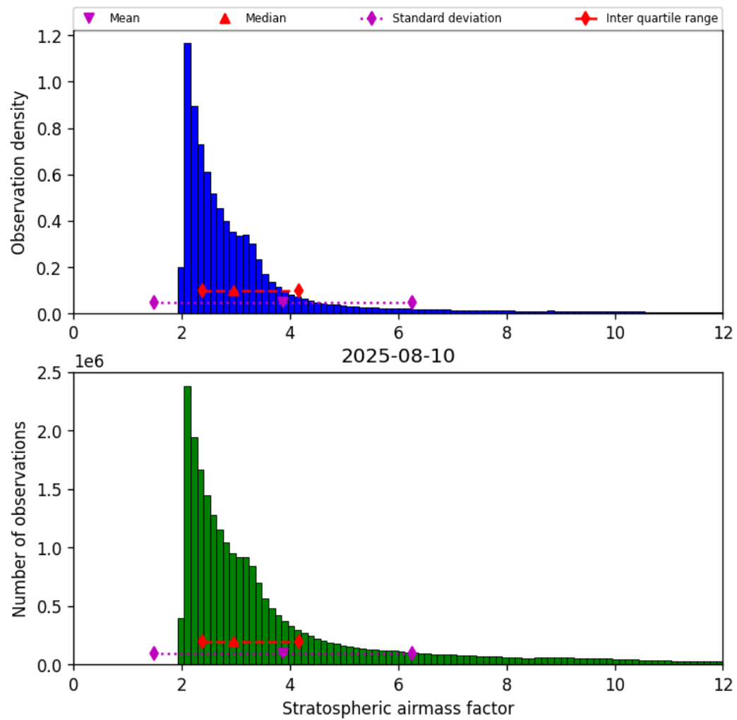
Figure 42: Histogram of “Stratospheric airmass factor” for 2025-08-10 to 2025-08-11
