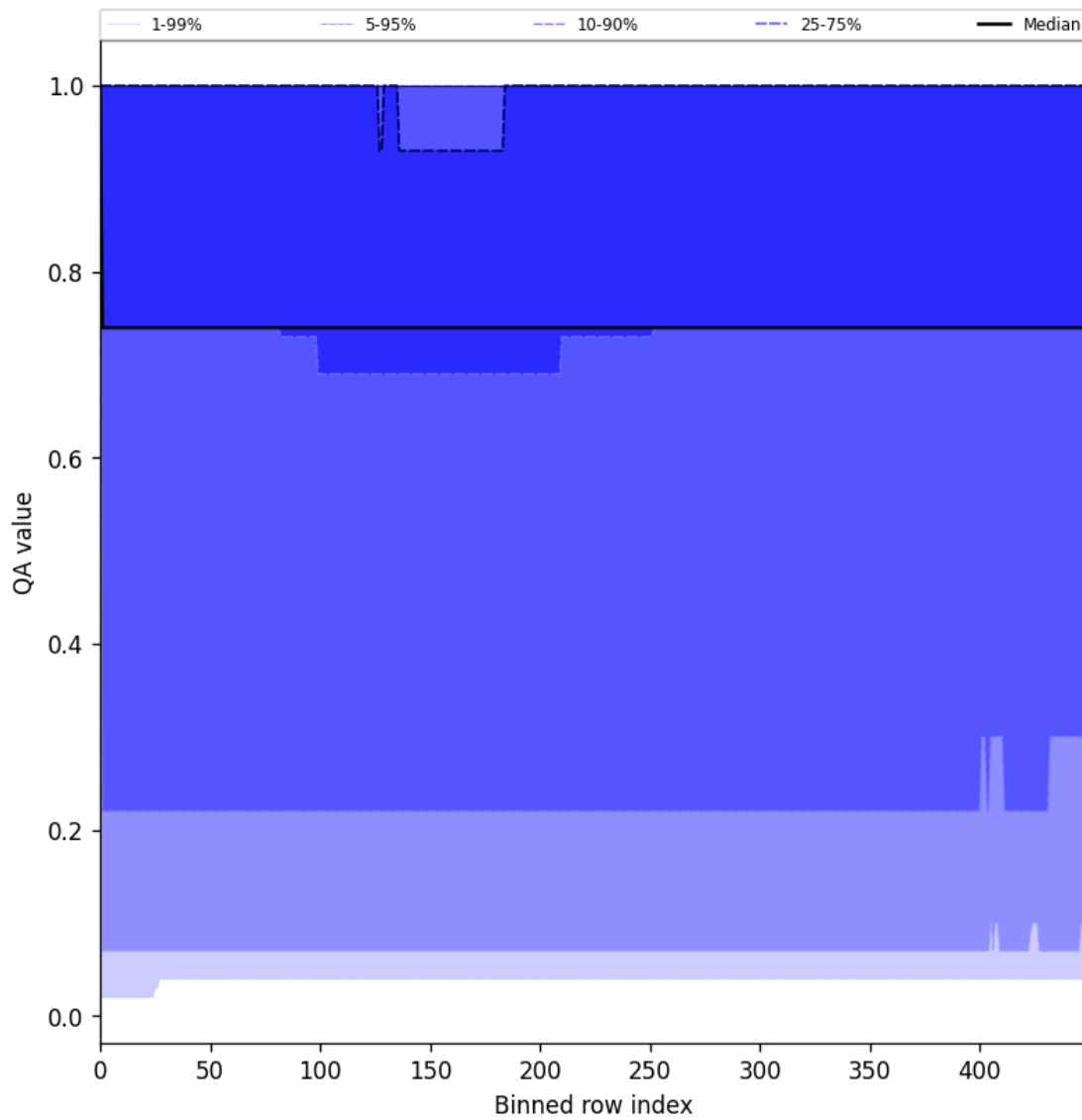
Figure 43: Along track statistics of “QA value” for 2025-08-10 to 2025-08-11
