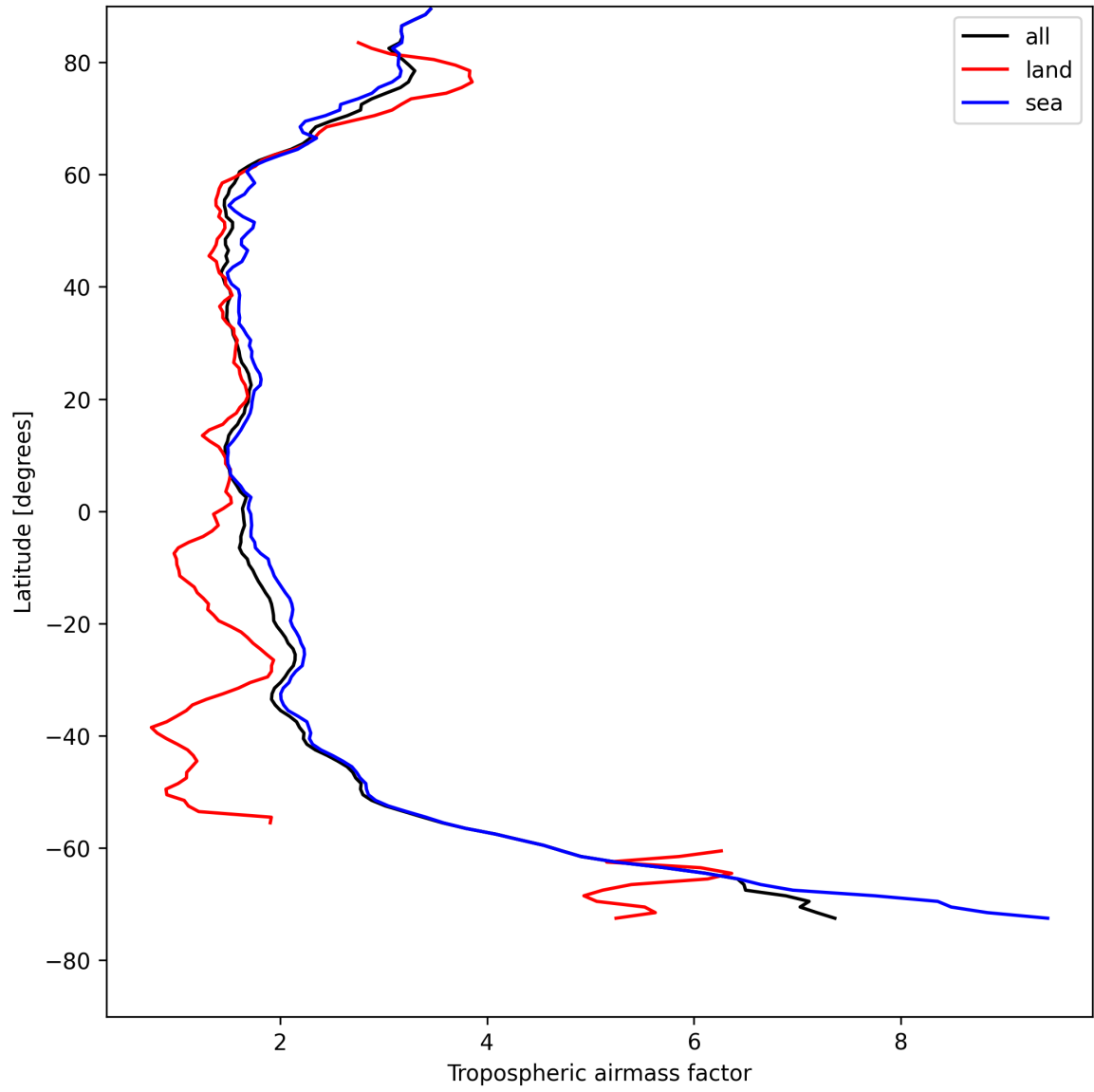
Figure 12: Zonal average of “Tropospheric air mass factor” for 2025-08-10 to 2025-08-11.
