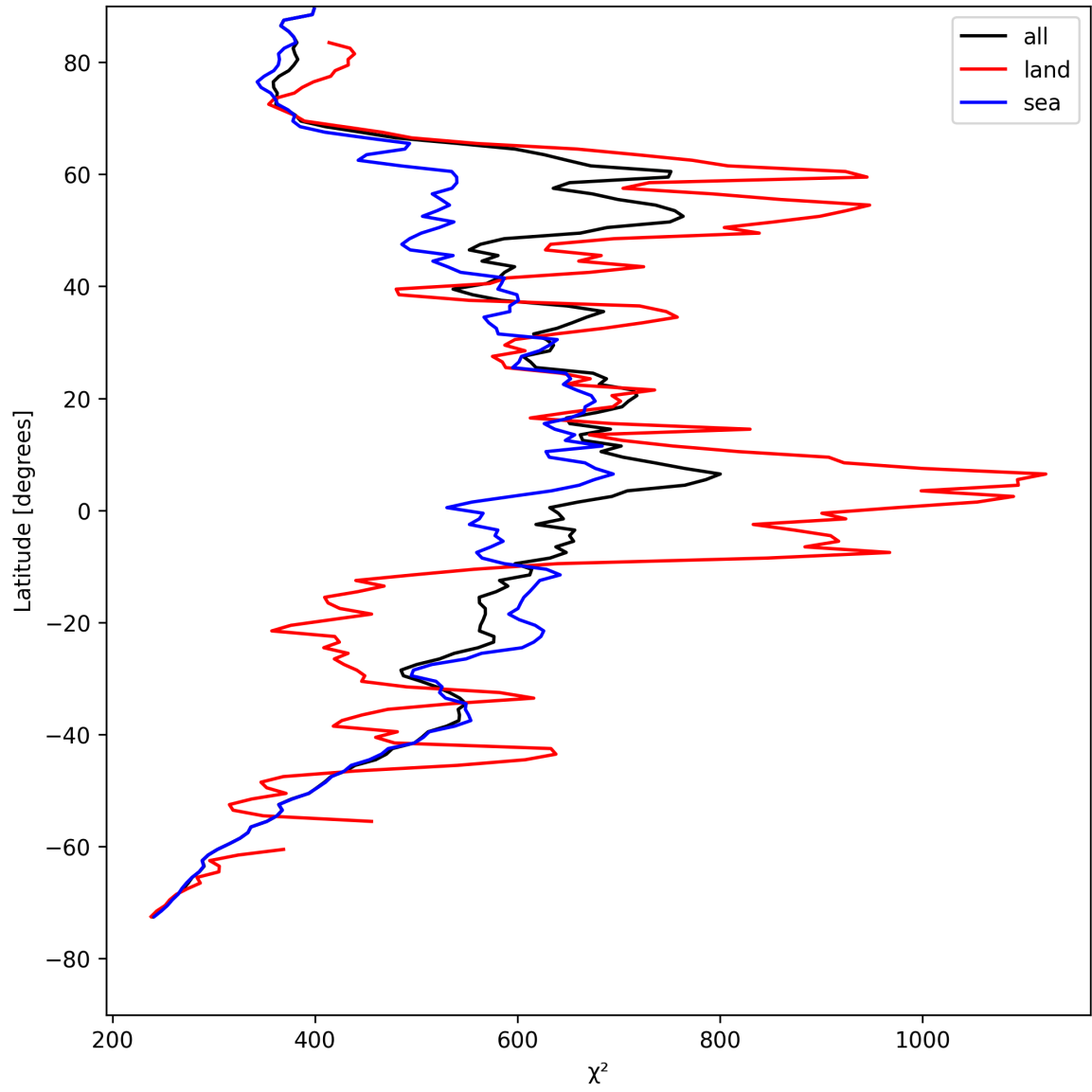
Figure 23: Zonal average of “ \chi^2 ” for 2025-08-10 to 2025-08-11.
