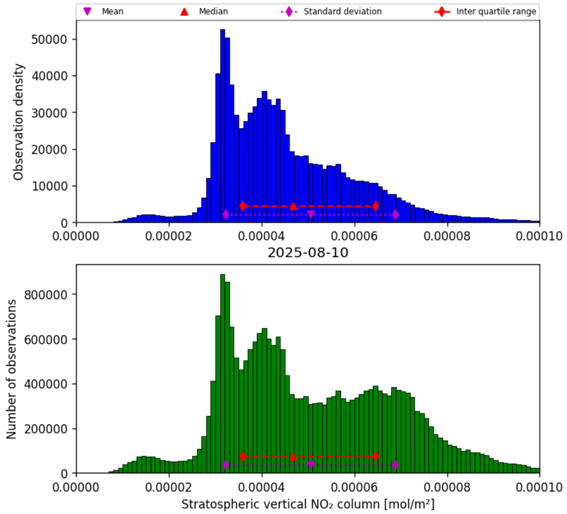
Figure 34: Histogram of “Stratospheric vertical NO 2 column” for 2025-08-10 to 2025-08-11
