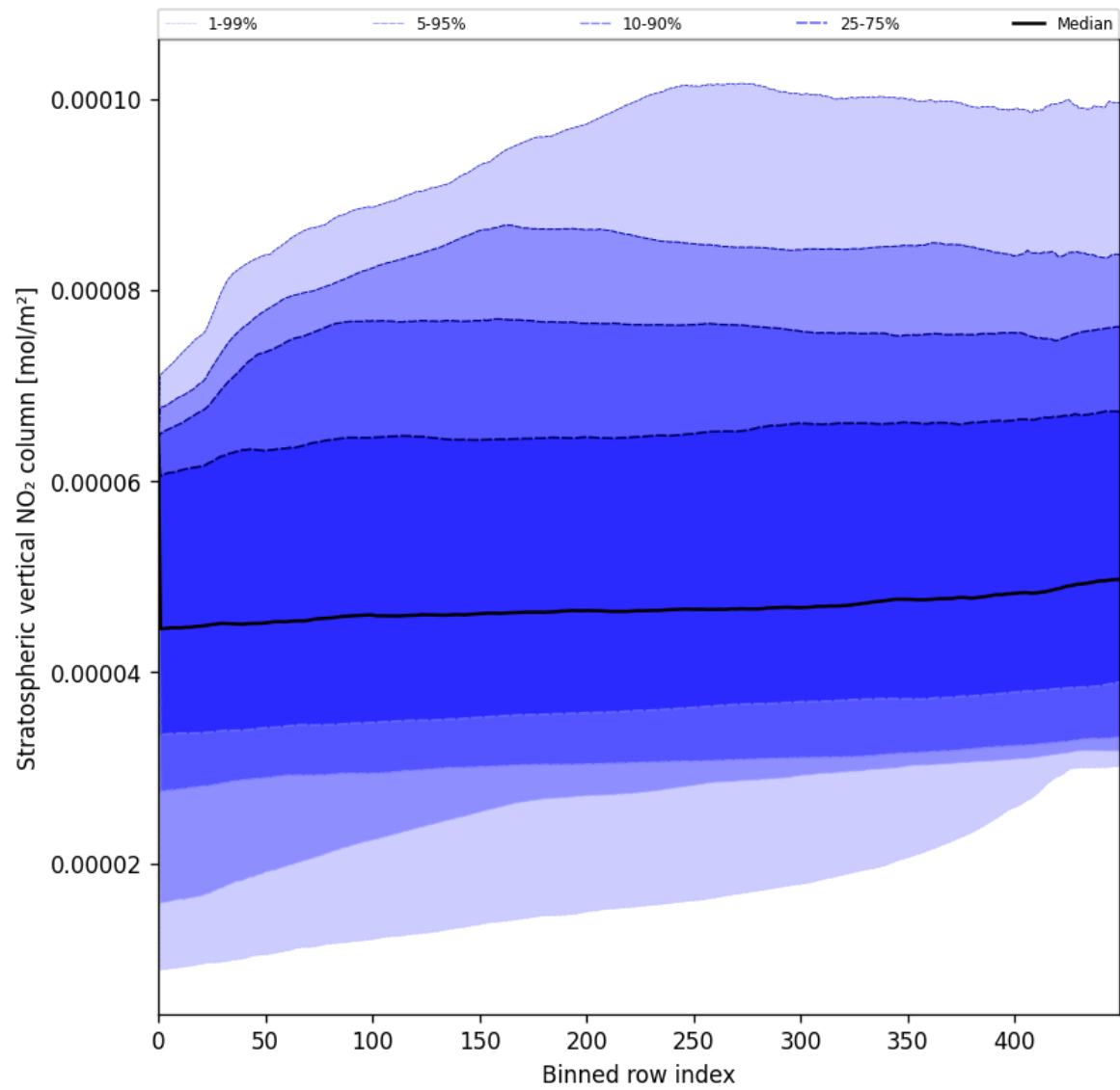
Figure 51: Along track statistics of "Stratospheric vertical NO 2 column" for 2025-08-10 to 2025-08-11
