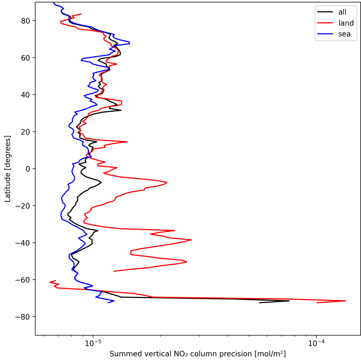
Figure 22: Zonal average of “Summed vertical NO 2 column precision” for 2025-08-10 to 2025-08-11.
