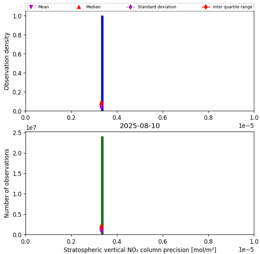
Figure 35: Histogram of “Stratospheric vertical NO 2 column precision” for 2025-08-10 to 2025-08-11
