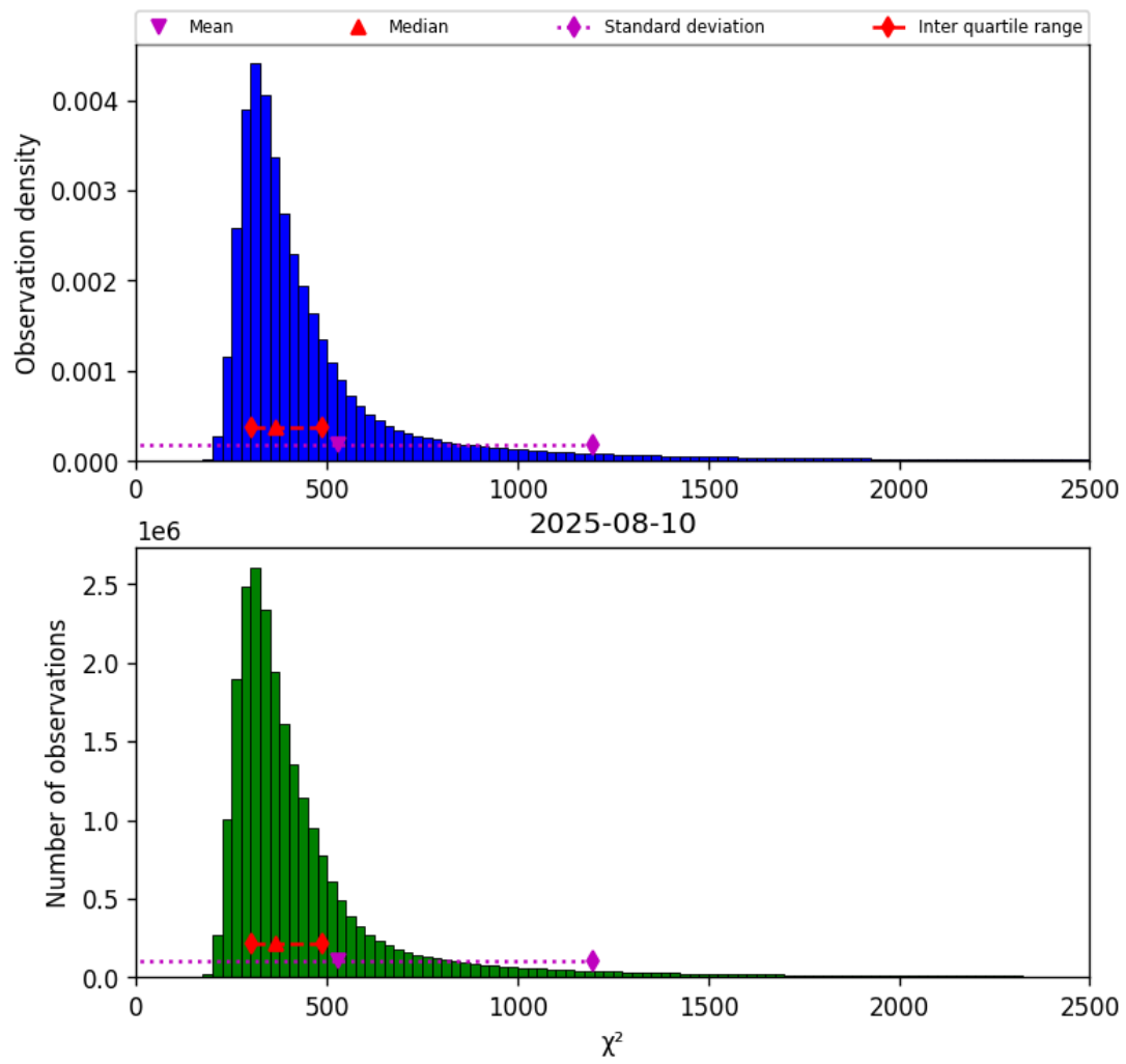
Figure 40: Histogram of “ \chi^2 ” for 2025-08-10 to 2025-08-11
