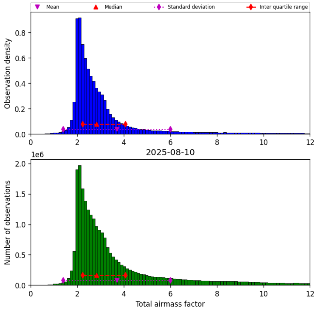
Figure 30: Histogram of “Total airmass factor” for 2025-08-10 to 2025-08-11
