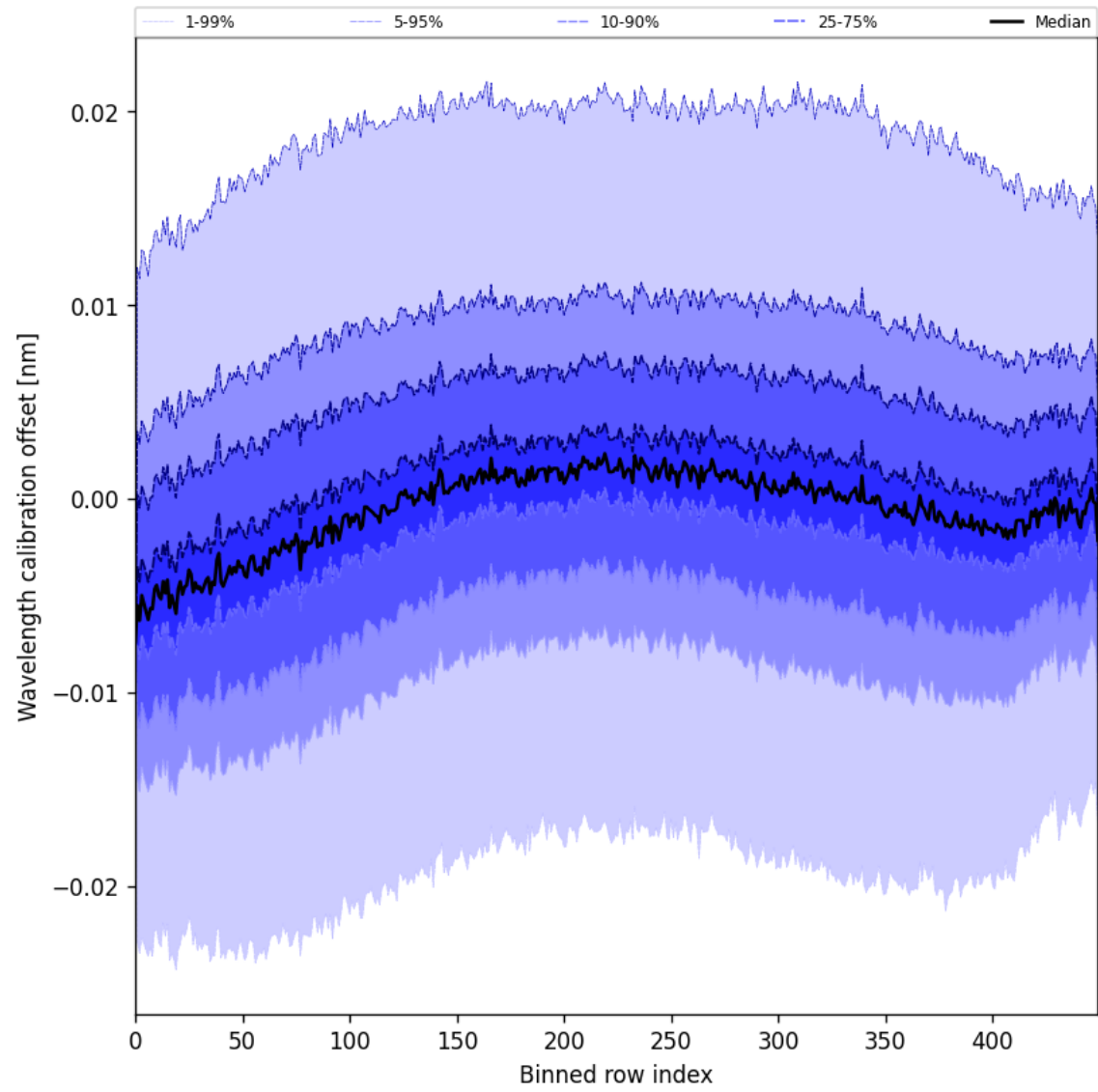
Figure 50: Along track statistics of “Wavelength calibration offset” for 2025-08-10 to 2025-08-11
