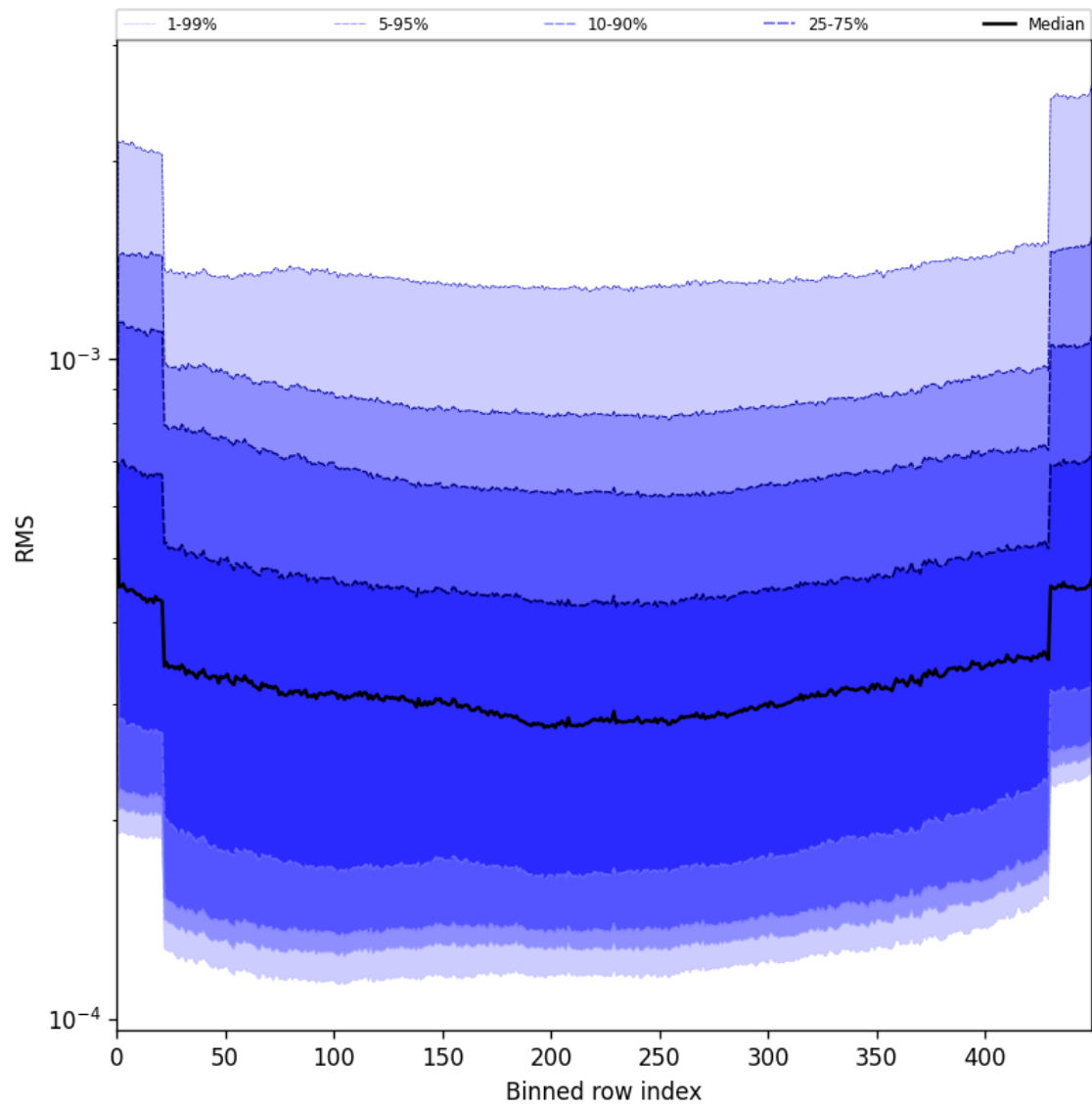
Figure 58: Along track statistics of “RMS” for 2025-08-10 to 2025-08-11
