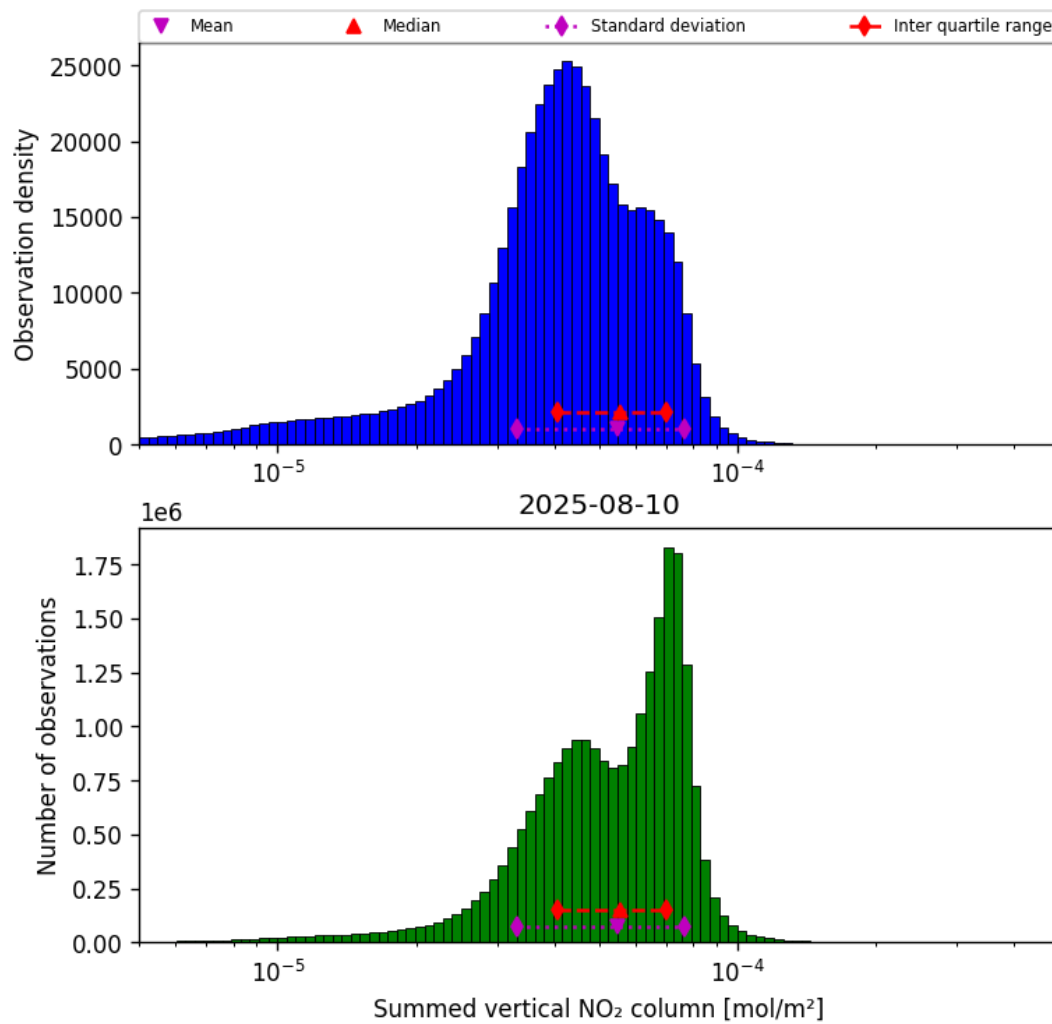
Figure 38: Histogram of “Summed vertical NO 2 column” for 2025-08-10 to 2025-08-11
