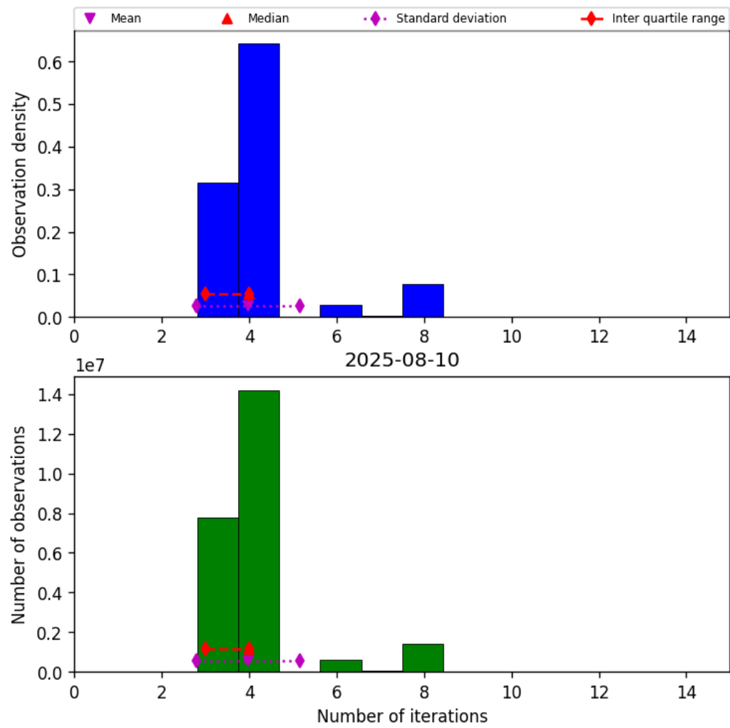
Figure 32: Histogram of “Number of iterations” for 2025-08-10 to 2025-08-11
