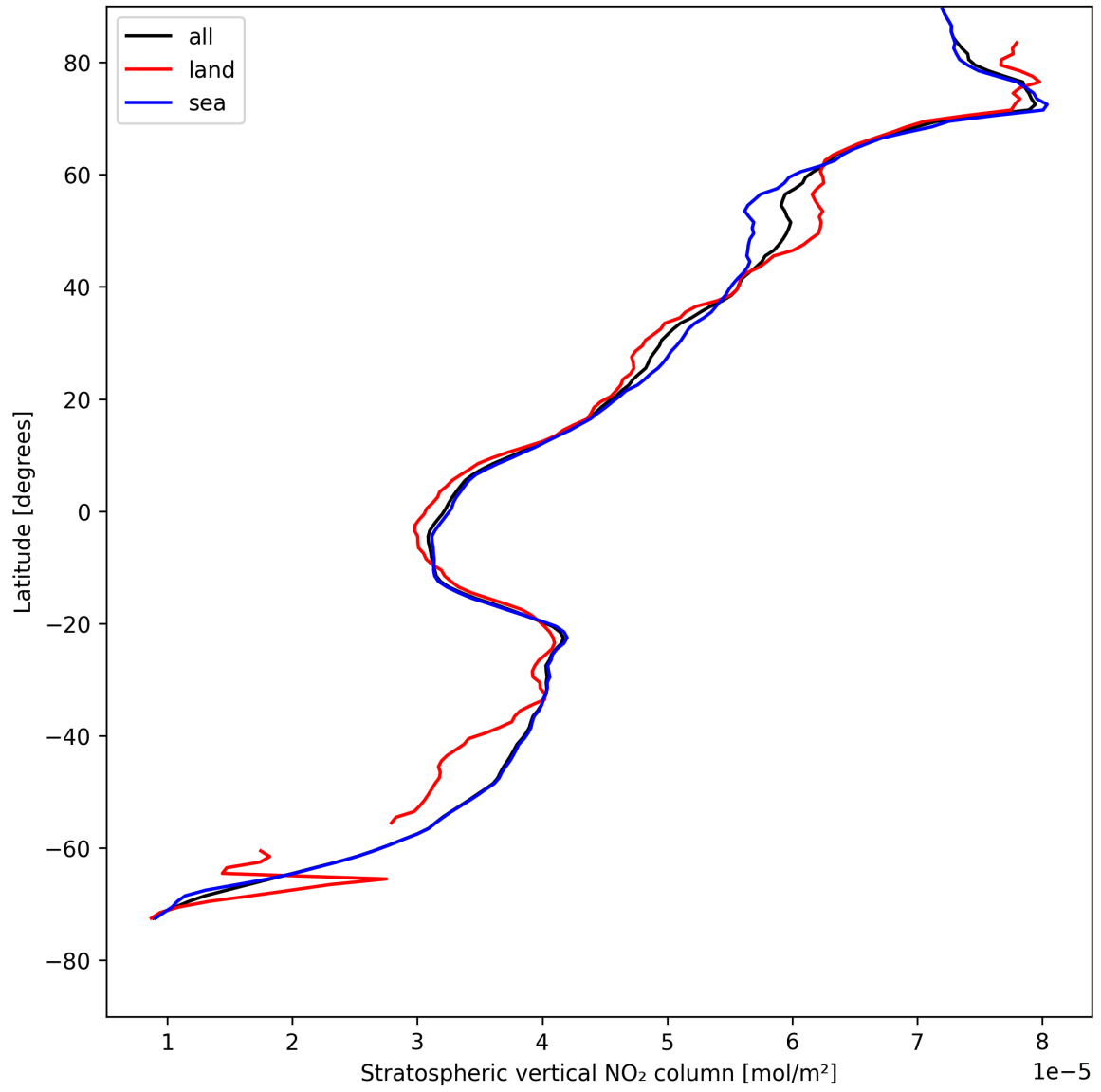
Figure 17: Zonal average of “Stratospheric vertical NO 2 column” for 2025-08-10 to 2025-08-11.
