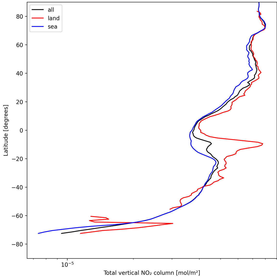
Figure 19: Zonal average of “Total vertical NO 2 column” for 2025-08-10 to 2025-08-11.
