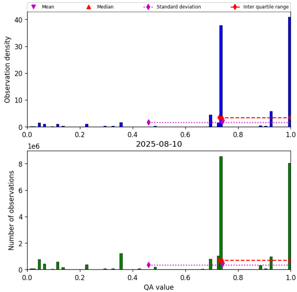
Figure 26: Histogram of “QA value” for 2025-08-10 to 2025-08-11
