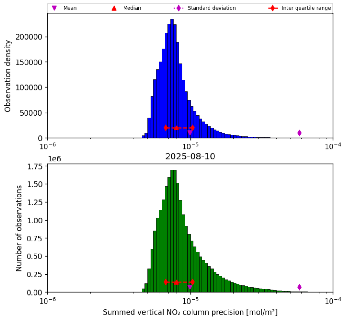
Figure 39: Histogram of “Summed vertical NO 2 column precision” for 2025-08-10 to 2025-08-11
