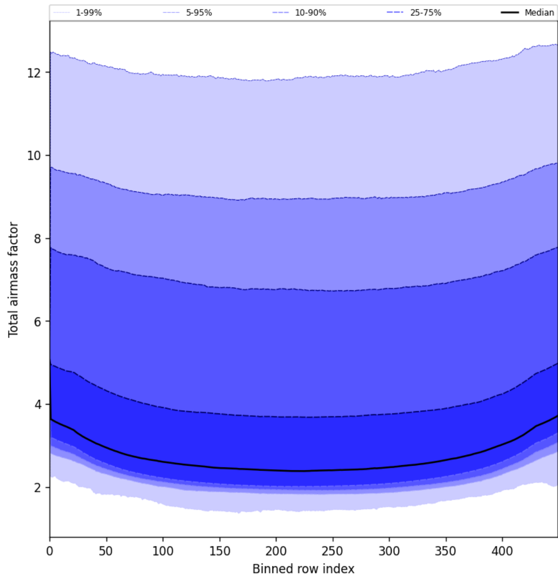
Figure 47: Along track statistics of “Total airmass factor” for 2025-08-10 to 2025-08-11
