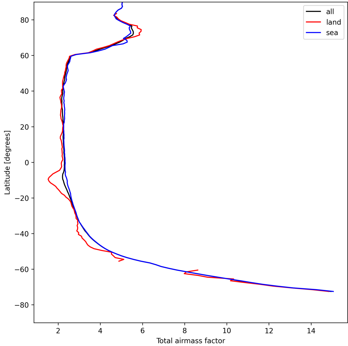
Figure 13: Zonal average of “Total airmass factor” for 2025-08-10 to 2025-08-11.
