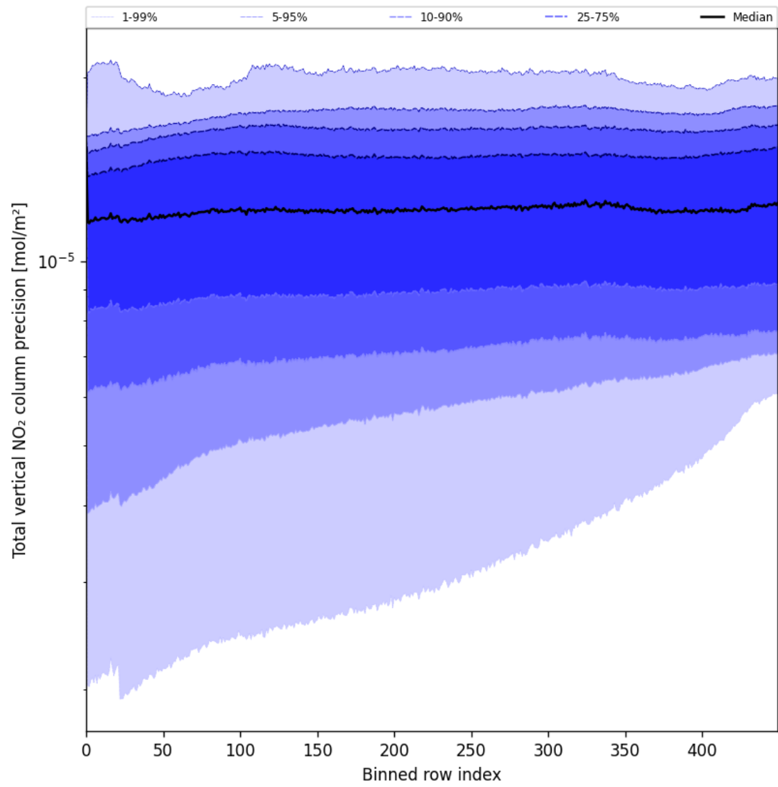
Figure 54: Along track statistics of “Total vertical NO 2 column precision” for 2025-08-10 to 2025-08-11
