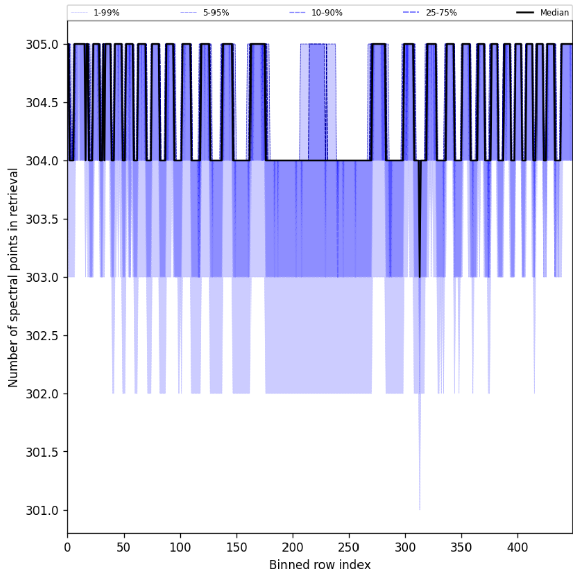
Figure 48: Along track statistics of “Number of spectral points in retrieval” for 2025-08-10 to 2025-08-11
