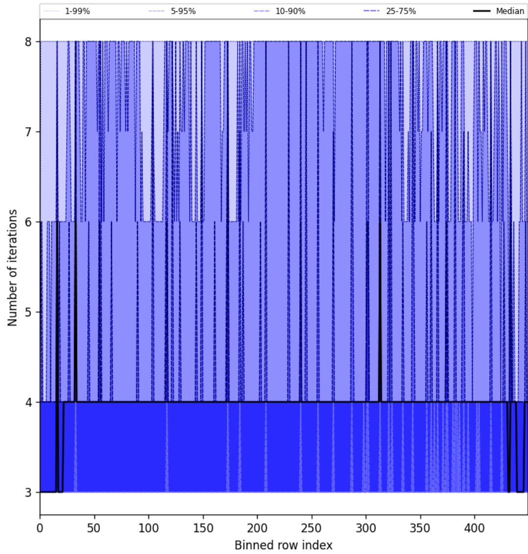
Figure 49: Along track statistics of “Number of iterations” for 2025-08-10 to 2025-08-11
