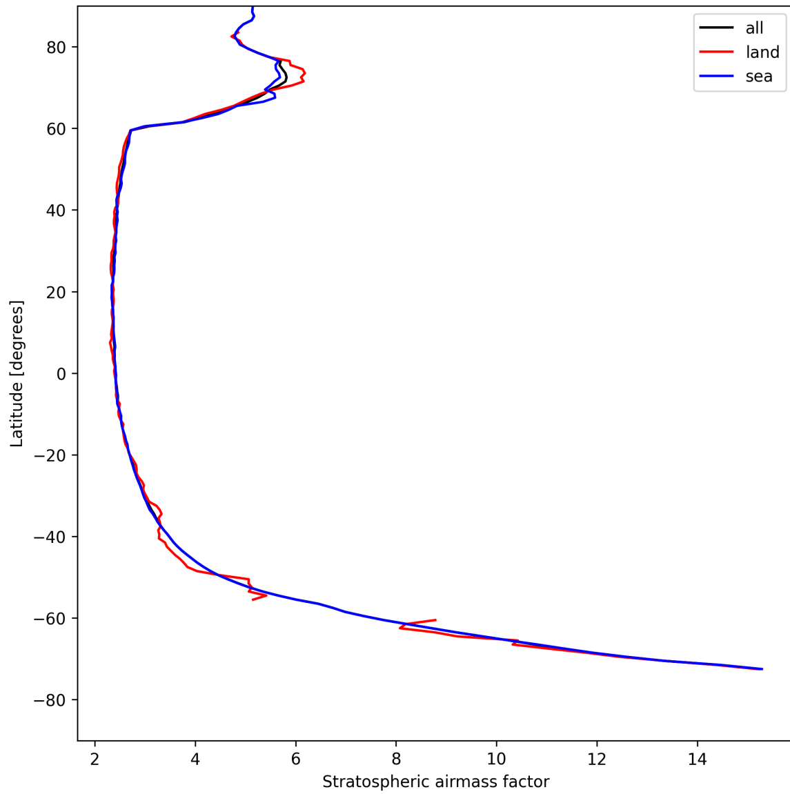
Figure 25: Zonal average of “Stratospheric air mass factor” for 2025-08-10 to 2025-08-11.
