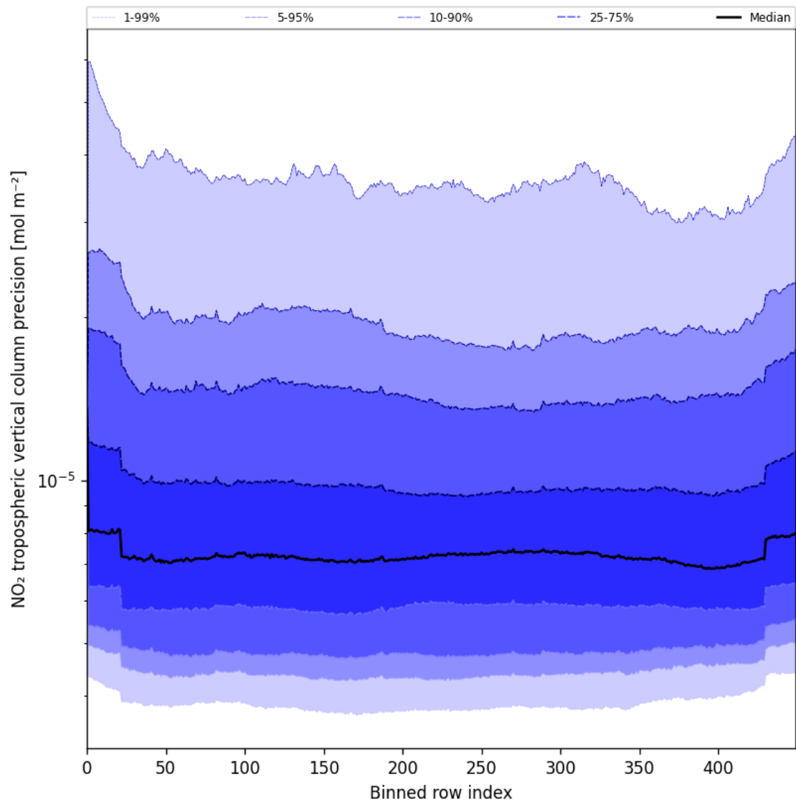
Figure 45: Along track statistics of “NO 2 tropospheric vertical column precision” for 2025-08-10 to 2025-08-11
