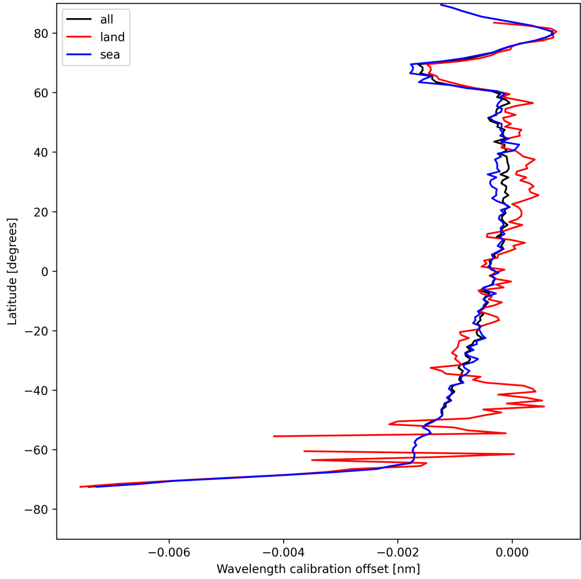
Figure 16: Zonal average of “Wavelength calibration offset” for 2025-08-10 to 2025-08-11.
