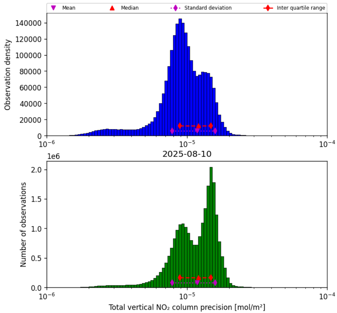
Figure 37: Histogram of “Total vertical NO 2 column precision” for 2025-08-10 to 2025-08-11
