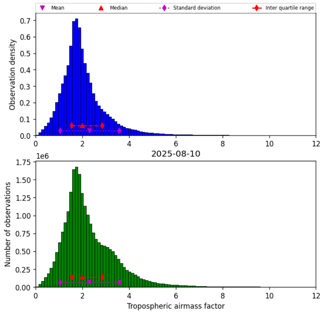
Figure 29: Histogram of “Tropospheric airmass factor” for 2025-08-10 to 2025-08-11
