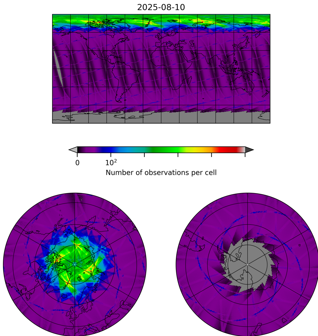
Figure 8: Map of the number of observations for 2025-08-10 to 2025-08-11
