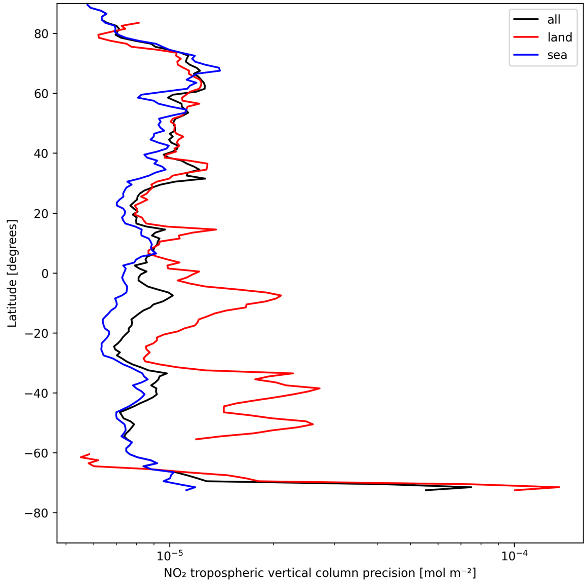
Figure 11: Zonal average of “NO 2 tropospheric vertical column precision” for 2025-08-10 to 2025-08-11.
