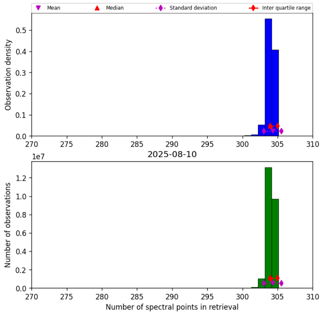
Figure 31: Histogram of “Number of spectral points in retrieval” for 2025-08-10 to 2025-08-11
