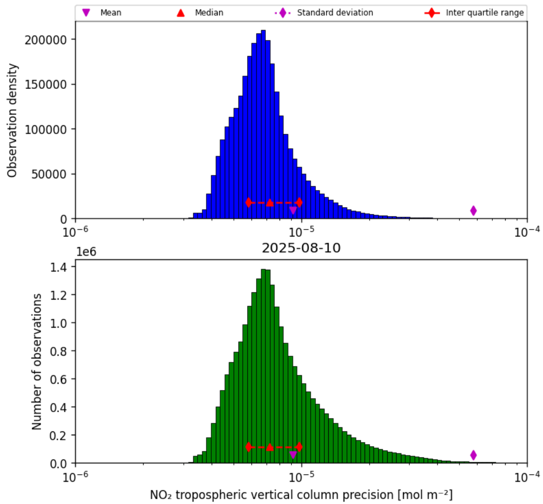
Figure 28: Histogram of “NO 2 tropospheric vertical column precision” for 2025-08-10 to 2025-08-11
