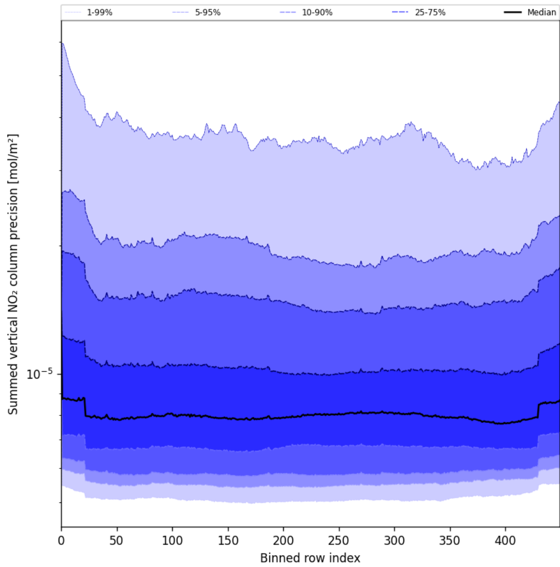
Figure 56: Along track statistics of “Summed vertical NO 2 column precision” for 2025-08-10 to 2025-08-11
