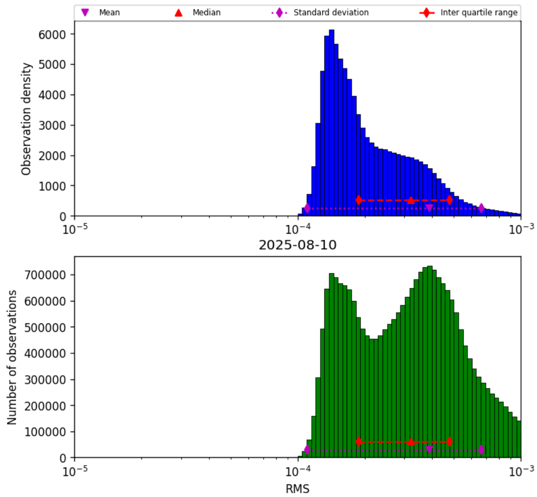
Figure 41: Histogram of “RMS” for 2025-08-10 to 2025-08-11
