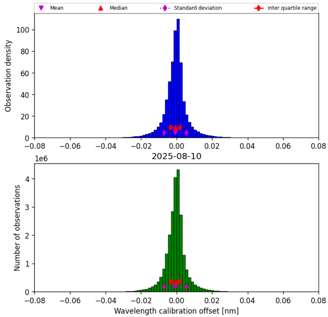
Figure 33: Histogram of “Wavelength calibration offset” for 2025-08-10 to 2025-08-11
