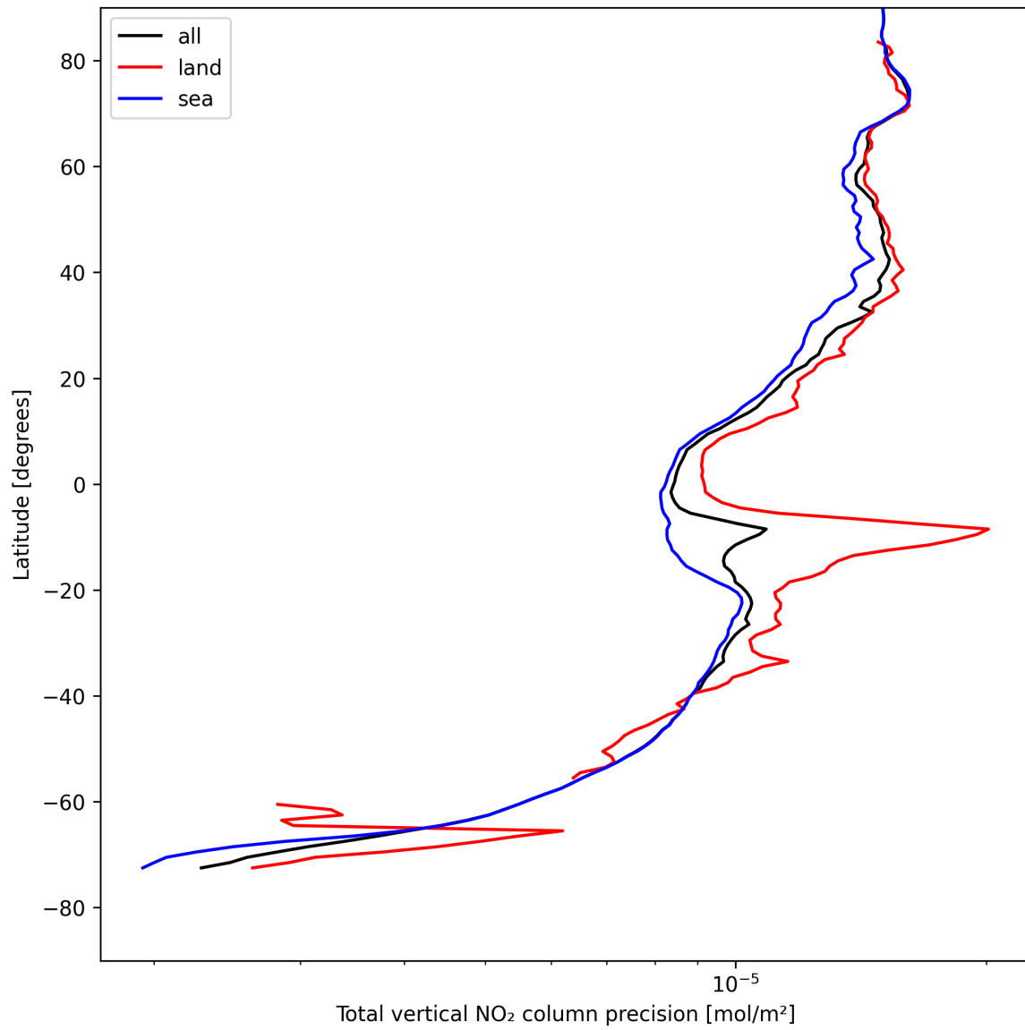
Figure 20: Zonal average of “Total vertical NO 2 column precision” for 2025-08-10 to 2025-08-11.
