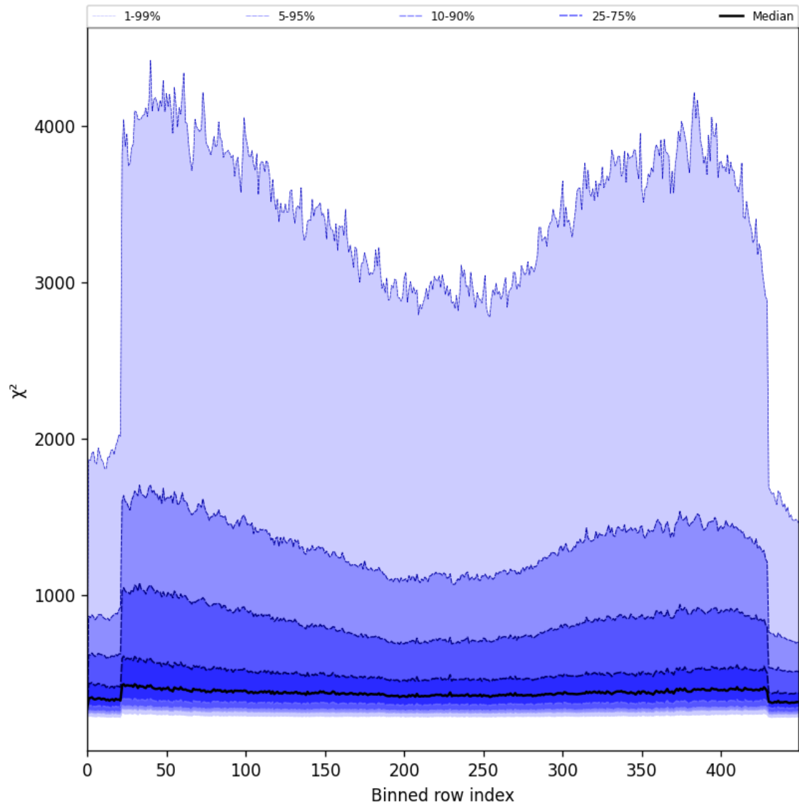
Figure 57: Along track statistics of “ \chi^2 ” for 2025-08-10 to 2025-08-11
