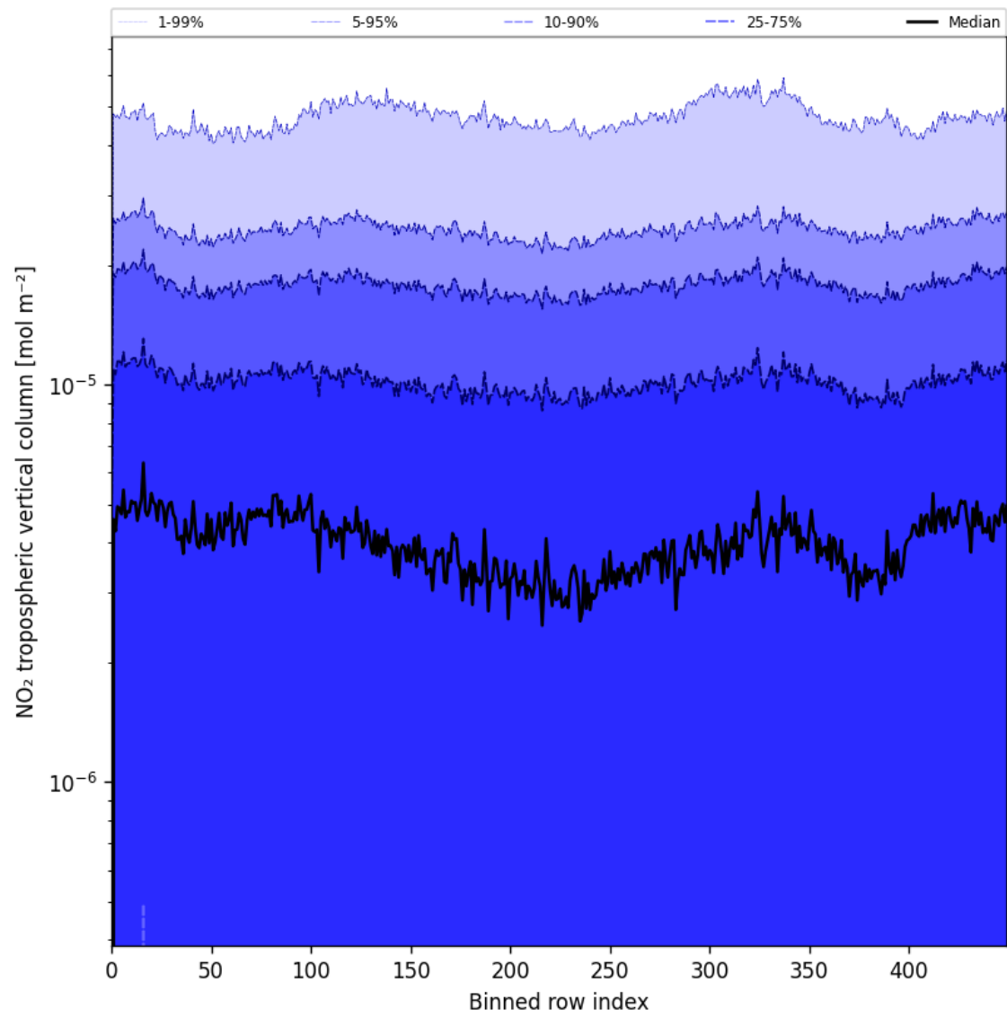
Figure 44: Along track statistics of “NO 2 tropospheric vertical column” for 2025-08-10 to 2025-08-11
