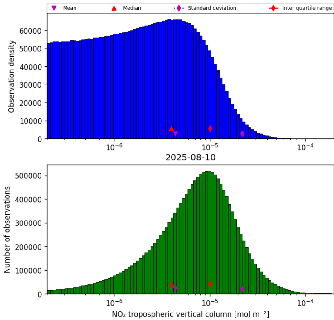
Figure 27: Histogram of “NO 2 tropospheric vertical column” for 2025-08-10 to 2025-08-11
