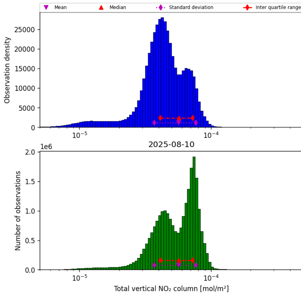
Figure 36: Histogram of “Total vertical NO 2 column” for 2025-08-10 to 2025-08-11
