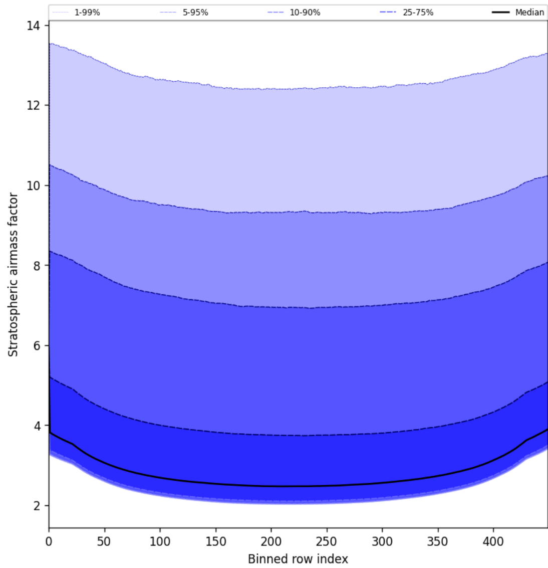
Figure 59: Along track statistics of “Stratospheric airmass factor” for 2025-08-10 to 2025-08-11
