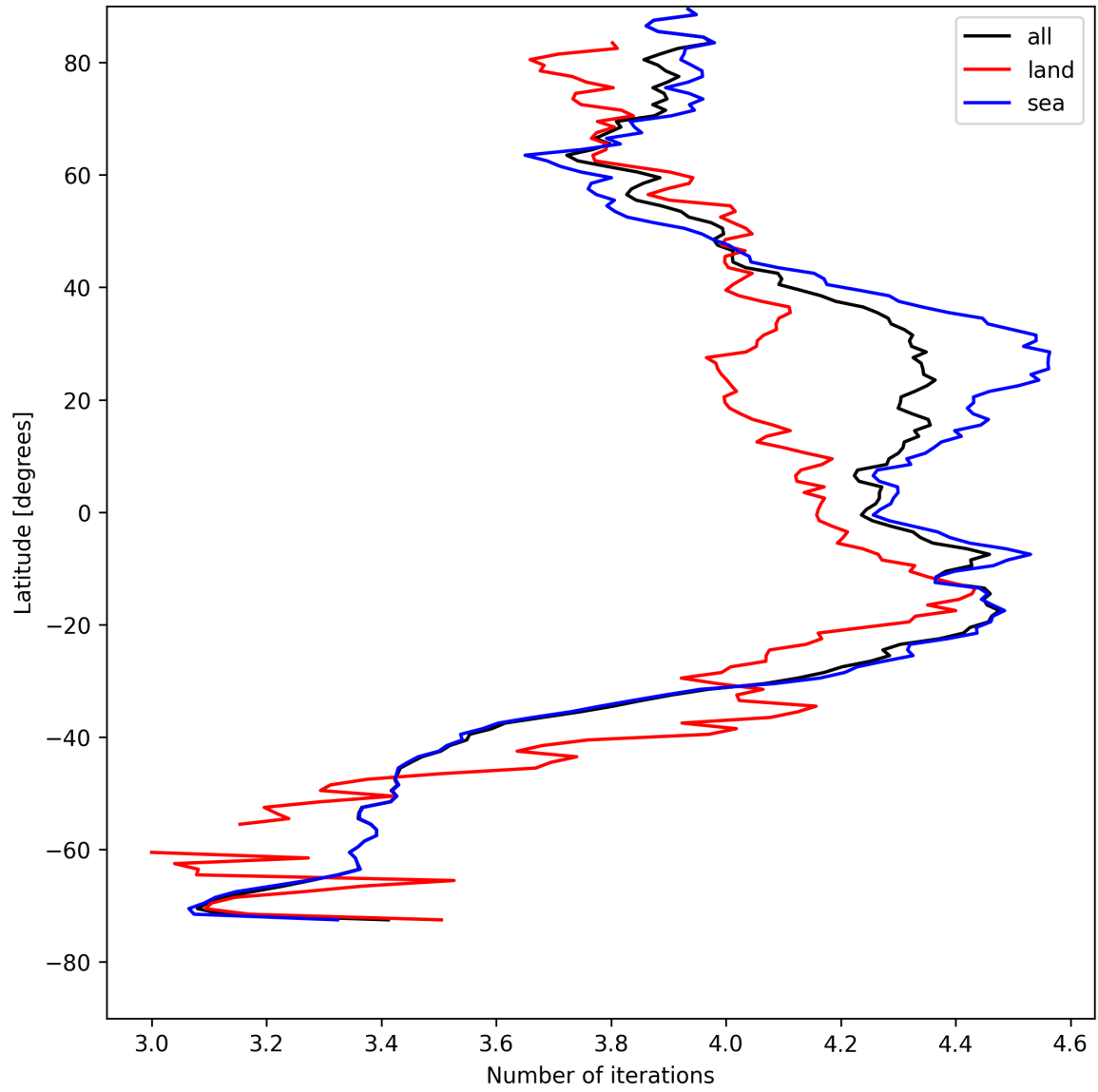
Figure 15: Zonal average of “Number of iterations” for 2025-08-10 to 2025-08-11.
