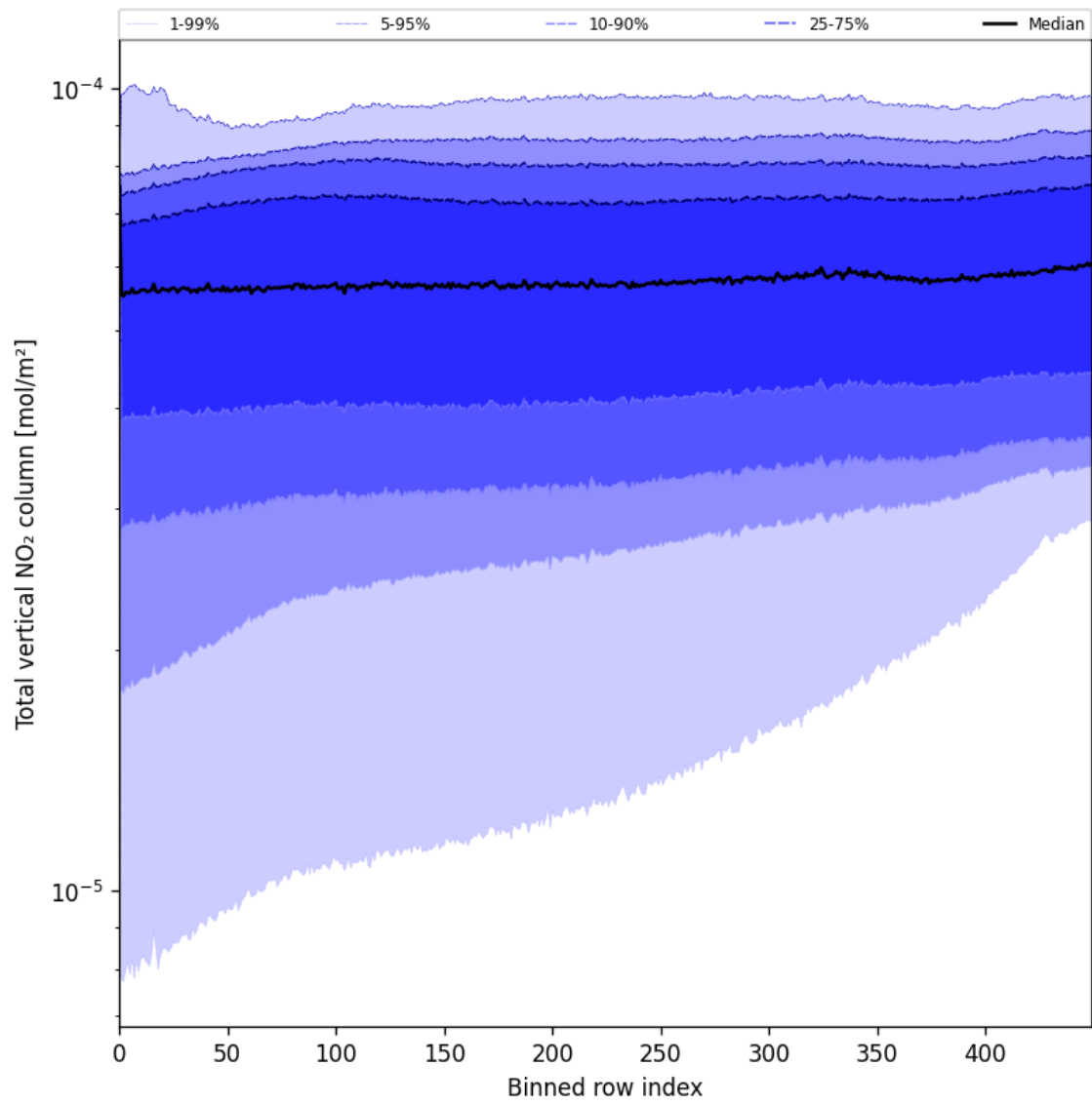
Figure 53: Along track statistics of “Total vertical NO 2 column” for 2025-08-10 to 2025-08-11
