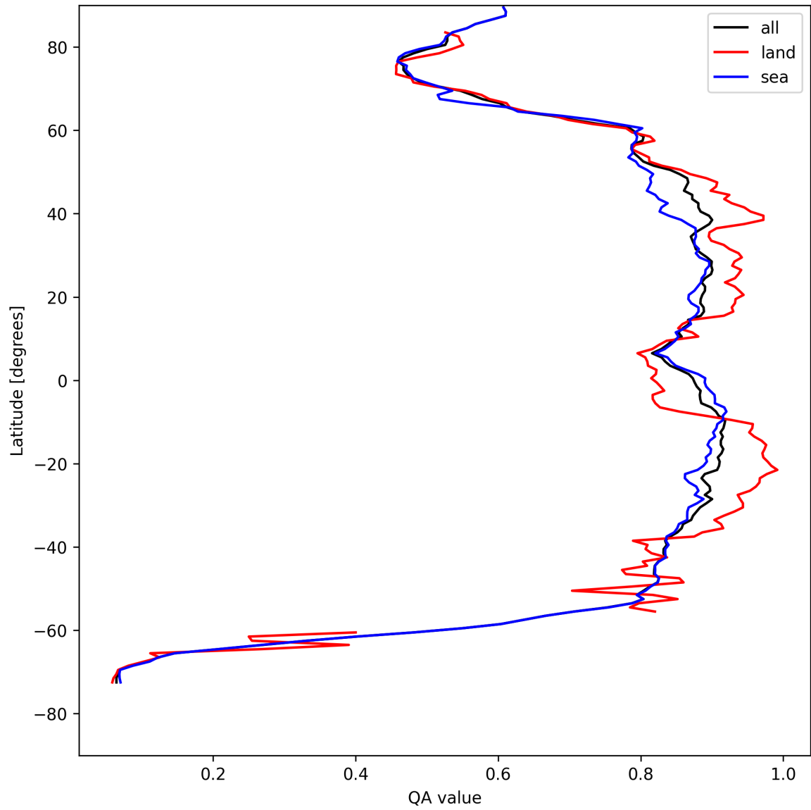
Figure 9: Zonal average of “QA value” for 2025-08-10 to 2025-08-11.
