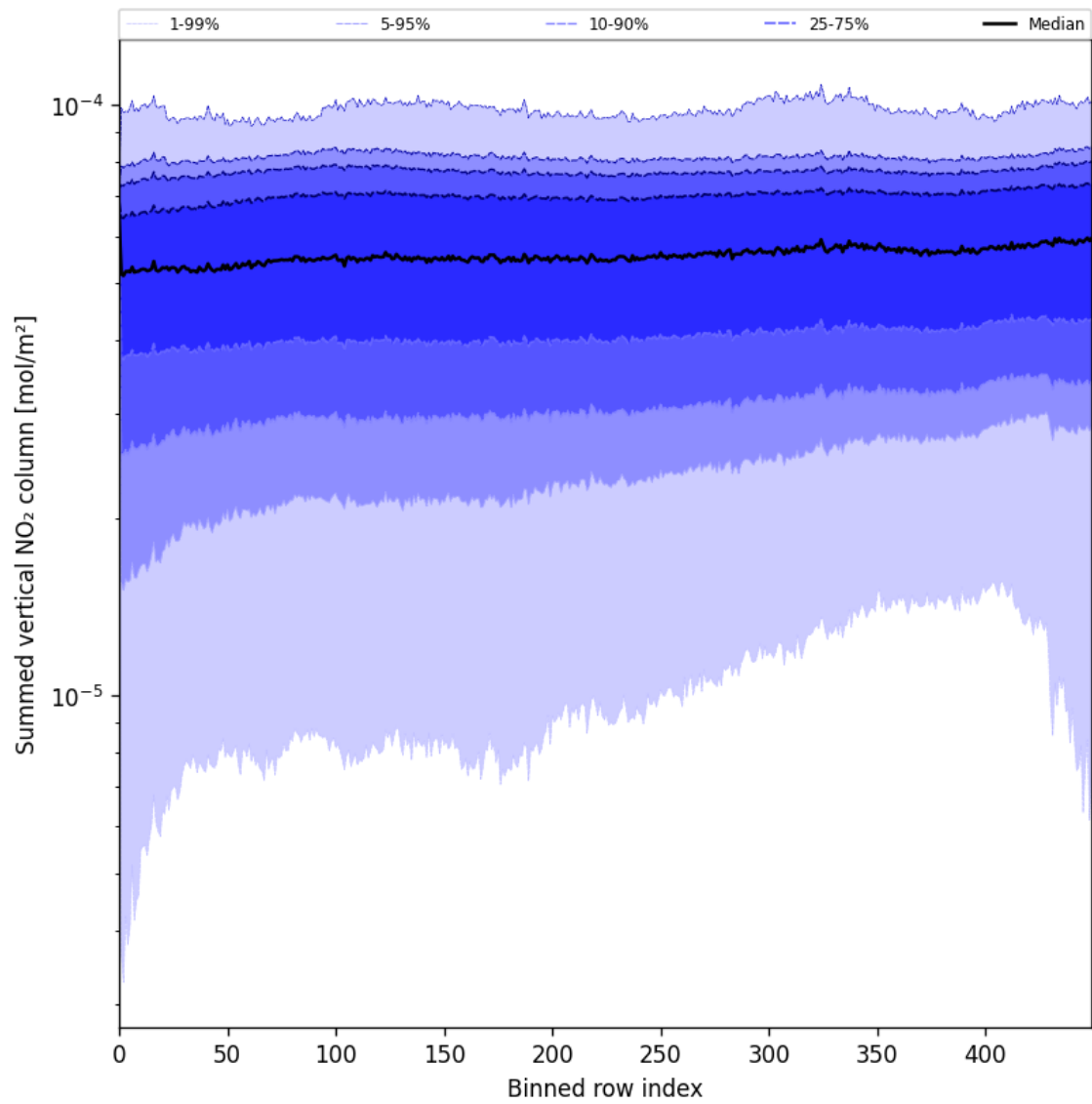
Figure 55: Along track statistics of “Summed vertical NO 2 column” for 2025-08-10 to 2025-08-11
