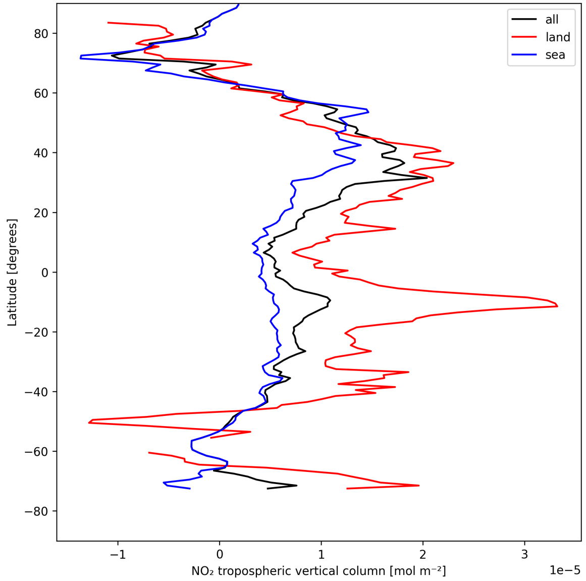
Figure 10: Zonal average of “NO 2 tropospheric vertical column” for 2025-08-10 to 2025-08-11.
