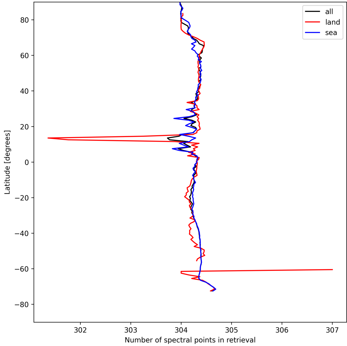
Figure 14: Zonal average of “Number of spectral points in retrieval” for 2025-08-10 to 2025-08-11.
