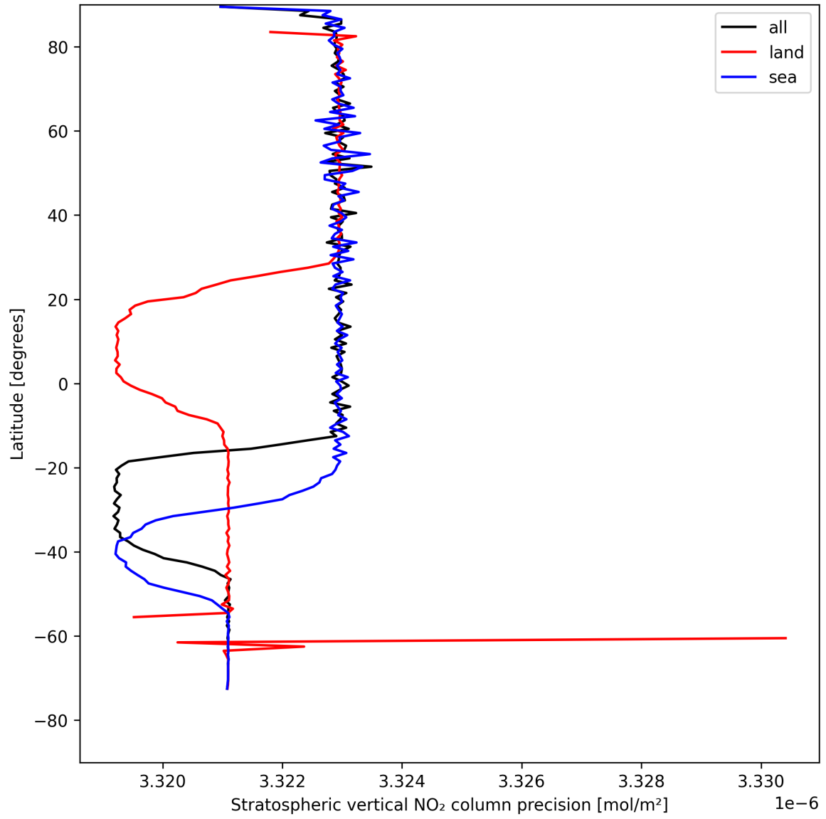
Figure 18: Zonal average of “Stratospheric vertical NO 2 column precision” for 2025-08-10 to 2025-08-11.
