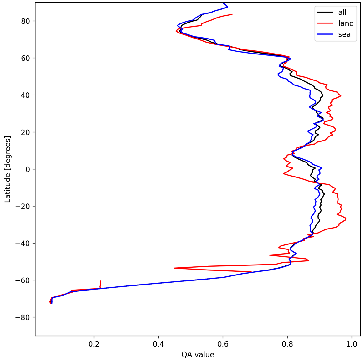
Figure 9: Zonal average of “QA value” for 2025-08-11 to 2025-08-12.
