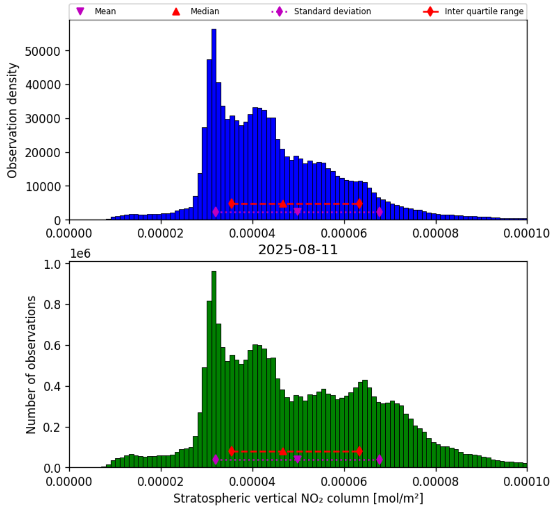
Figure 34: Histogram of “Stratospheric vertical NO 2 column” for 2025-08-11 to 2025-08-12
