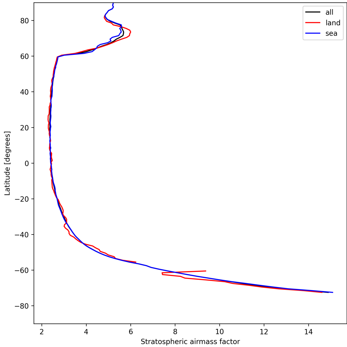
Figure 25: Zonal average of “Stratospheric air mass factor” for 2025-08-11 to 2025-08-12.
