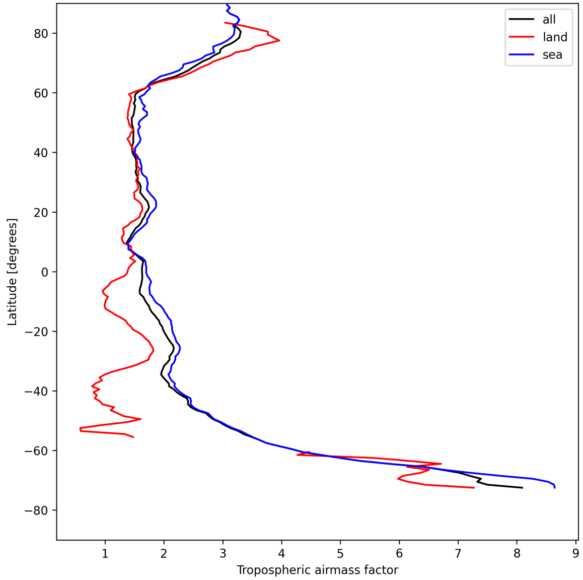
Figure 12: Zonal average of “Tropospheric air mass factor” for 2025-08-11 to 2025-08-12.
