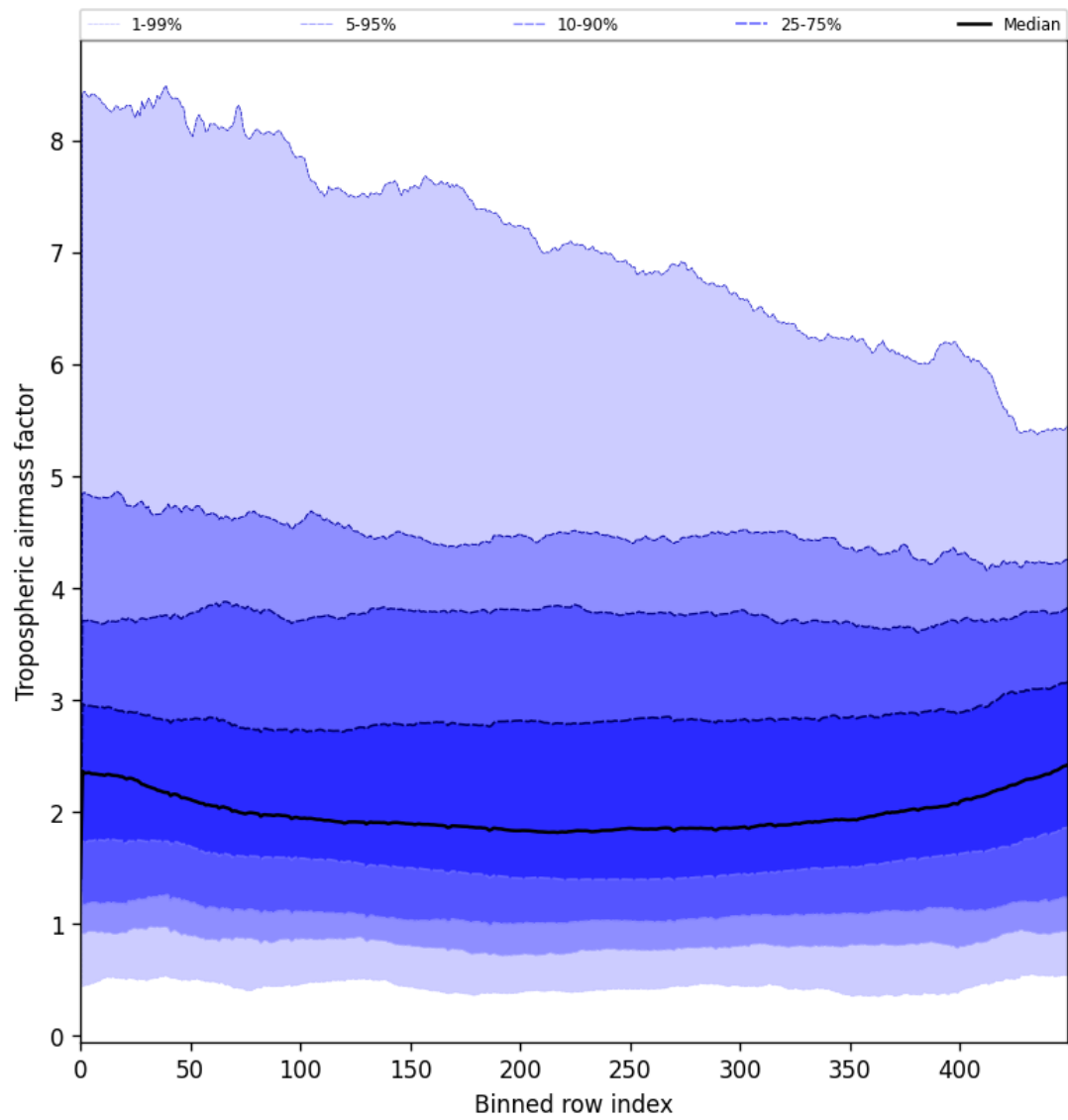
Figure 46: Along track statistics of “Tropospheric airmass factor” for 2025-08-11 to 2025-08-12
