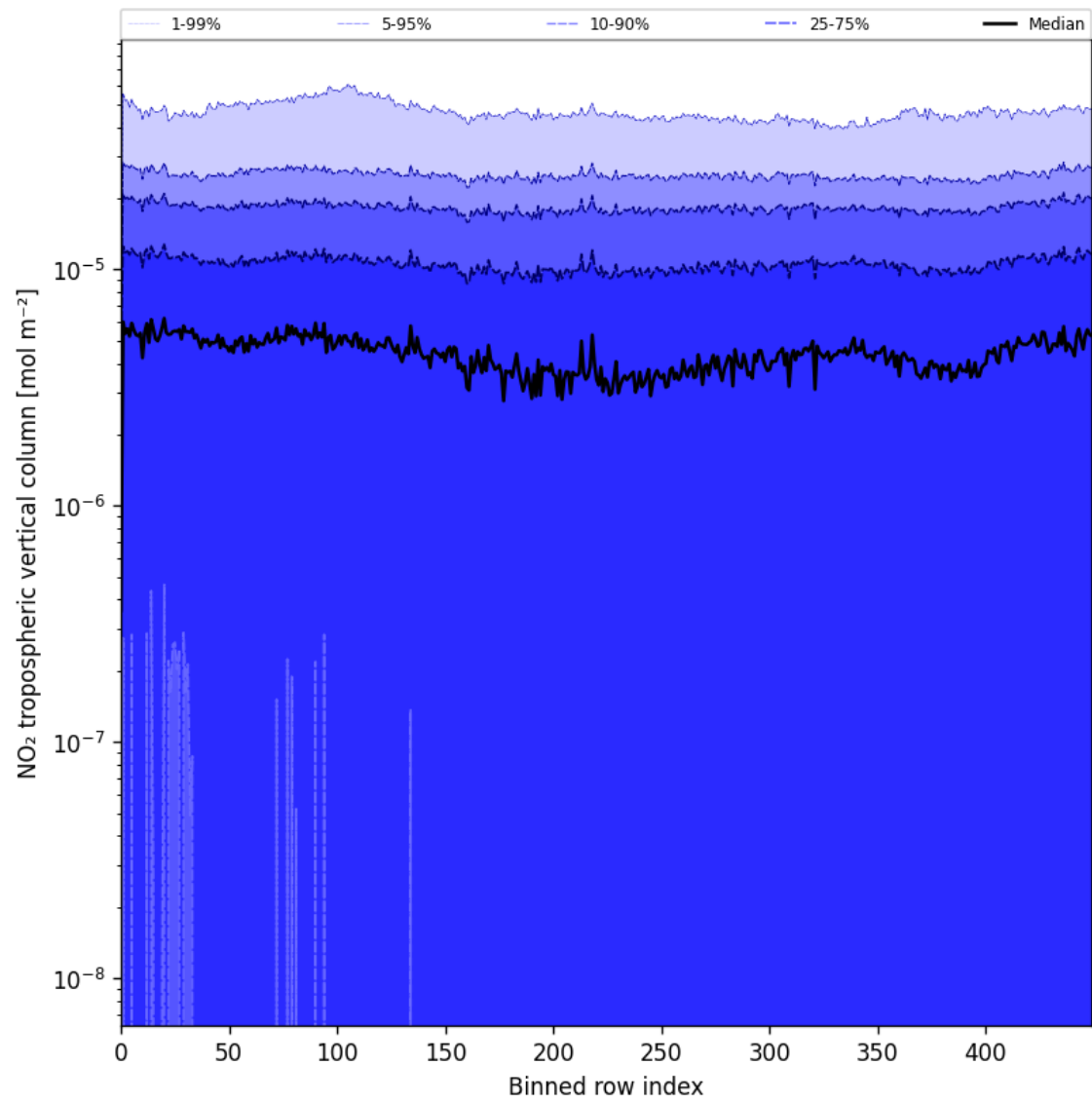
Figure 44: Along track statistics of “NO 2 tropospheric vertical column” for 2025-08-11 to 2025-08-12
