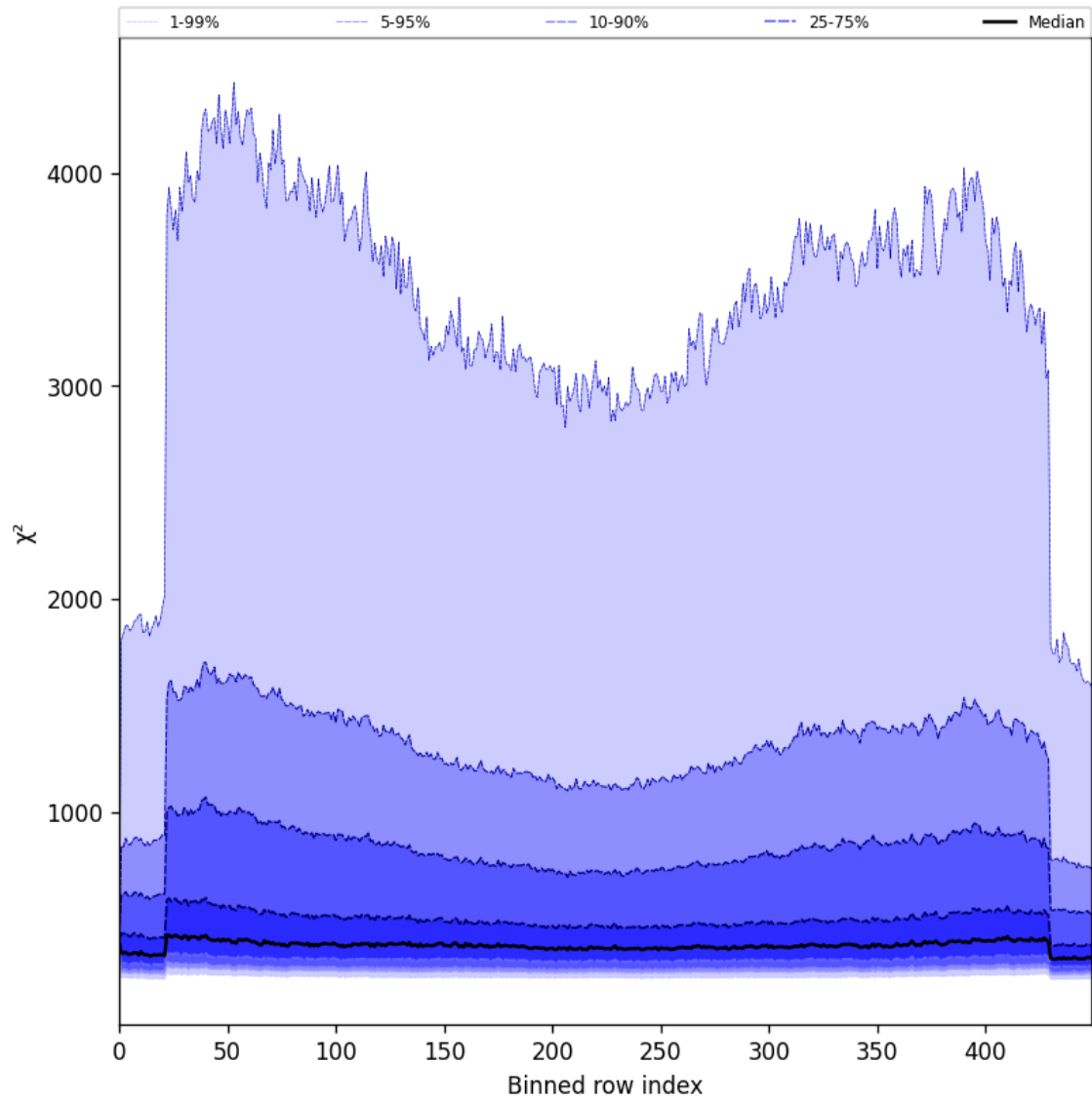
Figure 57: Along track statistics of “ \chi^2 ” for 2025-08-11 to 2025-08-12
