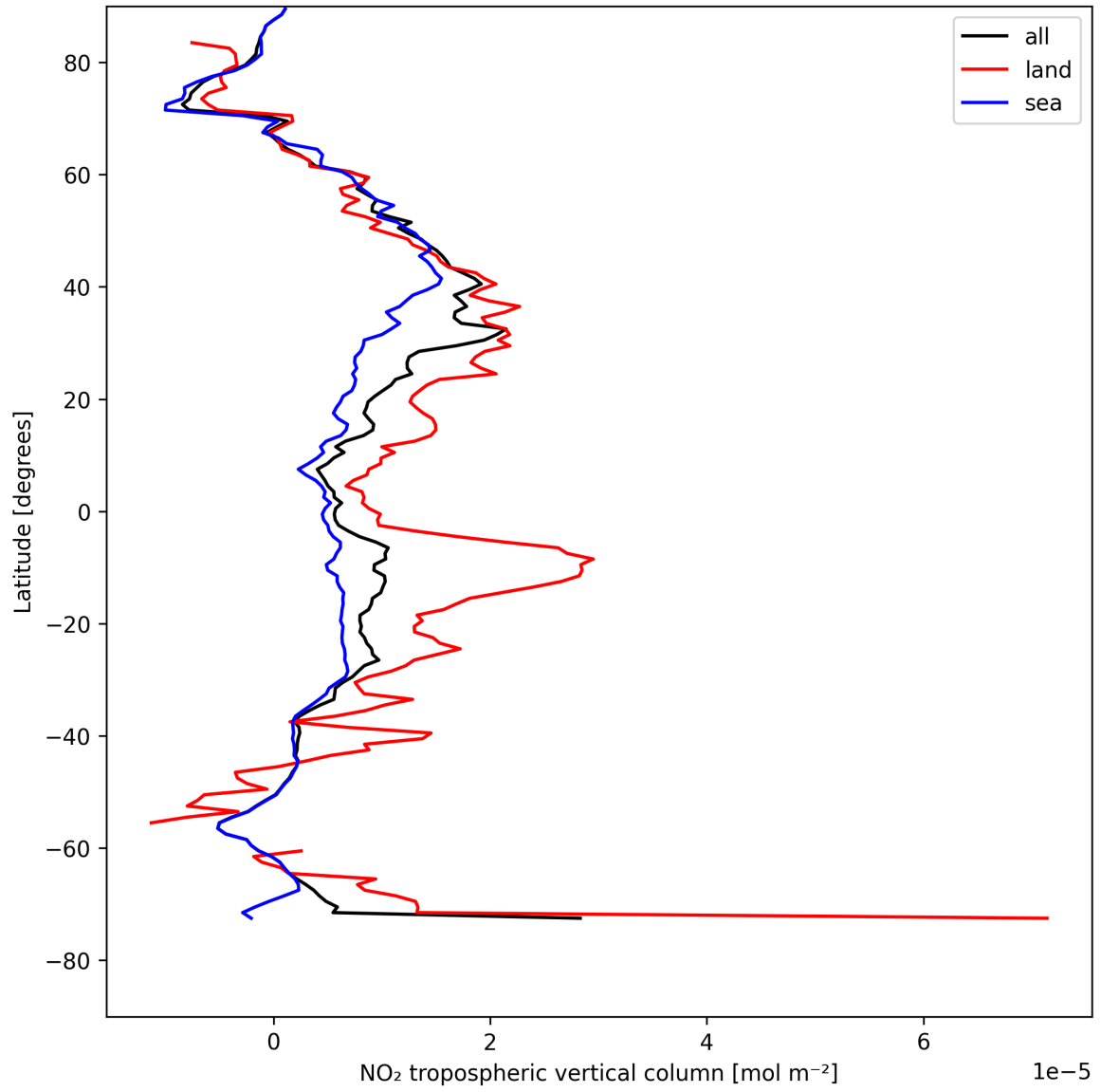
Figure 10: Zonal average of “NO 2 tropospheric vertical column” for 2025-08-11 to 2025-08-12.
