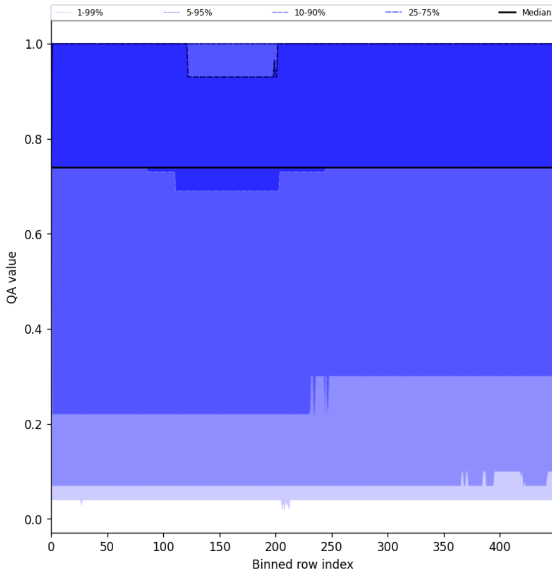
Figure 43: Along track statistics of “QA value” for 2025-08-11 to 2025-08-12
