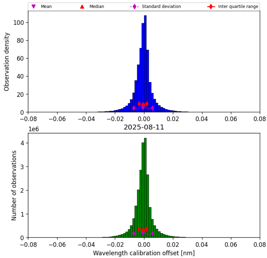
Figure 33: Histogram of “Wavelength calibration offset” for 2025-08-11 to 2025-08-12
