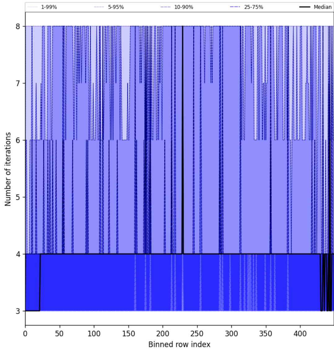
Figure 49: Along track statistics of “Number of iterations” for 2025-08-11 to 2025-08-12
