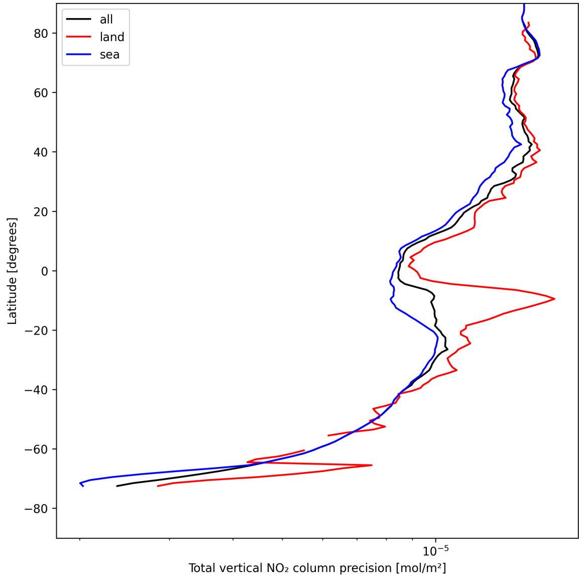
Figure 20: Zonal average of “Total vertical NO 2 column precision” for 2025-08-11 to 2025-08-12.
