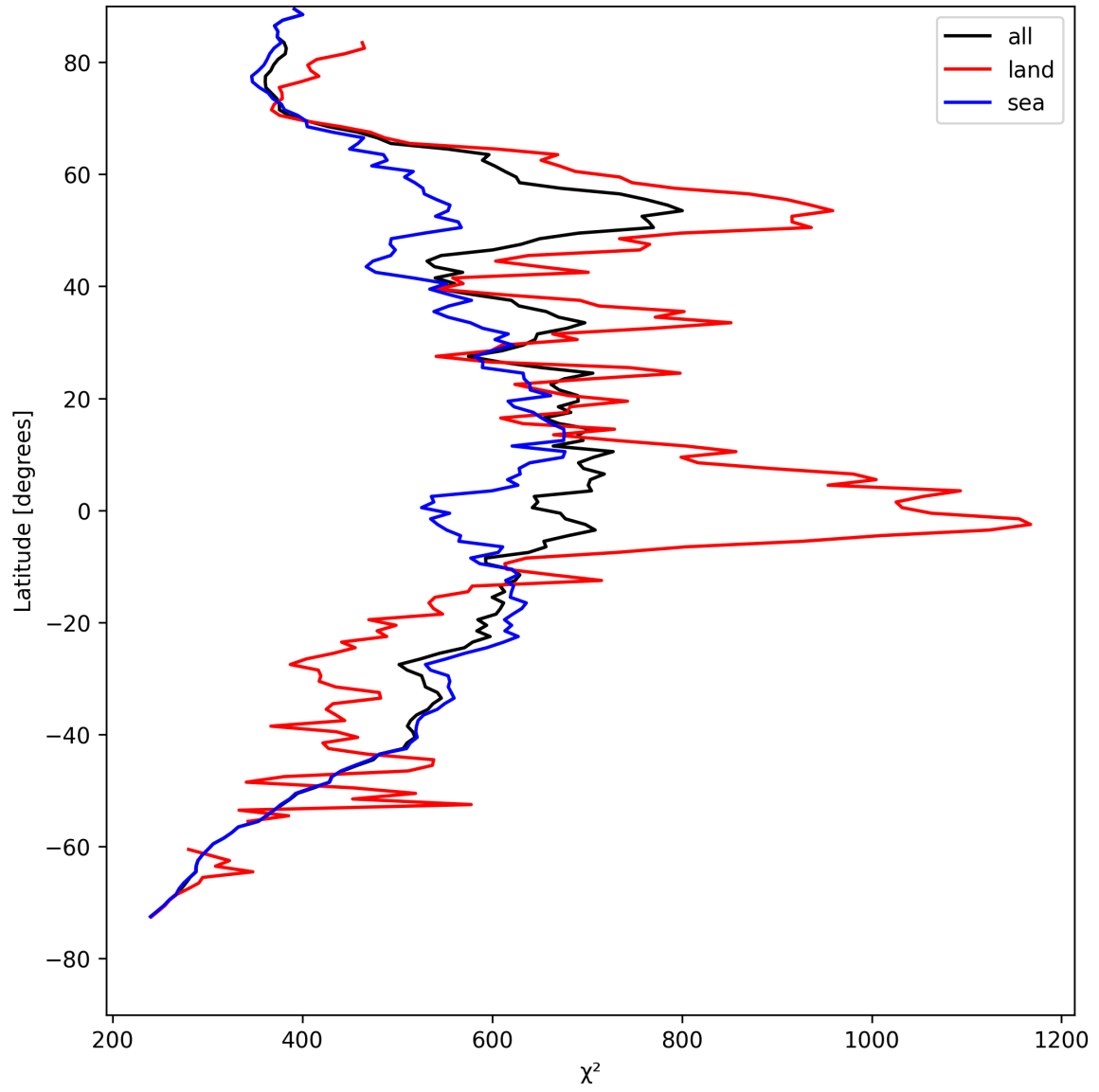
Figure 23: Zonal average of “ \chi^2 ” for 2025-08-11 to 2025-08-12.
