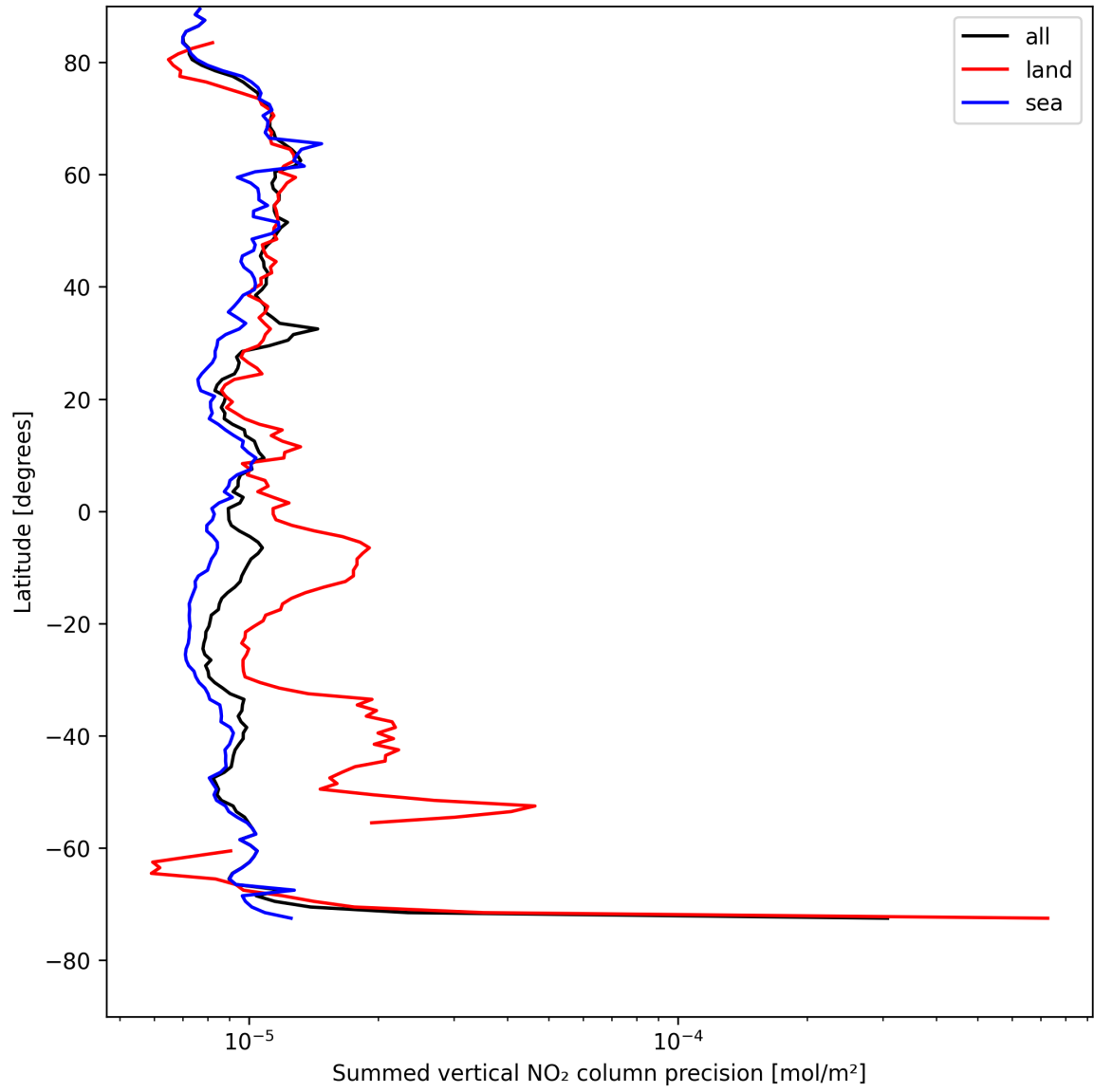
Figure 22: Zonal average of “Summed vertical NO 2 column precision” for 2025-08-11 to 2025-08-12.
