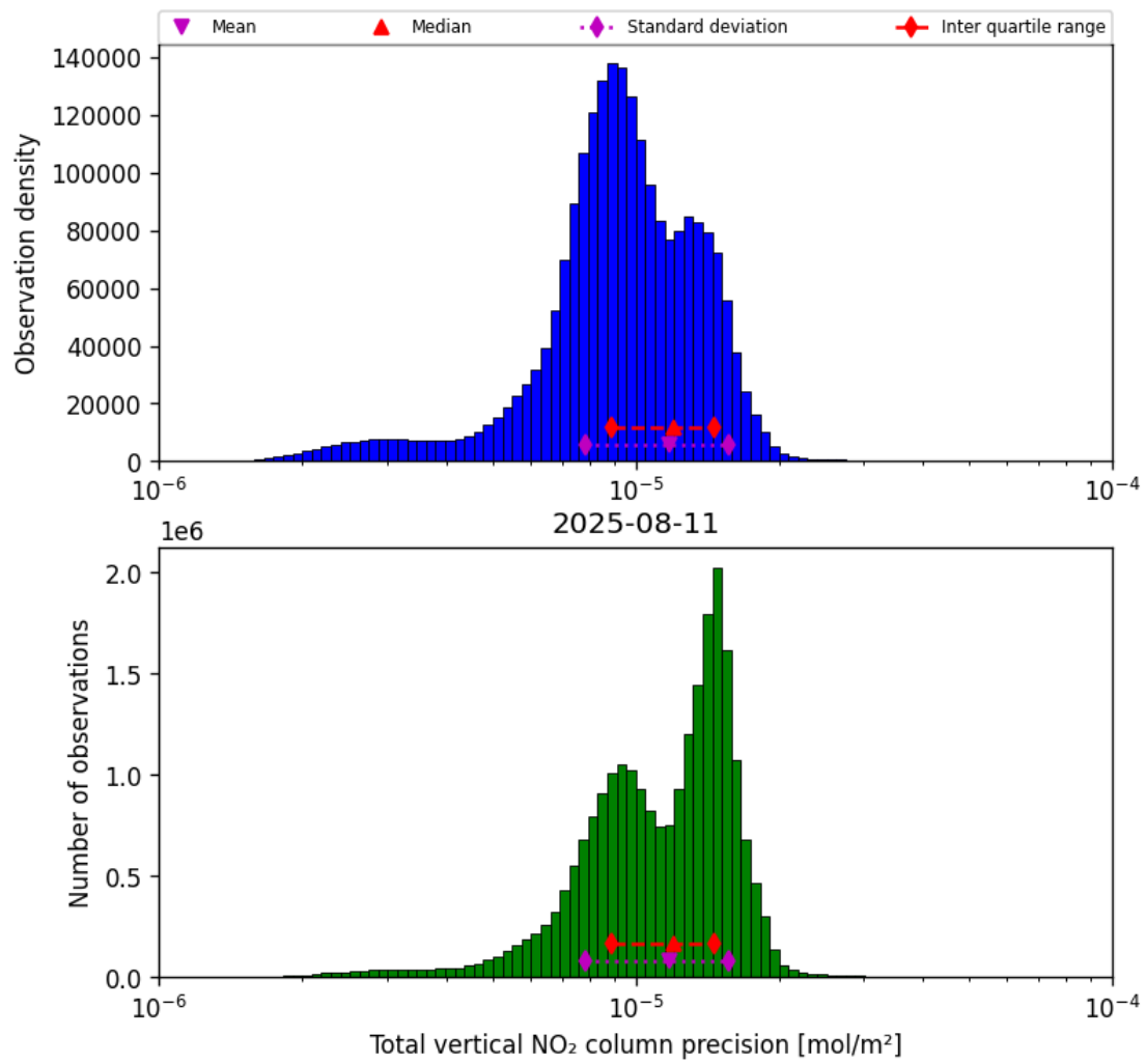
Figure 37: Histogram of “Total vertical NO 2 column precision” for 2025-08-11 to 2025-08-12
