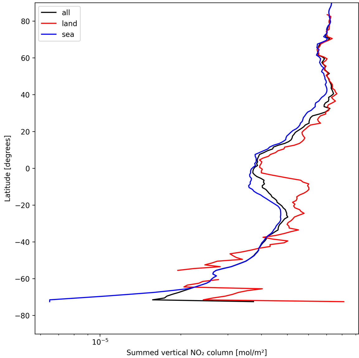
Figure 21: Zonal average of “Summed vertical NO 2 column” for 2025-08-11 to 2025-08-12.
