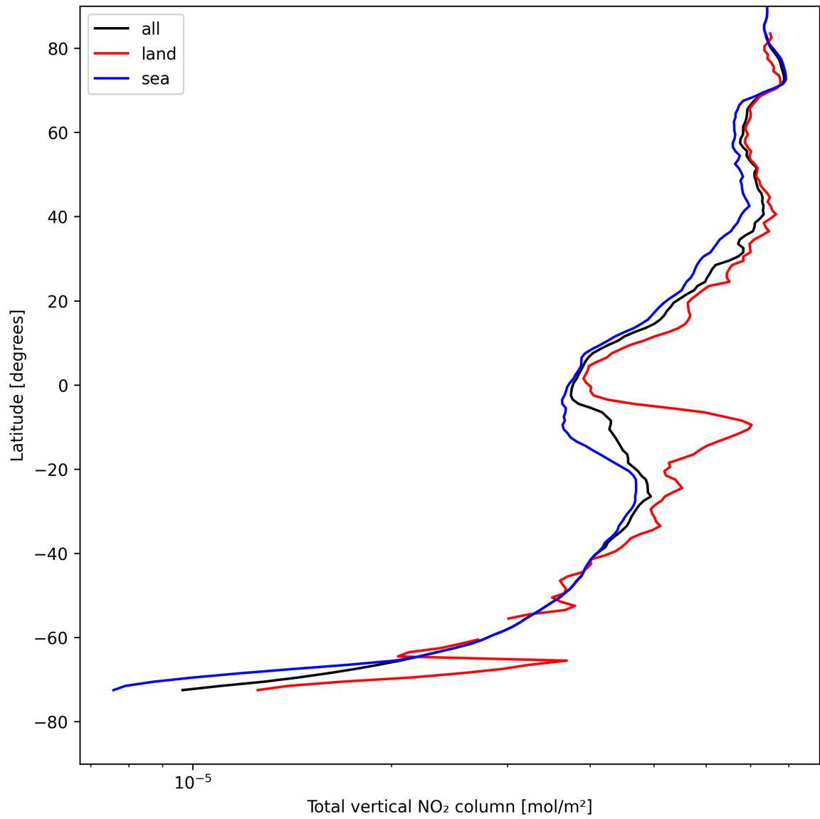
Figure 19: Zonal average of “Total vertical NO 2 column” for 2025-08-11 to 2025-08-12.
