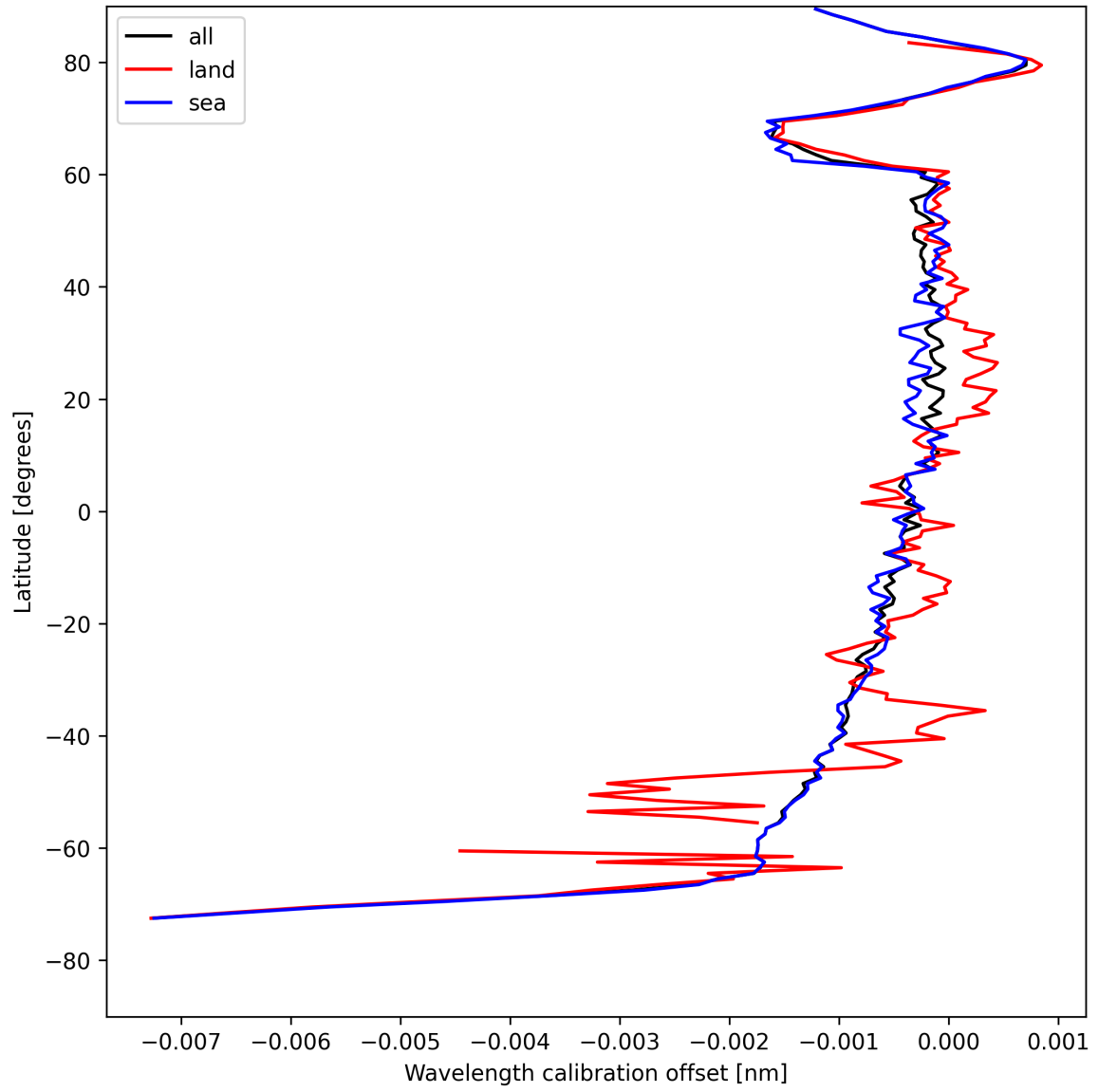
Figure 16: Zonal average of “Wavelength calibration offset” for 2025-08-11 to 2025-08-12.
