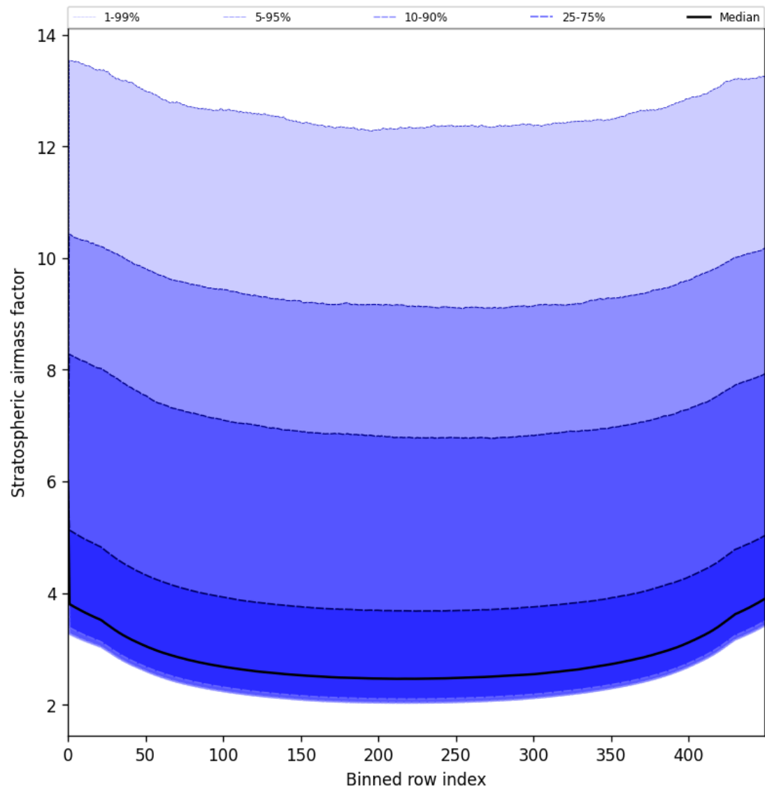
Figure 59: Along track statistics of “Stratospheric airmass factor” for 2025-08-11 to 2025-08-12
