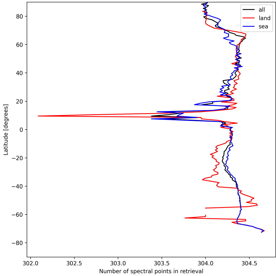
Figure 14: Zonal average of “Number of spectral points in retrieval” for 2025-08-11 to 2025-08-12.
