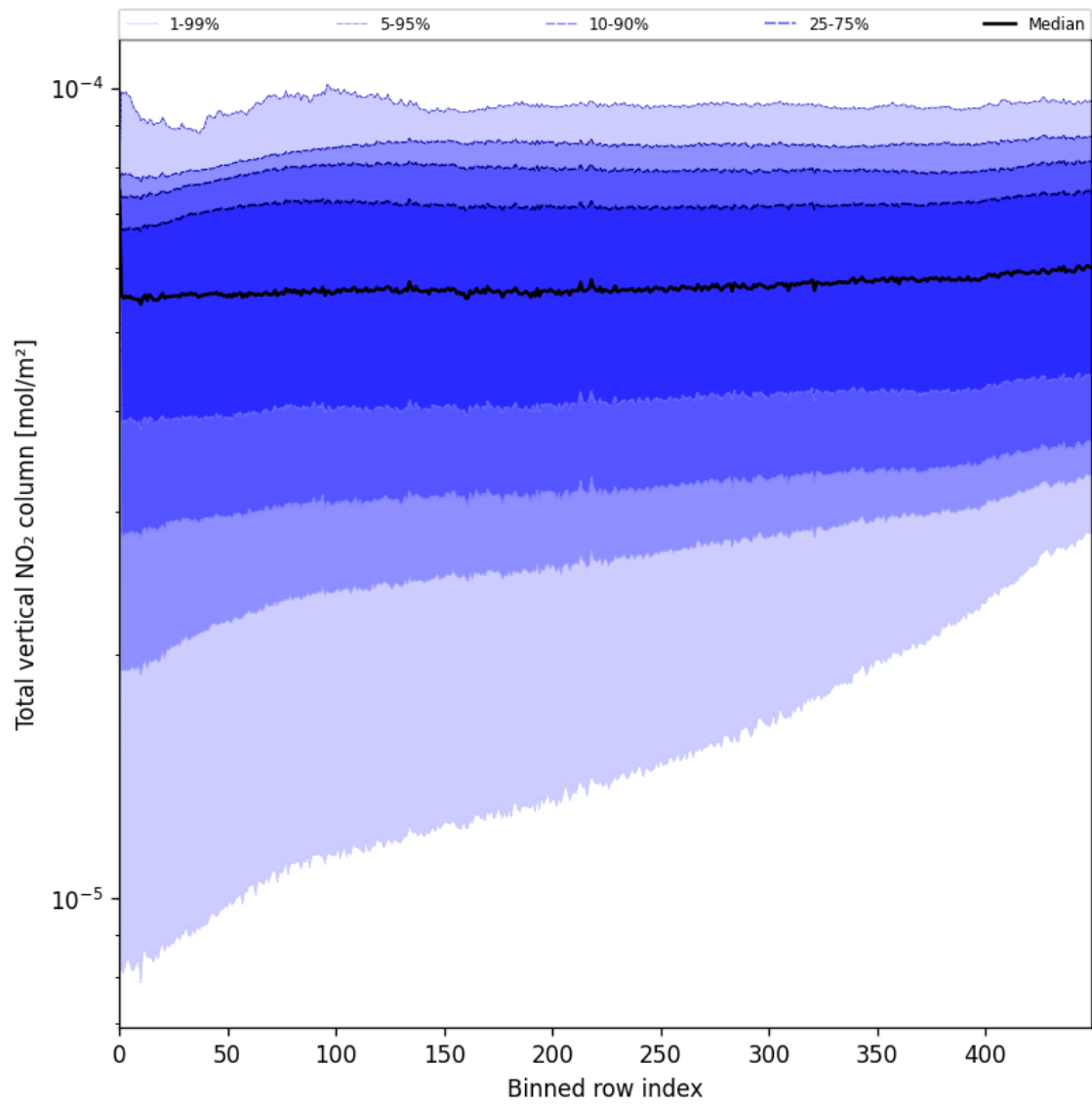
Figure 53: Along track statistics of “Total vertical NO 2 column” for 2025-08-11 to 2025-08-12
