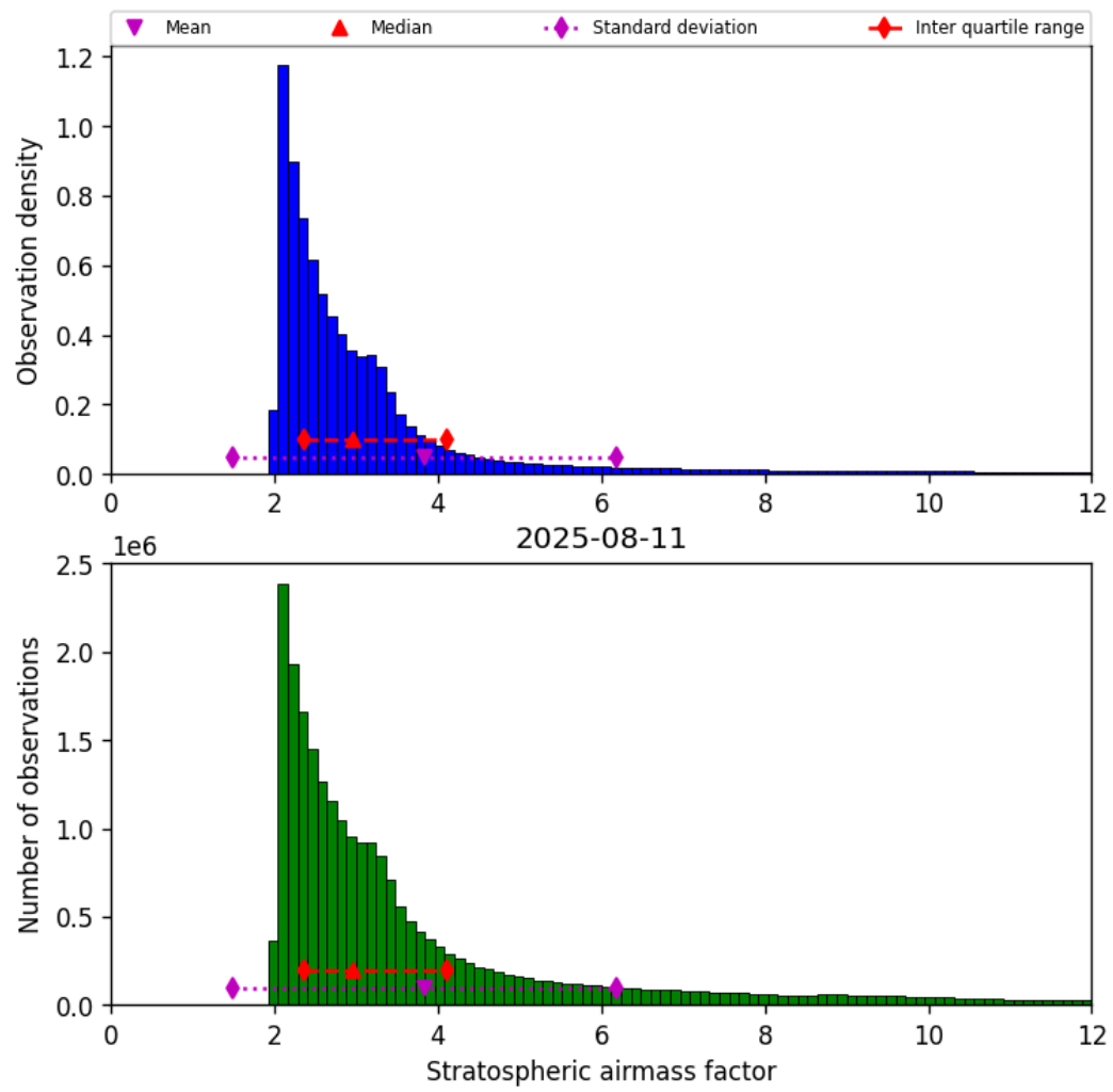
Figure 42: Histogram of “Stratospheric airmass factor” for 2025-08-11 to 2025-08-12
