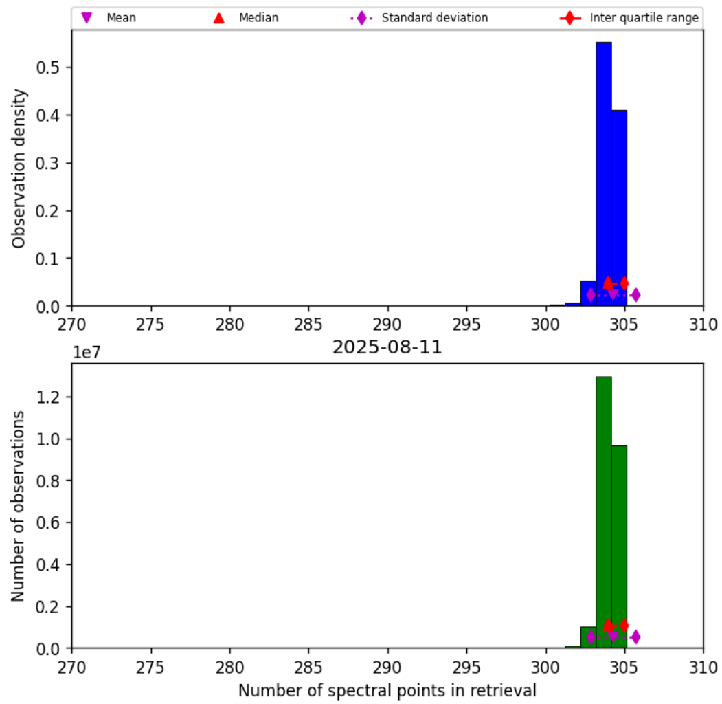
Figure 31: Histogram of “Number of spectral points in retrieval” for 2025-08-11 to 2025-08-12
