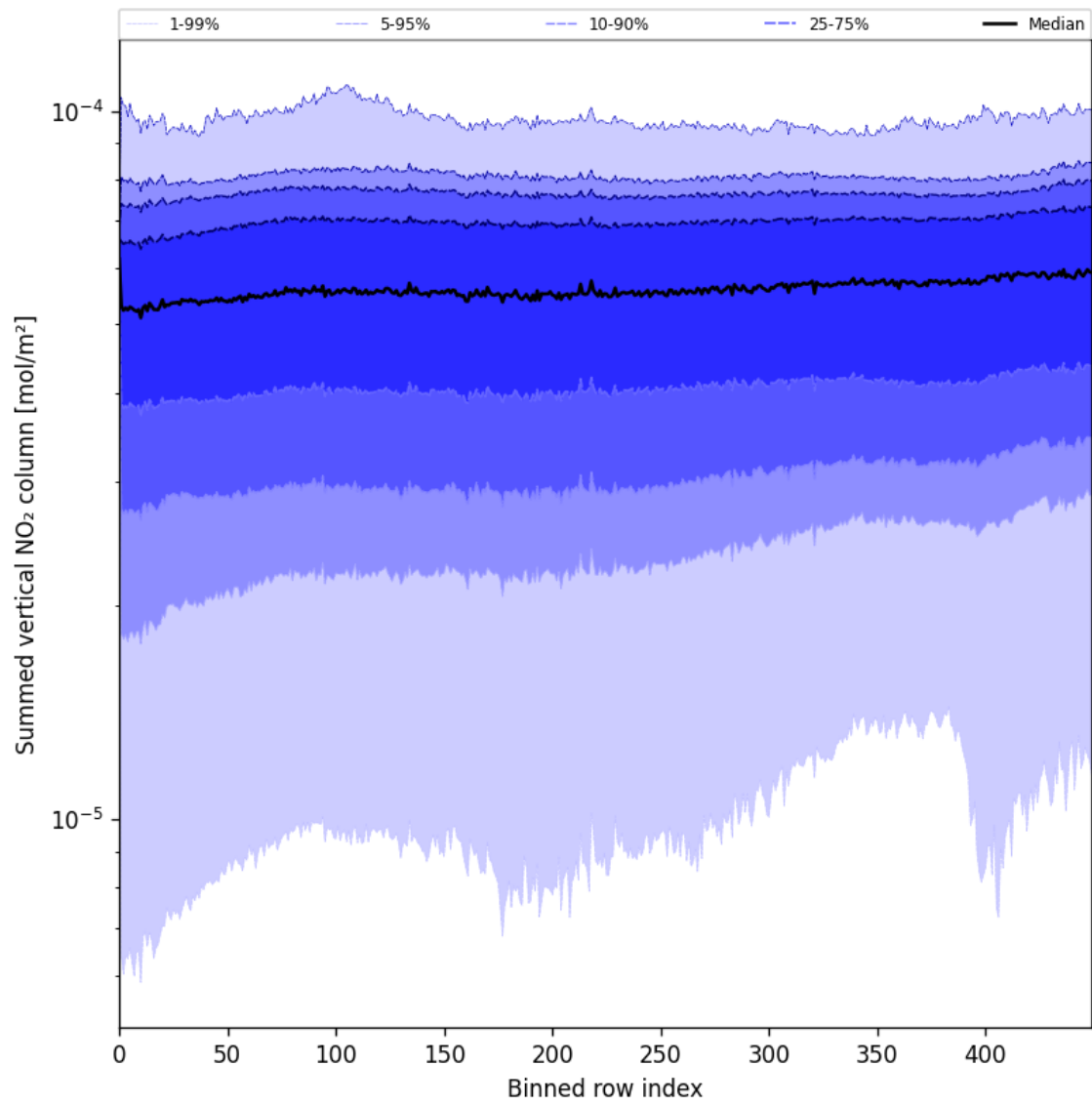
Figure 55: Along track statistics of “Summed vertical NO 2 column” for 2025-08-11 to 2025-08-12
