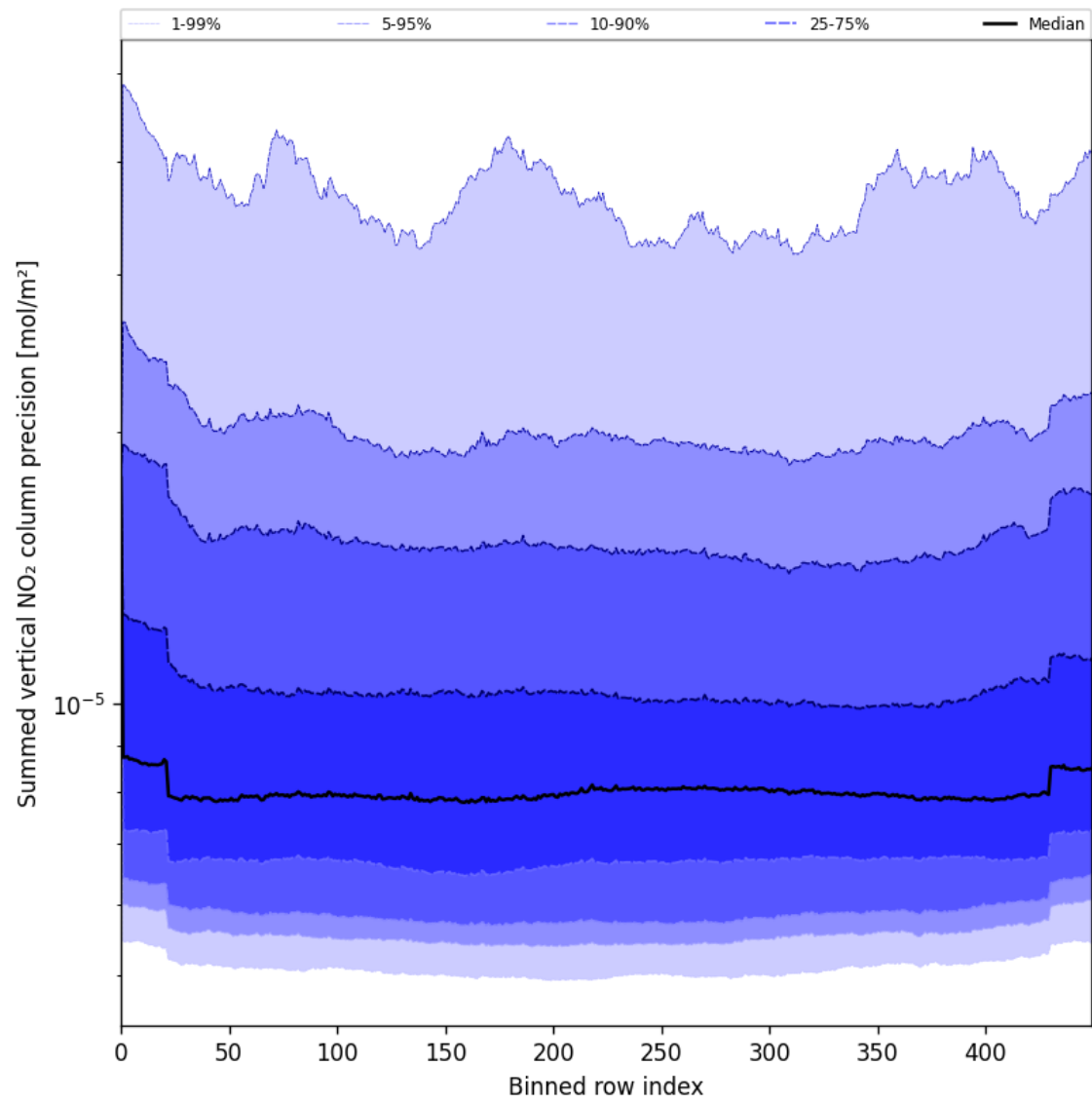
Figure 56: Along track statistics of “Summed vertical NO 2 column precision” for 2025-08-11 to 2025-08-12
