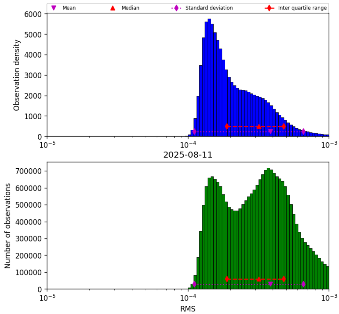
Figure 41: Histogram of “RMS” for 2025-08-11 to 2025-08-12
