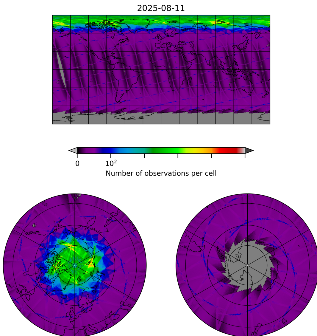
Figure 8: Map of the number of observations for 2025-08-11 to 2025-08-12
