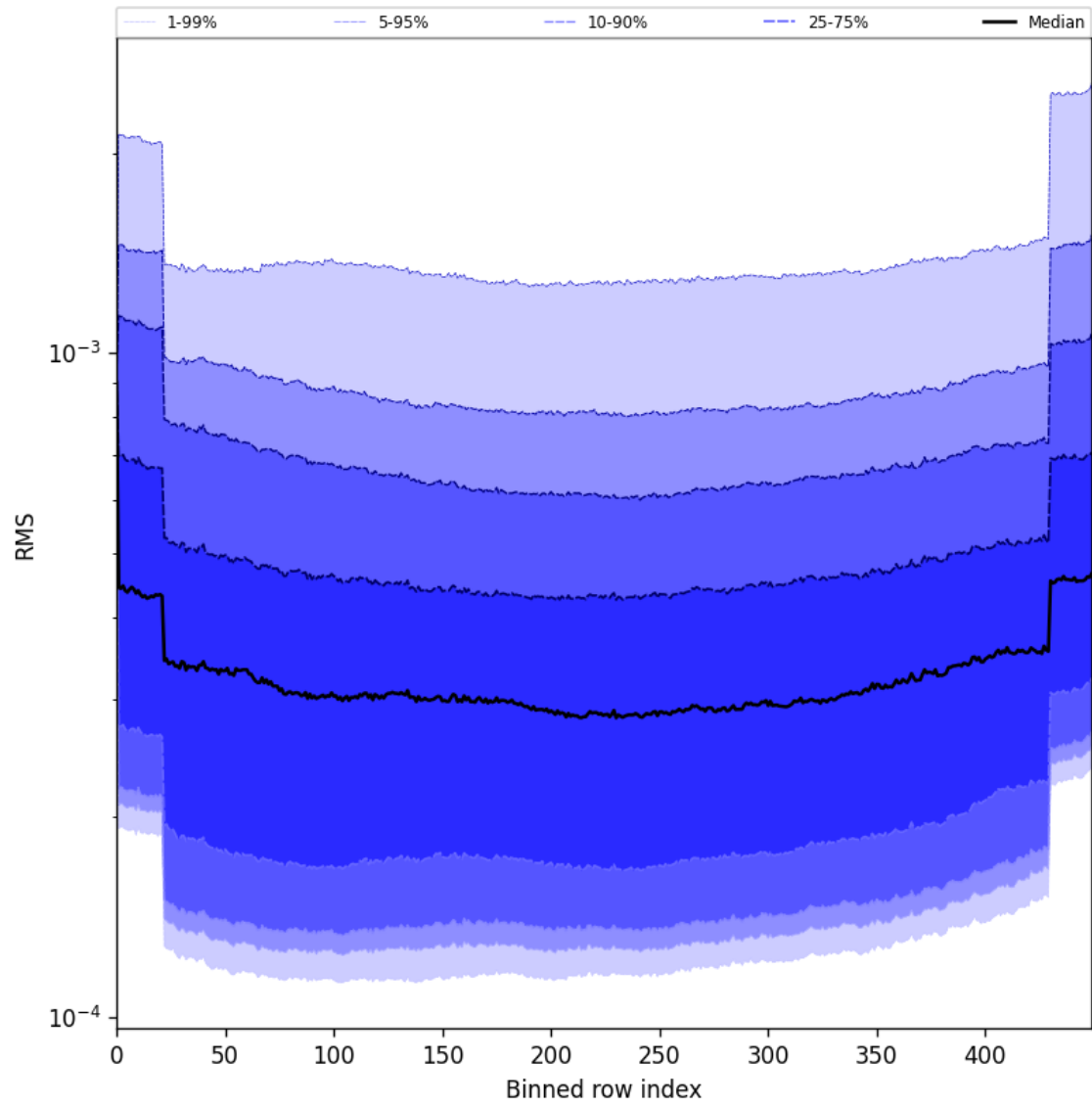
Figure 58: Along track statistics of “RMS” for 2025-08-11 to 2025-08-12
