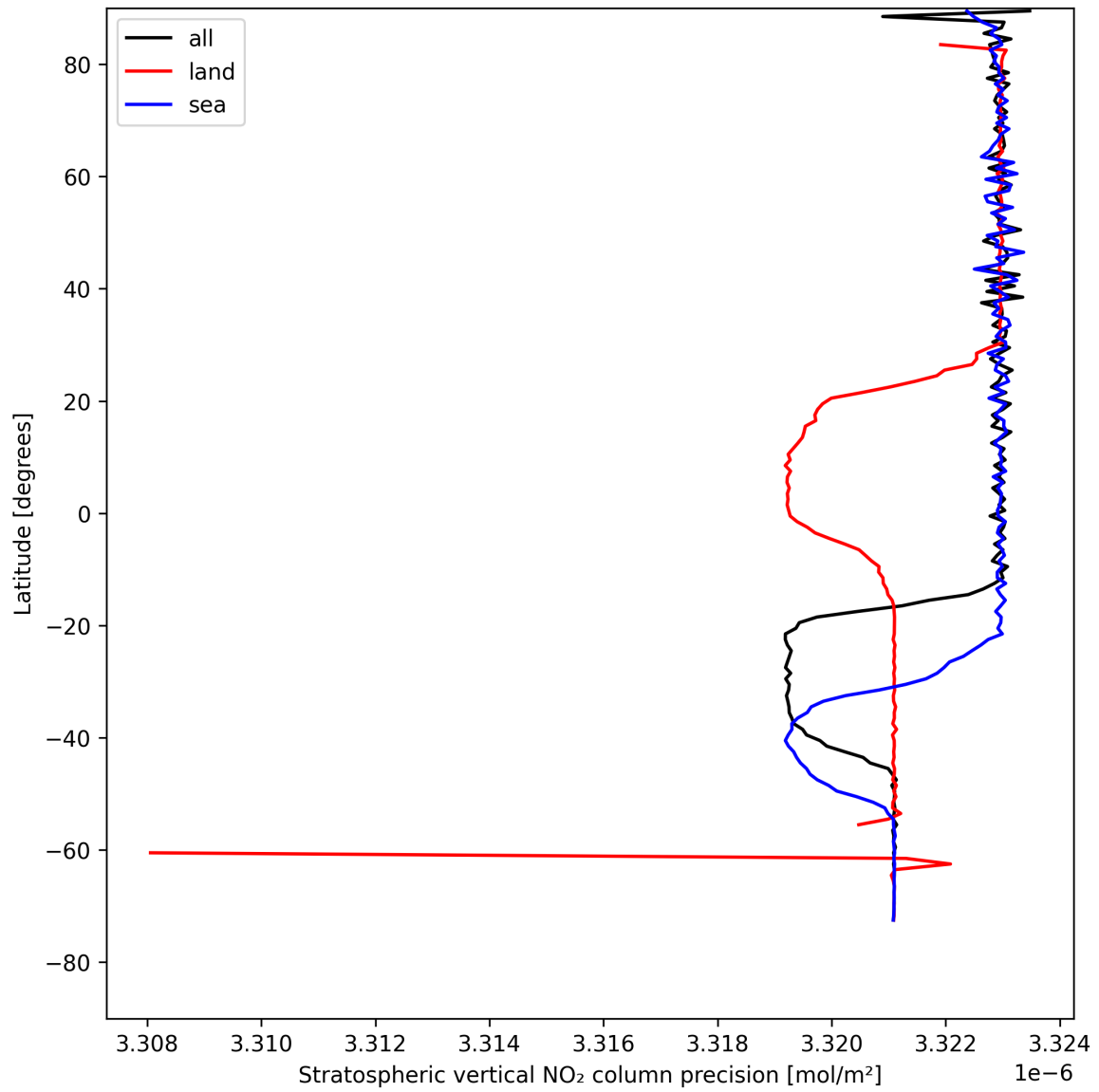
Figure 18: Zonal average of “Stratospheric vertical NO 2 column precision” for 2025-08-11 to 2025-08-12.
