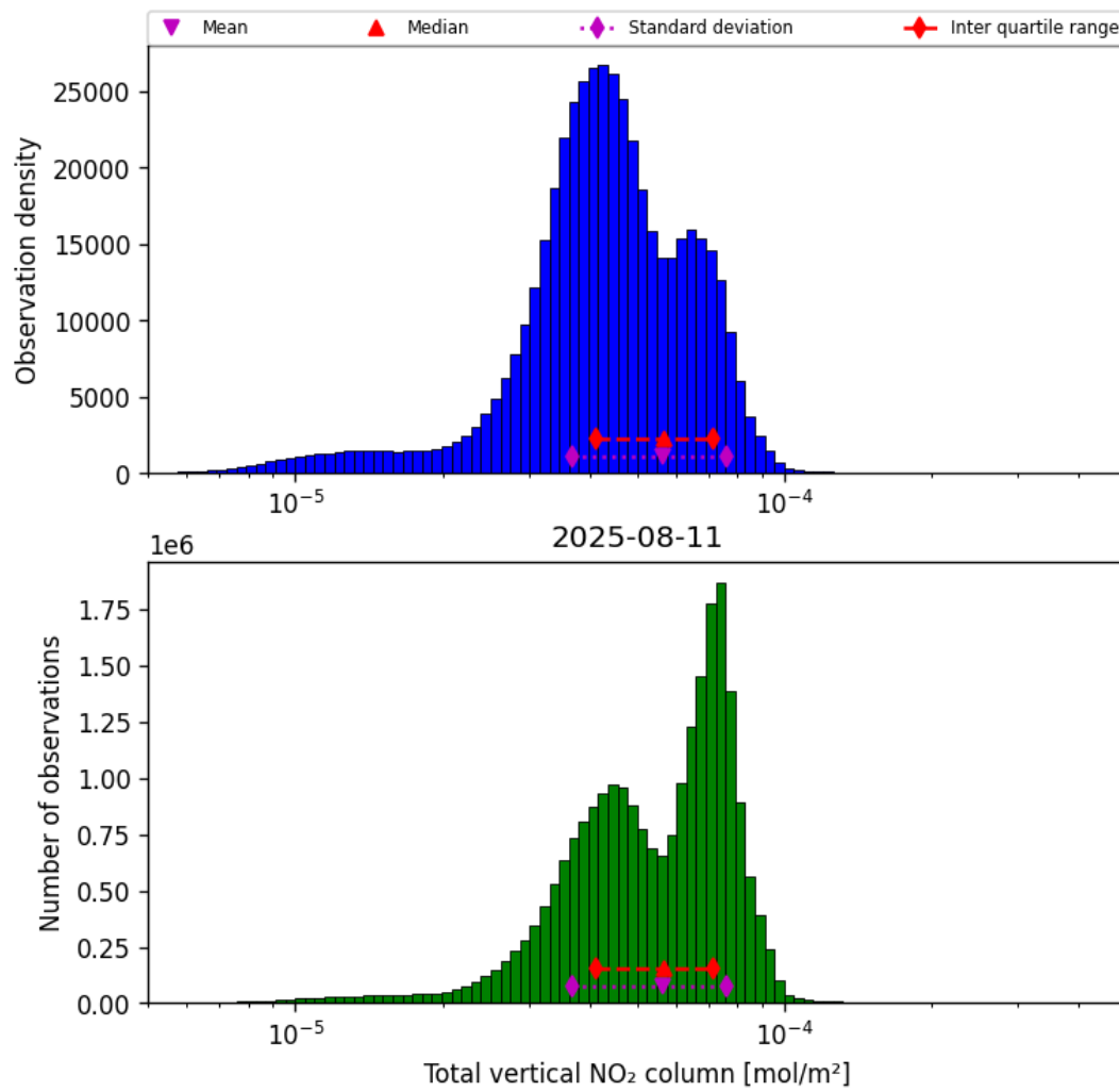
Figure 36: Histogram of “Total vertical NO 2 column” for 2025-08-11 to 2025-08-12
