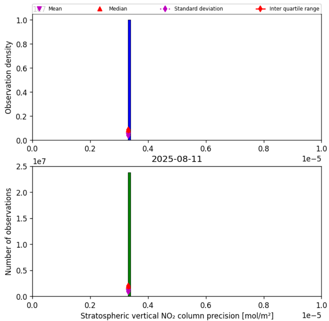
Figure 35: Histogram of “Stratospheric vertical NO 2 column precision” for 2025-08-11 to 2025-08-12
