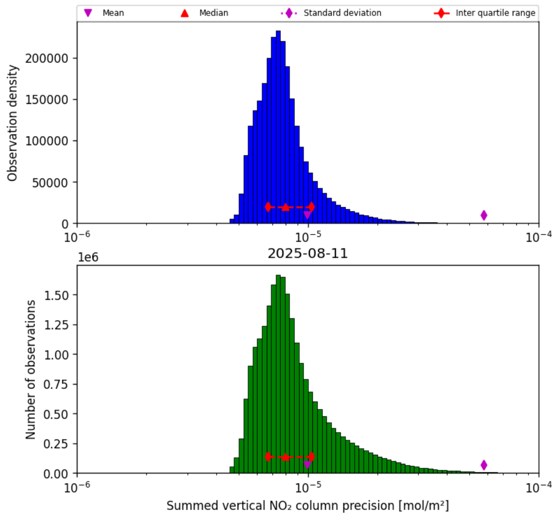
Figure 39: Histogram of “Summed vertical NO 2 column precision” for 2025-08-11 to 2025-08-12
