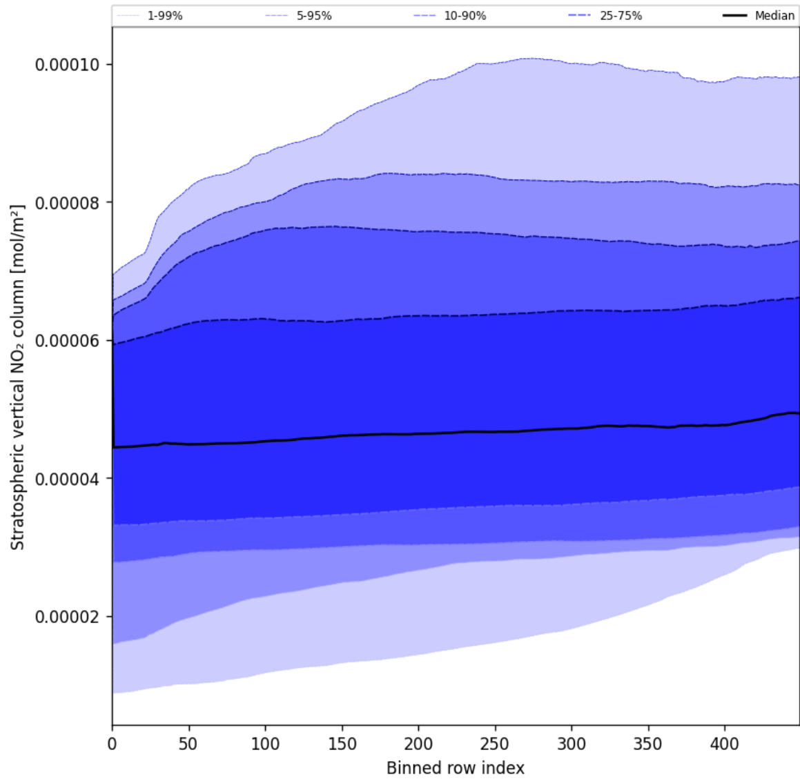
Figure 51: Along track statistics of “Stratospheric vertical NO 2 column” for 2025-08-11 to 2025-08-12
