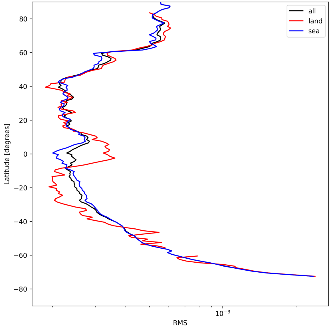
Figure 24: Zonal average of “RMS” for 2025-08-11 to 2025-08-12.
