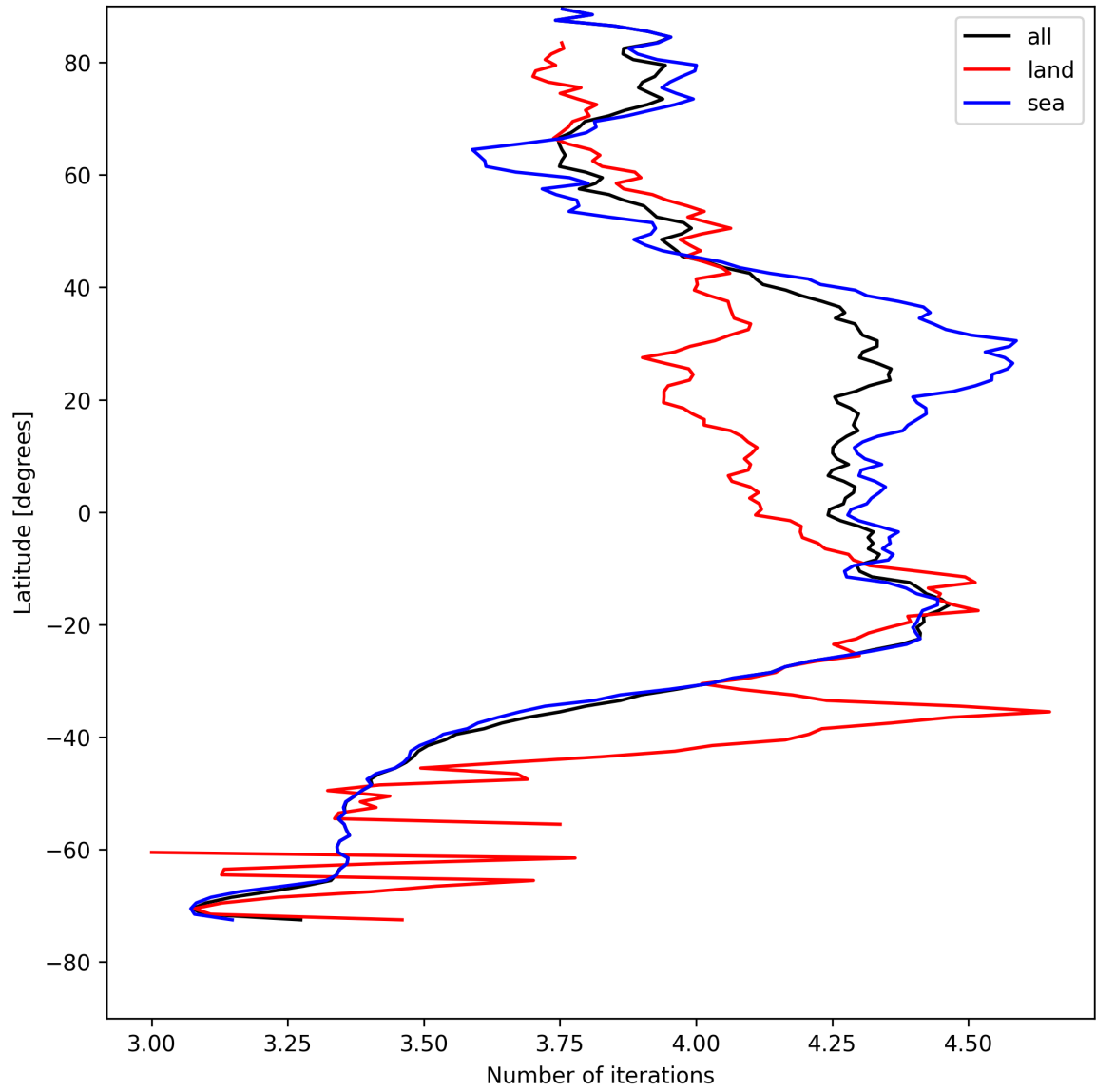
Figure 15: Zonal average of “Number of iterations” for 2025-08-11 to 2025-08-12.
