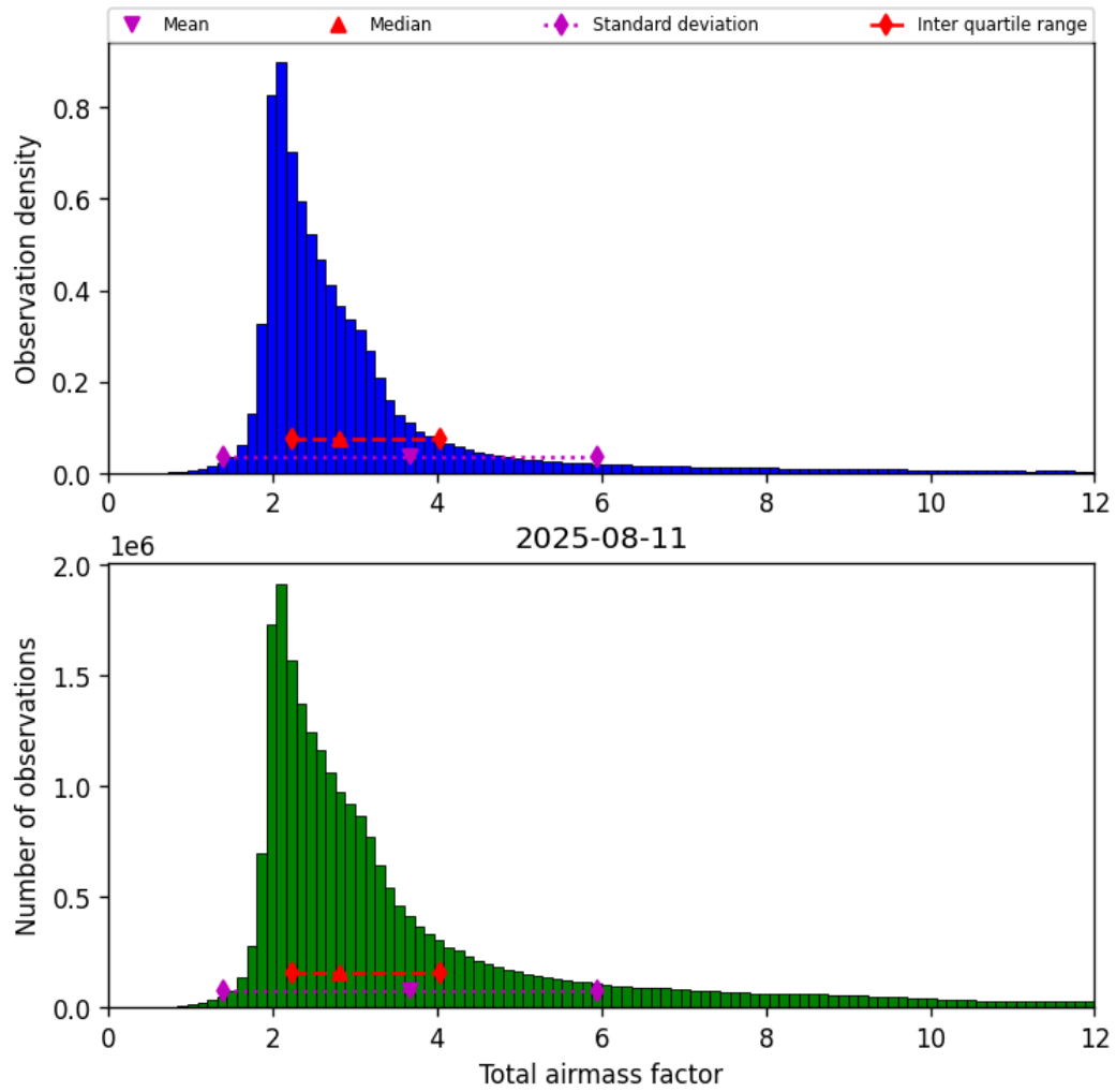
Figure 30: Histogram of “Total airmass factor” for 2025-08-11 to 2025-08-12
