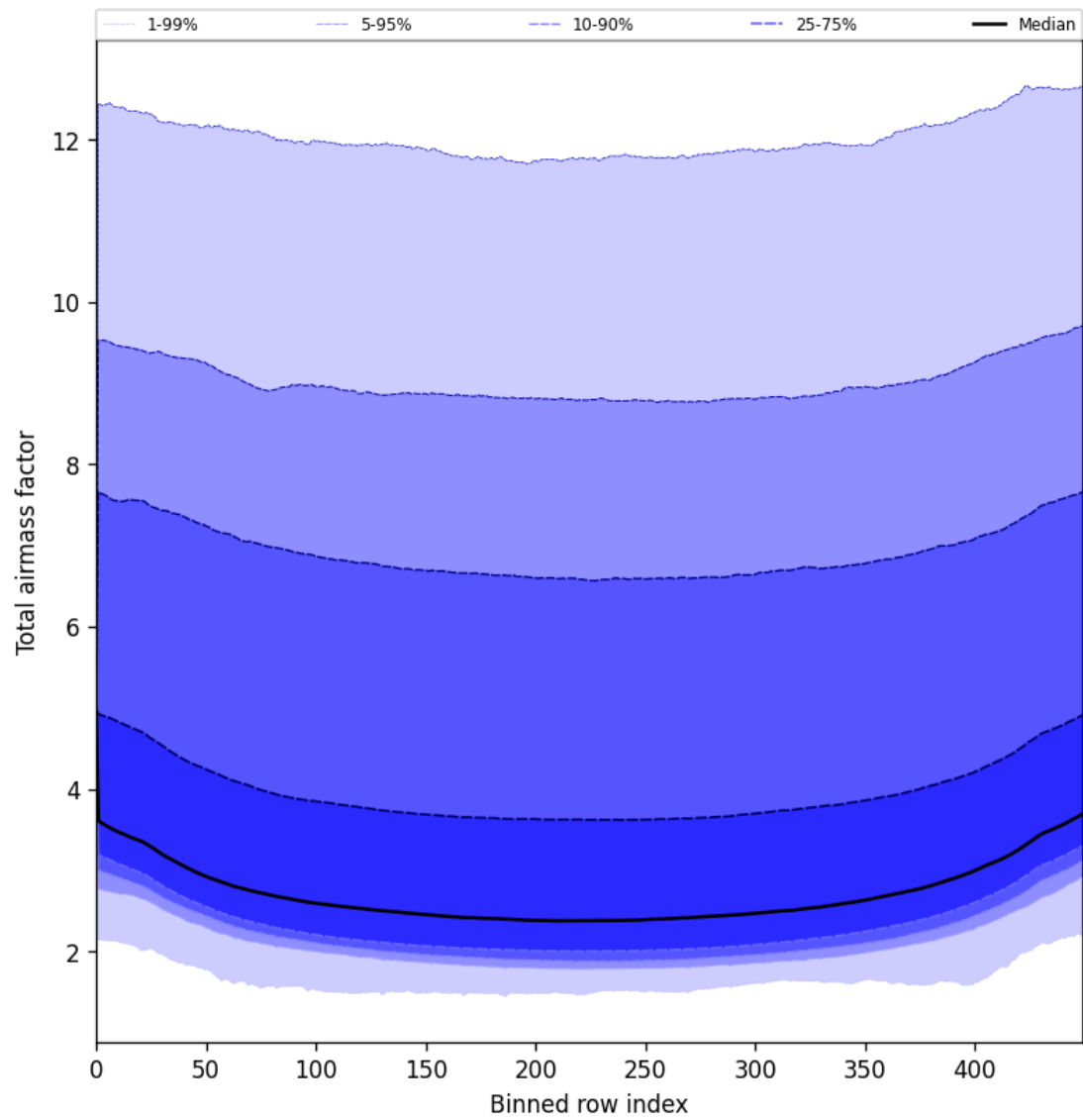
Figure 47: Along track statistics of “Total airmass factor” for 2025-08-11 to 2025-08-12
