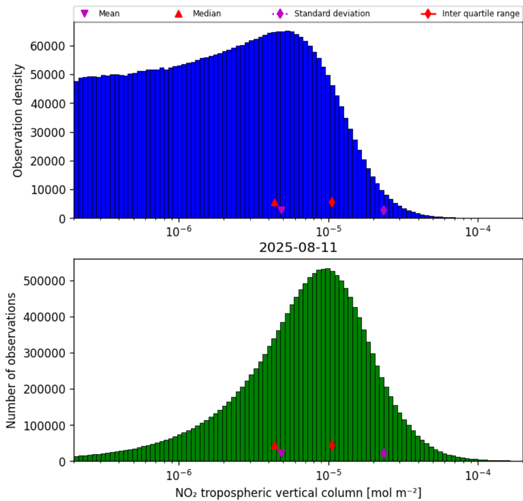
Figure 27: Histogram of “NO 2 tropospheric vertical column” for 2025-08-11 to 2025-08-12
