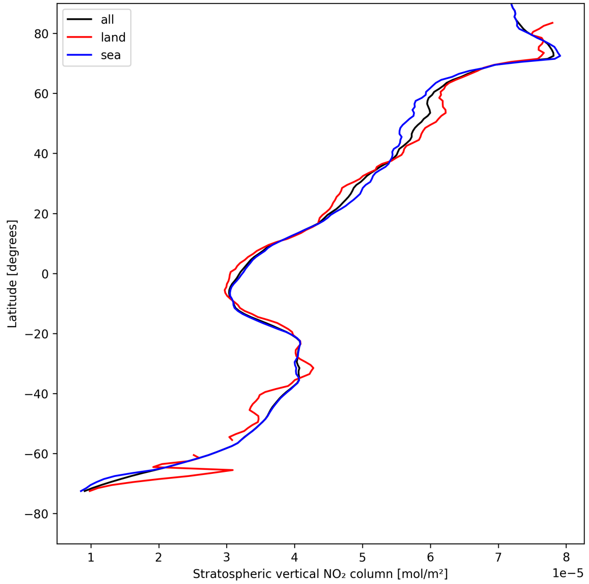
Figure 17: Zonal average of “Stratospheric vertical NO 2 column” for 2025-08-11 to 2025-08-12.
