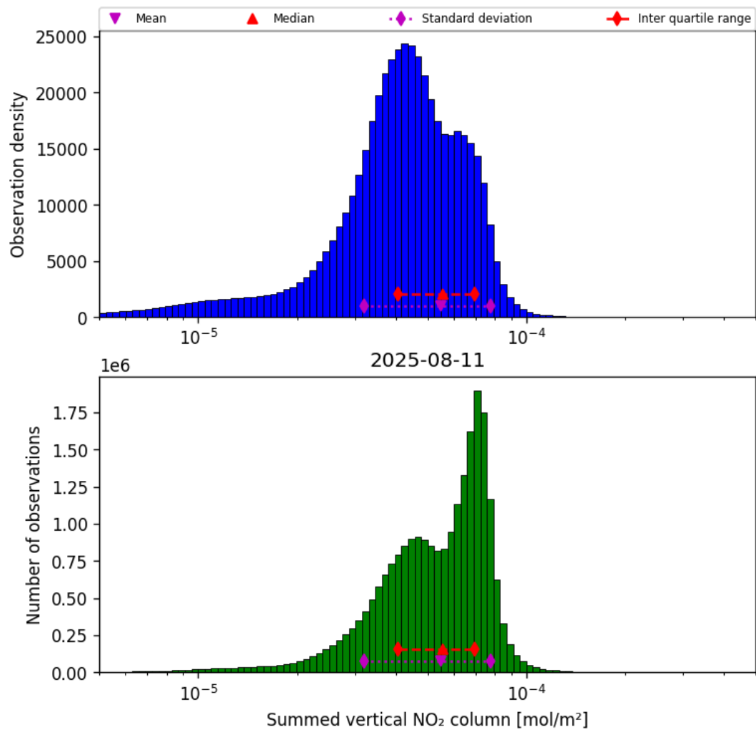
Figure 38: Histogram of “Summed vertical NO 2 column” for 2025-08-11 to 2025-08-12
