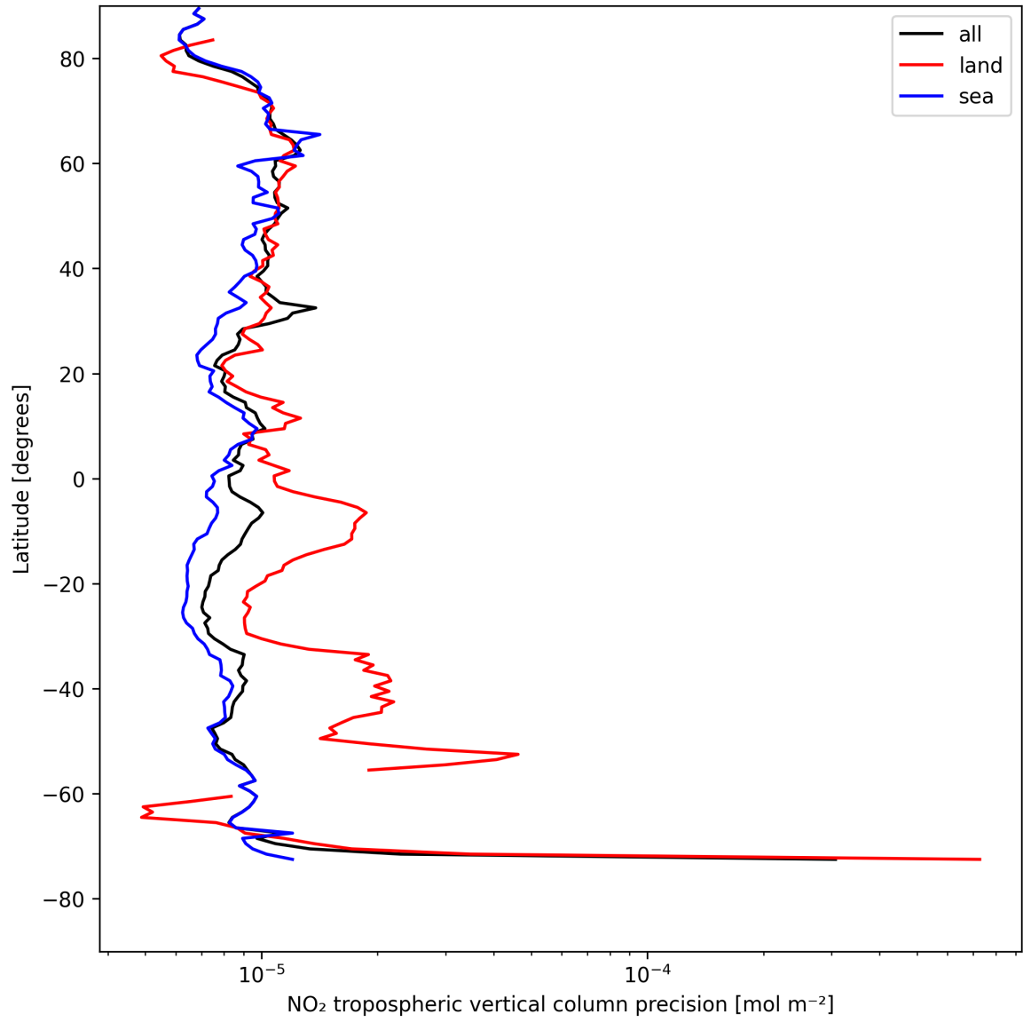
Figure 11: Zonal average of “NO 2 tropospheric vertical column precision” for 2025-08-11 to 2025-08-12.
