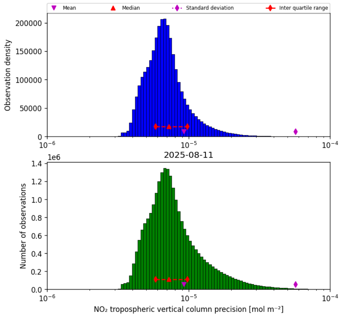
Figure 28: Histogram of “NO 2 tropospheric vertical column precision” for 2025-08-11 to 2025-08-12
