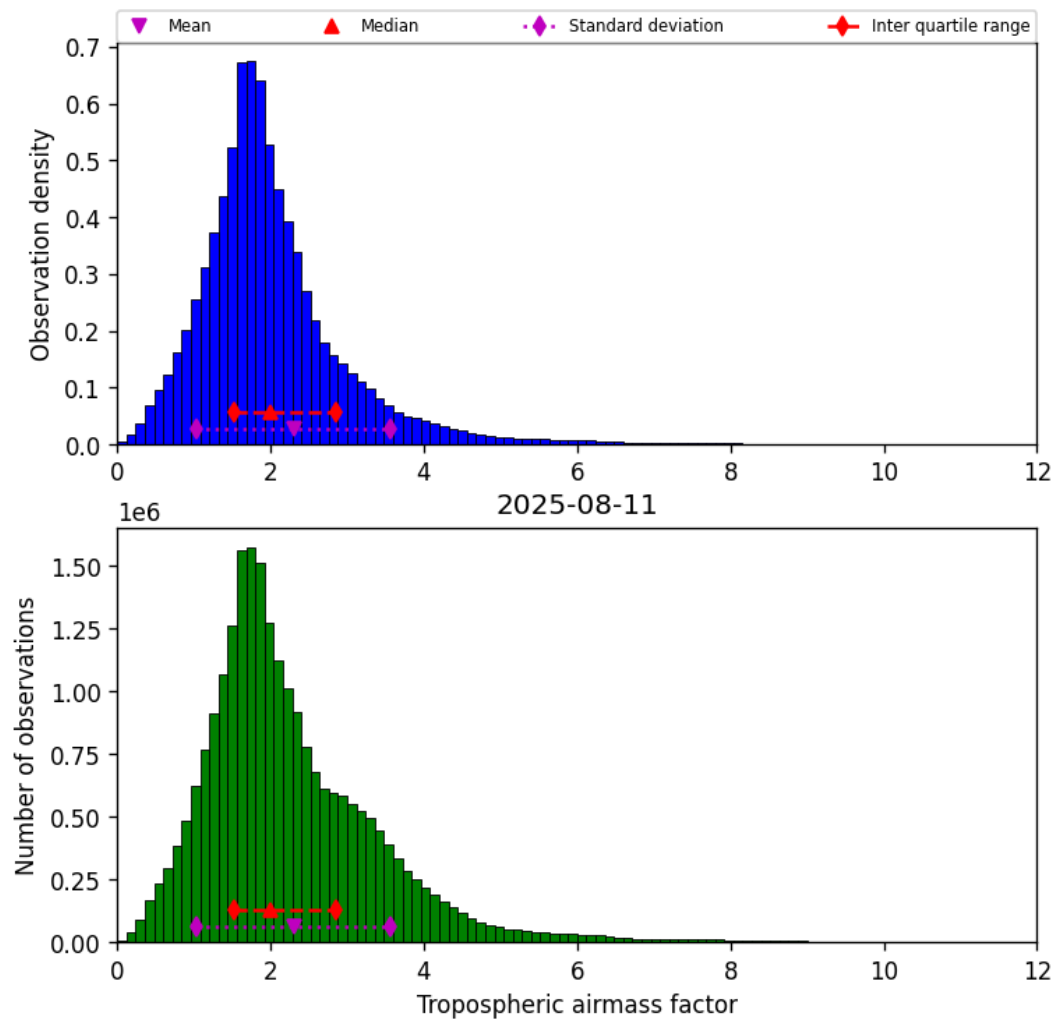
Figure 29: Histogram of “Tropospheric airmass factor” for 2025-08-11 to 2025-08-12
