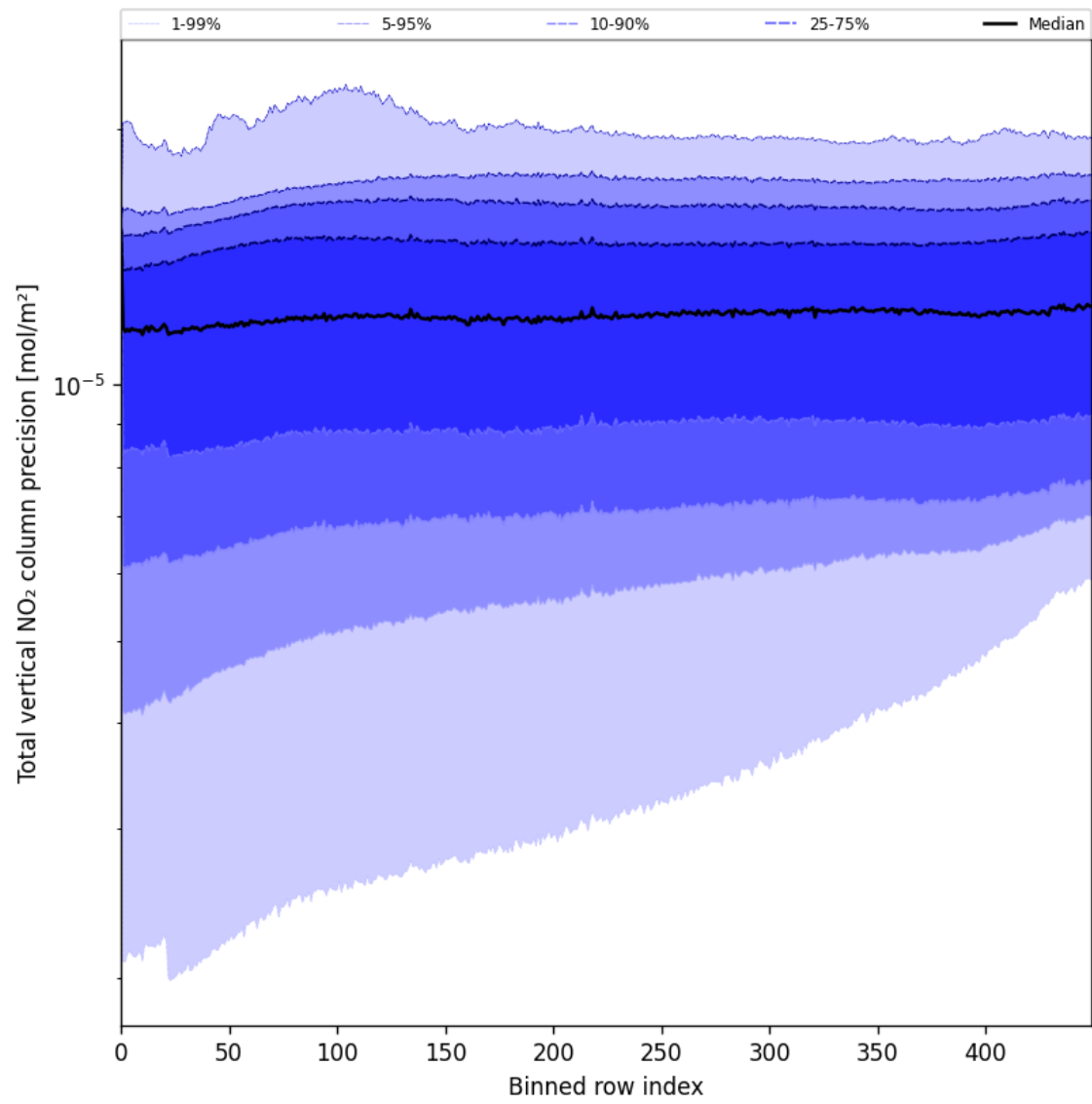
Figure 54: Along track statistics of “Total vertical NO 2 column precision” for 2025-08-11 to 2025-08-12
