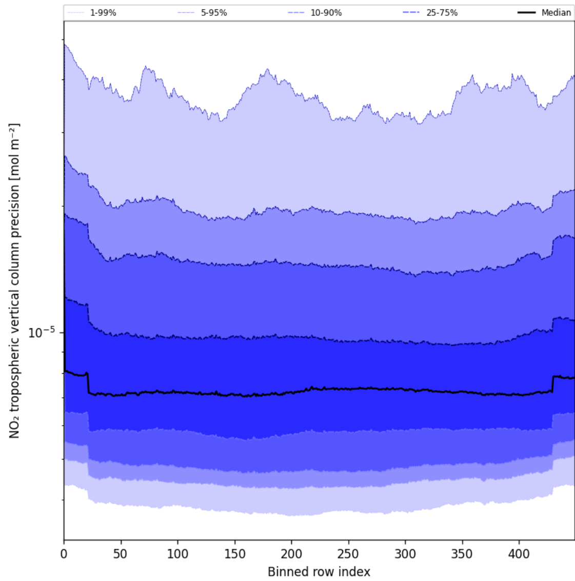
Figure 45: Along track statistics of “NO 2 tropospheric vertical column precision” for 2025-08-11 to 2025-08-12
