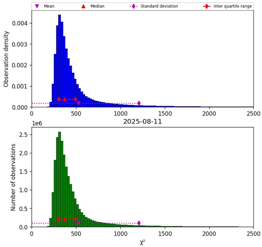
Figure 40: Histogram of “ \chi^2 ” for 2025-08-11 to 2025-08-12
