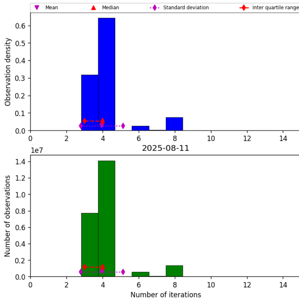
Figure 32: Histogram of “Number of iterations” for 2025-08-11 to 2025-08-12
