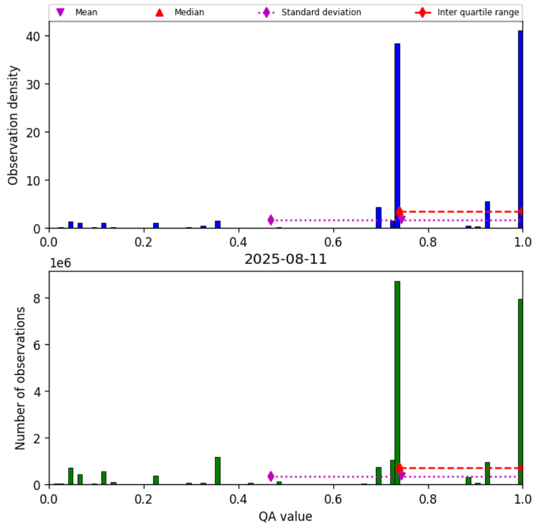
Figure 26: Histogram of “QA value” for 2025-08-11 to 2025-08-12
