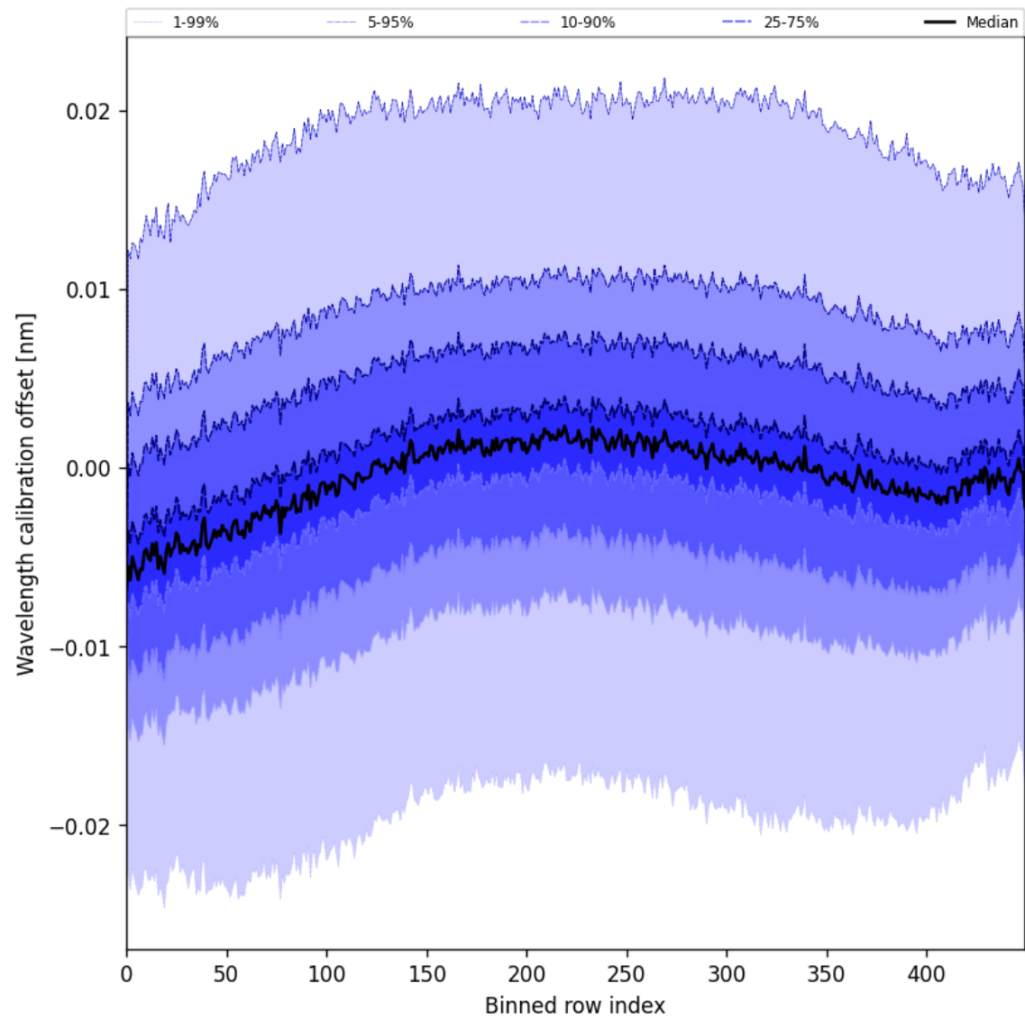
Figure 50: Along track statistics of “Wavelength calibration offset” for 2025-08-11 to 2025-08-12
