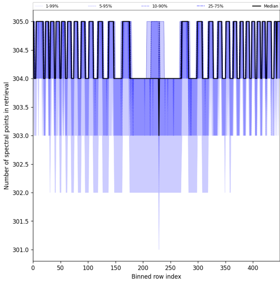
Figure 48: Along track statistics of “Number of spectral points in retrieval” for 2025-08-11 to 2025-08-12
