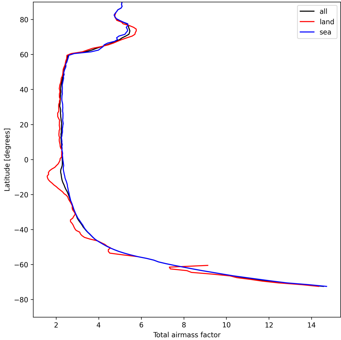
Figure 13: Zonal average of “Total airmass factor” for 2025-08-11 to 2025-08-12.
