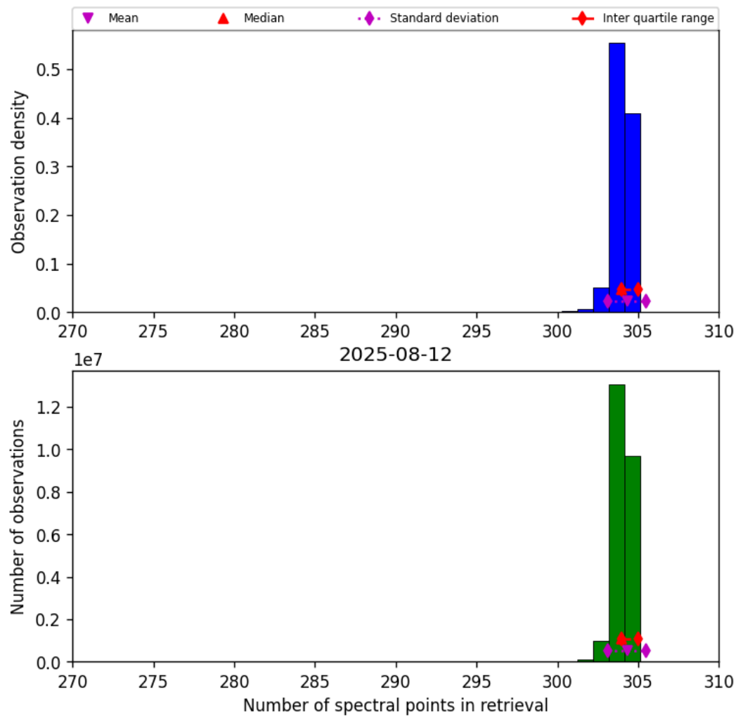
Figure 31: Histogram of “Number of spectral points in retrieval” for 2025-08-12 to 2025-08-12
