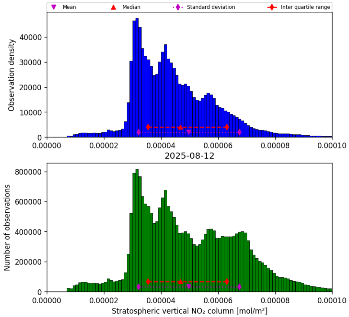
Figure 34: Histogram of “Stratospheric vertical NO 2 column” for 2025-08-12 to 2025-08-12
