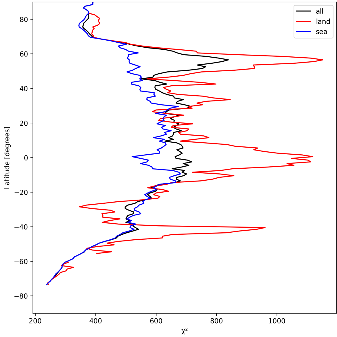
Figure 23: Zonal average of “ \chi^2 ” for 2025-08-12 to 2025-08-12.
