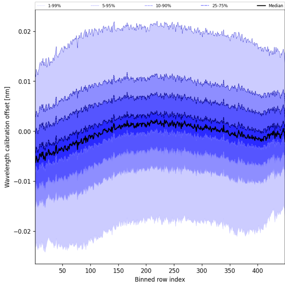
Figure 50: Along track statistics of “Wavelength calibration offset” for 2025-08-12 to 2025-08-12
