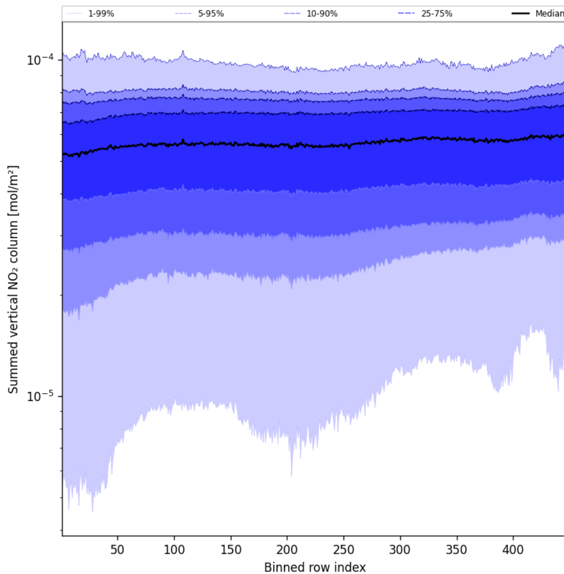
Figure 55: Along track statistics of “Summed vertical NO 2 column” for 2025-08-12 to 2025-08-12
