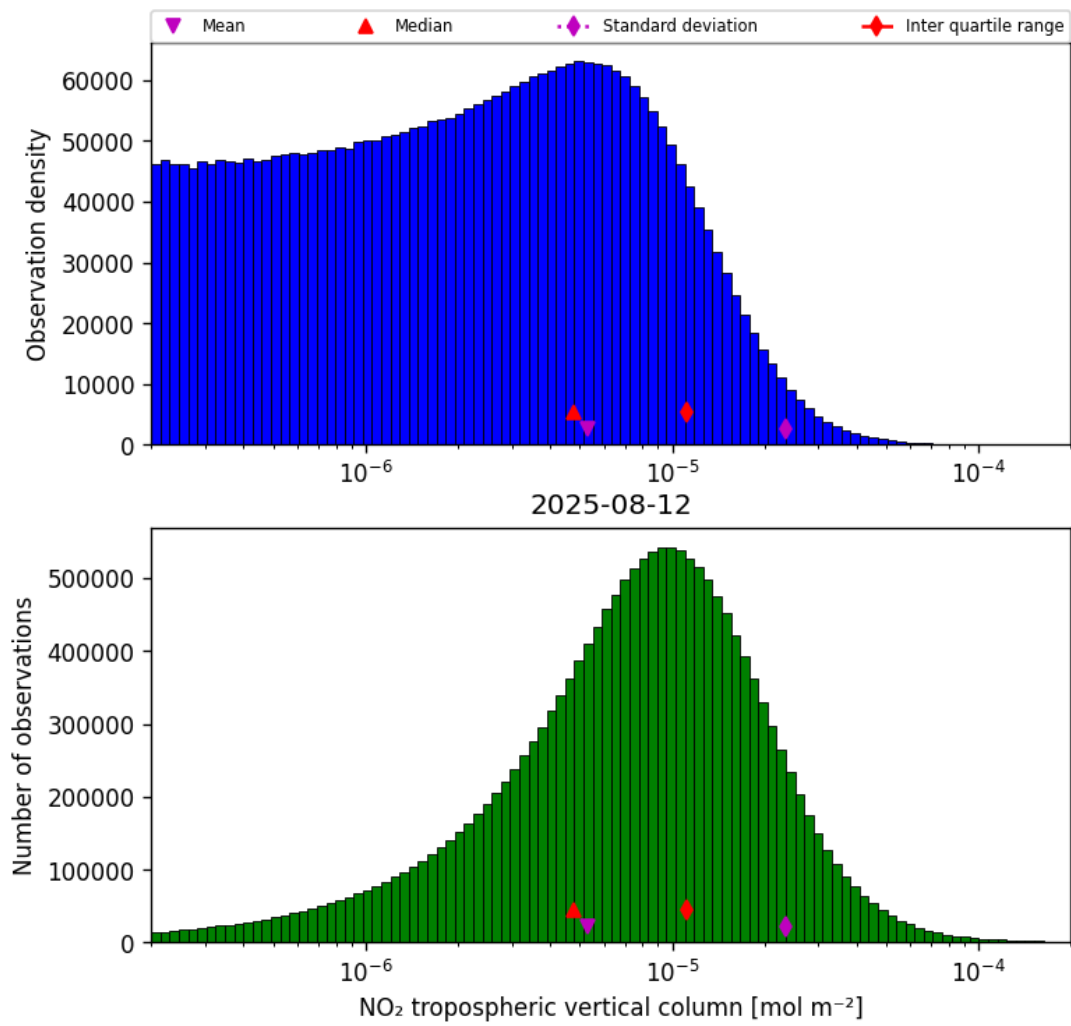
Figure 27: Histogram of “NO 2 tropospheric vertical column” for 2025-08-12 to 2025-08-12
