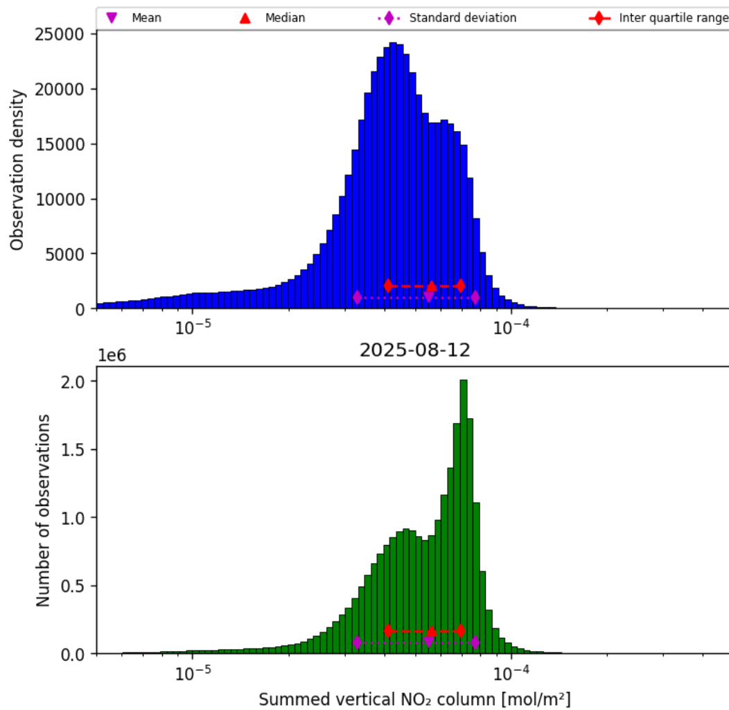
Figure 38: Histogram of "Summed vertical NO 2 column" for 2025-08-12 to 2025-08-12
