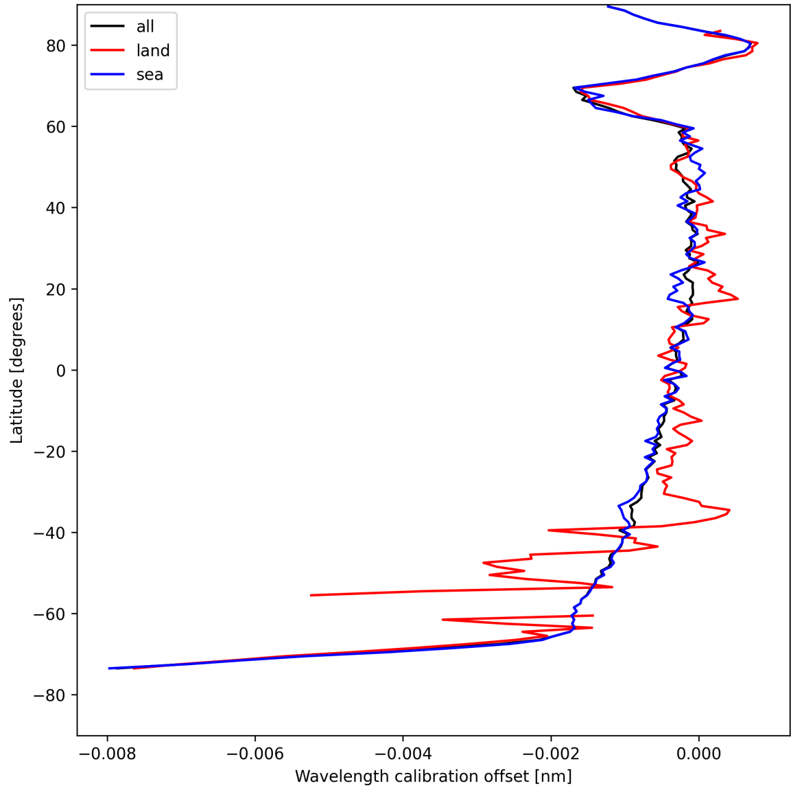
Figure 16: Zonal average of “Wavelength calibration offset” for 2025-08-12 to 2025-08-12.
