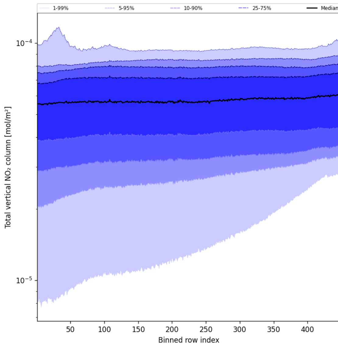
Figure 53: Along track statistics of “Total vertical NO 2 column” for 2025-08-12 to 2025-08-12
