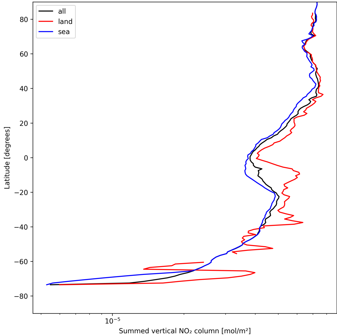
Figure 21: Zonal average of “Summed vertical NO 2 column” for 2025-08-12 to 2025-08-12.
