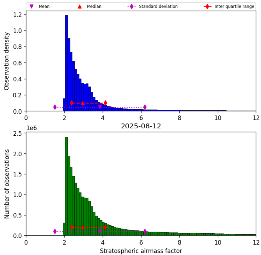
Figure 42: Histogram of “Stratospheric airmass factor” for 2025-08-12 to 2025-08-12
