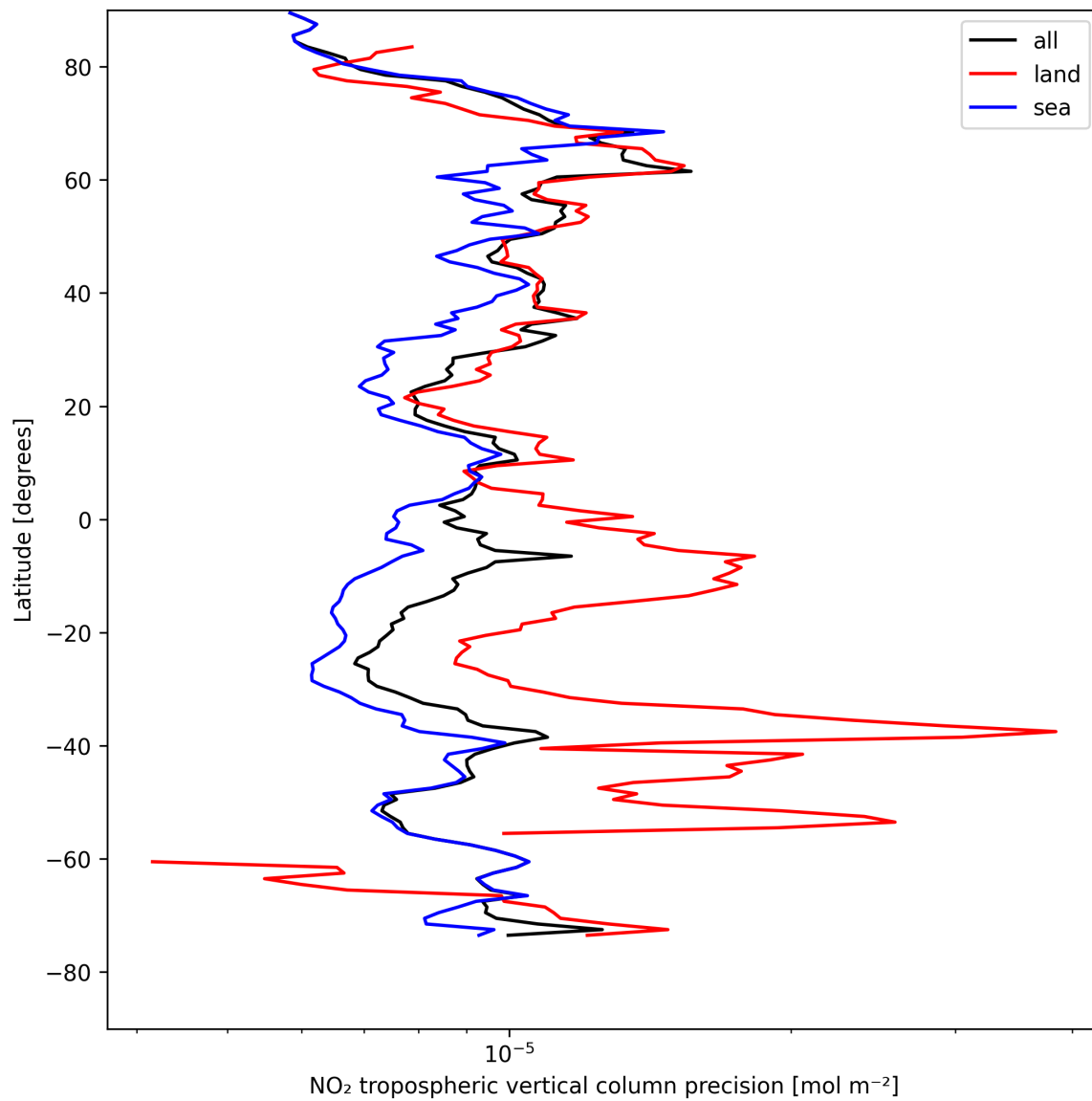
Figure 11: Zonal average of “NO 2 tropospheric vertical column precision” for 2025-08-12 to 2025-08-12.
