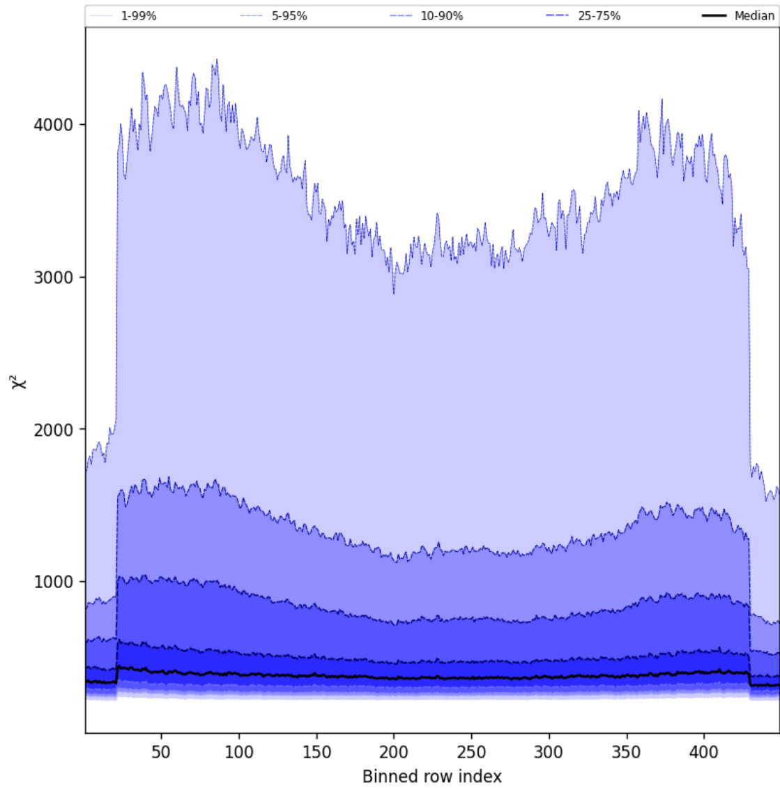
Figure 57: Along track statistics of “ \chi^2 ” for 2025-08-12 to 2025-08-12
