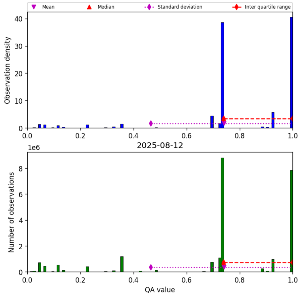
Figure 26: Histogram of “QA value” for 2025-08-12 to 2025-08-12
