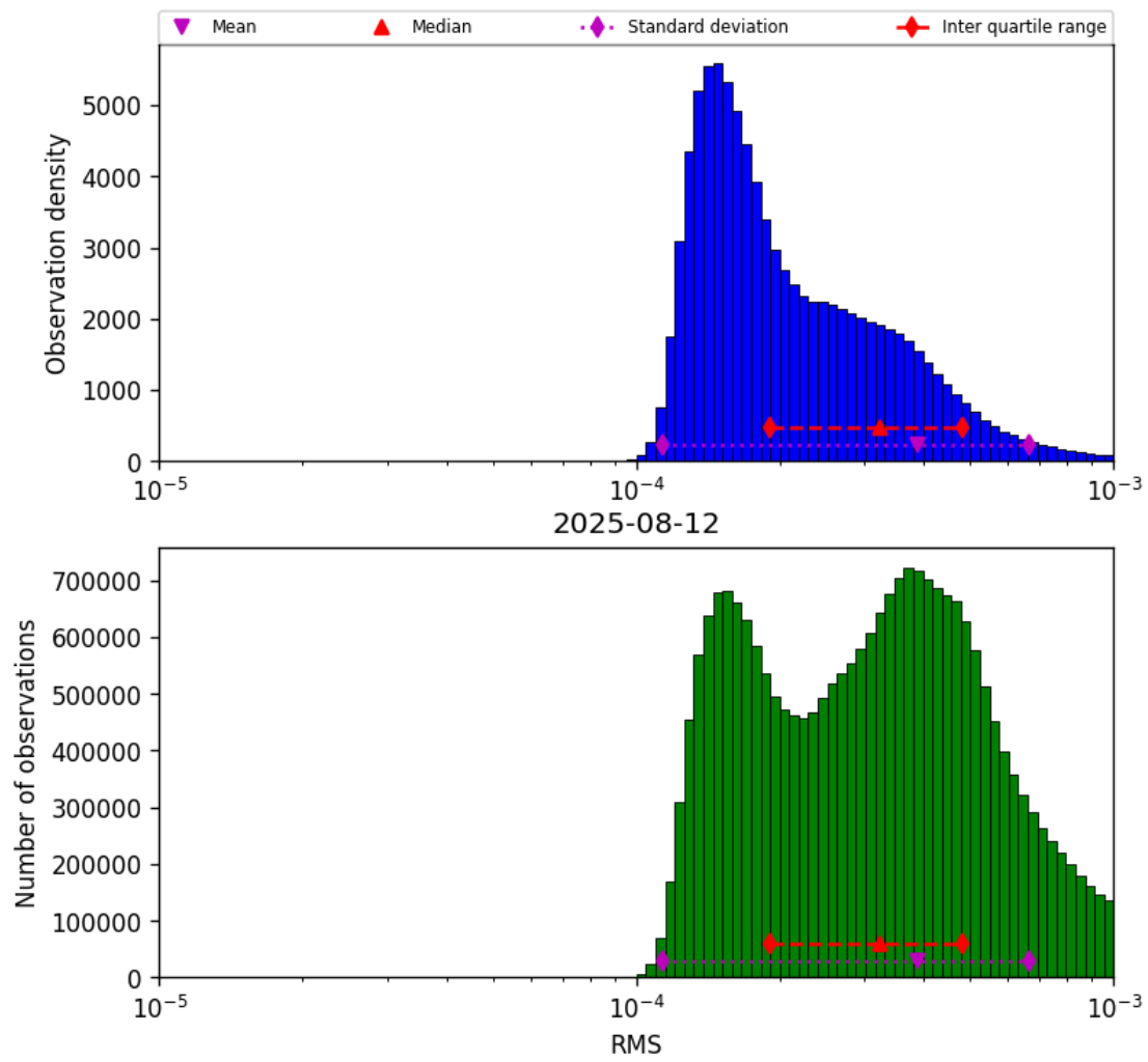
Figure 41: Histogram of “RMS” for 2025-08-12 to 2025-08-12
