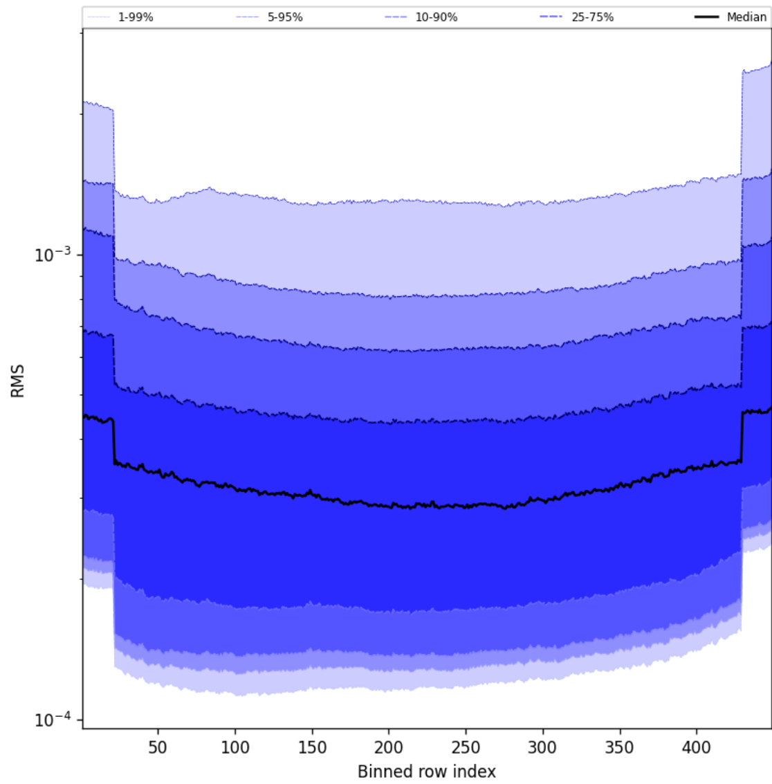
Figure 58: Along track statistics of “RMS” for 2025-08-12 to 2025-08-12
