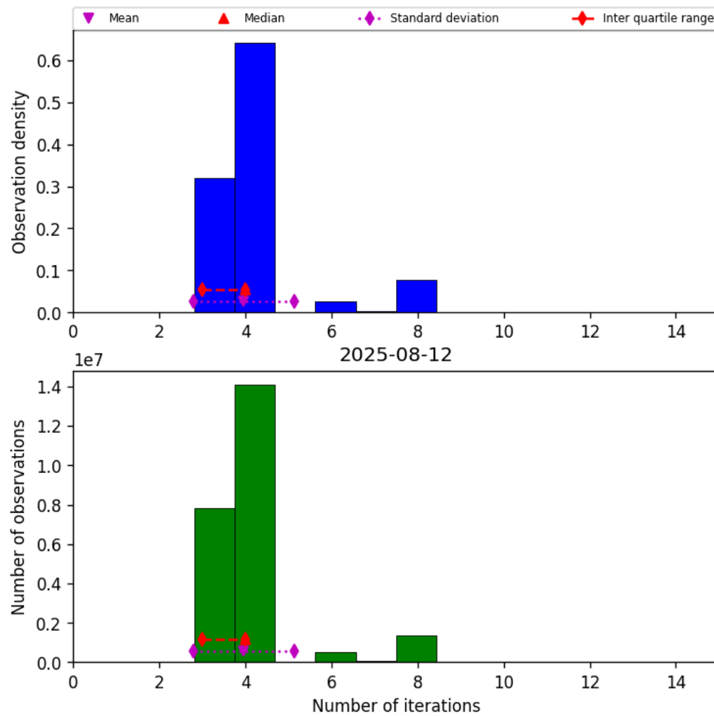
Figure 32: Histogram of “Number of iterations” for 2025-08-12 to 2025-08-12
