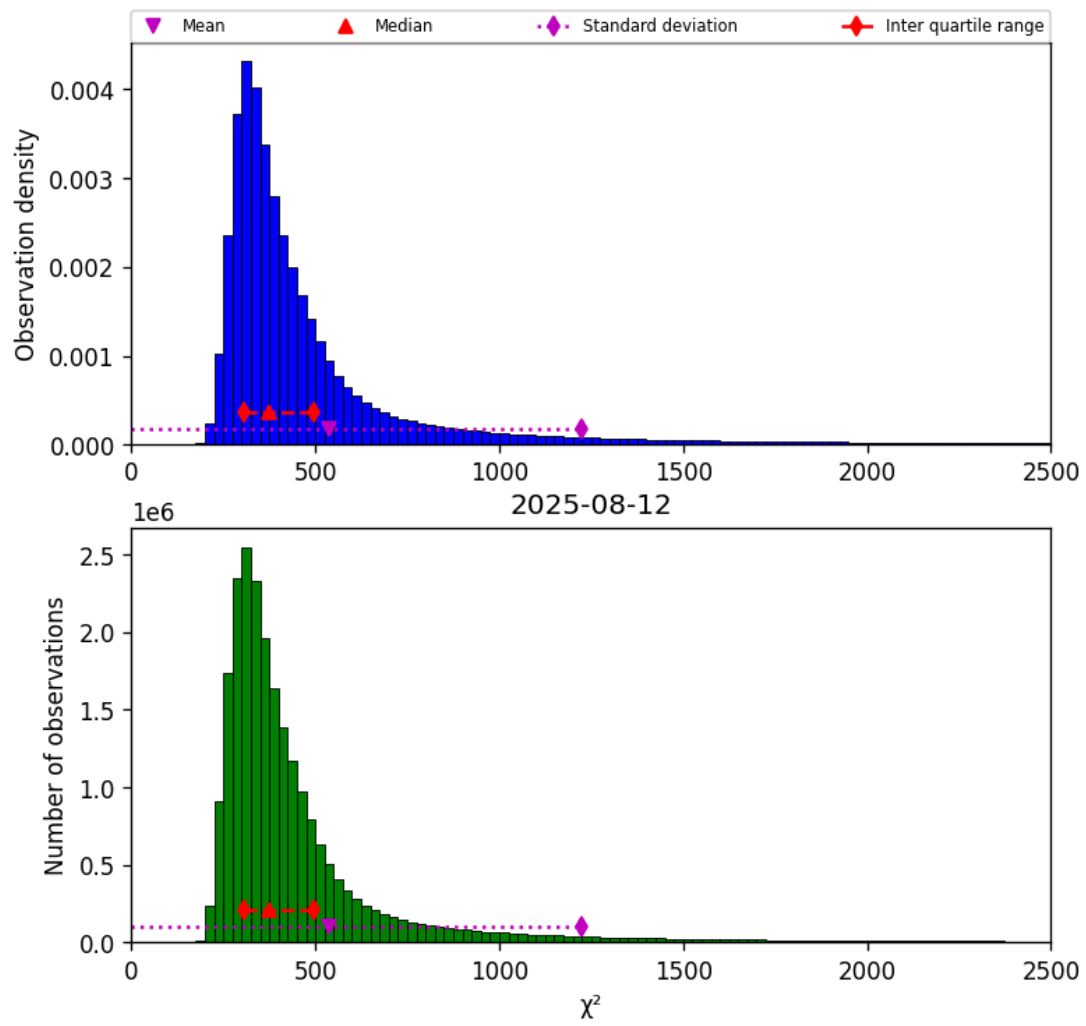
Figure 40: Histogram of “ \chi^2 ” for 2025-08-12 to 2025-08-12
