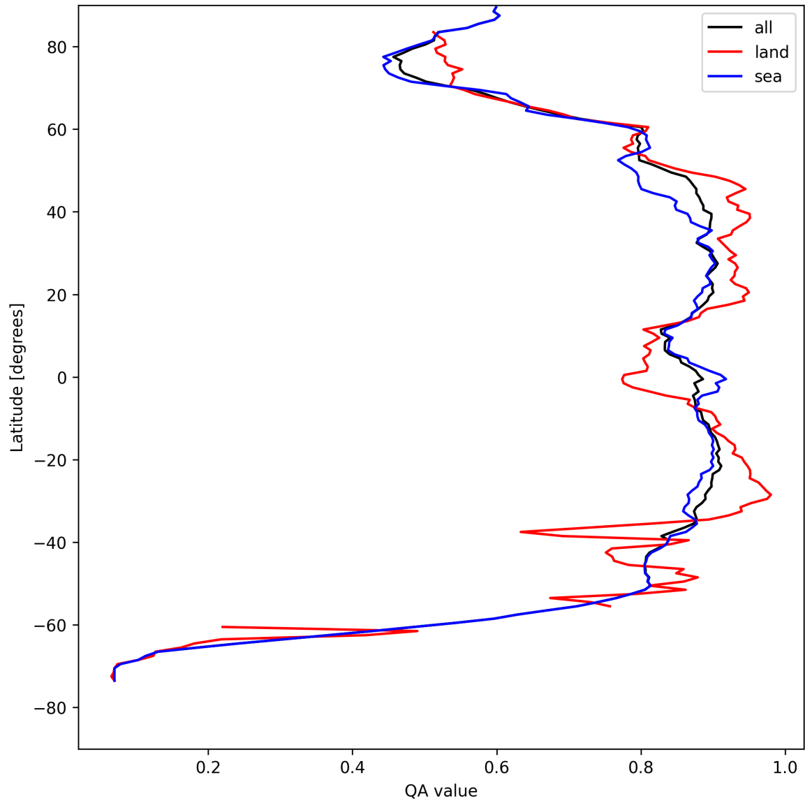
Figure 9: Zonal average of “QA value” for 2025-08-12 to 2025-08-12.
