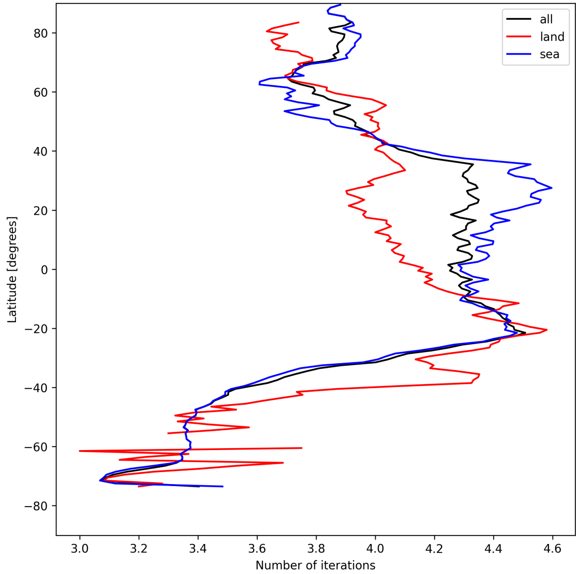
Figure 15: Zonal average of “Number of iterations” for 2025-08-12 to 2025-08-12.
