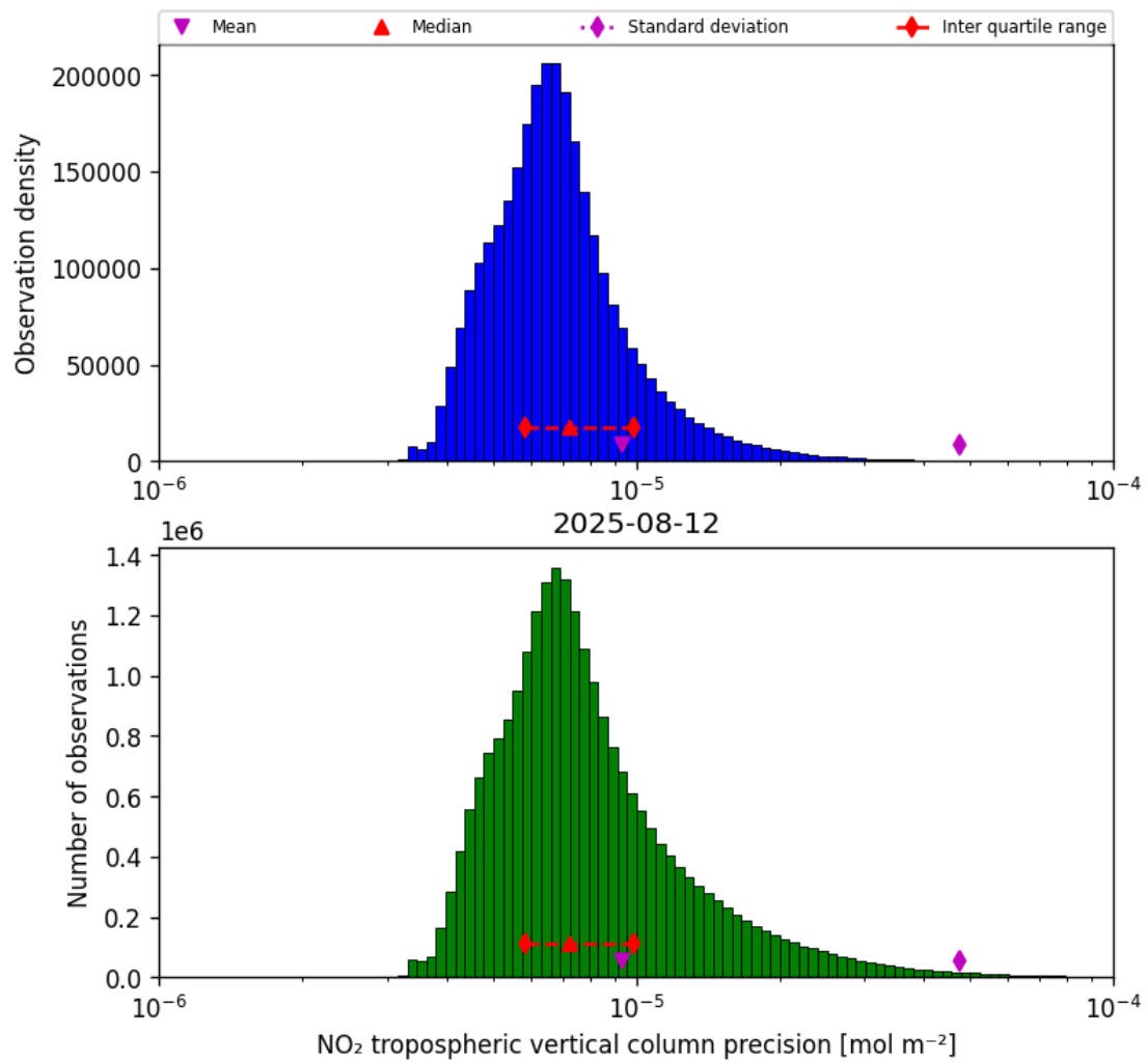
Figure 28: Histogram of “NO 2 tropospheric vertical column precision” for 2025-08-12 to 2025-08-12
