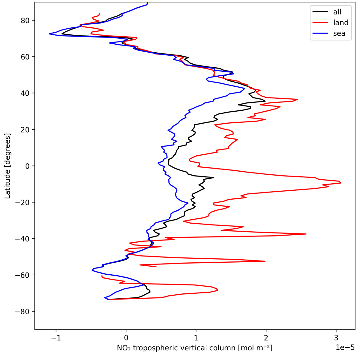
Figure 10: Zonal average of “NO 2 tropospheric vertical column” for 2025-08-12 to 2025-08-12.
