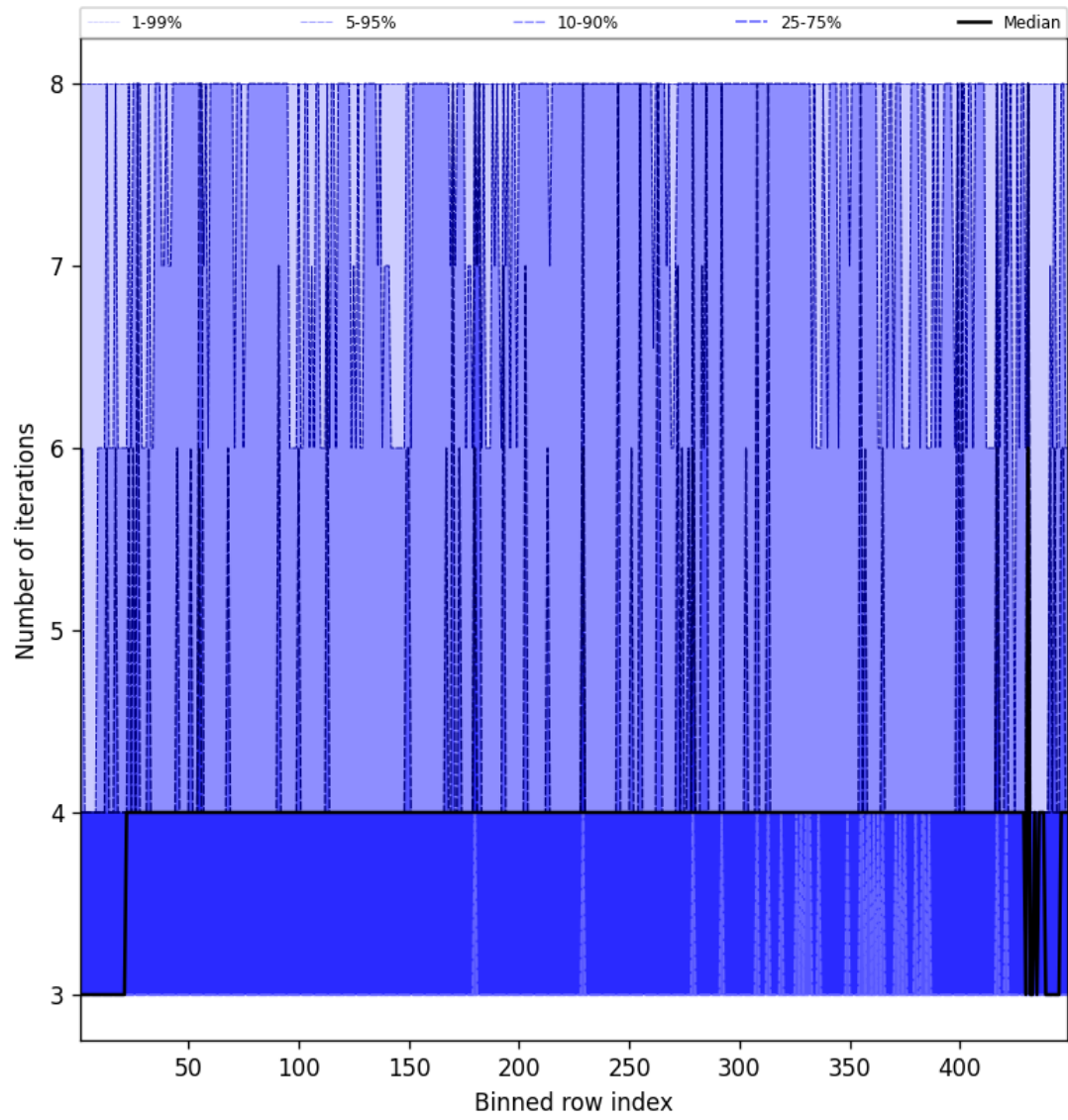
Figure 49: Along track statistics of “Number of iterations” for 2025-08-12 to 2025-08-12
