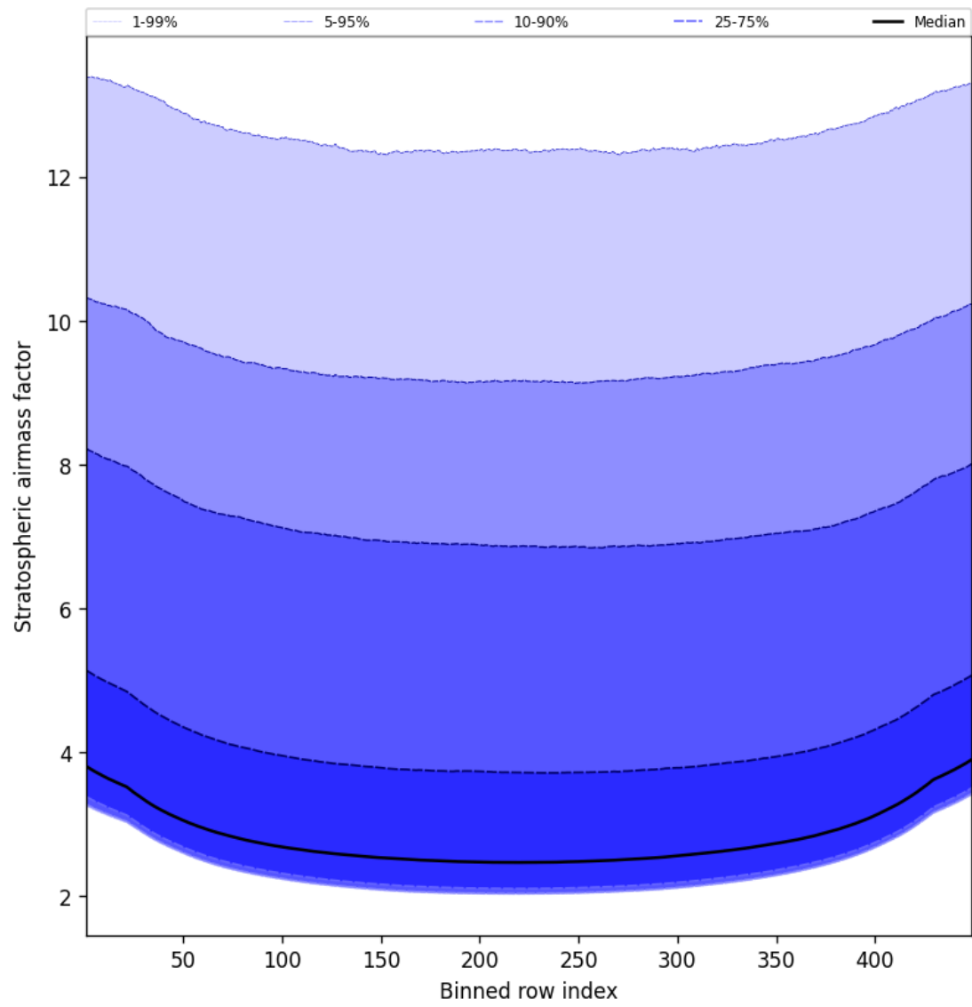
Figure 59: Along track statistics of “Stratospheric airmass factor” for 2025-08-12 to 2025-08-12
