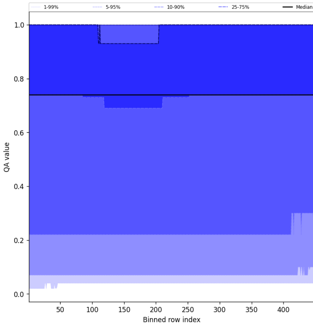
Figure 43: Along track statistics of “QA value” for 2025-08-12 to 2025-08-12
