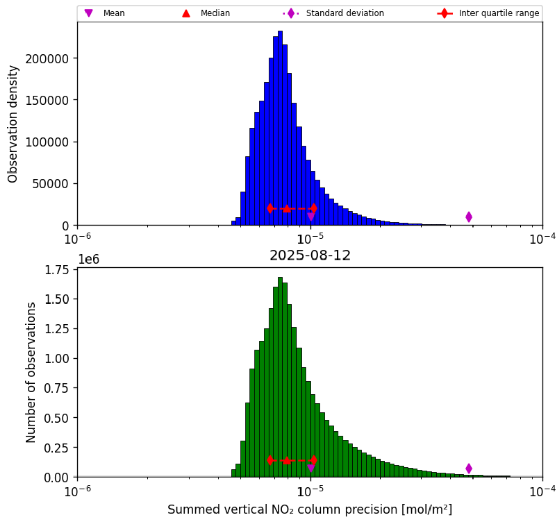
Figure 39: Histogram of "Summed vertical NO 2 column precision" for 2025-08-12 to 2025-08-12
