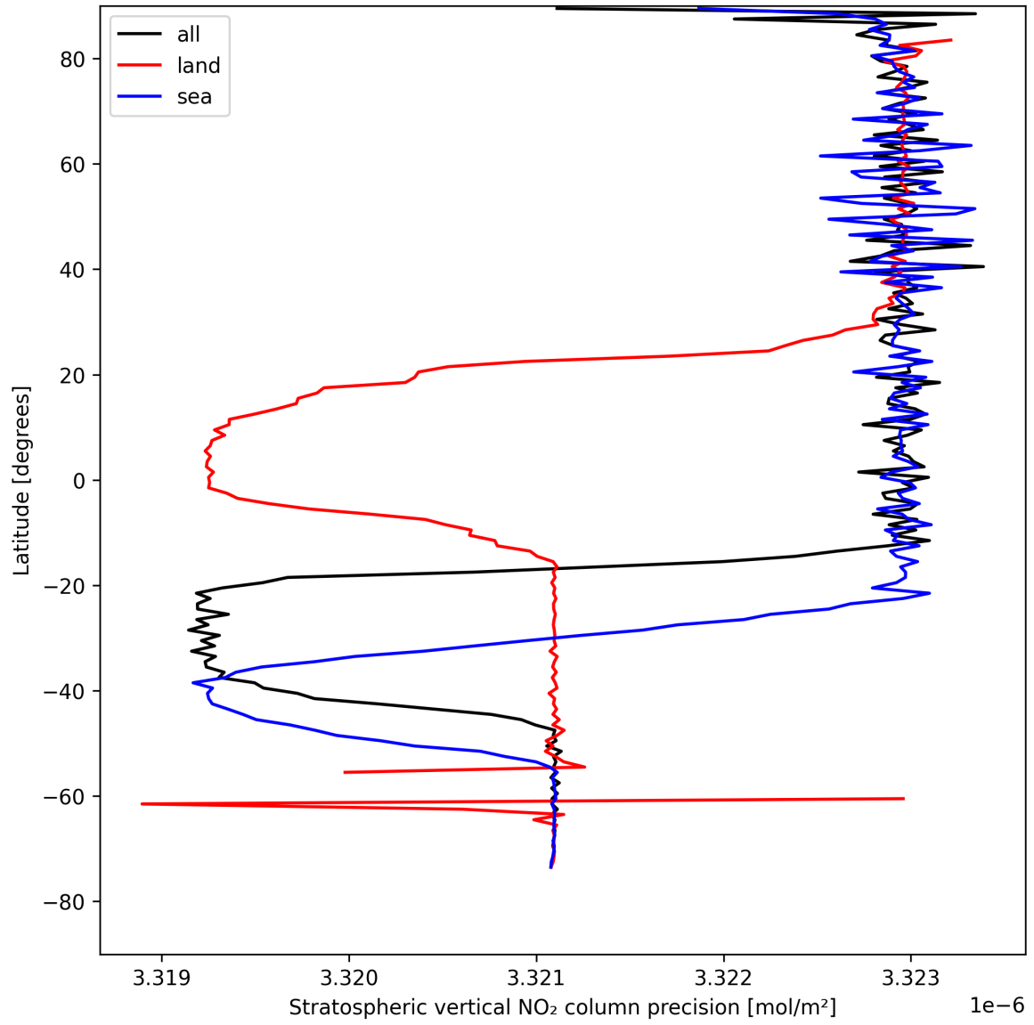
Figure 18: Zonal average of “Stratospheric vertical NO 2 column precision” for 2025-08-12 to 2025-08-12.
