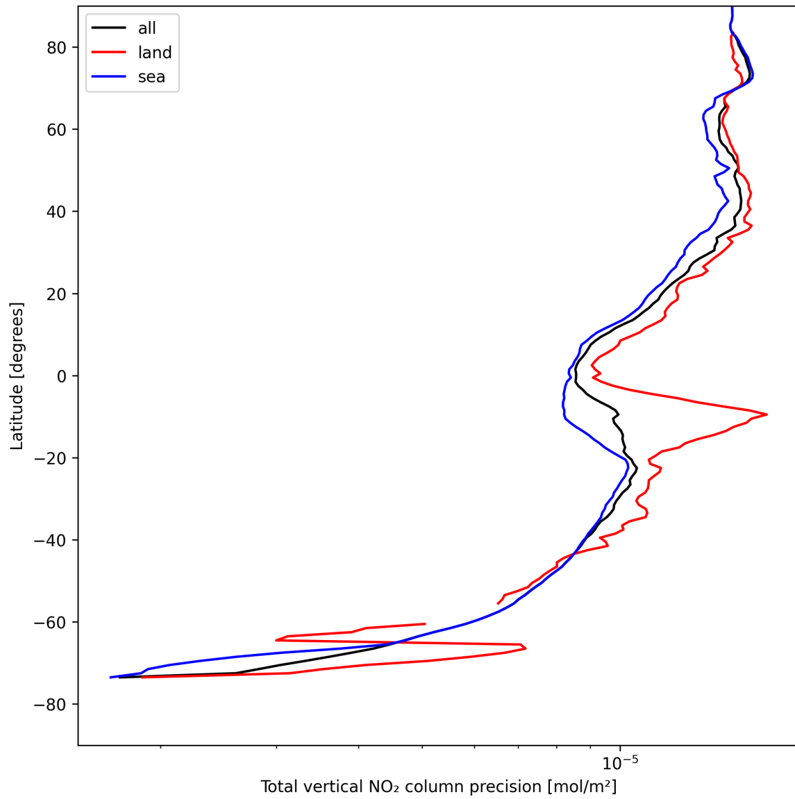
Figure 20: Zonal average of “Total vertical NO 2 column precision” for 2025-08-12 to 2025-08-12.
