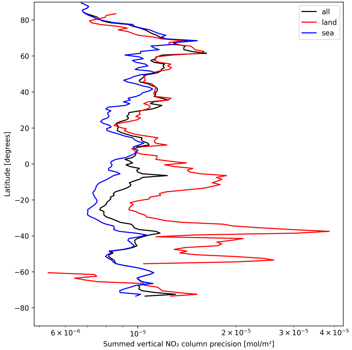
Figure 22: Zonal average of “Summed vertical NO 2 column precision” for 2025-08-12 to 2025-08-12.
