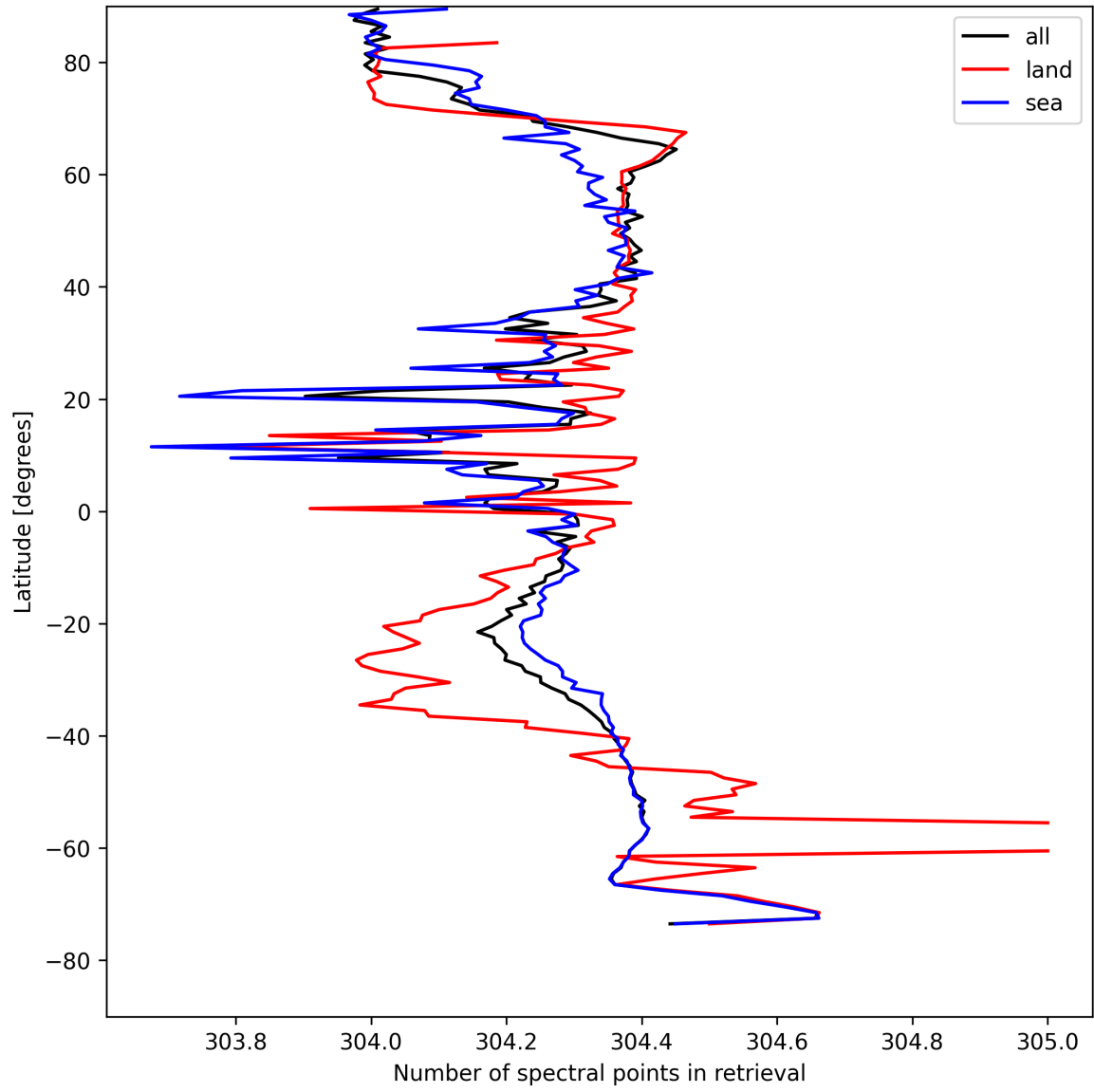
Figure 14: Zonal average of “Number of spectral points in retrieval” for 2025-08-12 to 2025-08-12.
