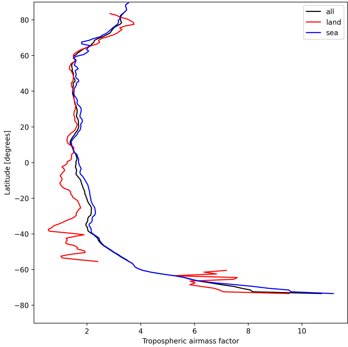
Figure 12: Zonal average of “Tropospheric air mass factor” for 2025-08-12 to 2025-08-12.
