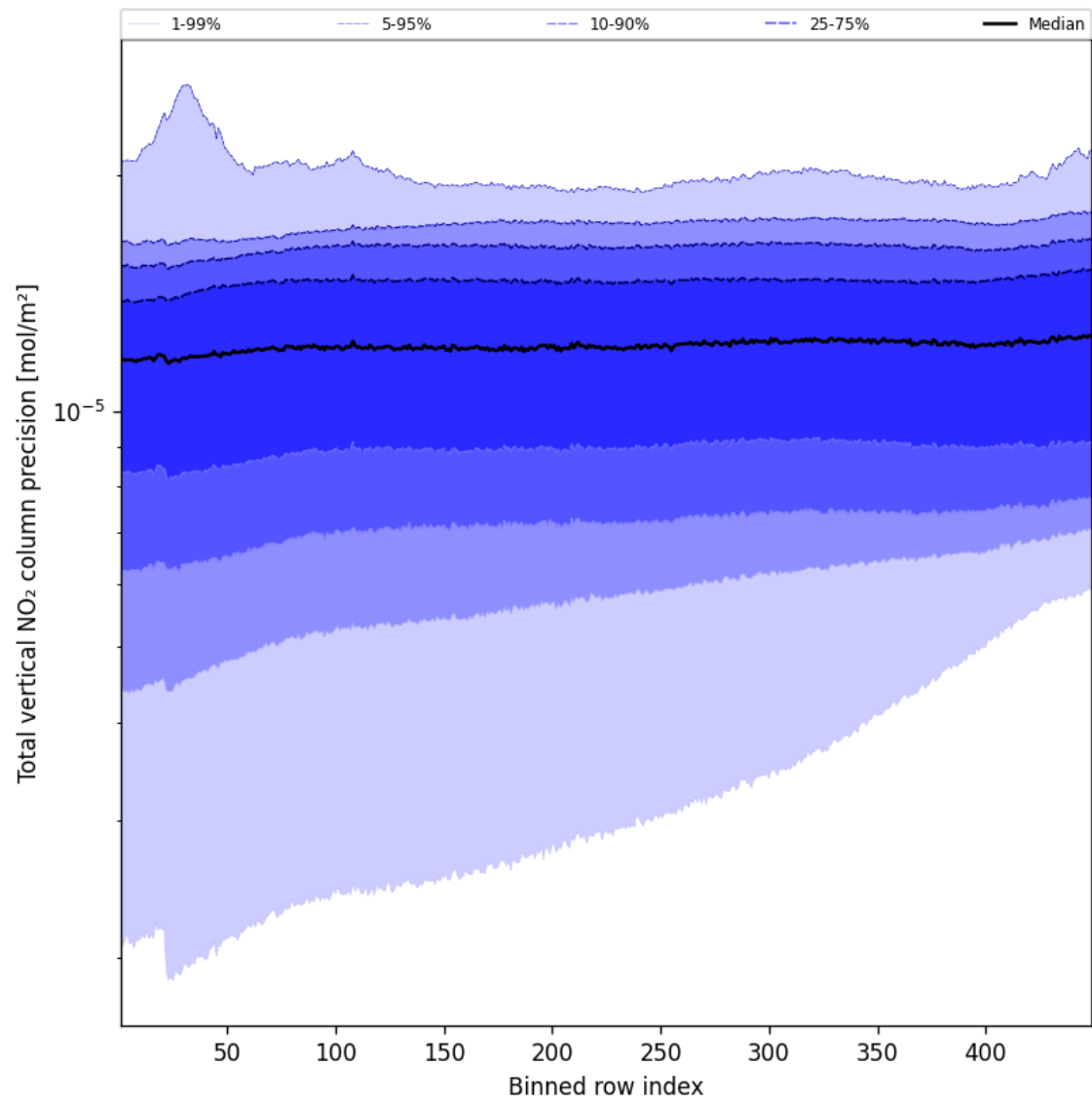
Figure 54: Along track statistics of “Total vertical NO 2 column precision” for 2025-08-12 to 2025-08-12
