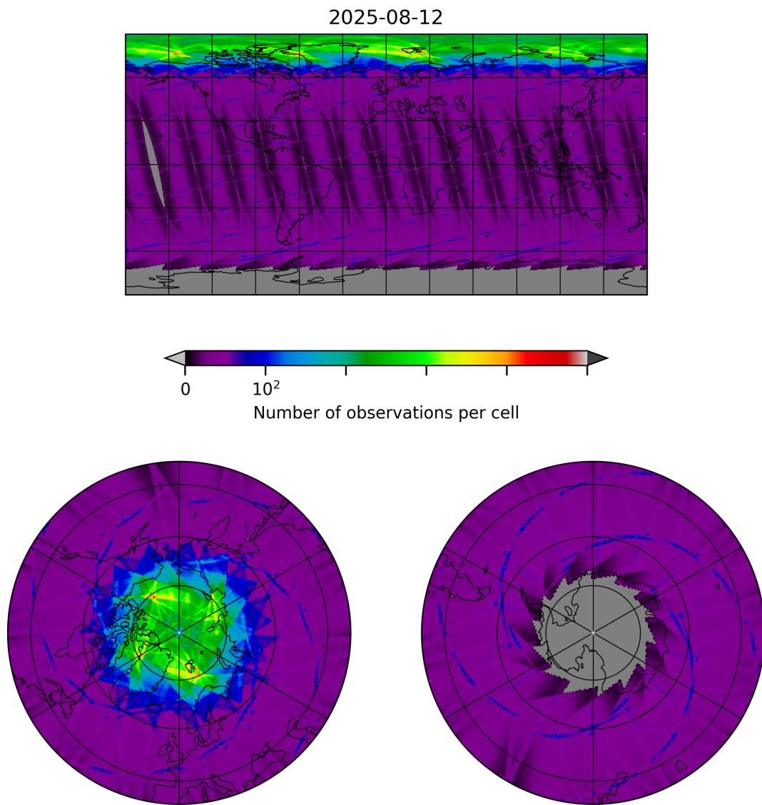
Figure 8: Map of the number of observations for 2025-08-12 to 2025-08-12
