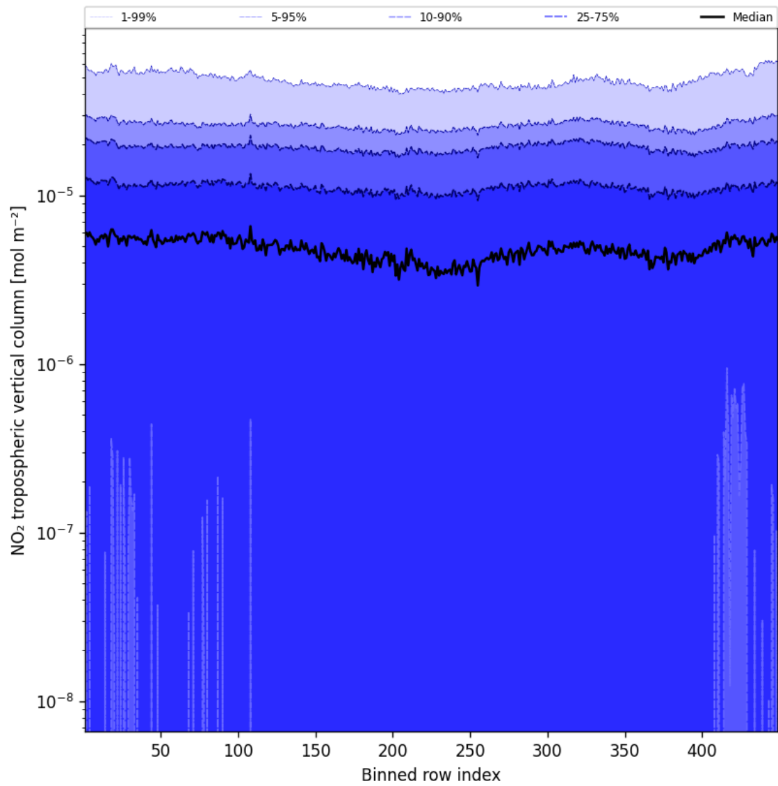
Figure 44: Along track statistics of “NO 2 tropospheric vertical column” for 2025-08-12 to 2025-08-12
