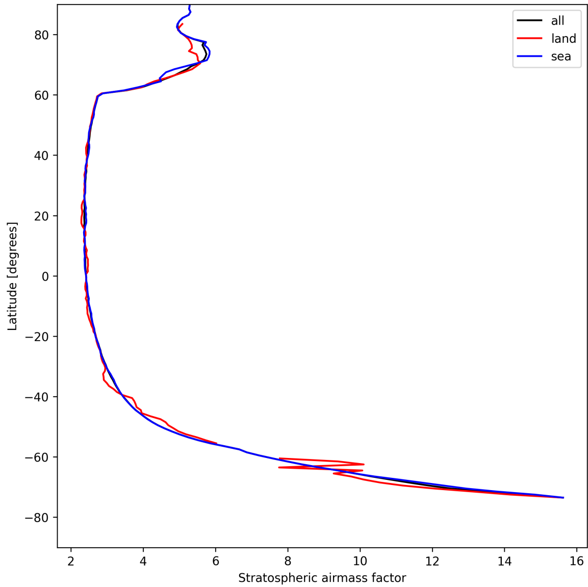
Figure 25: Zonal average of “Stratospheric airmass factor” for 2025-08-12 to 2025-08-12.
