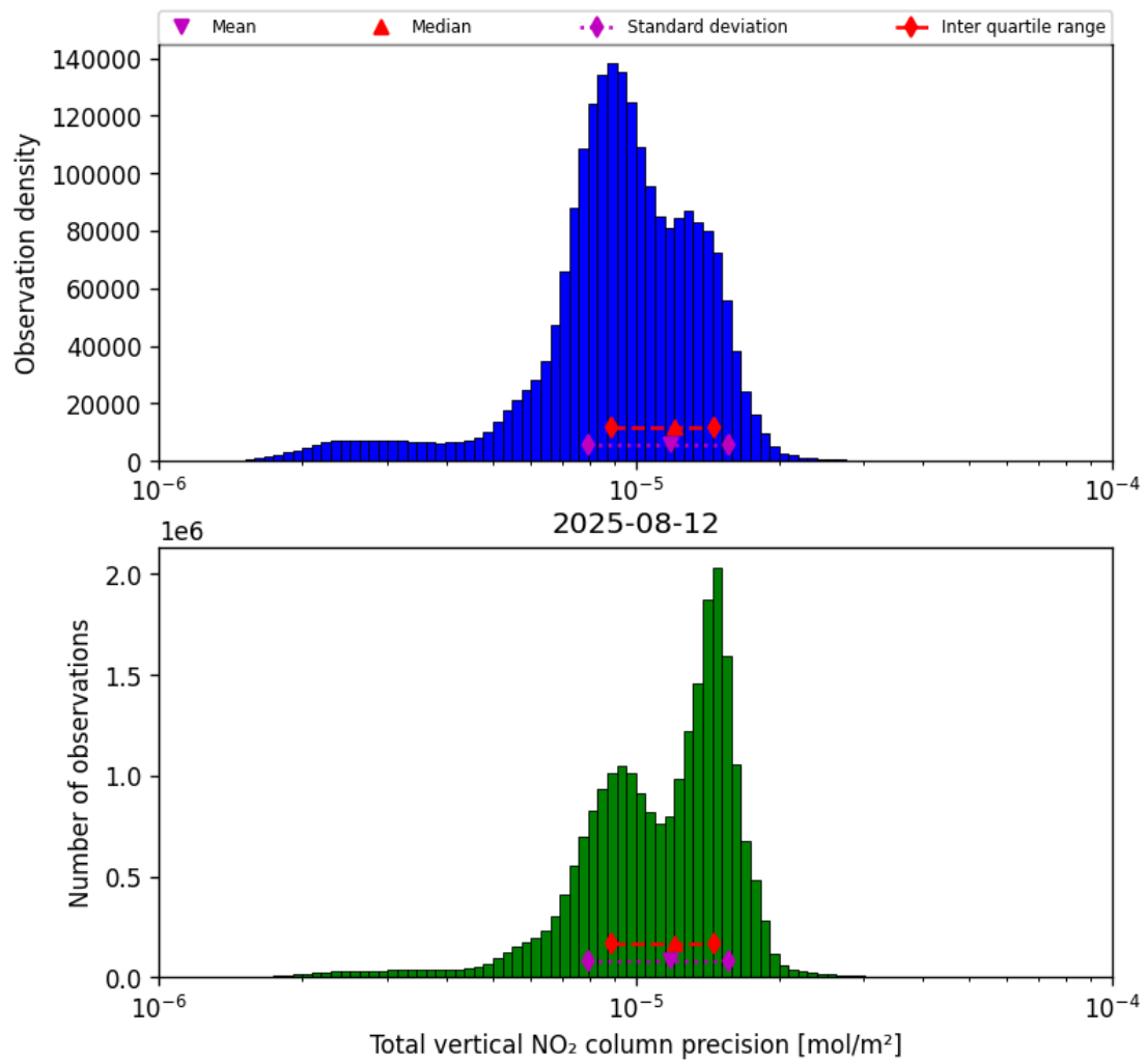
Figure 37: Histogram of “Total vertical NO 2 column precision” for 2025-08-12 to 2025-08-12
