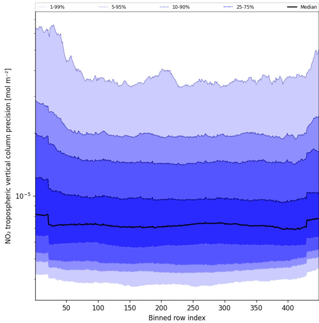
Figure 45: Along track statistics of “NO 2 tropospheric vertical column precision” for 2025-08-12 to 2025-08-12
