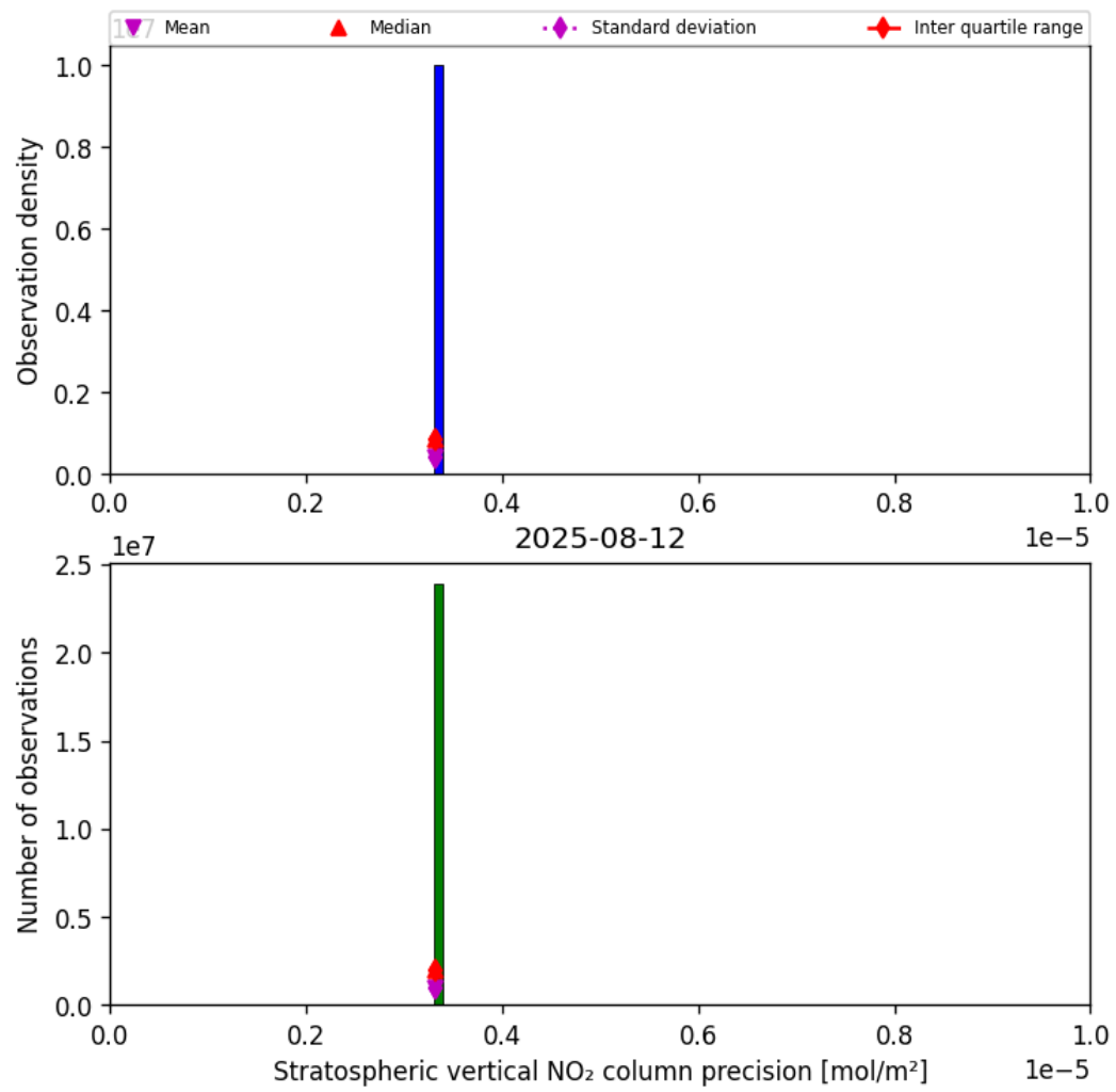
Figure 35: Histogram of “Stratospheric vertical NO 2 column precision” for 2025-08-12 to 2025-08-12
