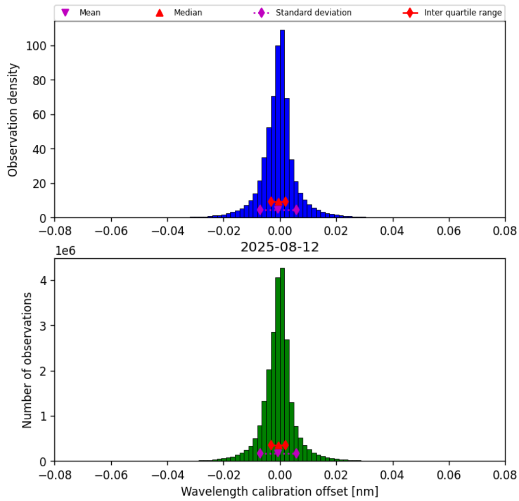
Figure 33: Histogram of “Wavelength calibration offset” for 2025-08-12 to 2025-08-12
