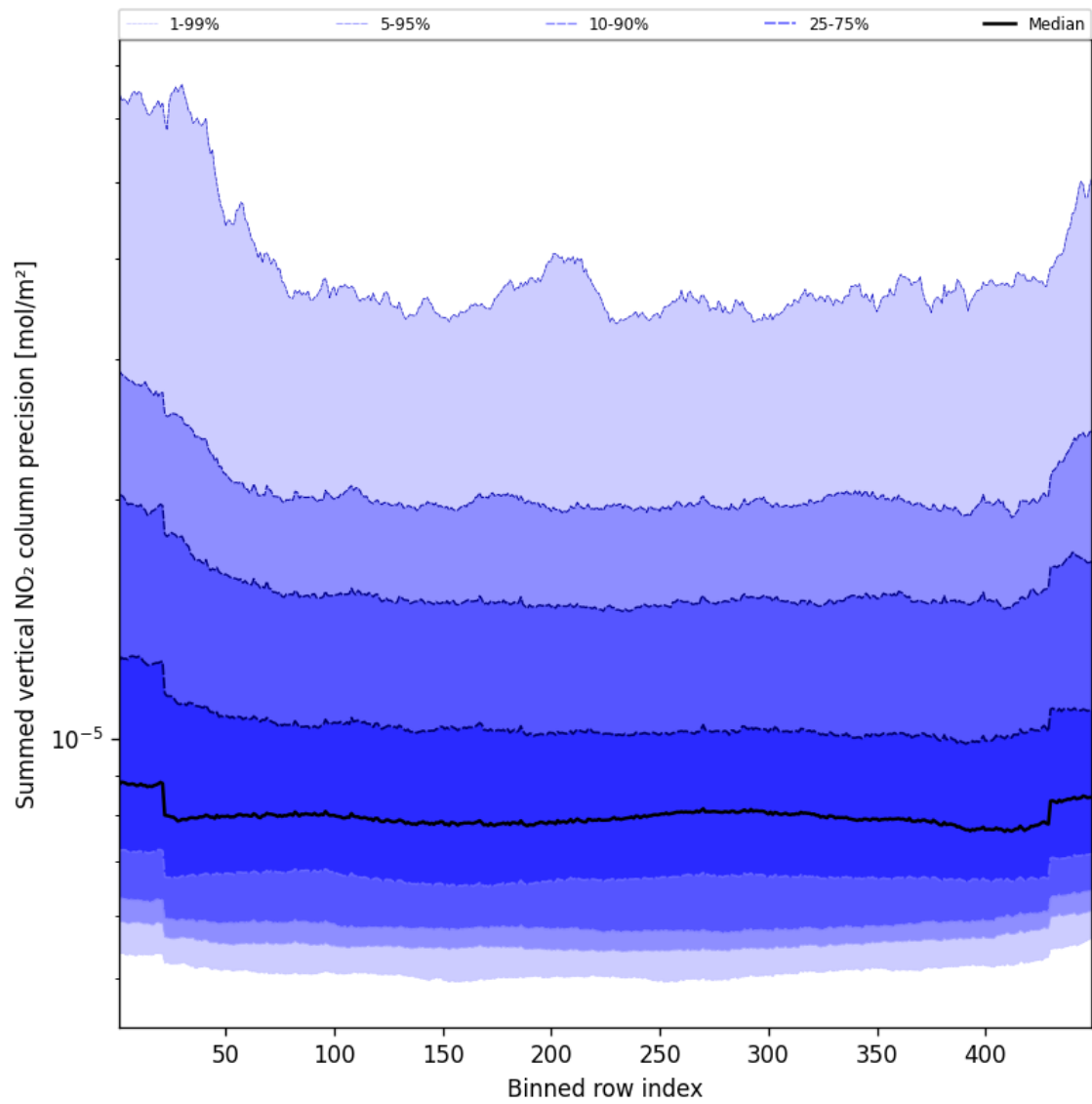
Figure 56: Along track statistics of “Summed vertical NO 2 column precision” for 2025-08-12 to 2025-08-12
