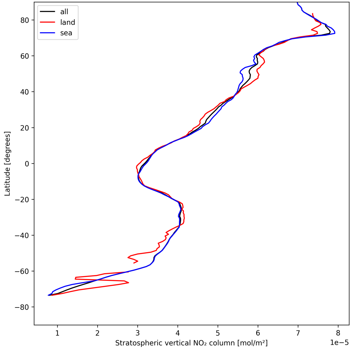
Figure 17: Zonal average of “Stratospheric vertical NO 2 column” for 2025-08-12 to 2025-08-12.
