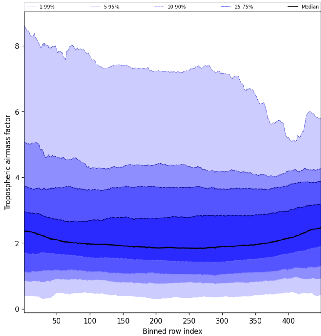
Figure 46: Along track statistics of “Tropospheric air mass factor” for 2025-08-12 to 2025-08-12
