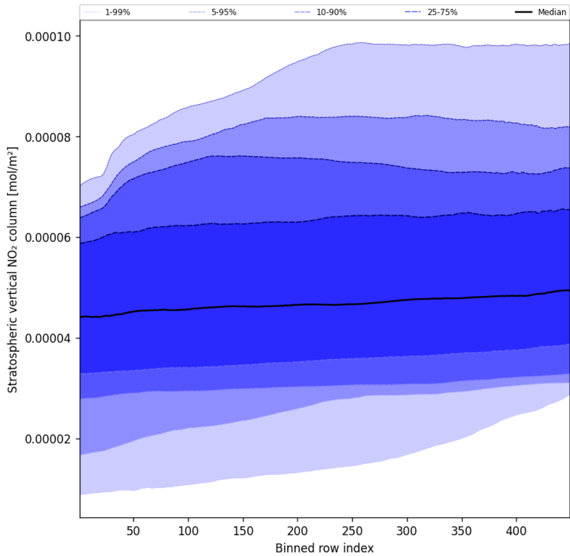
Figure 51: Along track statistics of “Stratospheric vertical NO 2 column” for 2025-08-12 to 2025-08-12
