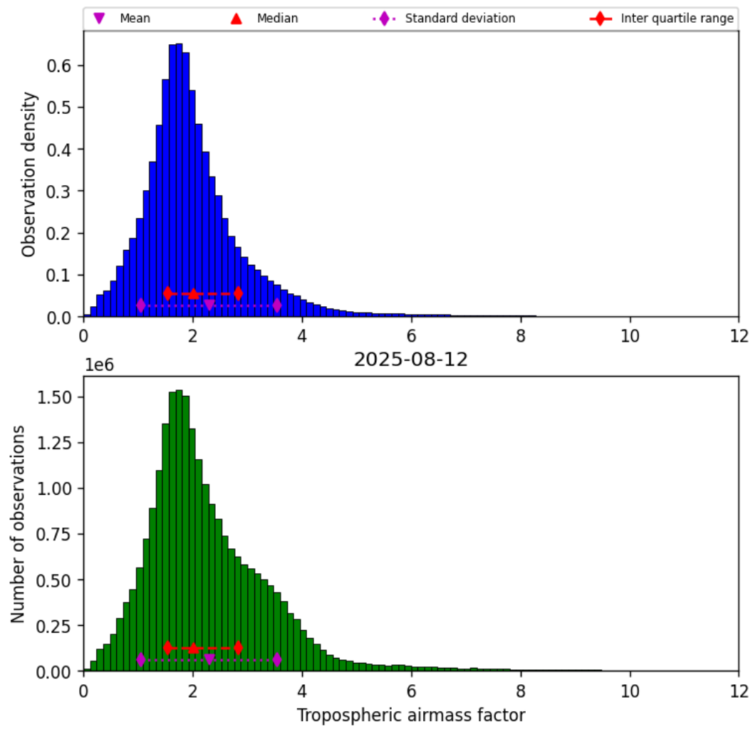
Figure 29: Histogram of “Tropospheric airmass factor” for 2025-08-12 to 2025-08-12
