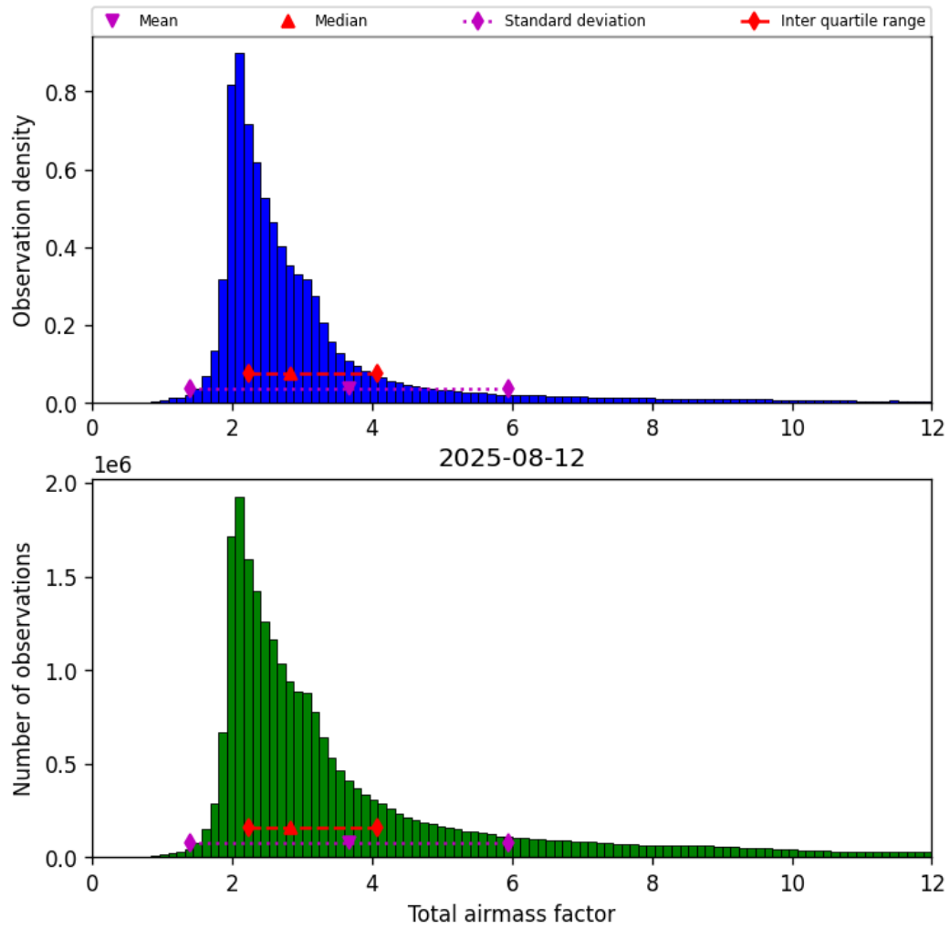
Figure 30: Histogram of “Total airmass factor” for 2025-08-12 to 2025-08-12
