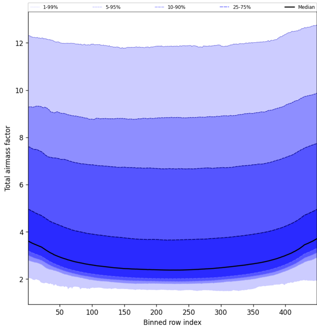
Figure 47: Along track statistics of “Total airmass factor” for 2025-08-12 to 2025-08-12
