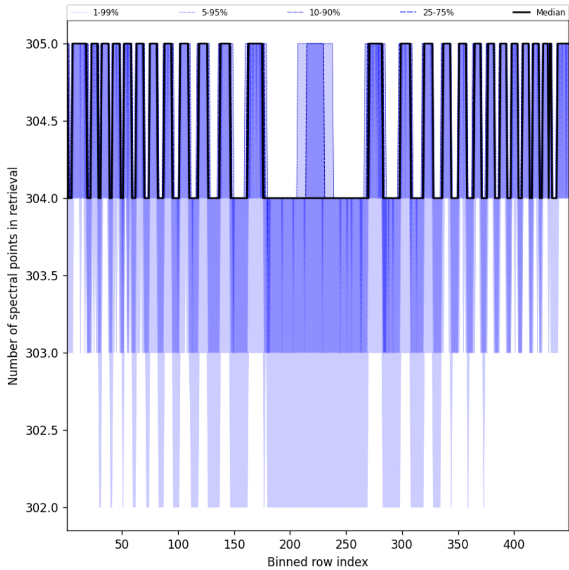
Figure 48: Along track statistics of “Number of spectral points in retrieval” for 2025-08-12 to 2025-08-12
