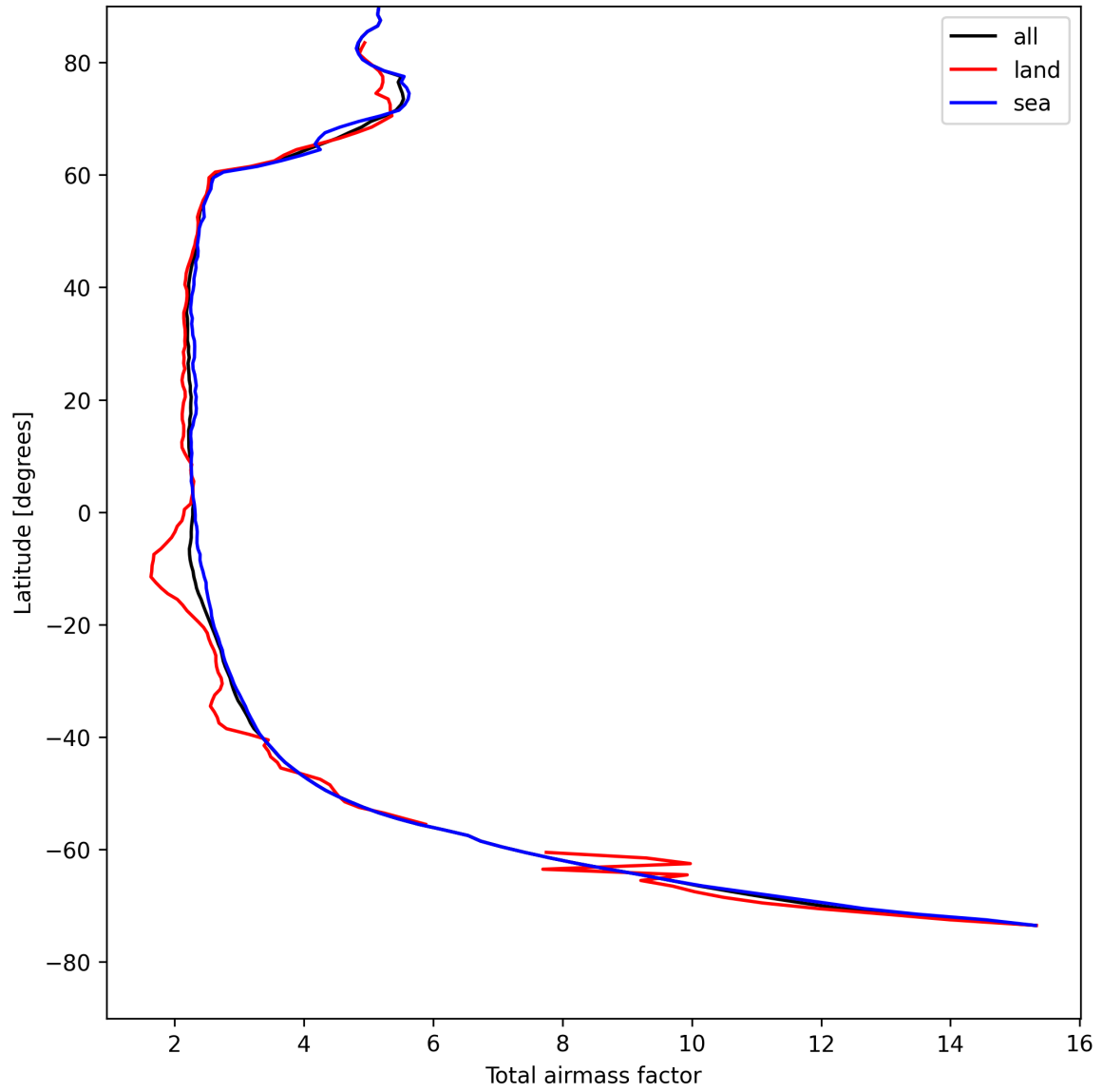
Figure 13: Zonal average of “Total airmass factor” for 2025-08-12 to 2025-08-12.
