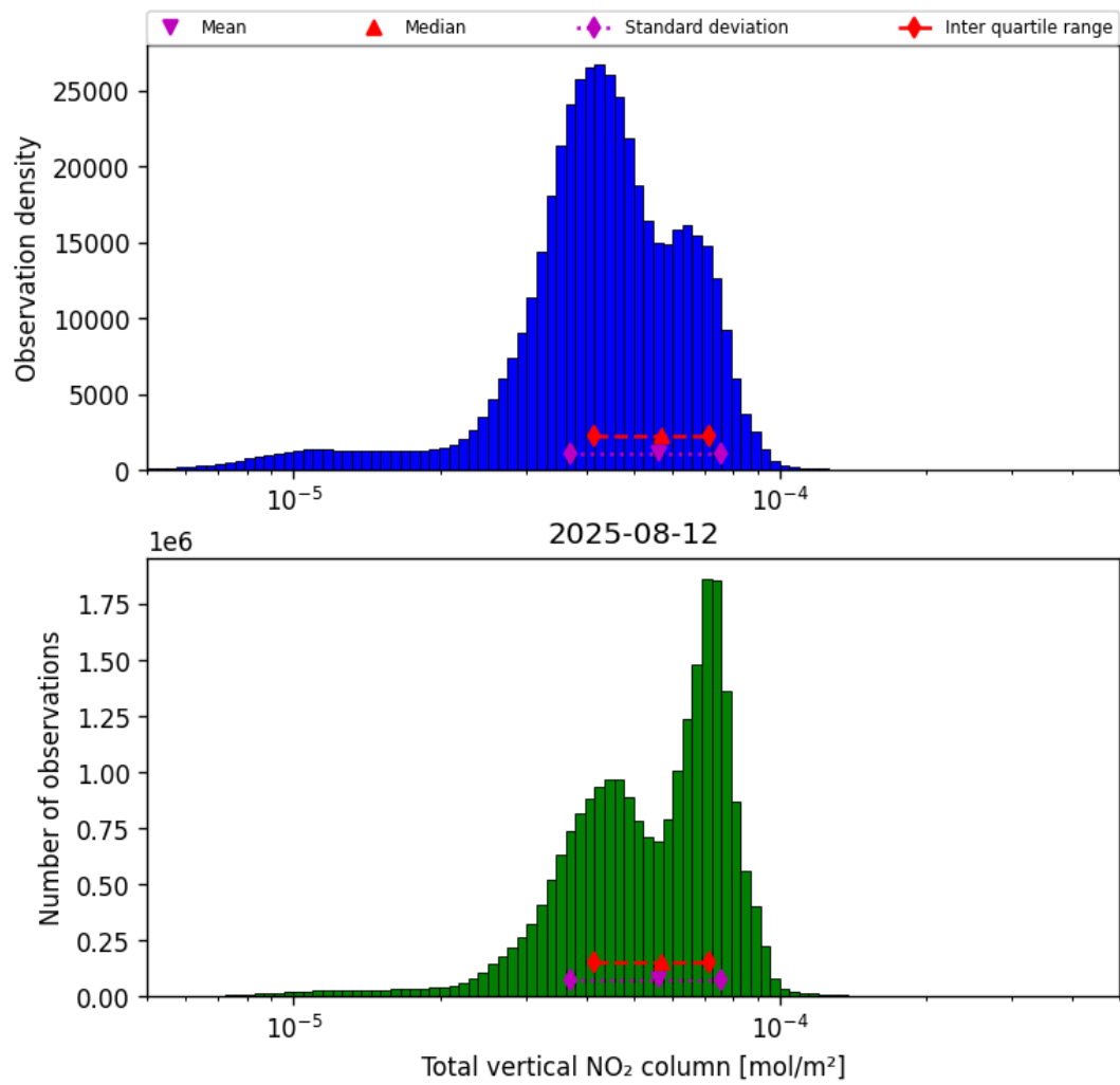
Figure 36: Histogram of “Total vertical NO 2 column” for 2025-08-12 to 2025-08-12
