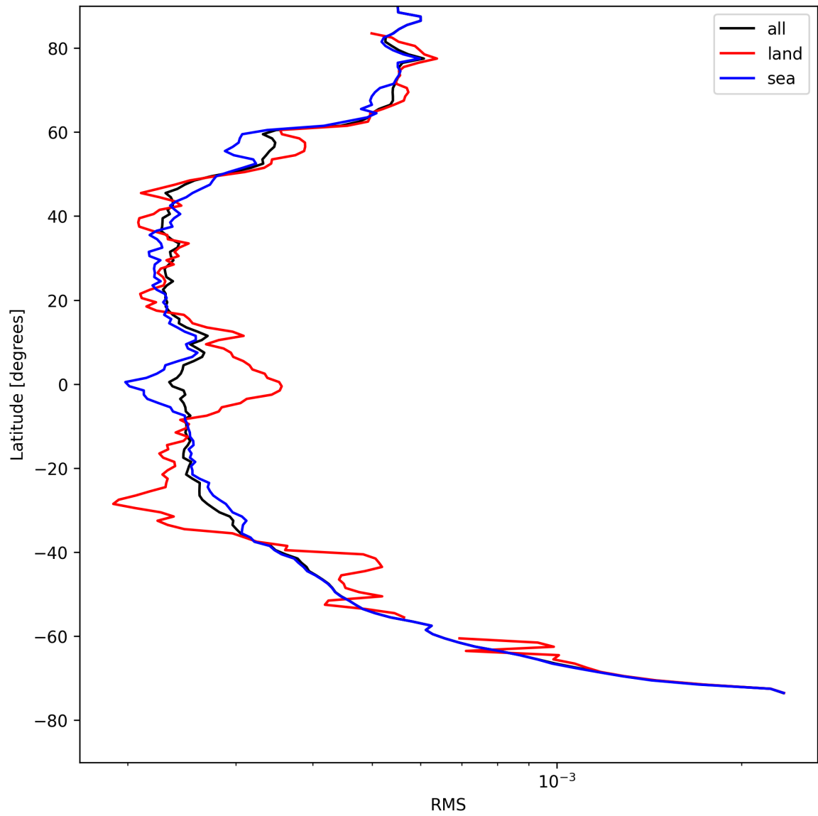
Figure 24: Zonal average of “RMS” for 2025-08-12 to 2025-08-12.
