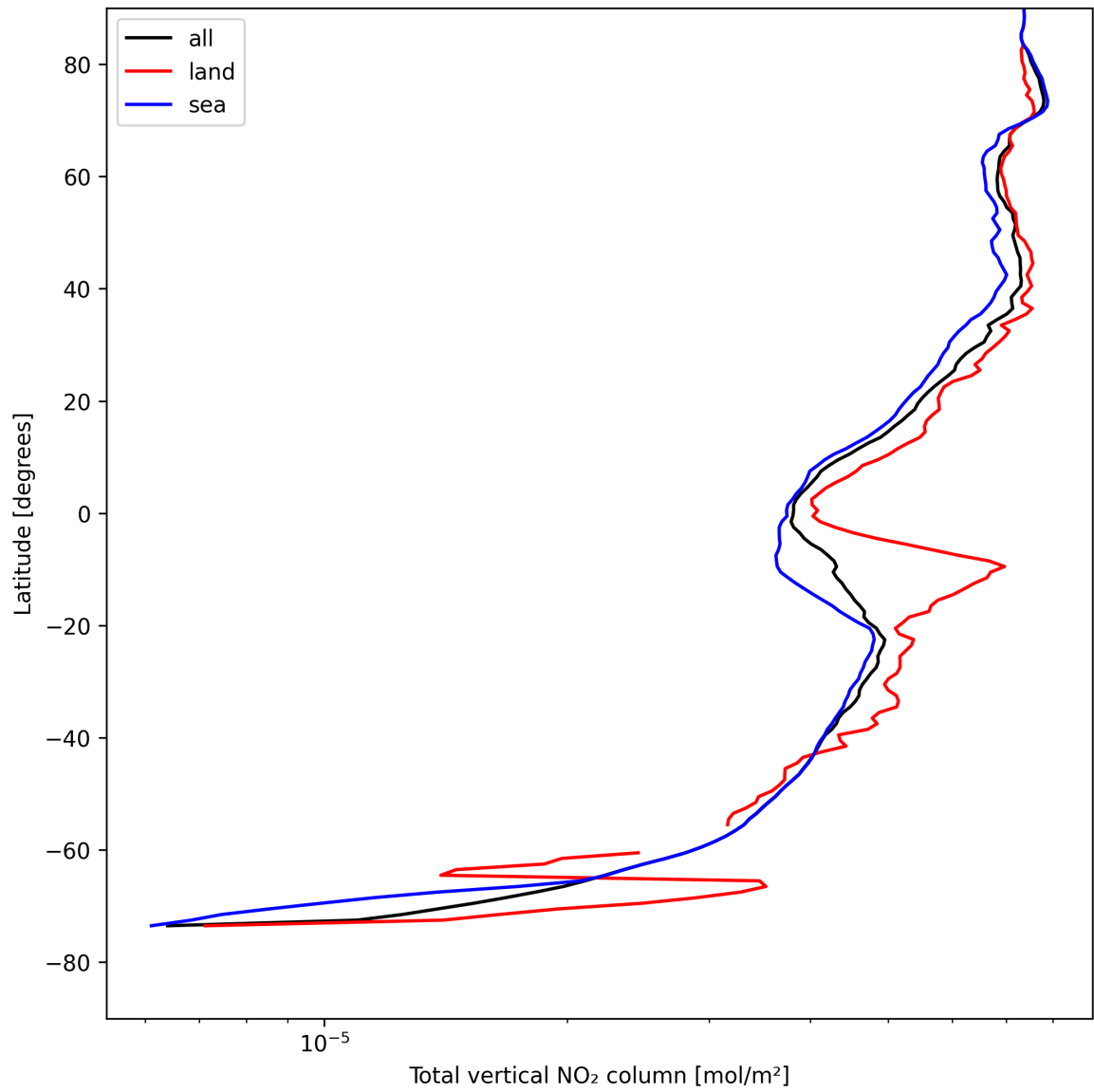
Figure 19: Zonal average of “Total vertical NO 2 column” for 2025-08-12 to 2025-08-12.
