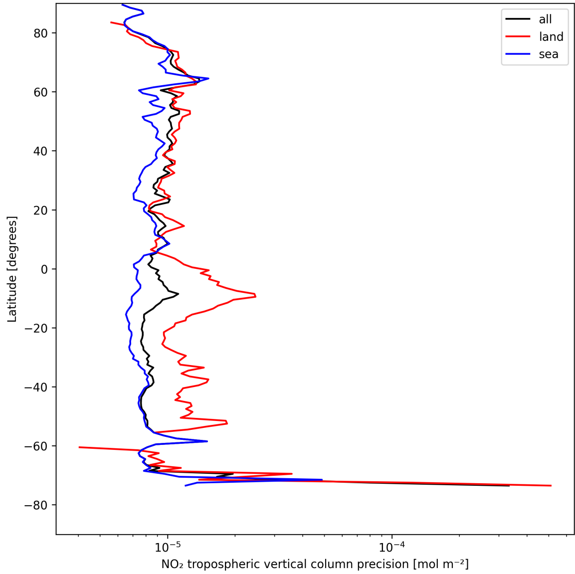
Figure 11: Zonal average of “NO 2 tropospheric vertical column precision” for 2025-08-14 to 2025-08-15.
