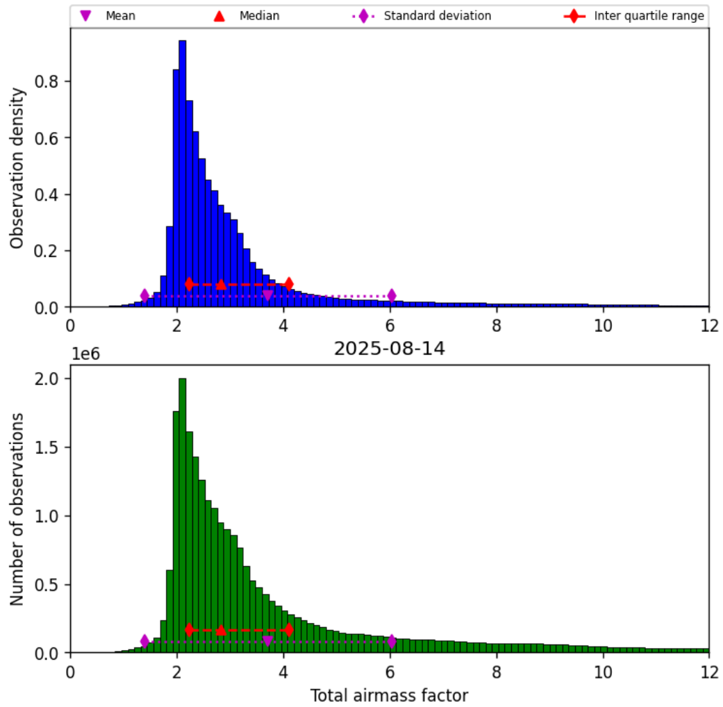
Figure 30: Histogram of “Total airmass factor” for 2025-08-14 to 2025-08-15
