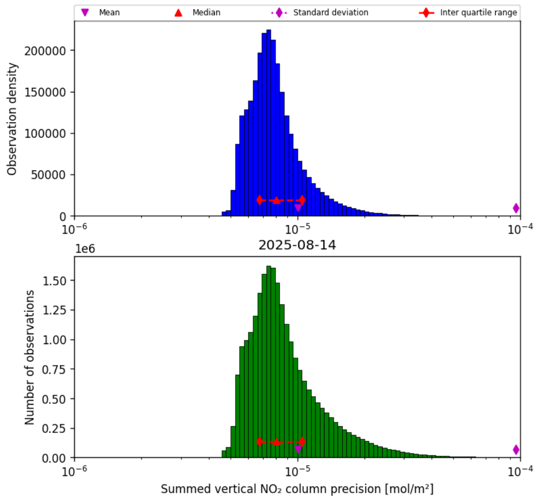
Figure 39: Histogram of “Summed vertical NO 2 column precision” for 2025-08-14 to 2025-08-15
