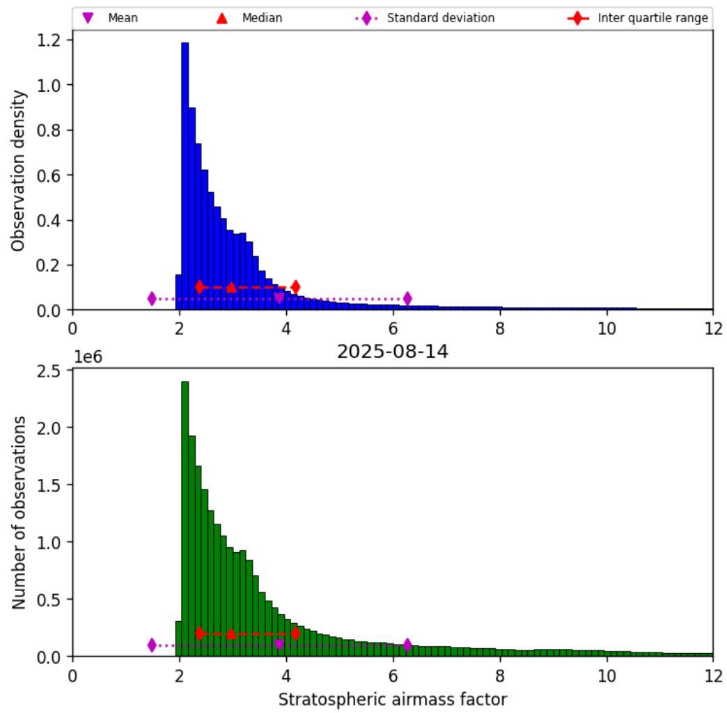
Figure 42: Histogram of “Stratospheric airmass factor” for 2025-08-14 to 2025-08-15
