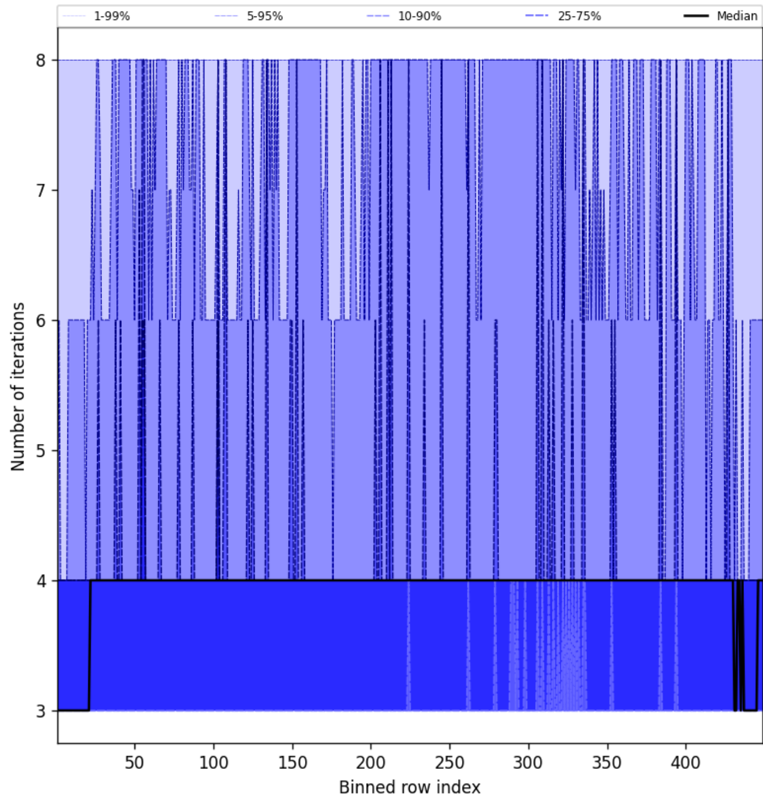
Figure 49: Along track statistics of “Number of iterations” for 2025-08-14 to 2025-08-15
