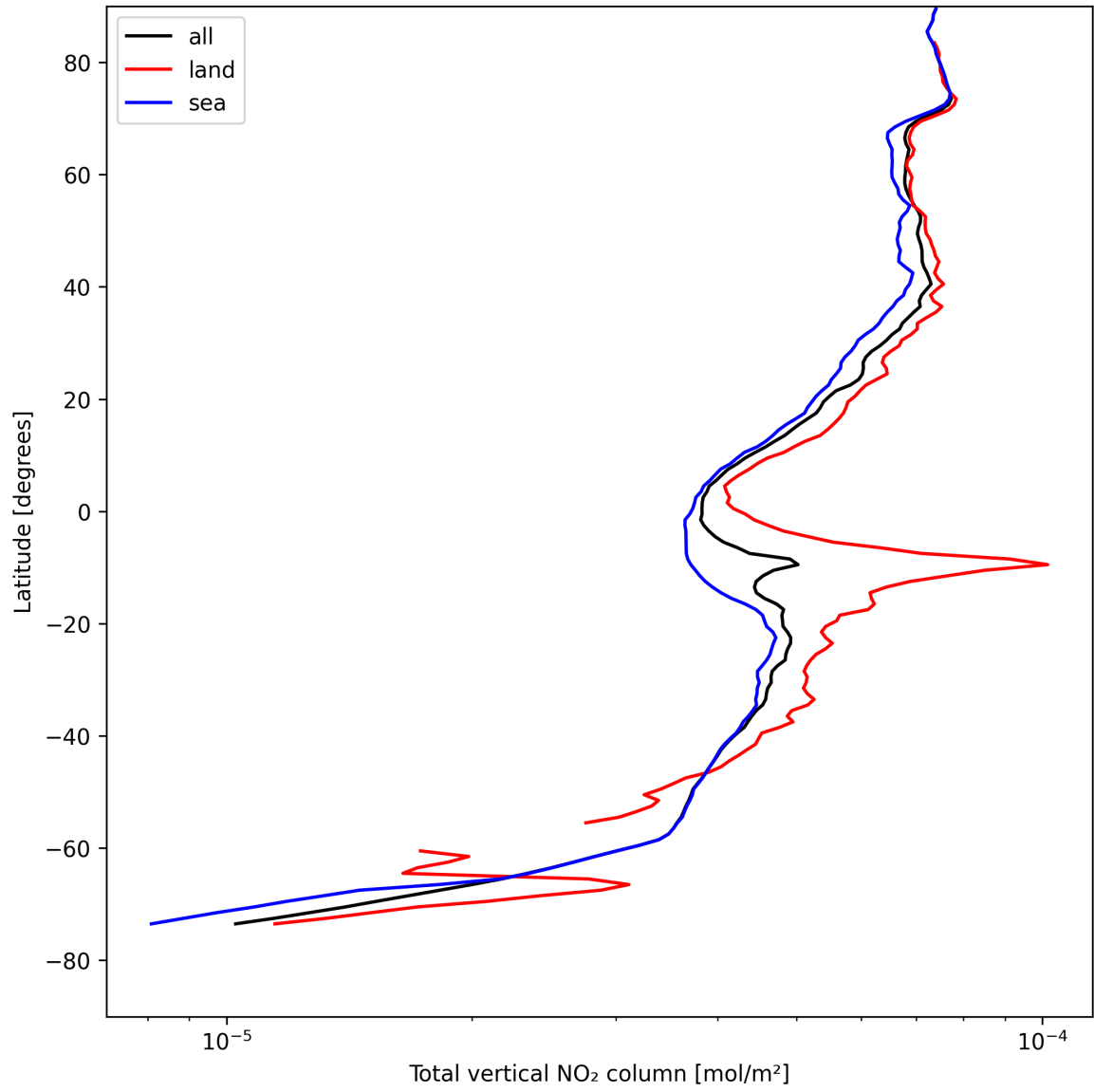
Figure 19: Zonal average of “Total vertical NO 2 column” for 2025-08-14 to 2025-08-15.
