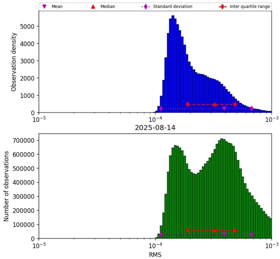
Figure 41: Histogram of “RMS” for 2025-08-14 to 2025-08-15
