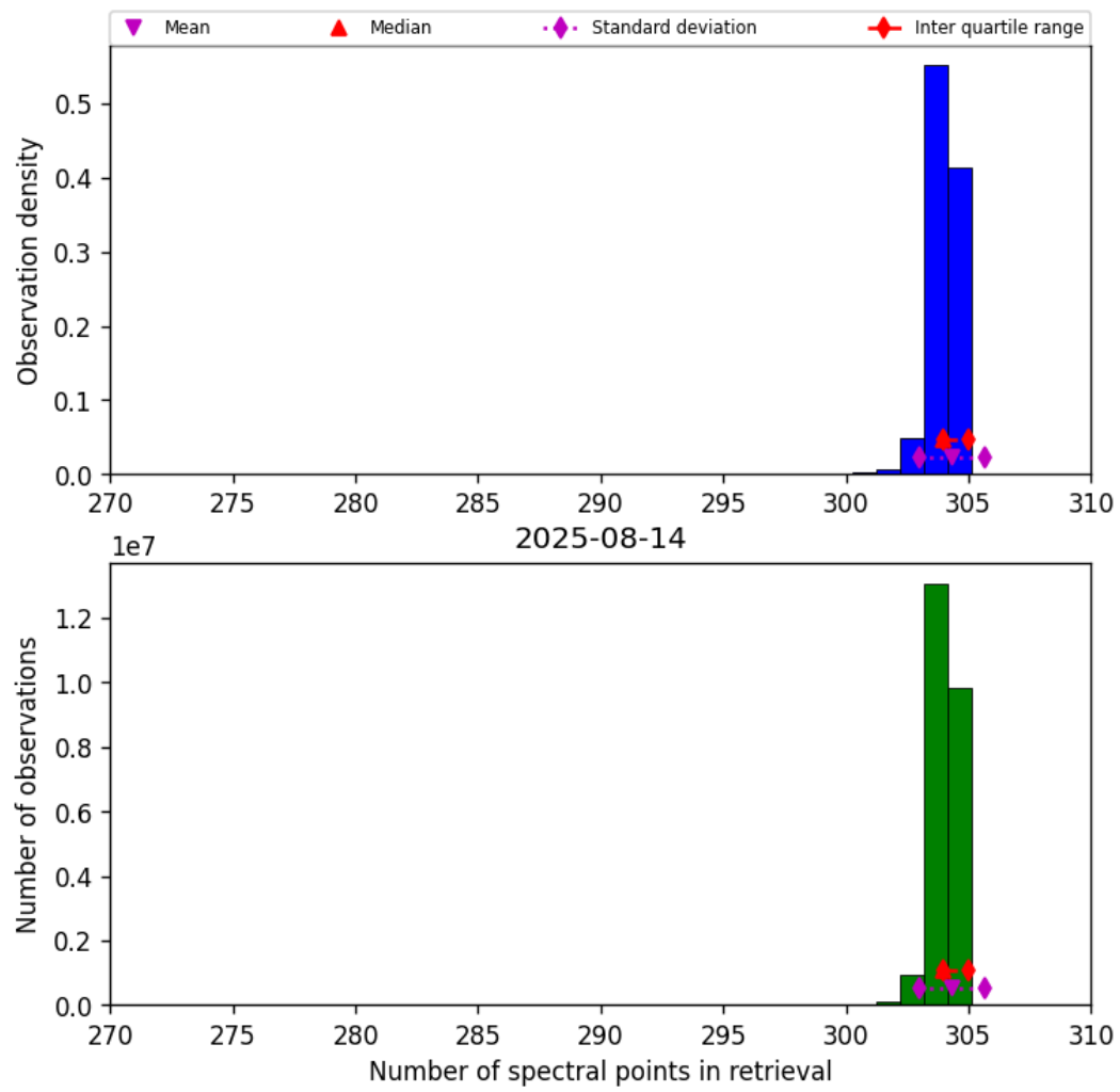
Figure 31: Histogram of “Number of spectral points in retrieval” for 2025-08-14 to 2025-08-15
