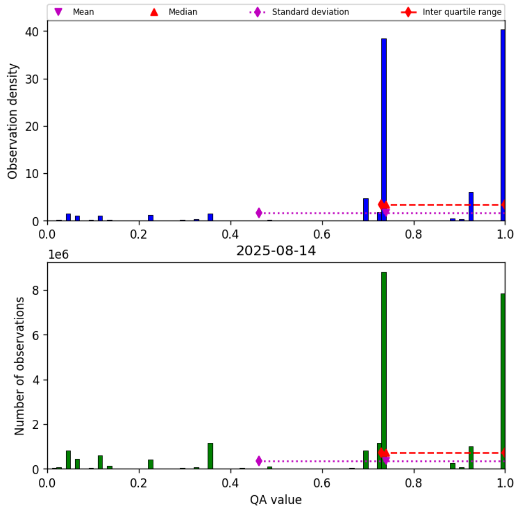
Figure 26: Histogram of “QA value” for 2025-08-14 to 2025-08-15
