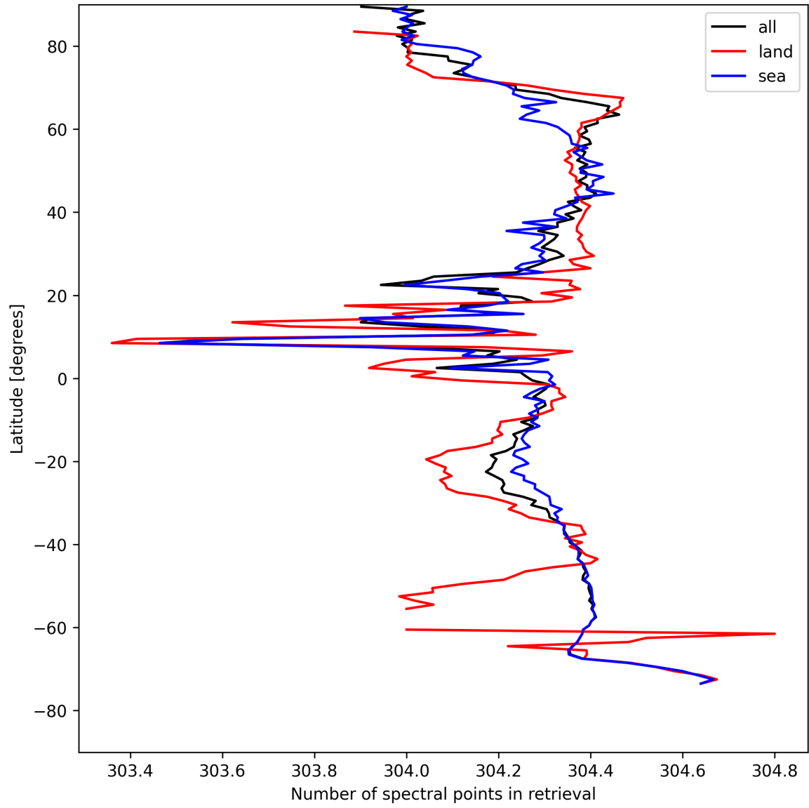
Figure 14: Zonal average of “Number of spectral points in retrieval” for 2025-08-14 to 2025-08-15.
