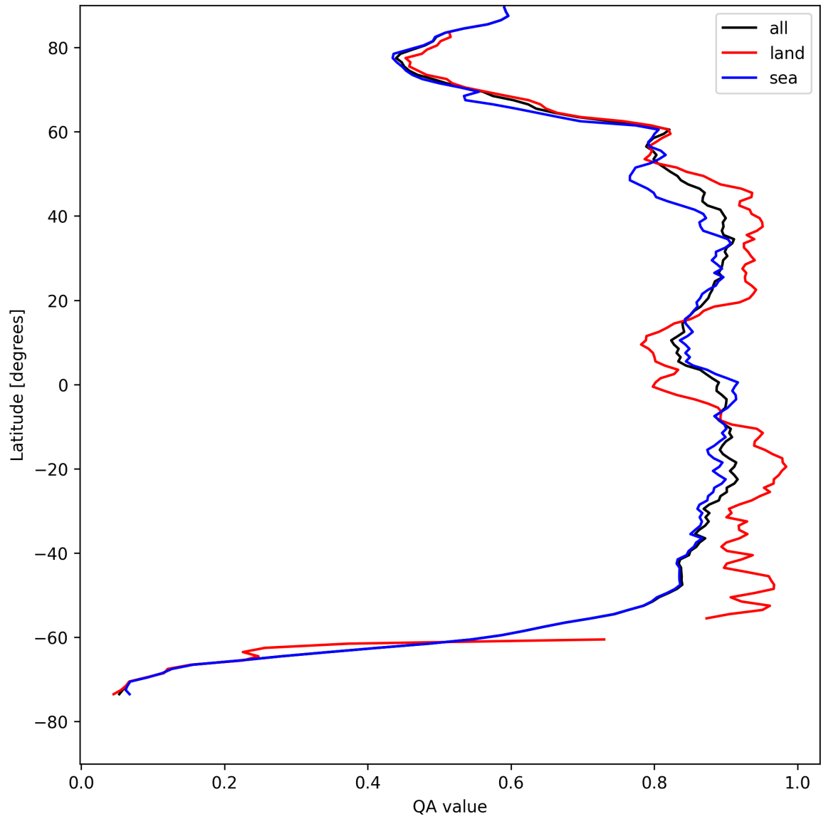
Figure 9: Zonal average of “QA value” for 2025-08-14 to 2025-08-15.
