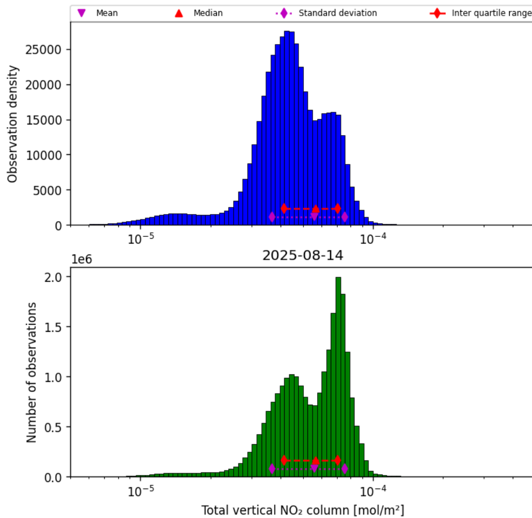
Figure 36: Histogram of “Total vertical NO 2 column” for 2025-08-14 to 2025-08-15
