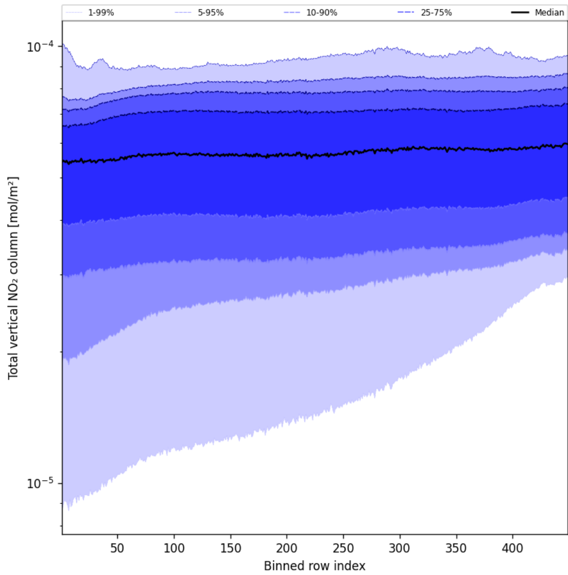
Figure 53: Along track statistics of “Total vertical NO 2 column” for 2025-08-14 to 2025-08-15
