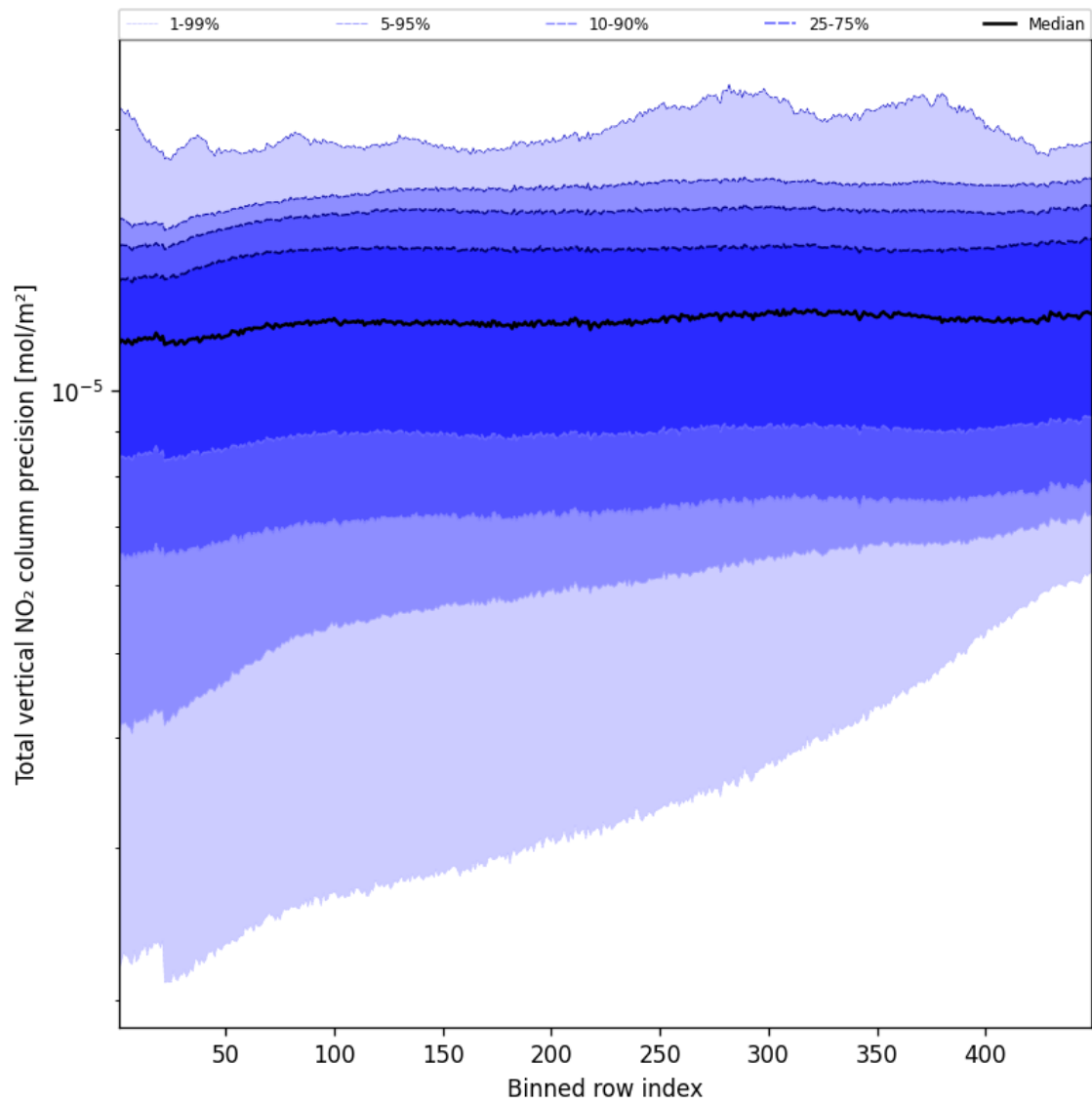
Figure 54: Along track statistics of “Total vertical NO 2 column precision” for 2025-08-14 to 2025-08-15
