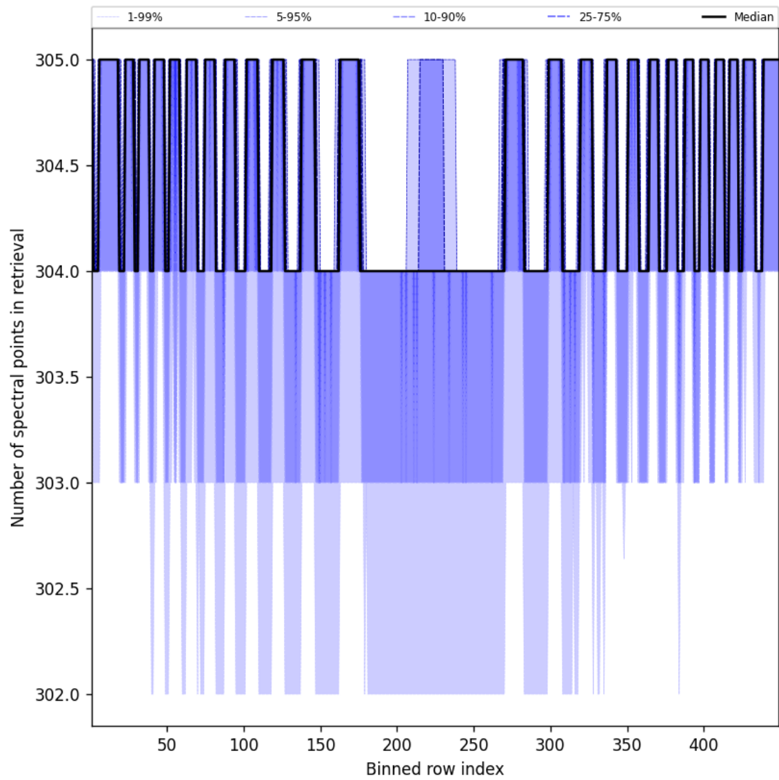
Figure 48: Along track statistics of “Number of spectral points in retrieval” for 2025-08-14 to 2025-08-15
