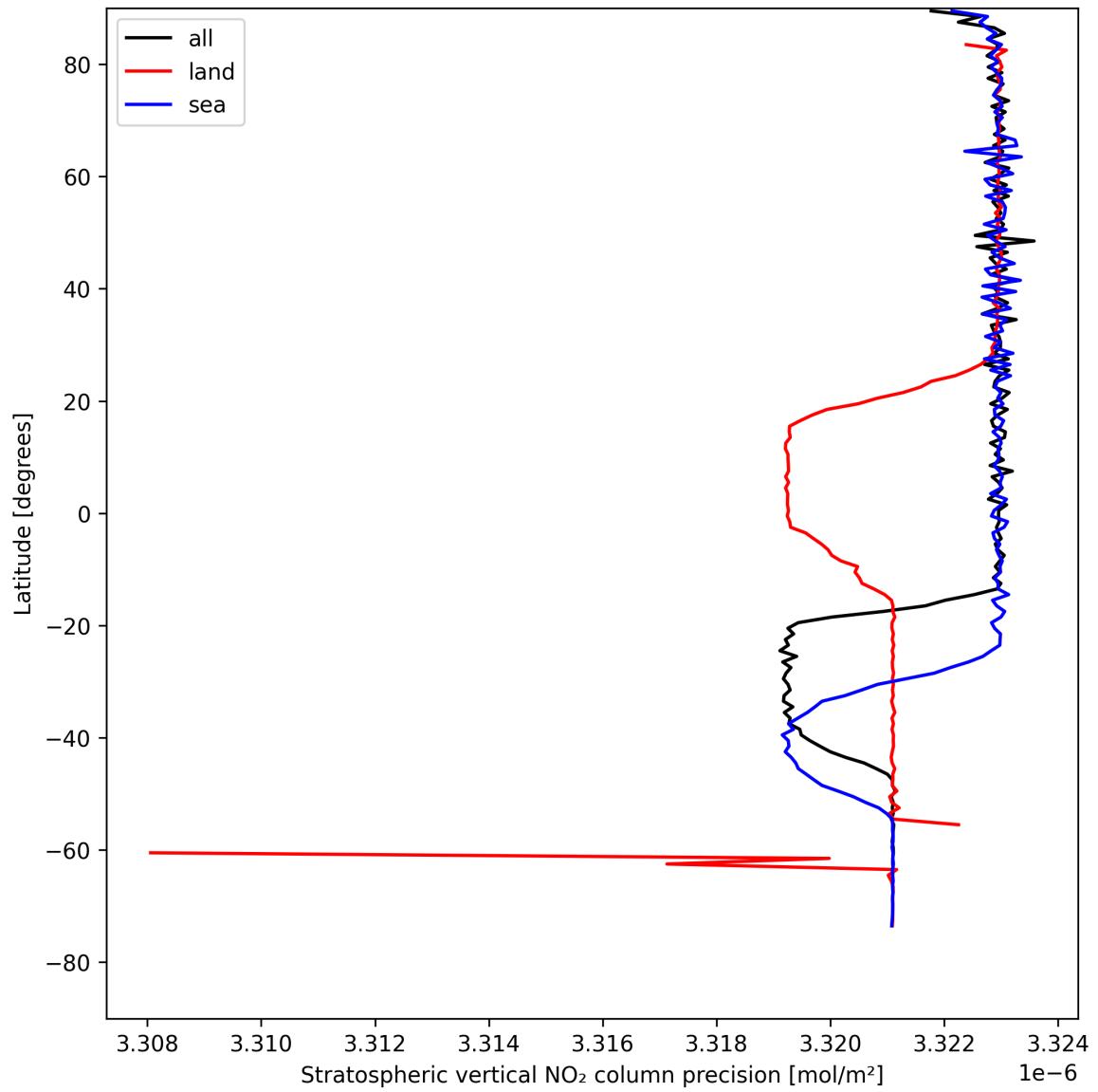
Figure 18: Zonal average of “Stratospheric vertical NO 2 column precision” for 2025-08-14 to 2025-08-15.
