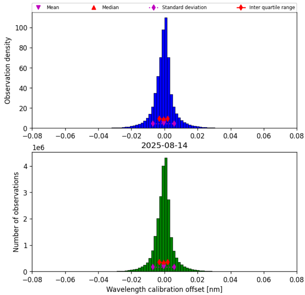
Figure 33: Histogram of “Wavelength calibration offset” for 2025-08-14 to 2025-08-15
