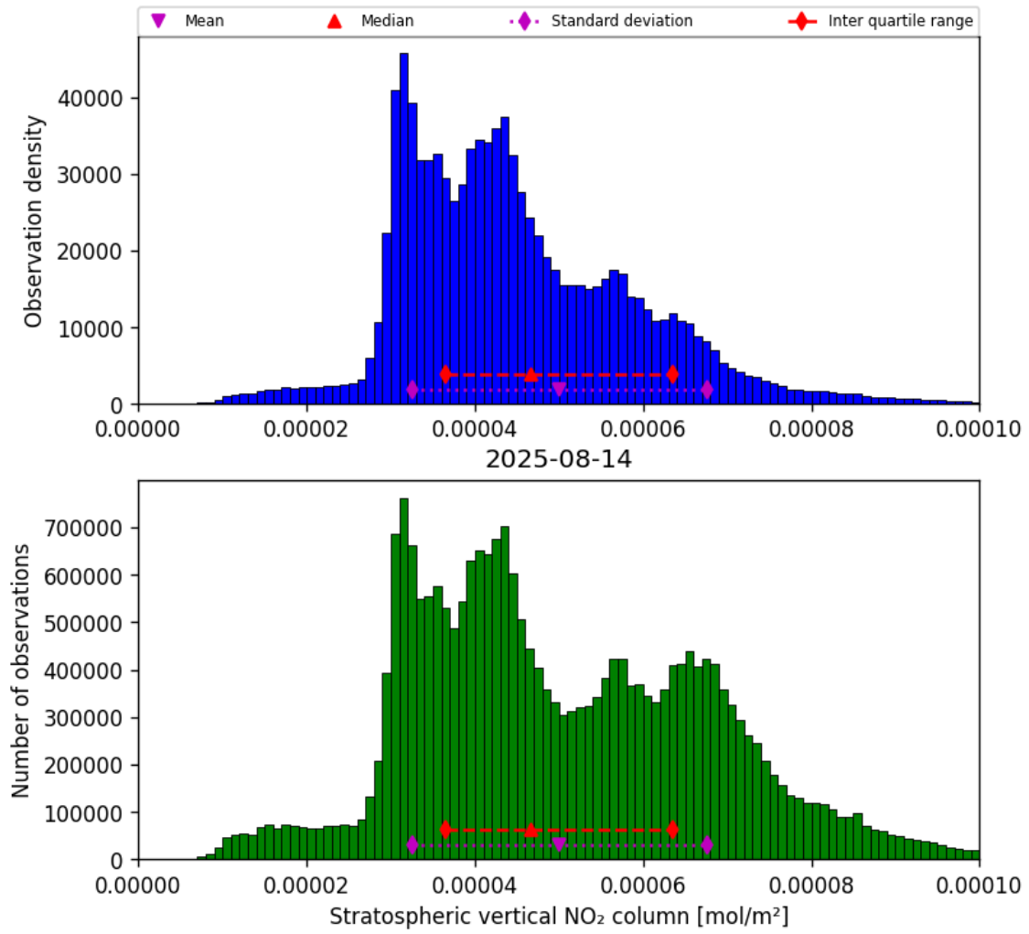
Figure 34: Histogram of “Stratospheric vertical NO 2 column” for 2025-08-14 to 2025-08-15
