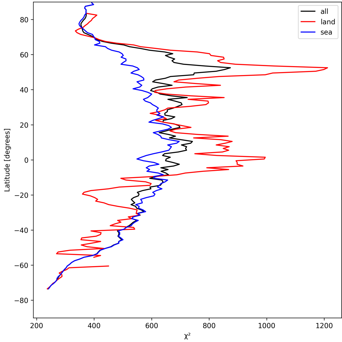
Figure 23: Zonal average of “ \chi^2 ” for 2025-08-14 to 2025-08-15.
