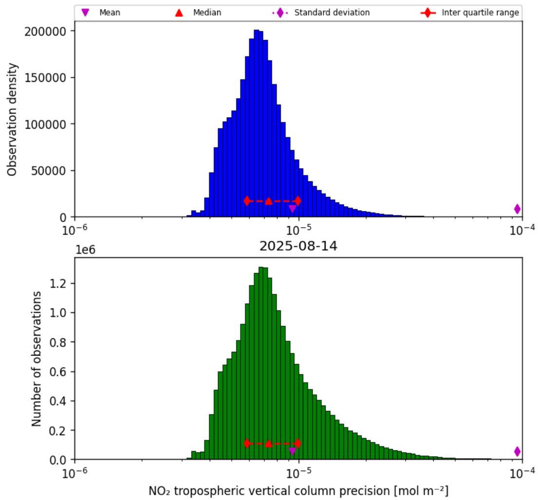
Figure 28: Histogram of “NO 2 tropospheric vertical column precision” for 2025-08-14 to 2025-08-15
