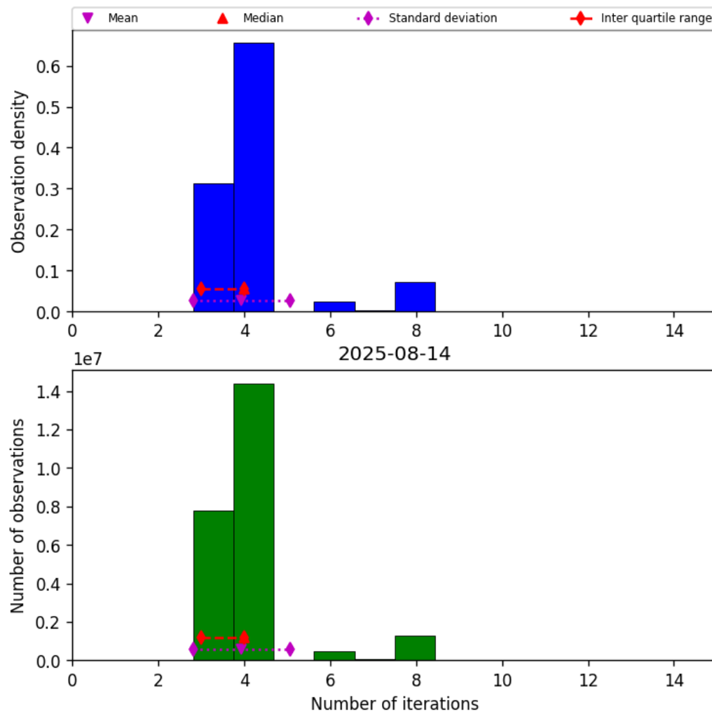
Figure 32: Histogram of “Number of iterations” for 2025-08-14 to 2025-08-15
