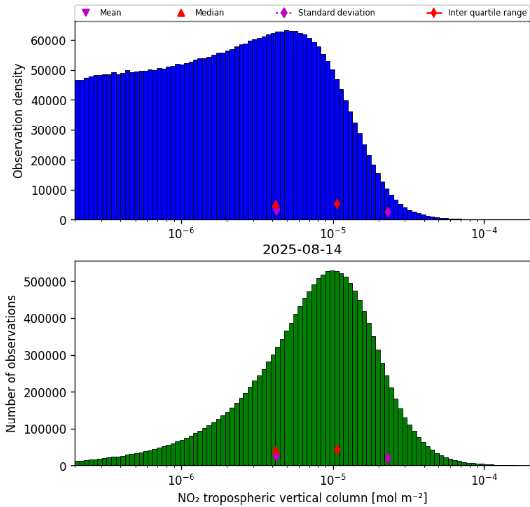
Figure 27: Histogram of “NO 2 tropospheric vertical column” for 2025-08-14 to 2025-08-15
