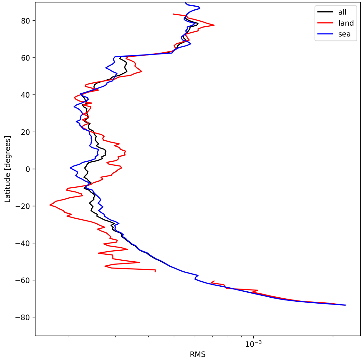
Figure 24: Zonal average of “RMS” for 2025-08-14 to 2025-08-15.
