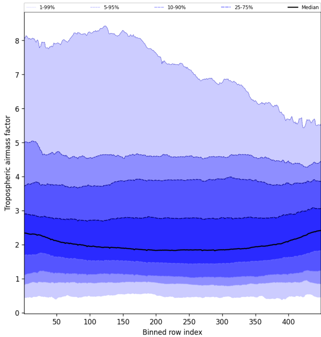
Figure 46: Along track statistics of “Tropospheric air mass factor” for 2025-08-14 to 2025-08-15
