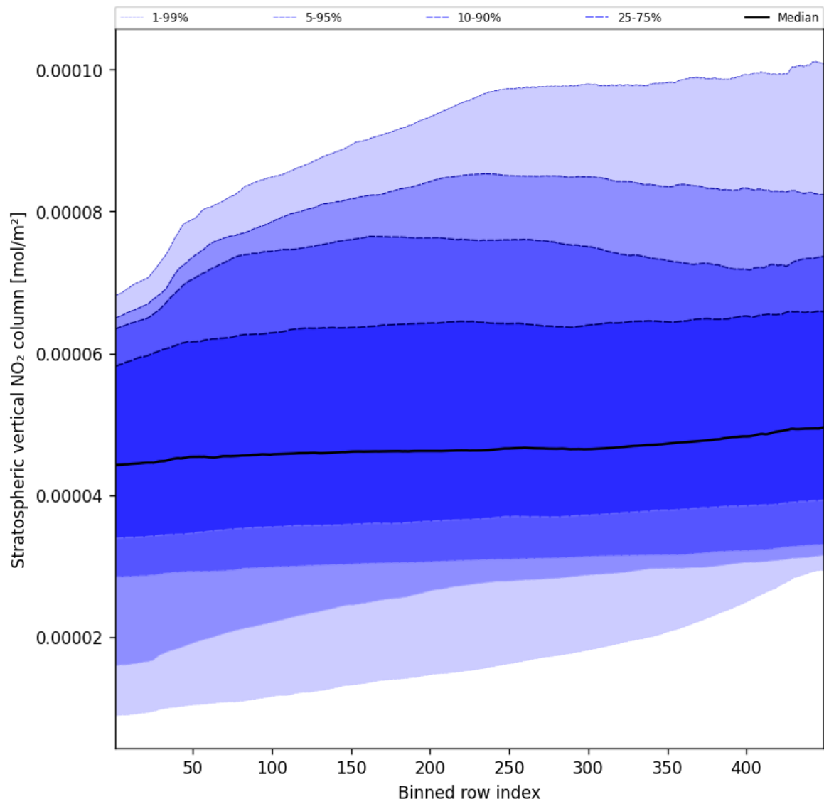
Figure 51: Along track statistics of “Stratospheric vertical NO 2 column” for 2025-08-14 to 2025-08-15
