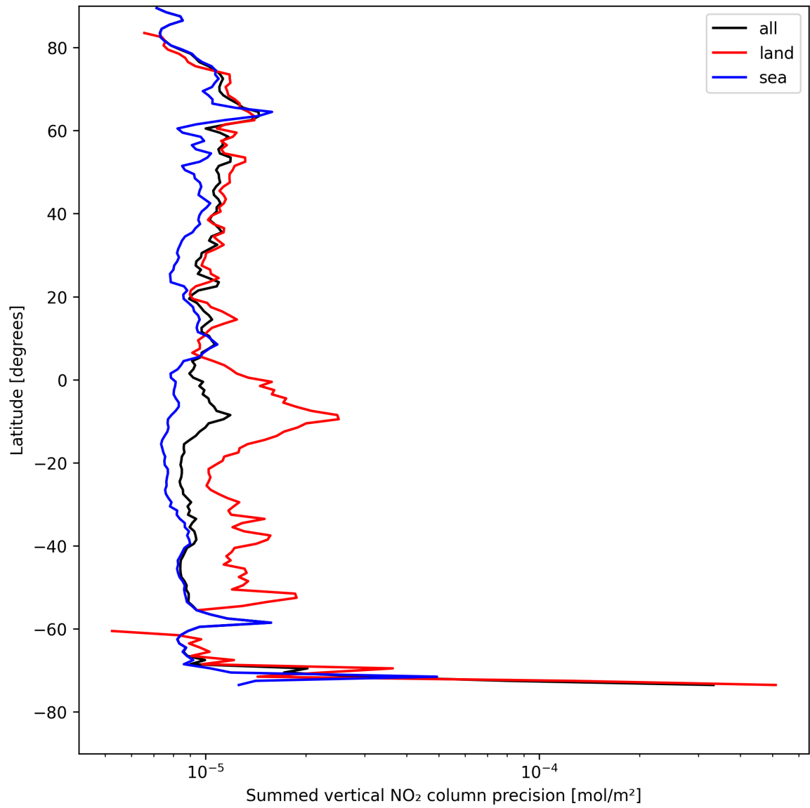
Figure 22: Zonal average of “Summed vertical NO 2 column precision” for 2025-08-14 to 2025-08-15.
