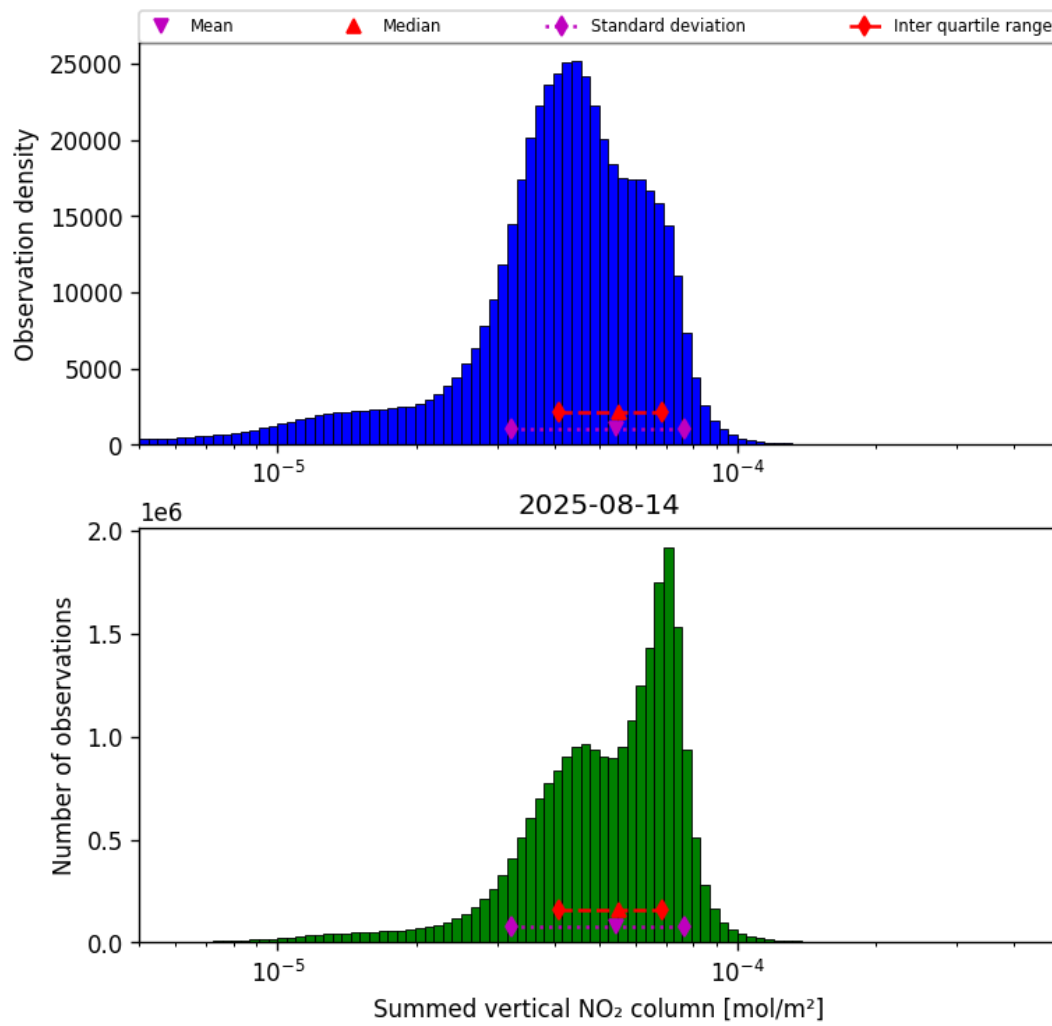
Figure 38: Histogram of “Summed vertical NO 2 column” for 2025-08-14 to 2025-08-15
