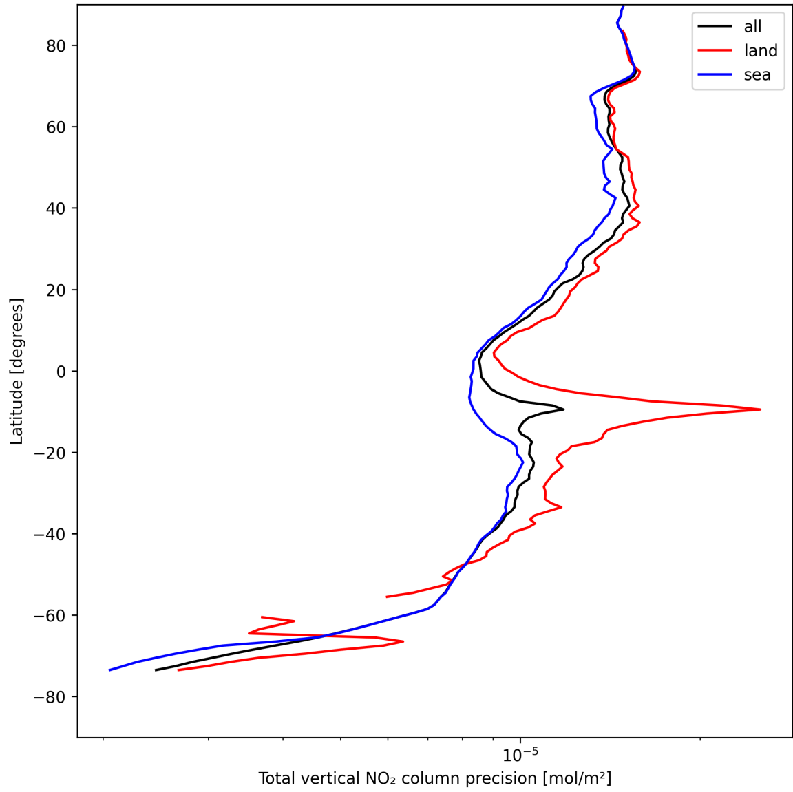
Figure 20: Zonal average of “Total vertical NO 2 column precision” for 2025-08-14 to 2025-08-15.
