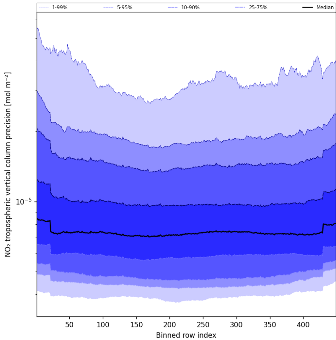
Figure 45: Along track statistics of “NO 2 tropospheric vertical column precision” for 2025-08-14 to 2025-08-15
