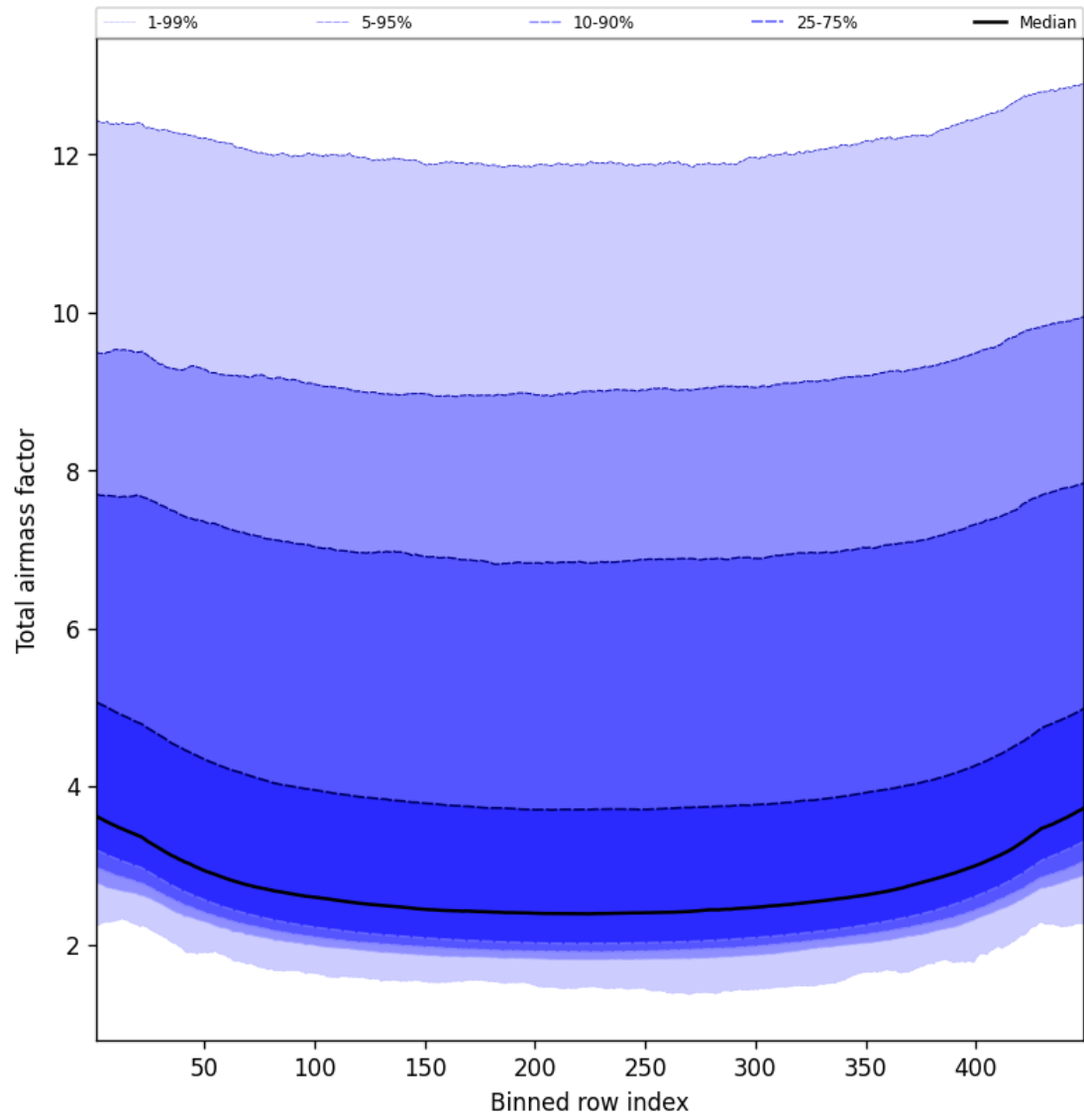
Figure 47: Along track statistics of “Total airmass factor” for 2025-08-14 to 2025-08-15
