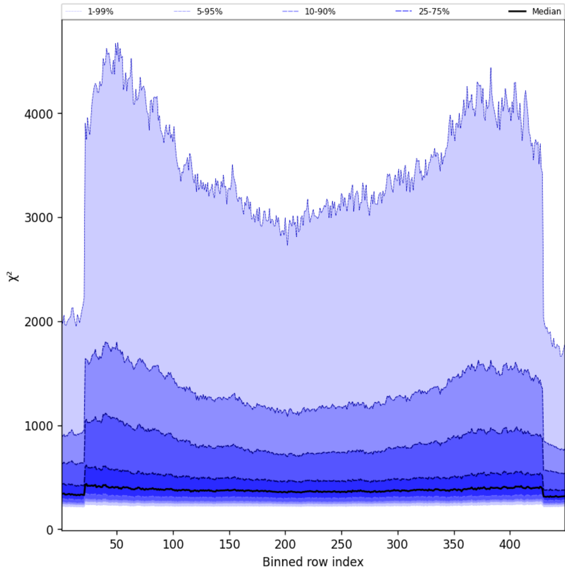
Figure 57: Along track statistics of “ \chi^2 ” for 2025-08-14 to 2025-08-15
