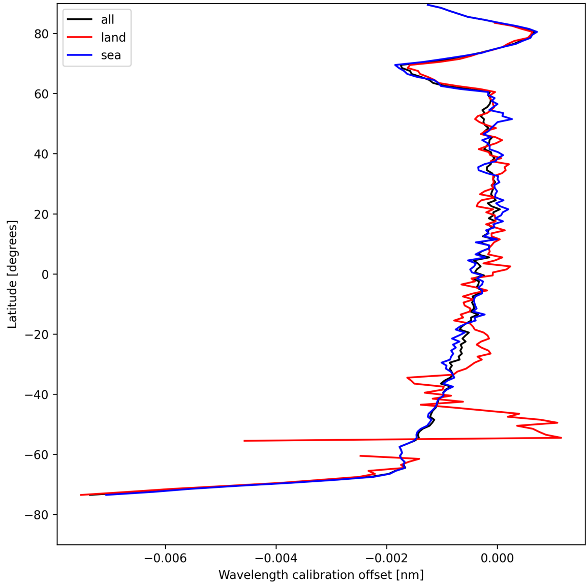
Figure 16: Zonal average of “Wavelength calibration offset” for 2025-08-14 to 2025-08-15.
