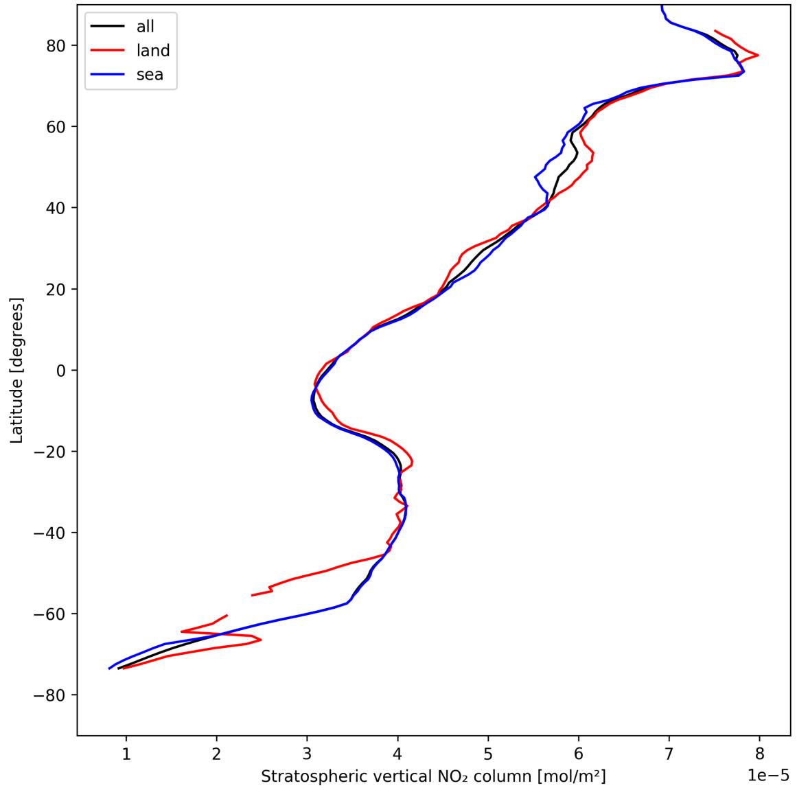
Figure 17: Zonal average of “Stratospheric vertical NO 2 column” for 2025-08-14 to 2025-08-15.
