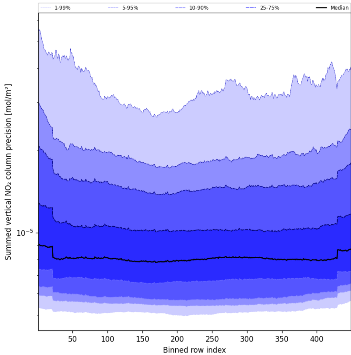
Figure 56: Along track statistics of “Summed vertical NO 2 column precision” for 2025-08-14 to 2025-08-15
