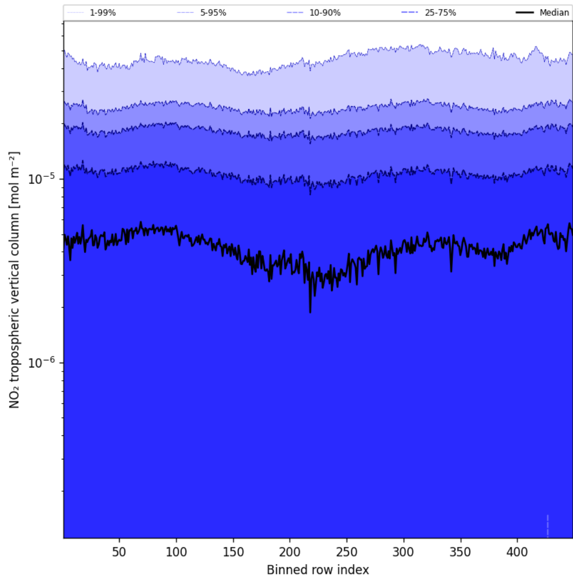
Figure 44: Along track statistics of “NO 2 tropospheric vertical column” for 2025-08-14 to 2025-08-15
