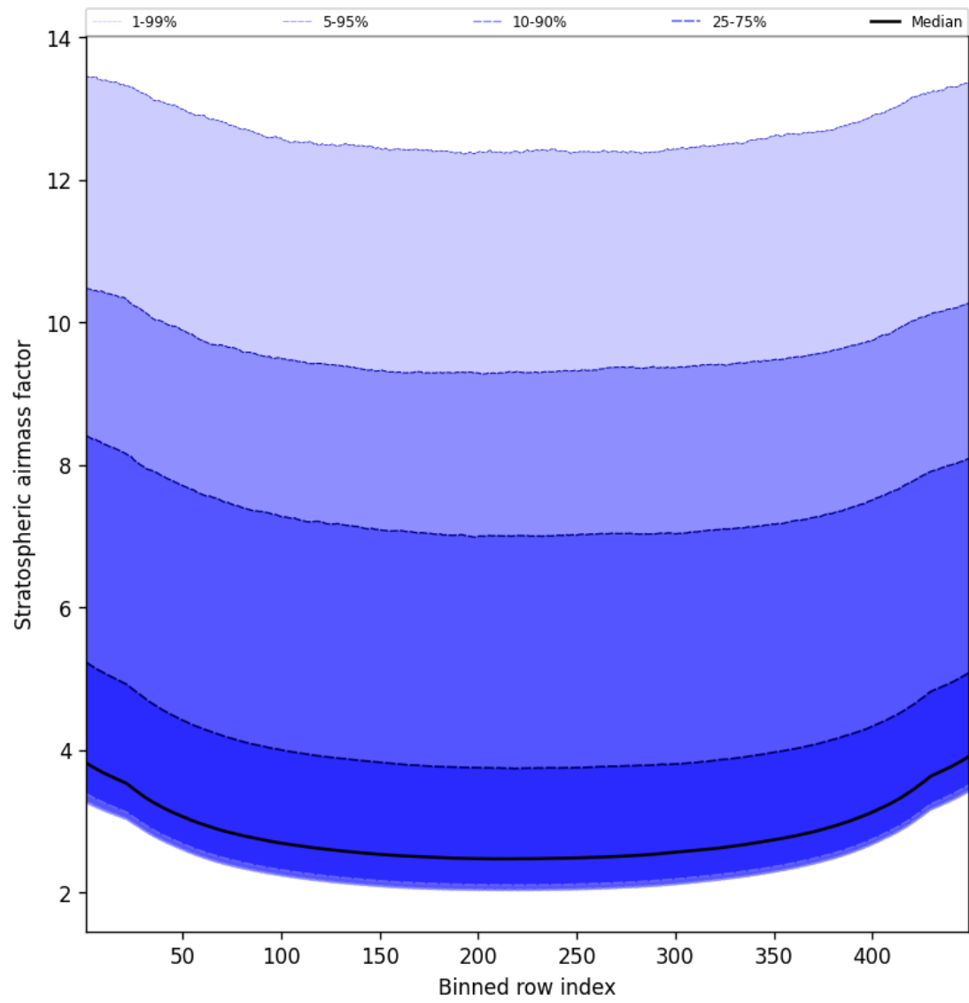
Figure 59: Along track statistics of “Stratospheric airmass factor” for 2025-08-14 to 2025-08-15
