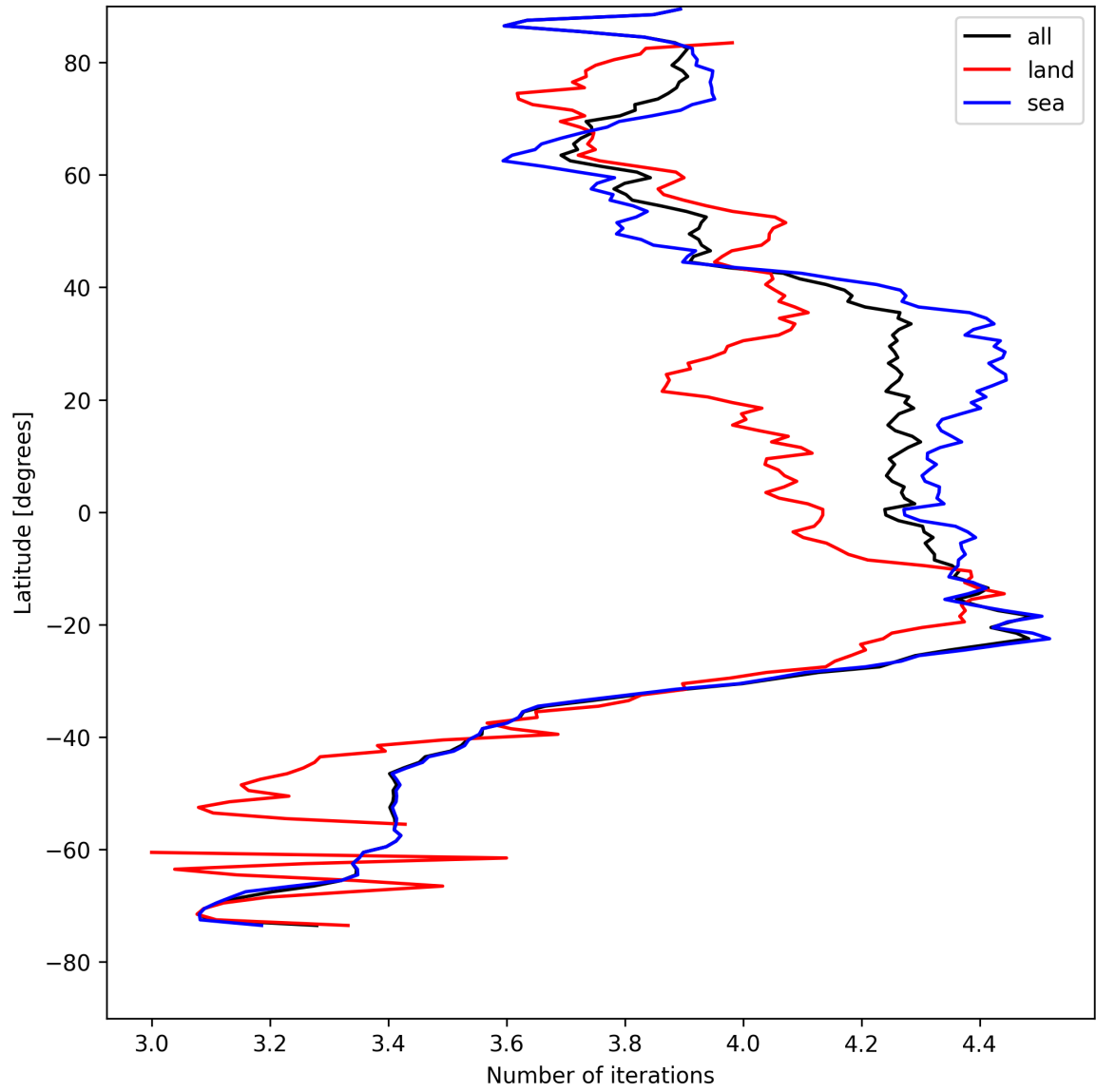
Figure 15: Zonal average of “Number of iterations” for 2025-08-14 to 2025-08-15.
