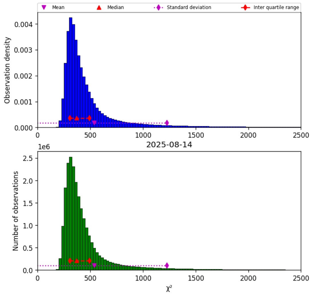
Figure 40: Histogram of “ \chi^2 ” for 2025-08-14 to 2025-08-15
