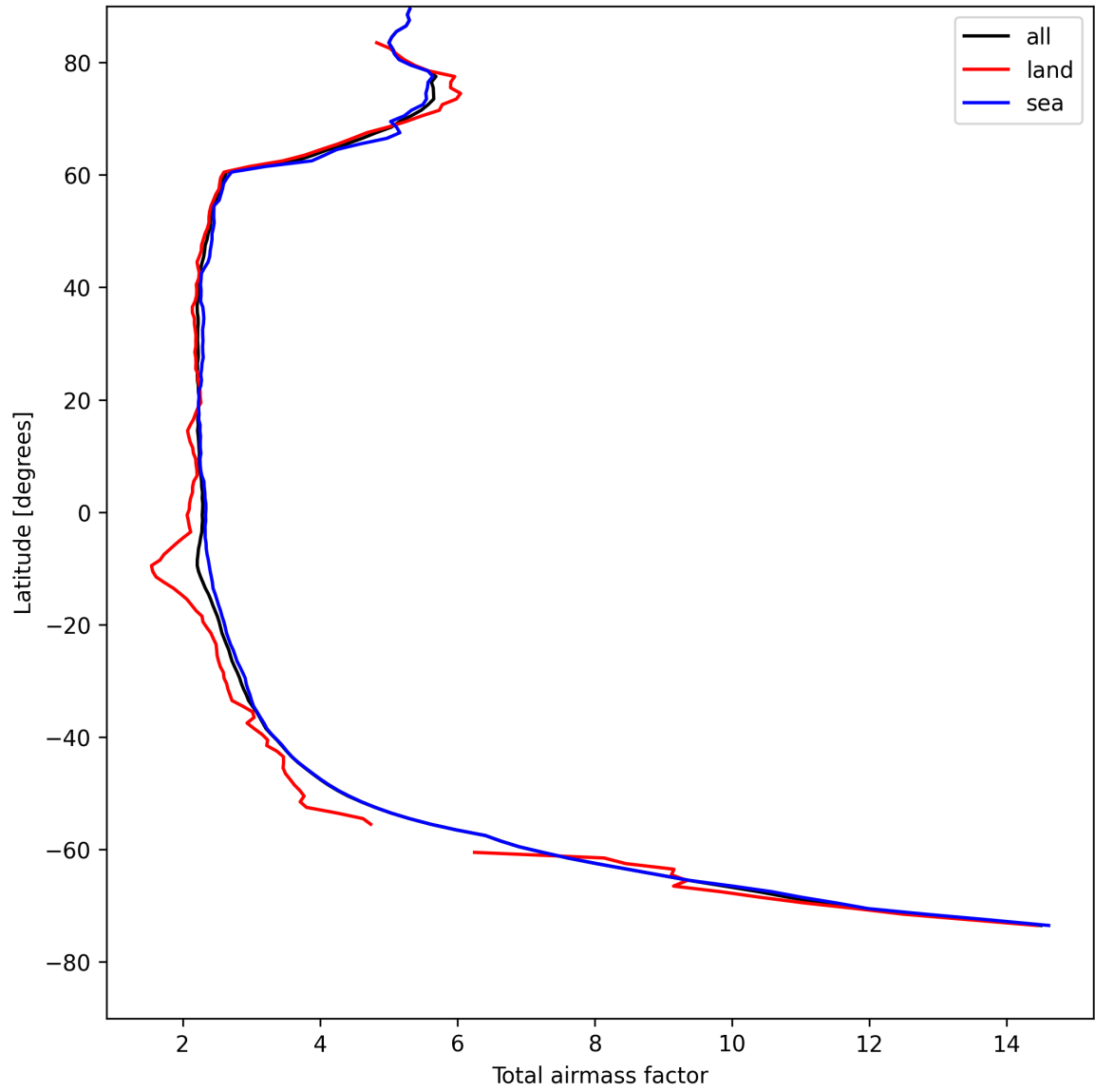
Figure 13: Zonal average of “Total airmass factor” for 2025-08-14 to 2025-08-15.
