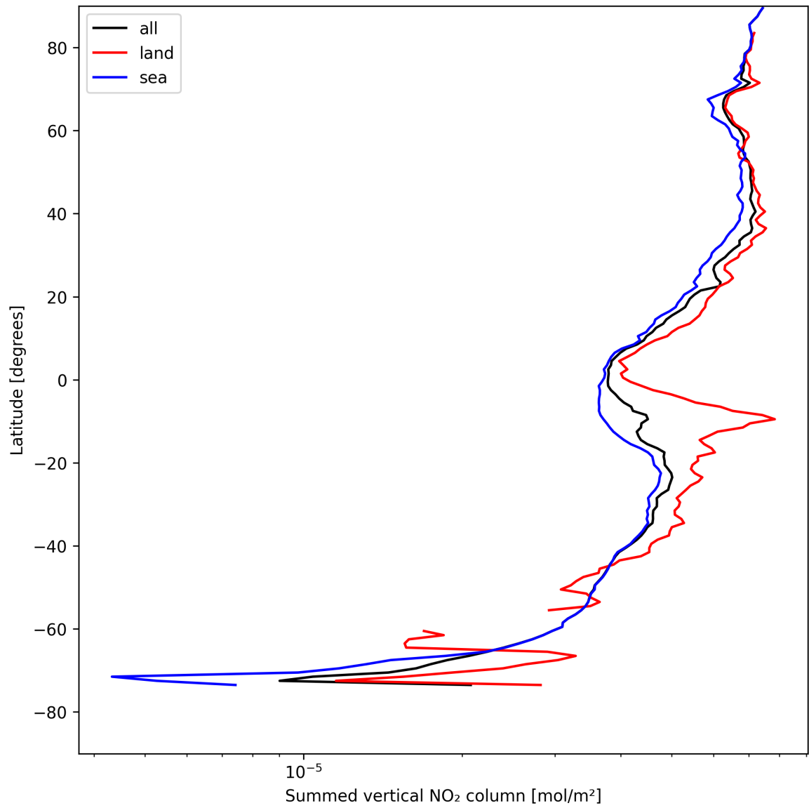
Figure 21: Zonal average of “Summed vertical NO 2 column” for 2025-08-14 to 2025-08-15.
