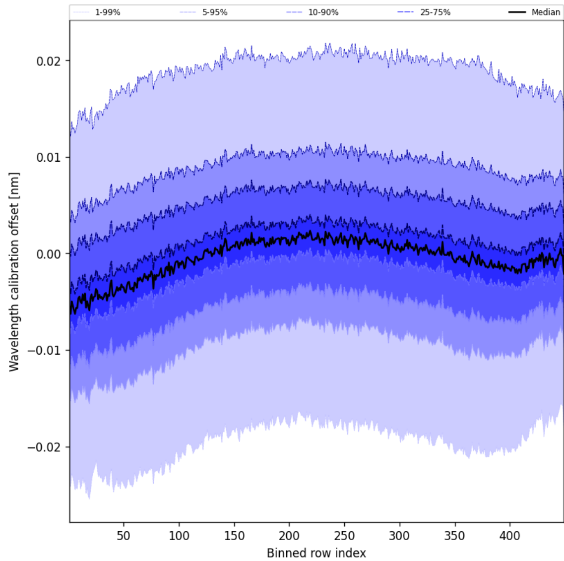
Figure 50: Along track statistics of “Wavelength calibration offset” for 2025-08-14 to 2025-08-15
