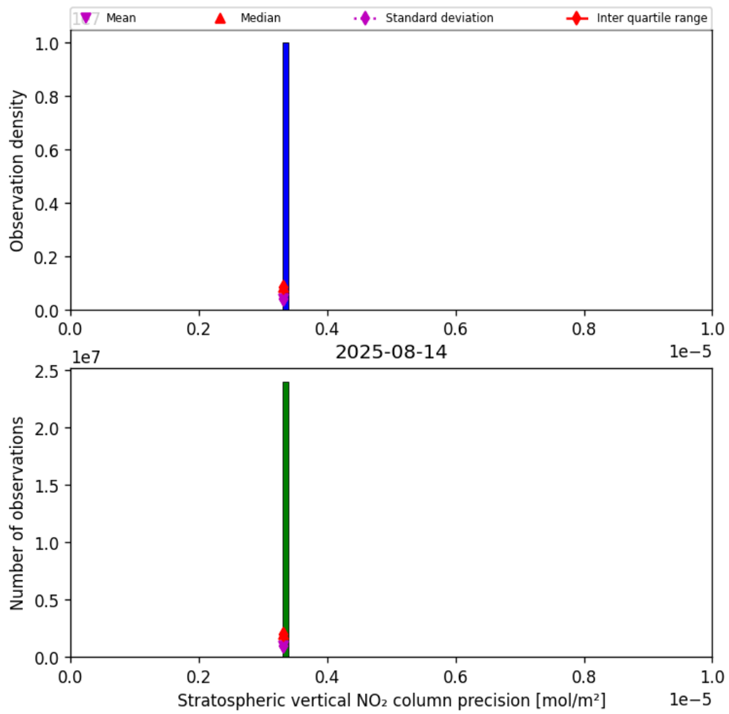
Figure 35: Histogram of “Stratospheric vertical NO 2 column precision” for 2025-08-14 to 2025-08-15
