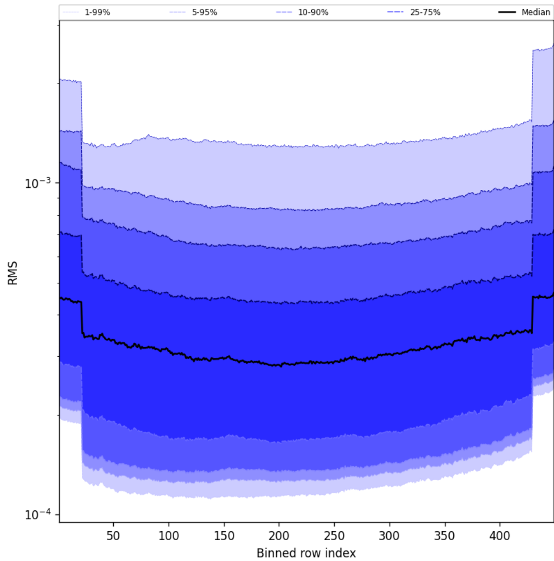
Figure 58: Along track statistics of “RMS” for 2025-08-14 to 2025-08-15
