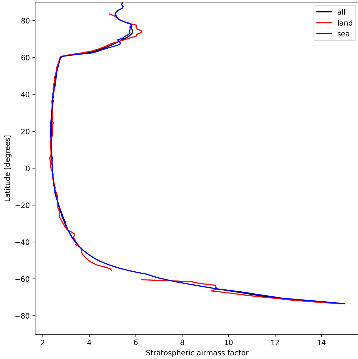
Figure 25: Zonal average of “Stratospheric airmass factor” for 2025-08-14 to 2025-08-15.
