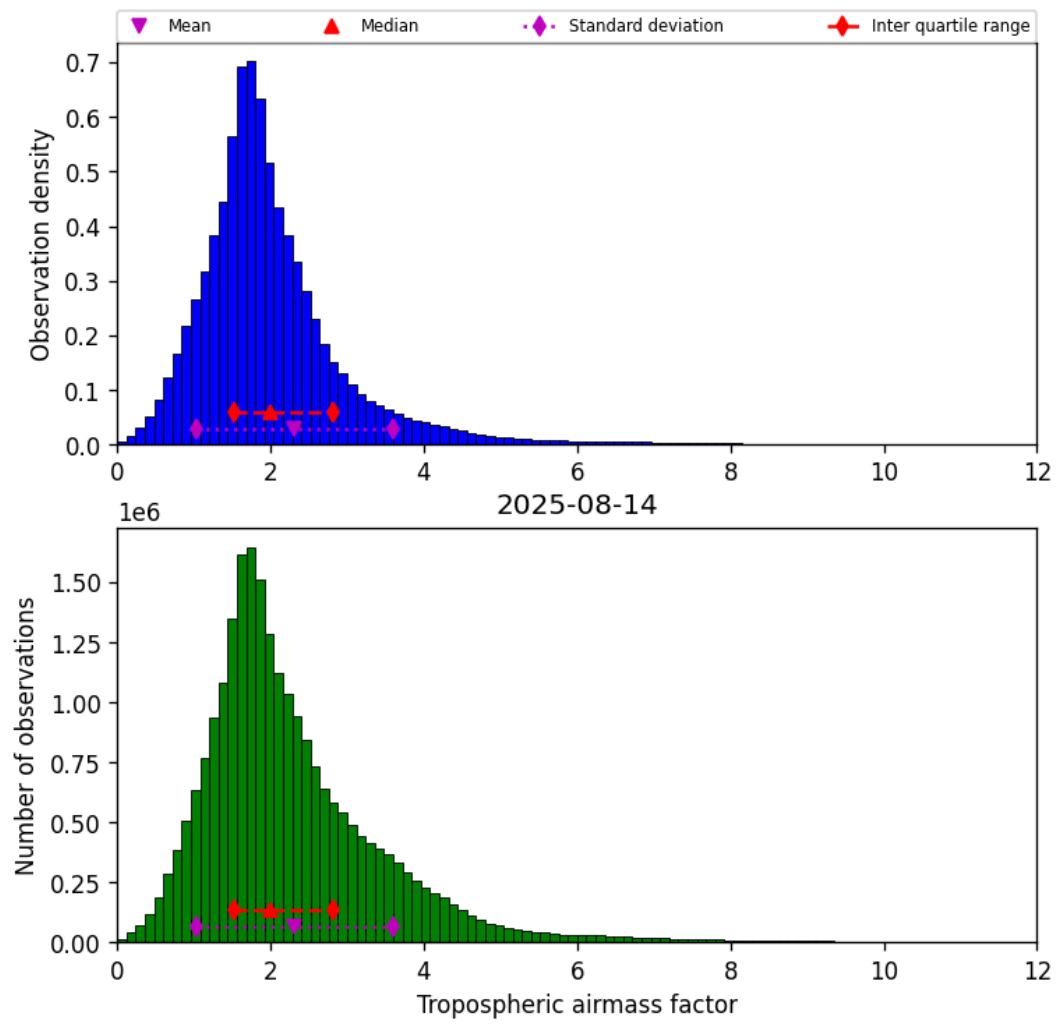
Figure 29: Histogram of “Tropospheric airmass factor” for 2025-08-14 to 2025-08-15
