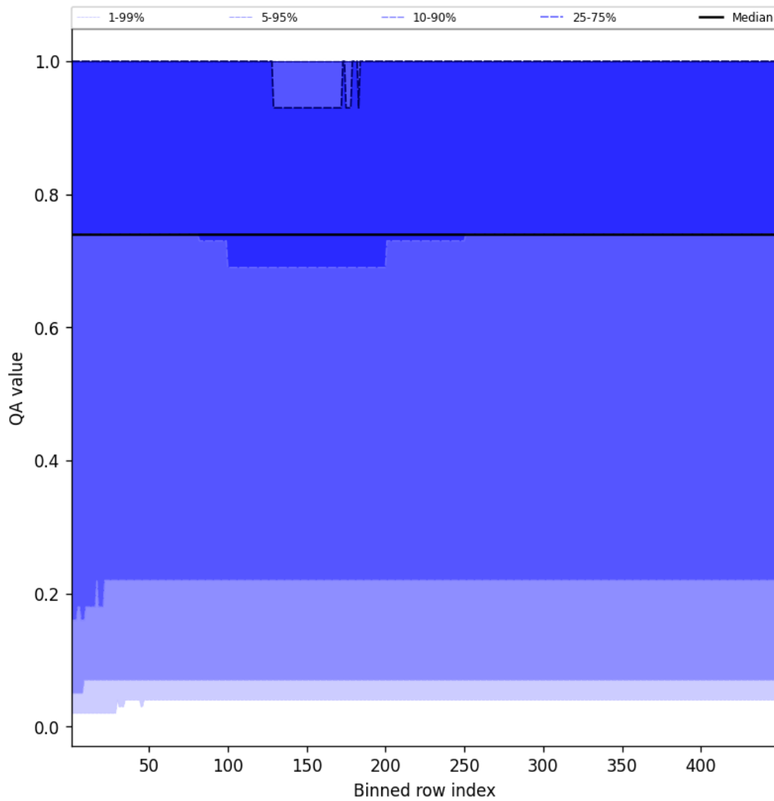
Figure 43: Along track statistics of “QA value” for 2025-08-14 to 2025-08-15
