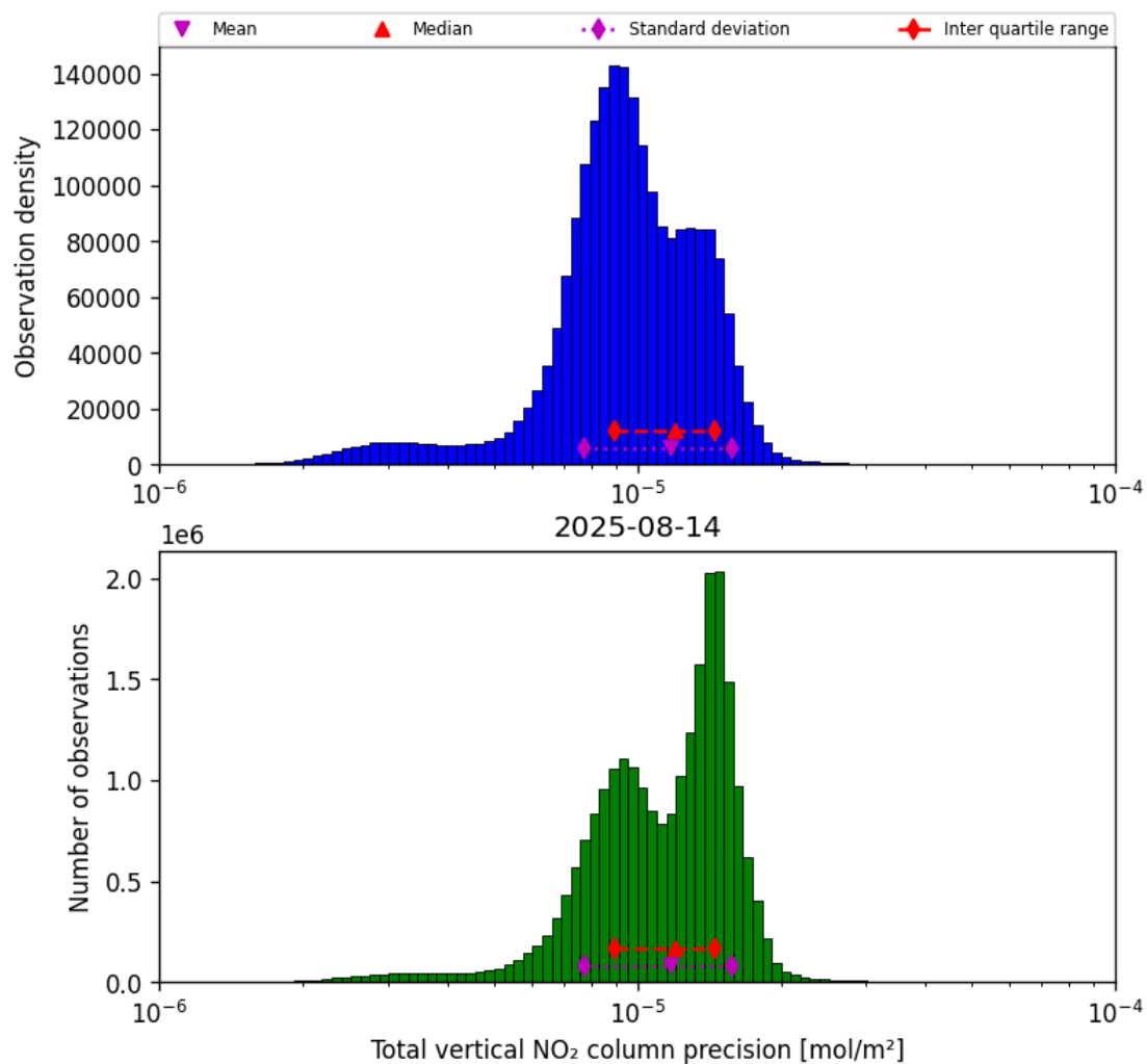
Figure 37: Histogram of “Total vertical NO 2 column precision” for 2025-08-14 to 2025-08-15
