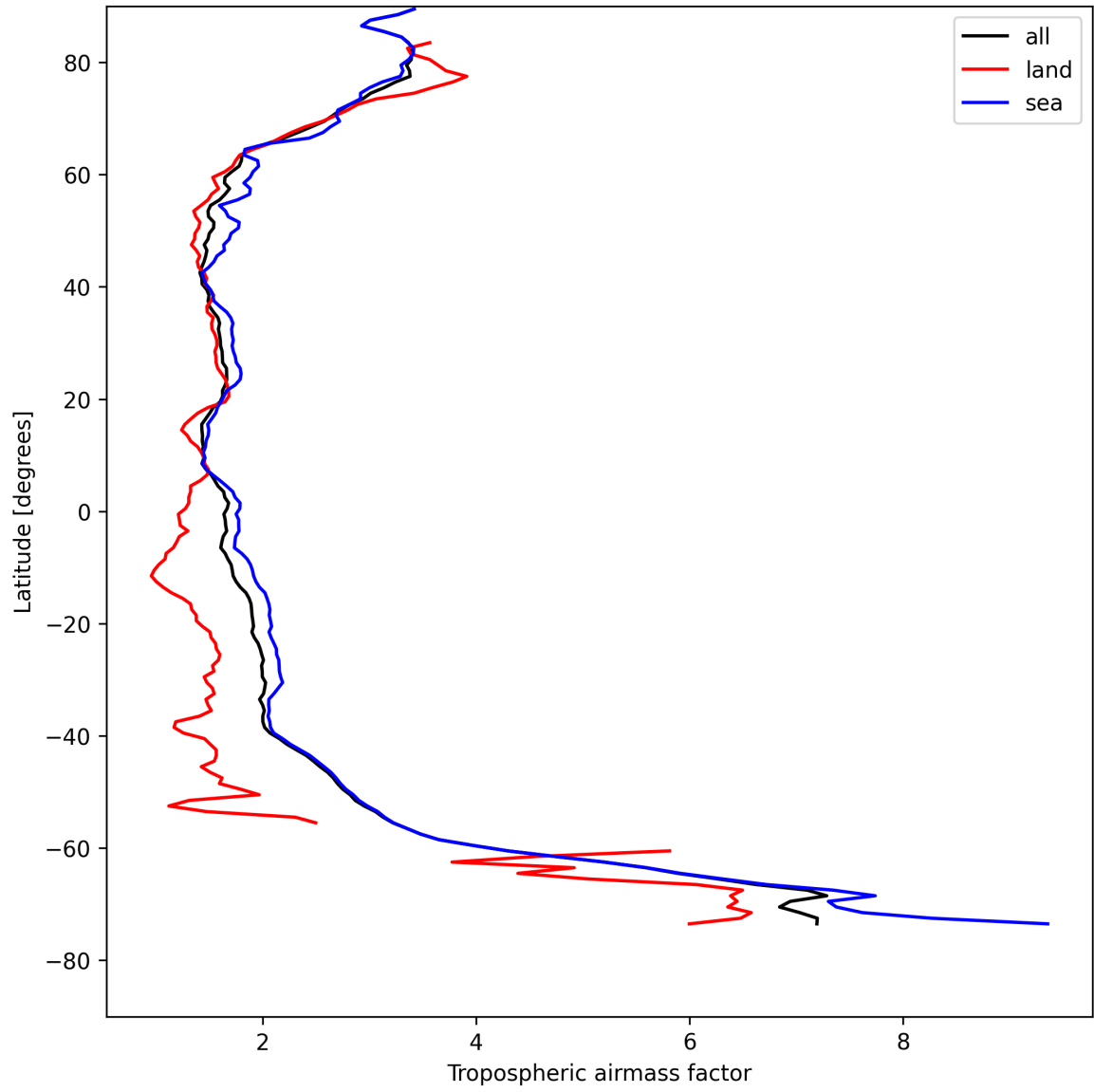
Figure 12: Zonal average of “Tropospheric airmass factor” for 2025-08-14 to 2025-08-15.
