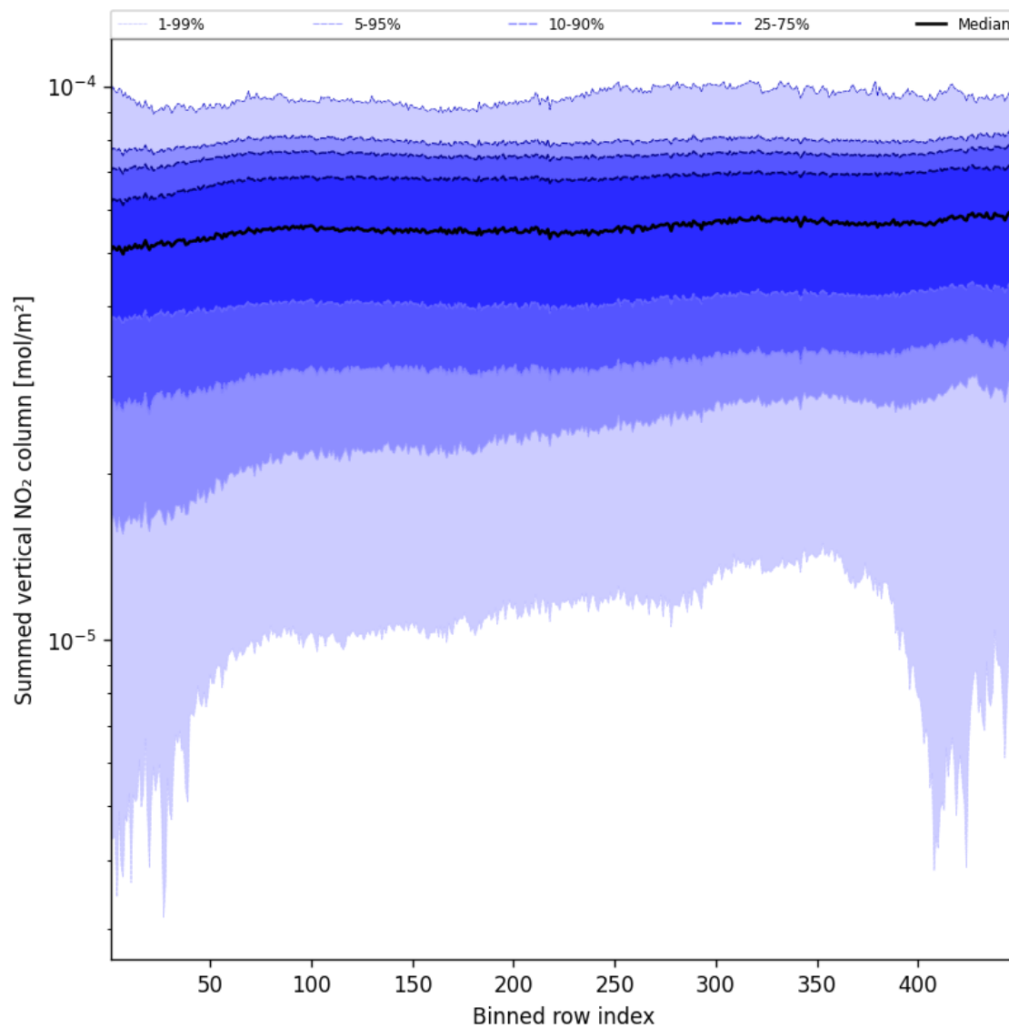
Figure 55: Along track statistics of “Summed vertical NO 2 column” for 2025-08-14 to 2025-08-15
