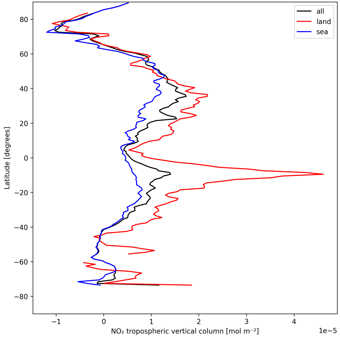
Figure 10: Zonal average of “NO 2 tropospheric vertical column” for 2025-08-14 to 2025-08-15.
