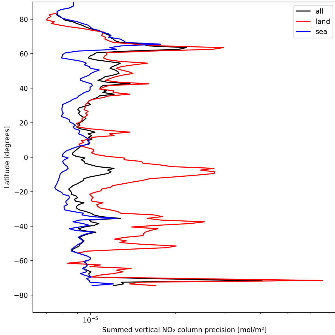
Figure 22: Zonal average of "Summed vertical NO 2 column precision" for 2025-08-15 to 2025-08-16.
