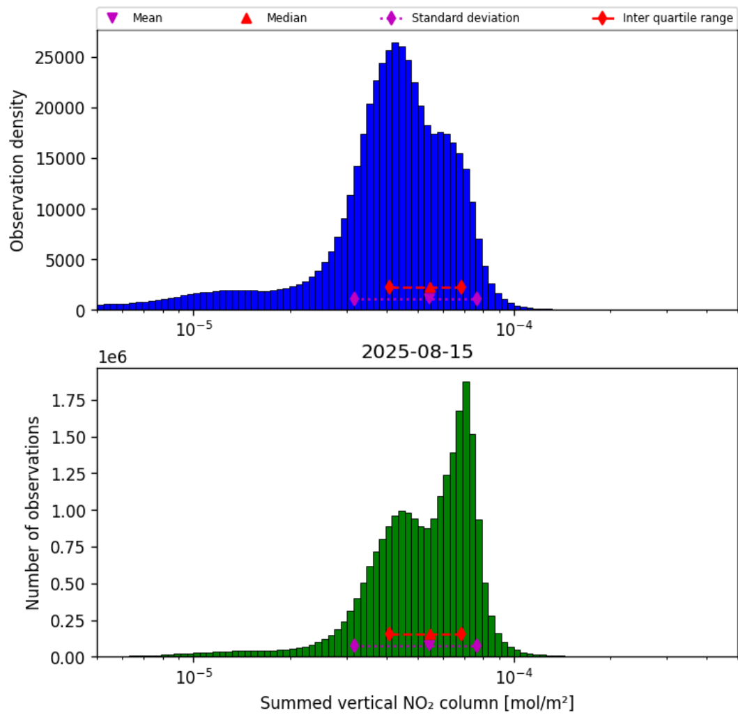
Figure 38: Histogram of "Summed vertical NO 2 column" for 2025-08-15 to 2025-08-16
