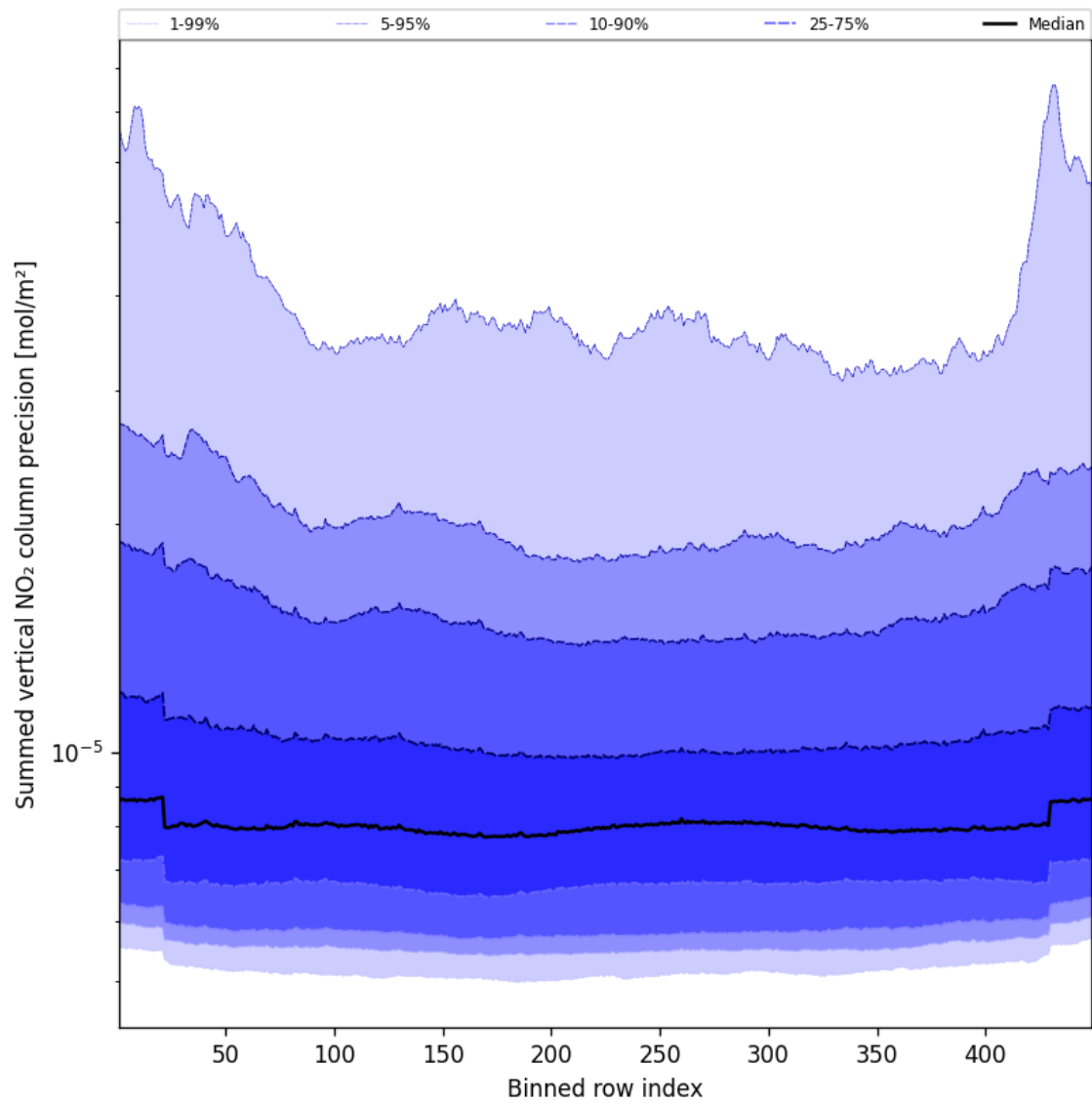
Figure 56: Along track statistics of “Summed vertical NO 2 column precision” for 2025-08-15 to 2025-08-16
