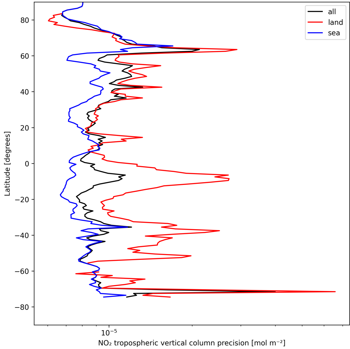
Figure 11: Zonal average of “NO 2 tropospheric vertical column precision” for 2025-08-15 to 2025-08-16.
