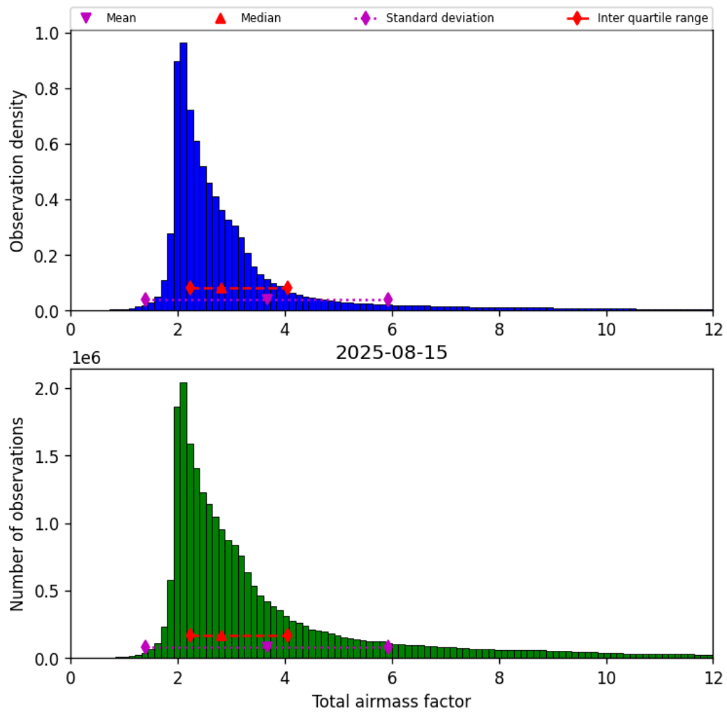
Figure 30: Histogram of “Total airmass factor” for 2025-08-15 to 2025-08-16
