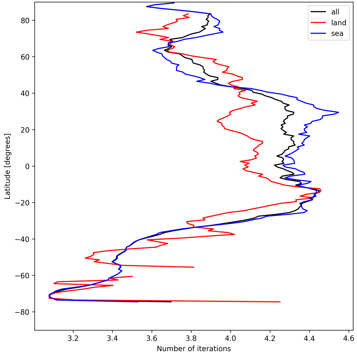
Figure 15: Zonal average of “Number of iterations” for 2025-08-15 to 2025-08-16.
