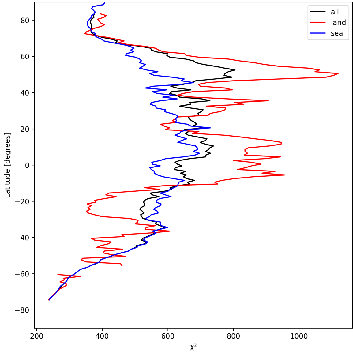
Figure 23: Zonal average of “ \chi^2 ” for 2025-08-15 to 2025-08-16.
