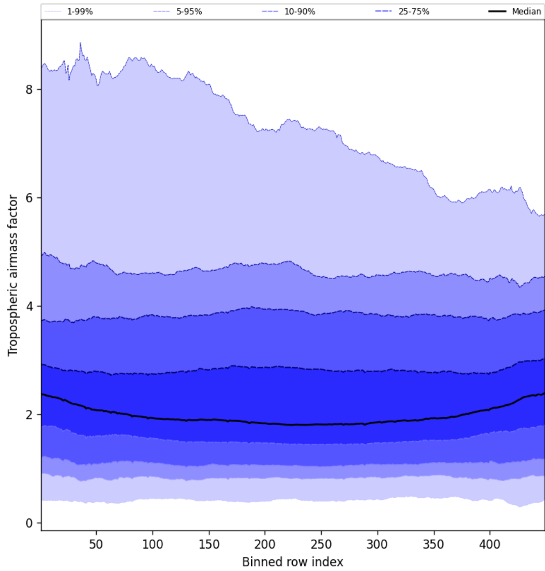
Figure 46: Along track statistics of “Tropospheric air mass factor” for 2025-08-15 to 2025-08-16
