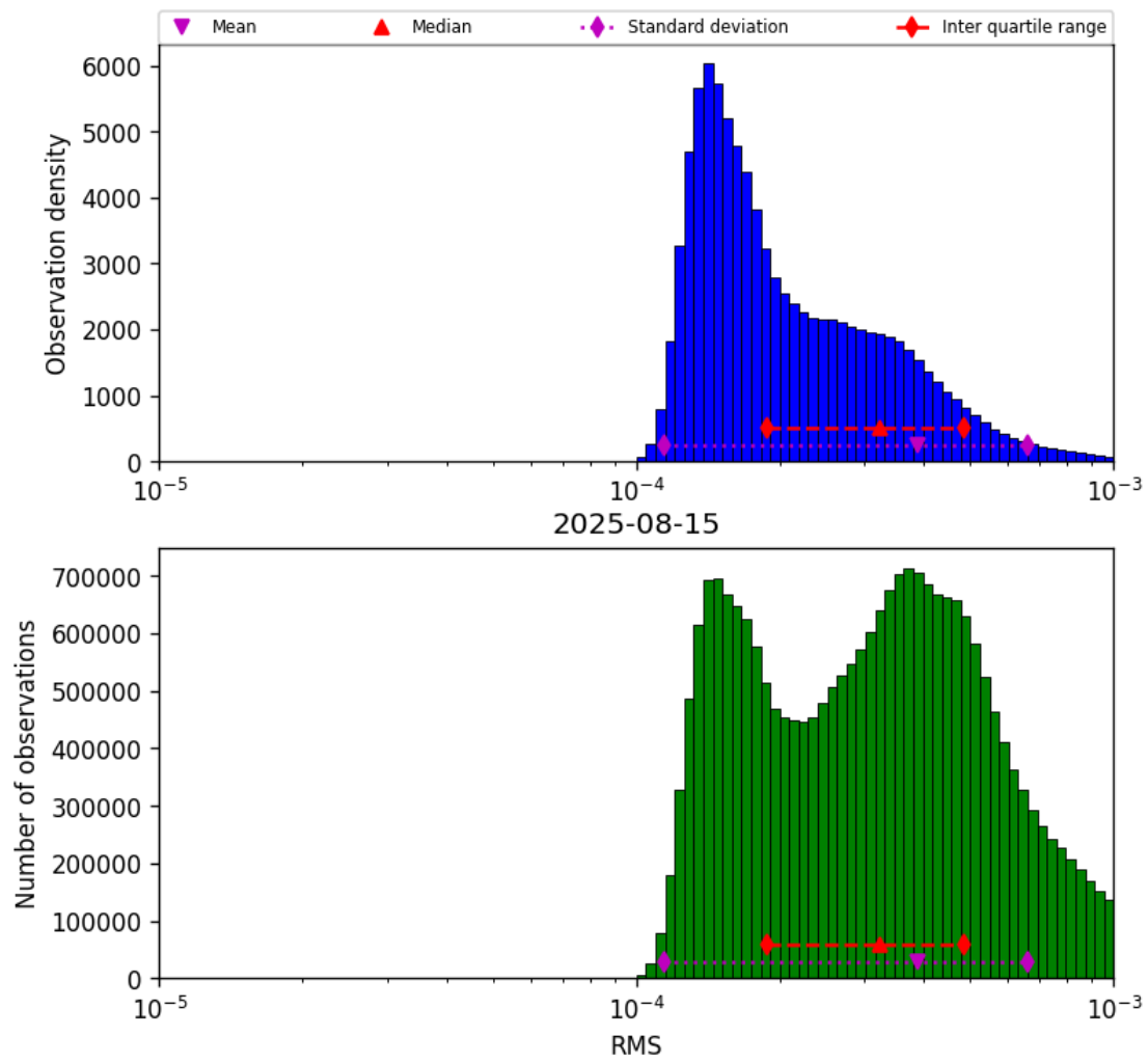
Figure 41: Histogram of “RMS” for 2025-08-15 to 2025-08-16
