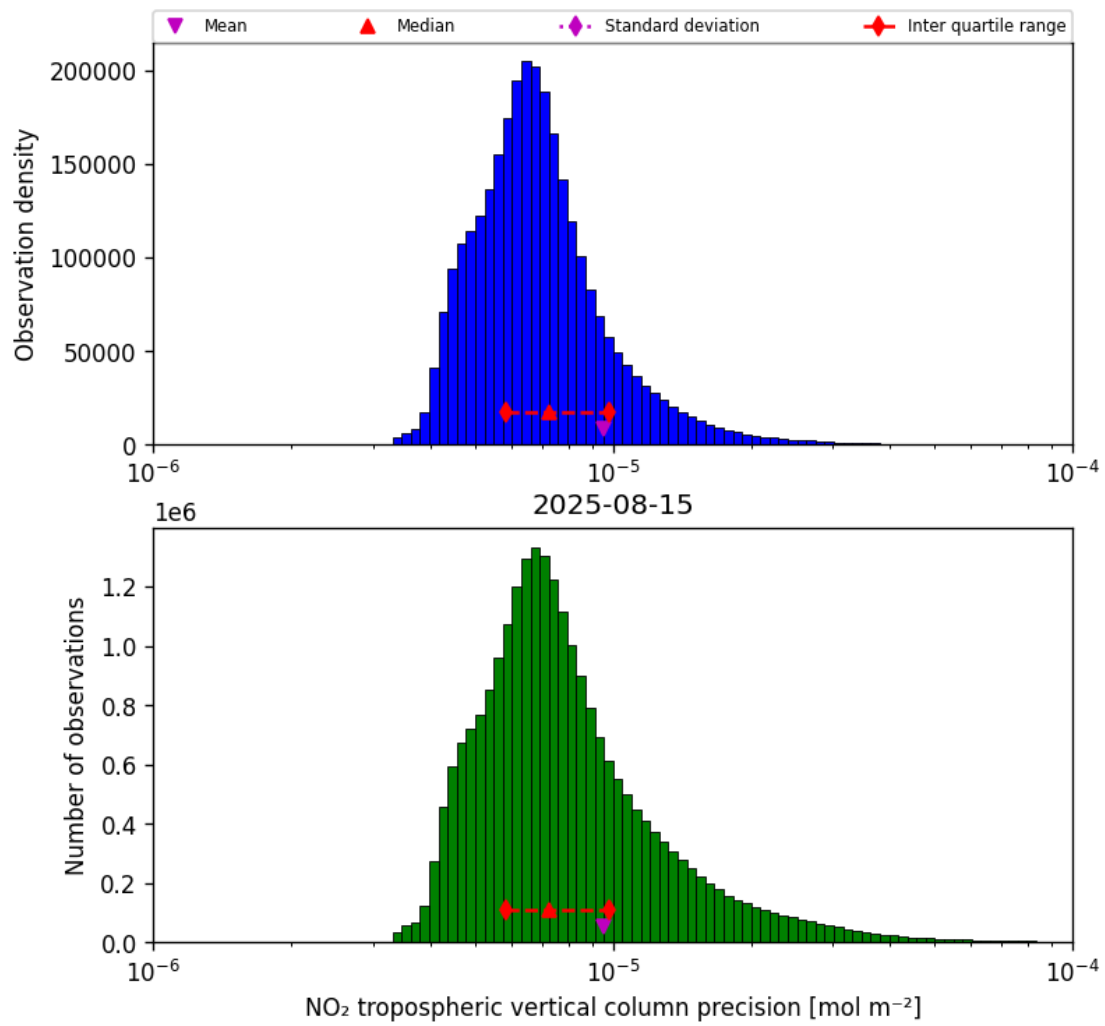
Figure 28: Histogram of “NO 2 tropospheric vertical column precision” for 2025-08-15 to 2025-08-16
