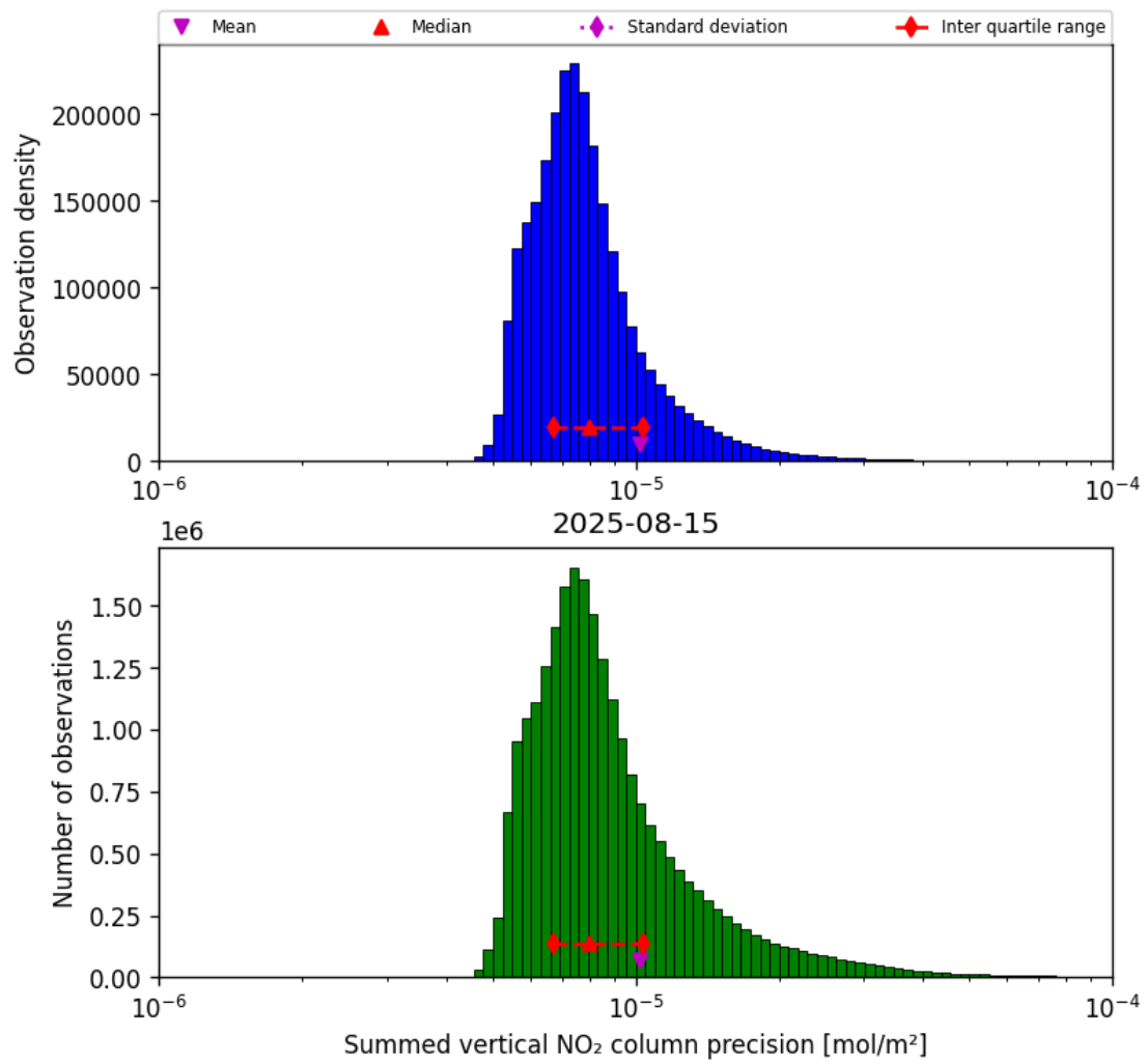
Figure 39: Histogram of “Summed vertical NO 2 column precision” for 2025-08-15 to 2025-08-16
