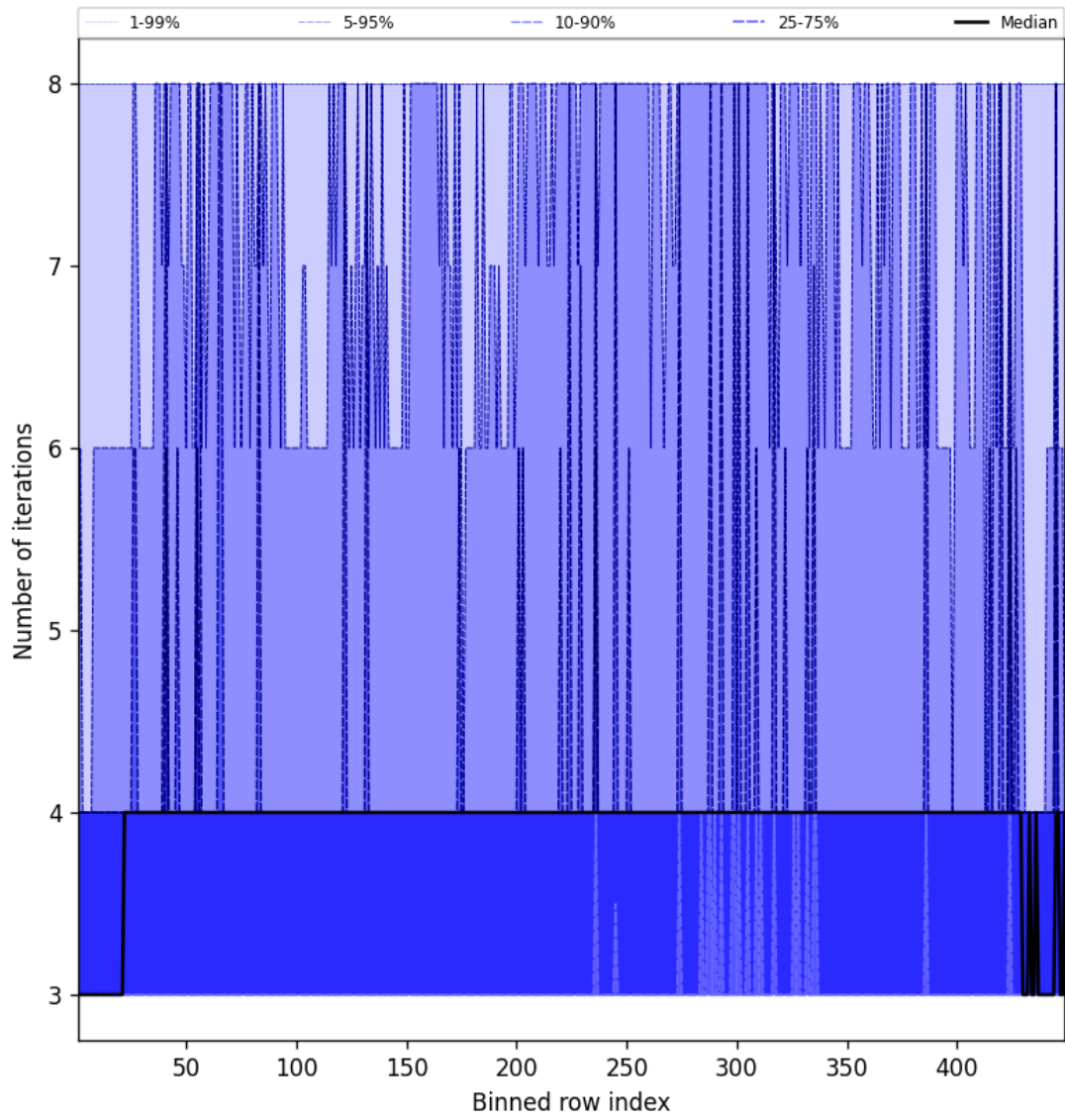
Figure 49: Along track statistics of “Number of iterations” for 2025-08-15 to 2025-08-16
