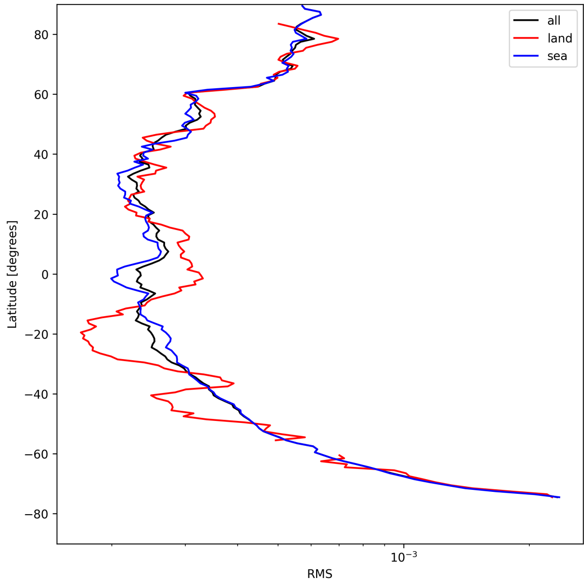
Figure 24: Zonal average of “RMS” for 2025-08-15 to 2025-08-16.
