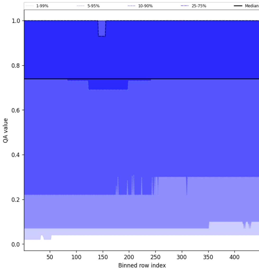
Figure 43: Along track statistics of “QA value” for 2025-08-15 to 2025-08-16
