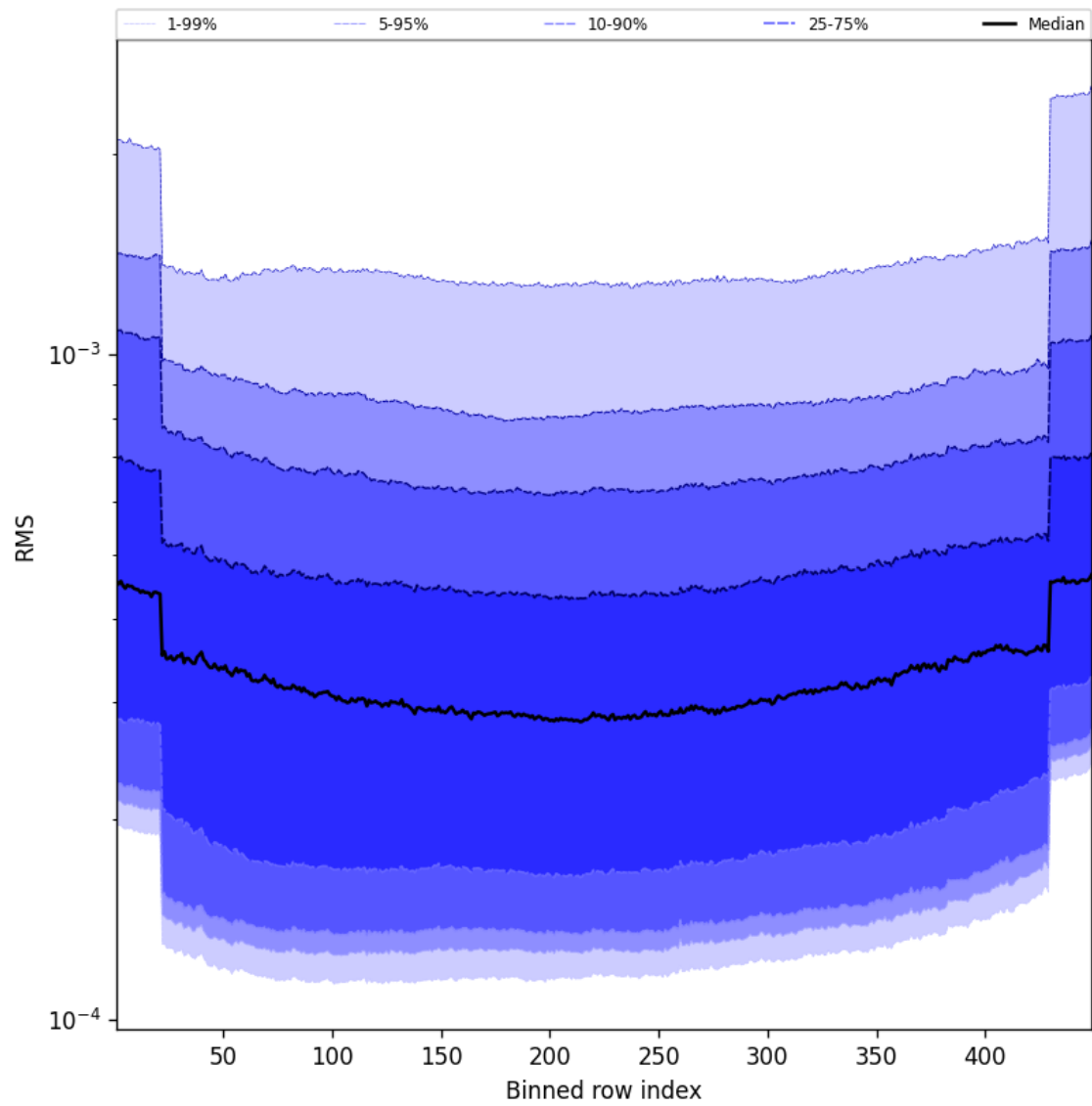
Figure 58: Along track statistics of “RMS” for 2025-08-15 to 2025-08-16
