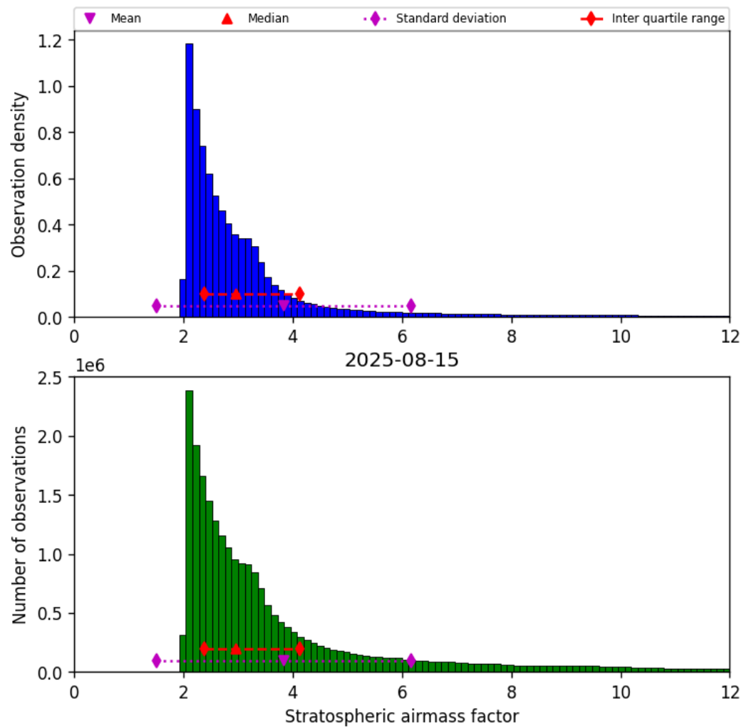
Figure 42: Histogram of “Stratospheric airmass factor” for 2025-08-15 to 2025-08-16
