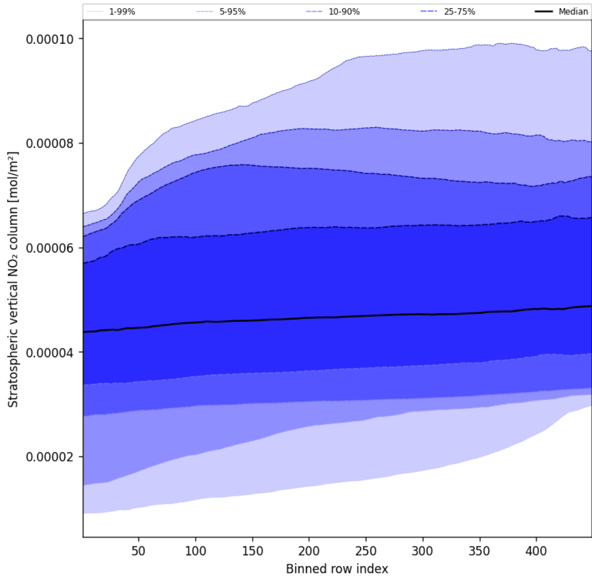
Figure 51: Along track statistics of “Stratospheric vertical NO 2 column” for 2025-08-15 to 2025-08-16
