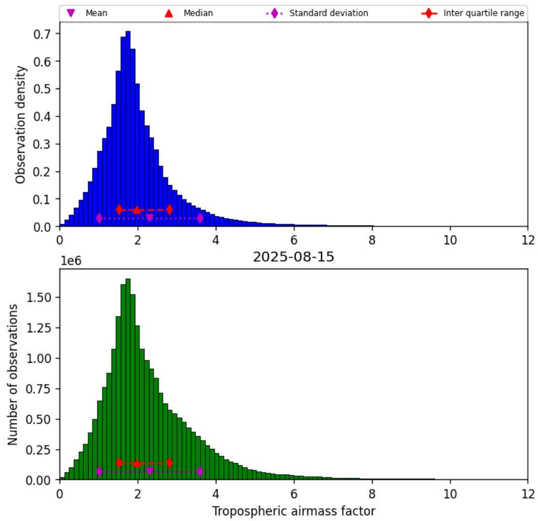
Figure 29: Histogram of “Tropospheric airmass factor” for 2025-08-15 to 2025-08-16
