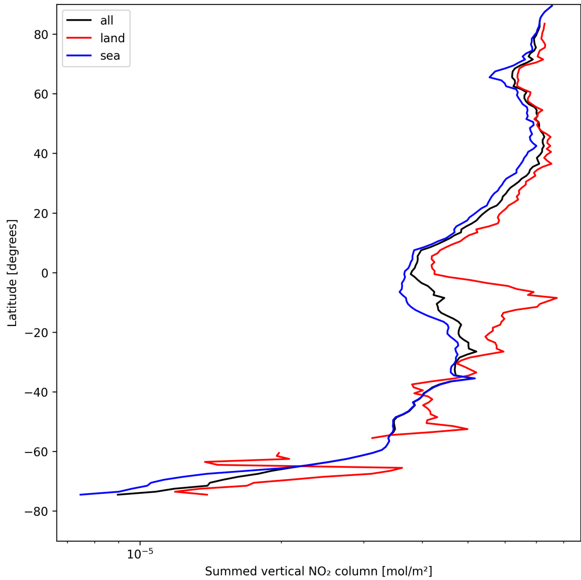
Figure 21: Zonal average of “Summed vertical NO 2 column” for 2025-08-15 to 2025-08-16.
