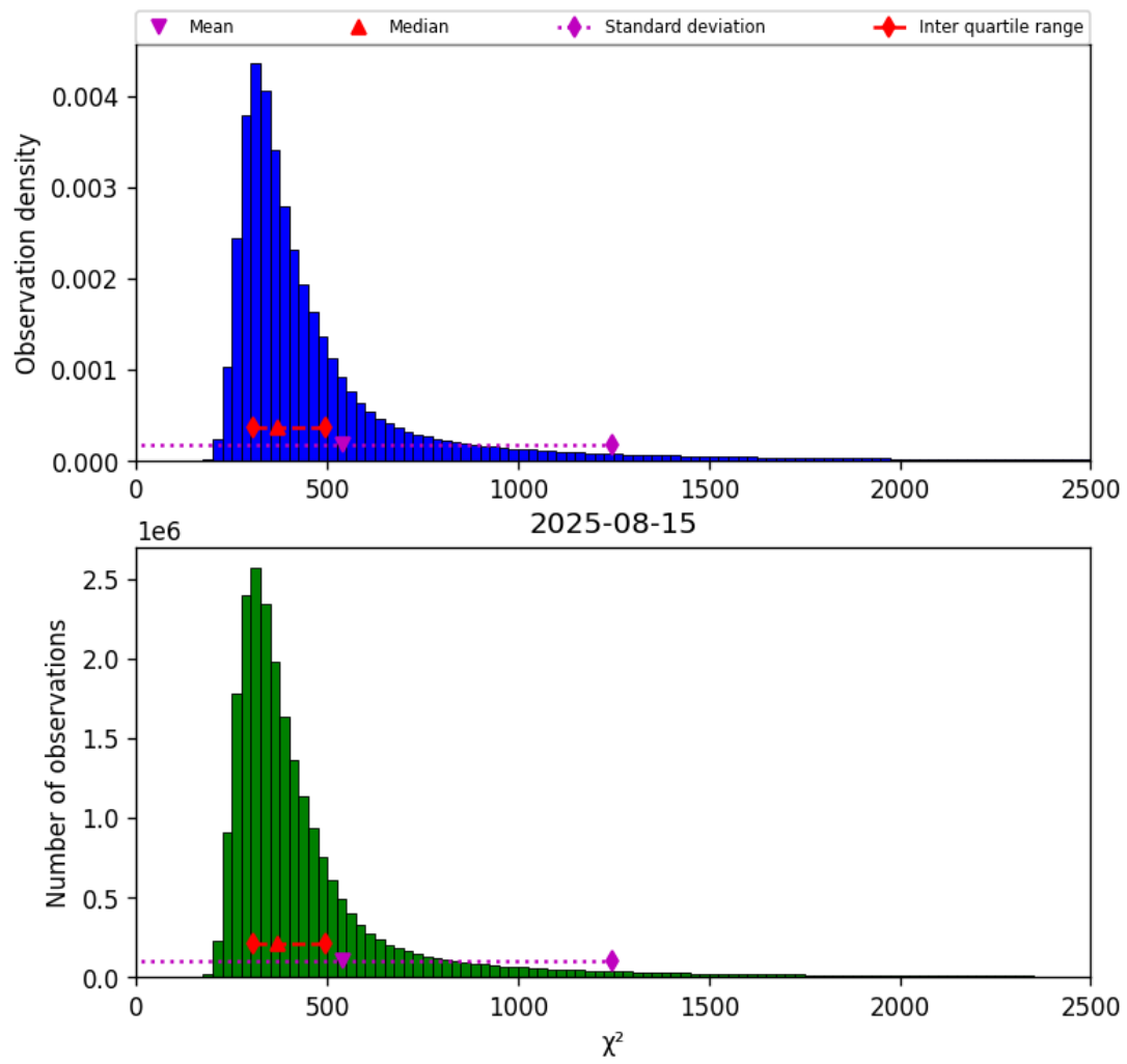
Figure 40: Histogram of “ \chi^2 ” for 2025-08-15 to 2025-08-16
