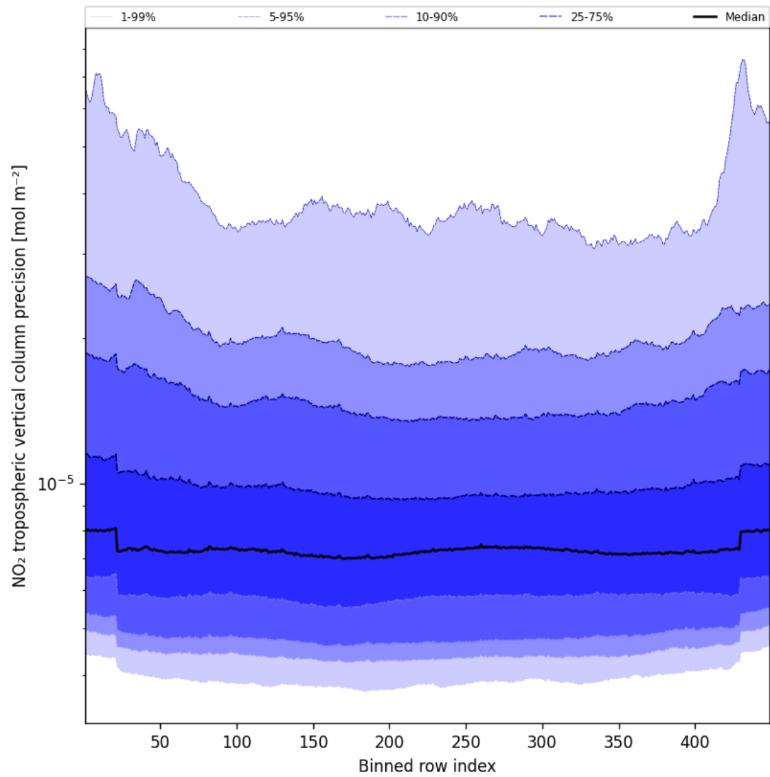
Figure 45: Along track statistics of “NO 2 tropospheric vertical column precision” for 2025-08-15 to 2025-08-16
