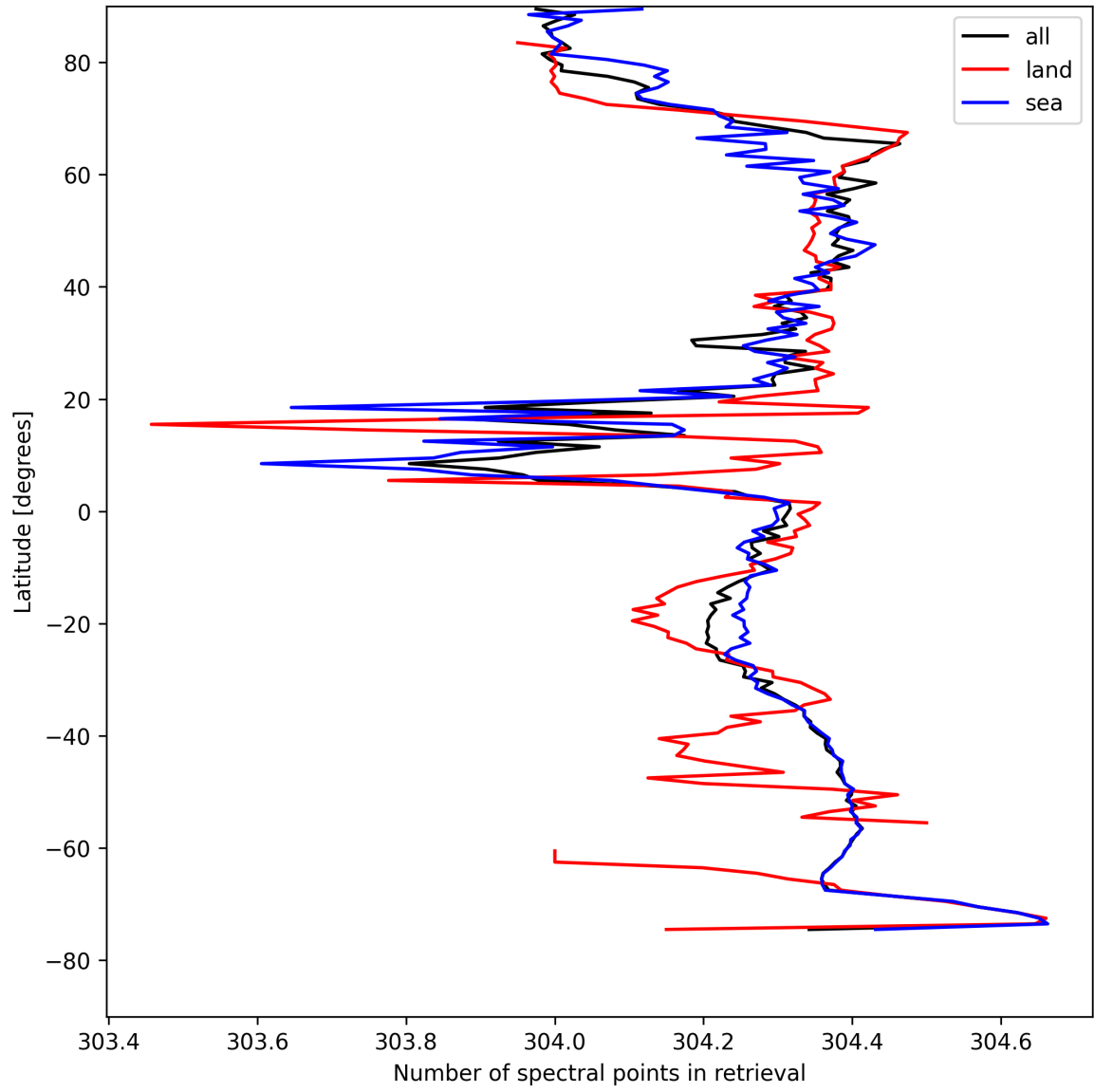
Figure 14: Zonal average of “Number of spectral points in retrieval” for 2025-08-15 to 2025-08-16.
