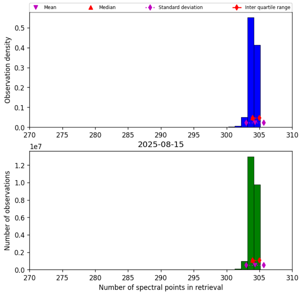
Figure 31: Histogram of “Number of spectral points in retrieval” for 2025-08-15 to 2025-08-16
