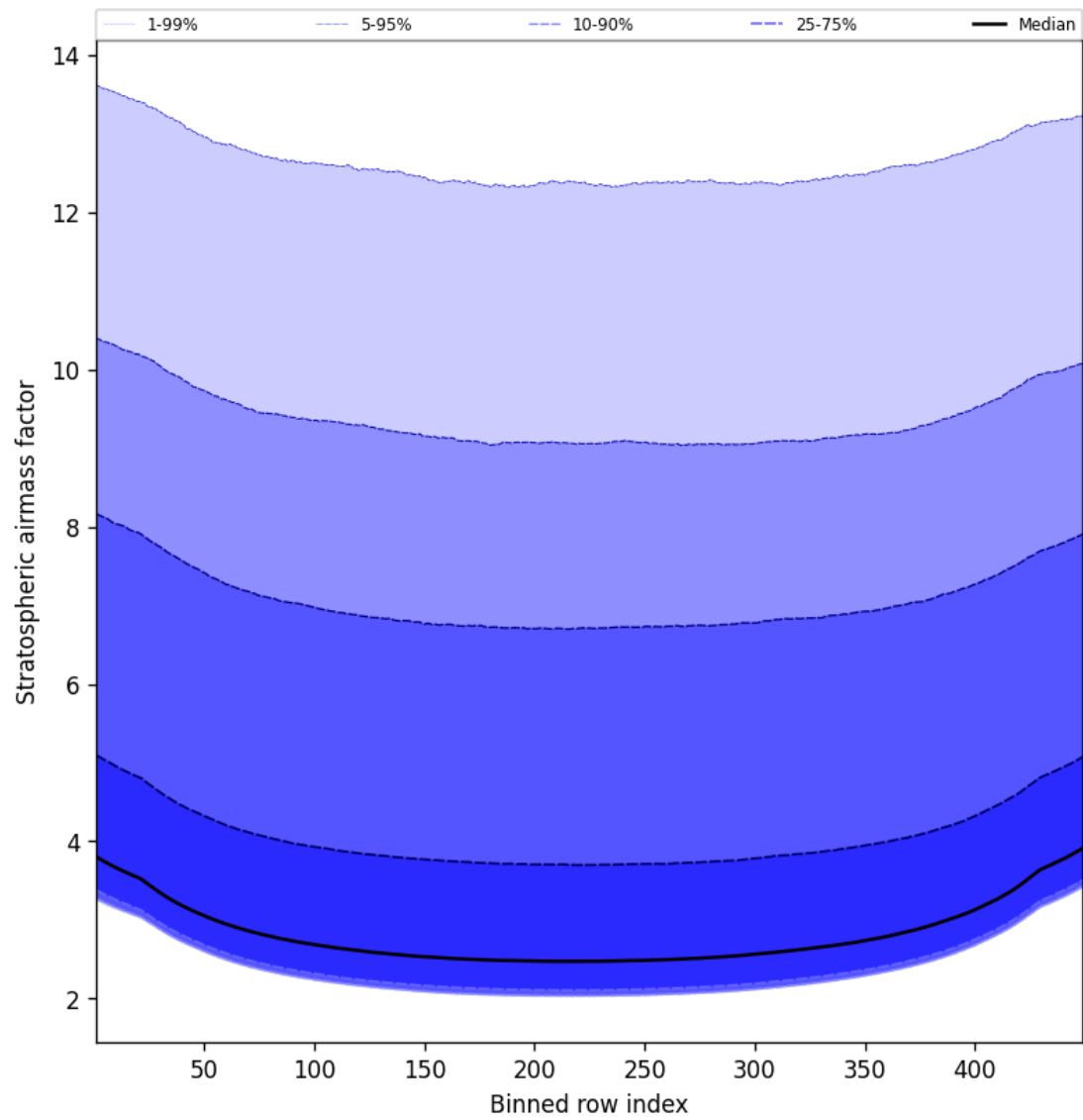
Figure 59: Along track statistics of “Stratospheric airmass factor” for 2025-08-15 to 2025-08-16
