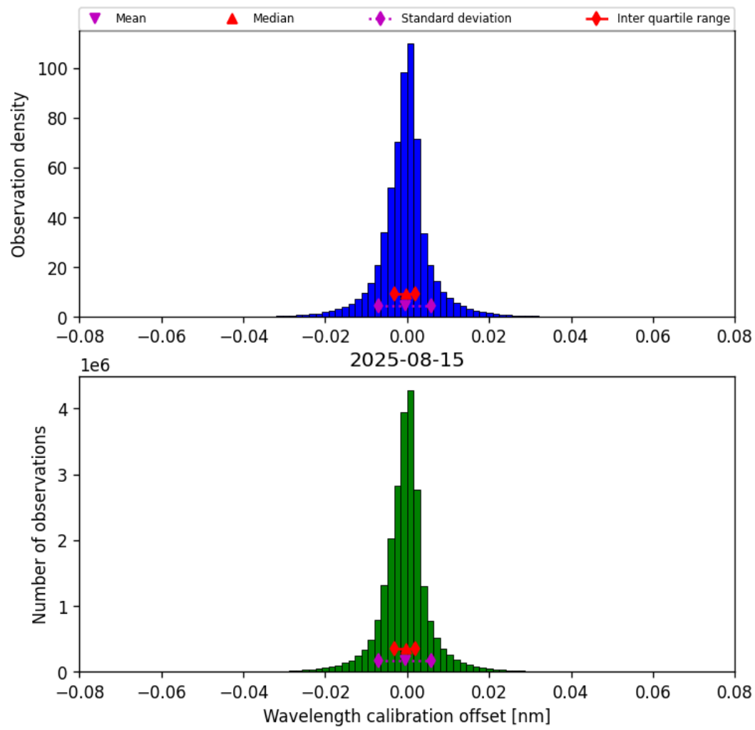
Figure 33: Histogram of “Wavelength calibration offset” for 2025-08-15 to 2025-08-16
