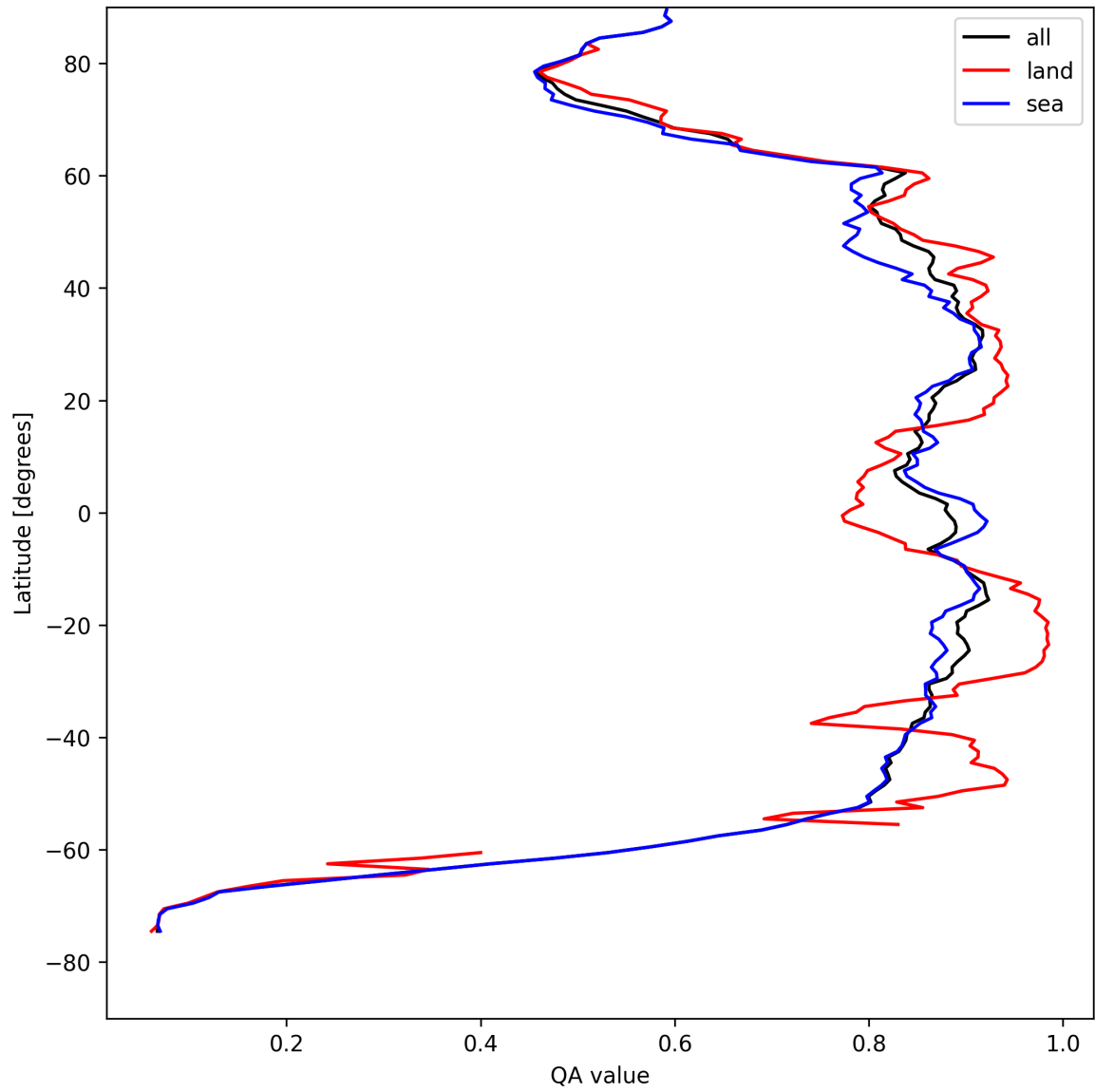
Figure 9: Zonal average of “QA value” for 2025-08-15 to 2025-08-16.
