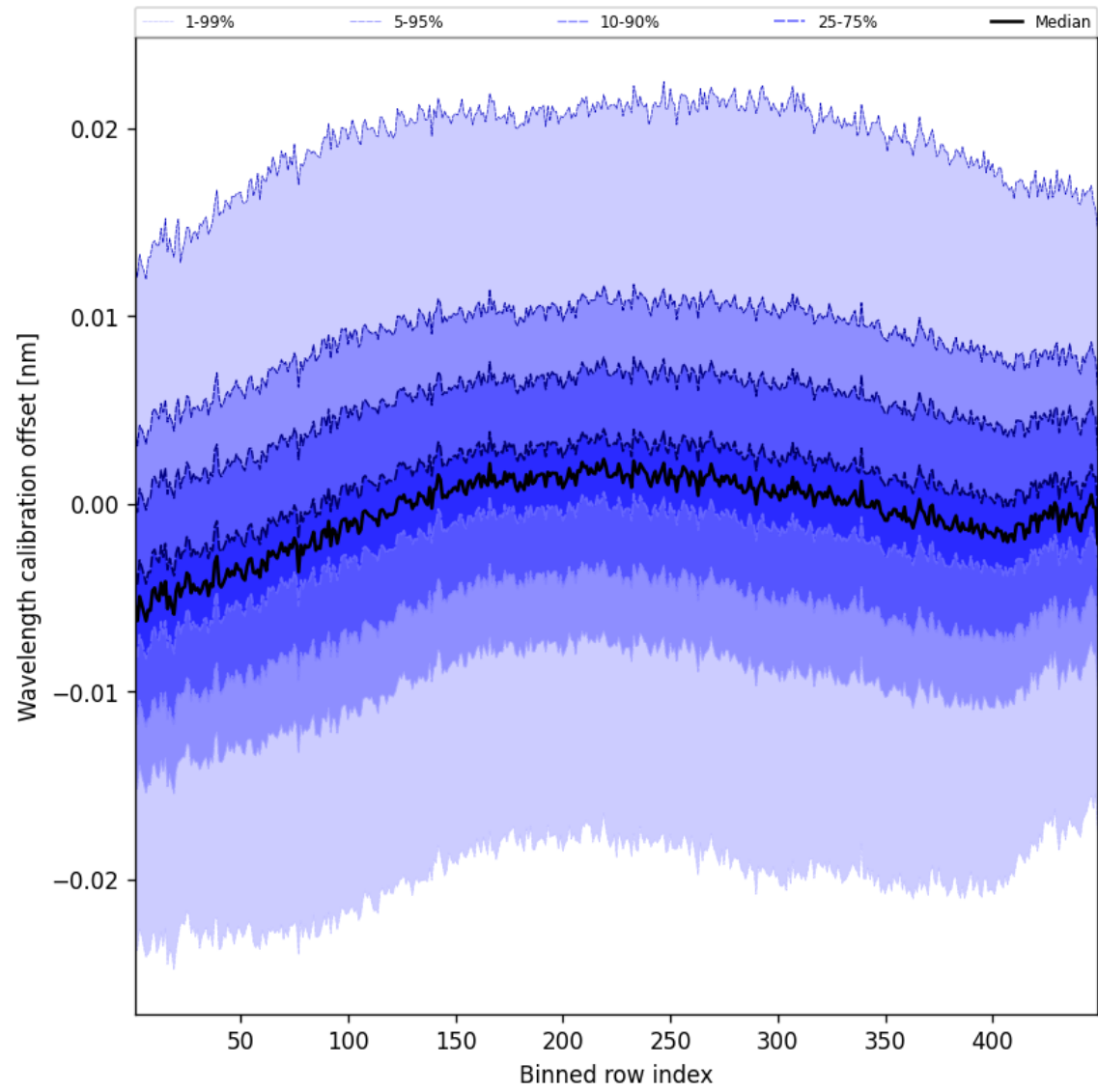
Figure 50: Along track statistics of “Wavelength calibration offset” for 2025-08-15 to 2025-08-16
