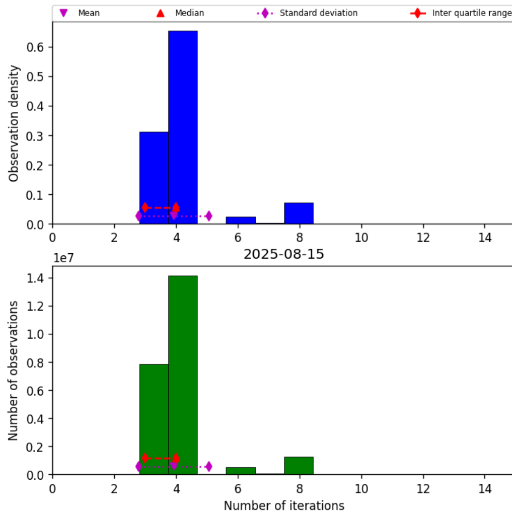
Figure 32: Histogram of “Number of iterations” for 2025-08-15 to 2025-08-16
