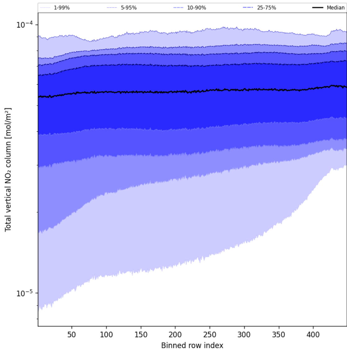
Figure 53: Along track statistics of “Total vertical NO 2 column” for 2025-08-15 to 2025-08-16
