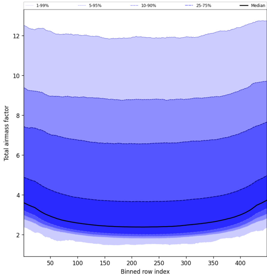
Figure 47: Along track statistics of “Total airmass factor” for 2025-08-15 to 2025-08-16
