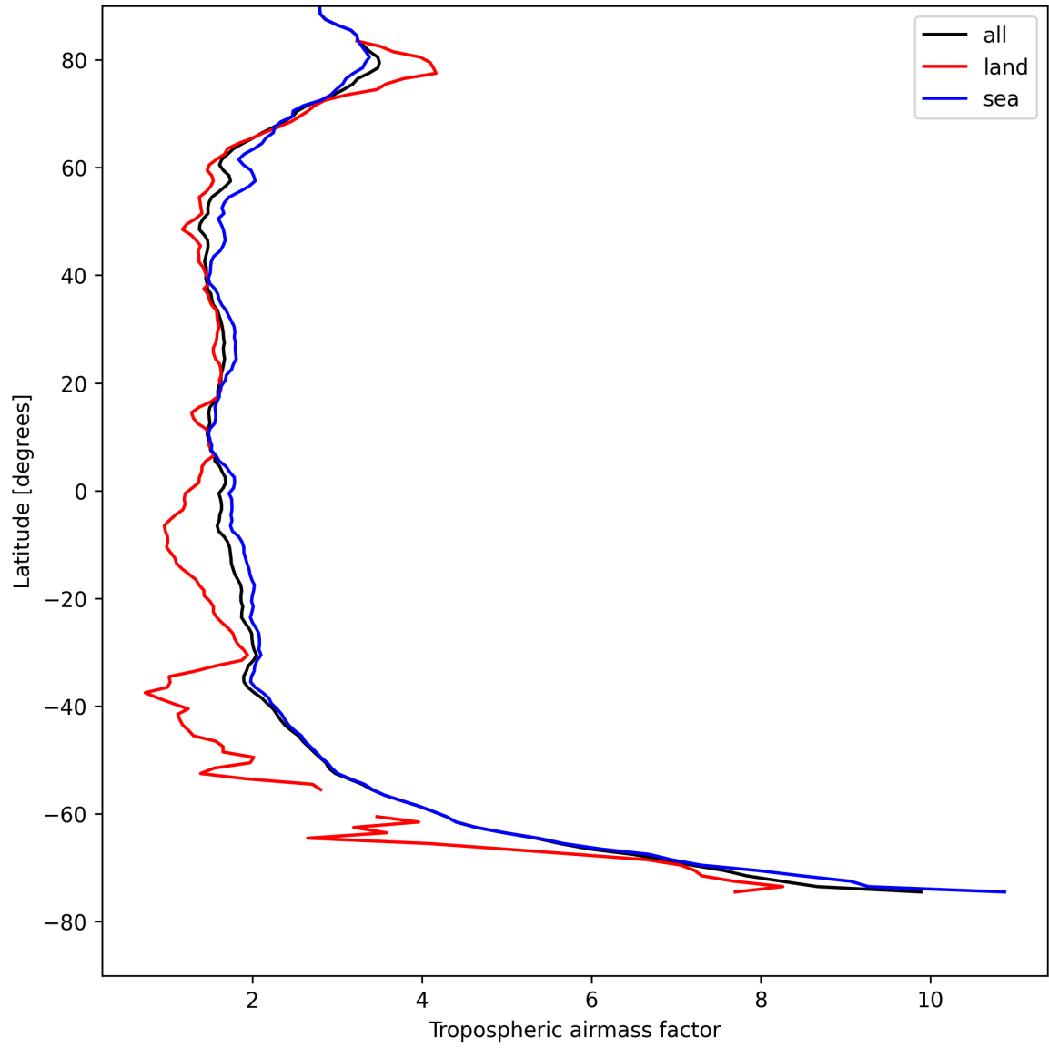
Figure 12: Zonal average of “Tropospheric air mass factor” for 2025-08-15 to 2025-08-16.
