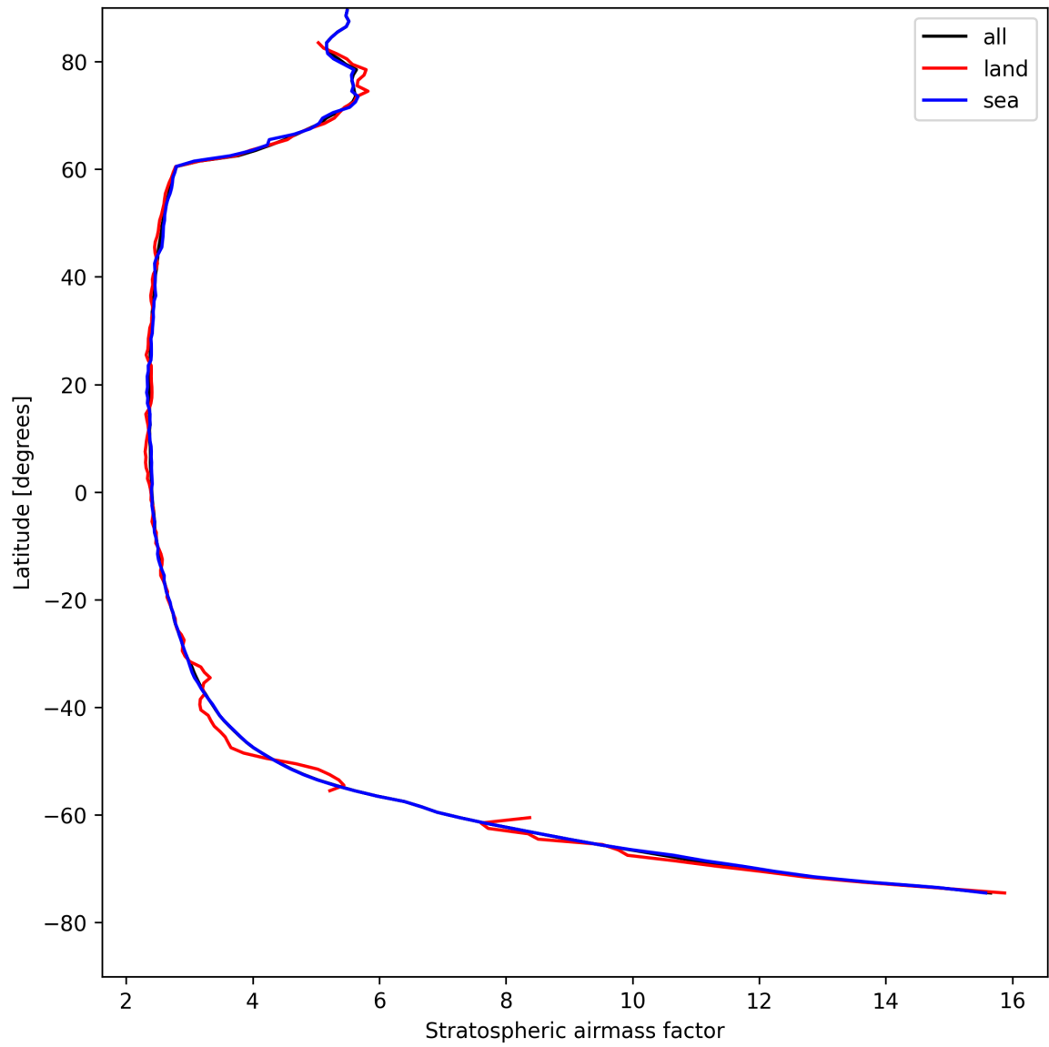
Figure 25: Zonal average of “Stratospheric air mass factor” for 2025-08-15 to 2025-08-16.
