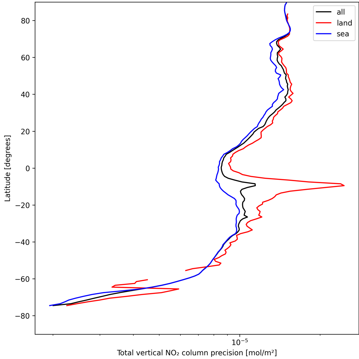
Figure 20: Zonal average of “Total vertical NO 2 column precision” for 2025-08-15 to 2025-08-16.
