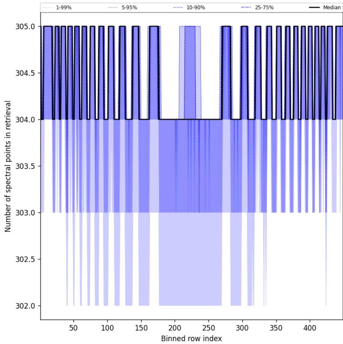
Figure 48: Along track statistics of “Number of spectral points in retrieval” for 2025-08-15 to 2025-08-16
