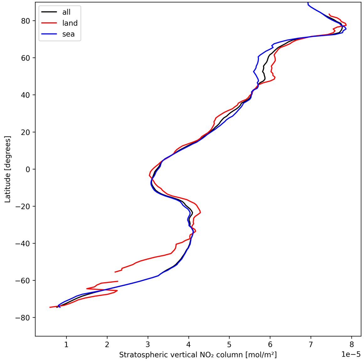
Figure 17: Zonal average of “Stratospheric vertical NO 2 column” for 2025-08-15 to 2025-08-16.
