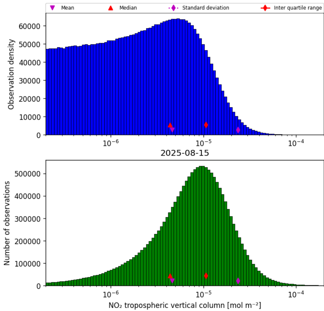
Figure 27: Histogram of “NO 2 tropospheric vertical column” for 2025-08-15 to 2025-08-16
