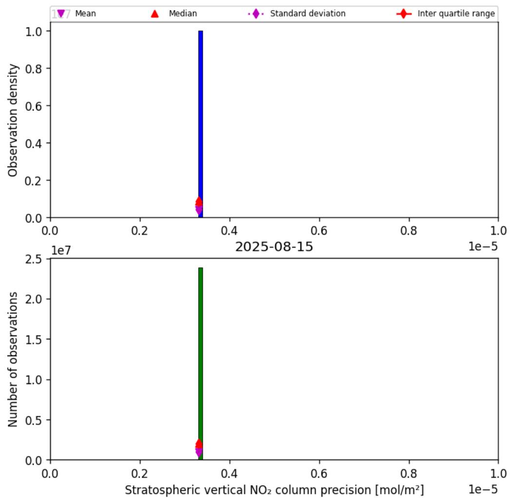
Figure 35: Histogram of “Stratospheric vertical NO 2 column precision” for 2025-08-15 to 2025-08-16
