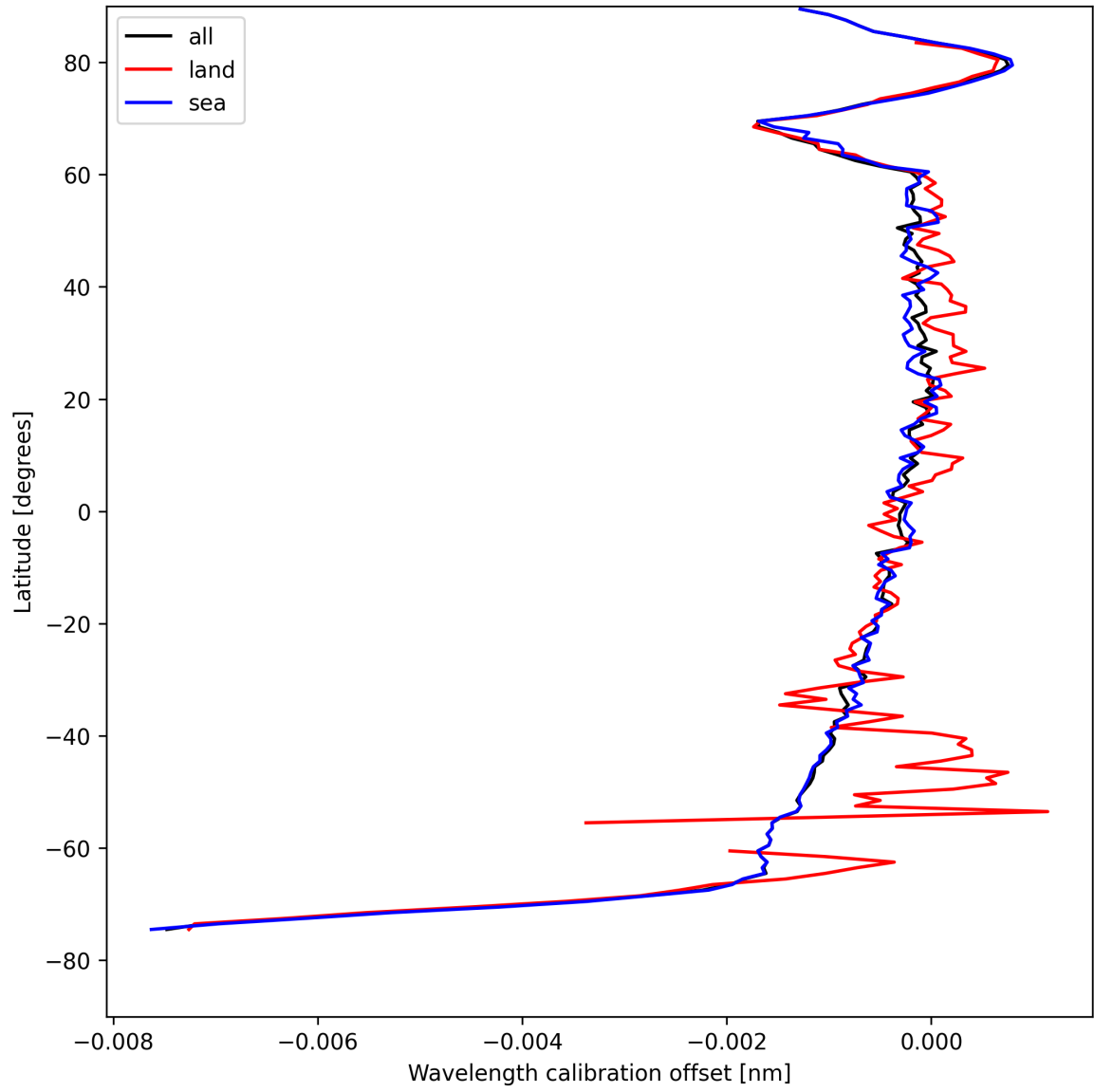
Figure 16: Zonal average of “Wavelength calibration offset” for 2025-08-15 to 2025-08-16.
