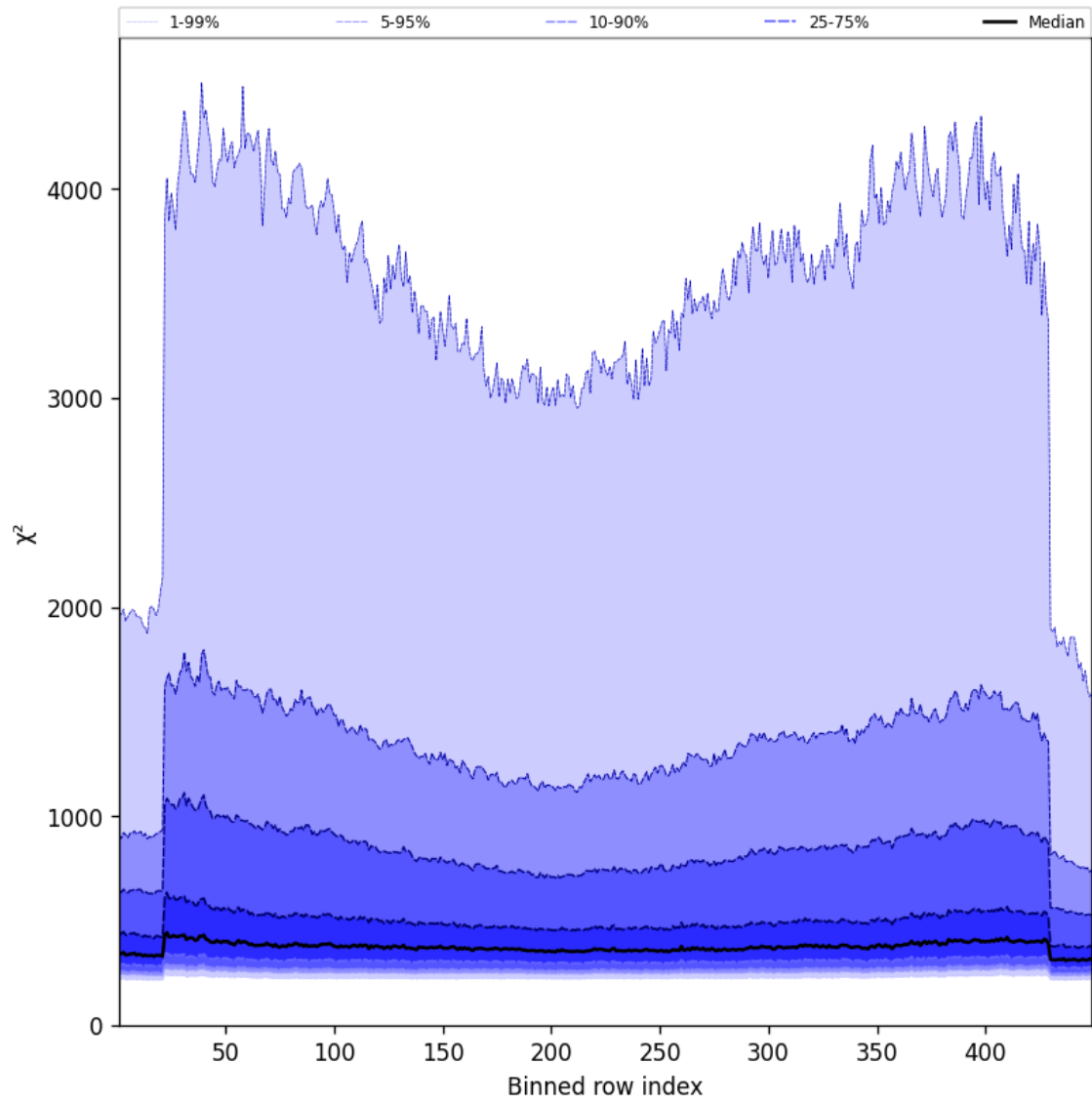
Figure 57: Along track statistics of “ \chi^2 ” for 2025-08-15 to 2025-08-16
