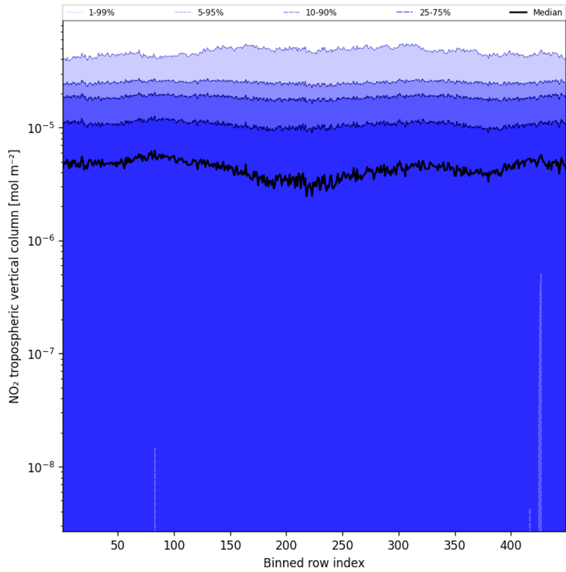
Figure 44: Along track statistics of “NO 2 tropospheric vertical column” for 2025-08-15 to 2025-08-16
