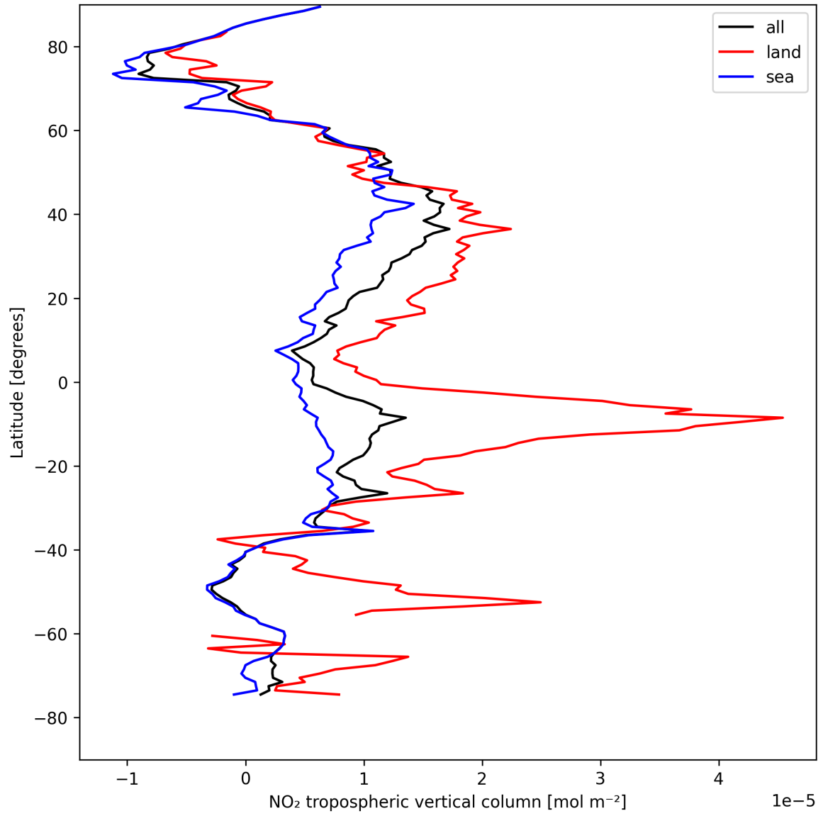
Figure 10: Zonal average of “NO 2 tropospheric vertical column” for 2025-08-15 to 2025-08-16.
