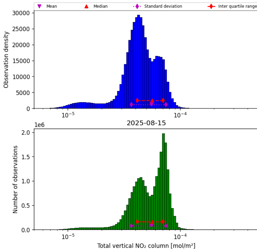
Figure 36: Histogram of “Total vertical NO 2 column” for 2025-08-15 to 2025-08-16
