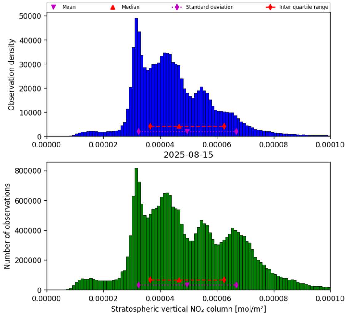
Figure 34: Histogram of “Stratospheric vertical NO 2 column” for 2025-08-15 to 2025-08-16
