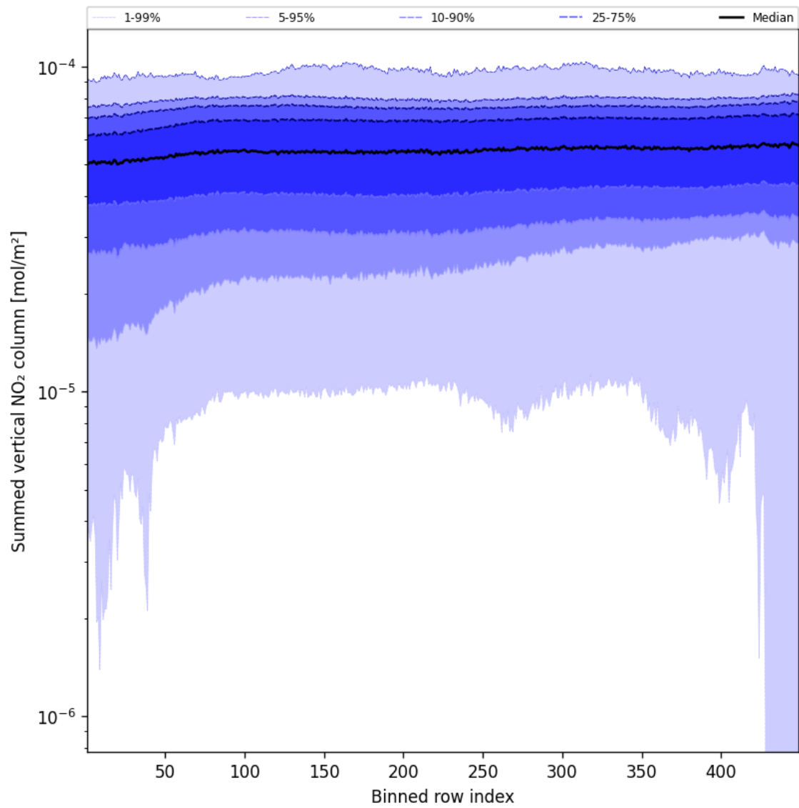
Figure 55: Along track statistics of “Summed vertical NO 2 column” for 2025-08-15 to 2025-08-16
