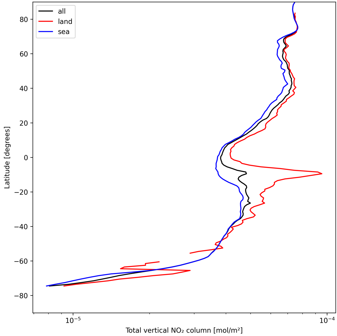
Figure 19: Zonal average of “Total vertical NO 2 column” for 2025-08-15 to 2025-08-16.
