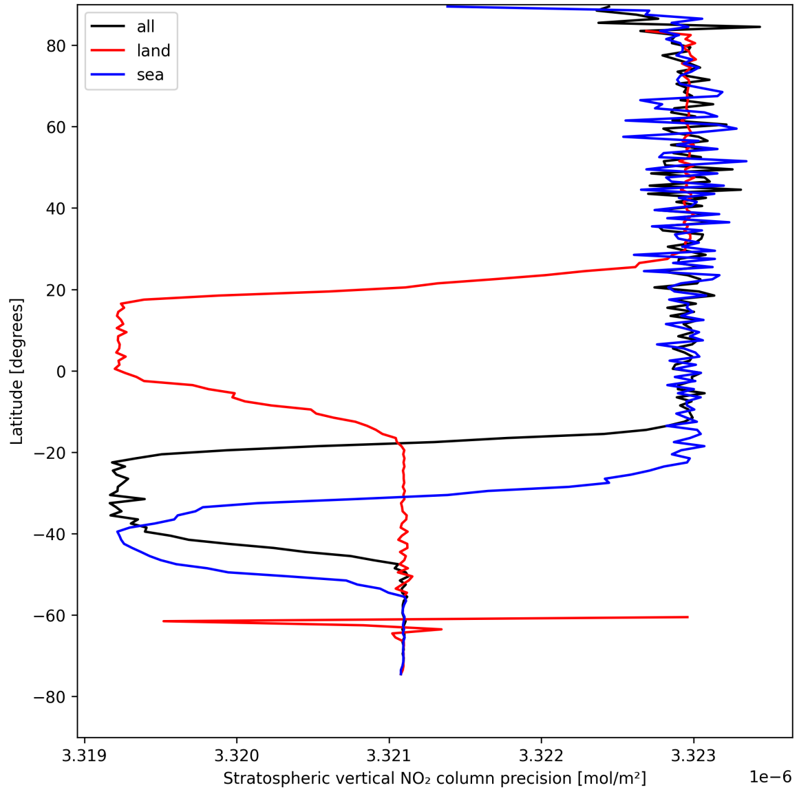
Figure 18: Zonal average of “Stratospheric vertical NO 2 column precision” for 2025-08-15 to 2025-08-16.
