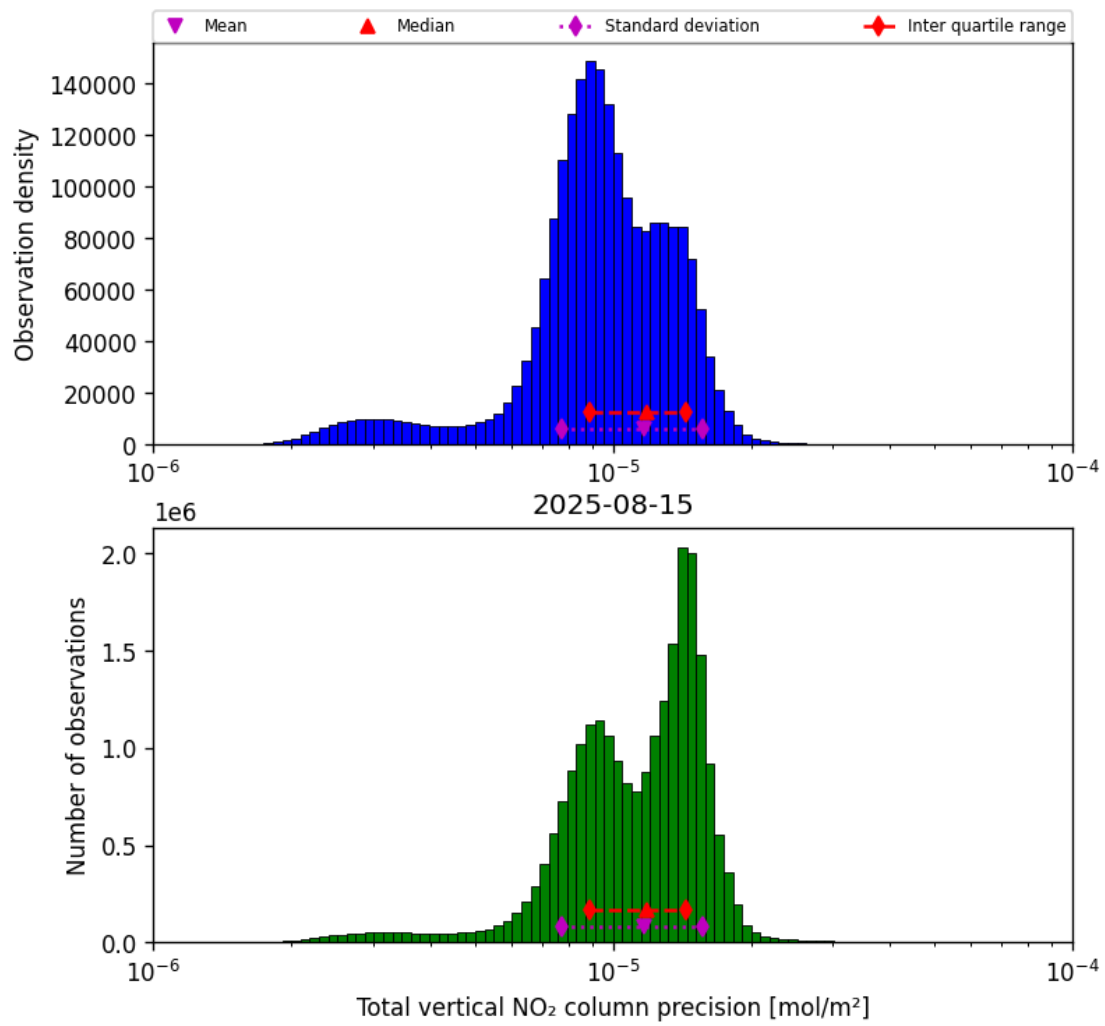
Figure 37: Histogram of “Total vertical NO 2 column precision” for 2025-08-15 to 2025-08-16
