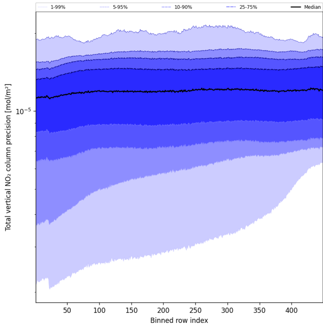
Figure 54: Along track statistics of “Total vertical NO 2 column precision” for 2025-08-15 to 2025-08-16
