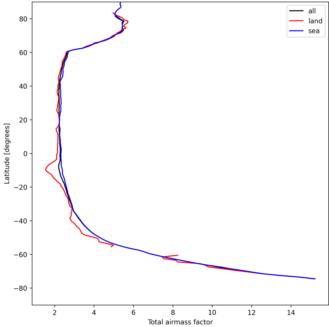
Figure 13: Zonal average of “Total airmass factor” for 2025-08-15 to 2025-08-16.
