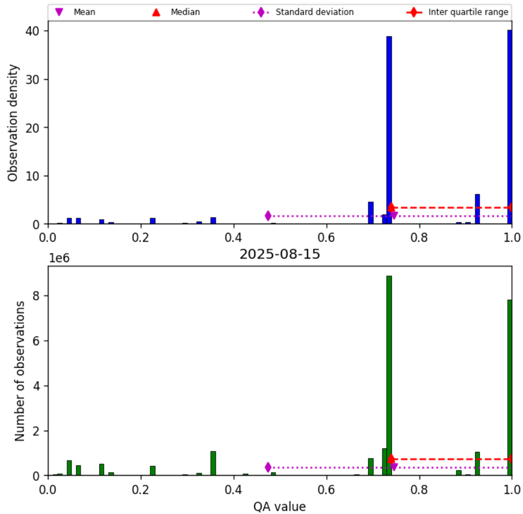
Figure 26: Histogram of “QA value” for 2025-08-15 to 2025-08-16
