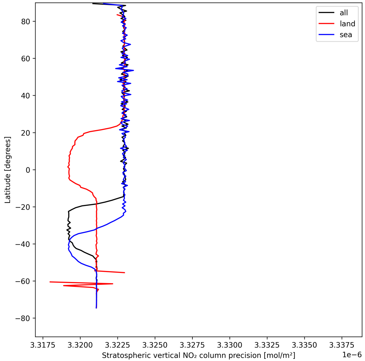
Figure 18: Zonal average of “Stratospheric vertical NO 2 column precision” for 2025-08-17 to 2025-08-17.
