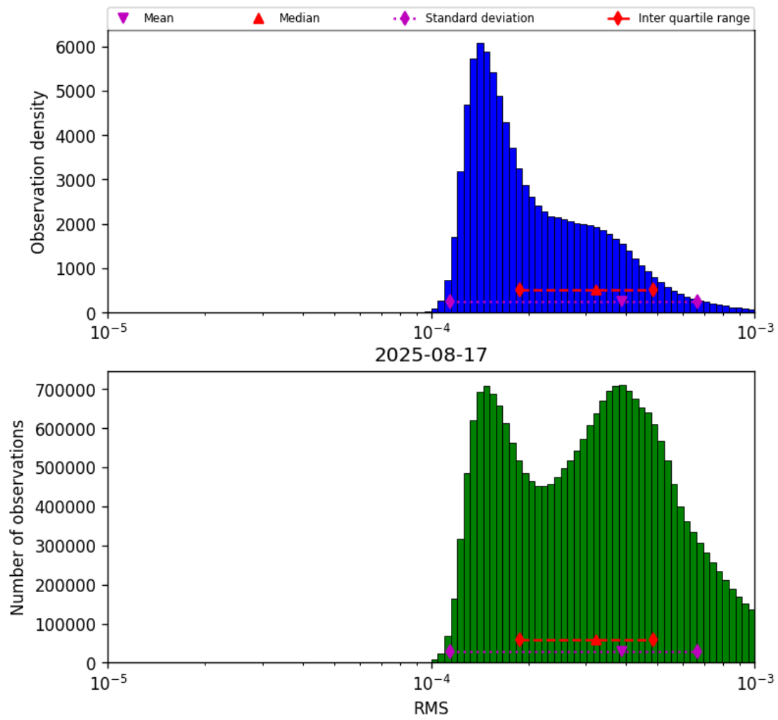
Figure 41: Histogram of “RMS” for 2025-08-17 to 2025-08-17
