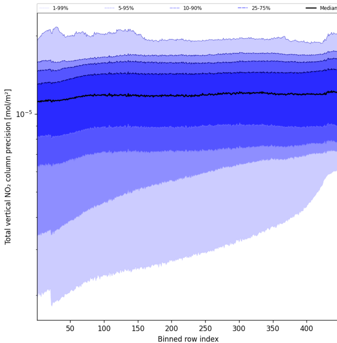
Figure 54: Along track statistics of “Total vertical NO 2 column precision” for 2025-08-17 to 2025-08-17
