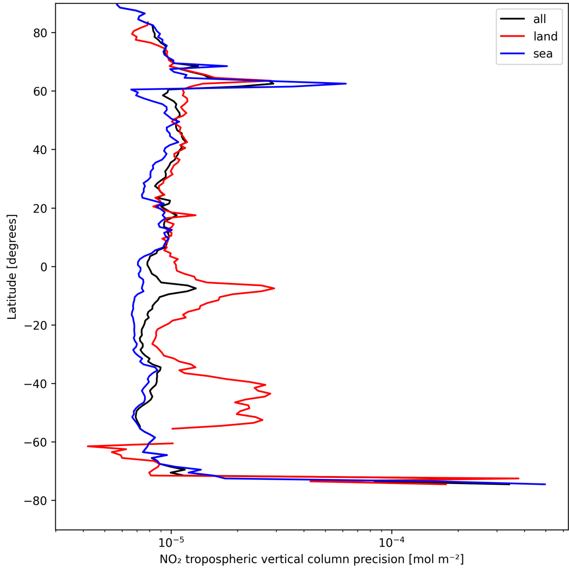
Figure 11: Zonal average of "NO 2 tropospheric vertical column precision" for 2025-08-17 to 2025-08-17.
