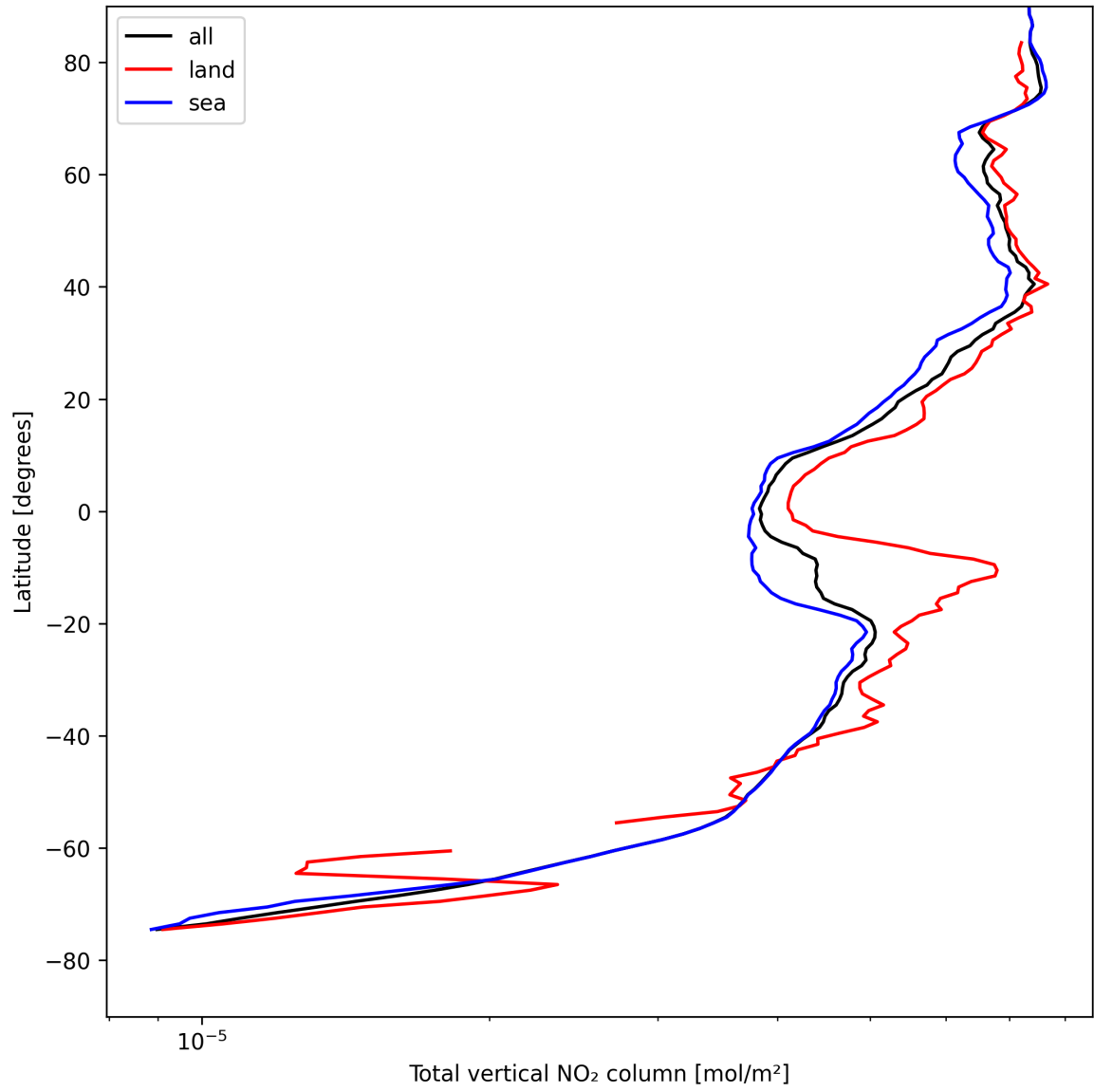
Figure 19: Zonal average of “Total vertical NO 2 column” for 2025-08-17 to 2025-08-17.
