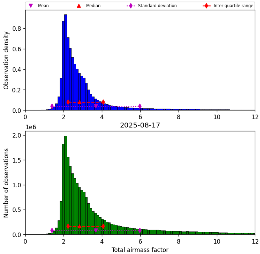
Figure 30: Histogram of “Total airmass factor” for 2025-08-17 to 2025-08-17
