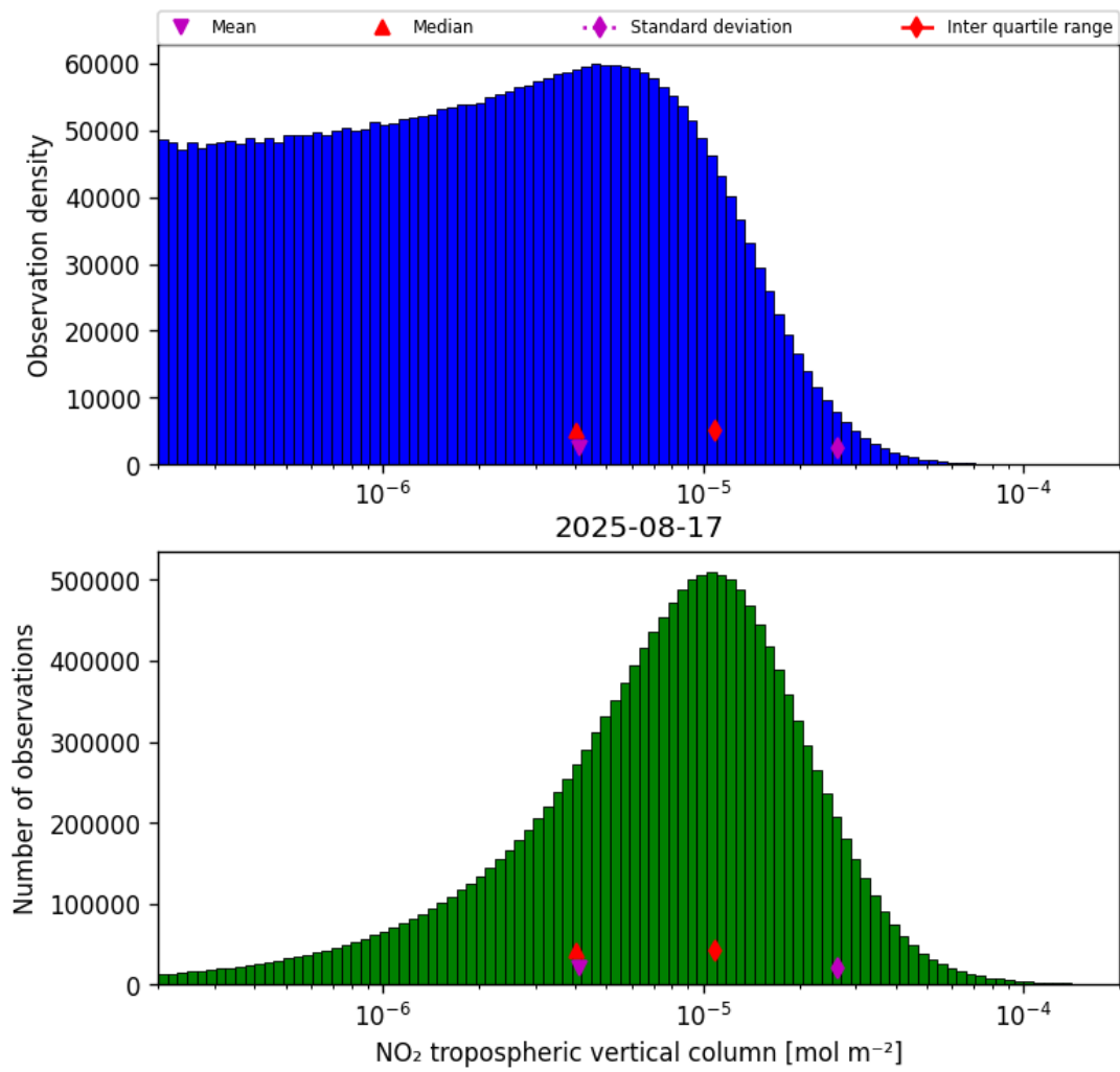
Figure 27: Histogram of “NO 2 tropospheric vertical column” for 2025-08-17 to 2025-08-17
