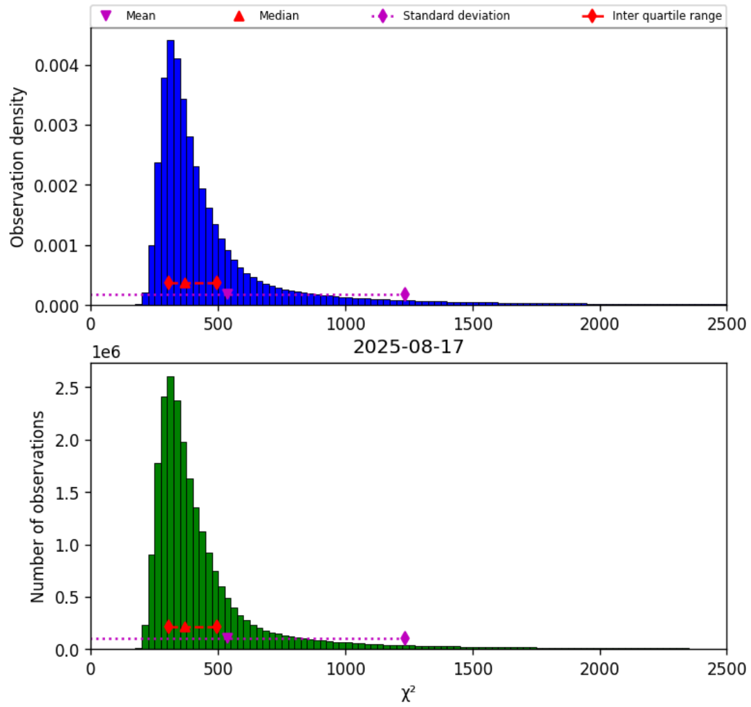
Figure 40: Histogram of “ \chi^2 ” for 2025-08-17 to 2025-08-17
