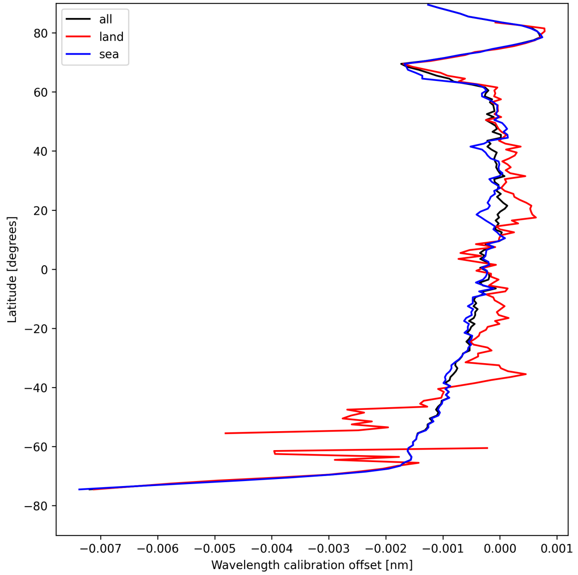
Figure 16: Zonal average of “Wavelength calibration offset” for 2025-08-17 to 2025-08-17.
