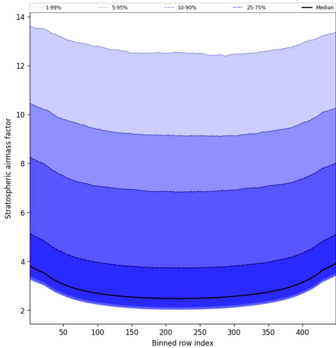
Figure 59: Along track statistics of “Stratospheric airmass factor” for 2025-08-17 to 2025-08-17
