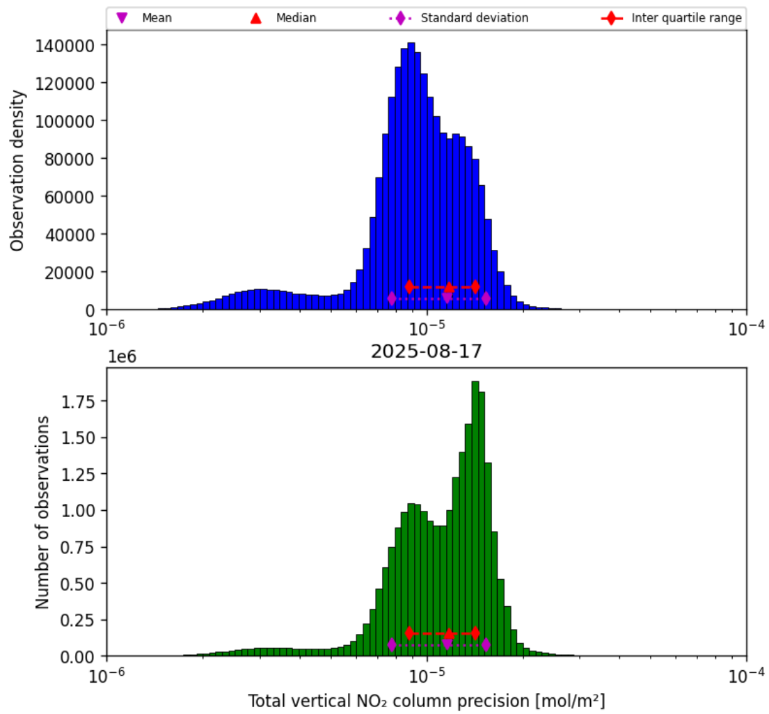
Figure 37: Histogram of “Total vertical NO 2 column precision” for 2025-08-17 to 2025-08-17
