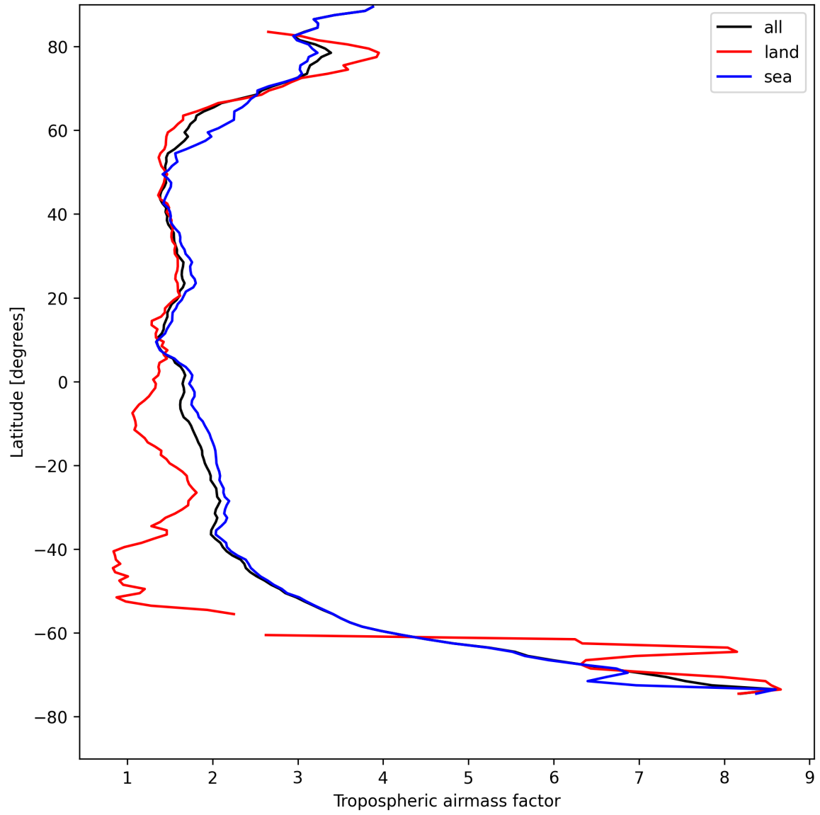
Figure 12: Zonal average of “Tropospheric airmass factor” for 2025-08-17 to 2025-08-17.
