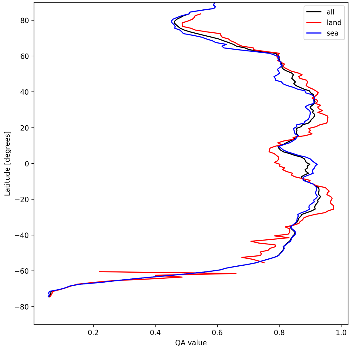
Figure 9: Zonal average of “QA value” for 2025-08-17 to 2025-08-17.
