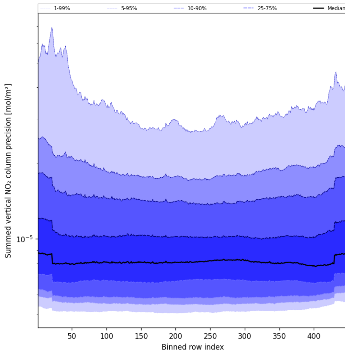
Figure 56: Along track statistics of “Summed vertical NO 2 column precision” for 2025-08-17 to 2025-08-17
