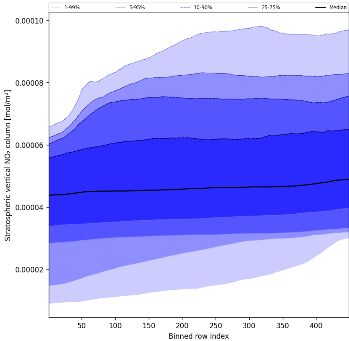
Figure 51: Along track statistics of “Stratospheric vertical NO 2 column” for 2025-08-17 to 2025-08-17
