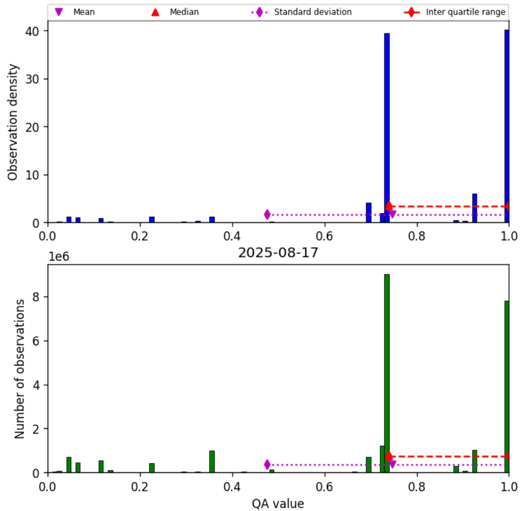
Figure 26: Histogram of “QA value” for 2025-08-17 to 2025-08-17
