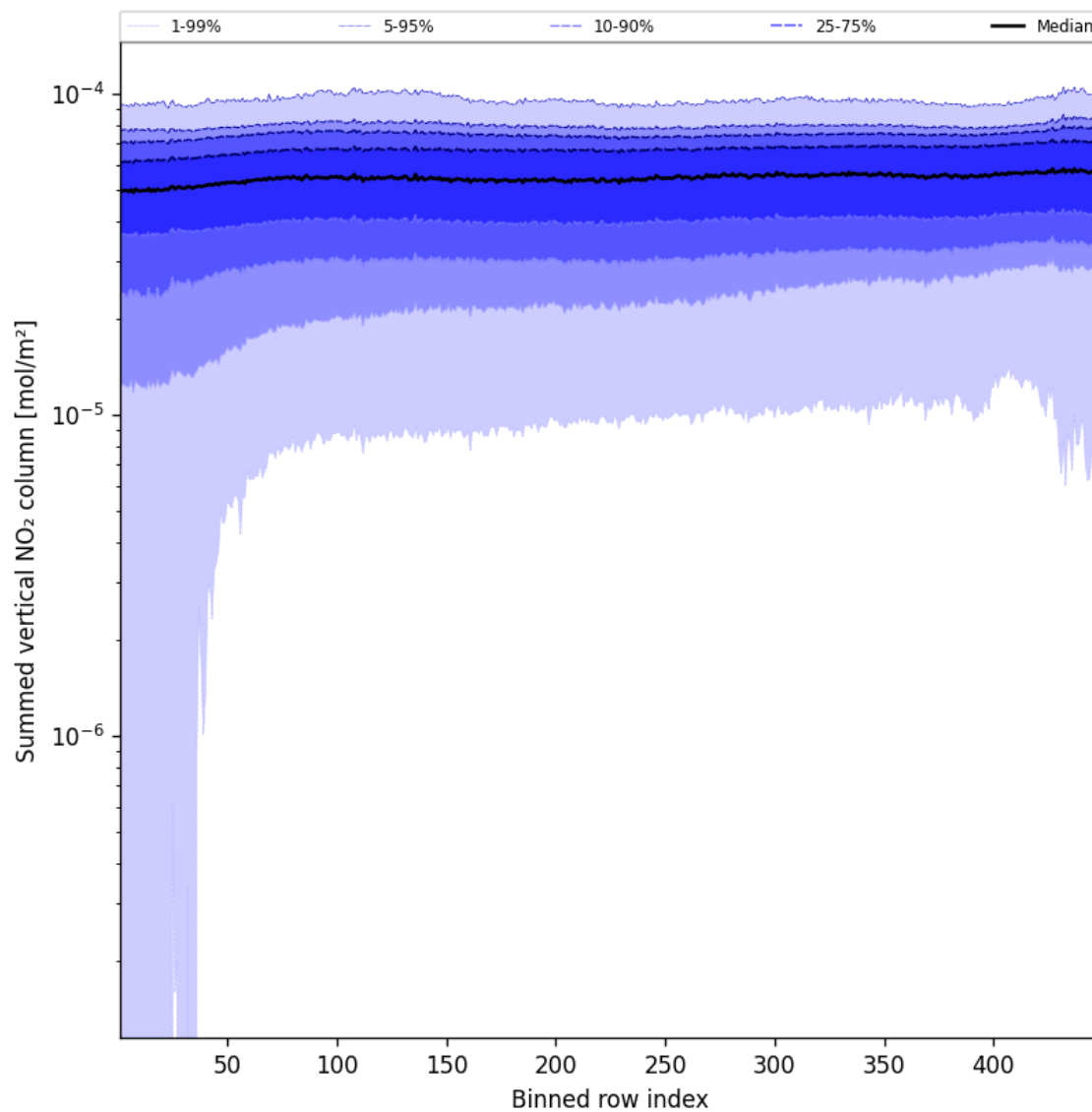
Figure 55: Along track statistics of “Summed vertical NO 2 column” for 2025-08-17 to 2025-08-17
