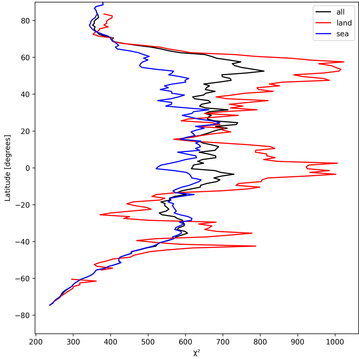
Figure 23: Zonal average of “ \chi^2 ” for 2025-08-17 to 2025-08-17.
