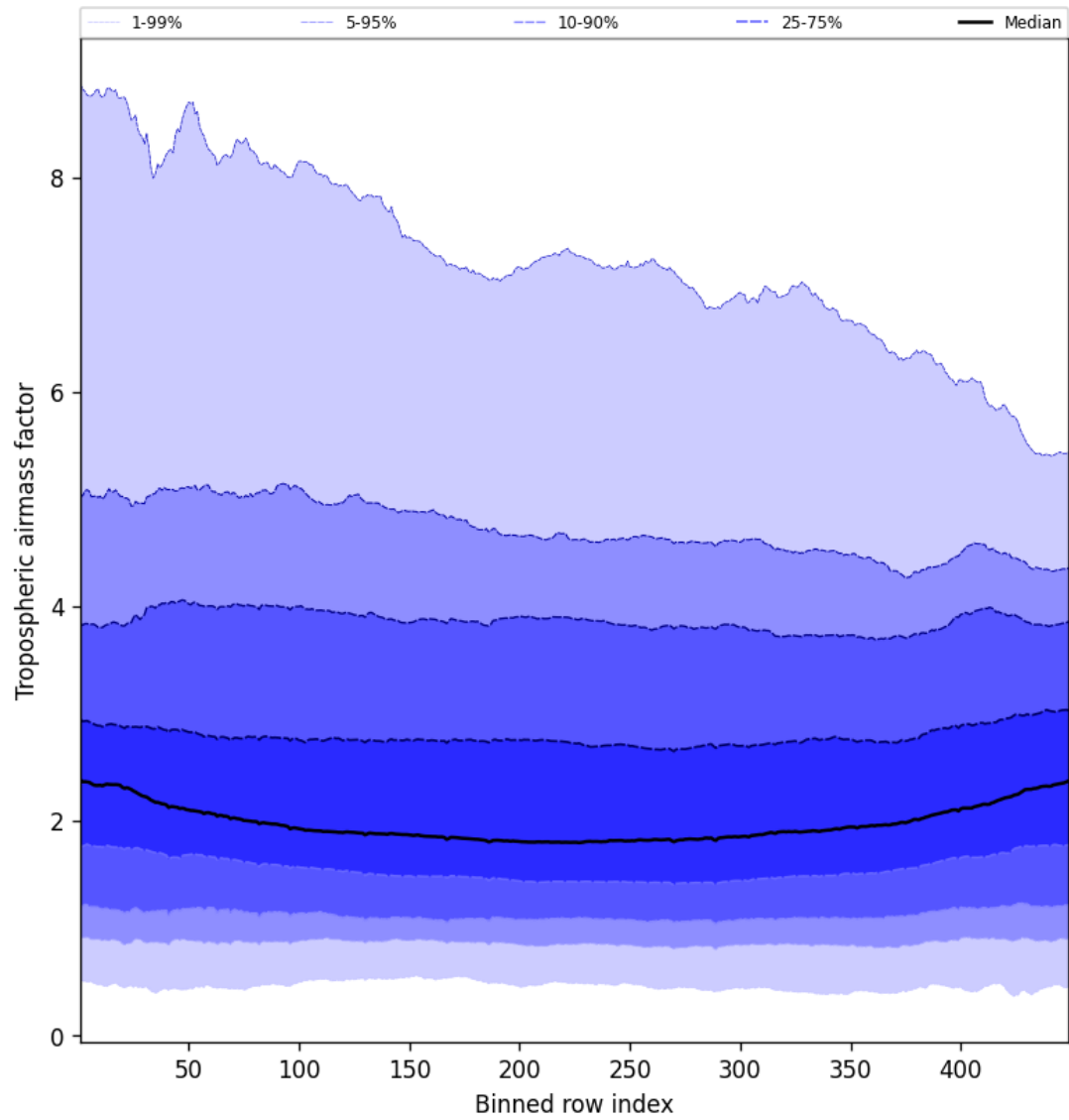
Figure 46: Along track statistics of “Tropospheric air mass factor” for 2025-08-17 to 2025-08-17
