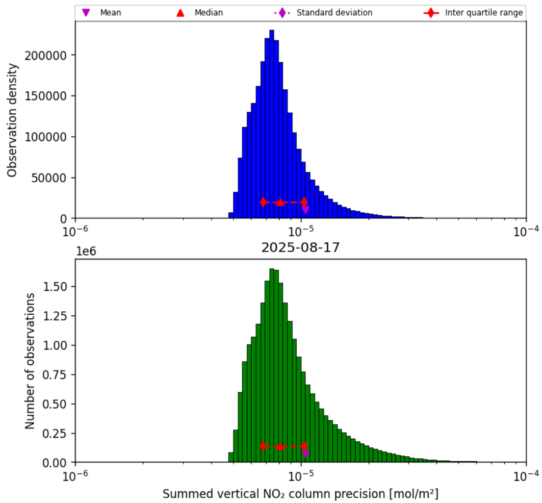
Figure 39: Histogram of "Summed vertical NO 2 column precision" for 2025-08-17 to 2025-08-17
