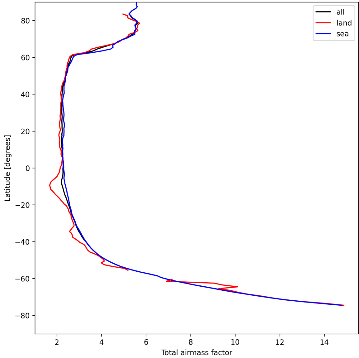
Figure 13: Zonal average of “Total airmass factor” for 2025-08-17 to 2025-08-17.
