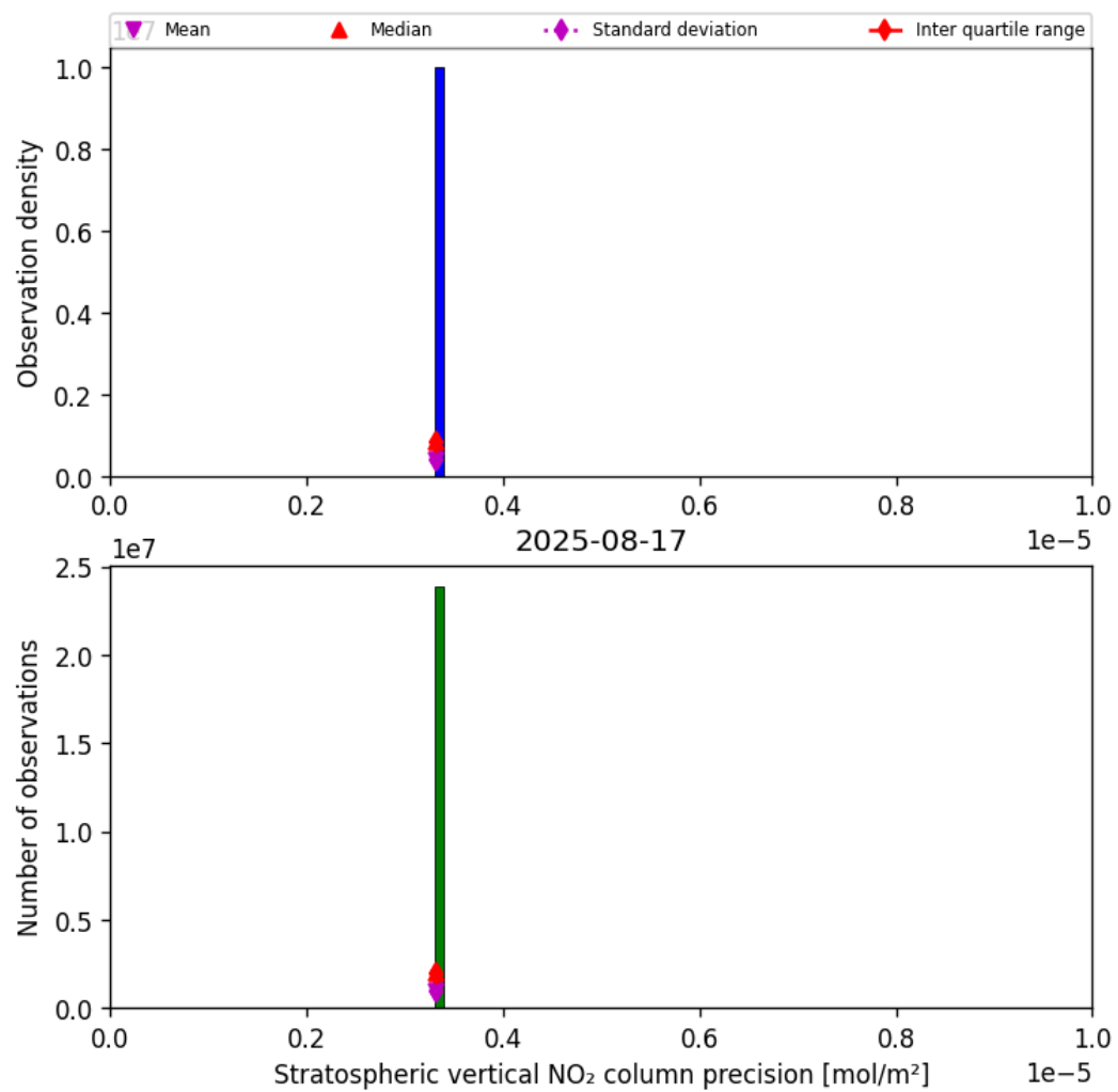
Figure 35: Histogram of “Stratospheric vertical NO 2 column precision” for 2025-08-17 to 2025-08-17
