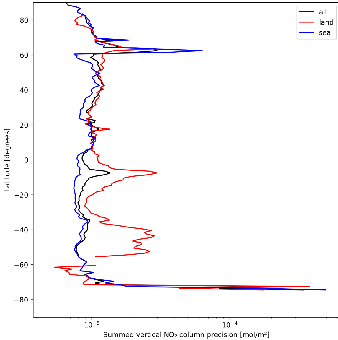
Figure 22: Zonal average of "Summed vertical NO 2 column precision" for 2025-08-17 to 2025-08-17.
