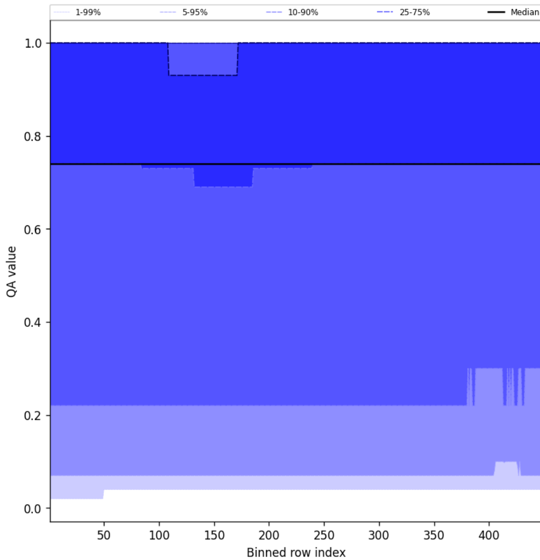
Figure 43: Along track statistics of “QA value” for 2025-08-17 to 2025-08-17
