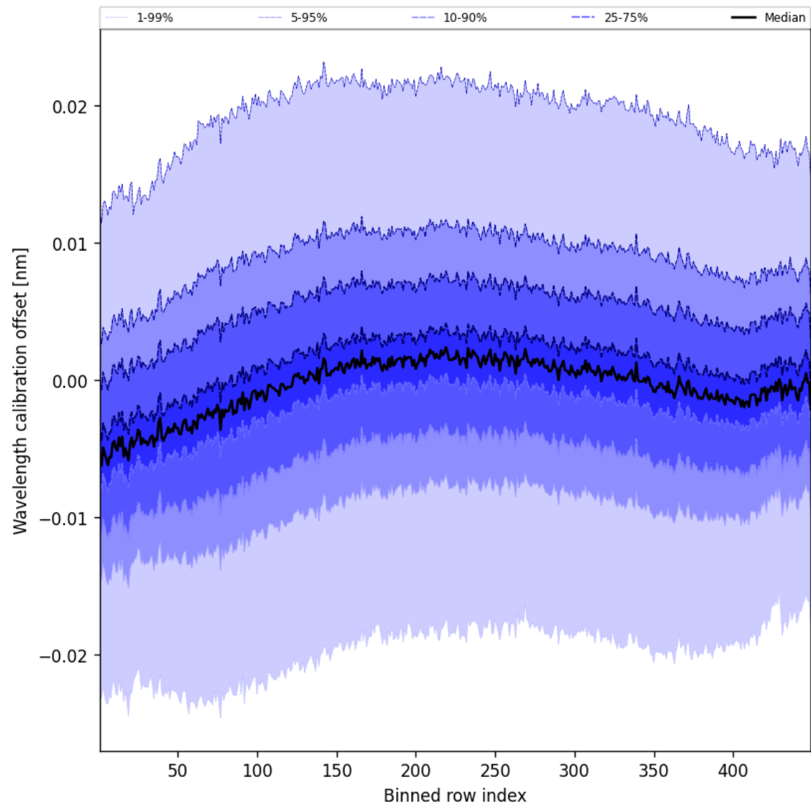
Figure 50: Along track statistics of “Wavelength calibration offset” for 2025-08-17 to 2025-08-17
