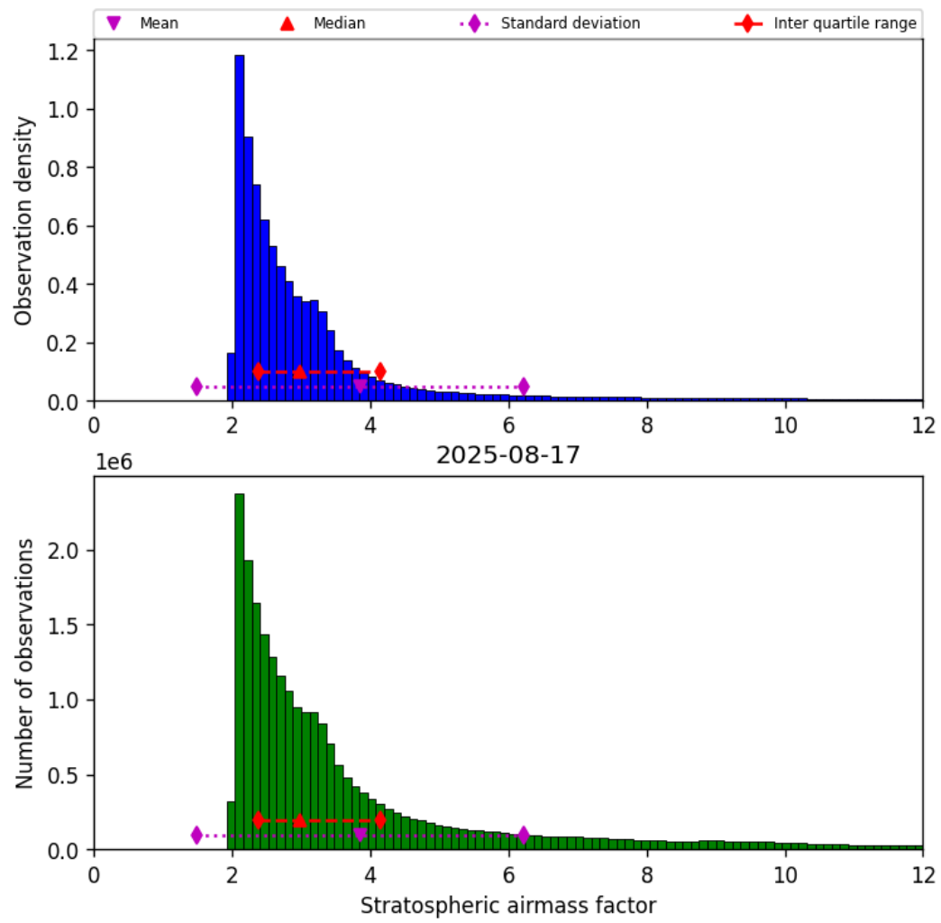
Figure 42: Histogram of “Stratospheric airmass factor” for 2025-08-17 to 2025-08-17
