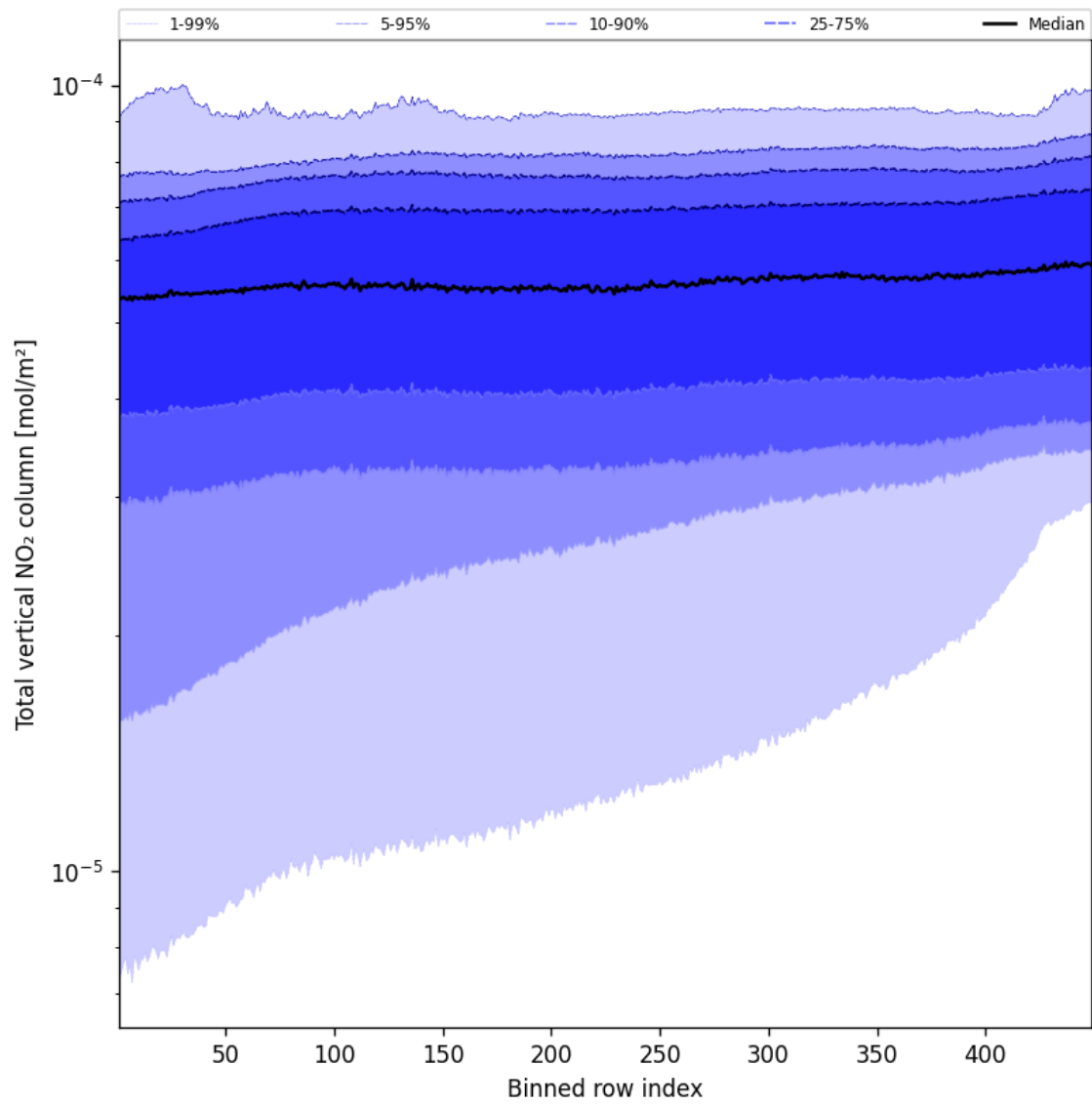
Figure 53: Along track statistics of “Total vertical NO 2 column” for 2025-08-17 to 2025-08-17
