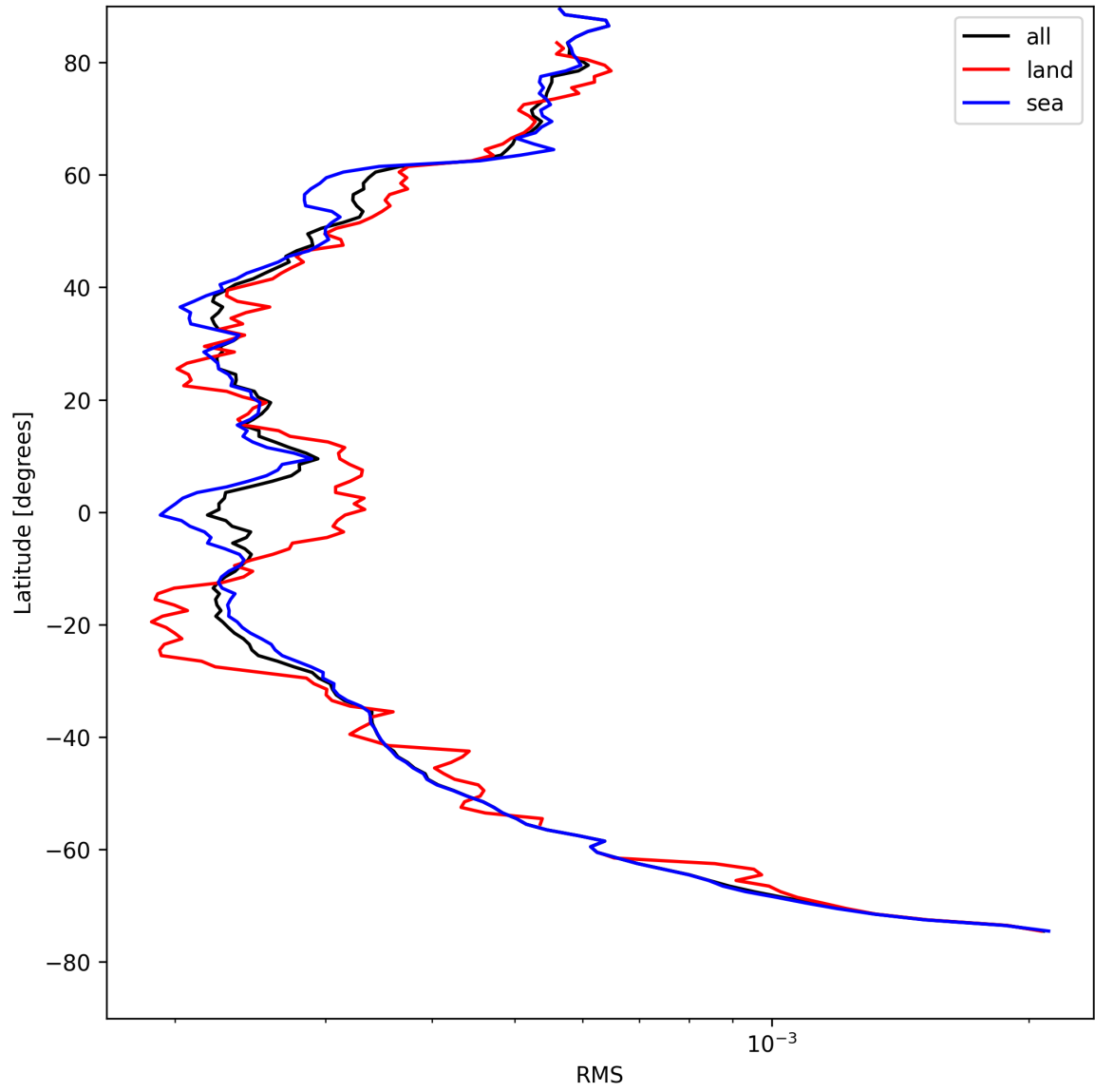
Figure 24: Zonal average of “RMS” for 2025-08-17 to 2025-08-17.
