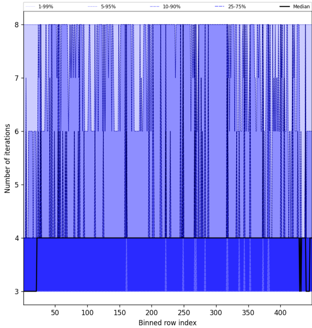
Figure 49: Along track statistics of "Number of iterations" for 2025-08-17 to 2025-08-17
