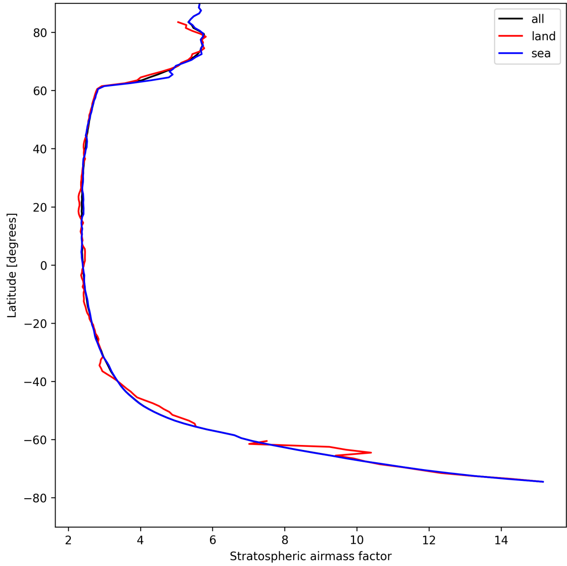
Figure 25: Zonal average of “Stratospheric airmass factor” for 2025-08-17 to 2025-08-17.
