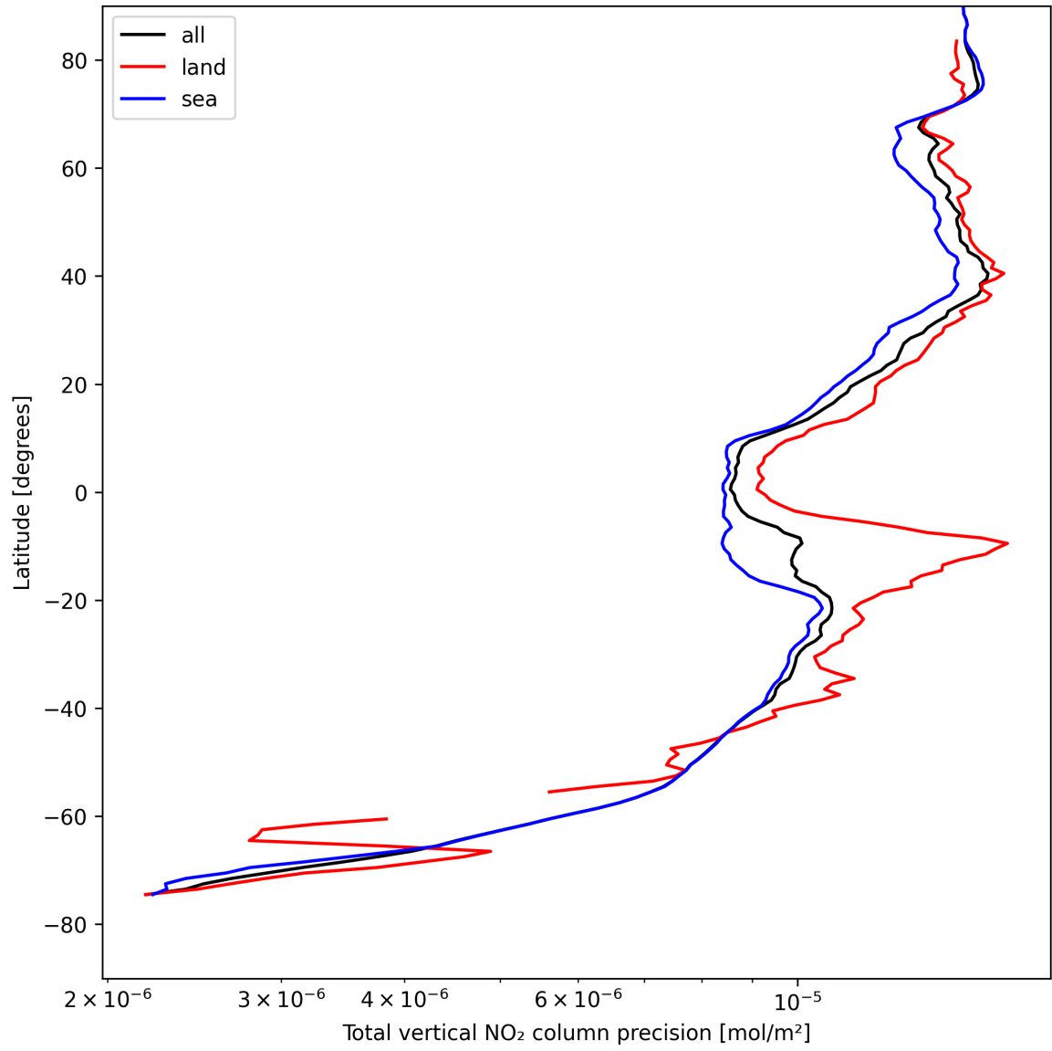
Figure 20: Zonal average of “Total vertical NO 2 column precision” for 2025-08-17 to 2025-08-17.
