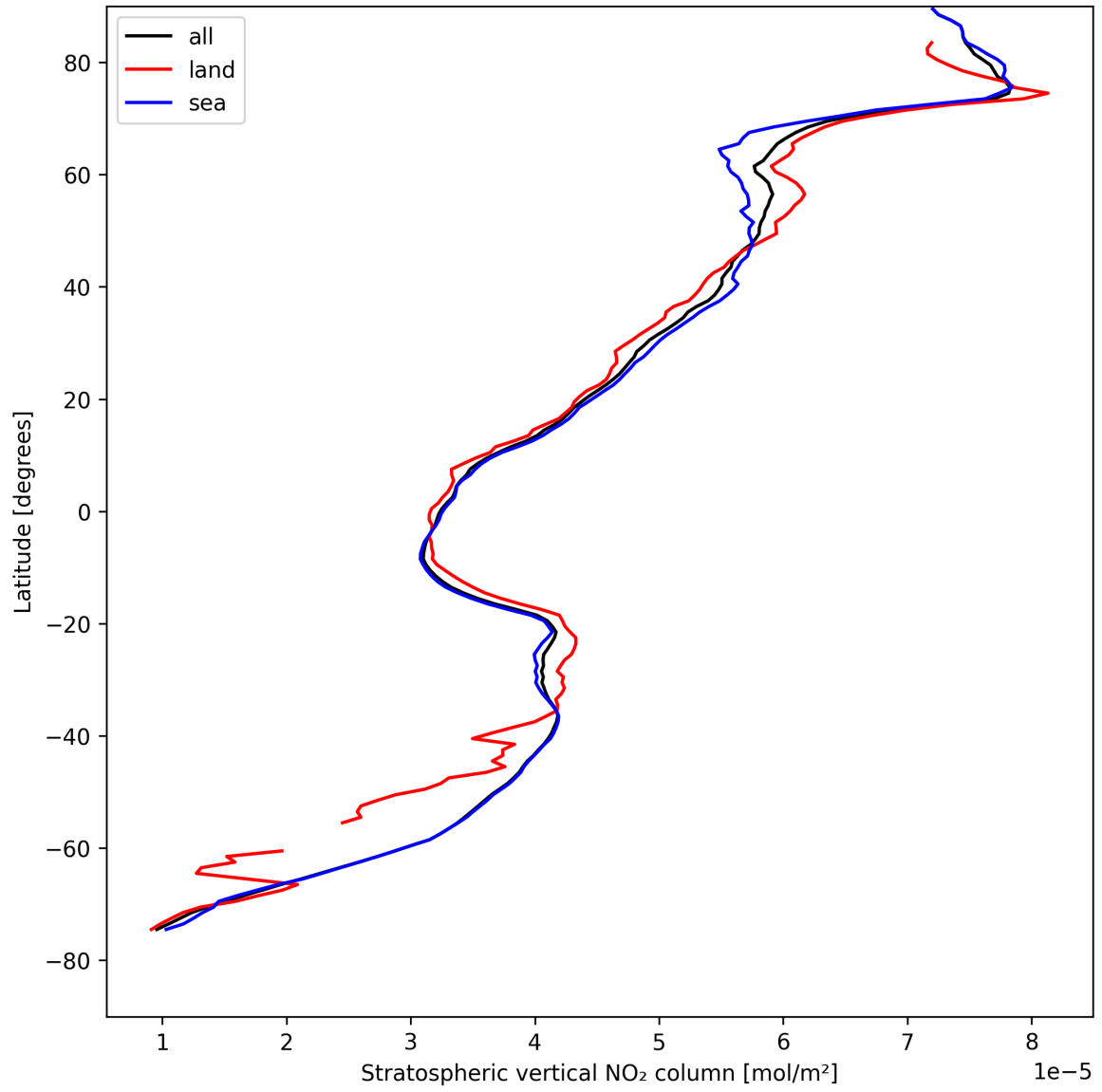
Figure 17: Zonal average of “Stratospheric vertical NO 2 column” for 2025-08-17 to 2025-08-17.
