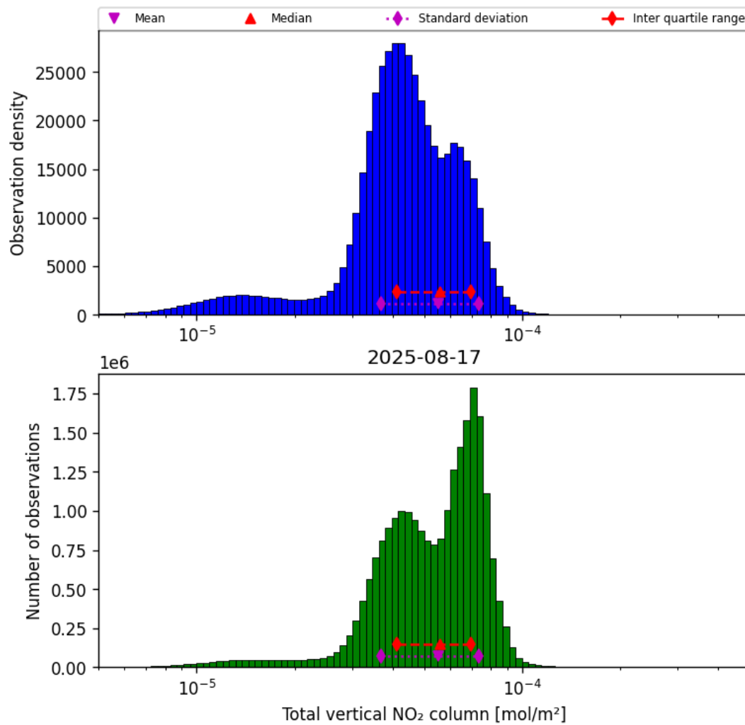
Figure 36: Histogram of “Total vertical NO 2 column” for 2025-08-17 to 2025-08-17
