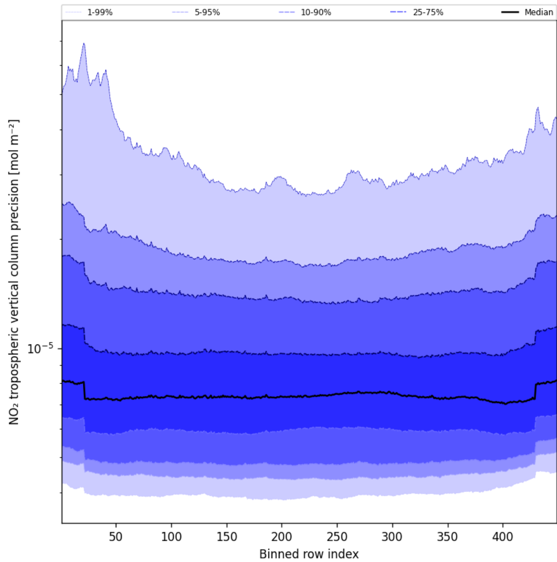
Figure 45: Along track statistics of “NO 2 tropospheric vertical column precision” for 2025-08-17 to 2025-08-17
