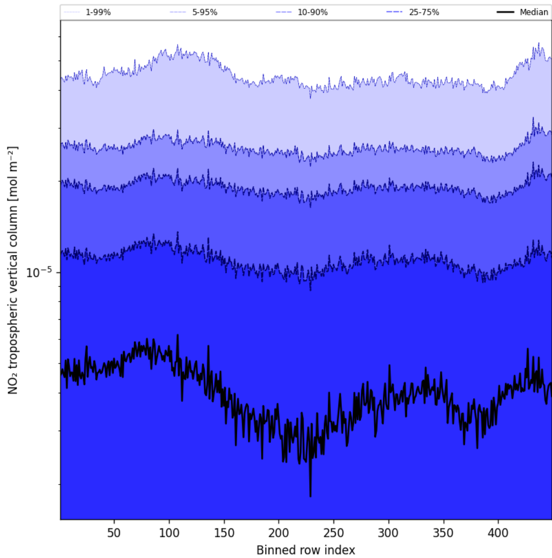
Figure 44: Along track statistics of “NO 2 tropospheric vertical column” for 2025-08-17 to 2025-08-17
