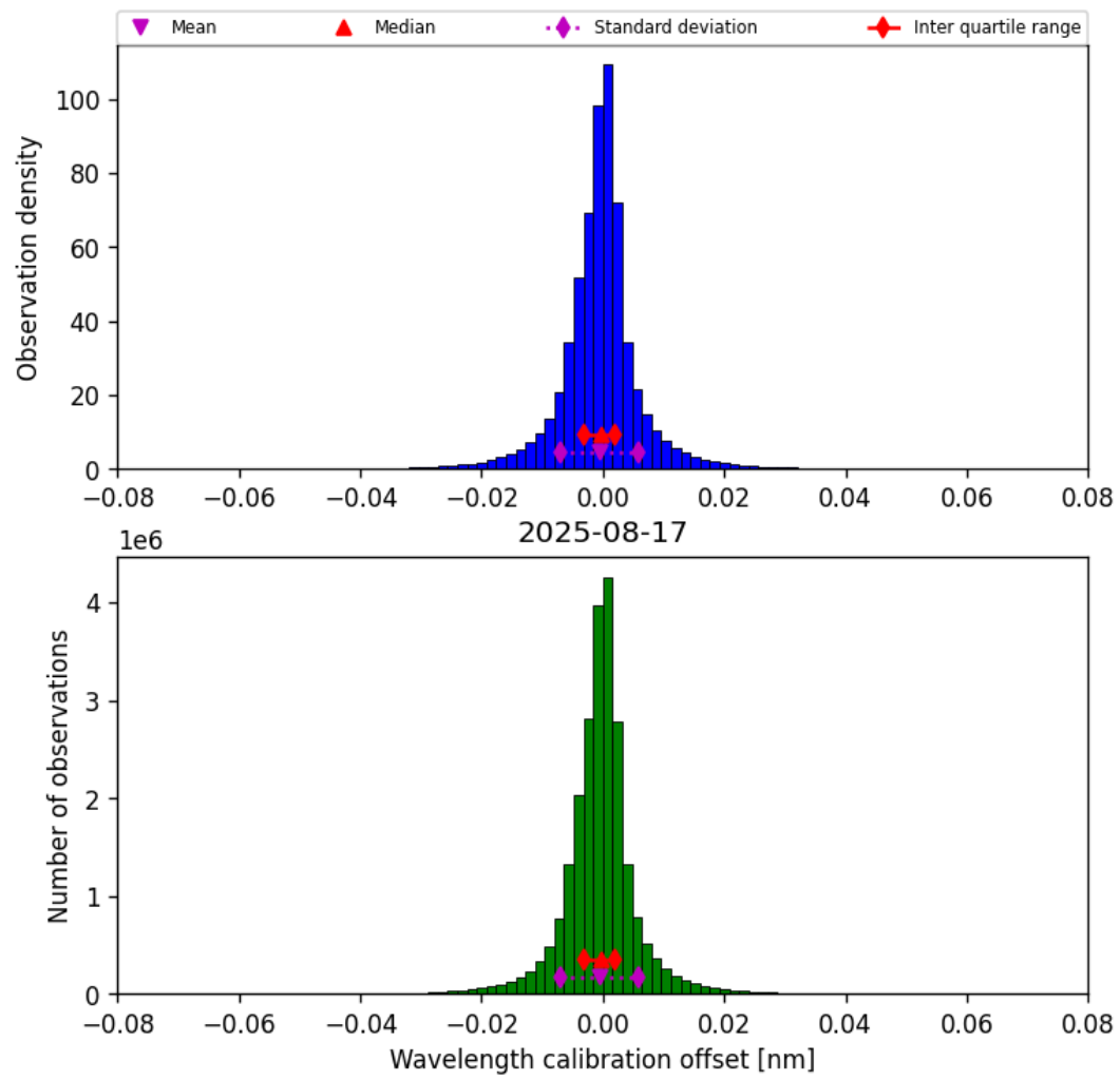
Figure 33: Histogram of “Wavelength calibration offset” for 2025-08-17 to 2025-08-17
