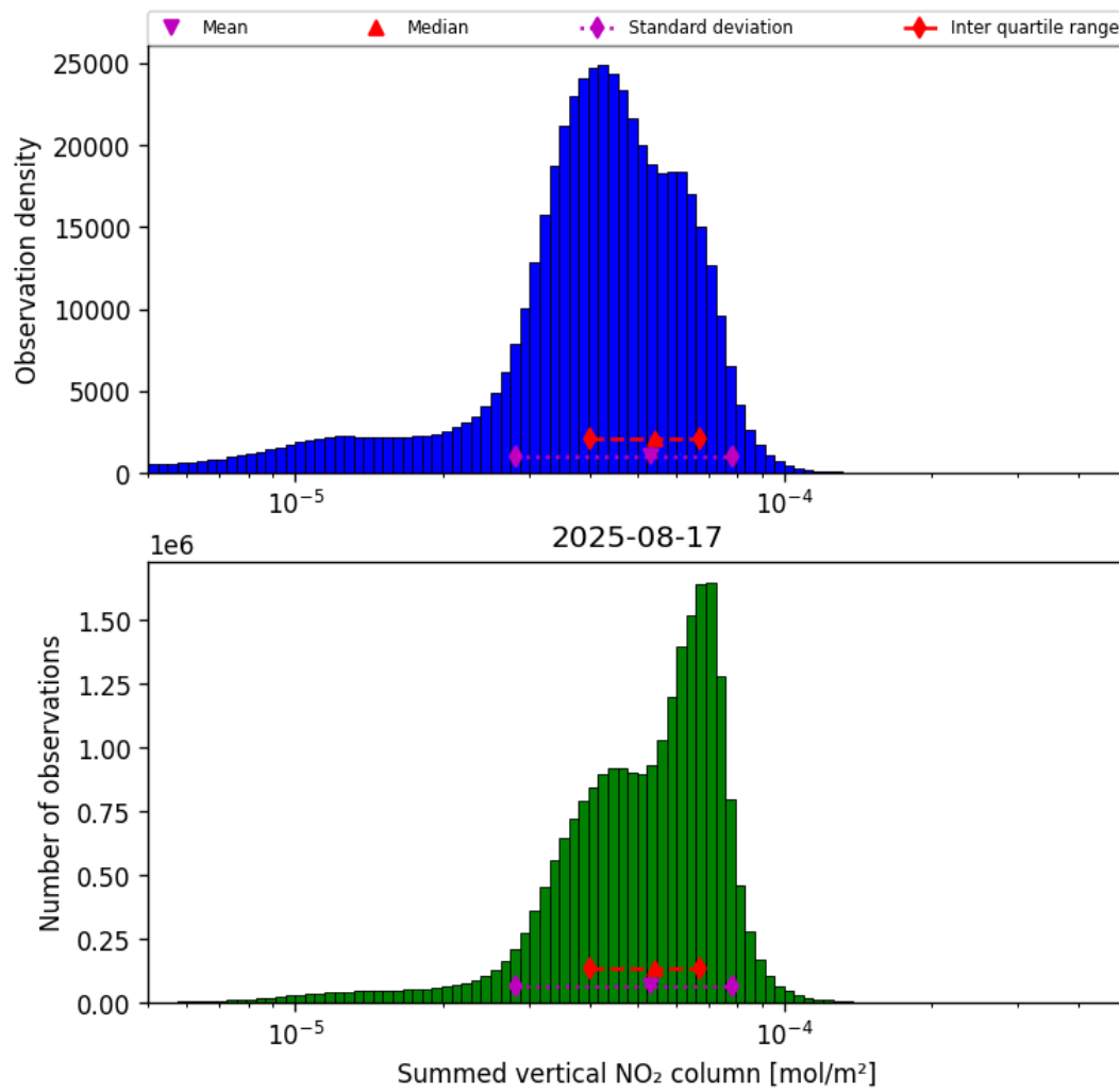
Figure 38: Histogram of “Summed vertical NO 2 column” for 2025-08-17 to 2025-08-17
