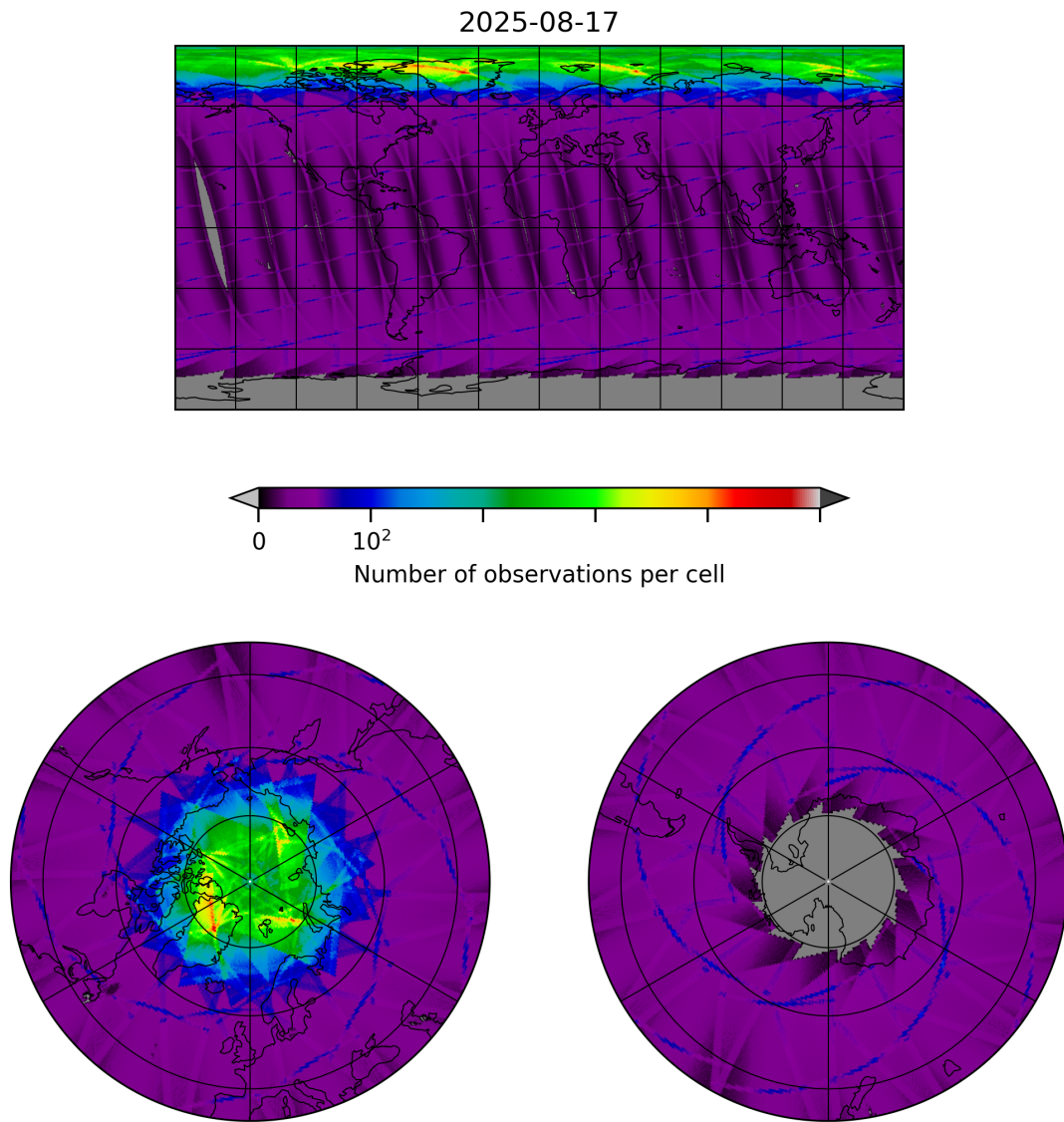
Figure 8: Map of the number of observations for 2025-08-17 to 2025-08-17
