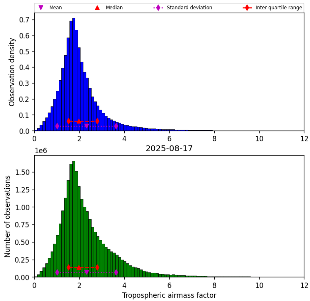
Figure 29: Histogram of “Tropospheric airmass factor” for 2025-08-17 to 2025-08-17
