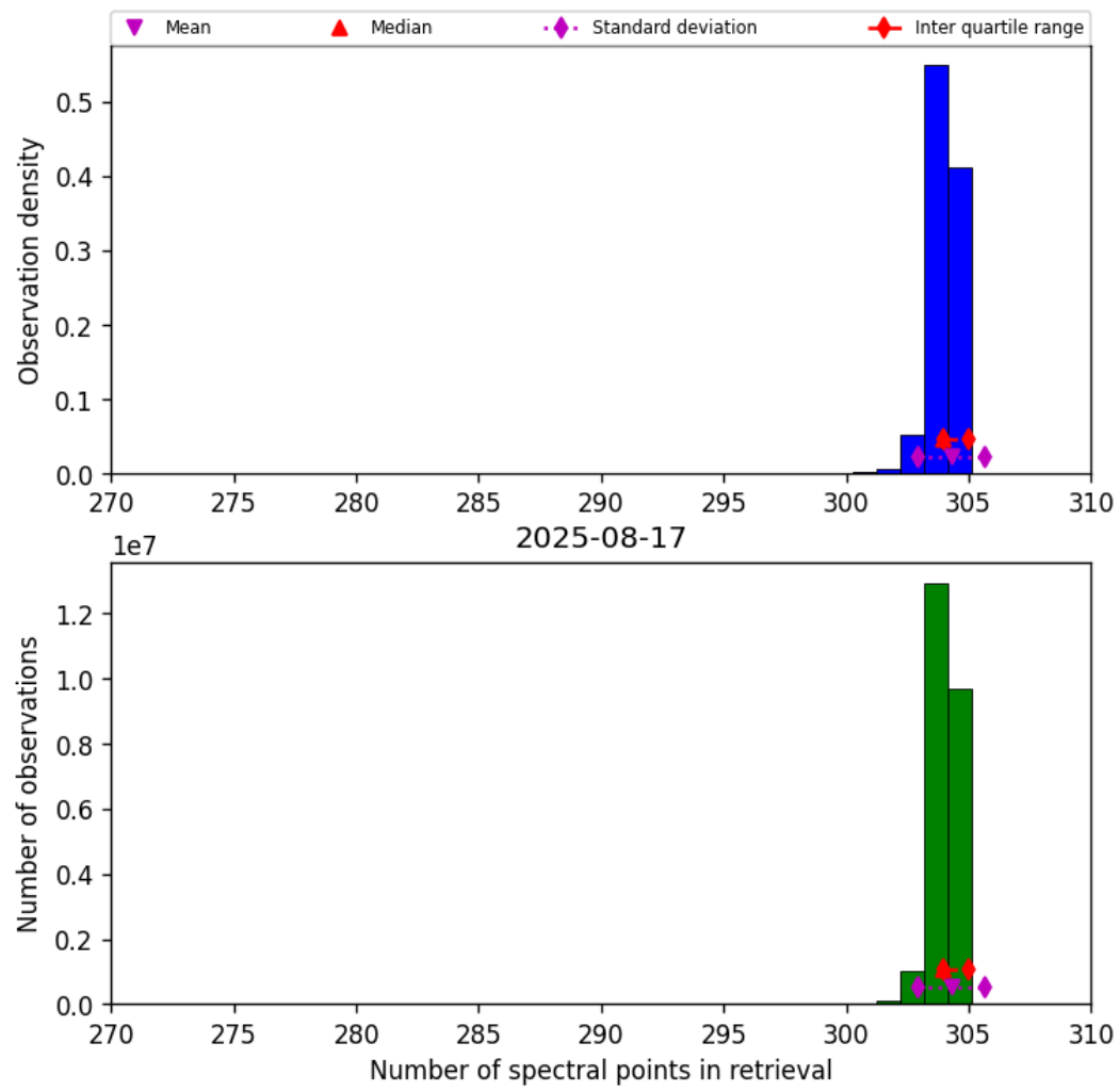
Figure 31: Histogram of “Number of spectral points in retrieval” for 2025-08-17 to 2025-08-17
