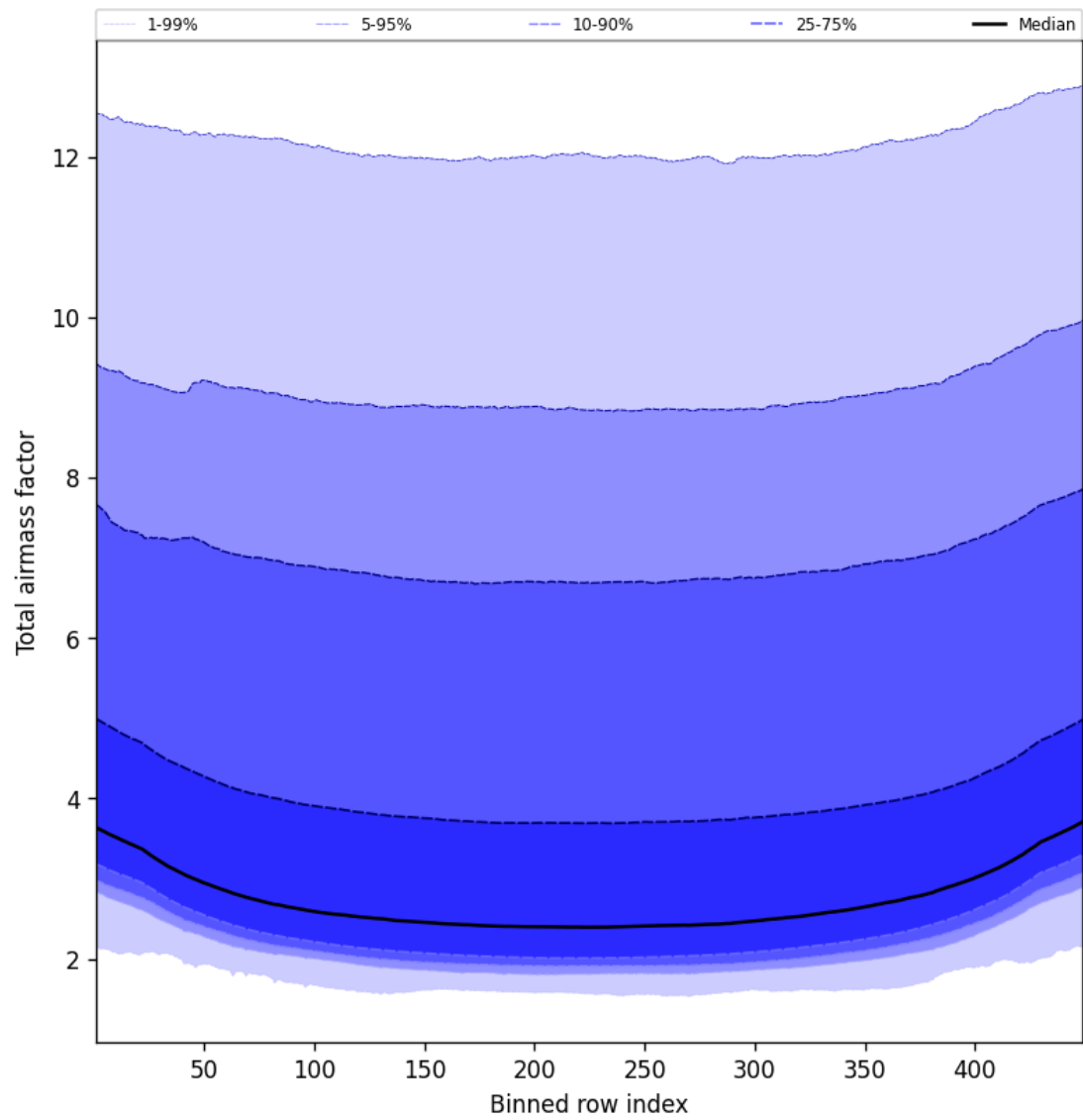
Figure 47: Along track statistics of “Total airmass factor” for 2025-08-17 to 2025-08-17
