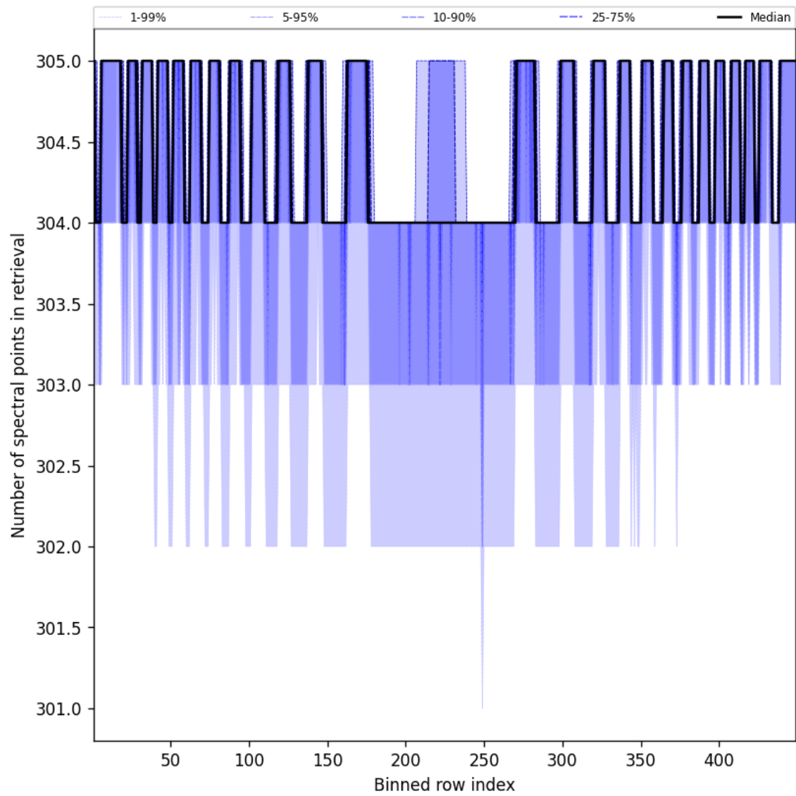
Figure 48: Along track statistics of “Number of spectral points in retrieval” for 2025-08-17 to 2025-08-17
