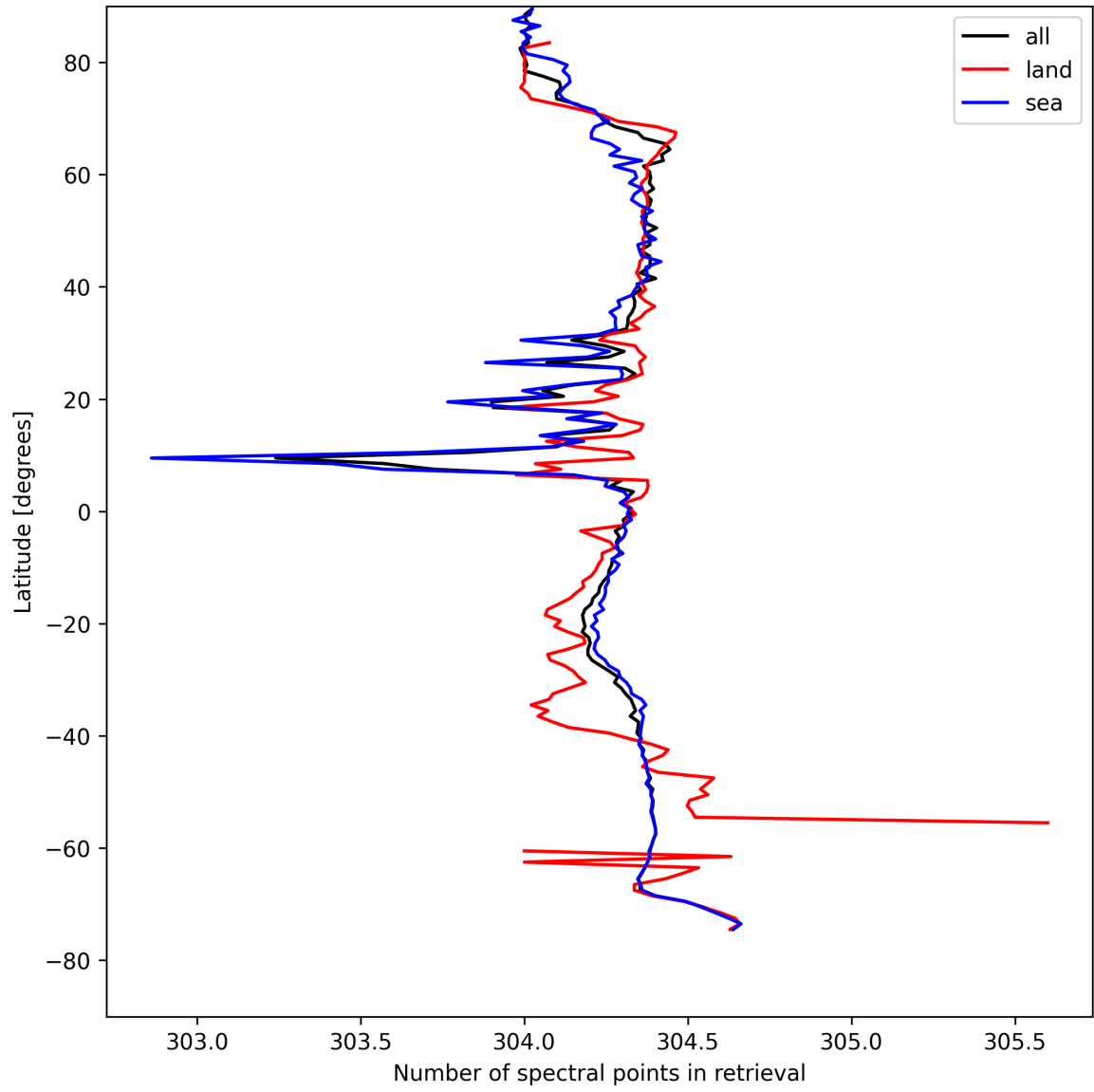
Figure 14: Zonal average of “Number of spectral points in retrieval” for 2025-08-17 to 2025-08-17.
