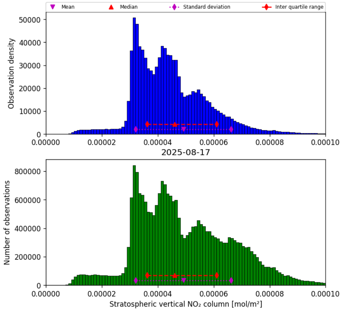
Figure 34: Histogram of “Stratospheric vertical NO 2 column” for 2025-08-17 to 2025-08-17
