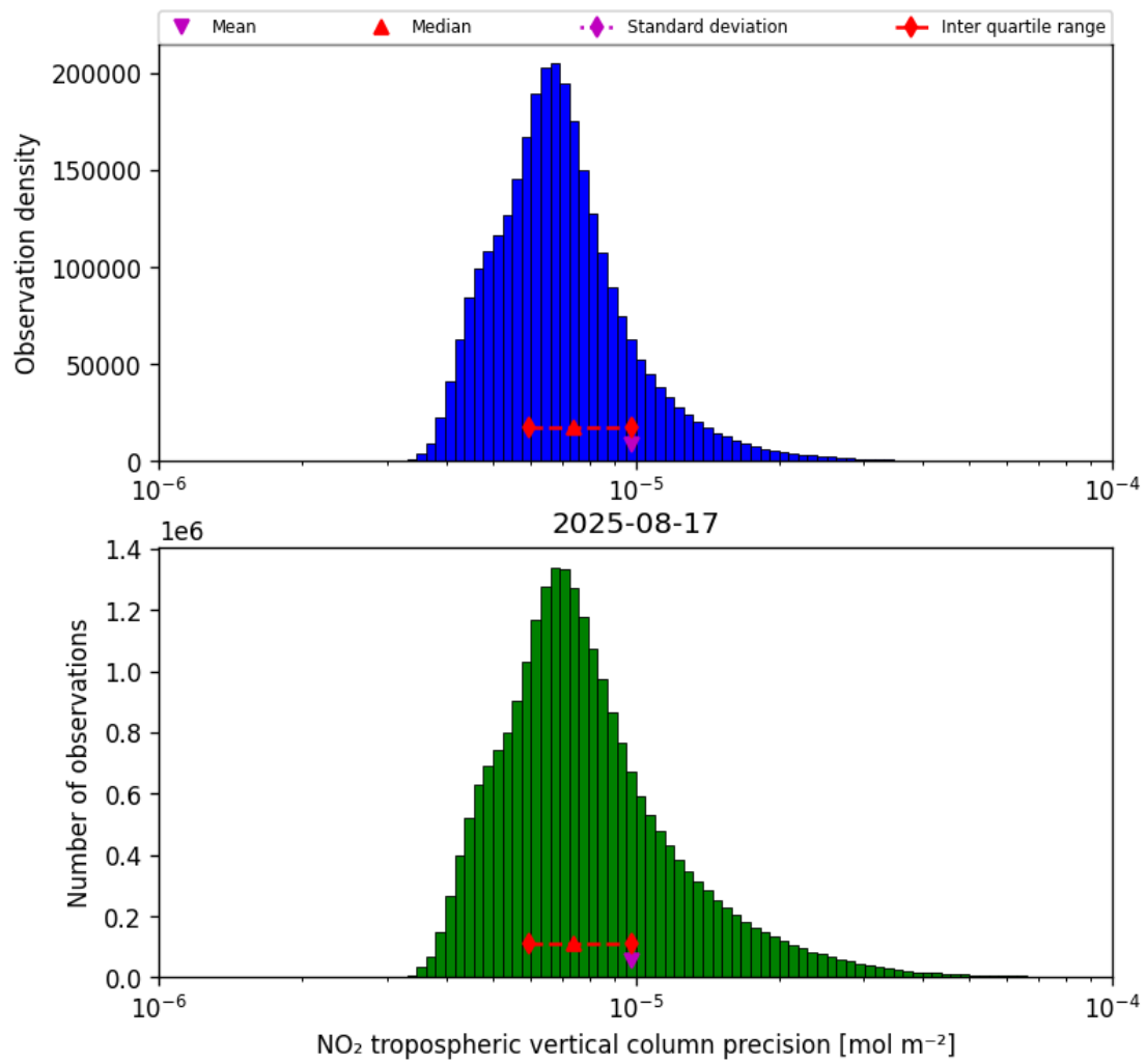
Figure 28: Histogram of “NO 2 tropospheric vertical column precision” for 2025-08-17 to 2025-08-17
