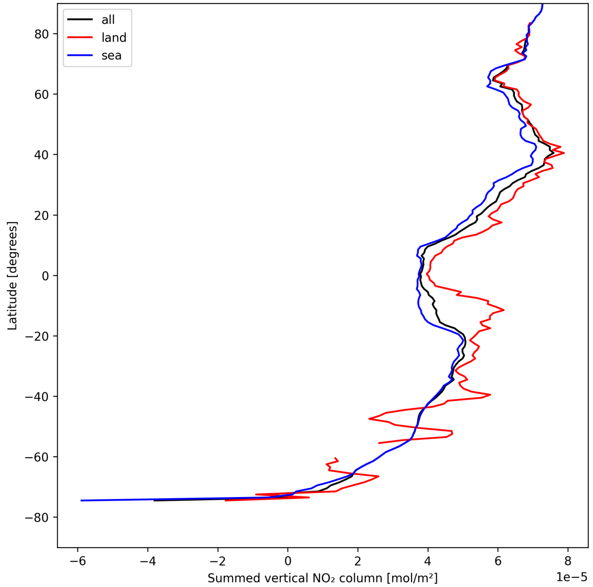
Figure 21: Zonal average of “Summed vertical NO 2 column” for 2025-08-17 to 2025-08-17.
