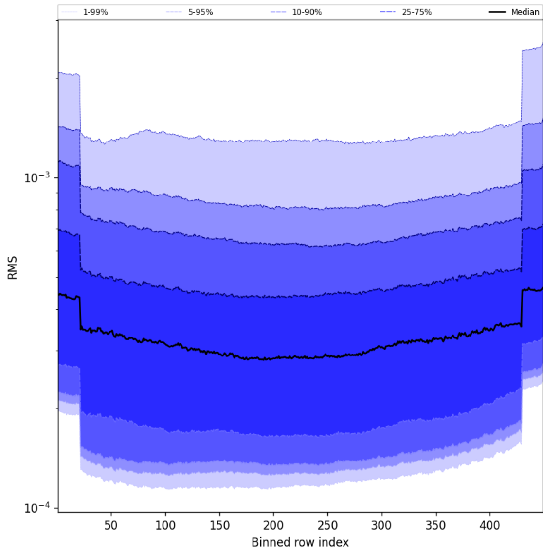
Figure 58: Along track statistics of “RMS” for 2025-08-17 to 2025-08-17
