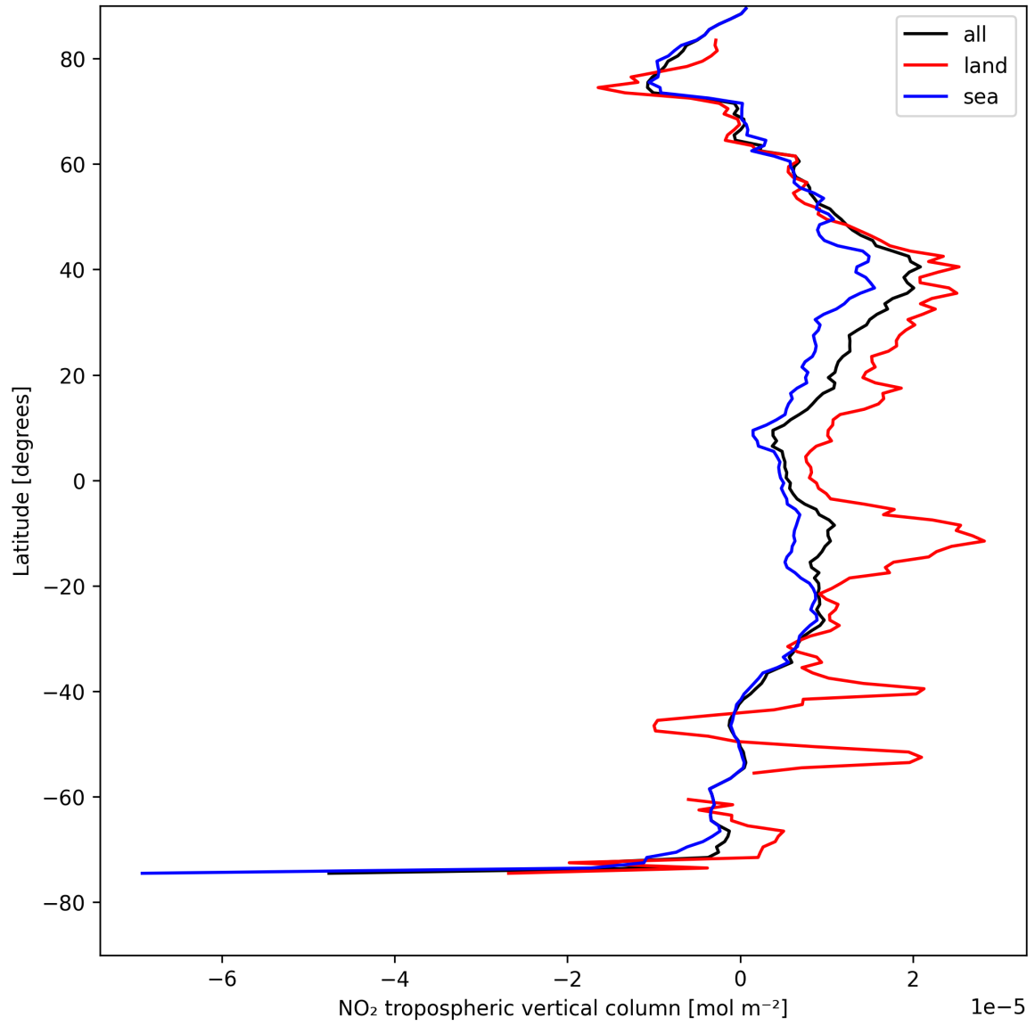
Figure 10: Zonal average of “NO 2 tropospheric vertical column” for 2025-08-17 to 2025-08-17.
