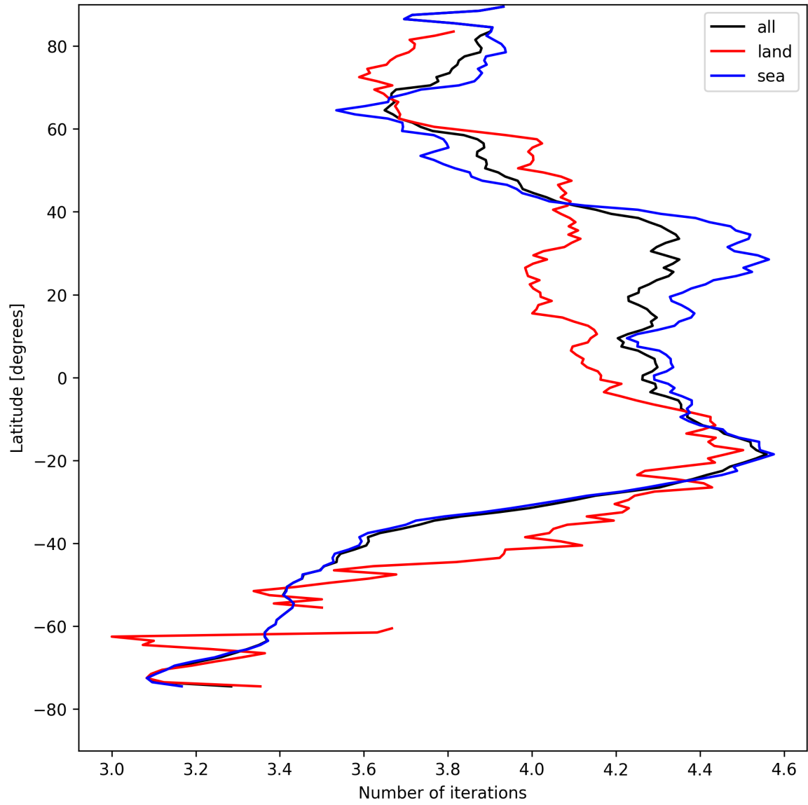
Figure 15: Zonal average of “Number of iterations” for 2025-08-17 to 2025-08-17.
