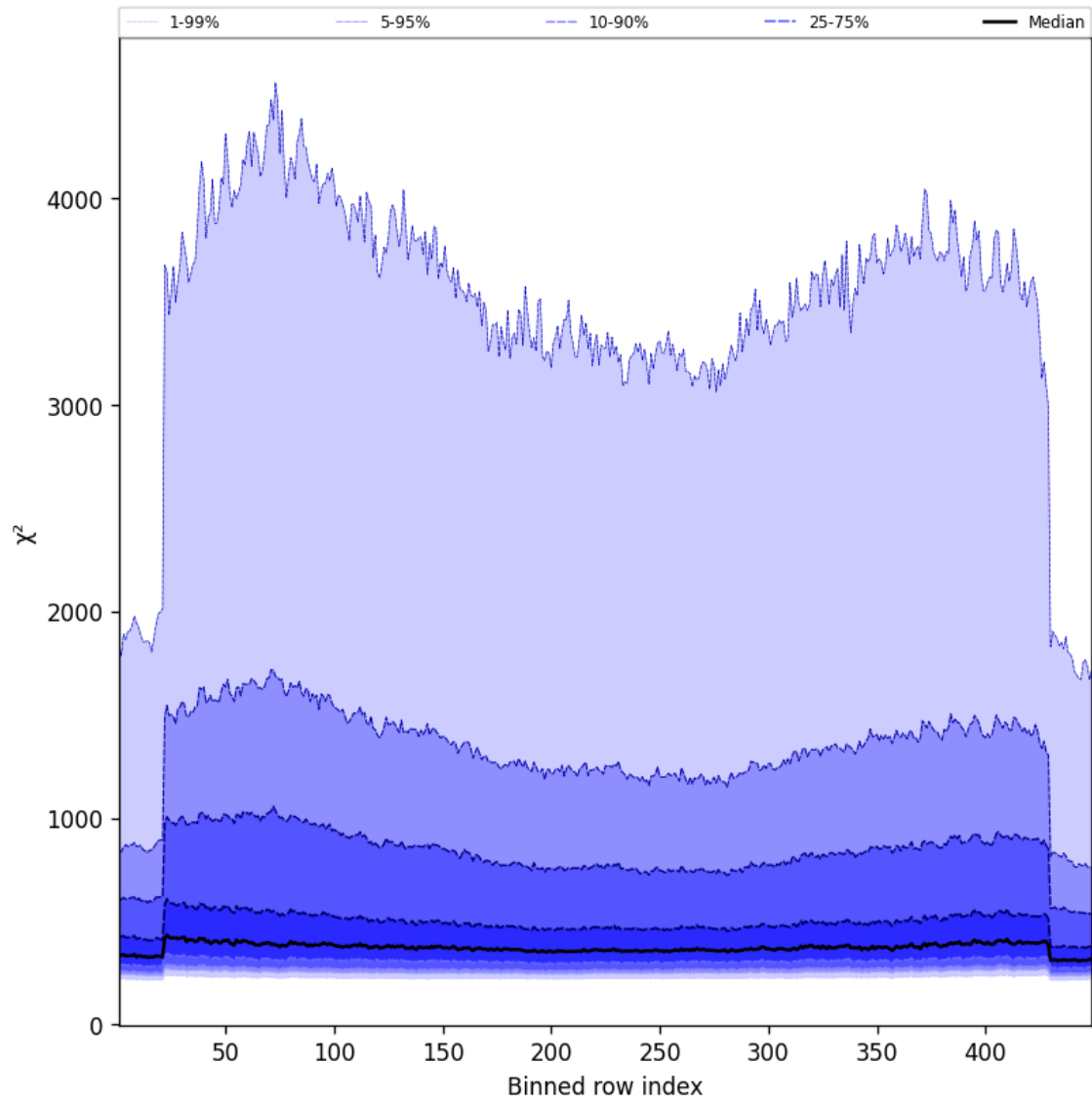
Figure 57: Along track statistics of “ \chi^2 ” for 2025-08-17 to 2025-08-17
