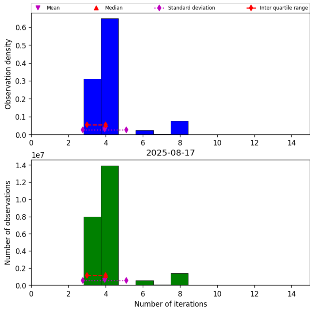
Figure 32: Histogram of “Number of iterations” for 2025-08-17 to 2025-08-17
