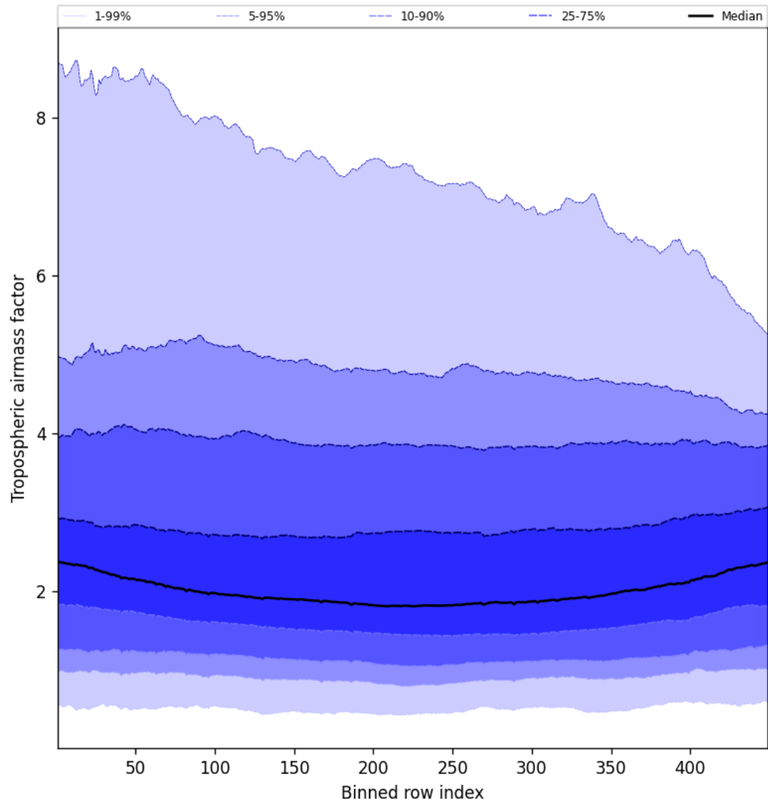
Figure 46: Along track statistics of “Tropospheric airmass factor” for 2025-08-18 to 2025-08-19
