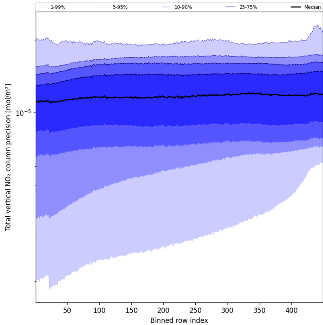
Figure 54: Along track statistics of “Total vertical NO 2 column precision” for 2025-08-18 to 2025-08-19
