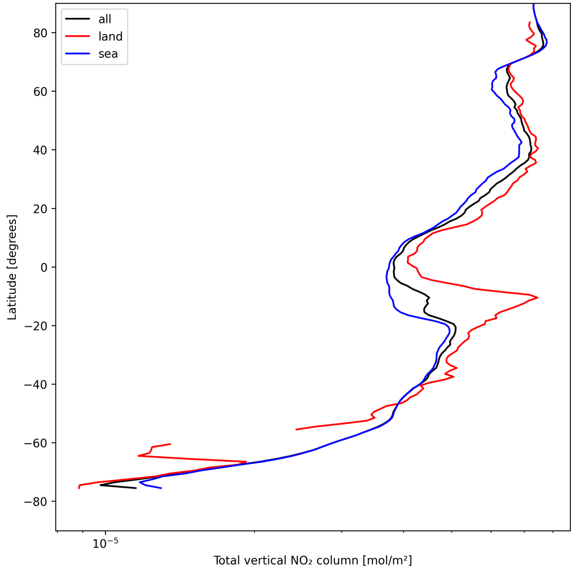
Figure 19: Zonal average of “Total vertical NO 2 column” for 2025-08-18 to 2025-08-19.
