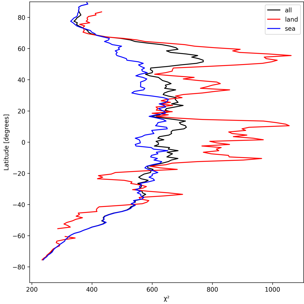
Figure 23: Zonal average of “ \chi^2 ” for 2025-08-18 to 2025-08-19.
