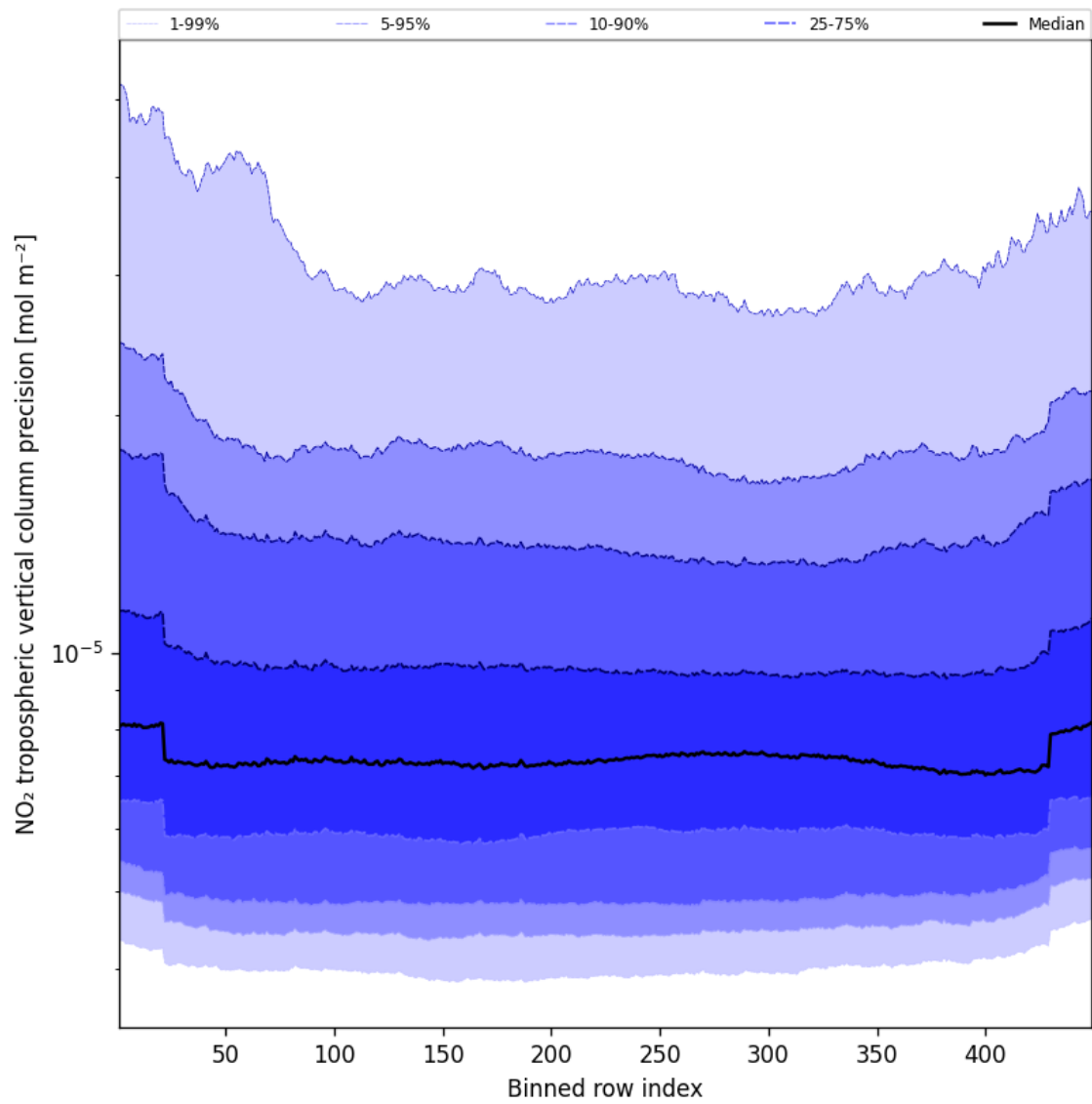
Figure 45: Along track statistics of “NO 2 tropospheric vertical column precision” for 2025-08-18 to 2025-08-19
