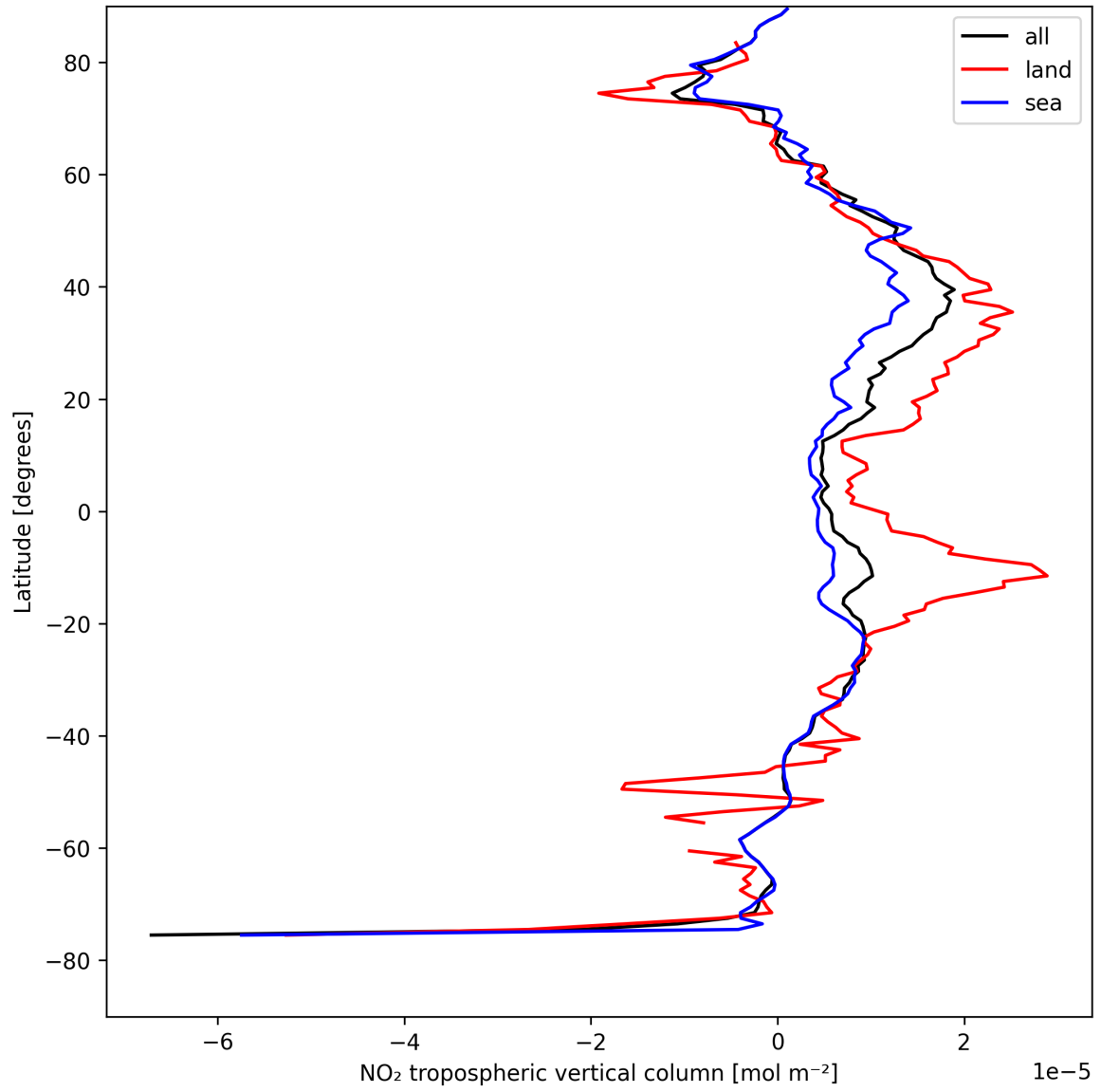
Figure 10: Zonal average of “NO 2 tropospheric vertical column” for 2025-08-18 to 2025-08-19.
