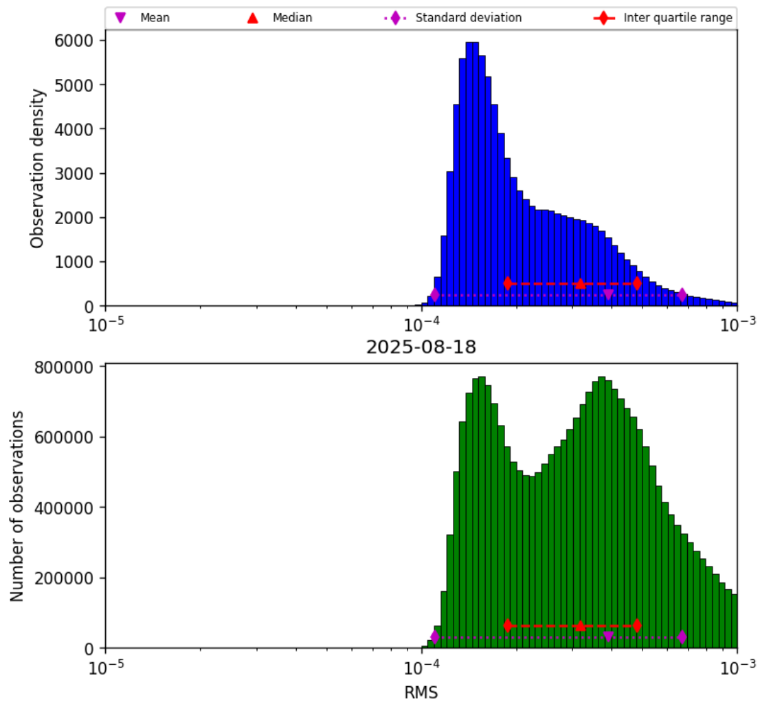
Figure 41: Histogram of “RMS” for 2025-08-18 to 2025-08-19
