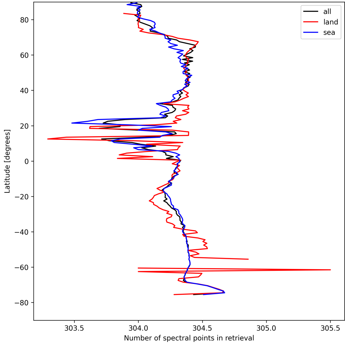
Figure 14: Zonal average of “Number of spectral points in retrieval” for 2025-08-18 to 2025-08-19.
