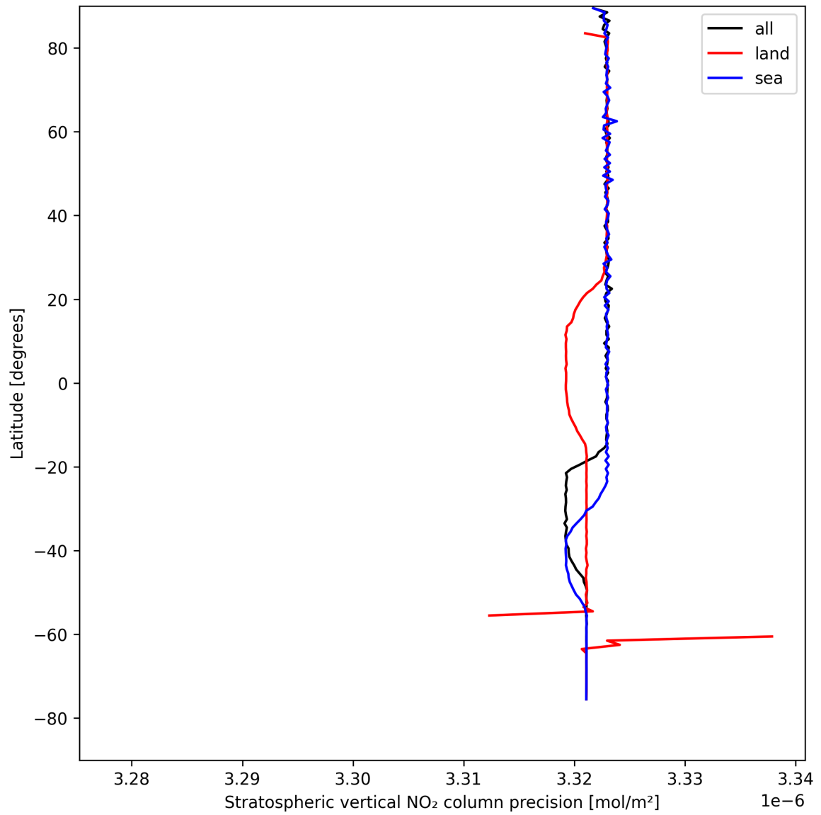
Figure 18: Zonal average of “Stratospheric vertical NO 2 column precision” for 2025-08-18 to 2025-08-19.
