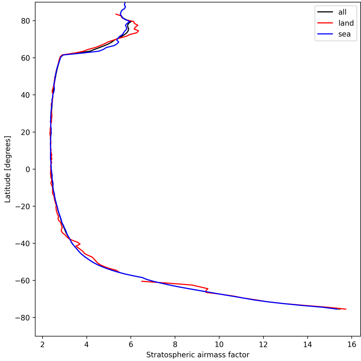
Figure 25: Zonal average of “Stratospheric airmass factor” for 2025-08-18 to 2025-08-19.
