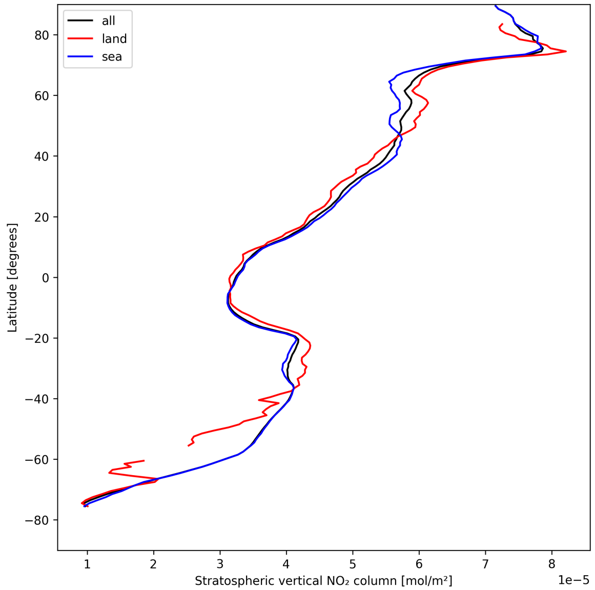
Figure 17: Zonal average of “Stratospheric vertical NO 2 column” for 2025-08-18 to 2025-08-19.
