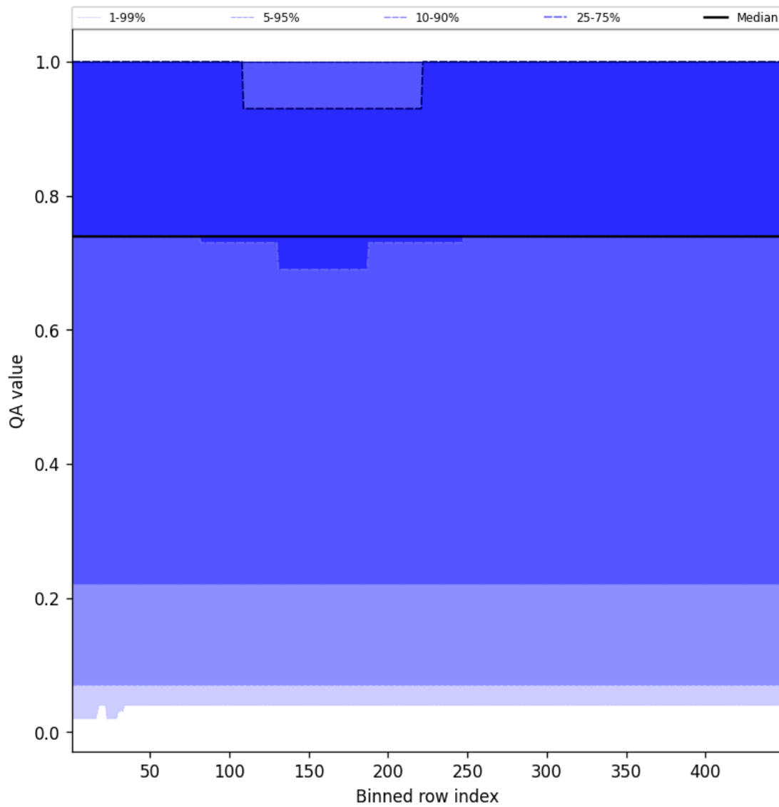
Figure 43: Along track statistics of “QA value” for 2025-08-18 to 2025-08-19
