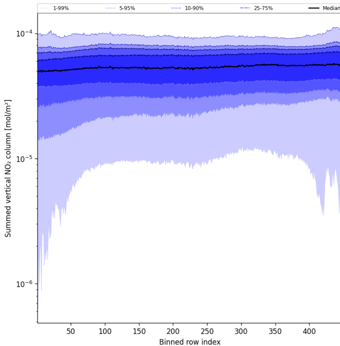
Figure 55: Along track statistics of “Summed vertical NO 2 column” for 2025-08-18 to 2025-08-19
