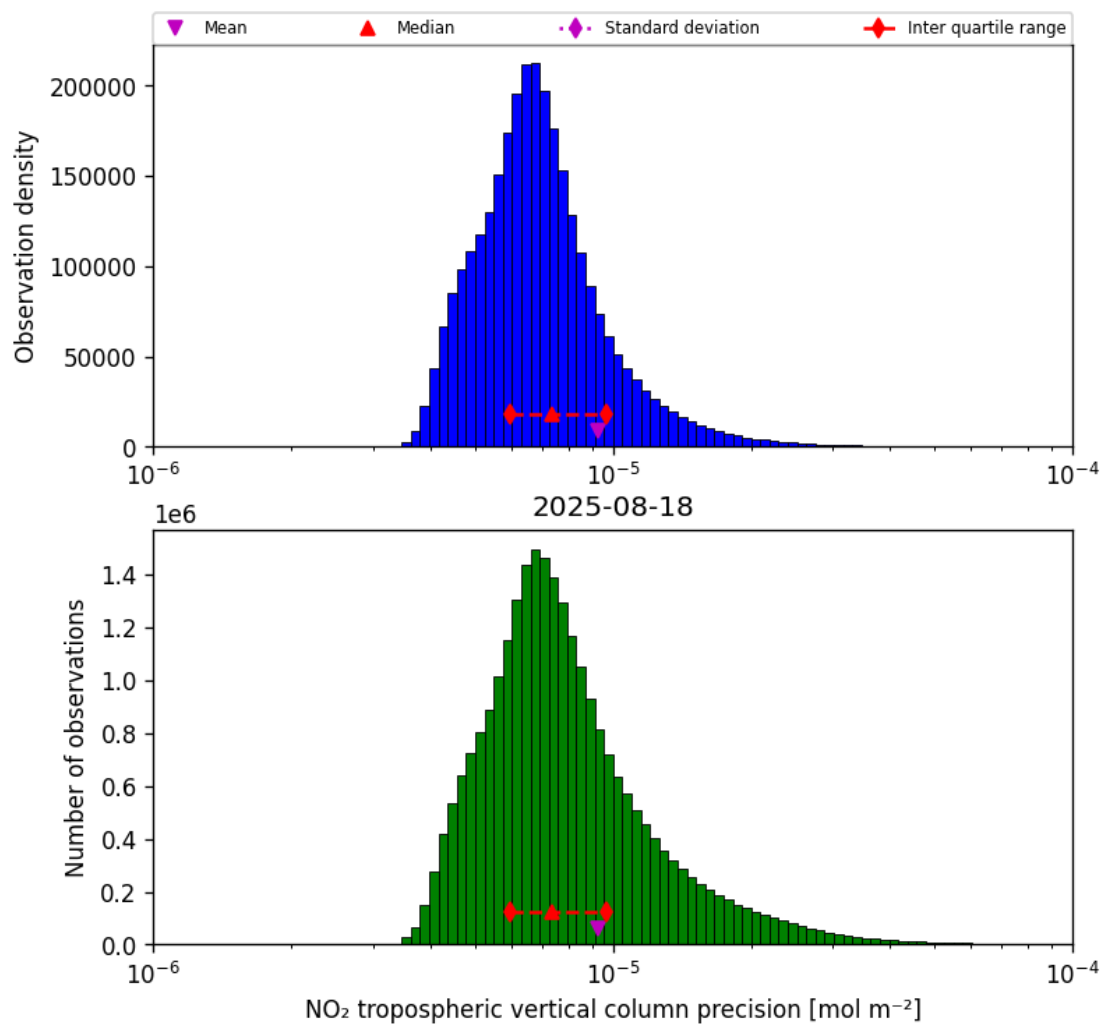
Figure 28: Histogram of “NO 2 tropospheric vertical column precision” for 2025-08-18 to 2025-08-19
