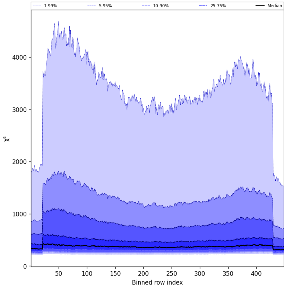
Figure 57: Along track statistics of “ \chi^2 ” for 2025-08-18 to 2025-08-19
