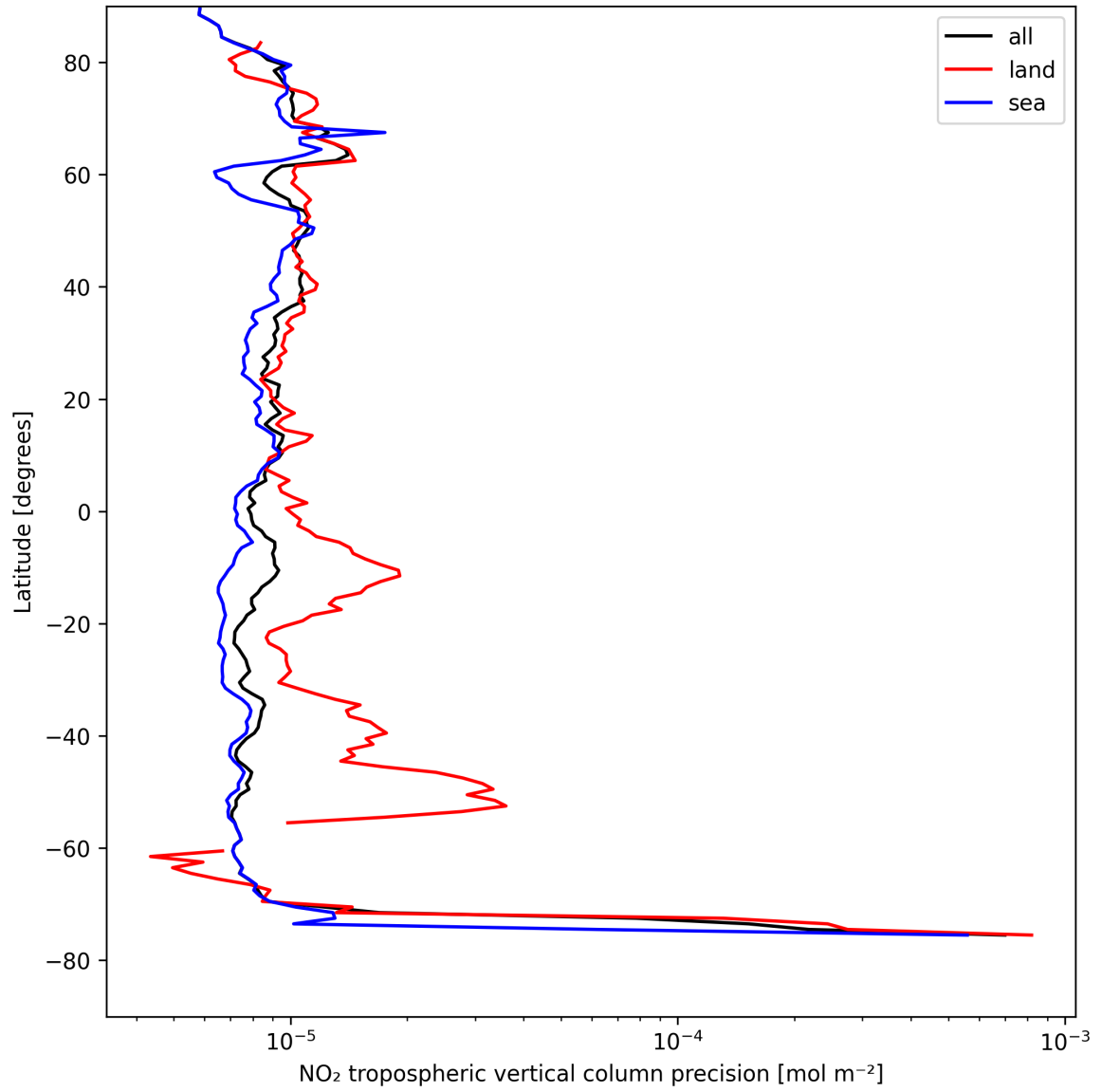
Figure 11: Zonal average of “NO 2 tropospheric vertical column precision” for 2025-08-18 to 2025-08-19.
