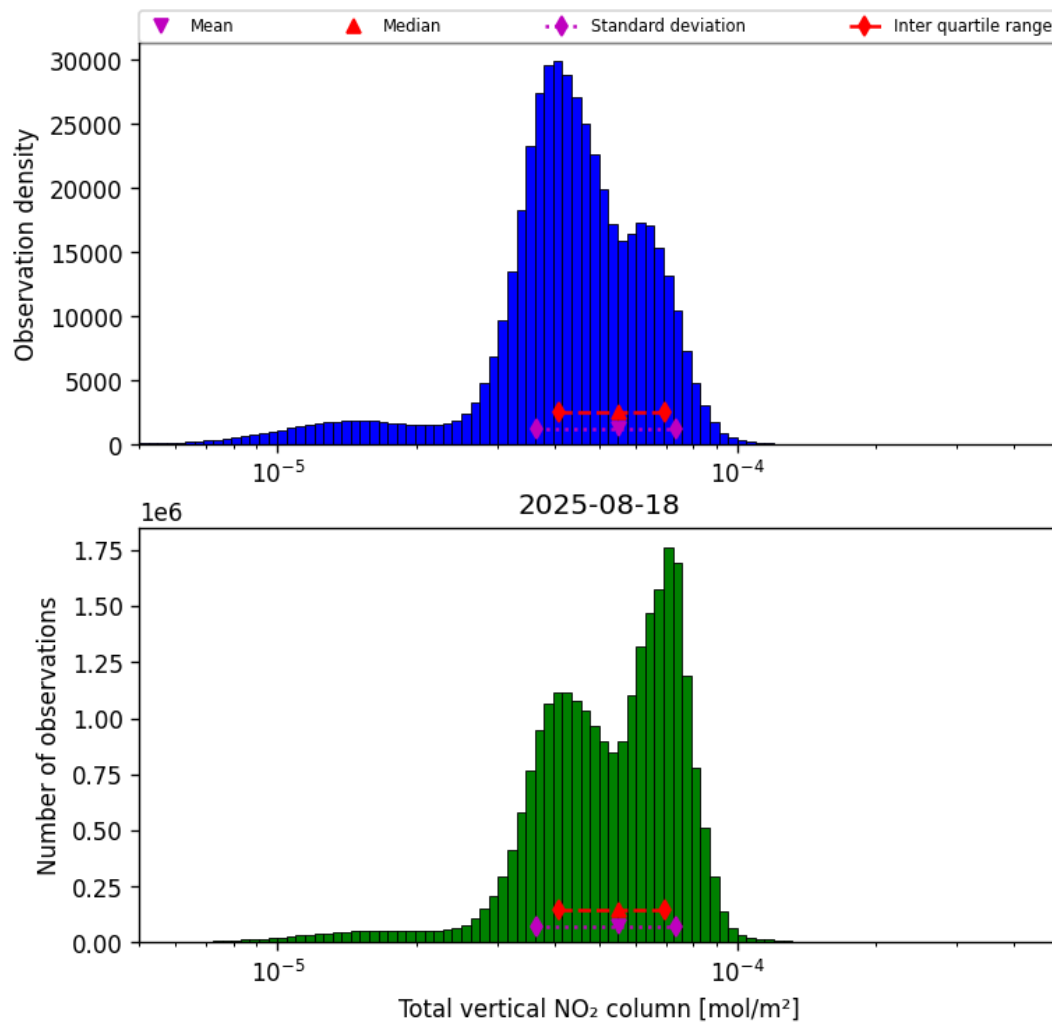
Figure 36: Histogram of “Total vertical NO 2 column” for 2025-08-18 to 2025-08-19
