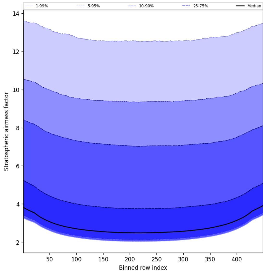
Figure 59: Along track statistics of “Stratospheric airmass factor” for 2025-08-18 to 2025-08-19
