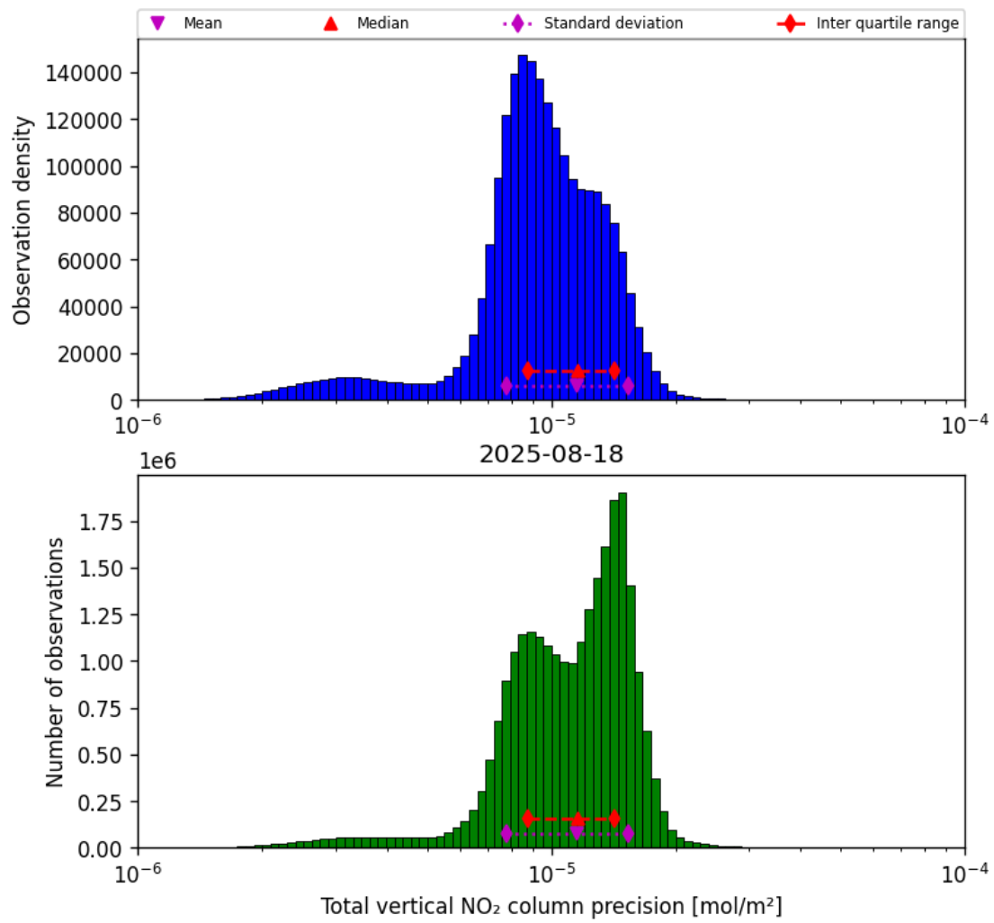
Figure 37: Histogram of “Total vertical NO 2 column precision” for 2025-08-18 to 2025-08-19
