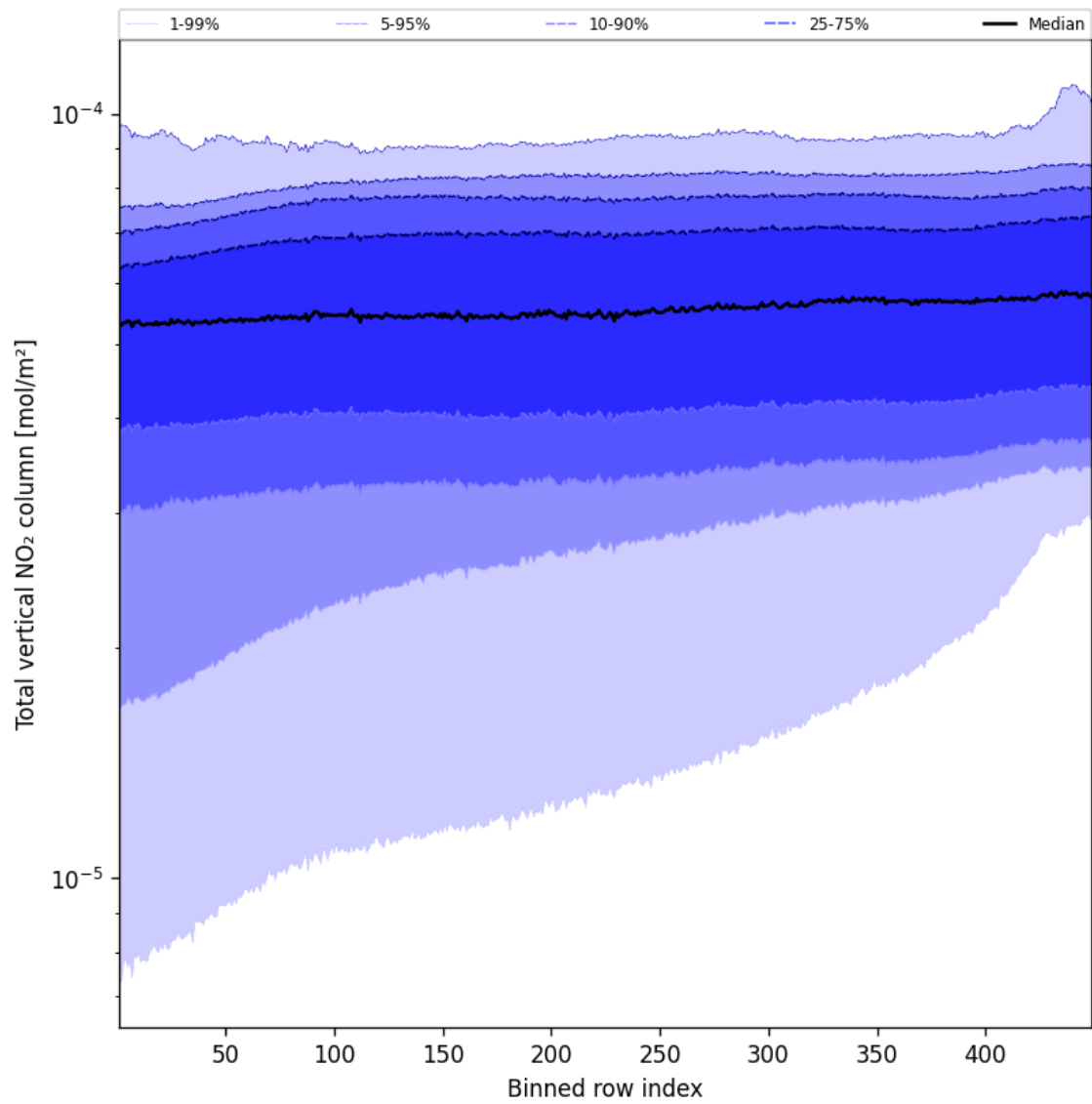
Figure 53: Along track statistics of “Total vertical NO 2 column” for 2025-08-18 to 2025-08-19
