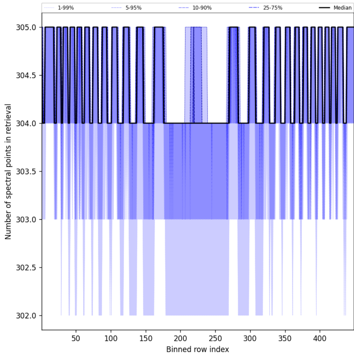
Figure 48: Along track statistics of “Number of spectral points in retrieval” for 2025-08-18 to 2025-08-19
