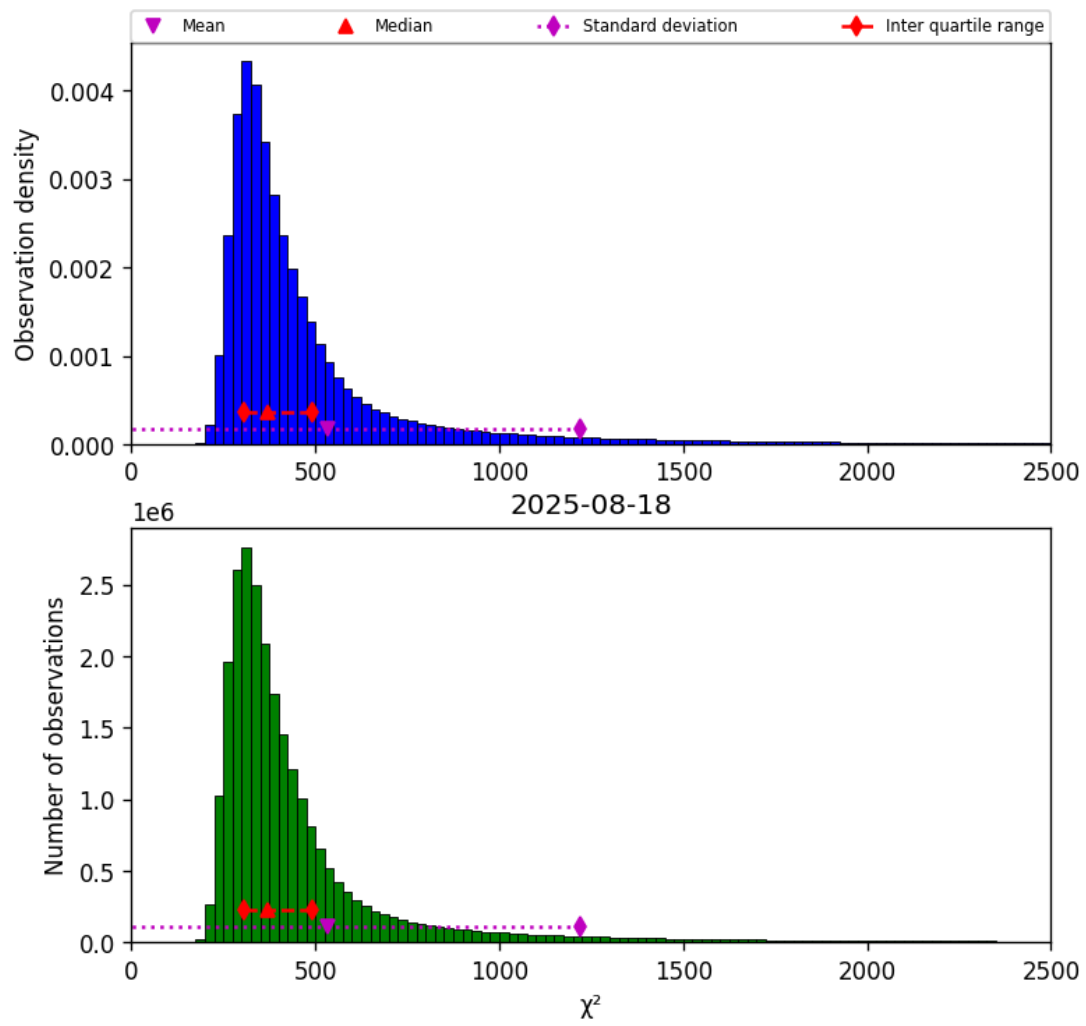
Figure 40: Histogram of “ \chi^2 ” for 2025-08-18 to 2025-08-19
