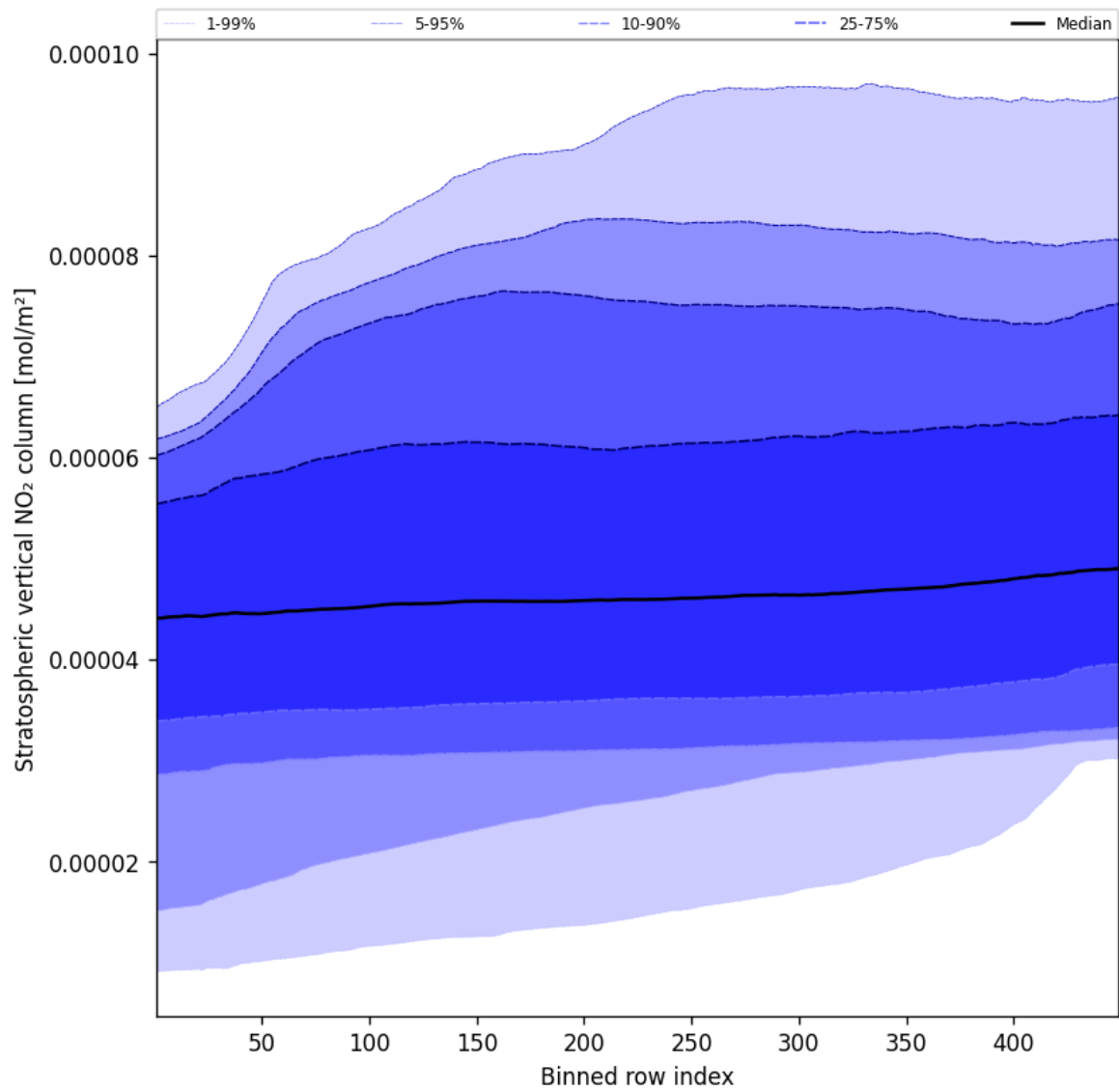
Figure 51: Along track statistics of “Stratospheric vertical NO 2 column” for 2025-08-18 to 2025-08-19
