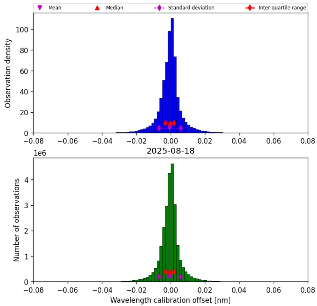
Figure 33: Histogram of “Wavelength calibration offset” for 2025-08-18 to 2025-08-19
