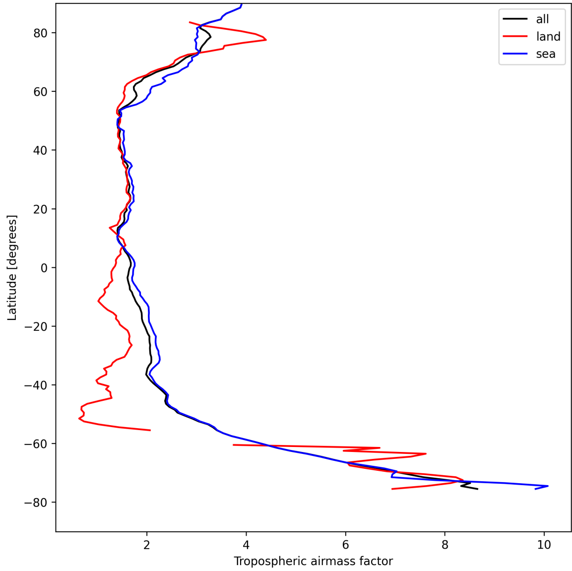
Figure 12: Zonal average of “Tropospheric airmass factor” for 2025-08-18 to 2025-08-19.
