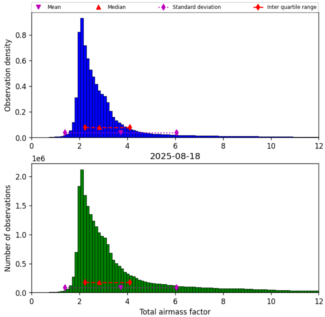
Figure 30: Histogram of “Total airmass factor” for 2025-08-18 to 2025-08-19
