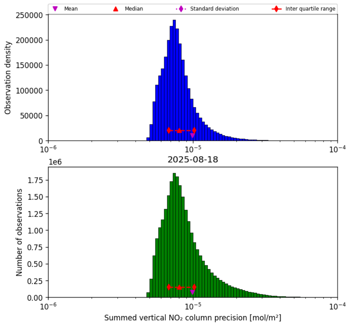
Figure 39: Histogram of “Summed vertical NO 2 column precision” for 2025-08-18 to 2025-08-19
