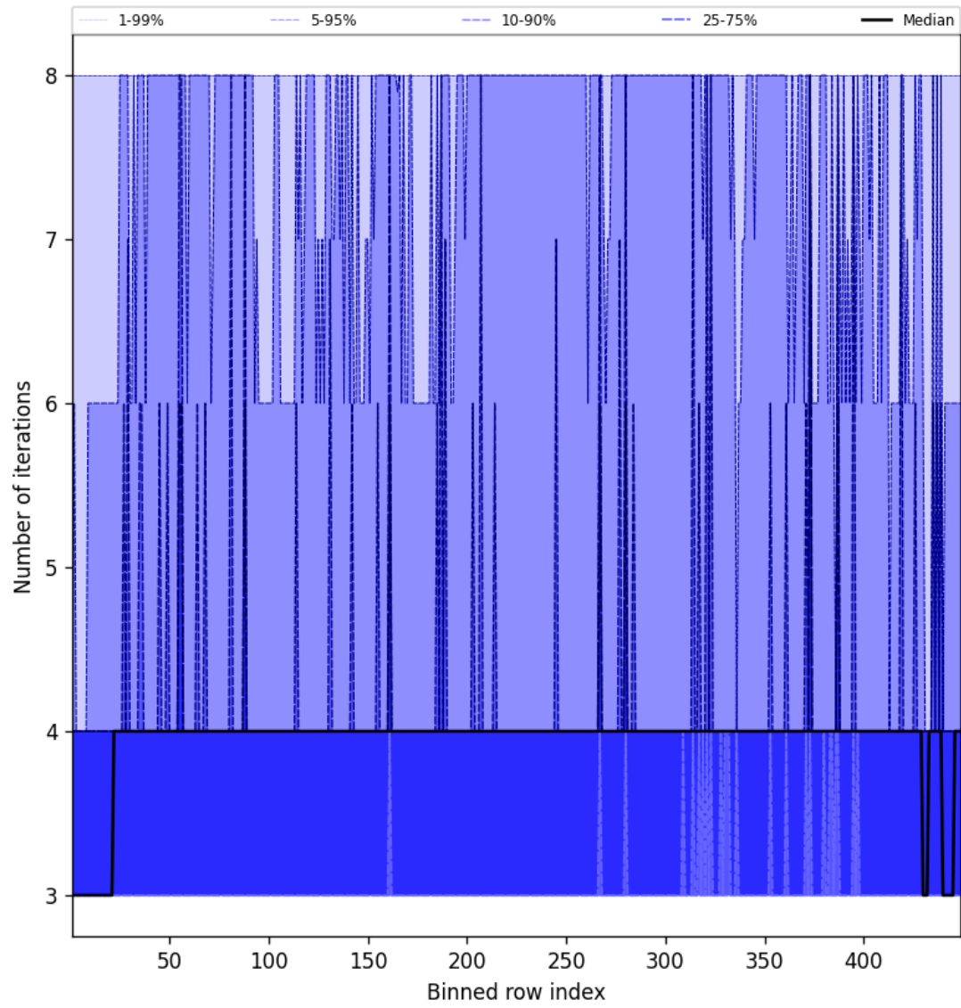
Figure 49: Along track statistics of “Number of iterations” for 2025-08-18 to 2025-08-19
