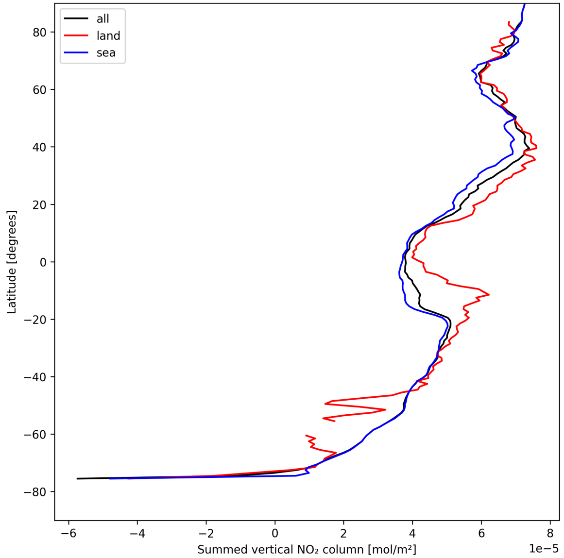
Figure 21: Zonal average of “Summed vertical NO 2 column” for 2025-08-18 to 2025-08-19.
