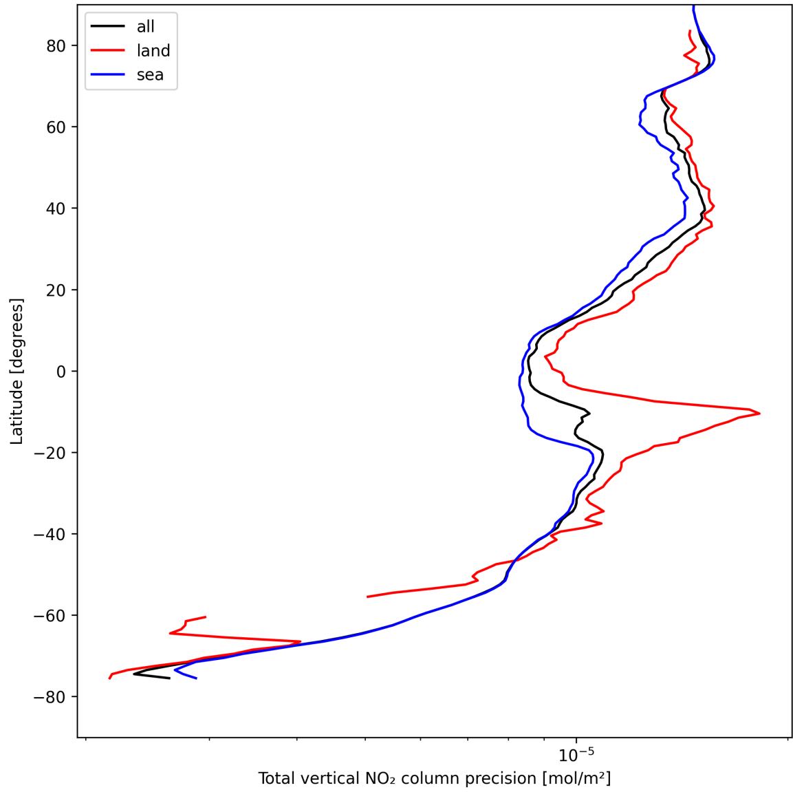
Figure 20: Zonal average of “Total vertical NO 2 column precision” for 2025-08-18 to 2025-08-19.
