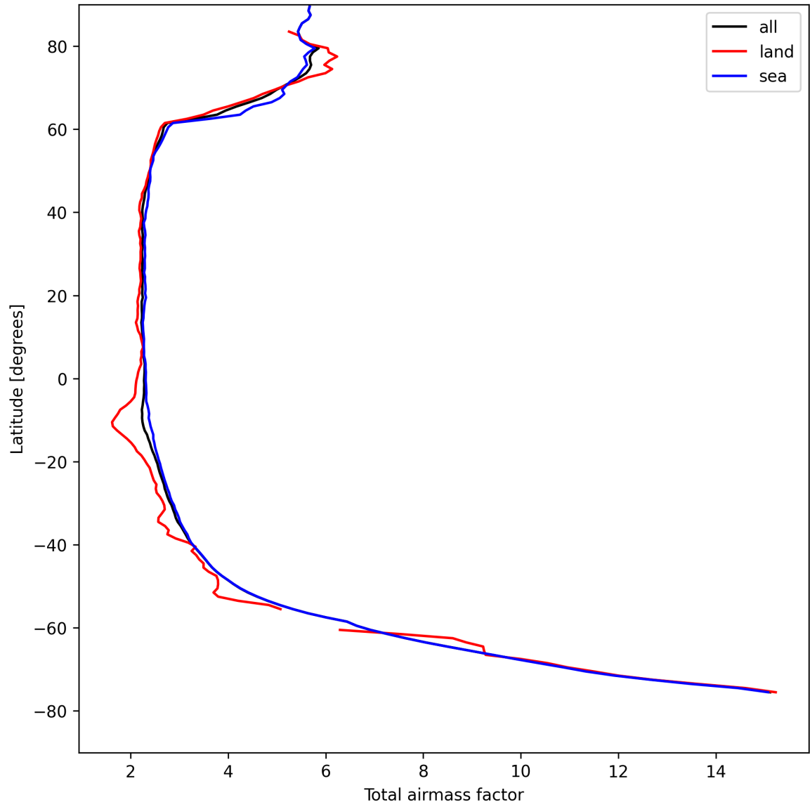
Figure 13: Zonal average of “Total airmass factor” for 2025-08-18 to 2025-08-19.
