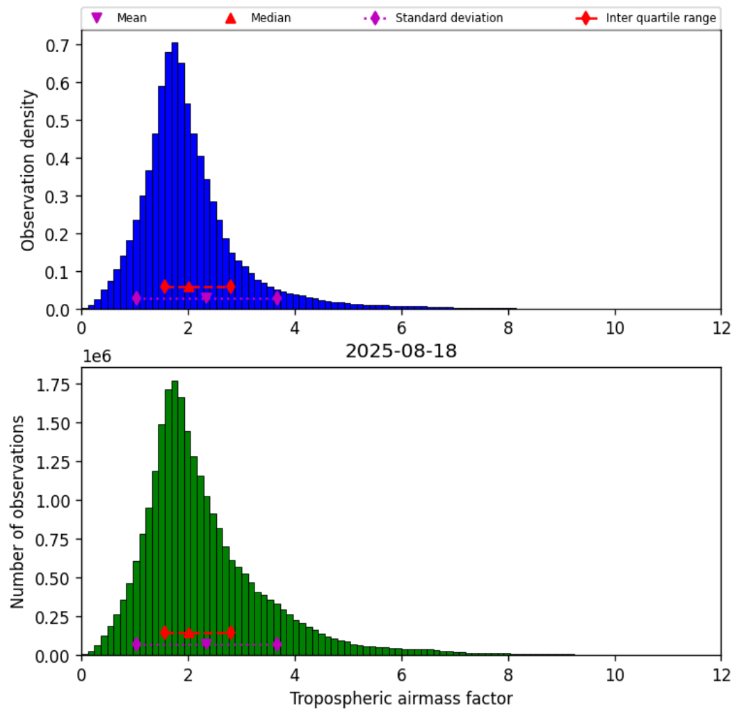
Figure 29: Histogram of “Tropospheric airmass factor” for 2025-08-18 to 2025-08-19
