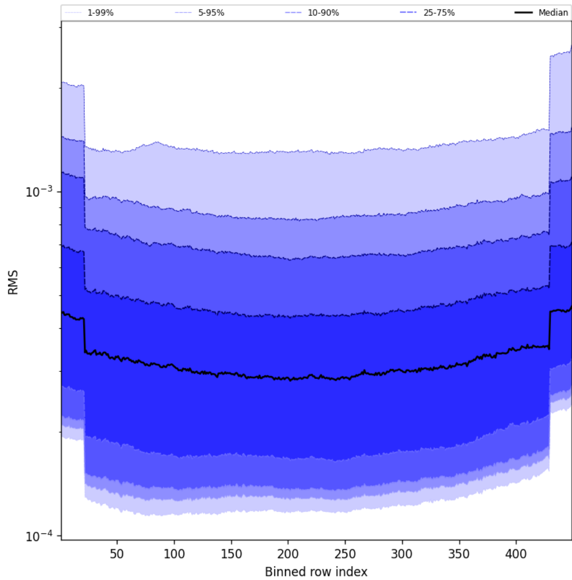
Figure 58: Along track statistics of “RMS” for 2025-08-18 to 2025-08-19
