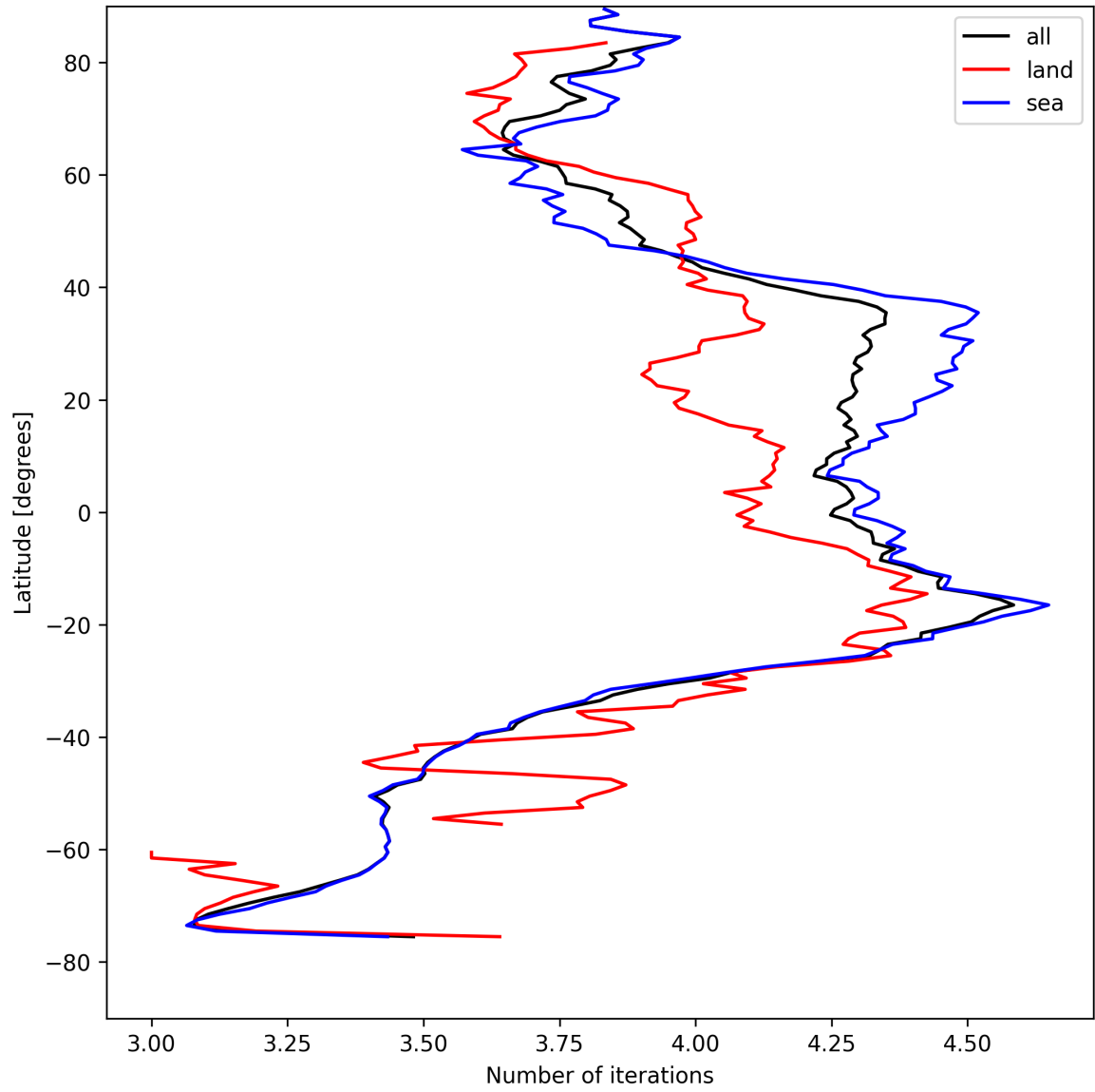
Figure 15: Zonal average of “Number of iterations” for 2025-08-18 to 2025-08-19.
