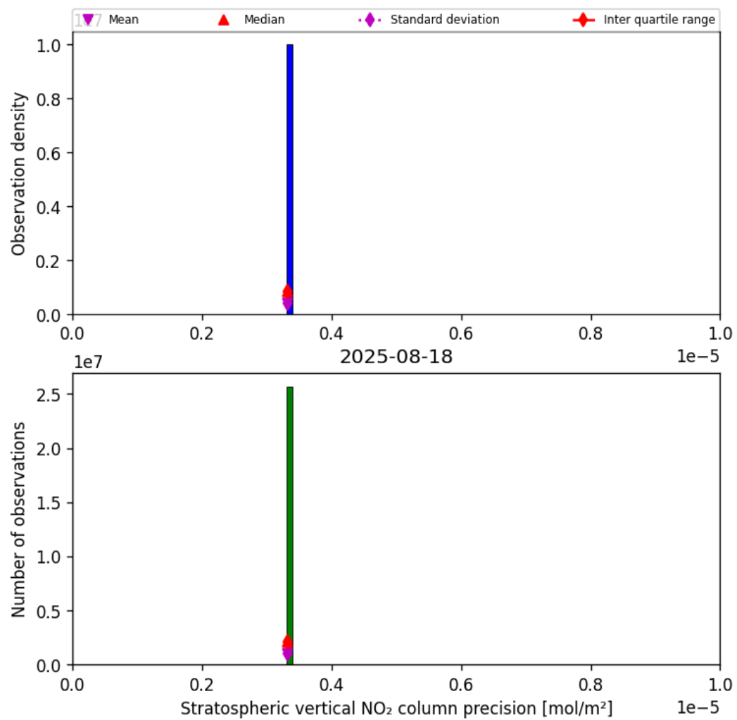
Figure 35: Histogram of “Stratospheric vertical NO 2 column precision” for 2025-08-18 to 2025-08-19
