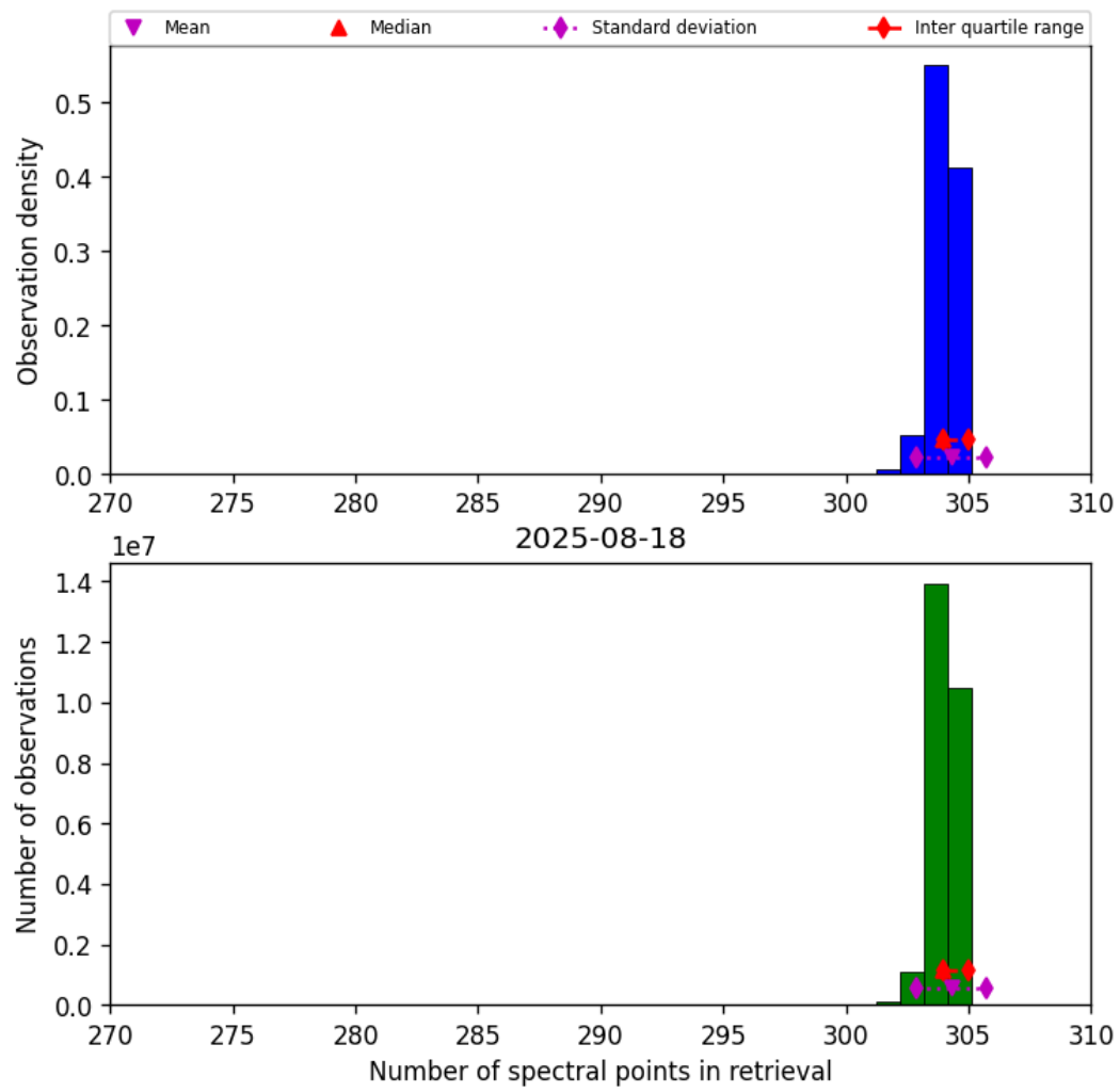
Figure 31: Histogram of “Number of spectral points in retrieval” for 2025-08-18 to 2025-08-19
