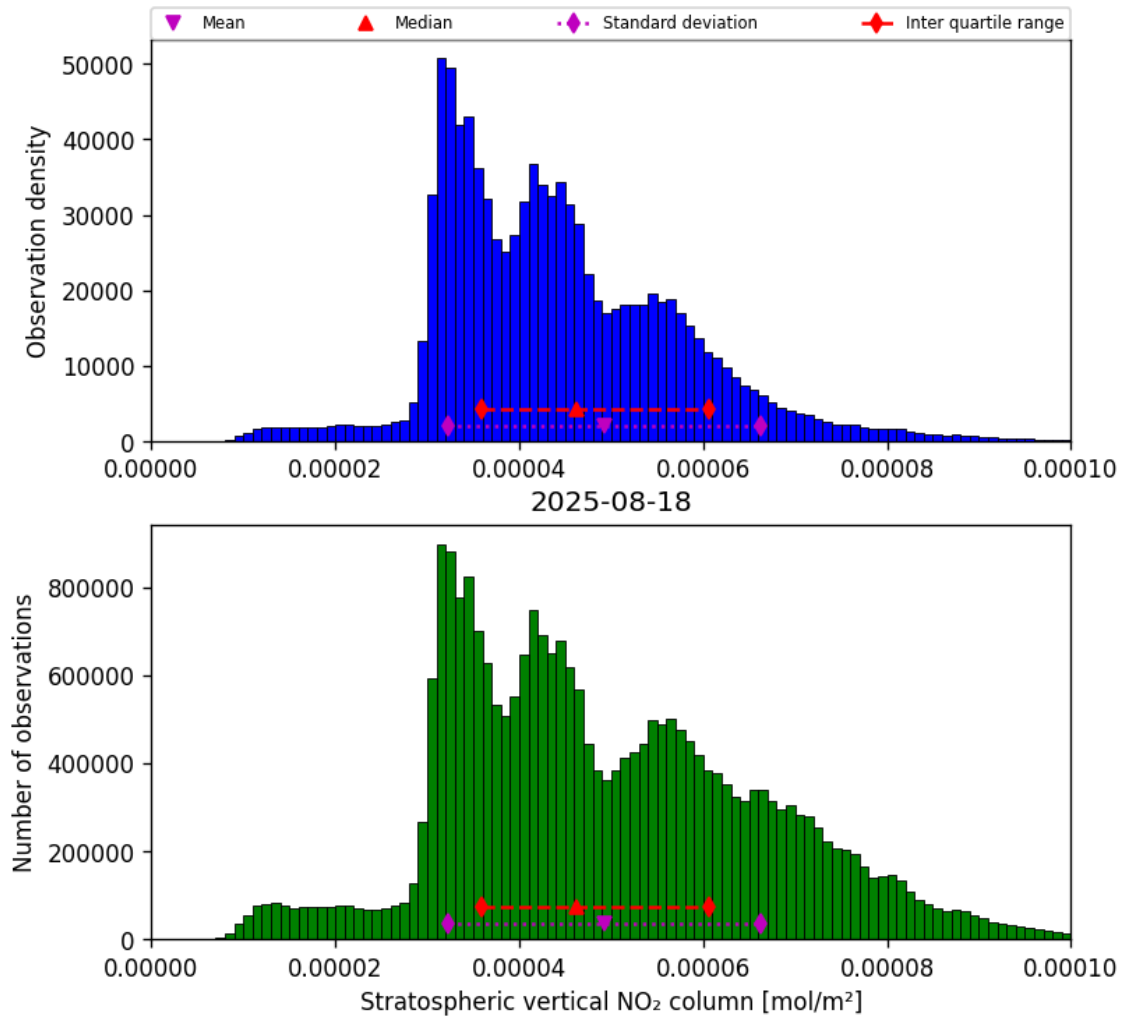
Figure 34: Histogram of “Stratospheric vertical NO 2 column” for 2025-08-18 to 2025-08-19
