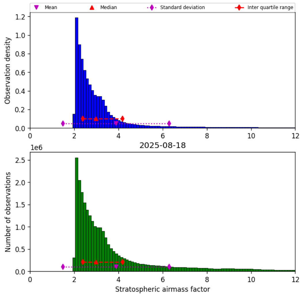
Figure 42: Histogram of “Stratospheric airmass factor” for 2025-08-18 to 2025-08-19
