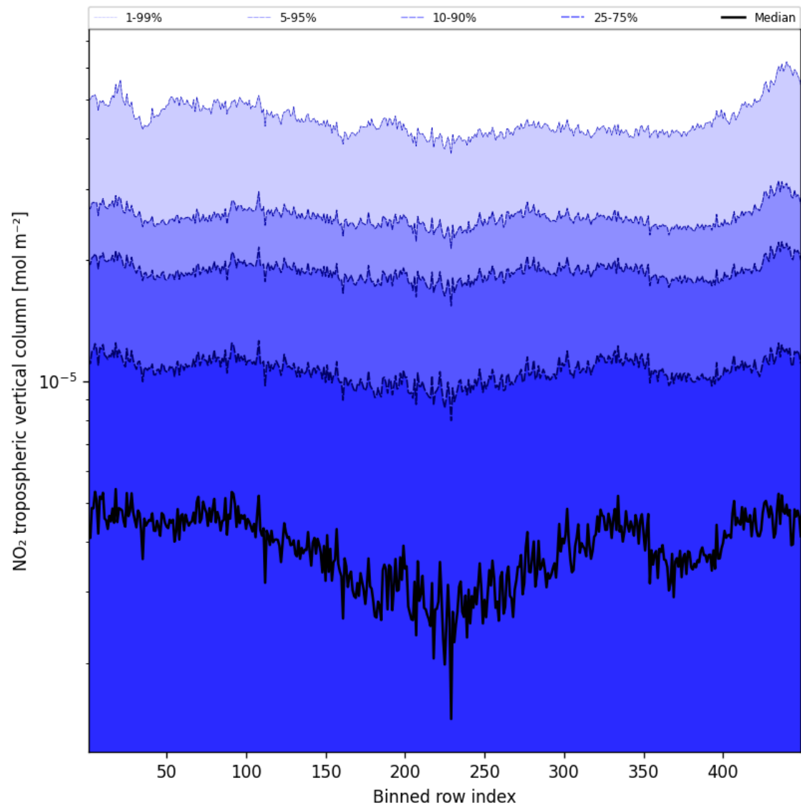
Figure 44: Along track statistics of “NO 2 tropospheric vertical column” for 2025-08-18 to 2025-08-19
