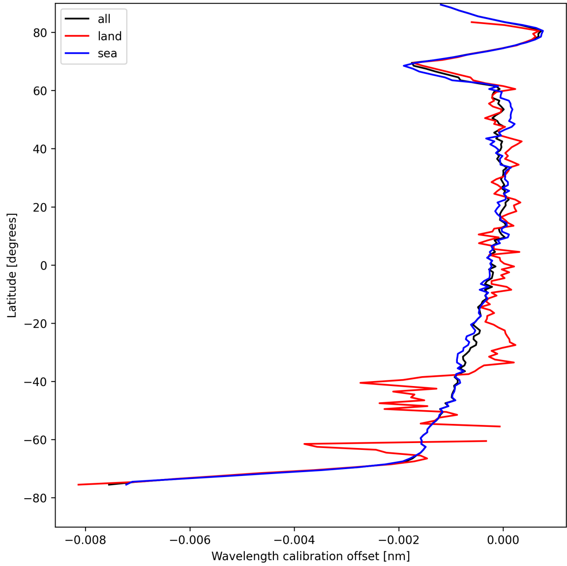
Figure 16: Zonal average of “Wavelength calibration offset” for 2025-08-18 to 2025-08-19.
