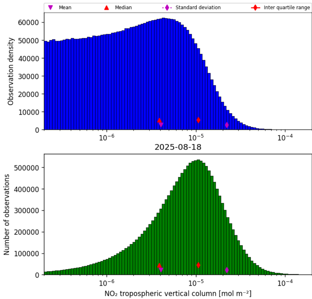
Figure 27: Histogram of “NO 2 tropospheric vertical column” for 2025-08-18 to 2025-08-19
