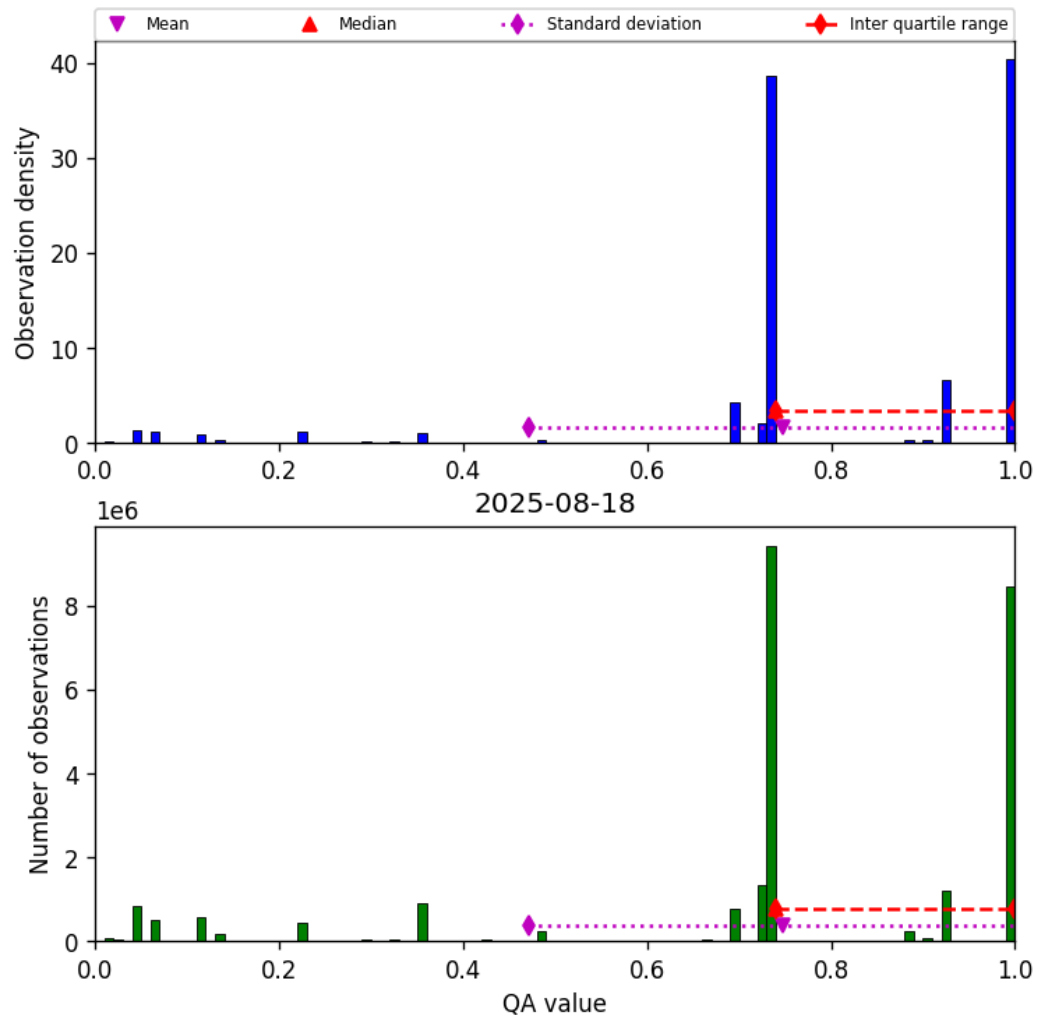
Figure 26: Histogram of “QA value” for 2025-08-18 to 2025-08-19
