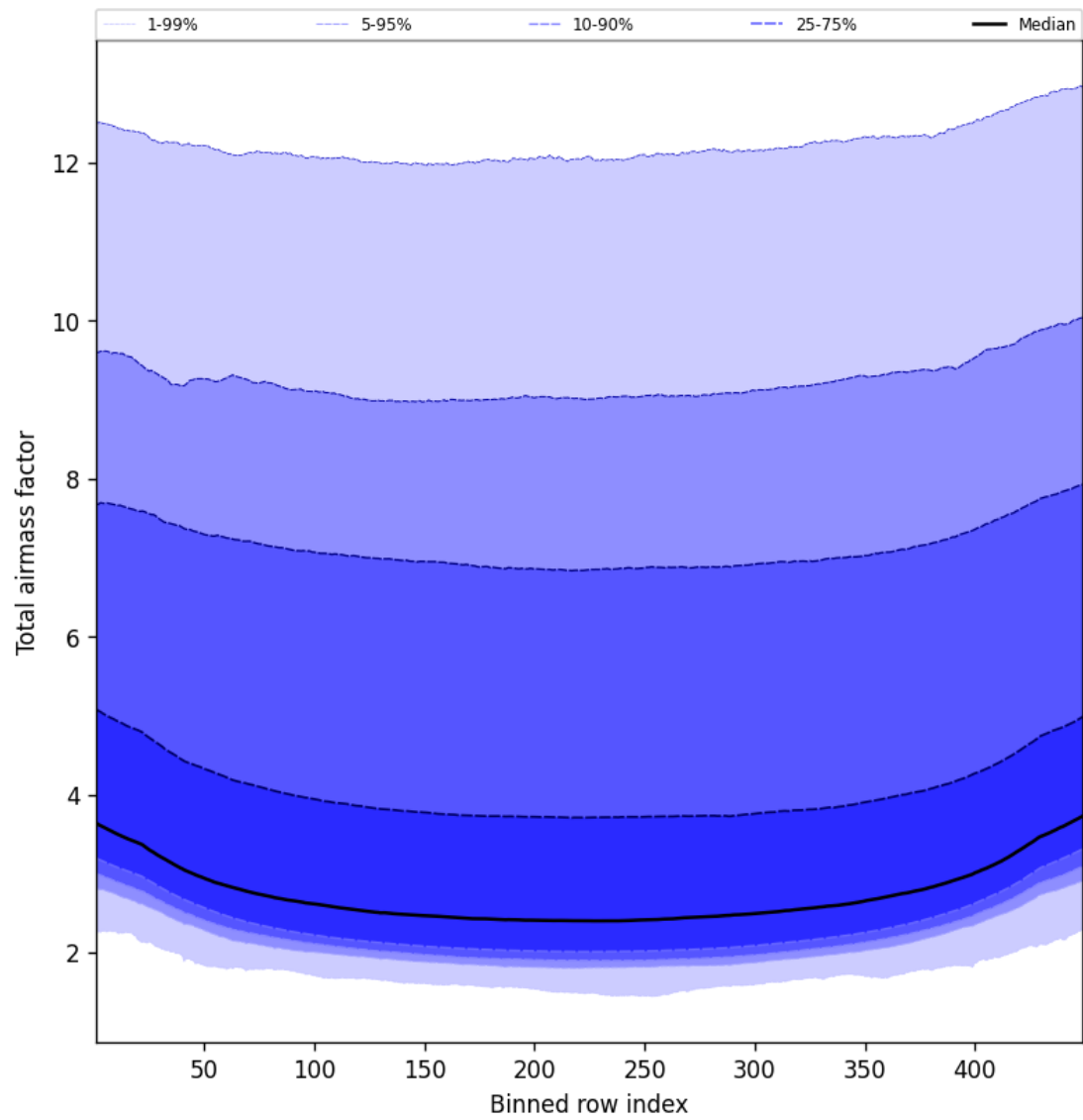
Figure 47: Along track statistics of “Total airmass factor” for 2025-08-18 to 2025-08-19
