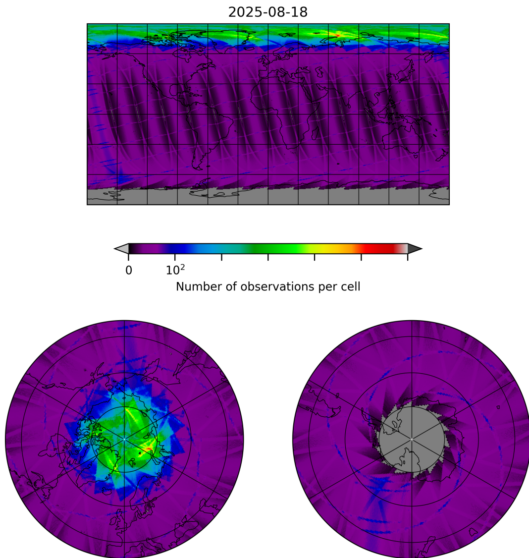
Figure 8: Map of the number of observations for 2025-08-18 to 2025-08-19
