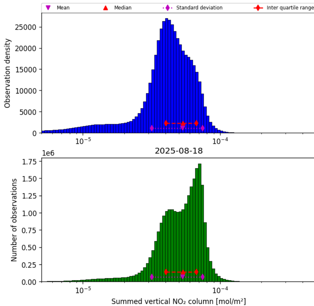
Figure 38: Histogram of “Summed vertical NO 2 column” for 2025-08-18 to 2025-08-19
