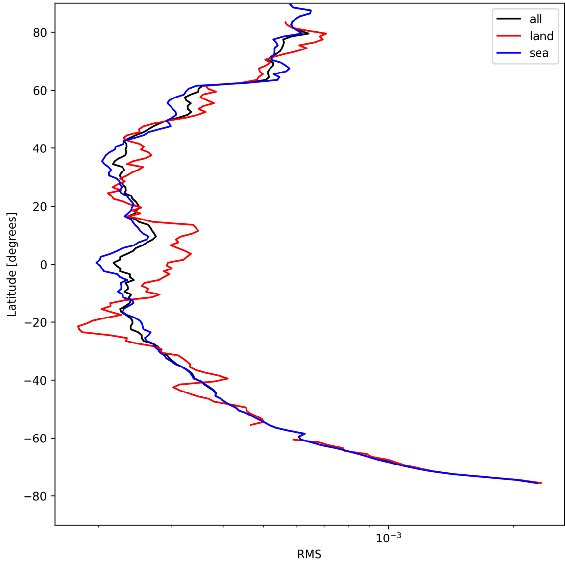
Figure 24: Zonal average of “RMS” for 2025-08-18 to 2025-08-19.
