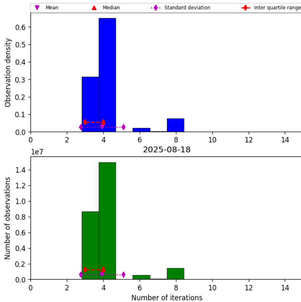
Figure 32: Histogram of “Number of iterations” for 2025-08-18 to 2025-08-19
