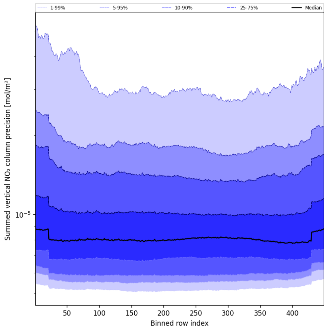
Figure 56: Along track statistics of “Summed vertical NO 2 column precision” for 2025-08-18 to 2025-08-19
