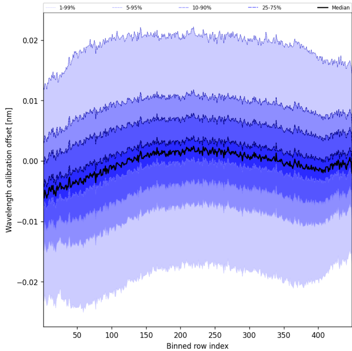
Figure 50: Along track statistics of “Wavelength calibration offset” for 2025-08-18 to 2025-08-19
