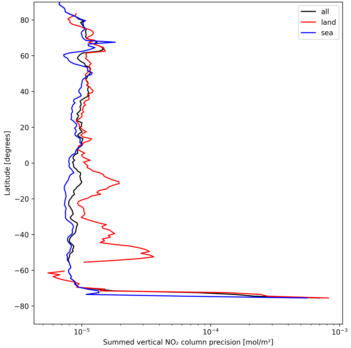
Figure 22: Zonal average of “Summed vertical NO 2 column precision” for 2025-08-18 to 2025-08-19.
