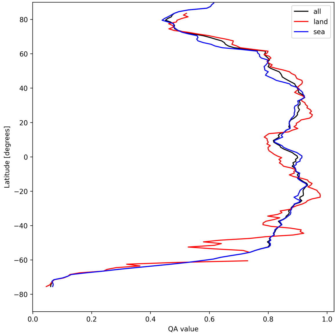
Figure 9: Zonal average of “QA value” for 2025-08-18 to 2025-08-19.
