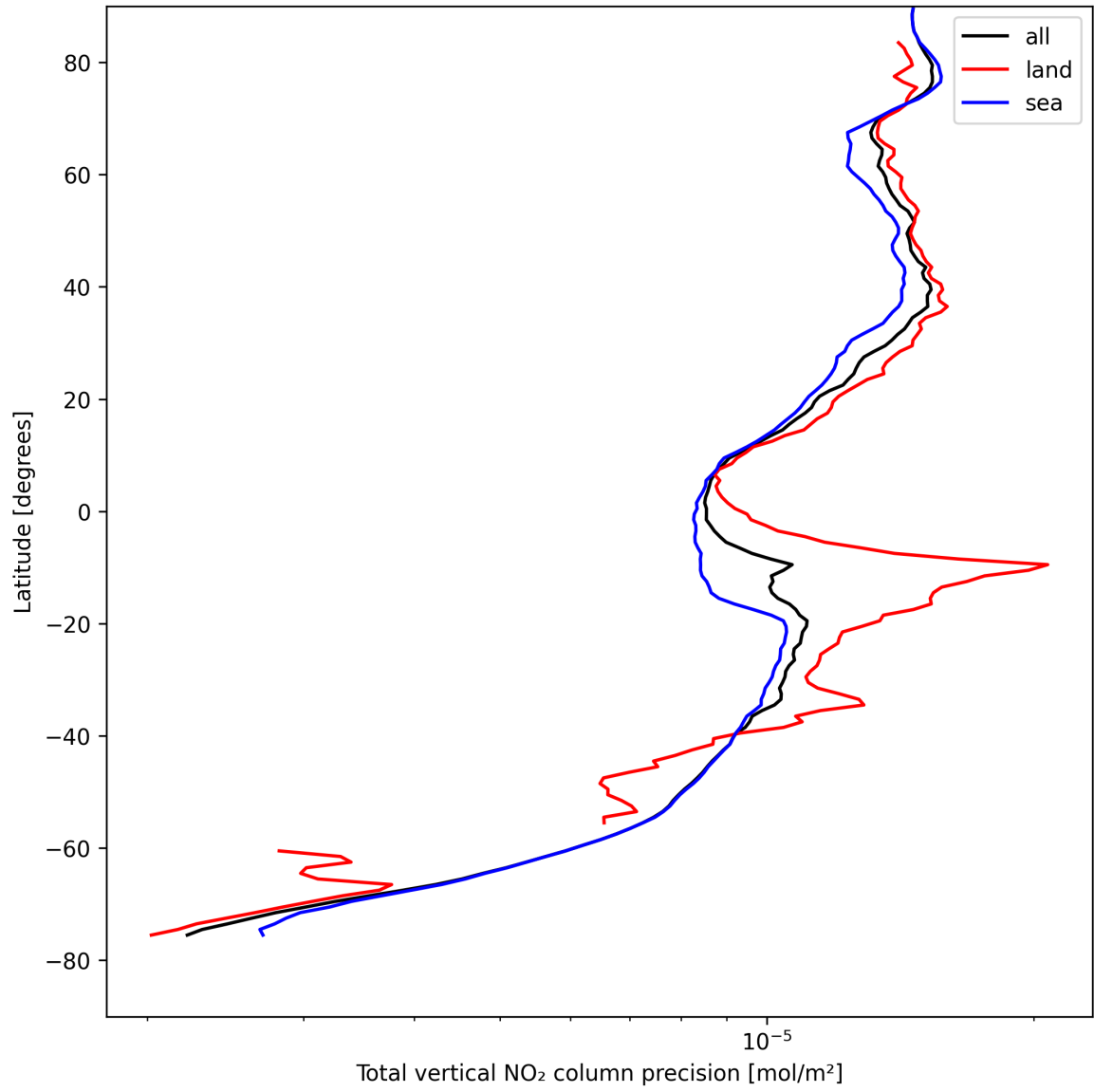
Figure 20: Zonal average of “Total vertical NO 2 column precision” for 2025-08-19 to 2025-08-20.
