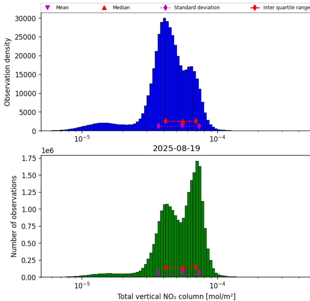
Figure 36: Histogram of “Total vertical NO 2 column” for 2025-08-19 to 2025-08-20
