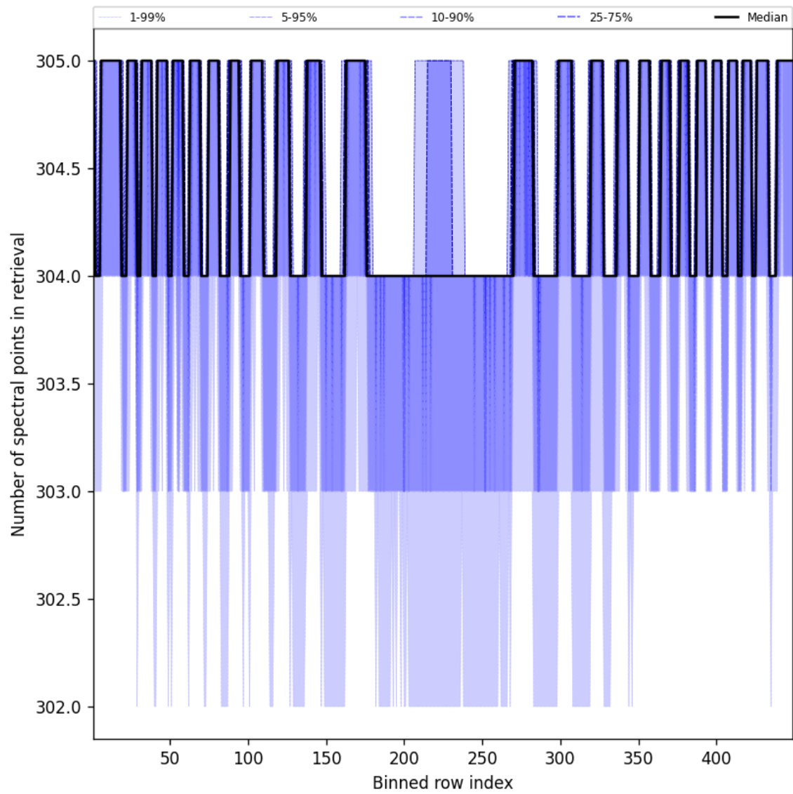
Figure 48: Along track statistics of “Number of spectral points in retrieval” for 2025-08-19 to 2025-08-20
