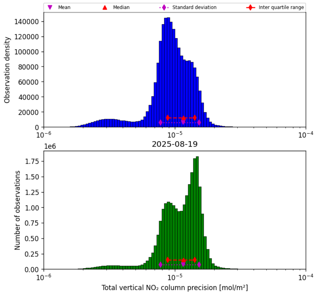
Figure 37: Histogram of “Total vertical NO 2 column precision” for 2025-08-19 to 2025-08-20
