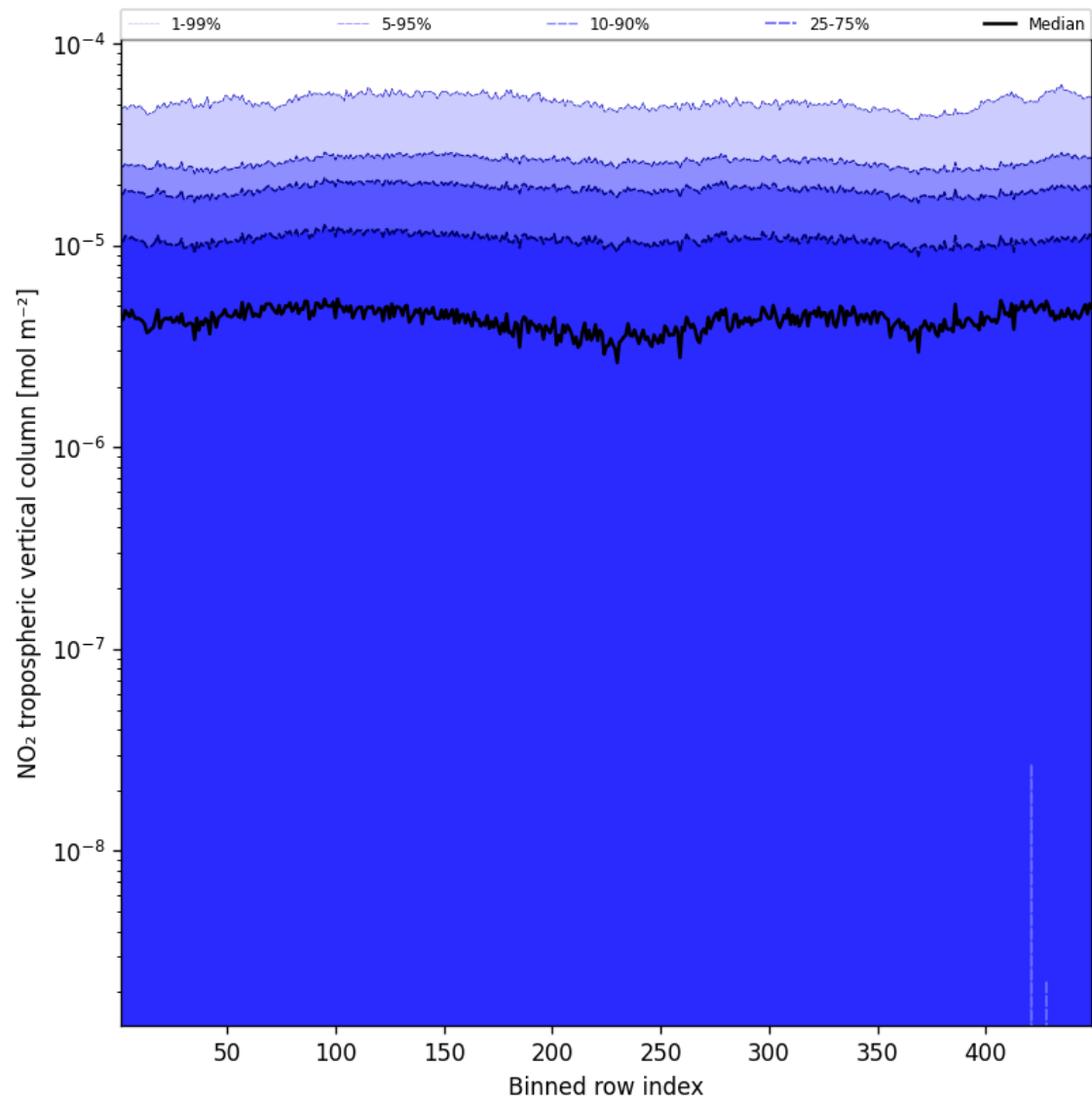
Figure 44: Along track statistics of “NO 2 tropospheric vertical column” for 2025-08-19 to 2025-08-20
