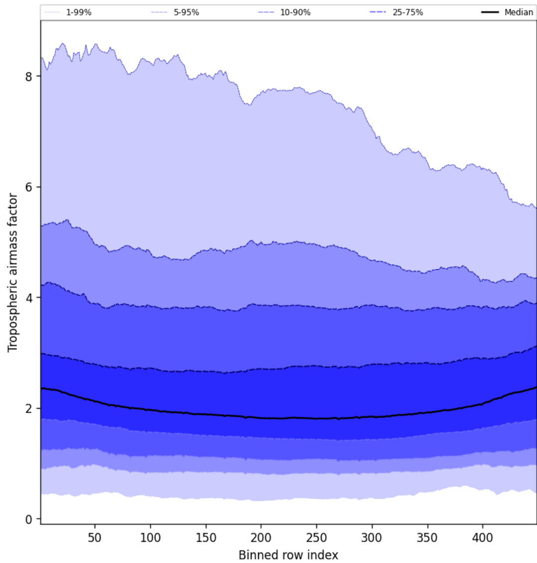
Figure 46: Along track statistics of “Tropospheric airmass factor” for 2025-08-19 to 2025-08-20
