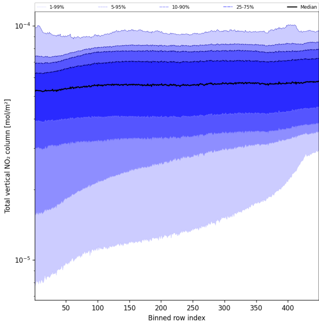
Figure 53: Along track statistics of “Total vertical NO 2 column” for 2025-08-19 to 2025-08-20
