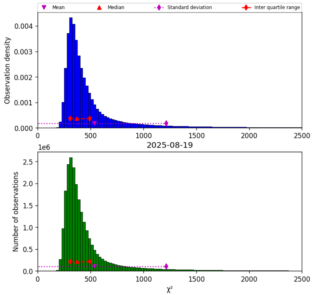
Figure 40: Histogram of “ \chi^2 ” for 2025-08-19 to 2025-08-20
