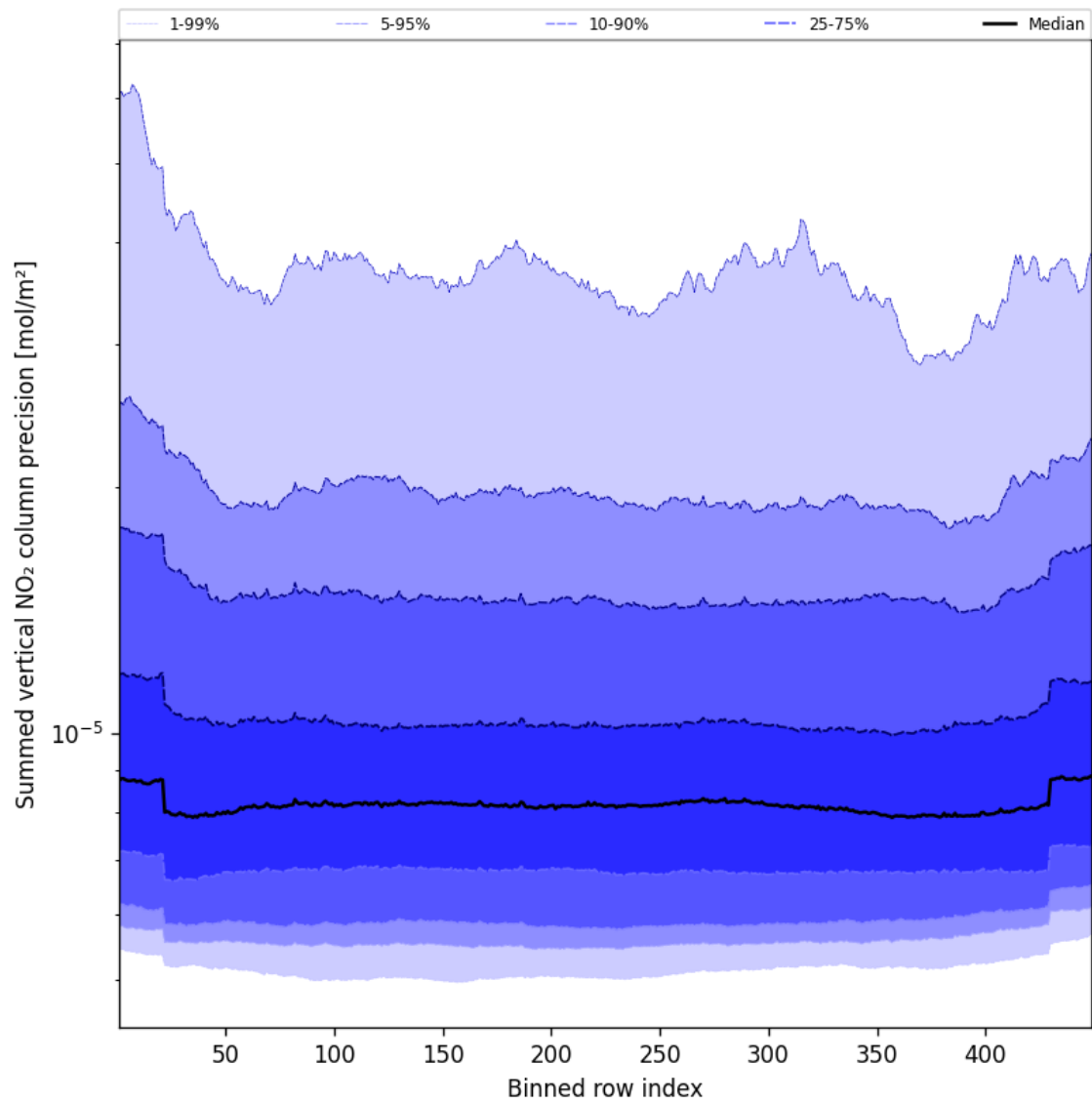
Figure 56: Along track statistics of “Summed vertical NO 2 column precision” for 2025-08-19 to 2025-08-20
