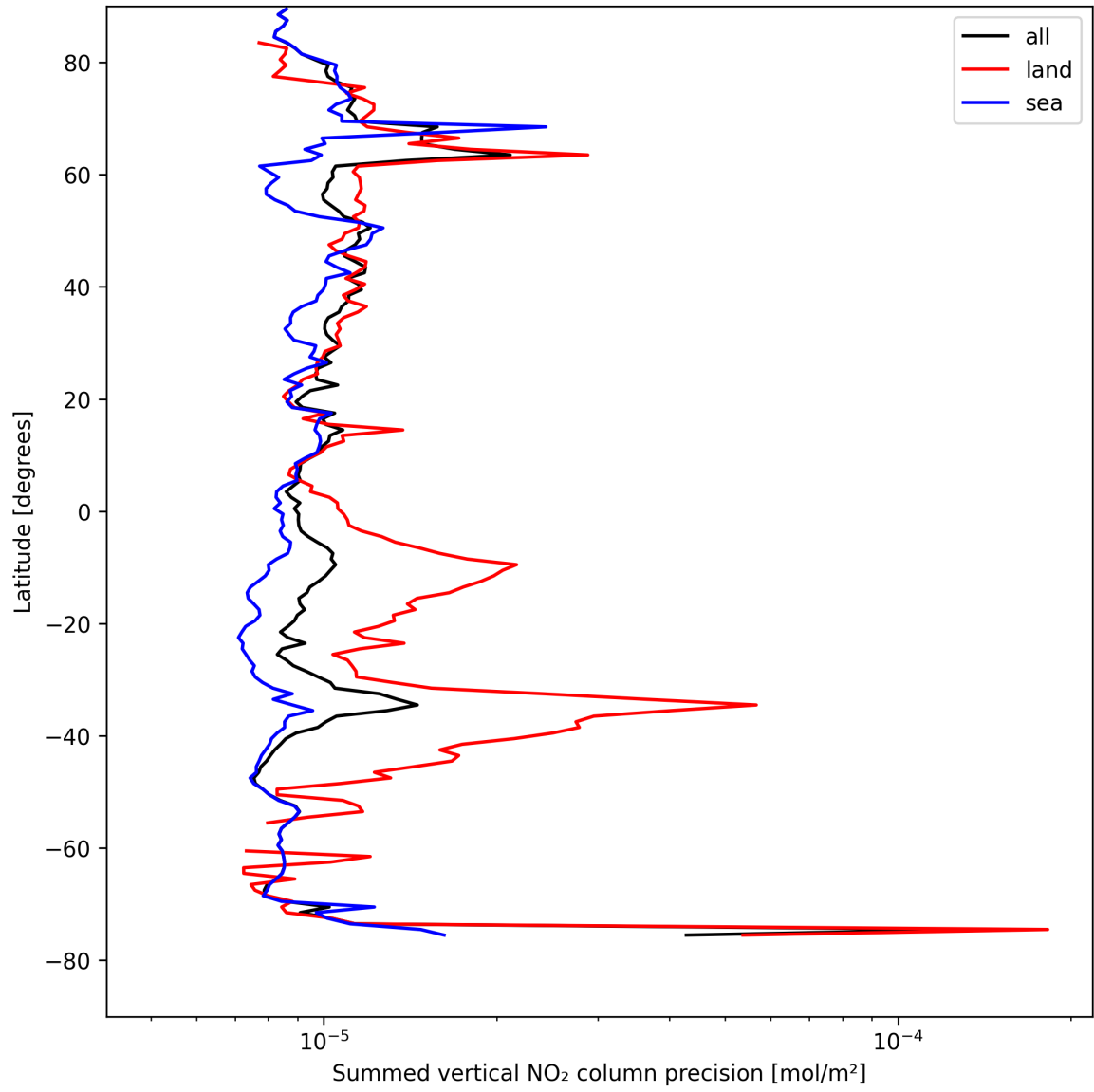
Figure 22: Zonal average of “Summed vertical NO 2 column precision” for 2025-08-19 to 2025-08-20.
