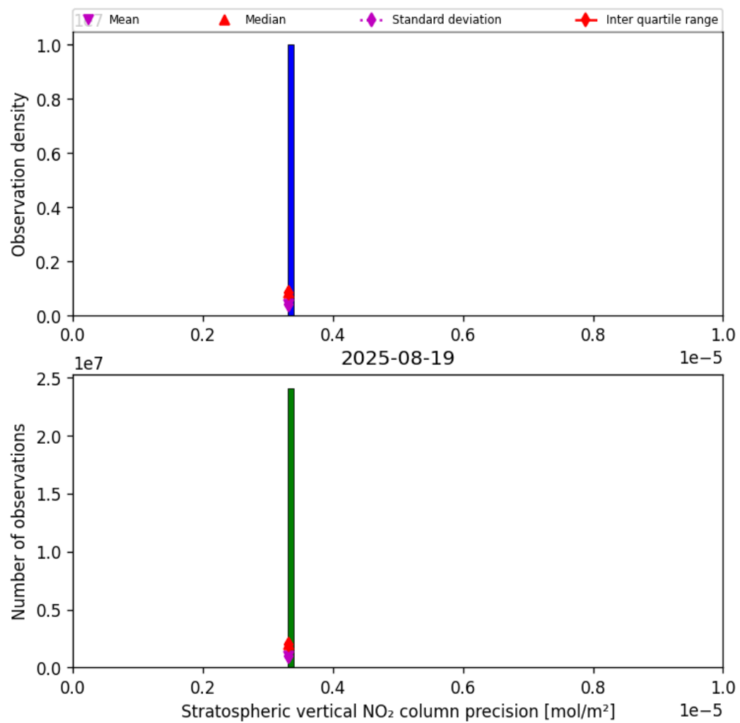
Figure 35: Histogram of “Stratospheric vertical NO 2 column precision” for 2025-08-19 to 2025-08-20
