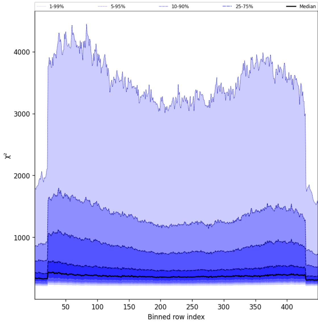
Figure 57: Along track statistics of “ \chi^2 ” for 2025-08-19 to 2025-08-20
