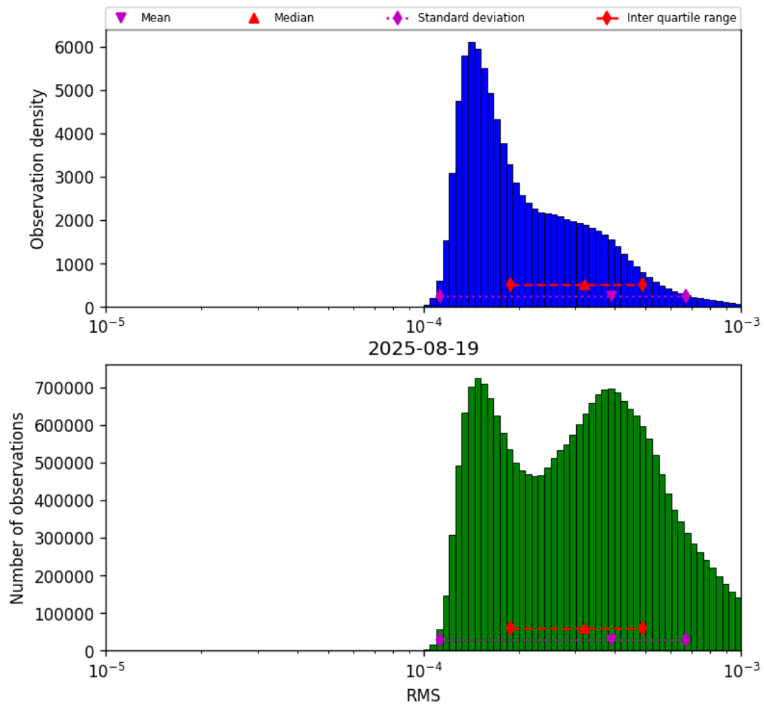
Figure 41: Histogram of “RMS” for 2025-08-19 to 2025-08-20
