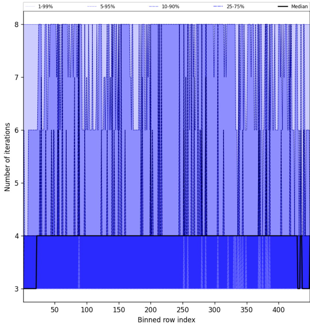
Figure 49: Along track statistics of “Number of iterations” for 2025-08-19 to 2025-08-20
