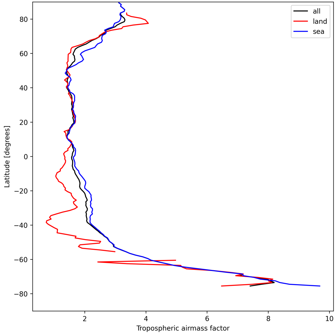
Figure 12: Zonal average of “Tropospheric airmass factor” for 2025-08-19 to 2025-08-20.
