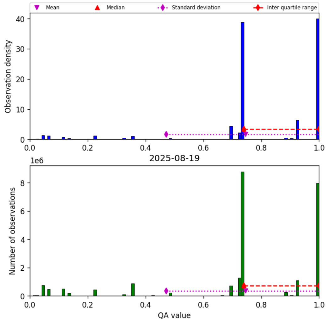
Figure 26: Histogram of “QA value” for 2025-08-19 to 2025-08-20
