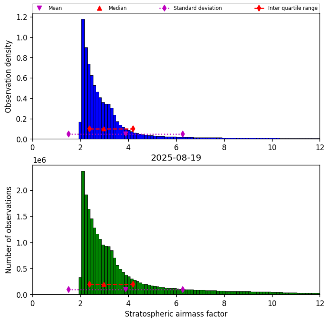
Figure 42: Histogram of “Stratospheric airmass factor” for 2025-08-19 to 2025-08-20
