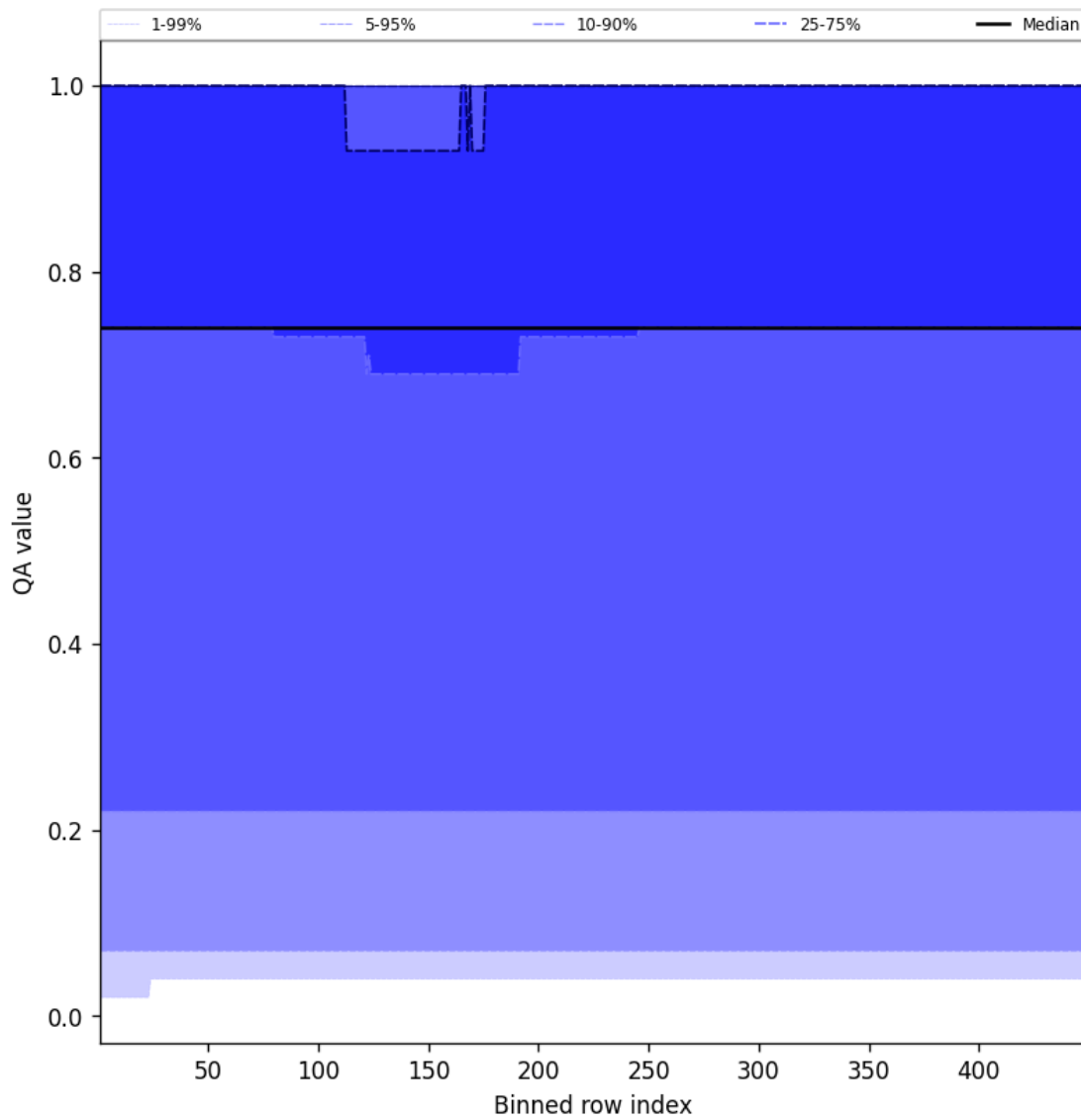
Figure 43: Along track statistics of “QA value” for 2025-08-19 to 2025-08-20
