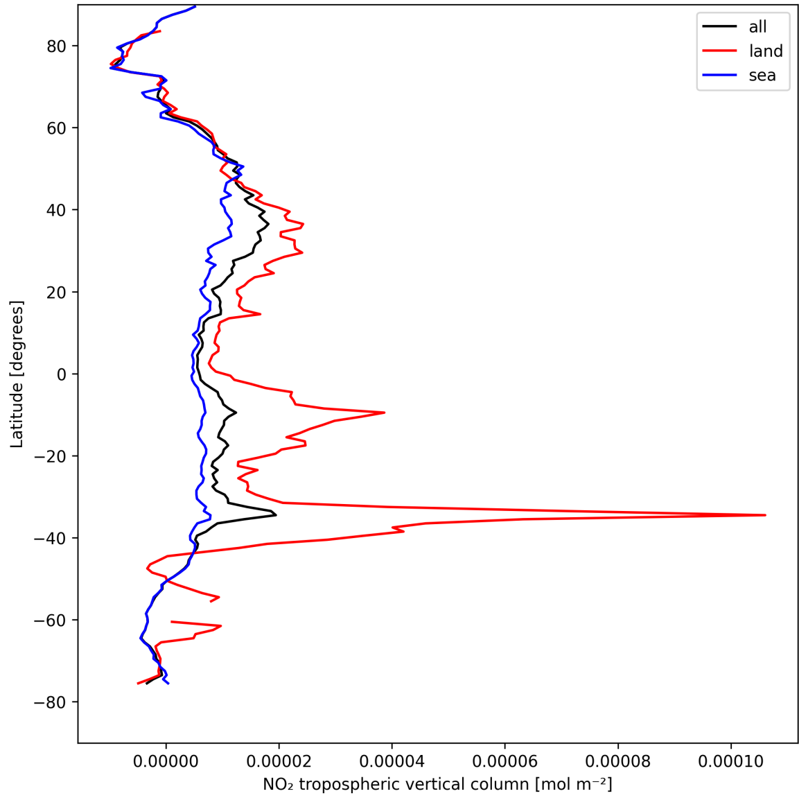
Figure 10: Zonal average of “NO 2 tropospheric vertical column” for 2025-08-19 to 2025-08-20.
