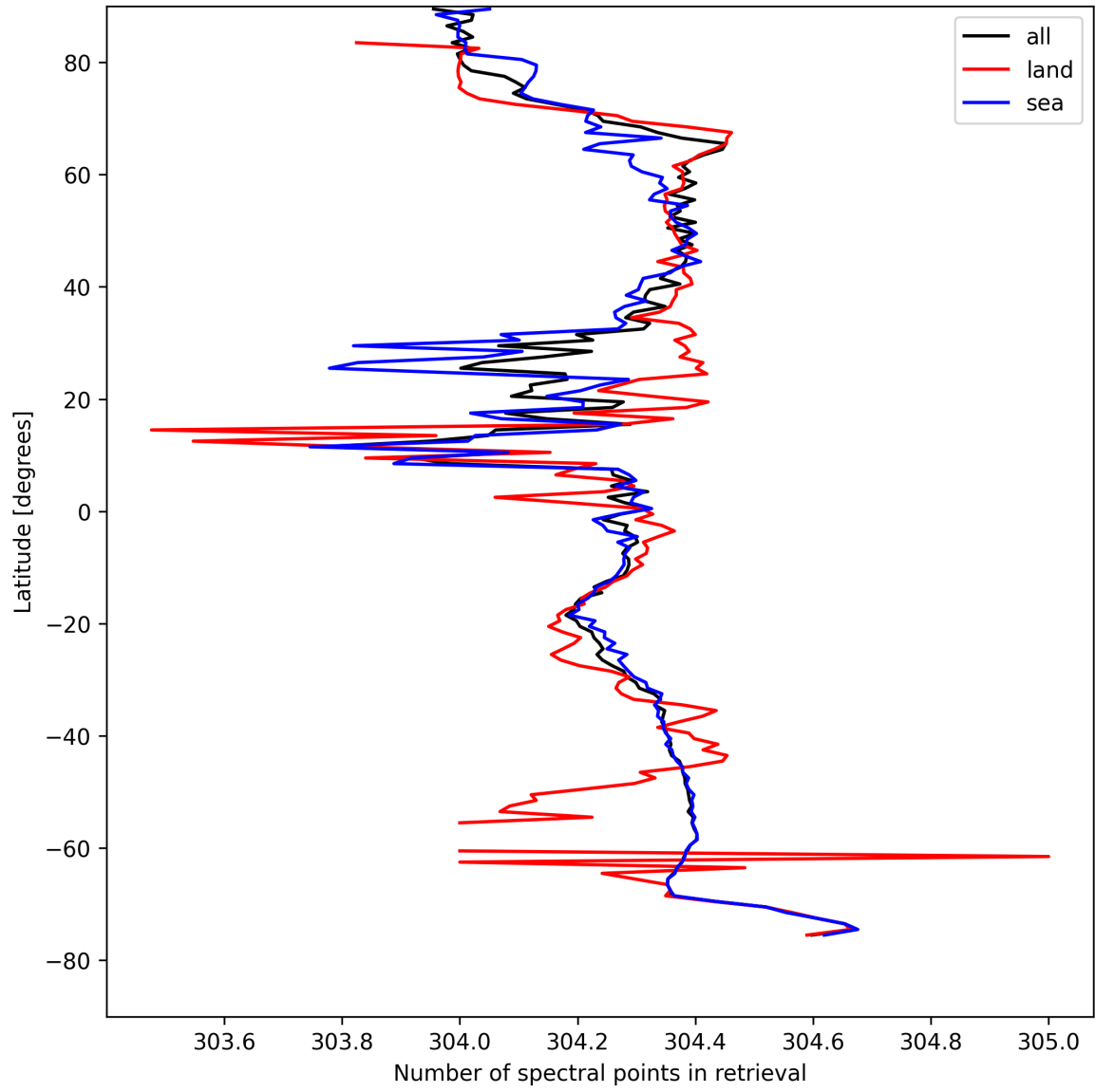
Figure 14: Zonal average of “Number of spectral points in retrieval” for 2025-08-19 to 2025-08-20.
