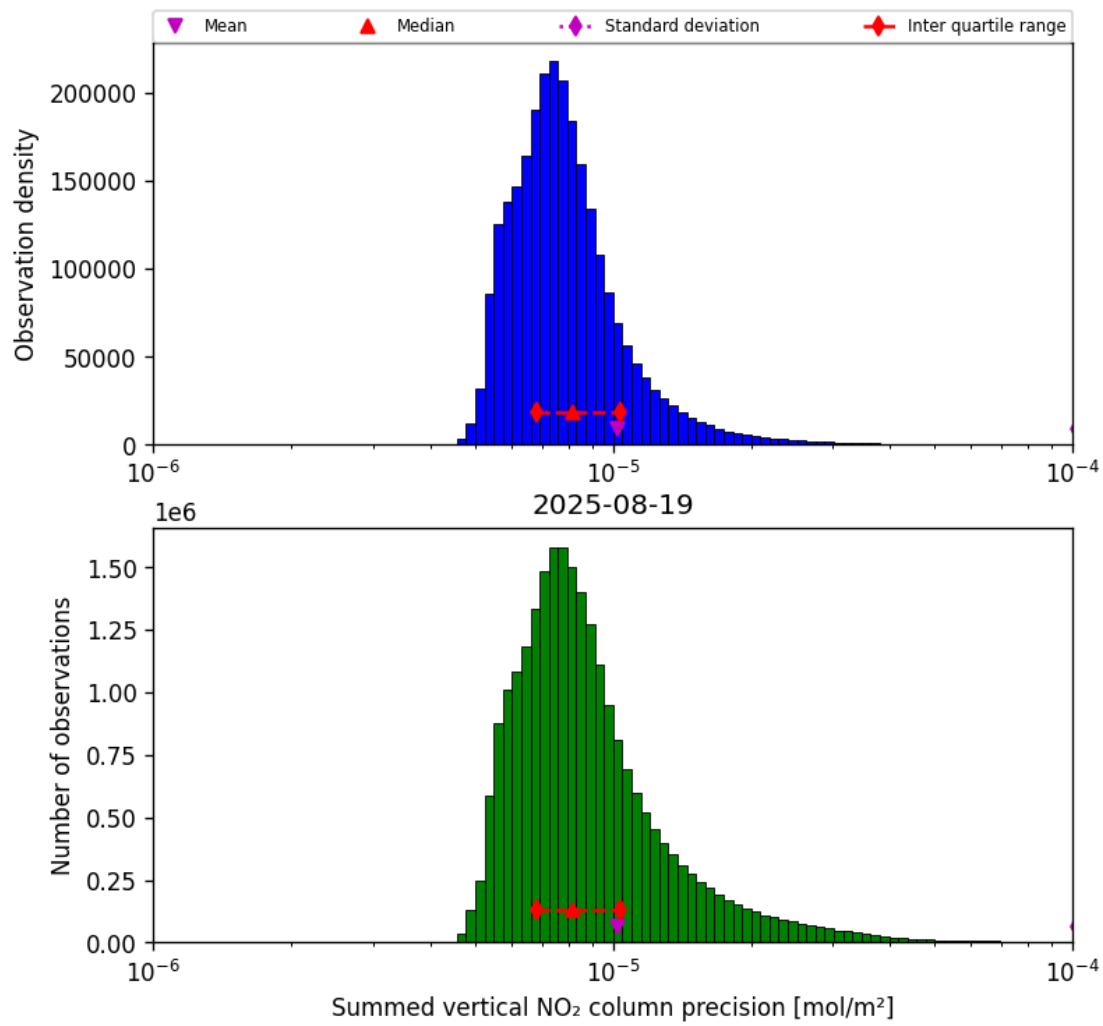
Figure 39: Histogram of “Summed vertical NO 2 column precision” for 2025-08-19 to 2025-08-20
