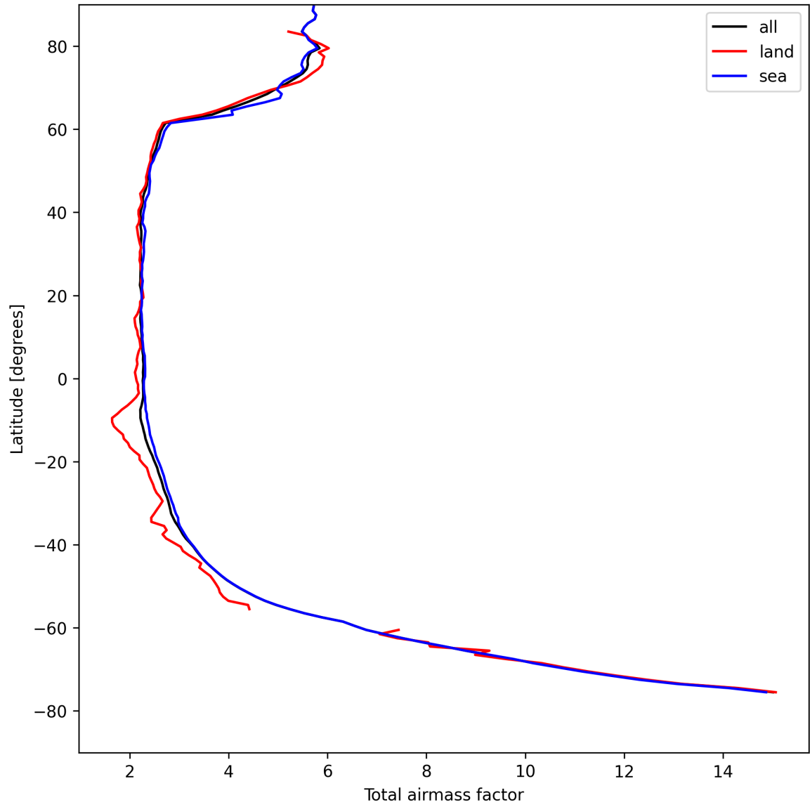
Figure 13: Zonal average of “Total airmass factor” for 2025-08-19 to 2025-08-20.
