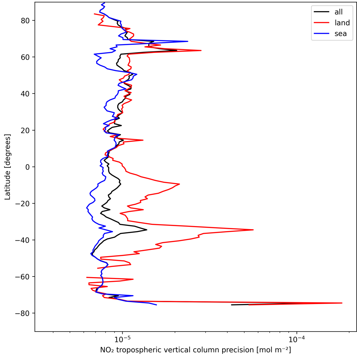
Figure 11: Zonal average of "NO 2 tropospheric vertical column precision" for 2025-08-19 to 2025-08-20.
