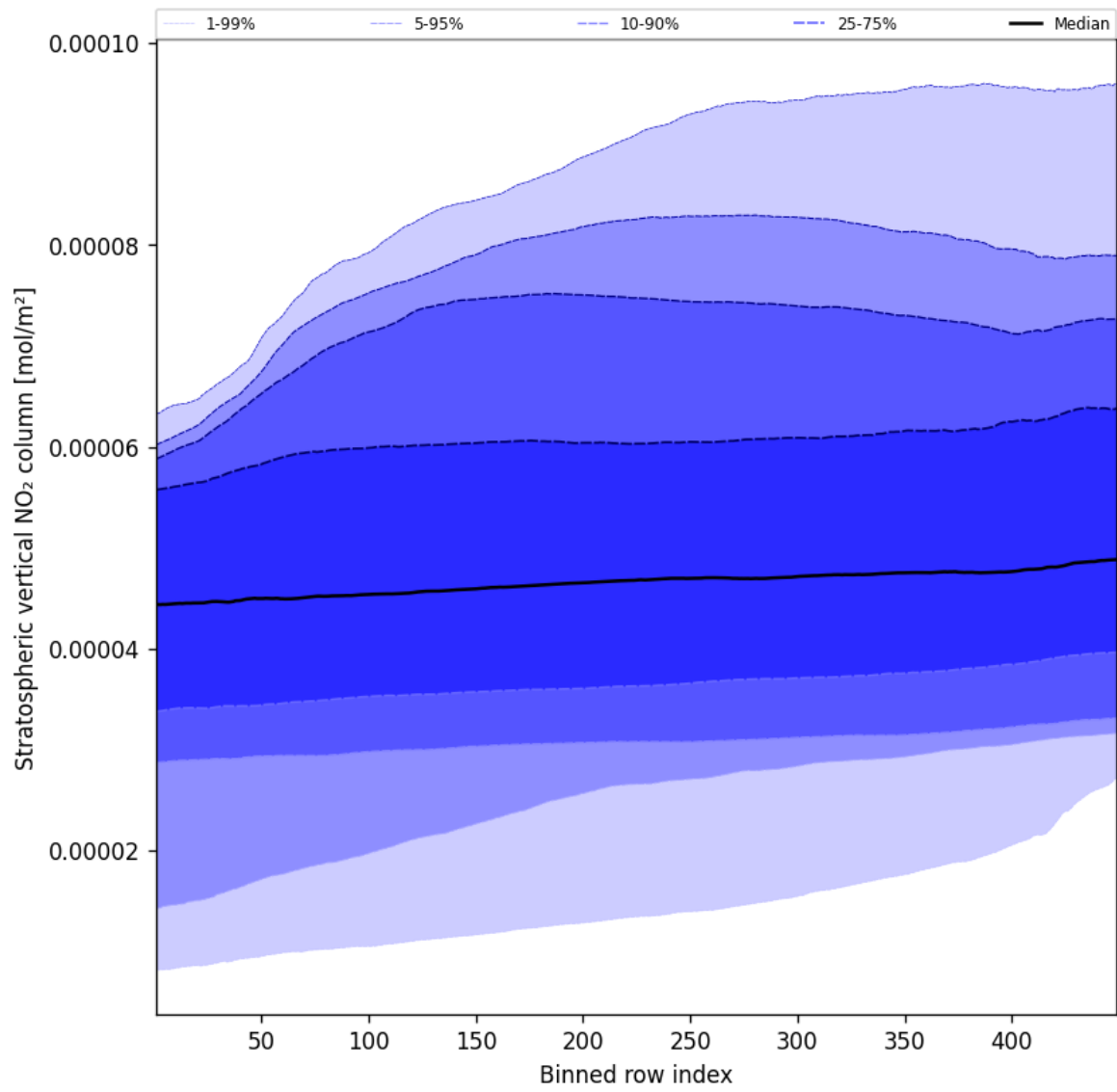
Figure 51: Along track statistics of “Stratospheric vertical NO 2 column” for 2025-08-19 to 2025-08-20
