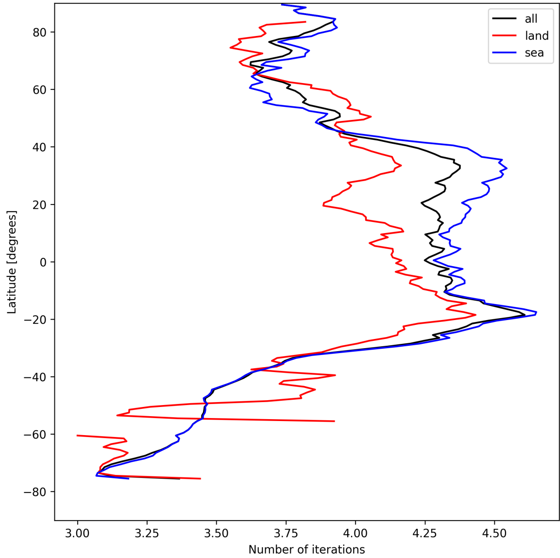
Figure 15: Zonal average of “Number of iterations” for 2025-08-19 to 2025-08-20.
