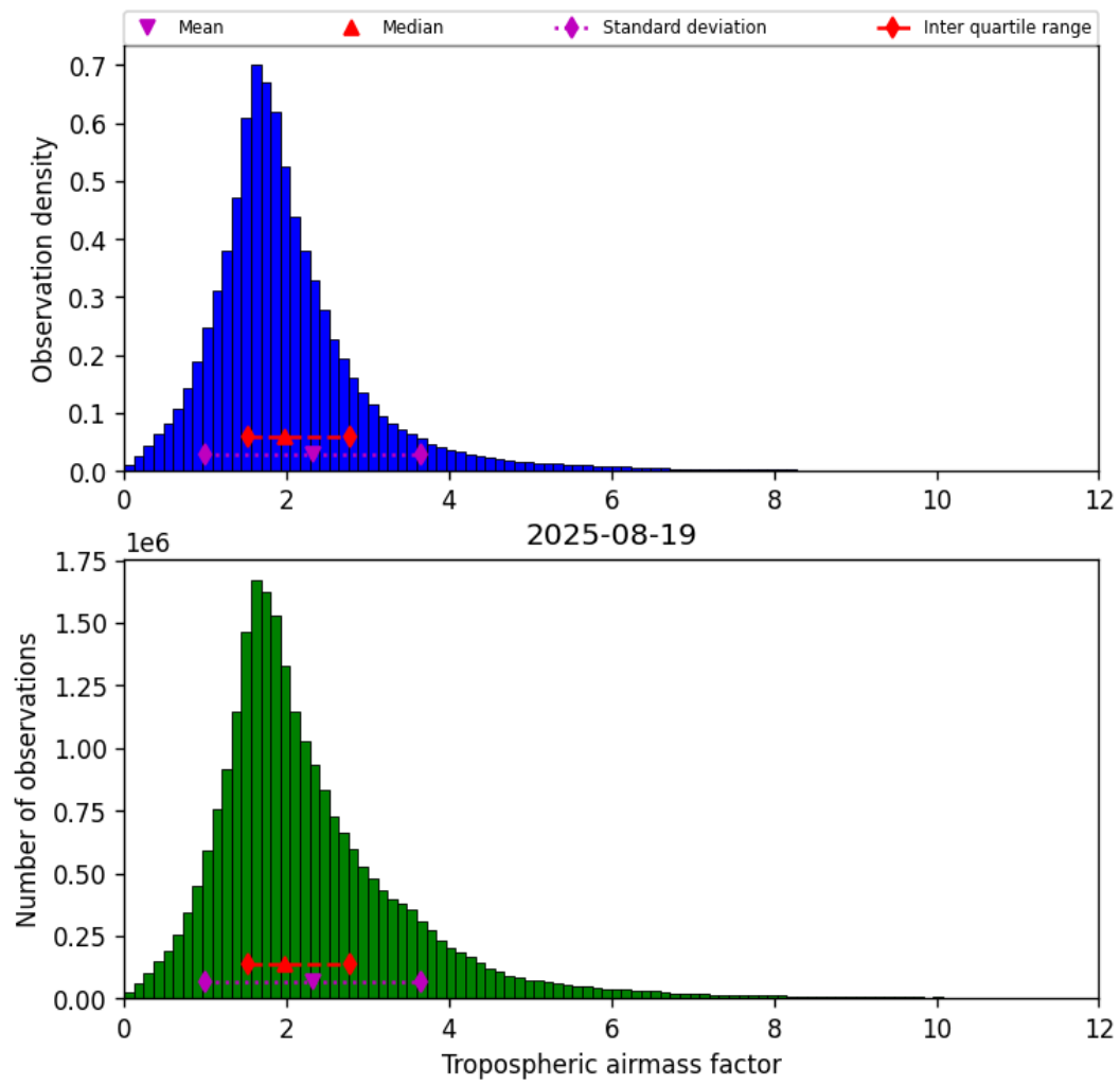
Figure 29: Histogram of “Tropospheric airmass factor” for 2025-08-19 to 2025-08-20
