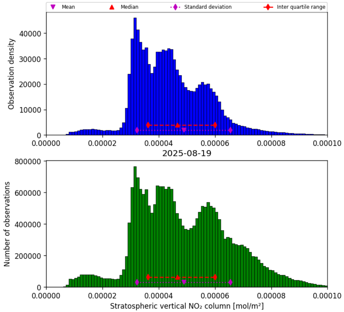
Figure 34: Histogram of “Stratospheric vertical NO 2 column” for 2025-08-19 to 2025-08-20
