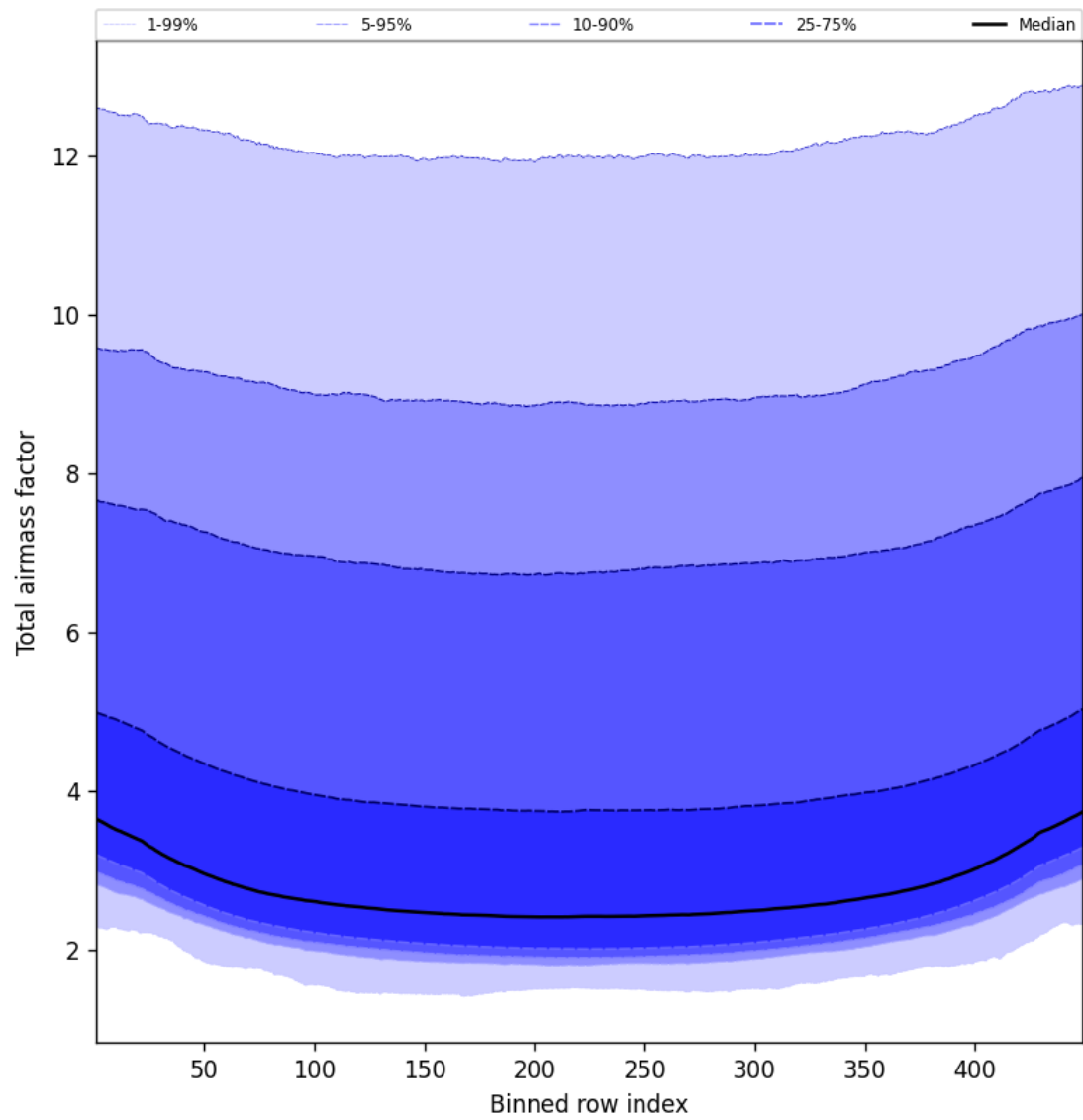
Figure 47: Along track statistics of “Total airmass factor” for 2025-08-19 to 2025-08-20
