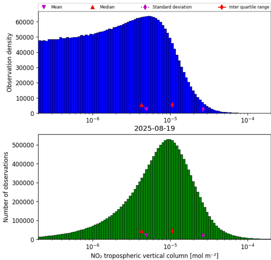
Figure 27: Histogram of “NO 2 tropospheric vertical column” for 2025-08-19 to 2025-08-20
