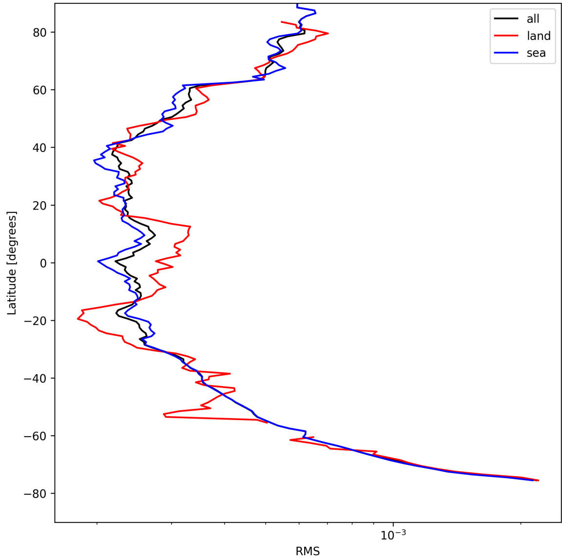
Figure 24: Zonal average of “RMS” for 2025-08-19 to 2025-08-20.
