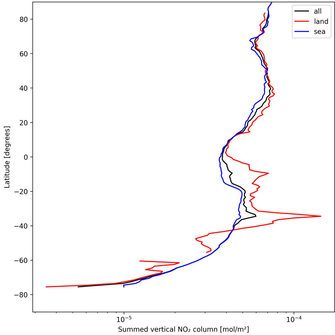
Figure 21: Zonal average of “Summed vertical NO 2 column” for 2025-08-19 to 2025-08-20.
