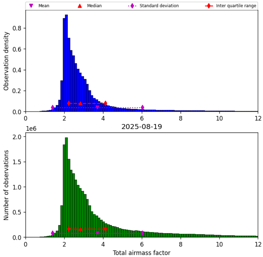
Figure 30: Histogram of “Total airmass factor” for 2025-08-19 to 2025-08-20
