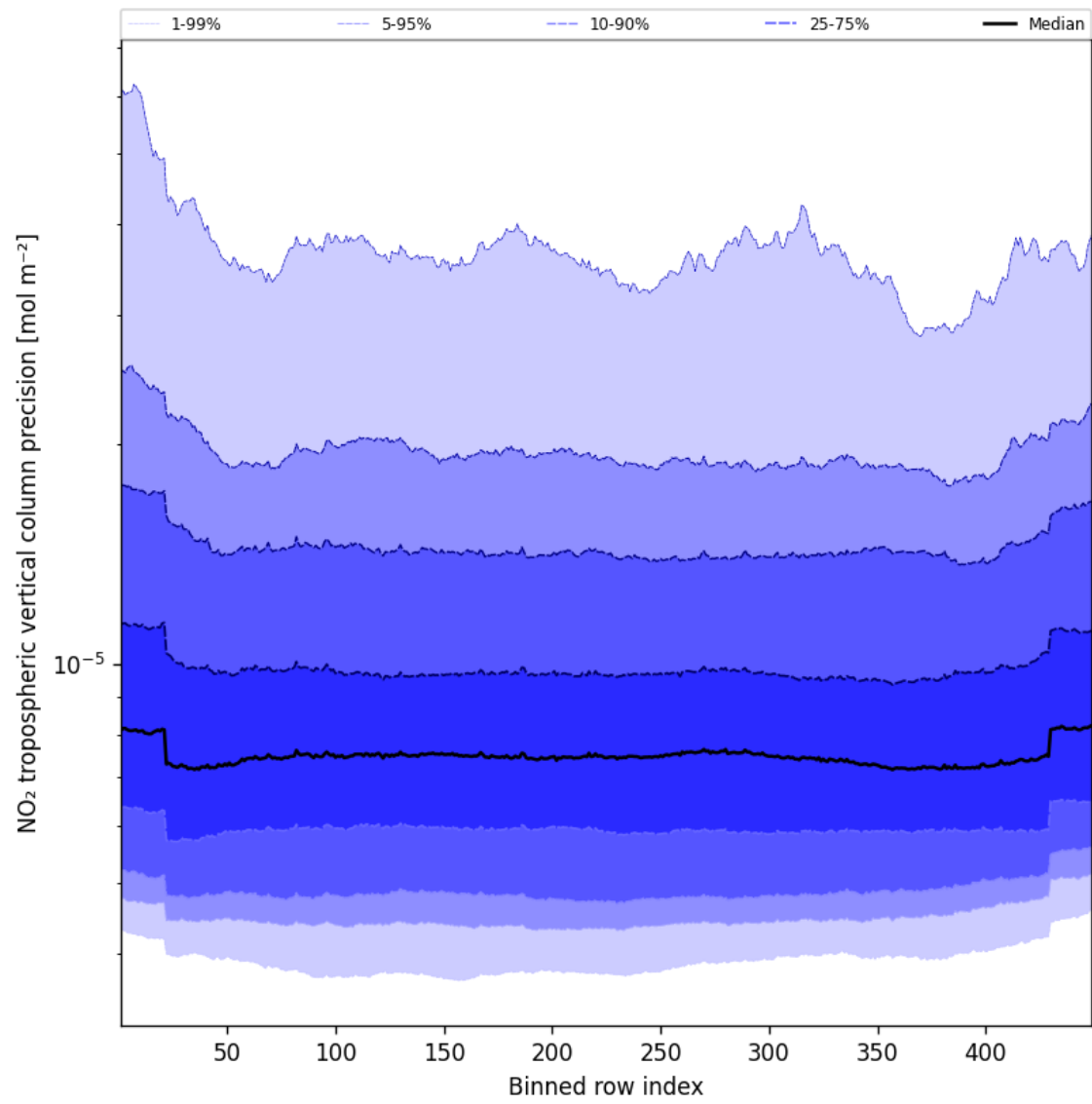
Figure 45: Along track statistics of “NO 2 tropospheric vertical column precision” for 2025-08-19 to 2025-08-20
