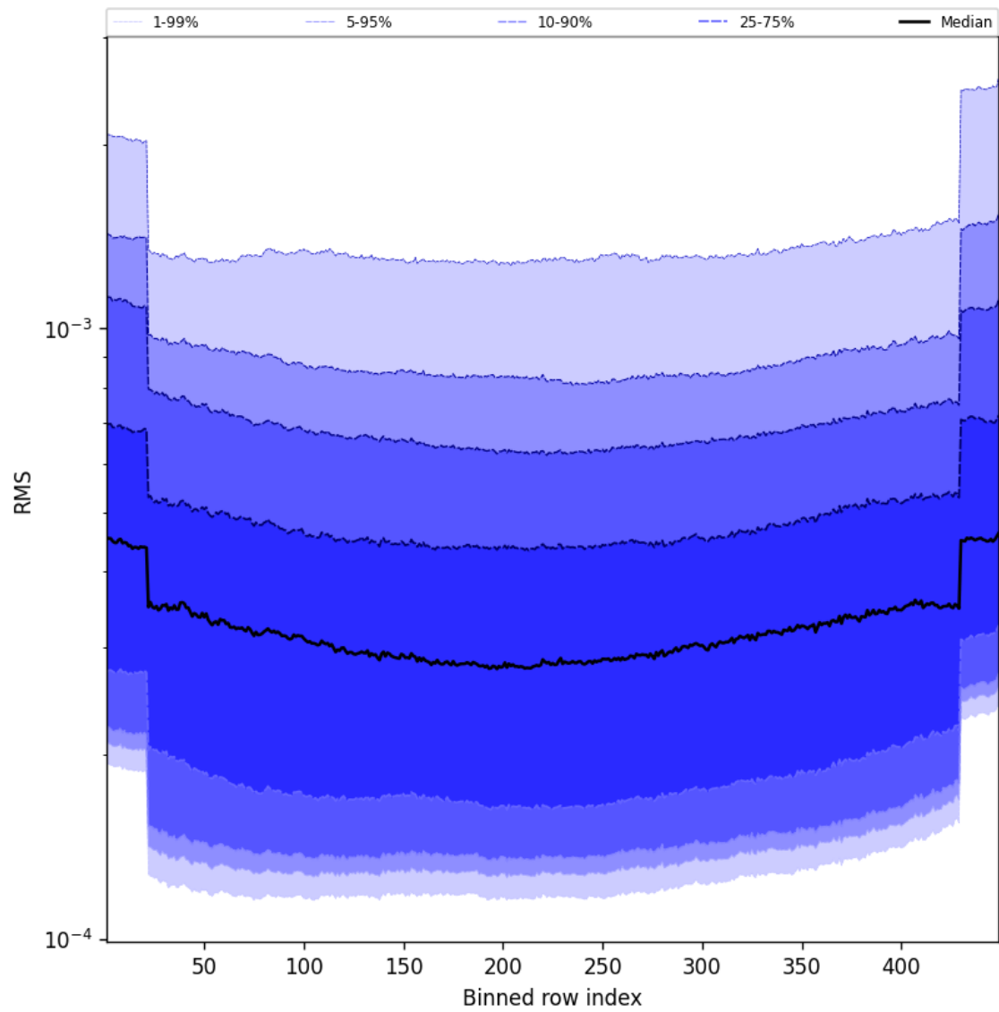
Figure 58: Along track statistics of “RMS” for 2025-08-19 to 2025-08-20
