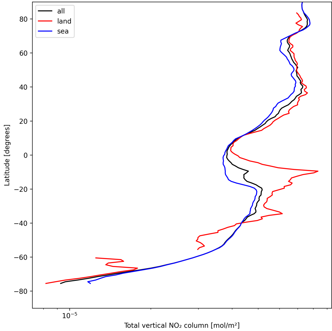
Figure 19: Zonal average of “Total vertical NO 2 column” for 2025-08-19 to 2025-08-20.
