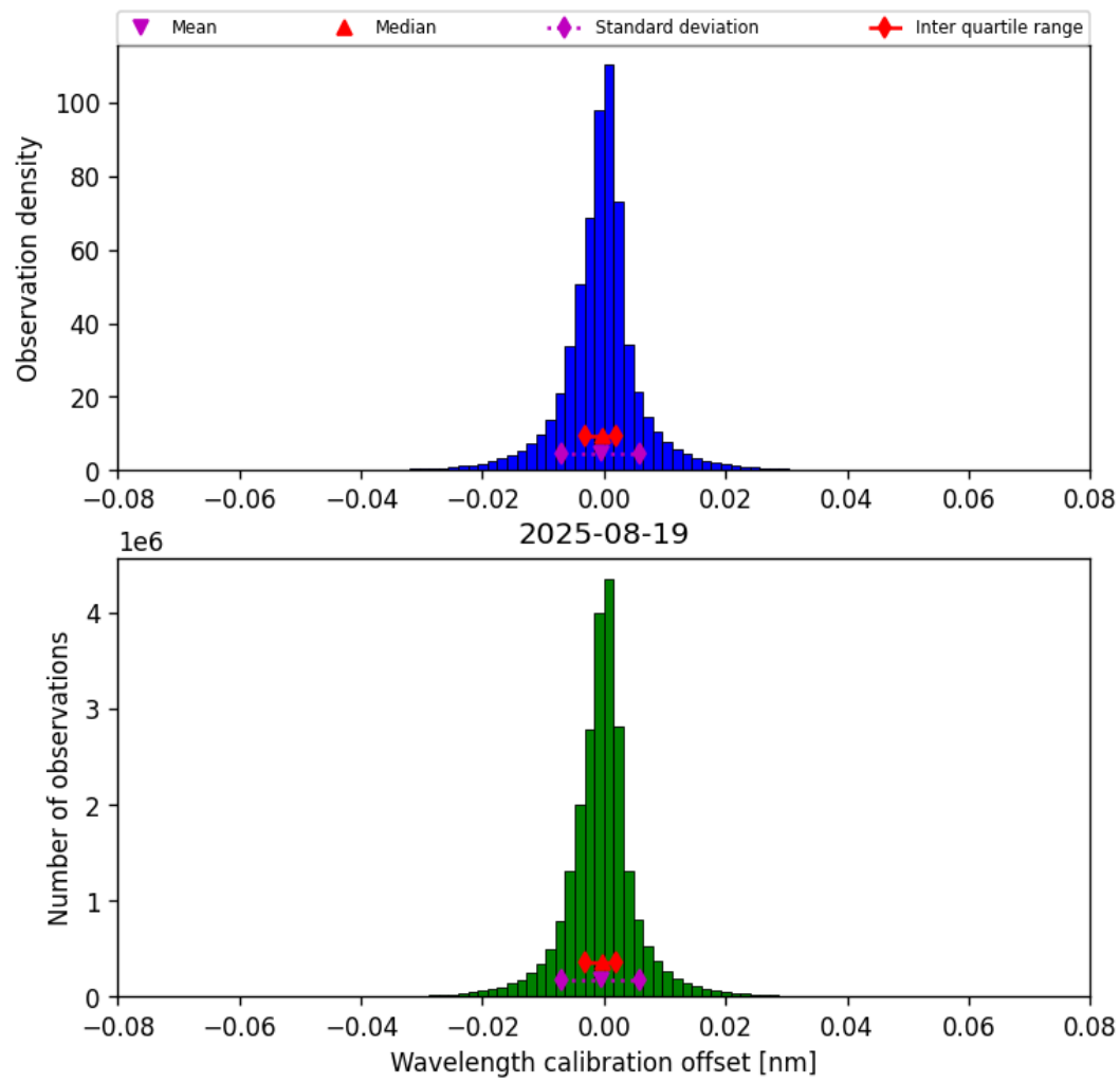
Figure 33: Histogram of “Wavelength calibration offset” for 2025-08-19 to 2025-08-20
