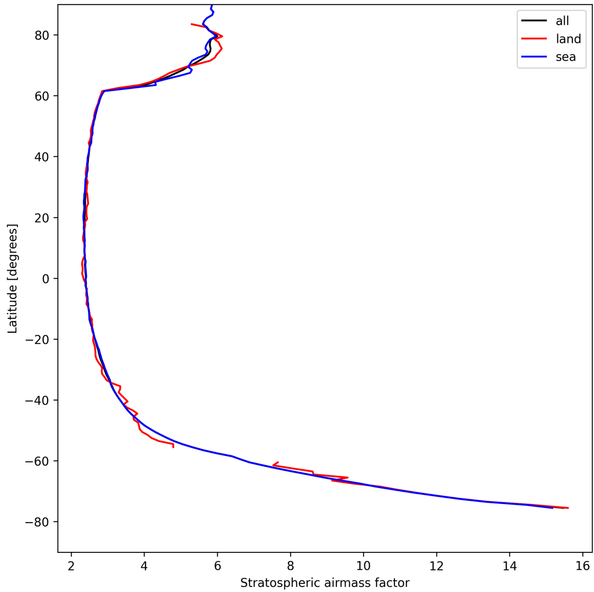
Figure 25: Zonal average of “Stratospheric airmass factor” for 2025-08-19 to 2025-08-20.
