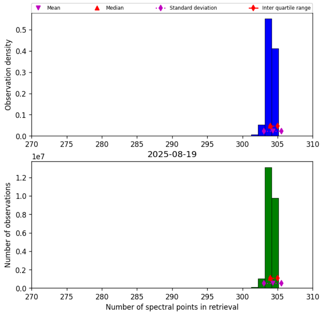
Figure 31: Histogram of “Number of spectral points in retrieval” for 2025-08-19 to 2025-08-20
