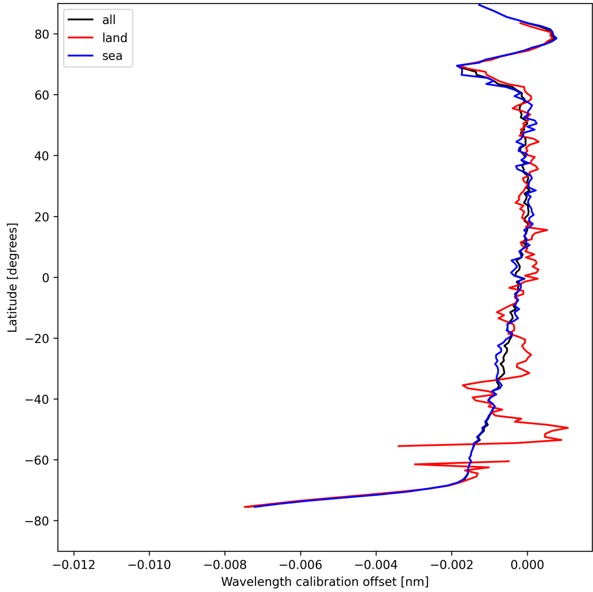
Figure 16: Zonal average of “Wavelength calibration offset” for 2025-08-19 to 2025-08-20.
