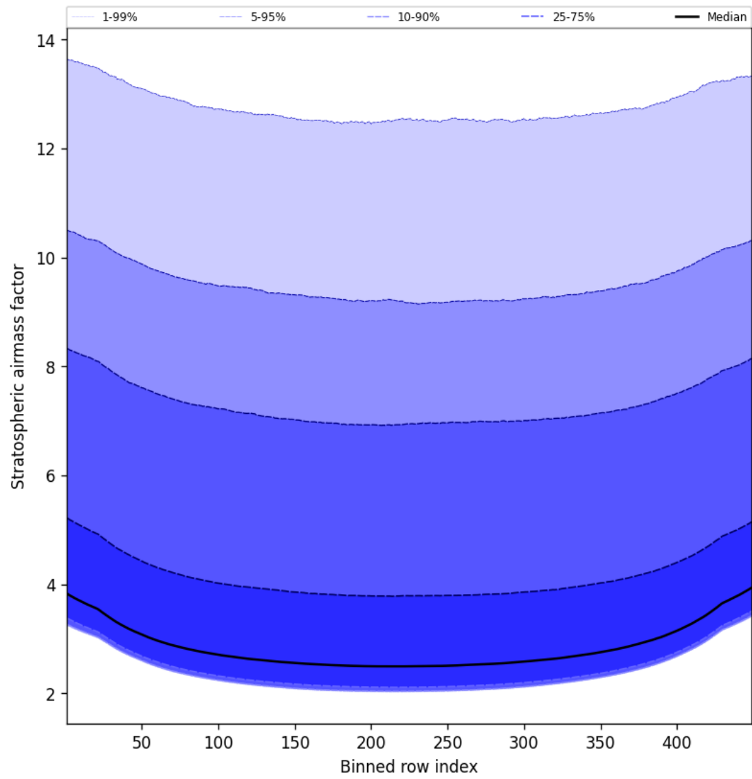
Figure 59: Along track statistics of “Stratospheric air mass factor” for 2025-08-19 to 2025-08-20
