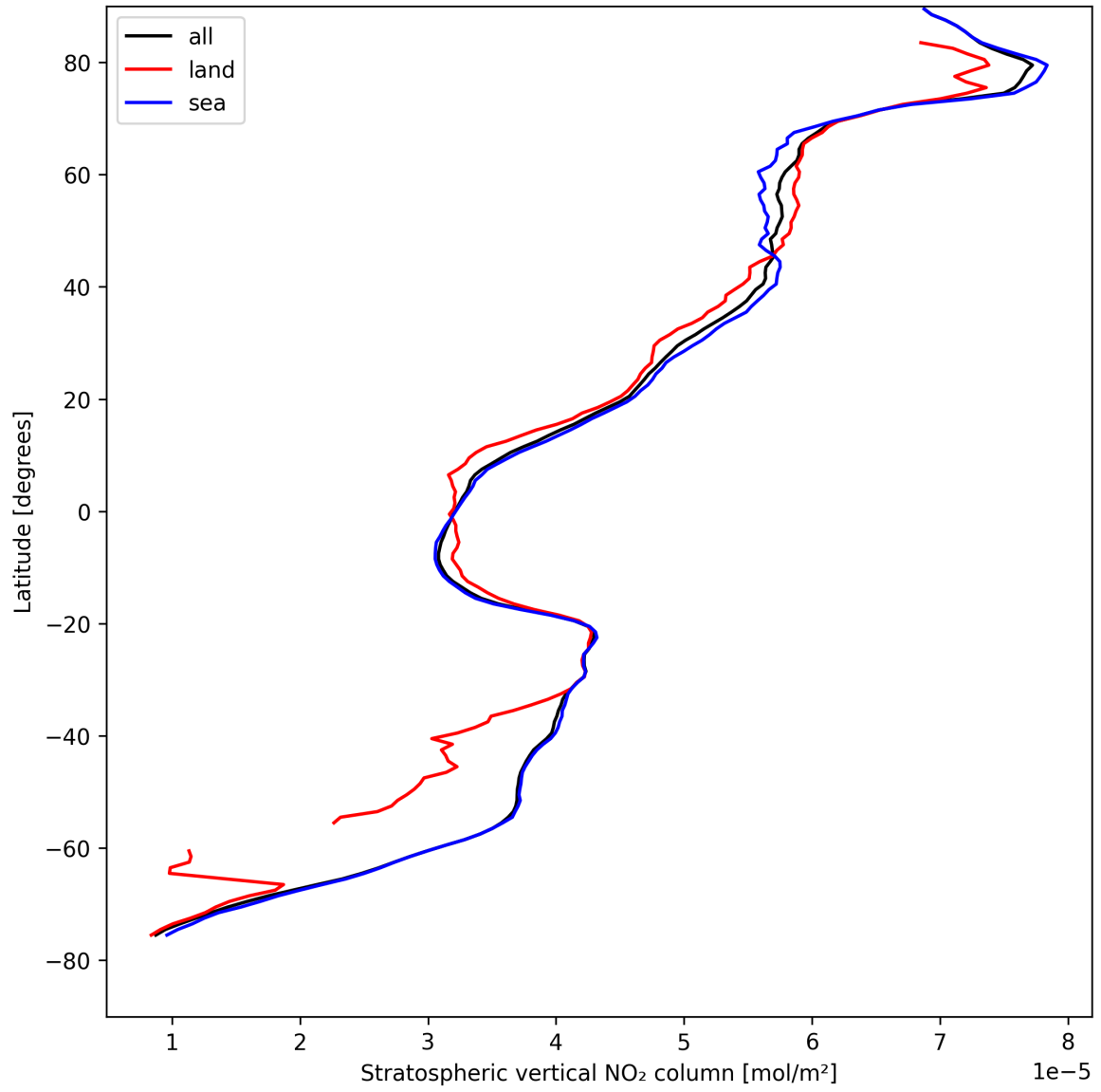
Figure 17: Zonal average of “Stratospheric vertical NO 2 column” for 2025-08-19 to 2025-08-20.
