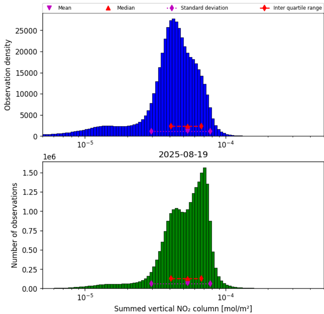
Figure 38: Histogram of “Summed vertical NO 2 column” for 2025-08-19 to 2025-08-20
