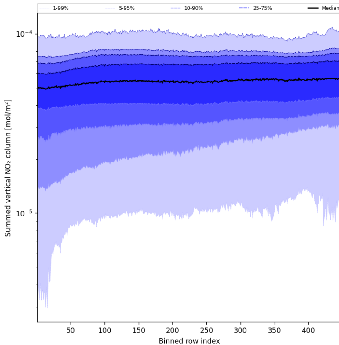
Figure 55: Along track statistics of “Summed vertical NO 2 column” for 2025-08-19 to 2025-08-20
