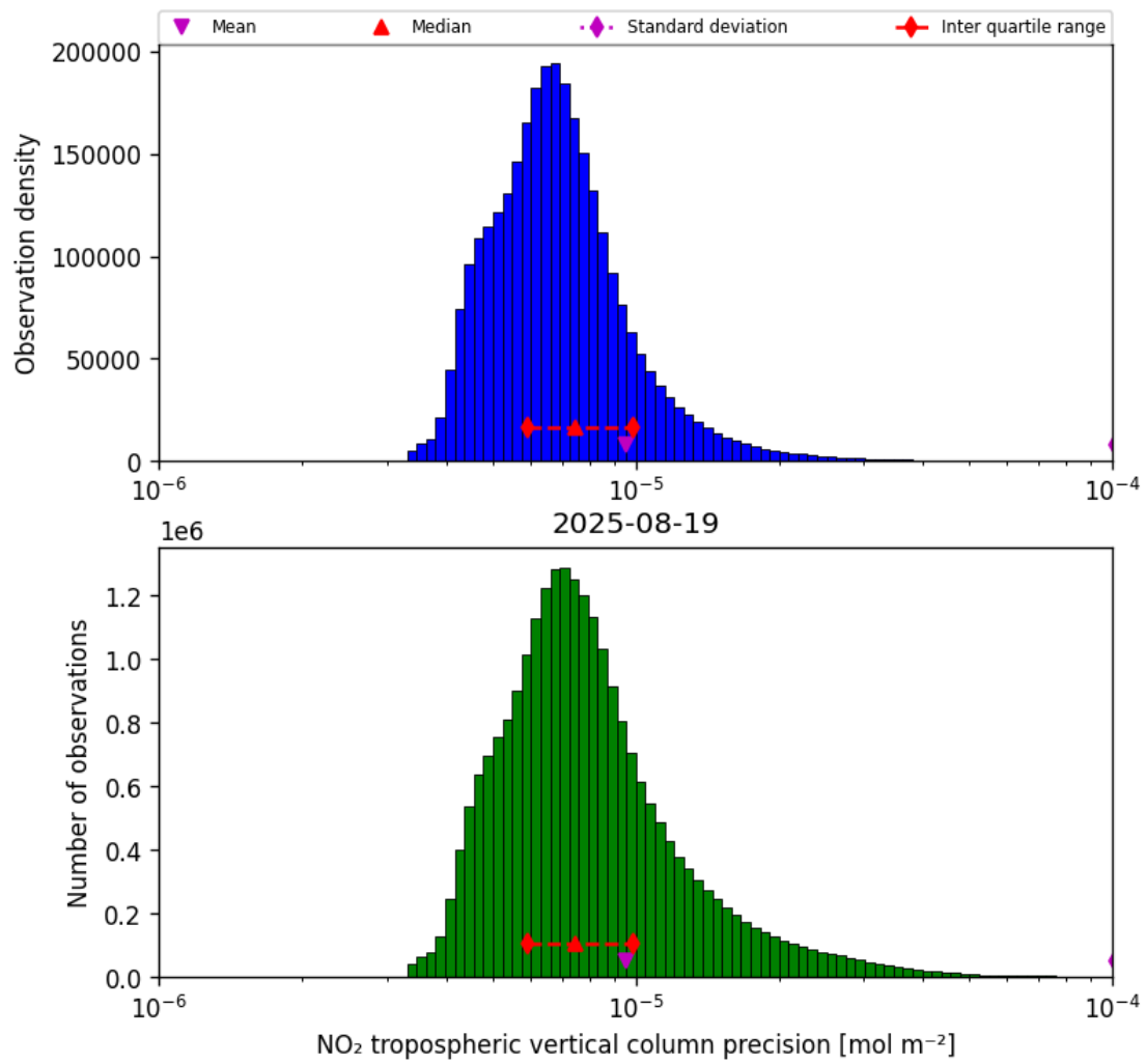
Figure 28: Histogram of “NO 2 tropospheric vertical column precision” for 2025-08-19 to 2025-08-20
