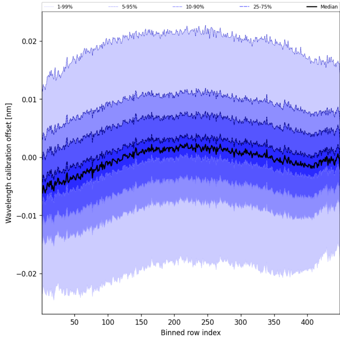
Figure 50: Along track statistics of “Wavelength calibration offset” for 2025-08-19 to 2025-08-20
