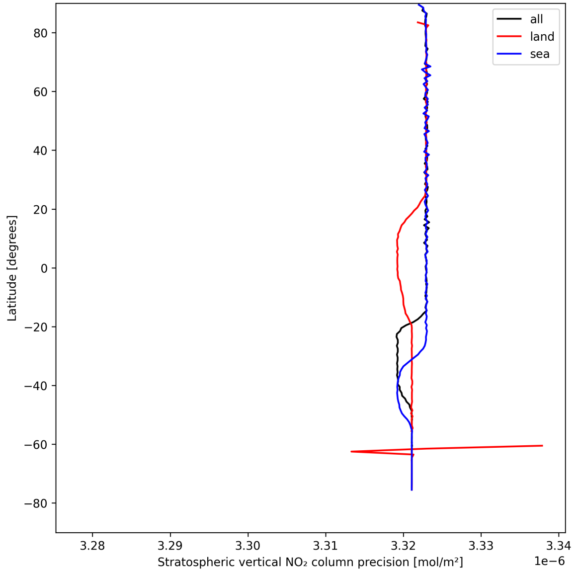
Figure 18: Zonal average of "Stratospheric vertical NO 2 column precision" for 2025-08-19 to 2025-08-20.
