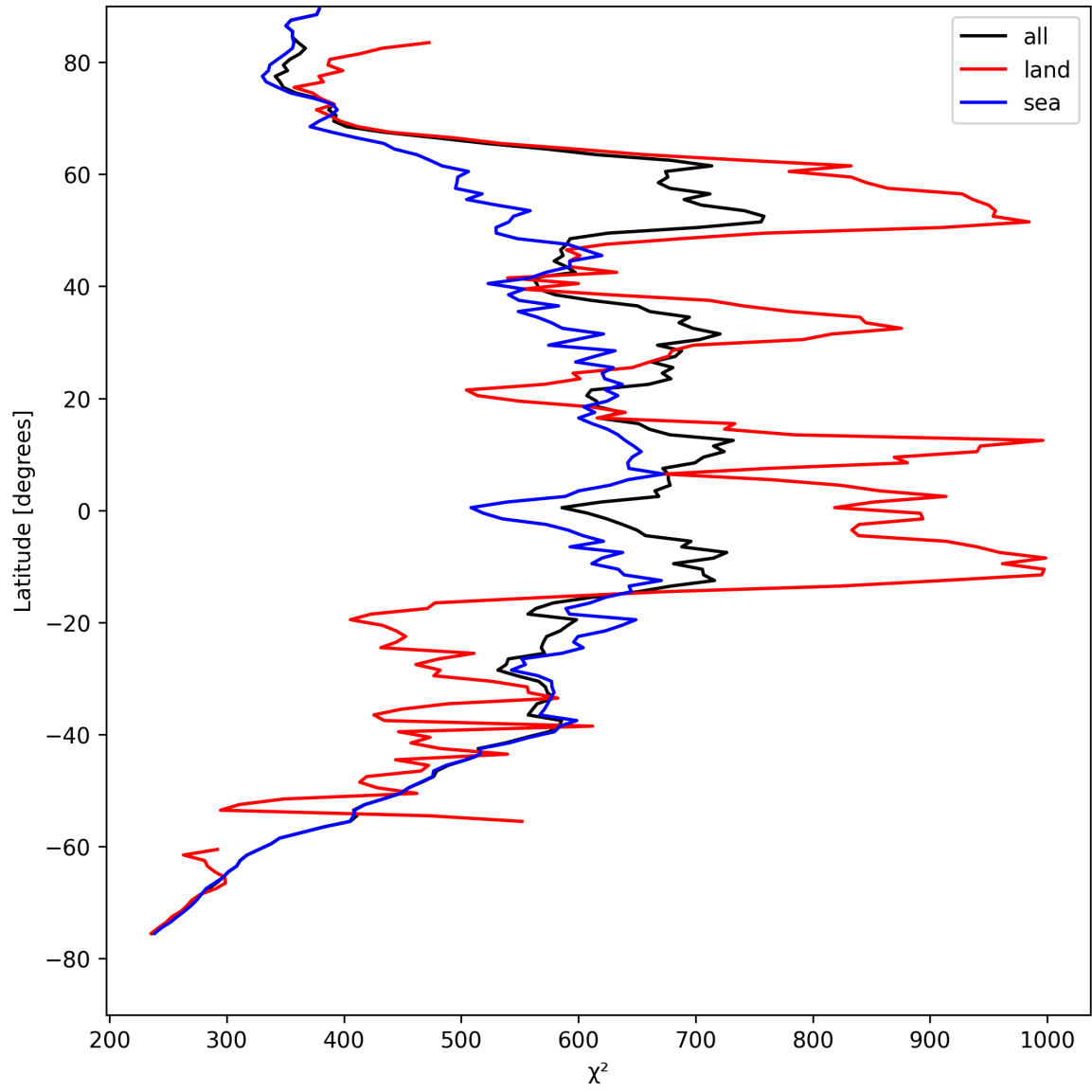
Figure 23: Zonal average of “ \chi^2 ” for 2025-08-19 to 2025-08-20.
