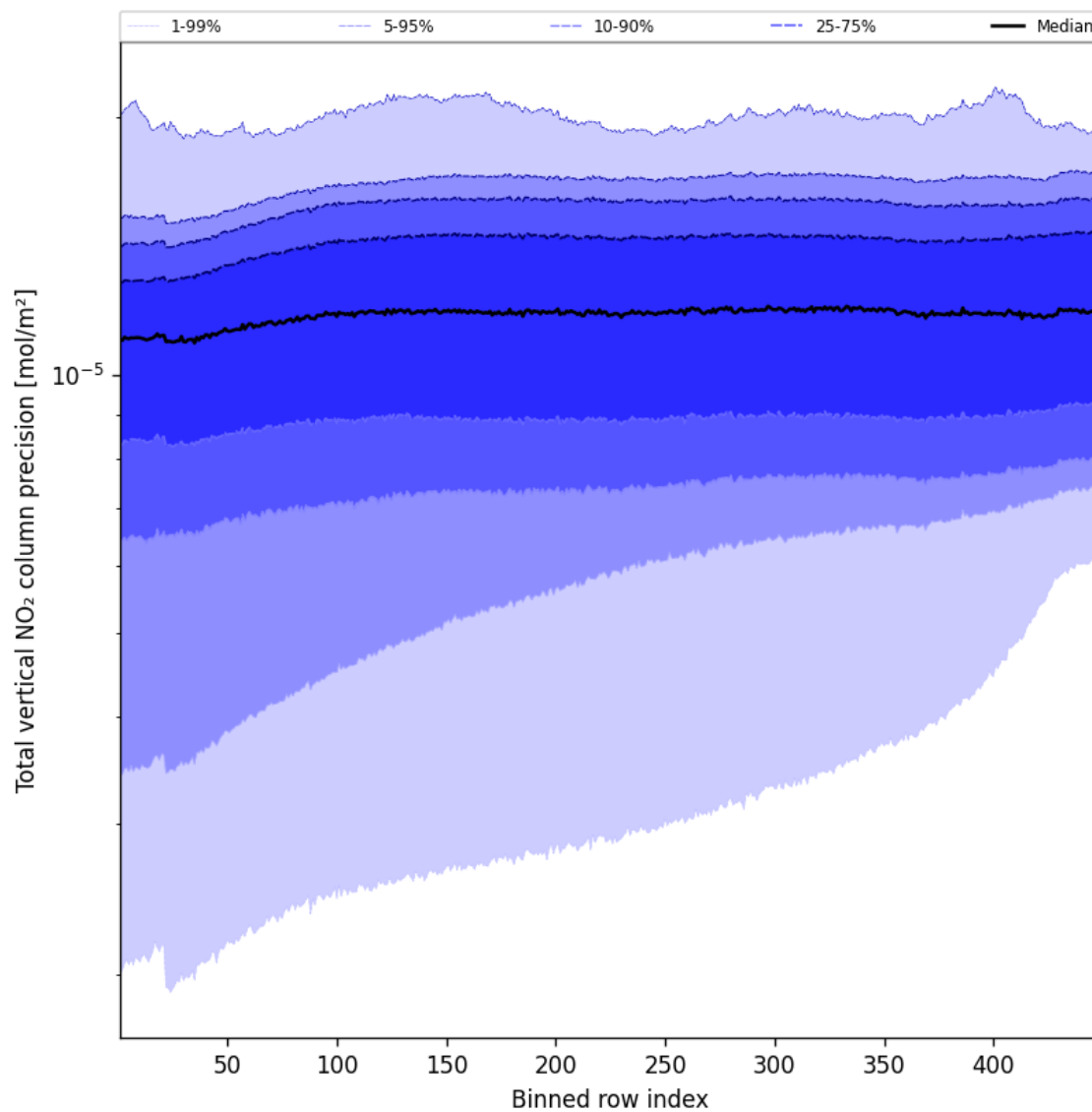
Figure 54: Along track statistics of “Total vertical NO 2 column precision” for 2025-08-19 to 2025-08-20
