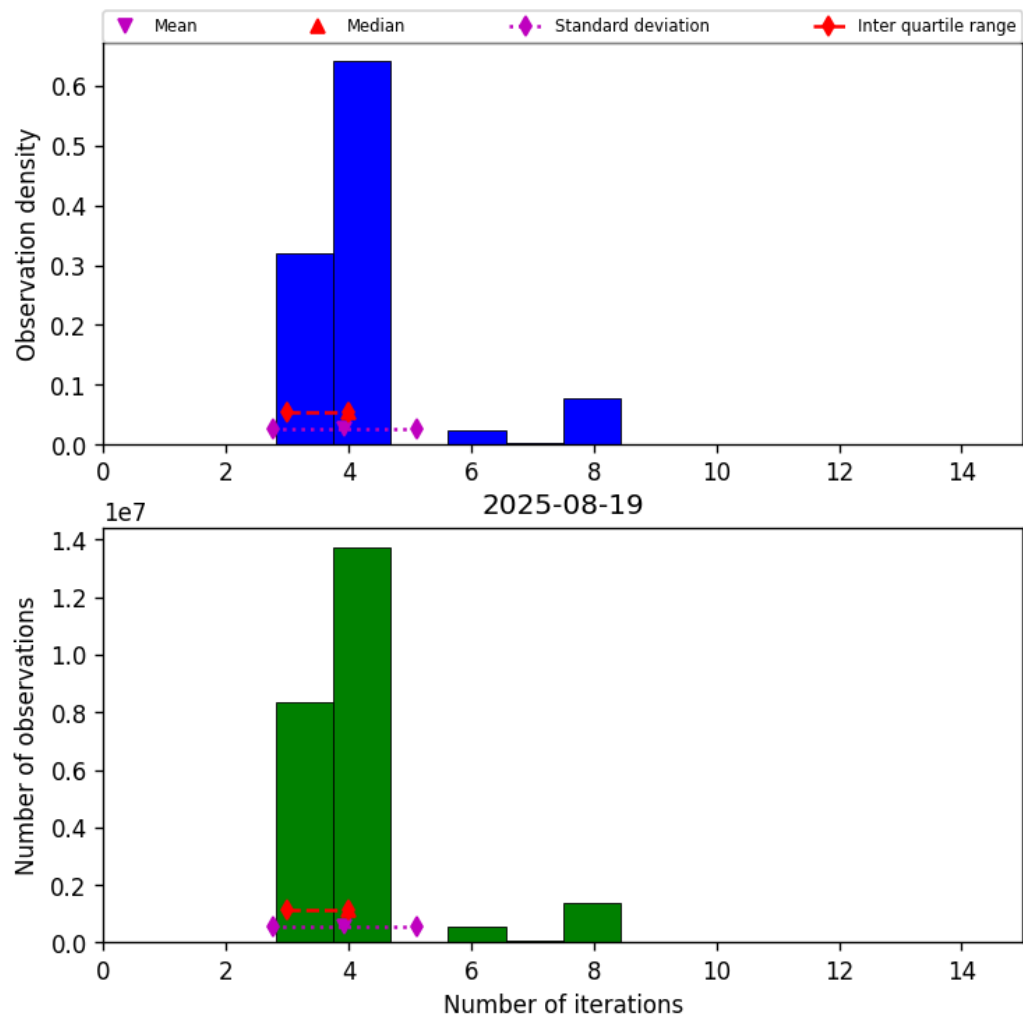
Figure 32: Histogram of “Number of iterations” for 2025-08-19 to 2025-08-20
