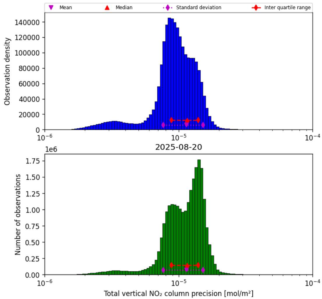
Figure 37: Histogram of “Total vertical NO 2 column precision” for 2025-08-20 to 2025-08-21
