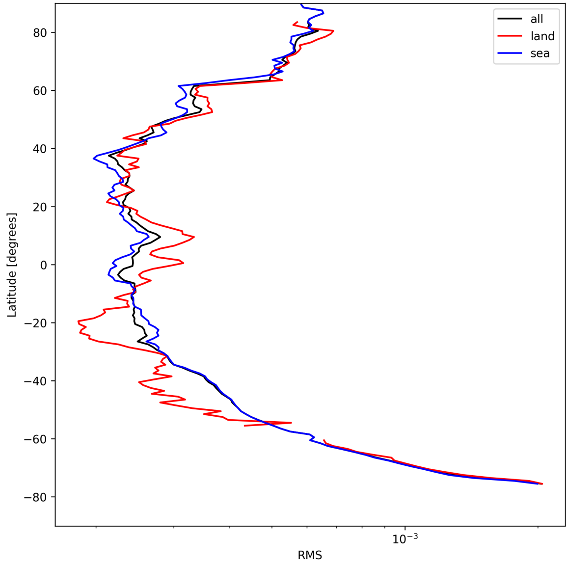
Figure 24: Zonal average of “RMS” for 2025-08-20 to 2025-08-21.
