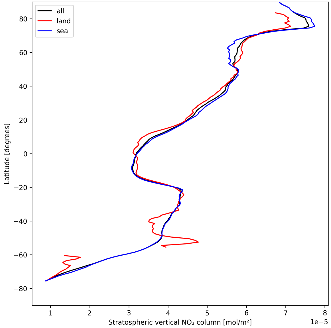
Figure 17: Zonal average of “Stratospheric vertical NO 2 column” for 2025-08-20 to 2025-08-21.
