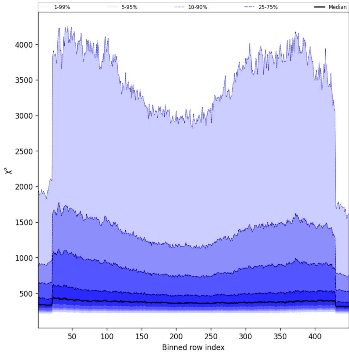
Figure 57: Along track statistics of “ \chi^2 ” for 2025-08-20 to 2025-08-21
