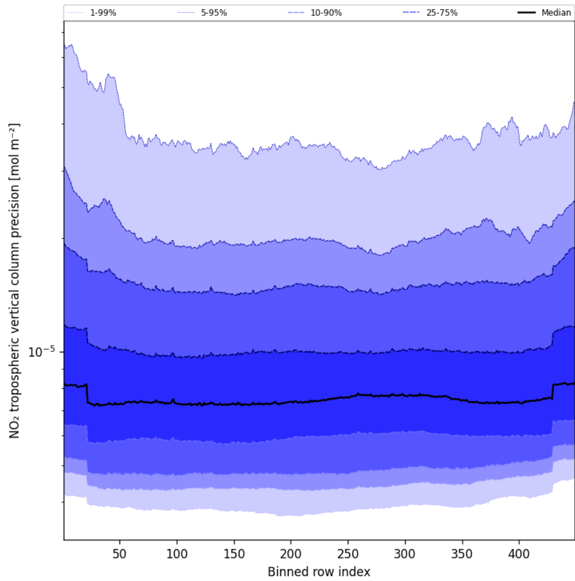
Figure 45: Along track statistics of “NO 2 tropospheric vertical column precision” for 2025-08-20 to 2025-08-21
