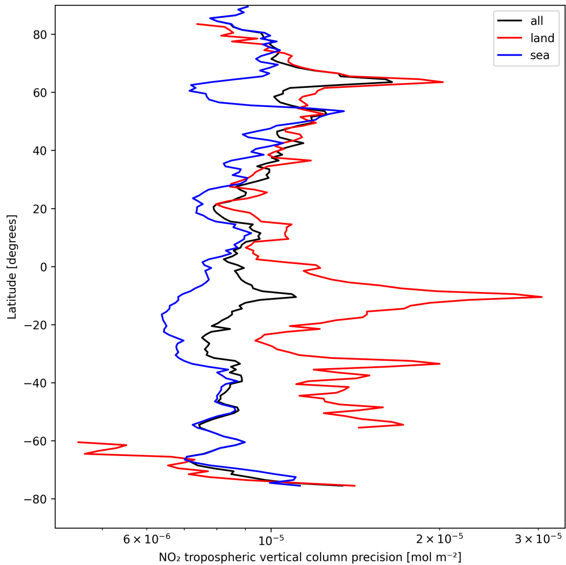
Figure 11: Zonal average of “NO 2 tropospheric vertical column precision” for 2025-08-20 to 2025-08-21.
