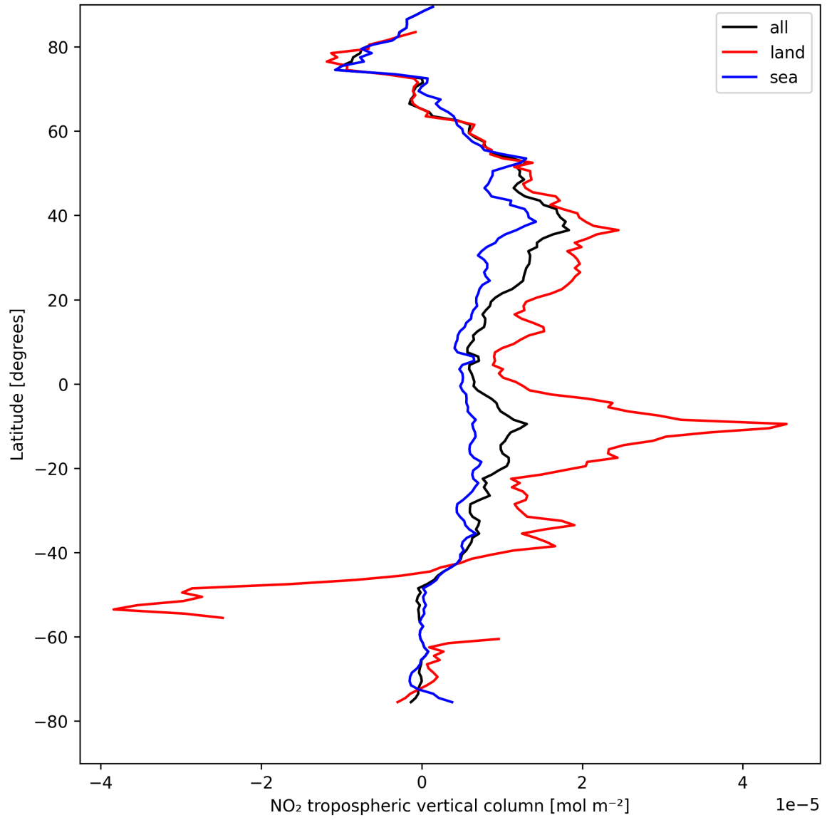
Figure 10: Zonal average of “NO 2 tropospheric vertical column” for 2025-08-20 to 2025-08-21.
