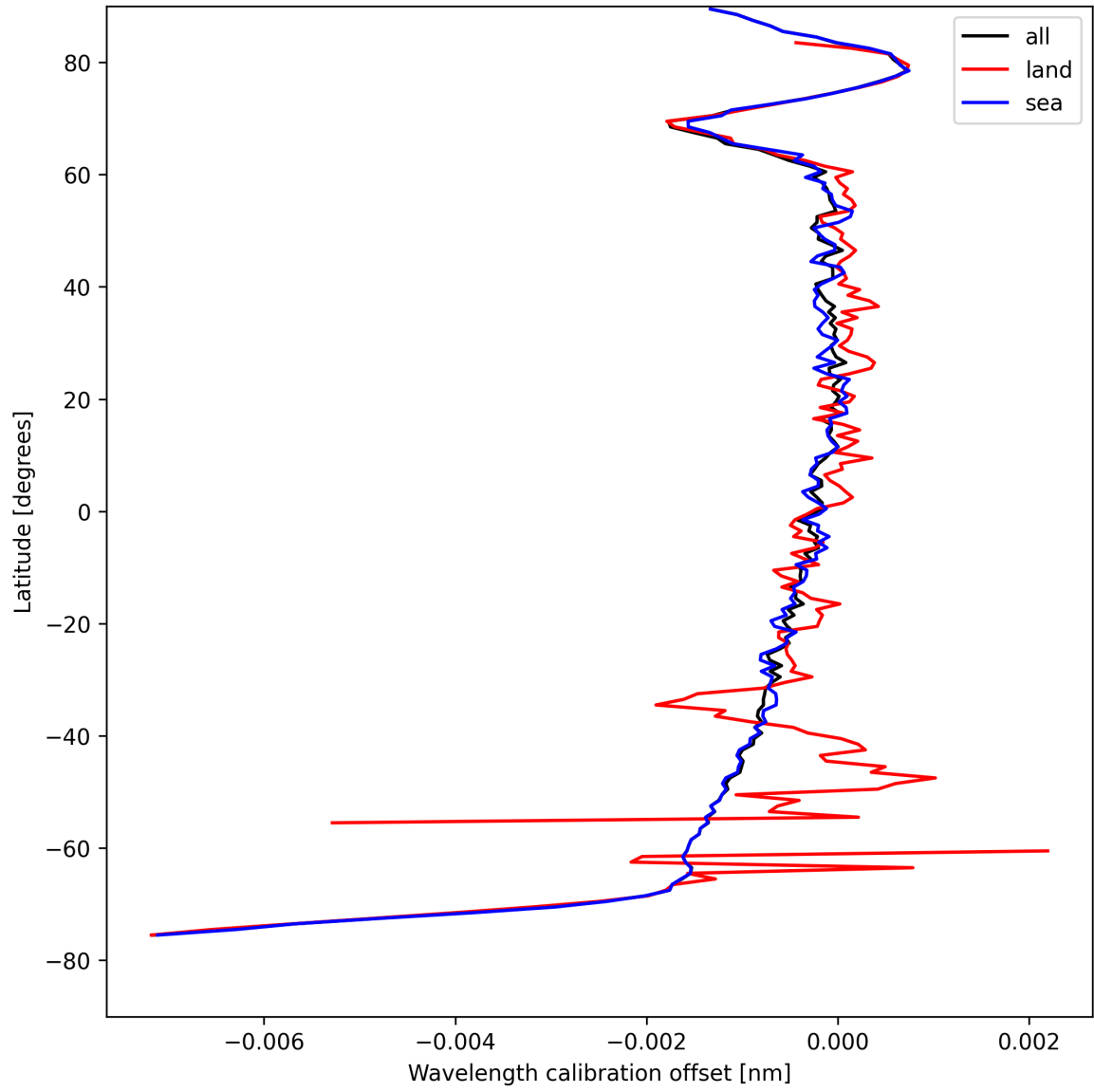
Figure 16: Zonal average of “Wavelength calibration offset” for 2025-08-20 to 2025-08-21.
