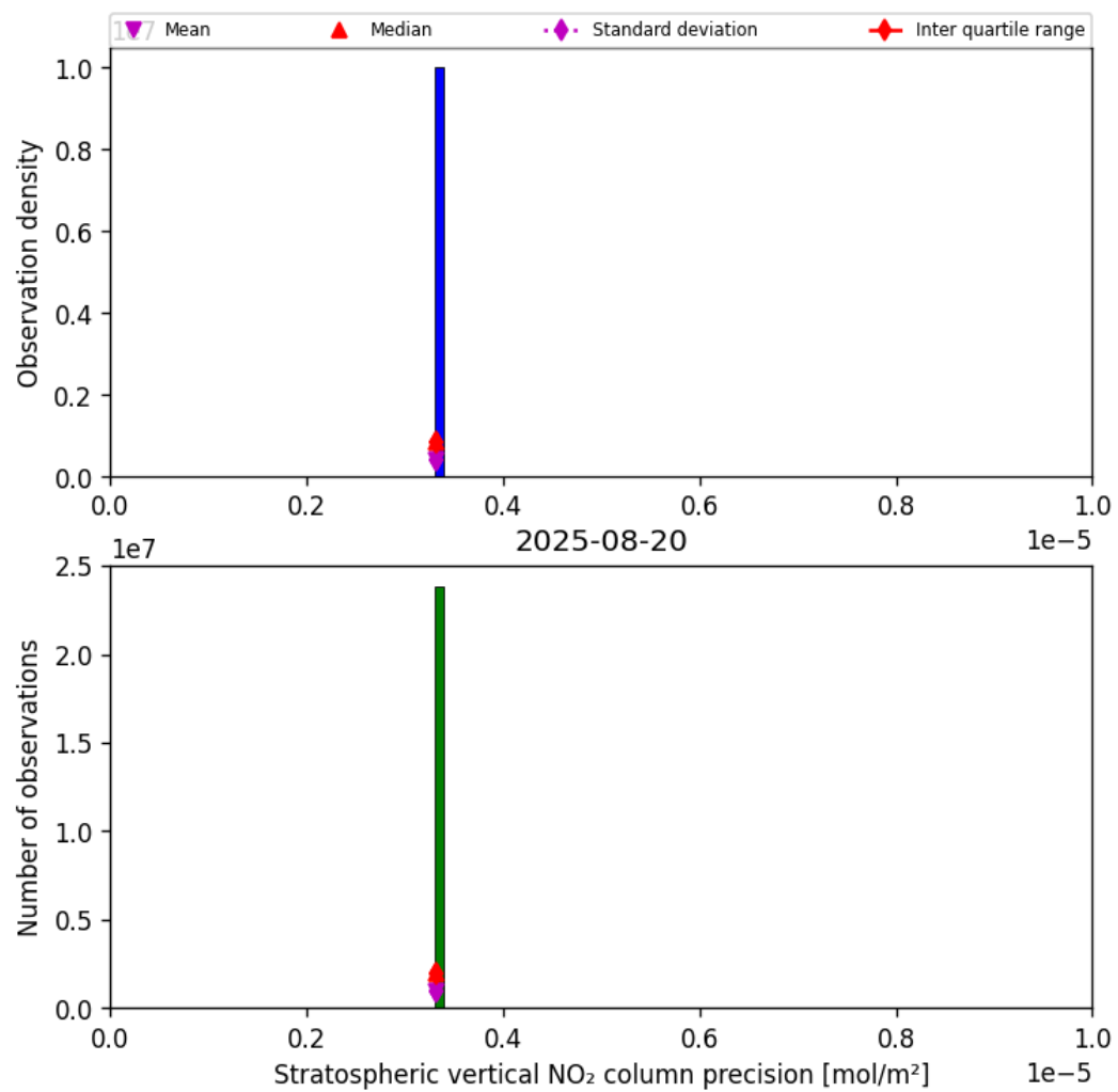
Figure 35: Histogram of “Stratospheric vertical NO 2 column precision” for 2025-08-20 to 2025-08-21
