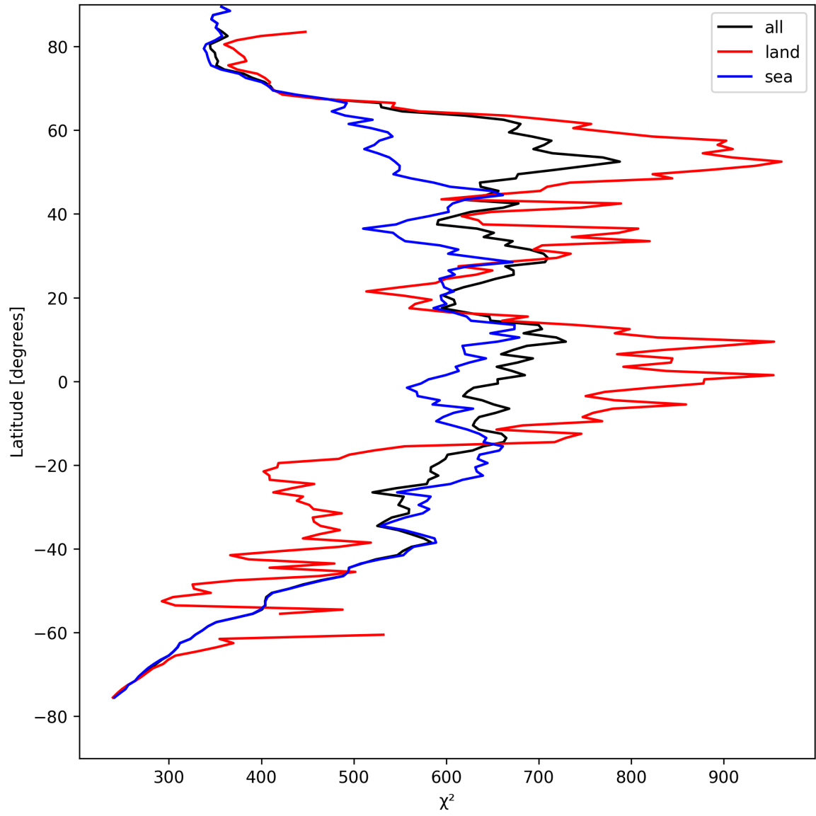
Figure 23: Zonal average of “ \chi^2 ” for 2025-08-20 to 2025-08-21.
