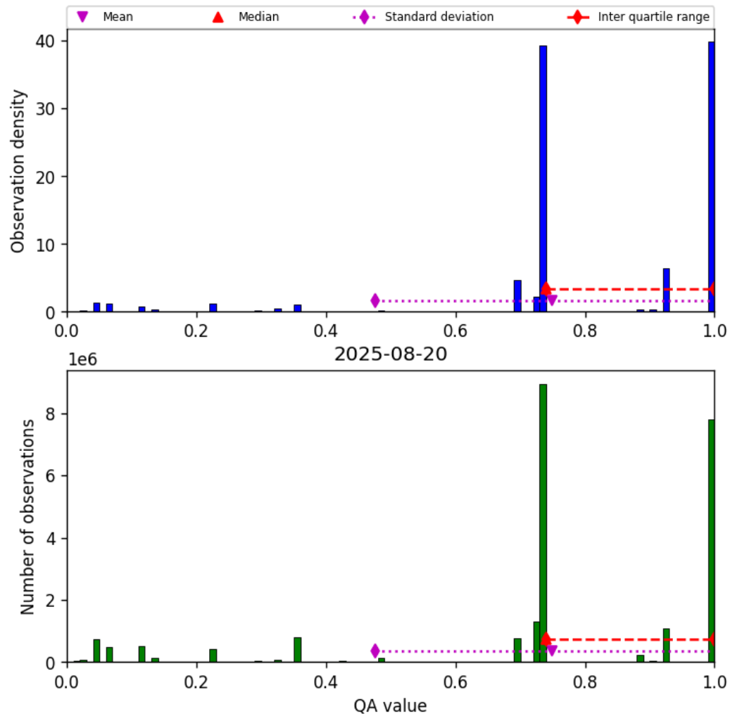
Figure 26: Histogram of “QA value” for 2025-08-20 to 2025-08-21
