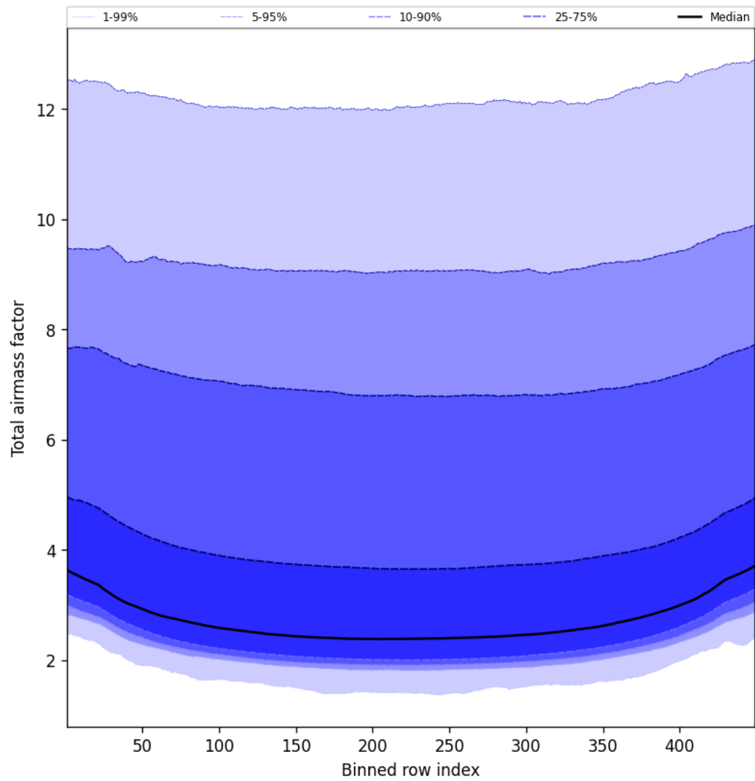
Figure 47: Along track statistics of “Total airmass factor” for 2025-08-20 to 2025-08-21
