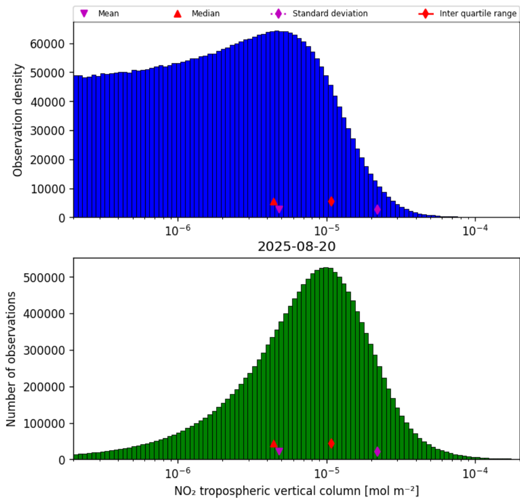
Figure 27: Histogram of “NO 2 tropospheric vertical column” for 2025-08-20 to 2025-08-21
