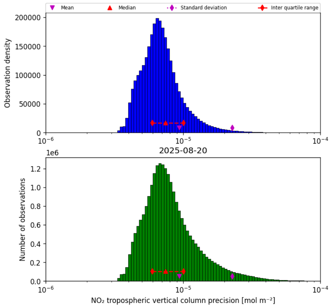
Figure 28: Histogram of “NO 2 tropospheric vertical column precision” for 2025-08-20 to 2025-08-21
