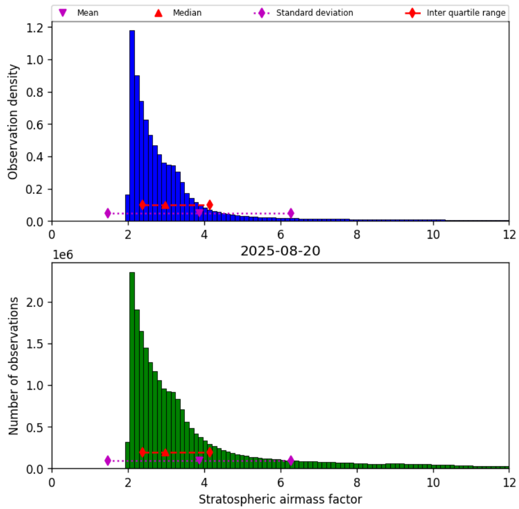
Figure 42: Histogram of “Stratospheric airmass factor” for 2025-08-20 to 2025-08-21
