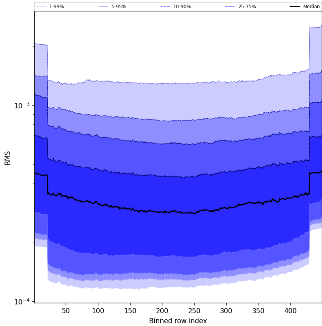
Figure 58: Along track statistics of “RMS” for 2025-08-20 to 2025-08-21
