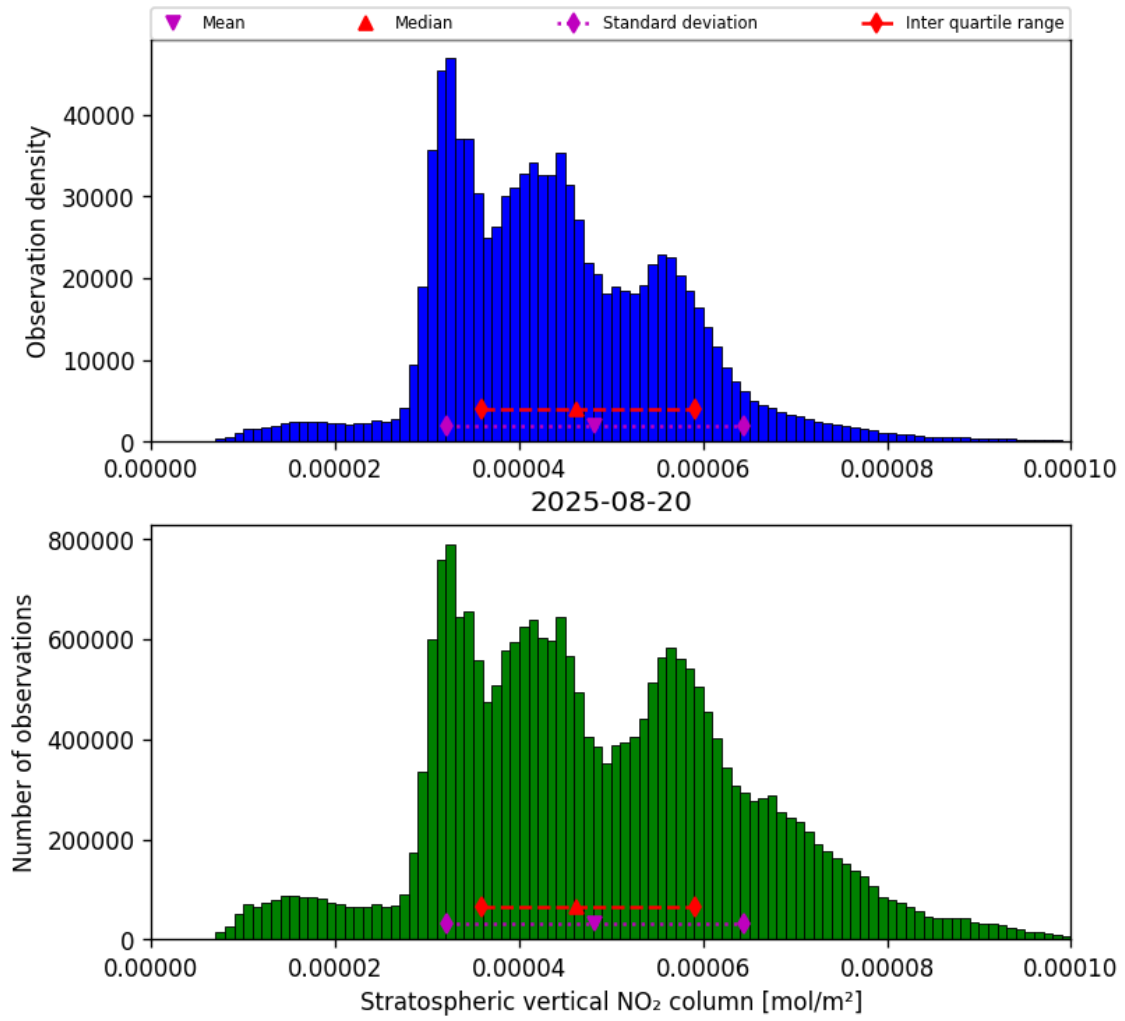
Figure 34: Histogram of “Stratospheric vertical NO 2 column” for 2025-08-20 to 2025-08-21
