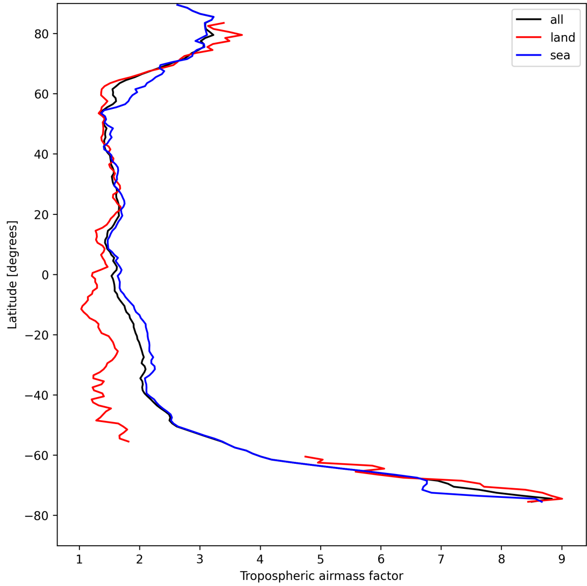
Figure 12: Zonal average of “Tropospheric airmass factor” for 2025-08-20 to 2025-08-21.
