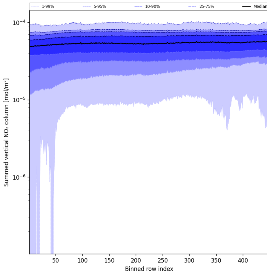
Figure 55: Along track statistics of “Summed vertical NO 2 column” for 2025-08-20 to 2025-08-21
