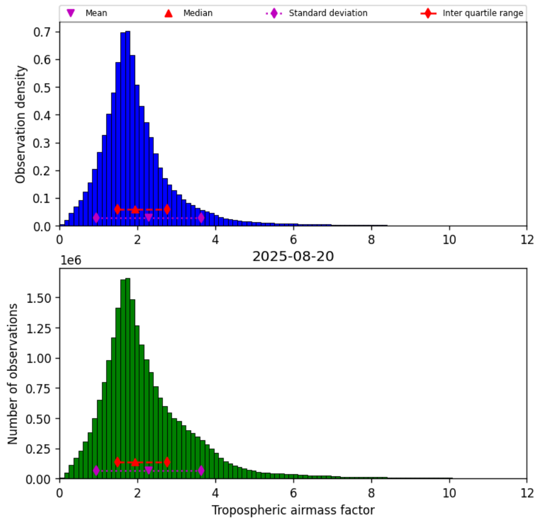
Figure 29: Histogram of “Tropospheric airmass factor” for 2025-08-20 to 2025-08-21
