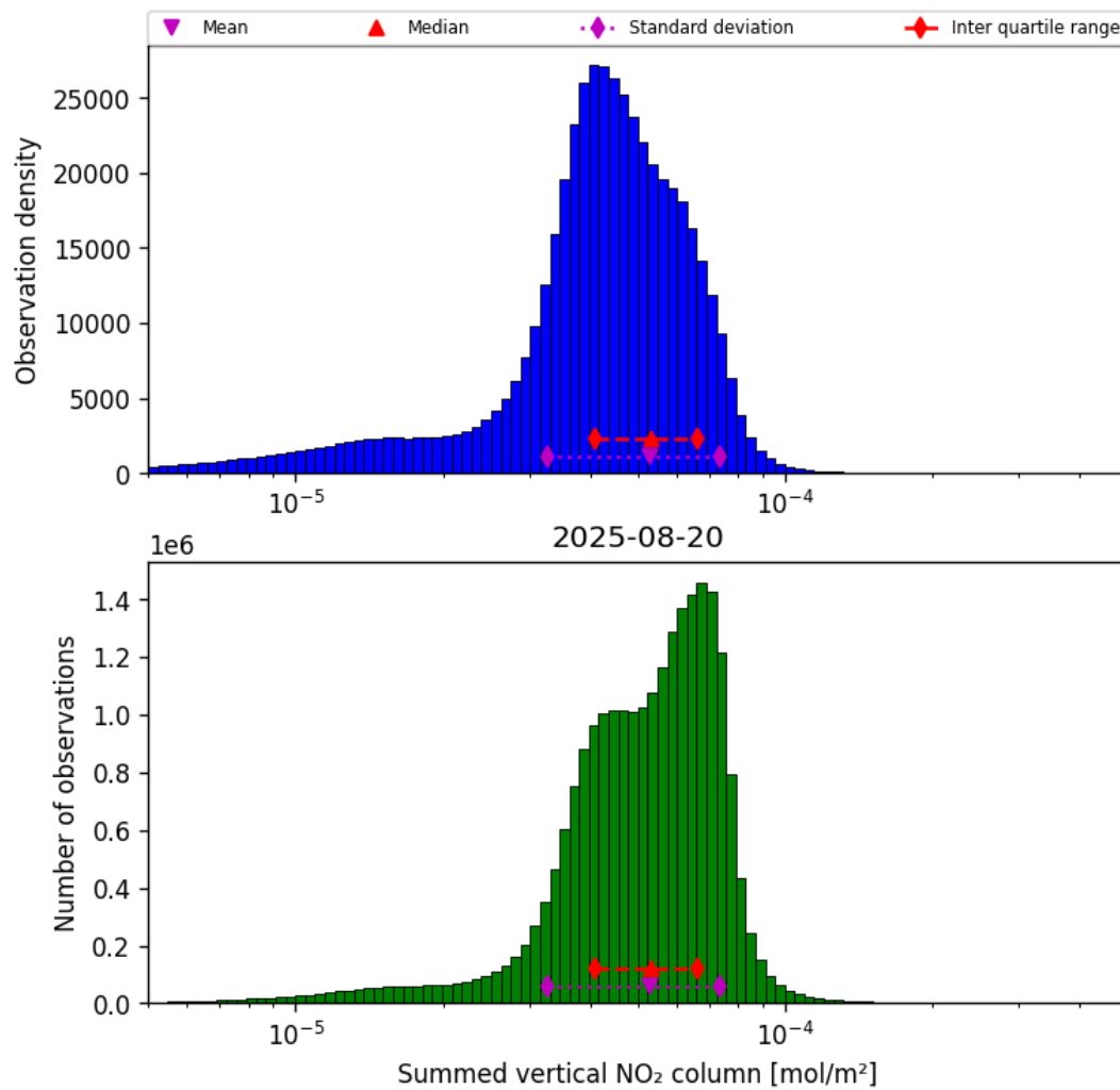
Figure 38: Histogram of "Summed vertical NO 2 column" for 2025-08-20 to 2025-08-21
