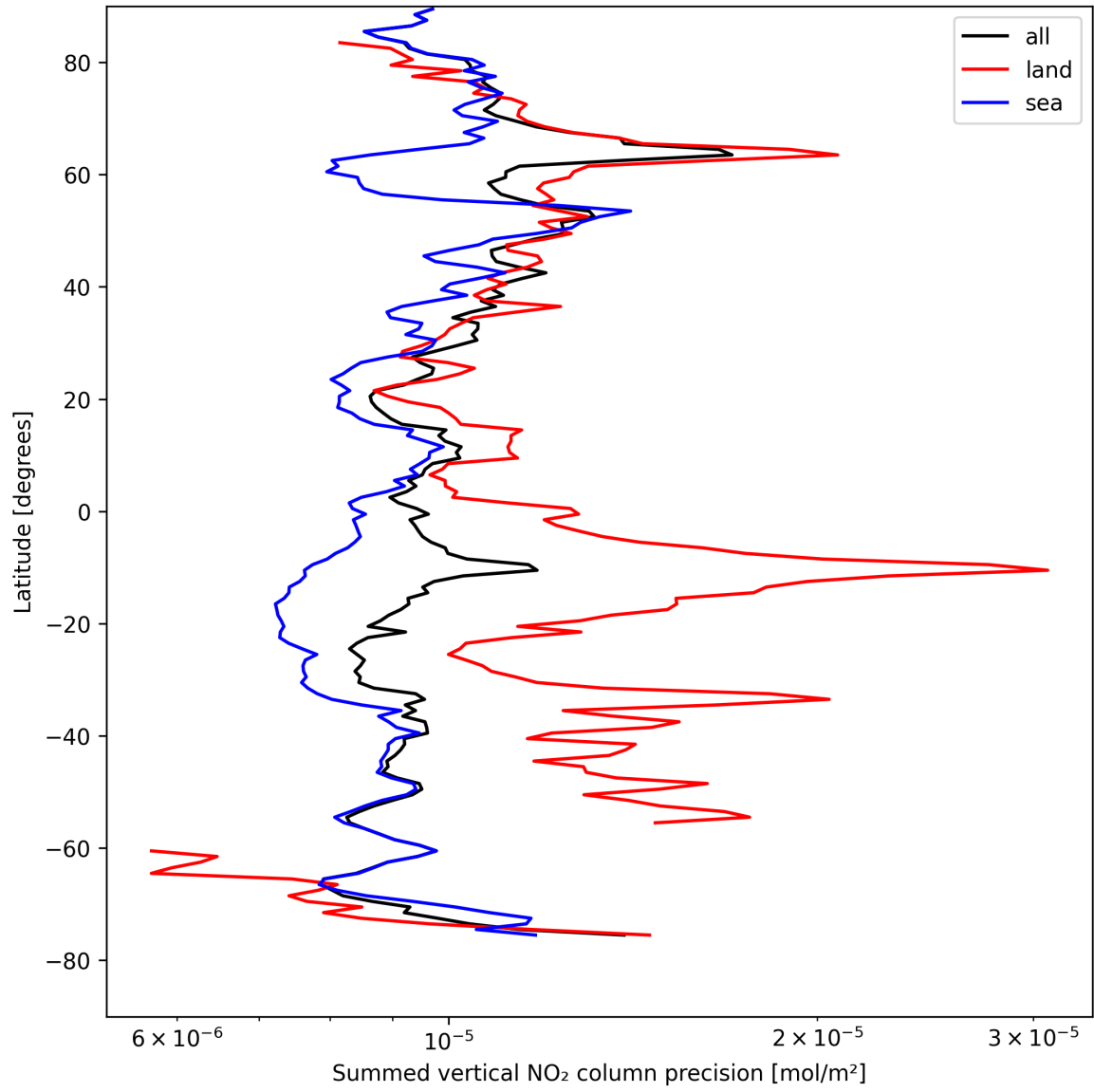
Figure 22: Zonal average of “Summed vertical NO 2 column precision” for 2025-08-20 to 2025-08-21.
