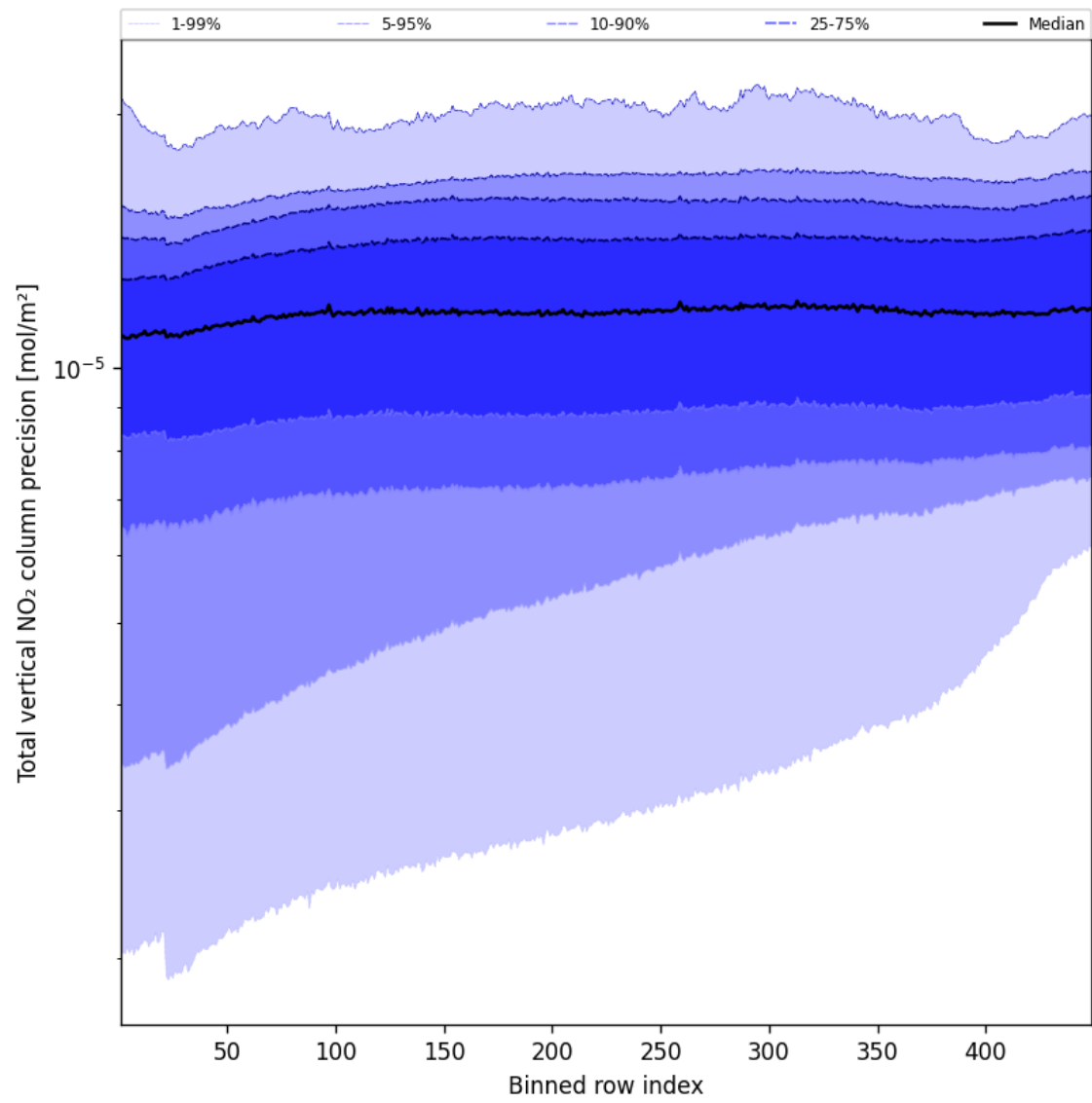
Figure 54: Along track statistics of “Total vertical NO 2 column precision” for 2025-08-20 to 2025-08-21
