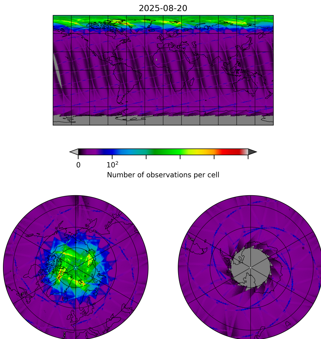
Figure 8: Map of the number of observations for 2025-08-20 to 2025-08-21
