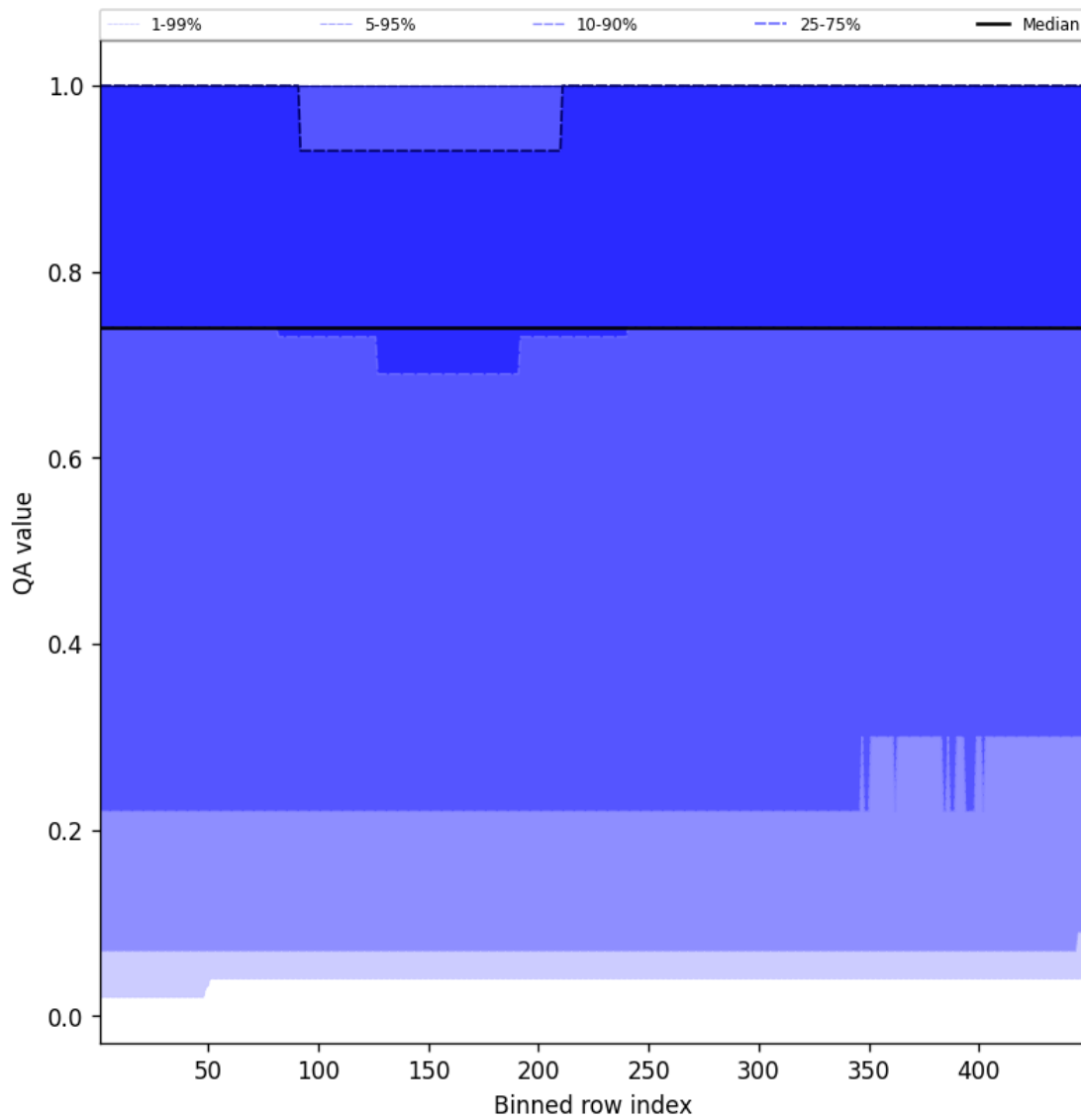
Figure 43: Along track statistics of "QA value" for 2025-08-20 to 2025-08-21
