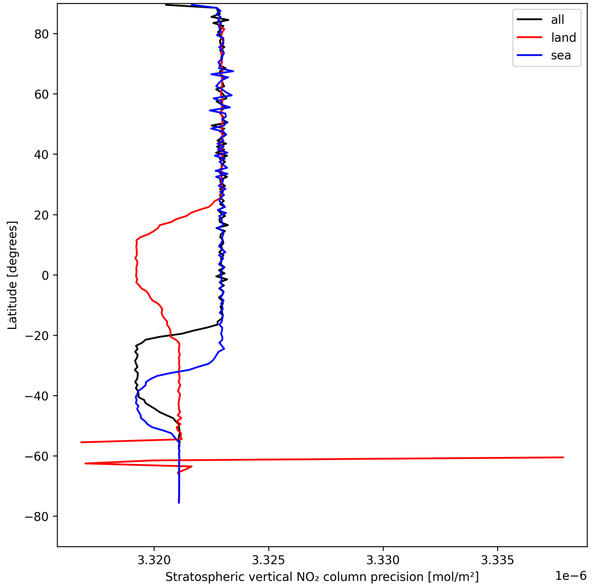
Figure 18: Zonal average of "Stratospheric vertical NO 2 column precision" for 2025-08-20 to 2025-08-21.
