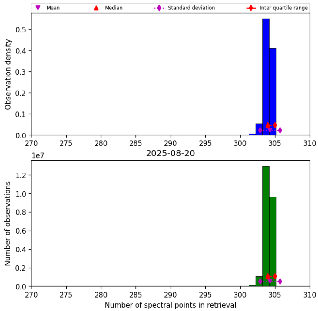
Figure 31: Histogram of “Number of spectral points in retrieval” for 2025-08-20 to 2025-08-21
