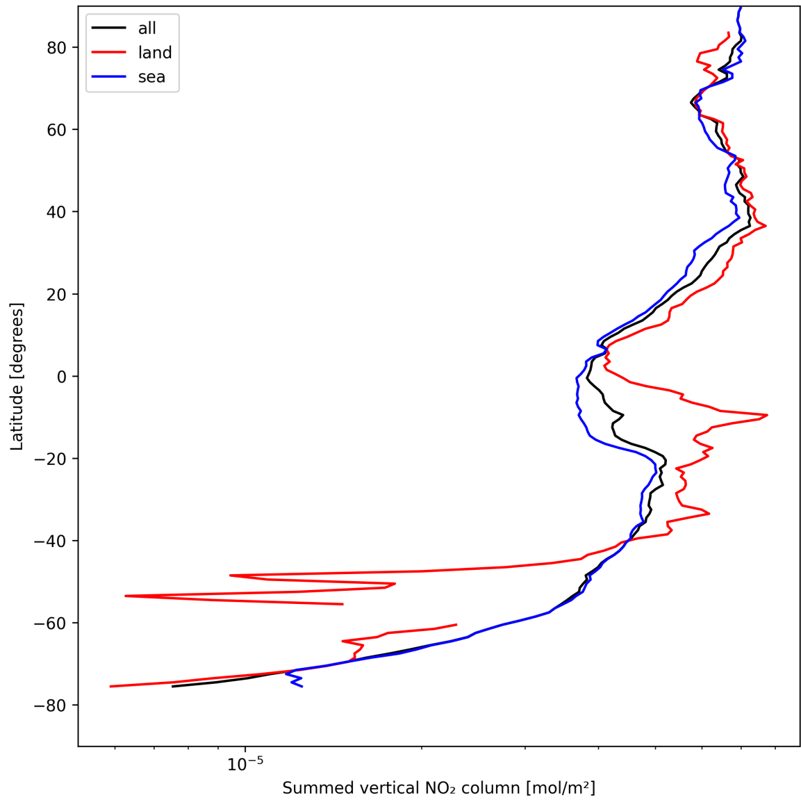
Figure 21: Zonal average of “Summed vertical NO 2 column” for 2025-08-20 to 2025-08-21.
