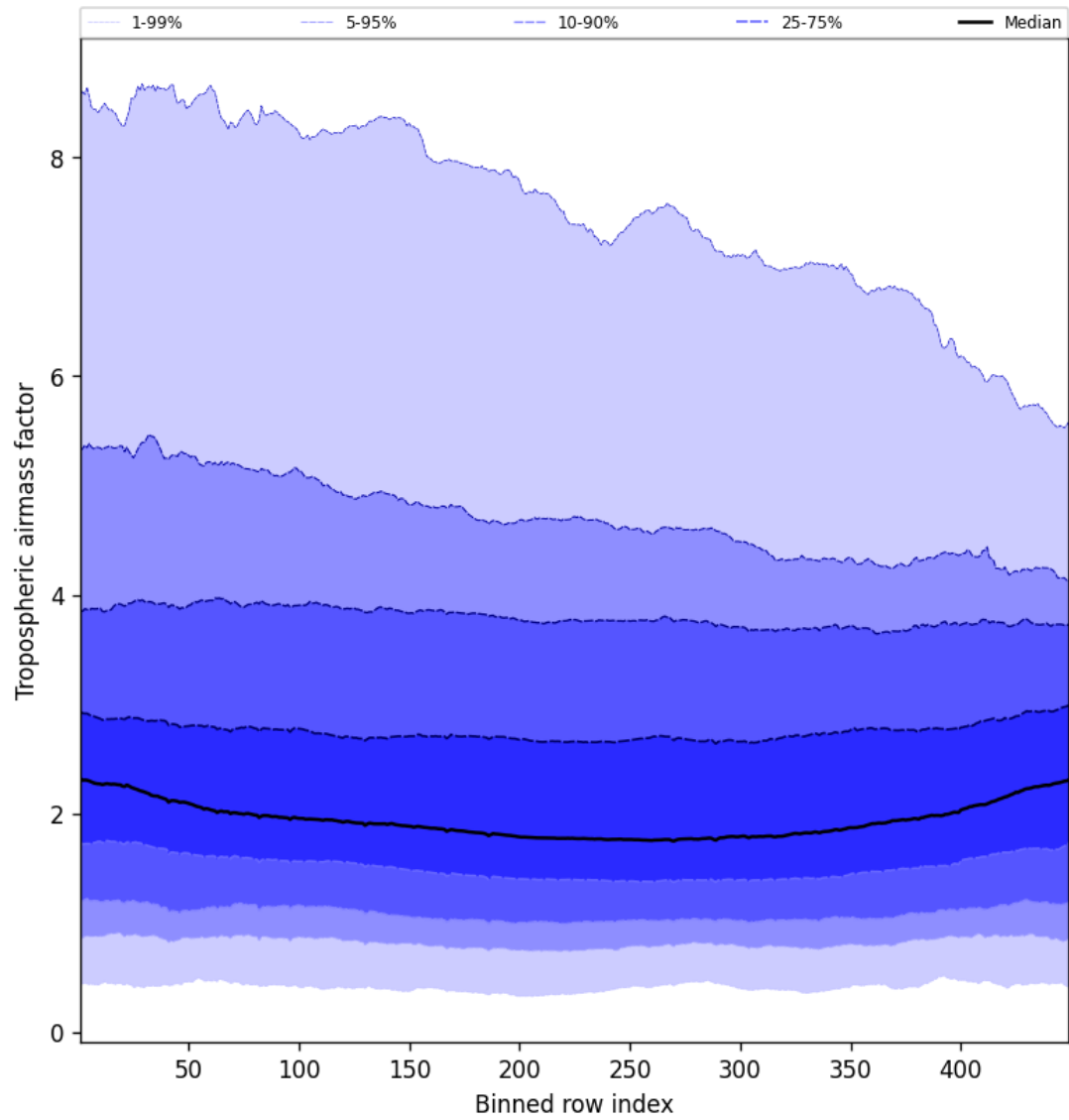
Figure 46: Along track statistics of “Tropospheric air mass factor” for 2025-08-20 to 2025-08-21
