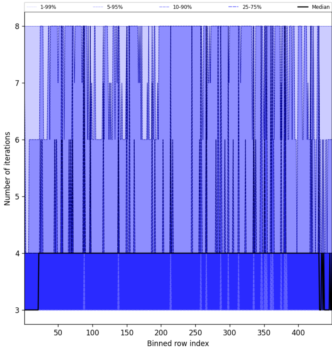
Figure 49: Along track statistics of “Number of iterations” for 2025-08-20 to 2025-08-21
