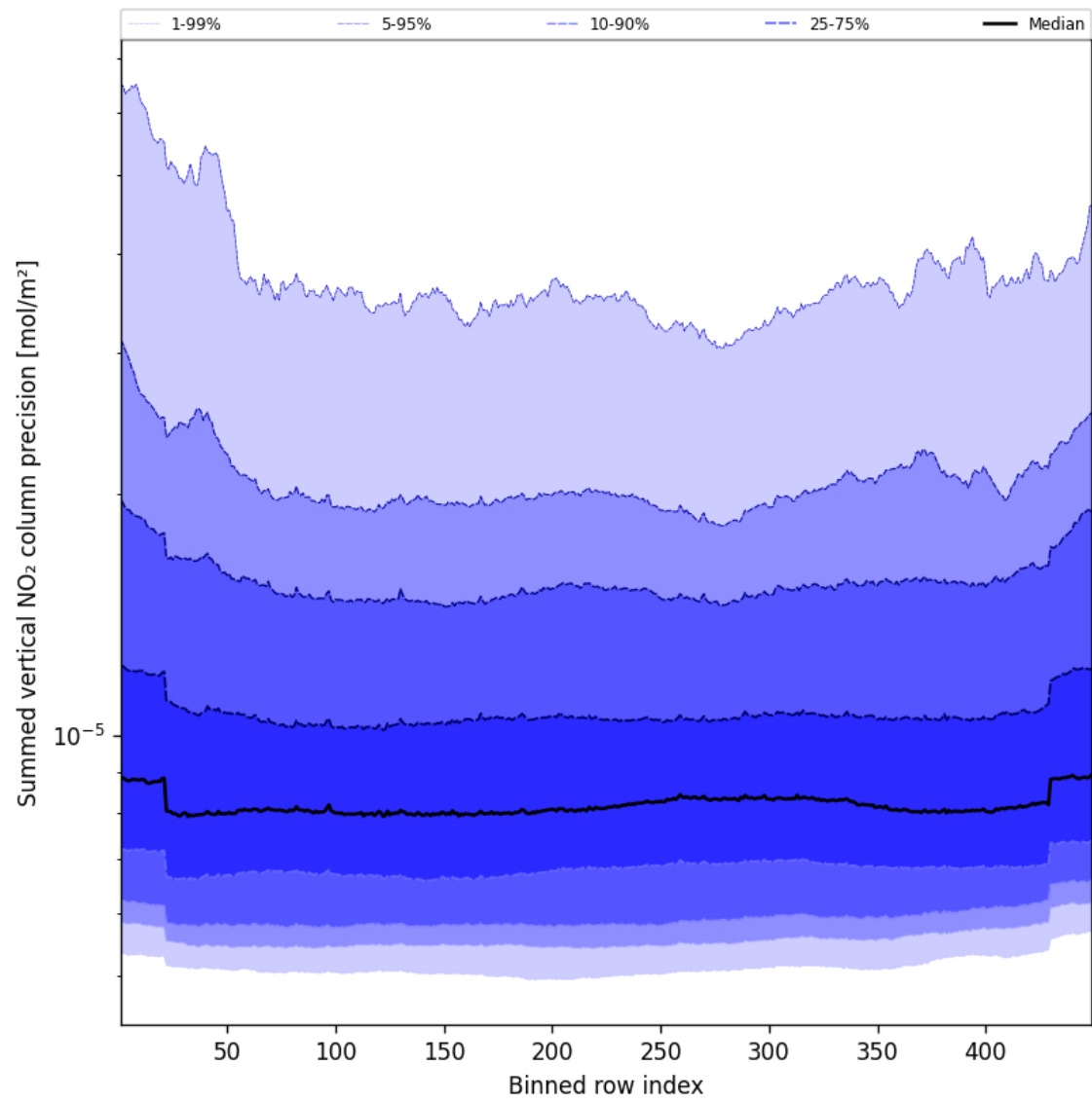
Figure 56: Along track statistics of “Summed vertical NO 2 column precision” for 2025-08-20 to 2025-08-21
