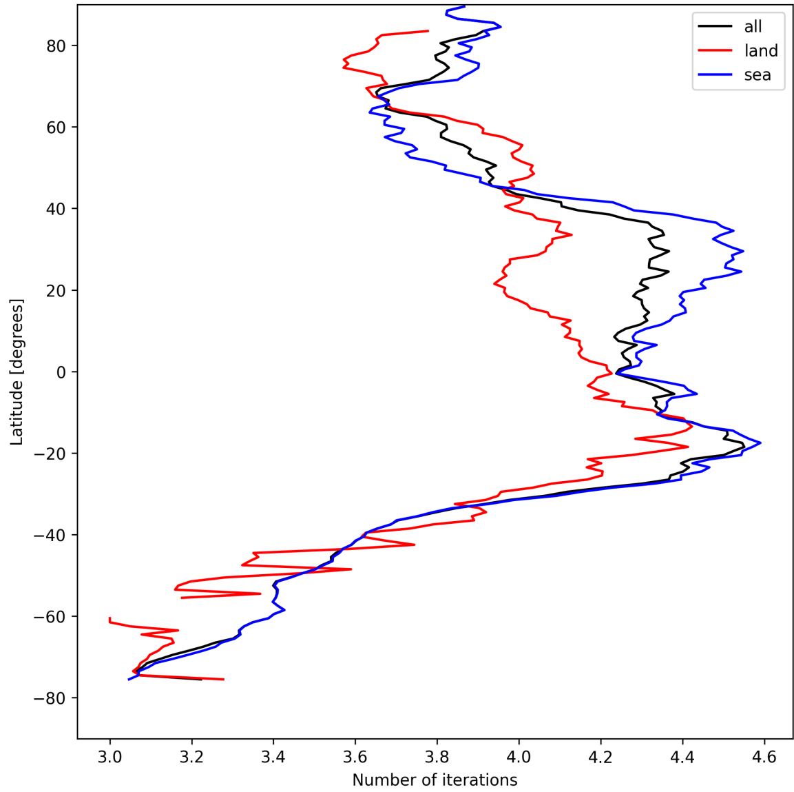
Figure 15: Zonal average of “Number of iterations” for 2025-08-20 to 2025-08-21.
