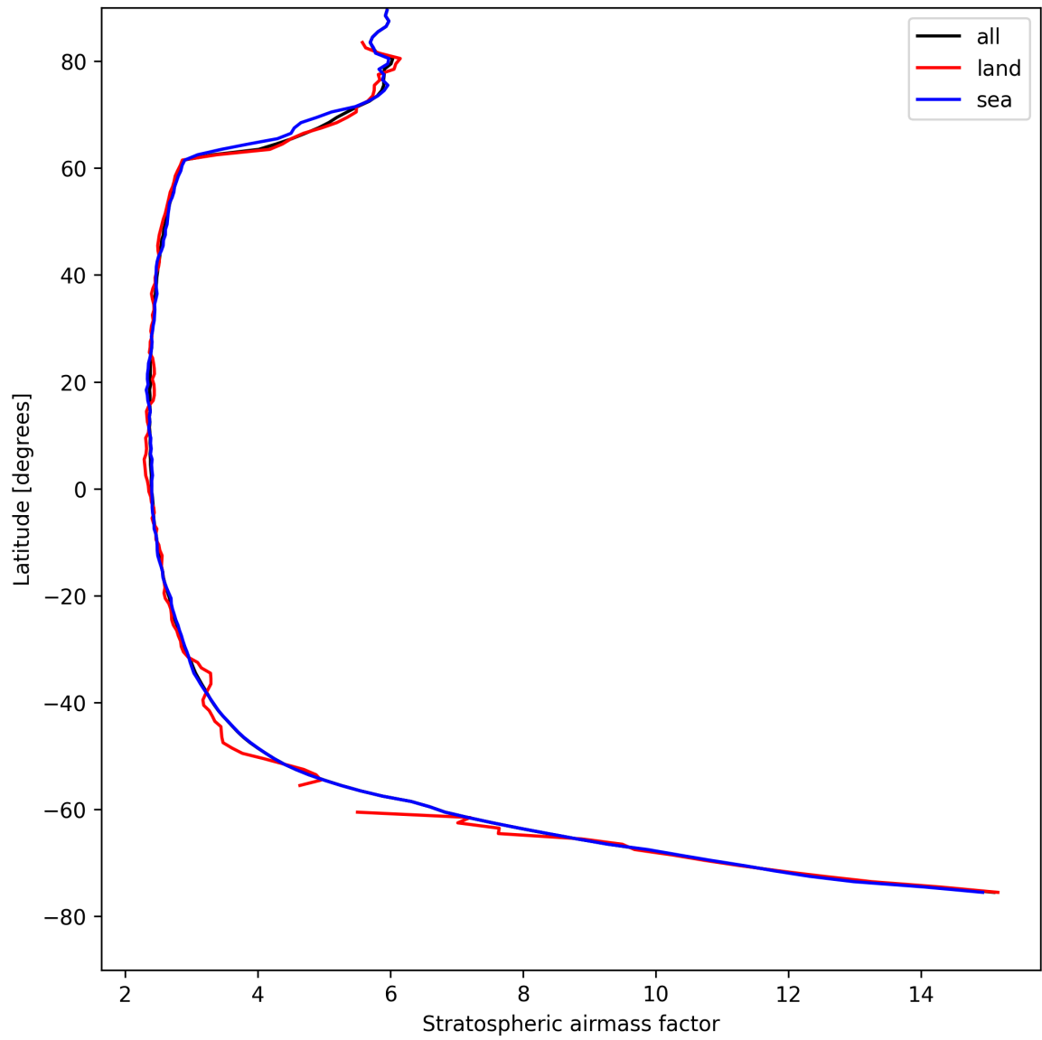
Figure 25: Zonal average of “Stratospheric airmass factor” for 2025-08-20 to 2025-08-21.
