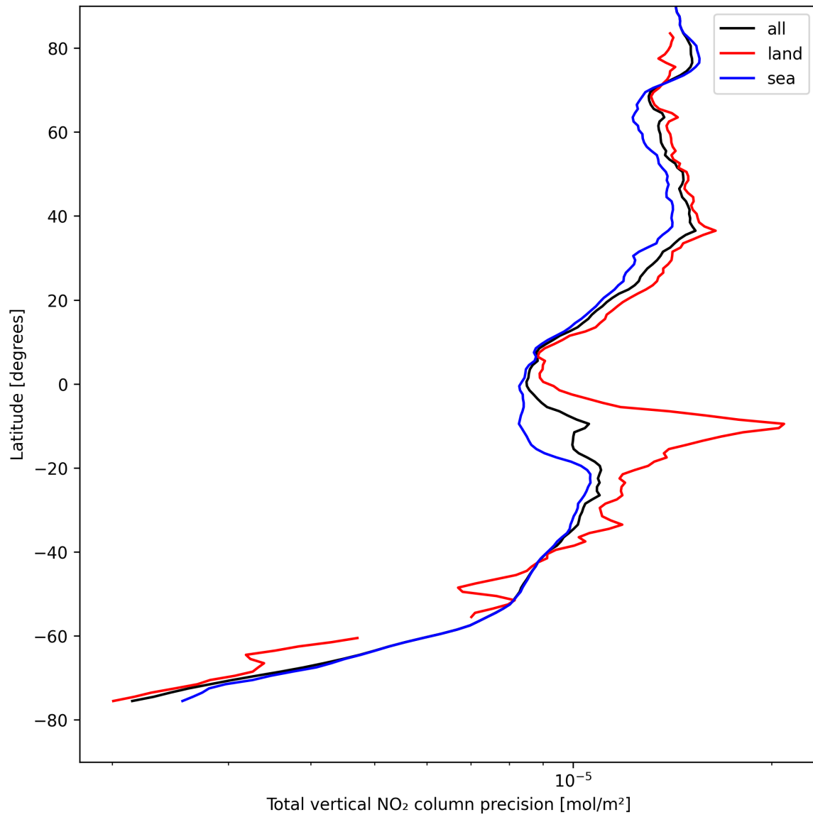
Figure 20: Zonal average of “Total vertical NO 2 column precision” for 2025-08-20 to 2025-08-21.
