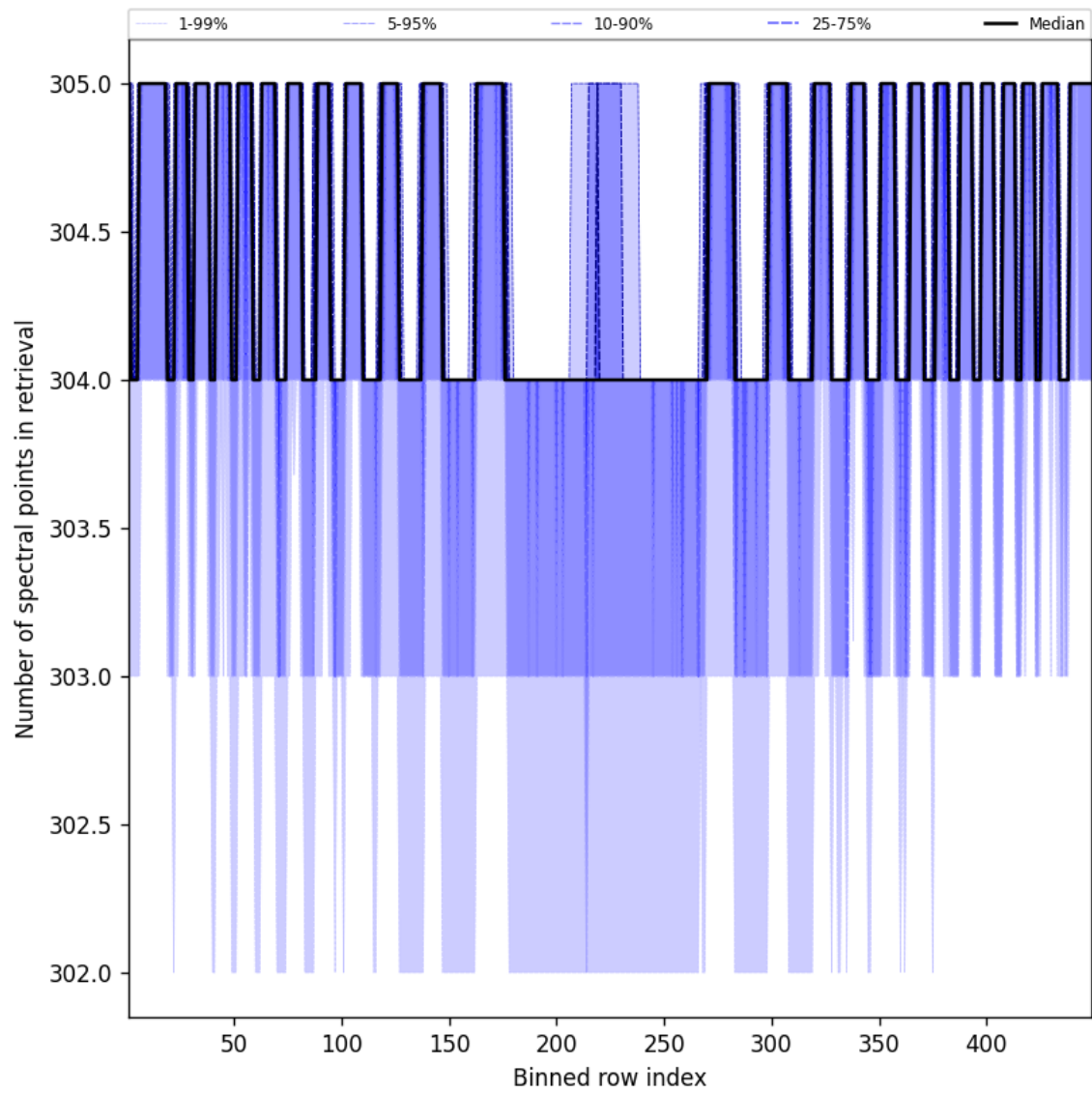
Figure 48: Along track statistics of “Number of spectral points in retrieval” for 2025-08-20 to 2025-08-21
