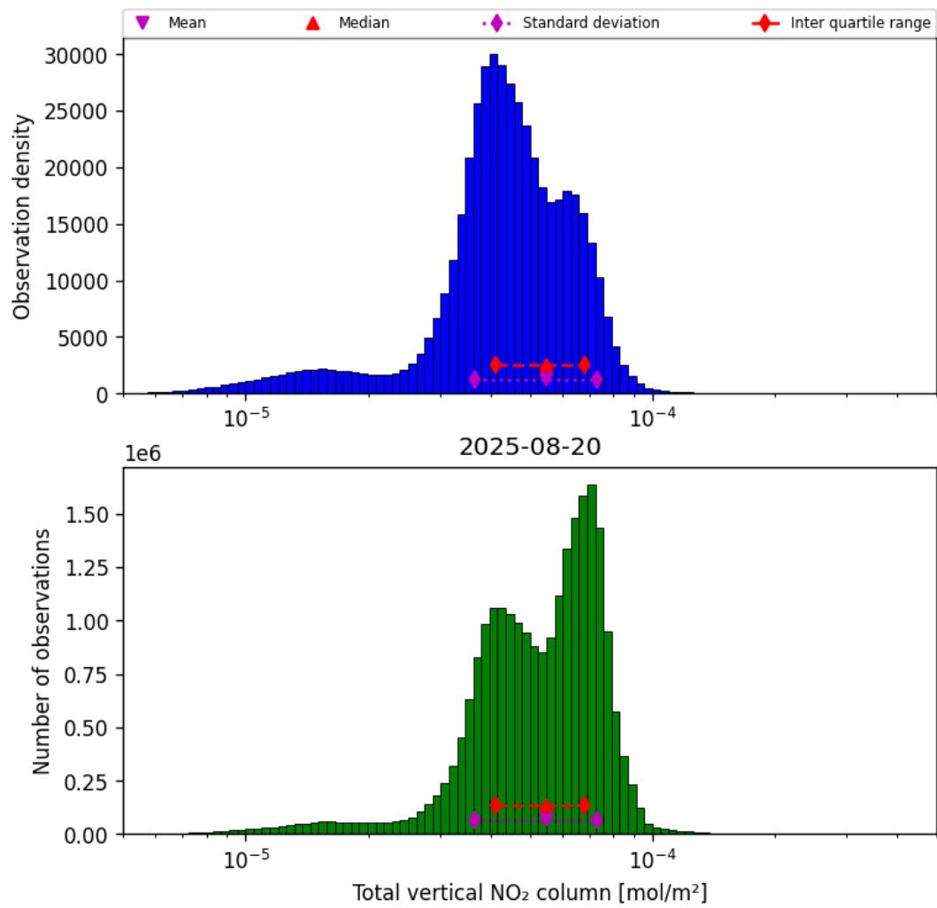
Figure 36: Histogram of “Total vertical NO 2 column” for 2025-08-20 to 2025-08-21
