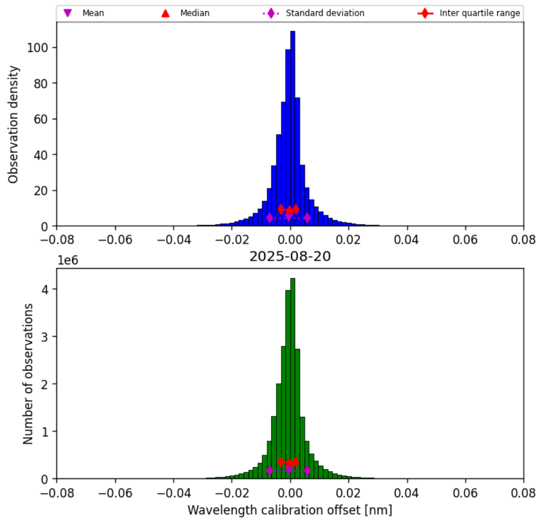
Figure 33: Histogram of “Wavelength calibration offset” for 2025-08-20 to 2025-08-21
