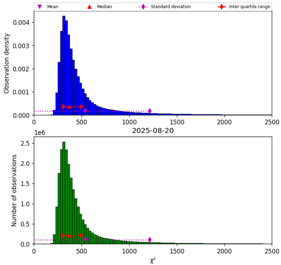
Figure 40: Histogram of “ \chi^2 ” for 2025-08-20 to 2025-08-21
