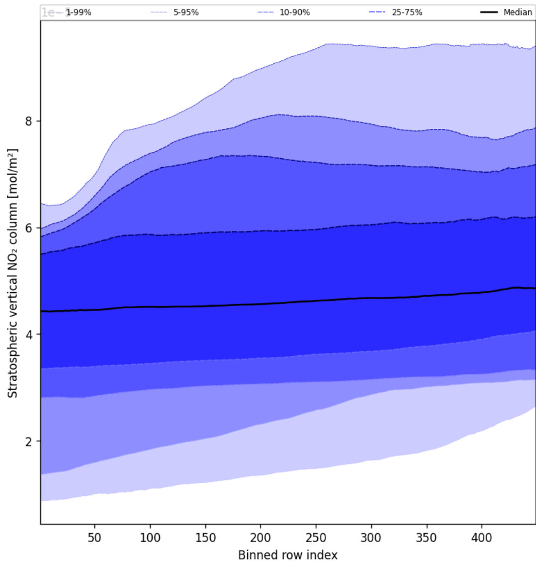
Figure 51: Along track statistics of “Stratospheric vertical NO 2 column” for 2025-08-20 to 2025-08-21
