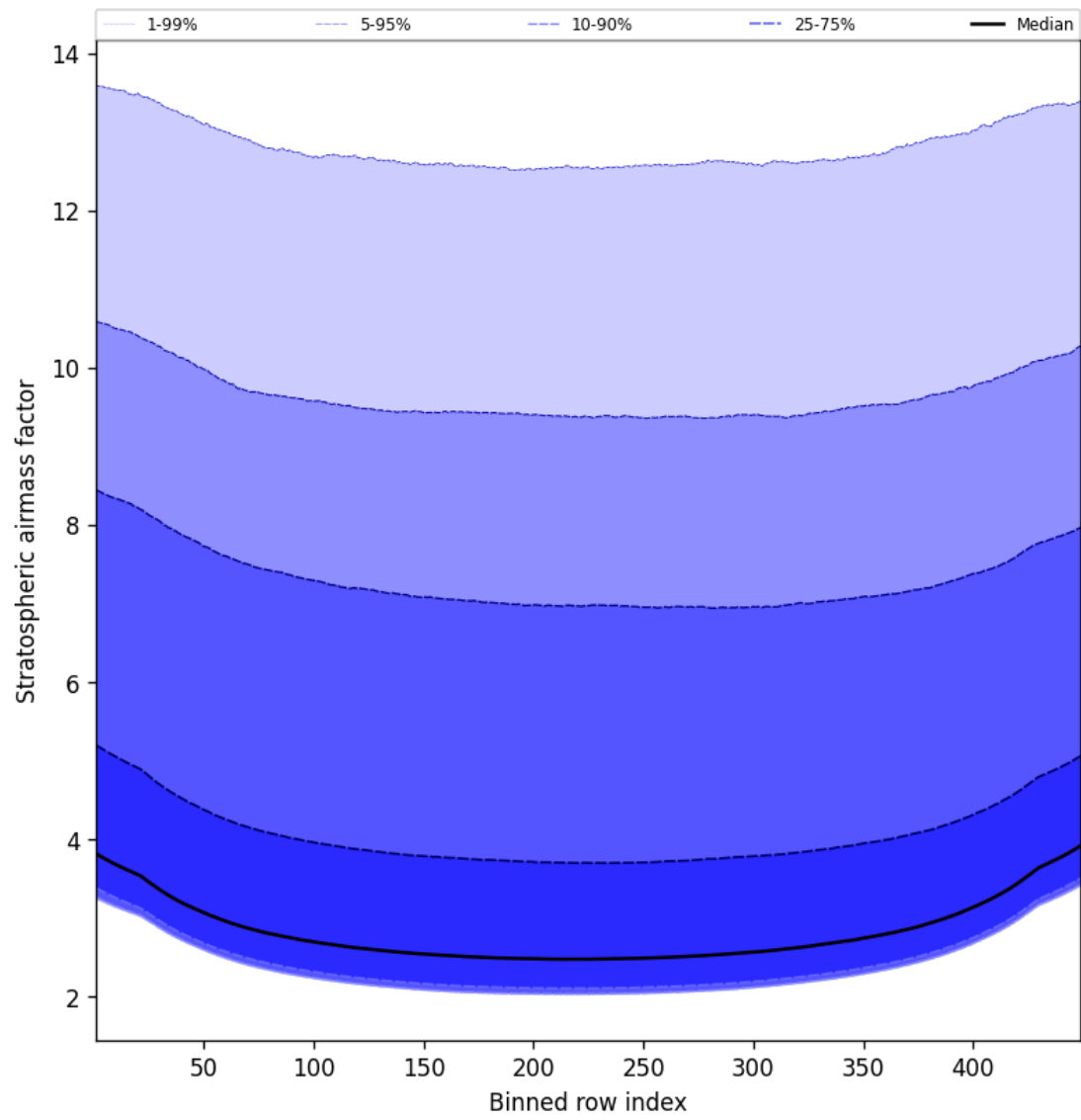
Figure 59: Along track statistics of “Stratospheric airmass factor” for 2025-08-20 to 2025-08-21
