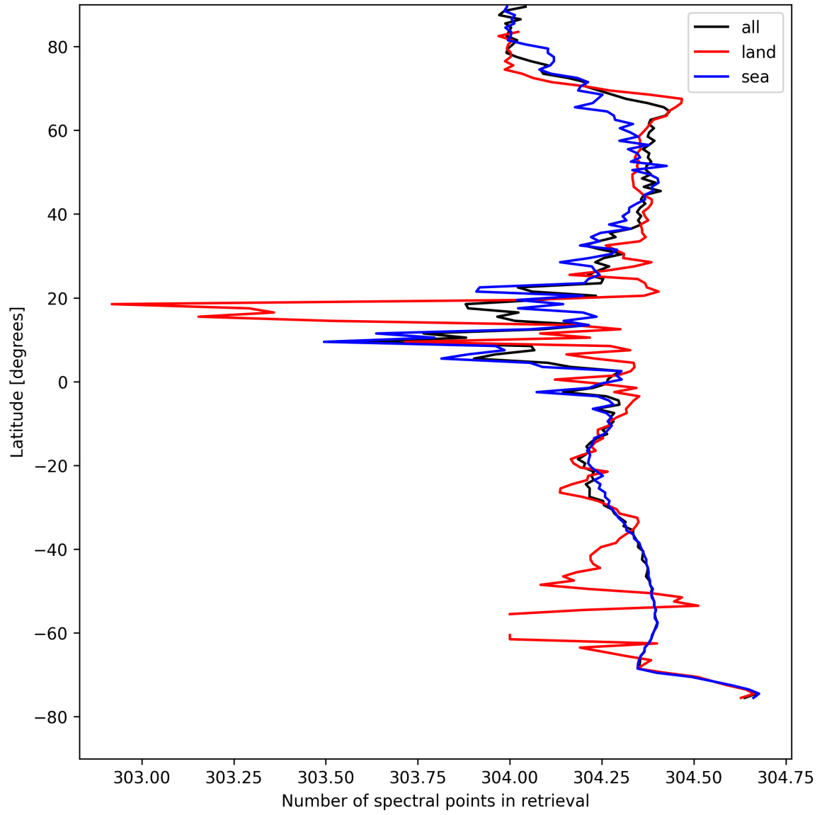
Figure 14: Zonal average of “Number of spectral points in retrieval” for 2025-08-20 to 2025-08-21.
