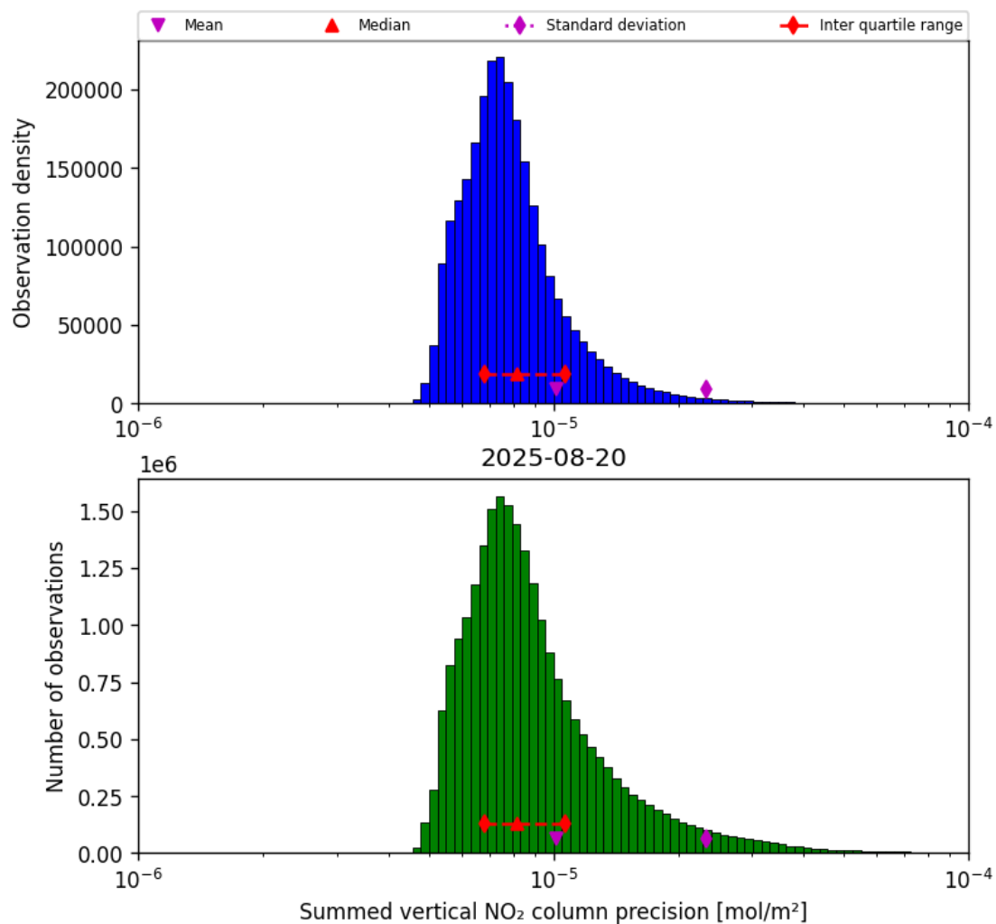
Figure 39: Histogram of “Summed vertical NO 2 column precision” for 2025-08-20 to 2025-08-21
