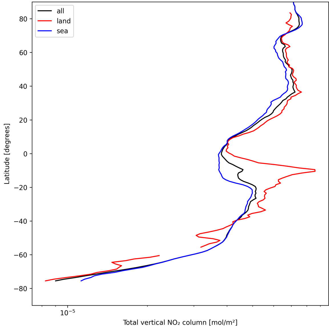
Figure 19: Zonal average of “Total vertical NO 2 column” for 2025-08-20 to 2025-08-21.
