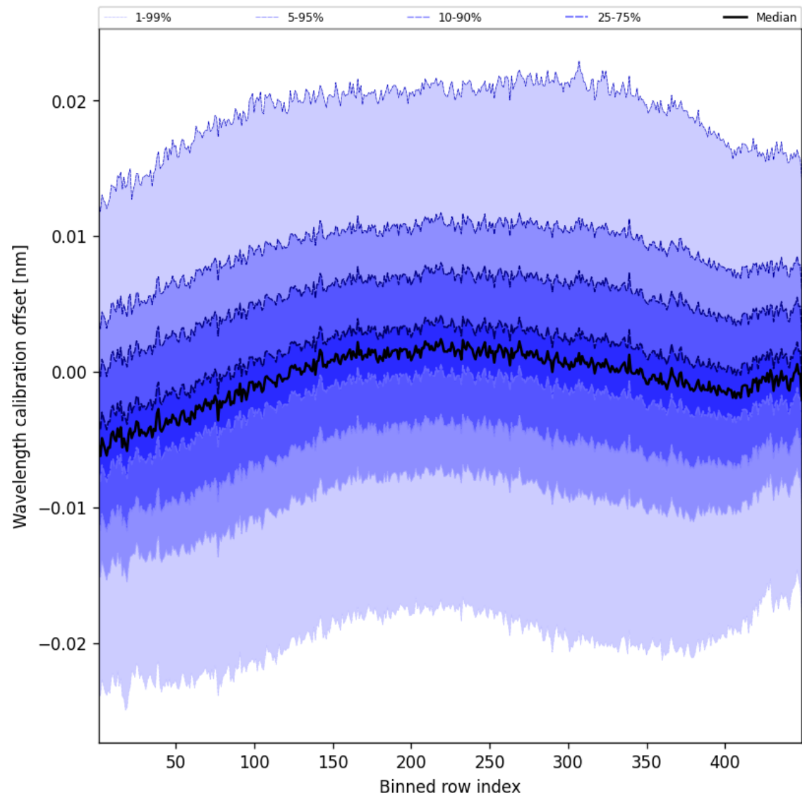
Figure 50: Along track statistics of “Wavelength calibration offset” for 2025-08-20 to 2025-08-21
