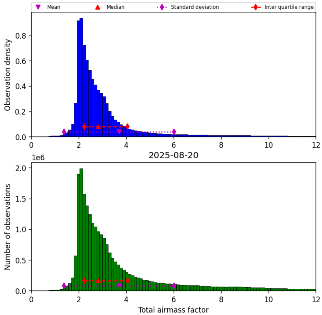
Figure 30: Histogram of “Total airmass factor” for 2025-08-20 to 2025-08-21
