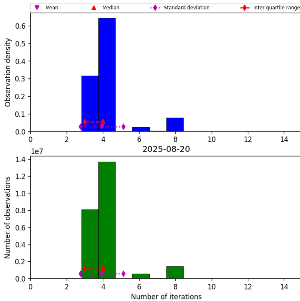
Figure 32: Histogram of “Number of iterations” for 2025-08-20 to 2025-08-21
