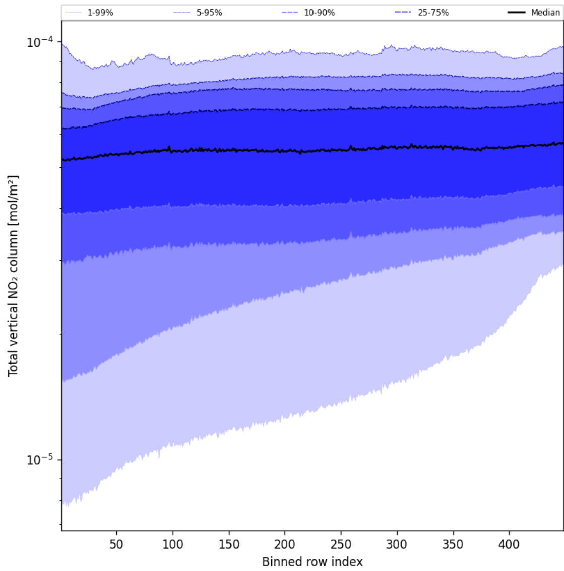
Figure 53: Along track statistics of “Total vertical NO 2 column” for 2025-08-20 to 2025-08-21
