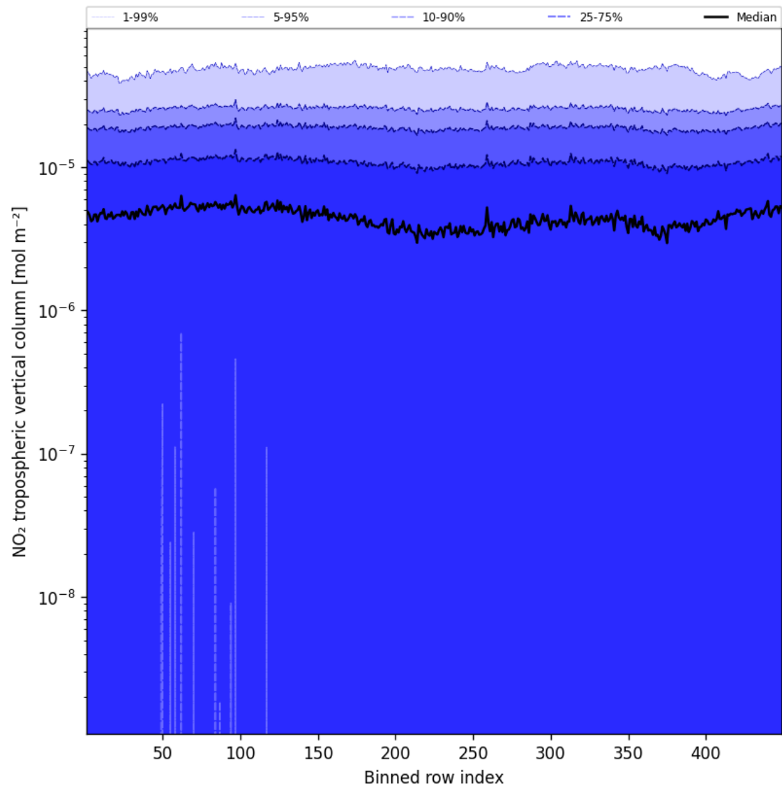
Figure 44: Along track statistics of "NO 2 tropospheric vertical column" for 2025-08-20 to 2025-08-21
