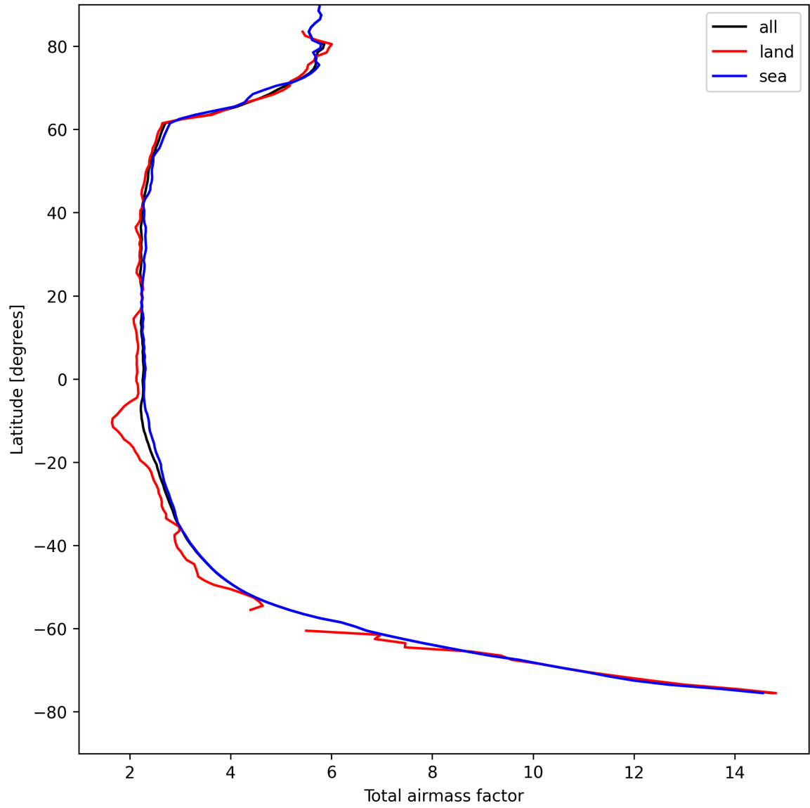
Figure 13: Zonal average of “Total airmass factor” for 2025-08-20 to 2025-08-21.
