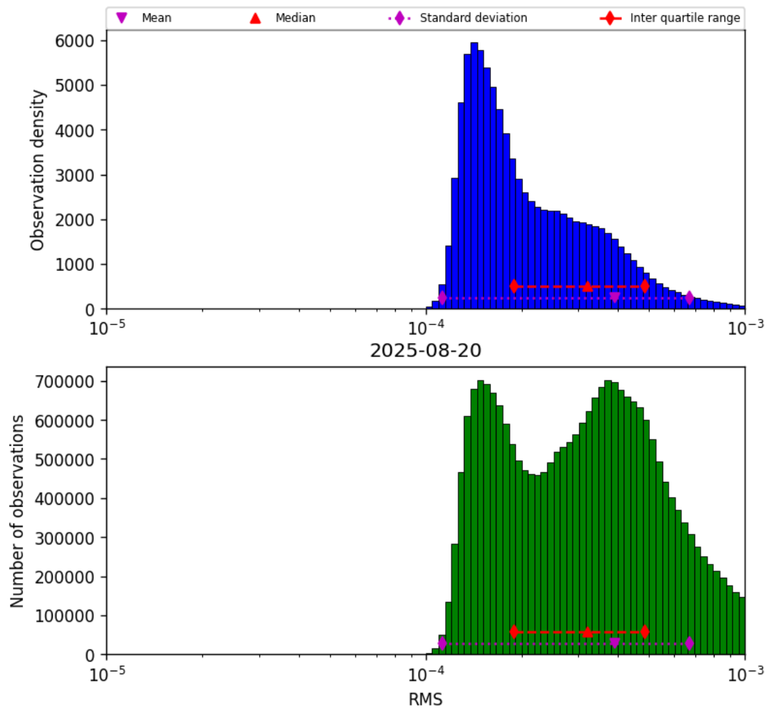
Figure 41: Histogram of “RMS” for 2025-08-20 to 2025-08-21
