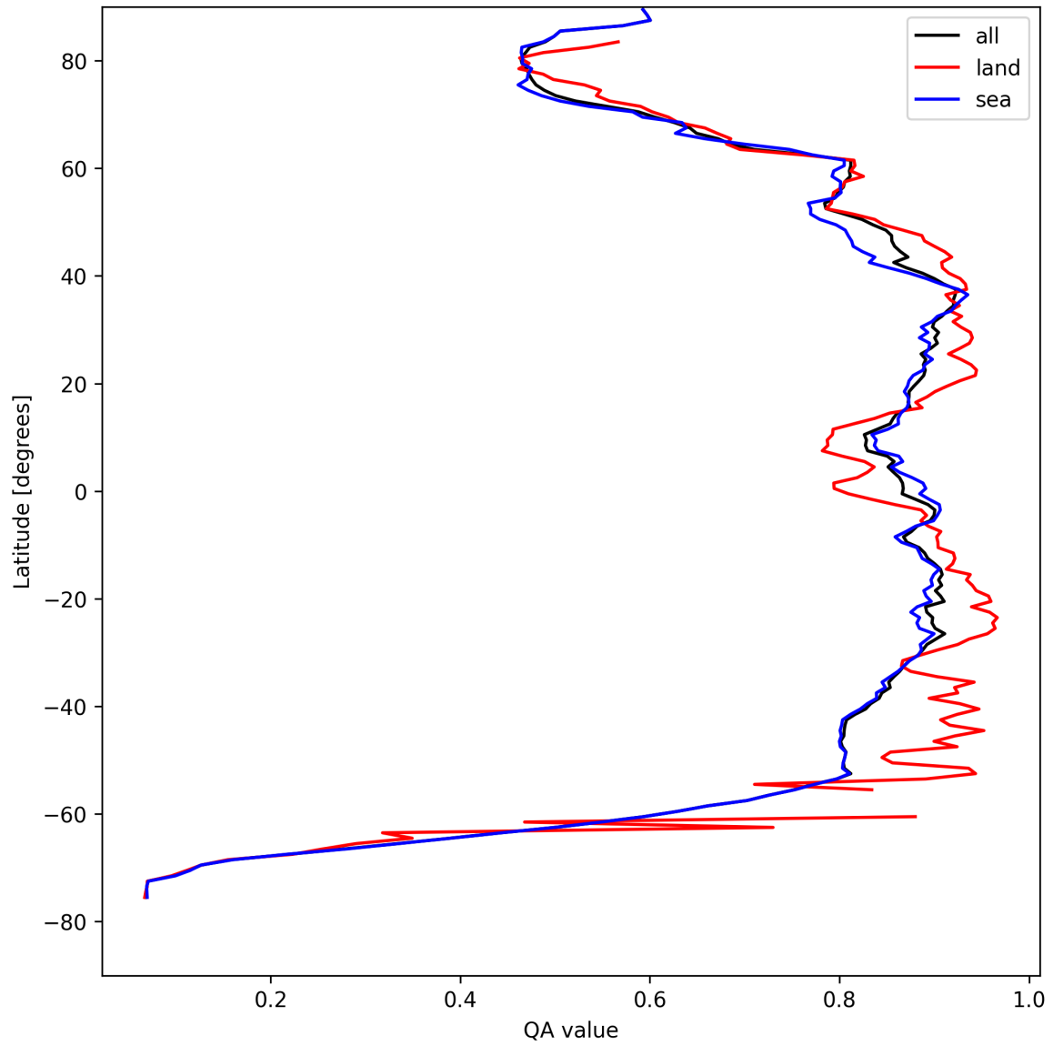
Figure 9: Zonal average of “QA value” for 2025-08-20 to 2025-08-21.
