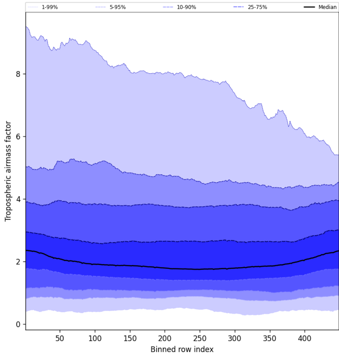
Figure 46: Along track statistics of “Tropospheric airmass factor” for 2025-08-22 to 2025-08-23
