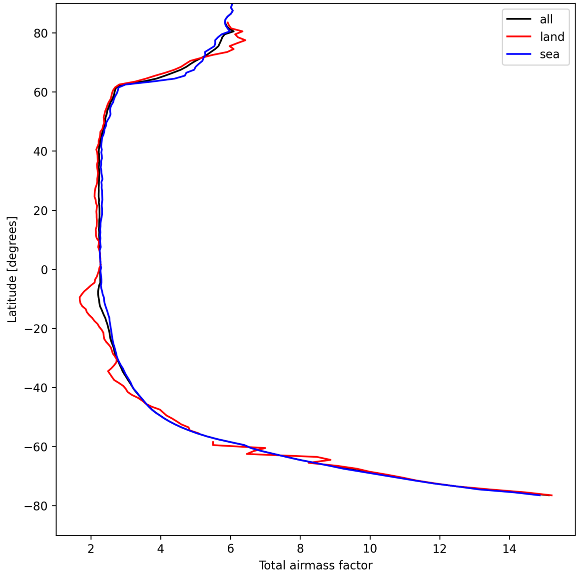
Figure 13: Zonal average of “Total airmass factor” for 2025-08-22 to 2025-08-23.
