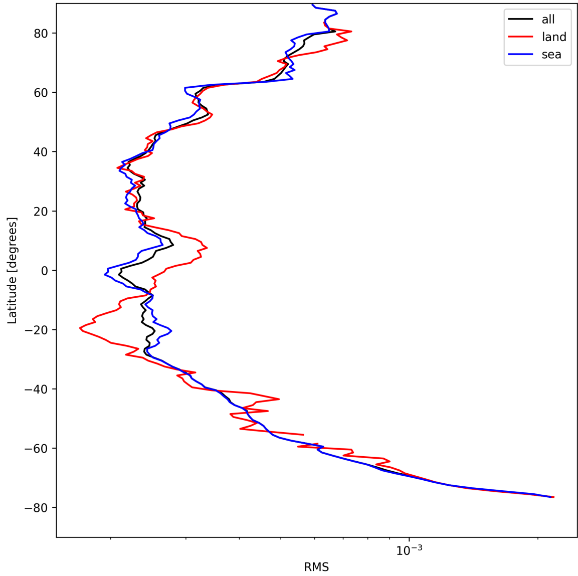
Figure 24: Zonal average of “RMS” for 2025-08-22 to 2025-08-23.
