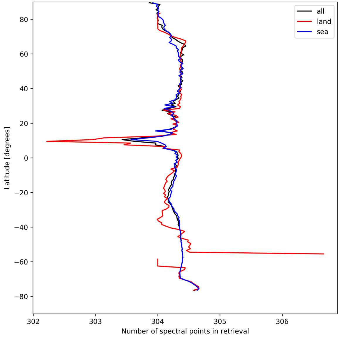
Figure 14: Zonal average of “Number of spectral points in retrieval” for 2025-08-22 to 2025-08-23.
