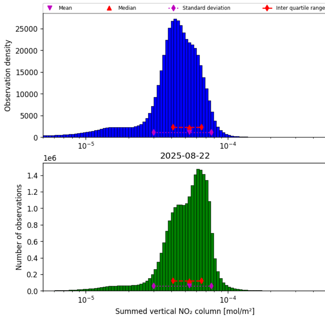
Figure 38: Histogram of “Summed vertical NO 2 column” for 2025-08-22 to 2025-08-23
