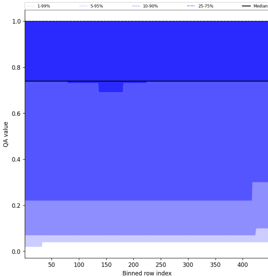
Figure 43: Along track statistics of “QA value” for 2025-08-22 to 2025-08-23
