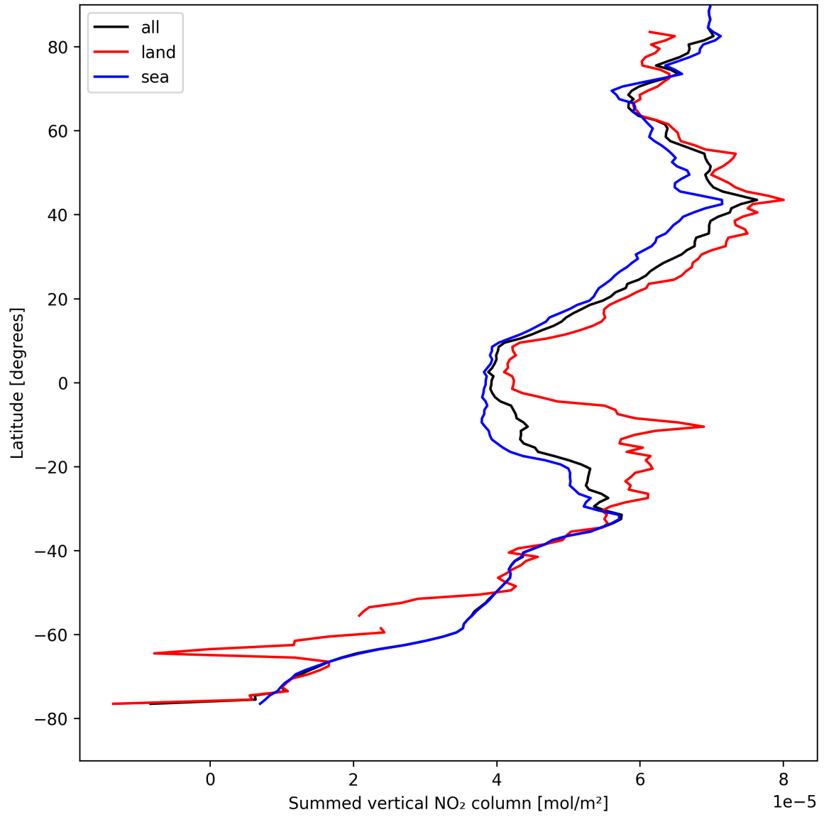
Figure 21: Zonal average of “Summed vertical NO 2 column” for 2025-08-22 to 2025-08-23.
