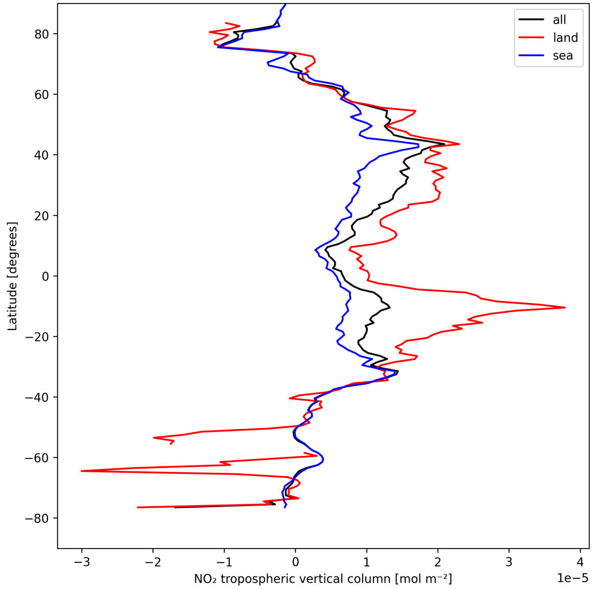
Figure 10: Zonal average of “NO 2 tropospheric vertical column” for 2025-08-22 to 2025-08-23.
