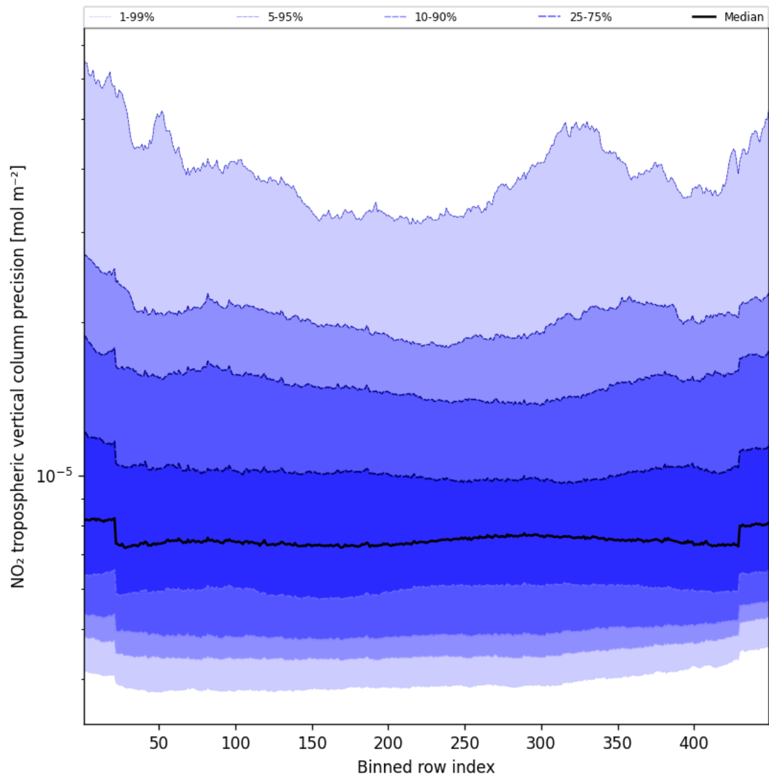
Figure 45: Along track statistics of “NO 2 tropospheric vertical column precision” for 2025-08-22 to 2025-08-23
