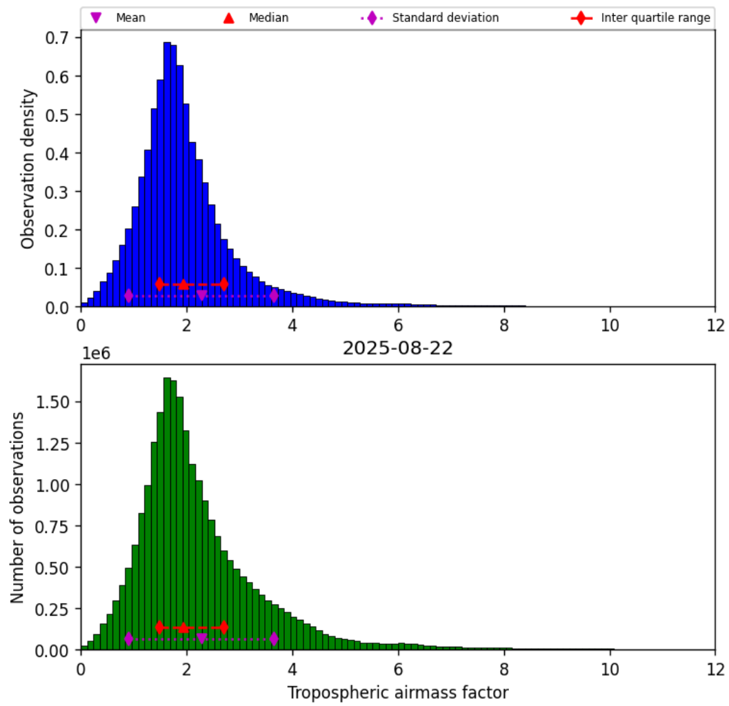
Figure 29: Histogram of “Tropospheric airmass factor” for 2025-08-22 to 2025-08-23
