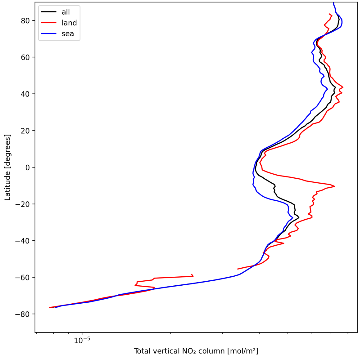
Figure 19: Zonal average of “Total vertical NO 2 column” for 2025-08-22 to 2025-08-23.
