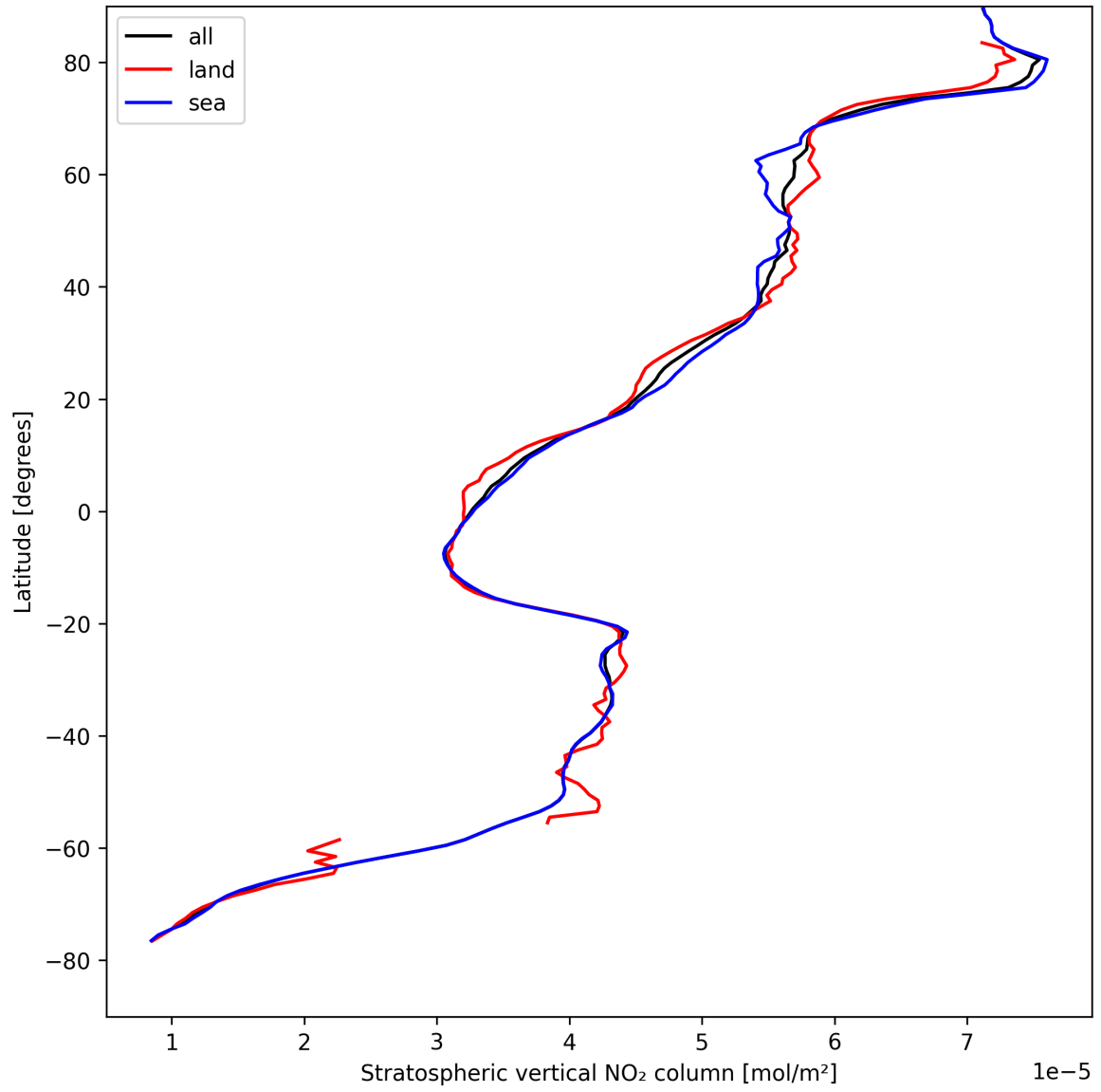
Figure 17: Zonal average of “Stratospheric vertical NO 2 column” for 2025-08-22 to 2025-08-23.
