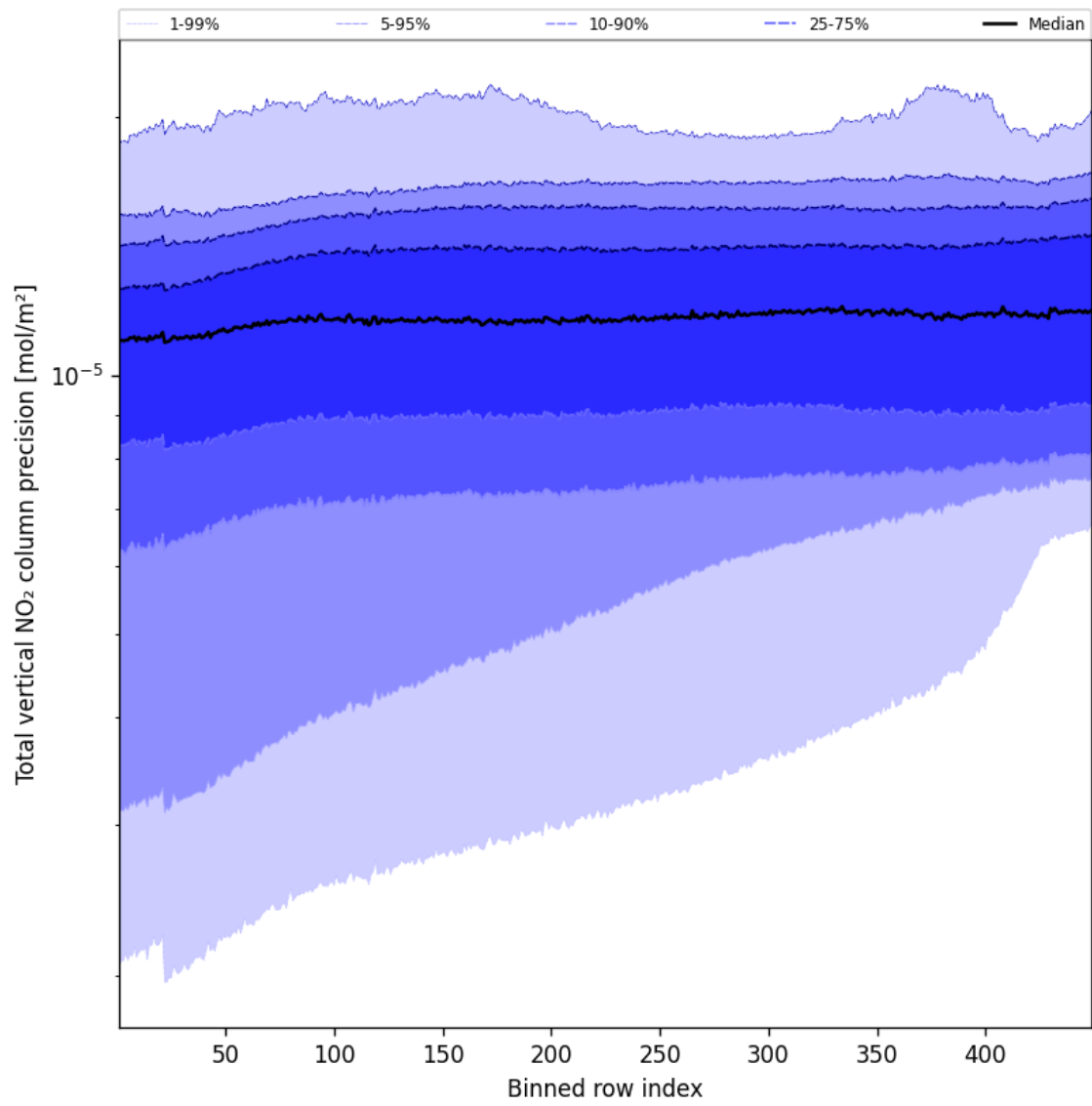
Figure 54: Along track statistics of “Total vertical NO 2 column precision” for 2025-08-22 to 2025-08-23
