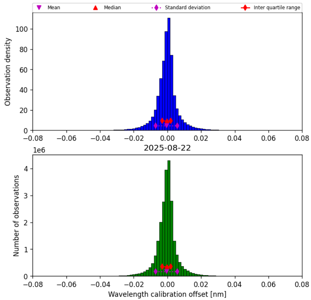
Figure 33: Histogram of “Wavelength calibration offset” for 2025-08-22 to 2025-08-23
