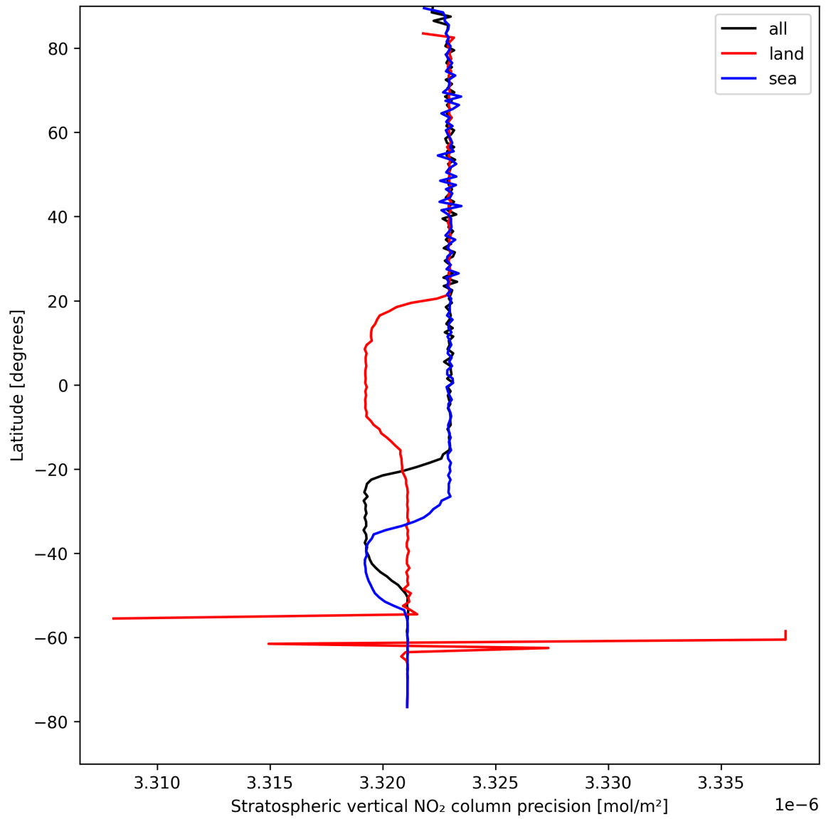
Figure 18: Zonal average of “Stratospheric vertical NO 2 column precision” for 2025-08-22 to 2025-08-23.
