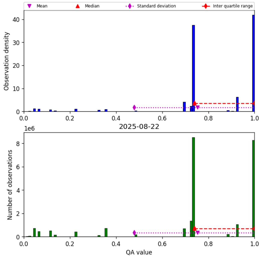
Figure 26: Histogram of “QA value” for 2025-08-22 to 2025-08-23
