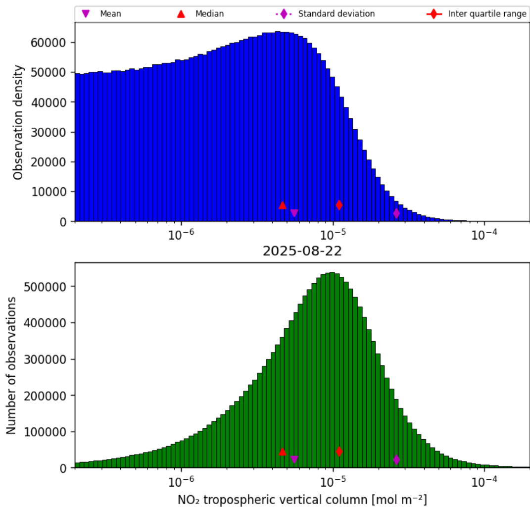
Figure 27: Histogram of “NO 2 tropospheric vertical column” for 2025-08-22 to 2025-08-23
