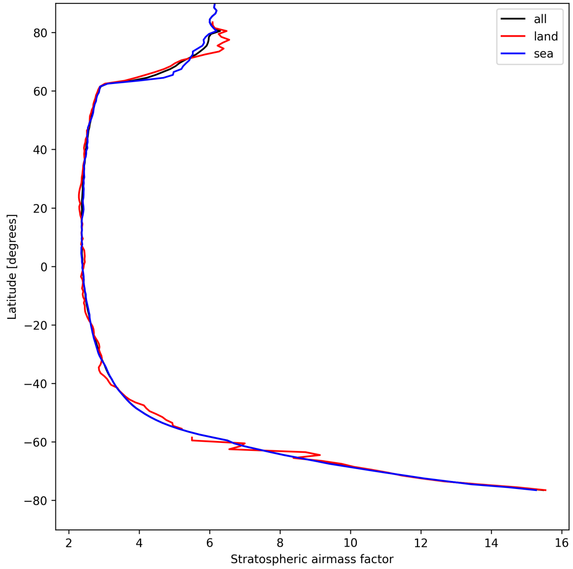
Figure 25: Zonal average of “Stratospheric airmass factor” for 2025-08-22 to 2025-08-23.
