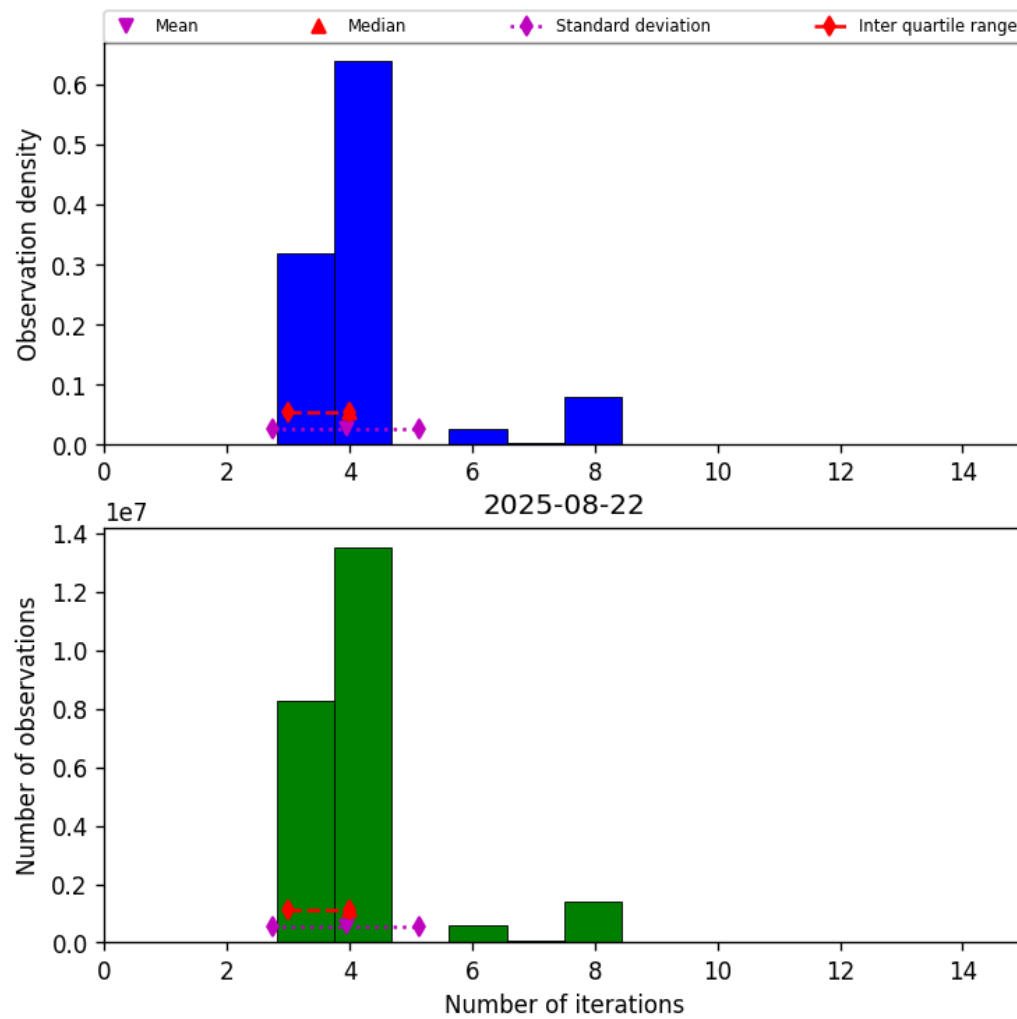
Figure 32: Histogram of “Number of iterations” for 2025-08-22 to 2025-08-23
