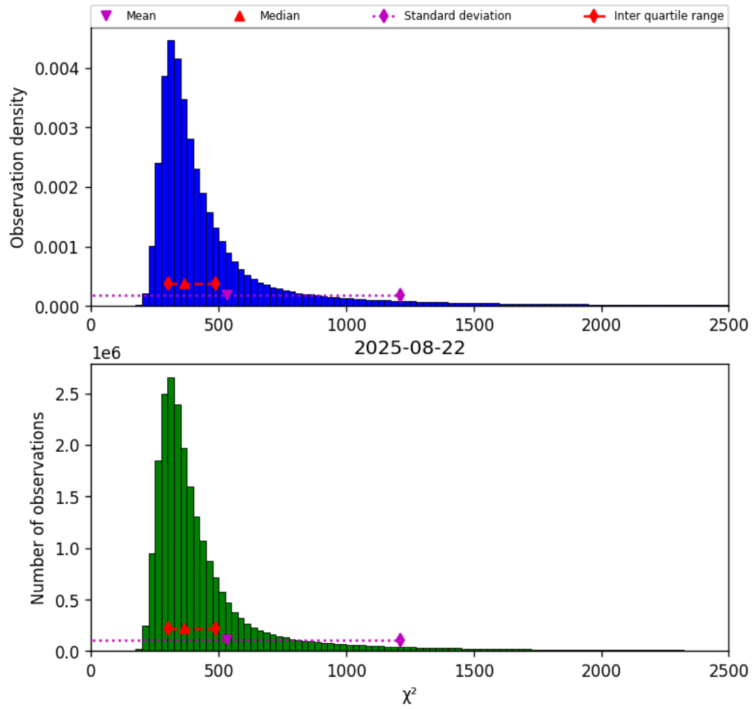
Figure 40: Histogram of “ \chi^2 ” for 2025-08-22 to 2025-08-23
