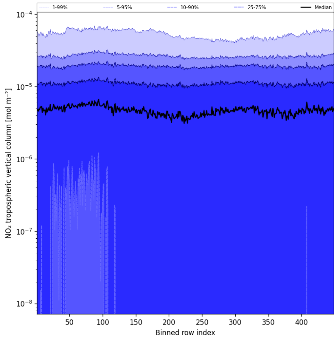
Figure 44: Along track statistics of “NO 2 tropospheric vertical column” for 2025-08-22 to 2025-08-23
