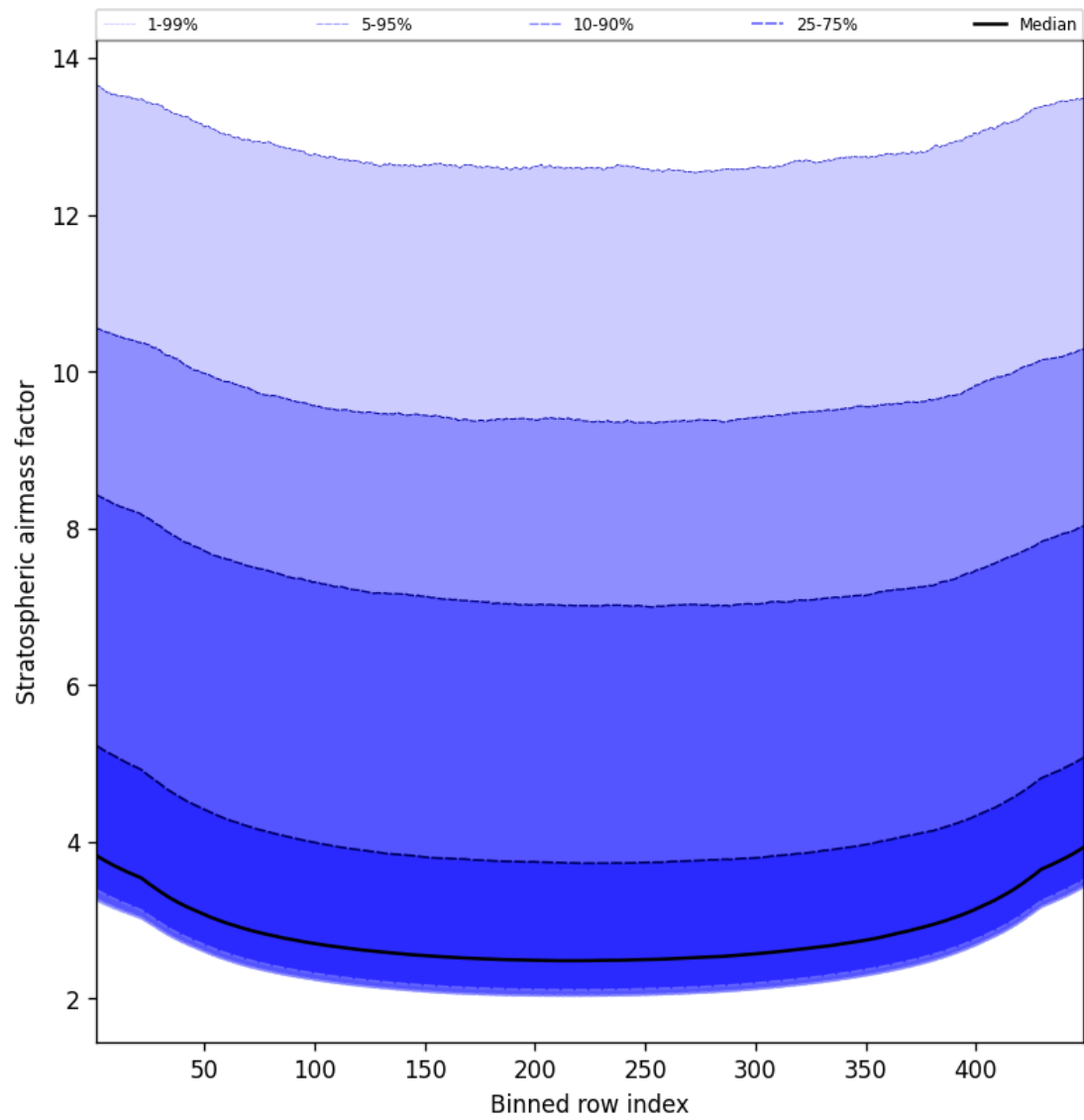
Figure 59: Along track statistics of “Stratospheric airmass factor” for 2025-08-22 to 2025-08-23
