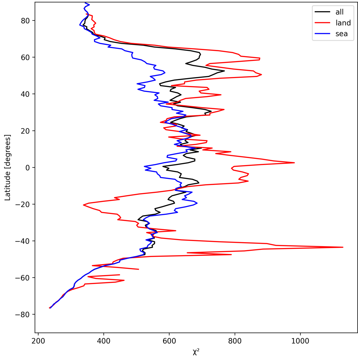
Figure 23: Zonal average of “ \chi^2 ” for 2025-08-22 to 2025-08-23.
