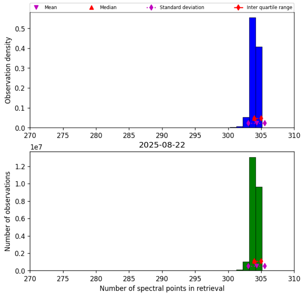
Figure 31: Histogram of “Number of spectral points in retrieval” for 2025-08-22 to 2025-08-23
