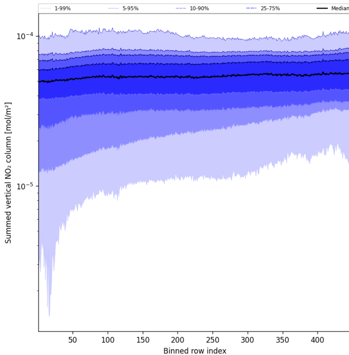
Figure 55: Along track statistics of “Summed vertical NO 2 column” for 2025-08-22 to 2025-08-23
