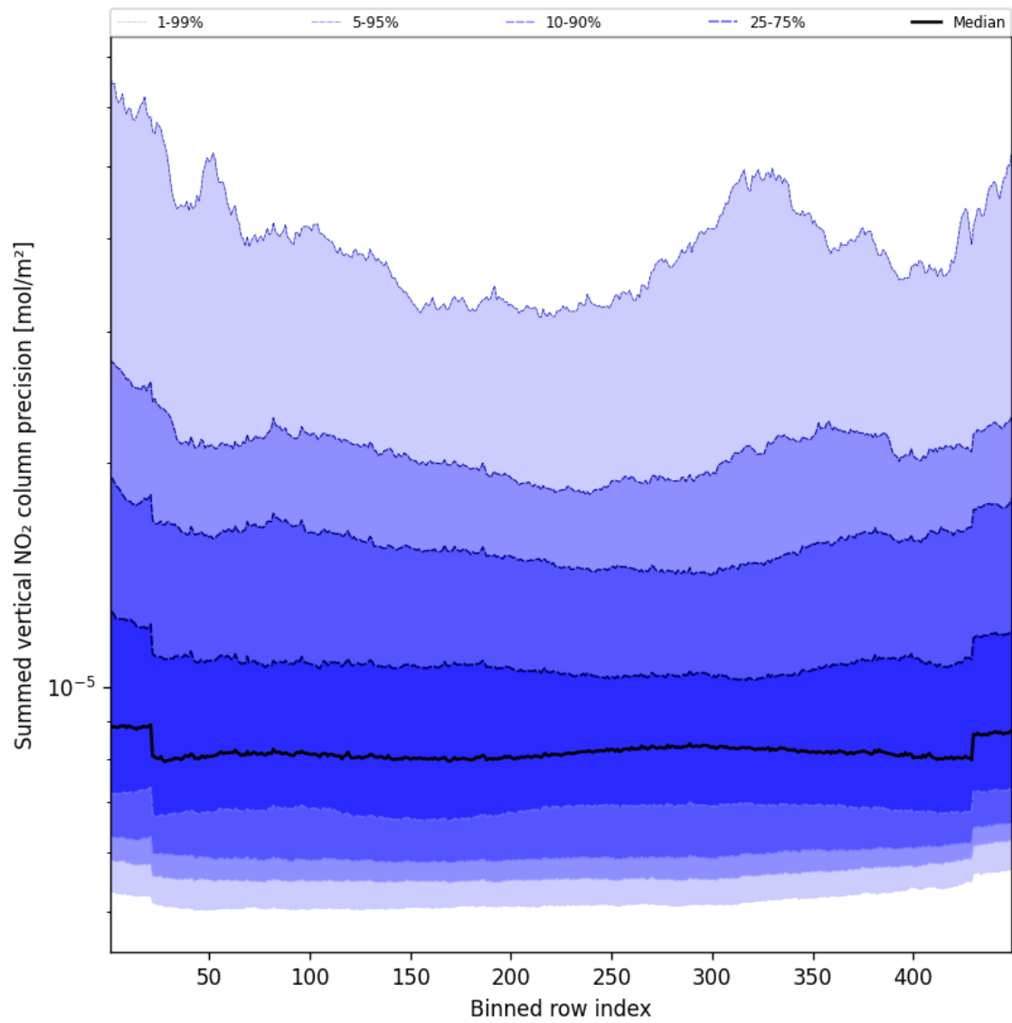
Figure 56: Along track statistics of “Summed vertical NO 2 column precision” for 2025-08-22 to 2025-08-23
