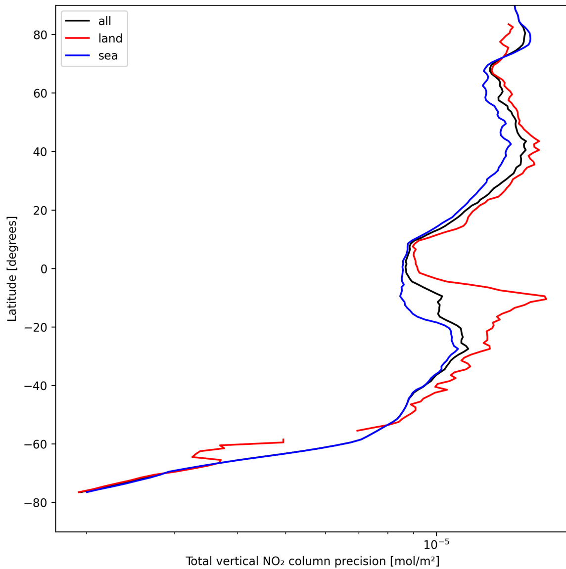
Figure 20: Zonal average of “Total vertical NO 2 column precision” for 2025-08-22 to 2025-08-23.
