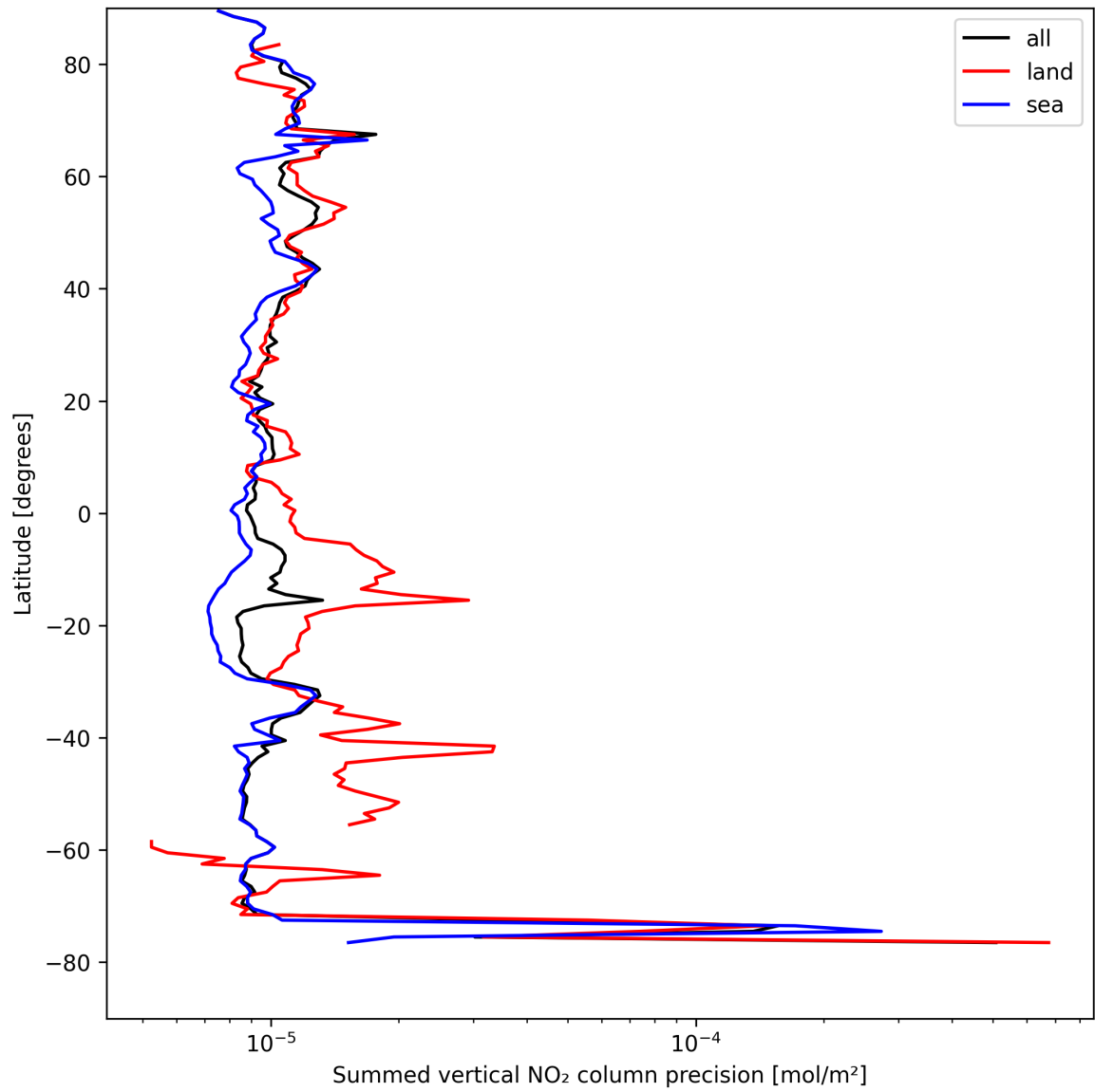
Figure 22: Zonal average of “Summed vertical NO 2 column precision” for 2025-08-22 to 2025-08-23.
