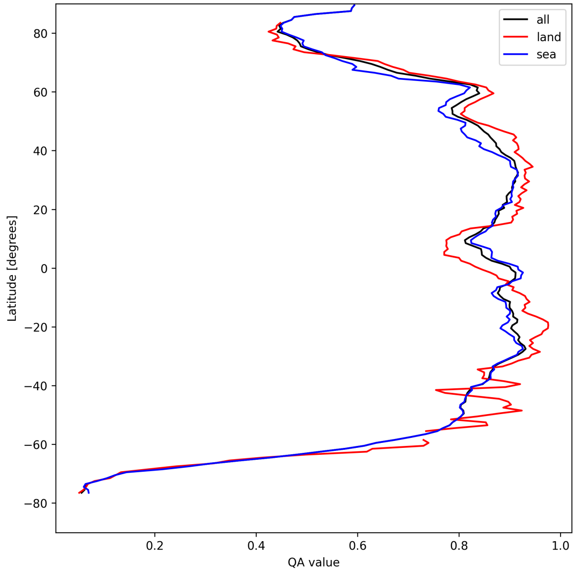
Figure 9: Zonal average of “QA value” for 2025-08-22 to 2025-08-23.
