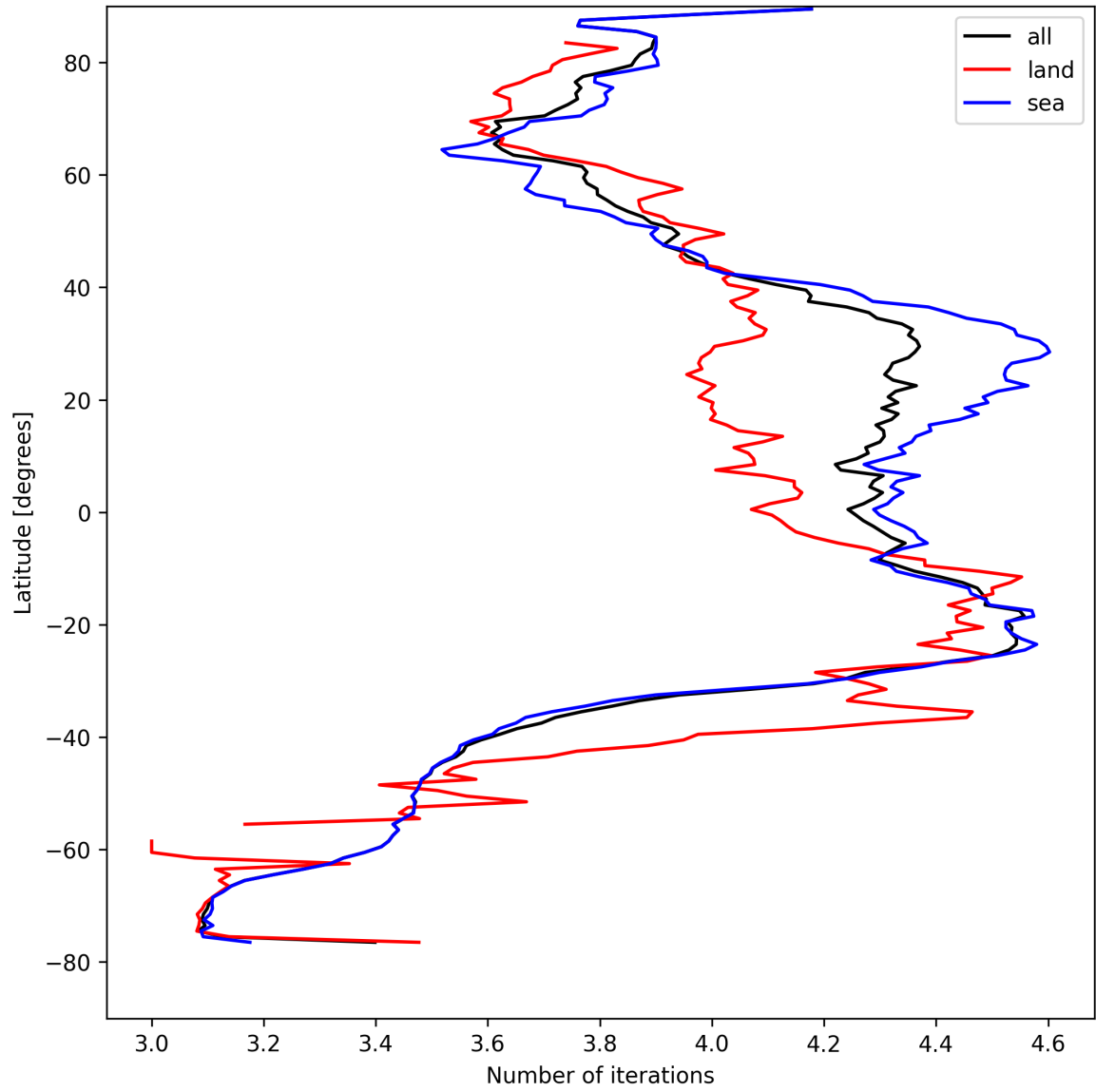
Figure 15: Zonal average of “Number of iterations” for 2025-08-22 to 2025-08-23.
