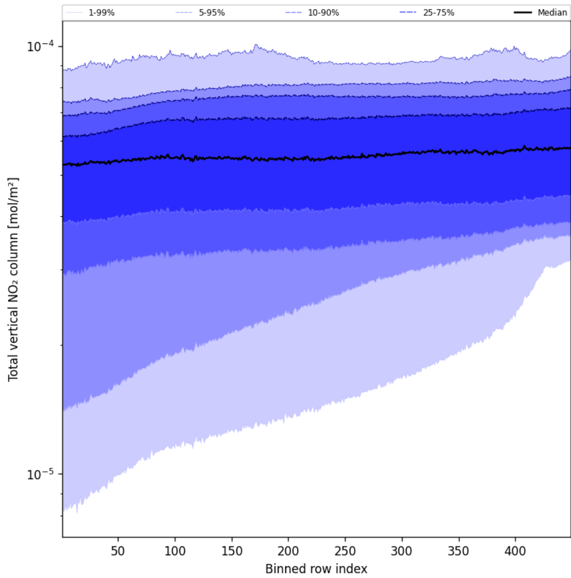
Figure 53: Along track statistics of “Total vertical NO 2 column” for 2025-08-22 to 2025-08-23
