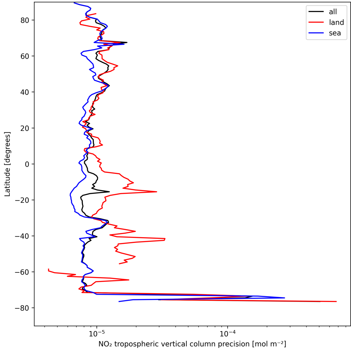
Figure 11: Zonal average of “NO 2 tropospheric vertical column precision” for 2025-08-22 to 2025-08-23.
