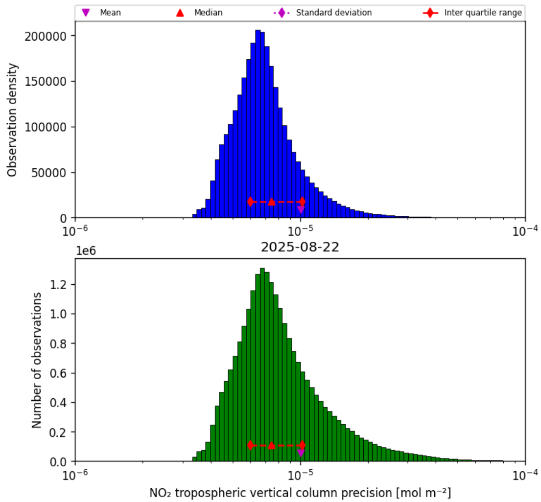
Figure 28: Histogram of “NO 2 tropospheric vertical column precision” for 2025-08-22 to 2025-08-23
