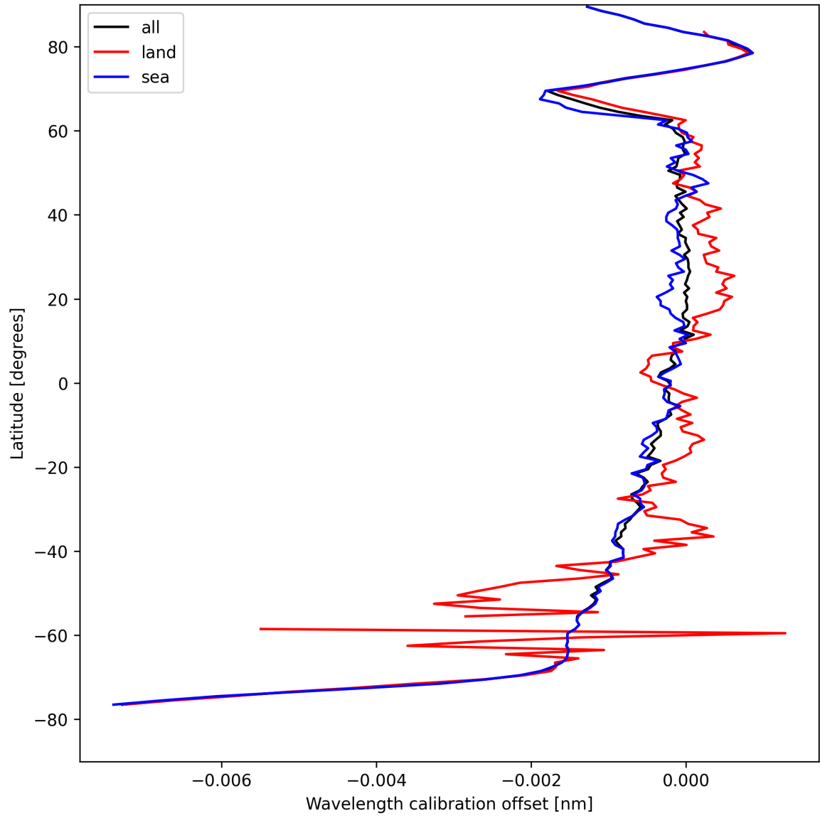
Figure 16: Zonal average of “Wavelength calibration offset” for 2025-08-22 to 2025-08-23.
