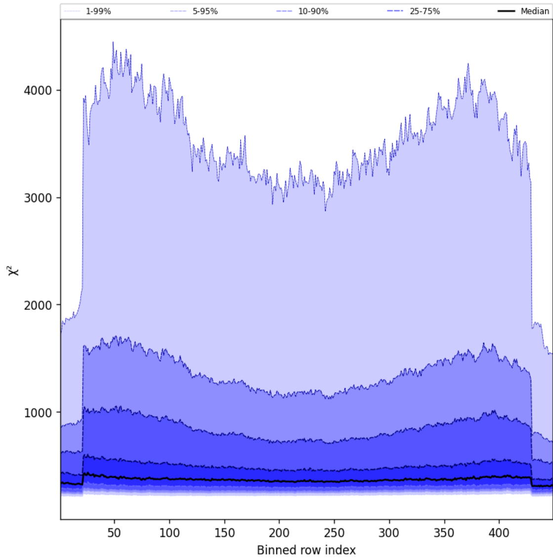
Figure 57: Along track statistics of “ \chi^2 ” for 2025-08-22 to 2025-08-23
