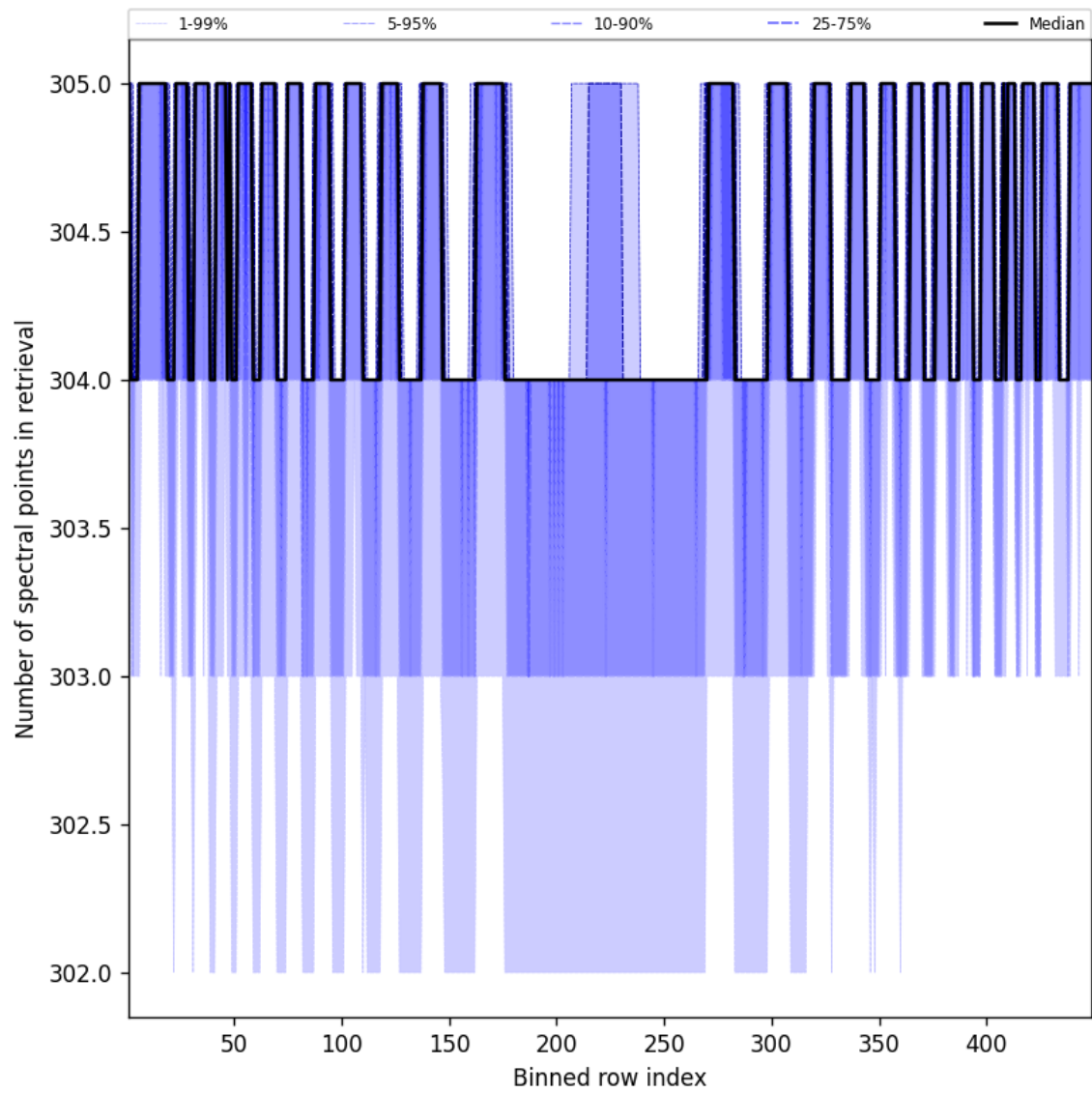
Figure 48: Along track statistics of “Number of spectral points in retrieval” for 2025-08-22 to 2025-08-23
