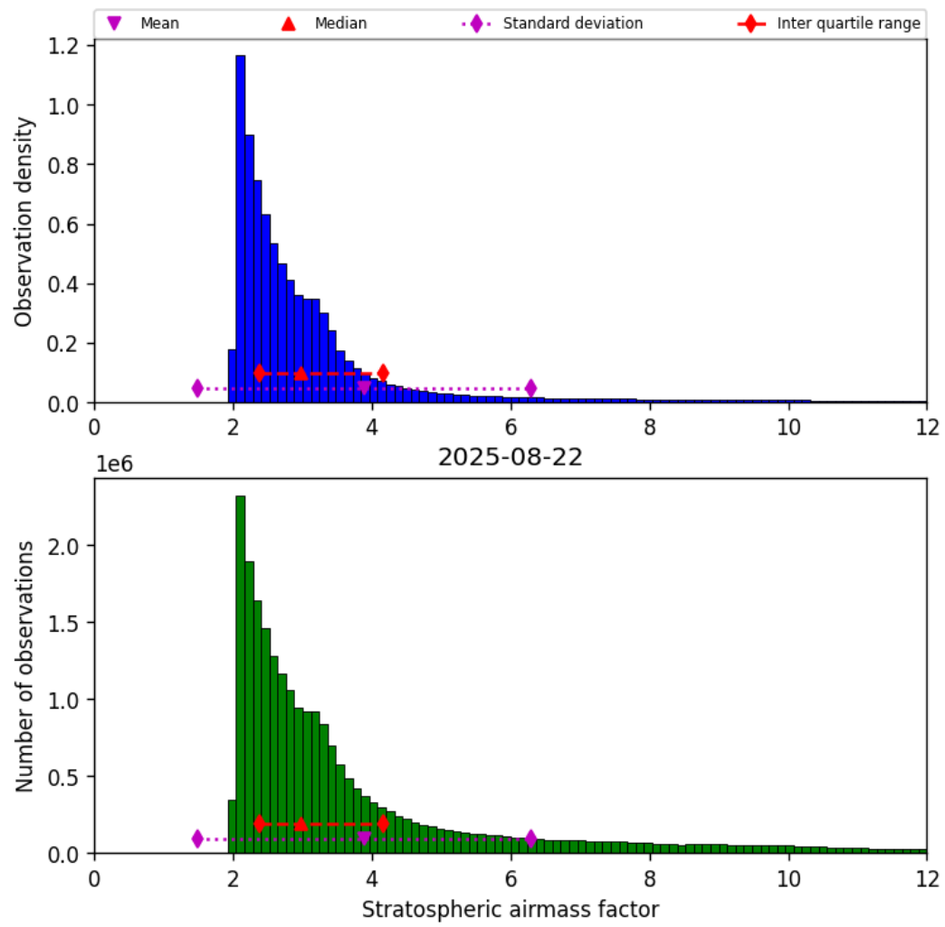
Figure 42: Histogram of “Stratospheric airmass factor” for 2025-08-22 to 2025-08-23
