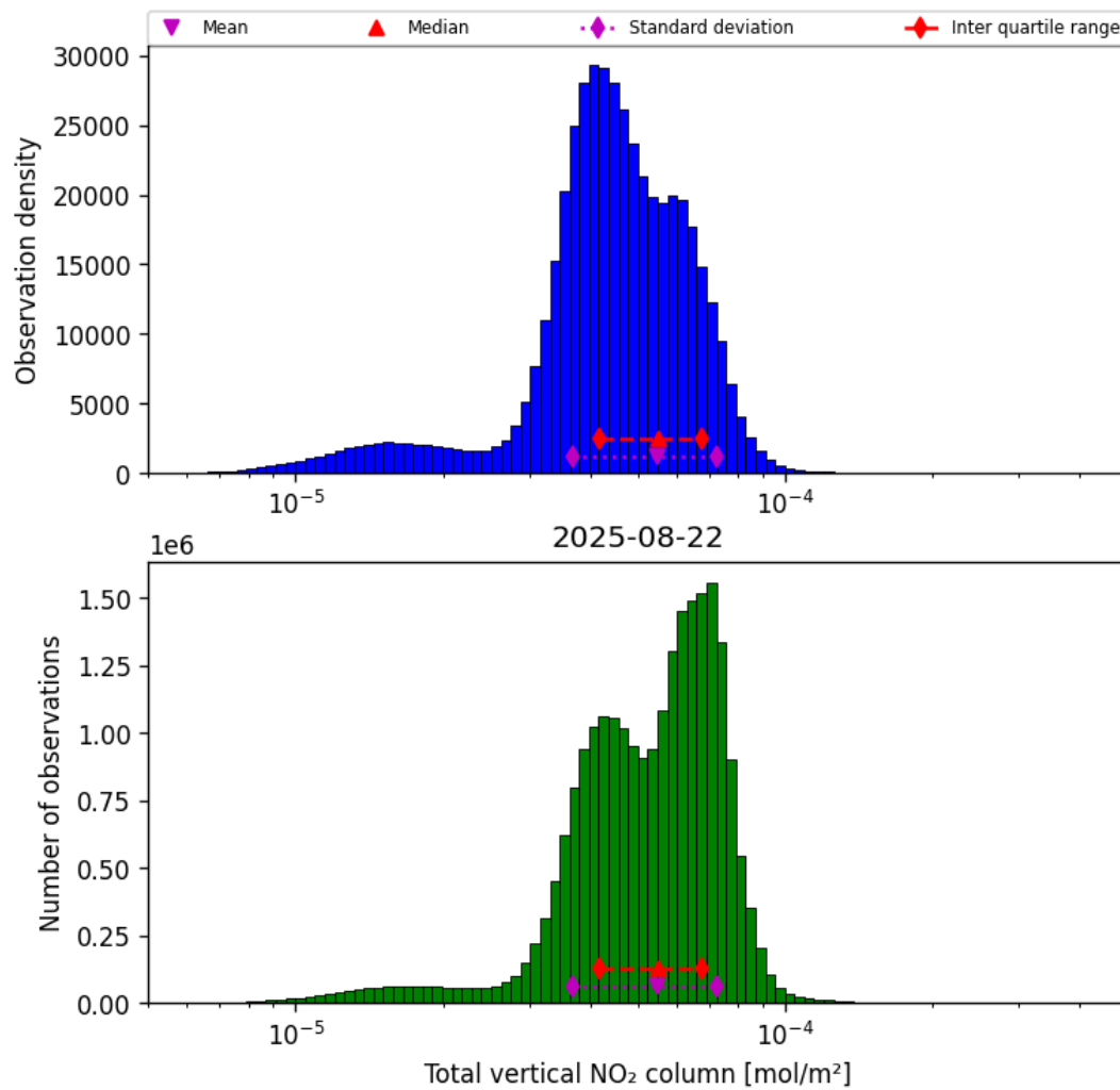
Figure 36: Histogram of “Total vertical NO 2 column” for 2025-08-22 to 2025-08-23
