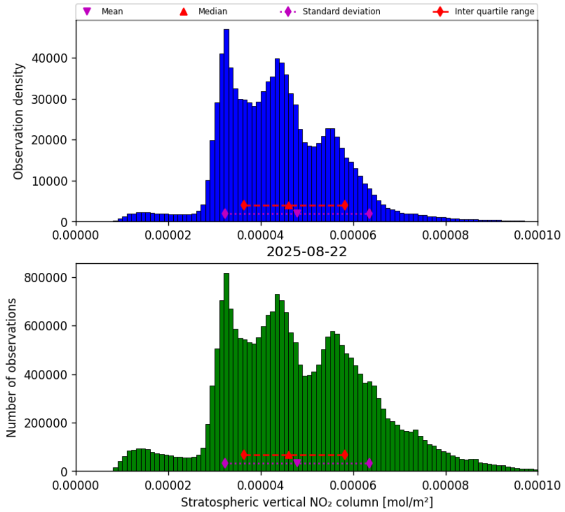
Figure 34: Histogram of “Stratospheric vertical NO 2 column” for 2025-08-22 to 2025-08-23
