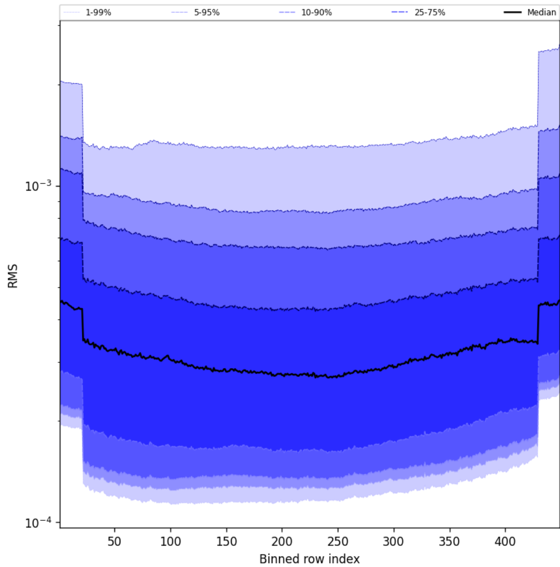
Figure 58: Along track statistics of “RMS” for 2025-08-22 to 2025-08-23
