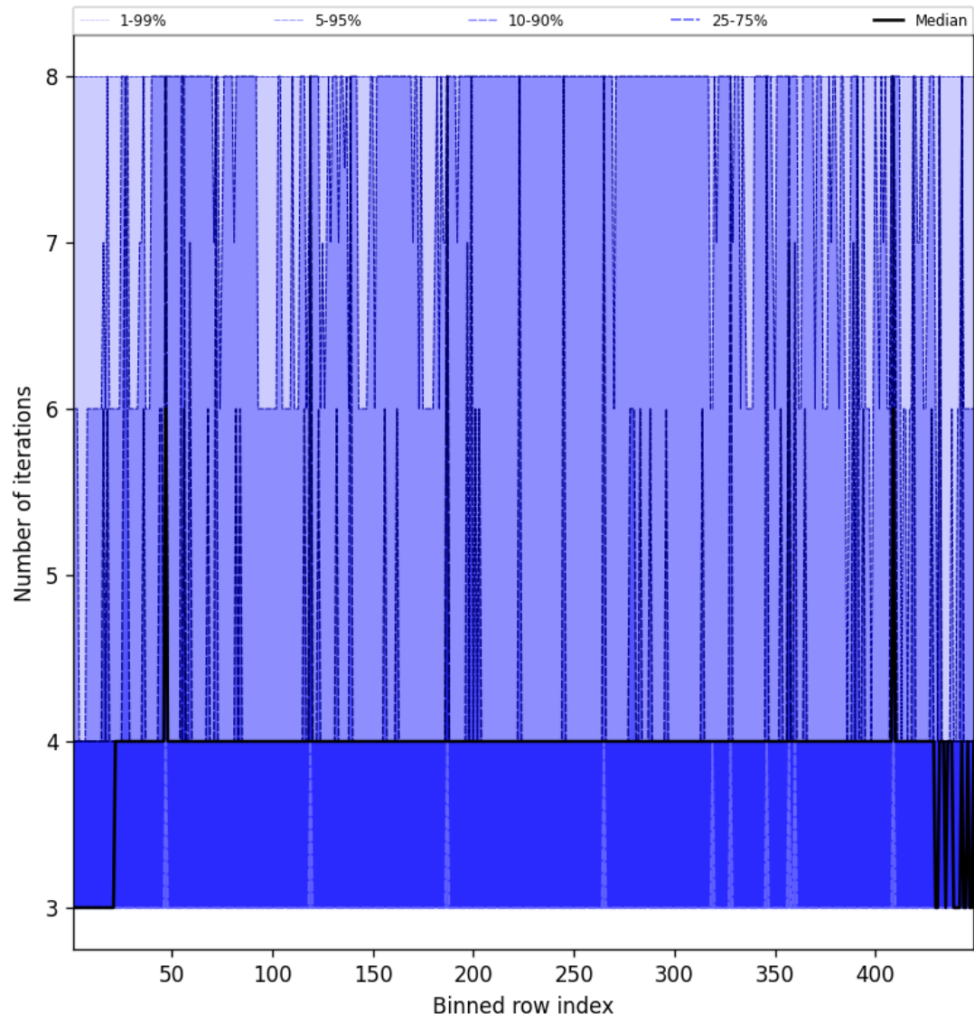
Figure 49: Along track statistics of “Number of iterations” for 2025-08-22 to 2025-08-23
