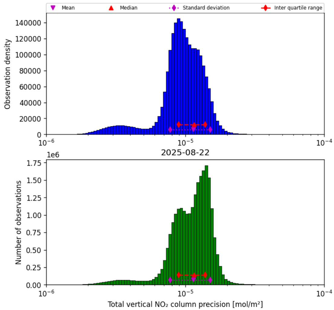
Figure 37: Histogram of “Total vertical NO 2 column precision” for 2025-08-22 to 2025-08-23
