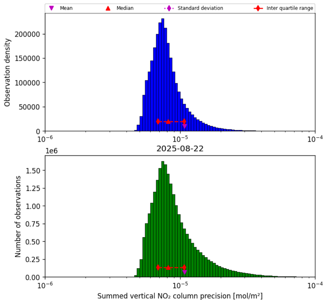
Figure 39: Histogram of “Summed vertical NO 2 column precision” for 2025-08-22 to 2025-08-23
