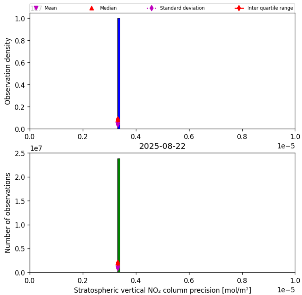
Figure 35: Histogram of “Stratospheric vertical NO 2 column precision” for 2025-08-22 to 2025-08-23
