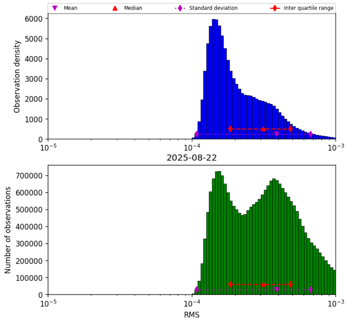
Figure 41: Histogram of “RMS” for 2025-08-22 to 2025-08-23
