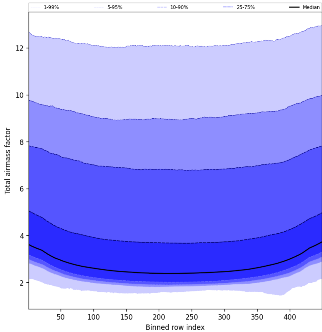
Figure 47: Along track statistics of “Total airmass factor” for 2025-08-22 to 2025-08-23
