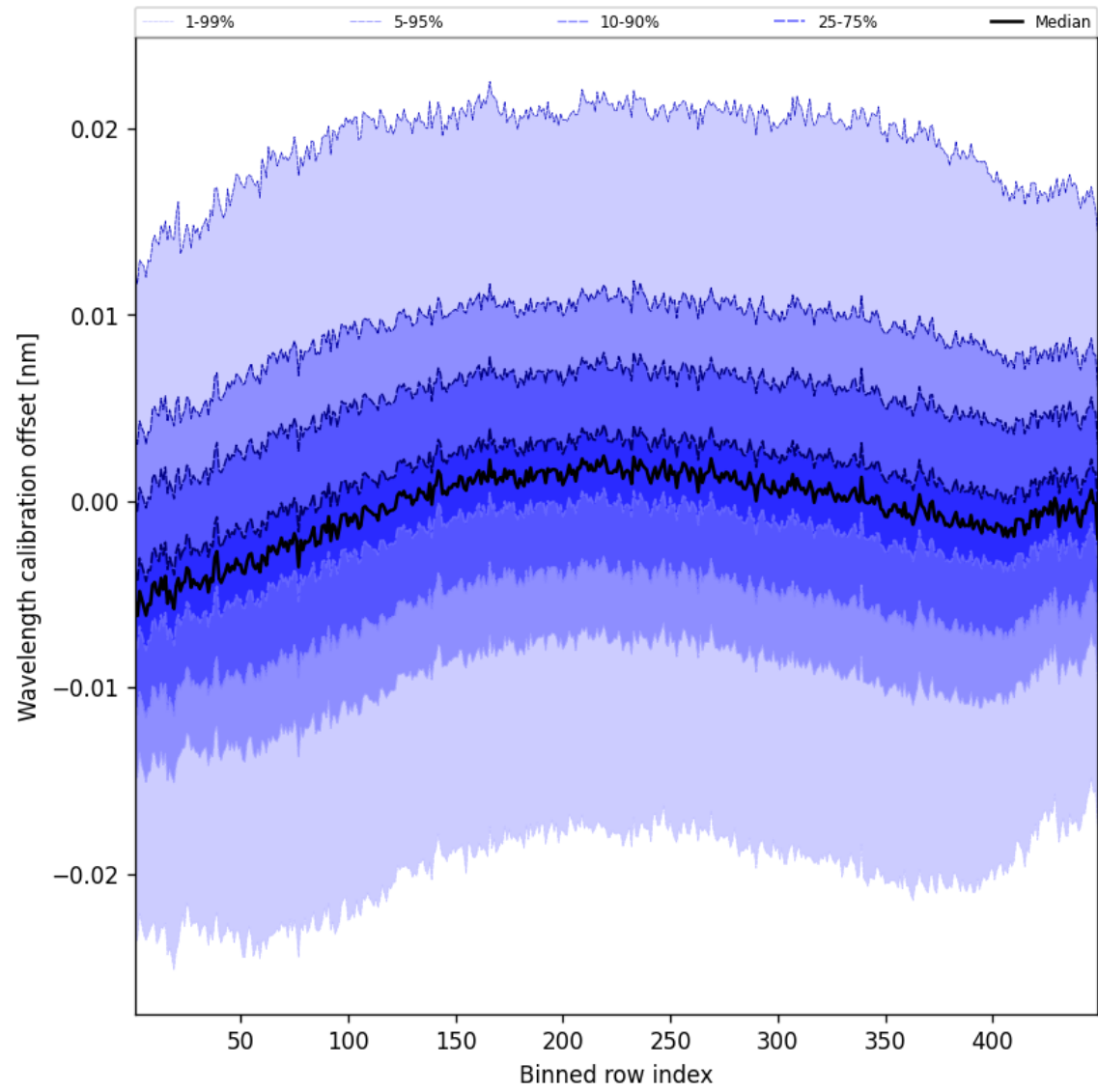
Figure 50: Along track statistics of “Wavelength calibration offset” for 2025-08-22 to 2025-08-23
