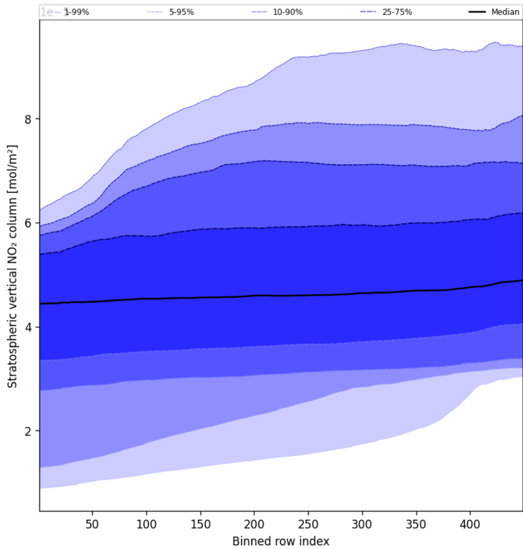
Figure 51: Along track statistics of “Stratospheric vertical NO 2 column” for 2025-08-22 to 2025-08-23
