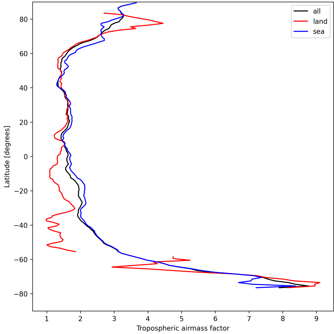
Figure 12: Zonal average of “Tropospheric airmass factor” for 2025-08-22 to 2025-08-23.
