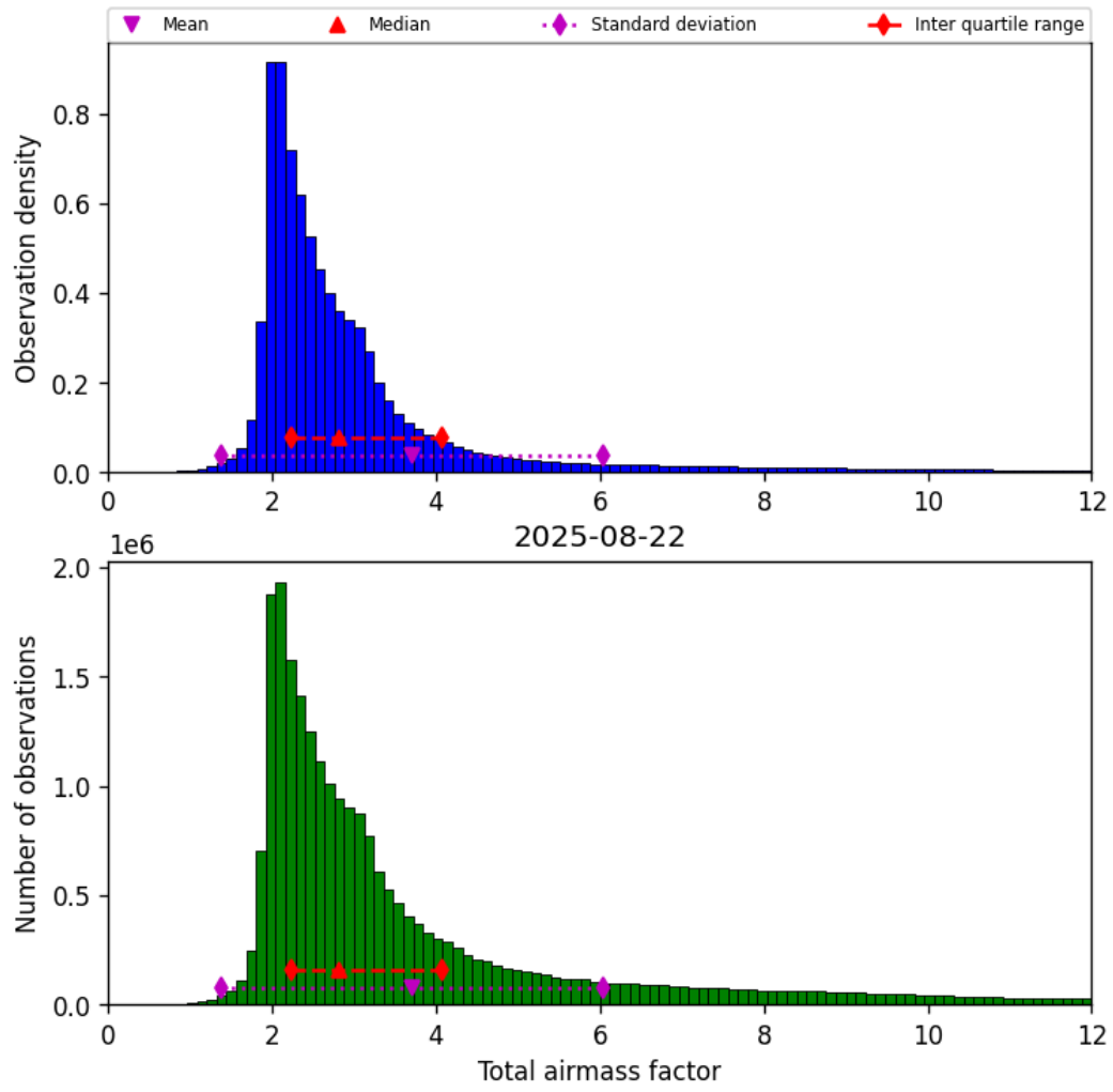
Figure 30: Histogram of “Total airmass factor” for 2025-08-22 to 2025-08-23
