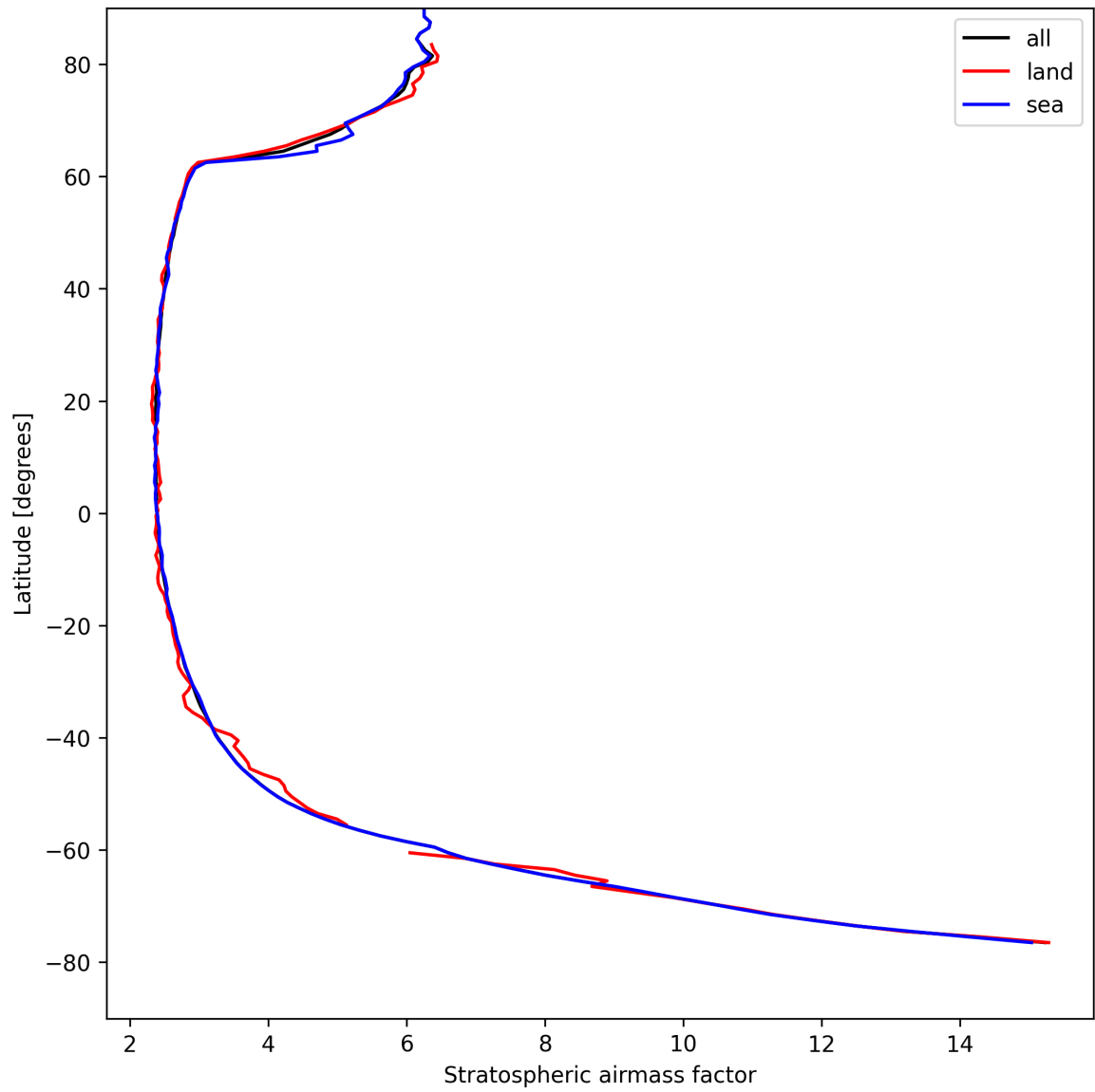
Figure 25: Zonal average of “Stratospheric airmass factor” for 2025-08-23 to 2025-08-23.
