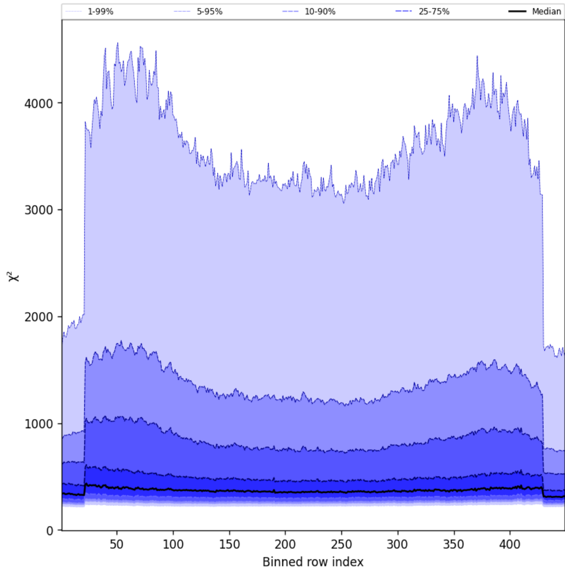
Figure 57: Along track statistics of “ \chi^2 ” for 2025-08-23 to 2025-08-23
