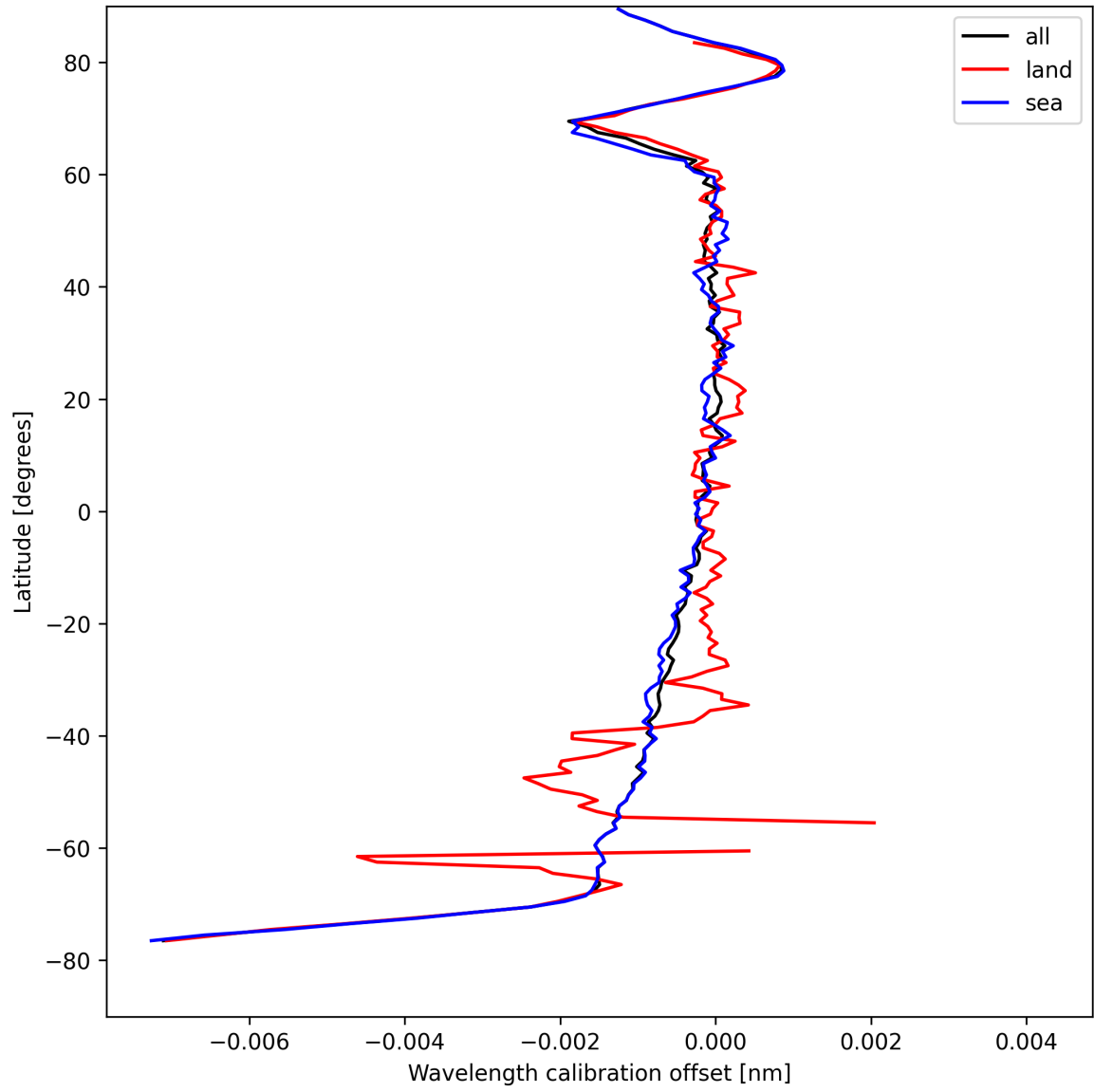
Figure 16: Zonal average of “Wavelength calibration offset” for 2025-08-23 to 2025-08-23.
