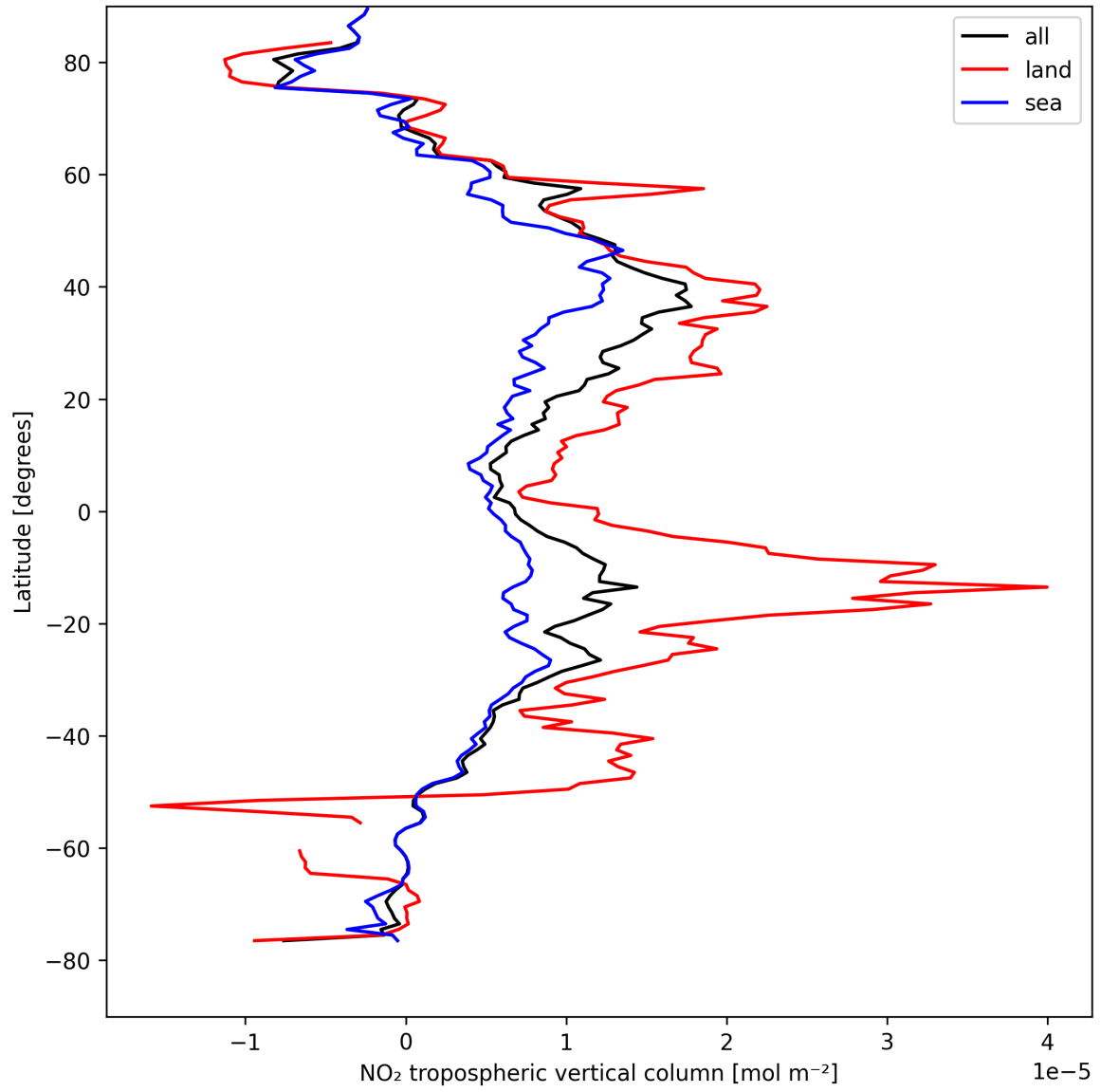
Figure 10: Zonal average of “NO 2 tropospheric vertical column” for 2025-08-23 to 2025-08-23.
