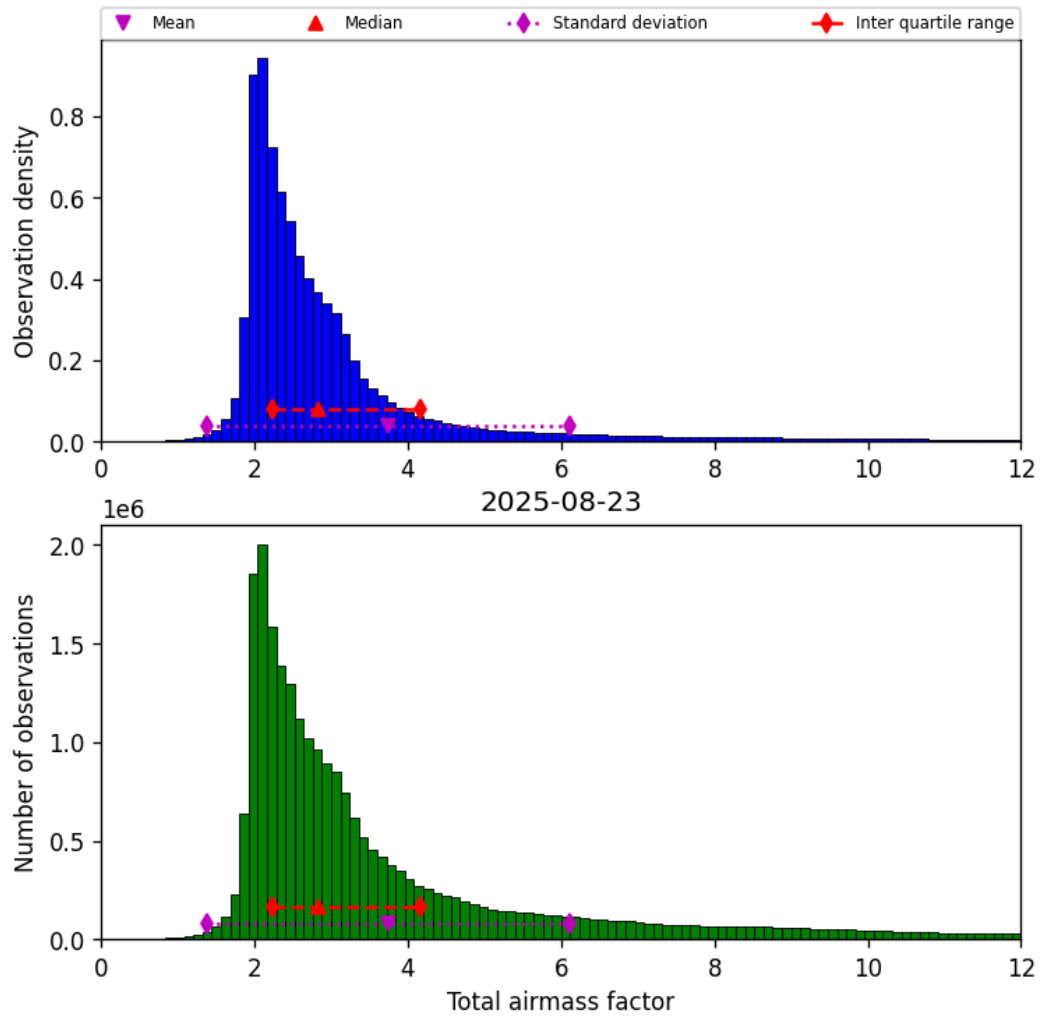
Figure 30: Histogram of “Total airmass factor” for 2025-08-23 to 2025-08-23
