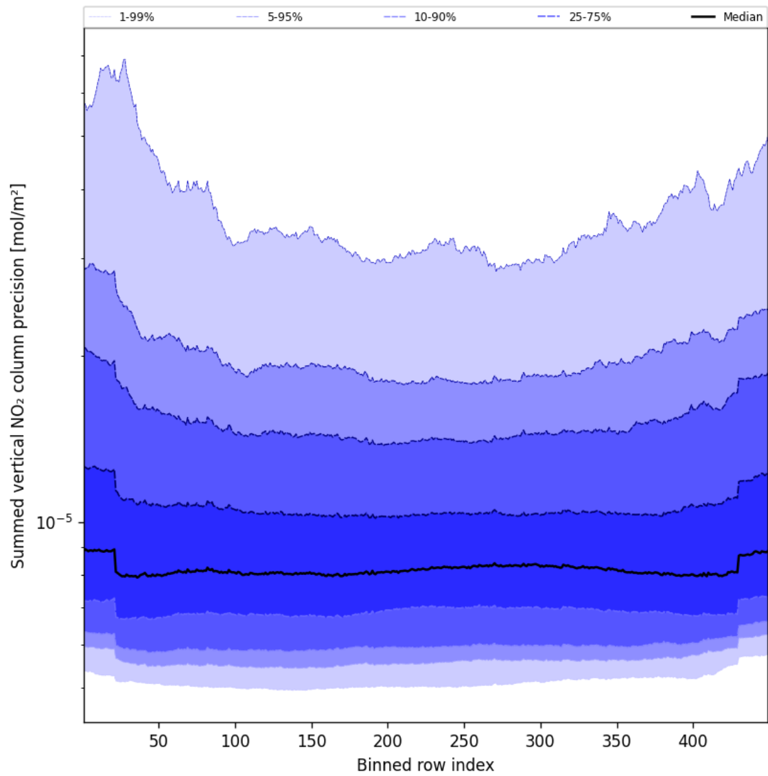
Figure 56: Along track statistics of “Summed vertical NO 2 column precision” for 2025-08-23 to 2025-08-23
