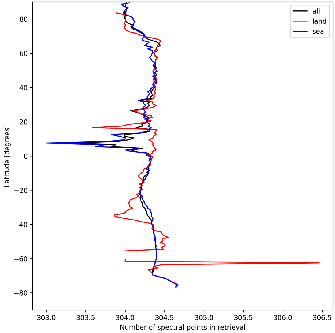
Figure 14: Zonal average of “Number of spectral points in retrieval” for 2025-08-23 to 2025-08-23.
