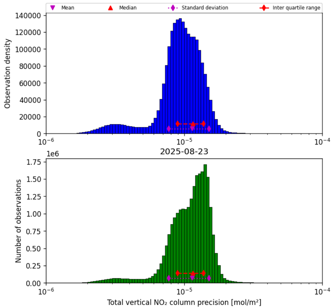
Figure 37: Histogram of “Total vertical NO 2 column precision” for 2025-08-23 to 2025-08-23
