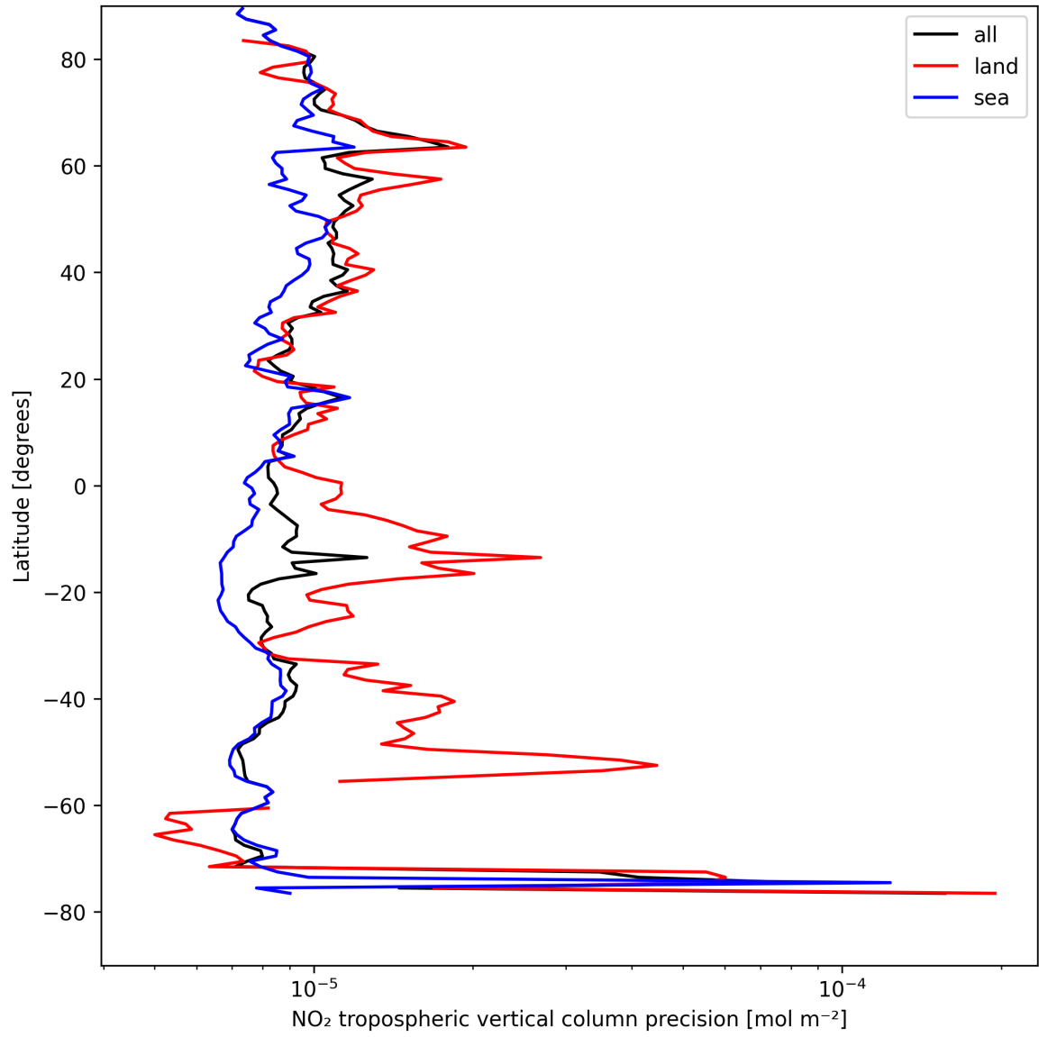
Figure 11: Zonal average of “NO 2 tropospheric vertical column precision” for 2025-08-23 to 2025-08-23.
