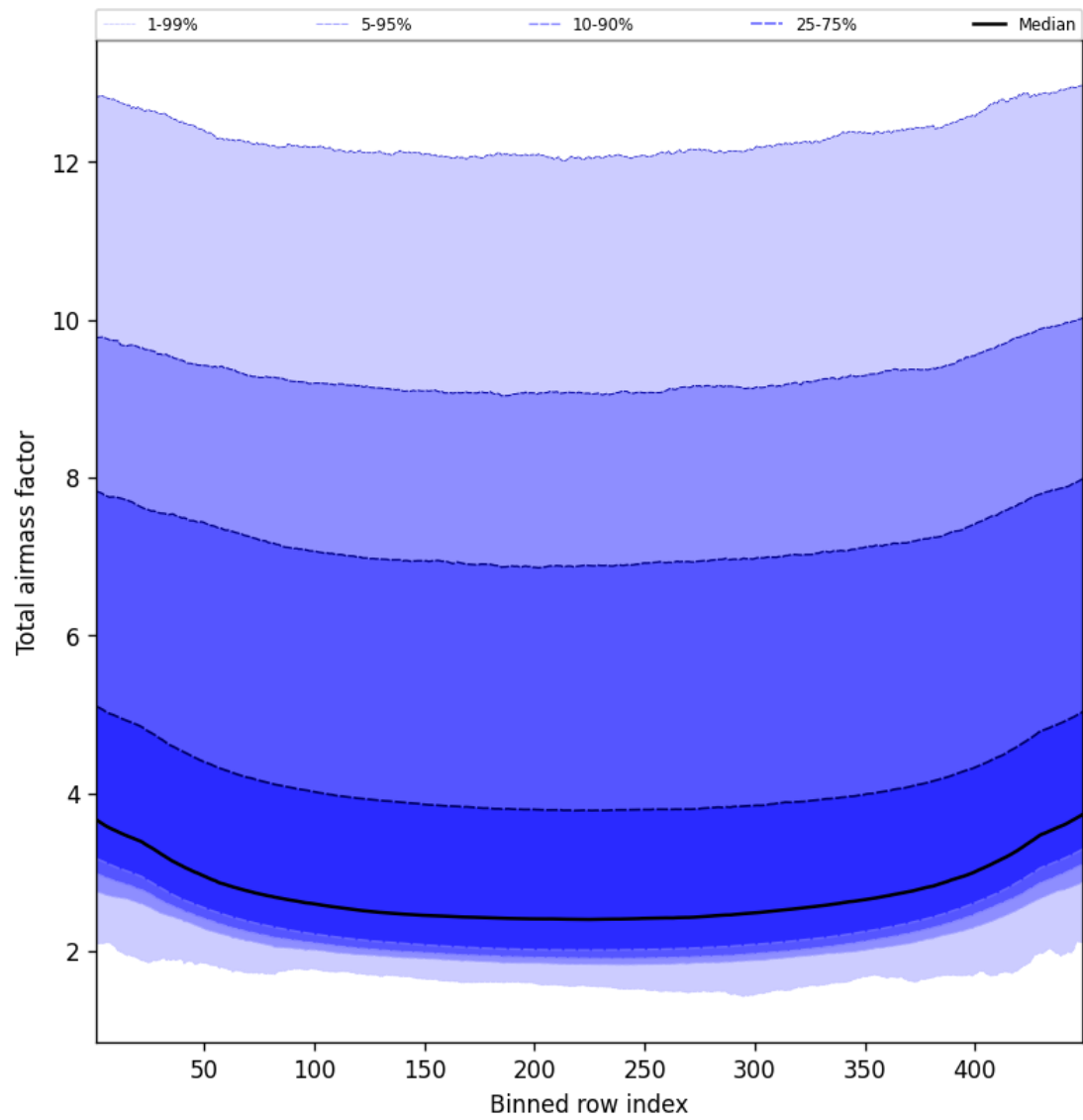
Figure 47: Along track statistics of “Total airmass factor” for 2025-08-23 to 2025-08-23
