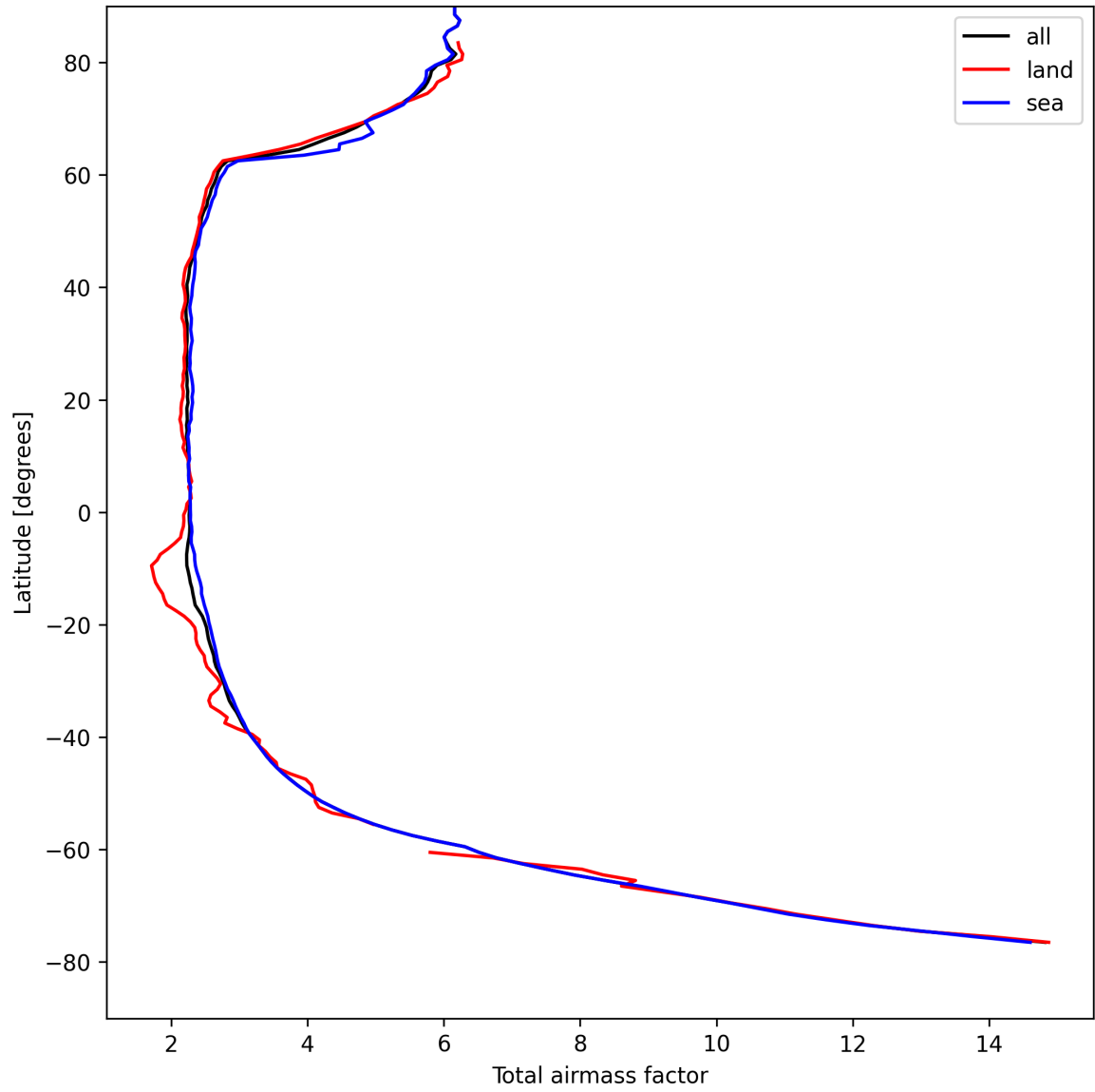
Figure 13: Zonal average of “Total airmass factor” for 2025-08-23 to 2025-08-23.
