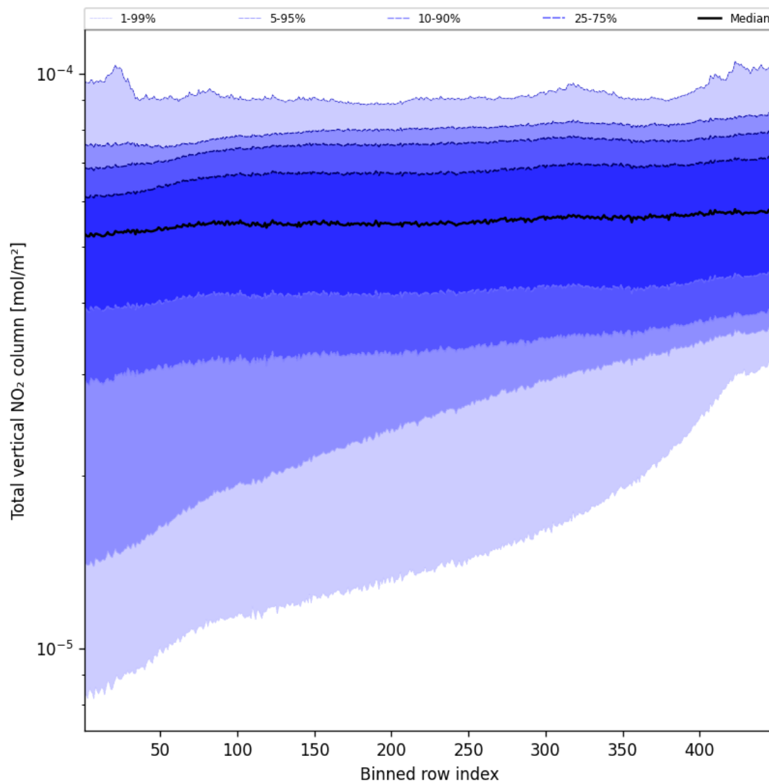
Figure 53: Along track statistics of “Total vertical NO 2 column” for 2025-08-23 to 2025-08-23
