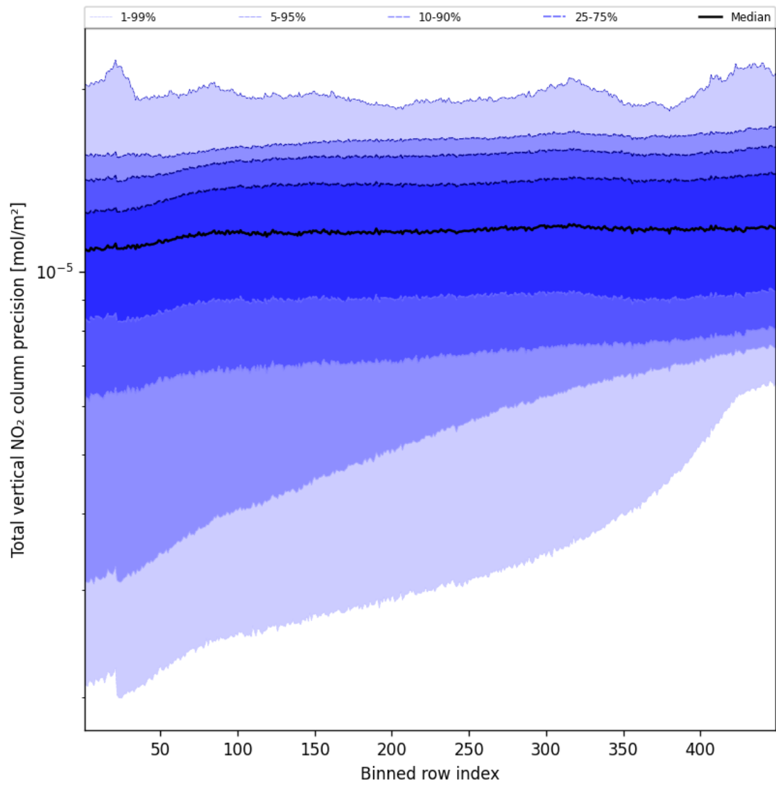
Figure 54: Along track statistics of “Total vertical NO 2 column precision” for 2025-08-23 to 2025-08-23
