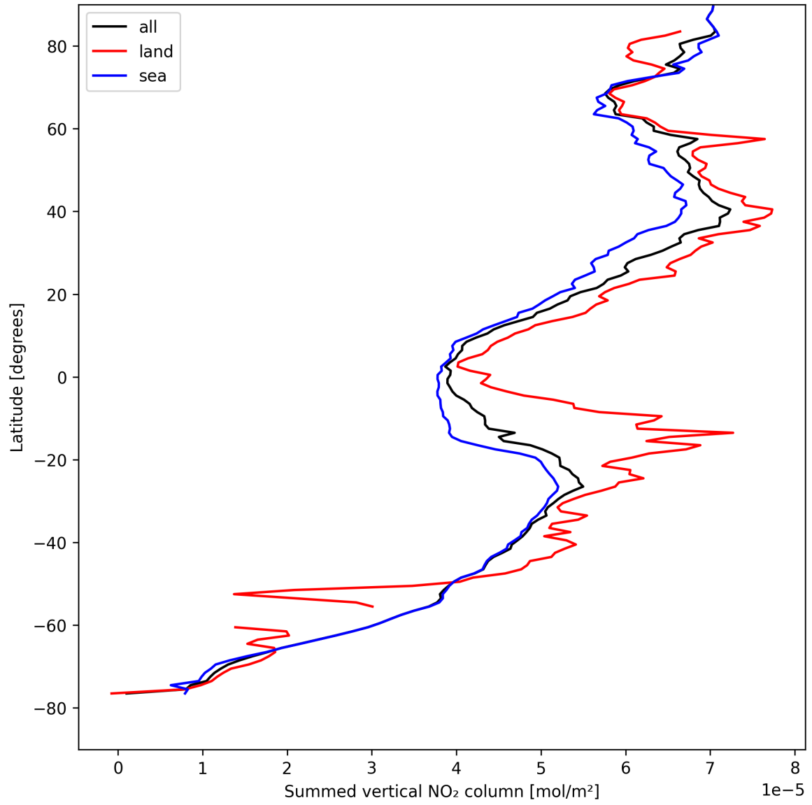
Figure 21: Zonal average of “Summed vertical NO 2 column” for 2025-08-23 to 2025-08-23.
