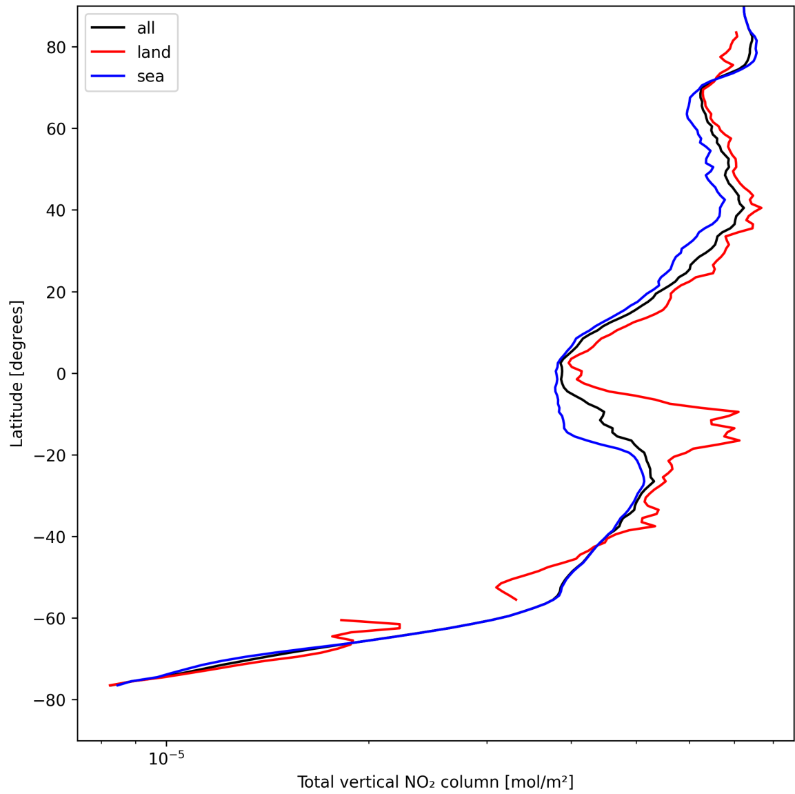
Figure 19: Zonal average of “Total vertical NO 2 column” for 2025-08-23 to 2025-08-23.
