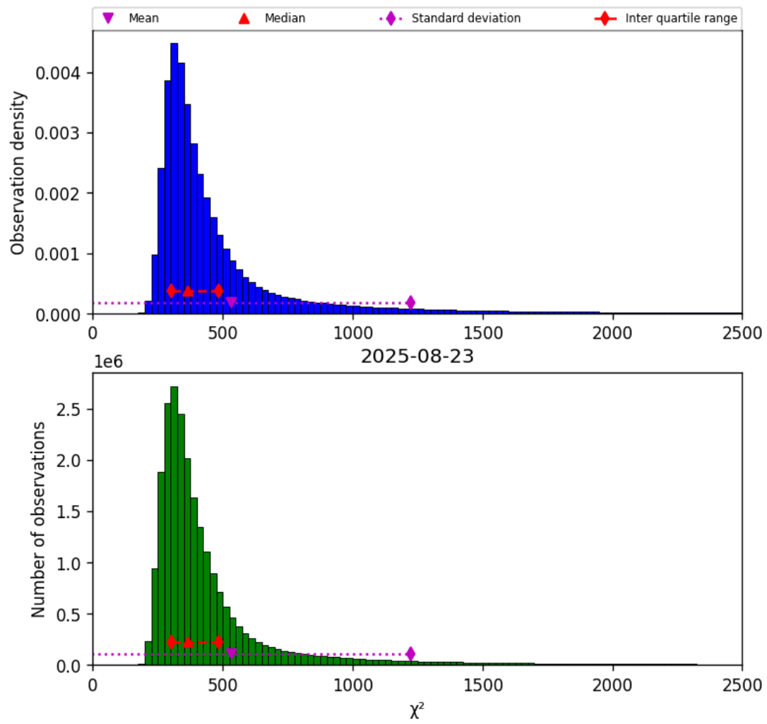
Figure 40: Histogram of “ \chi^2 ” for 2025-08-23 to 2025-08-23
