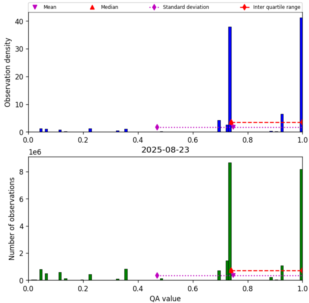
Figure 26: Histogram of “QA value” for 2025-08-23 to 2025-08-23
