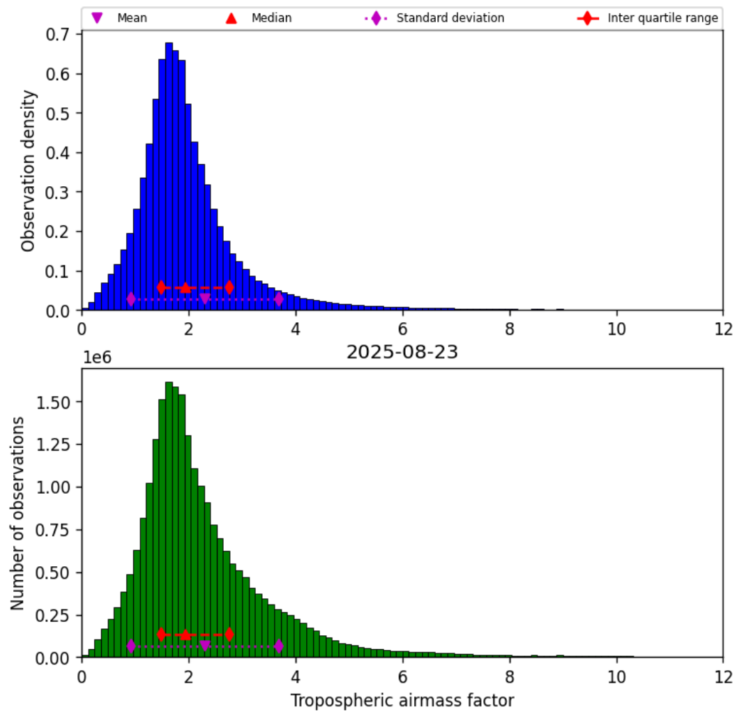
Figure 29: Histogram of “Tropospheric airmass factor” for 2025-08-23 to 2025-08-23
