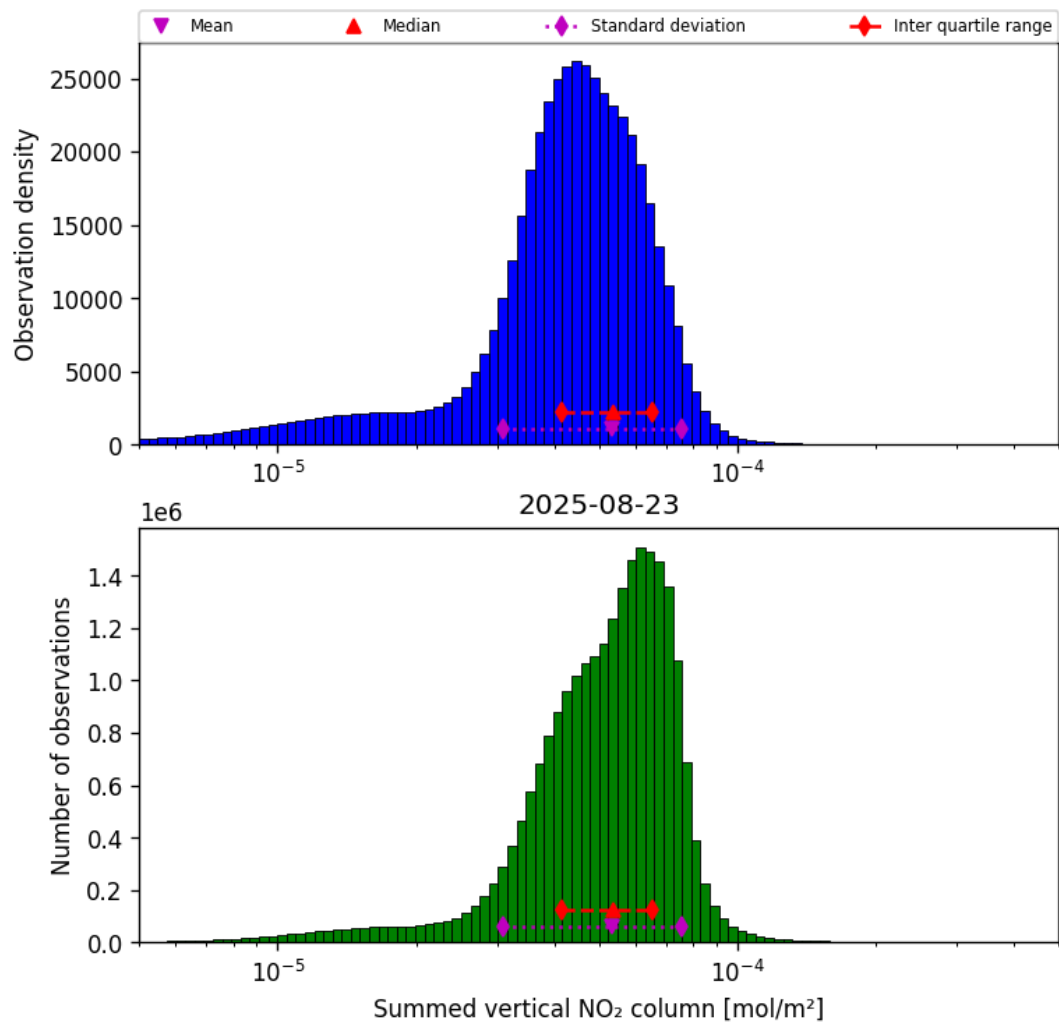
Figure 38: Histogram of "Summed vertical NO 2 column" for 2025-08-23 to 2025-08-23
