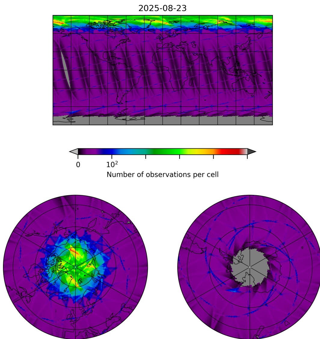
Figure 8: Map of the number of observations for 2025-08-23 to 2025-08-23
