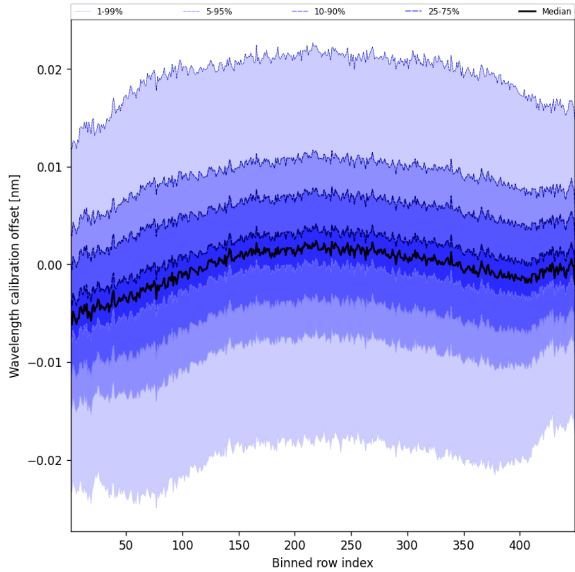
Figure 50: Along track statistics of “Wavelength calibration offset” for 2025-08-23 to 2025-08-23
