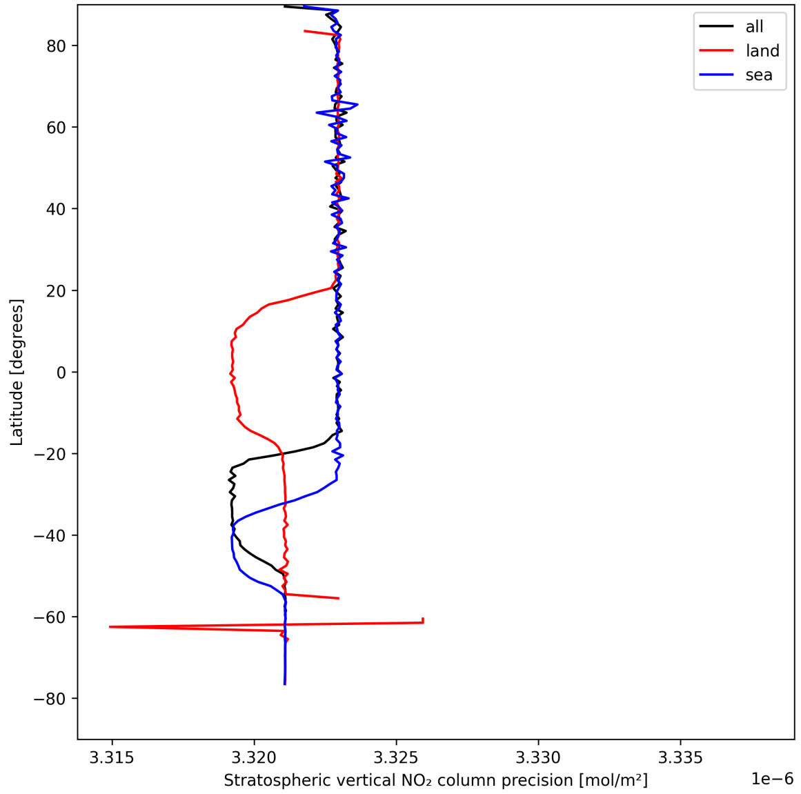
Figure 18: Zonal average of “Stratospheric vertical NO 2 column precision” for 2025-08-23 to 2025-08-23.
