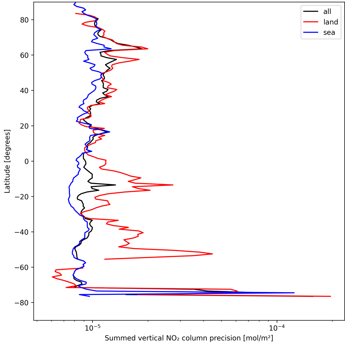
Figure 22: Zonal average of "Summed vertical NO 2 column precision" for 2025-08-23 to 2025-08-23.
