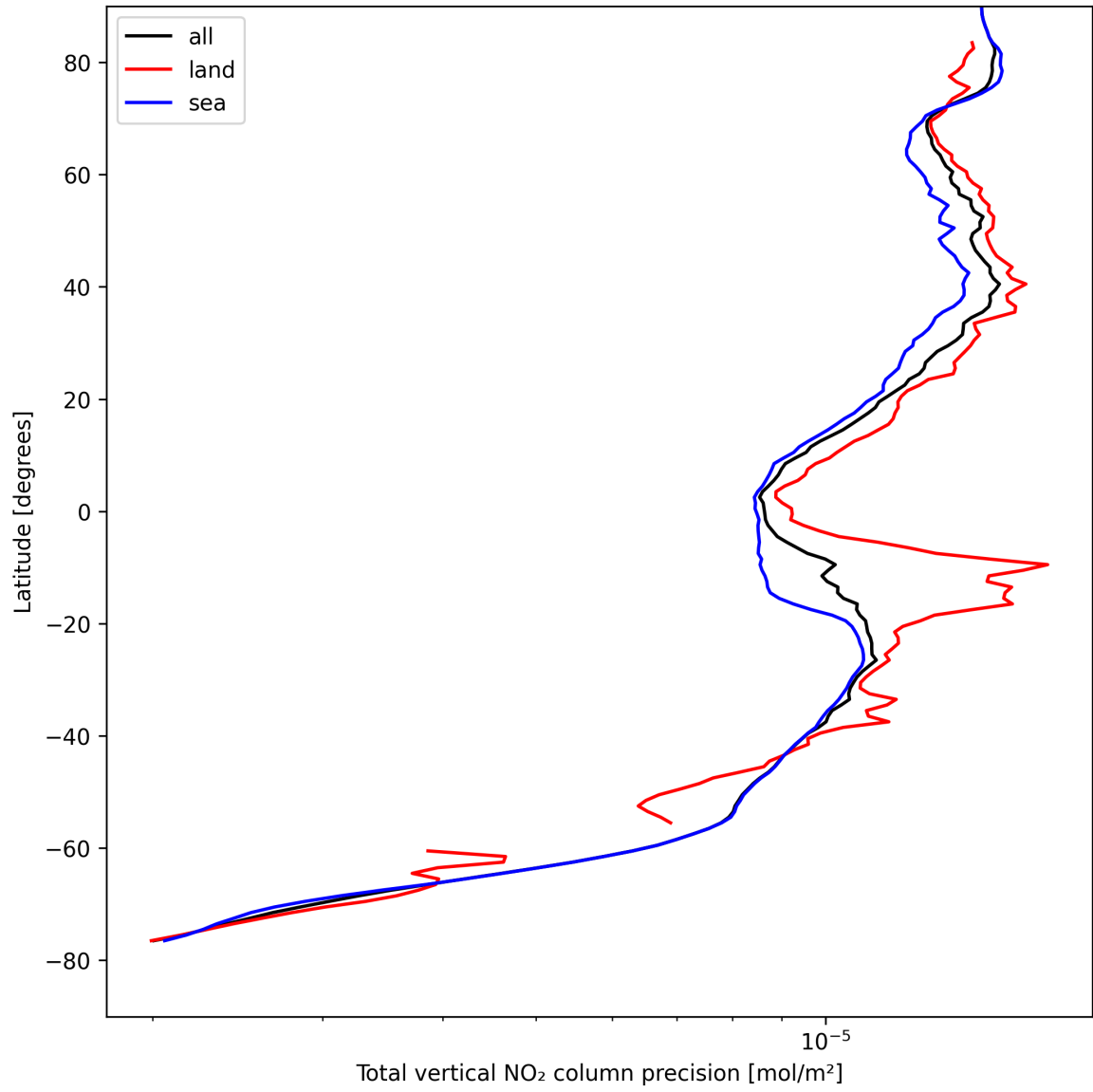
Figure 20: Zonal average of “Total vertical NO 2 column precision” for 2025-08-23 to 2025-08-23.
