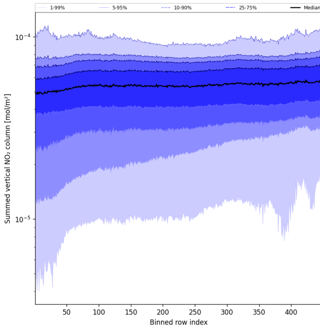
Figure 55: Along track statistics of “Summed vertical NO 2 column” for 2025-08-23 to 2025-08-23
