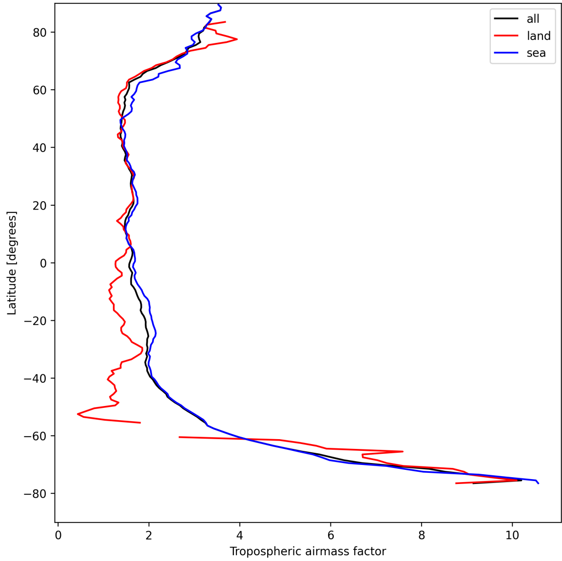
Figure 12: Zonal average of “Tropospheric airmass factor” for 2025-08-23 to 2025-08-23.
