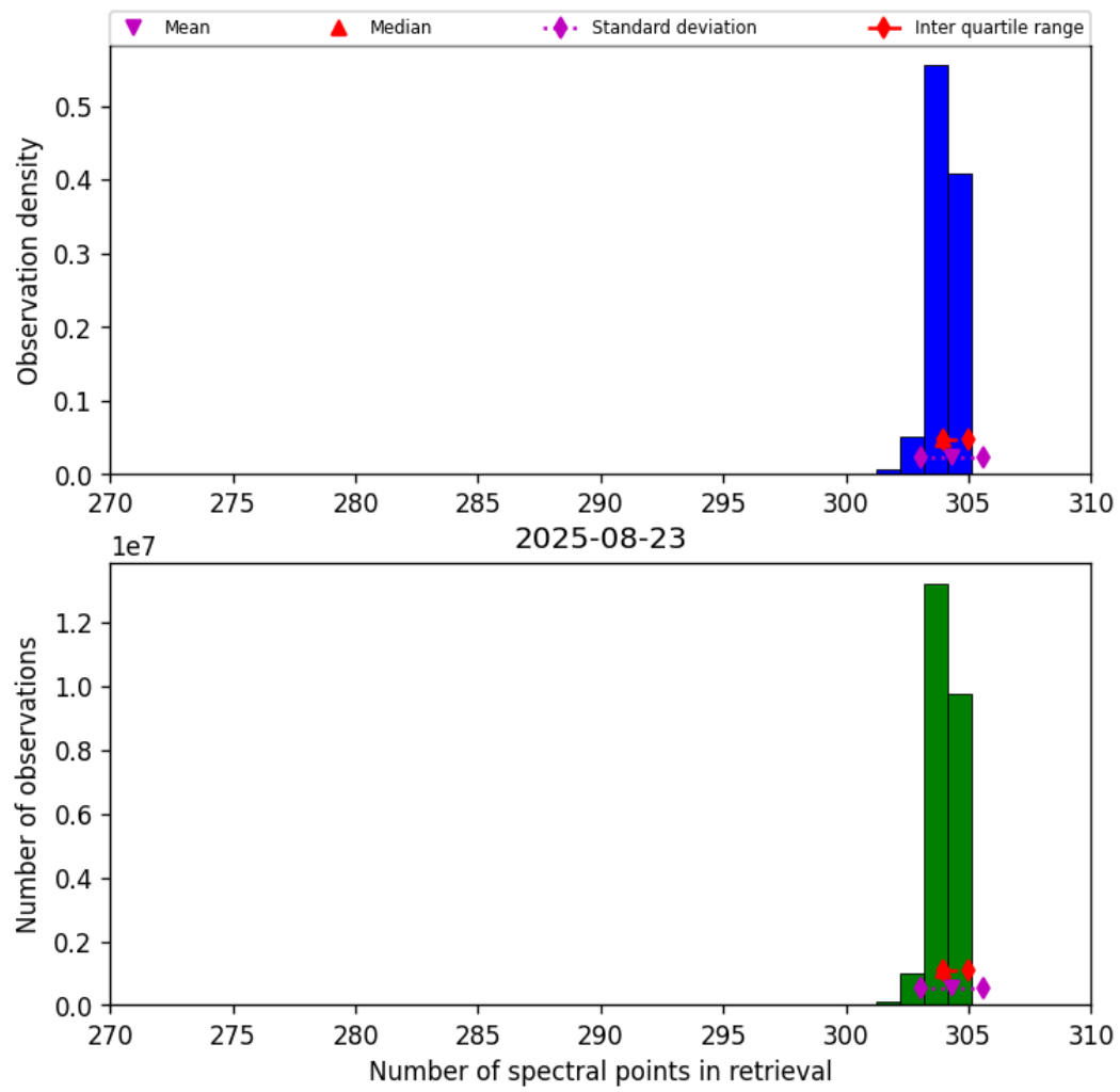
Figure 31: Histogram of “Number of spectral points in retrieval” for 2025-08-23 to 2025-08-23
