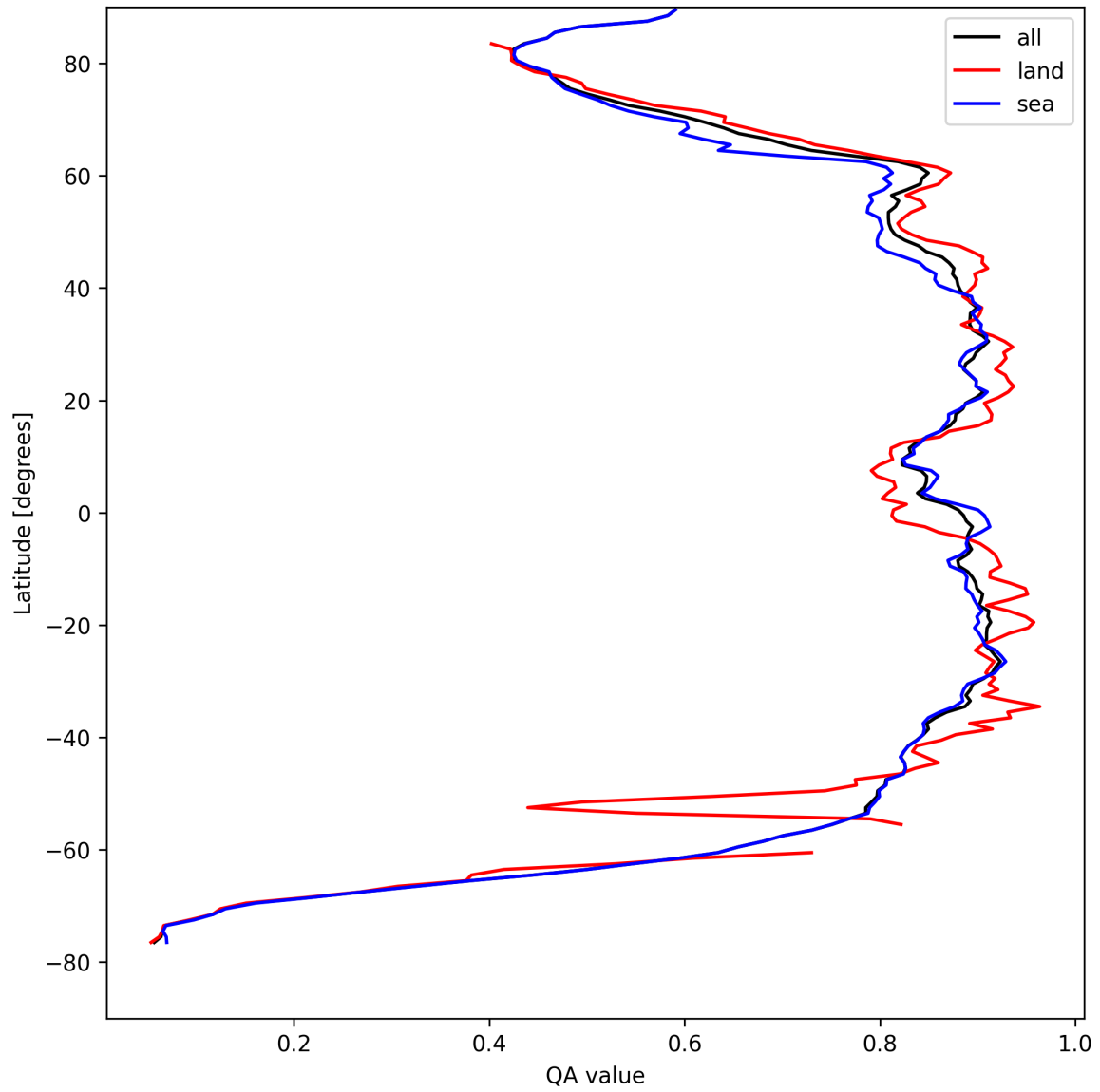
Figure 9: Zonal average of “QA value” for 2025-08-23 to 2025-08-23.
