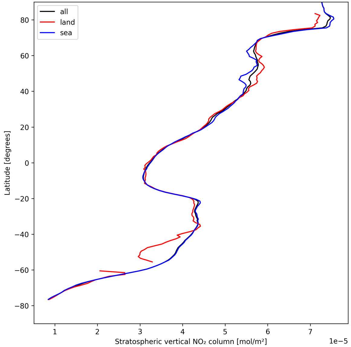
Figure 17: Zonal average of “Stratospheric vertical NO 2 column” for 2025-08-23 to 2025-08-23.
