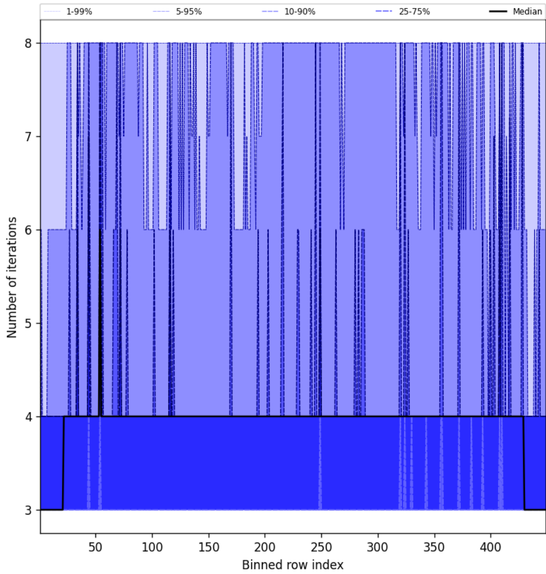
Figure 49: Along track statistics of “Number of iterations” for 2025-08-23 to 2025-08-23
