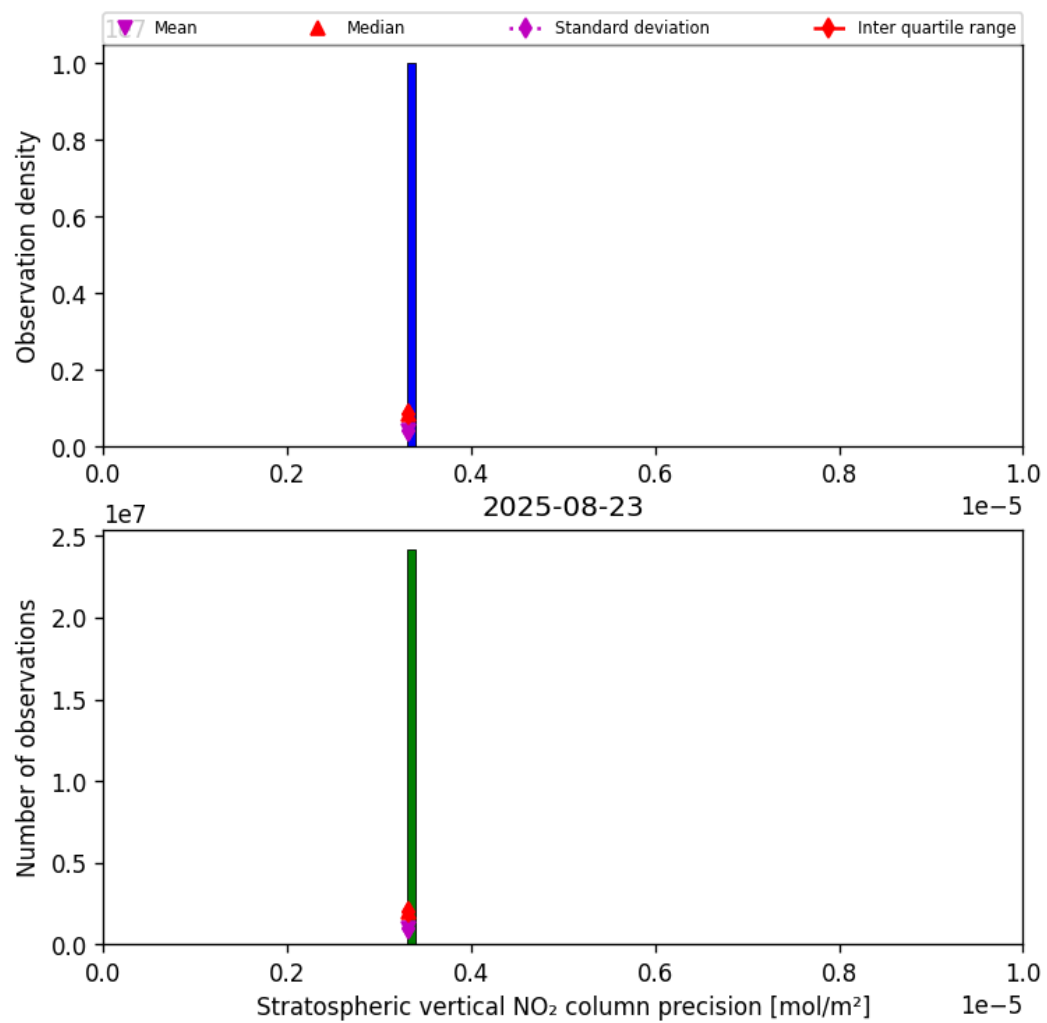
Figure 35: Histogram of “Stratospheric vertical NO 2 column precision” for 2025-08-23 to 2025-08-23
