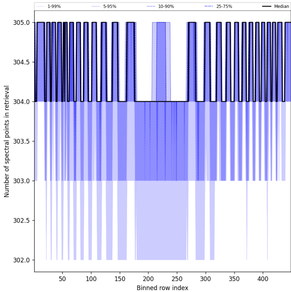
Figure 48: Along track statistics of “Number of spectral points in retrieval” for 2025-08-23 to 2025-08-23
