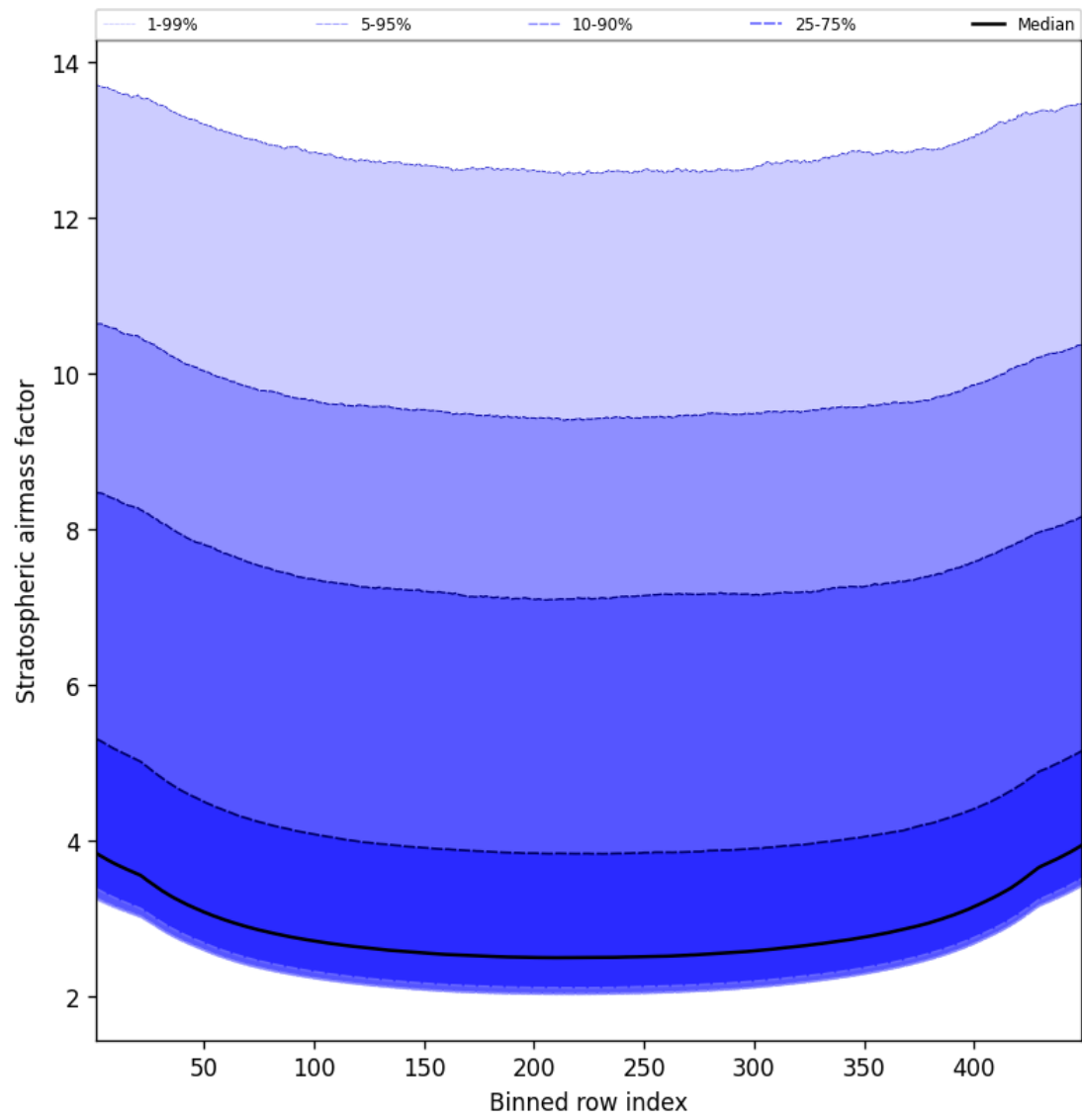
Figure 59: Along track statistics of “Stratospheric airmass factor” for 2025-08-23 to 2025-08-23
