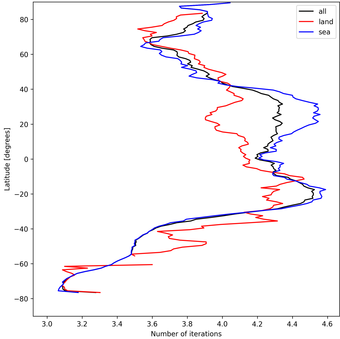
Figure 15: Zonal average of “Number of iterations” for 2025-08-23 to 2025-08-23.
