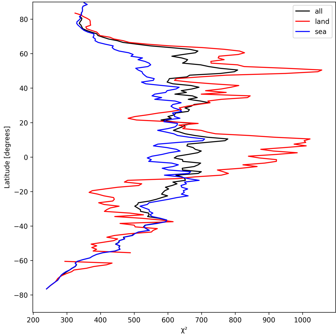
Figure 23: Zonal average of “ \chi^2 ” for 2025-08-23 to 2025-08-23.
