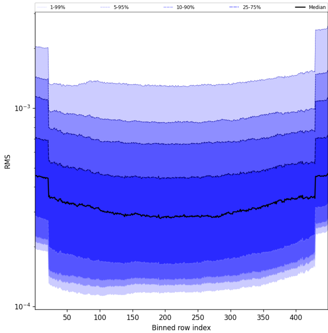
Figure 58: Along track statistics of “RMS” for 2025-08-23 to 2025-08-23
