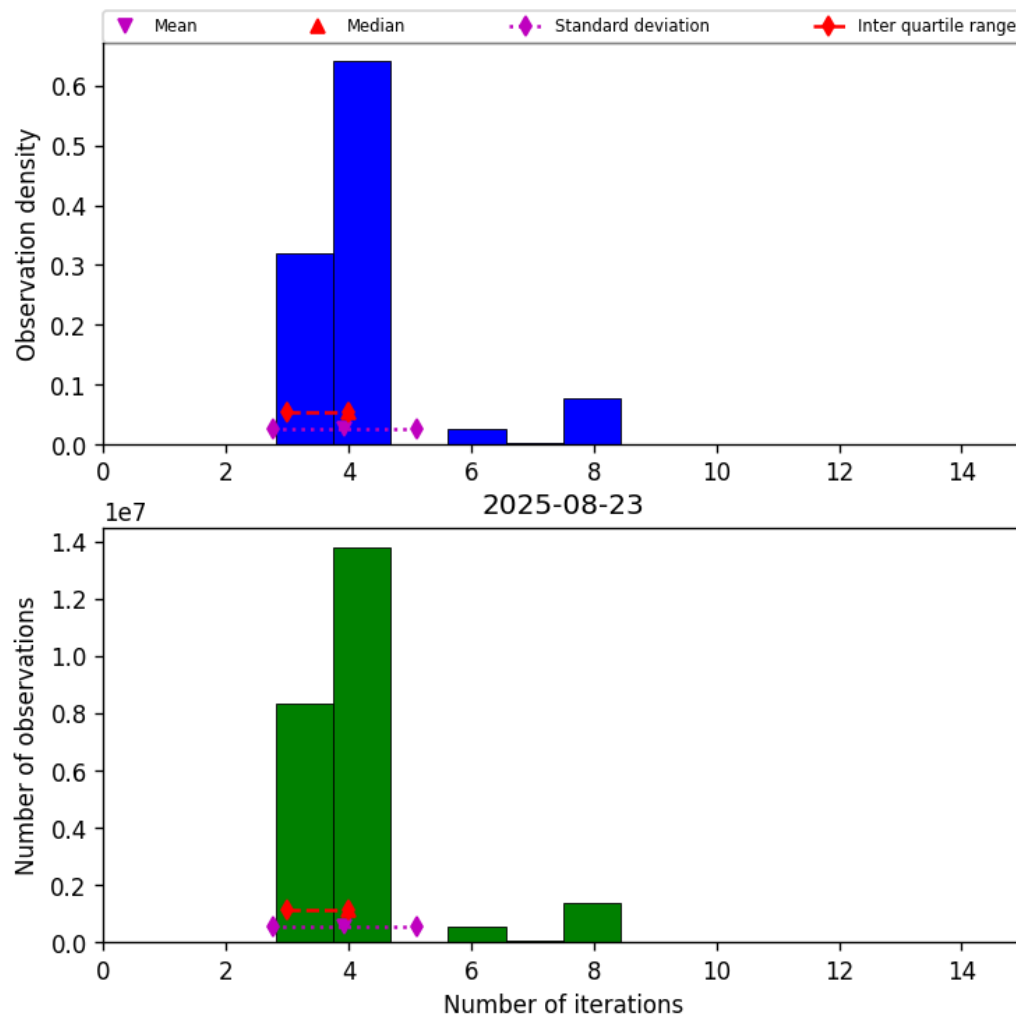
Figure 32: Histogram of “Number of iterations” for 2025-08-23 to 2025-08-23
