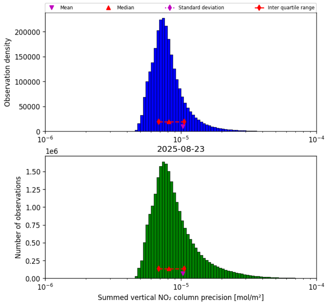
Figure 39: Histogram of “Summed vertical NO 2 column precision” for 2025-08-23 to 2025-08-23
