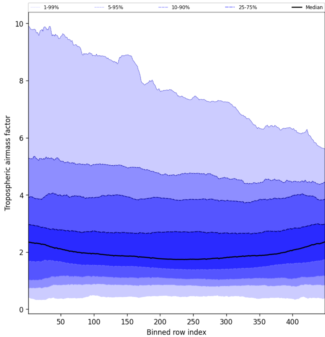
Figure 46: Along track statistics of “Tropospheric airmass factor” for 2025-08-23 to 2025-08-23
