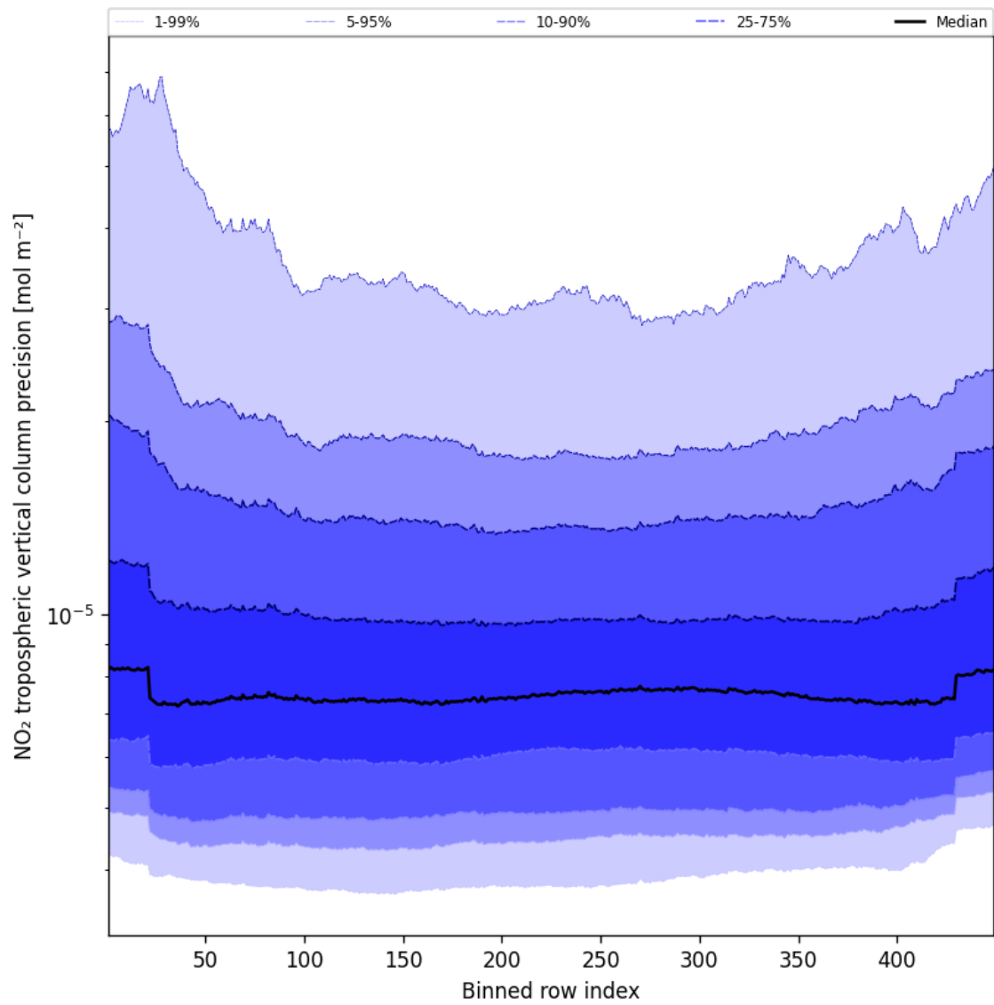
Figure 45: Along track statistics of “NO 2 tropospheric vertical column precision” for 2025-08-23 to 2025-08-23
