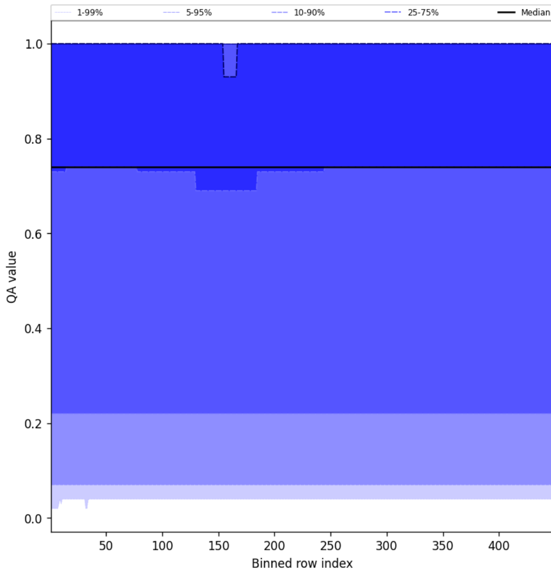
Figure 43: Along track statistics of “QA value” for 2025-08-23 to 2025-08-23
