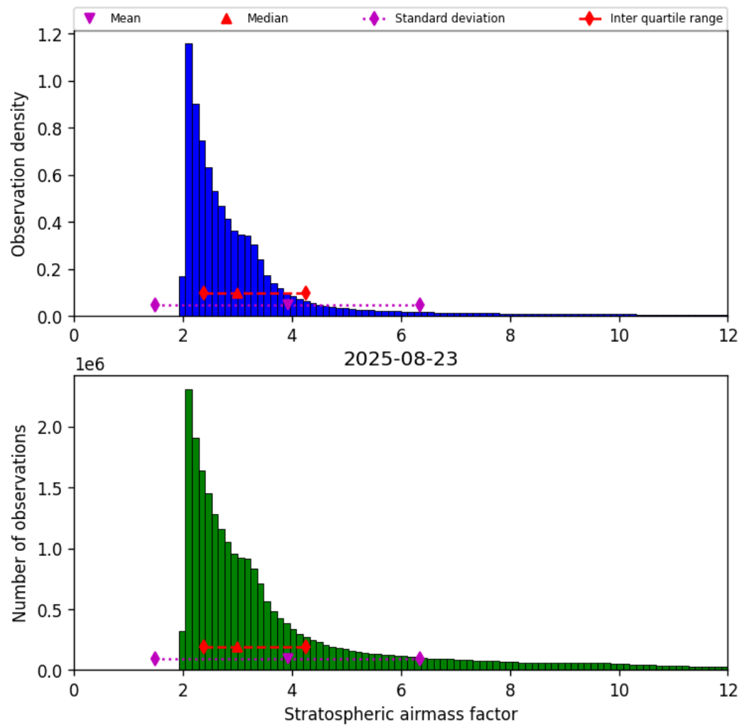
Figure 42: Histogram of “Stratospheric airmass factor” for 2025-08-23 to 2025-08-23
