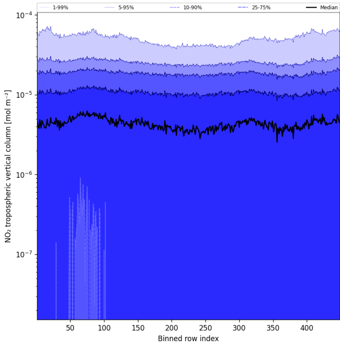
Figure 44: Along track statistics of “NO 2 tropospheric vertical column” for 2025-08-23 to 2025-08-23
