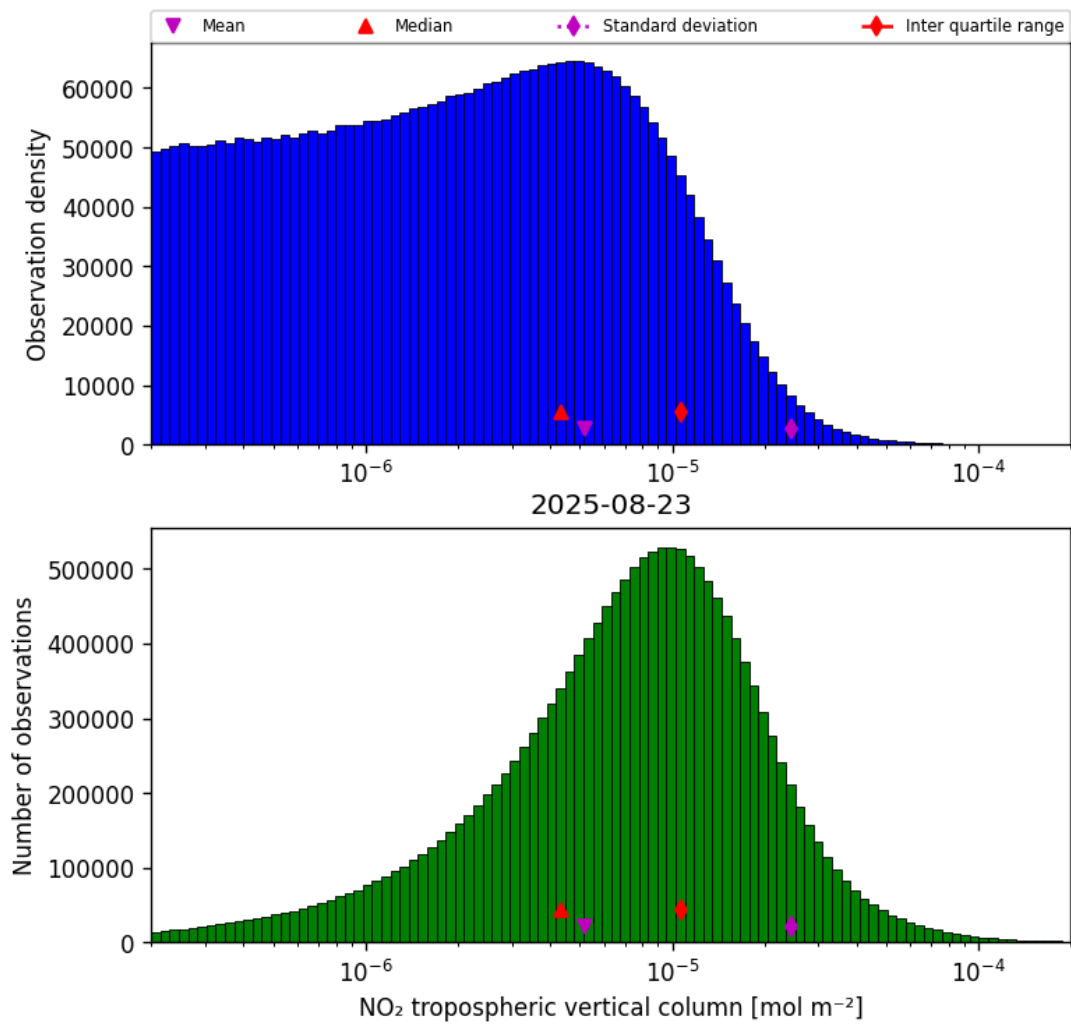
Figure 27: Histogram of “ \text{NO}_2 tropospheric vertical column” for 2025-08-23 to 2025-08-23
