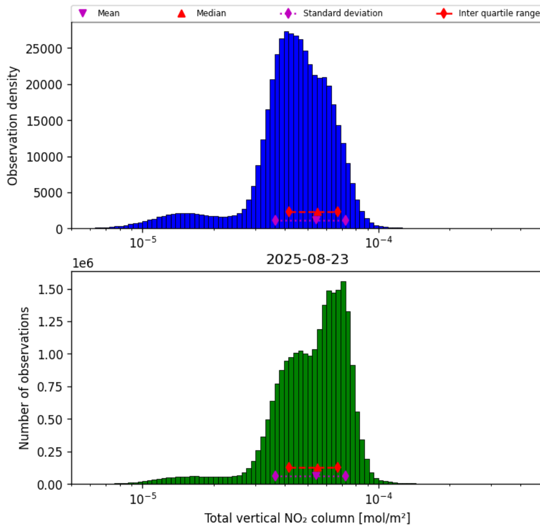
Figure 36: Histogram of “Total vertical NO 2 column” for 2025-08-23 to 2025-08-23
