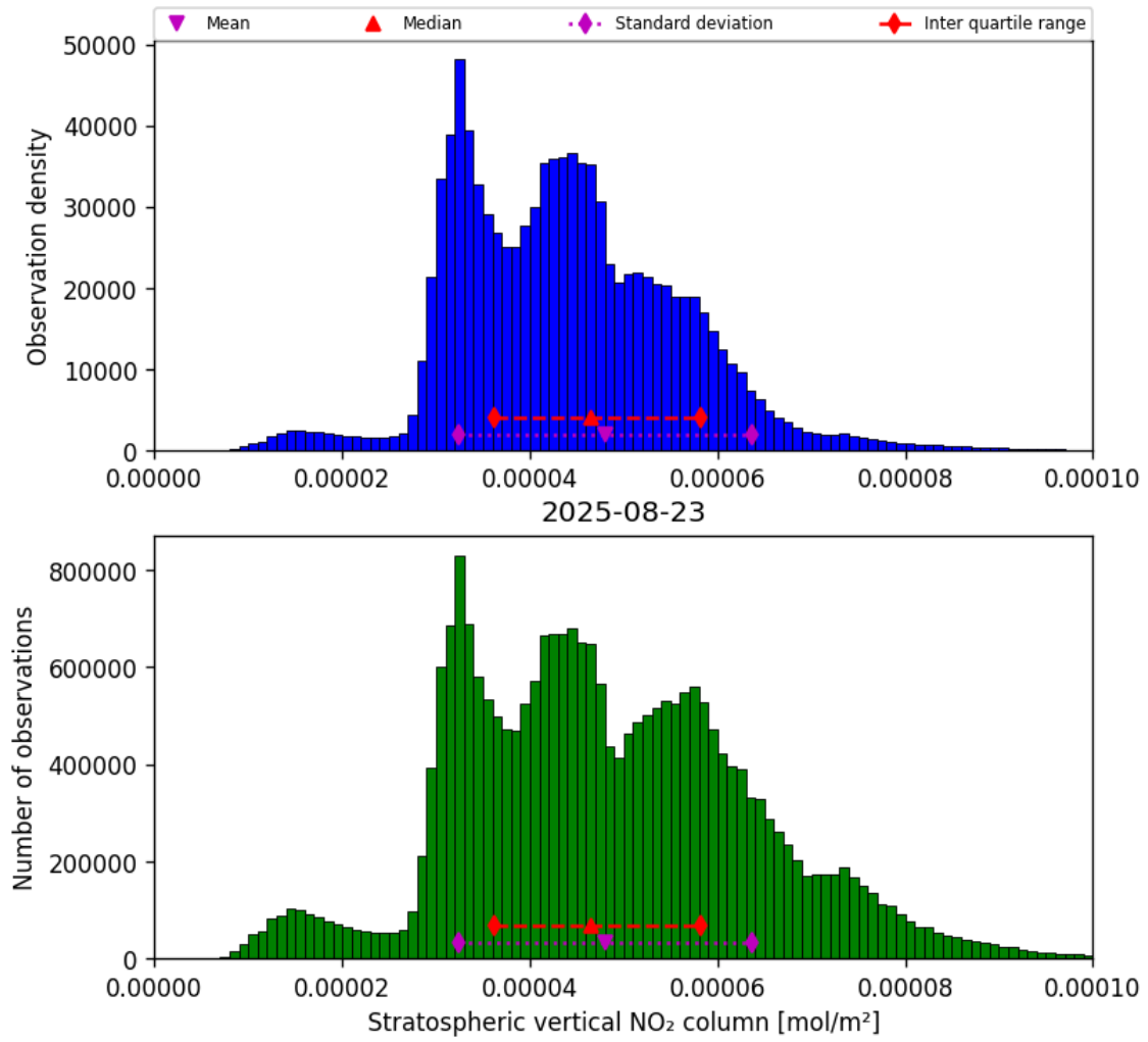
Figure 34: Histogram of “Stratospheric vertical NO 2 column” for 2025-08-23 to 2025-08-23
