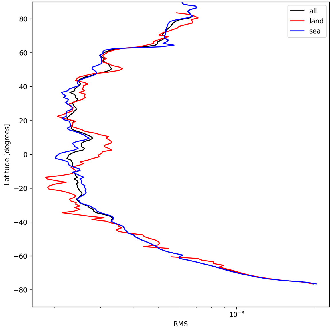
Figure 24: Zonal average of “RMS” for 2025-08-23 to 2025-08-23.
