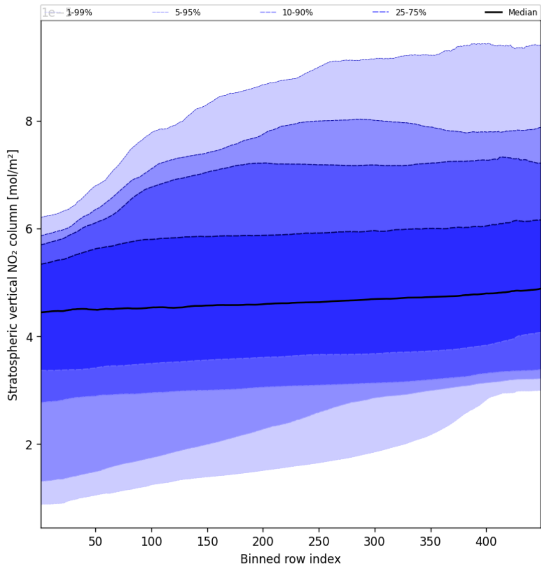
Figure 51: Along track statistics of “Stratospheric vertical NO 2 column” for 2025-08-23 to 2025-08-23
