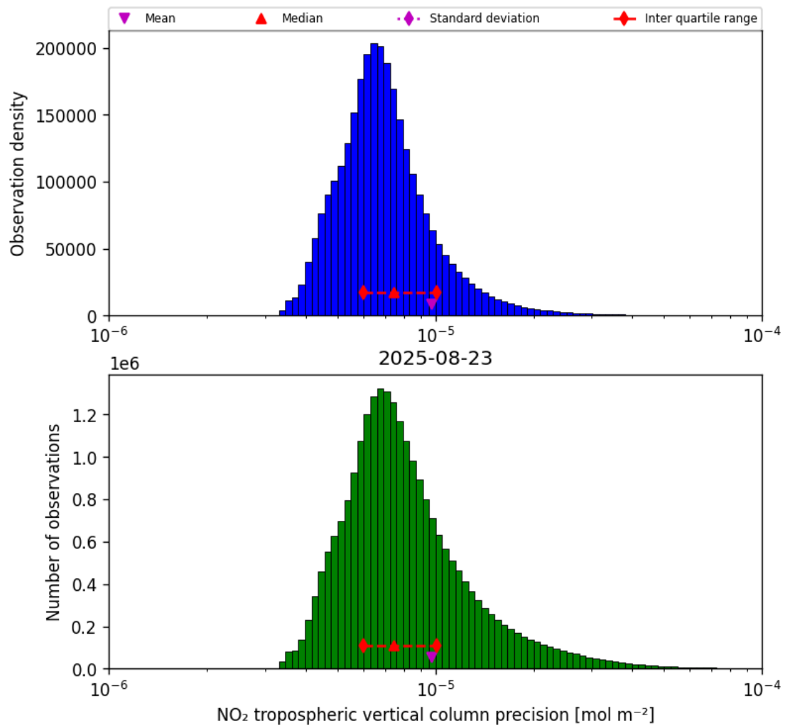
Figure 28: Histogram of “NO 2 tropospheric vertical column precision” for 2025-08-23 to 2025-08-23
