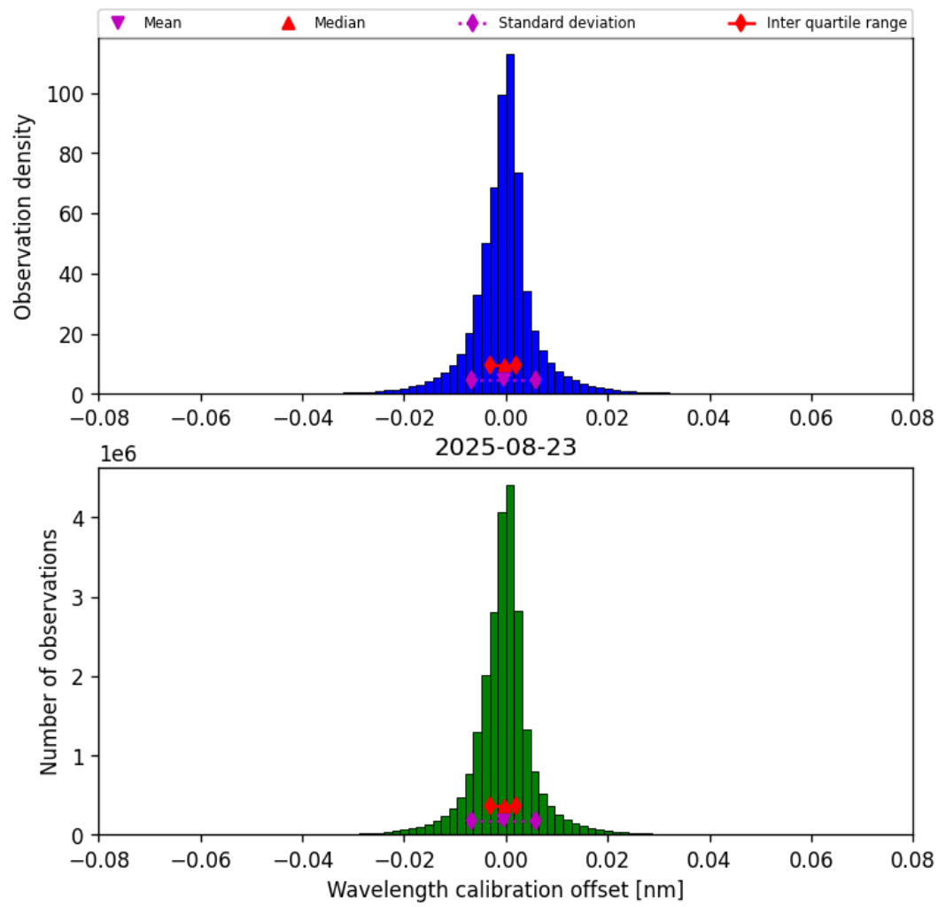
Figure 33: Histogram of “Wavelength calibration offset” for 2025-08-23 to 2025-08-23
