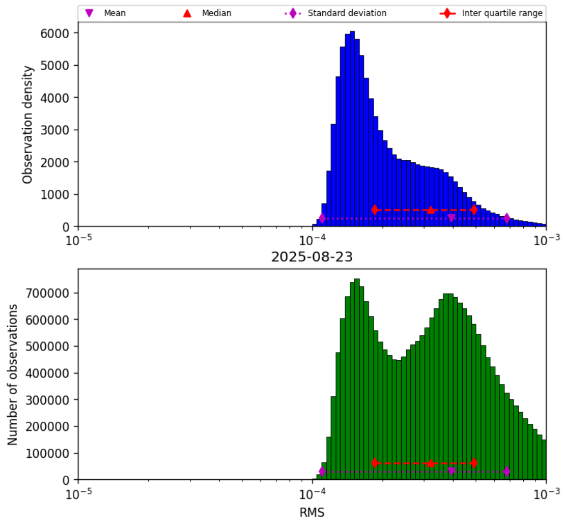
Figure 41: Histogram of “RMS” for 2025-08-23 to 2025-08-23
