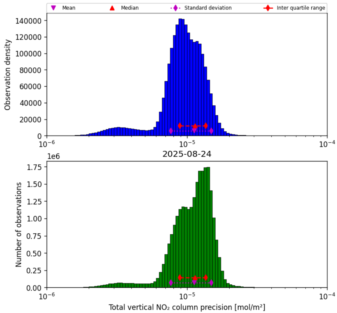
Figure 37: Histogram of “Total vertical NO 2 column precision” for 2025-08-24 to 2025-08-25
