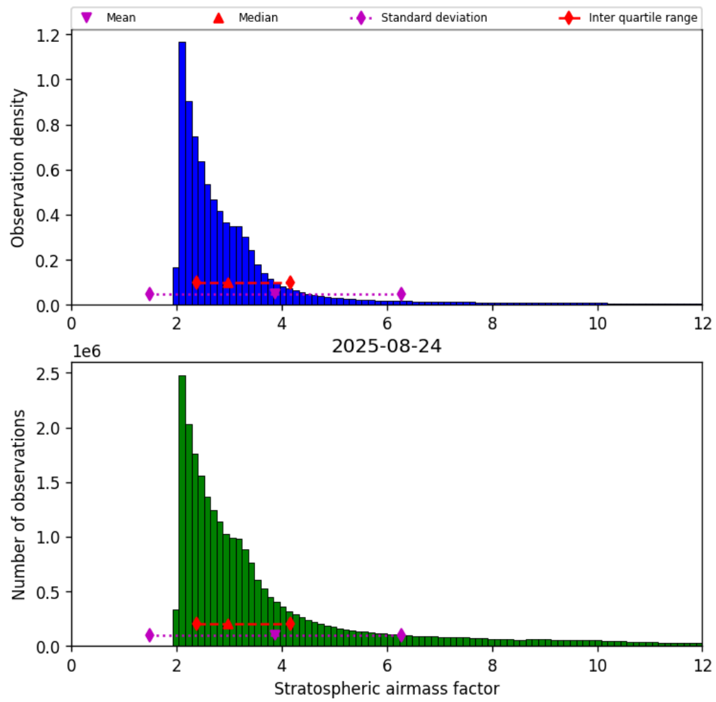
Figure 42: Histogram of “Stratospheric airmass factor” for 2025-08-24 to 2025-08-25
