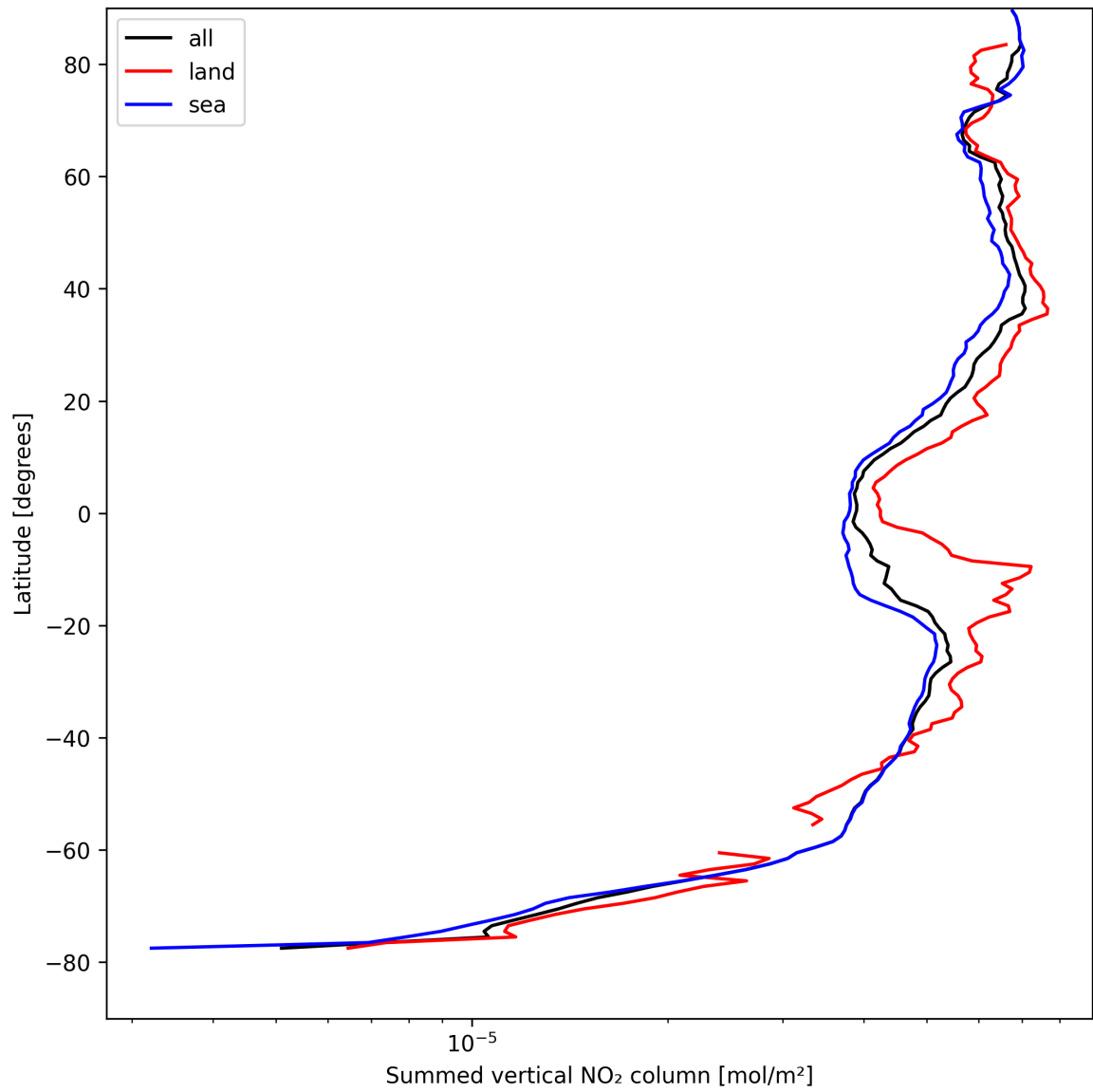
Figure 21: Zonal average of “Summed vertical NO 2 column” for 2025-08-24 to 2025-08-25.
