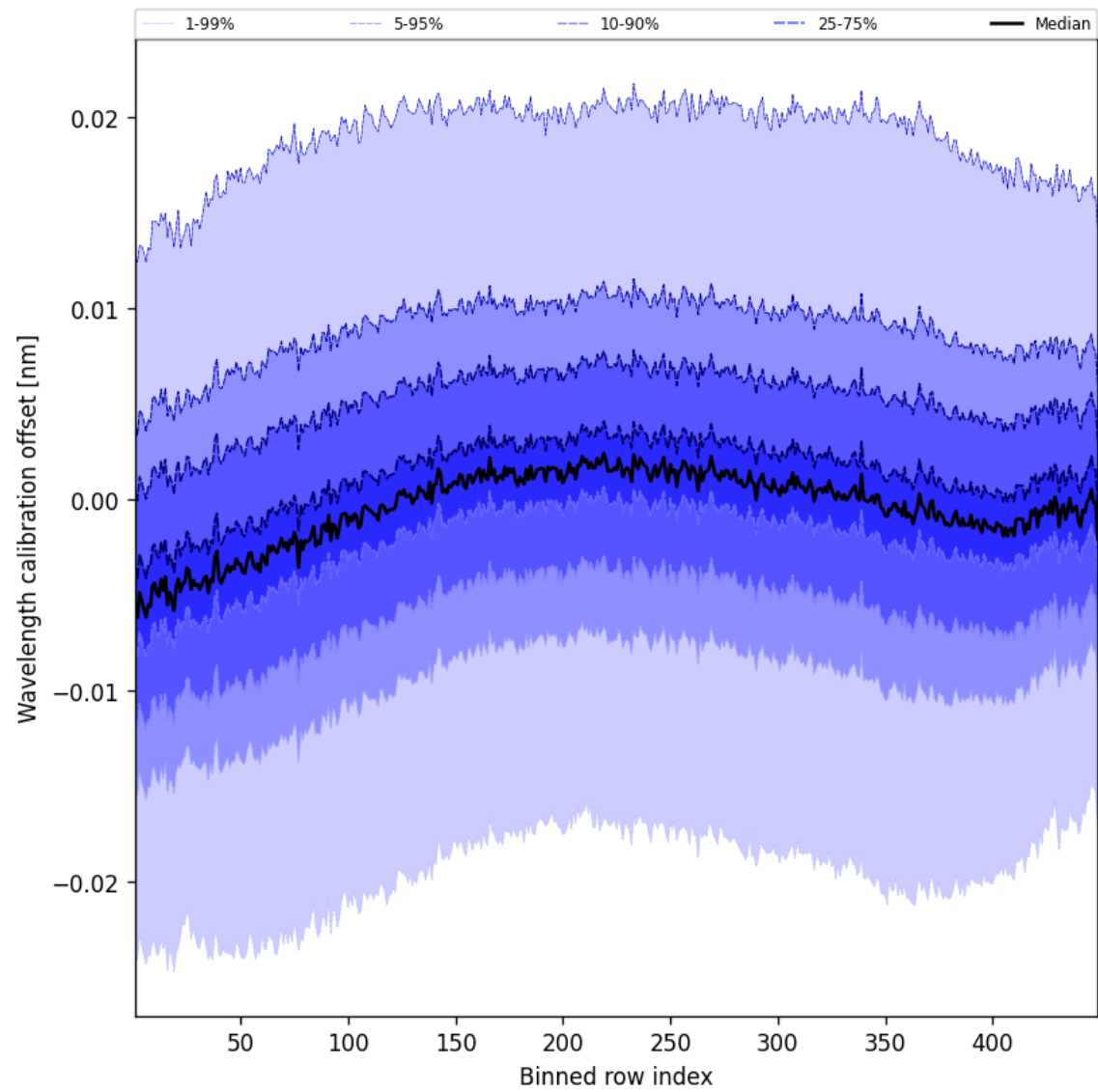
Figure 50: Along track statistics of “Wavelength calibration offset” for 2025-08-24 to 2025-08-25
