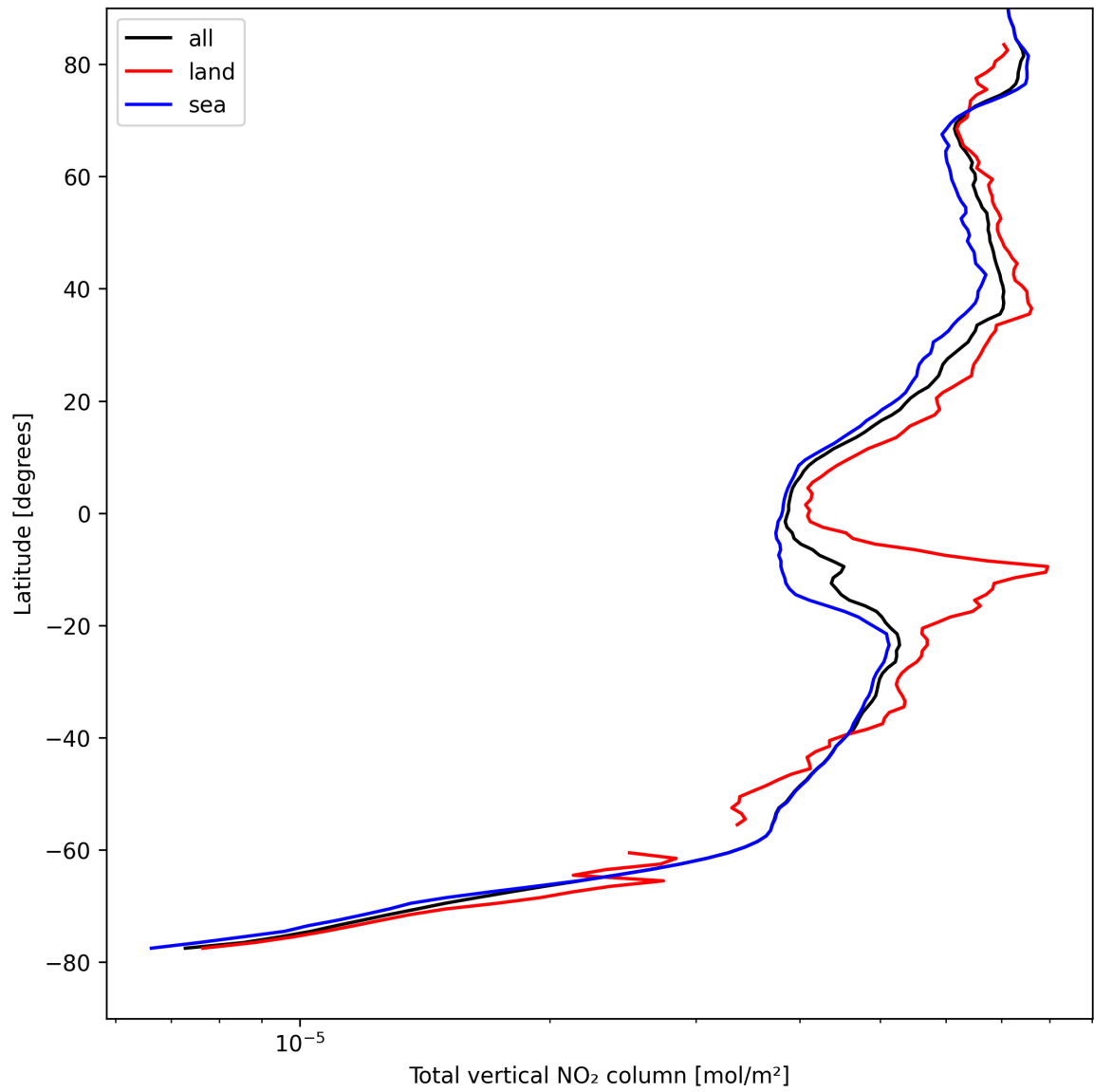
Figure 19: Zonal average of “Total vertical NO 2 column” for 2025-08-24 to 2025-08-25.
