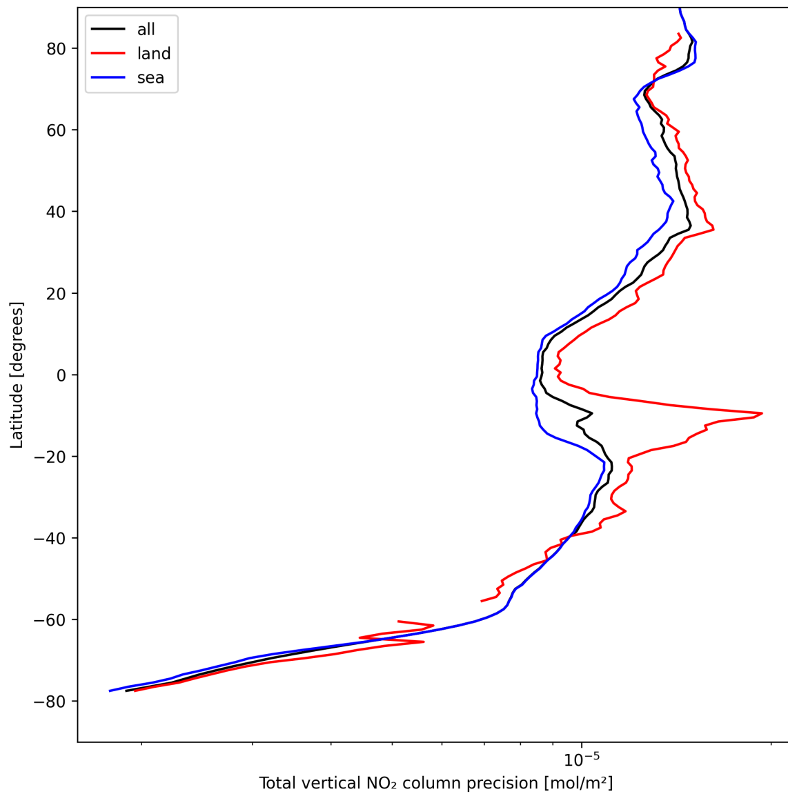
Figure 20: Zonal average of “Total vertical NO 2 column precision” for 2025-08-24 to 2025-08-25.
