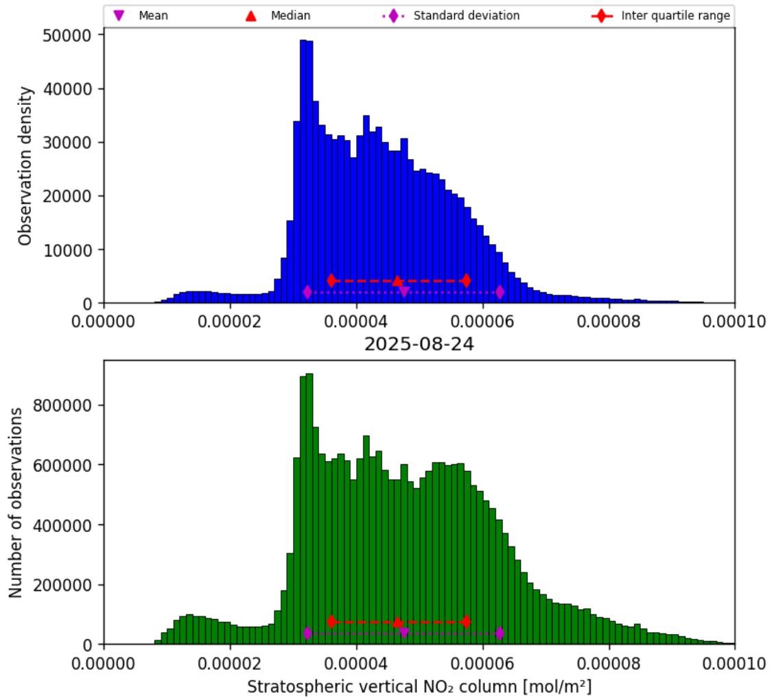
Figure 34: Histogram of “Stratospheric vertical NO 2 column” for 2025-08-24 to 2025-08-25
