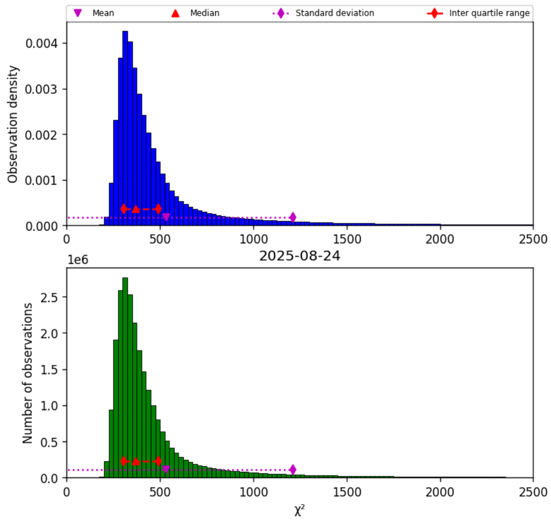
Figure 40: Histogram of “ \chi^2 ” for 2025-08-24 to 2025-08-25
