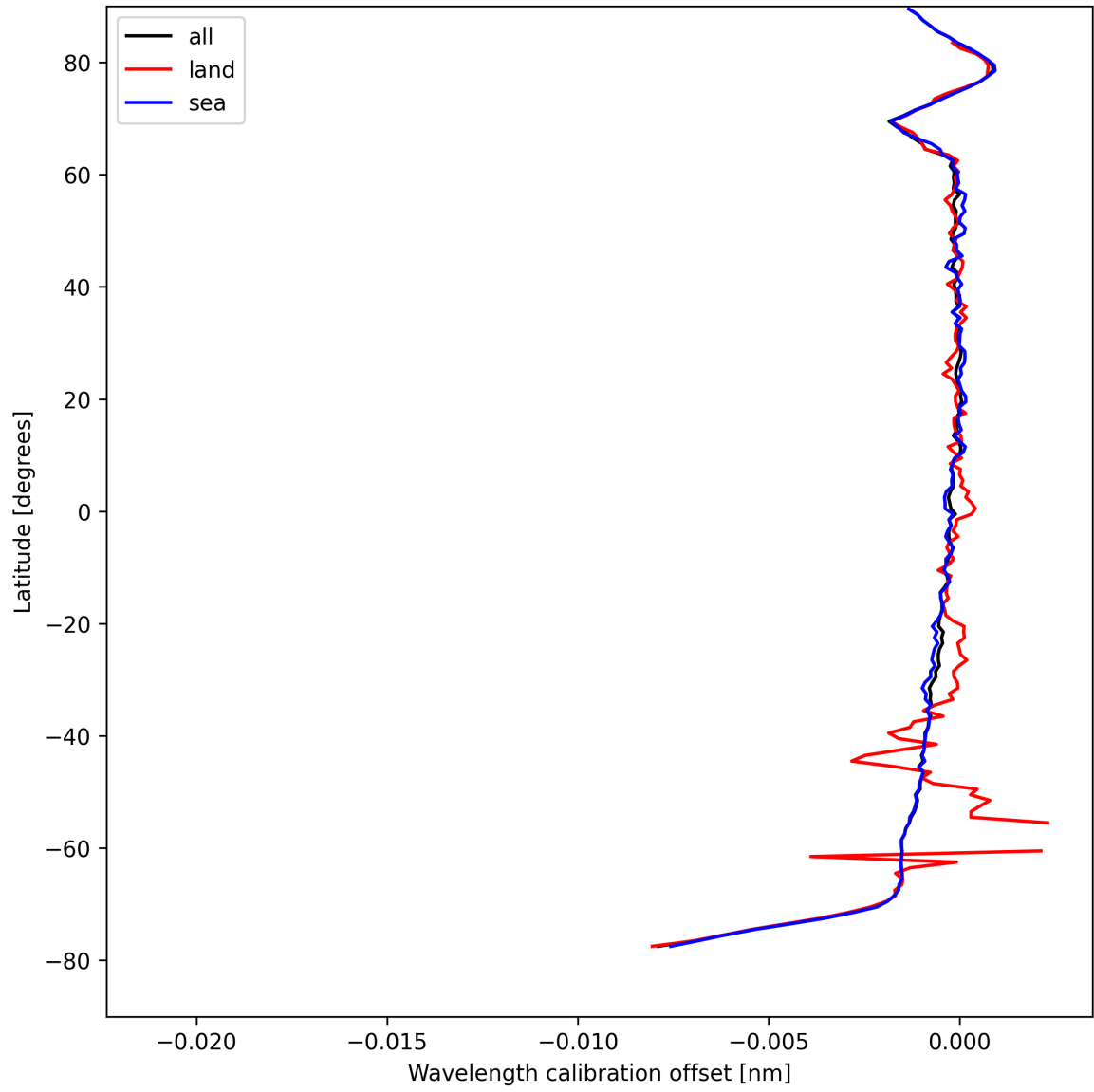
Figure 16: Zonal average of “Wavelength calibration offset” for 2025-08-24 to 2025-08-25.
