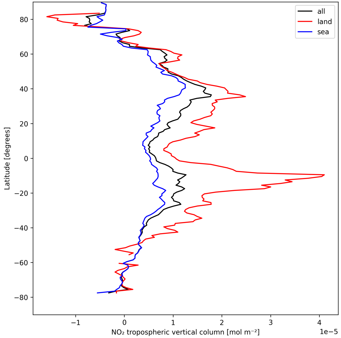
Figure 10: Zonal average of “NO 2 tropospheric vertical column” for 2025-08-24 to 2025-08-25.
