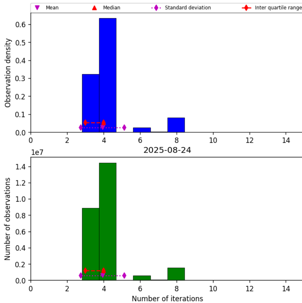
Figure 32: Histogram of “Number of iterations” for 2025-08-24 to 2025-08-25
