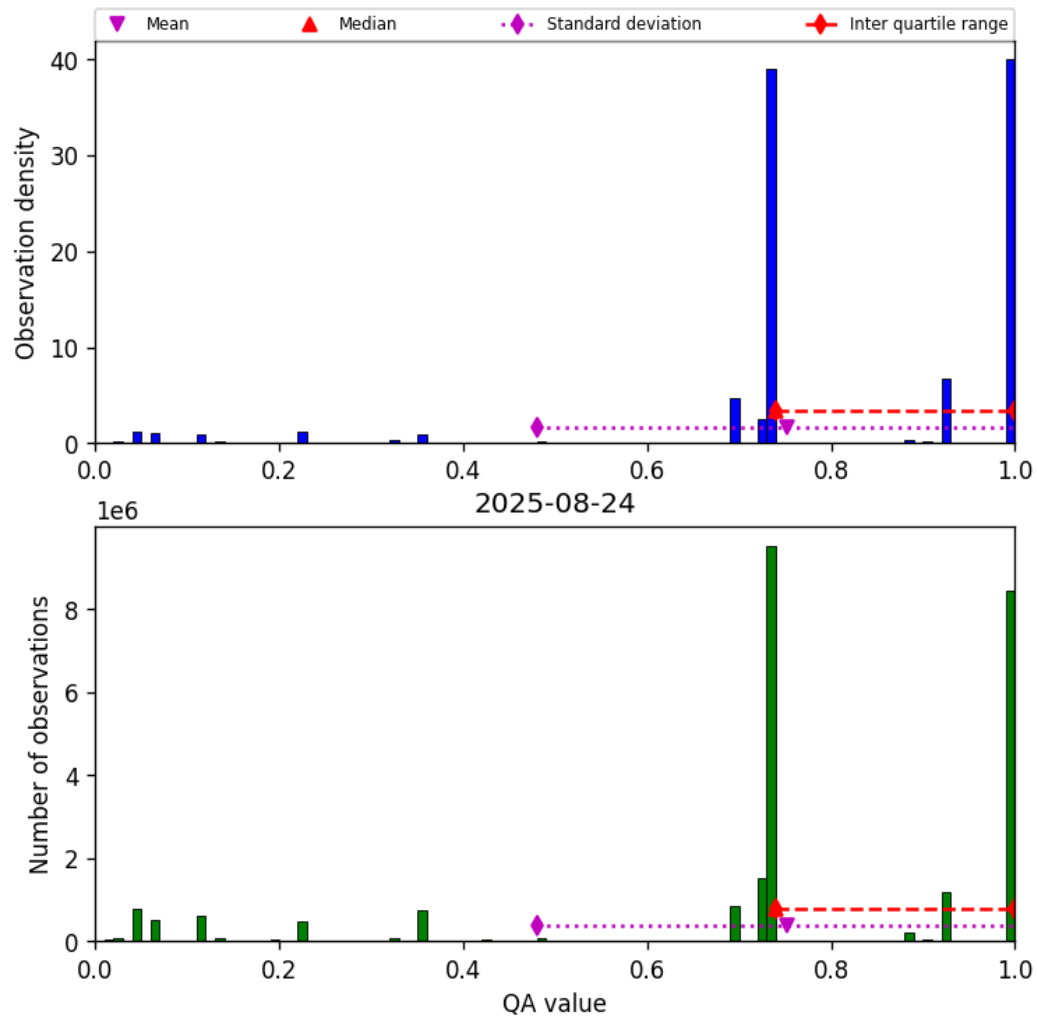
Figure 26: Histogram of “QA value” for 2025-08-24 to 2025-08-25
