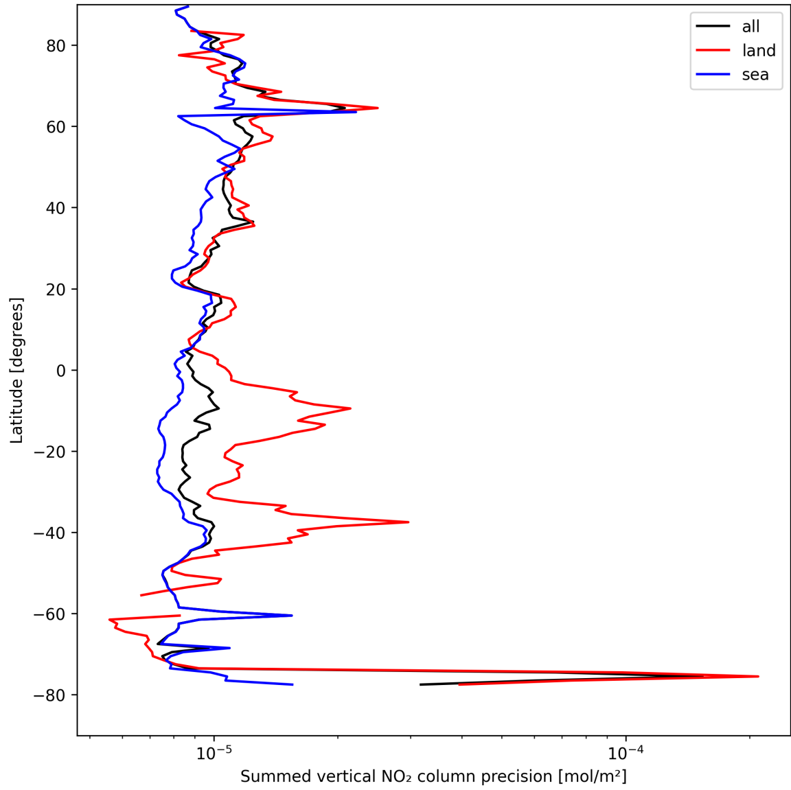
Figure 22: Zonal average of “Summed vertical NO 2 column precision” for 2025-08-24 to 2025-08-25.
