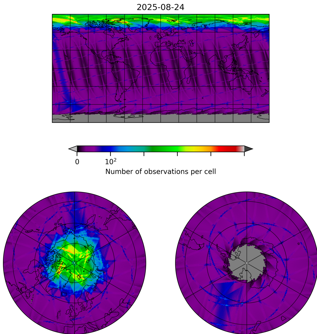
Figure 8: Map of the number of observations for 2025-08-24 to 2025-08-25
