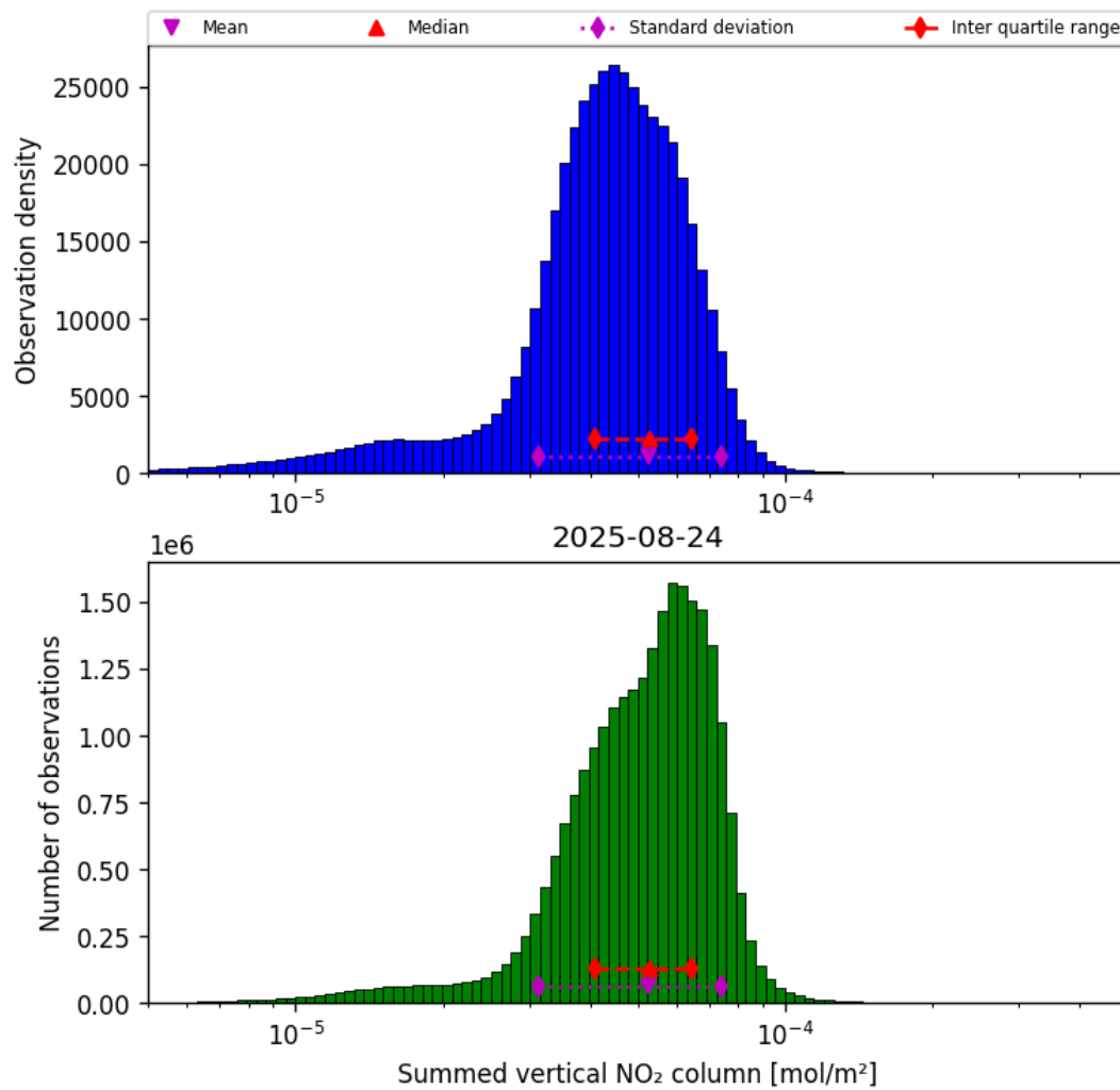
Figure 38: Histogram of “Summed vertical NO 2 column” for 2025-08-24 to 2025-08-25
