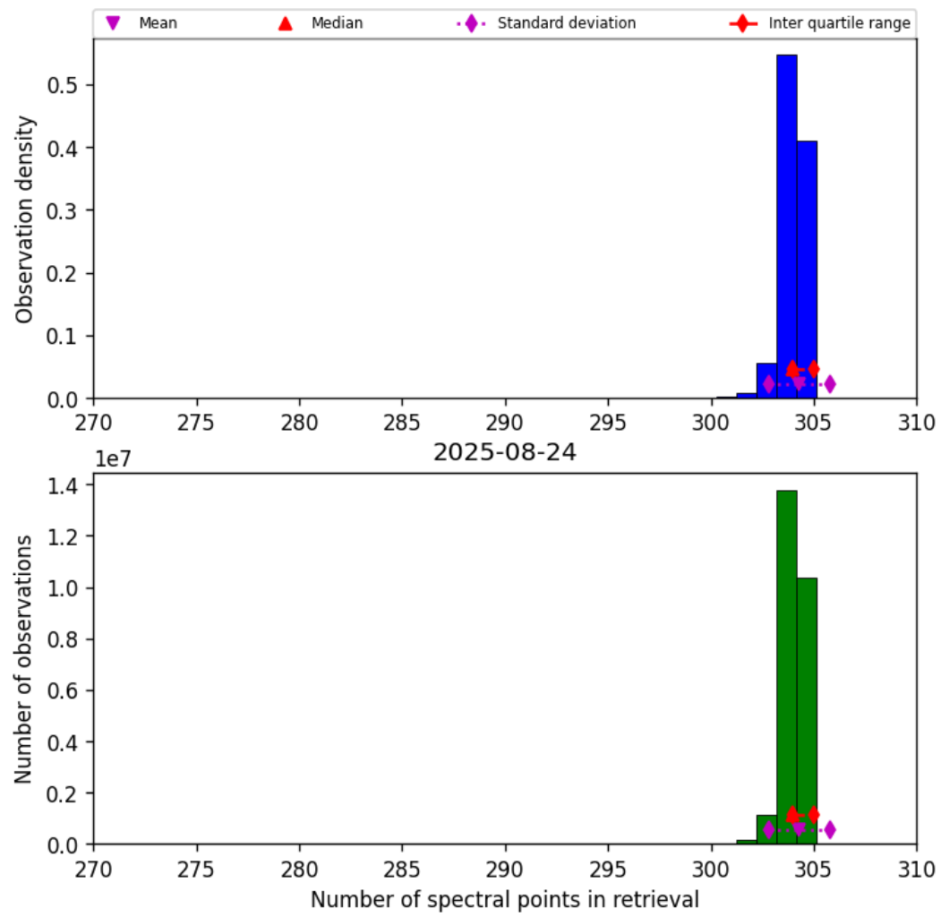
Figure 31: Histogram of “Number of spectral points in retrieval” for 2025-08-24 to 2025-08-25
