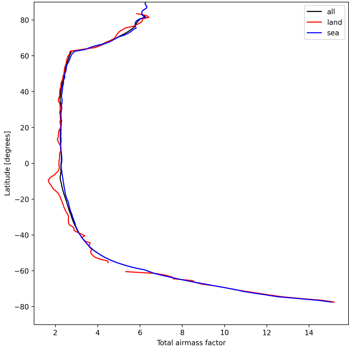
Figure 13: Zonal average of “Total airmass factor” for 2025-08-24 to 2025-08-25.
