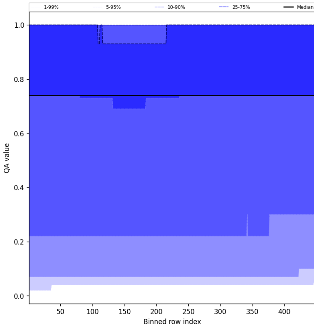
Figure 43: Along track statistics of “QA value” for 2025-08-24 to 2025-08-25
