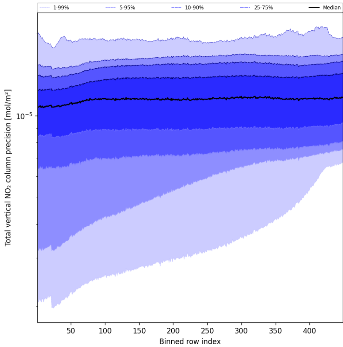
Figure 54: Along track statistics of “Total vertical NO 2 column precision” for 2025-08-24 to 2025-08-25
