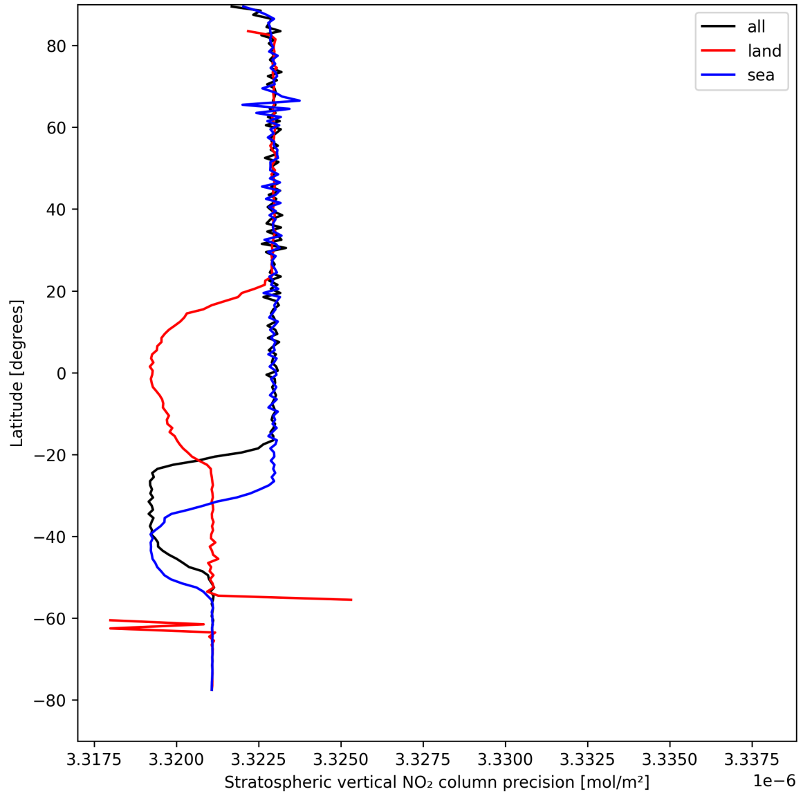
Figure 18: Zonal average of “Stratospheric vertical NO 2 column precision” for 2025-08-24 to 2025-08-25.
