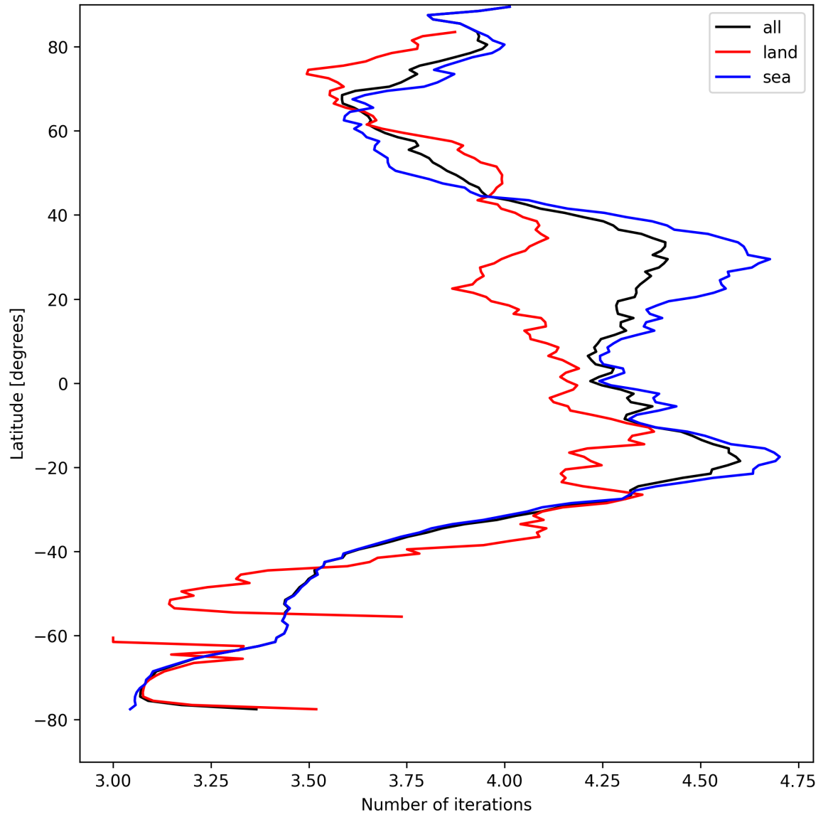
Figure 15: Zonal average of “Number of iterations” for 2025-08-24 to 2025-08-25.
