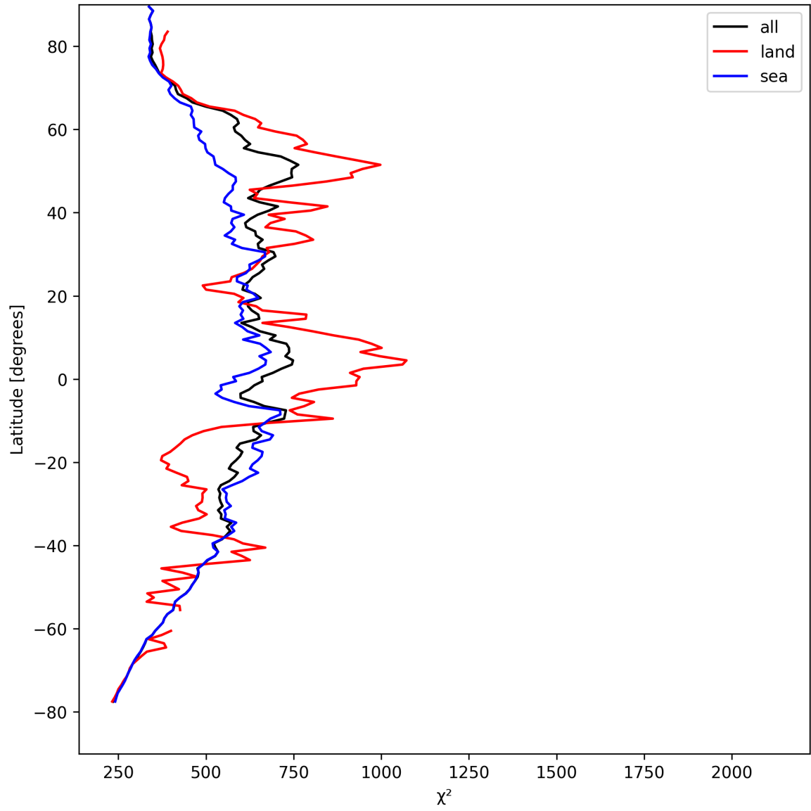
Figure 23: Zonal average of “ \chi^2 ” for 2025-08-24 to 2025-08-25.
