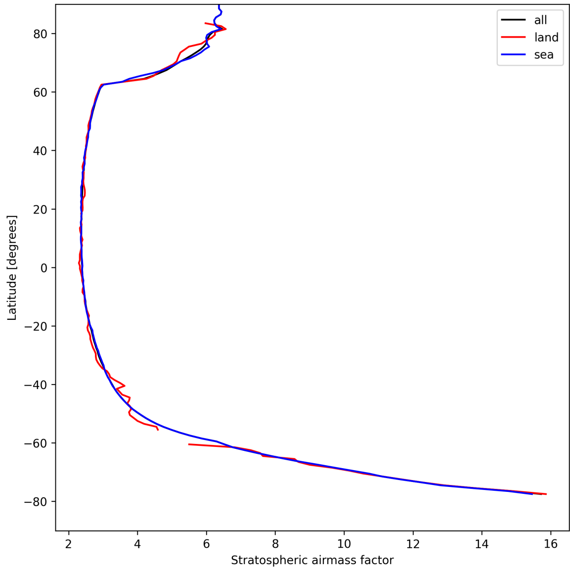
Figure 25: Zonal average of “Stratospheric airmass factor” for 2025-08-24 to 2025-08-25.
