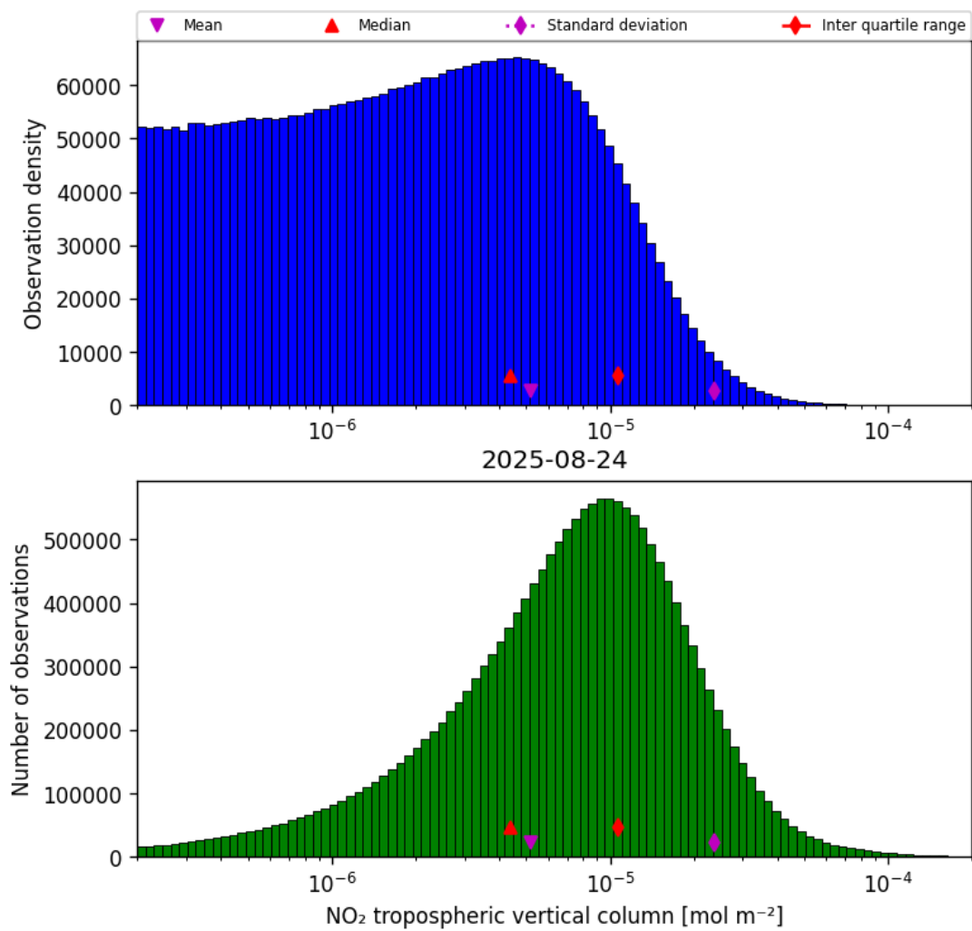
Figure 27: Histogram of “NO 2 tropospheric vertical column” for 2025-08-24 to 2025-08-25
