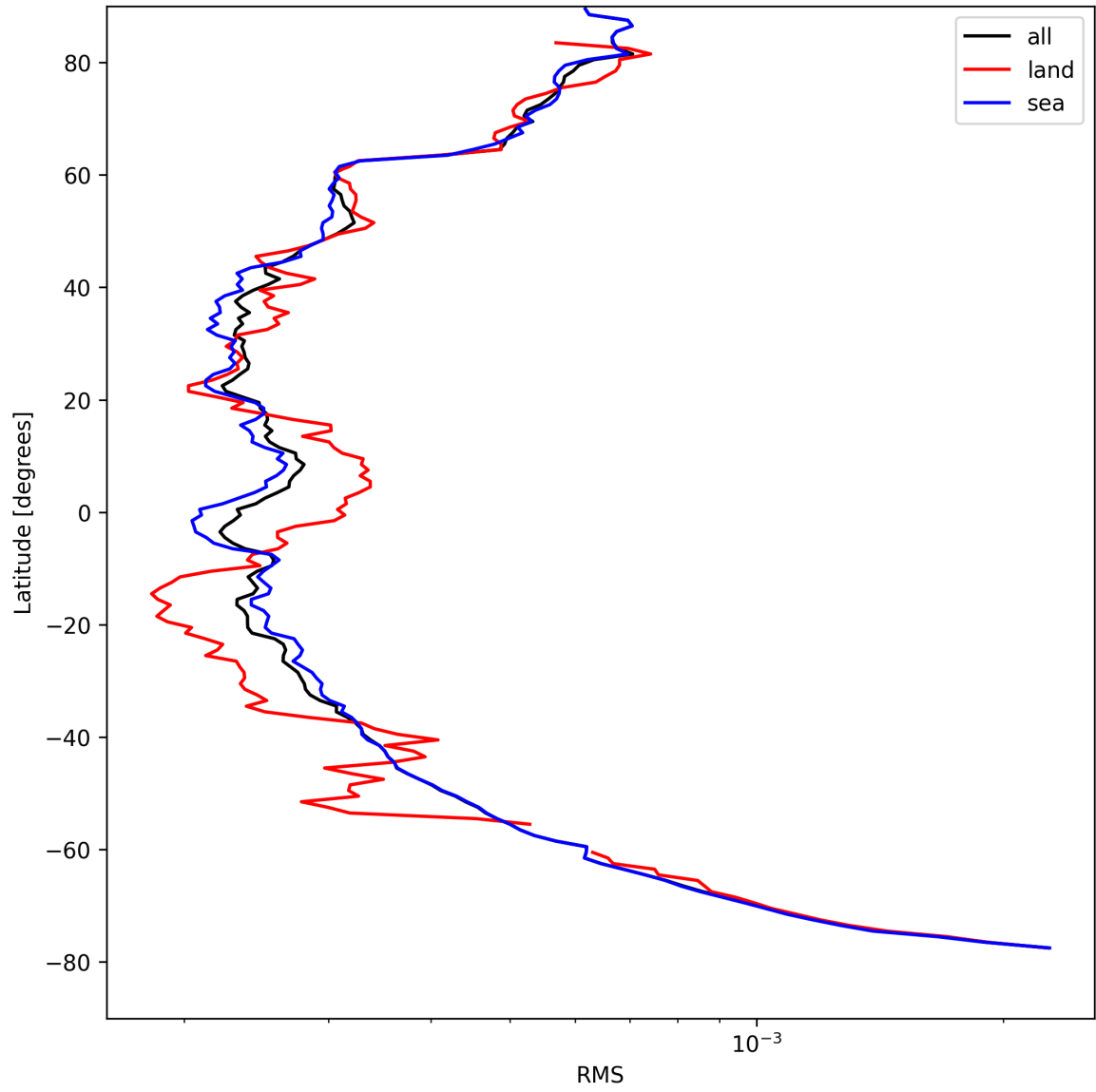
Figure 24: Zonal average of “RMS” for 2025-08-24 to 2025-08-25.
