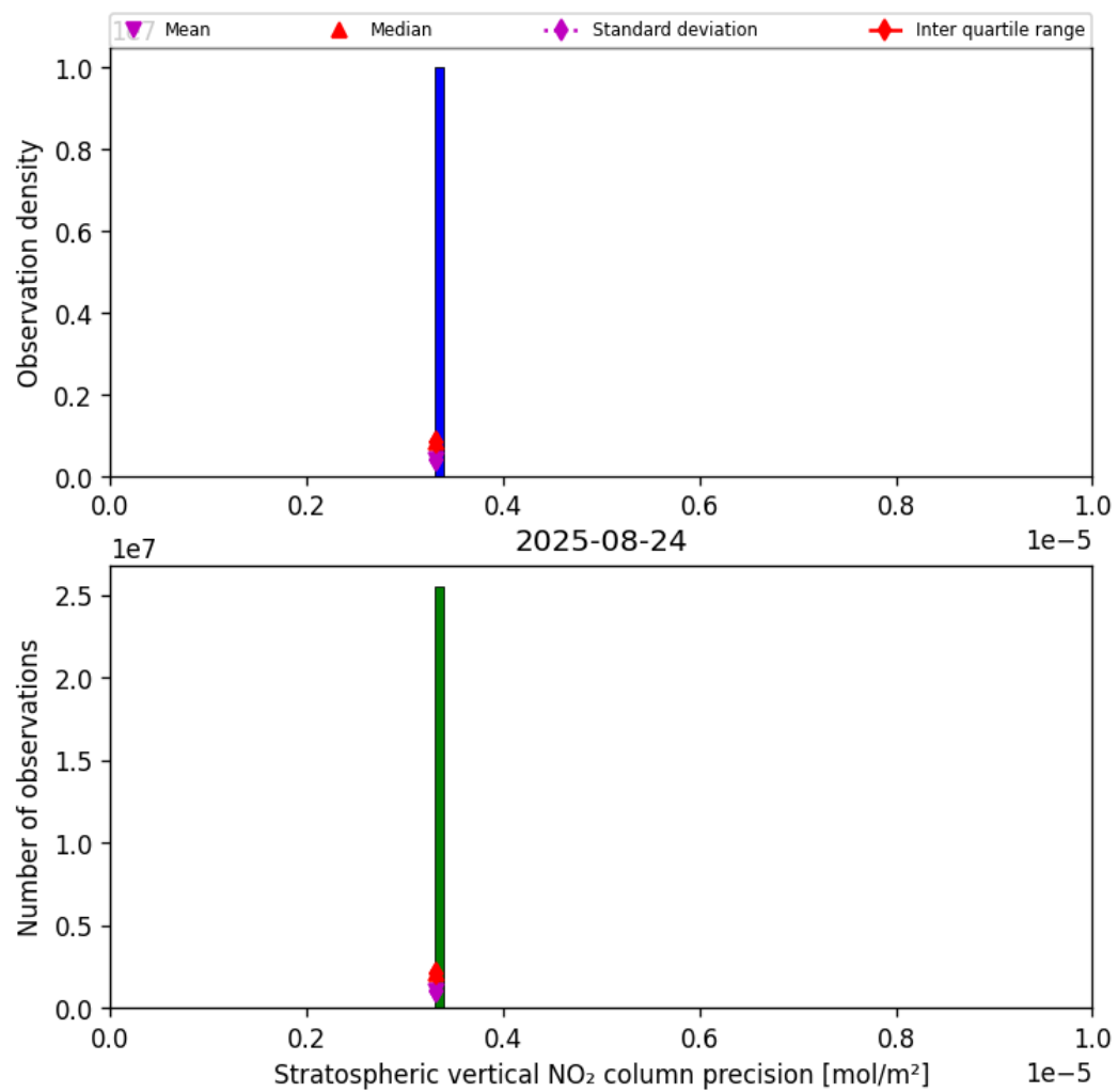
Figure 35: Histogram of “Stratospheric vertical NO 2 column precision” for 2025-08-24 to 2025-08-25
