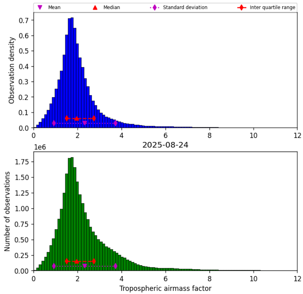
Figure 29: Histogram of “Tropospheric airmass factor” for 2025-08-24 to 2025-08-25
