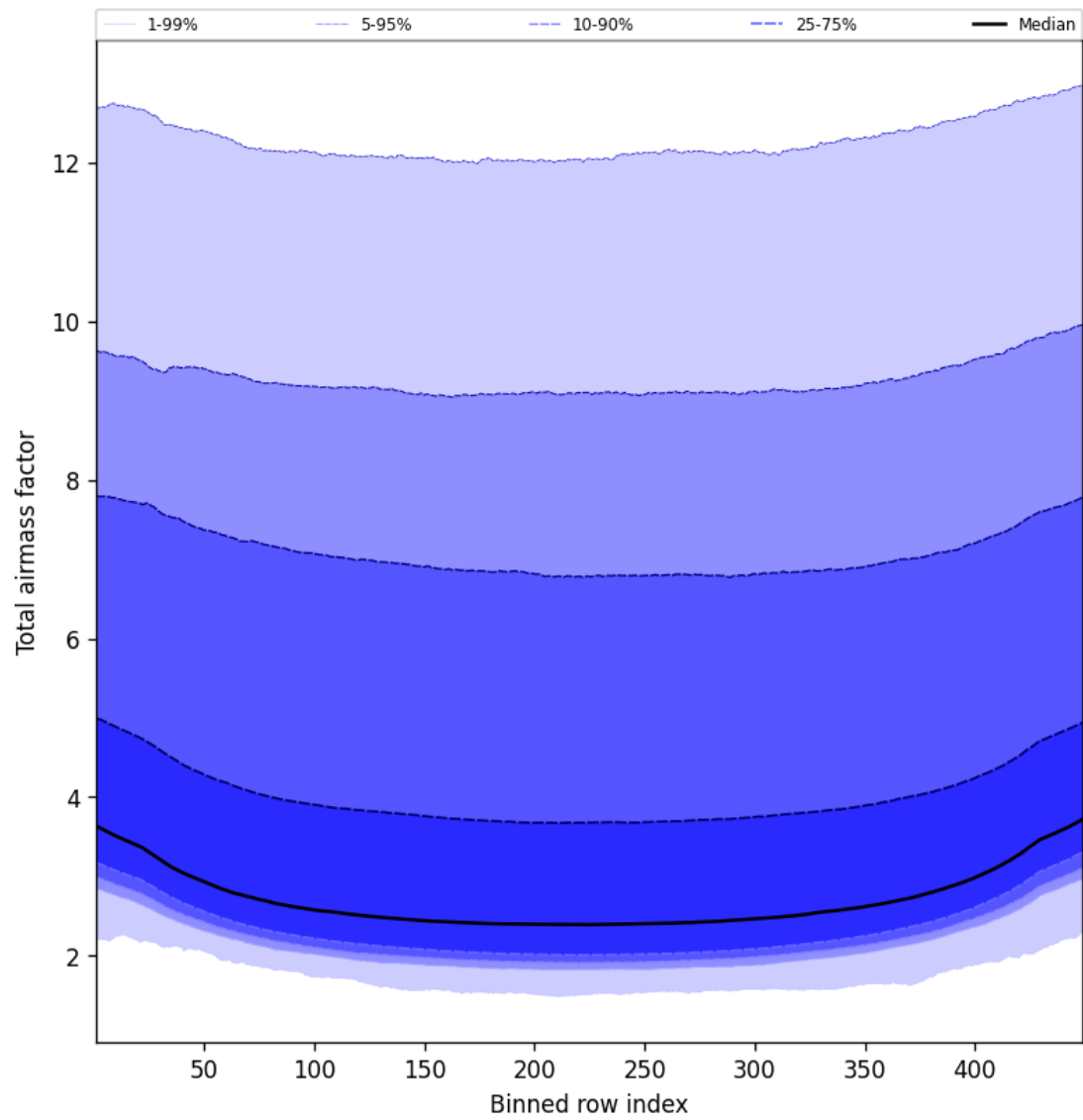
Figure 47: Along track statistics of “Total airmass factor” for 2025-08-24 to 2025-08-25
