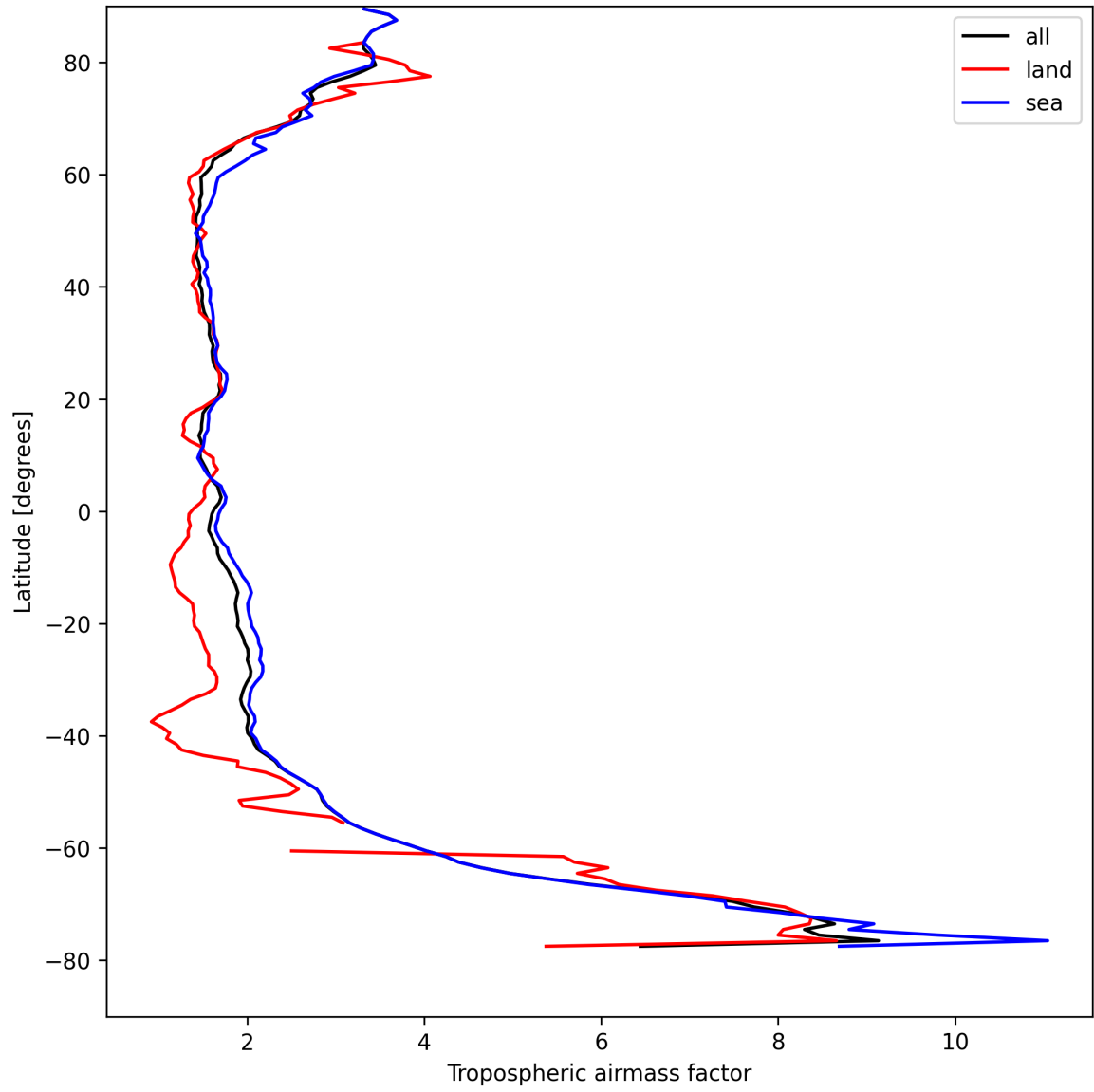
Figure 12: Zonal average of “Tropospheric airmass factor” for 2025-08-24 to 2025-08-25.
