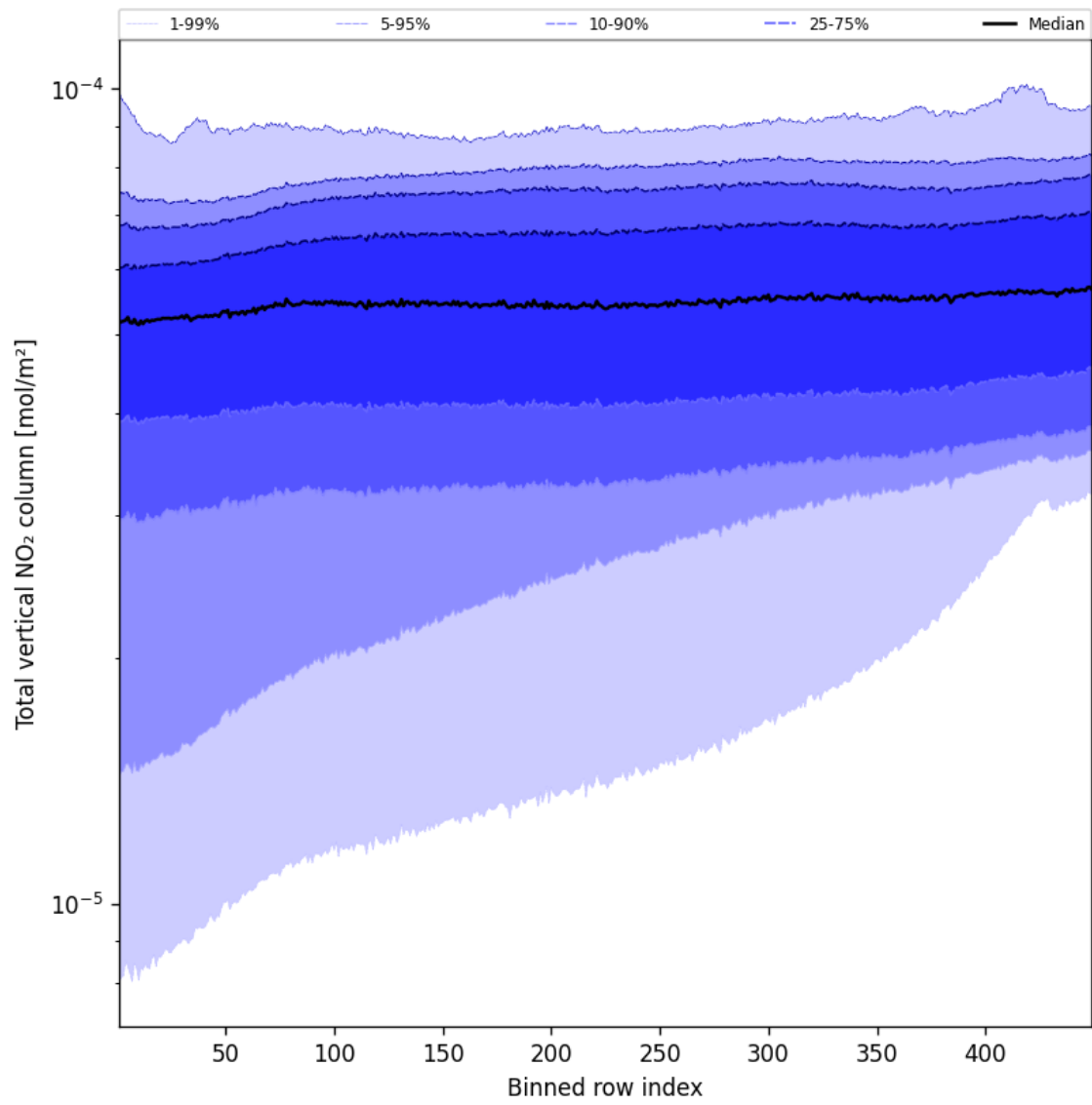
Figure 53: Along track statistics of “Total vertical NO 2 column” for 2025-08-24 to 2025-08-25
