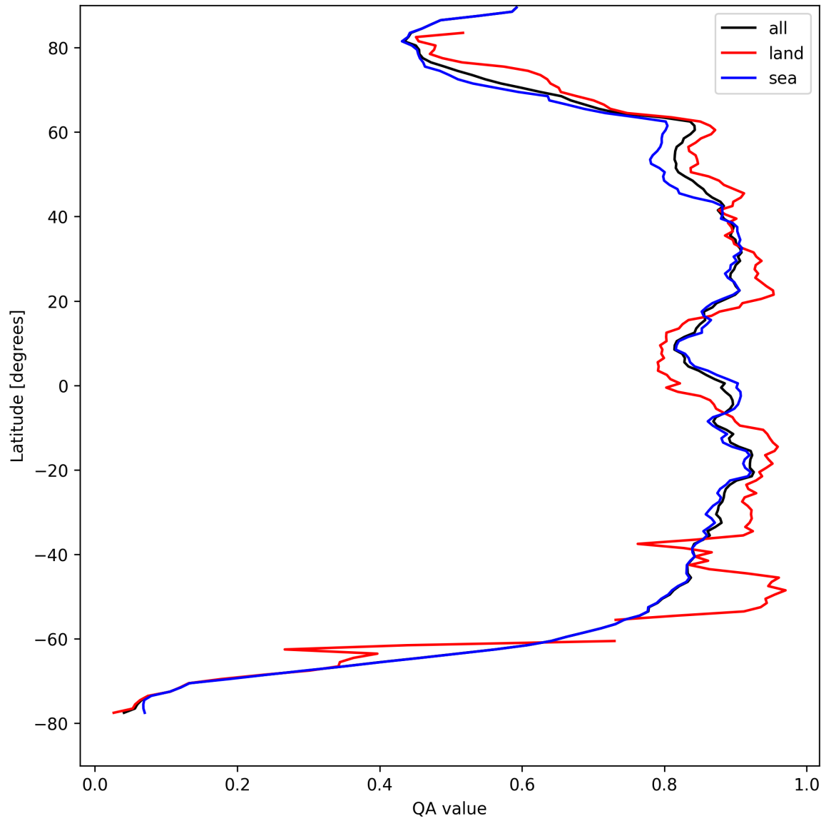
Figure 9: Zonal average of “QA value” for 2025-08-24 to 2025-08-25.
