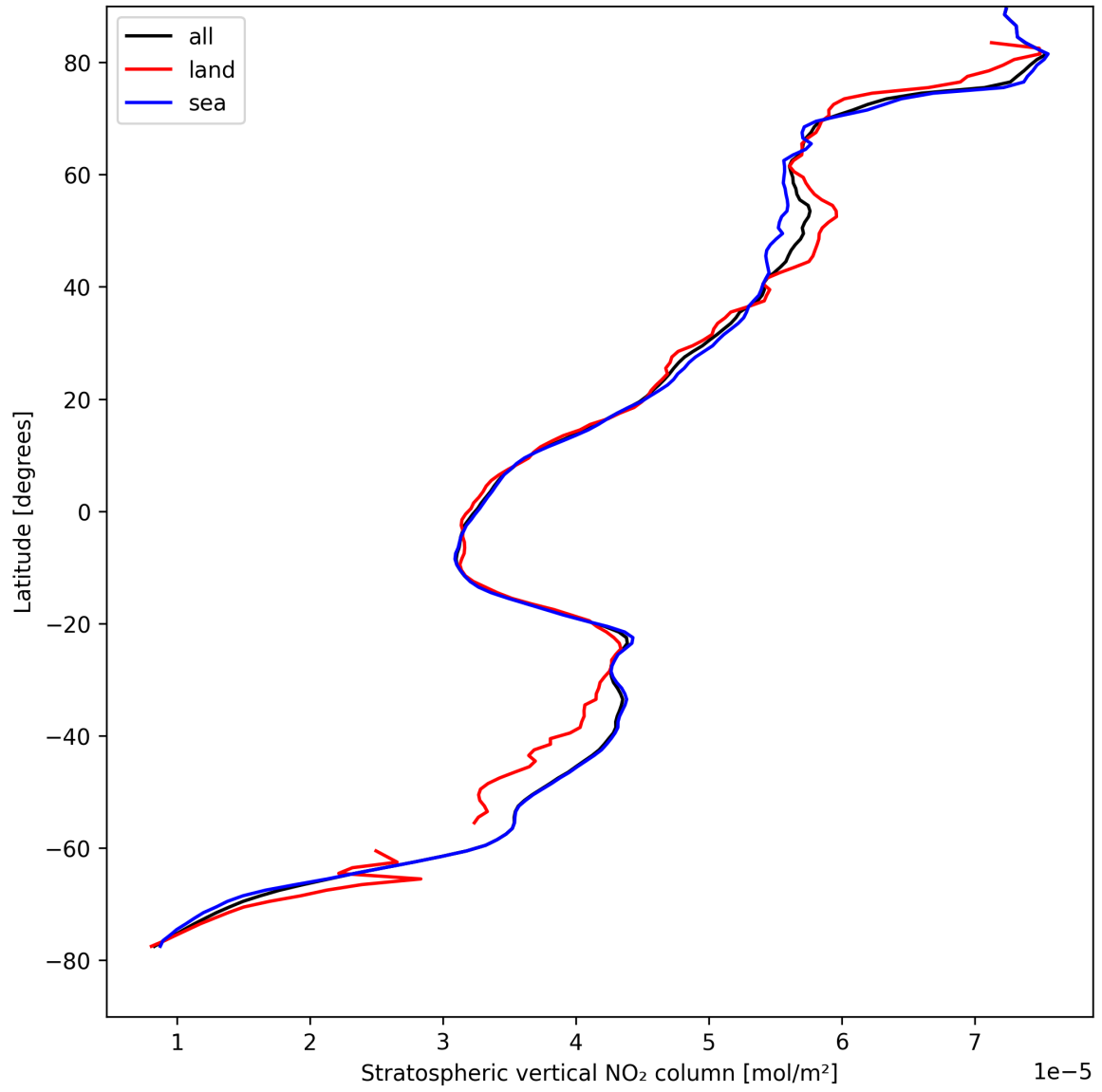
Figure 17: Zonal average of “Stratospheric vertical NO 2 column” for 2025-08-24 to 2025-08-25.
