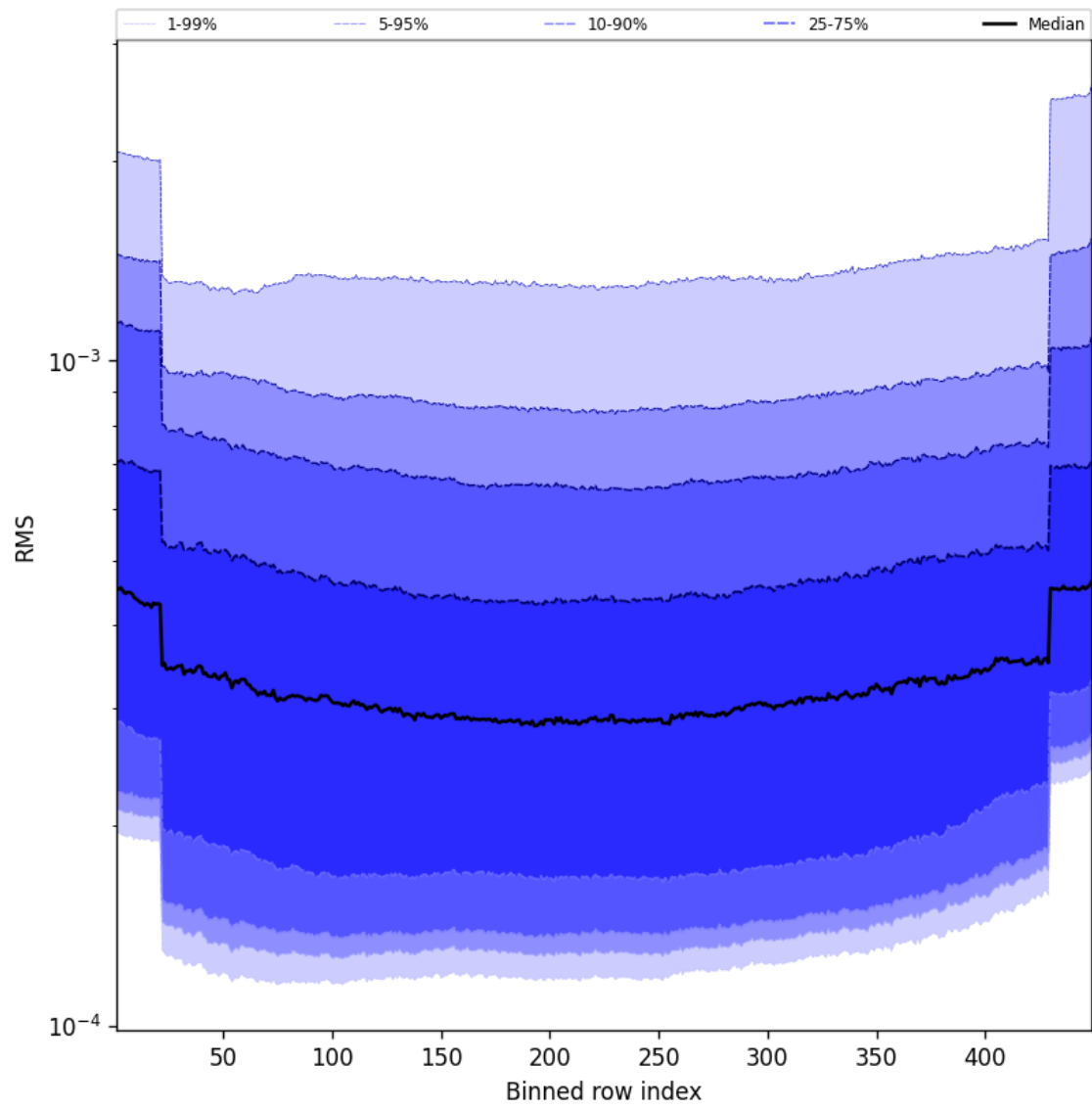
Figure 58: Along track statistics of “RMS” for 2025-08-24 to 2025-08-25
