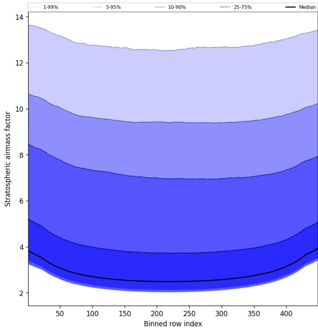
Figure 59: Along track statistics of “Stratospheric airmass factor” for 2025-08-24 to 2025-08-25
