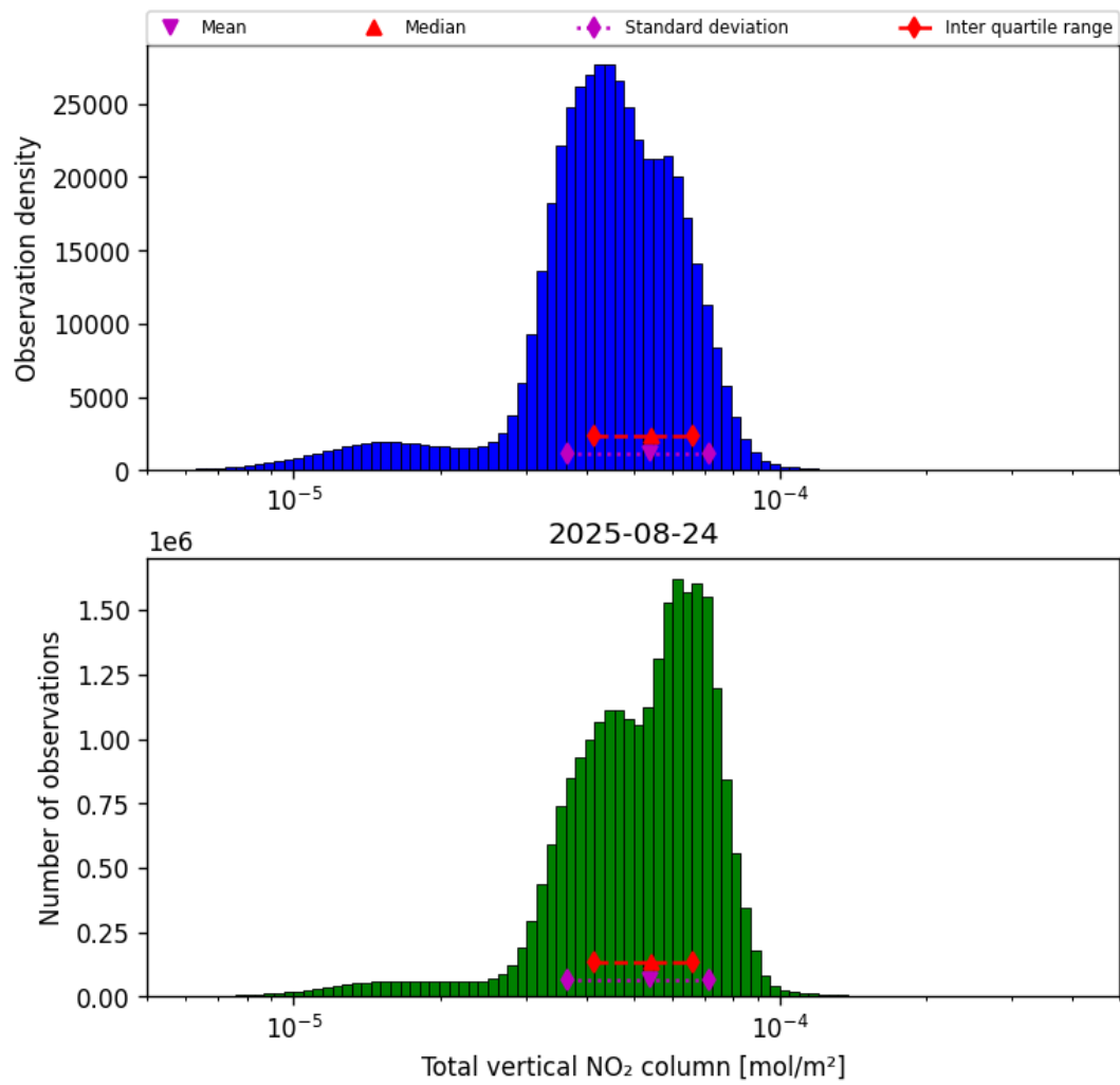
Figure 36: Histogram of “Total vertical NO 2 column” for 2025-08-24 to 2025-08-25
