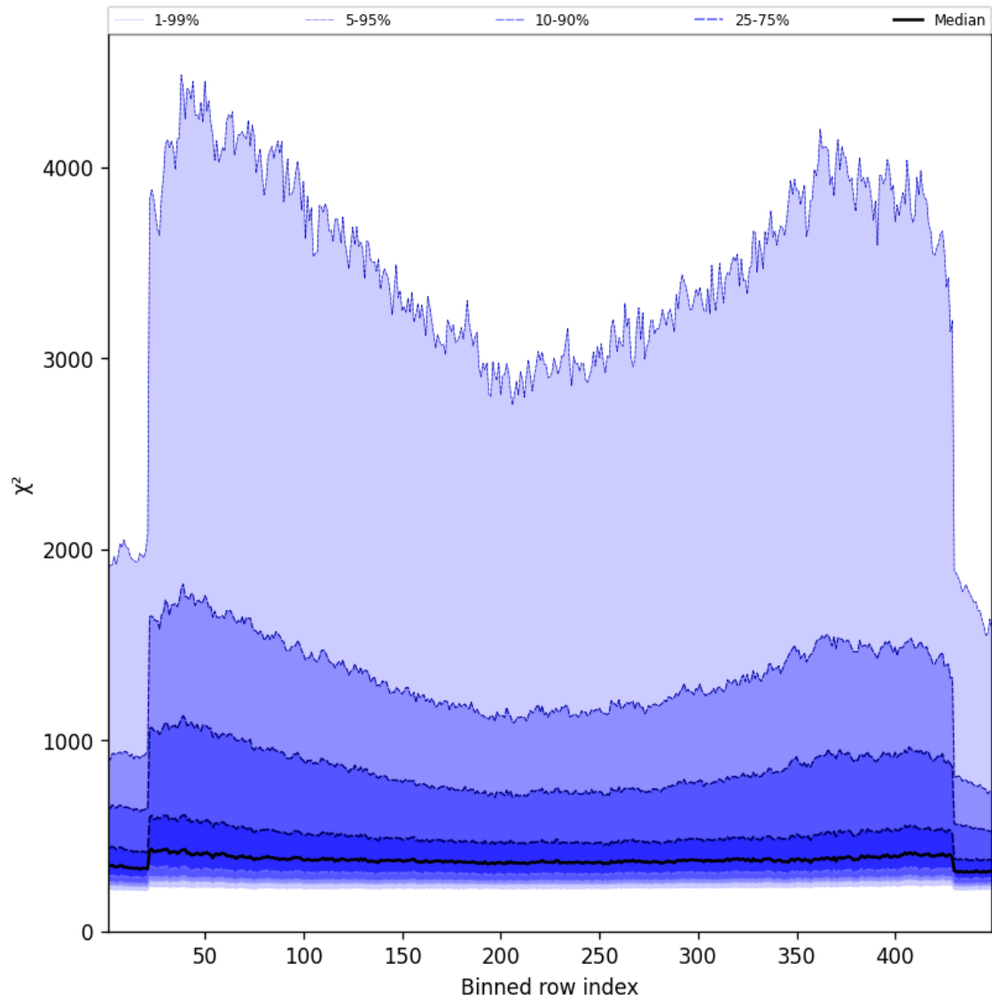
Figure 57: Along track statistics of “ \chi^2 ” for 2025-08-24 to 2025-08-25
