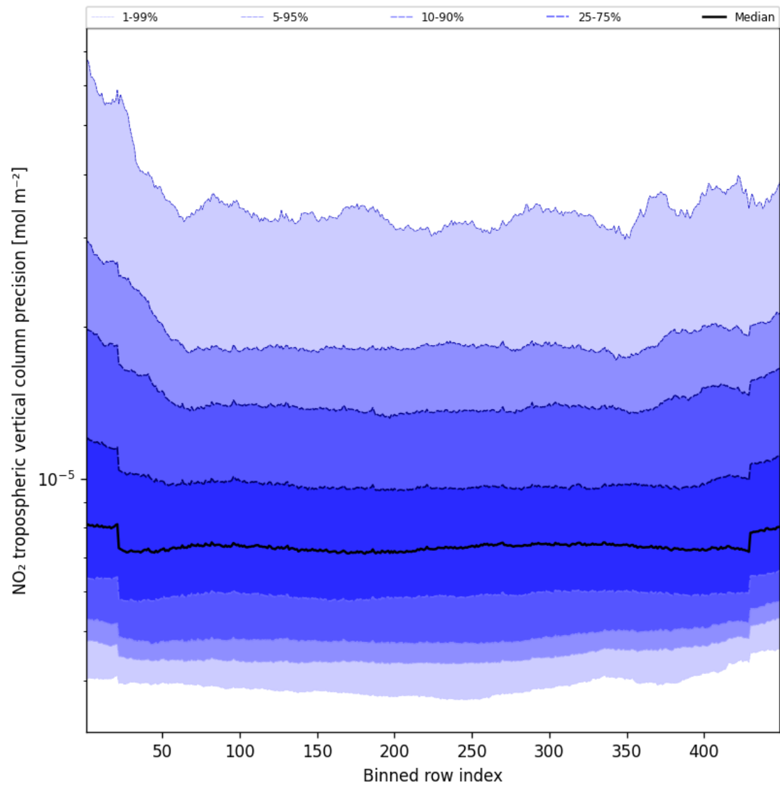
Figure 45: Along track statistics of “NO 2 tropospheric vertical column precision” for 2025-08-24 to 2025-08-25
