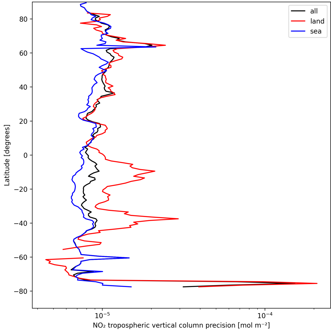
Figure 11: Zonal average of “NO 2 tropospheric vertical column precision” for 2025-08-24 to 2025-08-25.
