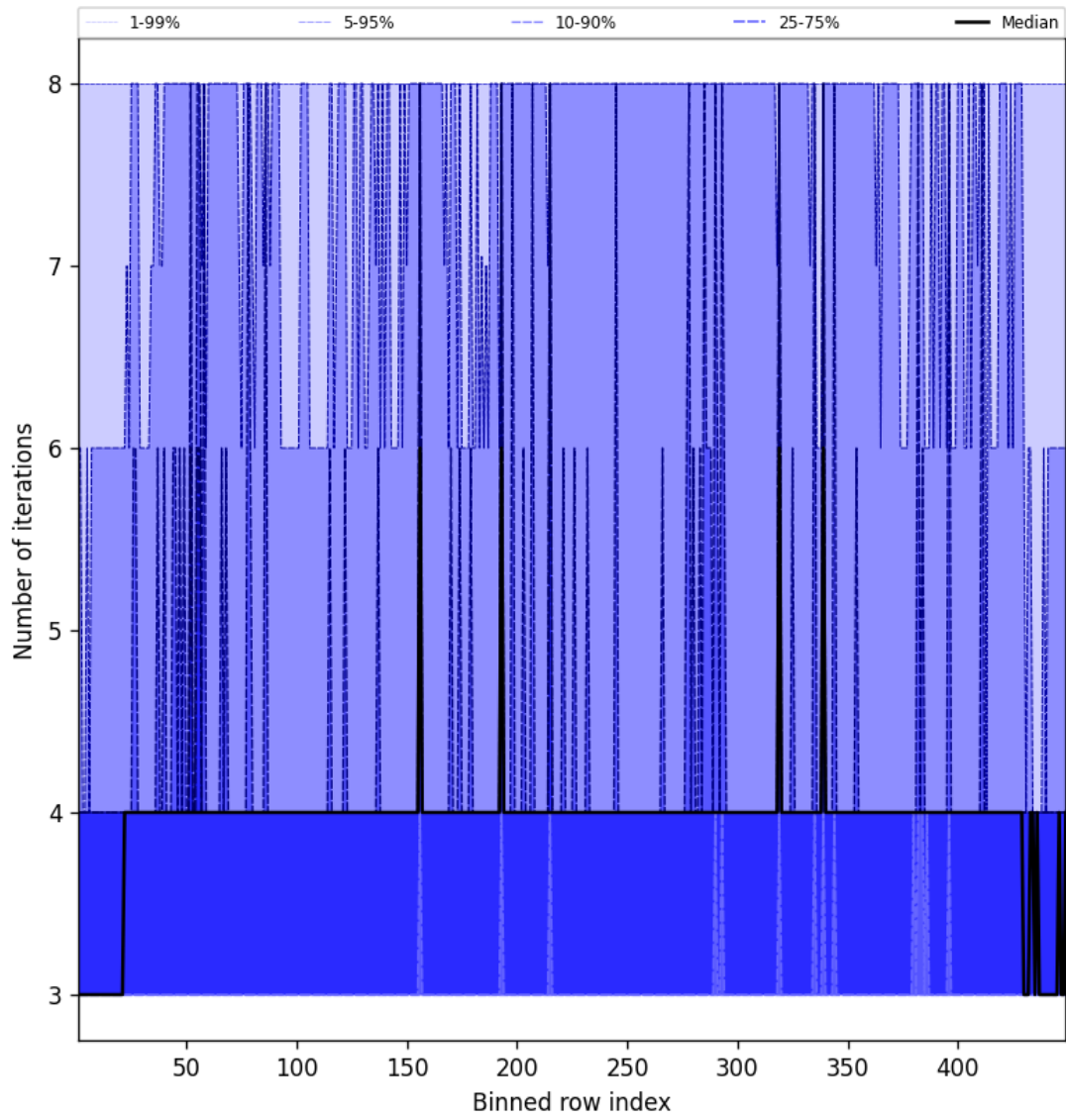
Figure 49: Along track statistics of “Number of iterations” for 2025-08-24 to 2025-08-25
