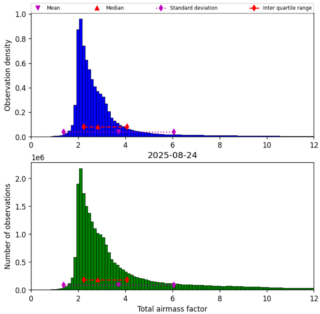
Figure 30: Histogram of “Total airmass factor” for 2025-08-24 to 2025-08-25
