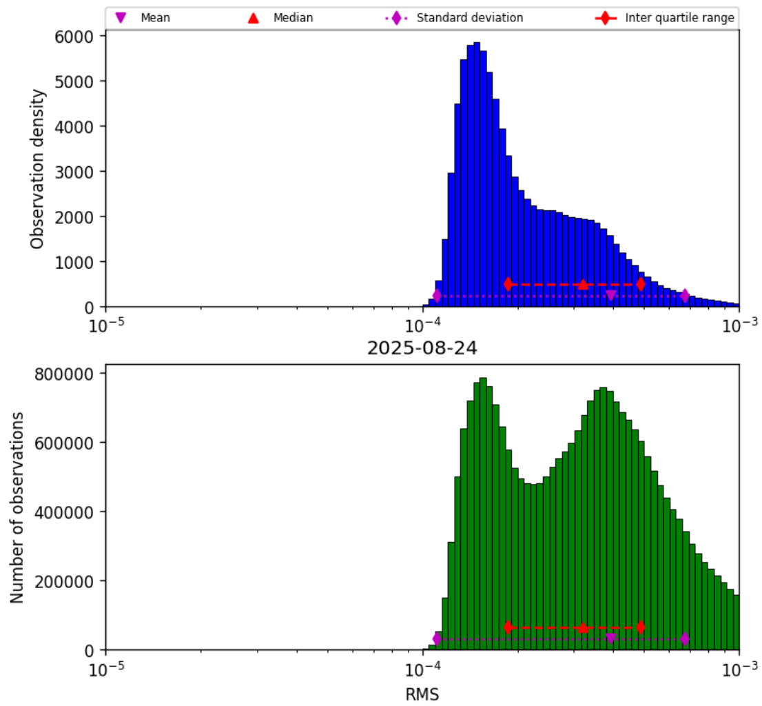
Figure 41: Histogram of “RMS” for 2025-08-24 to 2025-08-25
