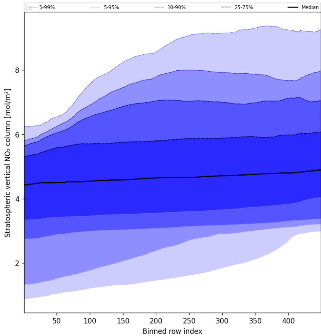
Figure 51: Along track statistics of “Stratospheric vertical NO 2 column” for 2025-08-24 to 2025-08-25
