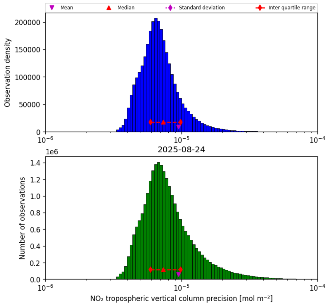
Figure 28: Histogram of “NO 2 tropospheric vertical column precision” for 2025-08-24 to 2025-08-25
