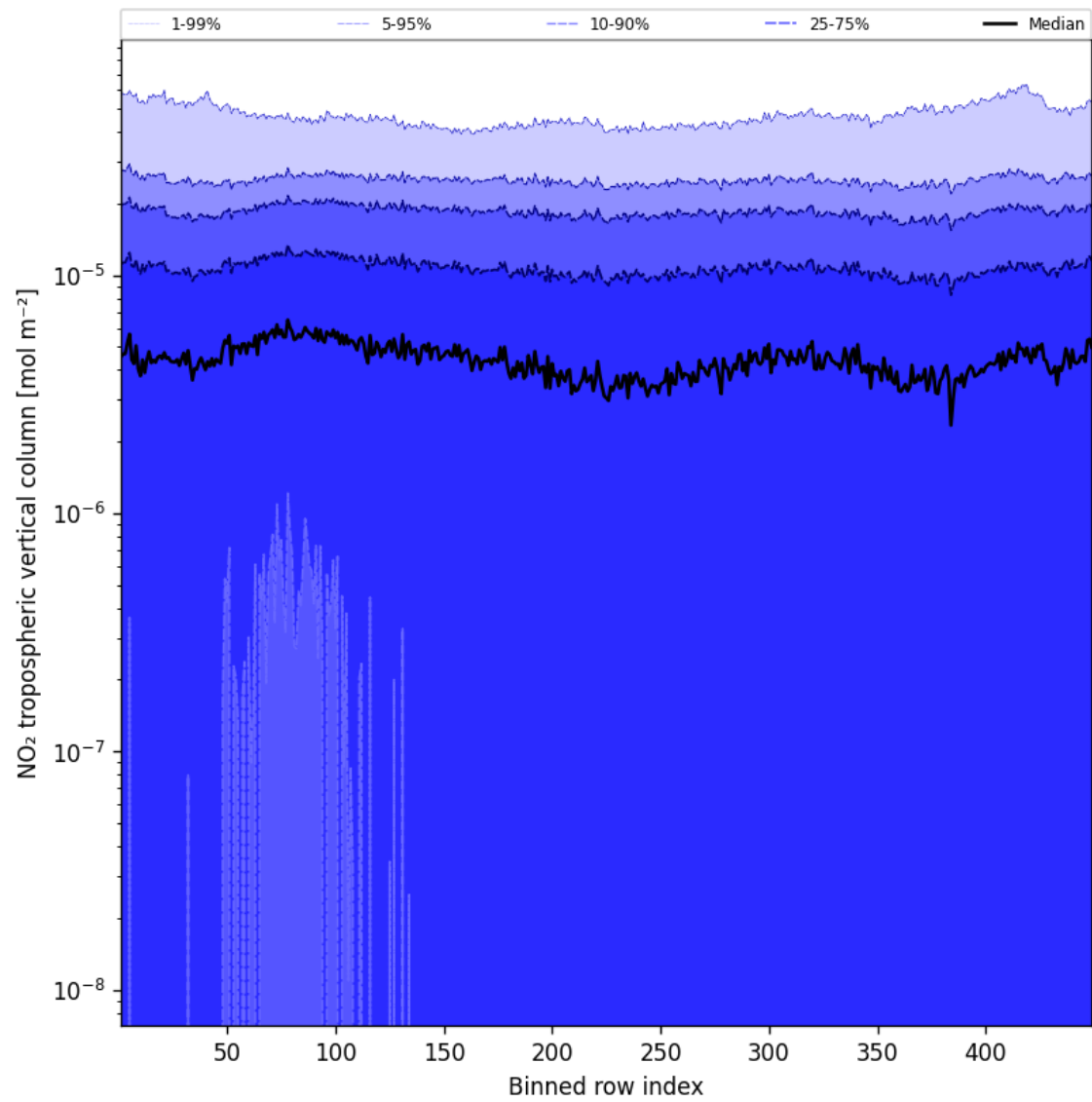
Figure 44: Along track statistics of “NO 2 tropospheric vertical column” for 2025-08-24 to 2025-08-25
