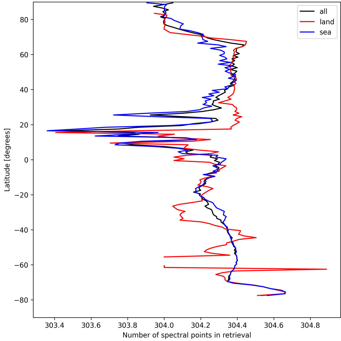
Figure 14: Zonal average of “Number of spectral points in retrieval” for 2025-08-24 to 2025-08-25.
