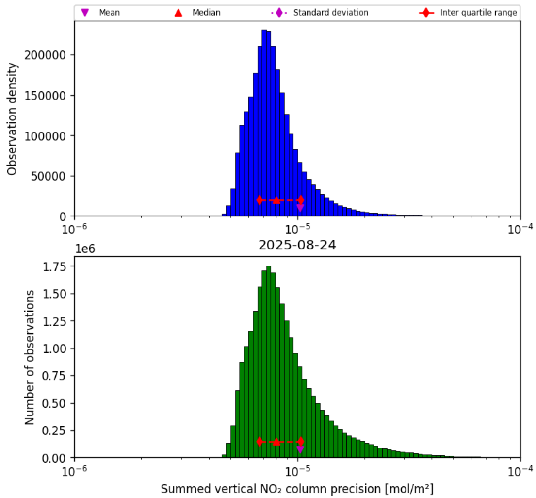
Figure 39: Histogram of “Summed vertical NO 2 column precision” for 2025-08-24 to 2025-08-25
