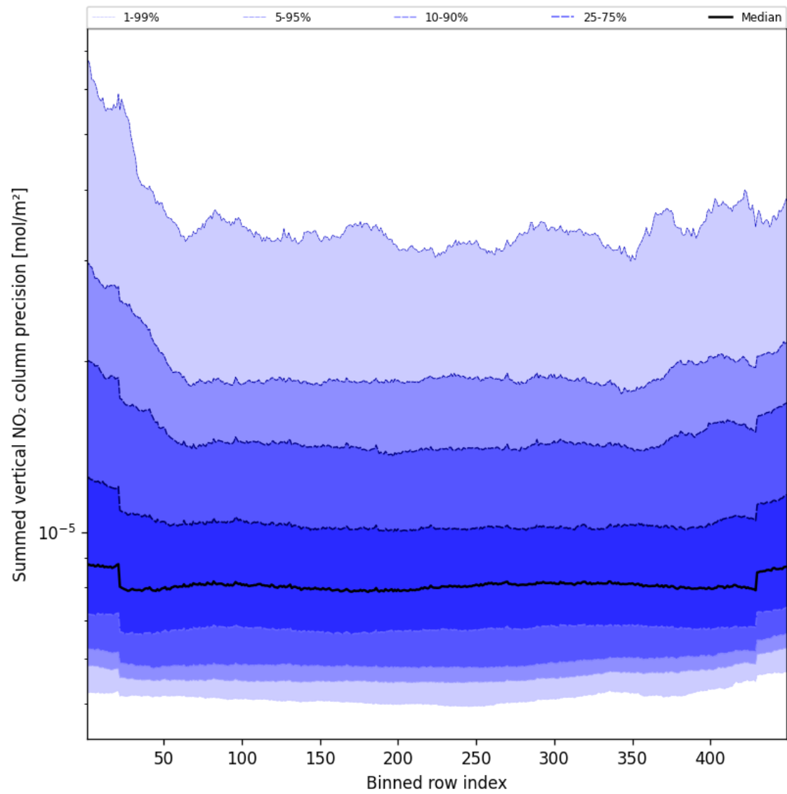
Figure 56: Along track statistics of “Summed vertical NO 2 column precision” for 2025-08-24 to 2025-08-25
