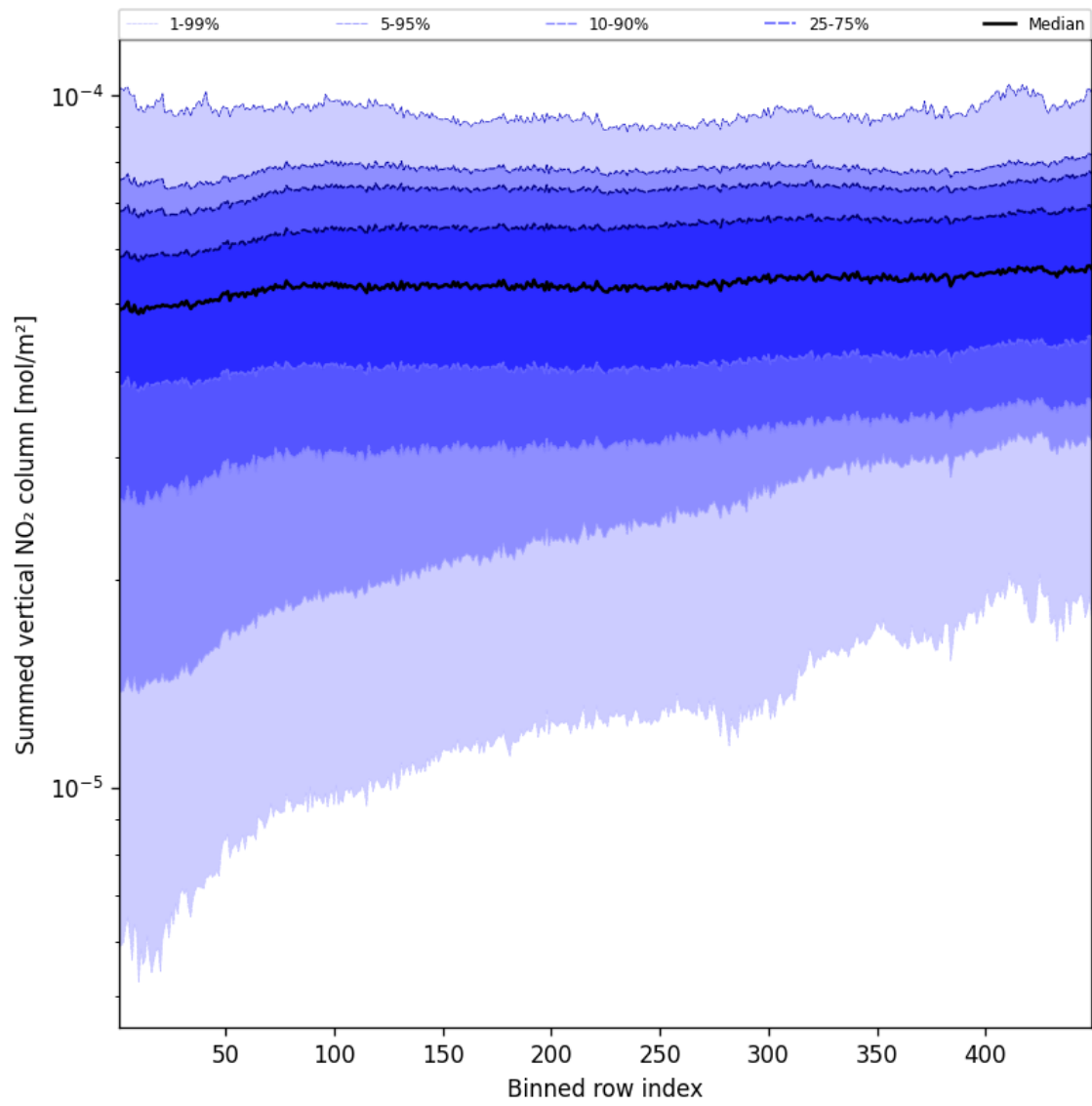
Figure 55: Along track statistics of “Summed vertical NO 2 column” for 2025-08-24 to 2025-08-25
