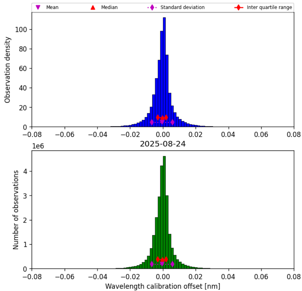
Figure 33: Histogram of “Wavelength calibration offset” for 2025-08-24 to 2025-08-25
