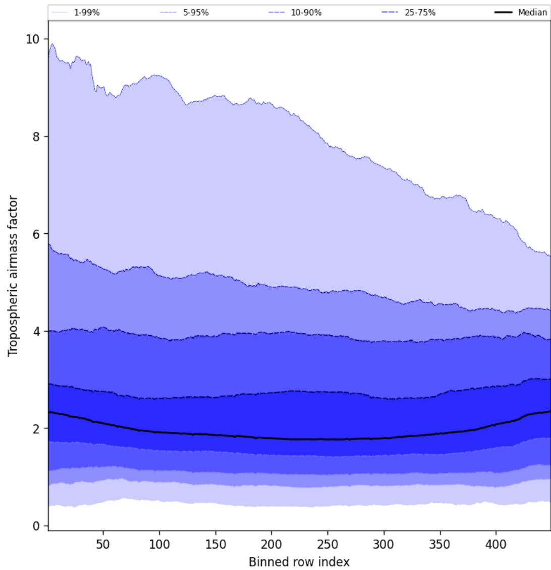
Figure 46: Along track statistics of “Tropospheric air mass factor” for 2025-08-24 to 2025-08-25
