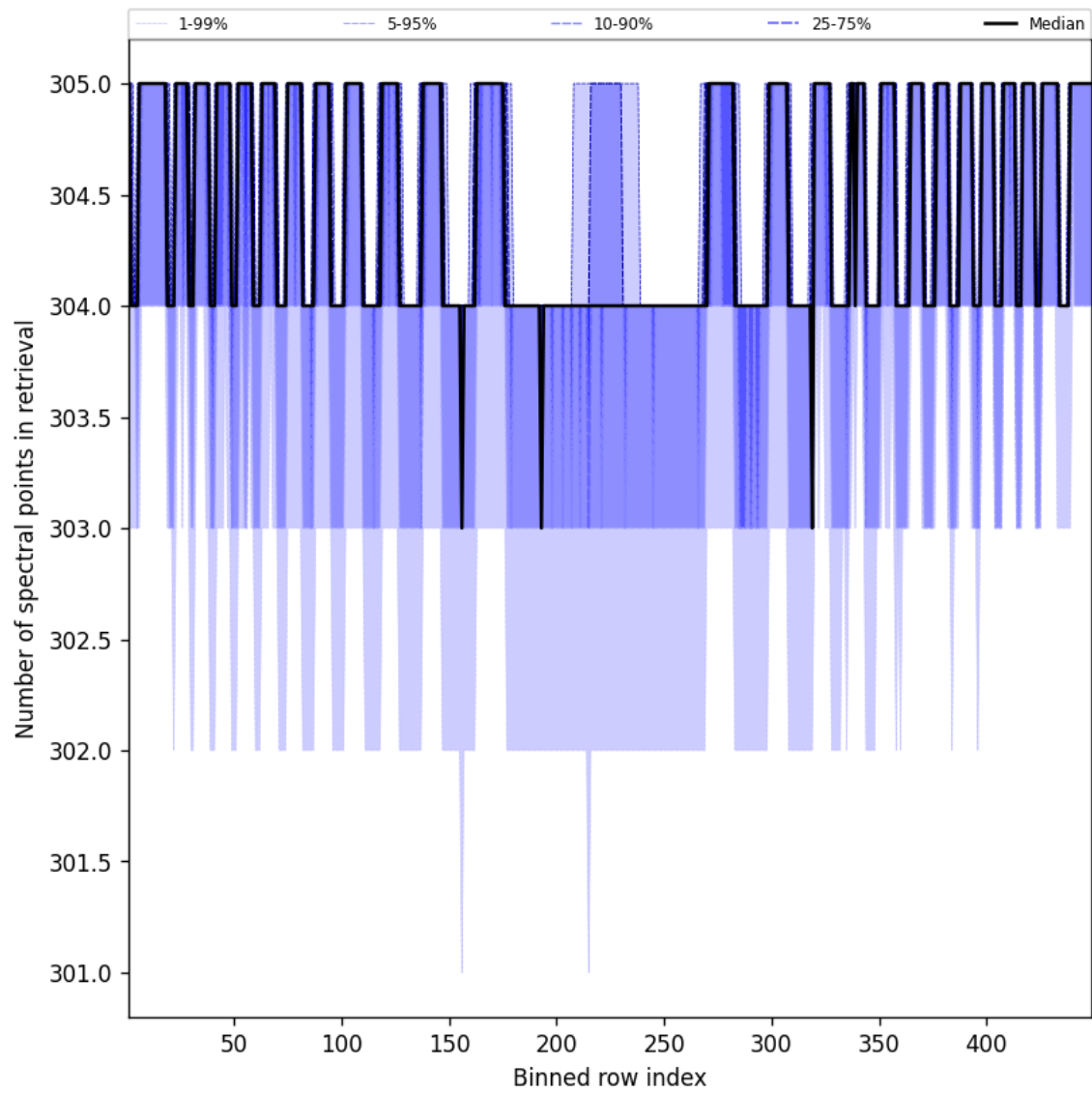
Figure 48: Along track statistics of “Number of spectral points in retrieval” for 2025-08-24 to 2025-08-25
