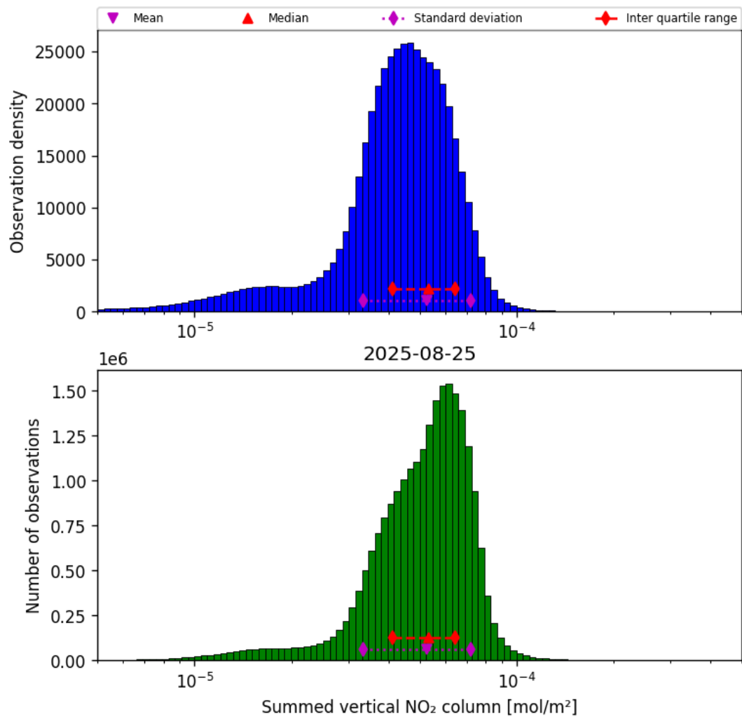
Figure 38: Histogram of “Summed vertical NO 2 column” for 2025-08-25 to 2025-08-26
