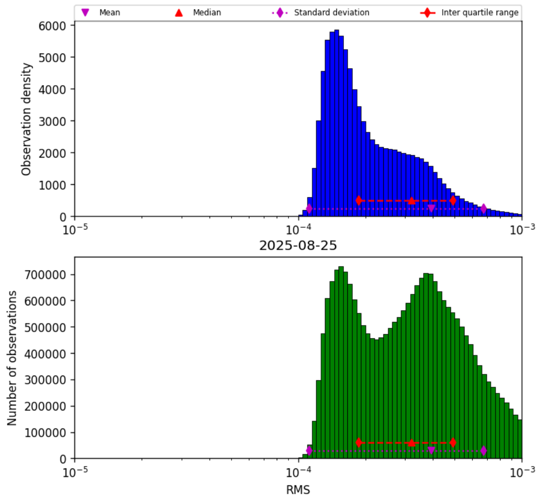
Figure 41: Histogram of “RMS” for 2025-08-25 to 2025-08-26
