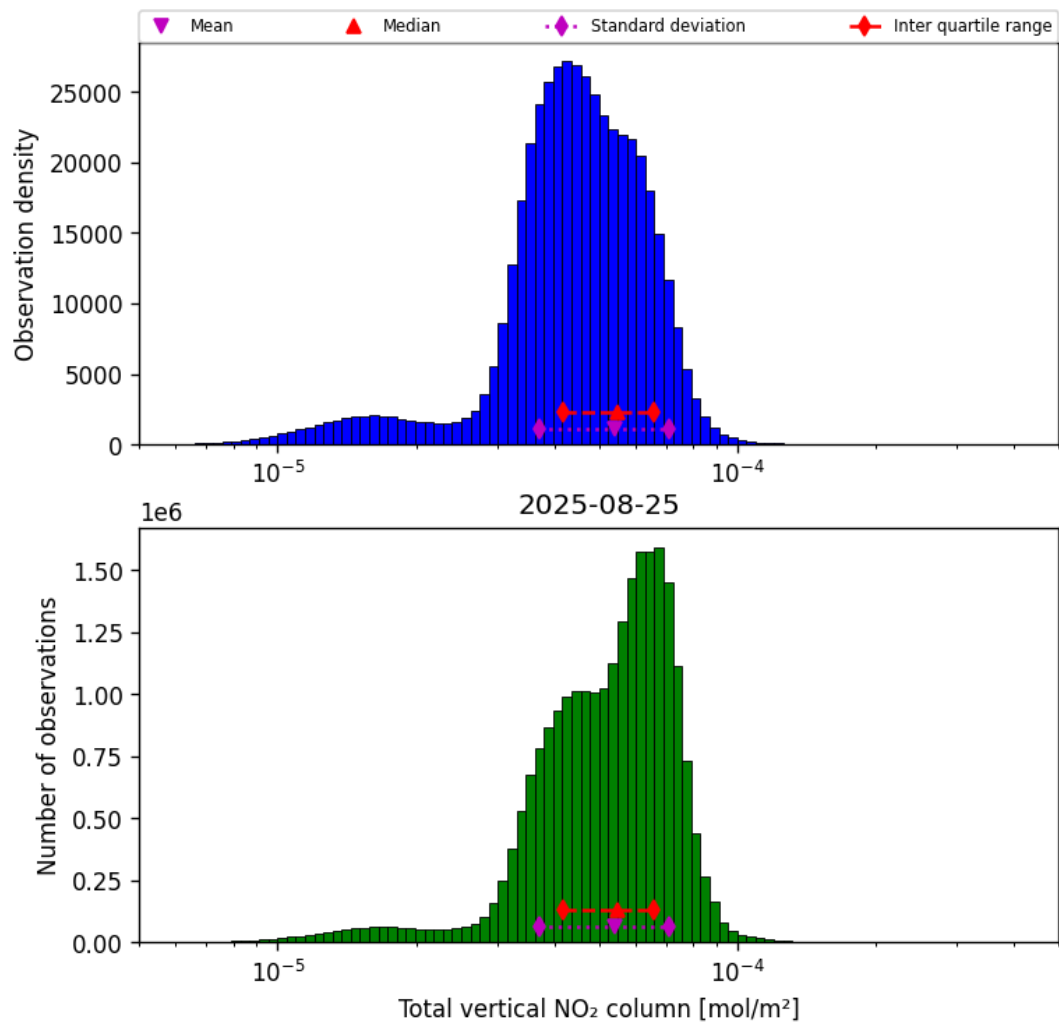
Figure 36: Histogram of “Total vertical NO 2 column” for 2025-08-25 to 2025-08-26
