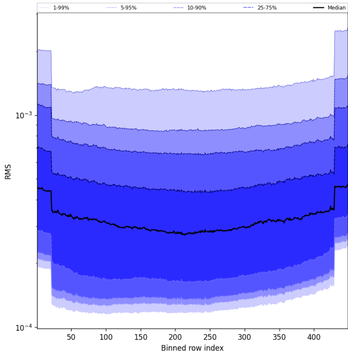
Figure 58: Along track statistics of “RMS” for 2025-08-25 to 2025-08-26
