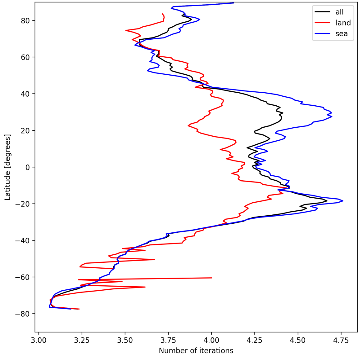
Figure 15: Zonal average of “Number of iterations” for 2025-08-25 to 2025-08-26.
