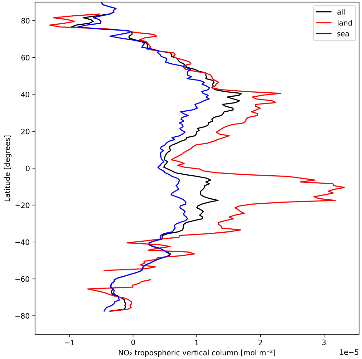
Figure 10: Zonal average of “NO 2 tropospheric vertical column” for 2025-08-25 to 2025-08-26.
