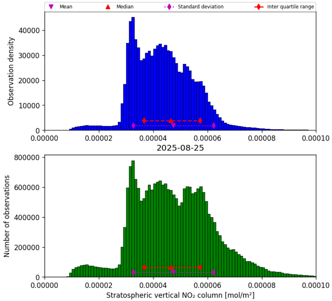
Figure 34: Histogram of “Stratospheric vertical NO 2 column” for 2025-08-25 to 2025-08-26
