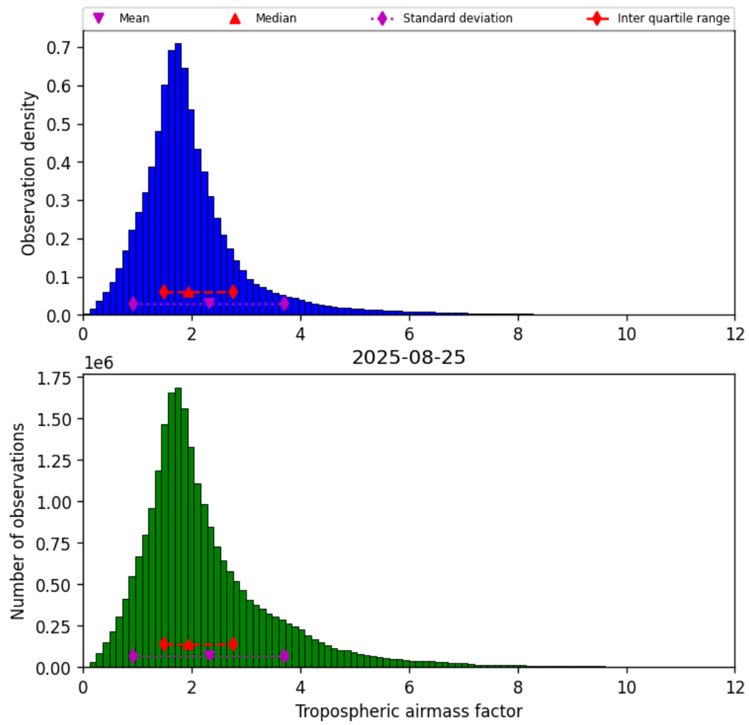
Figure 29: Histogram of “Tropospheric airmass factor” for 2025-08-25 to 2025-08-26
