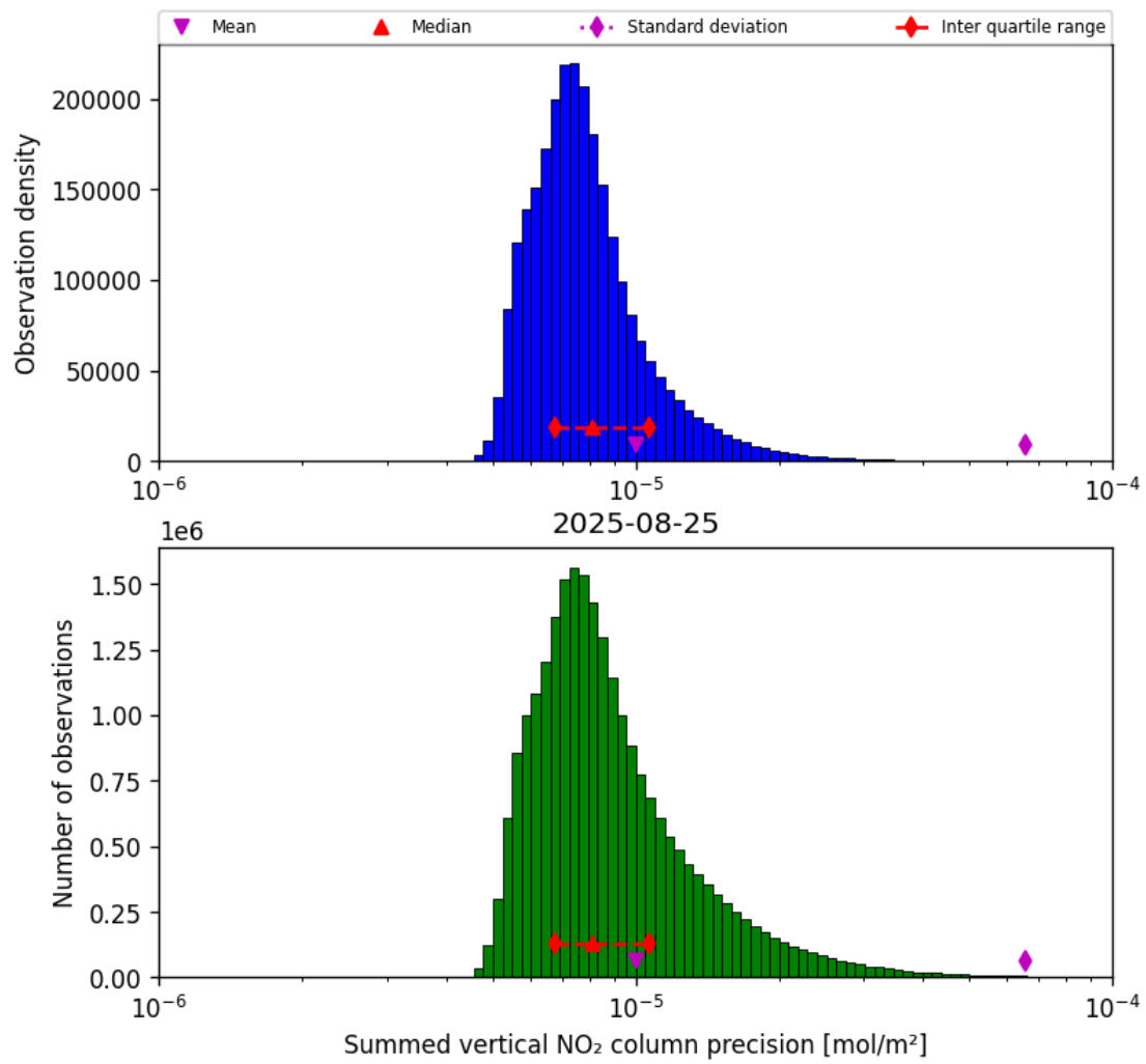
Figure 39: Histogram of "Summed vertical NO 2 column precision" for 2025-08-25 to 2025-08-26
