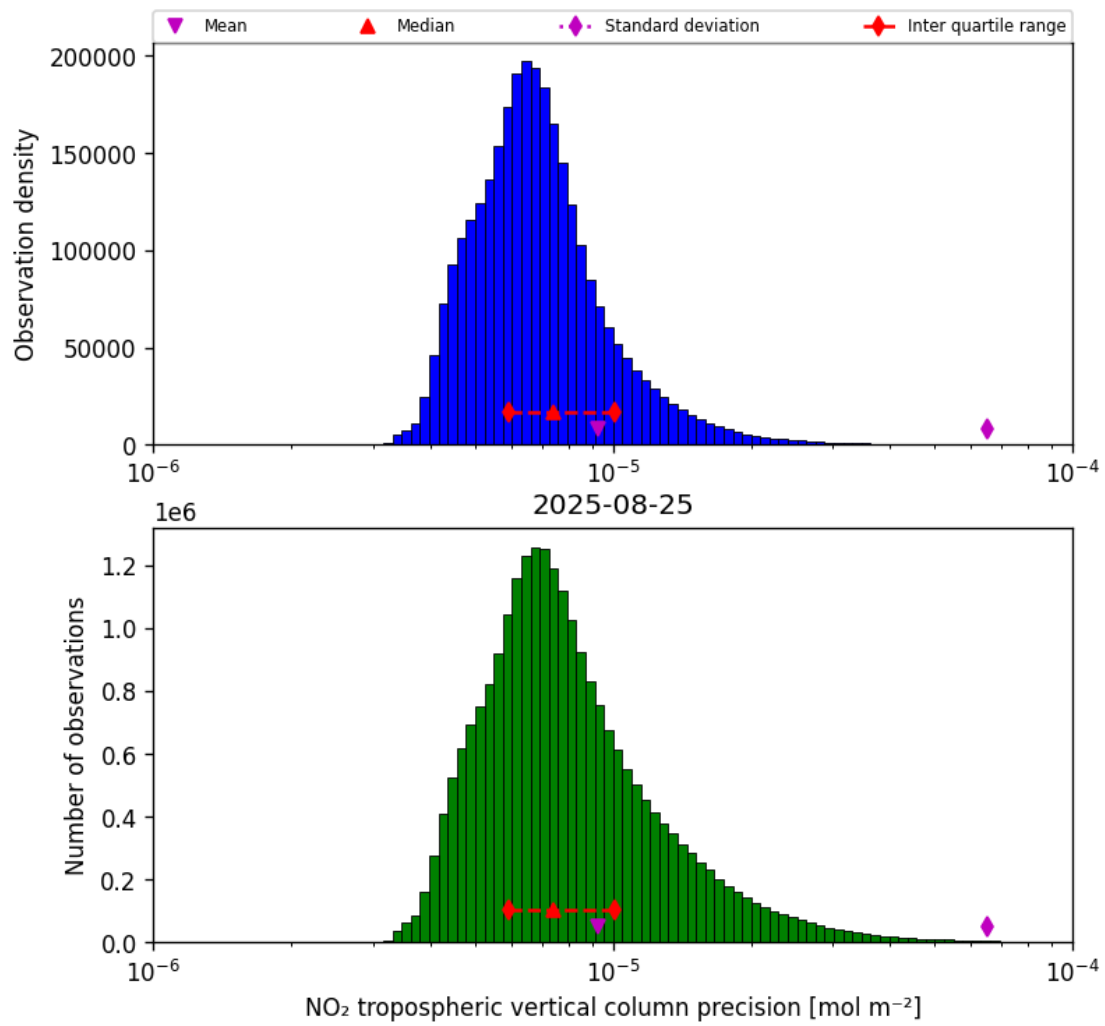
Figure 28: Histogram of “NO 2 tropospheric vertical column precision” for 2025-08-25 to 2025-08-26
