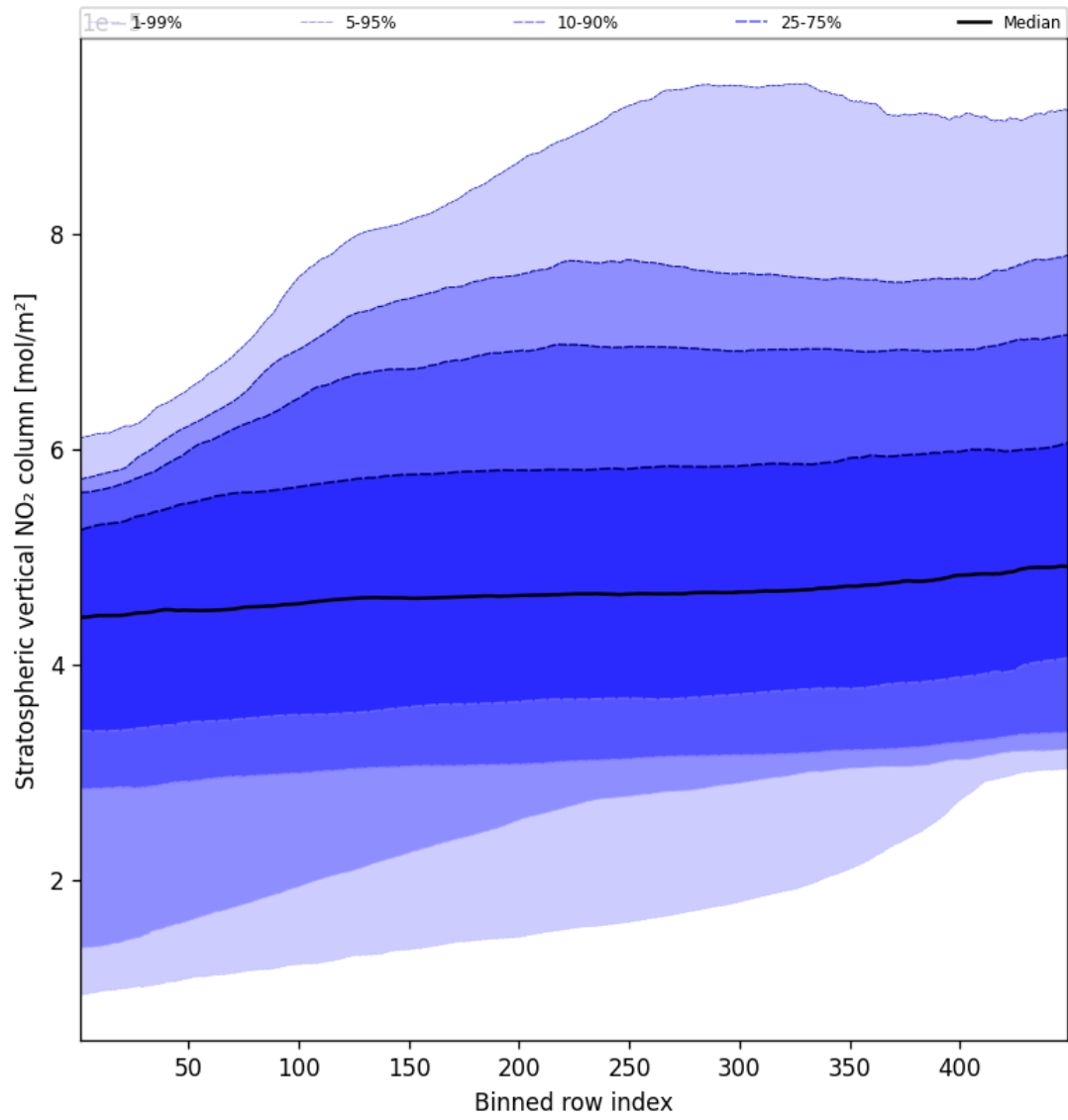
Figure 51: Along track statistics of “Stratospheric vertical NO 2 column” for 2025-08-25 to 2025-08-26
