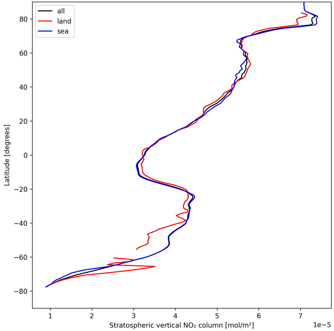
Figure 17: Zonal average of “Stratospheric vertical NO 2 column” for 2025-08-25 to 2025-08-26.
