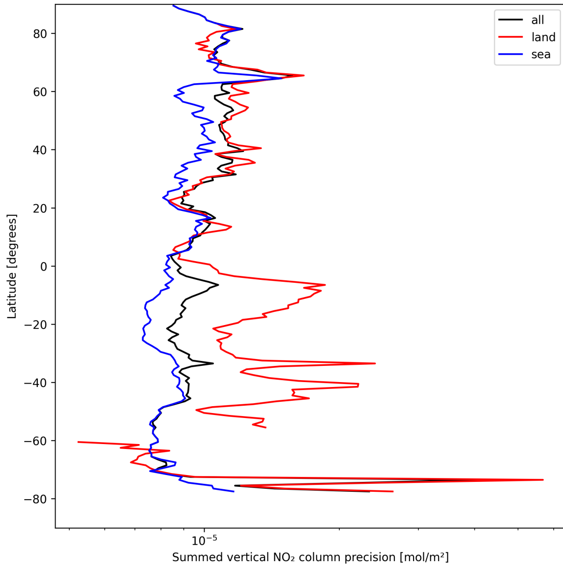
Figure 22: Zonal average of “Summed vertical NO 2 column precision” for 2025-08-25 to 2025-08-26.
