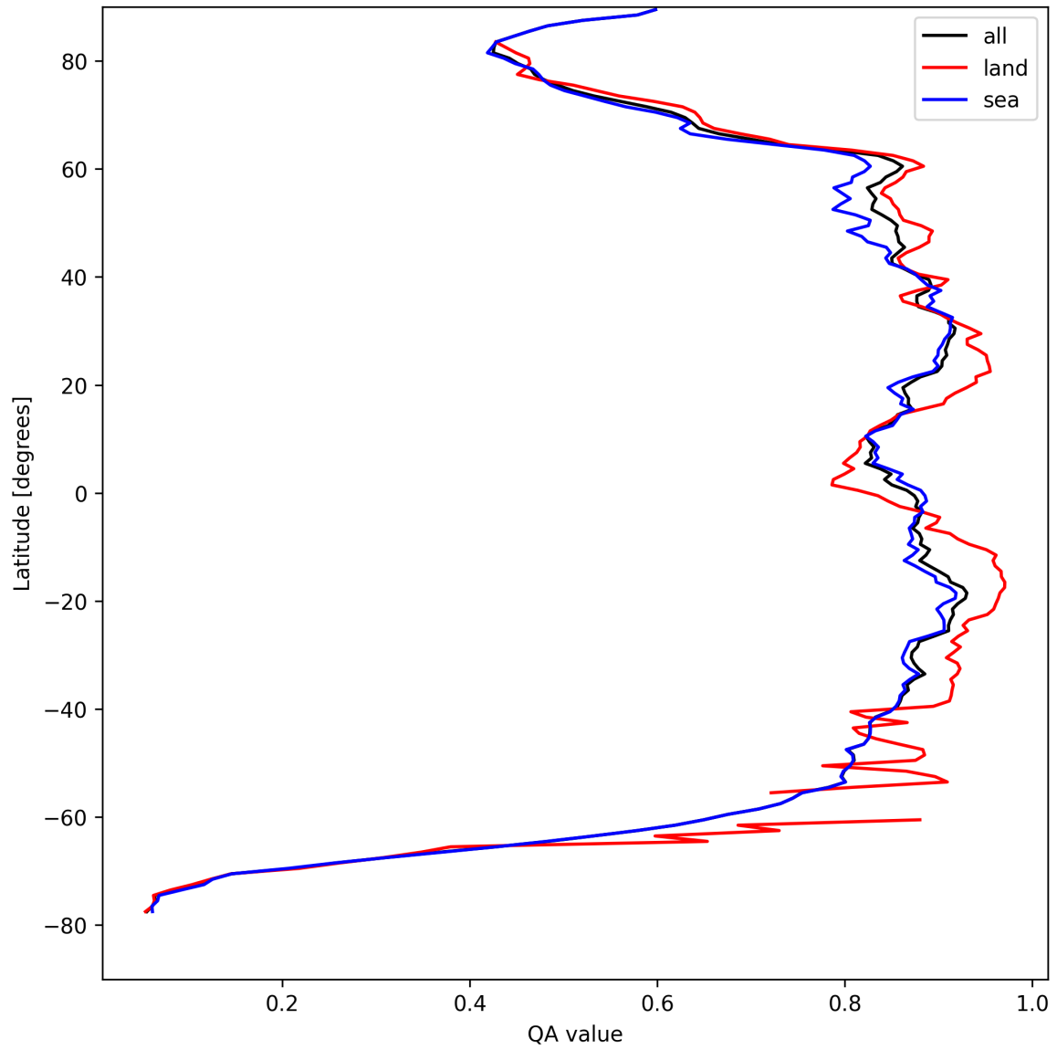
Figure 9: Zonal average of “QA value” for 2025-08-25 to 2025-08-26.
