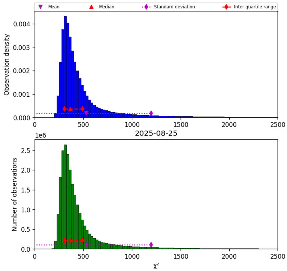
Figure 40: Histogram of “ \chi^2 ” for 2025-08-25 to 2025-08-26
