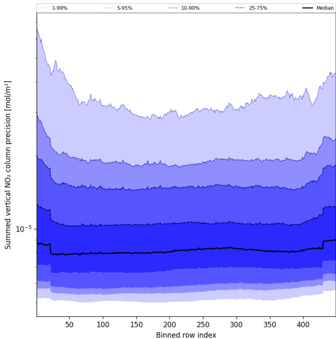
Figure 56: Along track statistics of “Summed vertical NO 2 column precision” for 2025-08-25 to 2025-08-26
