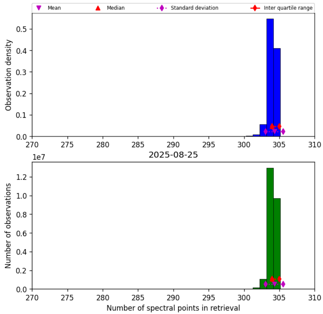
Figure 31: Histogram of “Number of spectral points in retrieval” for 2025-08-25 to 2025-08-26
