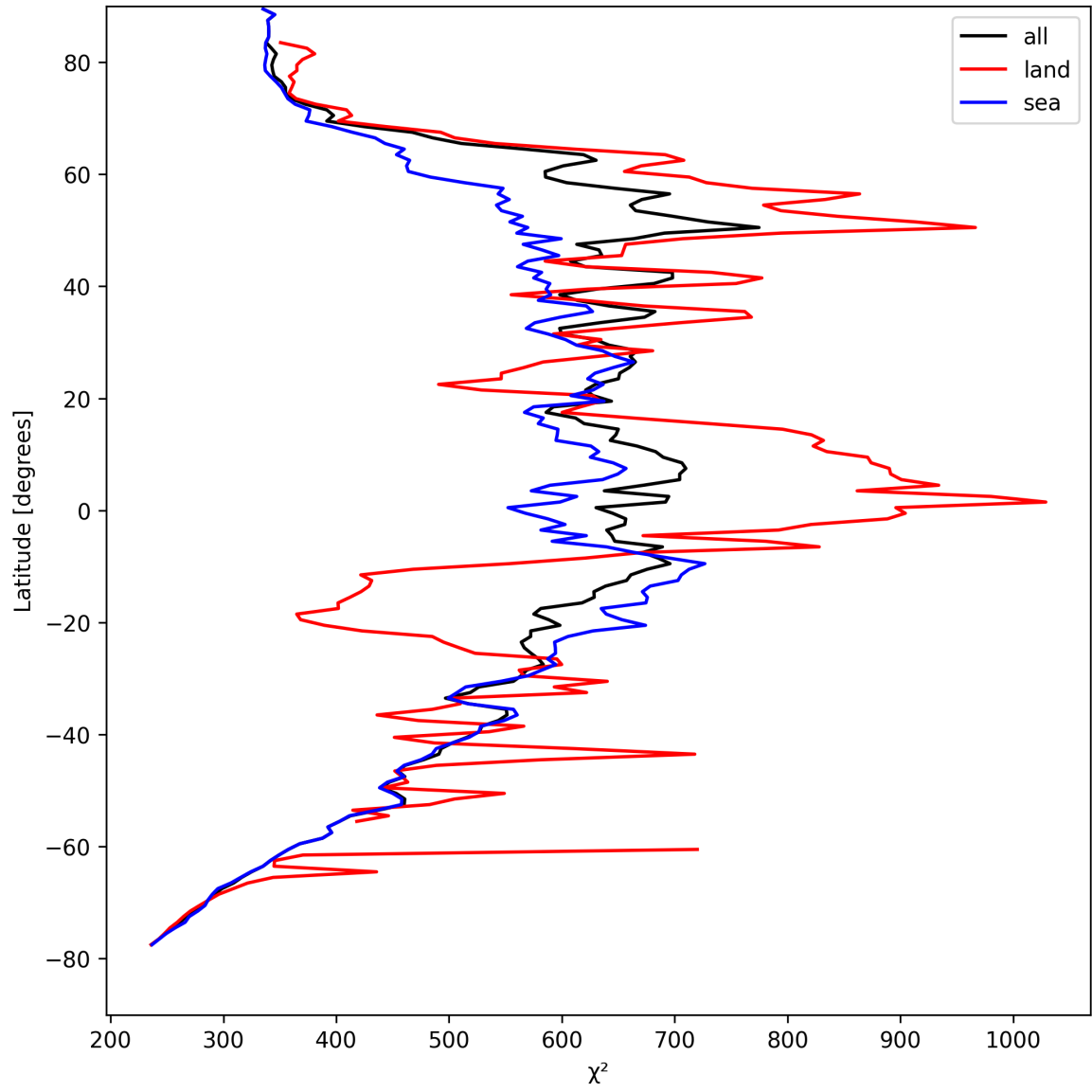
Figure 23: Zonal average of “ \chi^2 ” for 2025-08-25 to 2025-08-26.
