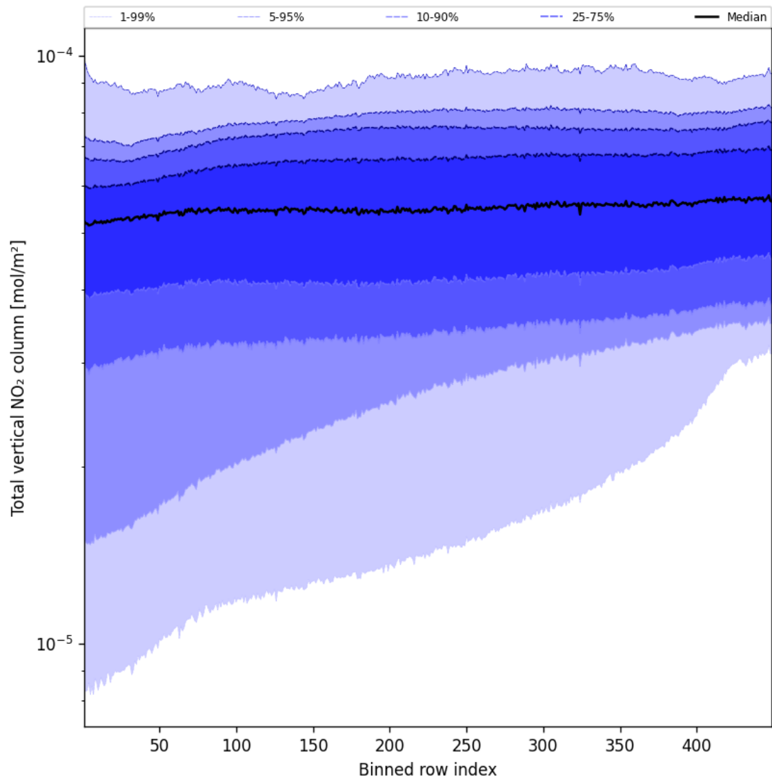
Figure 53: Along track statistics of “Total vertical NO 2 column” for 2025-08-25 to 2025-08-26
