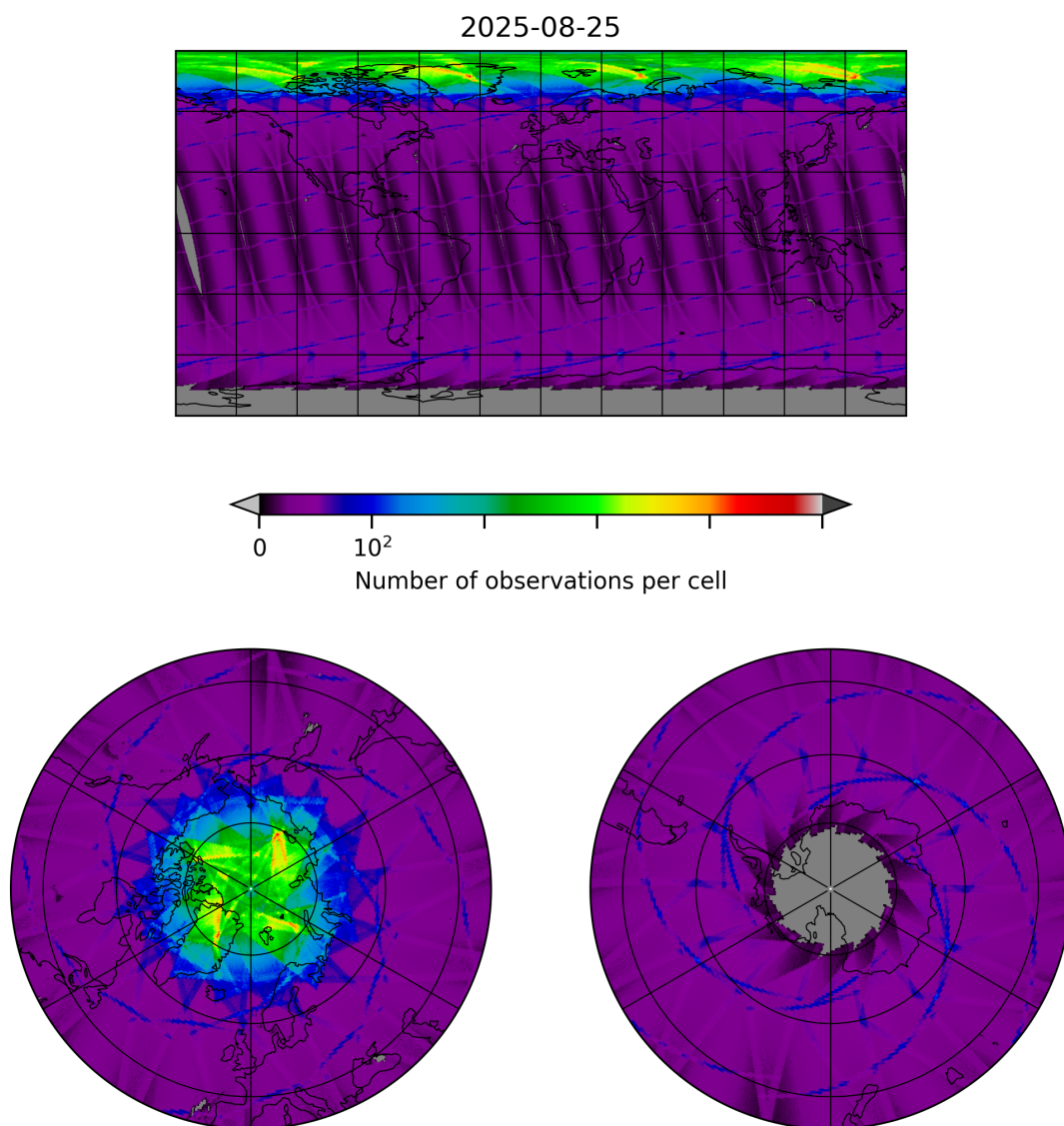
Figure 8: Map of the number of observations for 2025-08-25 to 2025-08-26
