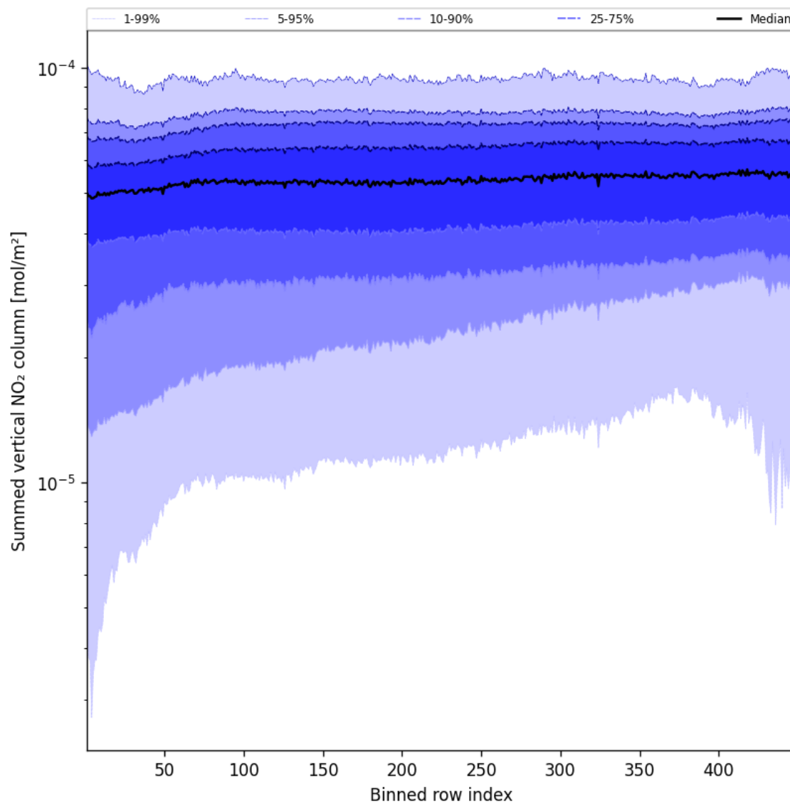
Figure 55: Along track statistics of “Summed vertical NO 2 column” for 2025-08-25 to 2025-08-26
