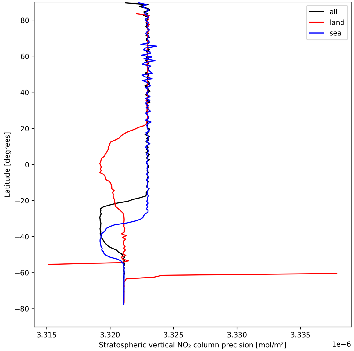
Figure 18: Zonal average of “Stratospheric vertical NO 2 column precision” for 2025-08-25 to 2025-08-26.
