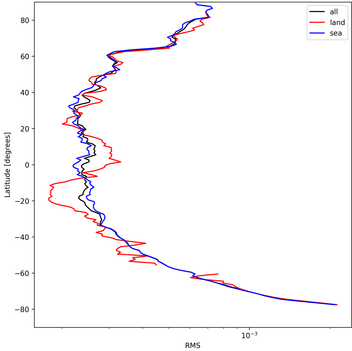
Figure 24: Zonal average of “RMS” for 2025-08-25 to 2025-08-26.
