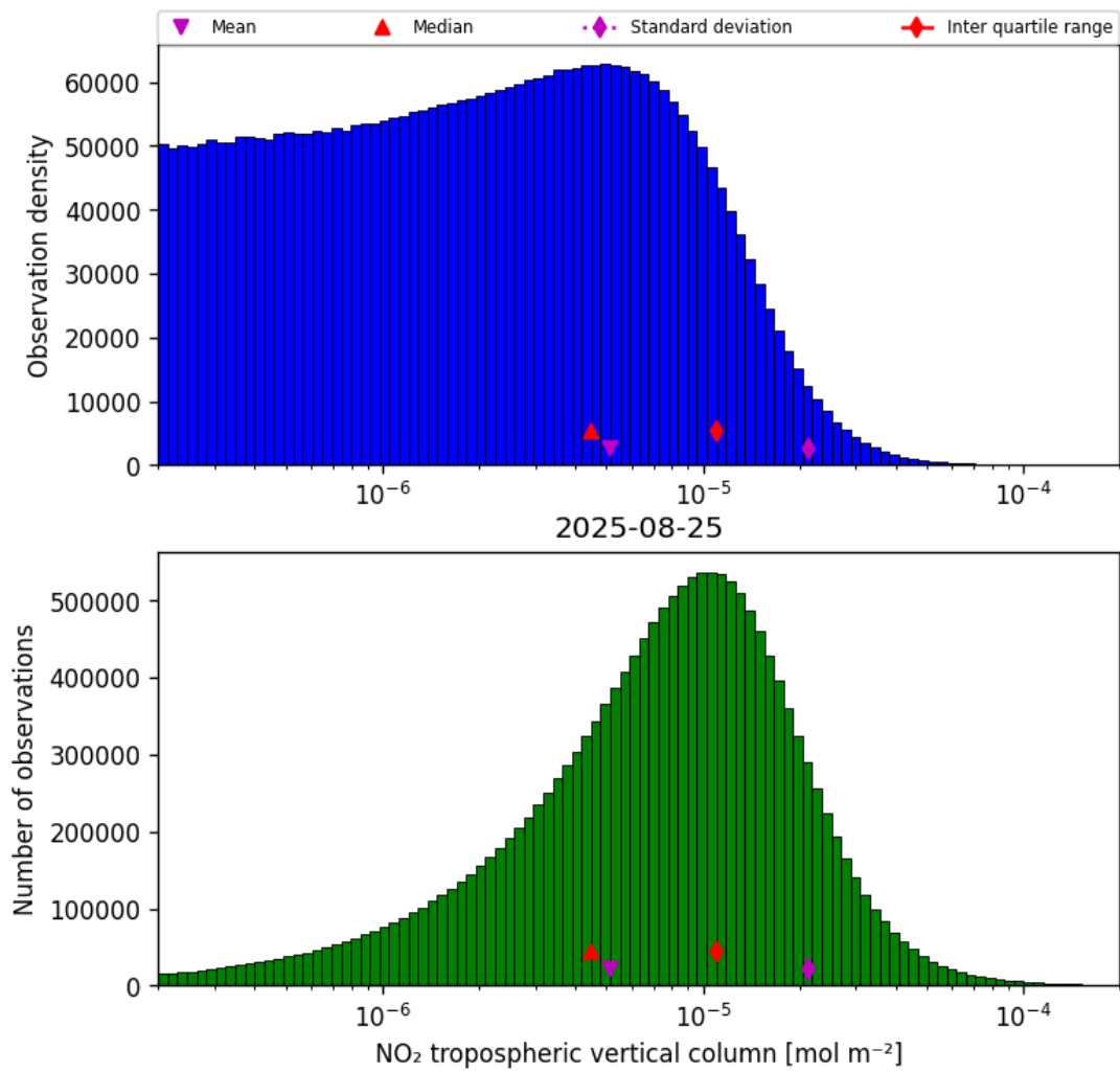
Figure 27: Histogram of “NO 2 tropospheric vertical column” for 2025-08-25 to 2025-08-26
