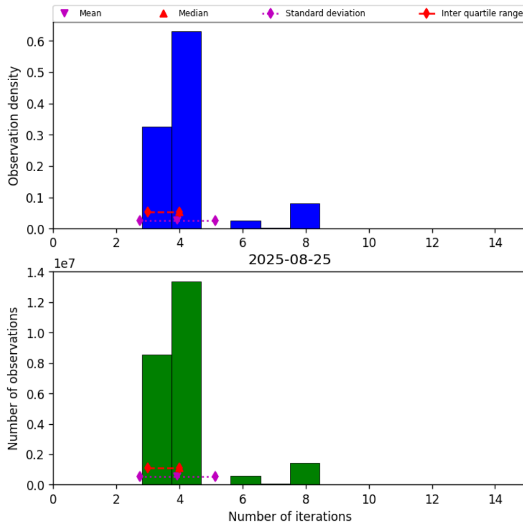
Figure 32: Histogram of “Number of iterations” for 2025-08-25 to 2025-08-26
