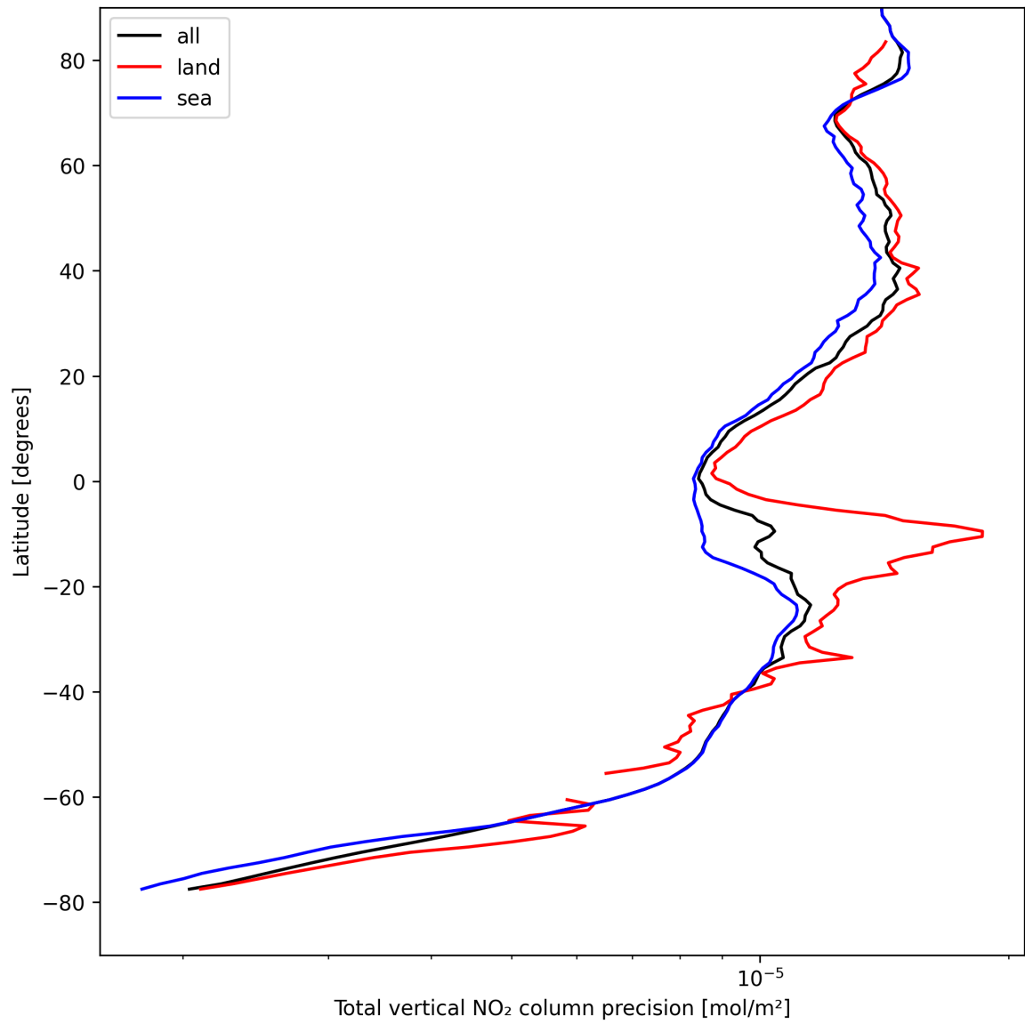
Figure 20: Zonal average of “Total vertical NO 2 column precision” for 2025-08-25 to 2025-08-26.
