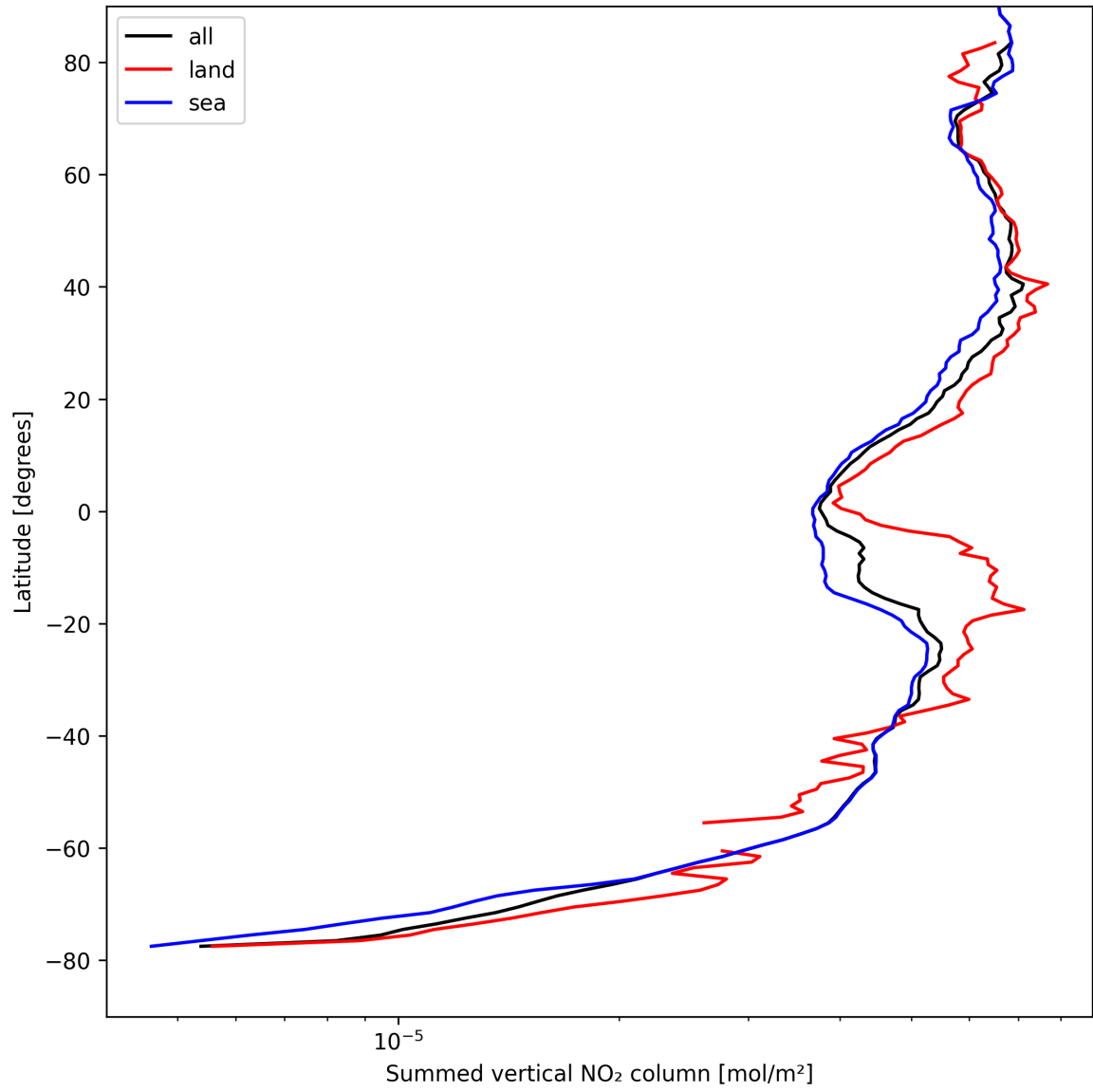
Figure 21: Zonal average of “Summed vertical NO 2 column” for 2025-08-25 to 2025-08-26.
