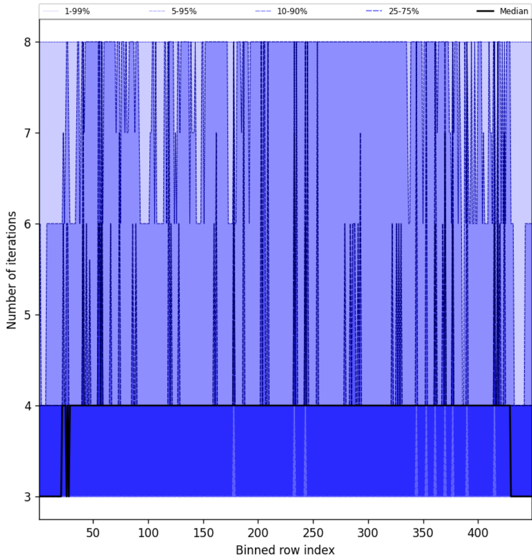
Figure 49: Along track statistics of “Number of iterations” for 2025-08-25 to 2025-08-26
