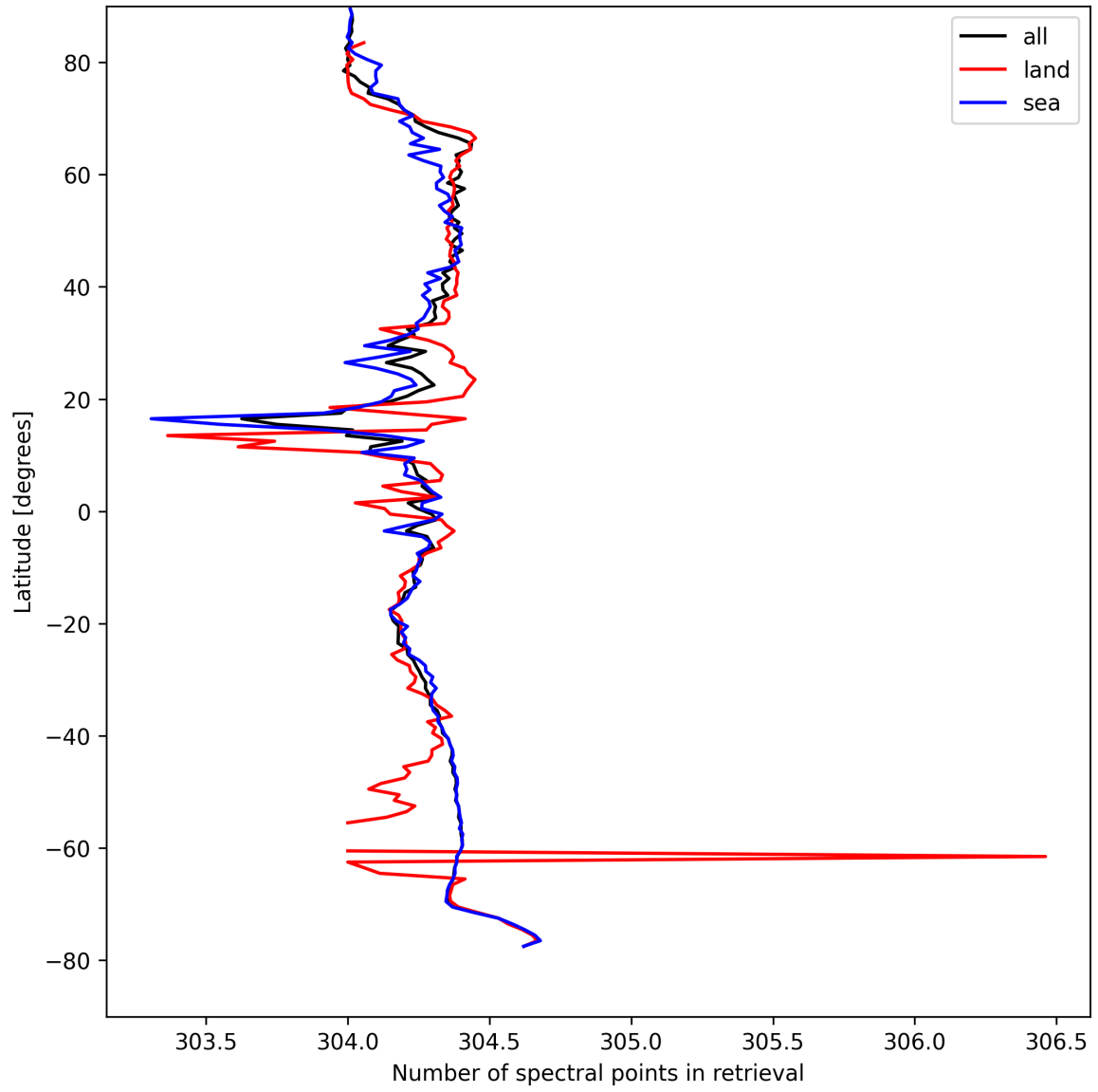
Figure 14: Zonal average of “Number of spectral points in retrieval” for 2025-08-25 to 2025-08-26.
