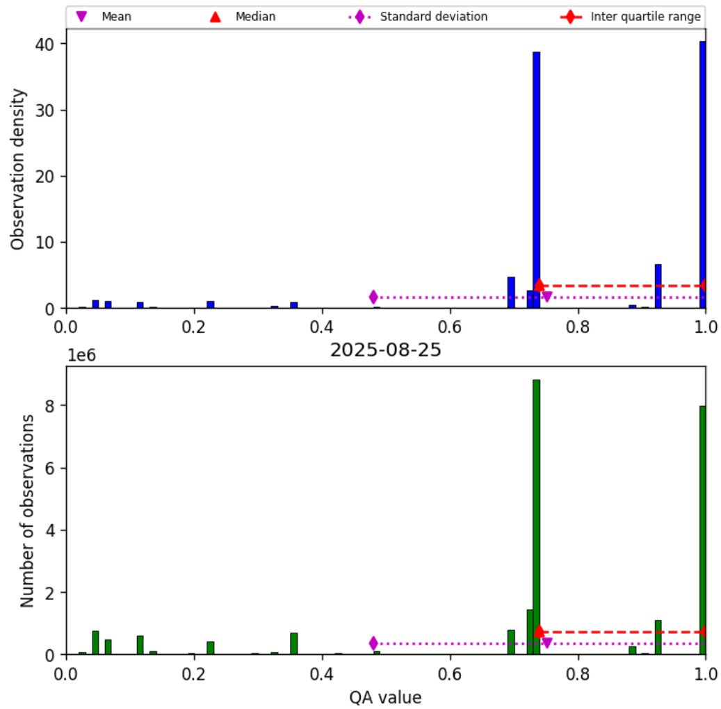
Figure 26: Histogram of “QA value” for 2025-08-25 to 2025-08-26
