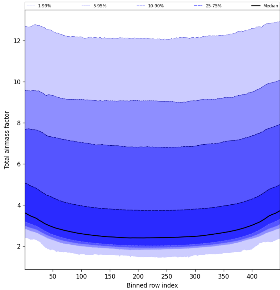
Figure 47: Along track statistics of “Total airmass factor” for 2025-08-25 to 2025-08-26
