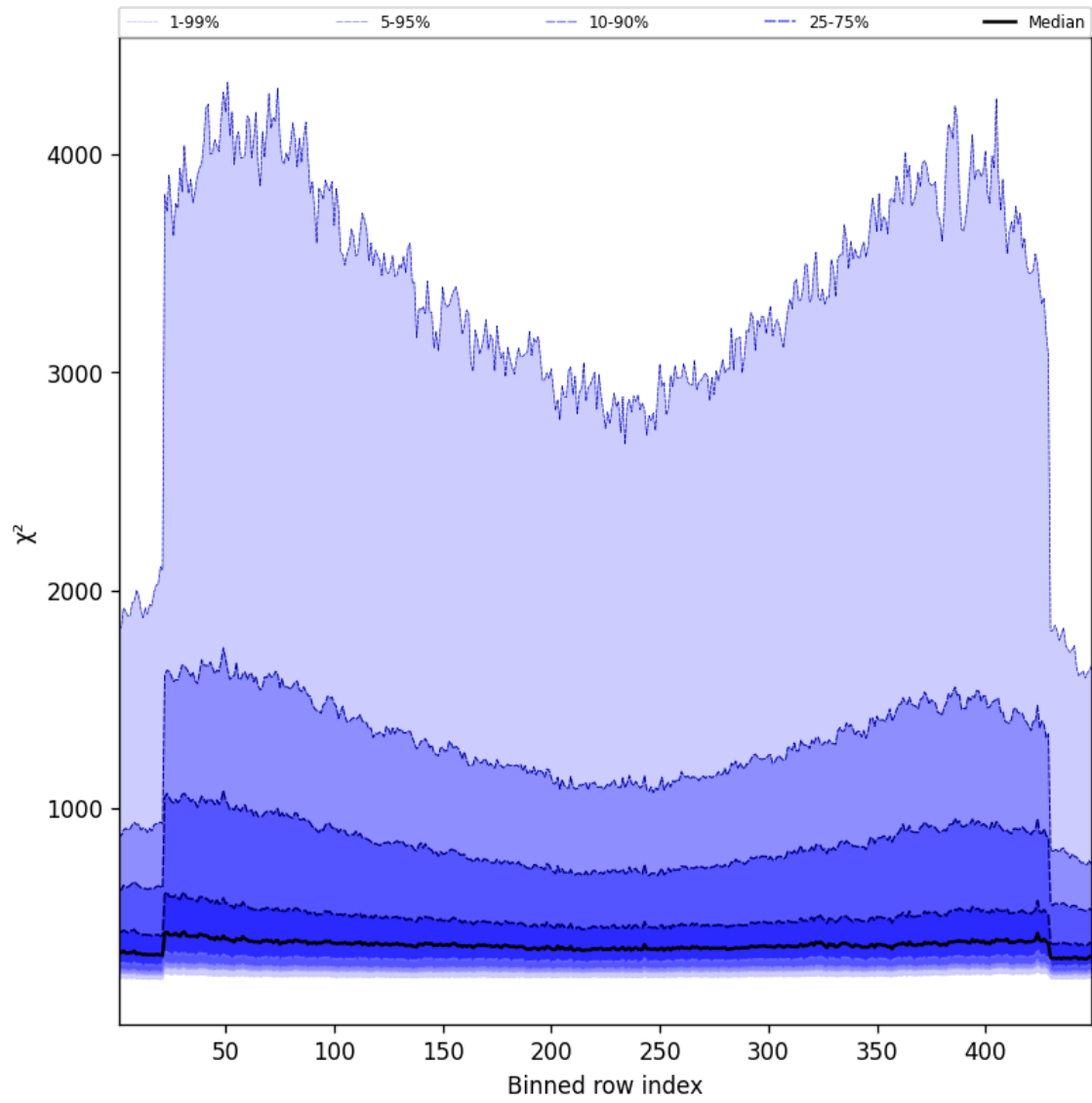
Figure 57: Along track statistics of “ \chi^2 ” for 2025-08-25 to 2025-08-26
