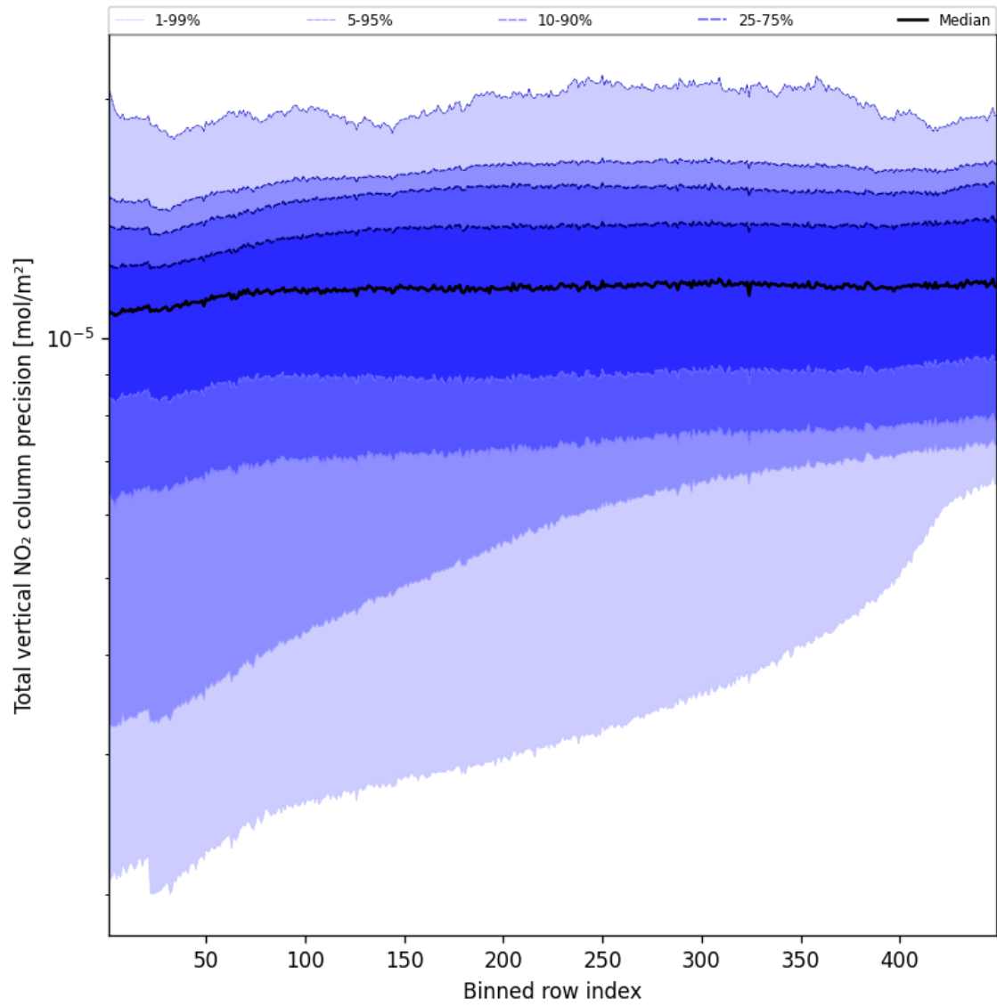
Figure 54: Along track statistics of “Total vertical NO 2 column precision” for 2025-08-25 to 2025-08-26
