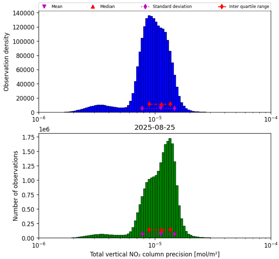
Figure 37: Histogram of “Total vertical NO 2 column precision” for 2025-08-25 to 2025-08-26
