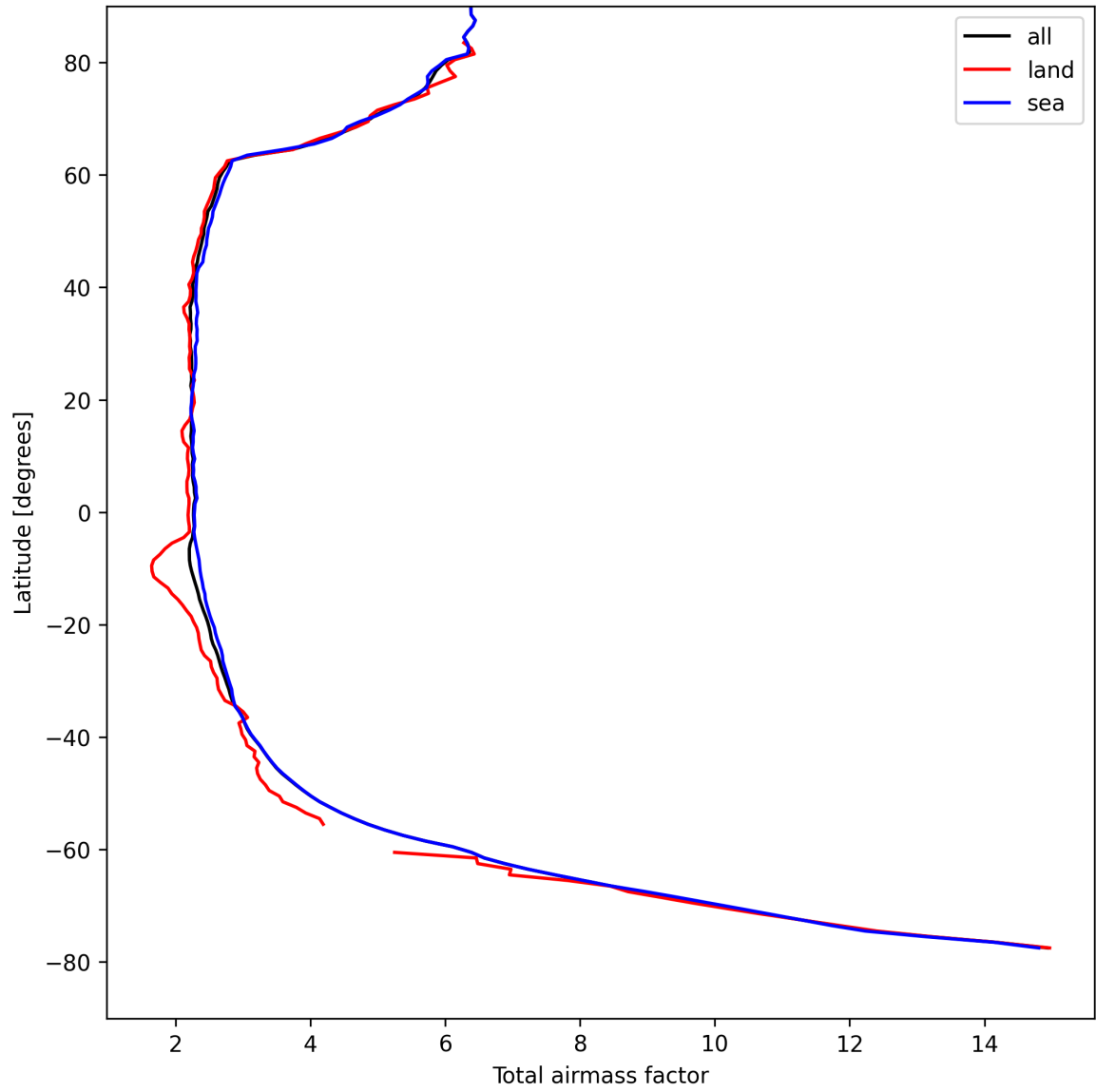
Figure 13: Zonal average of “Total airmass factor” for 2025-08-25 to 2025-08-26.
