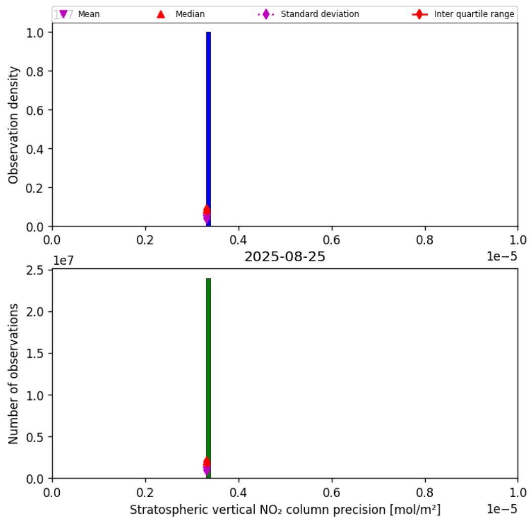
Figure 35: Histogram of “Stratospheric vertical NO 2 column precision” for 2025-08-25 to 2025-08-26
