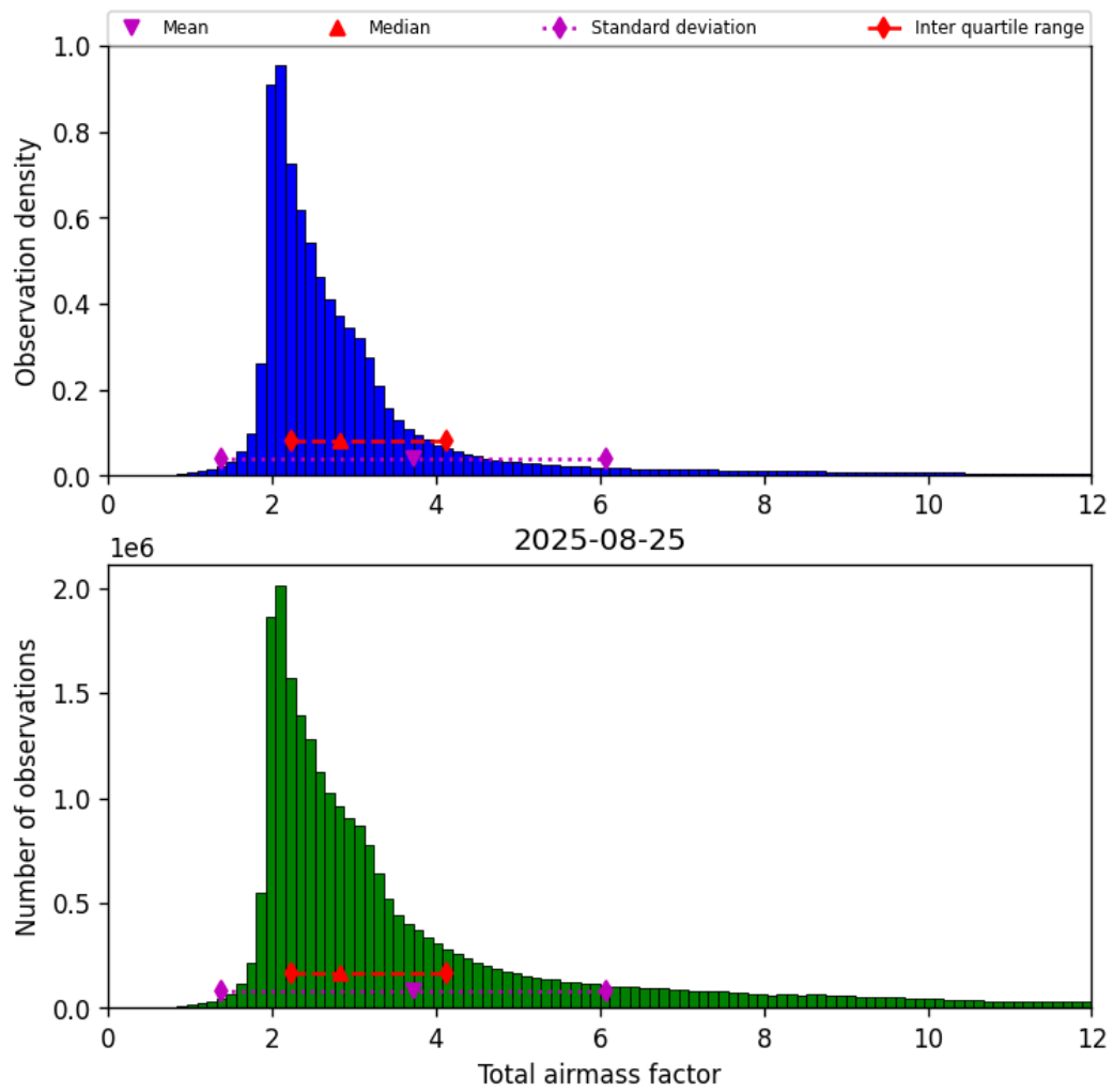
Figure 30: Histogram of “Total airmass factor” for 2025-08-25 to 2025-08-26
