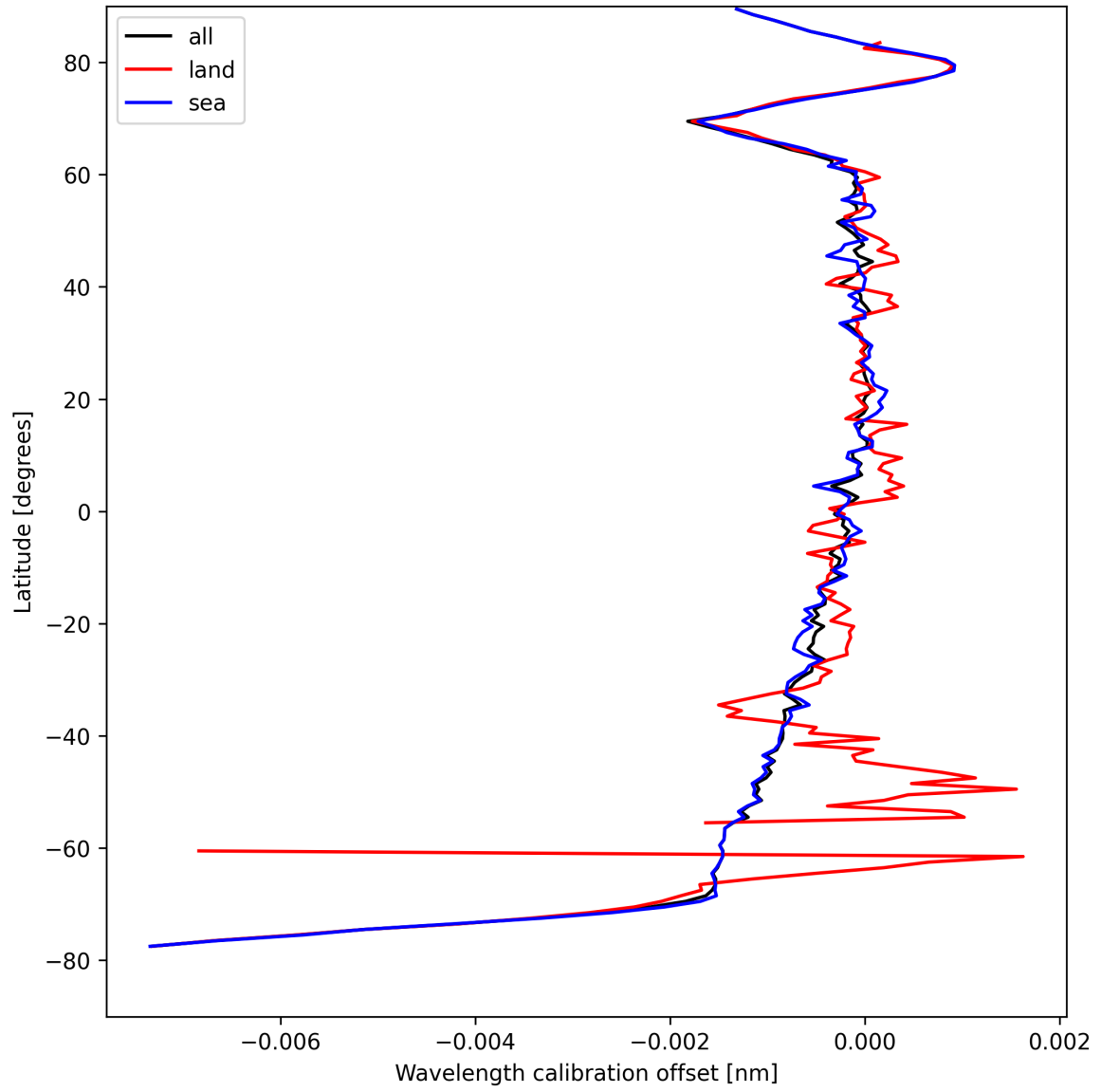
Figure 16: Zonal average of “Wavelength calibration offset” for 2025-08-25 to 2025-08-26.
