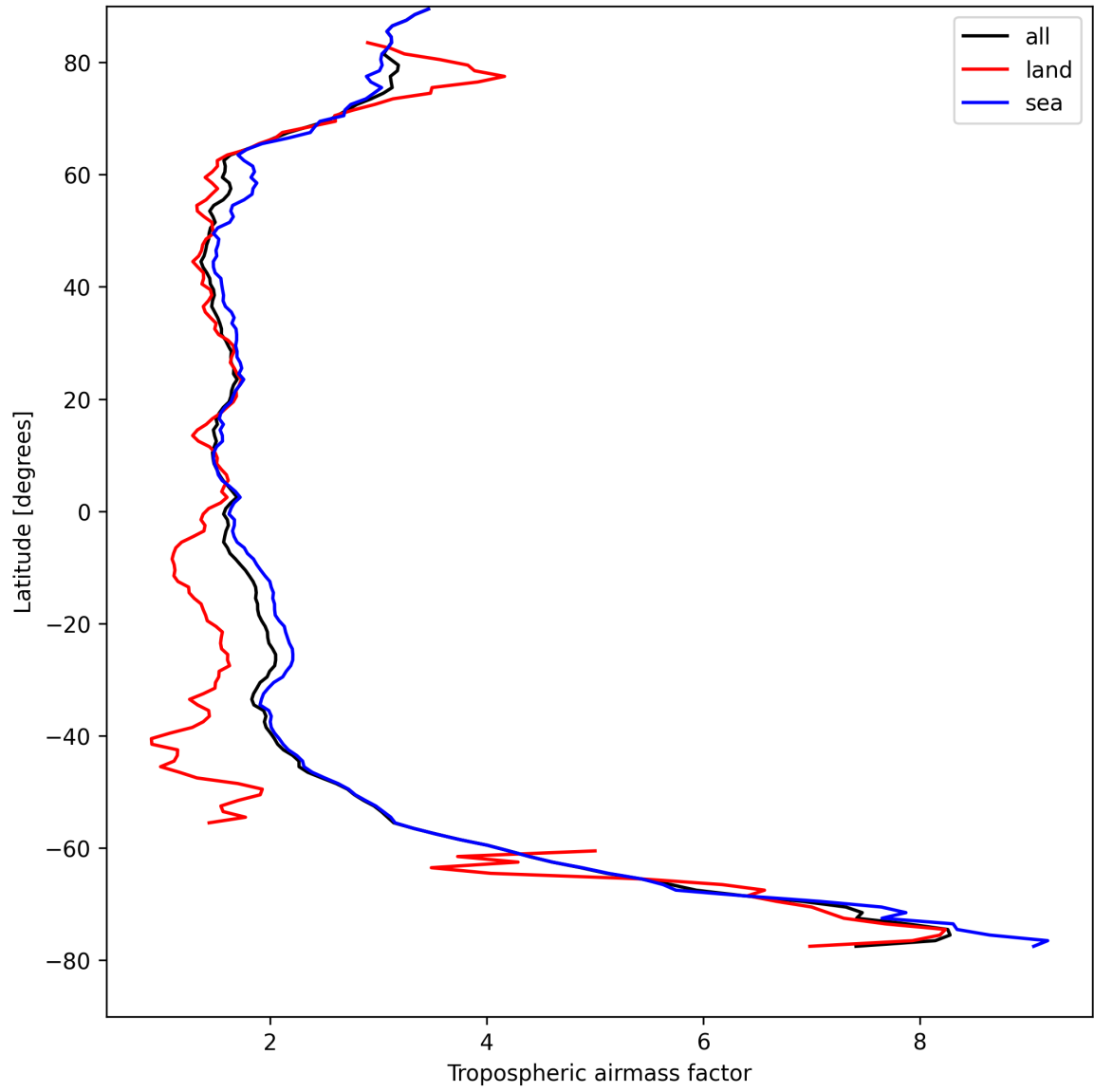
Figure 12: Zonal average of “Tropospheric airmass factor” for 2025-08-25 to 2025-08-26.
