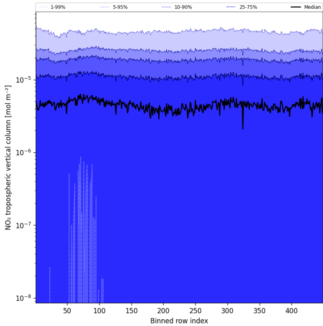
Figure 44: Along track statistics of “NO 2 tropospheric vertical column” for 2025-08-25 to 2025-08-26
