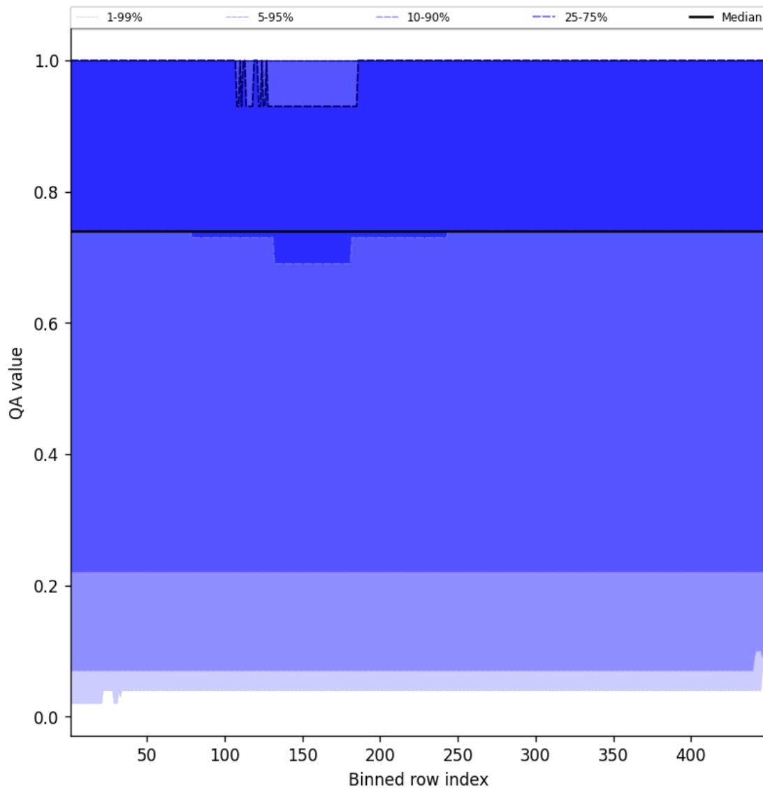
Figure 43: Along track statistics of “QA value” for 2025-08-25 to 2025-08-26
