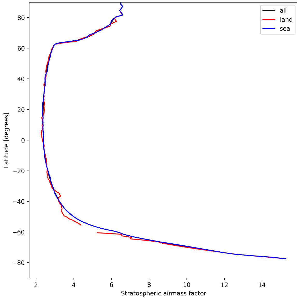
Figure 25: Zonal average of “Stratospheric airmass factor” for 2025-08-25 to 2025-08-26.
