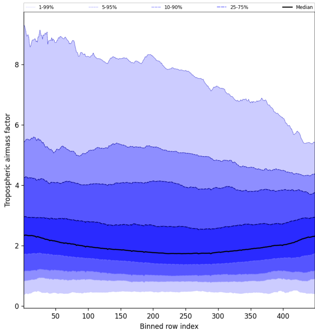
Figure 46: Along track statistics of “Tropospheric airmass factor” for 2025-08-25 to 2025-08-26
