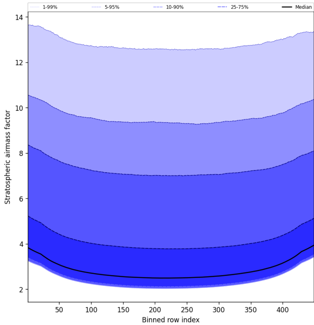
Figure 59: Along track statistics of “Stratospheric airmass factor” for 2025-08-25 to 2025-08-26
