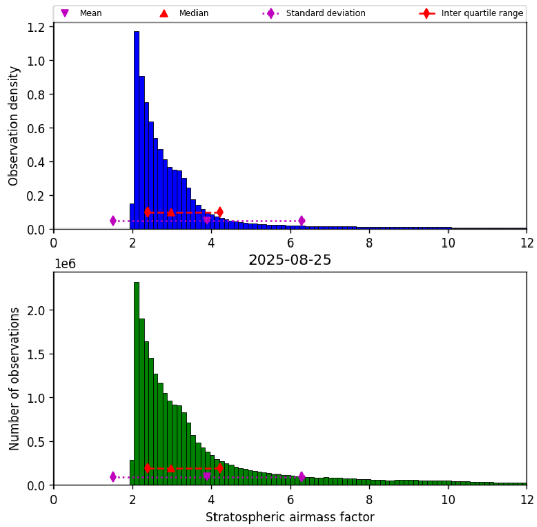
Figure 42: Histogram of “Stratospheric airmass factor” for 2025-08-25 to 2025-08-26
