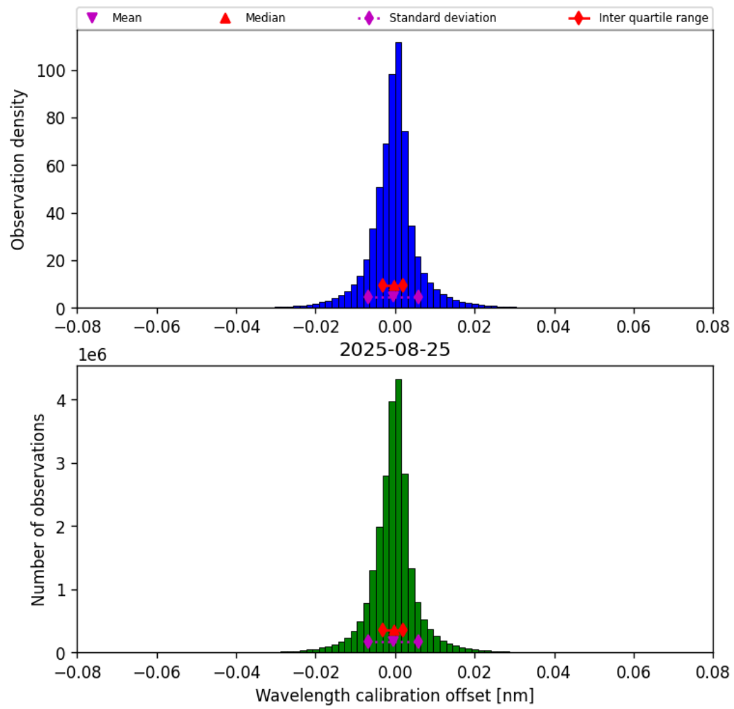
Figure 33: Histogram of “Wavelength calibration offset” for 2025-08-25 to 2025-08-26
