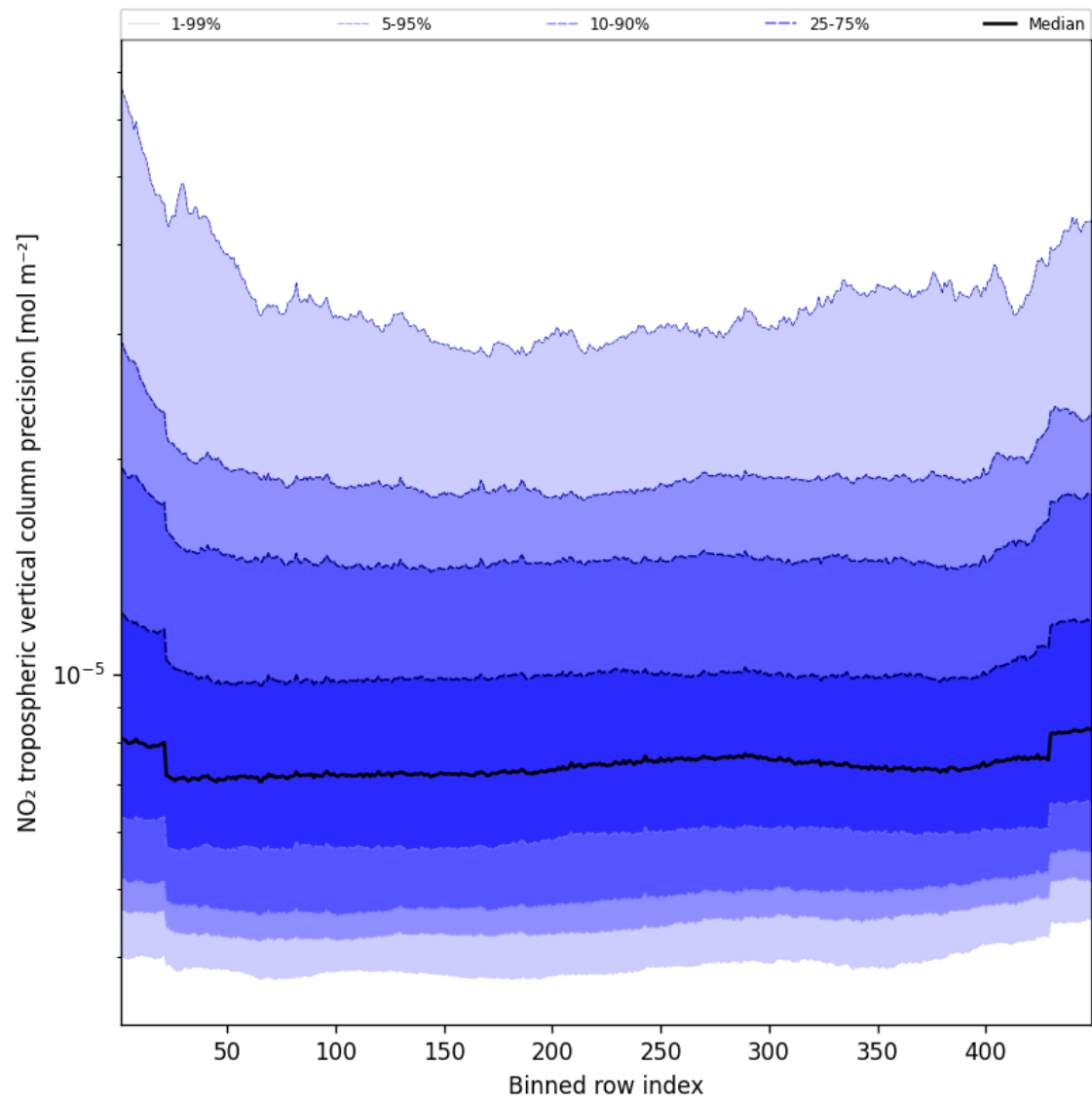
Figure 45: Along track statistics of “NO 2 tropospheric vertical column precision” for 2025-08-25 to 2025-08-26
