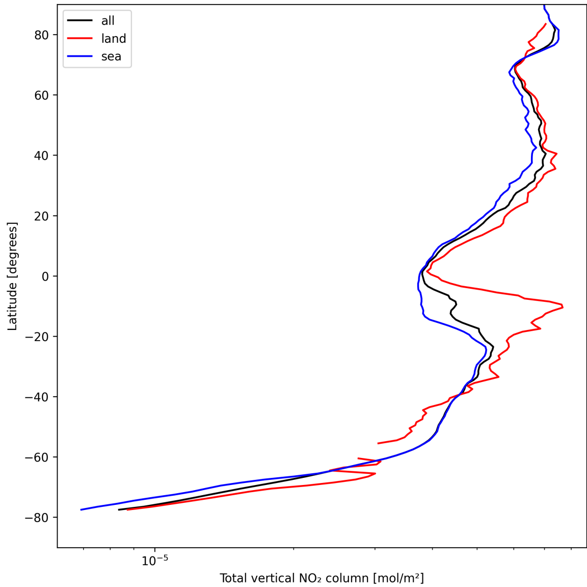
Figure 19: Zonal average of “Total vertical NO 2 column” for 2025-08-25 to 2025-08-26.
