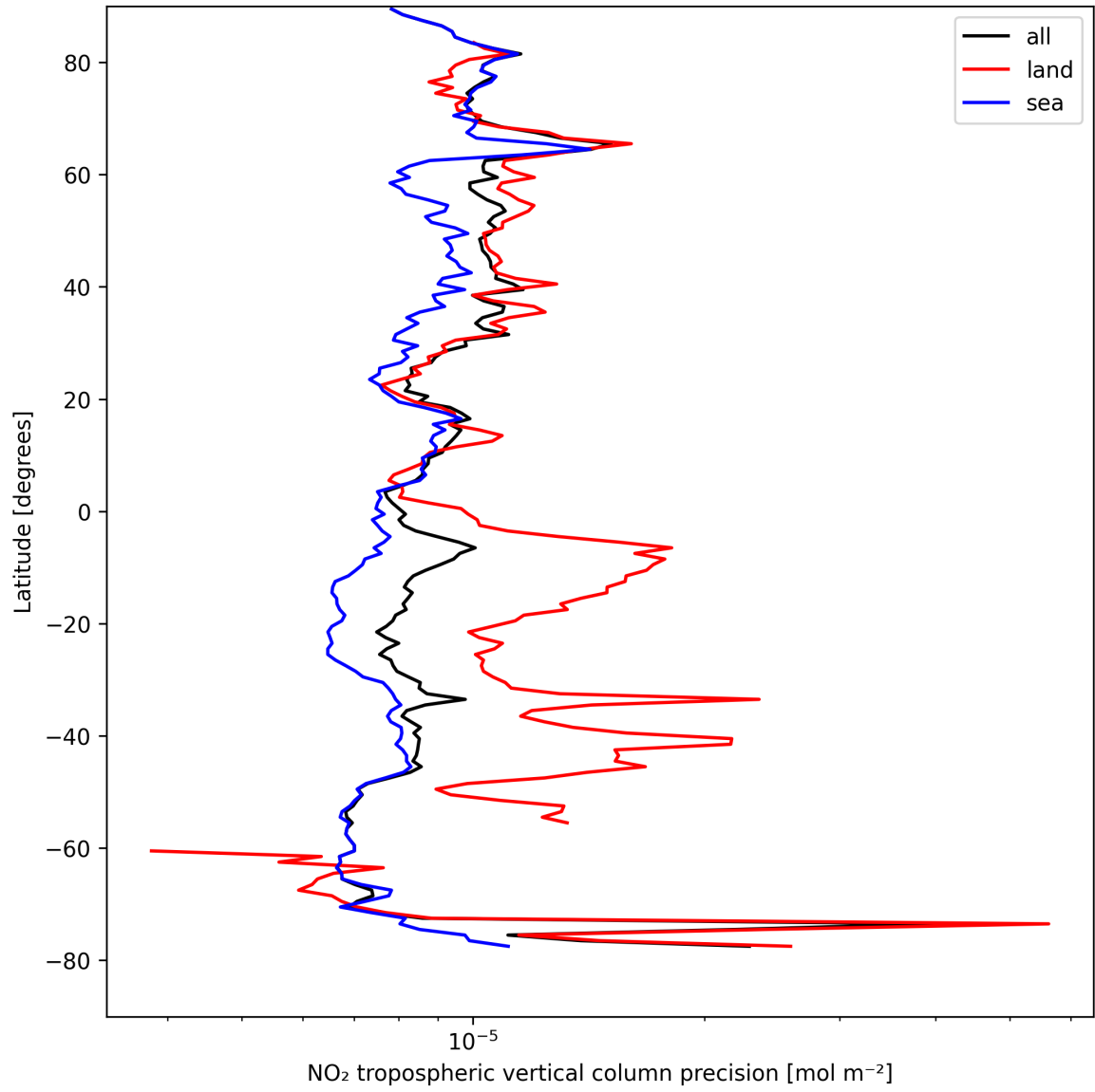
Figure 11: Zonal average of “NO 2 tropospheric vertical column precision” for 2025-08-25 to 2025-08-26.
