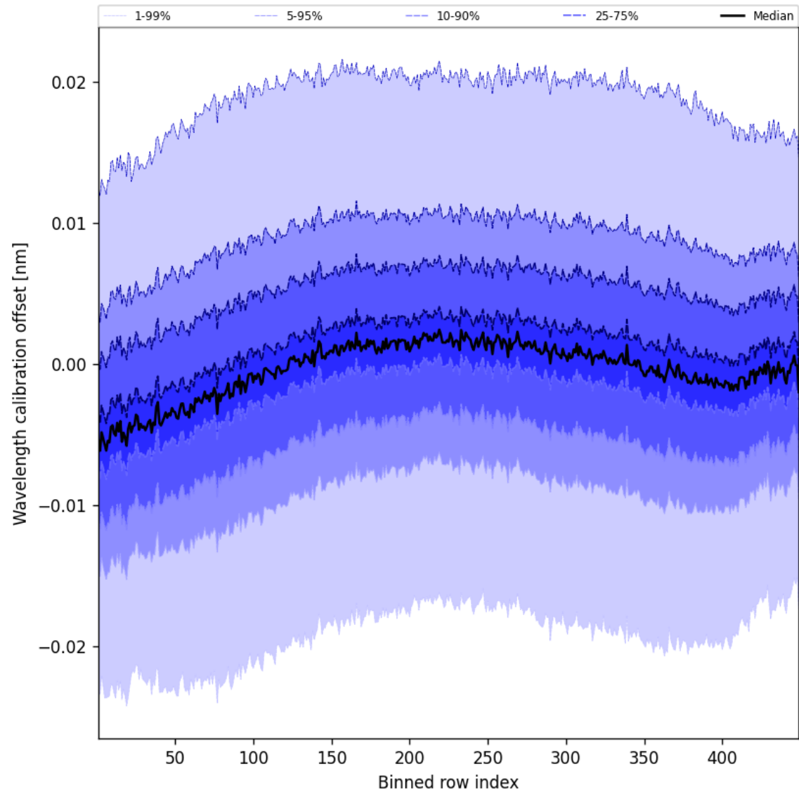
Figure 50: Along track statistics of “Wavelength calibration offset” for 2025-08-25 to 2025-08-26
