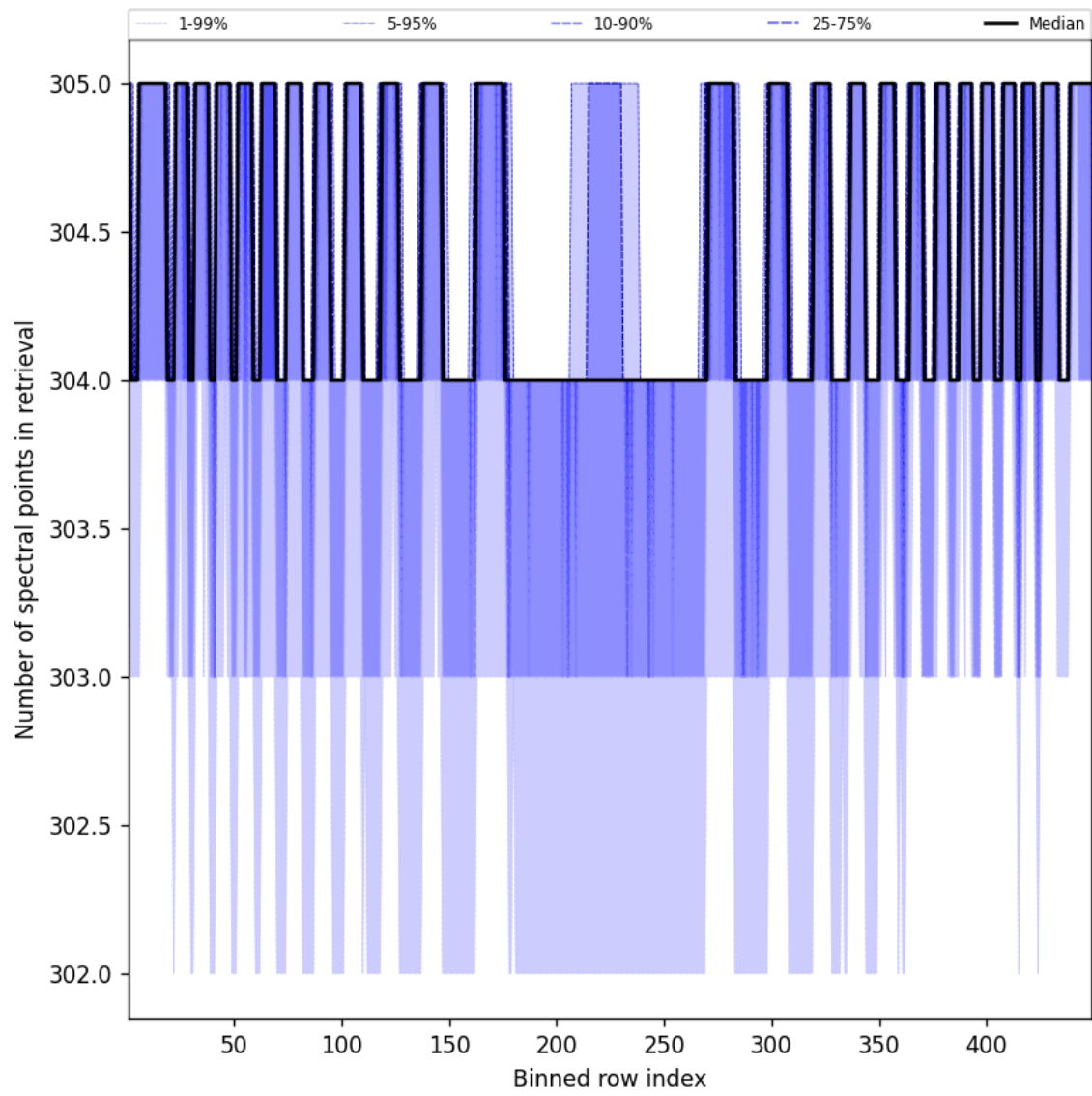
Figure 48: Along track statistics of “Number of spectral points in retrieval” for 2025-08-25 to 2025-08-26
