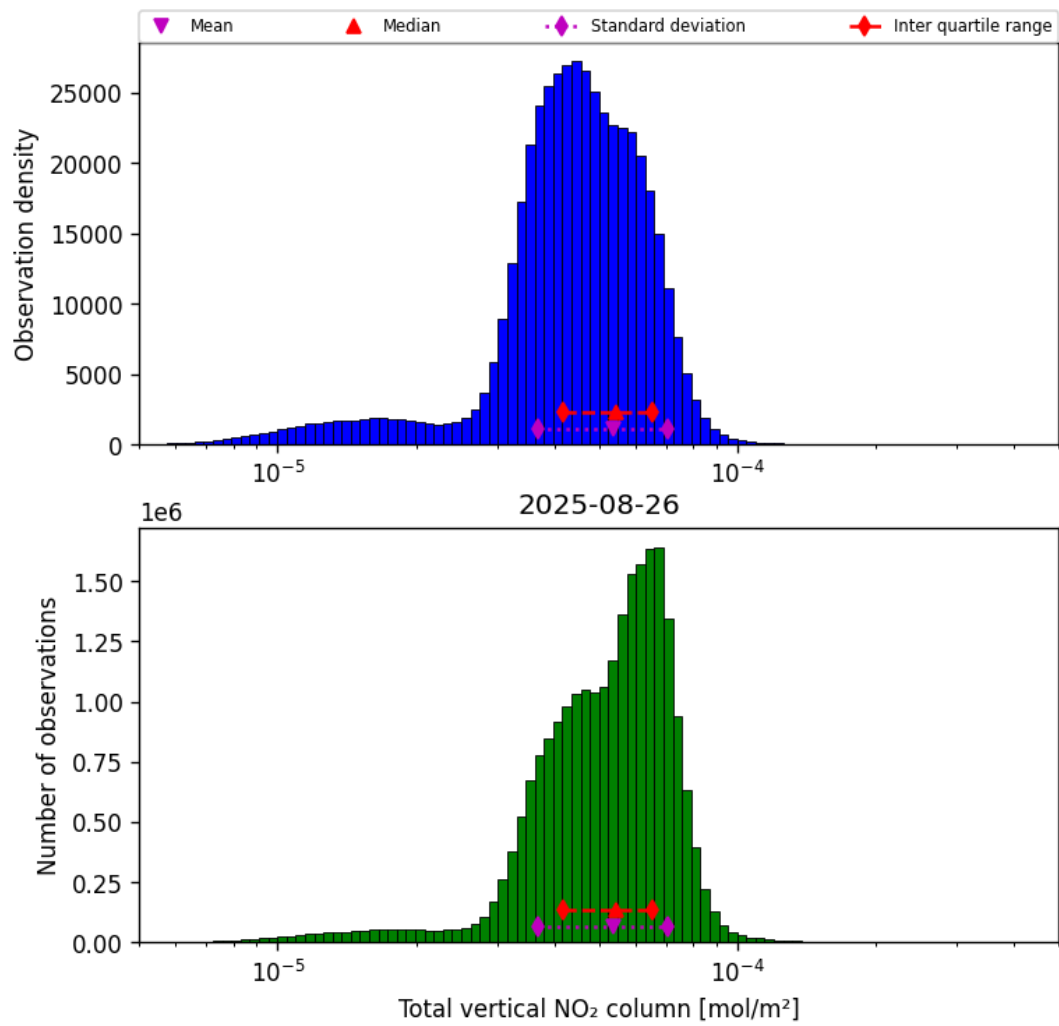
Figure 36: Histogram of “Total vertical NO 2 column” for 2025-08-26 to 2025-08-27
