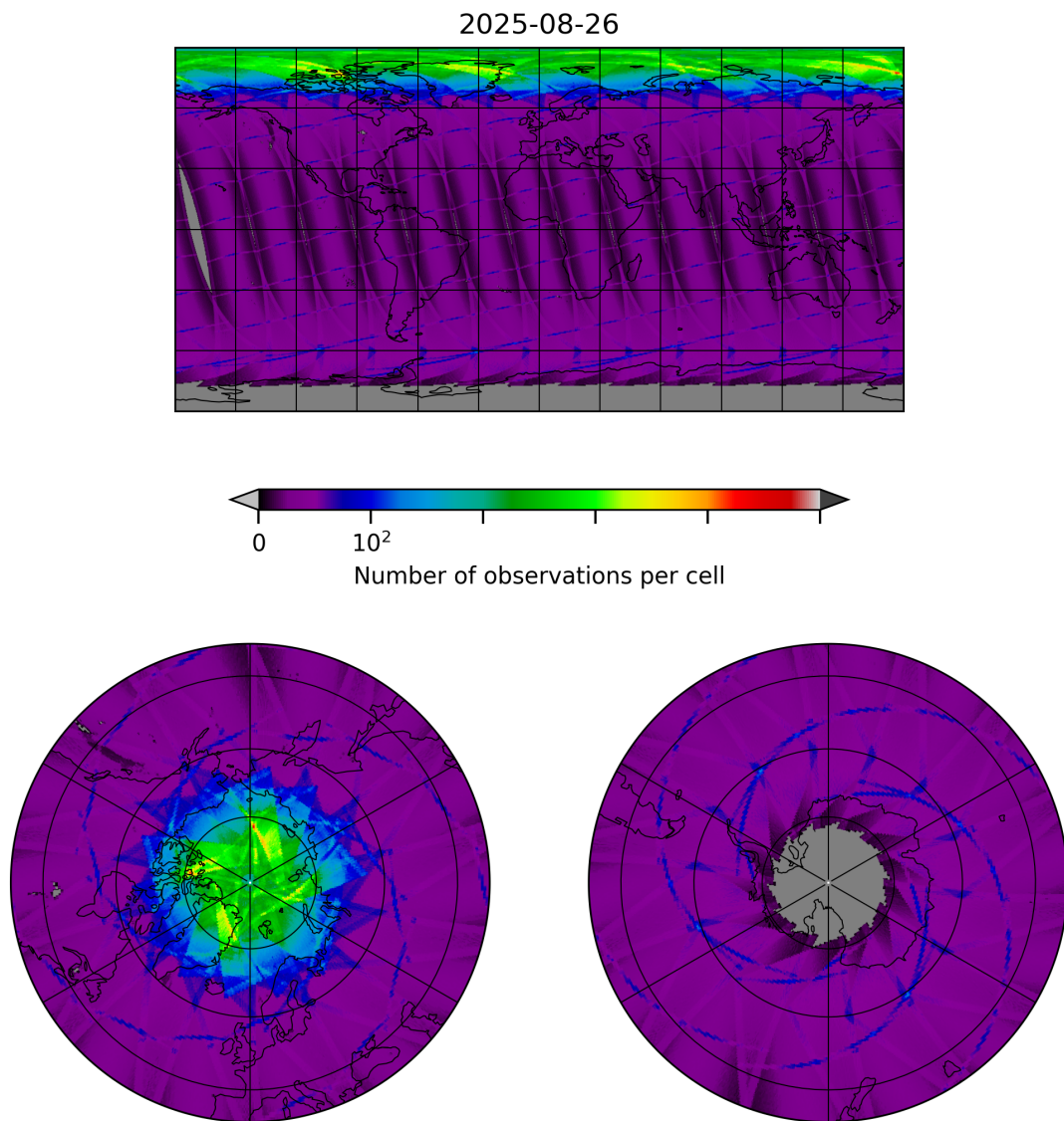
Figure 8: Map of the number of observations for 2025-08-26 to 2025-08-27
