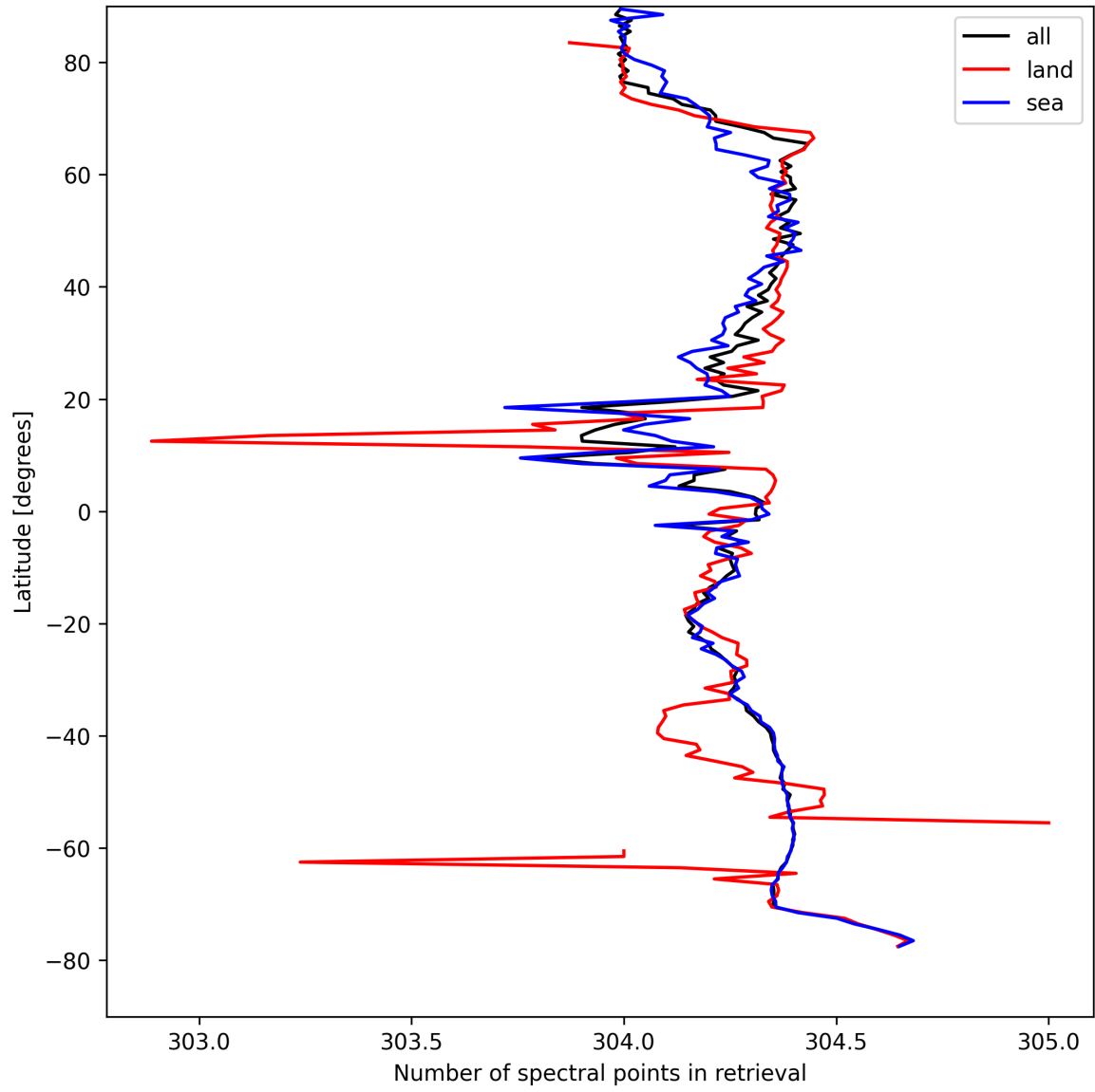
Figure 14: Zonal average of “Number of spectral points in retrieval” for 2025-08-26 to 2025-08-27.
