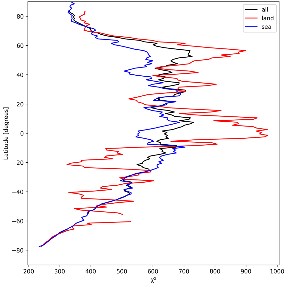
Figure 23: Zonal average of “ \chi^2 ” for 2025-08-26 to 2025-08-27.
