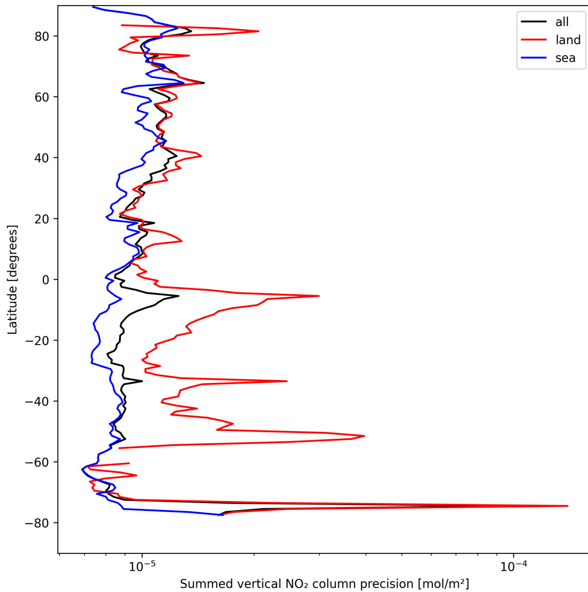
Figure 22: Zonal average of “Summed vertical NO 2 column precision” for 2025-08-26 to 2025-08-27.
