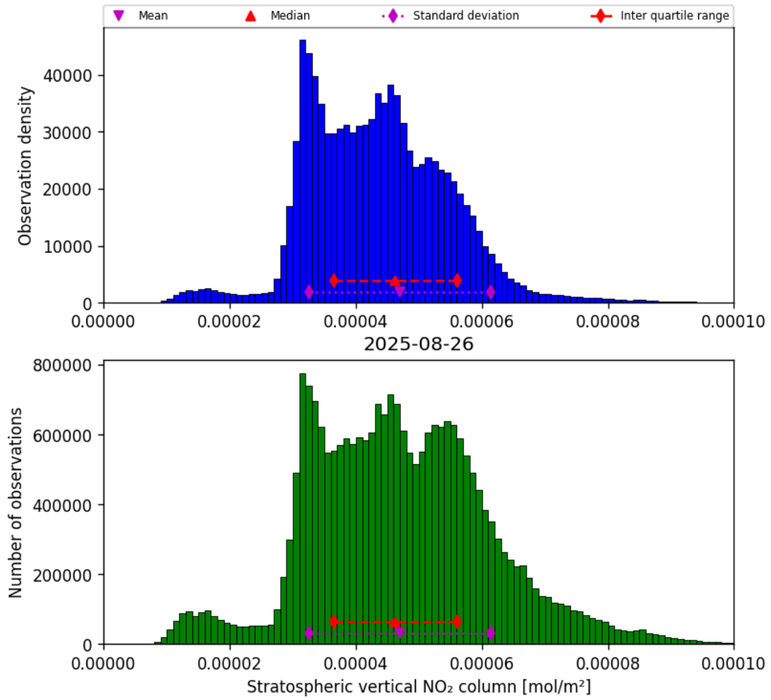
Figure 34: Histogram of “Stratospheric vertical NO 2 column” for 2025-08-26 to 2025-08-27
