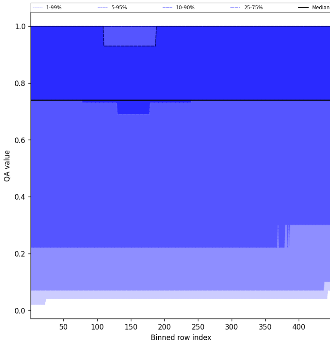
Figure 43: Along track statistics of “QA value” for 2025-08-26 to 2025-08-27
