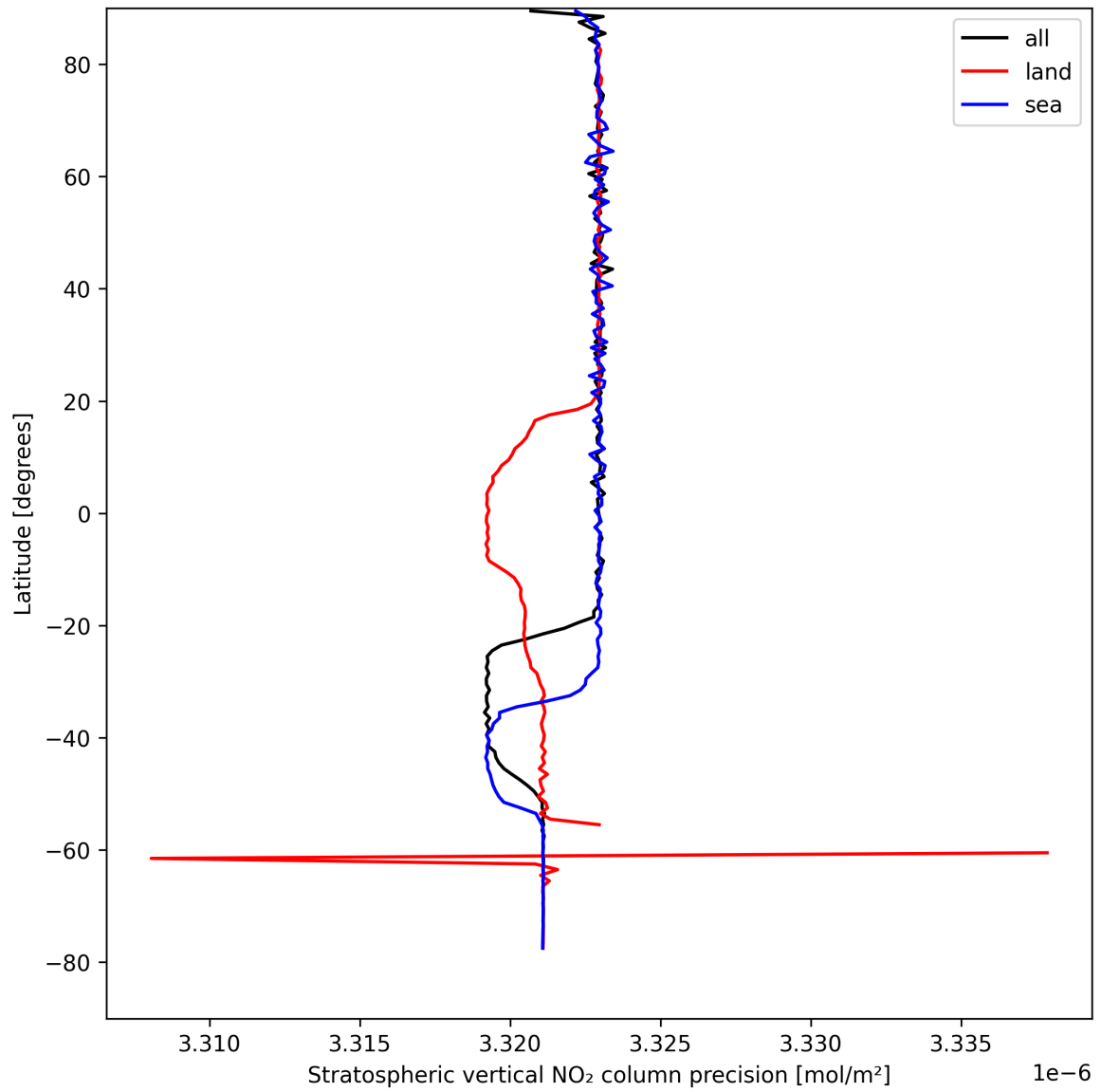
Figure 18: Zonal average of “Stratospheric vertical NO 2 column precision” for 2025-08-26 to 2025-08-27.
