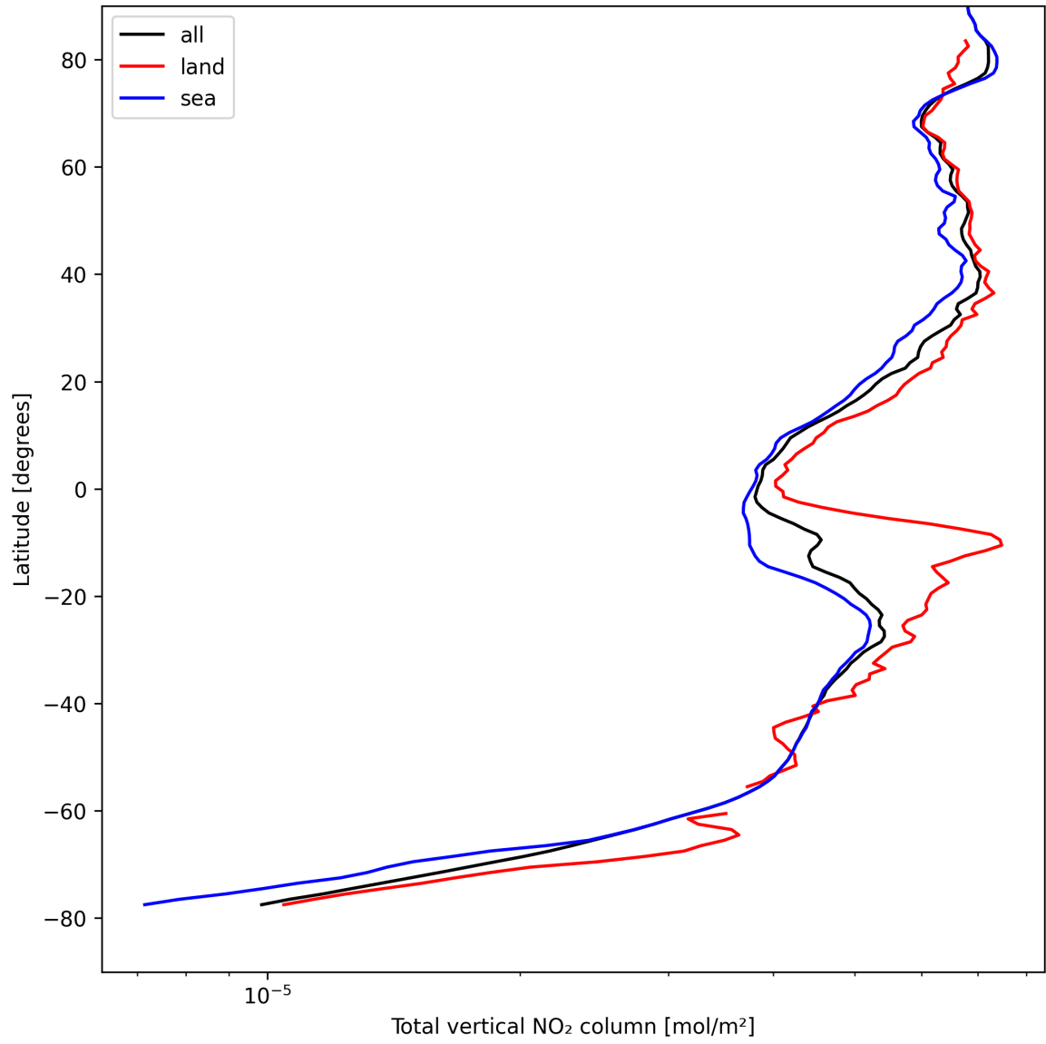
Figure 19: Zonal average of “Total vertical NO 2 column” for 2025-08-26 to 2025-08-27.
