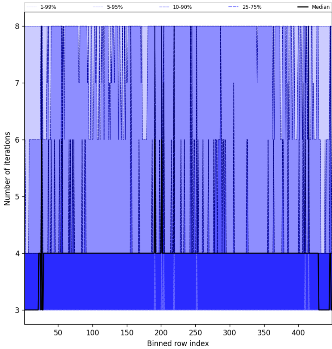
Figure 49: Along track statistics of “Number of iterations” for 2025-08-26 to 2025-08-27
