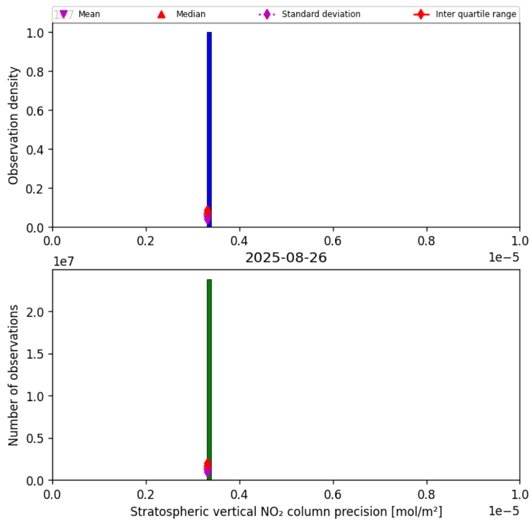
Figure 35: Histogram of “Stratospheric vertical NO 2 column precision” for 2025-08-26 to 2025-08-27
