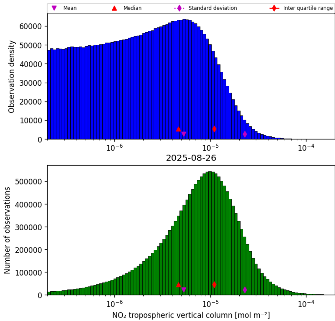
Figure 27: Histogram of “NO 2 tropospheric vertical column” for 2025-08-26 to 2025-08-27
