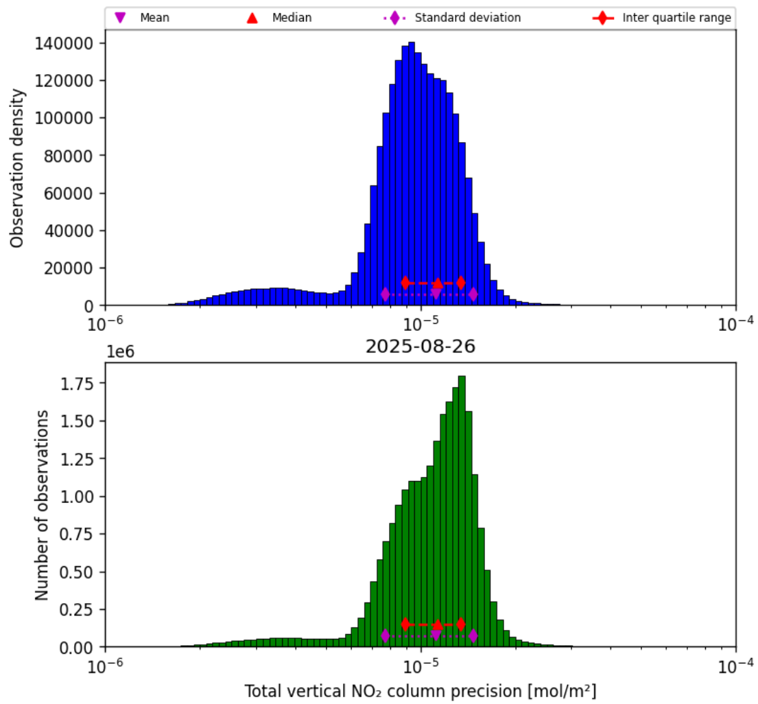
Figure 37: Histogram of “Total vertical NO 2 column precision” for 2025-08-26 to 2025-08-27
