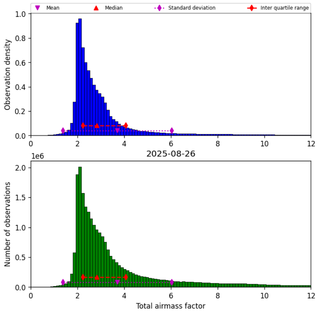
Figure 30: Histogram of “Total airmass factor” for 2025-08-26 to 2025-08-27
