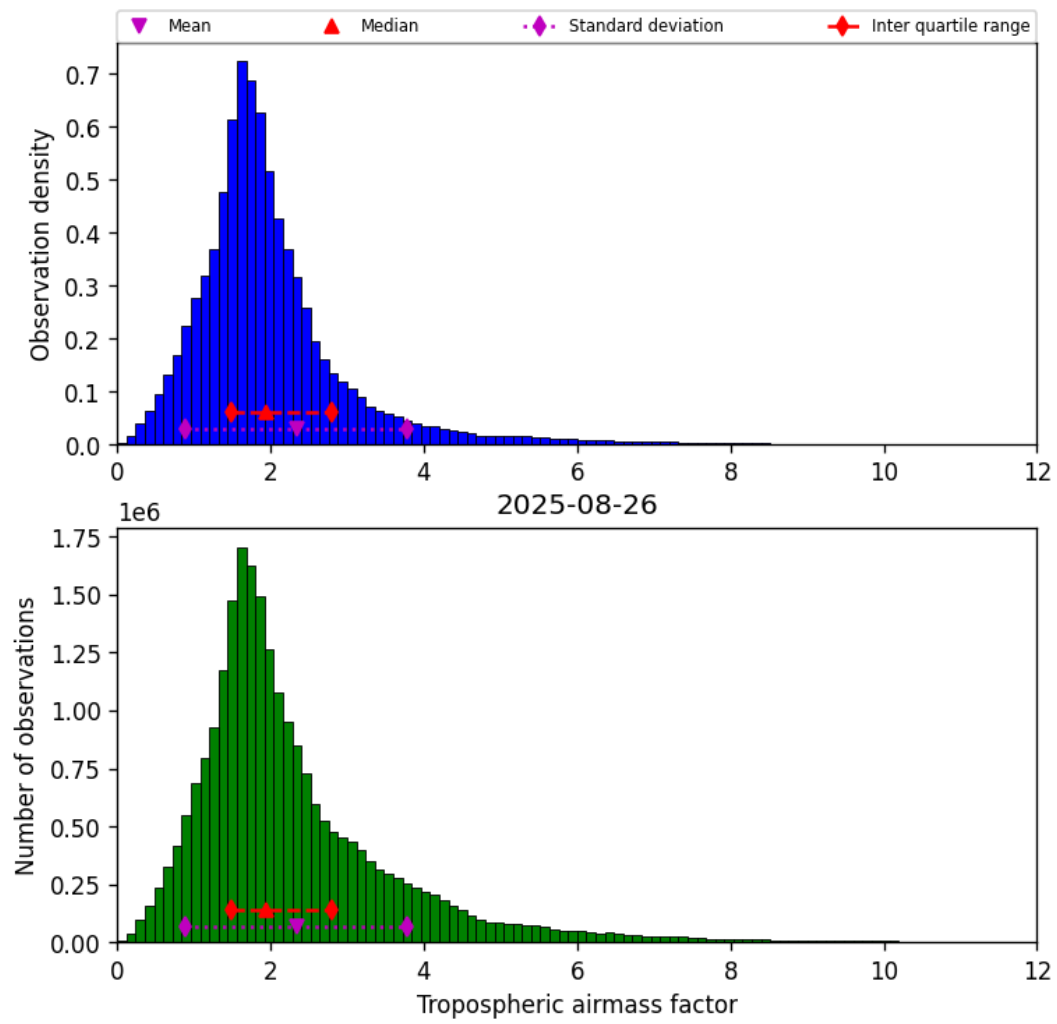
Figure 29: Histogram of “Tropospheric airmass factor” for 2025-08-26 to 2025-08-27
