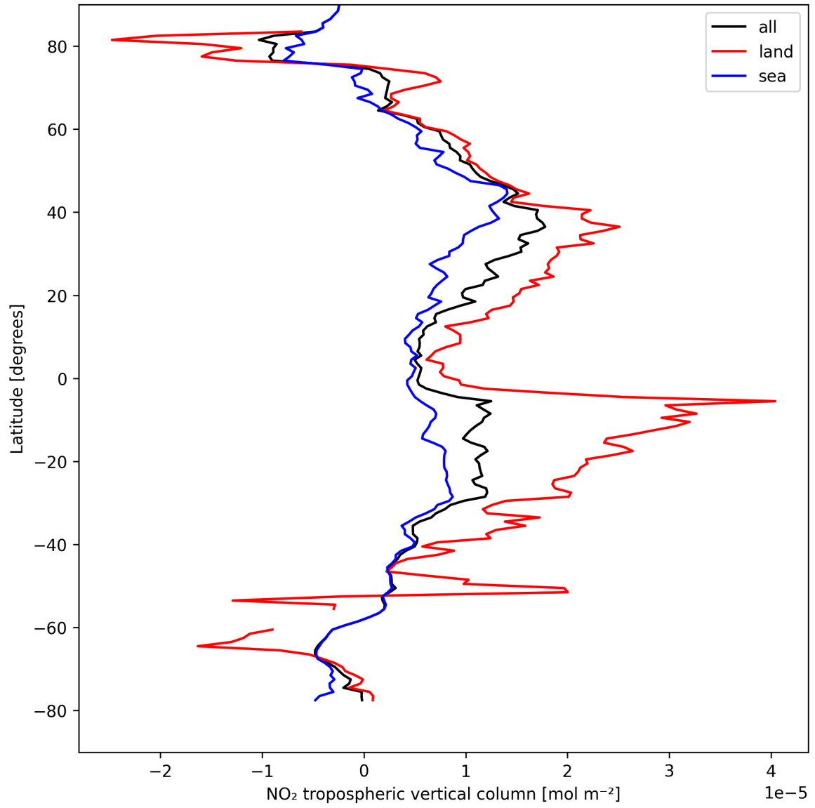
Figure 10: Zonal average of “NO 2 tropospheric vertical column” for 2025-08-26 to 2025-08-27.
