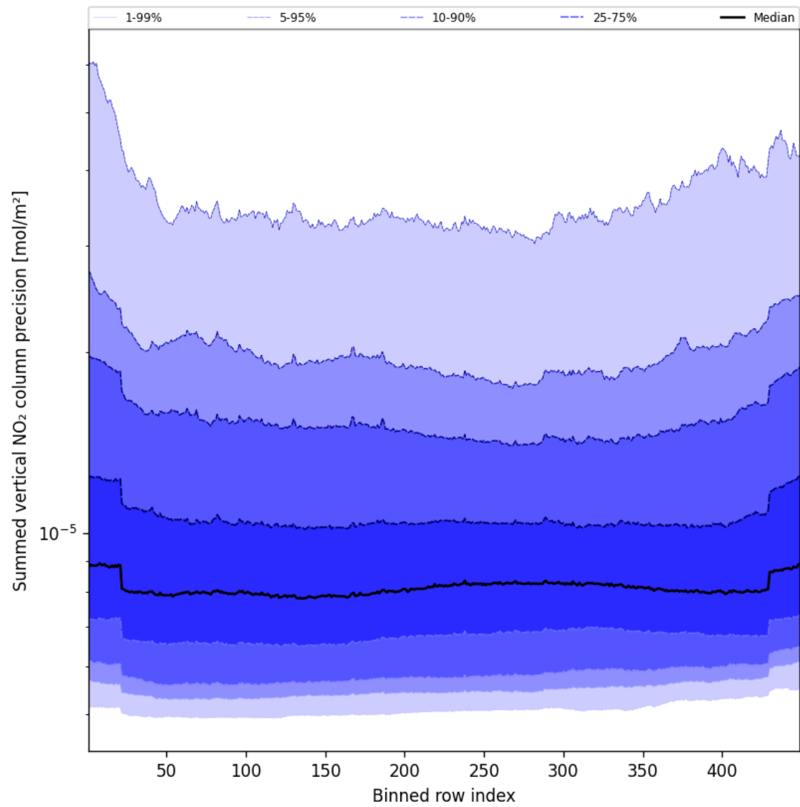
Figure 56: Along track statistics of “Summed vertical NO 2 column precision” for 2025-08-26 to 2025-08-27
