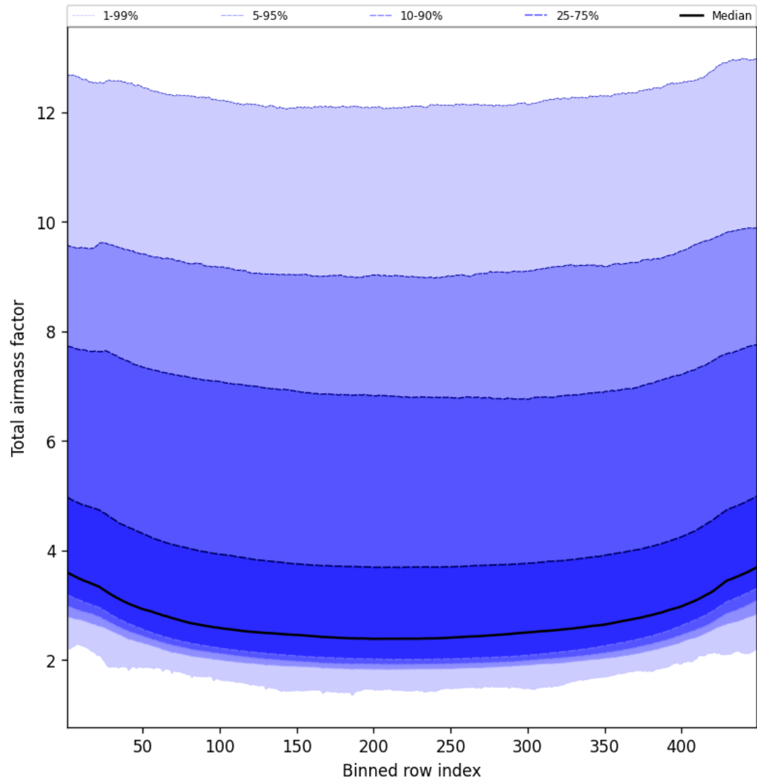
Figure 47: Along track statistics of “Total airmass factor” for 2025-08-26 to 2025-08-27
