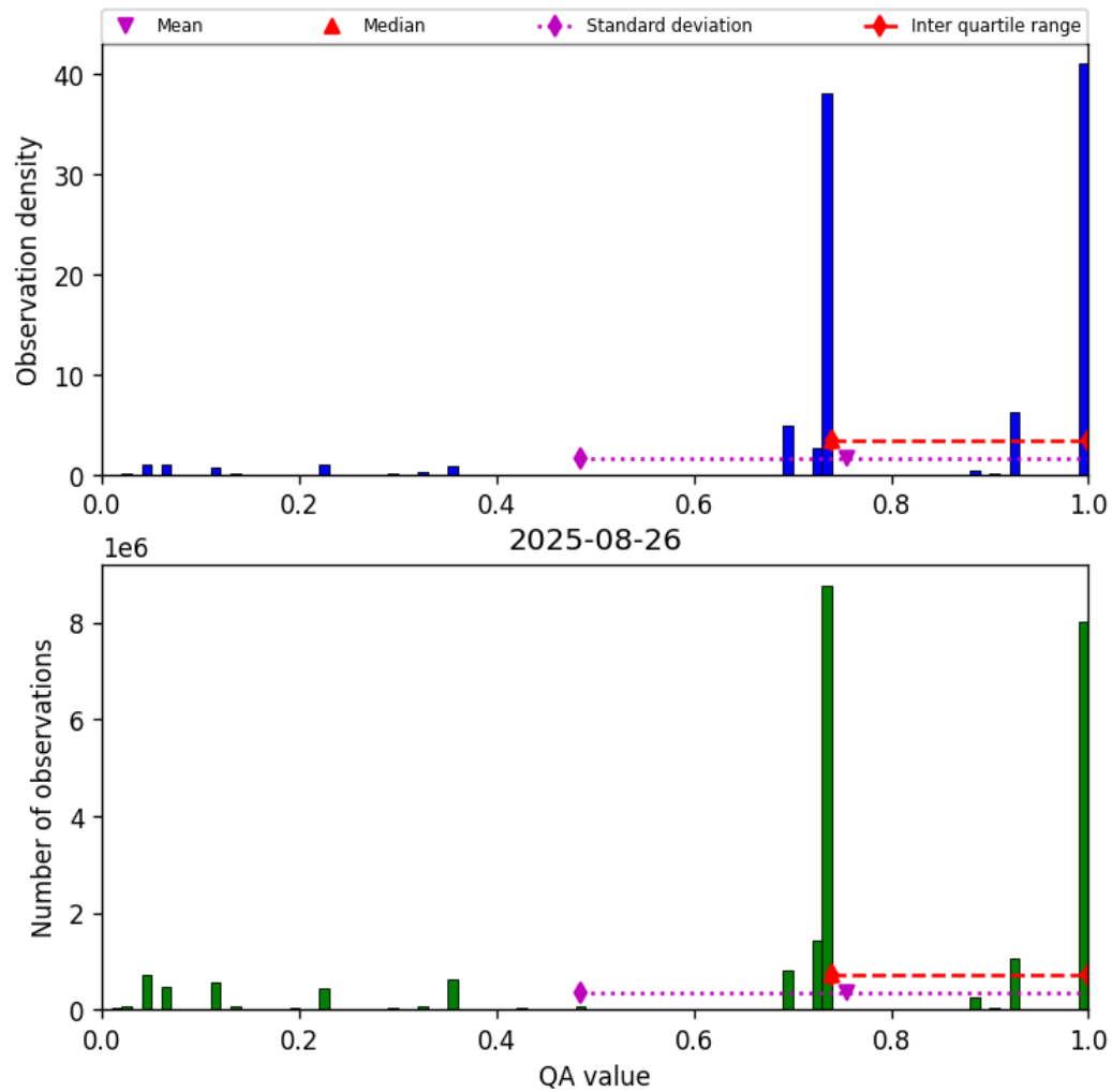
Figure 26: Histogram of “QA value” for 2025-08-26 to 2025-08-27
