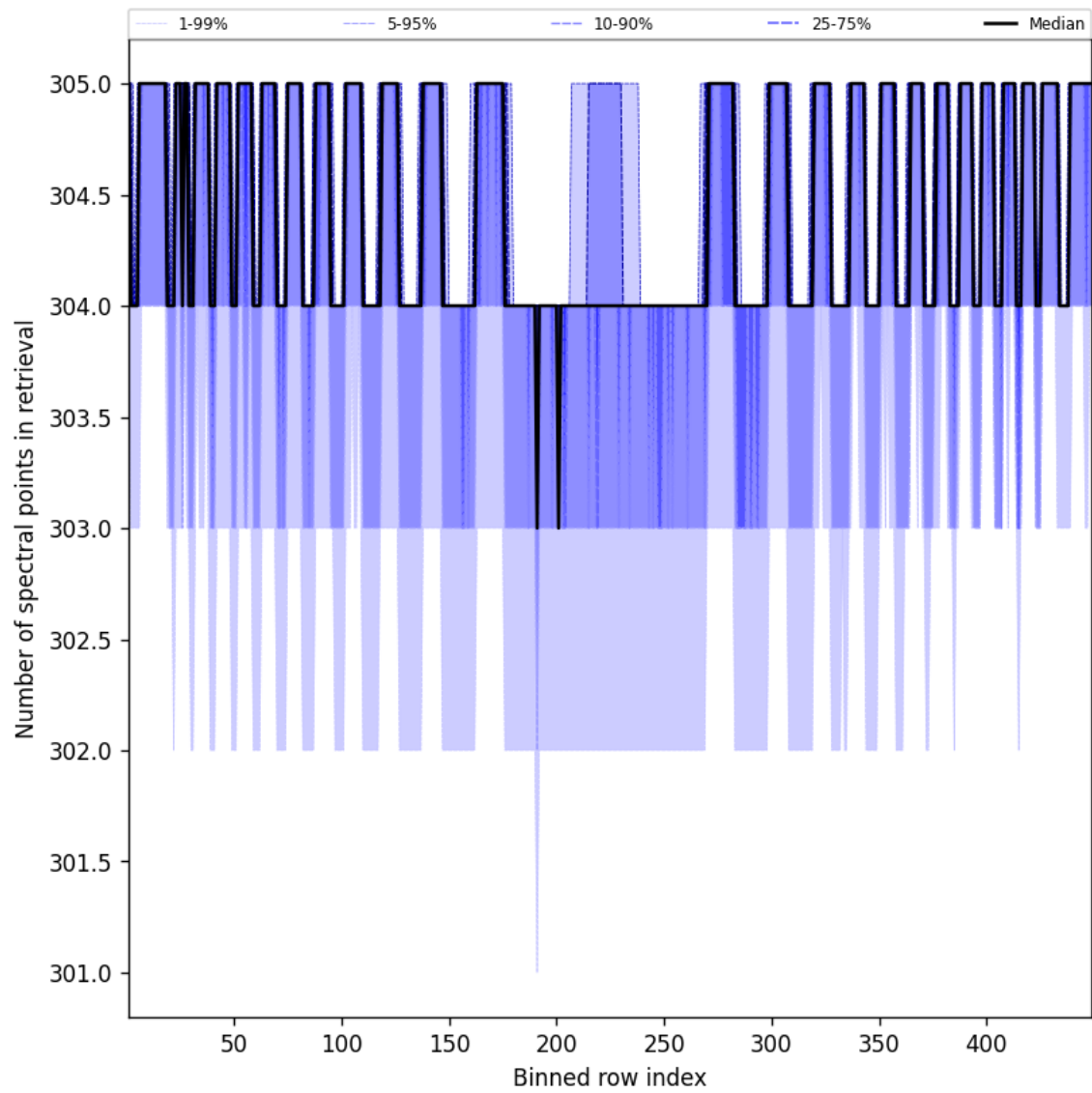
Figure 48: Along track statistics of “Number of spectral points in retrieval” for 2025-08-26 to 2025-08-27
