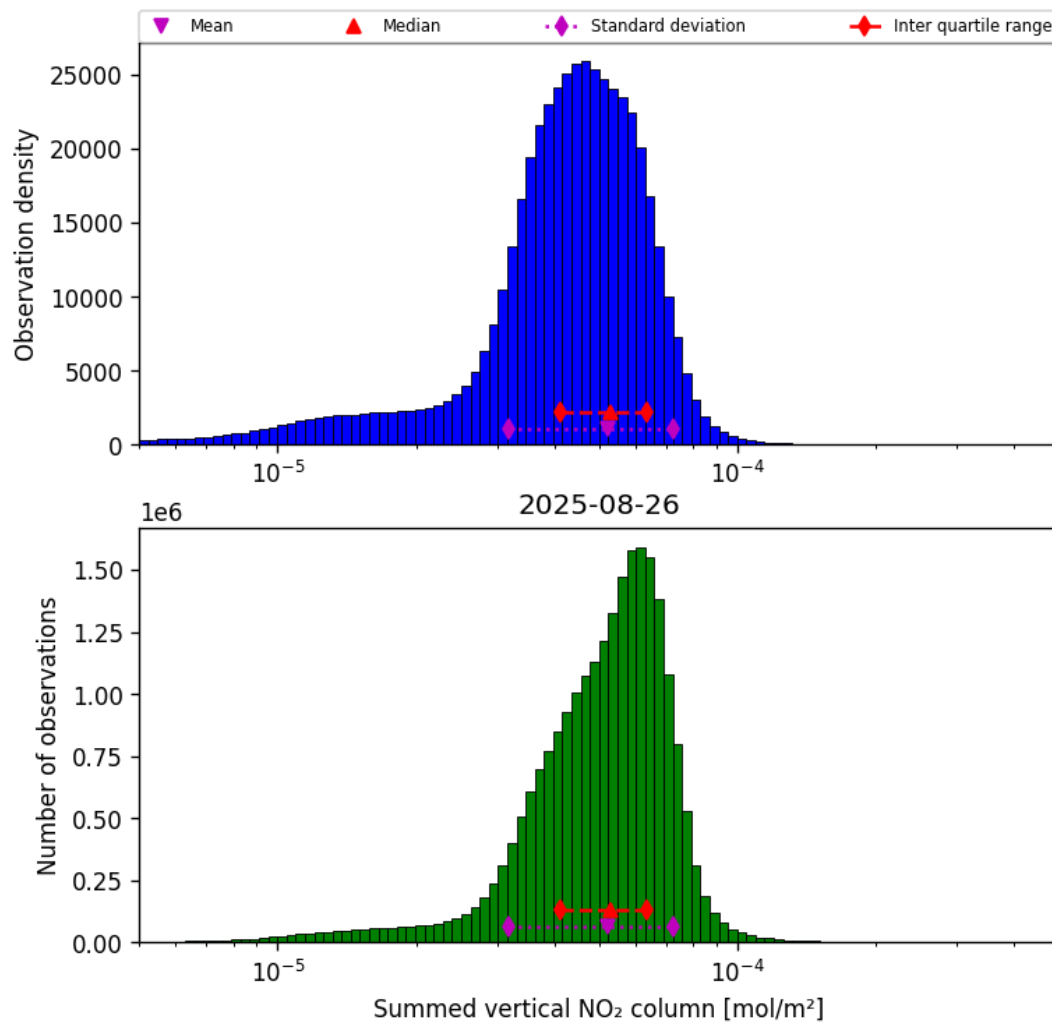
Figure 38: Histogram of “Summed vertical NO 2 column” for 2025-08-26 to 2025-08-27
