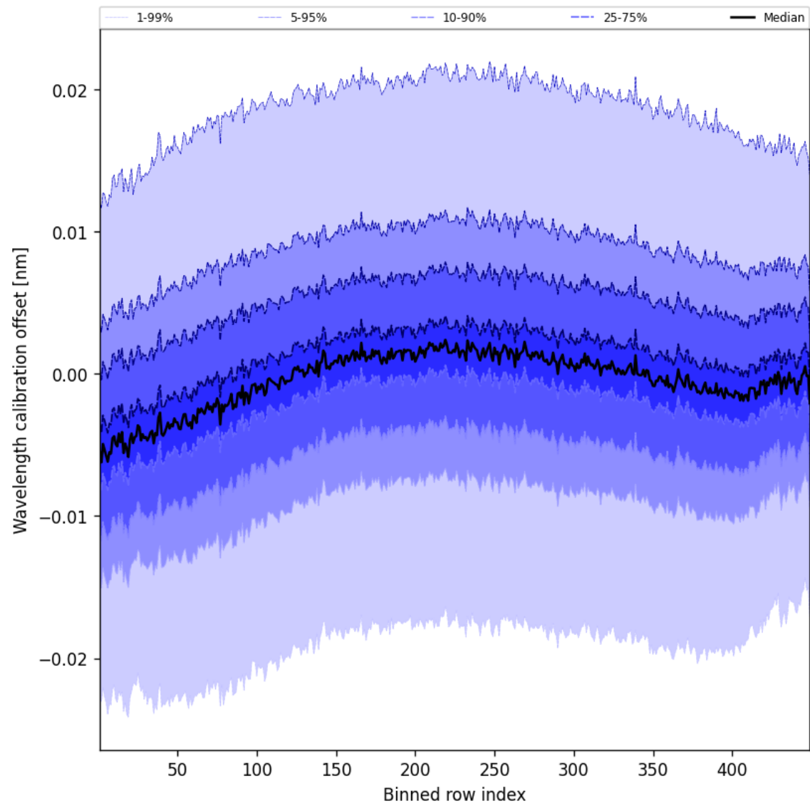
Figure 50: Along track statistics of “Wavelength calibration offset” for 2025-08-26 to 2025-08-27
