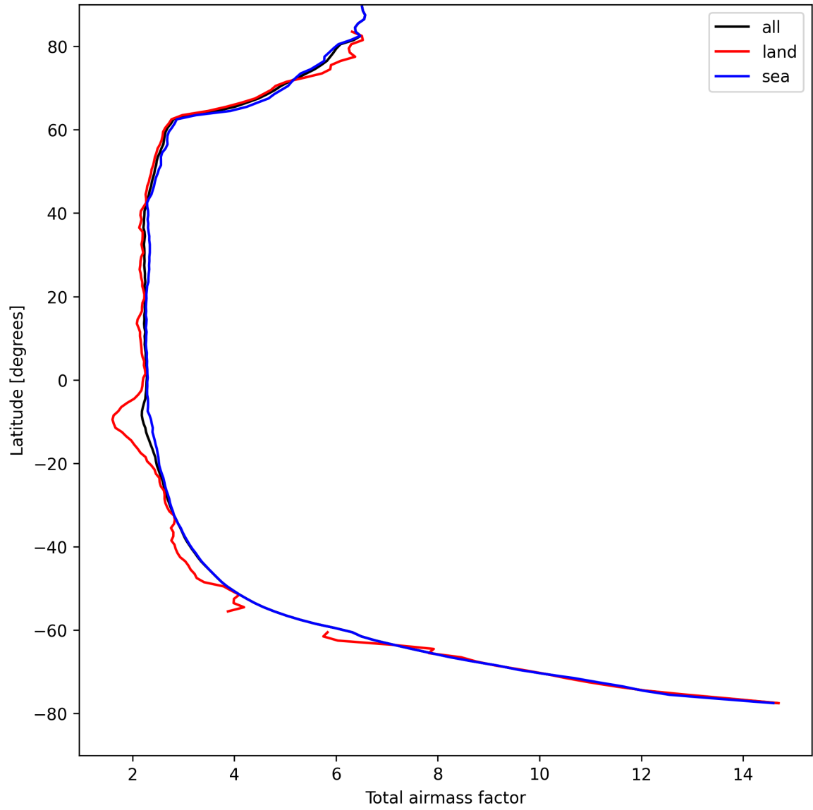
Figure 13: Zonal average of “Total airmass factor” for 2025-08-26 to 2025-08-27.
