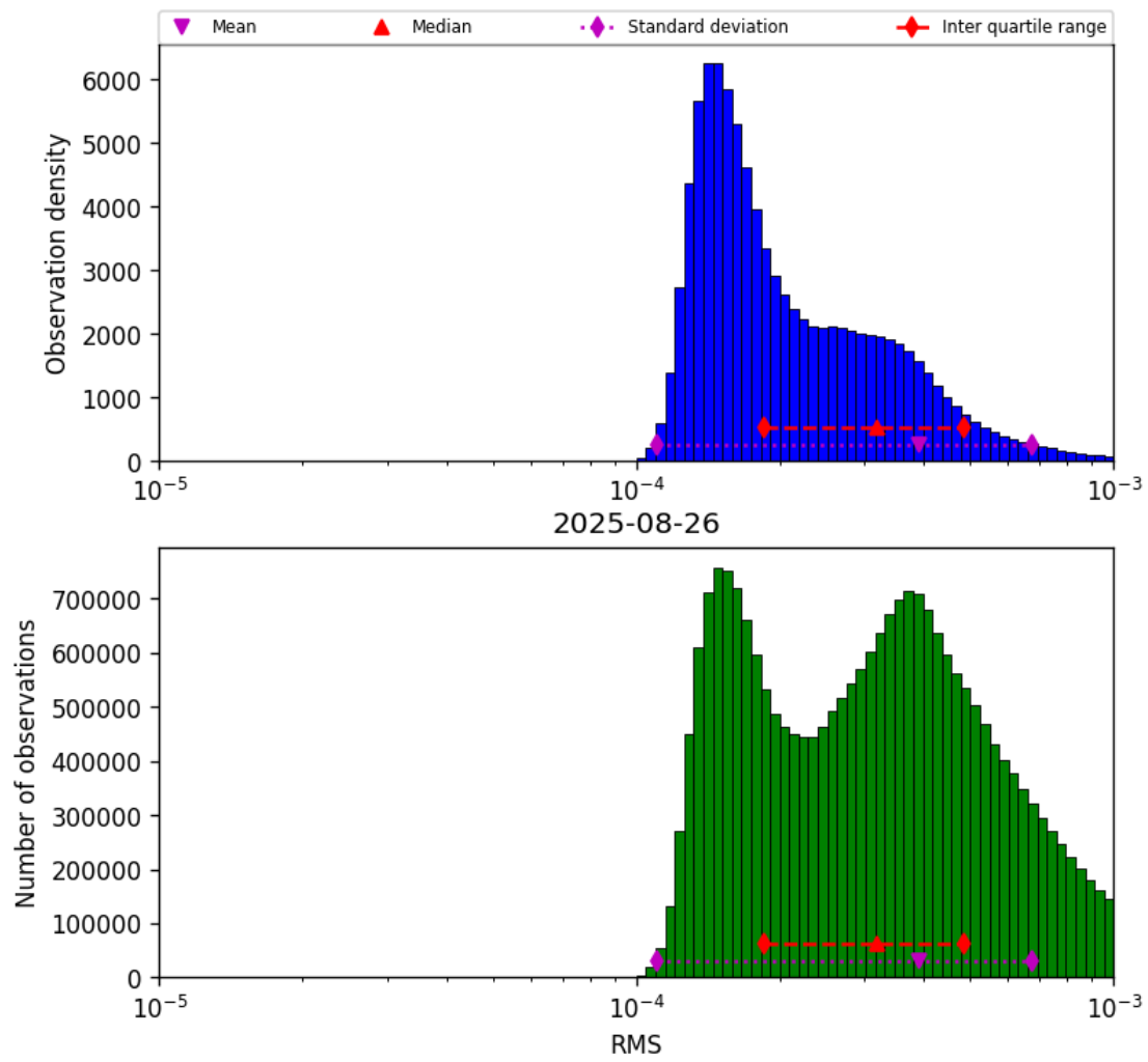
Figure 41: Histogram of “RMS” for 2025-08-26 to 2025-08-27
