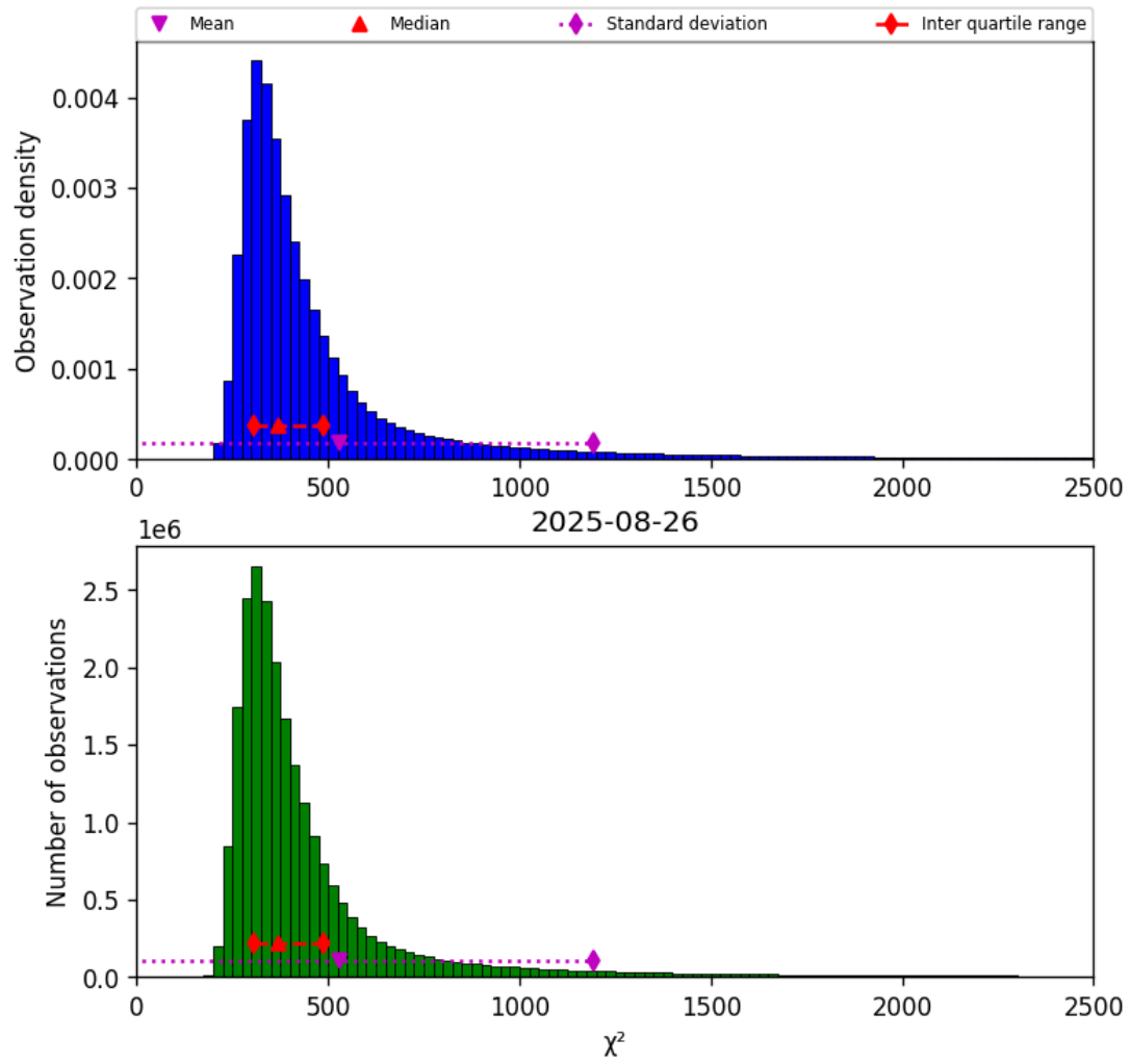
Figure 40: Histogram of “ \chi^2 ” for 2025-08-26 to 2025-08-27
