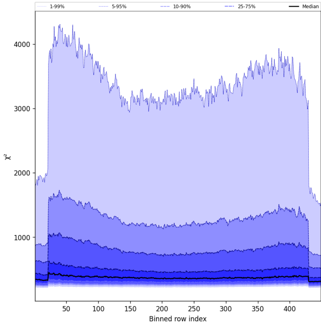
Figure 57: Along track statistics of “ \chi^2 ” for 2025-08-26 to 2025-08-27
