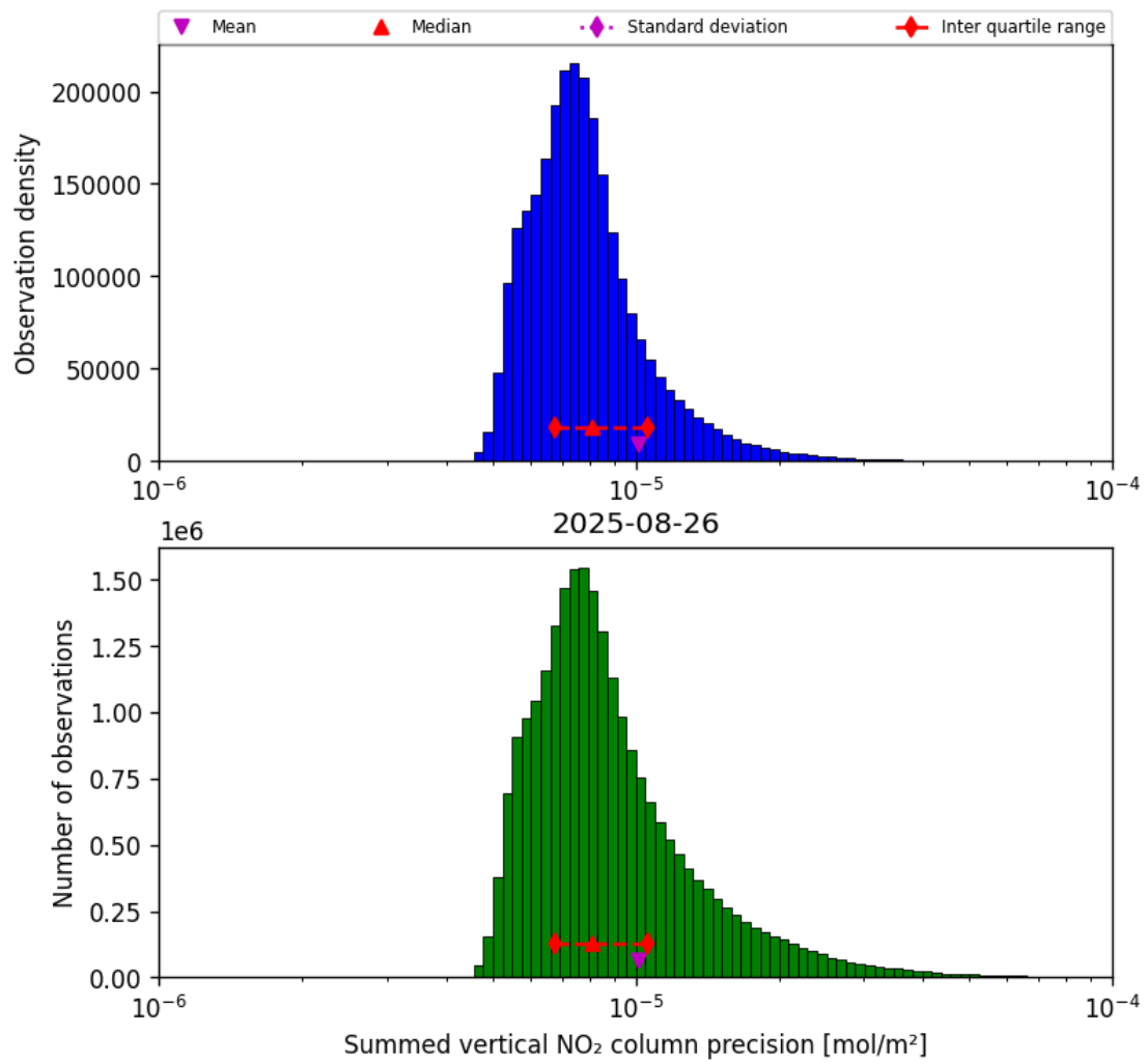
Figure 39: Histogram of “Summed vertical NO 2 column precision” for 2025-08-26 to 2025-08-27
