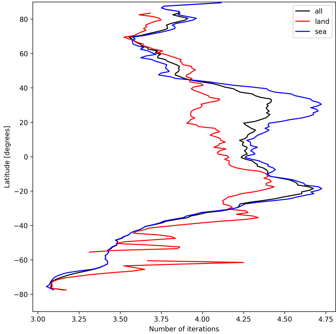
Figure 15: Zonal average of “Number of iterations” for 2025-08-26 to 2025-08-27.
