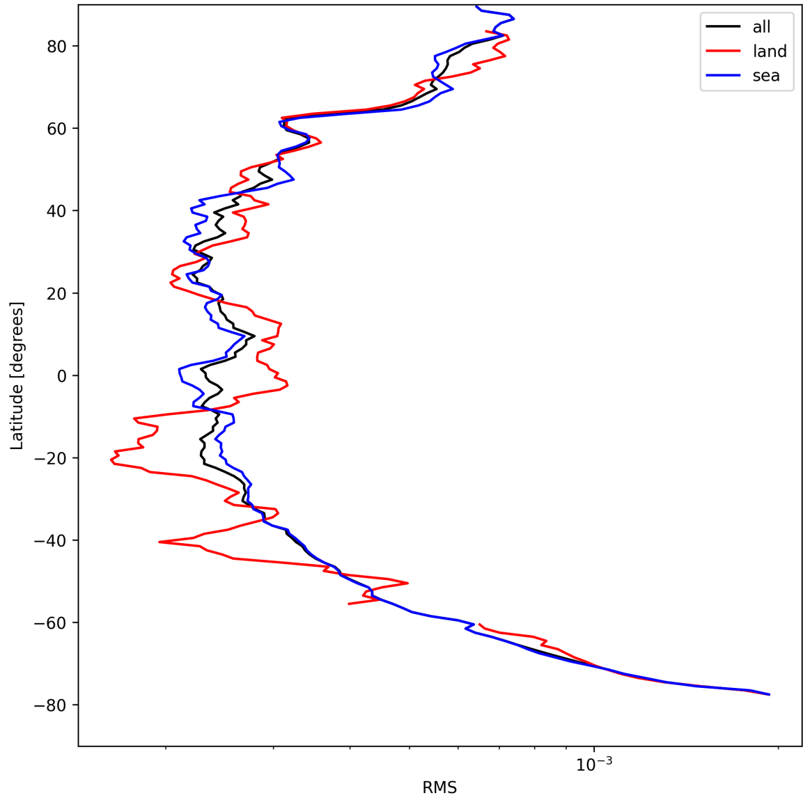
Figure 24: Zonal average of “RMS” for 2025-08-26 to 2025-08-27.
