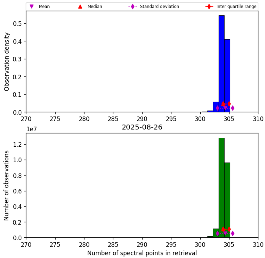
Figure 31: Histogram of “Number of spectral points in retrieval” for 2025-08-26 to 2025-08-27
