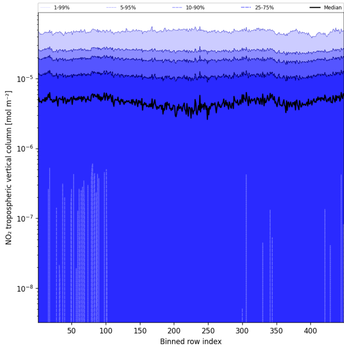
Figure 44: Along track statistics of “NO 2 tropospheric vertical column” for 2025-08-26 to 2025-08-27
