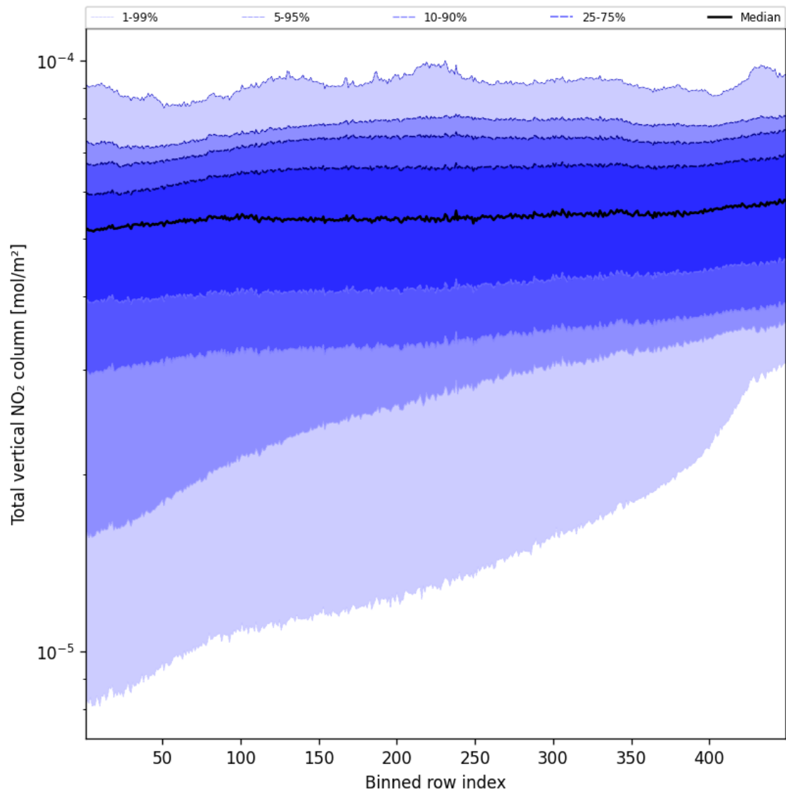
Figure 53: Along track statistics of “Total vertical NO 2 column” for 2025-08-26 to 2025-08-27
