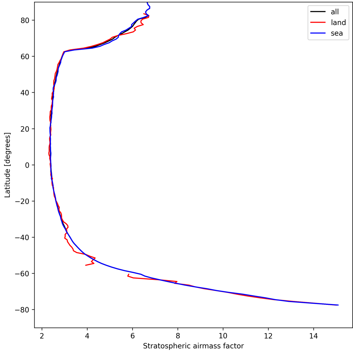
Figure 25: Zonal average of “Stratospheric airmass factor” for 2025-08-26 to 2025-08-27.
