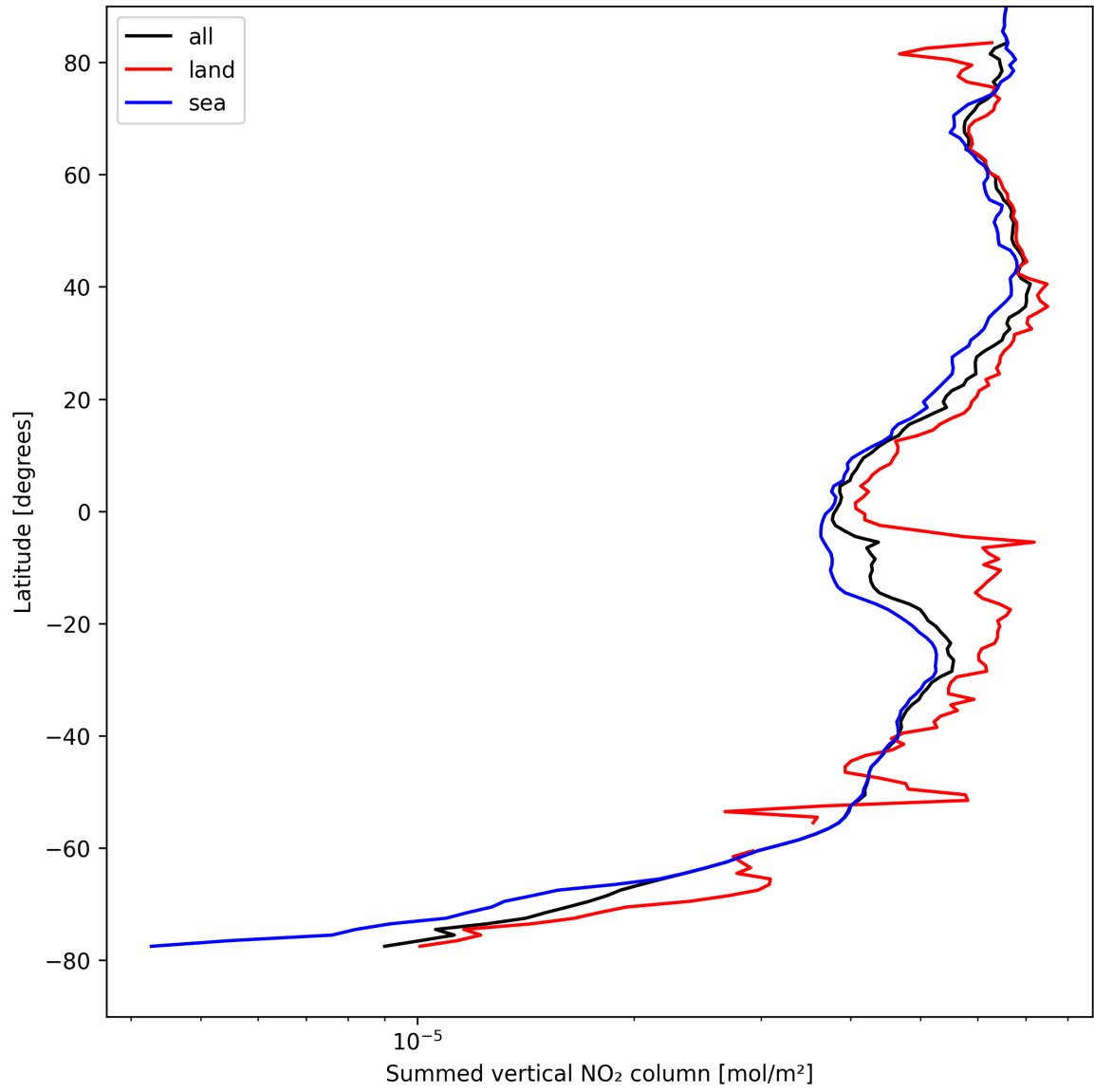
Figure 21: Zonal average of “Summed vertical NO 2 column” for 2025-08-26 to 2025-08-27.
