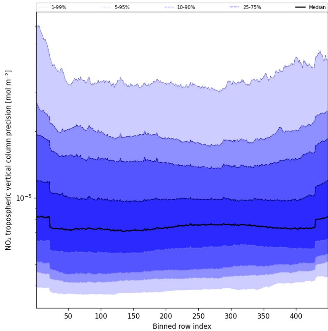
Figure 45: Along track statistics of “NO 2 tropospheric vertical column precision” for 2025-08-26 to 2025-08-27
