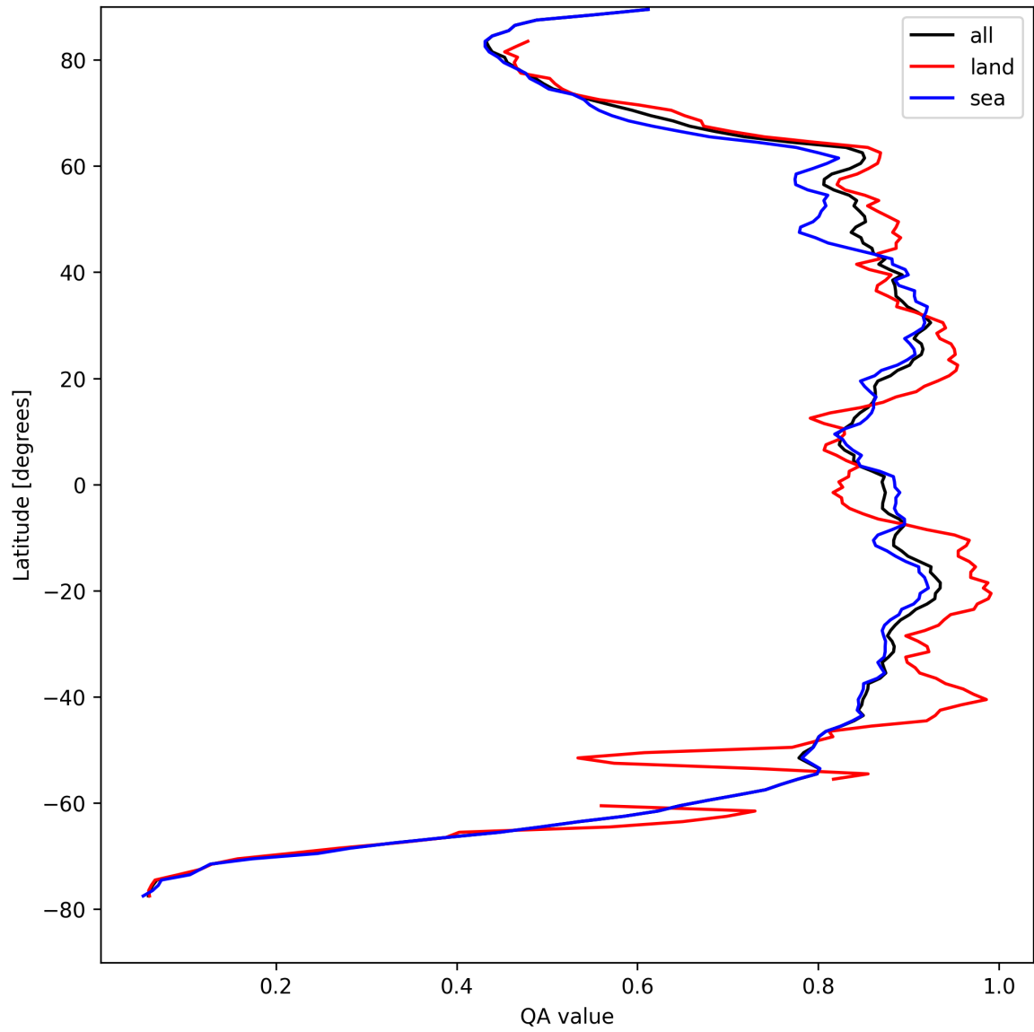
Figure 9: Zonal average of “QA value” for 2025-08-26 to 2025-08-27.
