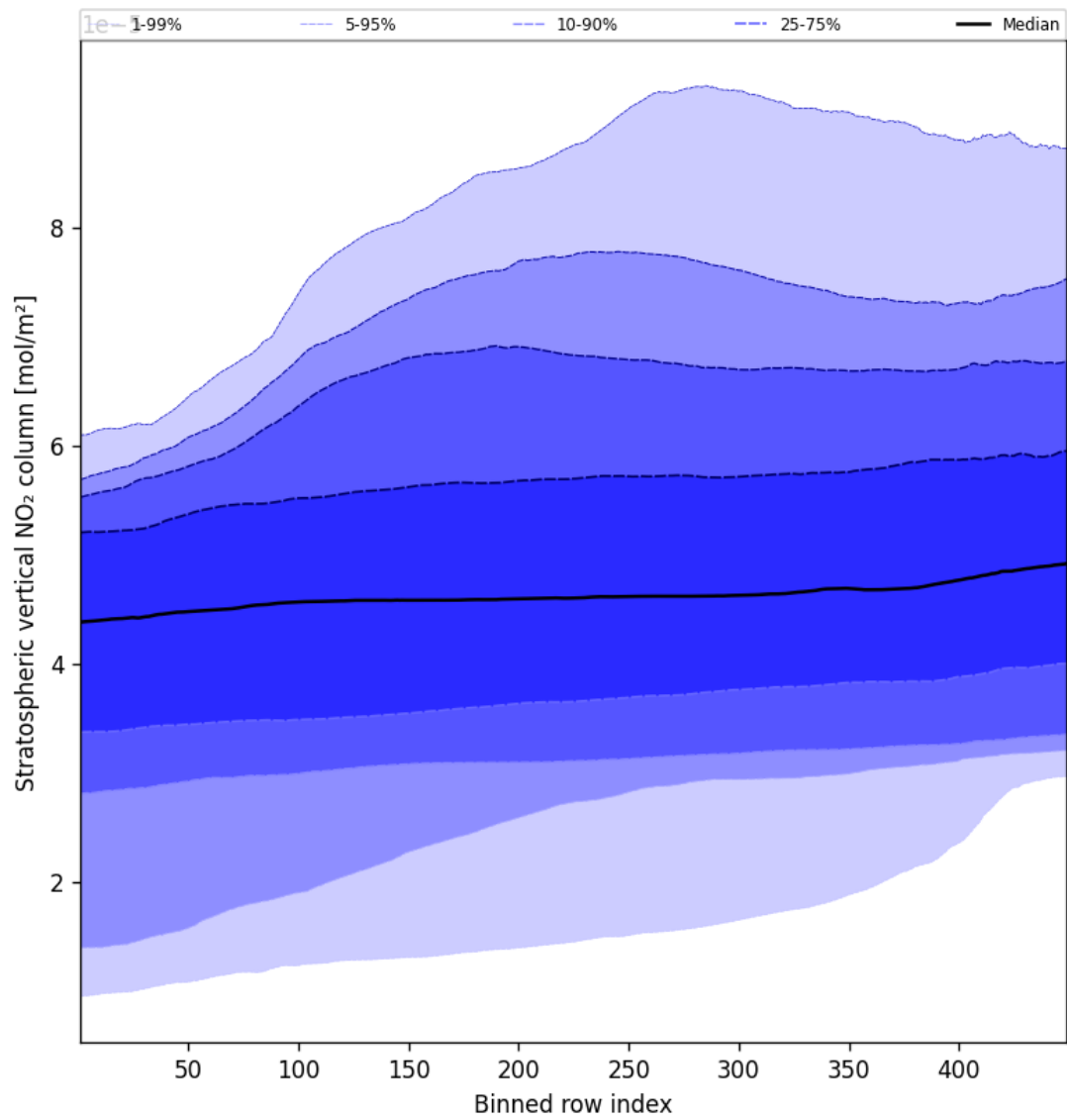
Figure 51: Along track statistics of “Stratospheric vertical NO 2 column” for 2025-08-26 to 2025-08-27
