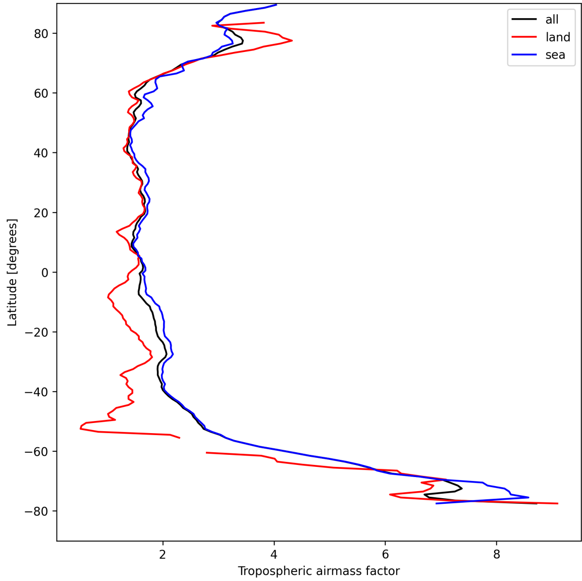
Figure 12: Zonal average of “Tropospheric airmass factor” for 2025-08-26 to 2025-08-27.
