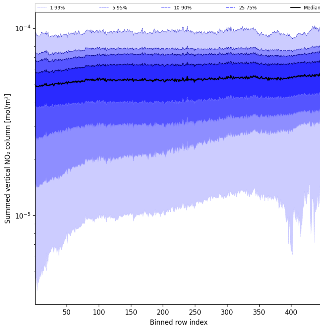
Figure 55: Along track statistics of “Summed vertical NO 2 column” for 2025-08-26 to 2025-08-27
