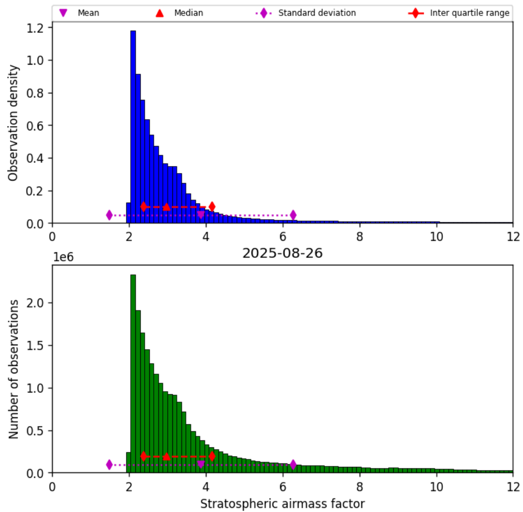
Figure 42: Histogram of “Stratospheric airmass factor” for 2025-08-26 to 2025-08-27
