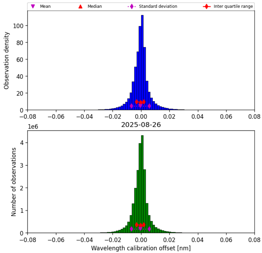
Figure 33: Histogram of “Wavelength calibration offset” for 2025-08-26 to 2025-08-27
