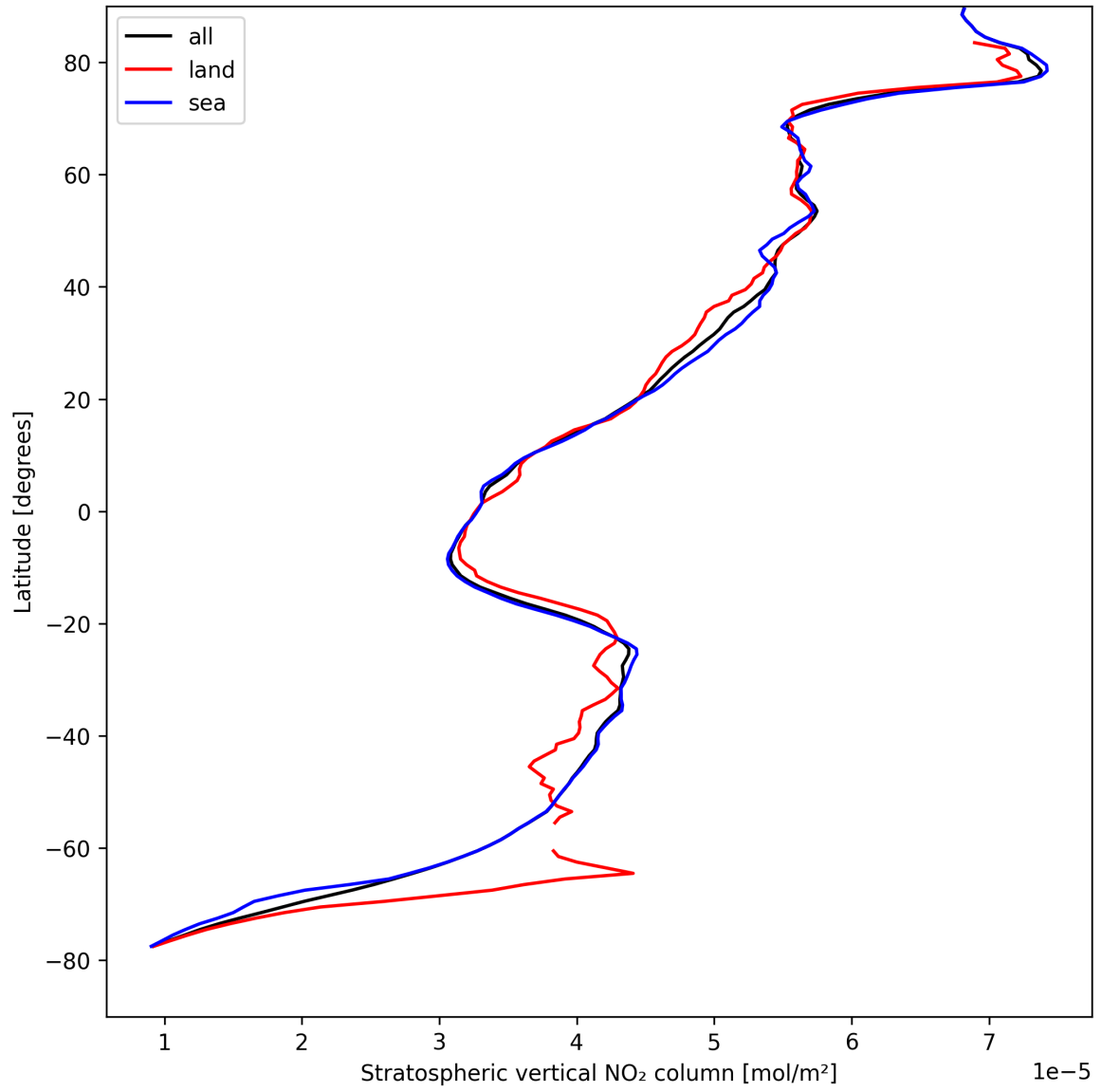
Figure 17: Zonal average of “Stratospheric vertical NO 2 column” for 2025-08-26 to 2025-08-27.
