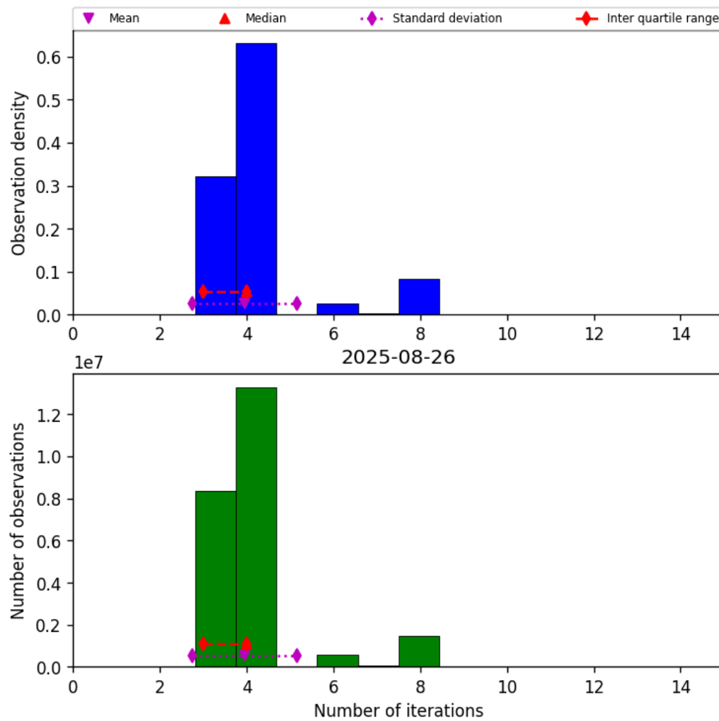
Figure 32: Histogram of “Number of iterations” for 2025-08-26 to 2025-08-27
