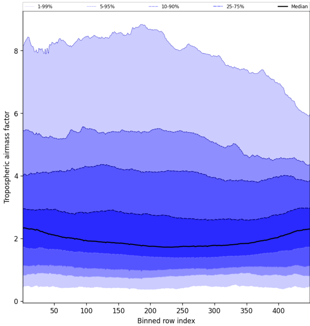
Figure 46: Along track statistics of “Tropospheric air mass factor” for 2025-08-26 to 2025-08-27
