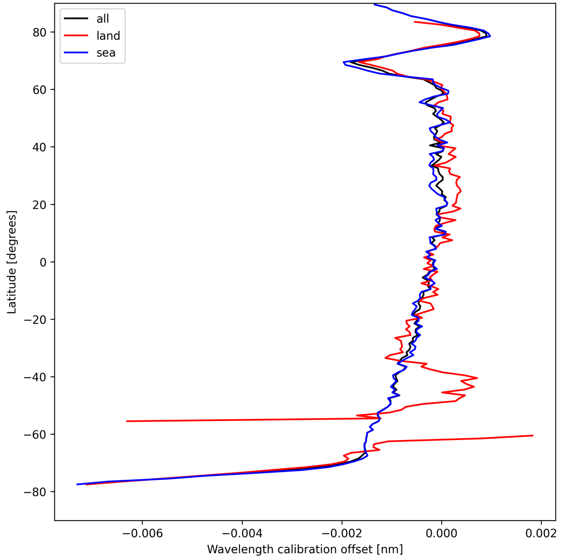
Figure 16: Zonal average of “Wavelength calibration offset” for 2025-08-26 to 2025-08-27.
