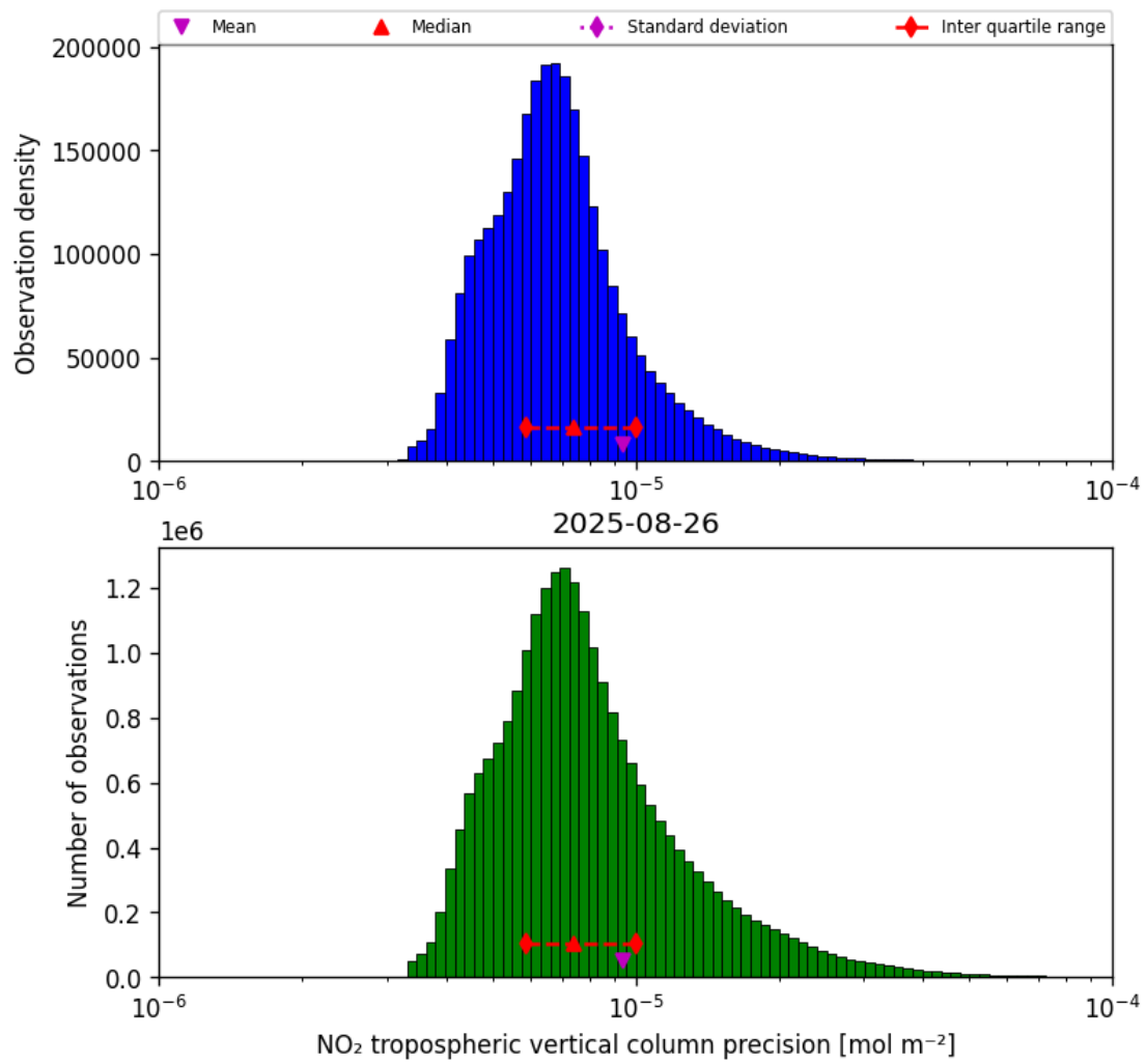
Figure 28: Histogram of “NO 2 tropospheric vertical column precision” for 2025-08-26 to 2025-08-27
