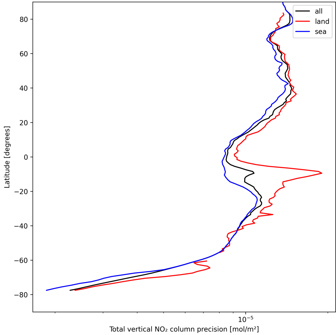
Figure 20: Zonal average of “Total vertical NO 2 column precision” for 2025-08-26 to 2025-08-27.
