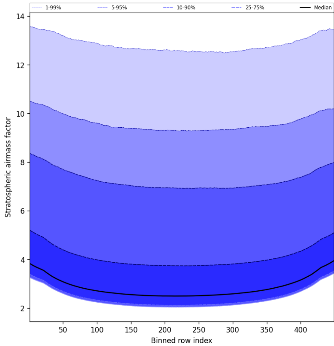
Figure 59: Along track statistics of “Stratospheric airmass factor” for 2025-08-26 to 2025-08-27
