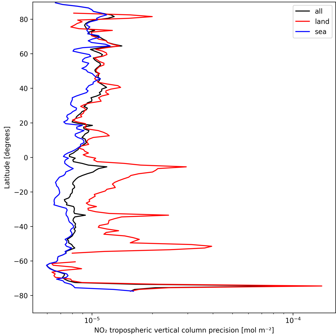
Figure 11: Zonal average of “NO 2 tropospheric vertical column precision” for 2025-08-26 to 2025-08-27.
