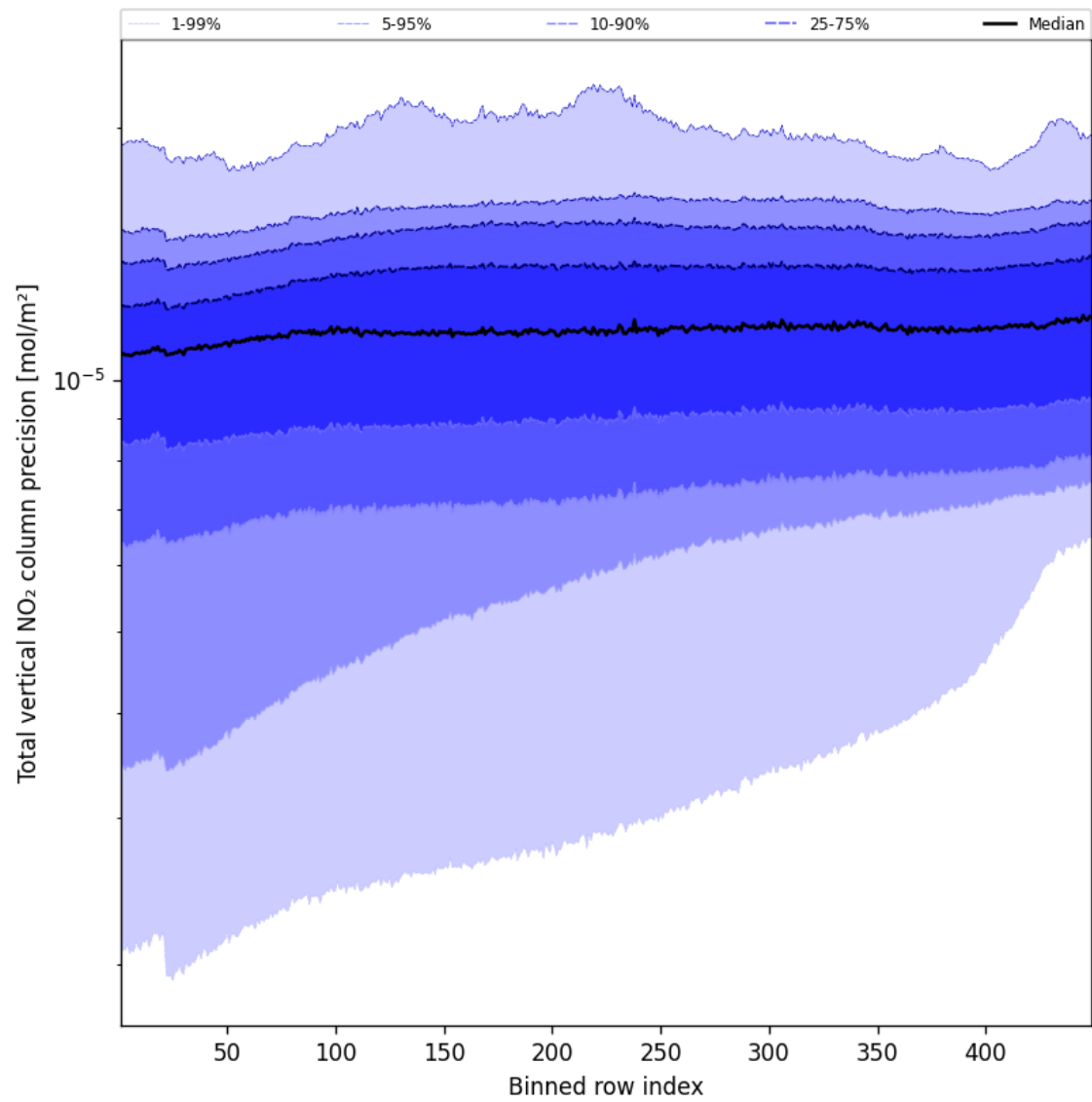
Figure 54: Along track statistics of “Total vertical NO 2 column precision” for 2025-08-26 to 2025-08-27
