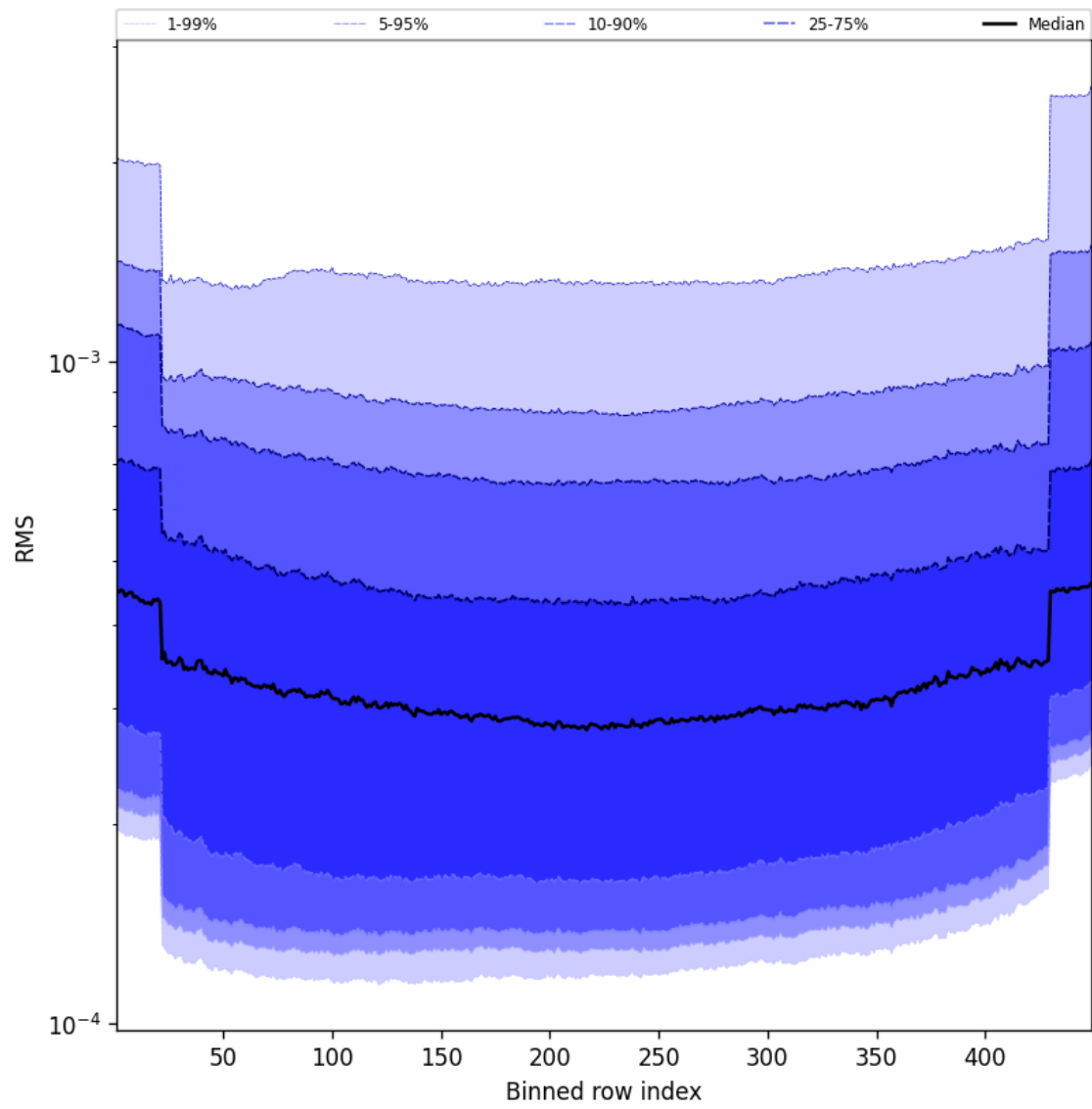
Figure 58: Along track statistics of “RMS” for 2025-08-26 to 2025-08-27
