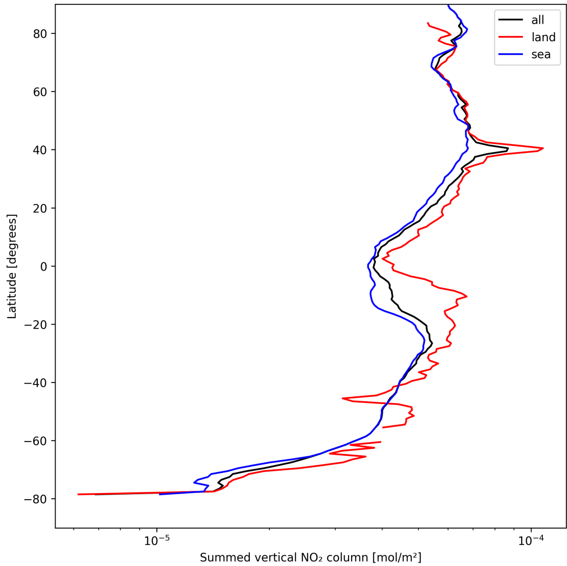
Figure 21: Zonal average of “Summed vertical NO 2 column” for 2025-08-27 to 2025-08-28.
