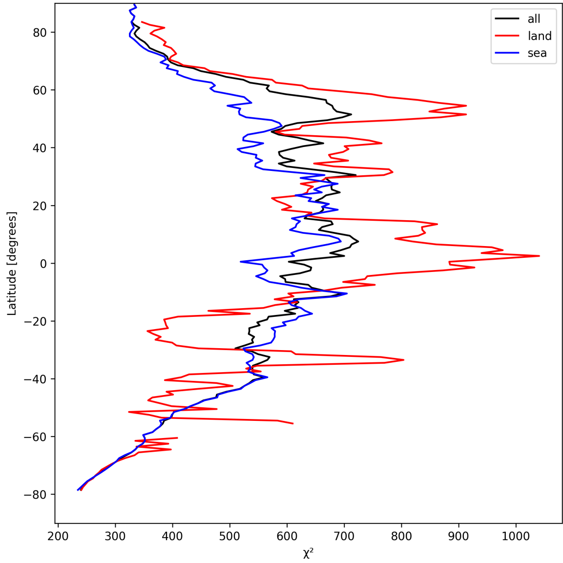
Figure 23: Zonal average of “ \chi^2 ” for 2025-08-27 to 2025-08-28.
