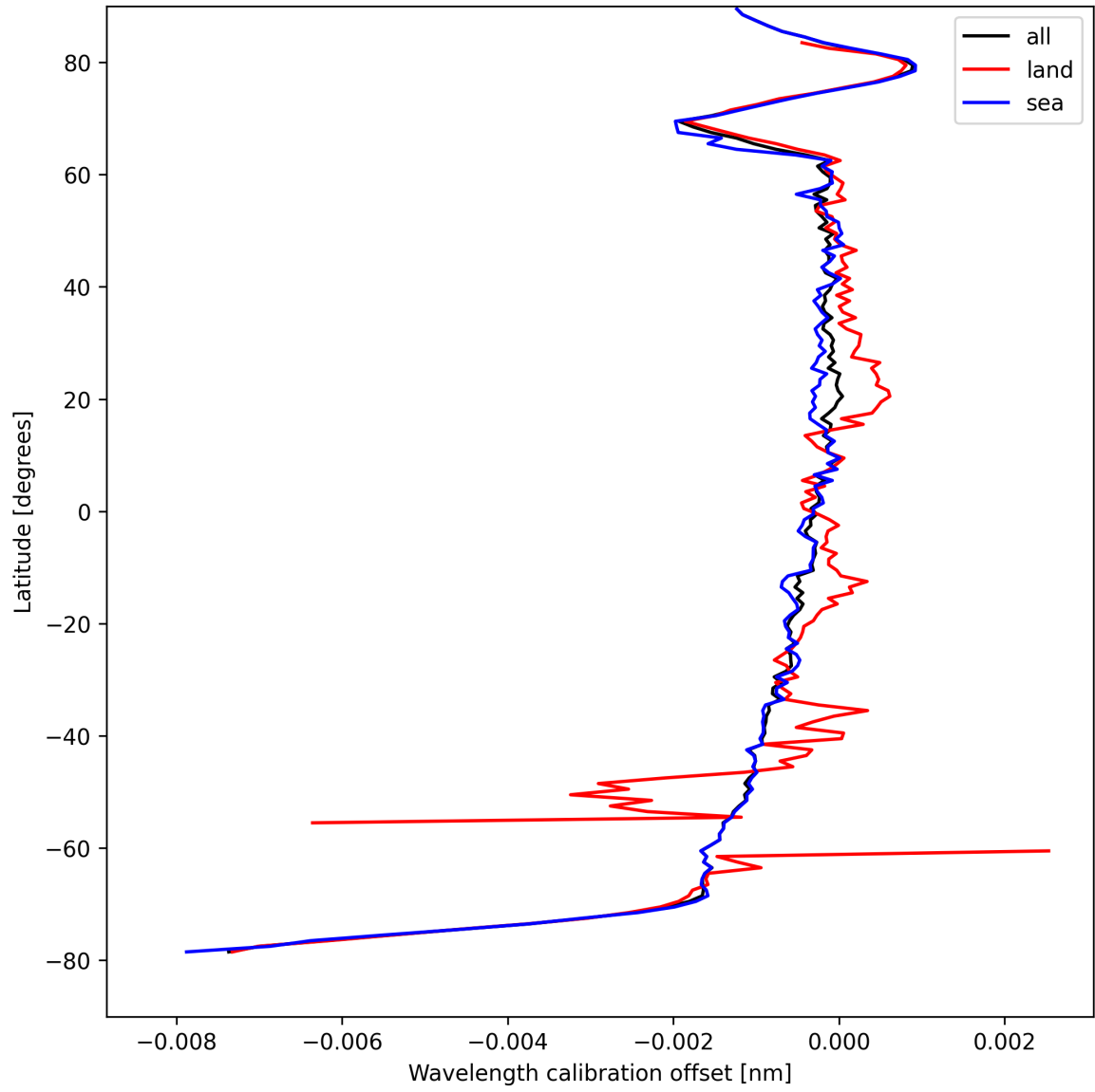
Figure 16: Zonal average of “Wavelength calibration offset” for 2025-08-27 to 2025-08-28.
