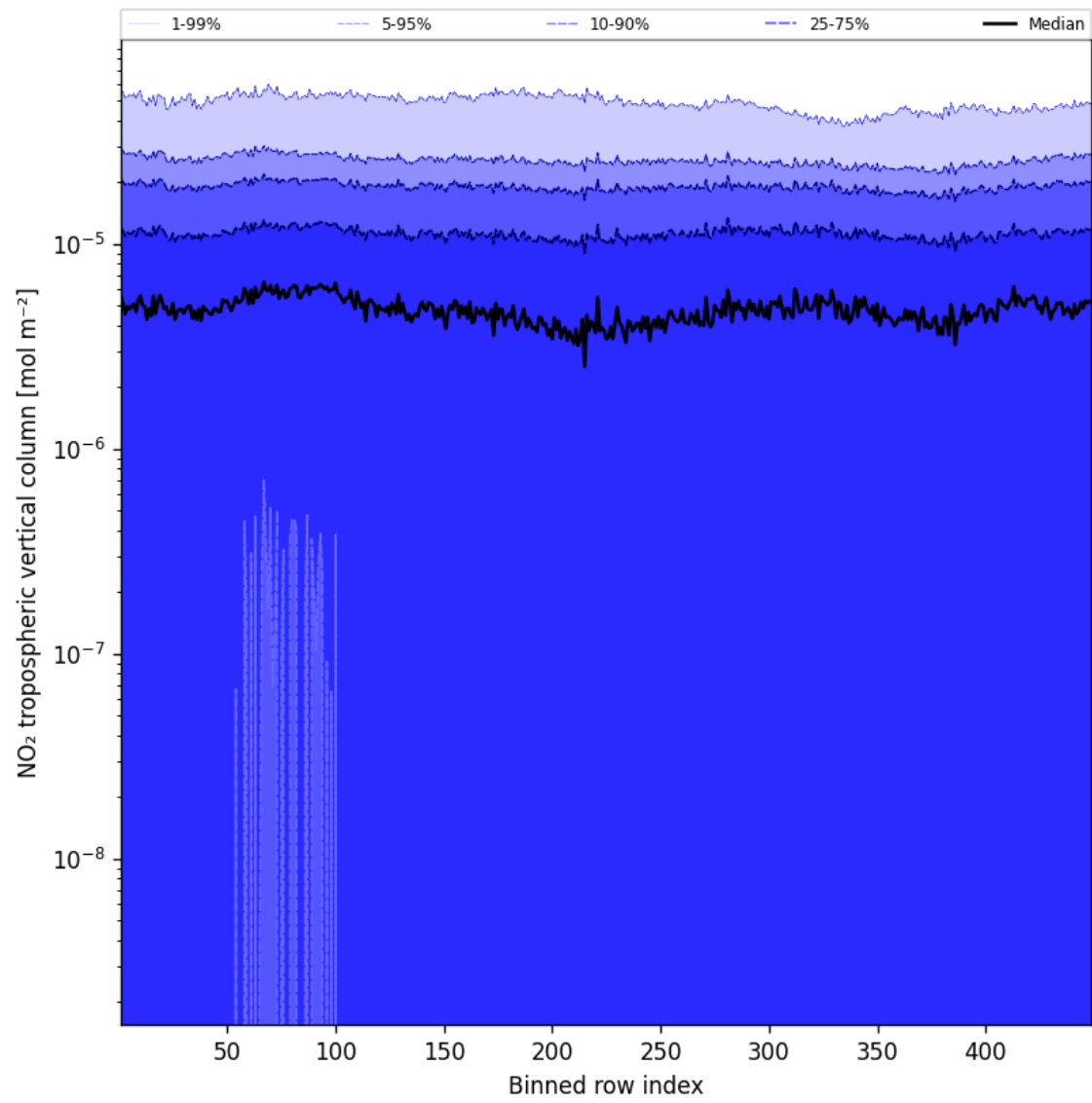
Figure 44: Along track statistics of “NO 2 tropospheric vertical column” for 2025-08-27 to 2025-08-28
