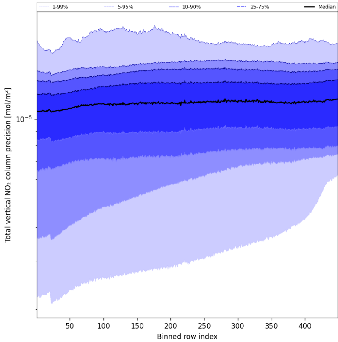
Figure 54: Along track statistics of “Total vertical NO 2 column precision” for 2025-08-27 to 2025-08-28
