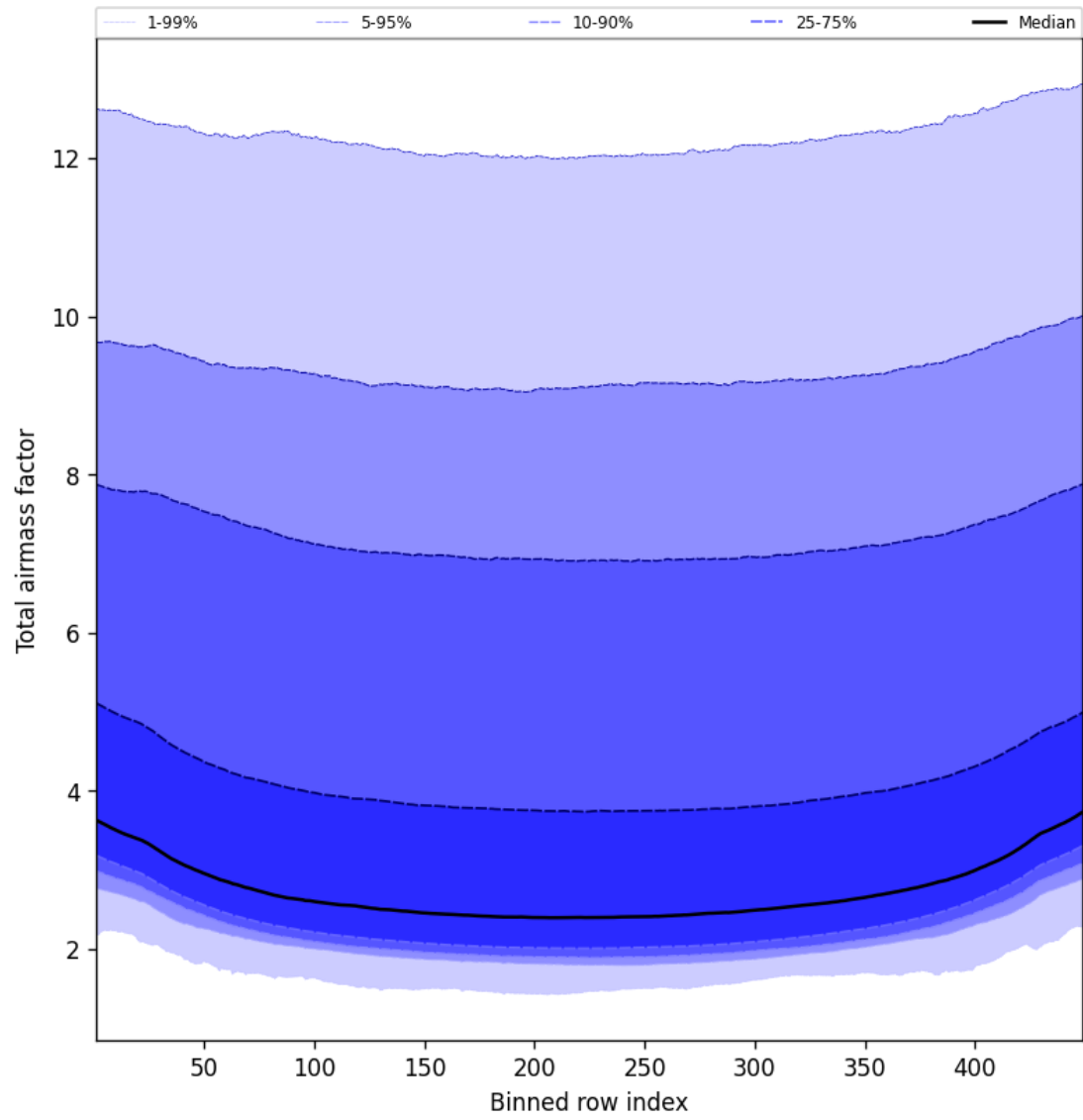
Figure 47: Along track statistics of “Total airmass factor” for 2025-08-27 to 2025-08-28
