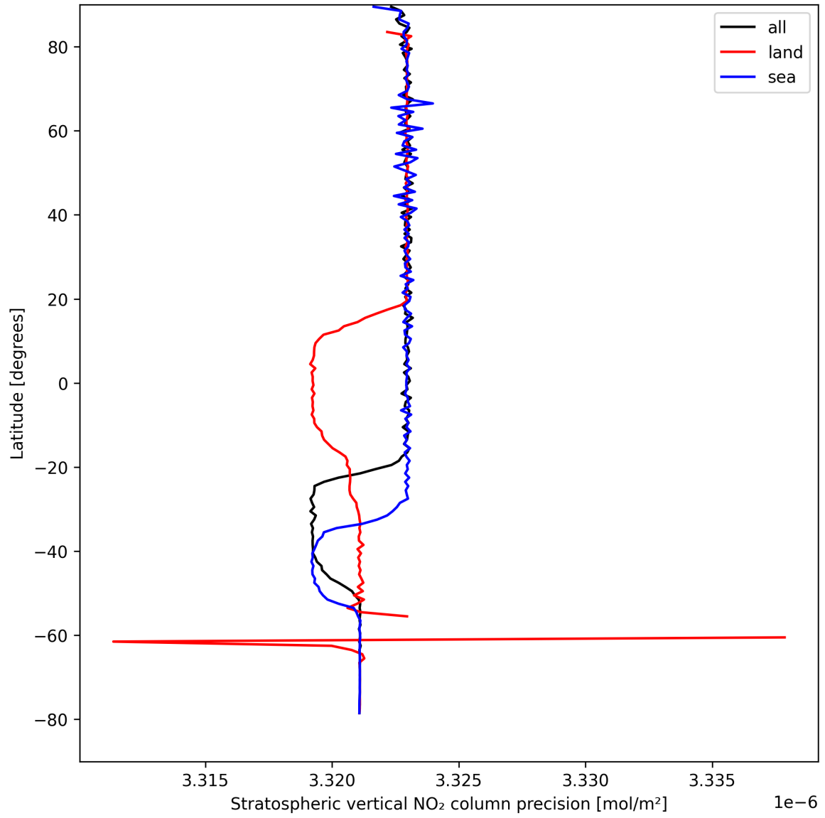
Figure 18: Zonal average of “Stratospheric vertical NO 2 column precision” for 2025-08-27 to 2025-08-28.
