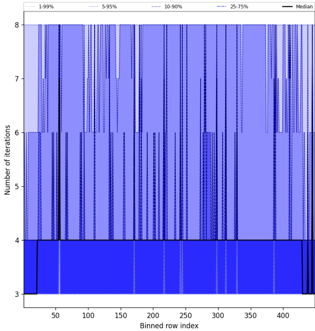
Figure 49: Along track statistics of “Number of iterations” for 2025-08-27 to 2025-08-28
