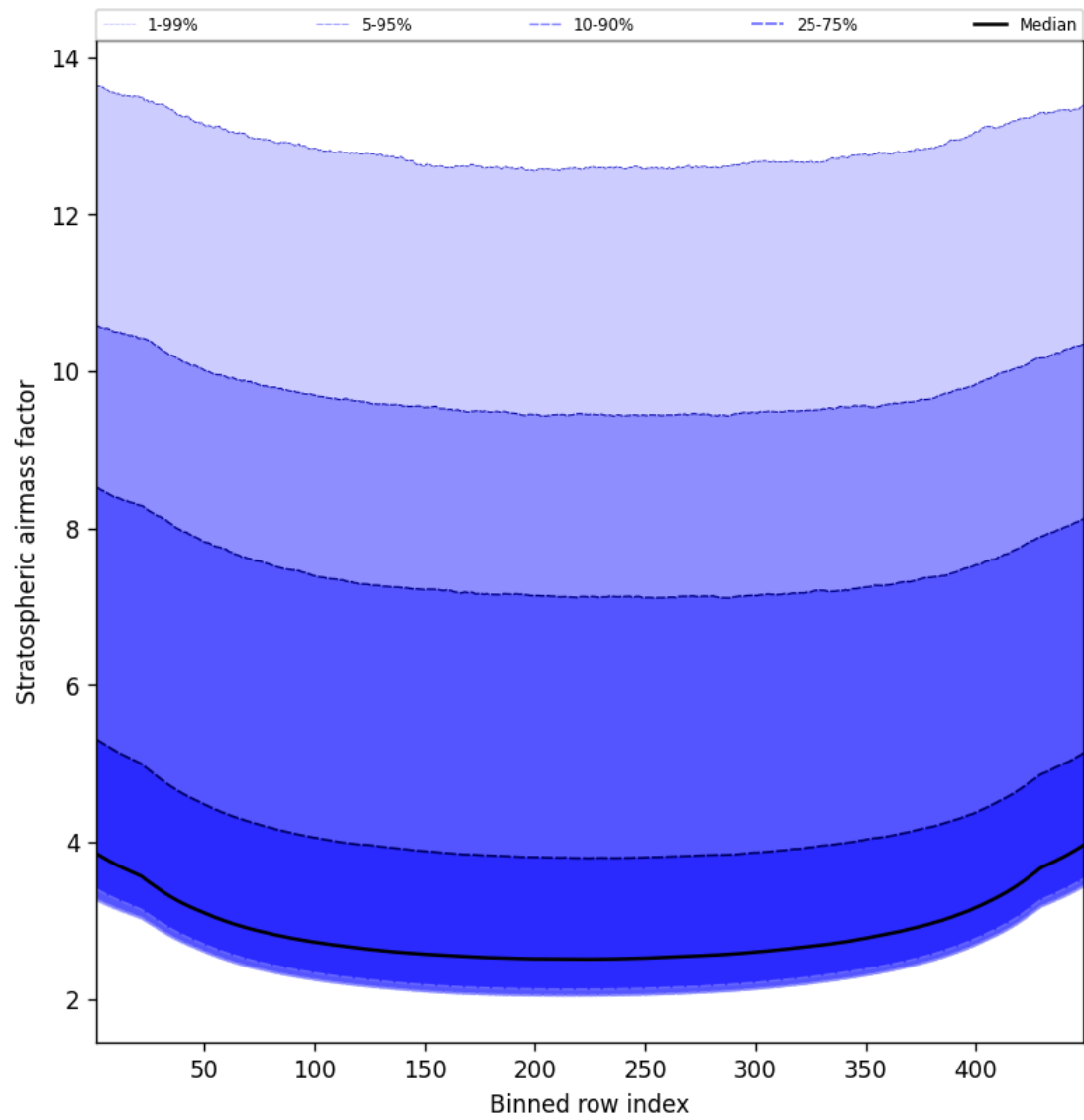
Figure 59: Along track statistics of “Stratospheric airmass factor” for 2025-08-27 to 2025-08-28
