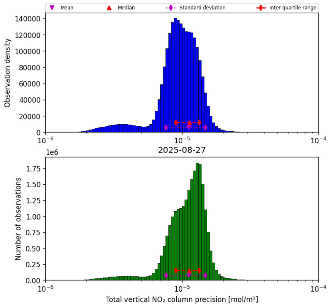
Figure 37: Histogram of “Total vertical NO 2 column precision” for 2025-08-27 to 2025-08-28
