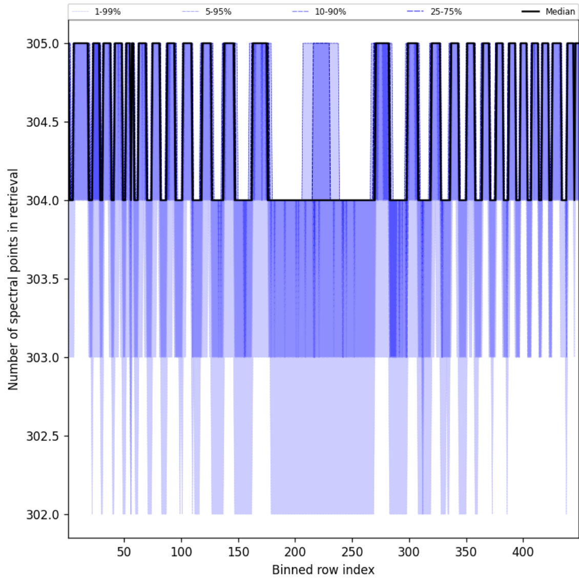
Figure 48: Along track statistics of “Number of spectral points in retrieval” for 2025-08-27 to 2025-08-28
