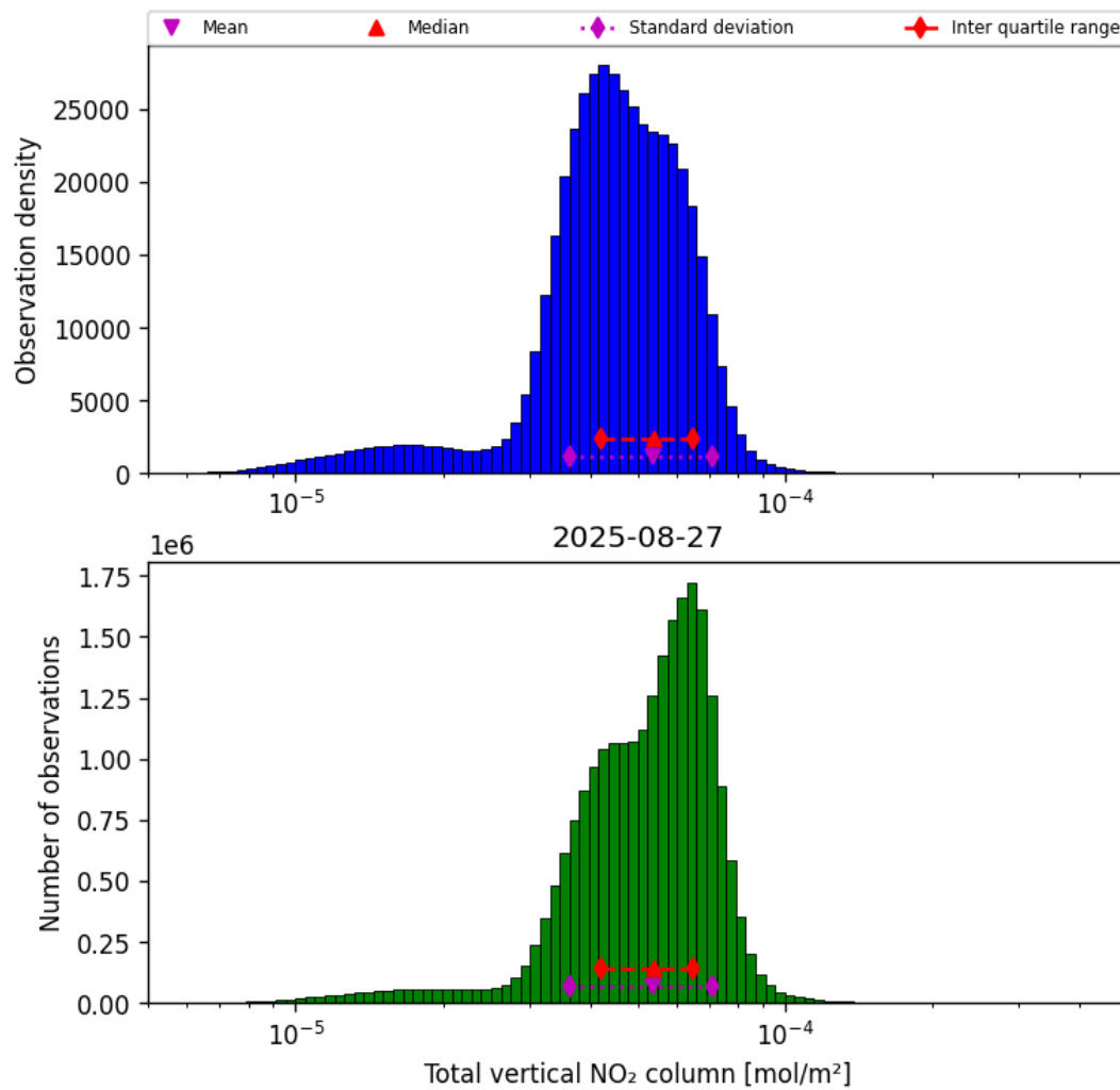
Figure 36: Histogram of “Total vertical NO 2 column” for 2025-08-27 to 2025-08-28
