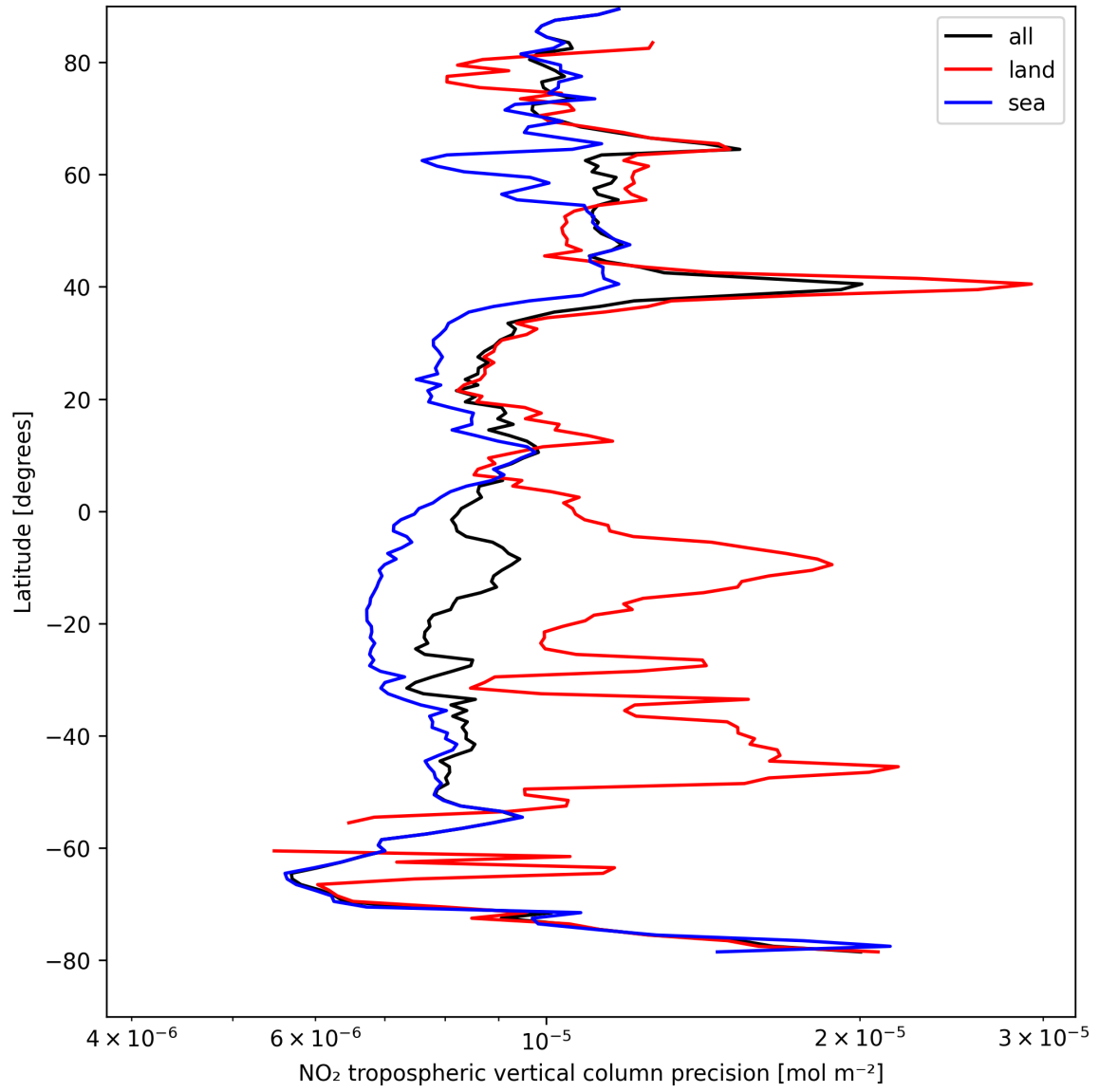
Figure 11: Zonal average of “NO 2 tropospheric vertical column precision” for 2025-08-27 to 2025-08-28.
