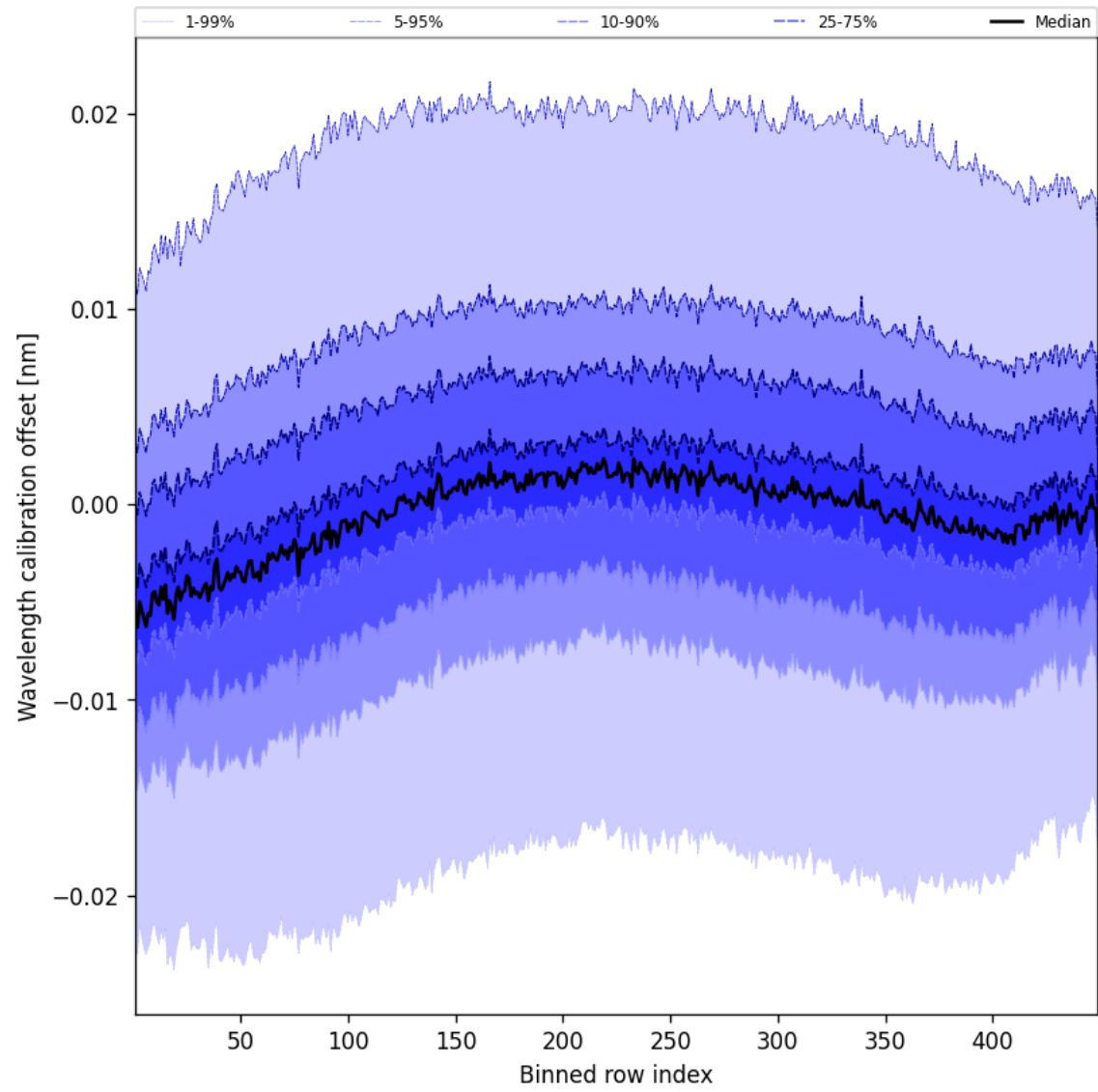
Figure 50: Along track statistics of “Wavelength calibration offset” for 2025-08-27 to 2025-08-28
