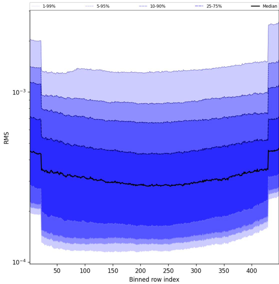
Figure 58: Along track statistics of “RMS” for 2025-08-27 to 2025-08-28
