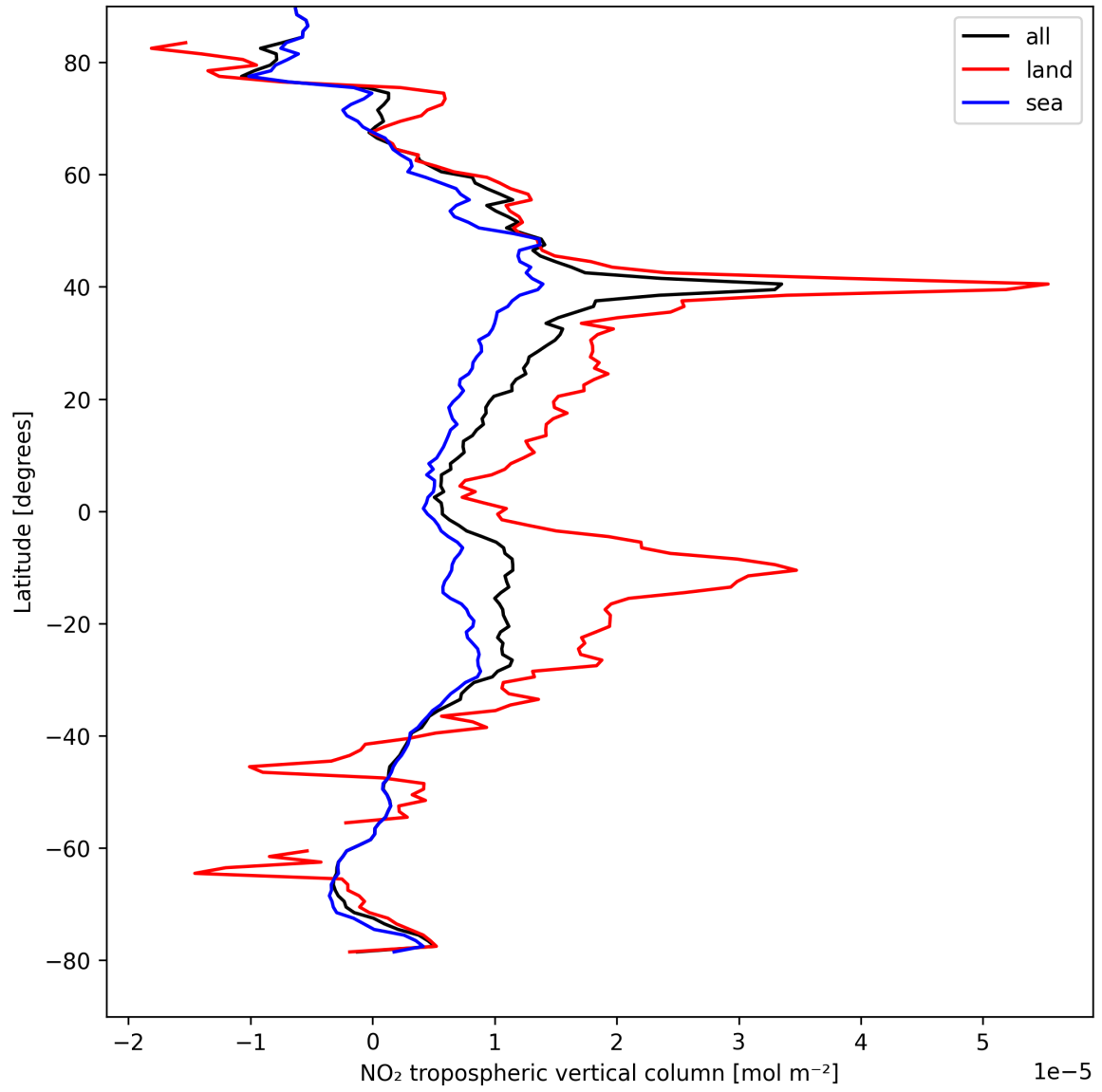
Figure 10: Zonal average of “NO 2 tropospheric vertical column” for 2025-08-27 to 2025-08-28.
