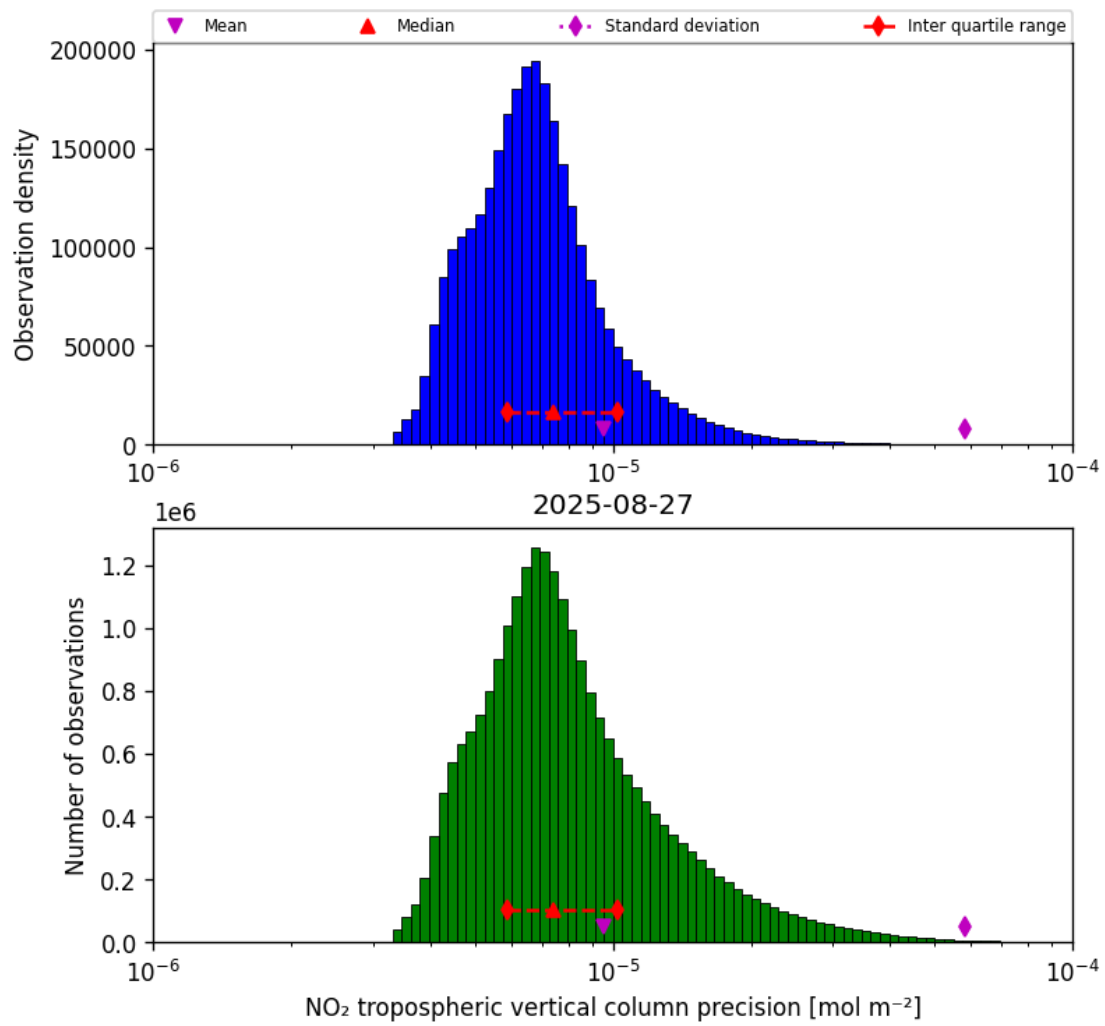
Figure 28: Histogram of “NO 2 tropospheric vertical column precision” for 2025-08-27 to 2025-08-28
