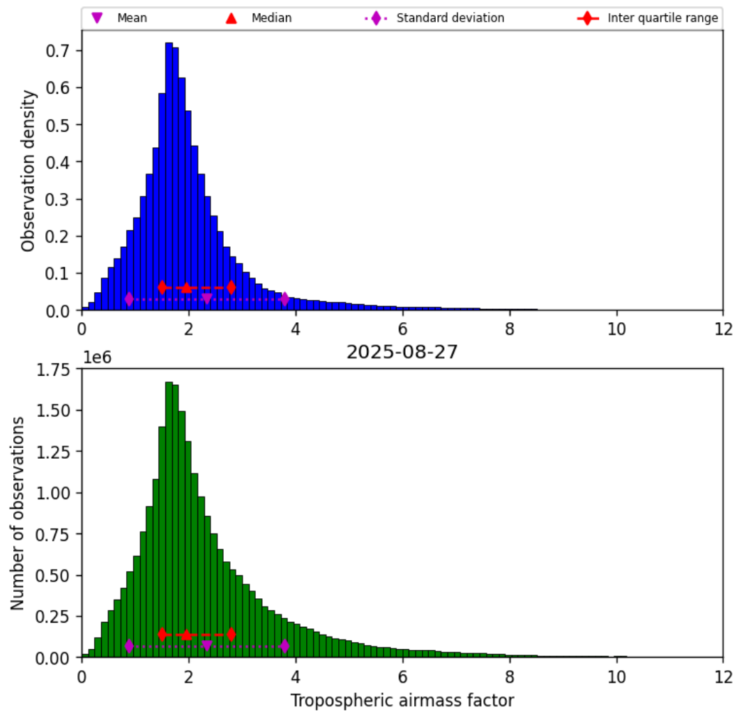
Figure 29: Histogram of “Tropospheric airmass factor” for 2025-08-27 to 2025-08-28
