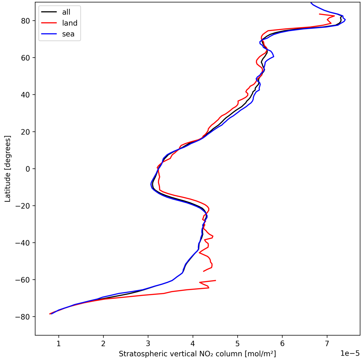
Figure 17: Zonal average of “Stratospheric vertical NO 2 column” for 2025-08-27 to 2025-08-28.
