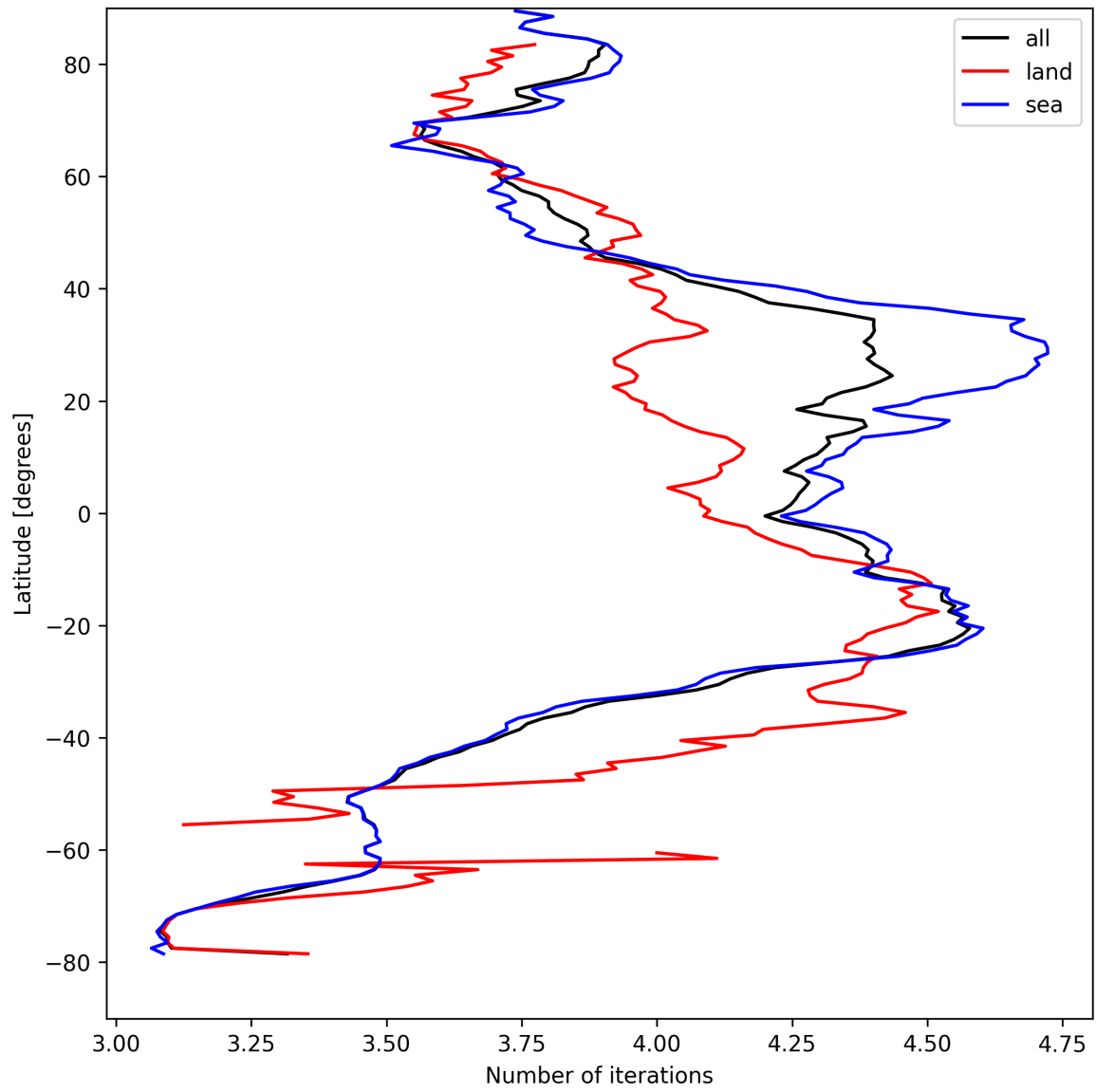
Figure 15: Zonal average of “Number of iterations” for 2025-08-27 to 2025-08-28.
