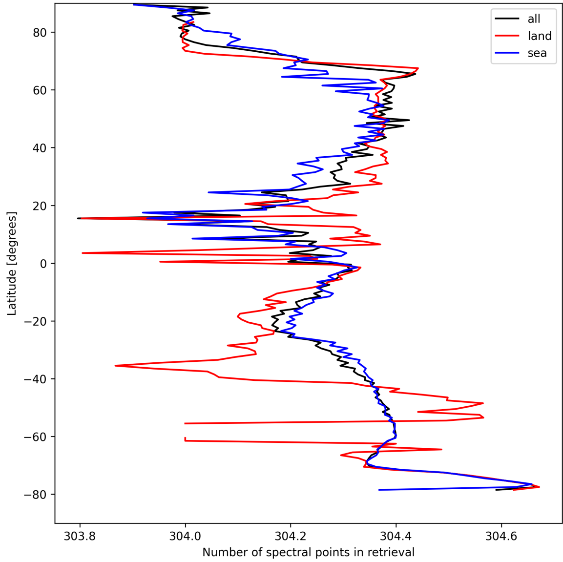
Figure 14: Zonal average of “Number of spectral points in retrieval” for 2025-08-27 to 2025-08-28.
