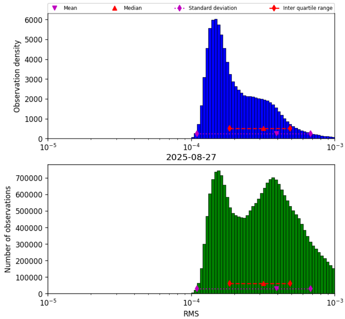
Figure 41: Histogram of “RMS” for 2025-08-27 to 2025-08-28
