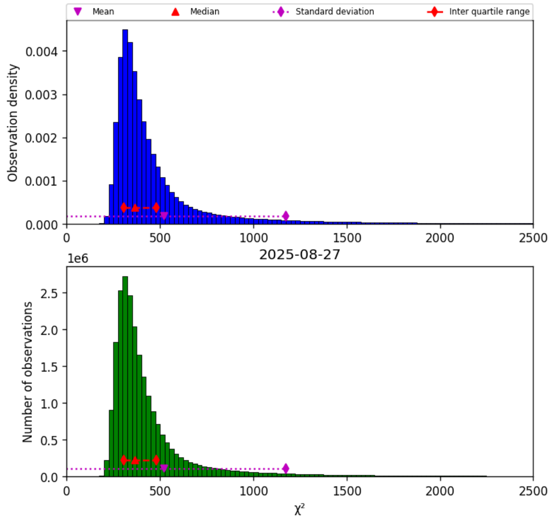
Figure 40: Histogram of “ \chi^2 ” for 2025-08-27 to 2025-08-28
