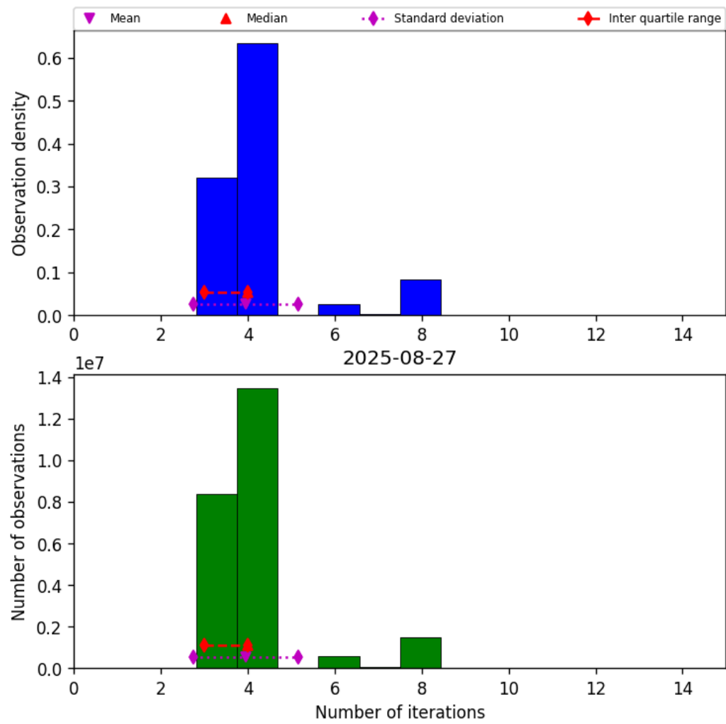
Figure 32: Histogram of “Number of iterations” for 2025-08-27 to 2025-08-28
