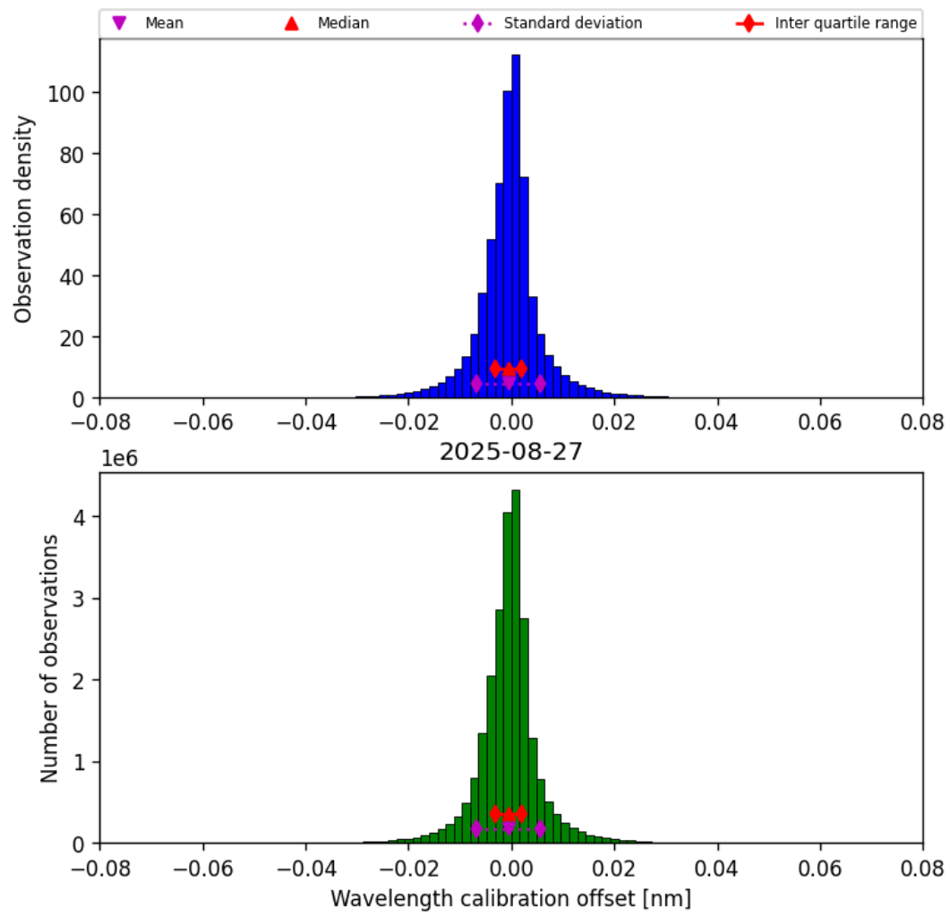
Figure 33: Histogram of “Wavelength calibration offset” for 2025-08-27 to 2025-08-28
