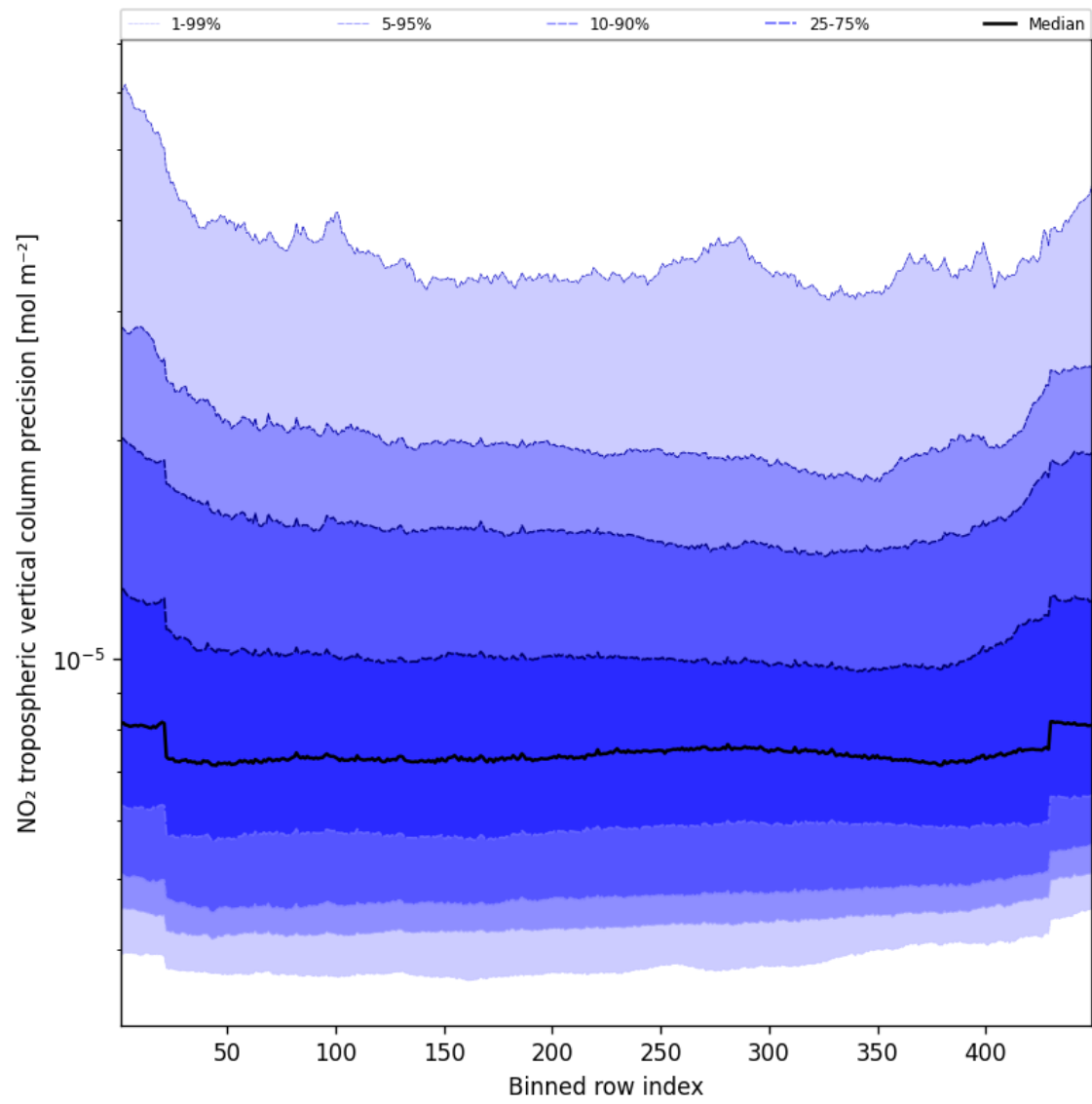
Figure 45: Along track statistics of “NO 2 tropospheric vertical column precision” for 2025-08-27 to 2025-08-28
