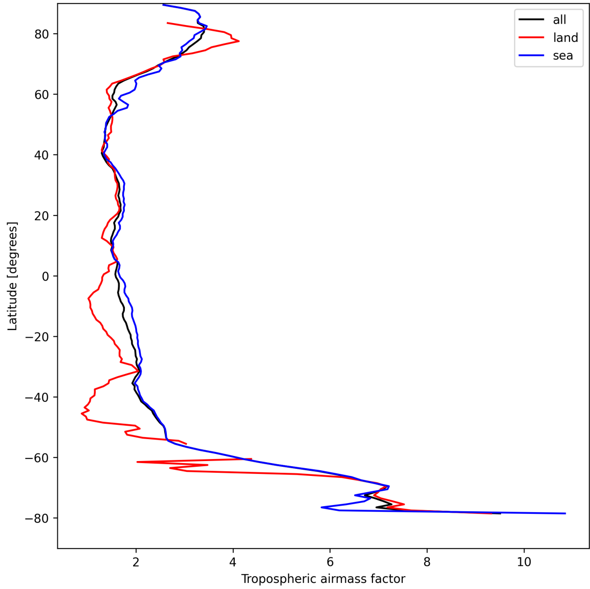
Figure 12: Zonal average of “Tropospheric airmass factor” for 2025-08-27 to 2025-08-28.
