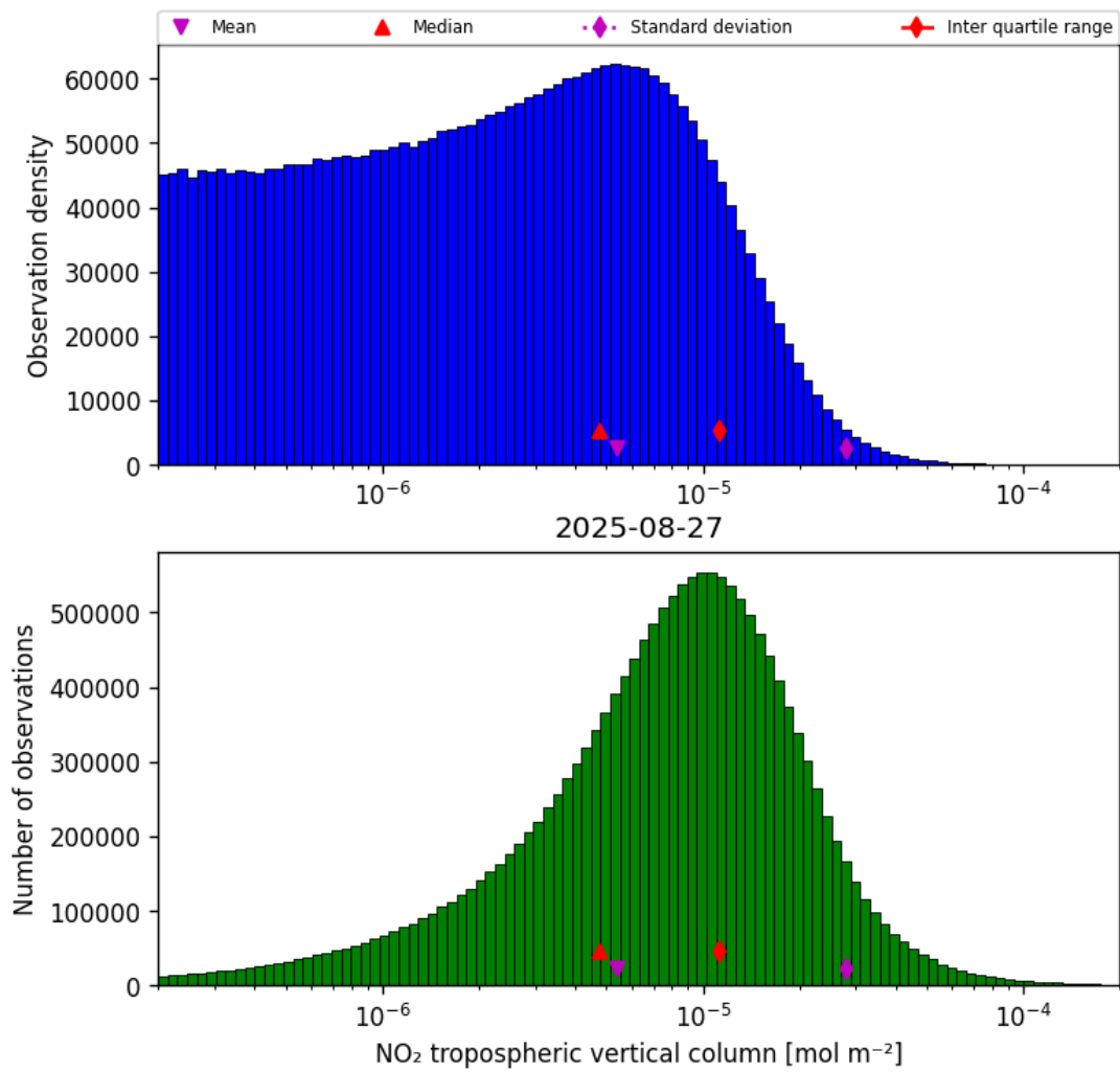
Figure 27: Histogram of “NO 2 tropospheric vertical column” for 2025-08-27 to 2025-08-28
