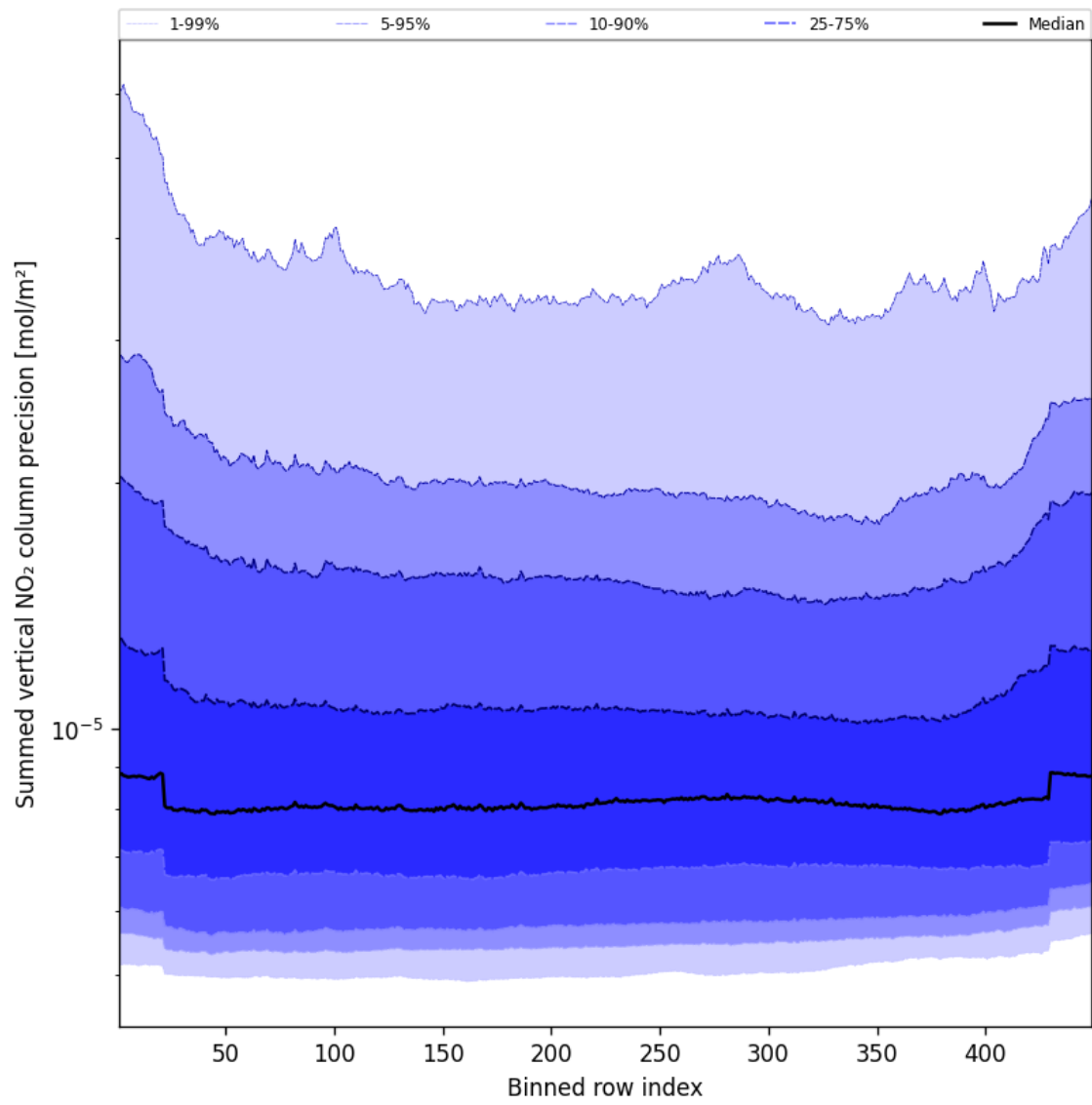
Figure 56: Along track statistics of “Summed vertical NO 2 column precision” for 2025-08-27 to 2025-08-28
