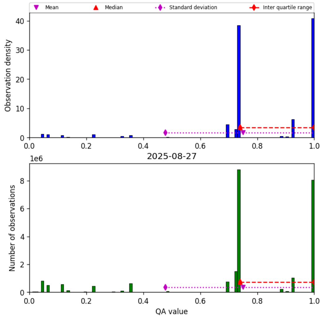
Figure 26: Histogram of “QA value” for 2025-08-27 to 2025-08-28
