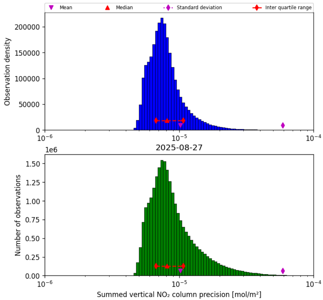
Figure 39: Histogram of “Summed vertical NO 2 column precision” for 2025-08-27 to 2025-08-28
