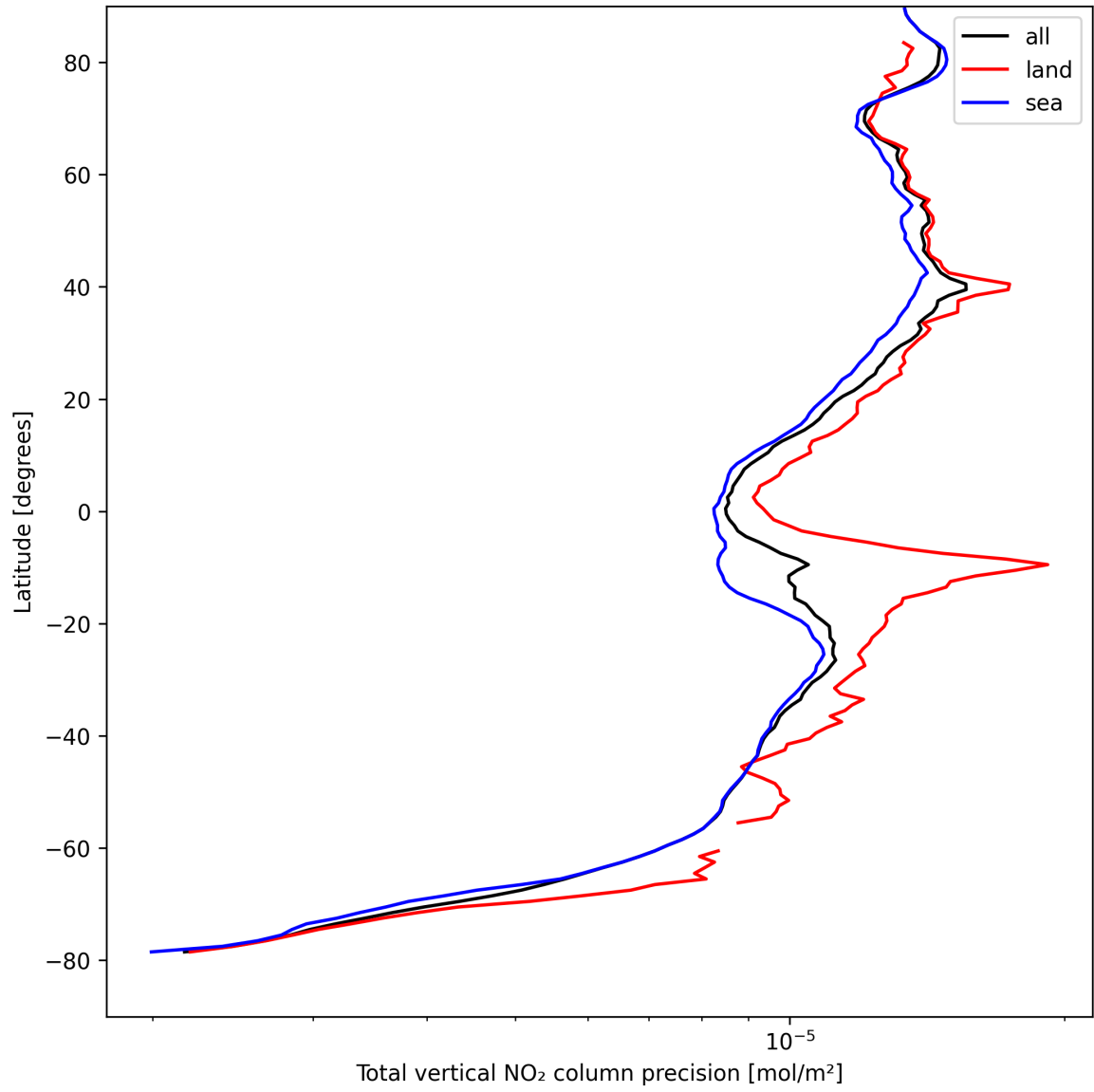
Figure 20: Zonal average of “Total vertical NO 2 column precision” for 2025-08-27 to 2025-08-28.
