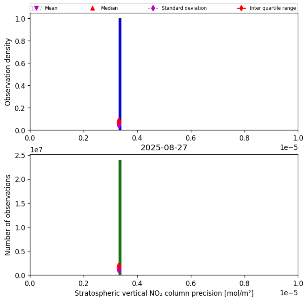
Figure 35: Histogram of “Stratospheric vertical NO 2 column precision” for 2025-08-27 to 2025-08-28
