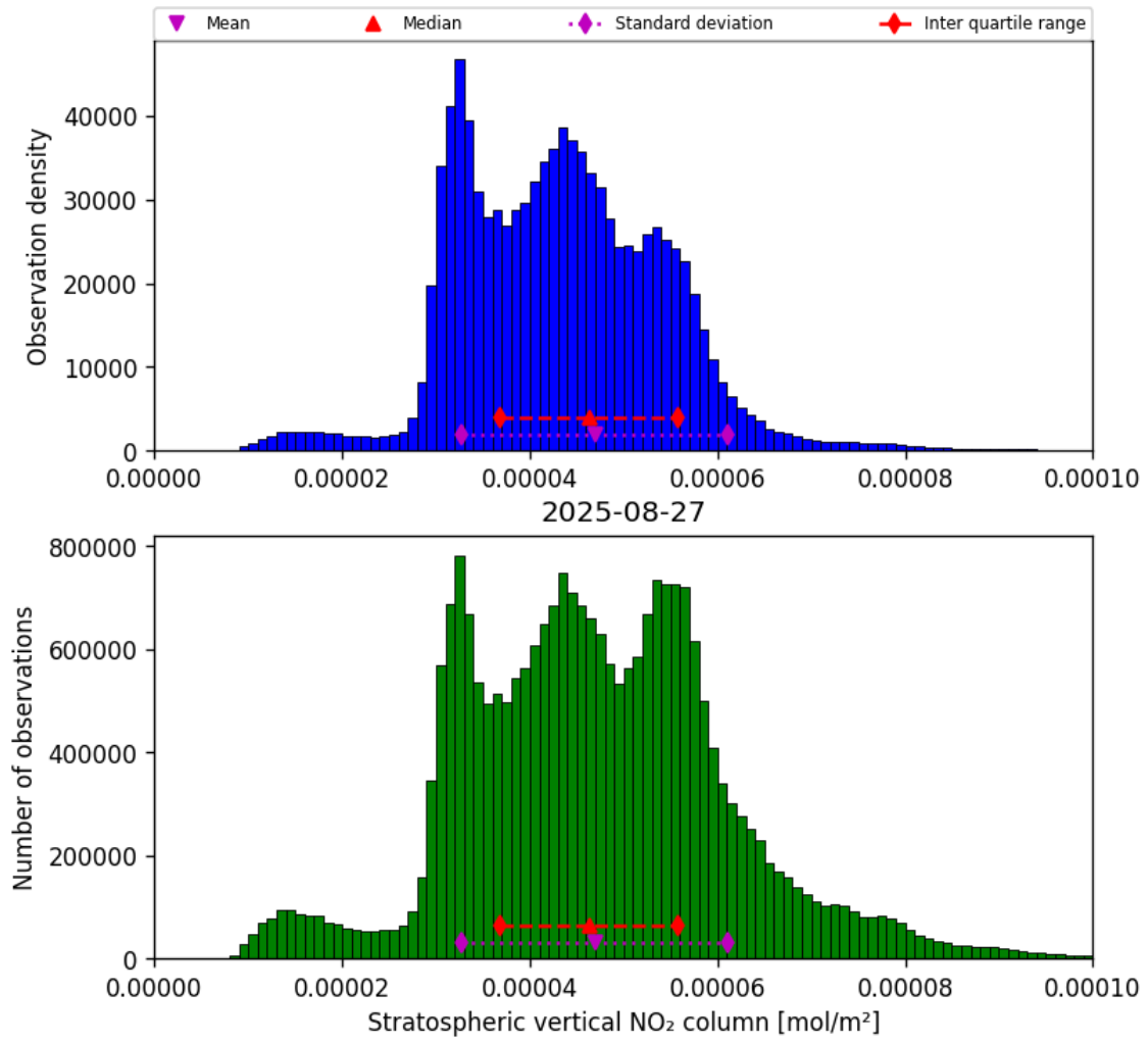
Figure 34: Histogram of “Stratospheric vertical NO 2 column” for 2025-08-27 to 2025-08-28
