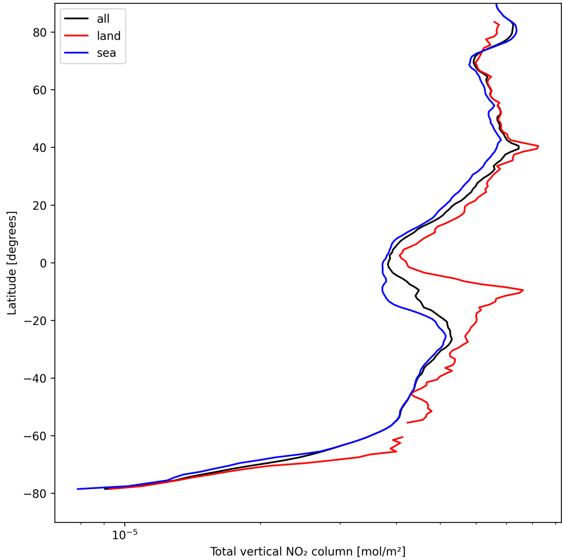
Figure 19: Zonal average of “Total vertical NO 2 column” for 2025-08-27 to 2025-08-28.
