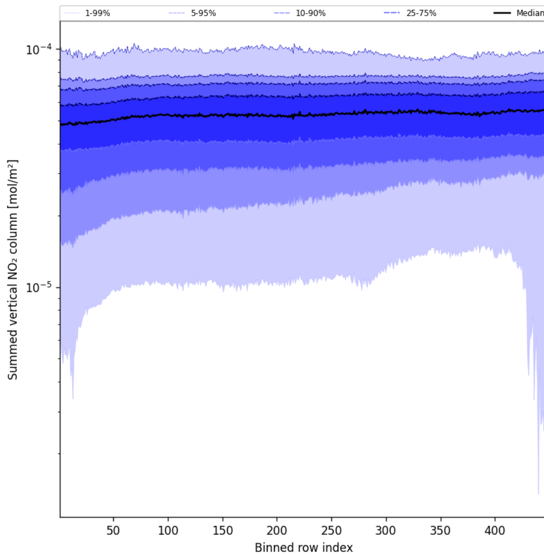
Figure 55: Along track statistics of “Summed vertical NO 2 column” for 2025-08-27 to 2025-08-28
