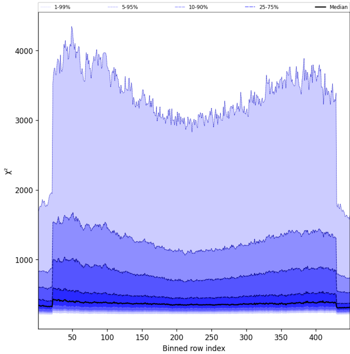
Figure 57: Along track statistics of “ \chi^2 ” for 2025-08-27 to 2025-08-28
