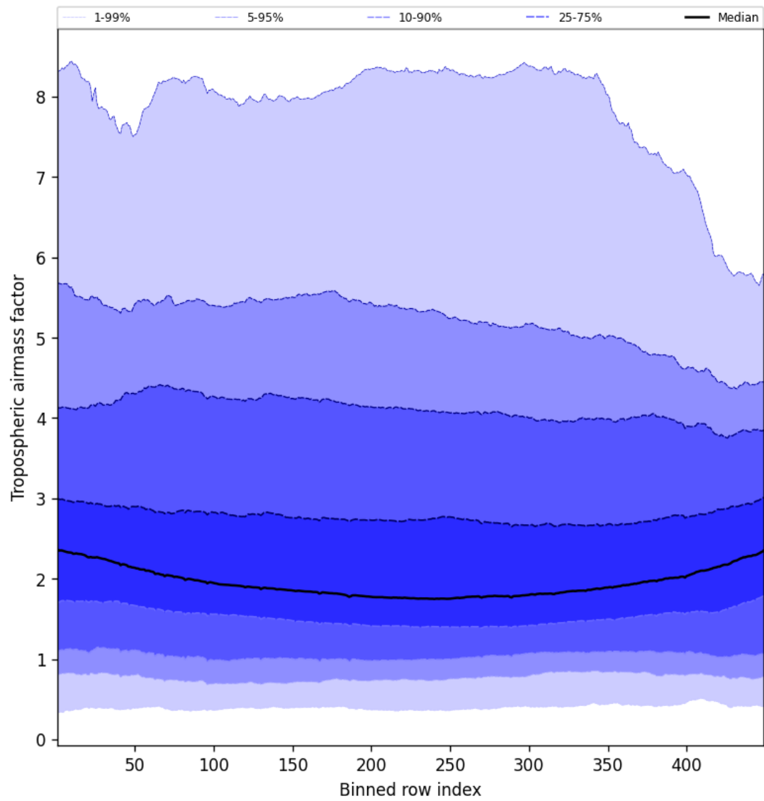
Figure 46: Along track statistics of “Tropospheric airmass factor” for 2025-08-27 to 2025-08-28
