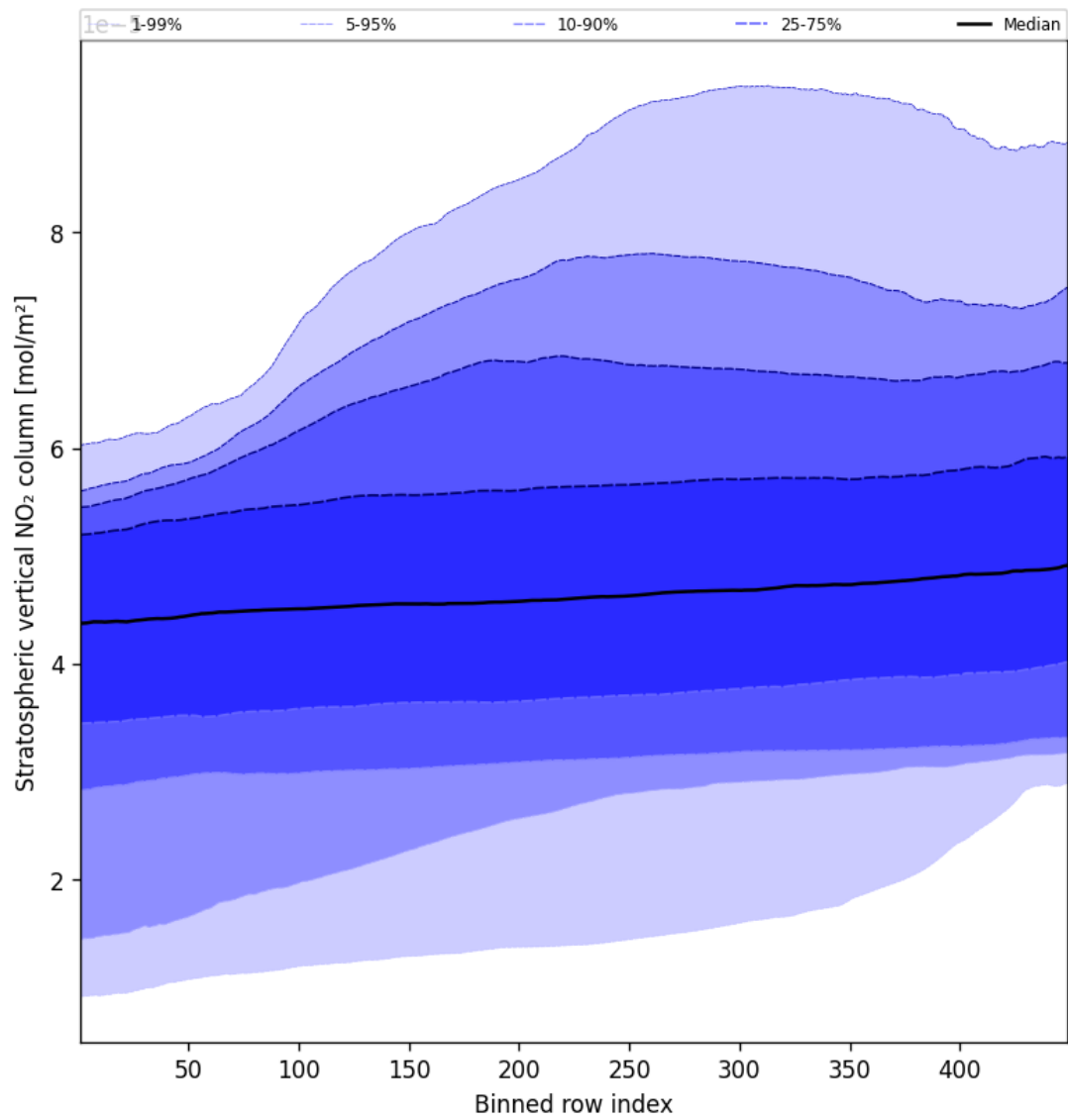
Figure 51: Along track statistics of “Stratospheric vertical NO 2 column” for 2025-08-27 to 2025-08-28
