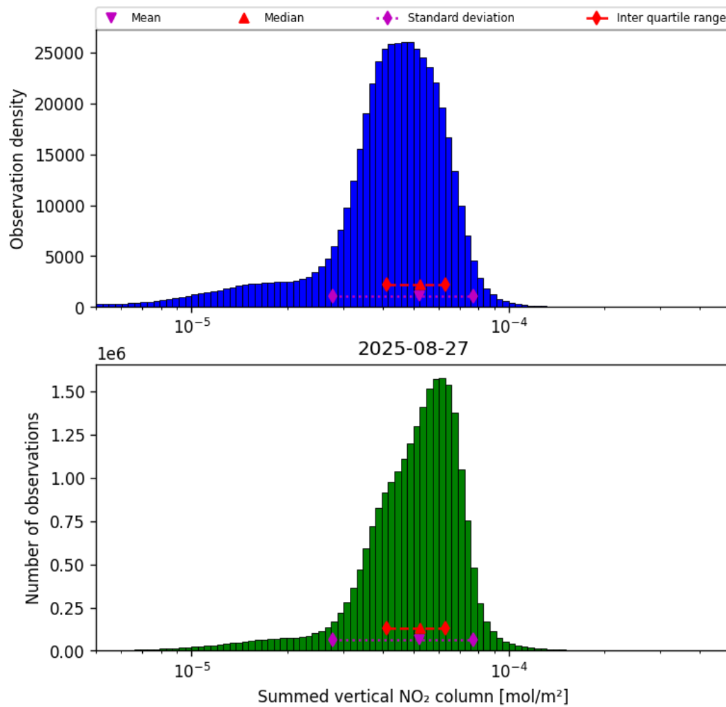
Figure 38: Histogram of “Summed vertical NO 2 column” for 2025-08-27 to 2025-08-28
