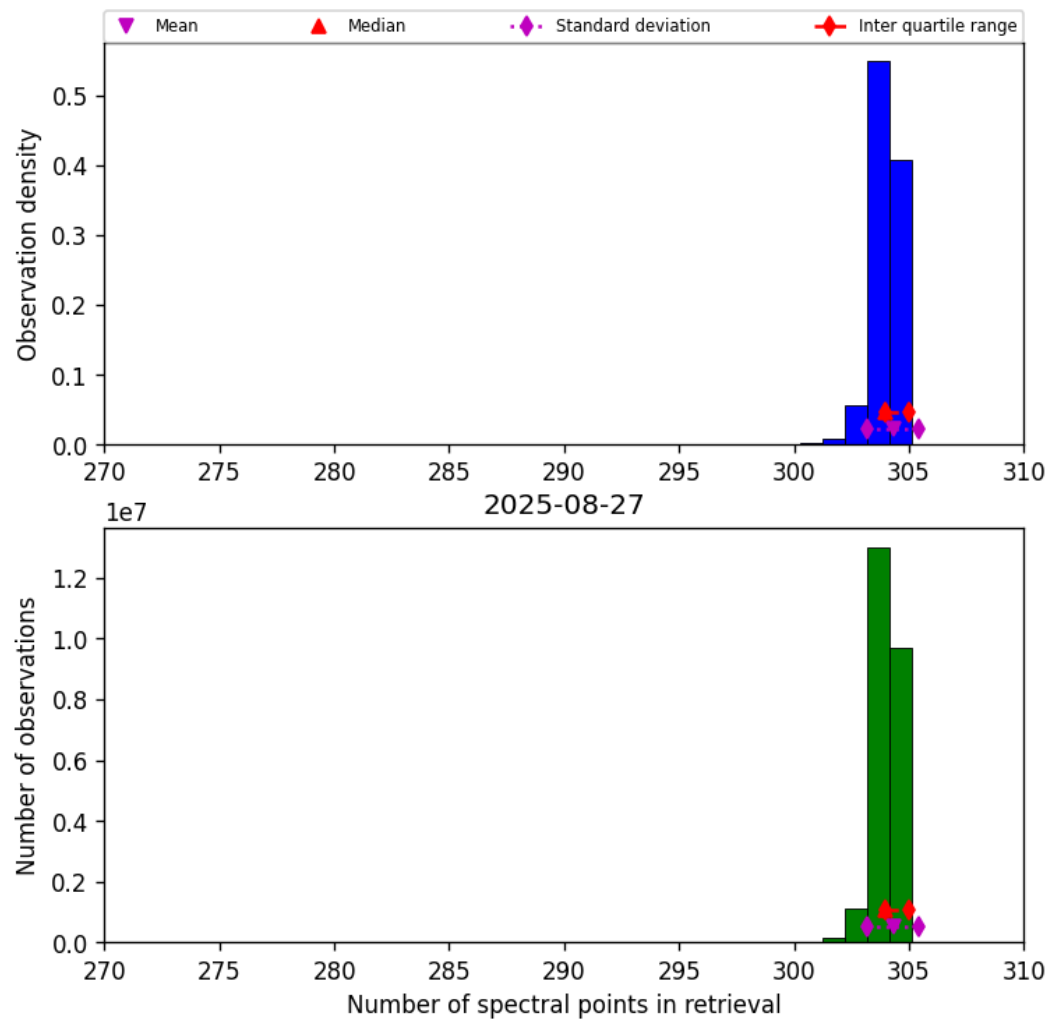
Figure 31: Histogram of “Number of spectral points in retrieval” for 2025-08-27 to 2025-08-28
