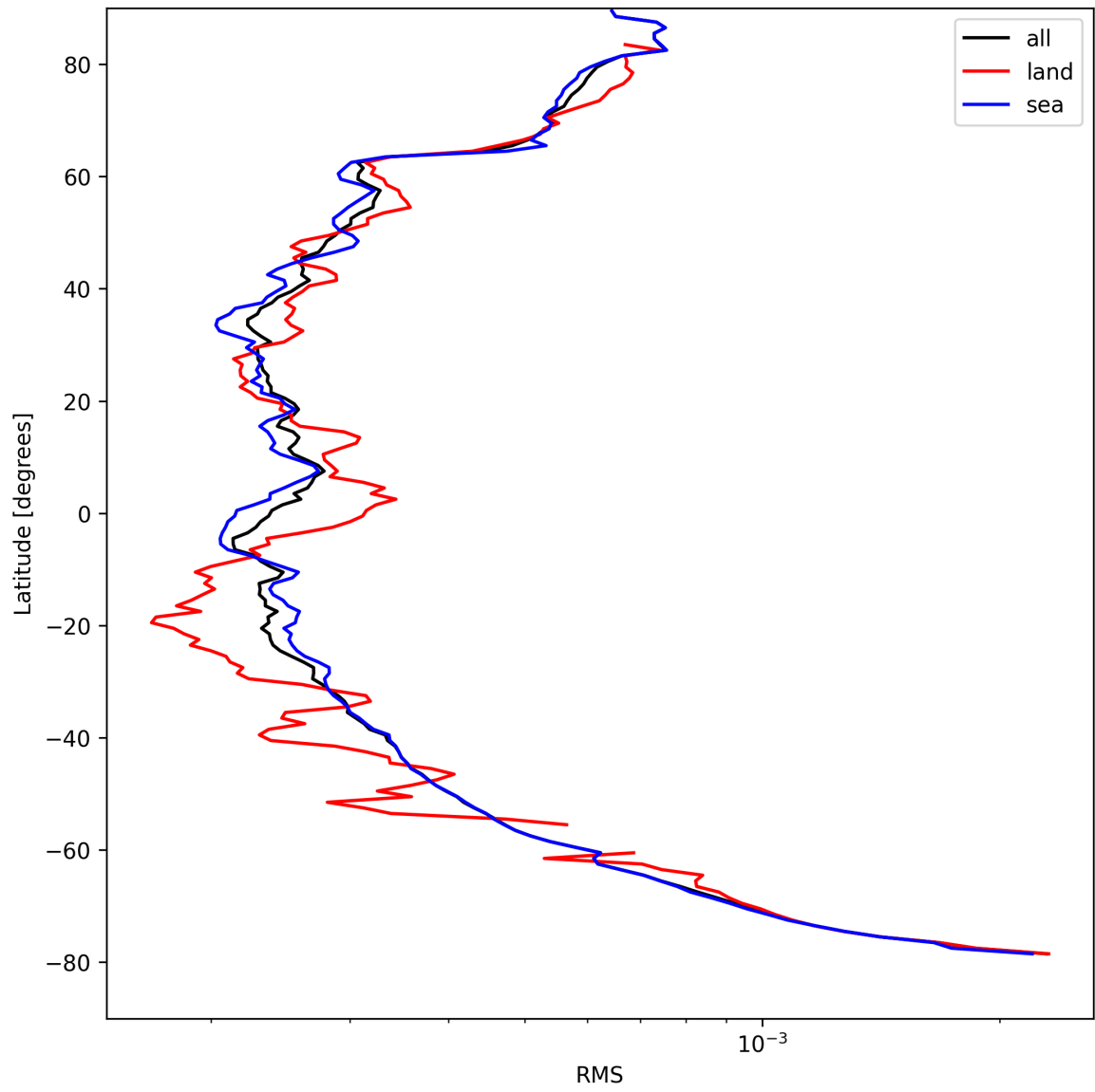
Figure 24: Zonal average of “RMS” for 2025-08-27 to 2025-08-28.
