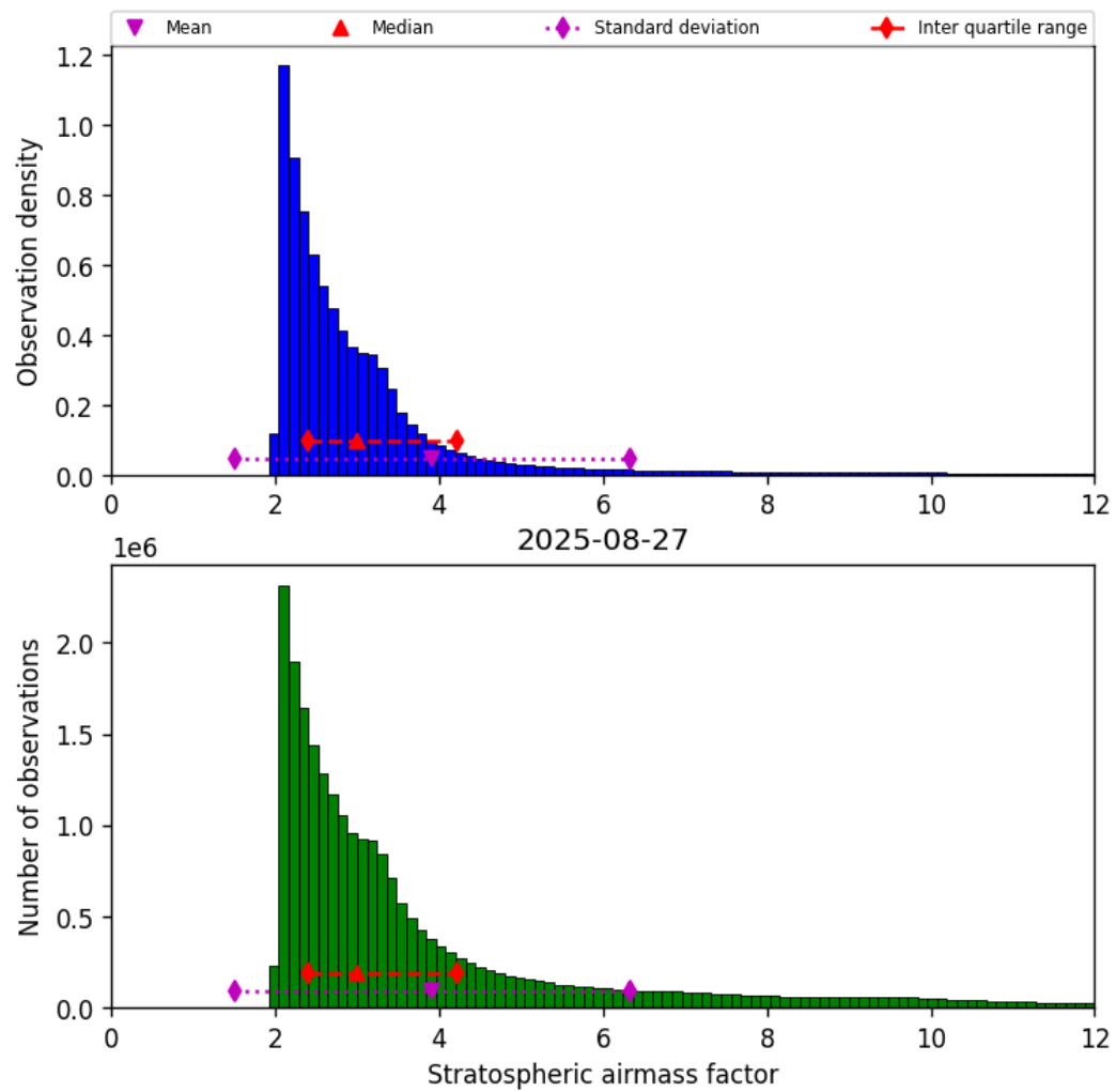
Figure 42: Histogram of “Stratospheric airmass factor” for 2025-08-27 to 2025-08-28
