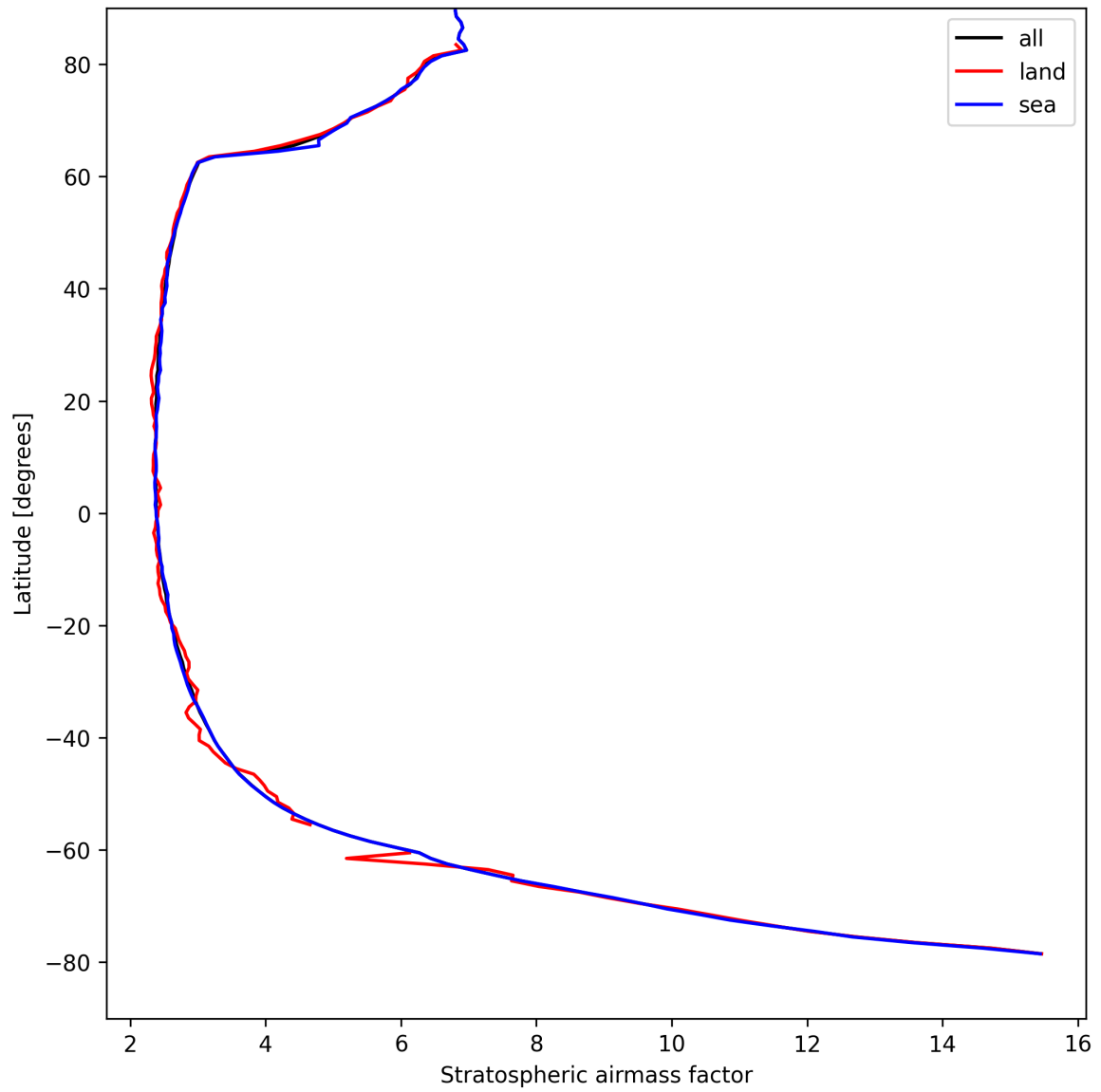
Figure 25: Zonal average of “Stratospheric airmass factor” for 2025-08-27 to 2025-08-28.
