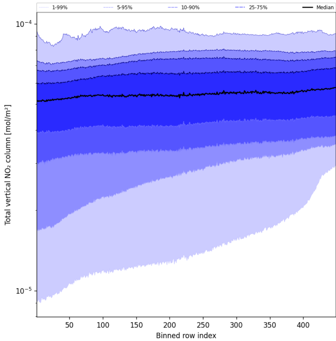
Figure 53: Along track statistics of “Total vertical NO 2 column” for 2025-08-27 to 2025-08-28
