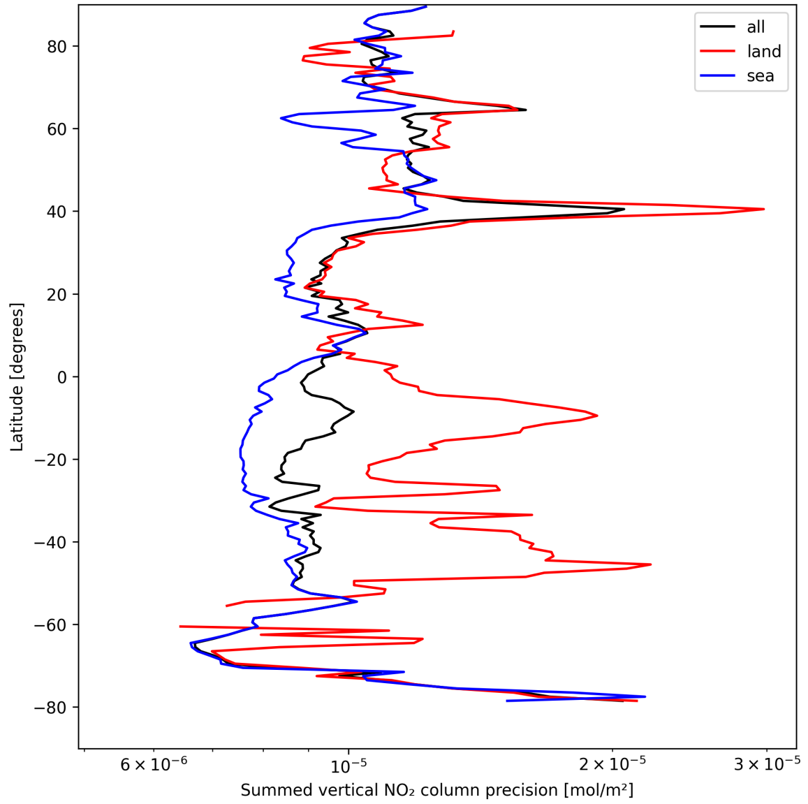
Figure 22: Zonal average of “Summed vertical NO 2 column precision” for 2025-08-27 to 2025-08-28.
