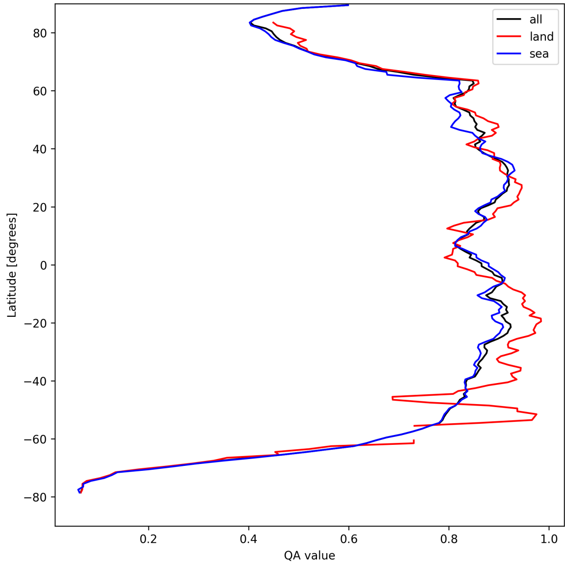
Figure 9: Zonal average of “QA value” for 2025-08-27 to 2025-08-28.
