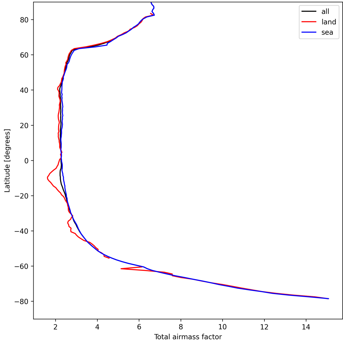
Figure 13: Zonal average of “Total airmass factor” for 2025-08-27 to 2025-08-28.
