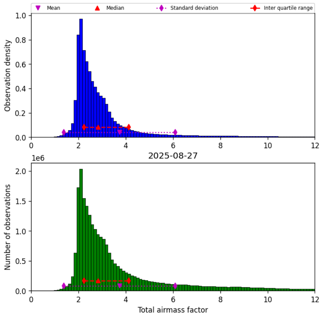
Figure 30: Histogram of “Total airmass factor” for 2025-08-27 to 2025-08-28
