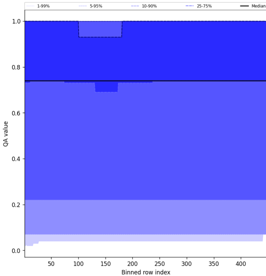
Figure 43: Along track statistics of “QA value” for 2025-08-27 to 2025-08-28
