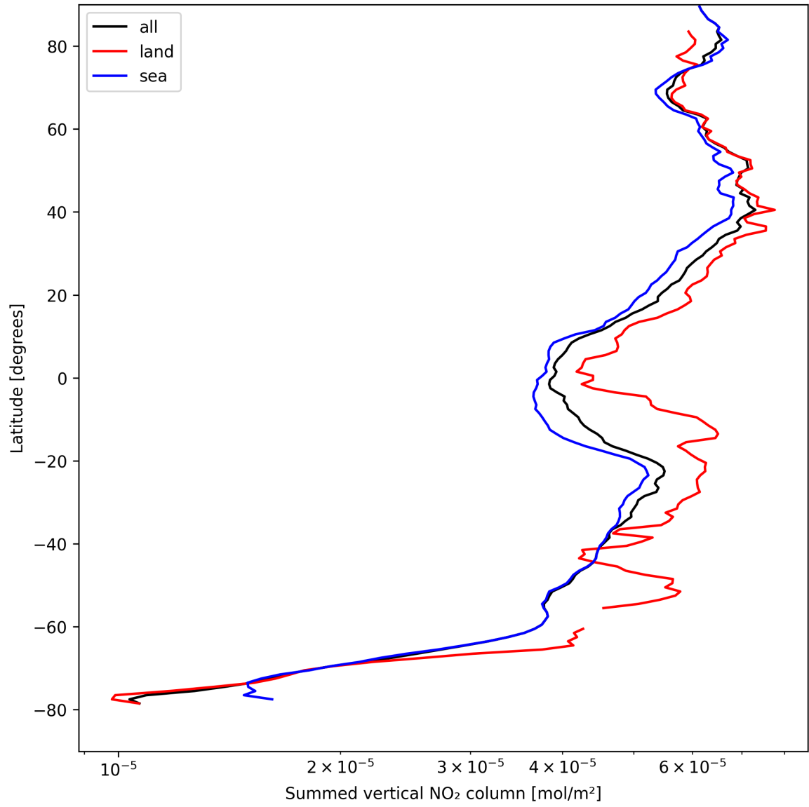
Figure 21: Zonal average of “Summed vertical NO 2 column” for 2025-08-28 to 2025-08-28.
