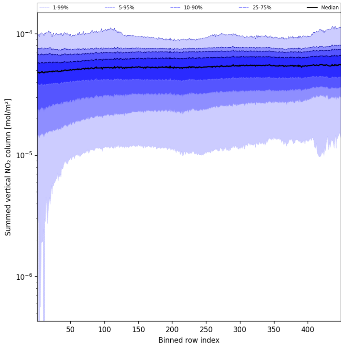
Figure 55: Along track statistics of “Summed vertical NO 2 column” for 2025-08-28 to 2025-08-28
