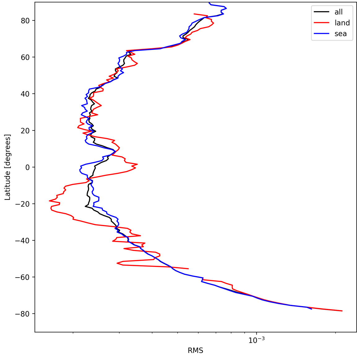
Figure 24: Zonal average of “RMS” for 2025-08-28 to 2025-08-28.
