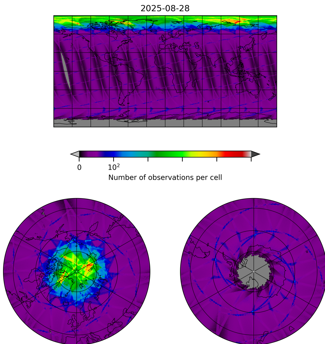
Figure 8: Map of the number of observations for 2025-08-28 to 2025-08-28
