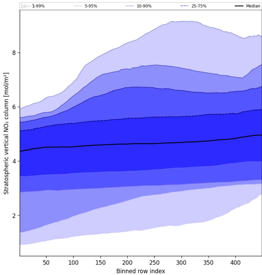
Figure 51: Along track statistics of “Stratospheric vertical NO 2 column” for 2025-08-28 to 2025-08-28
