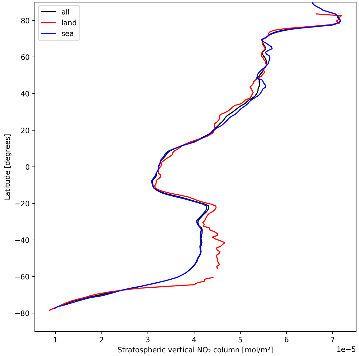
Figure 17: Zonal average of “Stratospheric vertical NO 2 column” for 2025-08-28 to 2025-08-28.
