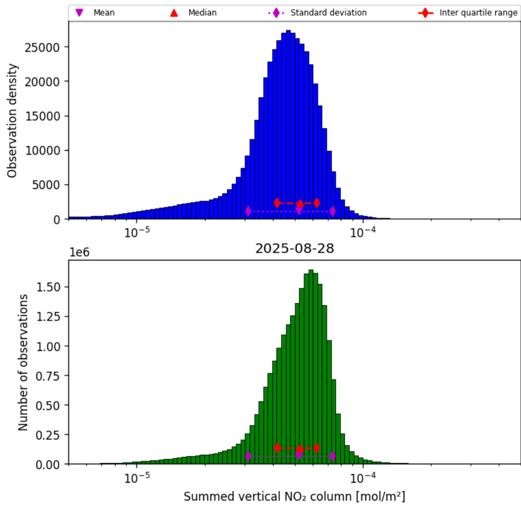
Figure 38: Histogram of “Summed vertical NO 2 column” for 2025-08-28 to 2025-08-28
