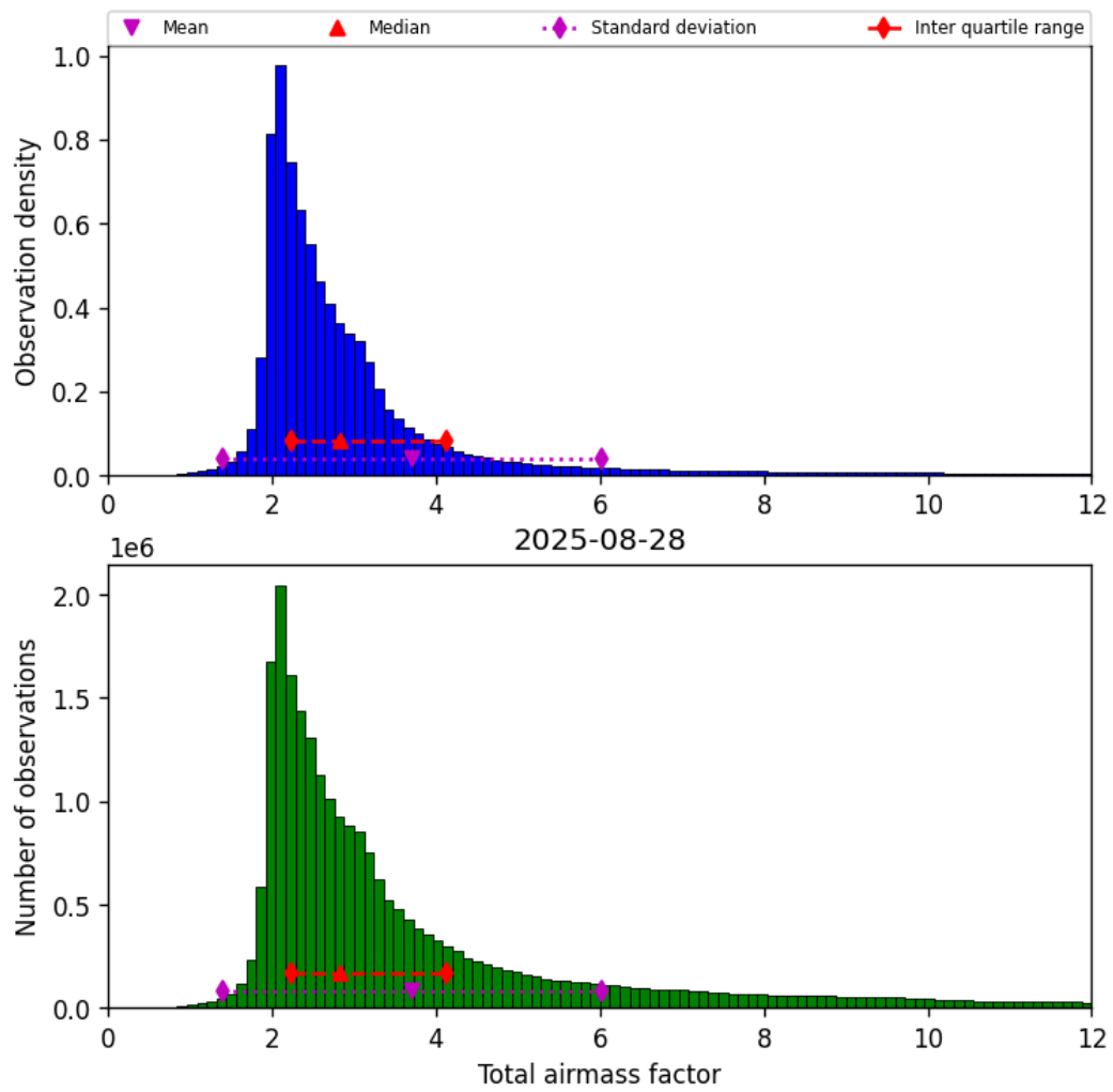
Figure 30: Histogram of “Total airmass factor” for 2025-08-28 to 2025-08-28
