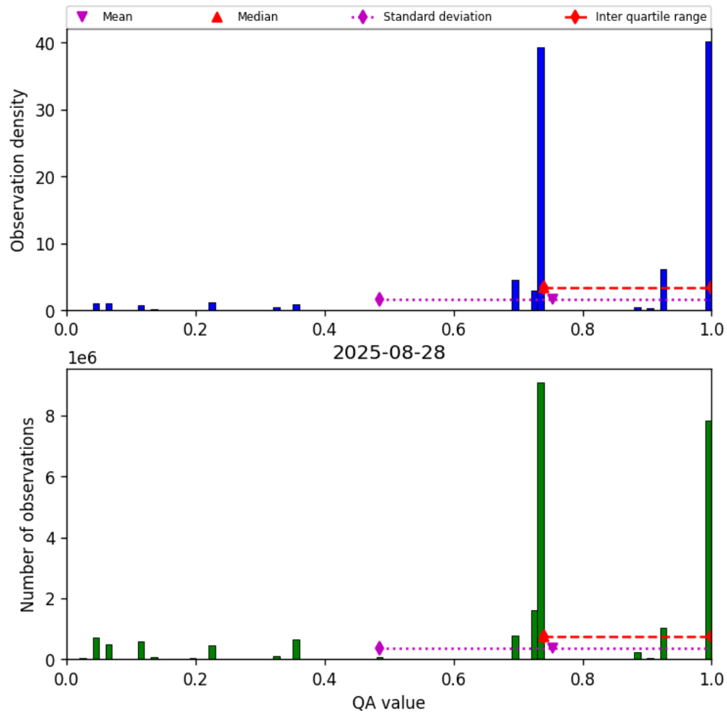
Figure 26: Histogram of “QA value” for 2025-08-28 to 2025-08-28
