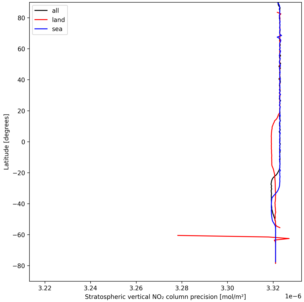
Figure 18: Zonal average of “Stratospheric vertical NO 2 column precision” for 2025-08-28 to 2025-08-28.
