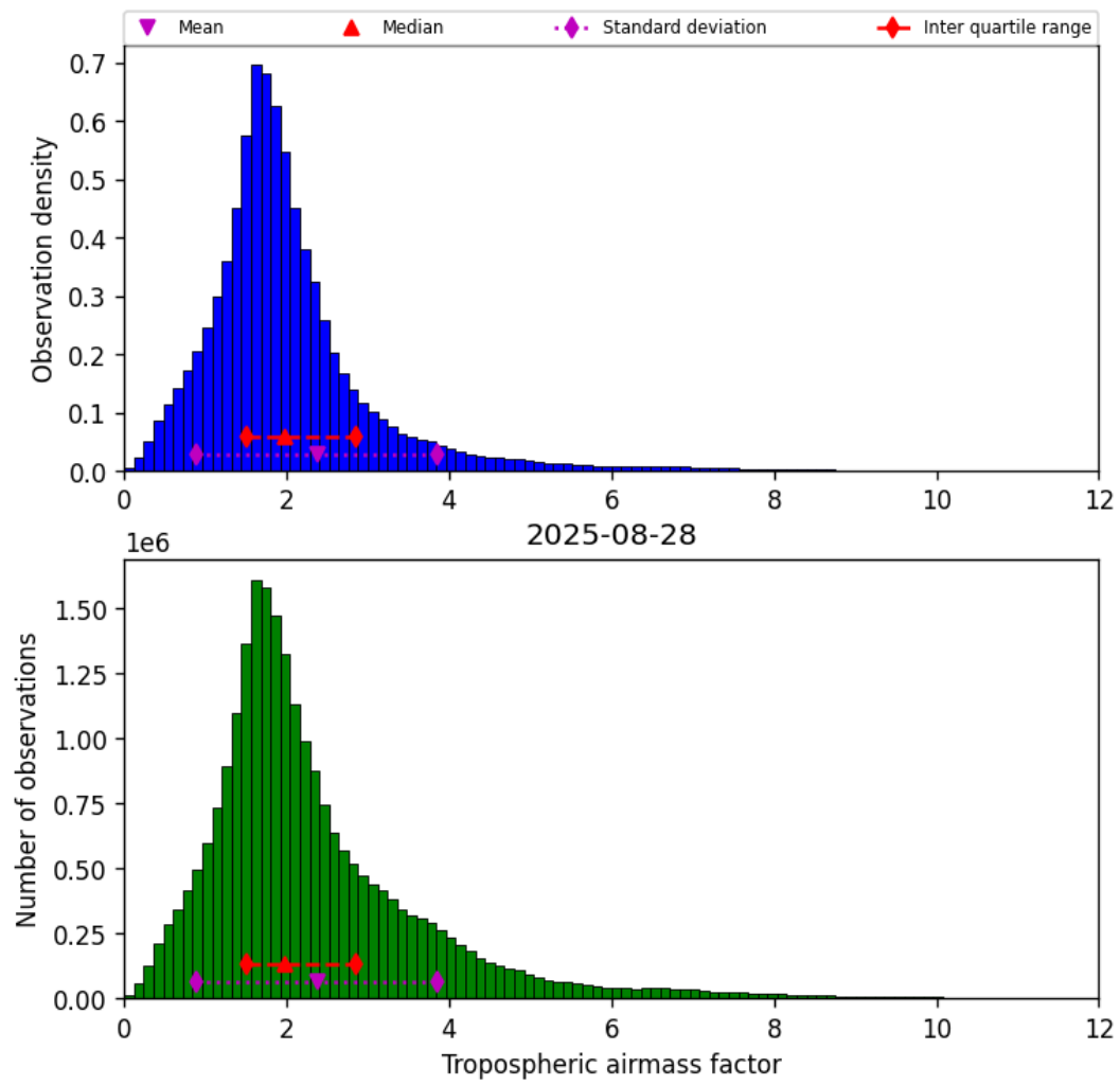
Figure 29: Histogram of “Tropospheric airmass factor” for 2025-08-28 to 2025-08-28
