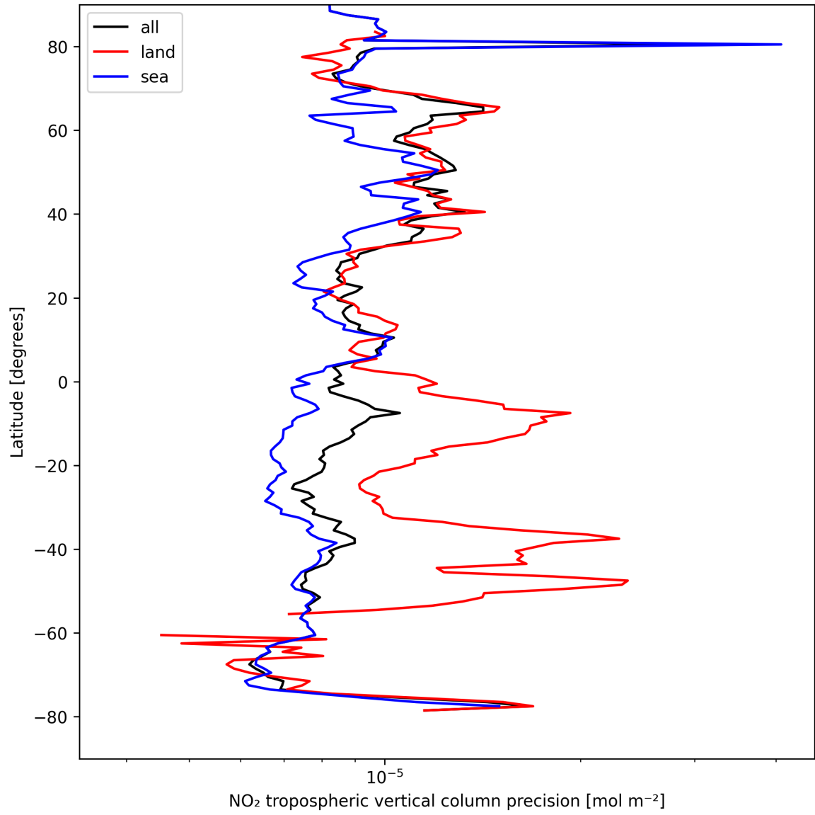
Figure 11: Zonal average of “NO 2 tropospheric vertical column precision” for 2025-08-28 to 2025-08-28.
