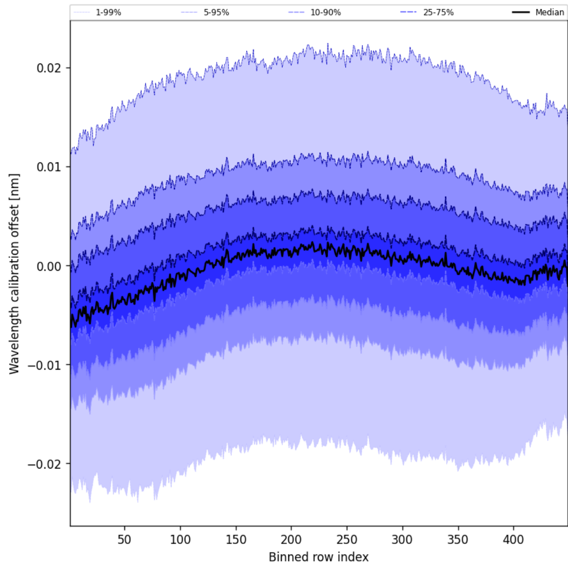
Figure 50: Along track statistics of “Wavelength calibration offset” for 2025-08-28 to 2025-08-28
