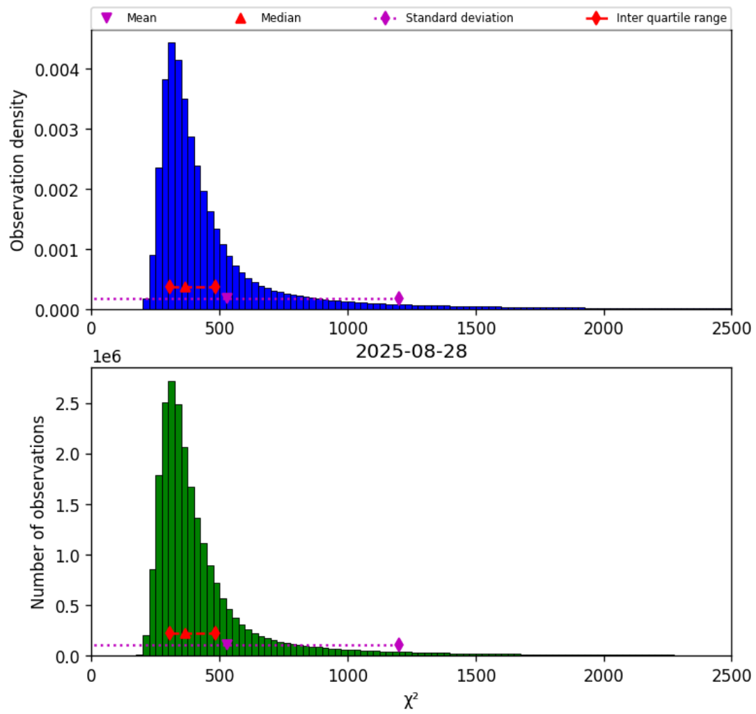
Figure 40: Histogram of “ \chi^2 ” for 2025-08-28 to 2025-08-28
