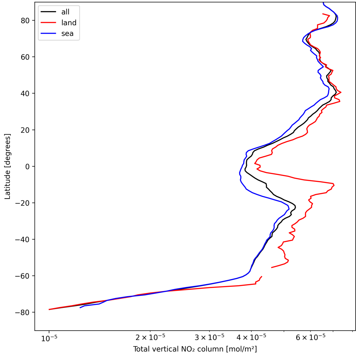
Figure 19: Zonal average of “Total vertical NO 2 column” for 2025-08-28 to 2025-08-28.
