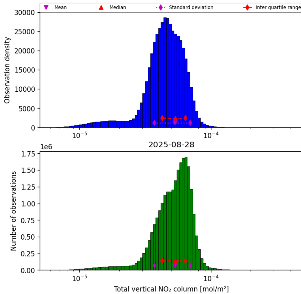
Figure 36: Histogram of “Total vertical NO 2 column” for 2025-08-28 to 2025-08-28
