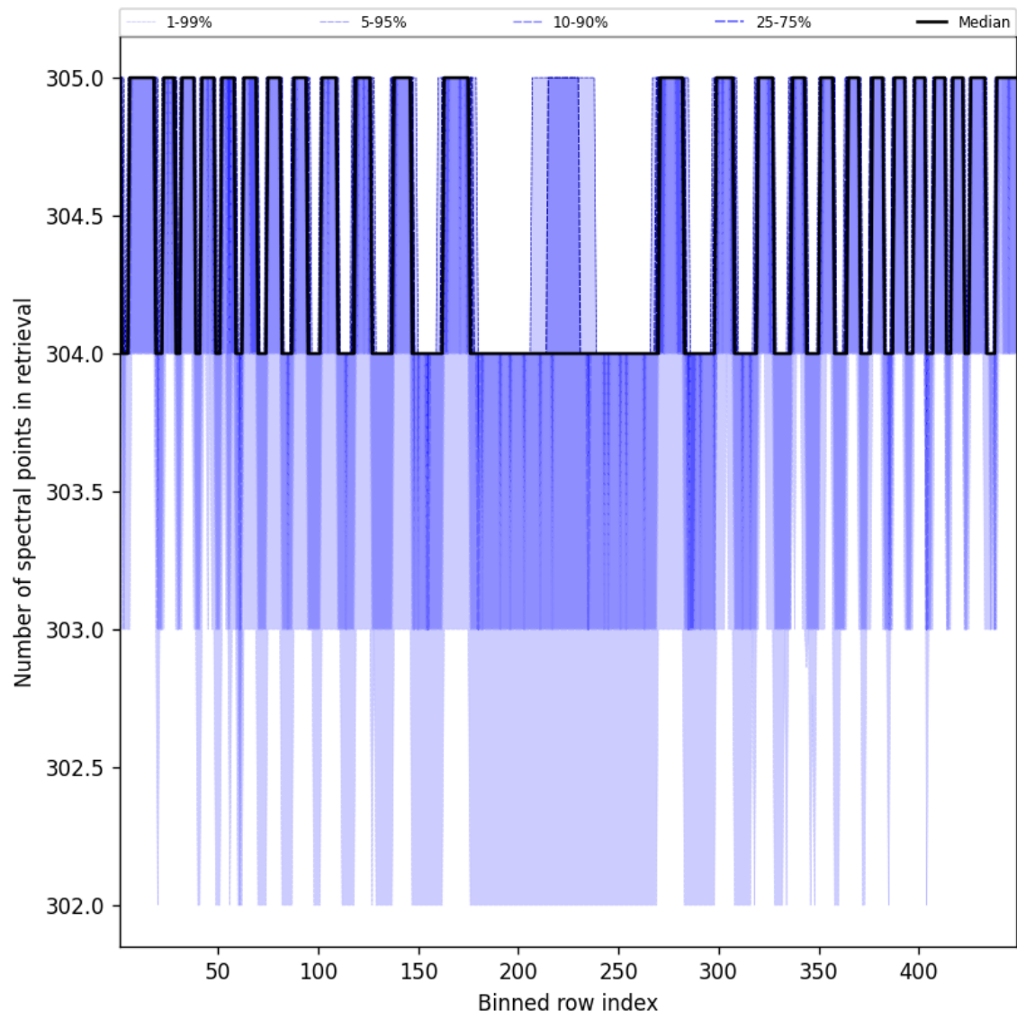
Figure 48: Along track statistics of “Number of spectral points in retrieval” for 2025-08-28 to 2025-08-28
