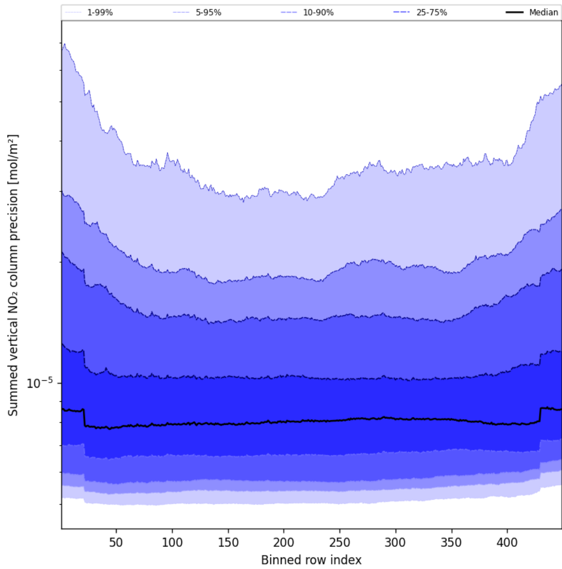
Figure 56: Along track statistics of “Summed vertical NO 2 column precision” for 2025-08-28 to 2025-08-28
