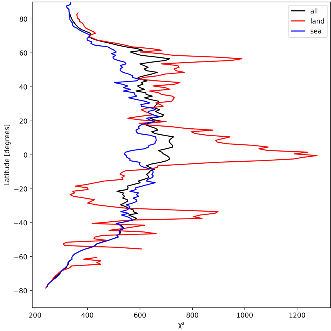
Figure 23: Zonal average of “ \chi^2 ” for 2025-08-28 to 2025-08-28.
