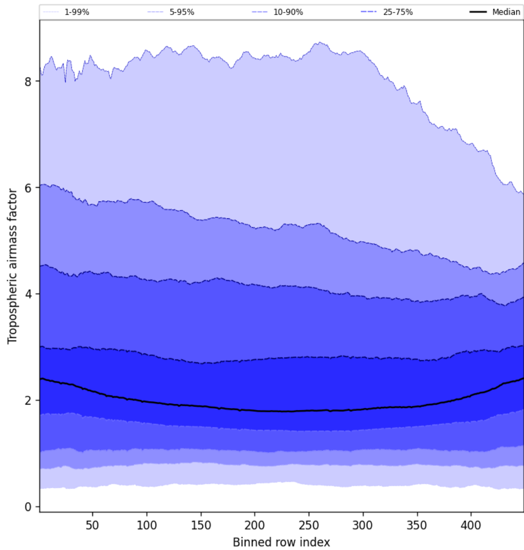
Figure 46: Along track statistics of “Tropospheric air mass factor” for 2025-08-28 to 2025-08-28
