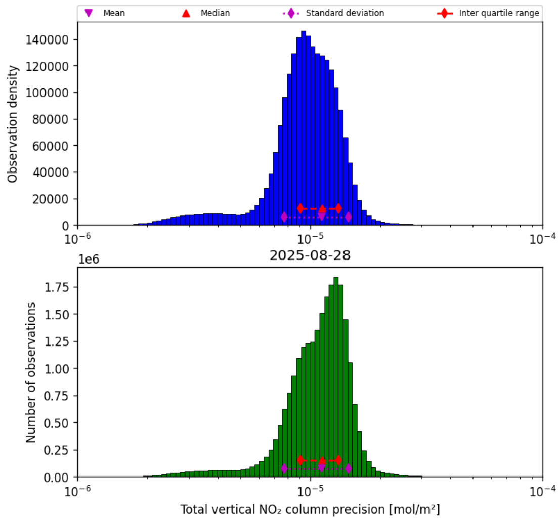
Figure 37: Histogram of "Total vertical NO 2 column precision" for 2025-08-28 to 2025-08-28
