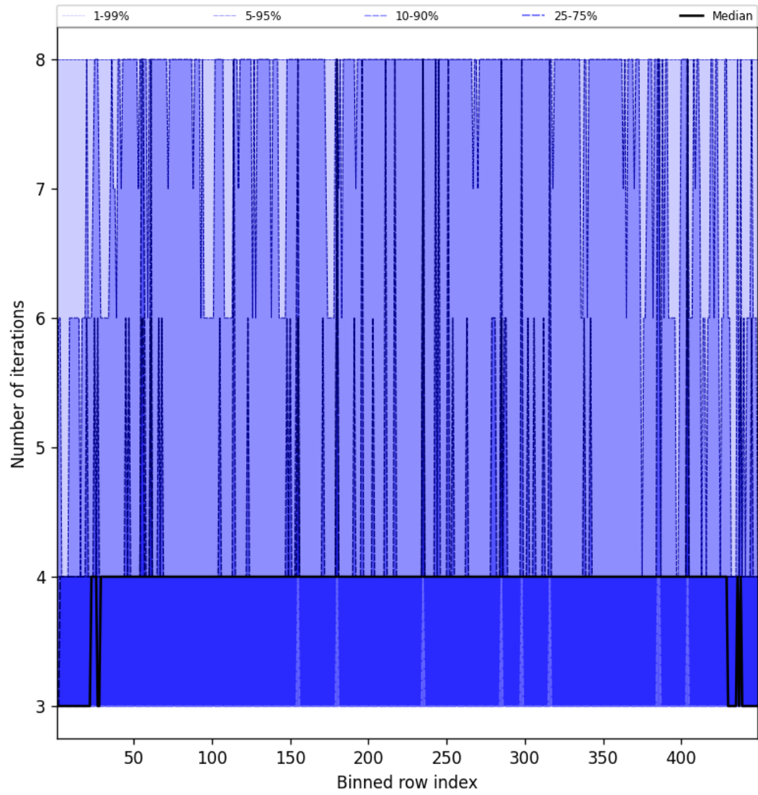
Figure 49: Along track statistics of “Number of iterations” for 2025-08-28 to 2025-08-28
