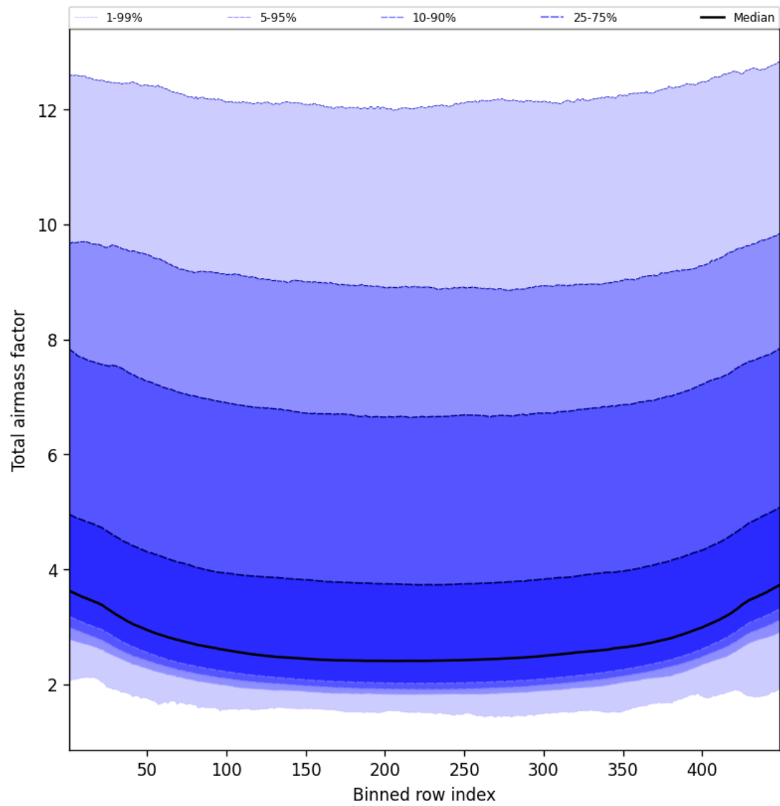
Figure 47: Along track statistics of “Total airmass factor” for 2025-08-28 to 2025-08-28
