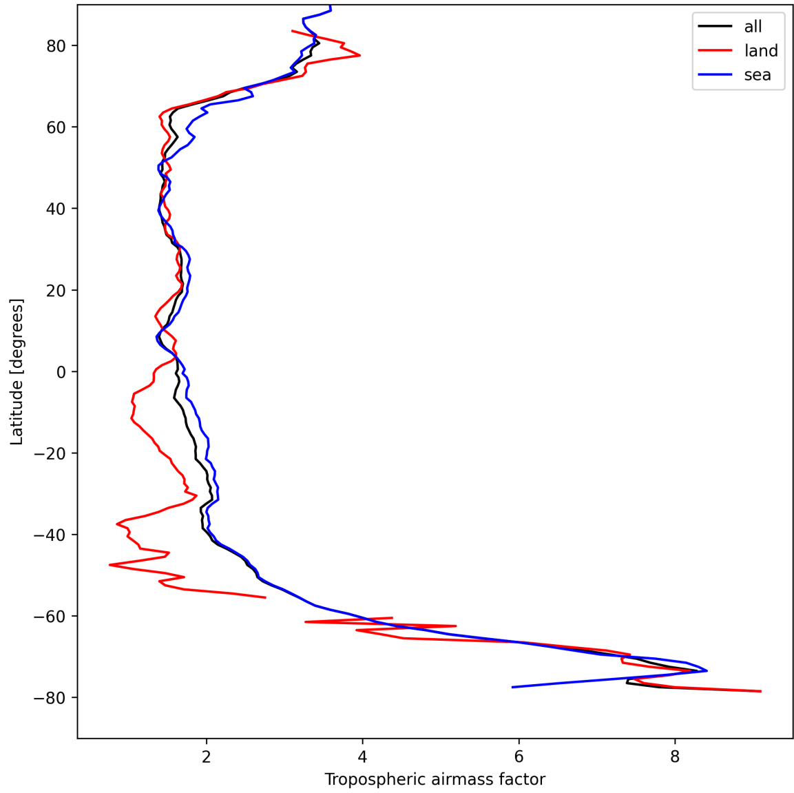
Figure 12: Zonal average of “Tropospheric airmass factor” for 2025-08-28 to 2025-08-28.
