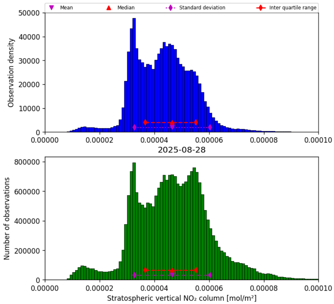
Figure 34: Histogram of “Stratospheric vertical NO 2 column” for 2025-08-28 to 2025-08-28
