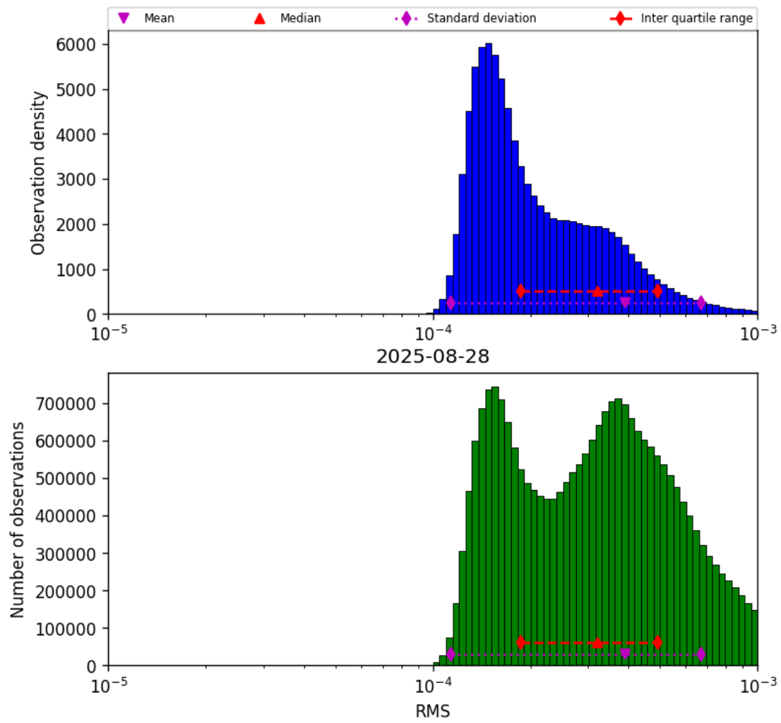
Figure 41: Histogram of “RMS” for 2025-08-28 to 2025-08-28
