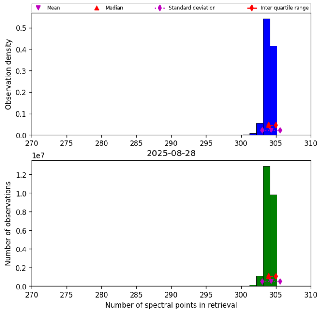
Figure 31: Histogram of “Number of spectral points in retrieval” for 2025-08-28 to 2025-08-28
