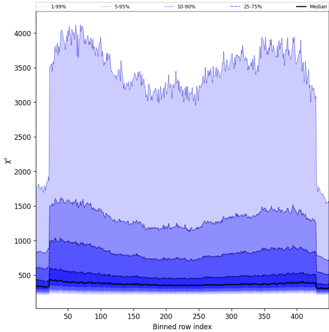
Figure 57: Along track statistics of “ \chi^2 ” for 2025-08-28 to 2025-08-28
