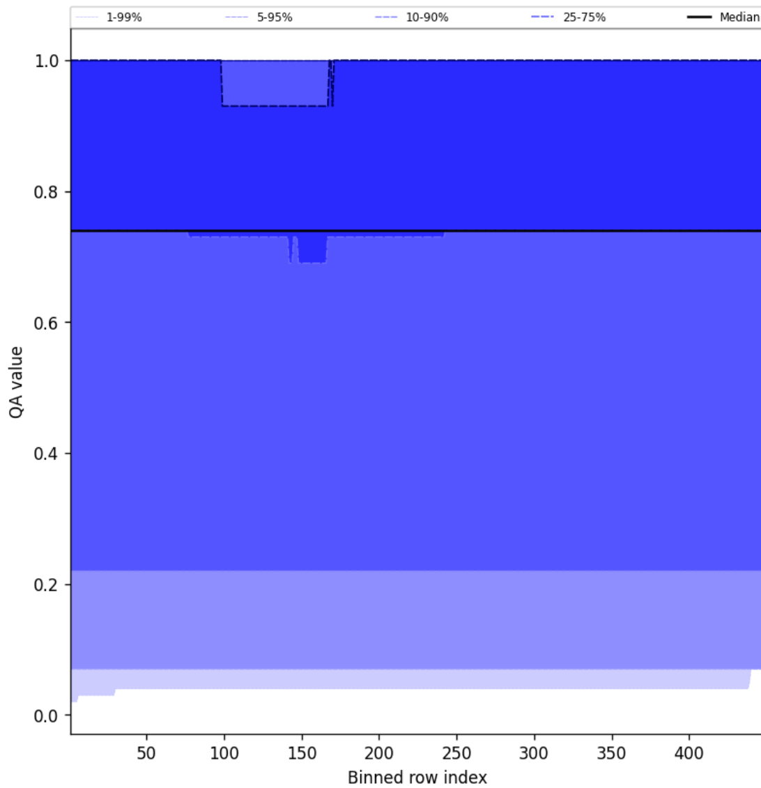
Figure 43: Along track statistics of “QA value” for 2025-08-28 to 2025-08-28
