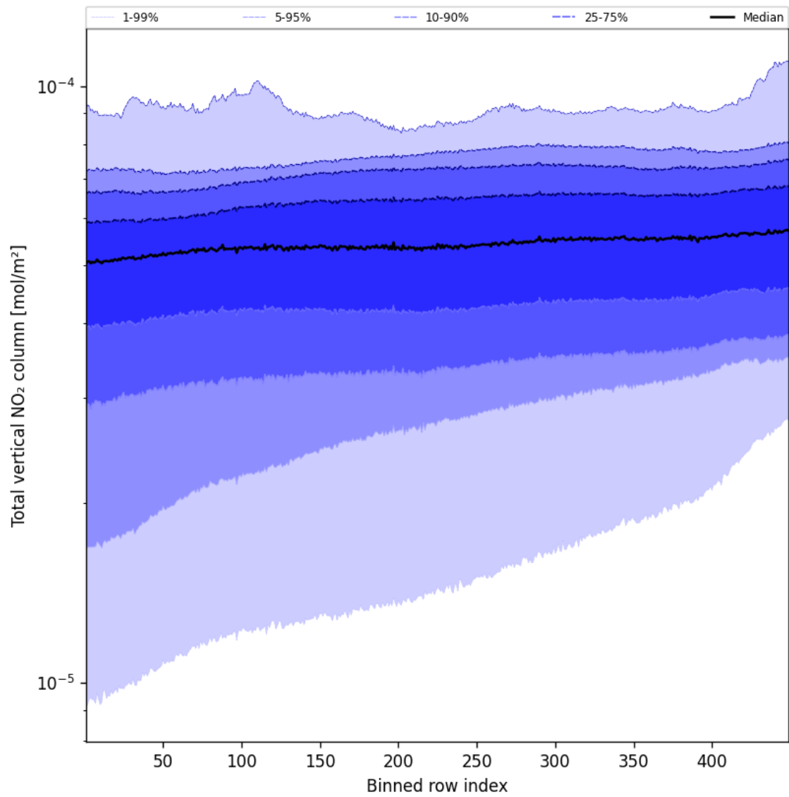
Figure 53: Along track statistics of “Total vertical NO 2 column” for 2025-08-28 to 2025-08-28
