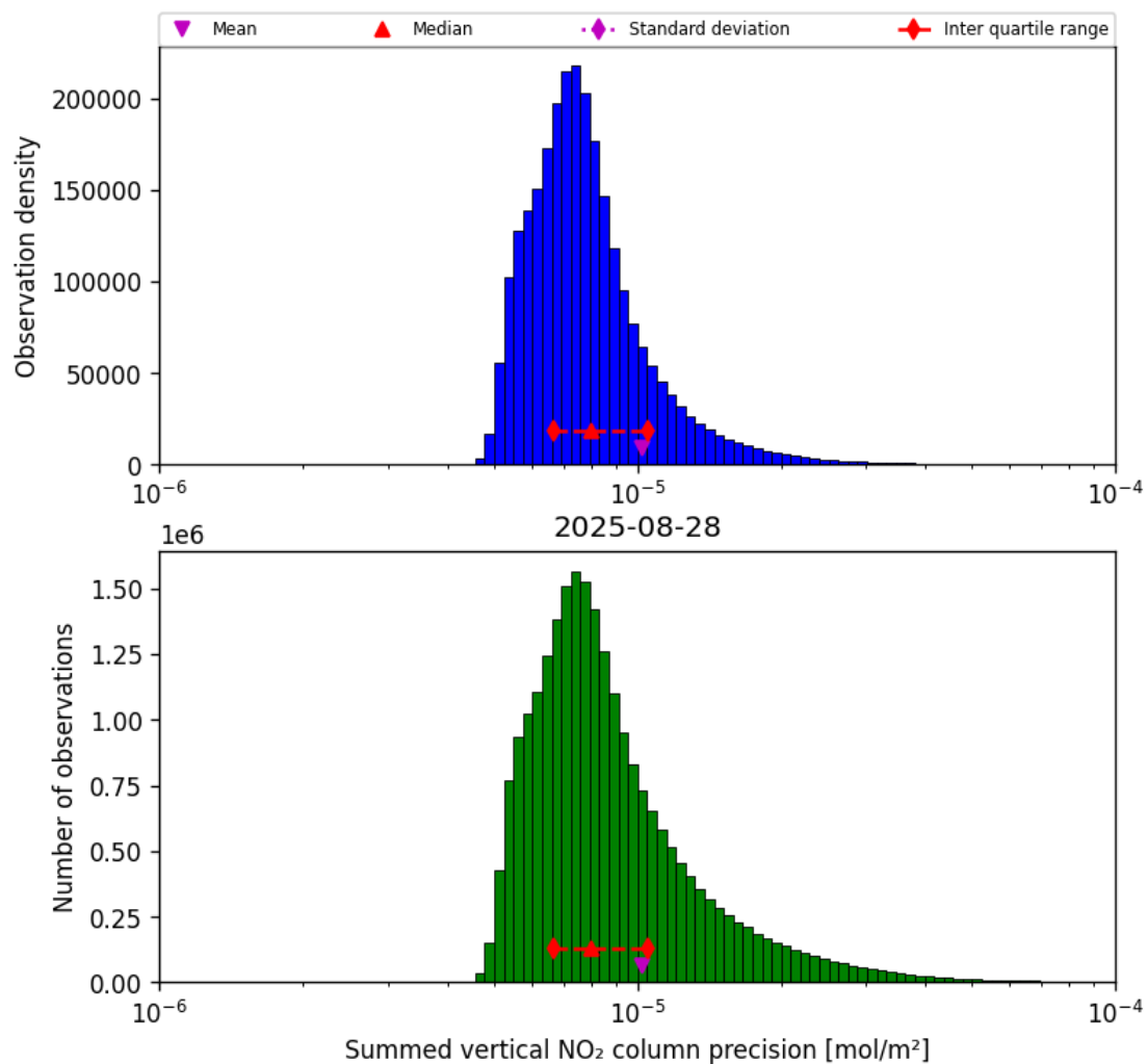
Figure 39: Histogram of "Summed vertical NO 2 column precision" for 2025-08-28 to 2025-08-28
