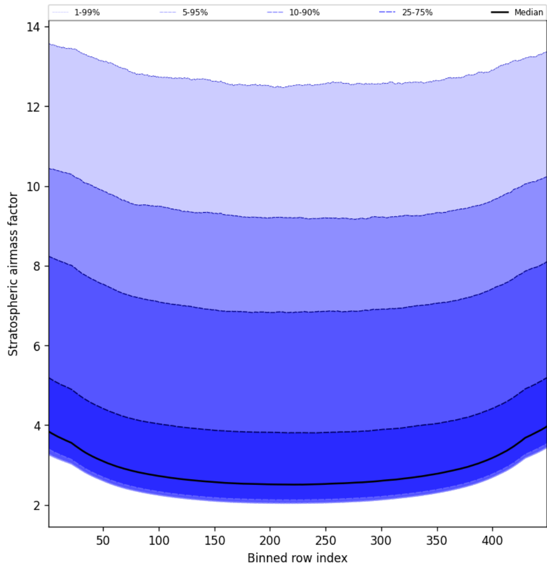
Figure 59: Along track statistics of “Stratospheric airmass factor” for 2025-08-28 to 2025-08-28
