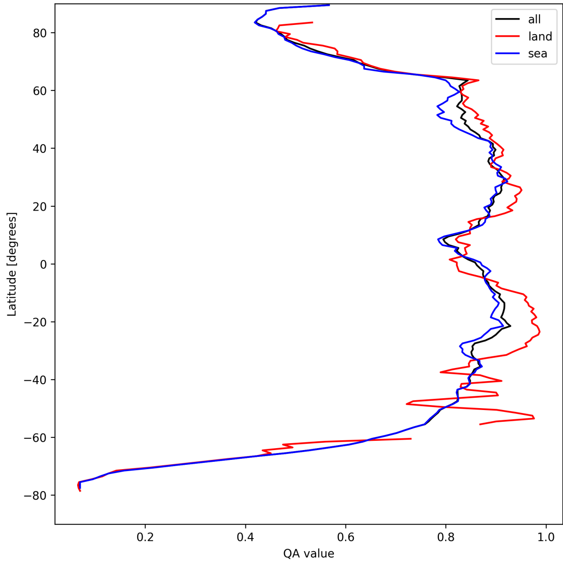
Figure 9: Zonal average of “QA value” for 2025-08-28 to 2025-08-28.
