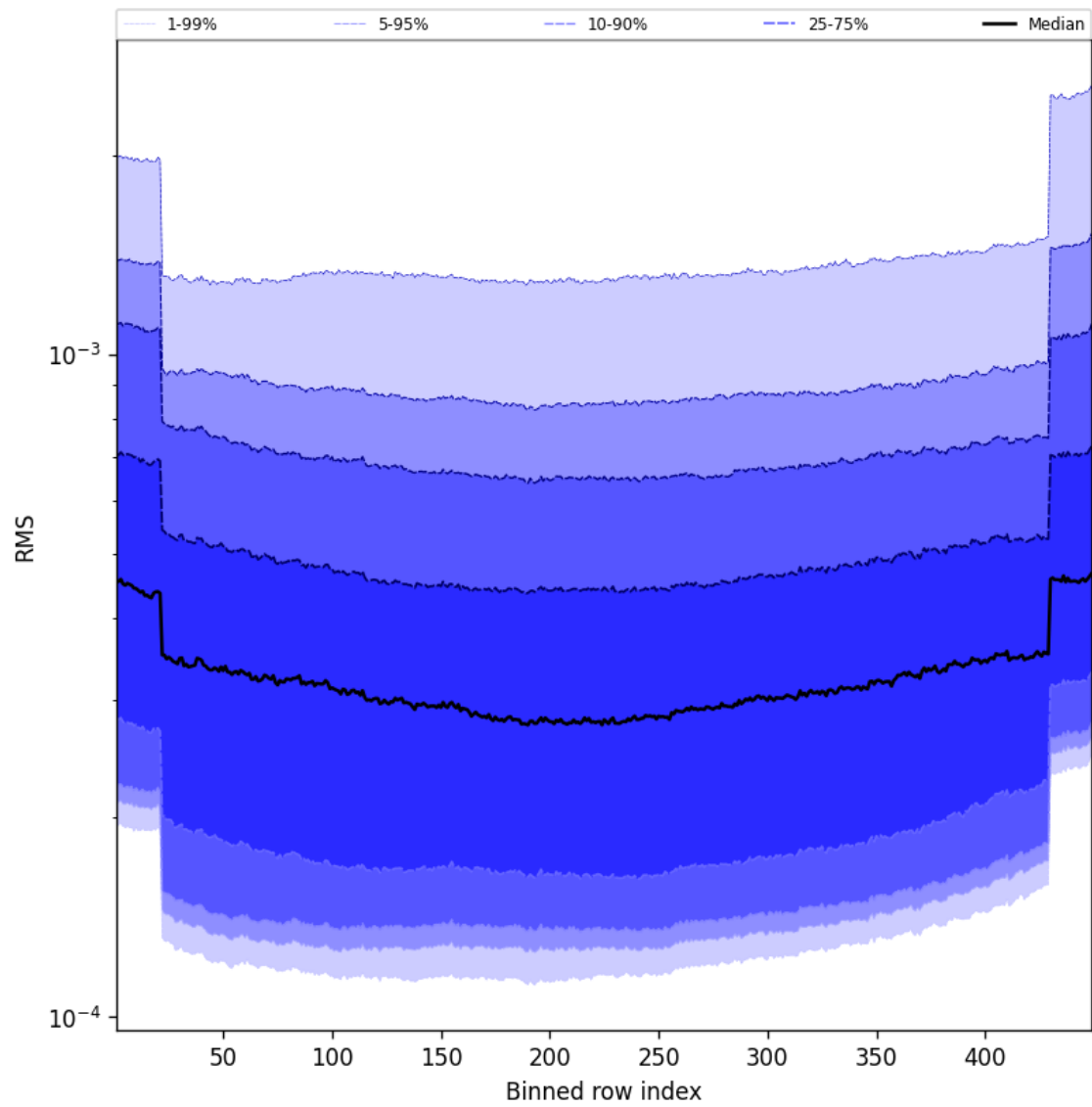
Figure 58: Along track statistics of “RMS” for 2025-08-28 to 2025-08-28
