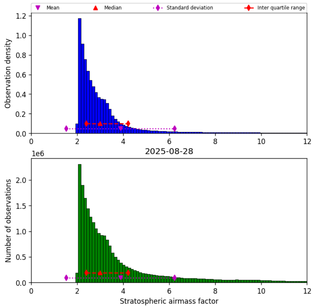
Figure 42: Histogram of “Stratospheric airmass factor” for 2025-08-28 to 2025-08-28
