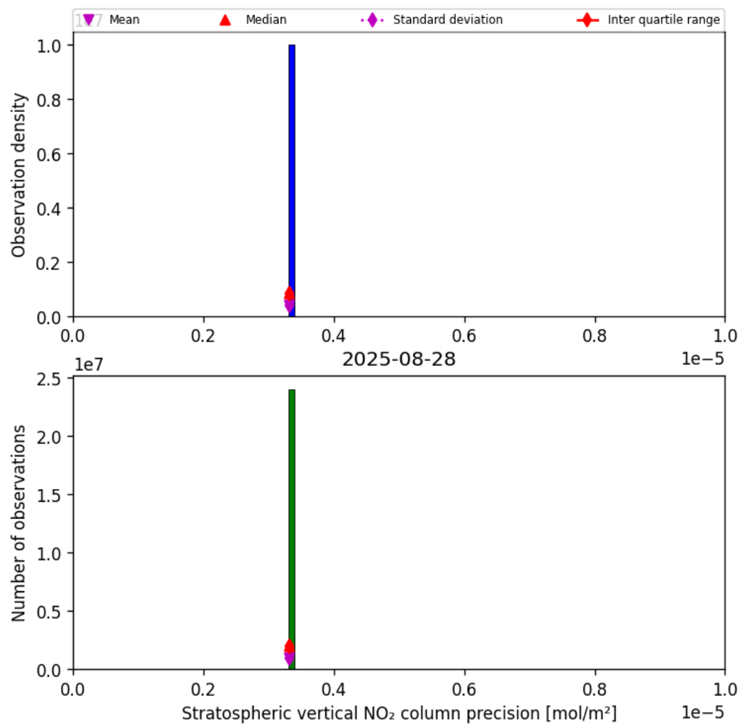
Figure 35: Histogram of “Stratospheric vertical NO 2 column precision” for 2025-08-28 to 2025-08-28
