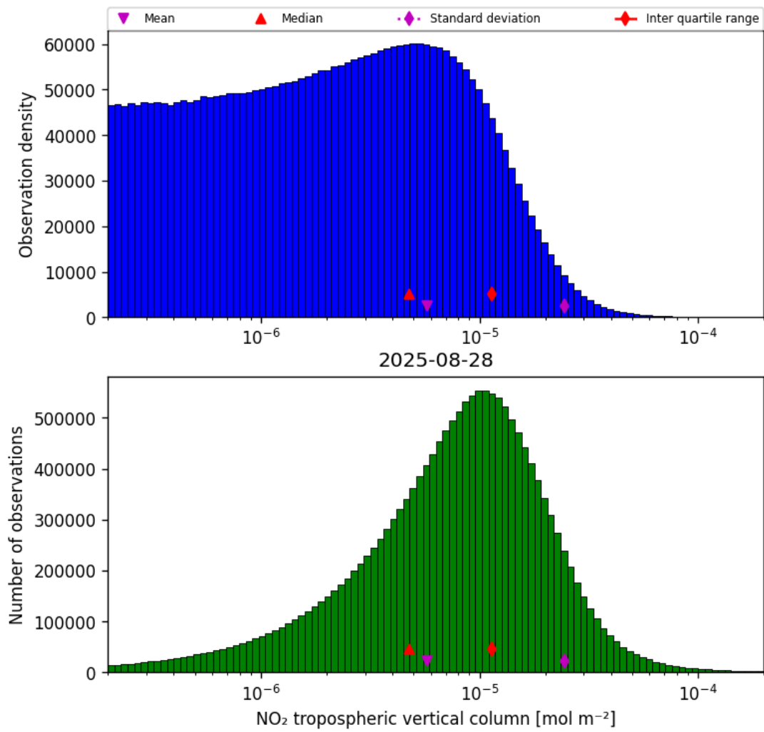
Figure 27: Histogram of “NO 2 tropospheric vertical column” for 2025-08-28 to 2025-08-28
