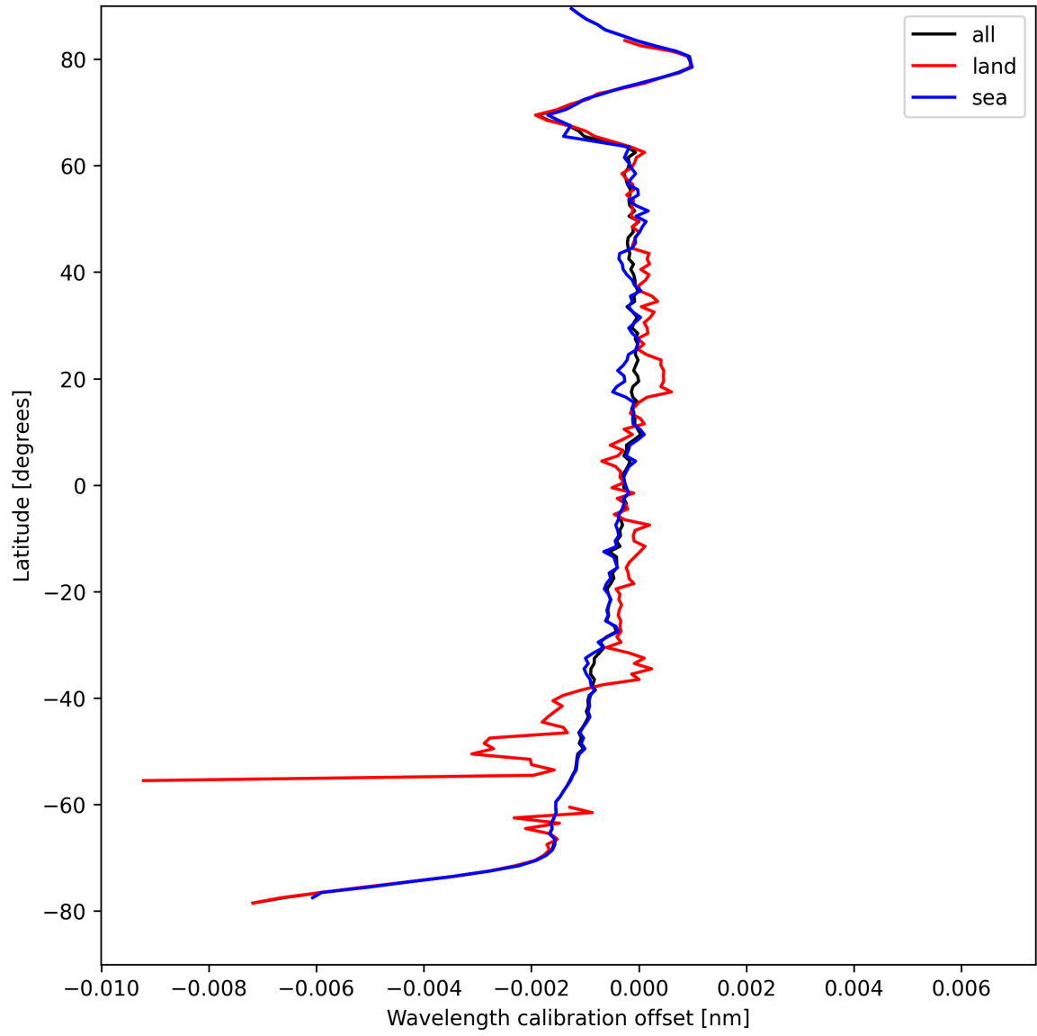
Figure 16: Zonal average of “Wavelength calibration offset” for 2025-08-28 to 2025-08-28.
