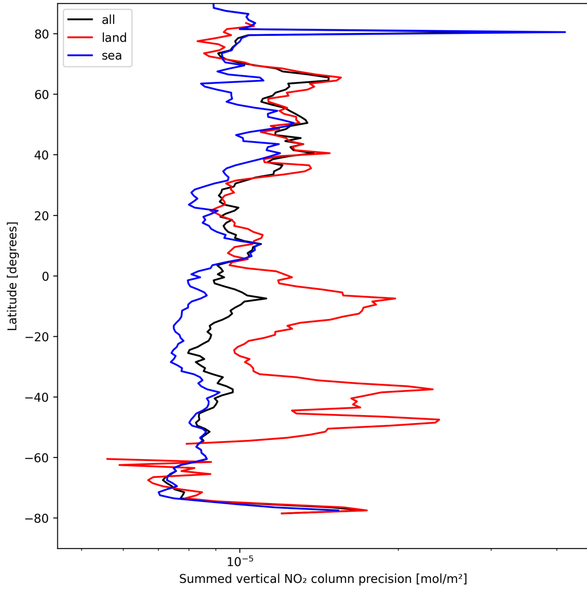
Figure 22: Zonal average of “Summed vertical NO 2 column precision” for 2025-08-28 to 2025-08-28.
