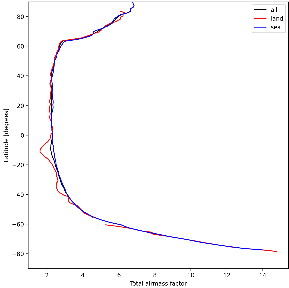
Figure 13: Zonal average of “Total airmass factor” for 2025-08-28 to 2025-08-28.
