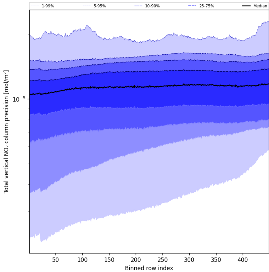
Figure 54: Along track statistics of “Total vertical NO 2 column precision” for 2025-08-28 to 2025-08-28
