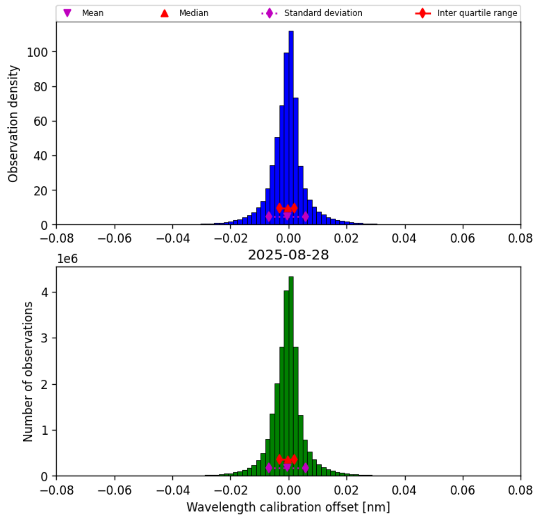
Figure 33: Histogram of “Wavelength calibration offset” for 2025-08-28 to 2025-08-28
