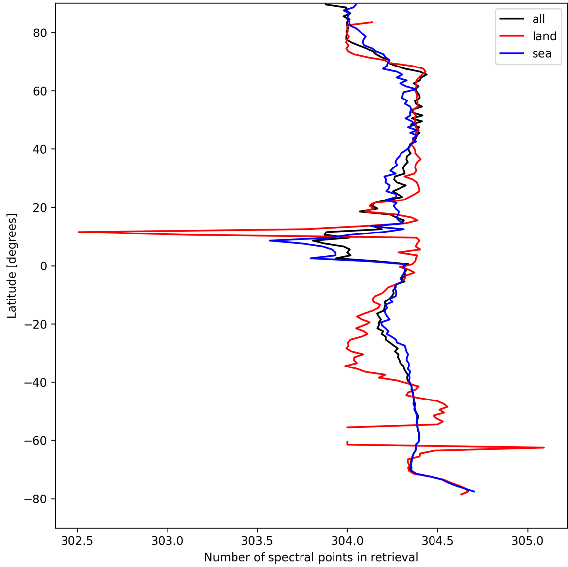
Figure 14: Zonal average of “Number of spectral points in retrieval” for 2025-08-28 to 2025-08-28.
