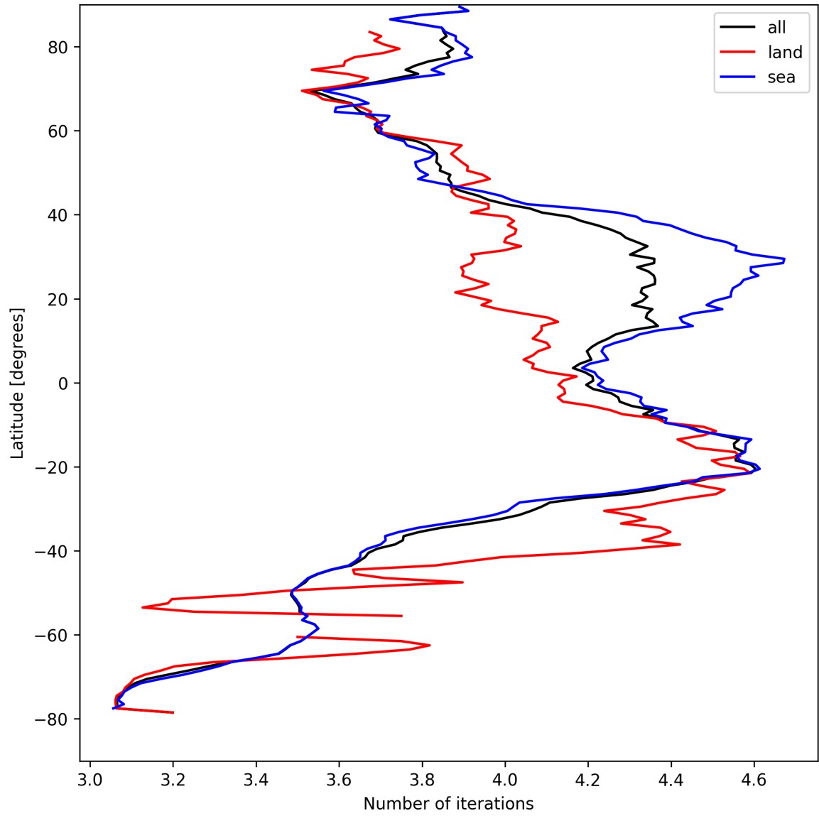
Figure 15: Zonal average of “Number of iterations” for 2025-08-28 to 2025-08-28.
