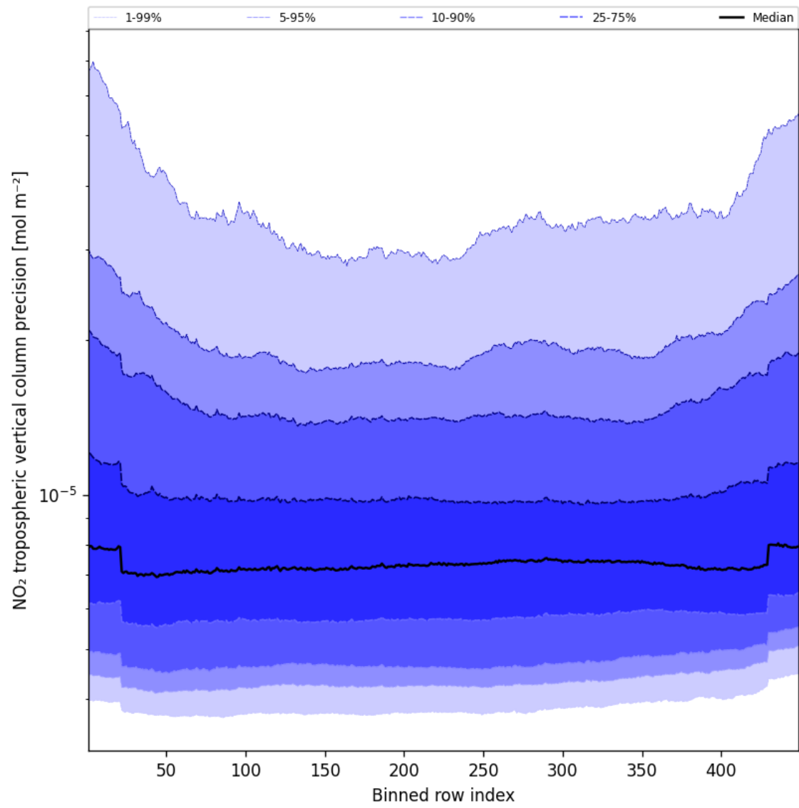
Figure 45: Along track statistics of “NO 2 tropospheric vertical column precision” for 2025-08-28 to 2025-08-28
