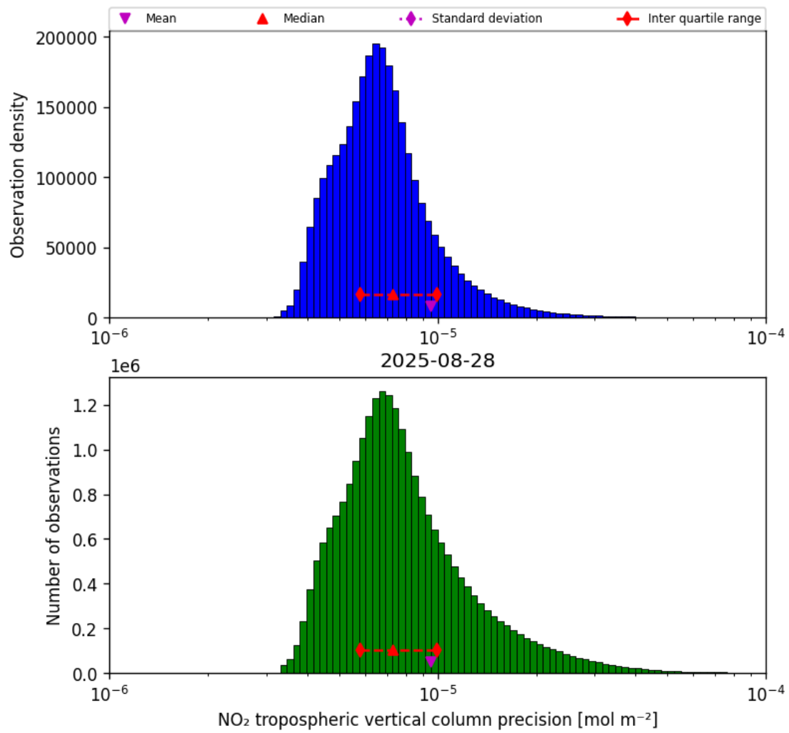
Figure 28: Histogram of “NO 2 tropospheric vertical column precision” for 2025-08-28 to 2025-08-28
