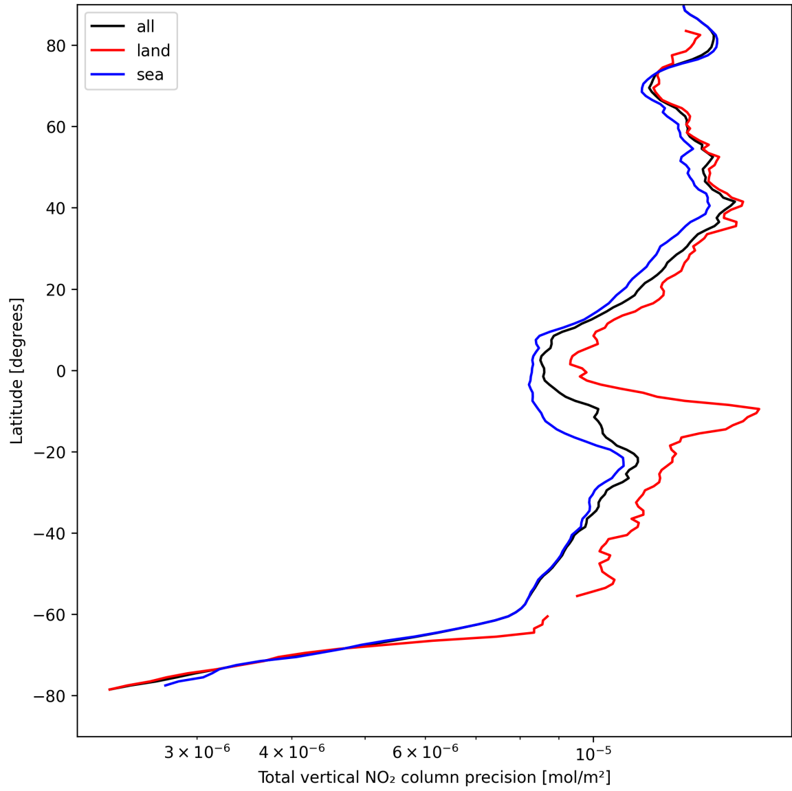
Figure 20: Zonal average of “Total vertical NO 2 column precision” for 2025-08-28 to 2025-08-28.
