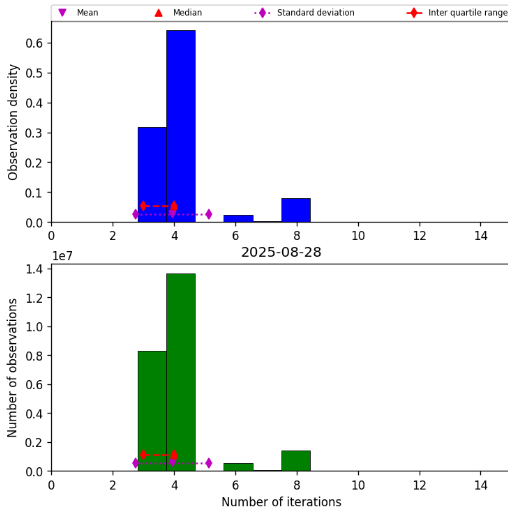
Figure 32: Histogram of “Number of iterations” for 2025-08-28 to 2025-08-28
