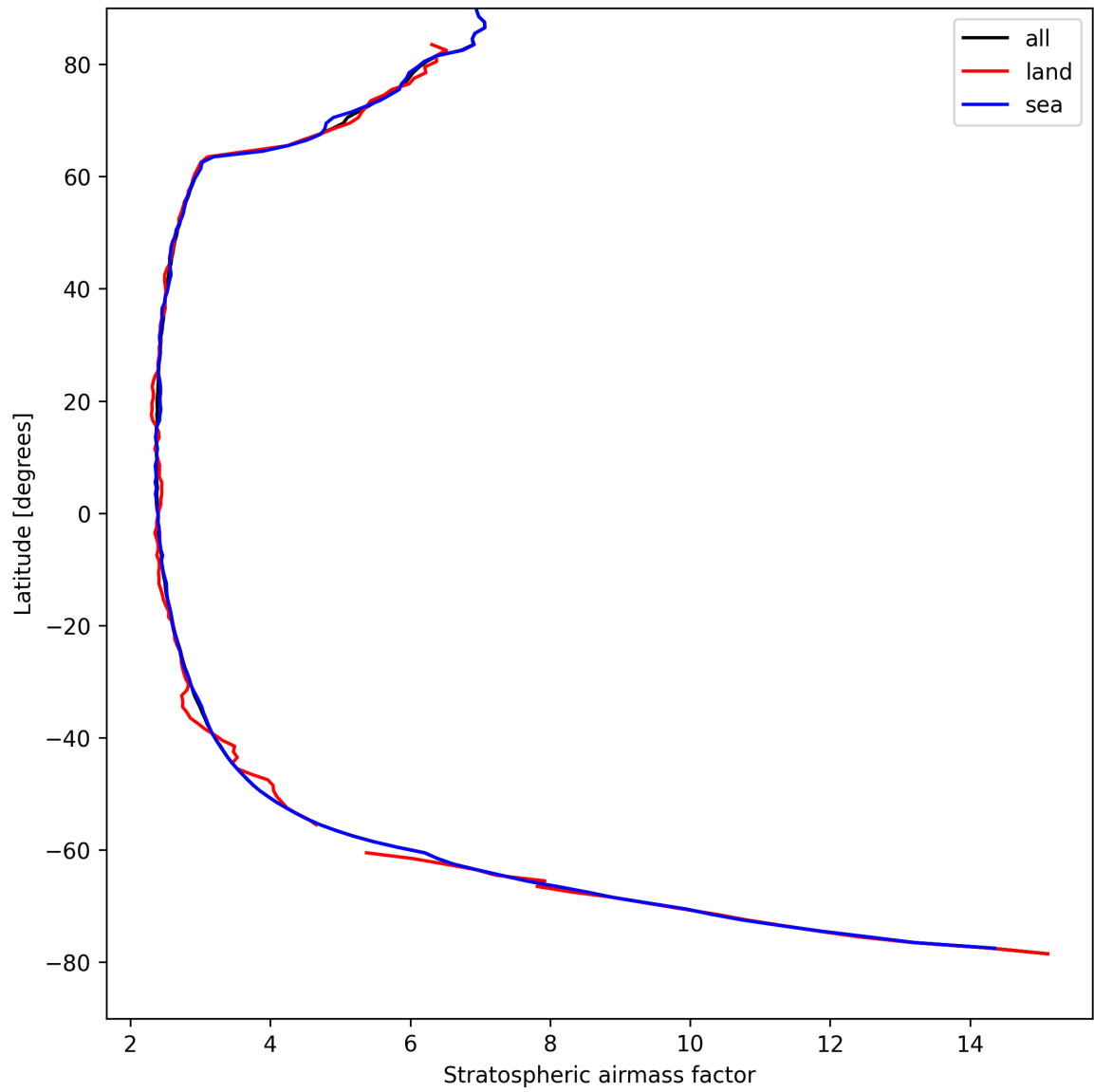
Figure 25: Zonal average of “Stratospheric air mass factor” for 2025-08-28 to 2025-08-28.
