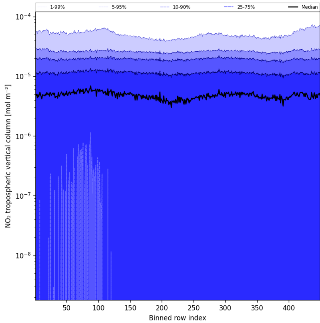
Figure 44: Along track statistics of “NO 2 tropospheric vertical column” for 2025-08-28 to 2025-08-28
