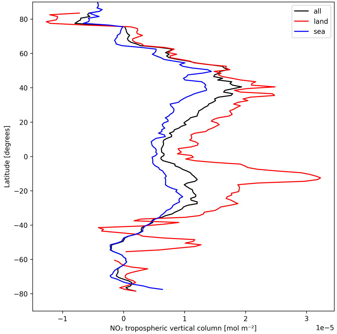
Figure 10: Zonal average of “NO 2 tropospheric vertical column” for 2025-08-28 to 2025-08-28.
