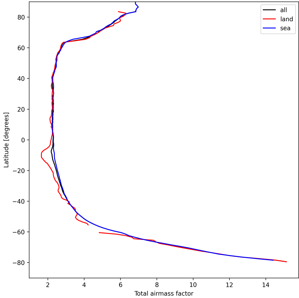
Figure 13: Zonal average of “Total airmass factor” for 2025-08-29 to 2025-08-30.
