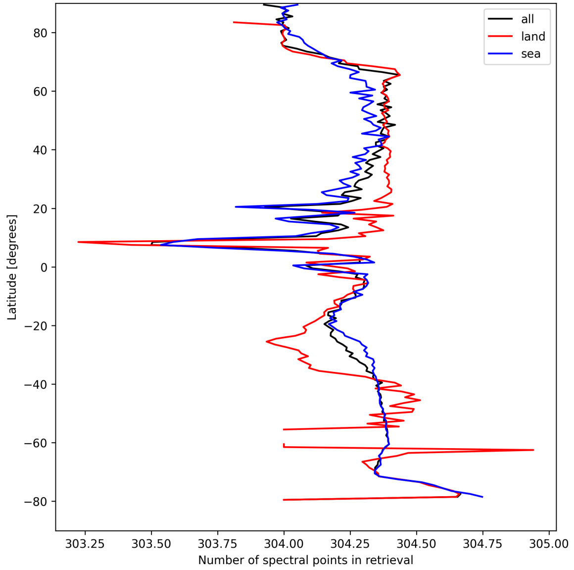
Figure 14: Zonal average of “Number of spectral points in retrieval” for 2025-08-29 to 2025-08-30.
