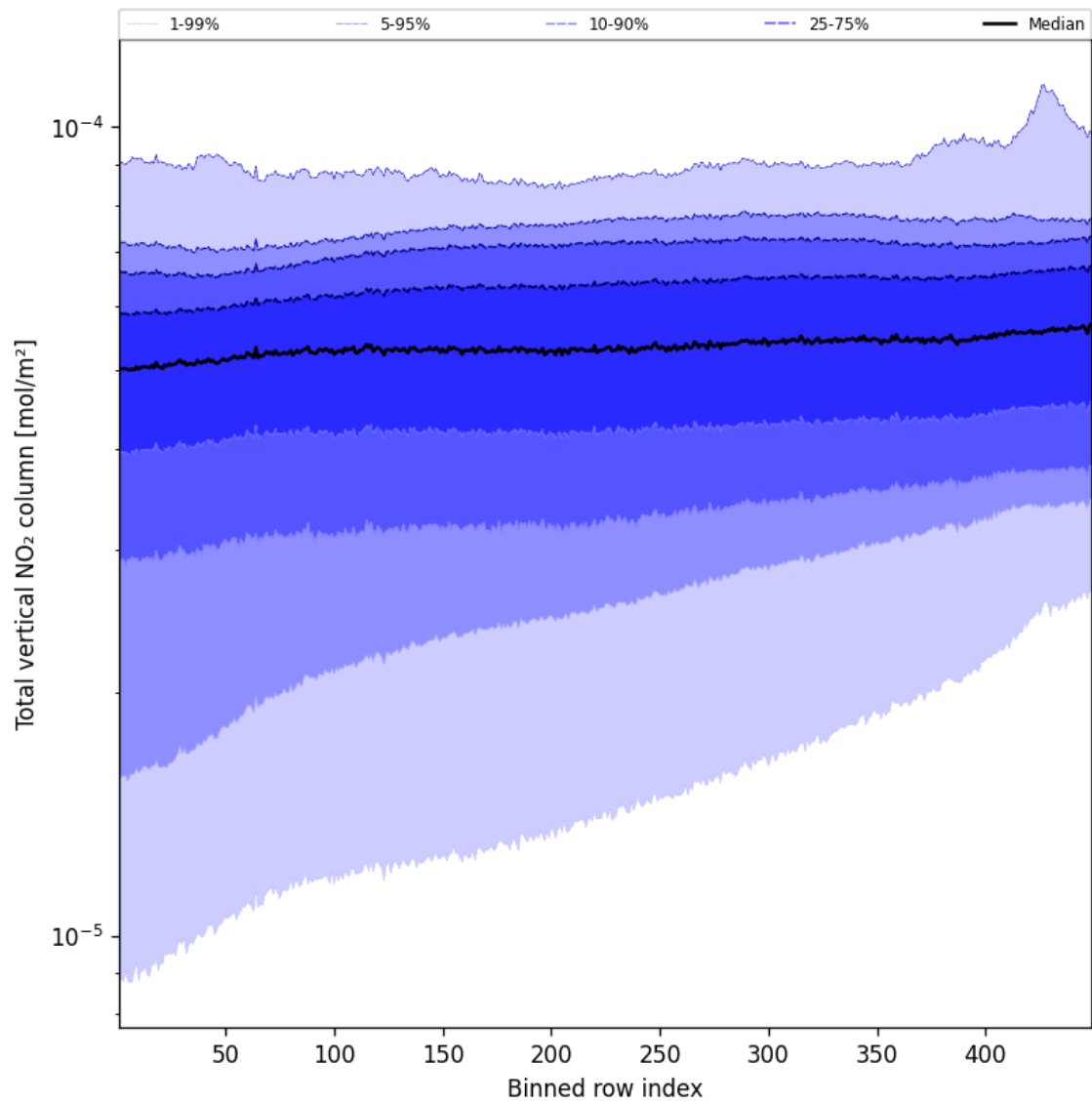
Figure 53: Along track statistics of “Total vertical NO 2 column” for 2025-08-29 to 2025-08-30
