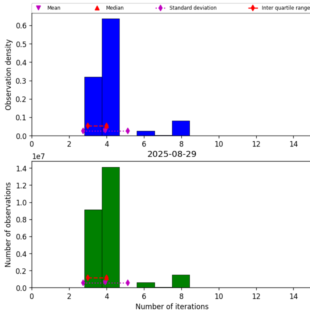
Figure 32: Histogram of “Number of iterations” for 2025-08-29 to 2025-08-30
