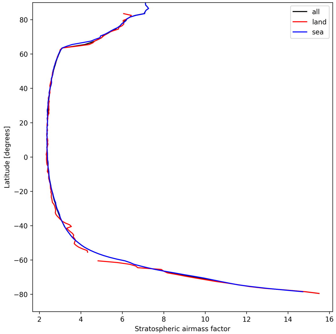
Figure 25: Zonal average of “Stratospheric airmass factor” for 2025-08-29 to 2025-08-30.
