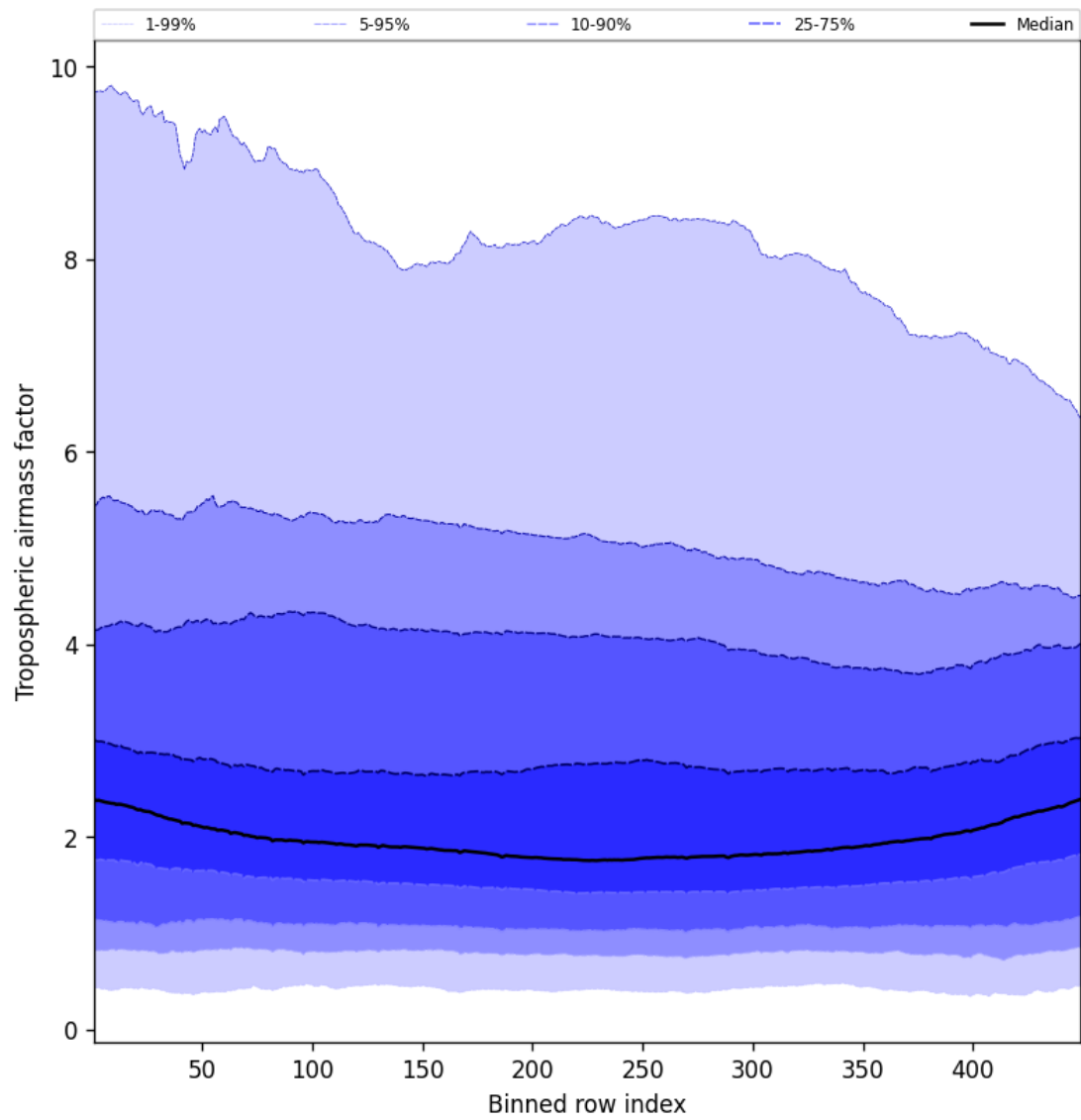
Figure 46: Along track statistics of “Tropospheric airmass factor” for 2025-08-29 to 2025-08-30
