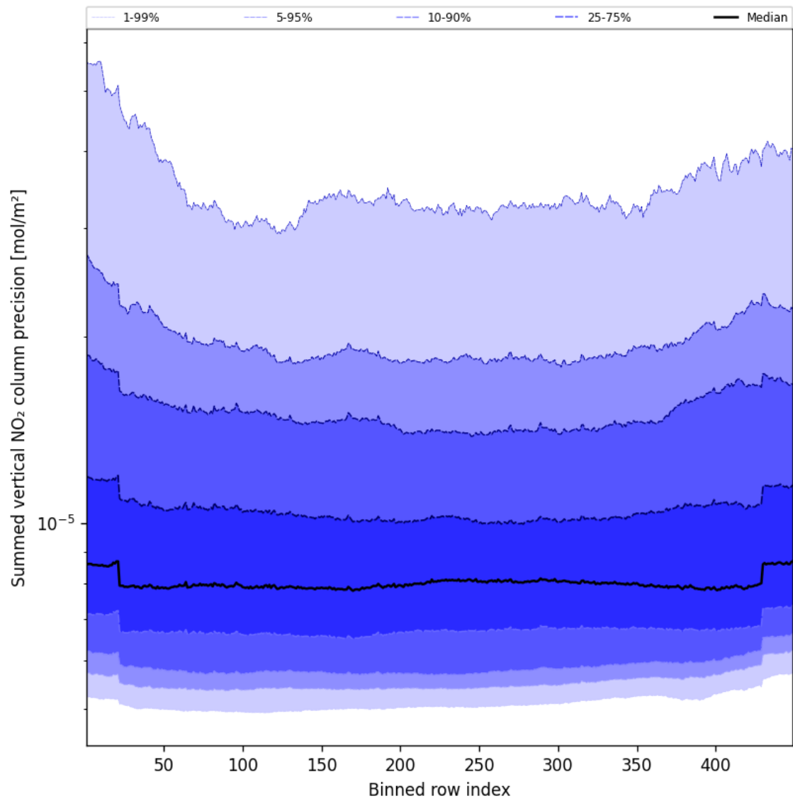
Figure 56: Along track statistics of “Summed vertical NO 2 column precision” for 2025-08-29 to 2025-08-30
