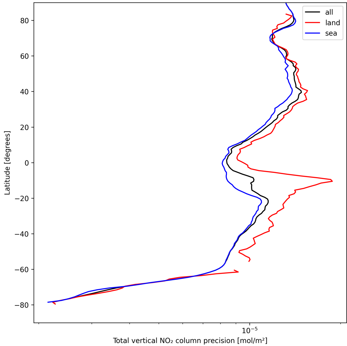
Figure 20: Zonal average of “Total vertical NO 2 column precision” for 2025-08-29 to 2025-08-30.
