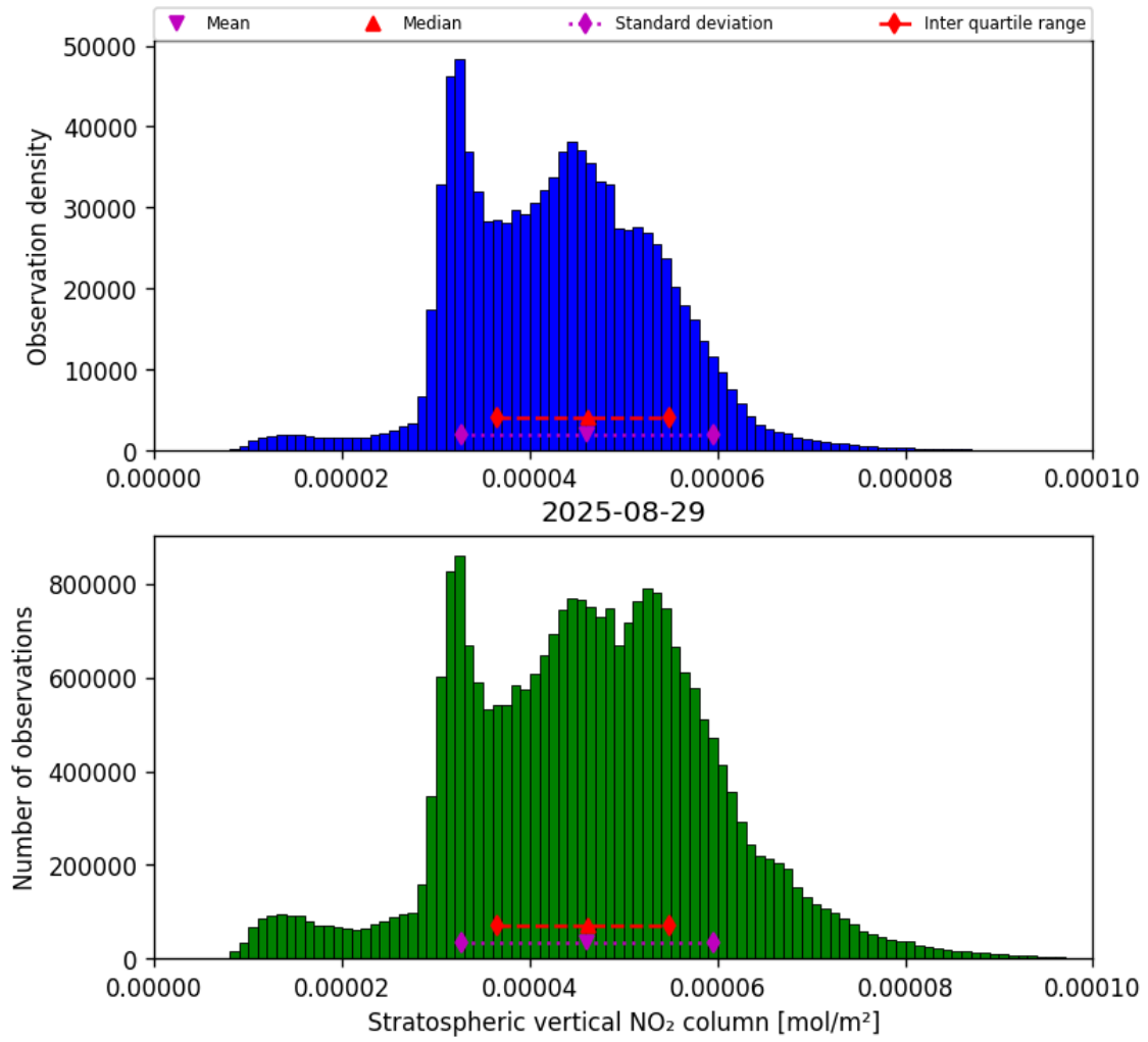
Figure 34: Histogram of “Stratospheric vertical NO 2 column” for 2025-08-29 to 2025-08-30
