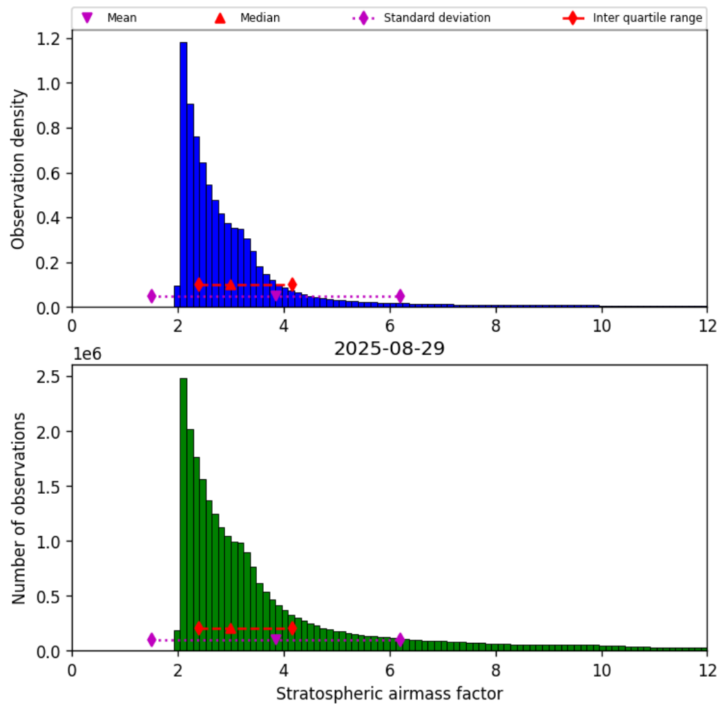
Figure 42: Histogram of “Stratospheric airmass factor” for 2025-08-29 to 2025-08-30
