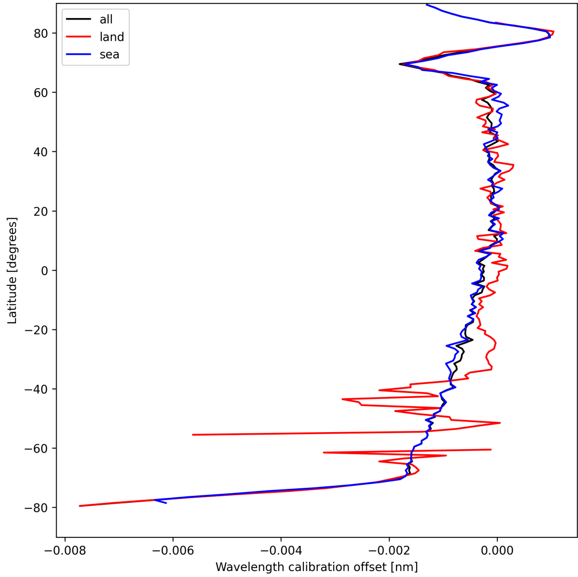
Figure 16: Zonal average of “Wavelength calibration offset” for 2025-08-29 to 2025-08-30.
