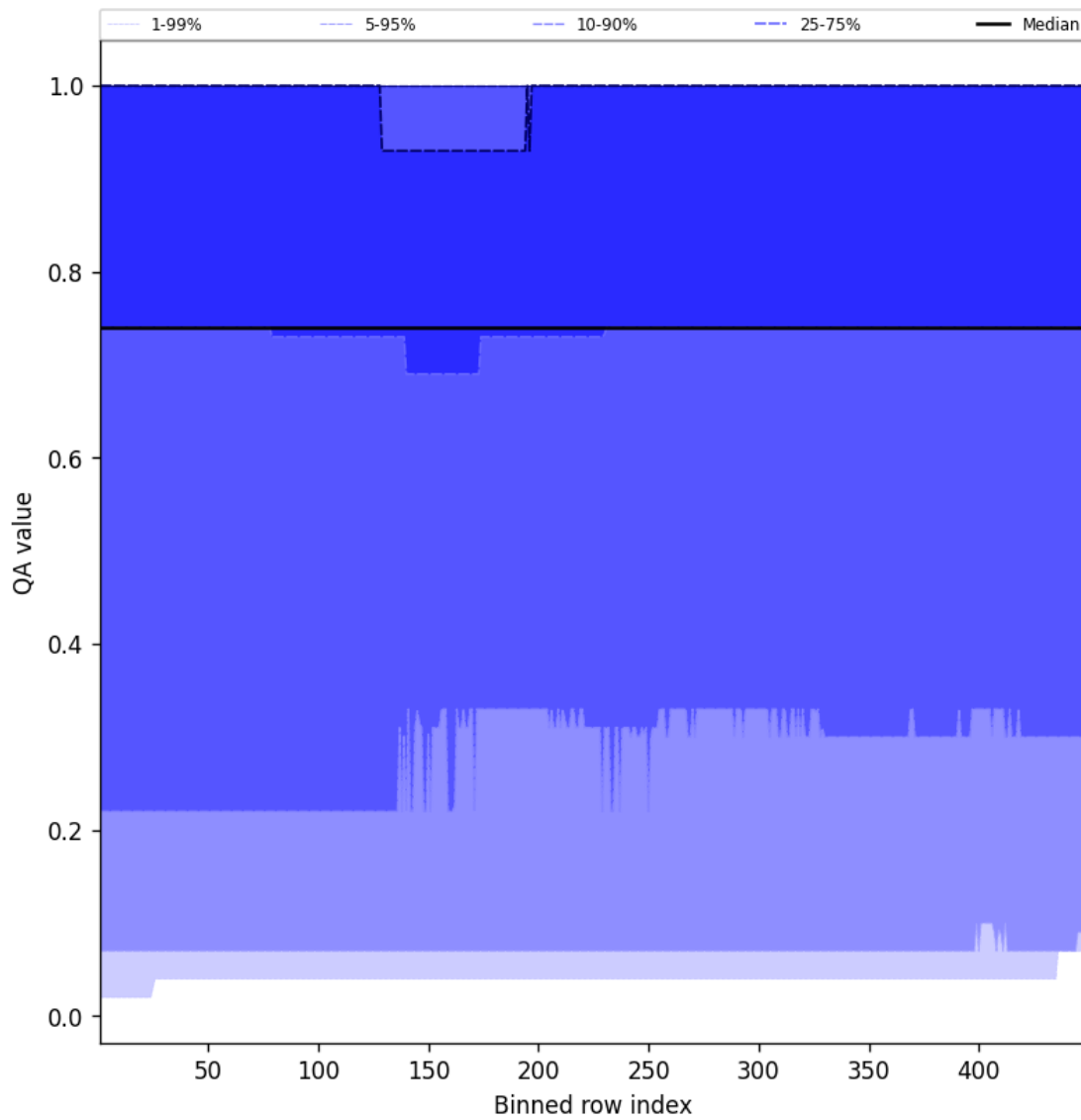
Figure 43: Along track statistics of “QA value” for 2025-08-29 to 2025-08-30
