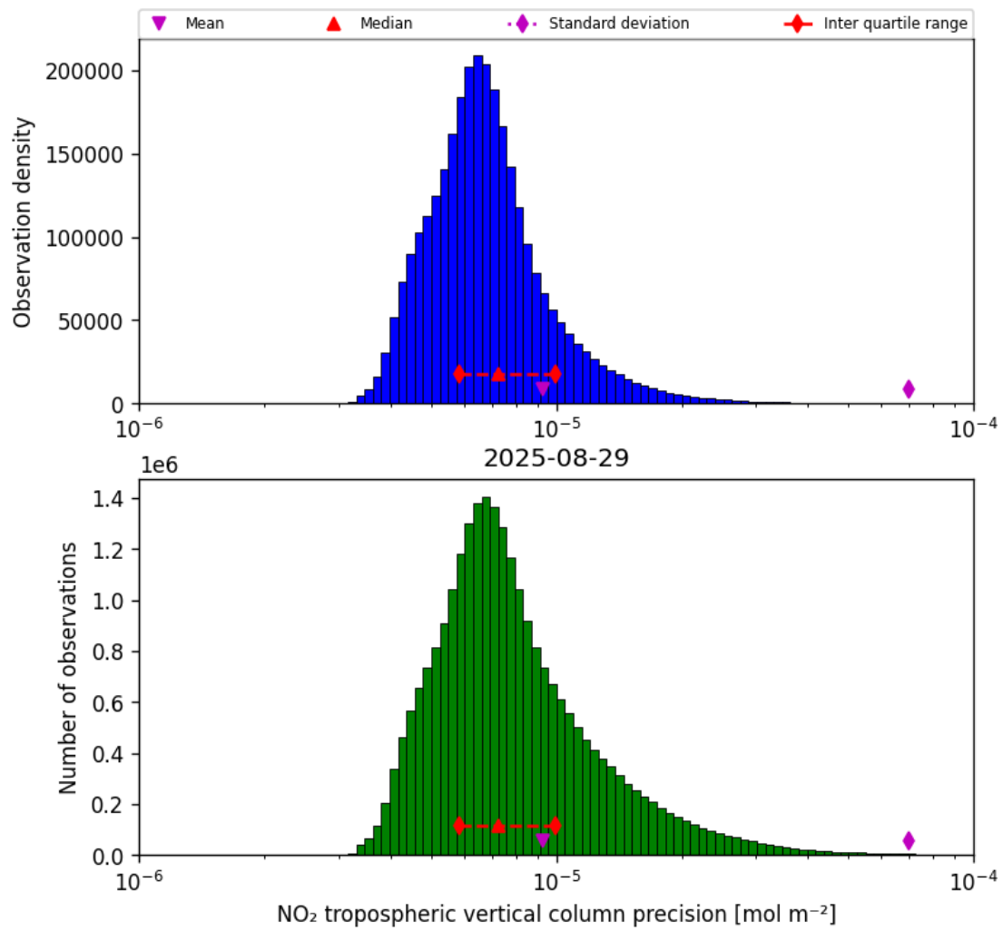
Figure 28: Histogram of “NO 2 tropospheric vertical column precision” for 2025-08-29 to 2025-08-30
