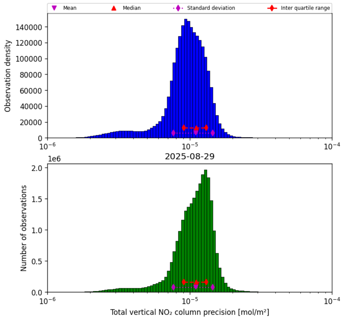
Figure 37: Histogram of "Total vertical NO 2 column precision" for 2025-08-29 to 2025-08-30
