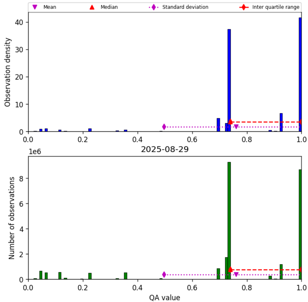
Figure 26: Histogram of “QA value” for 2025-08-29 to 2025-08-30
