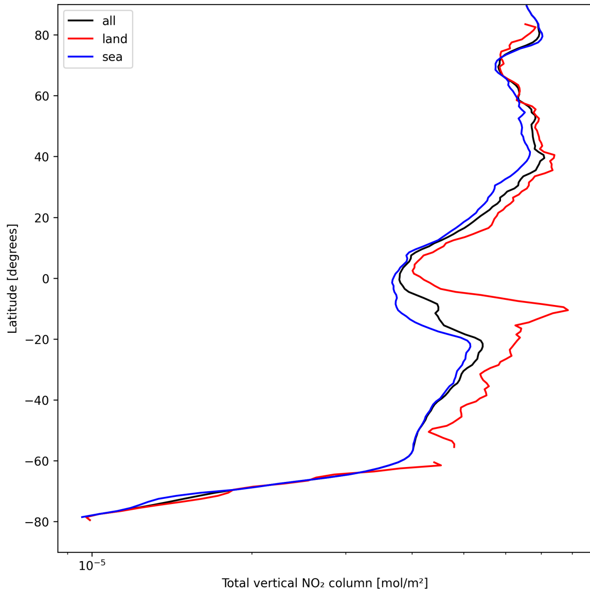
Figure 19: Zonal average of “Total vertical NO 2 column” for 2025-08-29 to 2025-08-30.
