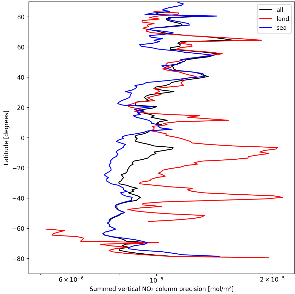
Figure 22: Zonal average of “Summed vertical NO 2 column precision” for 2025-08-29 to 2025-08-30.
