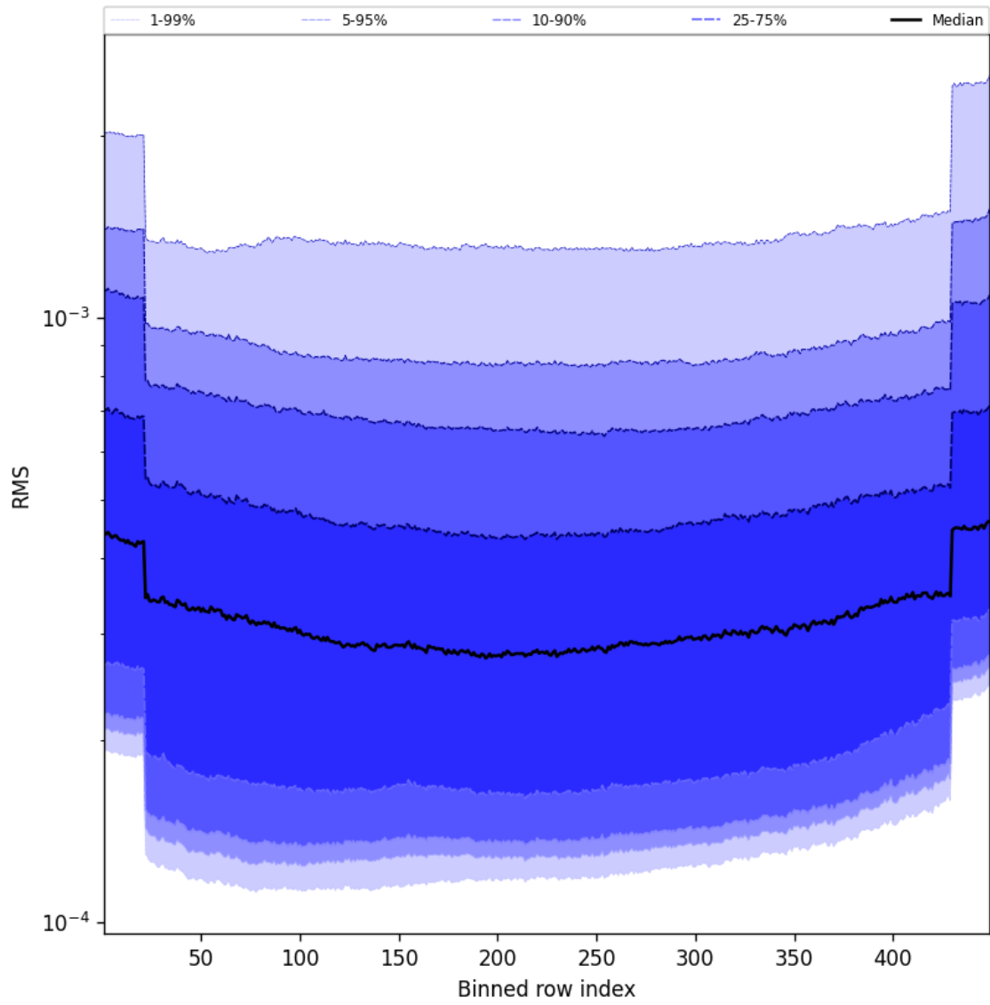
Figure 58: Along track statistics of “RMS” for 2025-08-29 to 2025-08-30
