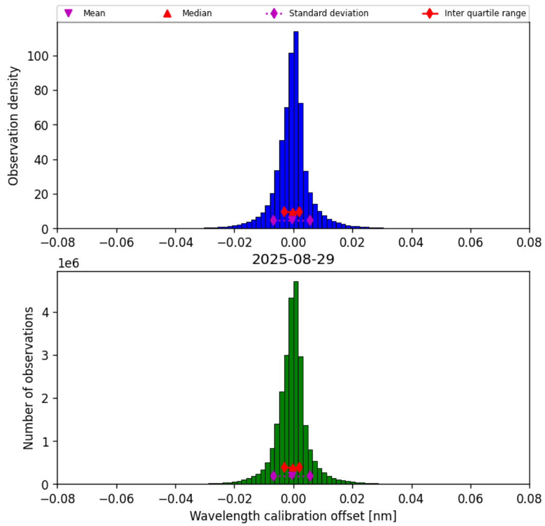
Figure 33: Histogram of “Wavelength calibration offset” for 2025-08-29 to 2025-08-30
