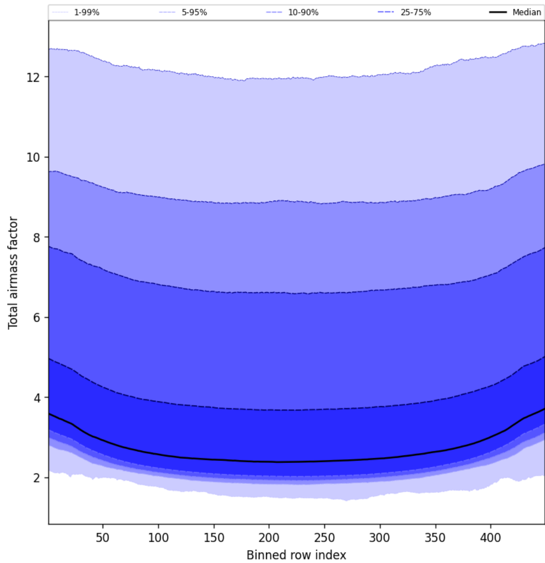
Figure 47: Along track statistics of “Total airmass factor” for 2025-08-29 to 2025-08-30
