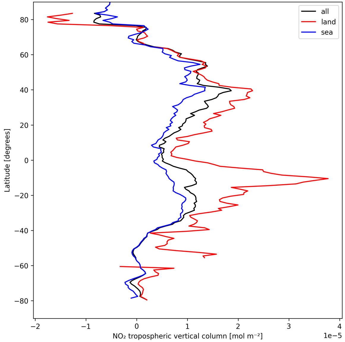
Figure 10: Zonal average of “NO 2 tropospheric vertical column” for 2025-08-29 to 2025-08-30.
