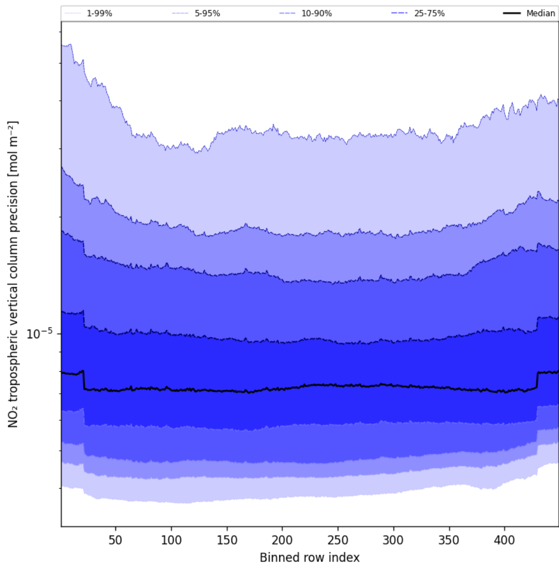
Figure 45: Along track statistics of “NO 2 tropospheric vertical column precision” for 2025-08-29 to 2025-08-30
