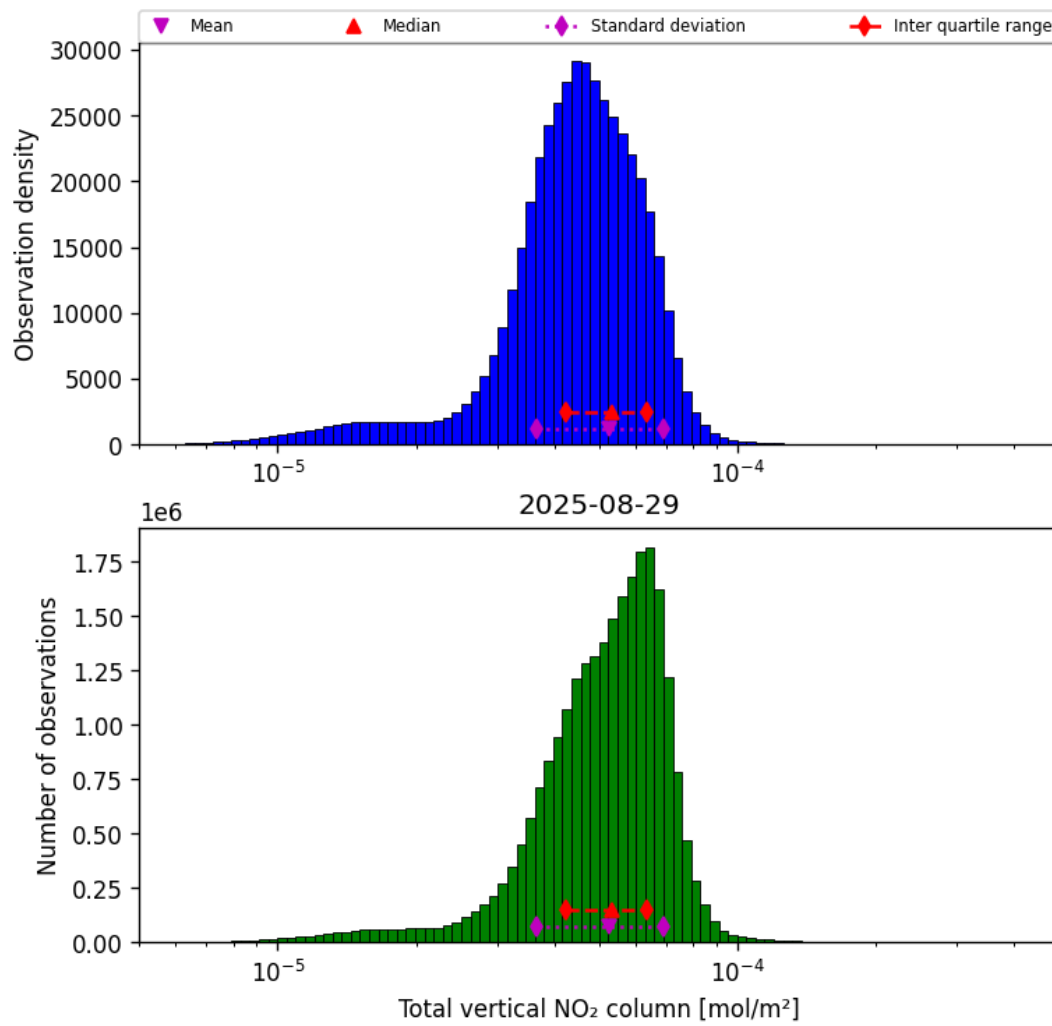
Figure 36: Histogram of “Total vertical NO 2 column” for 2025-08-29 to 2025-08-30
