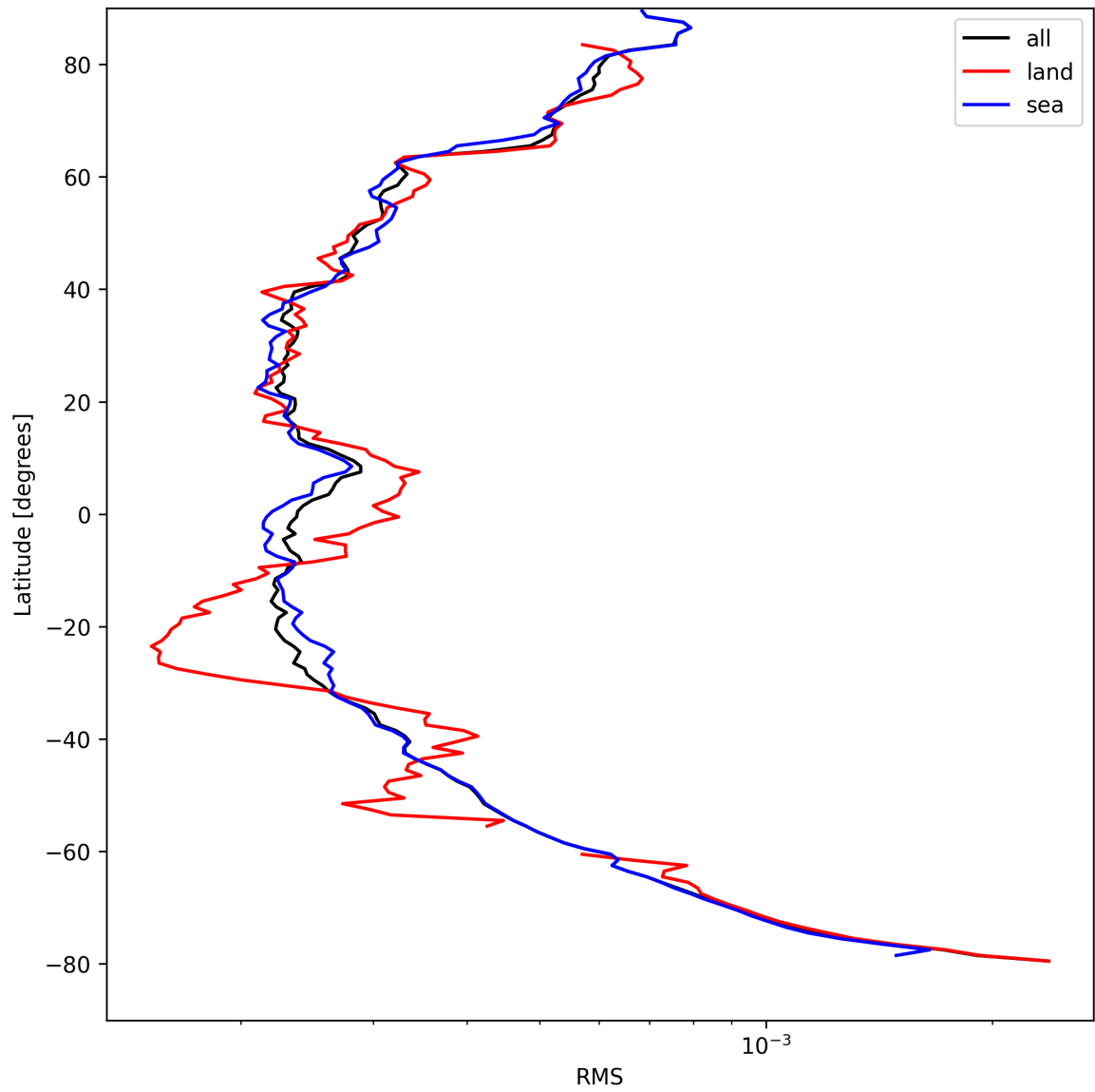
Figure 24: Zonal average of “RMS” for 2025-08-29 to 2025-08-30.
