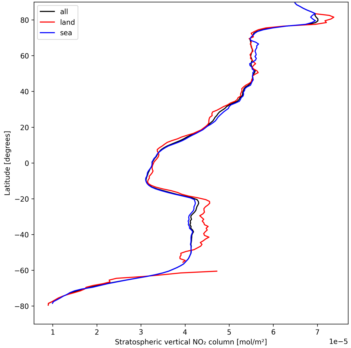
Figure 17: Zonal average of “Stratospheric vertical NO 2 column” for 2025-08-29 to 2025-08-30.
