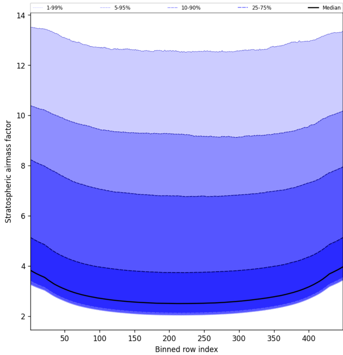
Figure 59: Along track statistics of “Stratospheric airmass factor” for 2025-08-29 to 2025-08-30
