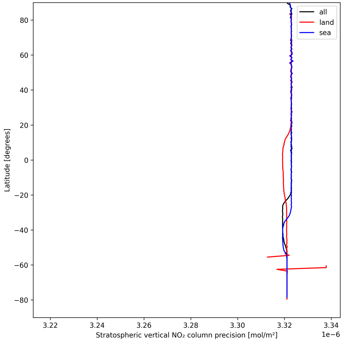
Figure 18: Zonal average of “Stratospheric vertical NO 2 column precision” for 2025-08-29 to 2025-08-30.
