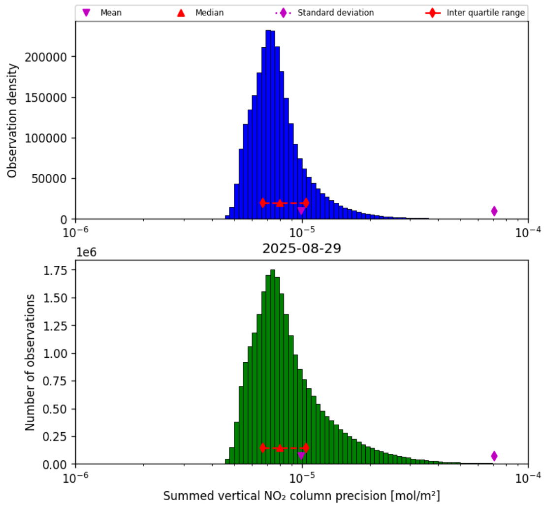
Figure 39: Histogram of “Summed vertical NO 2 column precision” for 2025-08-29 to 2025-08-30
