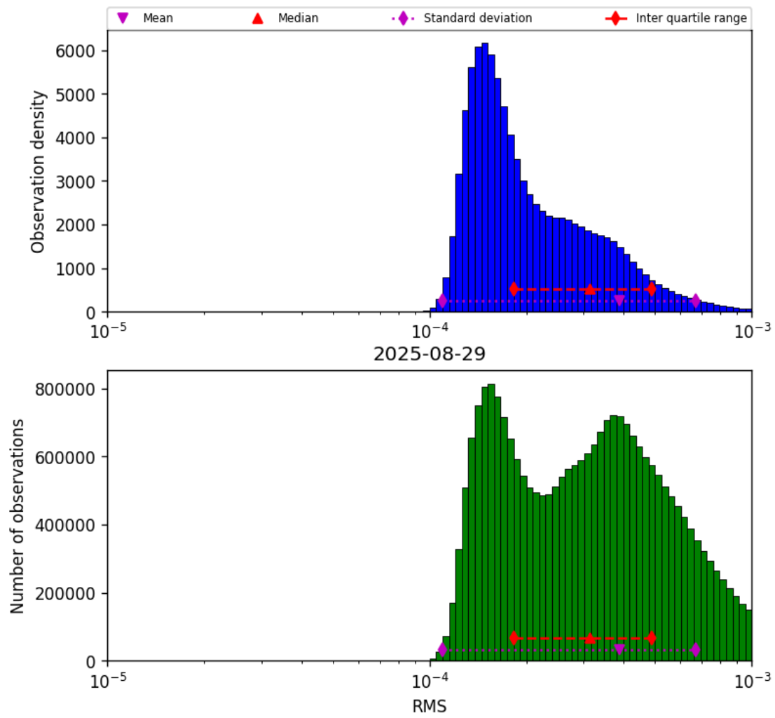
Figure 41: Histogram of “RMS” for 2025-08-29 to 2025-08-30
