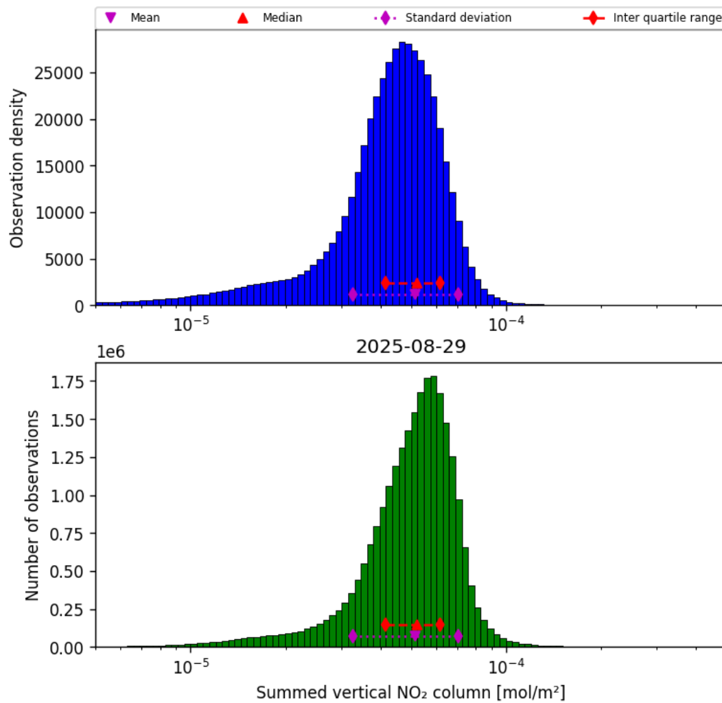
Figure 38: Histogram of “Summed vertical NO 2 column” for 2025-08-29 to 2025-08-30
