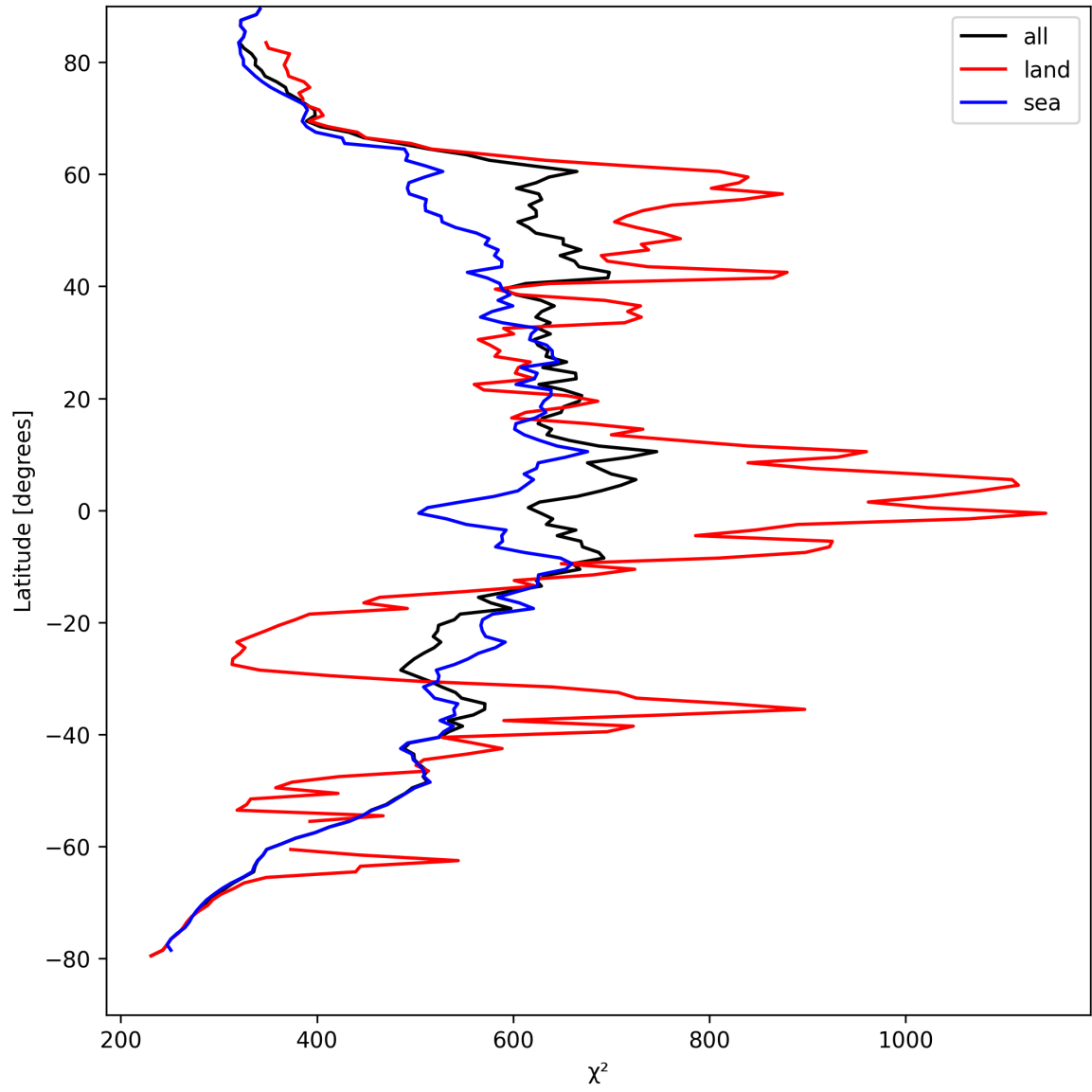
Figure 23: Zonal average of “ \chi^2 ” for 2025-08-29 to 2025-08-30.
