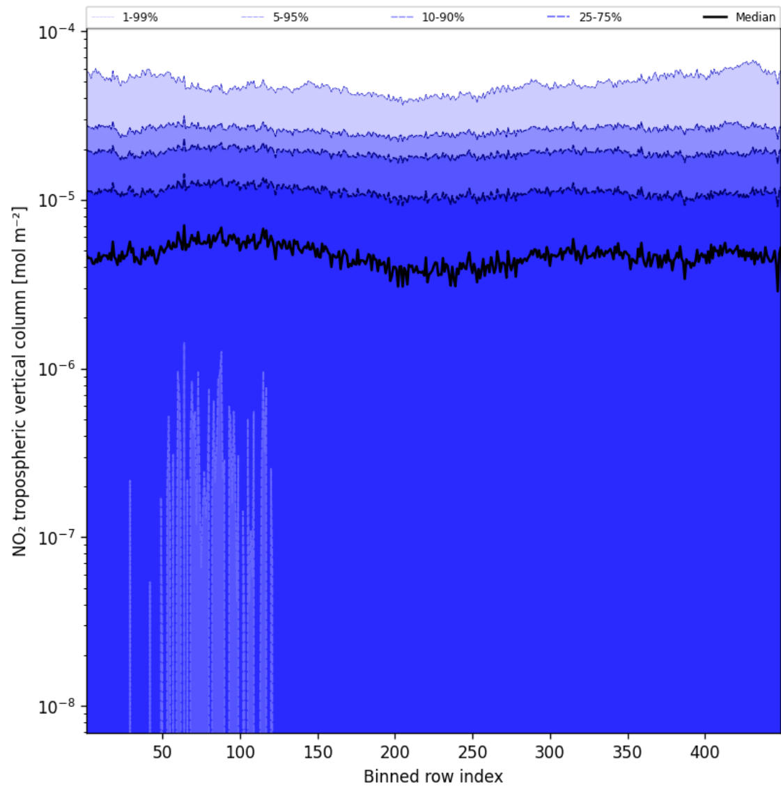
Figure 44: Along track statistics of “NO 2 tropospheric vertical column” for 2025-08-29 to 2025-08-30
