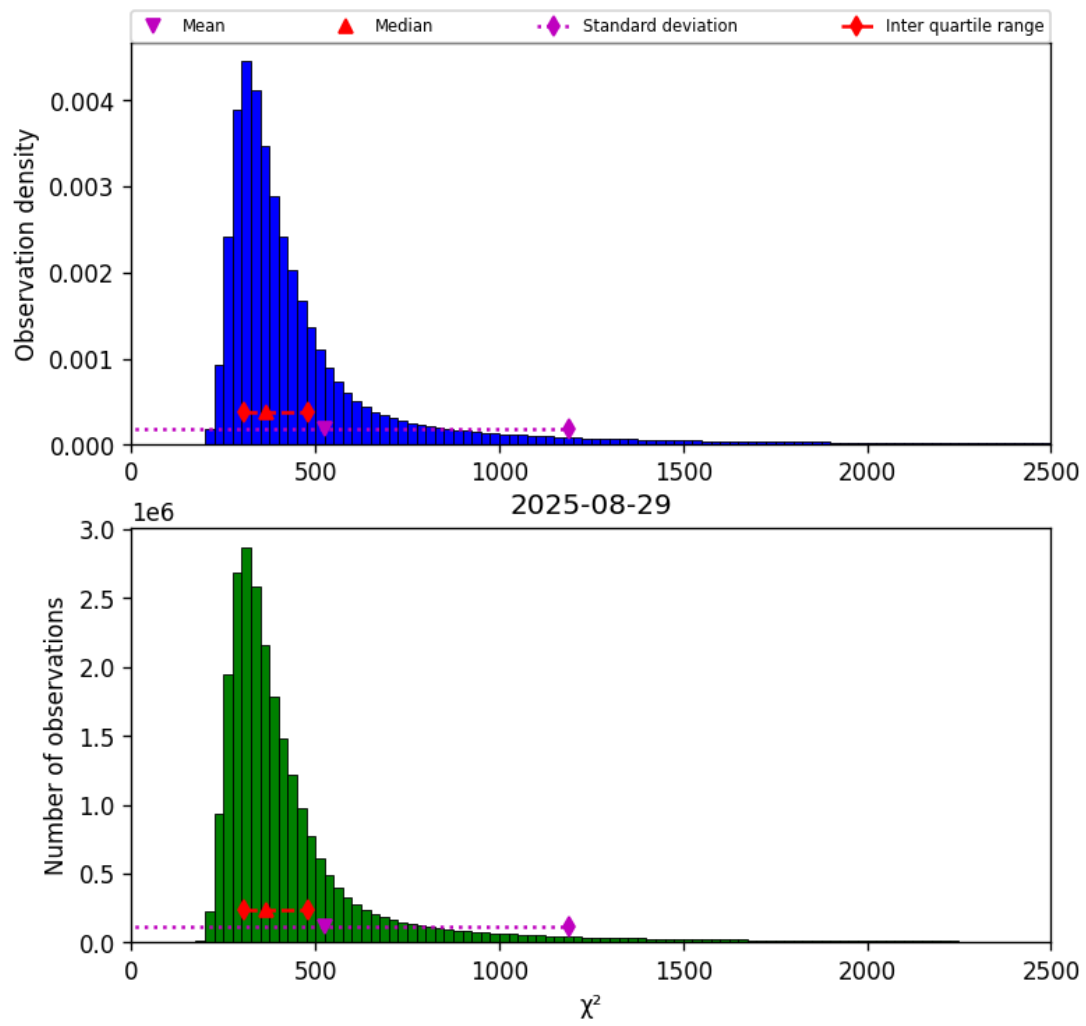
Figure 40: Histogram of " \chi^2 " for 2025-08-29 to 2025-08-30
