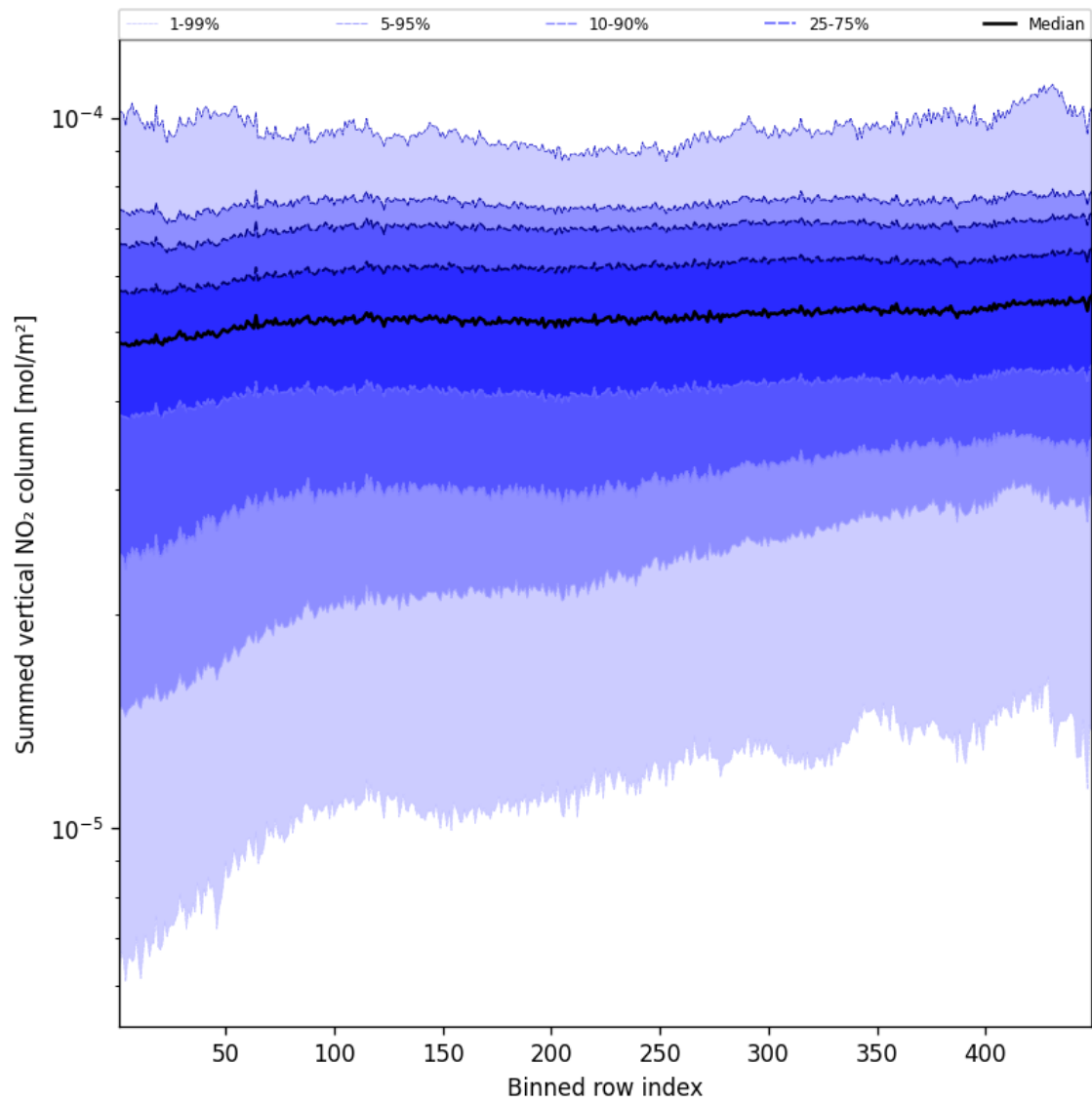
Figure 55: Along track statistics of “Summed vertical NO 2 column” for 2025-08-29 to 2025-08-30
