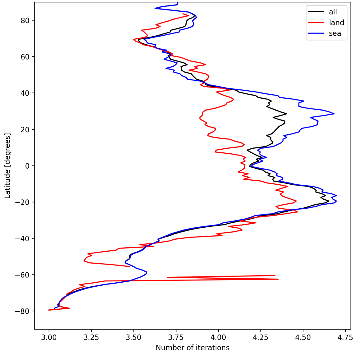
Figure 15: Zonal average of “Number of iterations” for 2025-08-29 to 2025-08-30.
