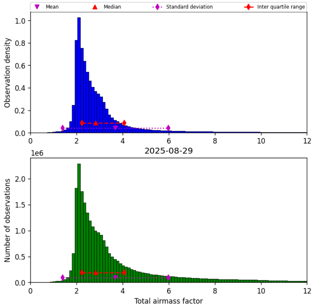
Figure 30: Histogram of “Total airmass factor” for 2025-08-29 to 2025-08-30
