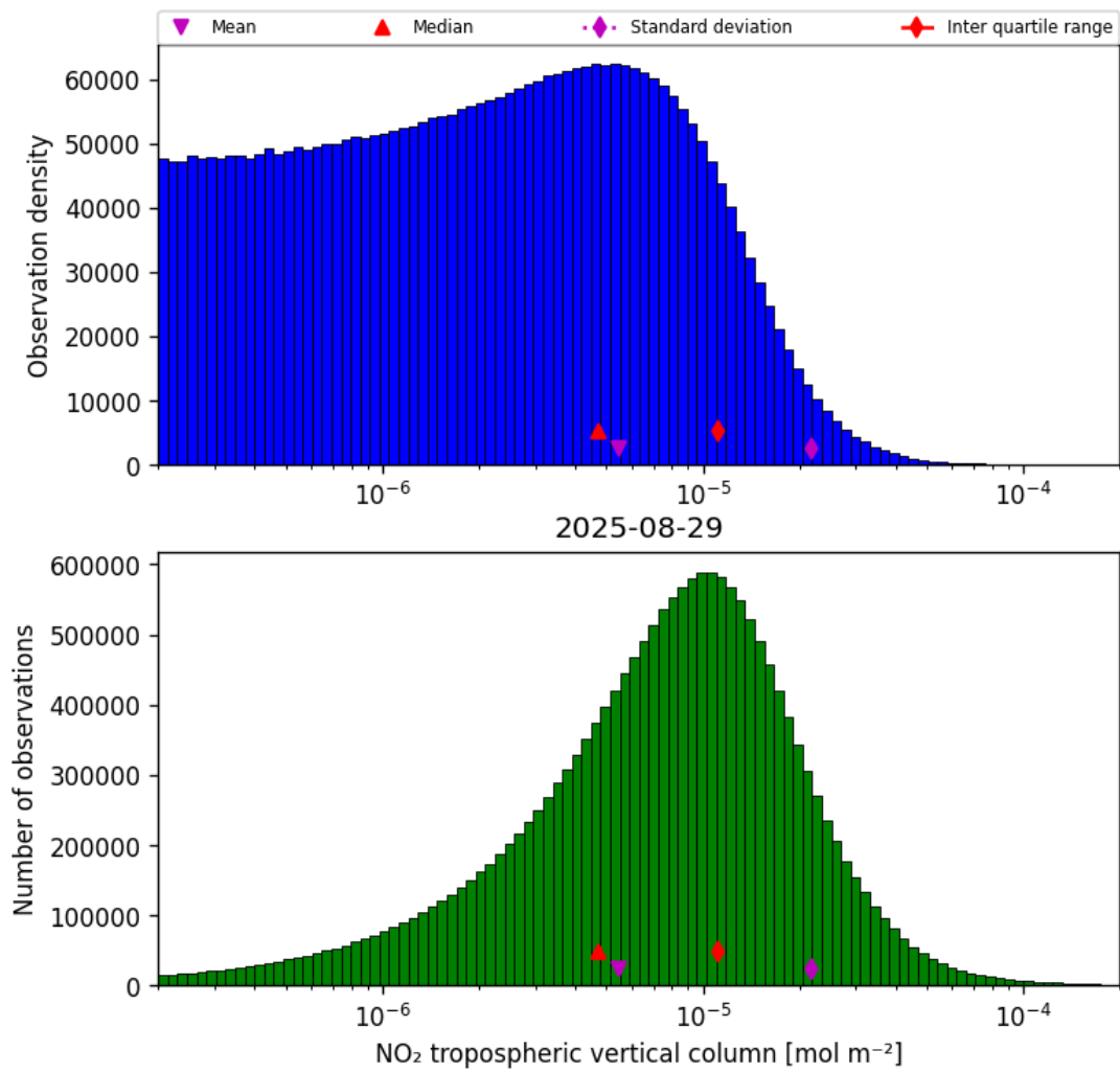
Figure 27: Histogram of “NO 2 tropospheric vertical column” for 2025-08-29 to 2025-08-30
