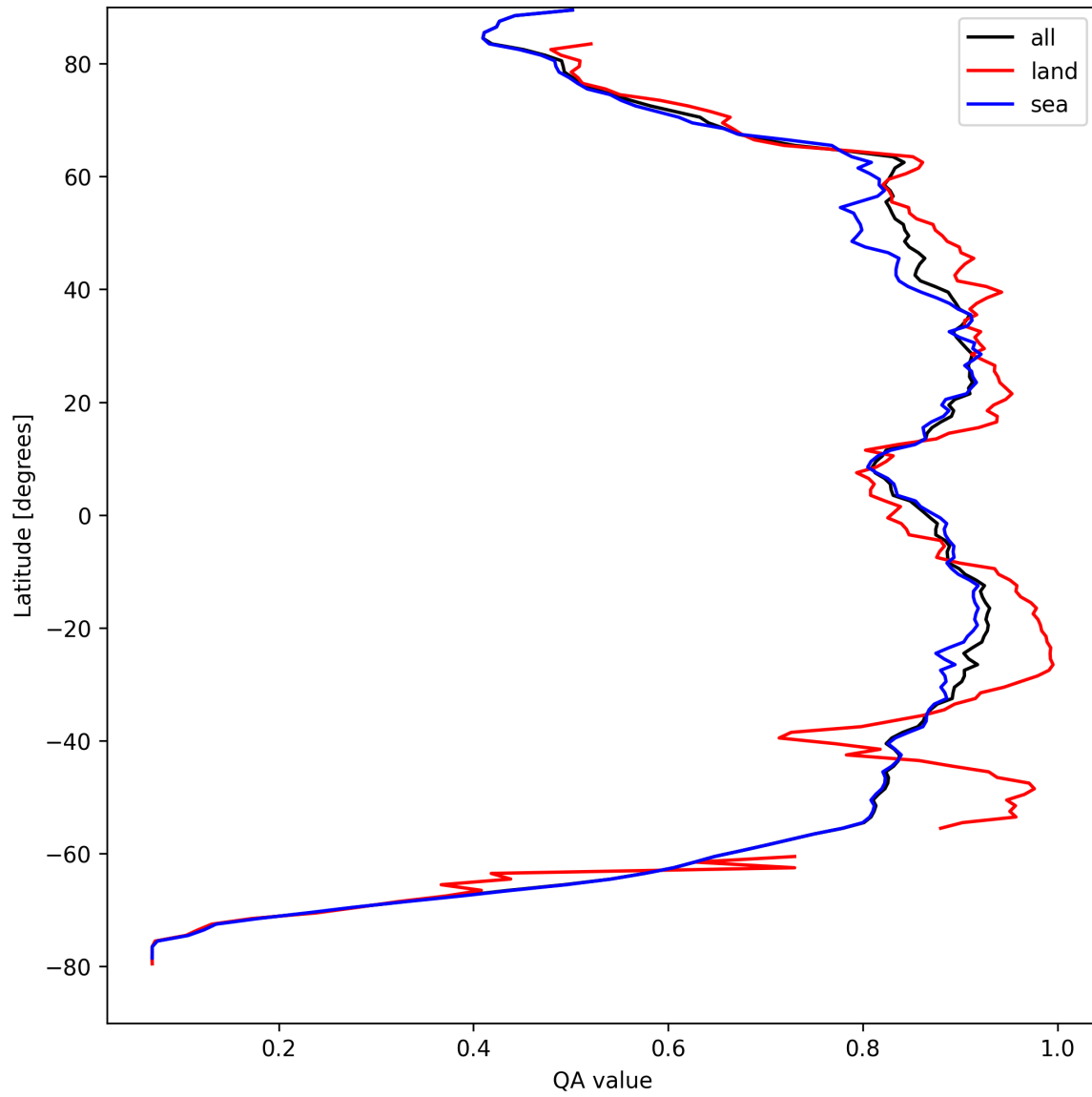
Figure 9: Zonal average of “QA value” for 2025-08-29 to 2025-08-30.
