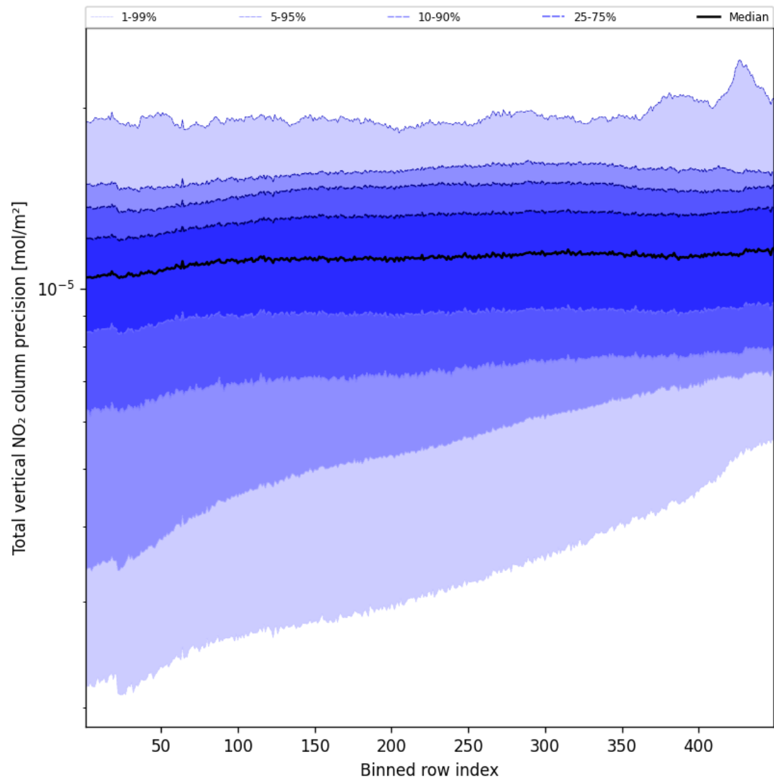
Figure 54: Along track statistics of “Total vertical NO 2 column precision” for 2025-08-29 to 2025-08-30
