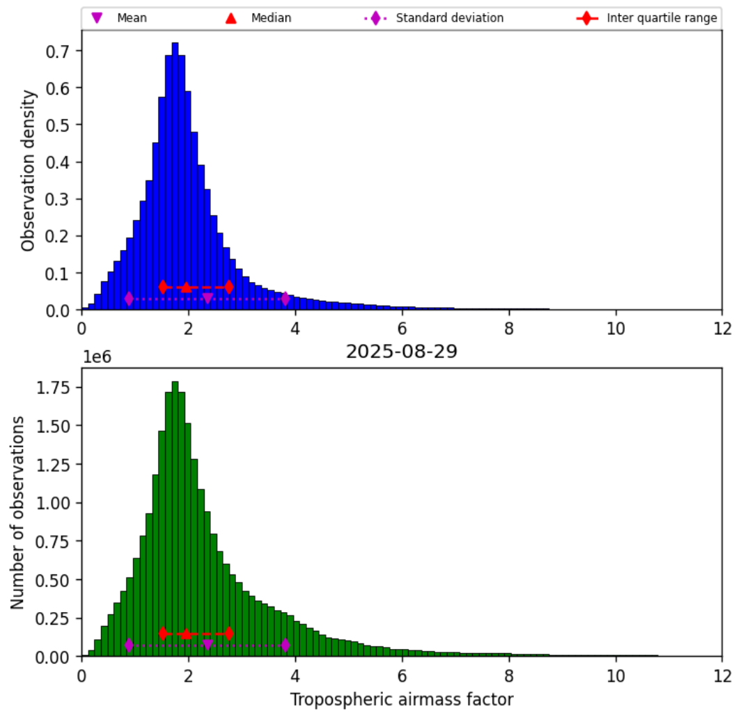
Figure 29: Histogram of “Tropospheric airmass factor” for 2025-08-29 to 2025-08-30
