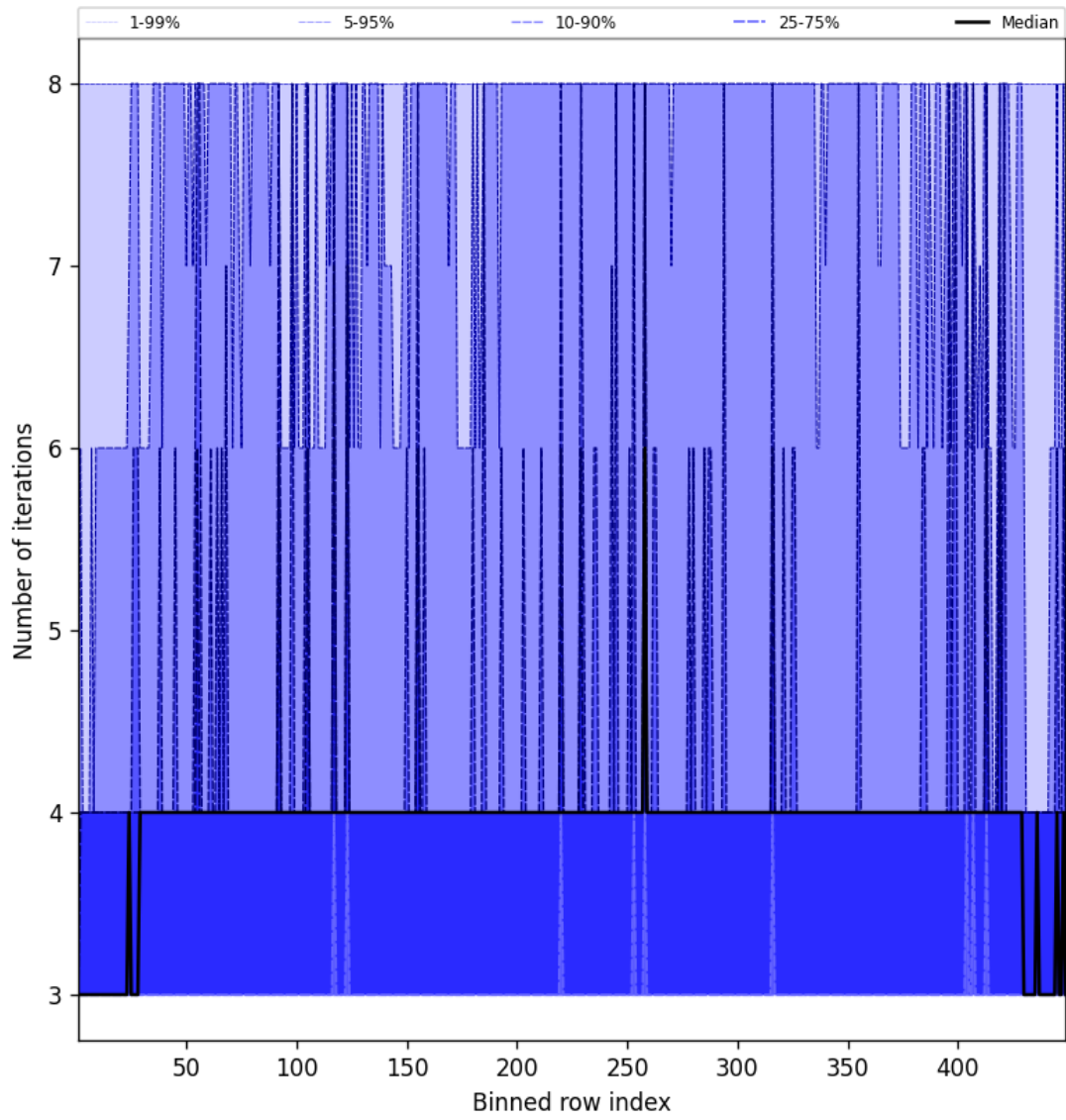
Figure 49: Along track statistics of “Number of iterations” for 2025-08-29 to 2025-08-30
