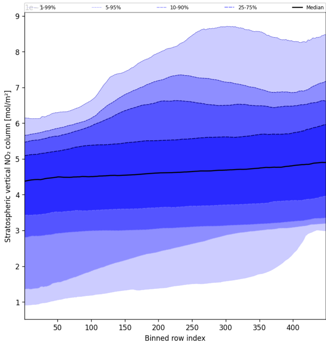
Figure 51: Along track statistics of “Stratospheric vertical NO 2 column” for 2025-08-29 to 2025-08-30
