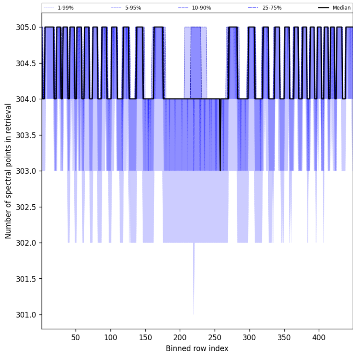
Figure 48: Along track statistics of “Number of spectral points in retrieval” for 2025-08-29 to 2025-08-30
