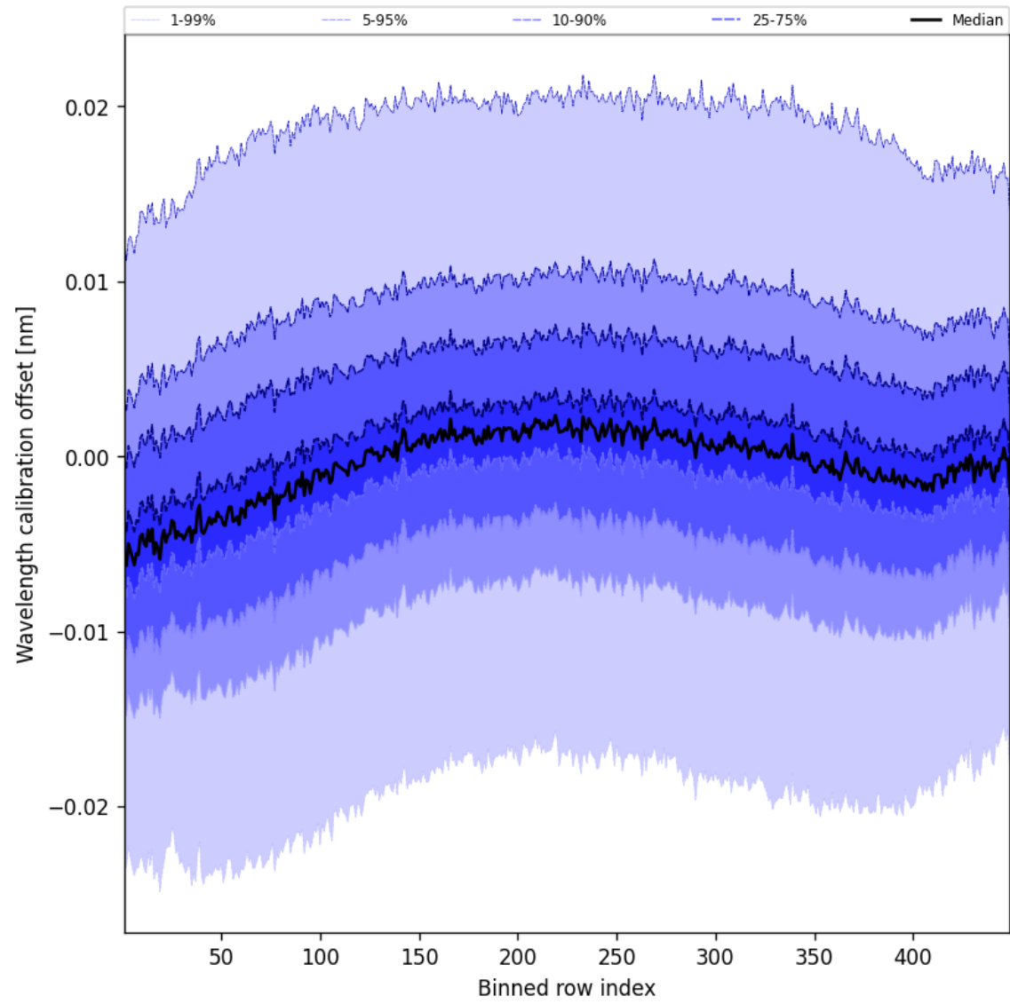
Figure 50: Along track statistics of “Wavelength calibration offset” for 2025-08-29 to 2025-08-30
