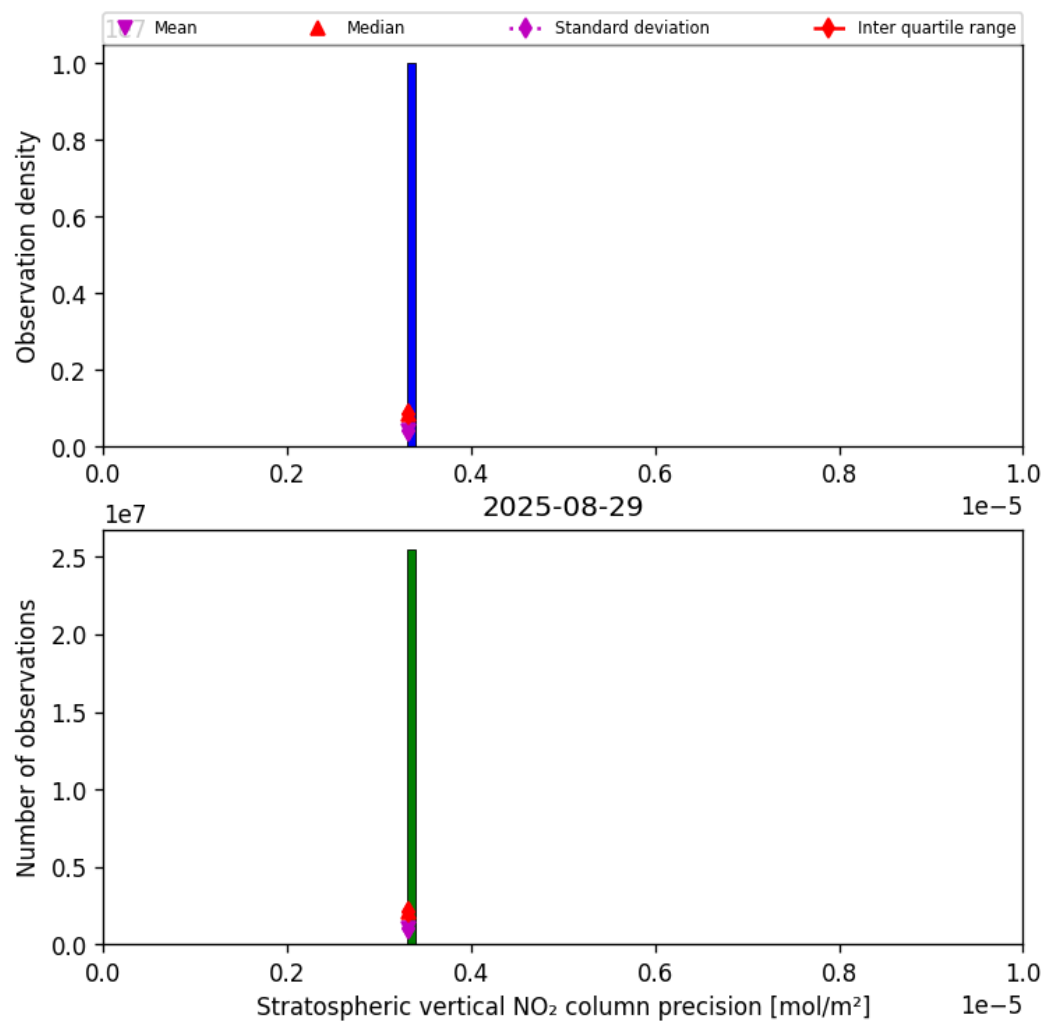
Figure 35: Histogram of “Stratospheric vertical NO 2 column precision” for 2025-08-29 to 2025-08-30
