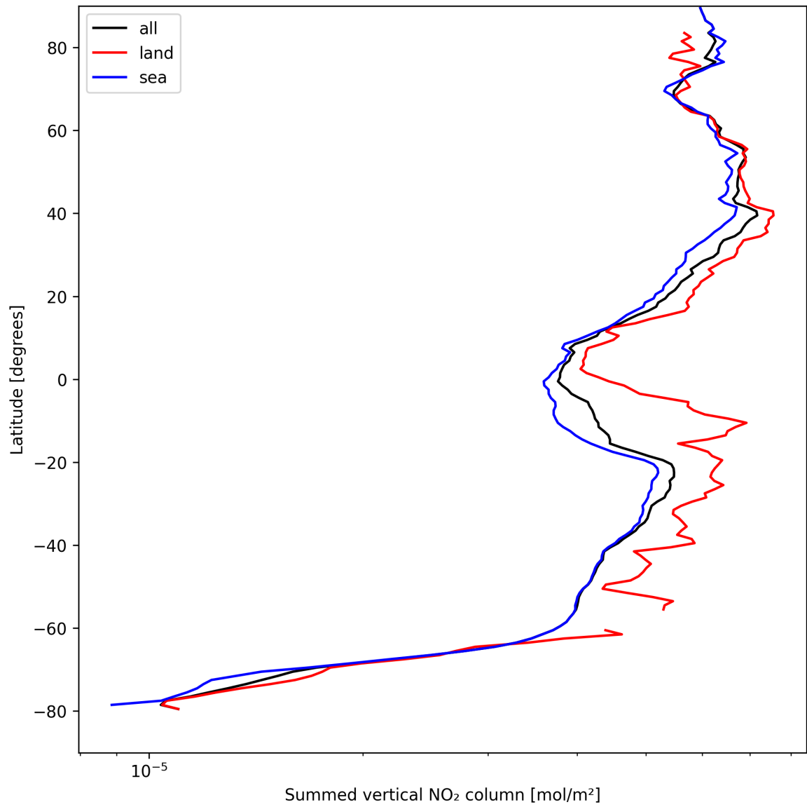
Figure 21: Zonal average of “Summed vertical NO 2 column” for 2025-08-29 to 2025-08-30.
