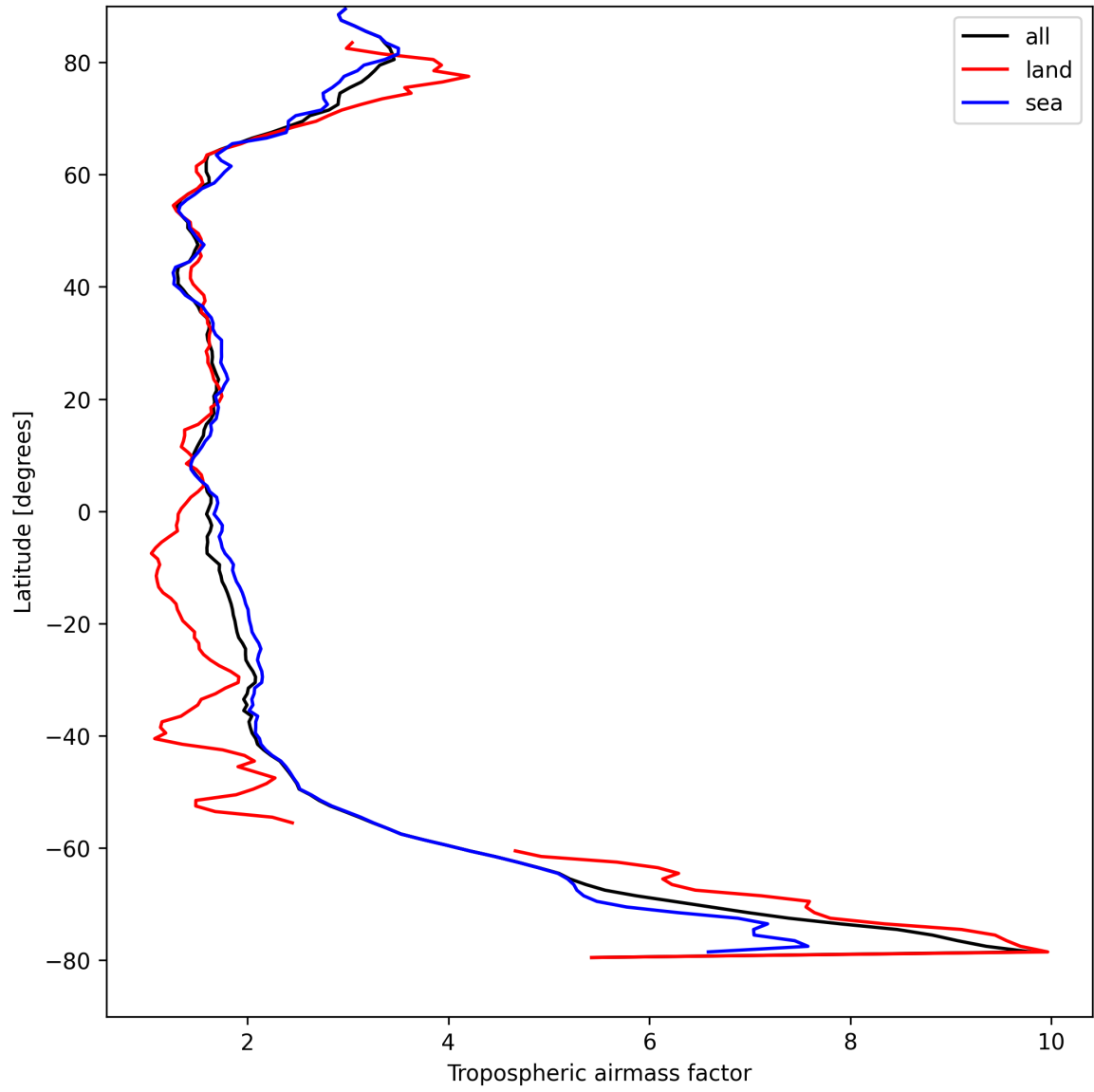
Figure 12: Zonal average of “Tropospheric airmass factor” for 2025-08-29 to 2025-08-30.
