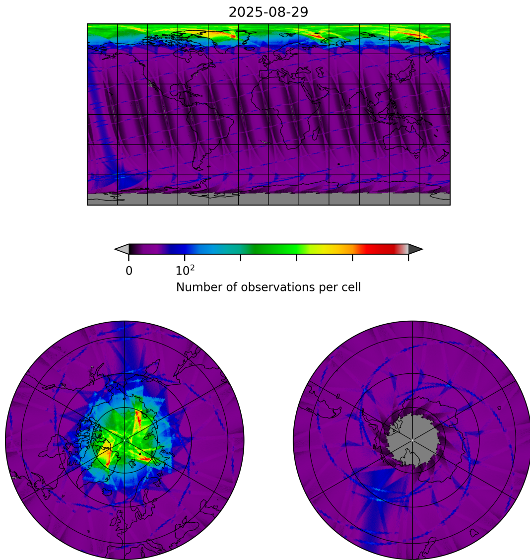
Figure 8: Map of the number of observations for 2025-08-29 to 2025-08-30
