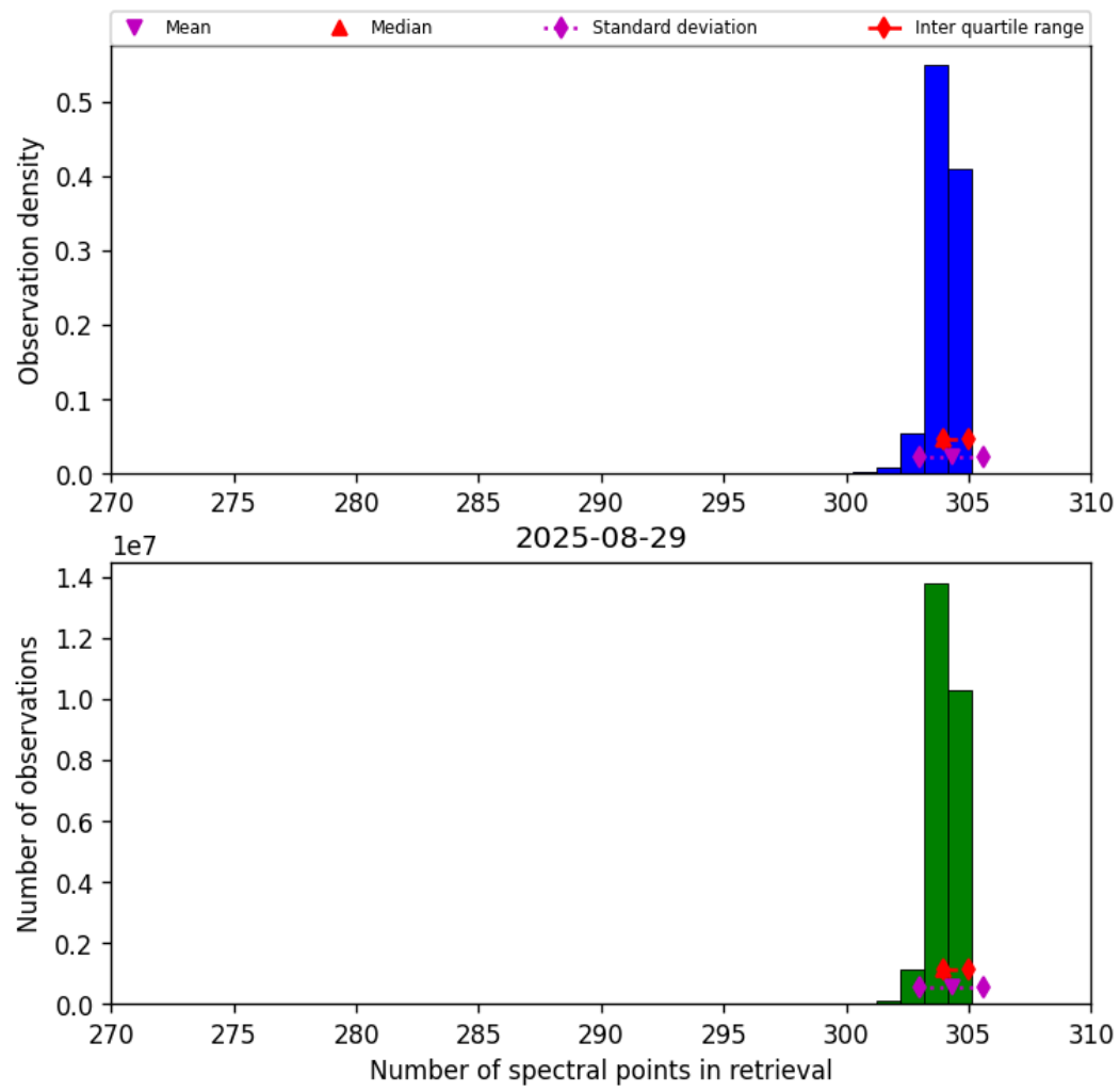
Figure 31: Histogram of “Number of spectral points in retrieval” for 2025-08-29 to 2025-08-30
