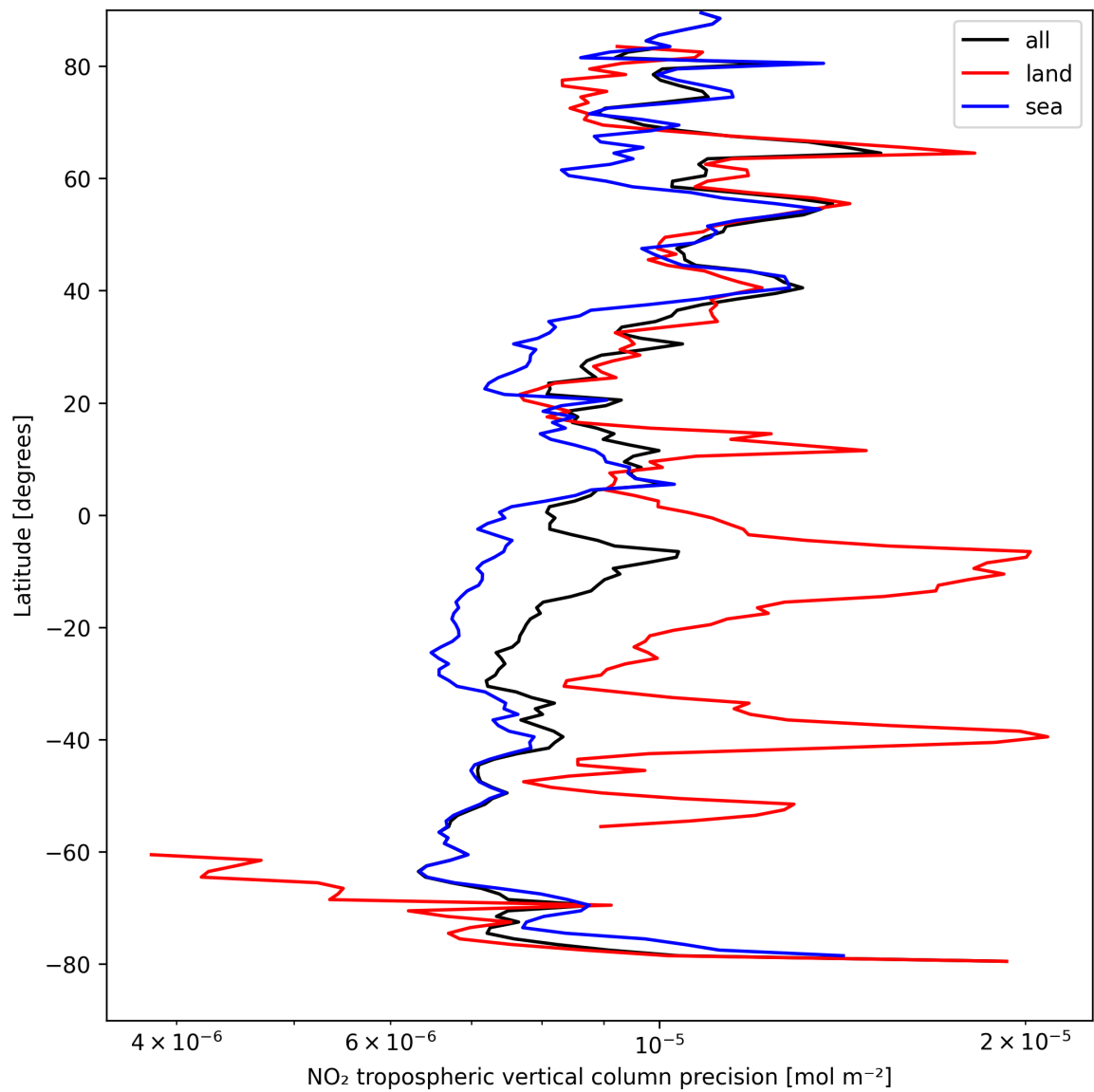
Figure 11: Zonal average of “NO 2 tropospheric vertical column precision” for 2025-08-29 to 2025-08-30.
