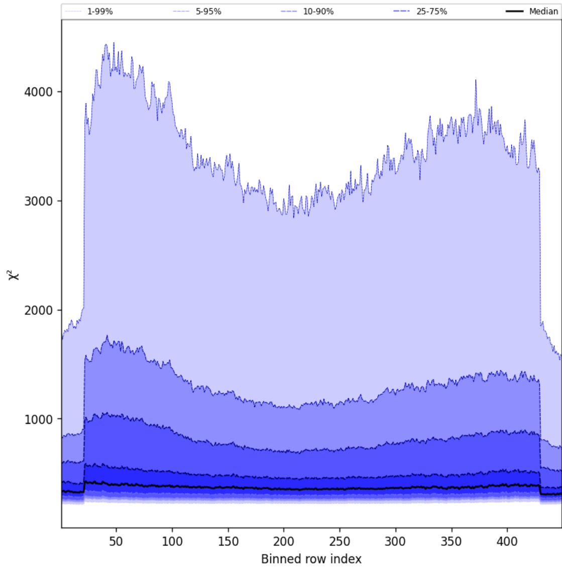
Figure 57: Along track statistics of “ \chi^2 ” for 2025-08-29 to 2025-08-30
