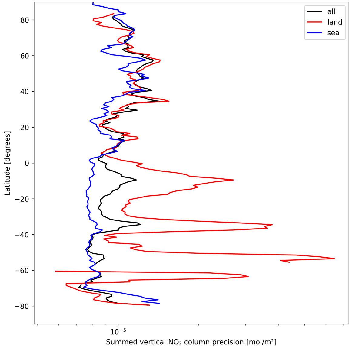
Figure 22: Zonal average of “Summed vertical NO 2 column precision” for 2025-08-30 to 2025-08-31.
