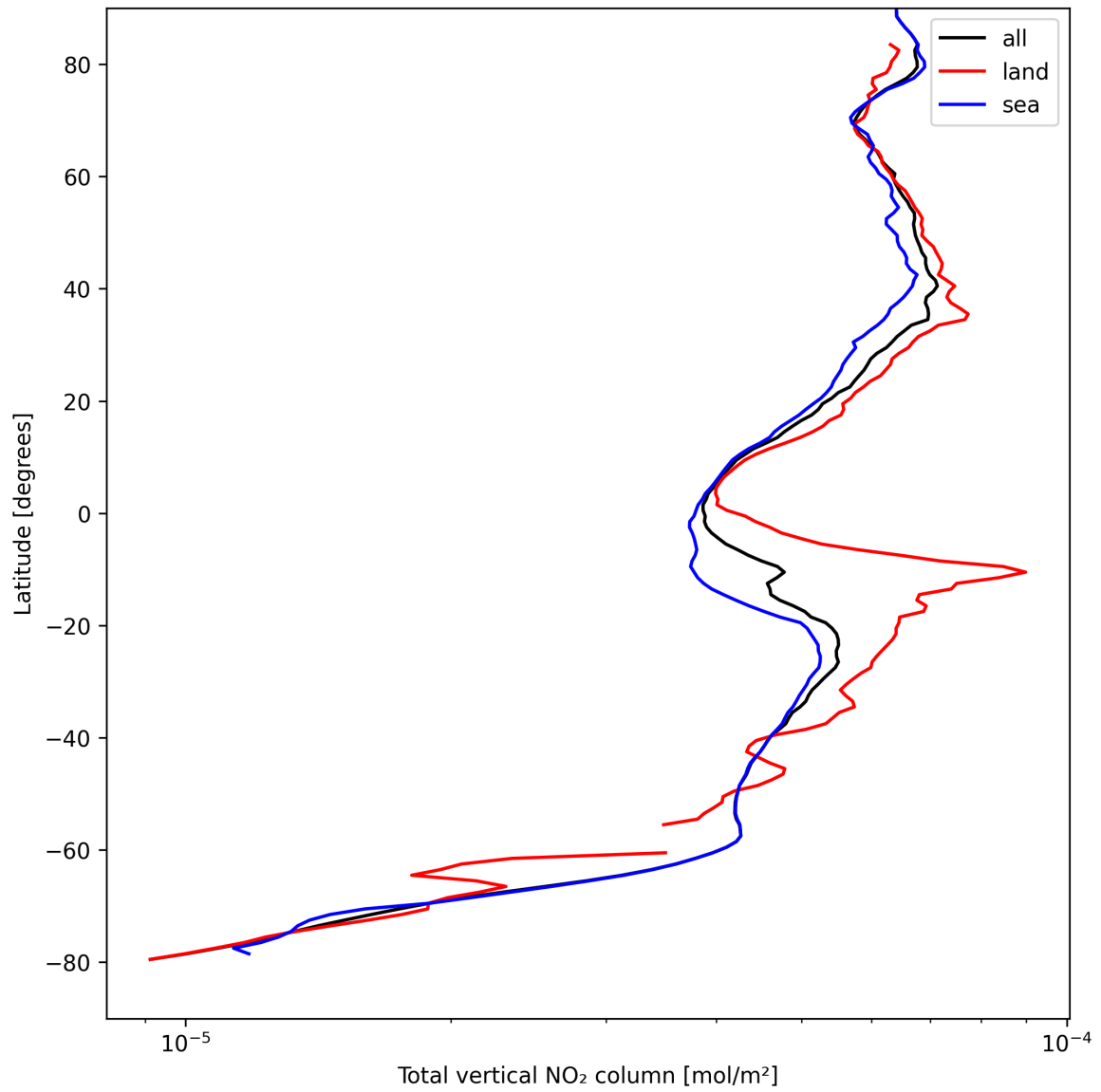
Figure 19: Zonal average of “Total vertical NO 2 column” for 2025-08-30 to 2025-08-31.
