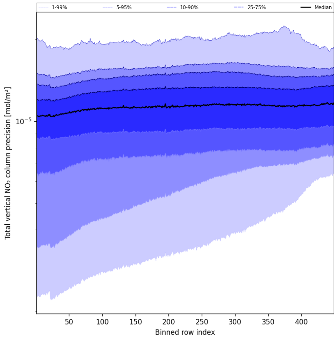
Figure 54: Along track statistics of “Total vertical NO 2 column precision” for 2025-08-30 to 2025-08-31
