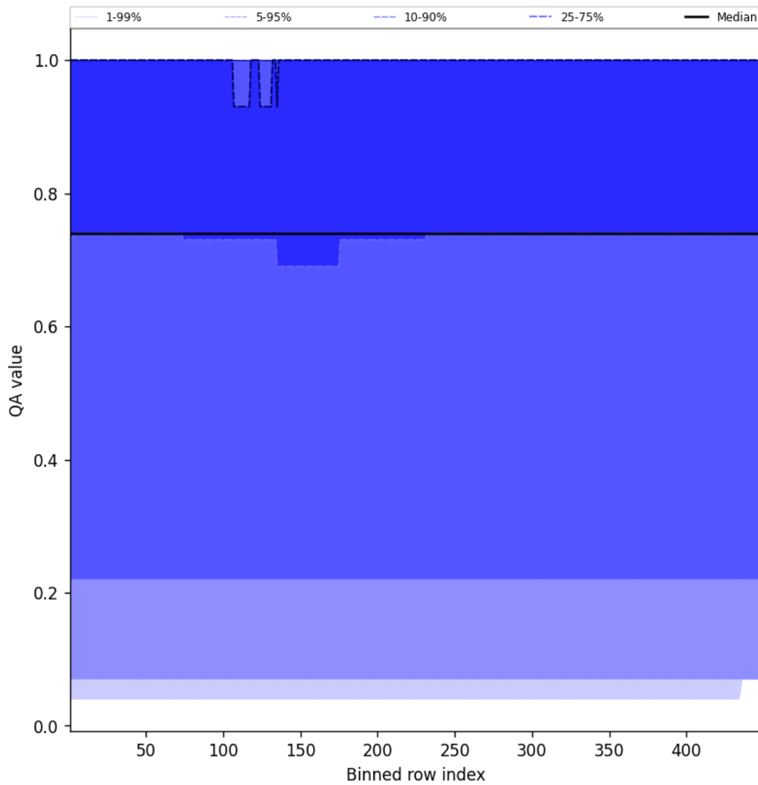
Figure 43: Along track statistics of “QA value” for 2025-08-30 to 2025-08-31
