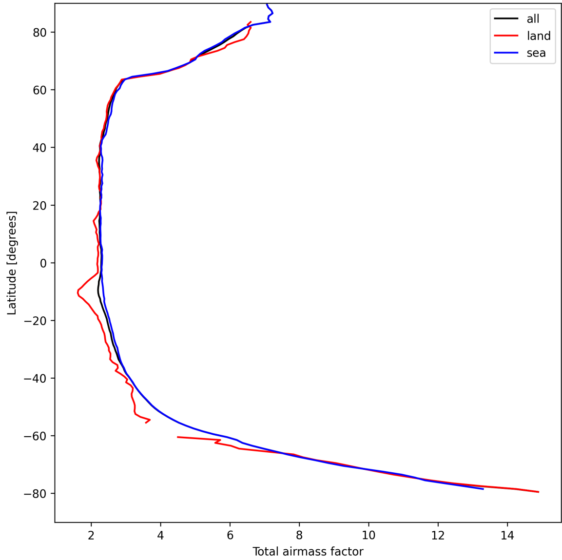
Figure 13: Zonal average of “Total airmass factor” for 2025-08-30 to 2025-08-31.
