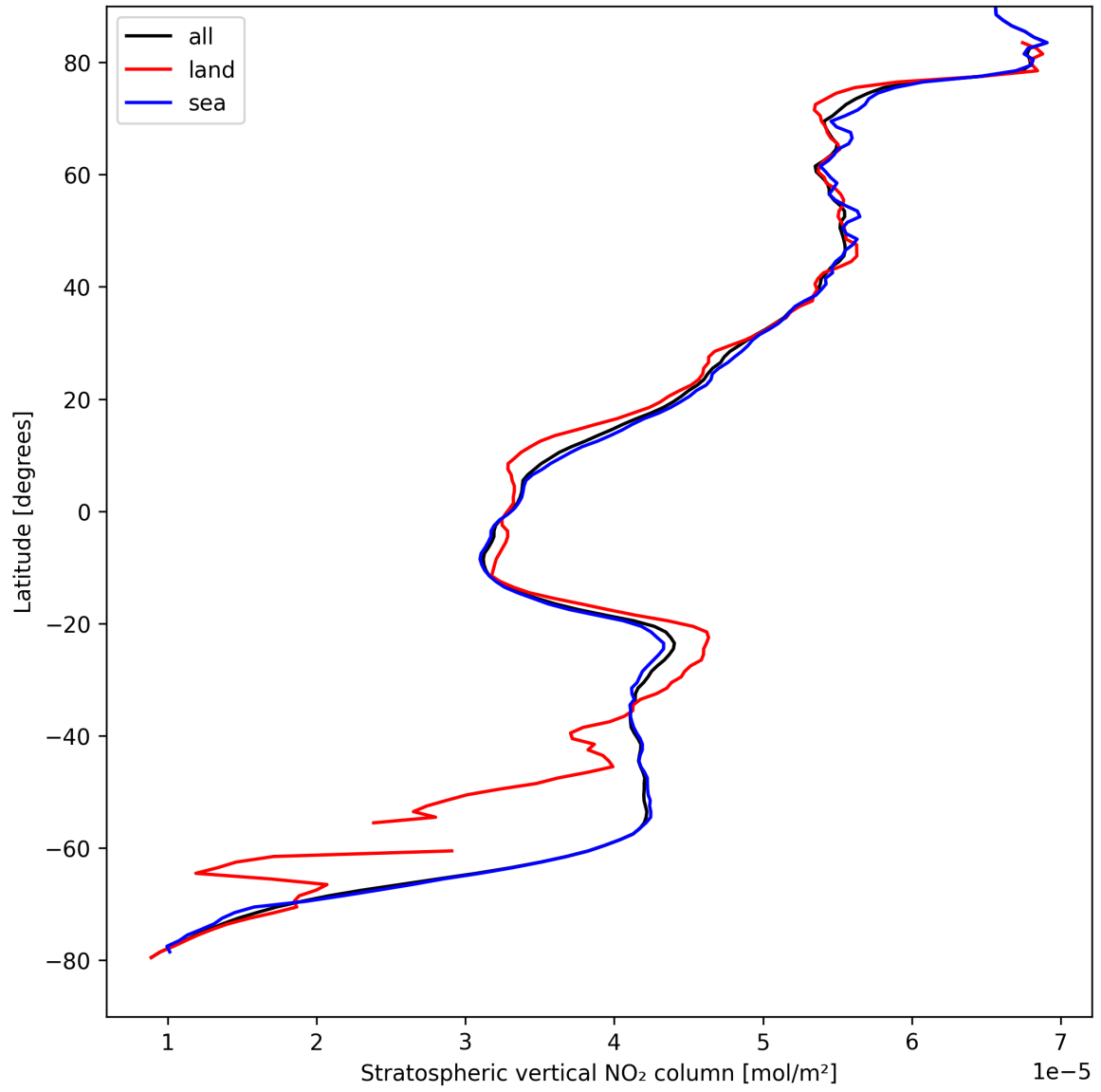
Figure 17: Zonal average of “Stratospheric vertical NO 2 column” for 2025-08-30 to 2025-08-31.
