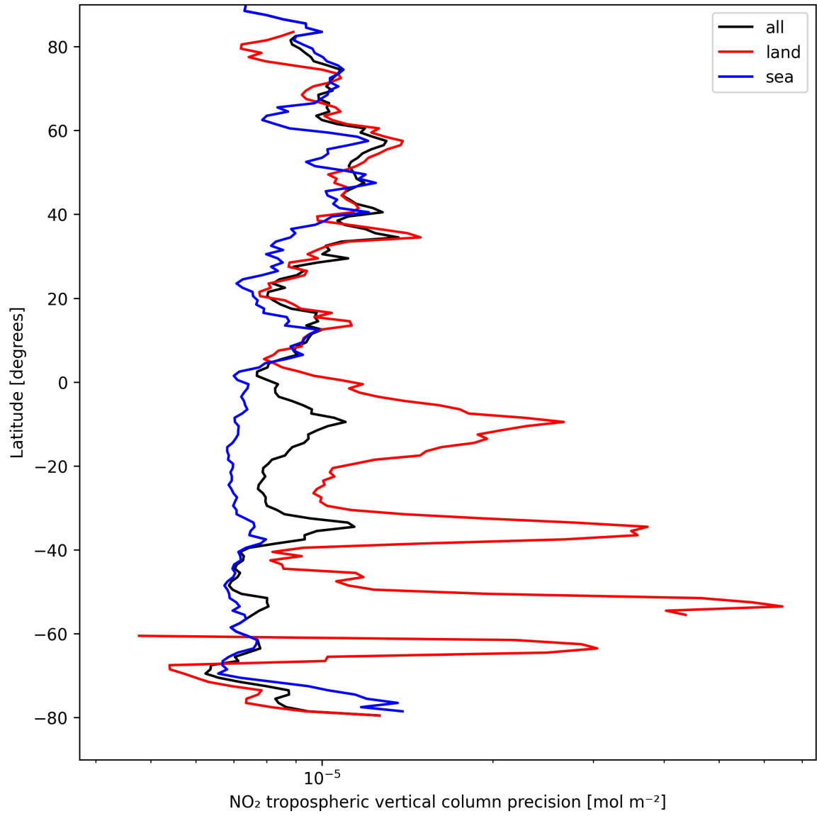
Figure 11: Zonal average of “NO 2 tropospheric vertical column precision” for 2025-08-30 to 2025-08-31.
