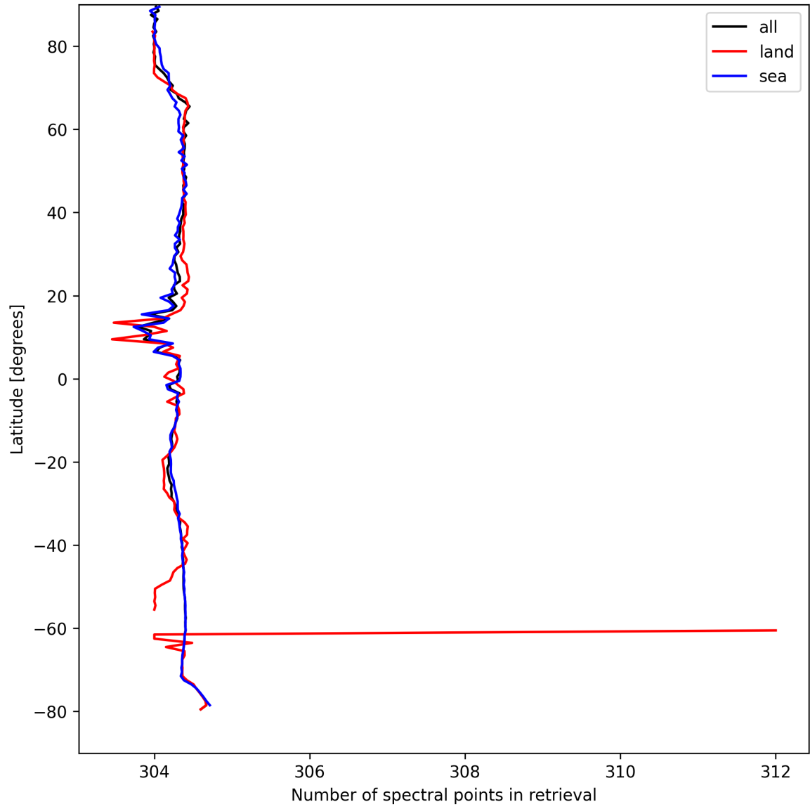
Figure 14: Zonal average of “Number of spectral points in retrieval” for 2025-08-30 to 2025-08-31.
