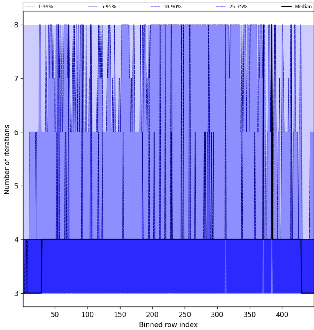
Figure 49: Along track statistics of “Number of iterations” for 2025-08-30 to 2025-08-31
