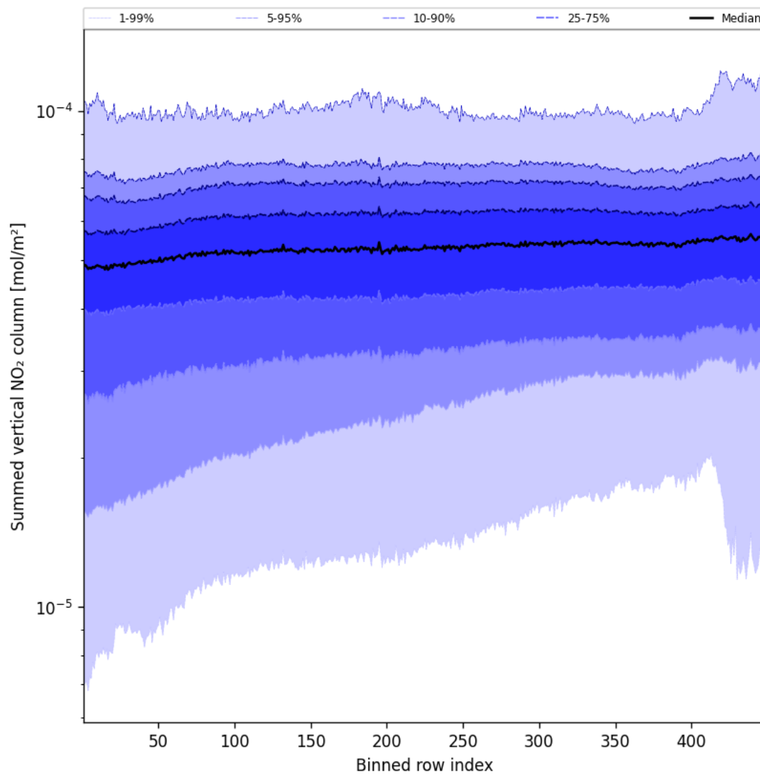
Figure 55: Along track statistics of “Summed vertical NO 2 column” for 2025-08-30 to 2025-08-31
