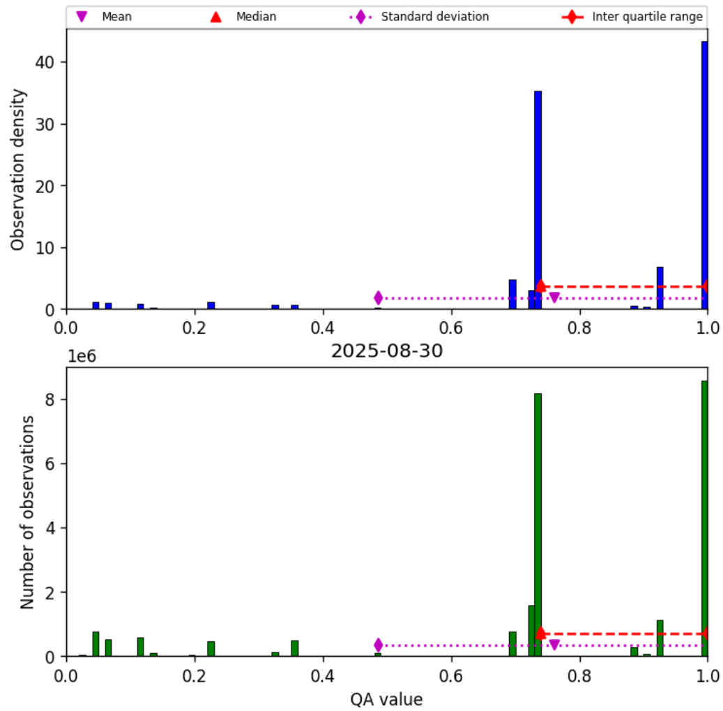
Figure 26: Histogram of “QA value” for 2025-08-30 to 2025-08-31
