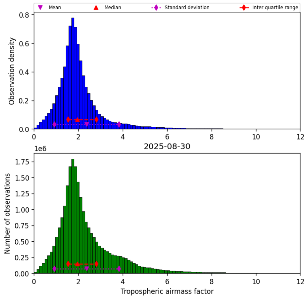
Figure 29: Histogram of “Tropospheric airmass factor” for 2025-08-30 to 2025-08-31
