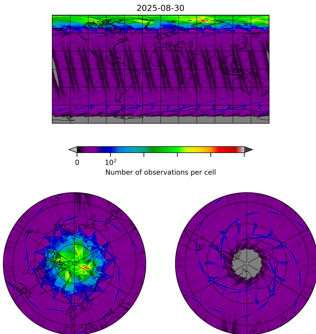
Figure 8: Map of the number of observations for 2025-08-30 to 2025-08-31
