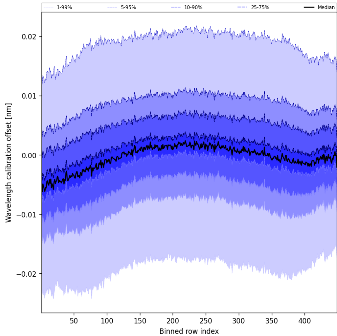
Figure 50: Along track statistics of “Wavelength calibration offset” for 2025-08-30 to 2025-08-31
