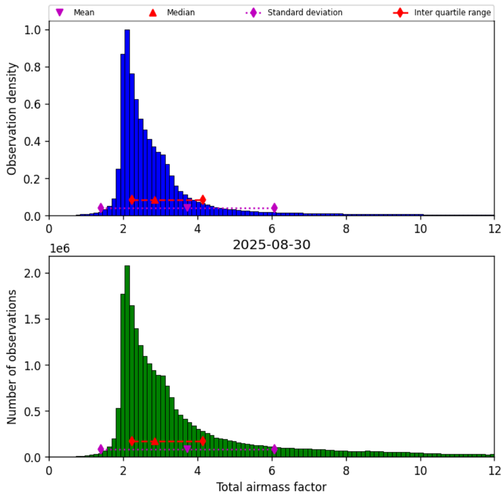
Figure 30: Histogram of “Total airmass factor” for 2025-08-30 to 2025-08-31
