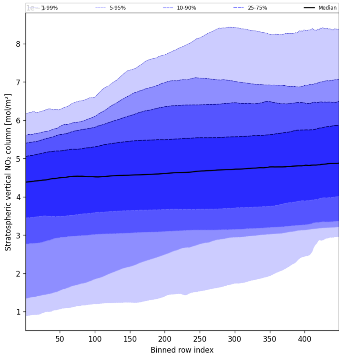
Figure 51: Along track statistics of “Stratospheric vertical NO 2 column” for 2025-08-30 to 2025-08-31
