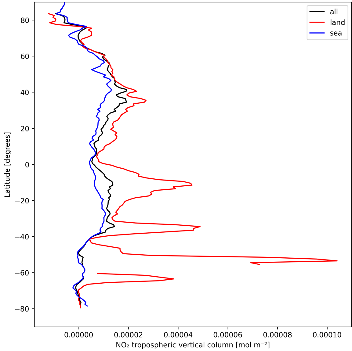
Figure 10: Zonal average of “NO 2 tropospheric vertical column” for 2025-08-30 to 2025-08-31.
