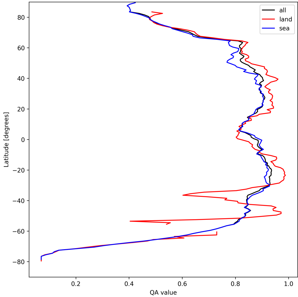
Figure 9: Zonal average of “QA value” for 2025-08-30 to 2025-08-31.
