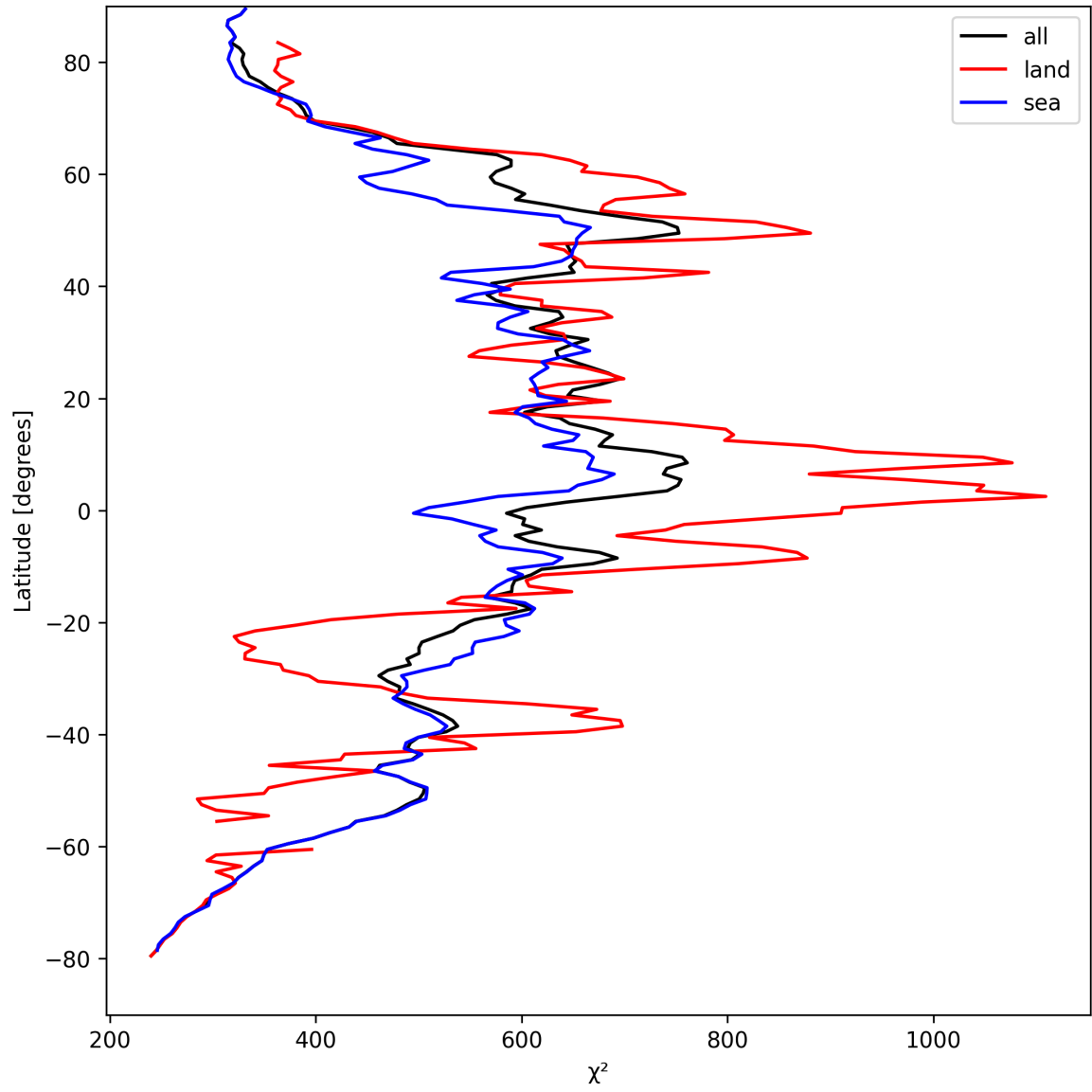
Figure 23: Zonal average of “ \chi^2 ” for 2025-08-30 to 2025-08-31.
