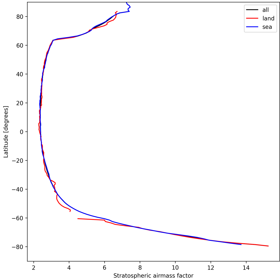
Figure 25: Zonal average of “Stratospheric airmass factor” for 2025-08-30 to 2025-08-31.
