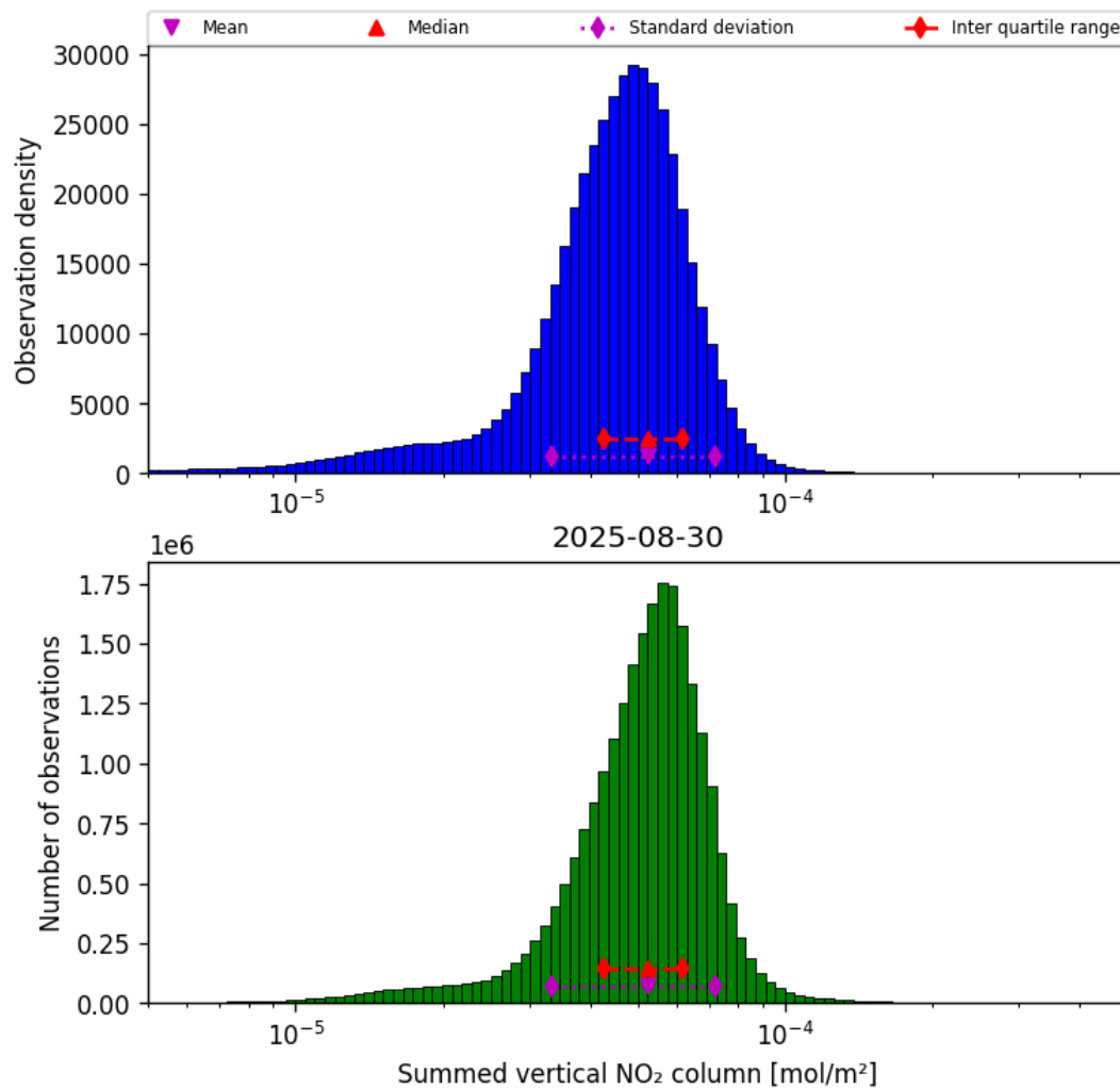
Figure 38: Histogram of "Summed vertical NO 2 column" for 2025-08-30 to 2025-08-31
