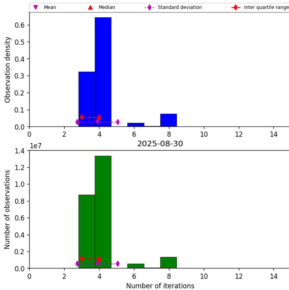
Figure 32: Histogram of “Number of iterations” for 2025-08-30 to 2025-08-31
