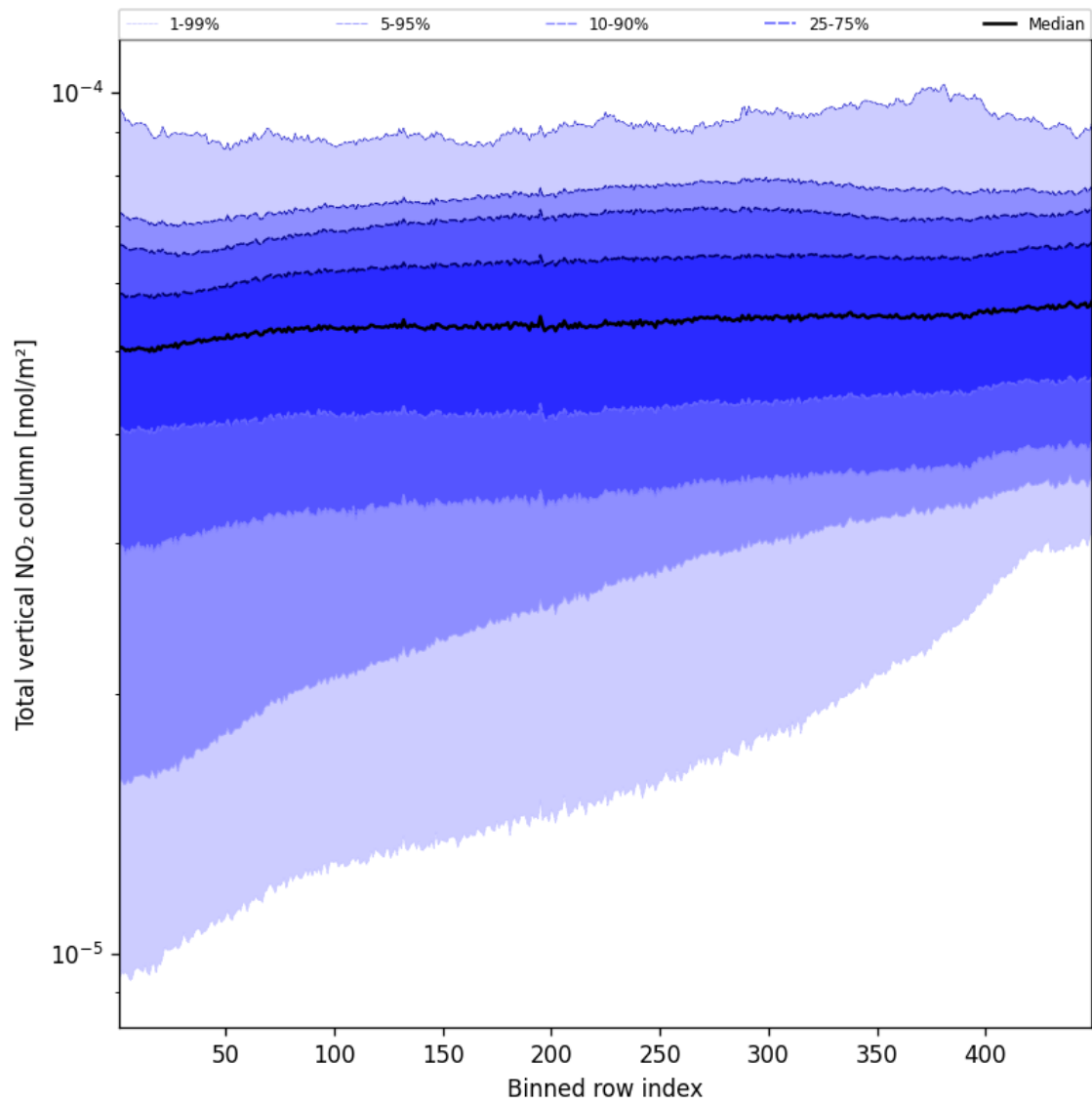
Figure 53: Along track statistics of “Total vertical NO 2 column” for 2025-08-30 to 2025-08-31
