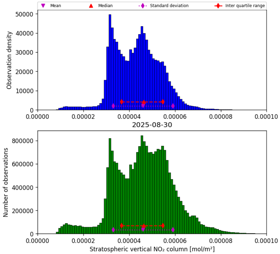
Figure 34: Histogram of “Stratospheric vertical NO 2 column” for 2025-08-30 to 2025-08-31
