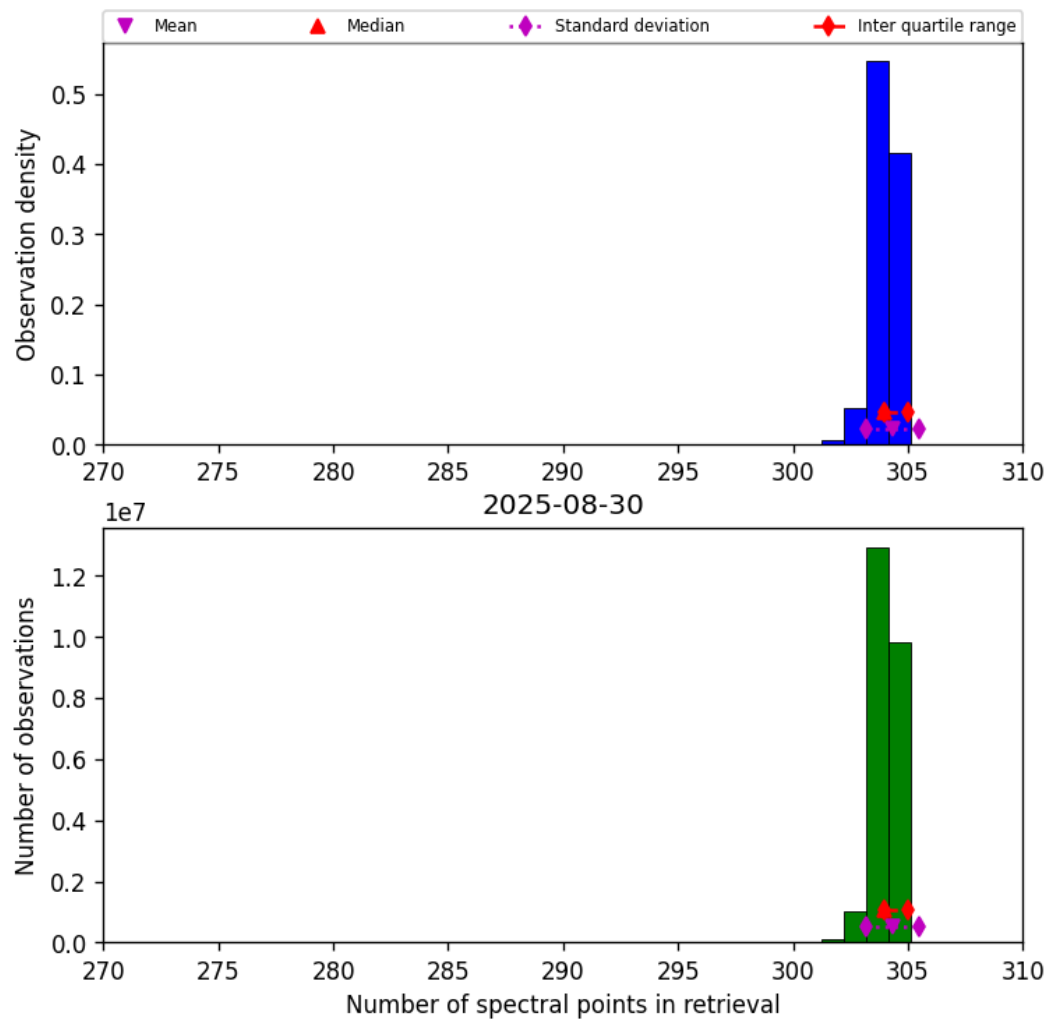
Figure 31: Histogram of “Number of spectral points in retrieval” for 2025-08-30 to 2025-08-31
