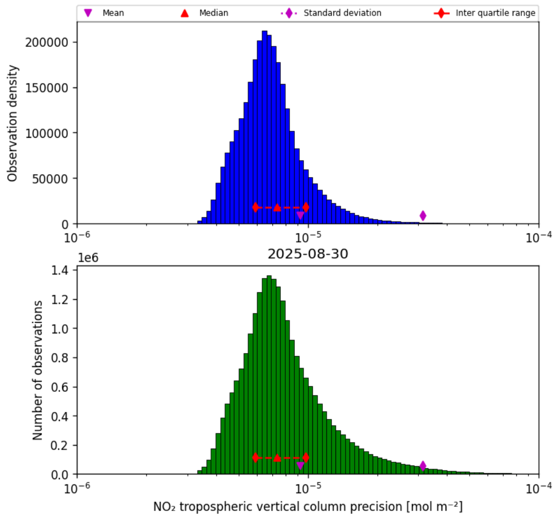
Figure 28: Histogram of “NO 2 tropospheric vertical column precision” for 2025-08-30 to 2025-08-31
