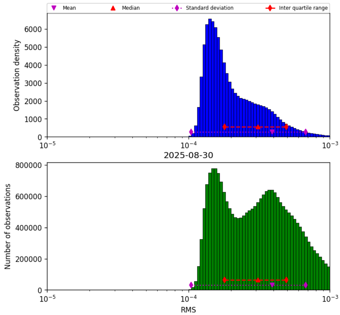
Figure 41: Histogram of “RMS” for 2025-08-30 to 2025-08-31
