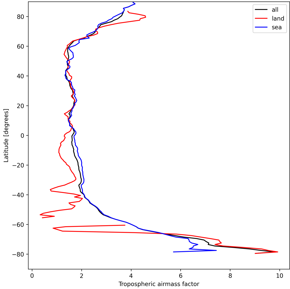
Figure 12: Zonal average of “Tropospheric airmass factor” for 2025-08-30 to 2025-08-31.
