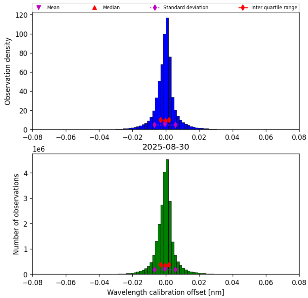
Figure 33: Histogram of “Wavelength calibration offset” for 2025-08-30 to 2025-08-31
