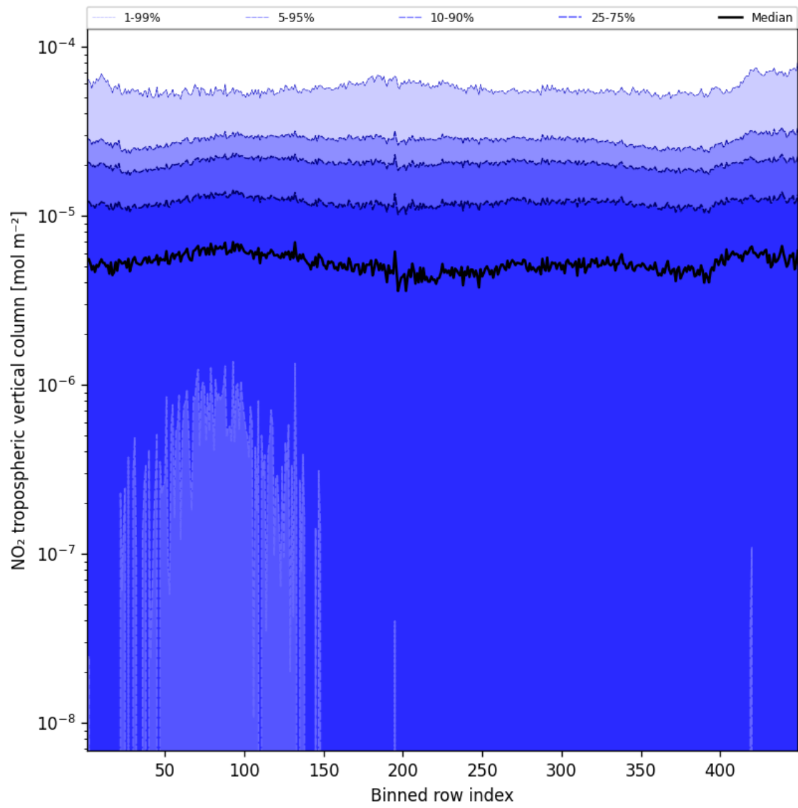
Figure 44: Along track statistics of “NO 2 tropospheric vertical column” for 2025-08-30 to 2025-08-31
