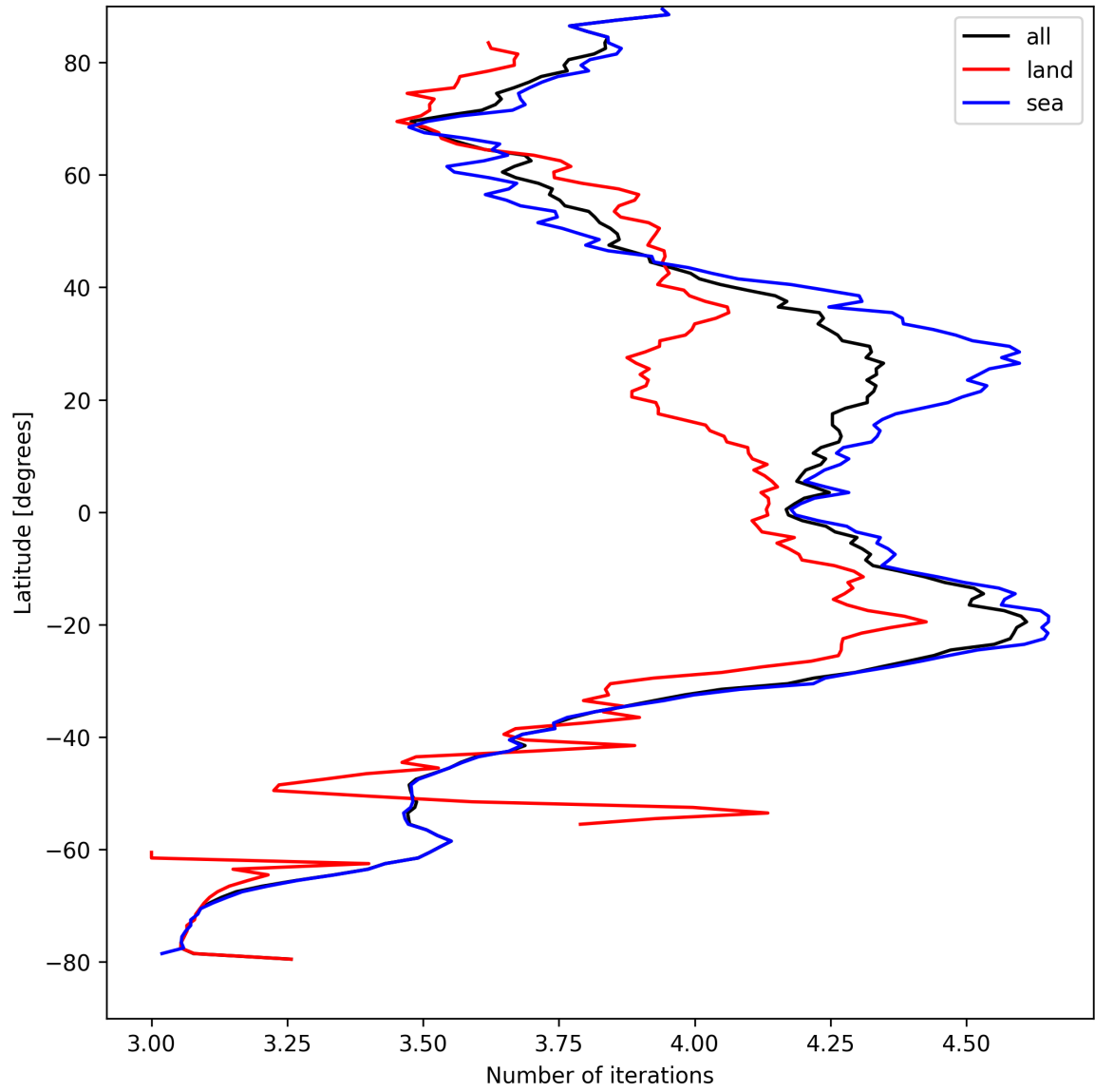
Figure 15: Zonal average of “Number of iterations” for 2025-08-30 to 2025-08-31.
