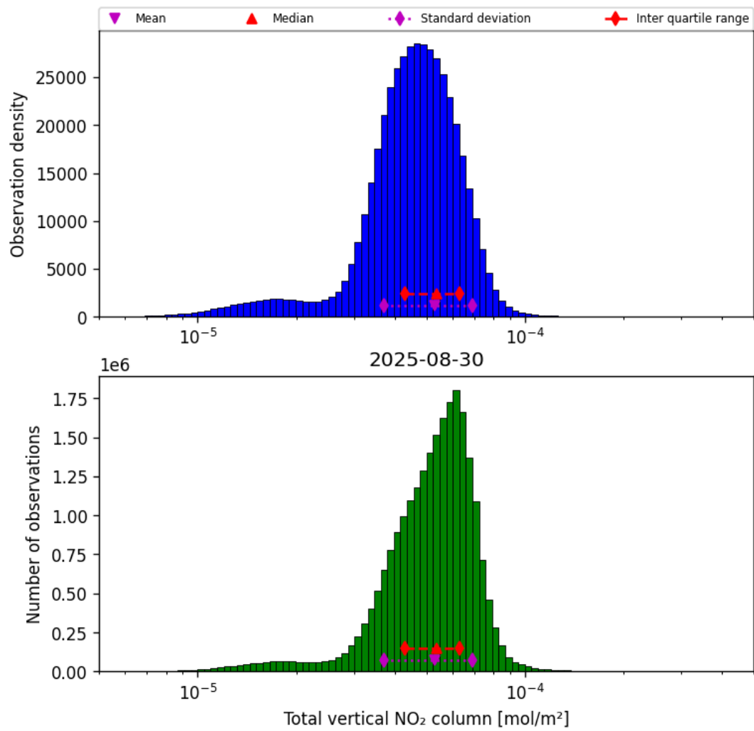
Figure 36: Histogram of “Total vertical NO 2 column” for 2025-08-30 to 2025-08-31
