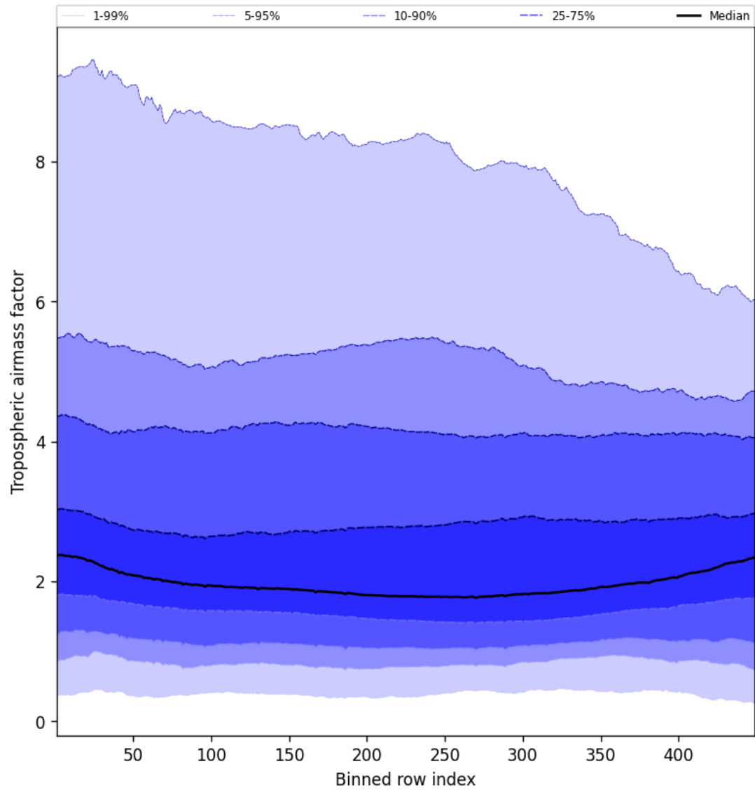
Figure 46: Along track statistics of “Tropospheric air mass factor” for 2025-08-30 to 2025-08-31
