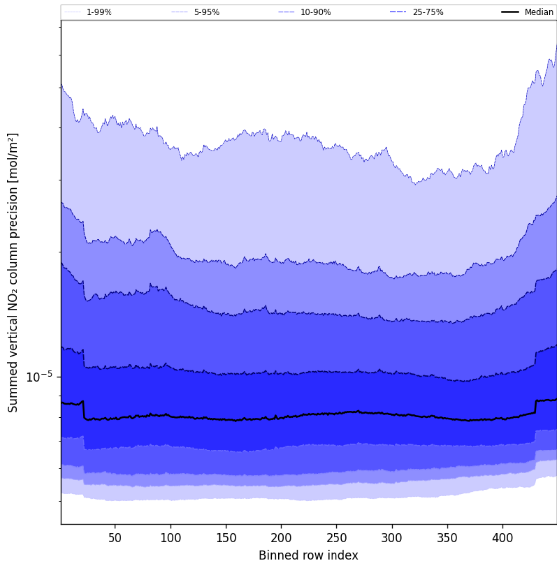
Figure 56: Along track statistics of “Summed vertical NO 2 column precision” for 2025-08-30 to 2025-08-31
