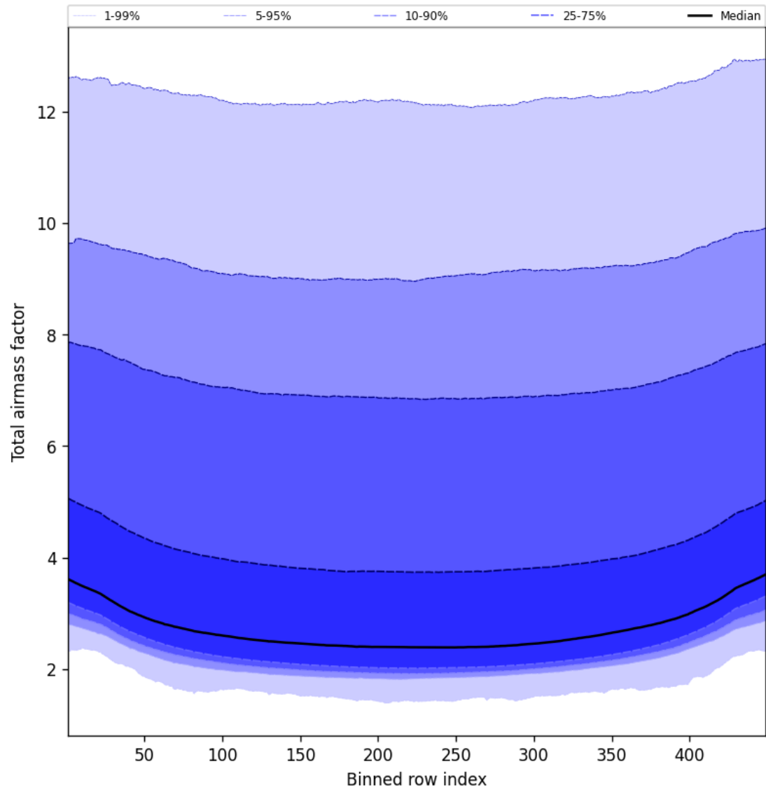
Figure 47: Along track statistics of “Total airmass factor” for 2025-08-30 to 2025-08-31
