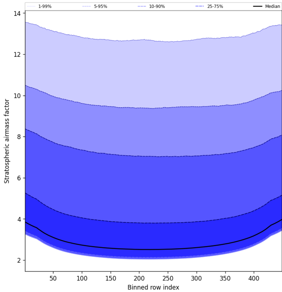
Figure 59: Along track statistics of “Stratospheric airmass factor” for 2025-08-30 to 2025-08-31
