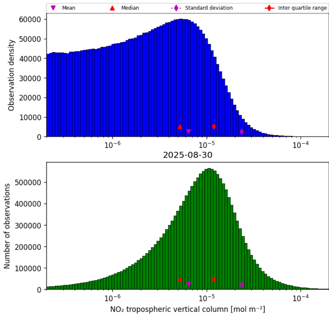
Figure 27: Histogram of “NO 2 tropospheric vertical column” for 2025-08-30 to 2025-08-31
