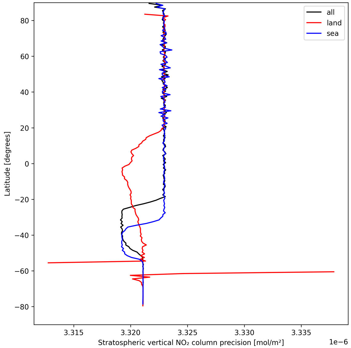
Figure 18: Zonal average of “Stratospheric vertical NO 2 column precision” for 2025-08-30 to 2025-08-31.
