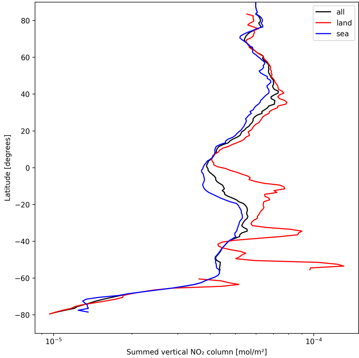
Figure 21: Zonal average of “Summed vertical NO 2 column” for 2025-08-30 to 2025-08-31.
