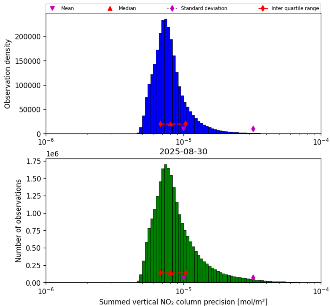
Figure 39: Histogram of “Summed vertical NO 2 column precision” for 2025-08-30 to 2025-08-31
