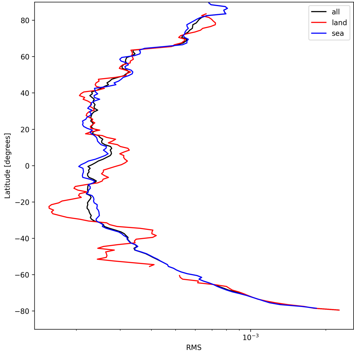
Figure 24: Zonal average of “RMS” for 2025-08-30 to 2025-08-31.
