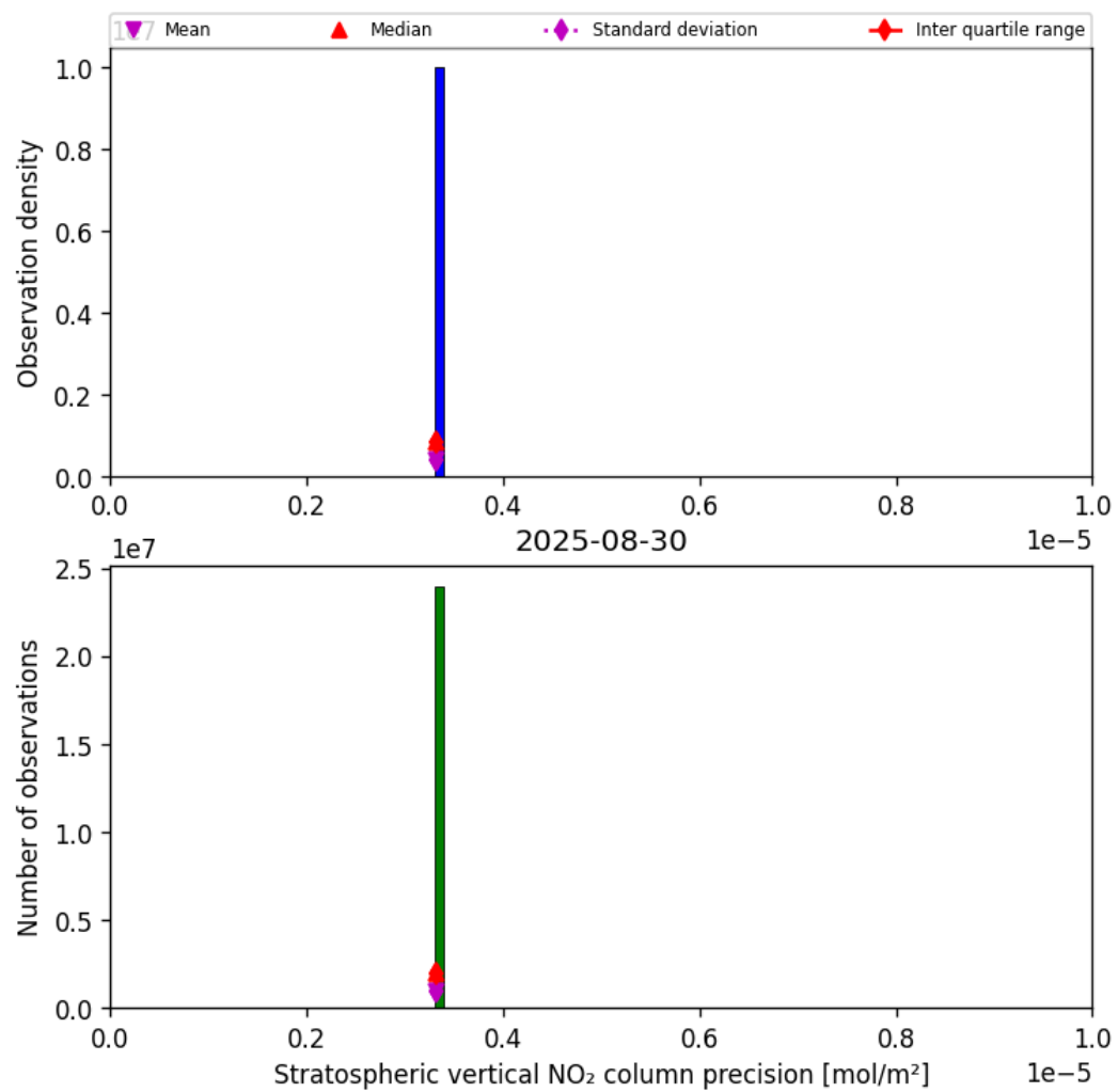
Figure 35: Histogram of “Stratospheric vertical NO 2 column precision” for 2025-08-30 to 2025-08-31
