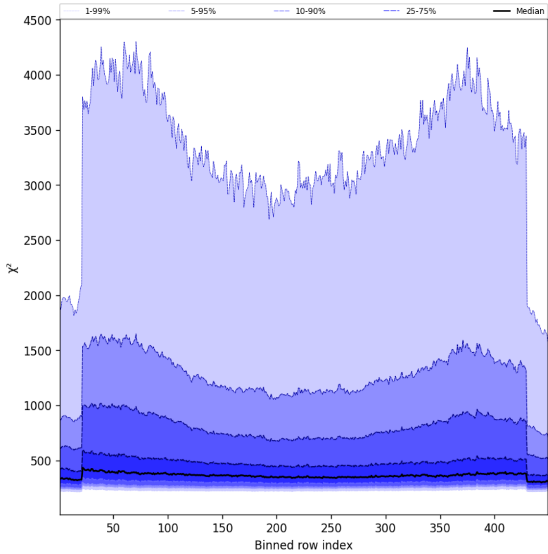
Figure 57: Along track statistics of “ \chi^2 ” for 2025-08-30 to 2025-08-31
