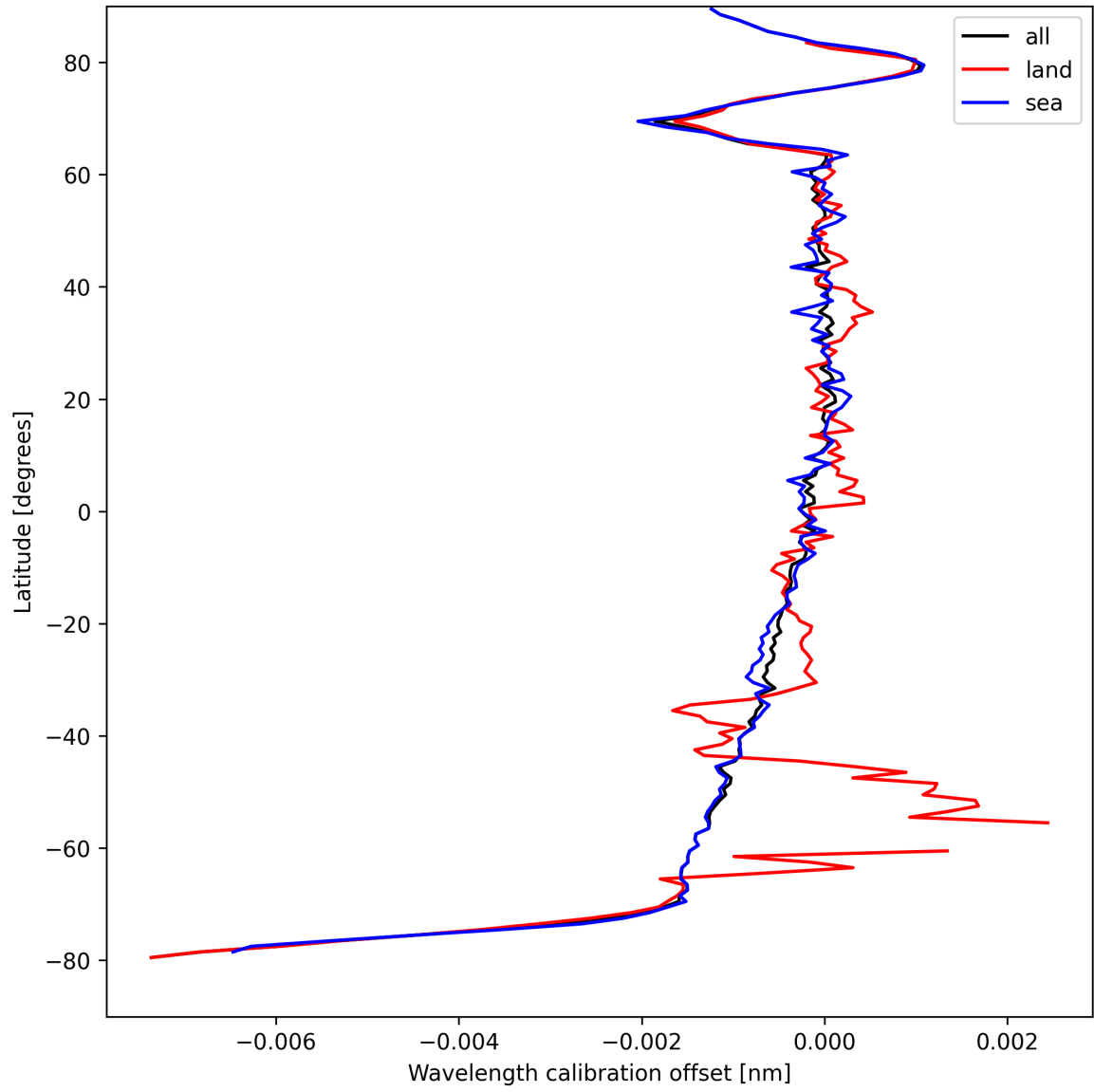
Figure 16: Zonal average of “Wavelength calibration offset” for 2025-08-30 to 2025-08-31.
