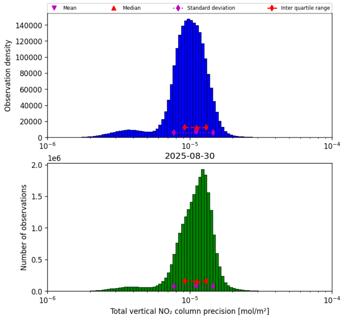
Figure 37: Histogram of “Total vertical NO 2 column precision” for 2025-08-30 to 2025-08-31
