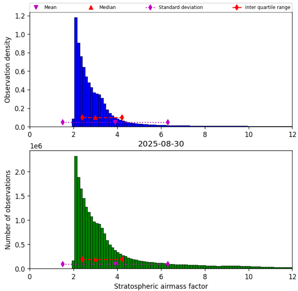
Figure 42: Histogram of “Stratospheric airmass factor” for 2025-08-30 to 2025-08-31
