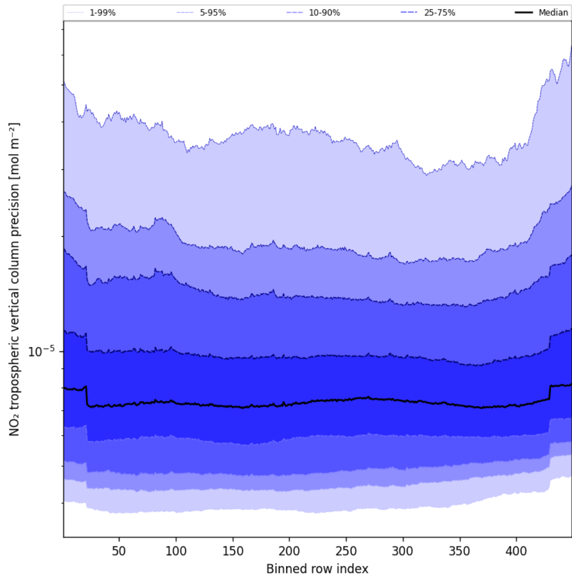
Figure 45: Along track statistics of “NO 2 tropospheric vertical column precision” for 2025-08-30 to 2025-08-31
