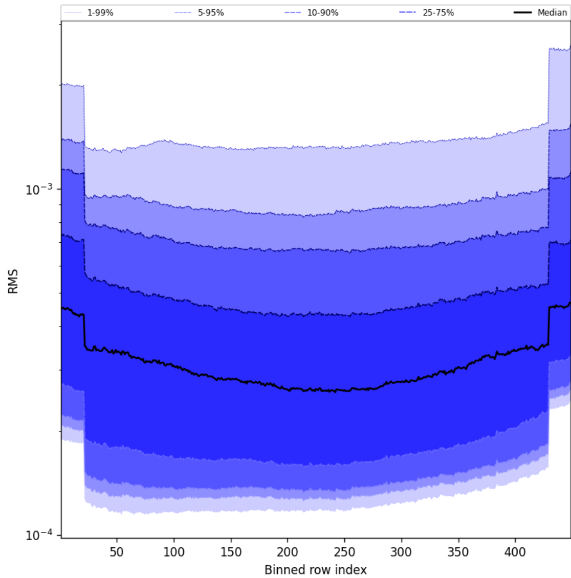
Figure 58: Along track statistics of “RMS” for 2025-08-30 to 2025-08-31
