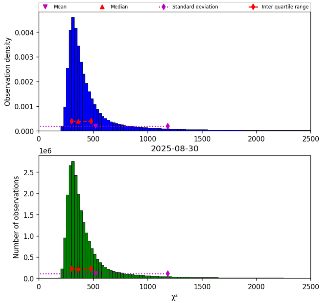
Figure 40: Histogram of “ \chi^2 ” for 2025-08-30 to 2025-08-31
