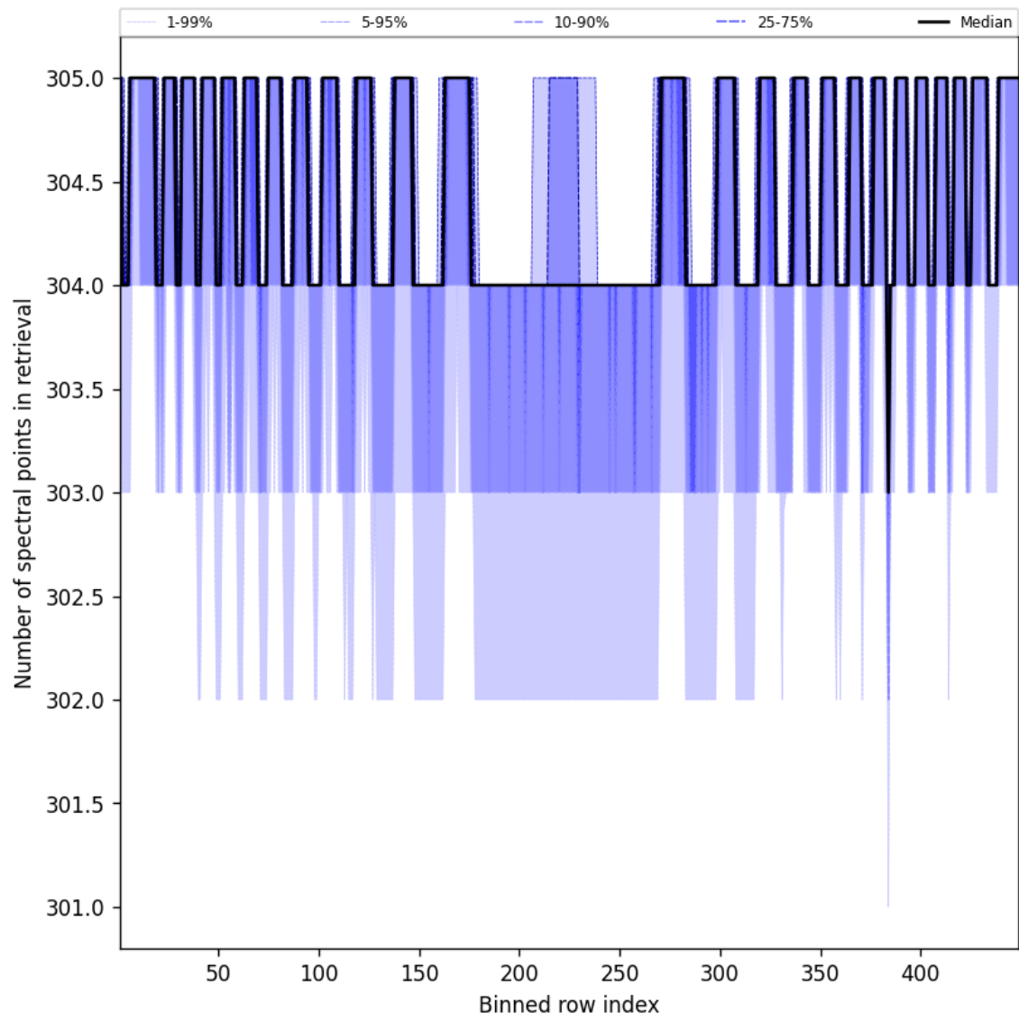
Figure 48: Along track statistics of “Number of spectral points in retrieval” for 2025-08-30 to 2025-08-31
