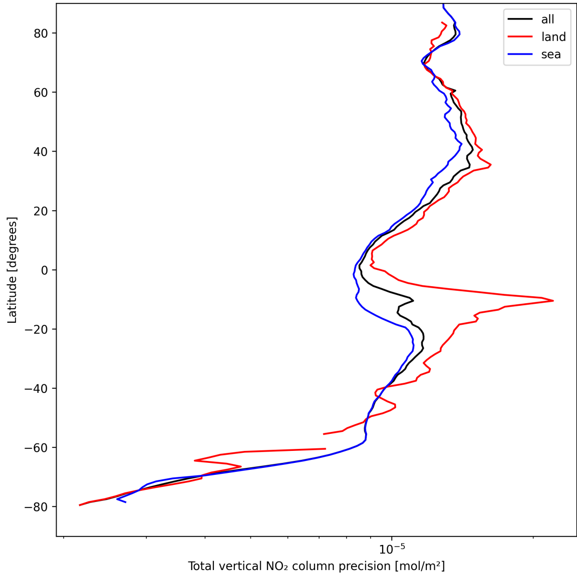
Figure 20: Zonal average of “Total vertical NO 2 column precision” for 2025-08-30 to 2025-08-31.
