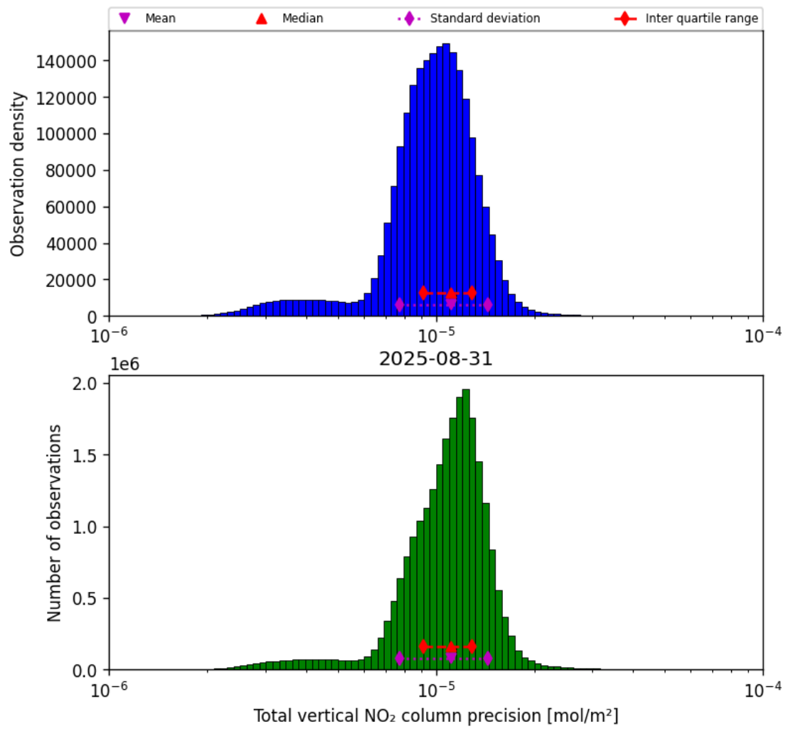
Figure 37: Histogram of “Total vertical NO 2 column precision” for 2025-08-31 to 2025-09-01
