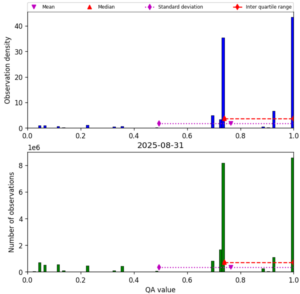
Figure 26: Histogram of “QA value” for 2025-08-31 to 2025-09-01
