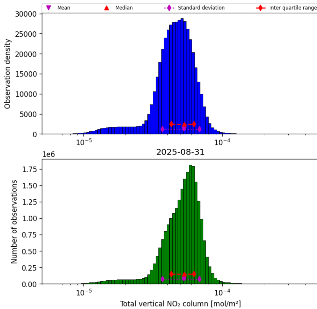
Figure 36: Histogram of "Total vertical NO 2 column" for 2025-08-31 to 2025-09-01
