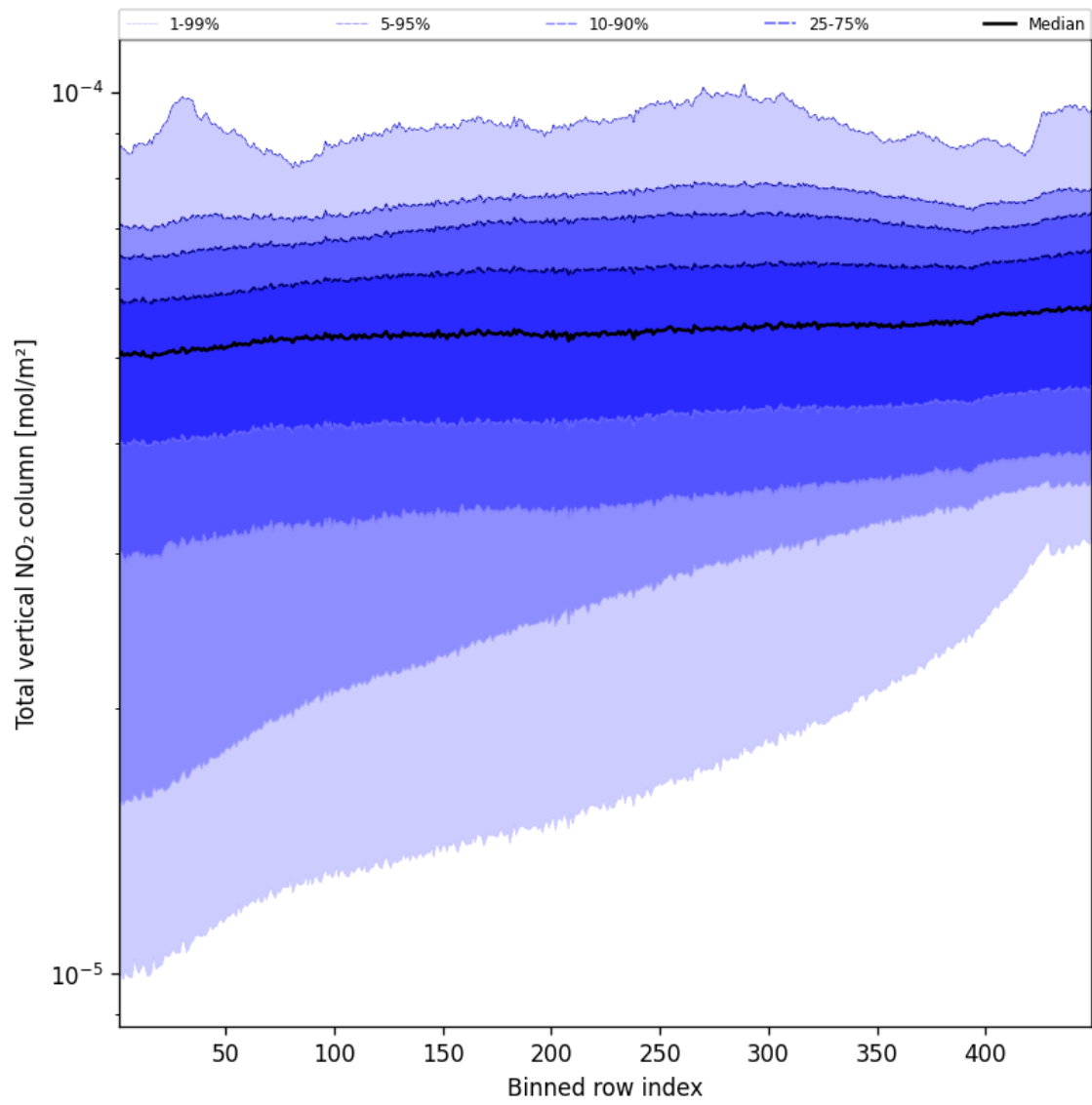
Figure 53: Along track statistics of “Total vertical NO 2 column” for 2025-08-31 to 2025-09-01
