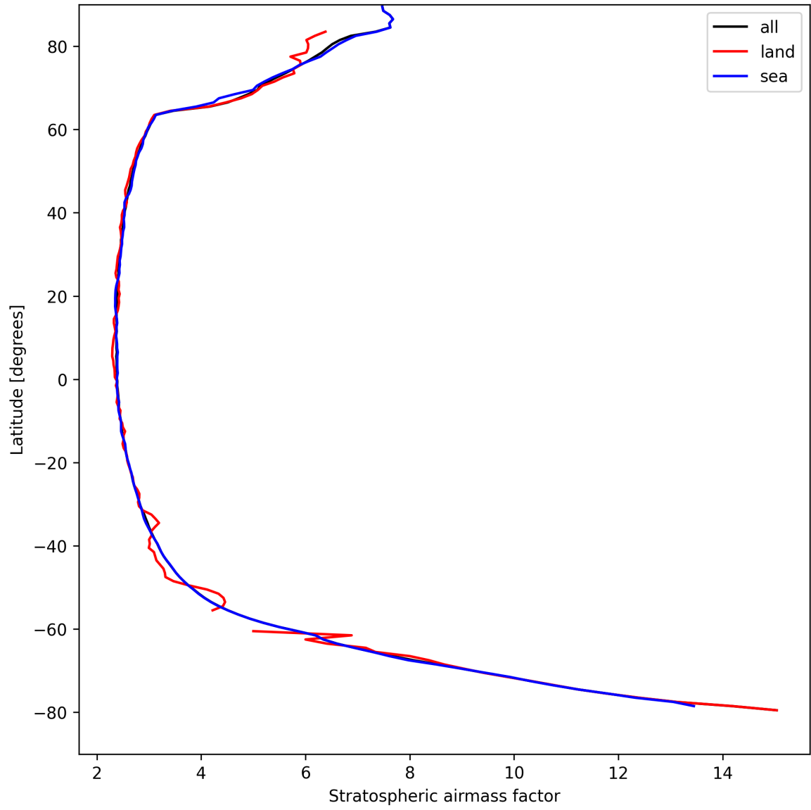
Figure 25: Zonal average of “Stratospheric airmass factor” for 2025-08-31 to 2025-09-01.
