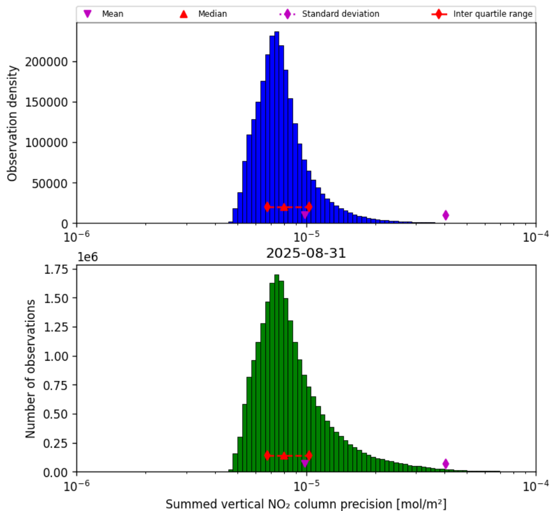
Figure 39: Histogram of "Summed vertical NO 2 column precision" for 2025-08-31 to 2025-09-01
