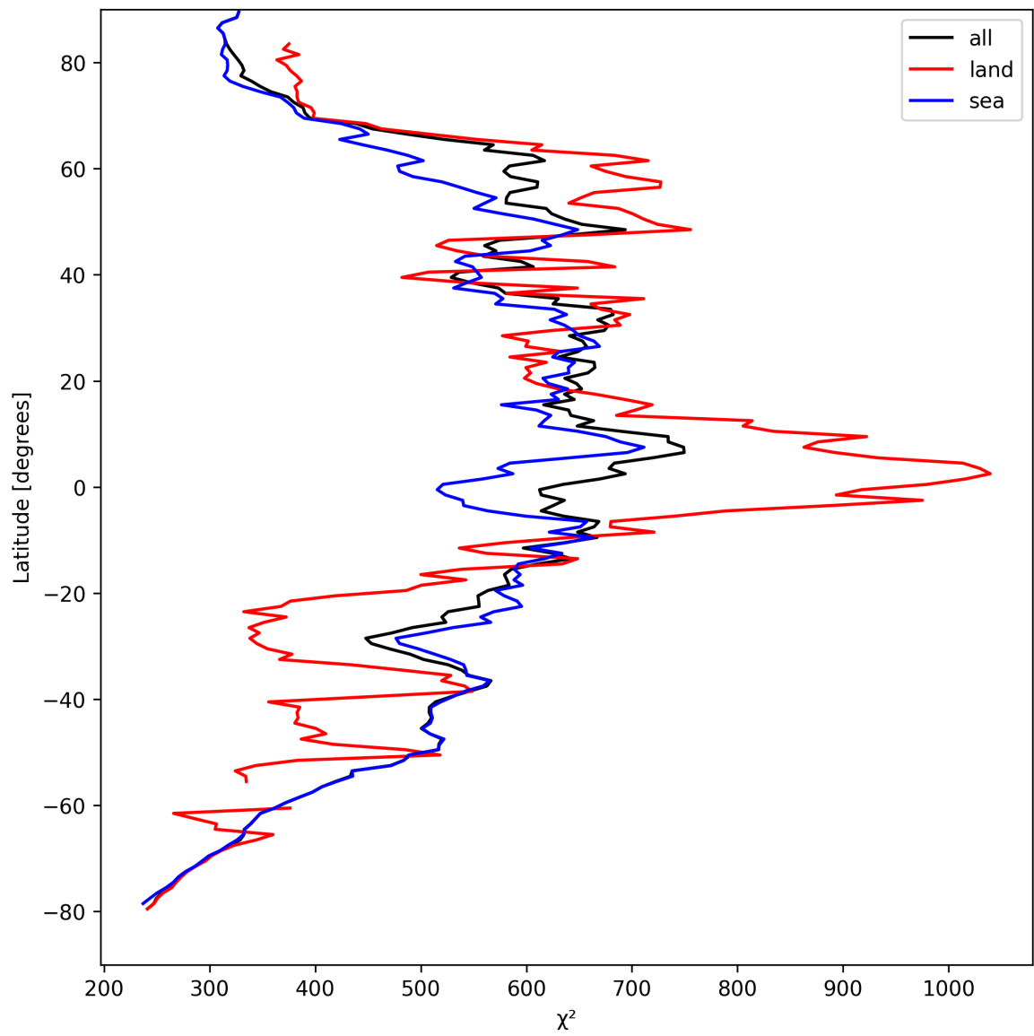
Figure 23: Zonal average of “ \chi^2 ” for 2025-08-31 to 2025-09-01.
