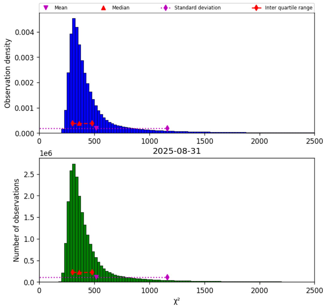
Figure 40: Histogram of “ \chi^2 ” for 2025-08-31 to 2025-09-01
