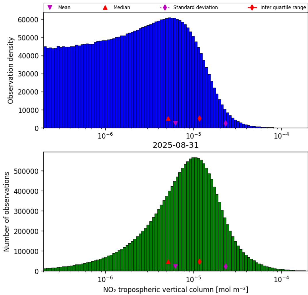
Figure 27: Histogram of “NO 2 tropospheric vertical column” for 2025-08-31 to 2025-09-01
