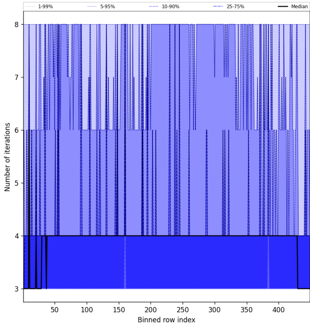
Figure 49: Along track statistics of “Number of iterations” for 2025-08-31 to 2025-09-01
