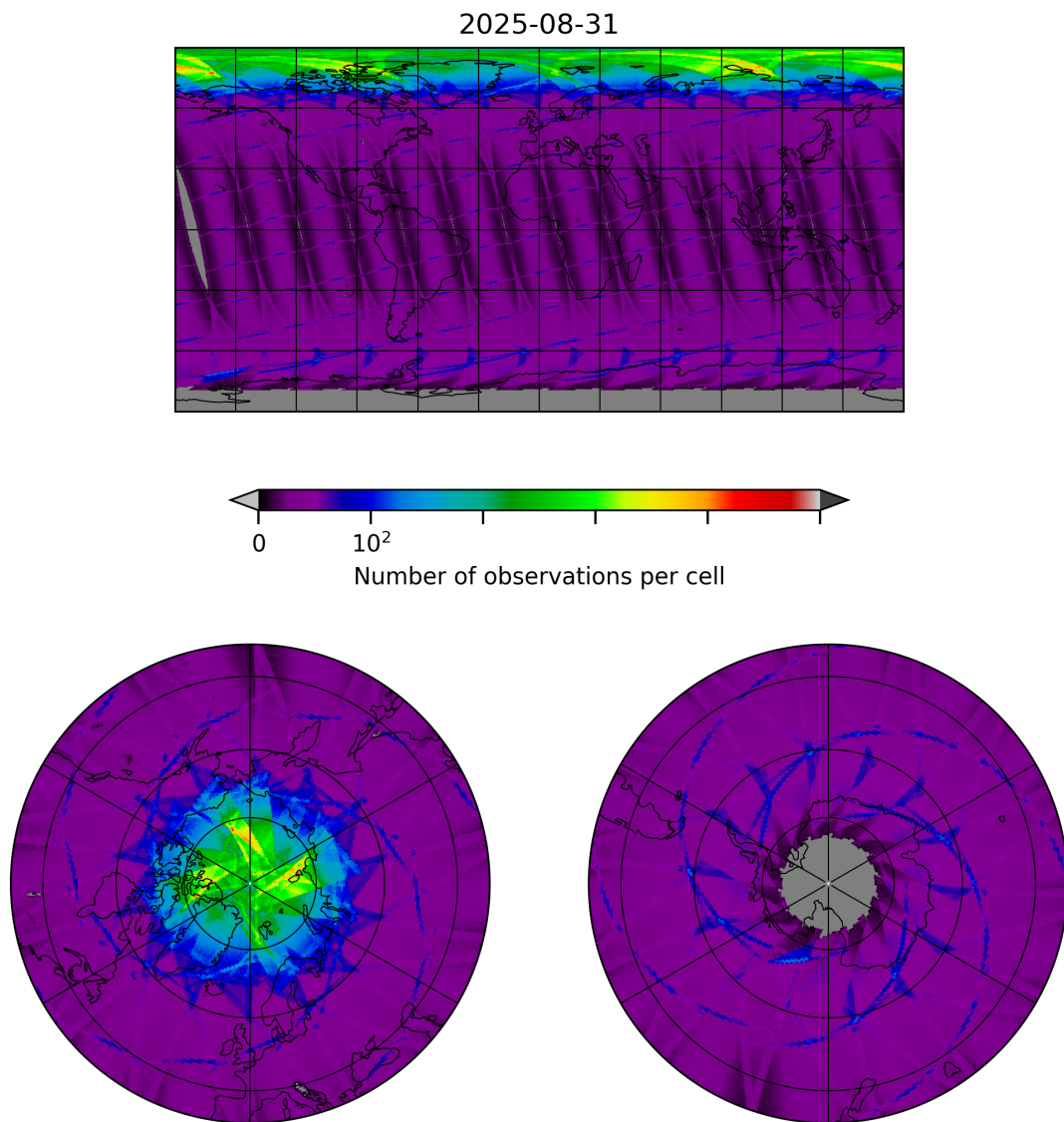
Figure 8: Map of the number of observations for 2025-08-31 to 2025-09-01
