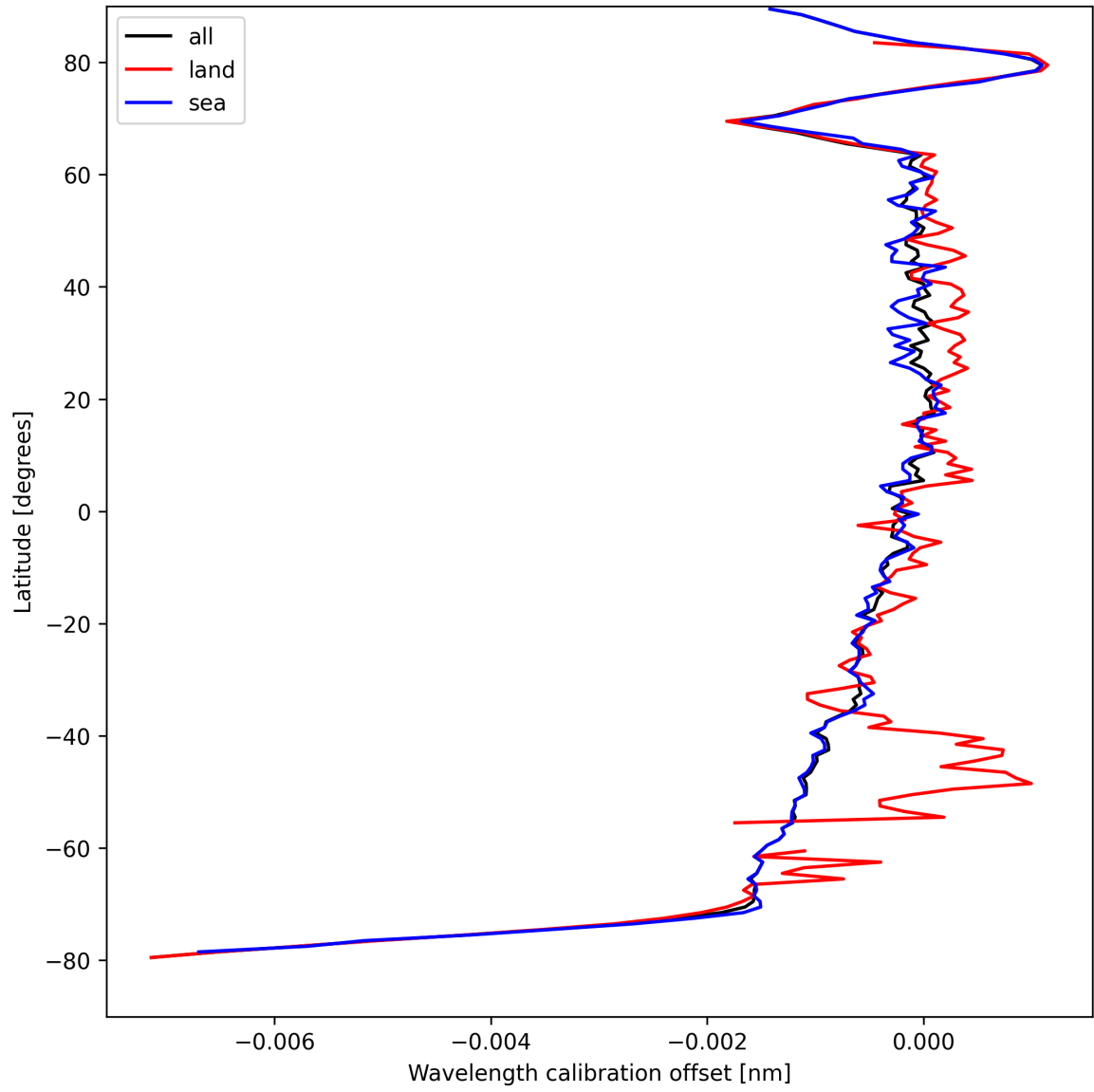
Figure 16: Zonal average of “Wavelength calibration offset” for 2025-08-31 to 2025-09-01.
