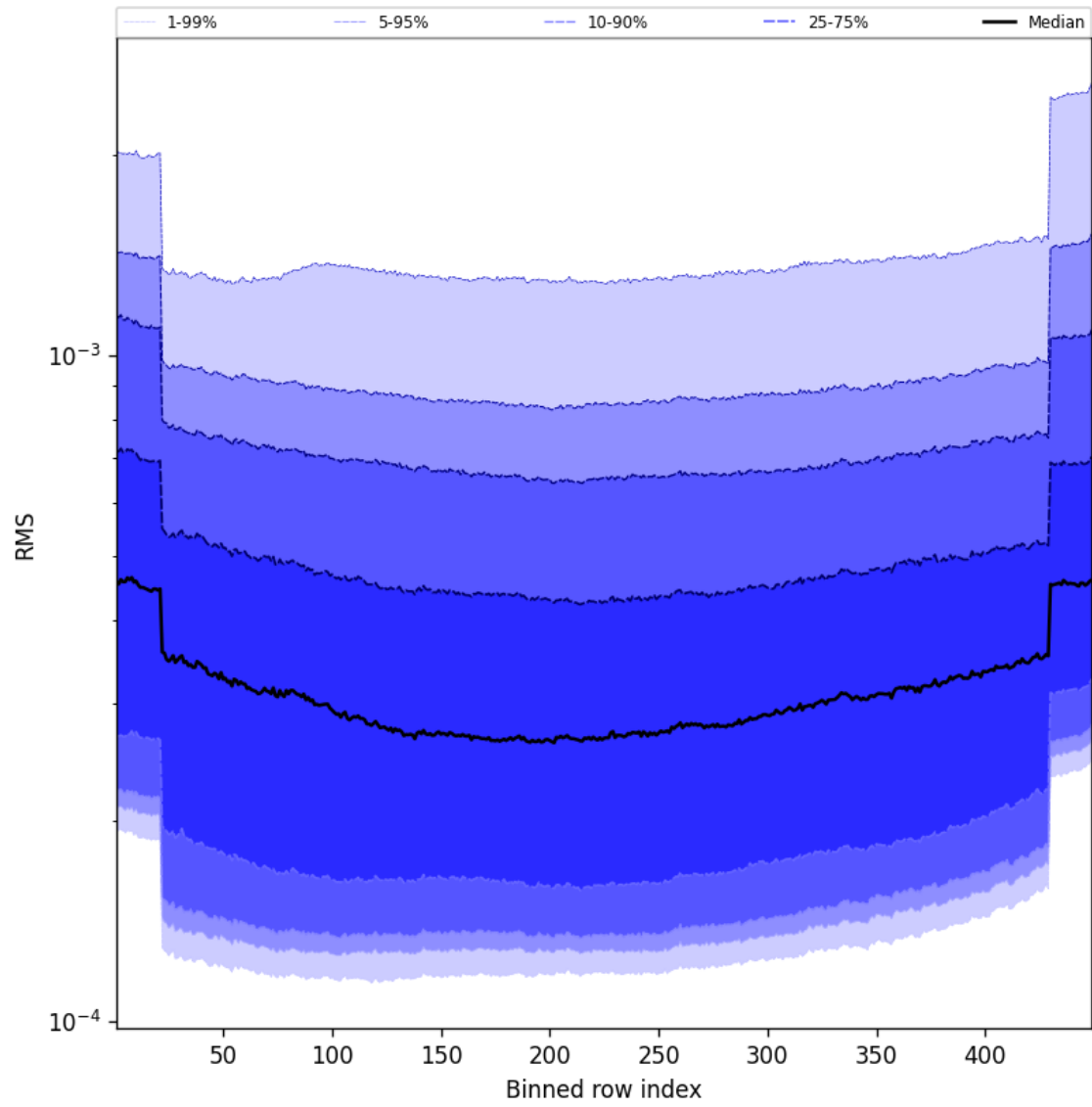
Figure 58: Along track statistics of “RMS” for 2025-08-31 to 2025-09-01
