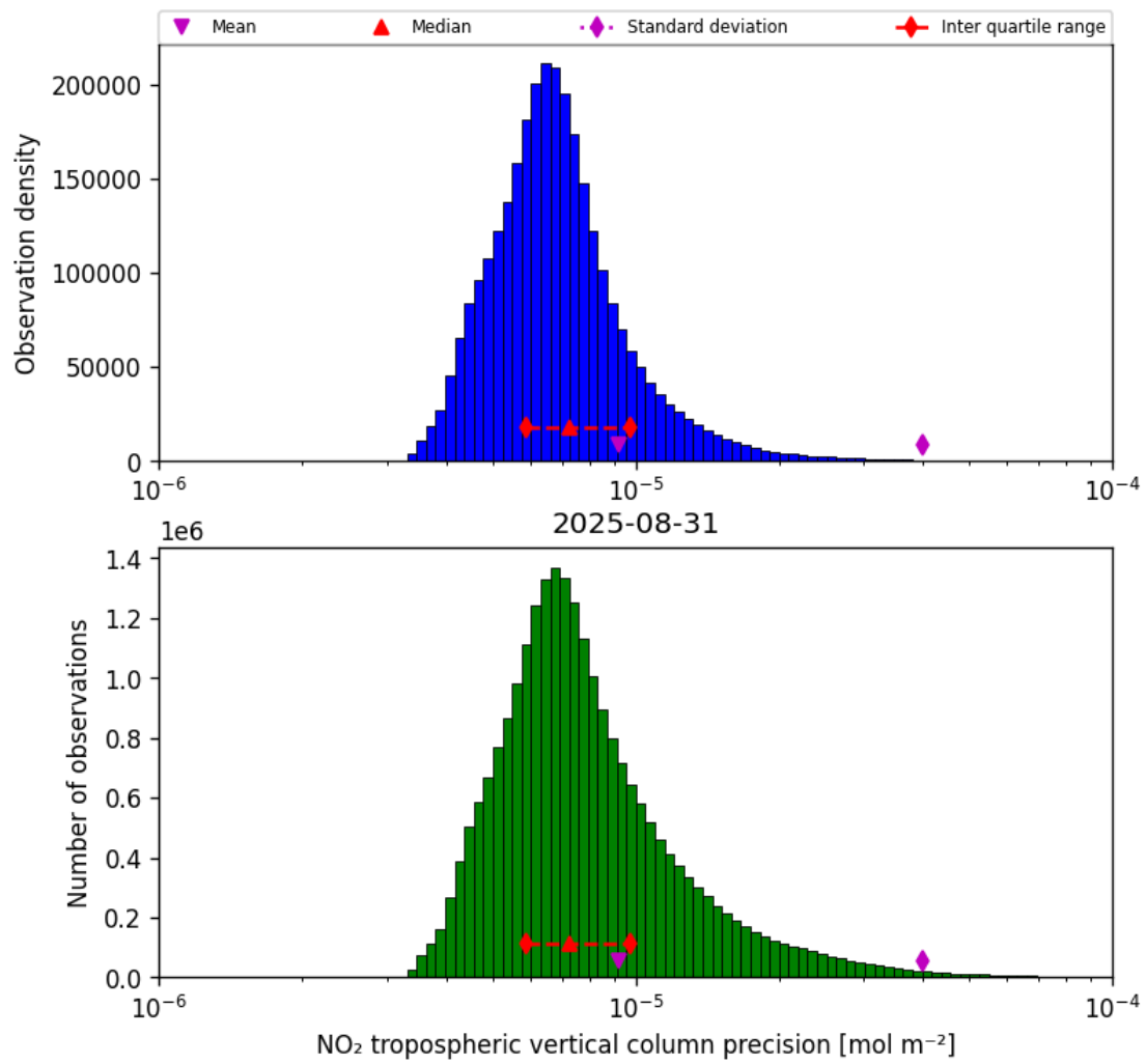
Figure 28: Histogram of “NO 2 tropospheric vertical column precision” for 2025-08-31 to 2025-09-01
