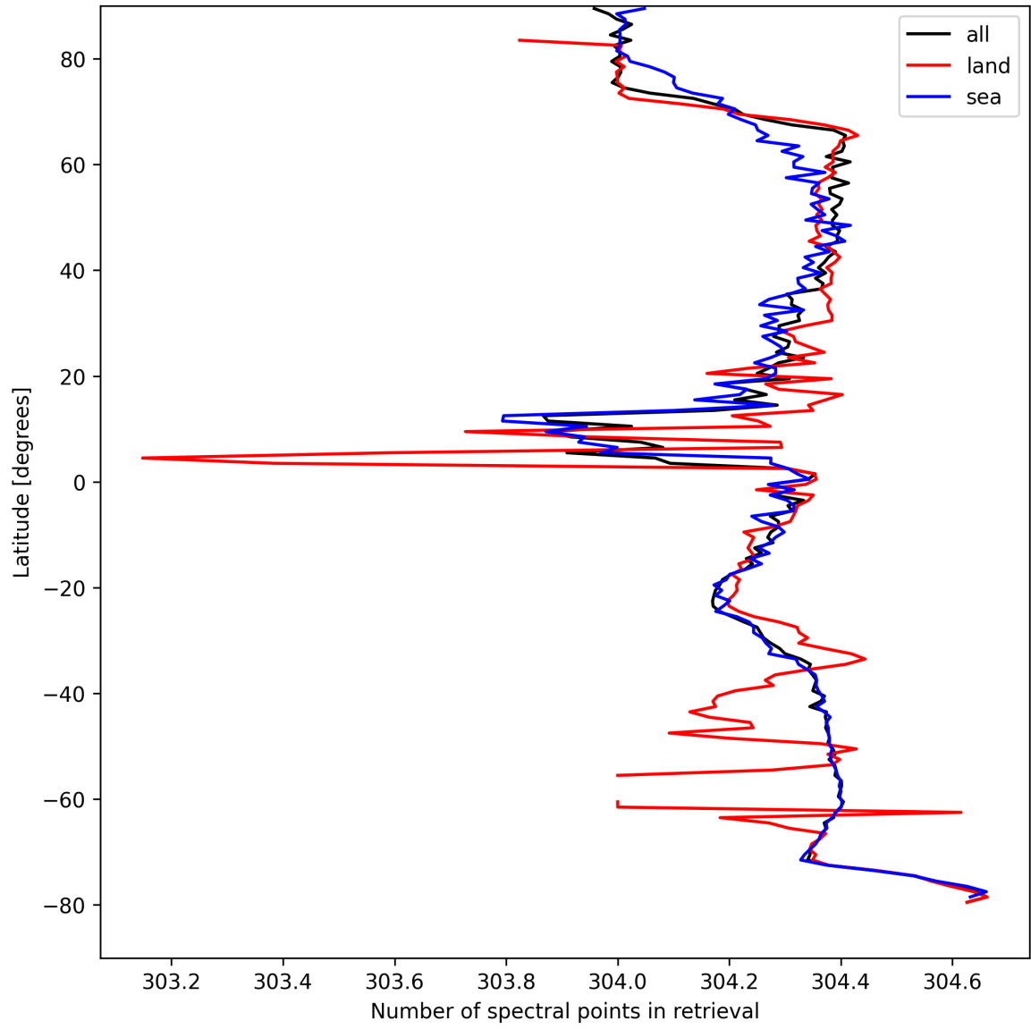
Figure 14: Zonal average of “Number of spectral points in retrieval” for 2025-08-31 to 2025-09-01.
