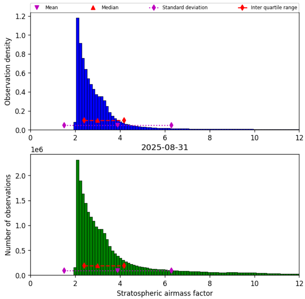
Figure 42: Histogram of “Stratospheric airmass factor” for 2025-08-31 to 2025-09-01
