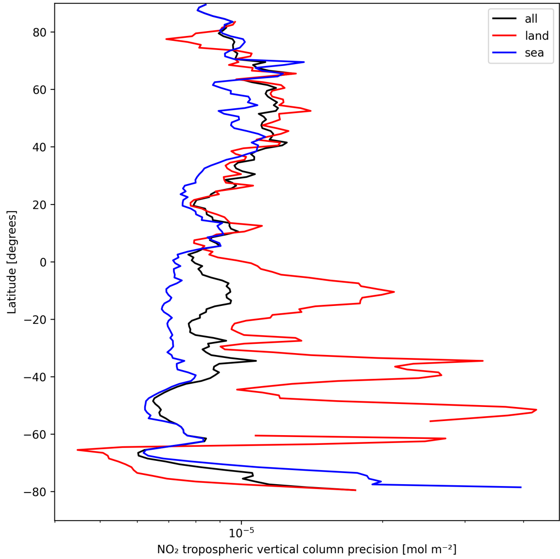
Figure 11: Zonal average of “NO 2 tropospheric vertical column precision” for 2025-08-31 to 2025-09-01.
