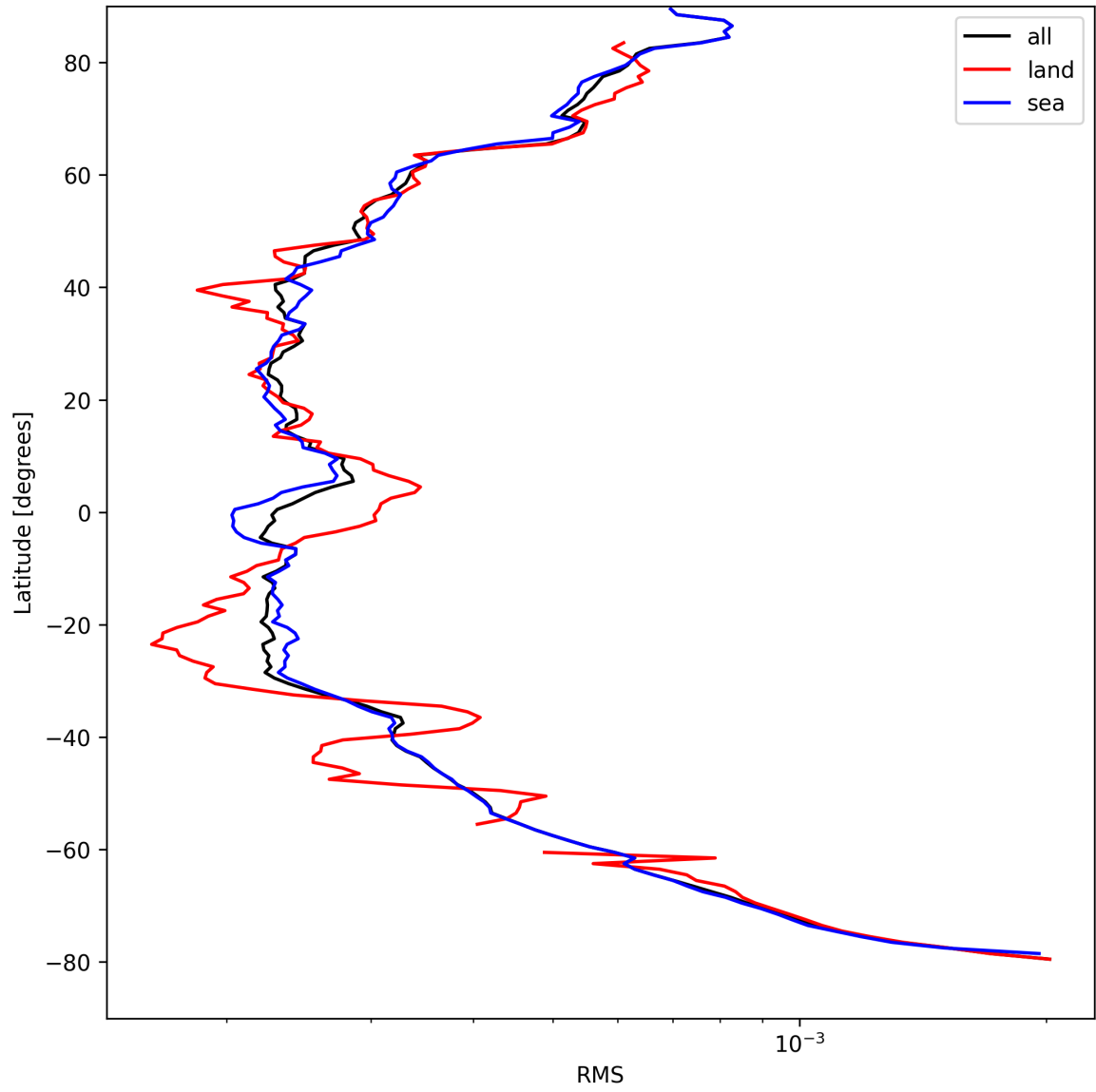
Figure 24: Zonal average of “RMS” for 2025-08-31 to 2025-09-01.
