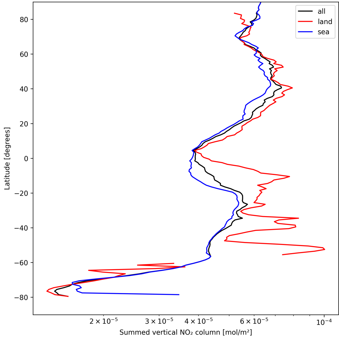
Figure 21: Zonal average of “Summed vertical NO 2 column” for 2025-08-31 to 2025-09-01.
