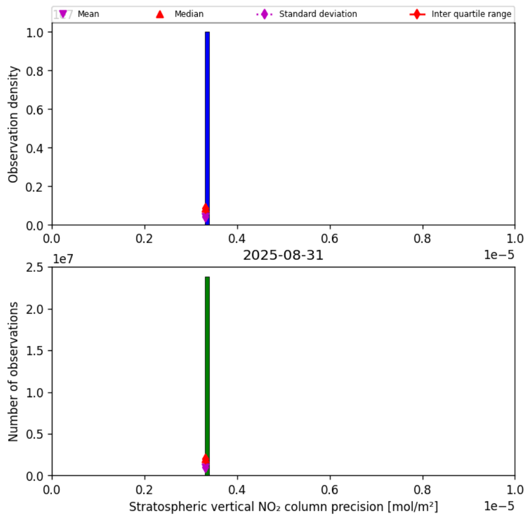
Figure 35: Histogram of “Stratospheric vertical NO 2 column precision” for 2025-08-31 to 2025-09-01
