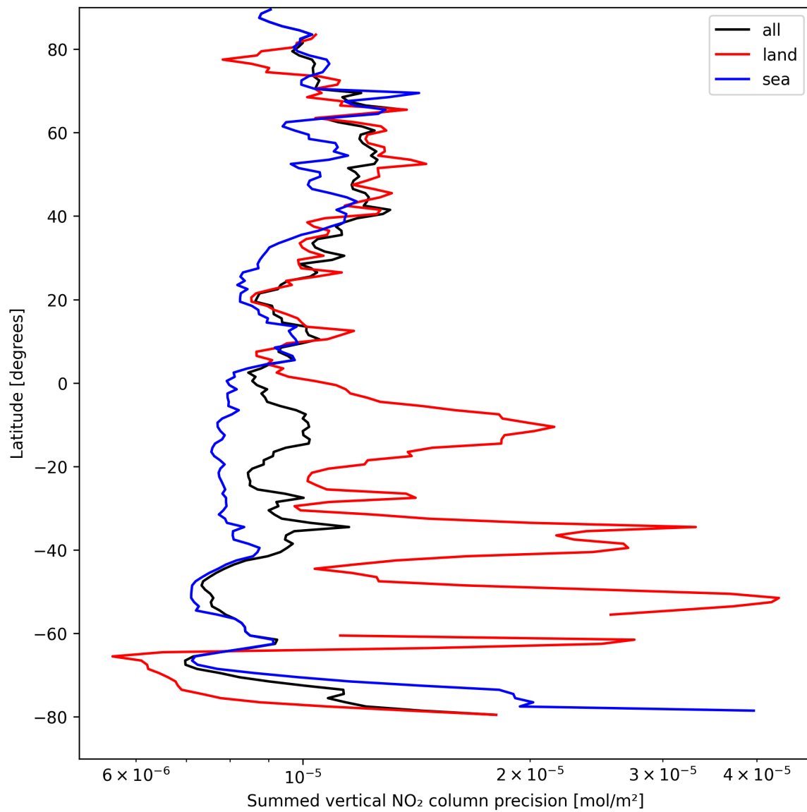
Figure 22: Zonal average of “Summed vertical NO 2 column precision” for 2025-08-31 to 2025-09-01.
