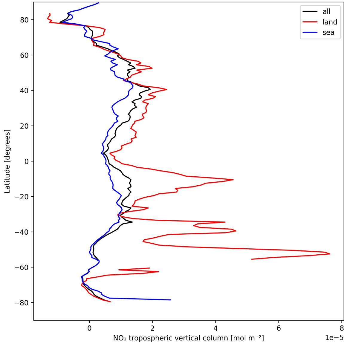
Figure 10: Zonal average of “NO 2 tropospheric vertical column” for 2025-08-31 to 2025-09-01.
