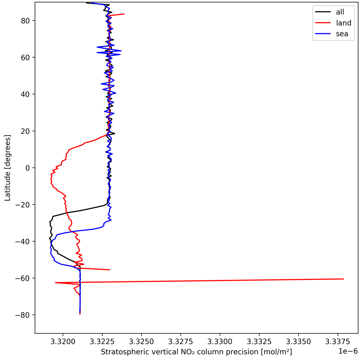
Figure 18: Zonal average of “Stratospheric vertical NO 2 column precision” for 2025-08-31 to 2025-09-01.
