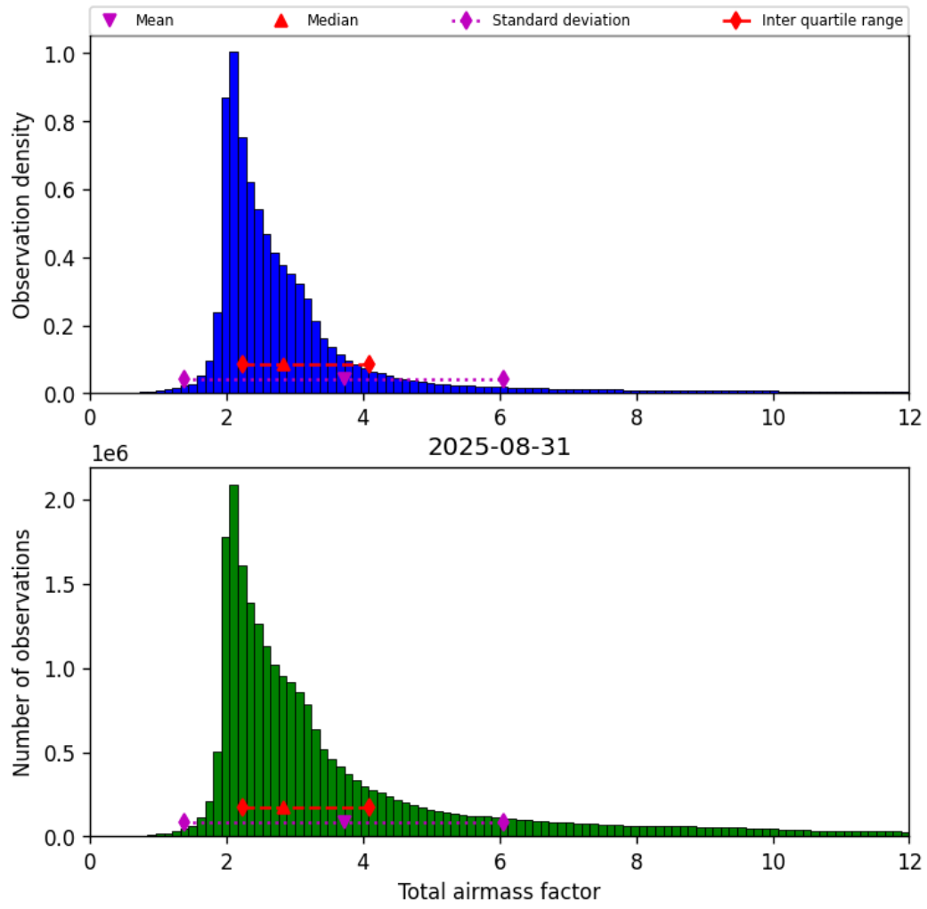
Figure 30: Histogram of “Total airmass factor” for 2025-08-31 to 2025-09-01
