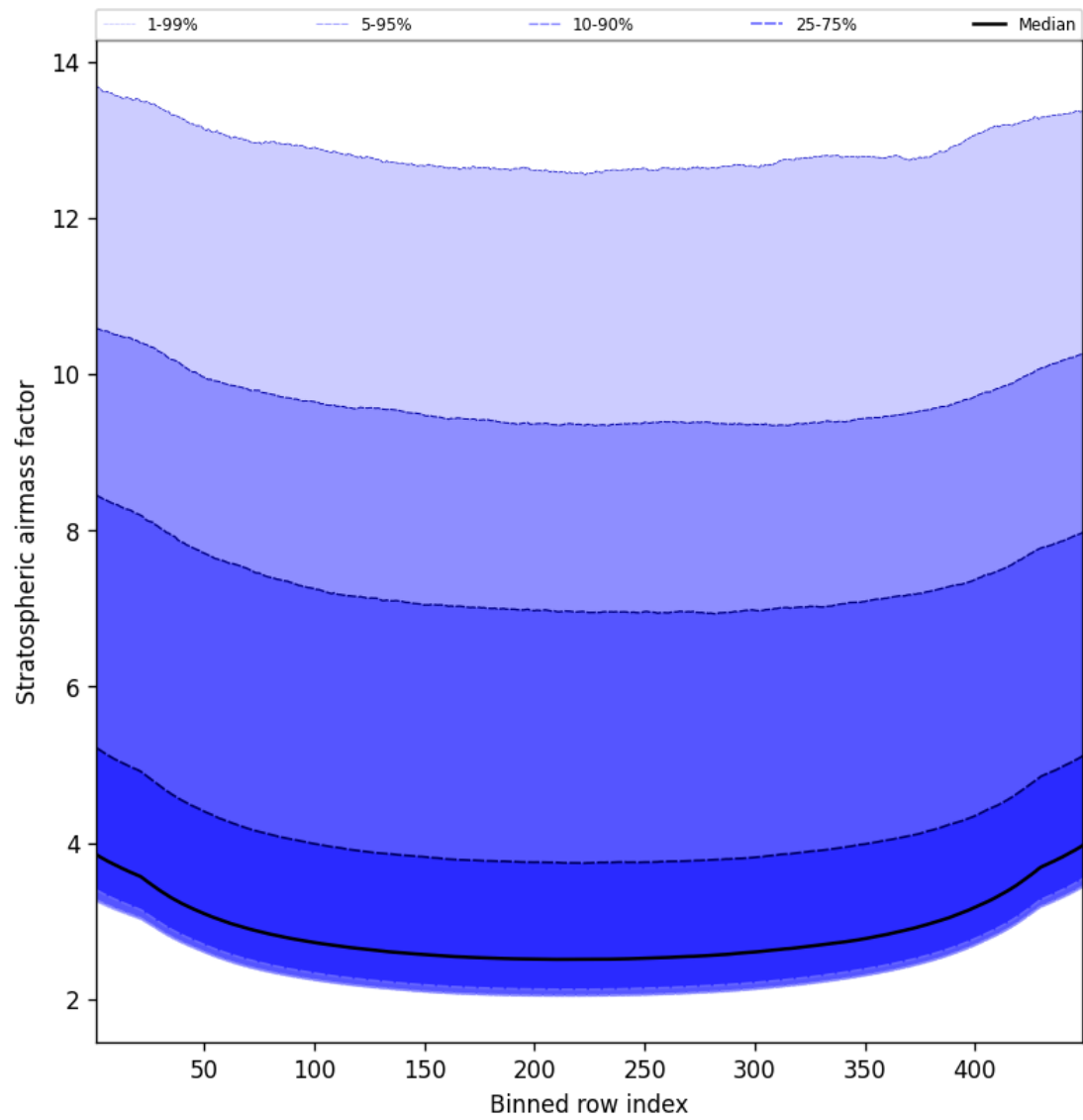
Figure 59: Along track statistics of “Stratospheric airmass factor” for 2025-08-31 to 2025-09-01
