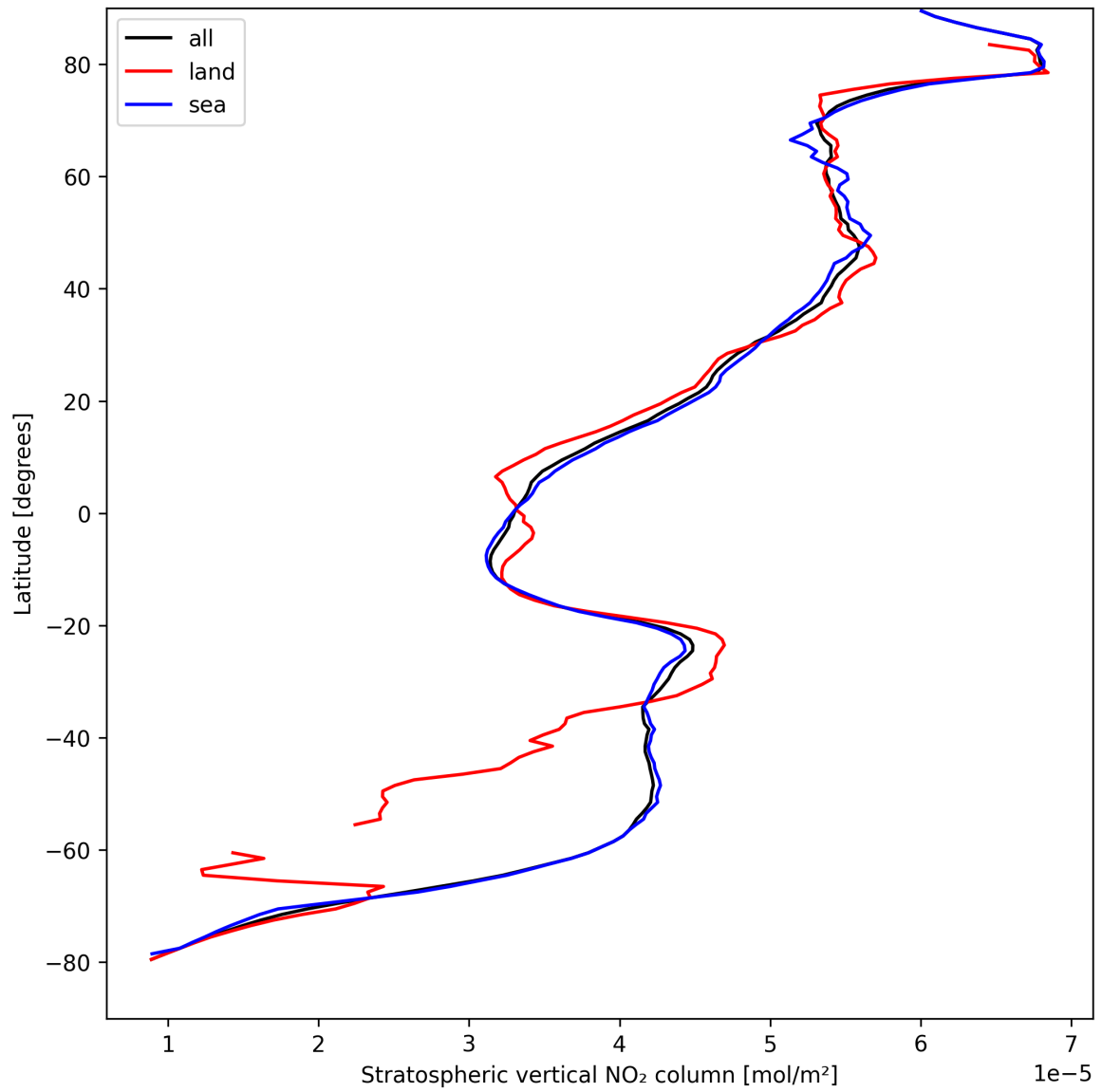
Figure 17: Zonal average of “Stratospheric vertical NO 2 column” for 2025-08-31 to 2025-09-01.
