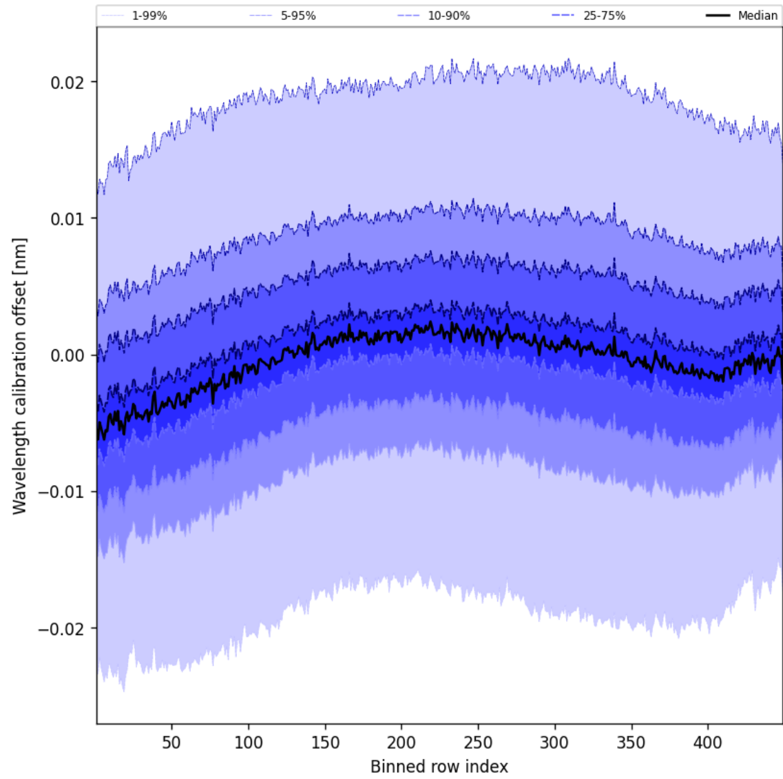
Figure 50: Along track statistics of “Wavelength calibration offset” for 2025-08-31 to 2025-09-01
