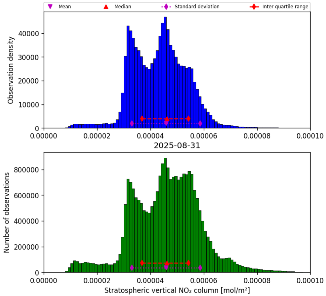
Figure 34: Histogram of “Stratospheric vertical NO 2 column” for 2025-08-31 to 2025-09-01
