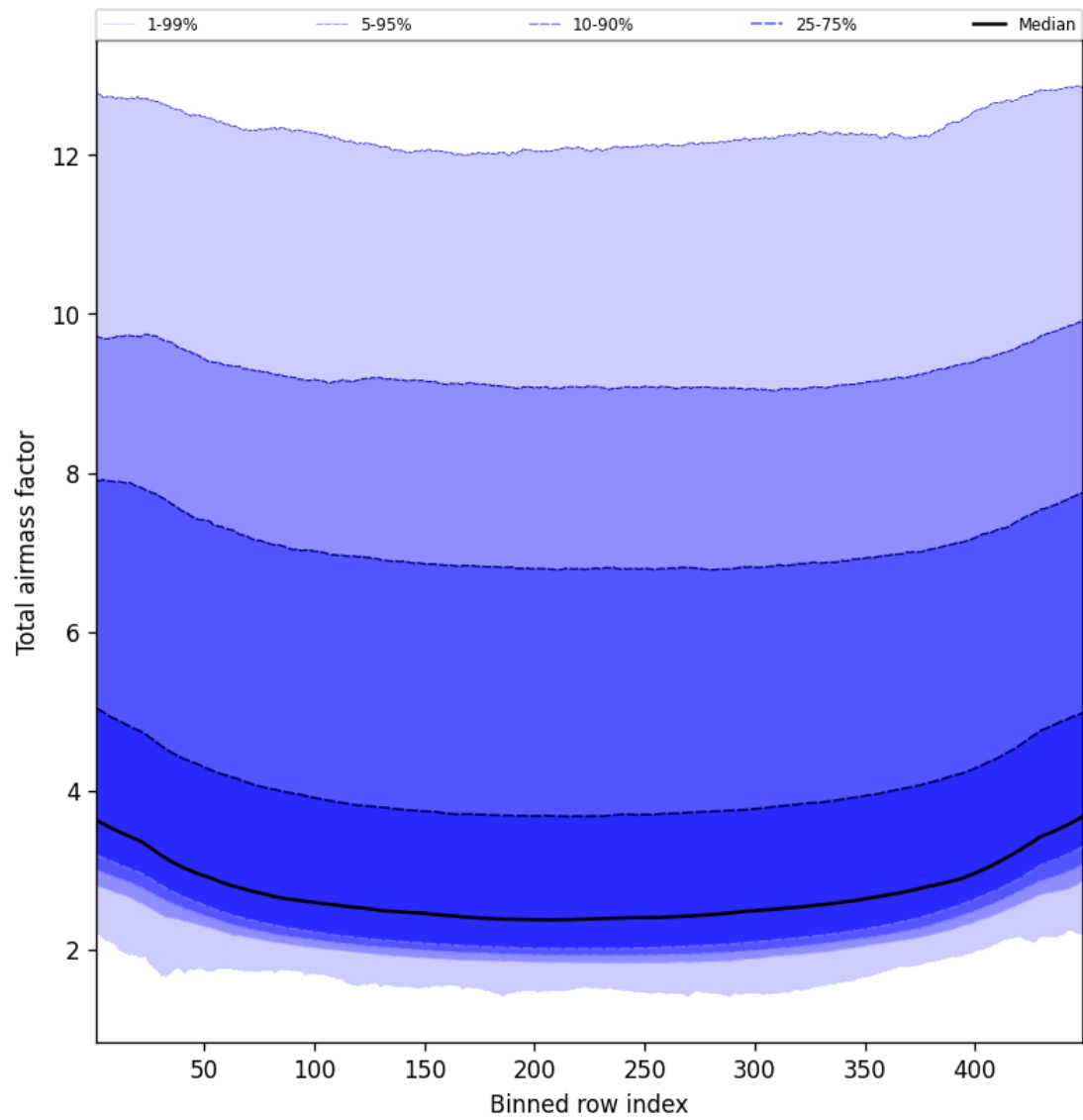
Figure 47: Along track statistics of “Total airmass factor” for 2025-08-31 to 2025-09-01
