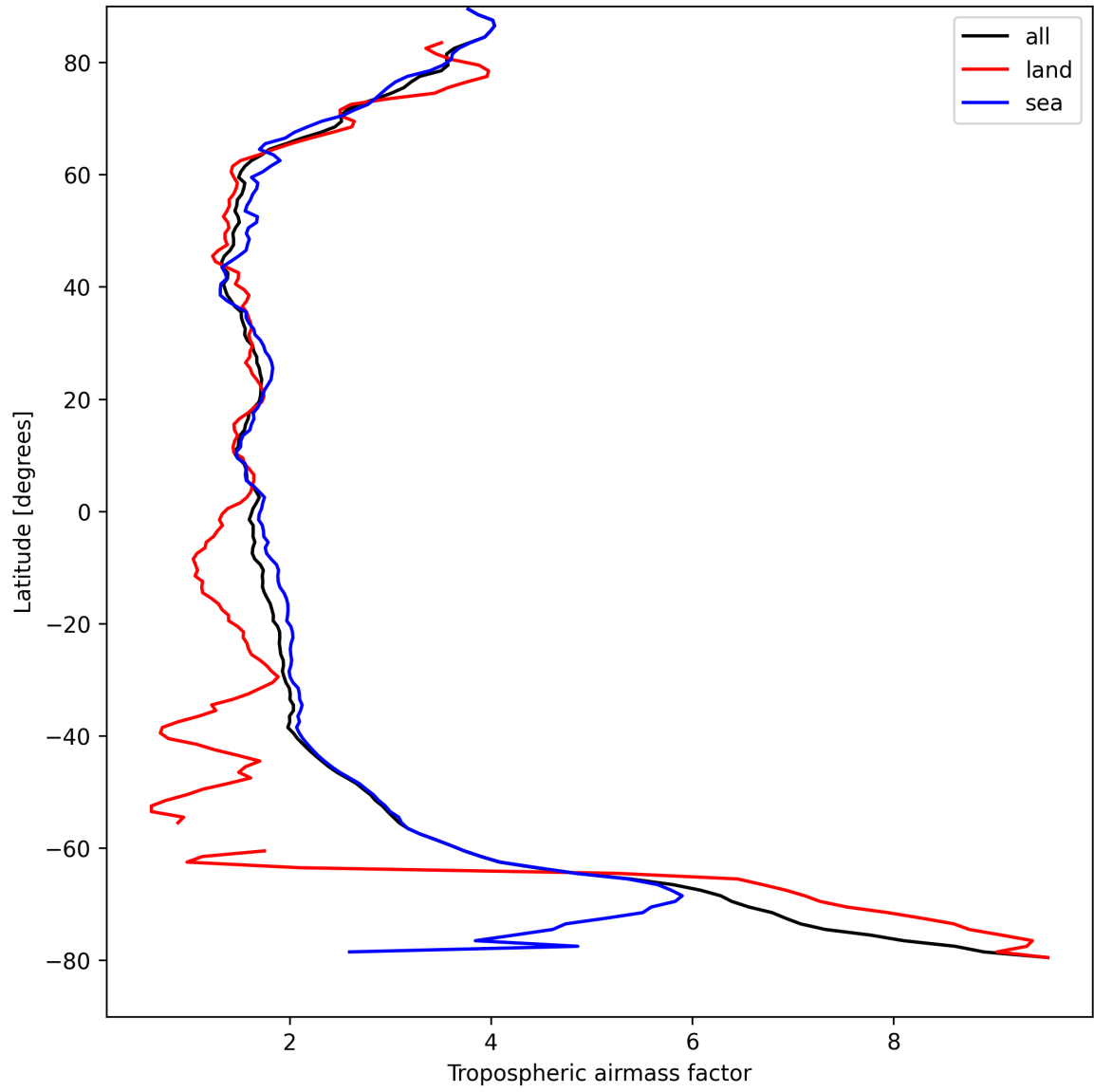
Figure 12: Zonal average of “Tropospheric airmass factor” for 2025-08-31 to 2025-09-01.
