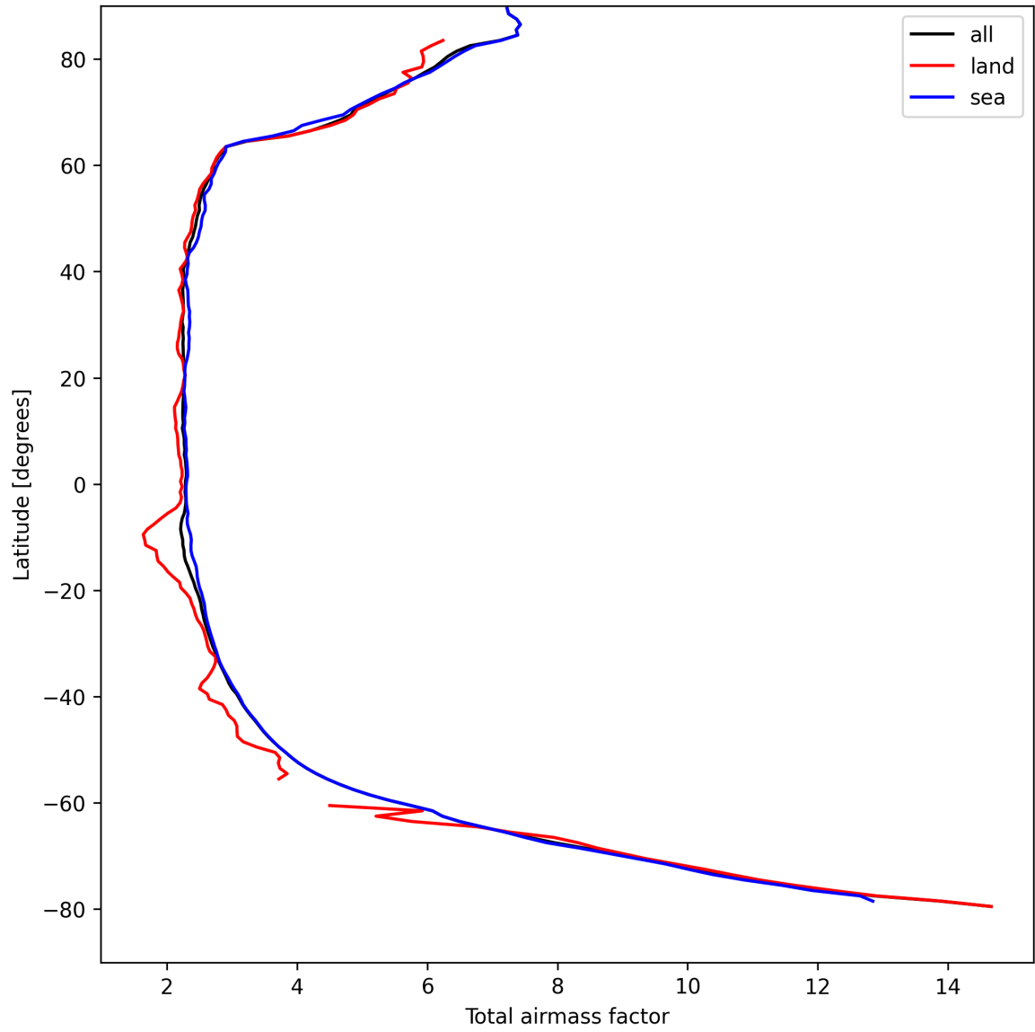
Figure 13: Zonal average of “Total airmass factor” for 2025-08-31 to 2025-09-01.
