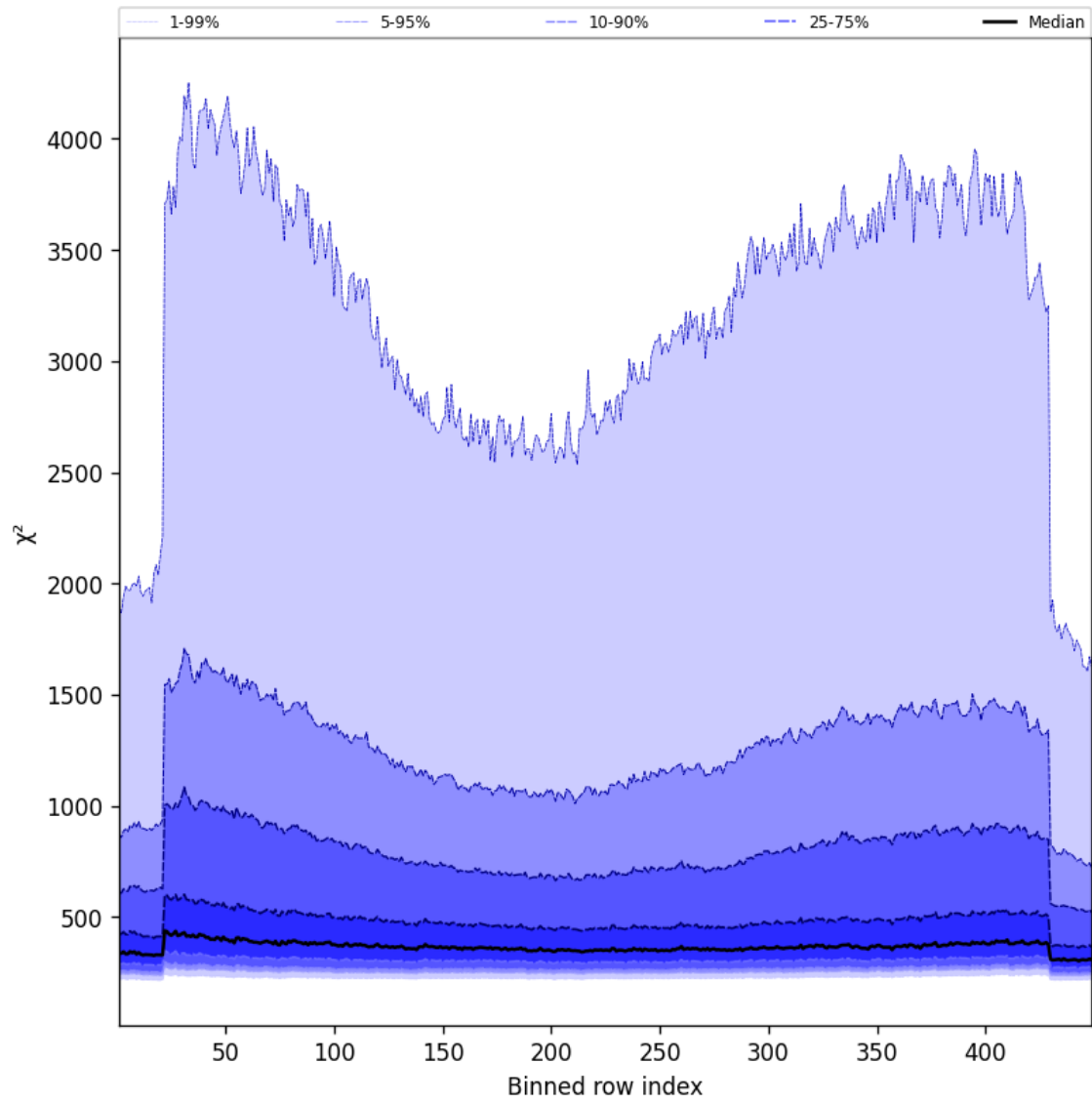
Figure 57: Along track statistics of “ \chi^2 ” for 2025-08-31 to 2025-09-01
