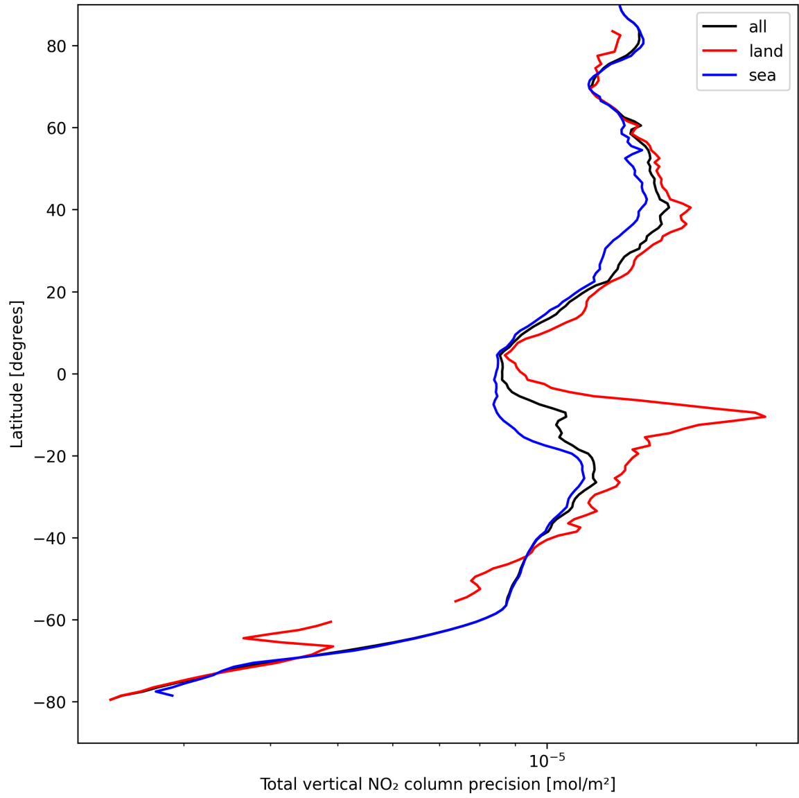
Figure 20: Zonal average of “Total vertical NO 2 column precision” for 2025-08-31 to 2025-09-01.
