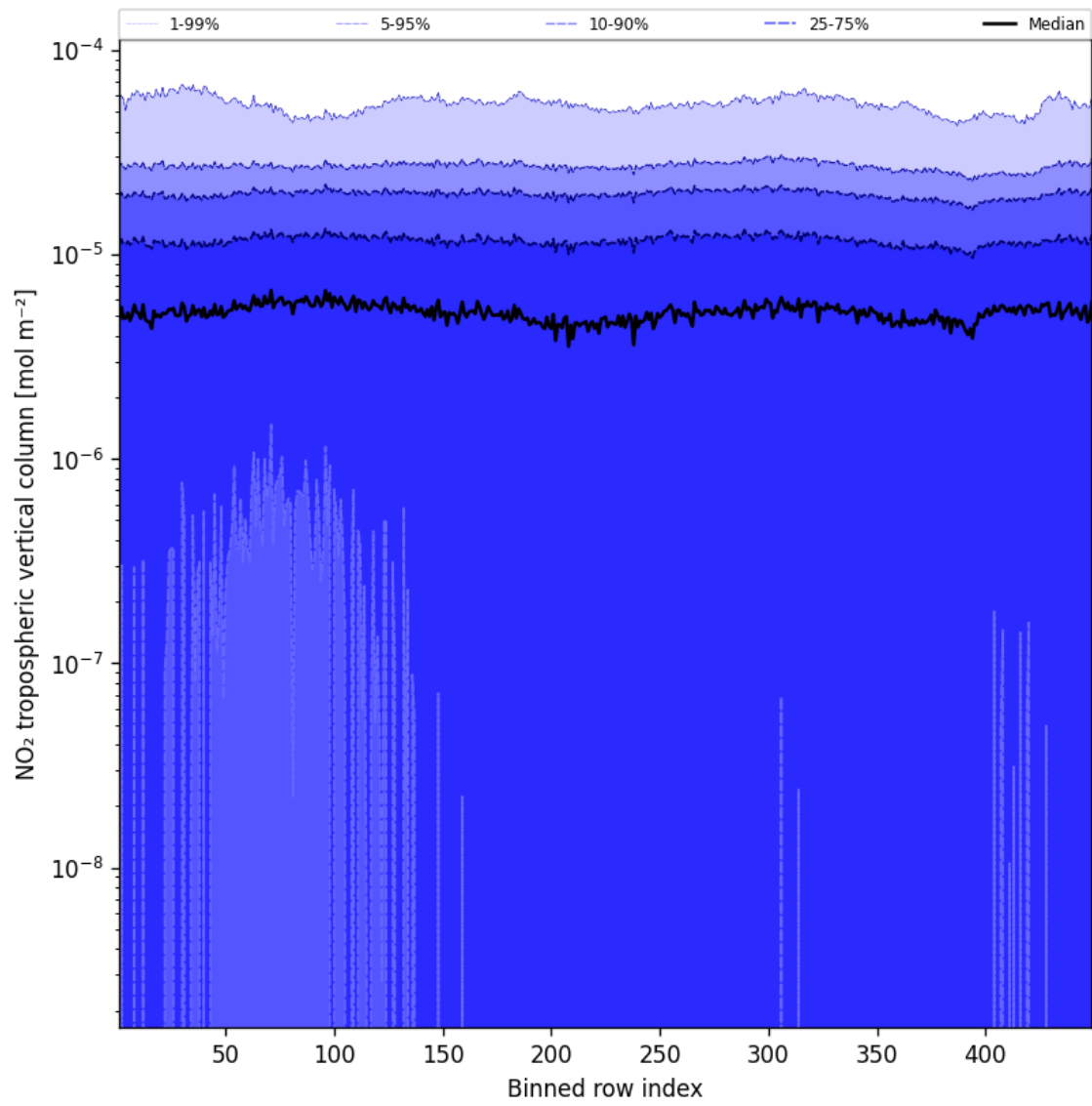
Figure 44: Along track statistics of “NO 2 tropospheric vertical column” for 2025-08-31 to 2025-09-01
