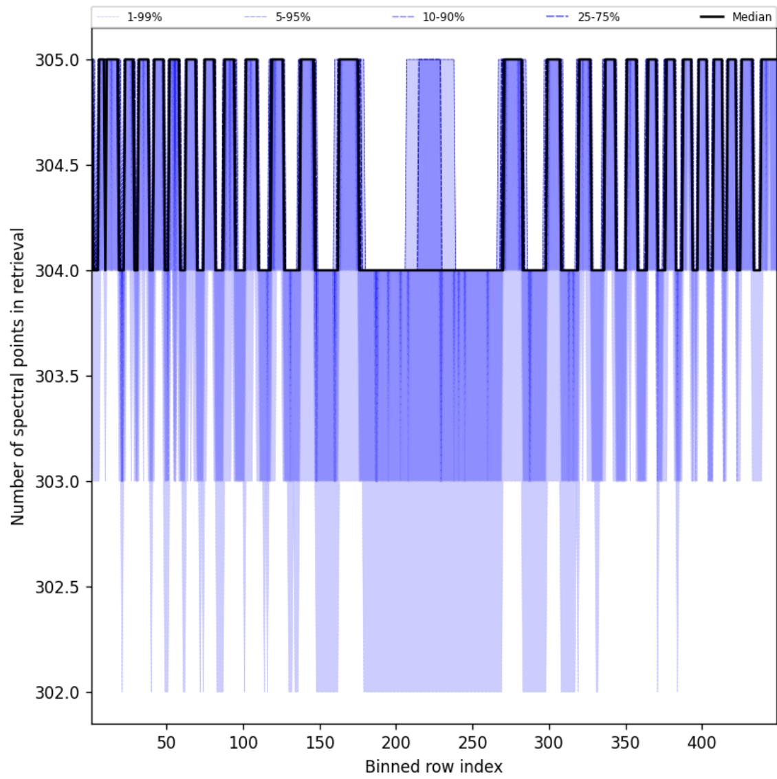
Figure 48: Along track statistics of “Number of spectral points in retrieval” for 2025-08-31 to 2025-09-01
