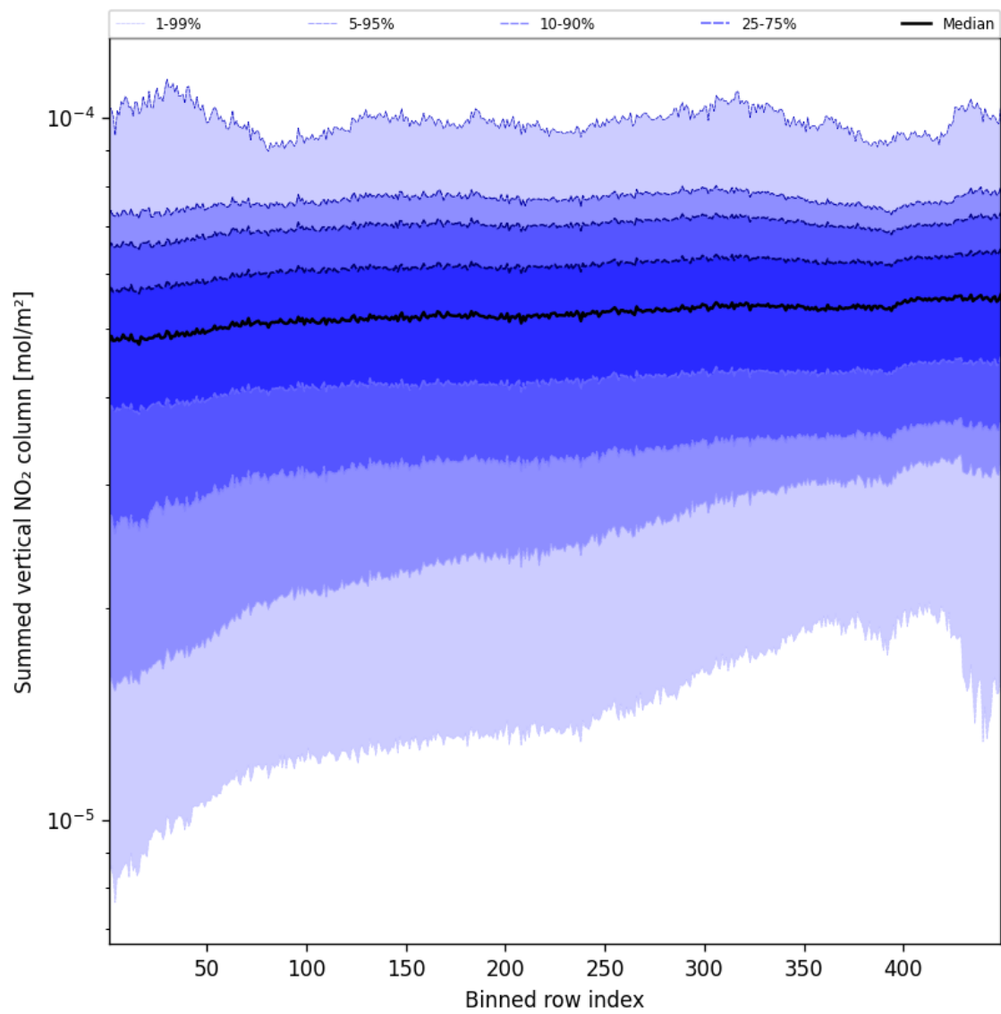
Figure 55: Along track statistics of “Summed vertical NO 2 column” for 2025-08-31 to 2025-09-01
