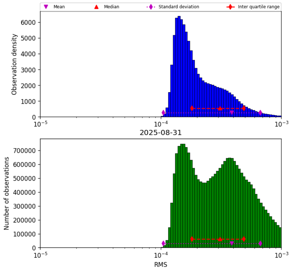
Figure 41: Histogram of “RMS” for 2025-08-31 to 2025-09-01
