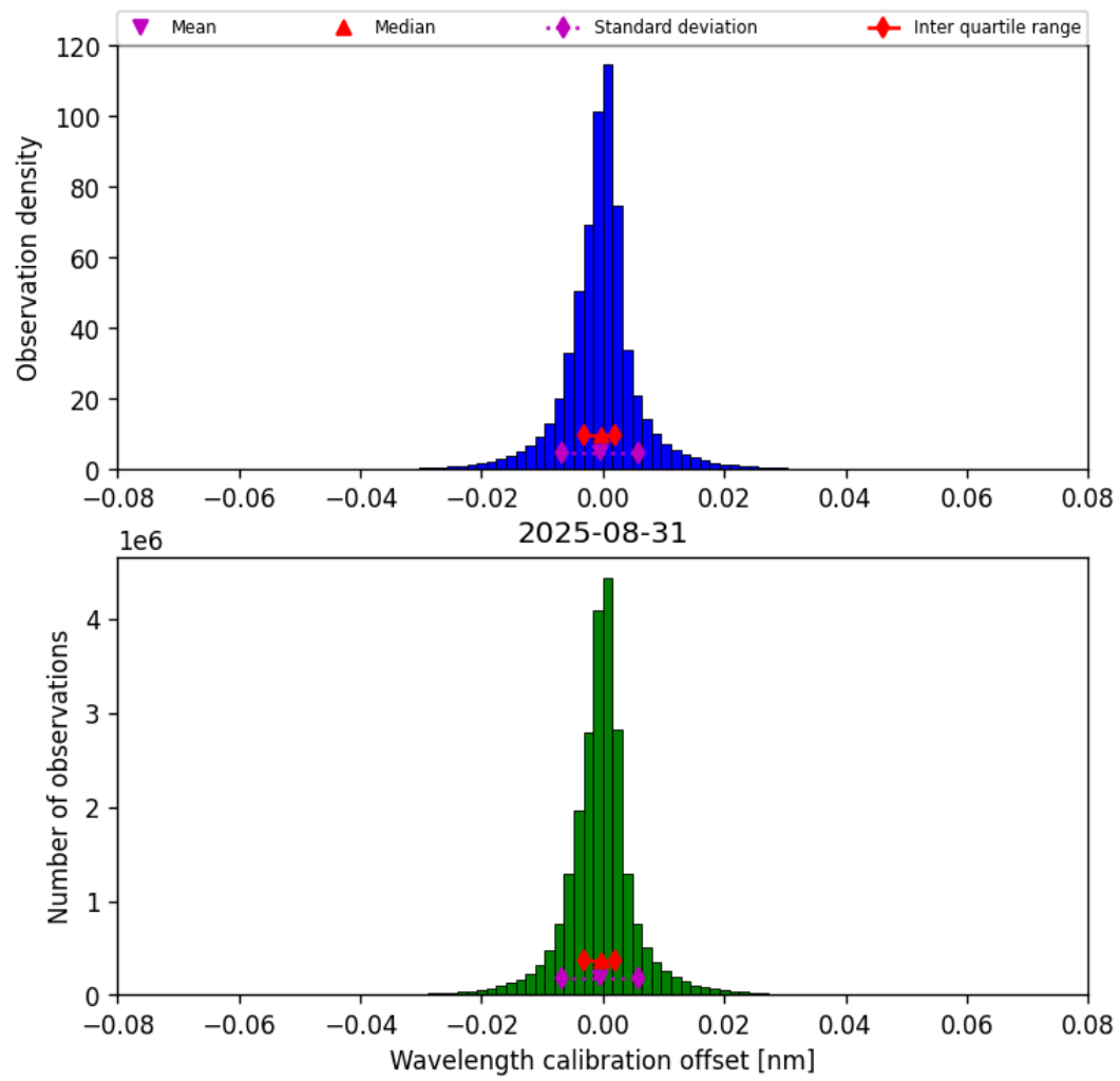
Figure 33: Histogram of “Wavelength calibration offset” for 2025-08-31 to 2025-09-01
