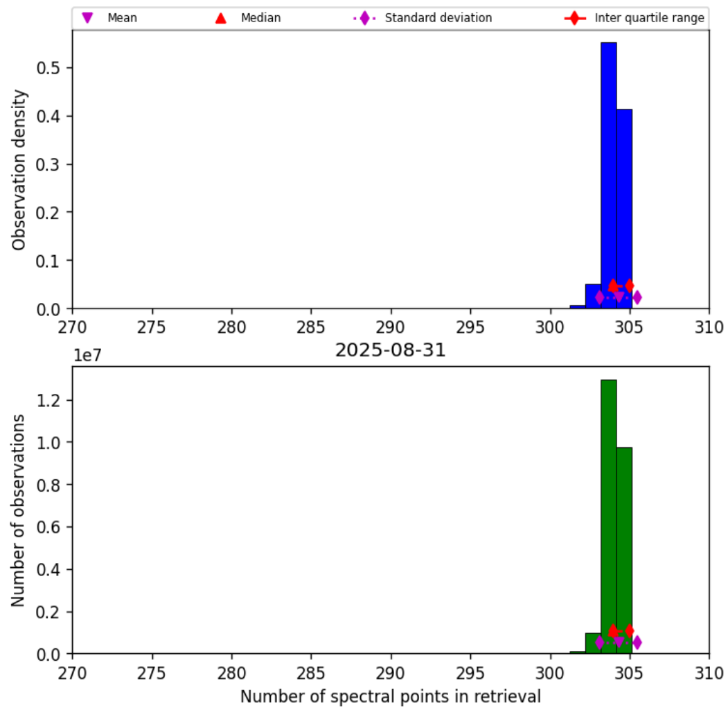
Figure 31: Histogram of “Number of spectral points in retrieval” for 2025-08-31 to 2025-09-01
