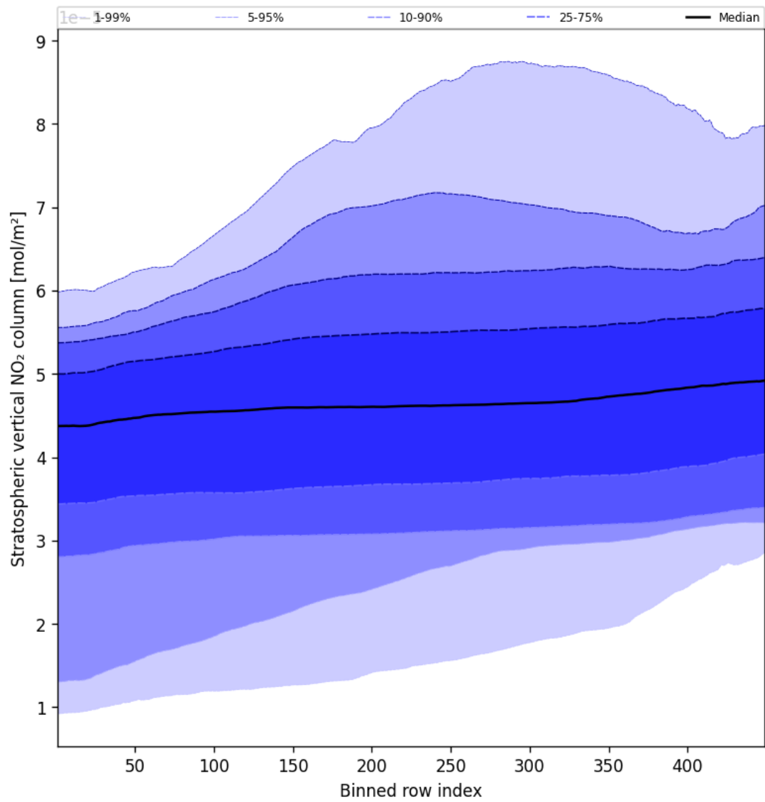
Figure 51: Along track statistics of “Stratospheric vertical NO 2 column” for 2025-08-31 to 2025-09-01
