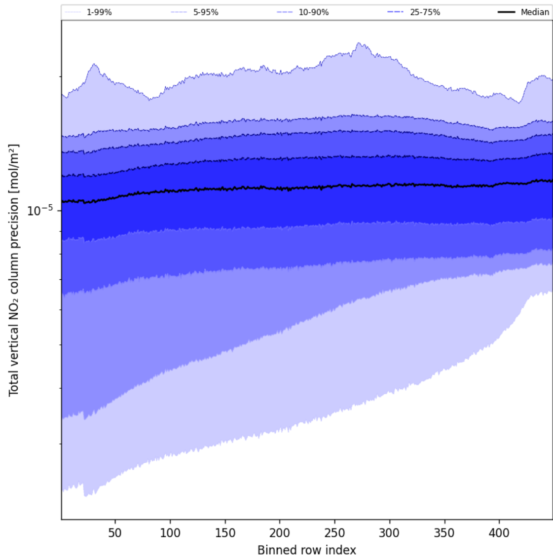
Figure 54: Along track statistics of “Total vertical NO 2 column precision” for 2025-08-31 to 2025-09-01
