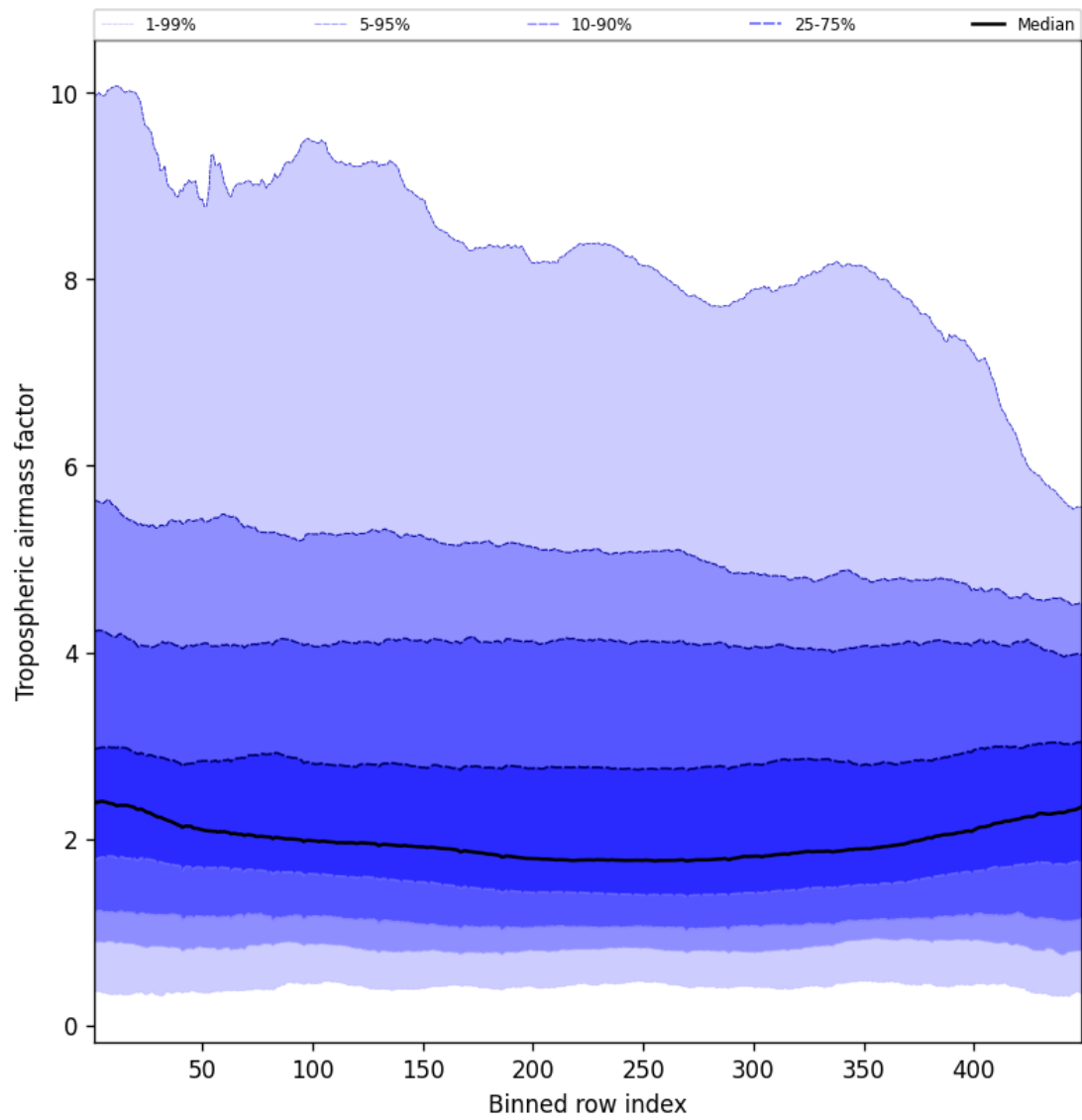
Figure 46: Along track statistics of “Tropospheric airmass factor” for 2025-08-31 to 2025-09-01
