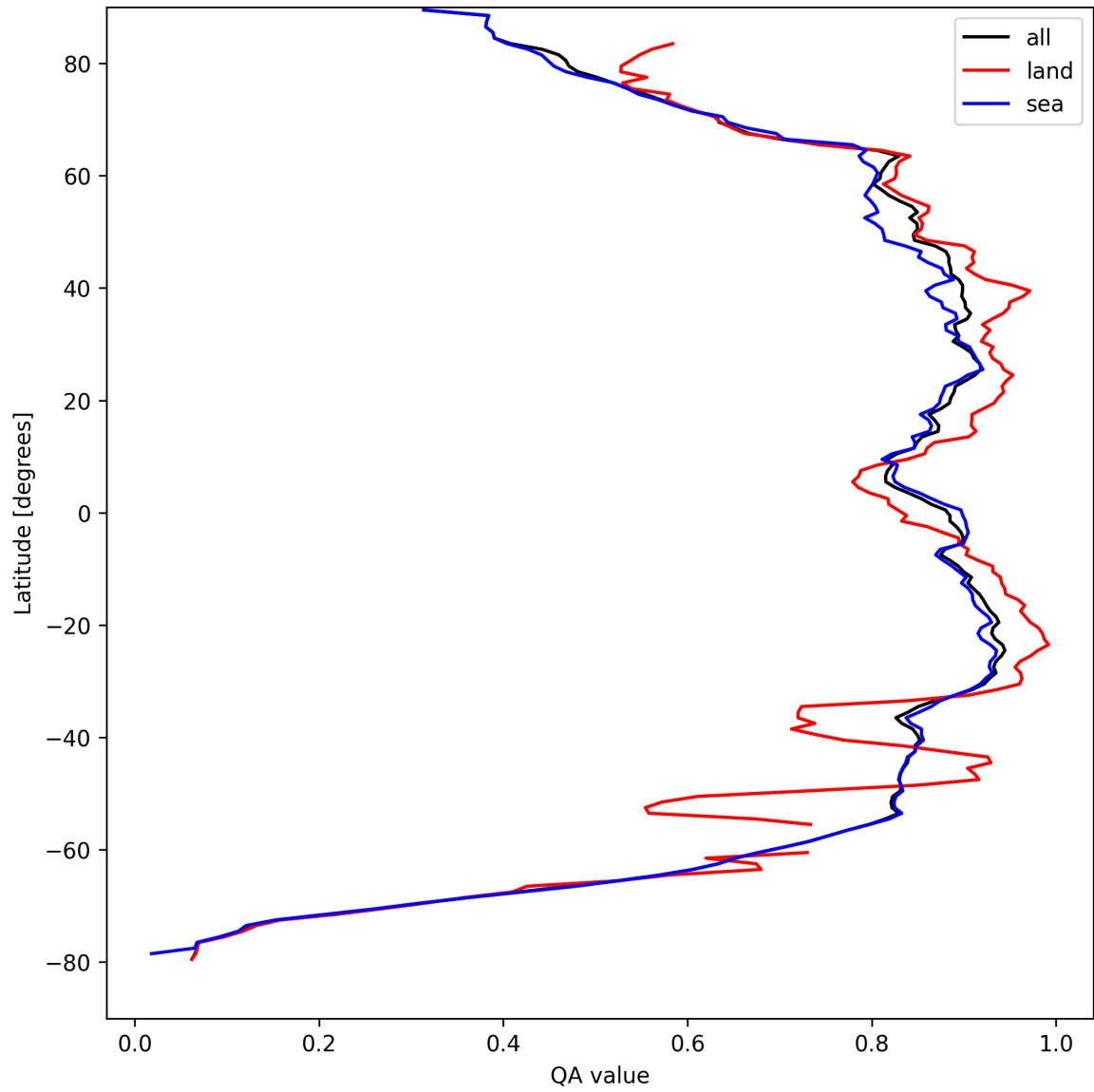
Figure 9: Zonal average of “QA value” for 2025-08-31 to 2025-09-01.
