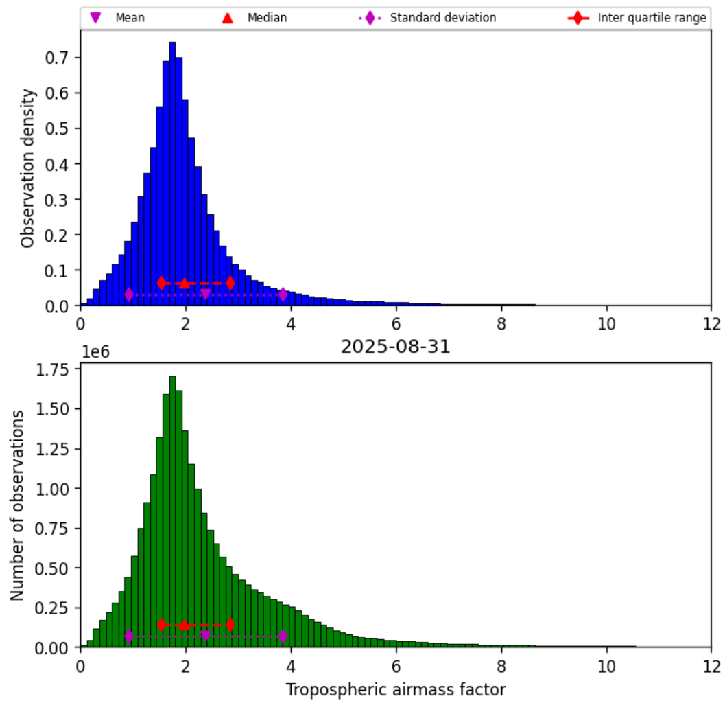
Figure 29: Histogram of “Tropospheric airmass factor” for 2025-08-31 to 2025-09-01
