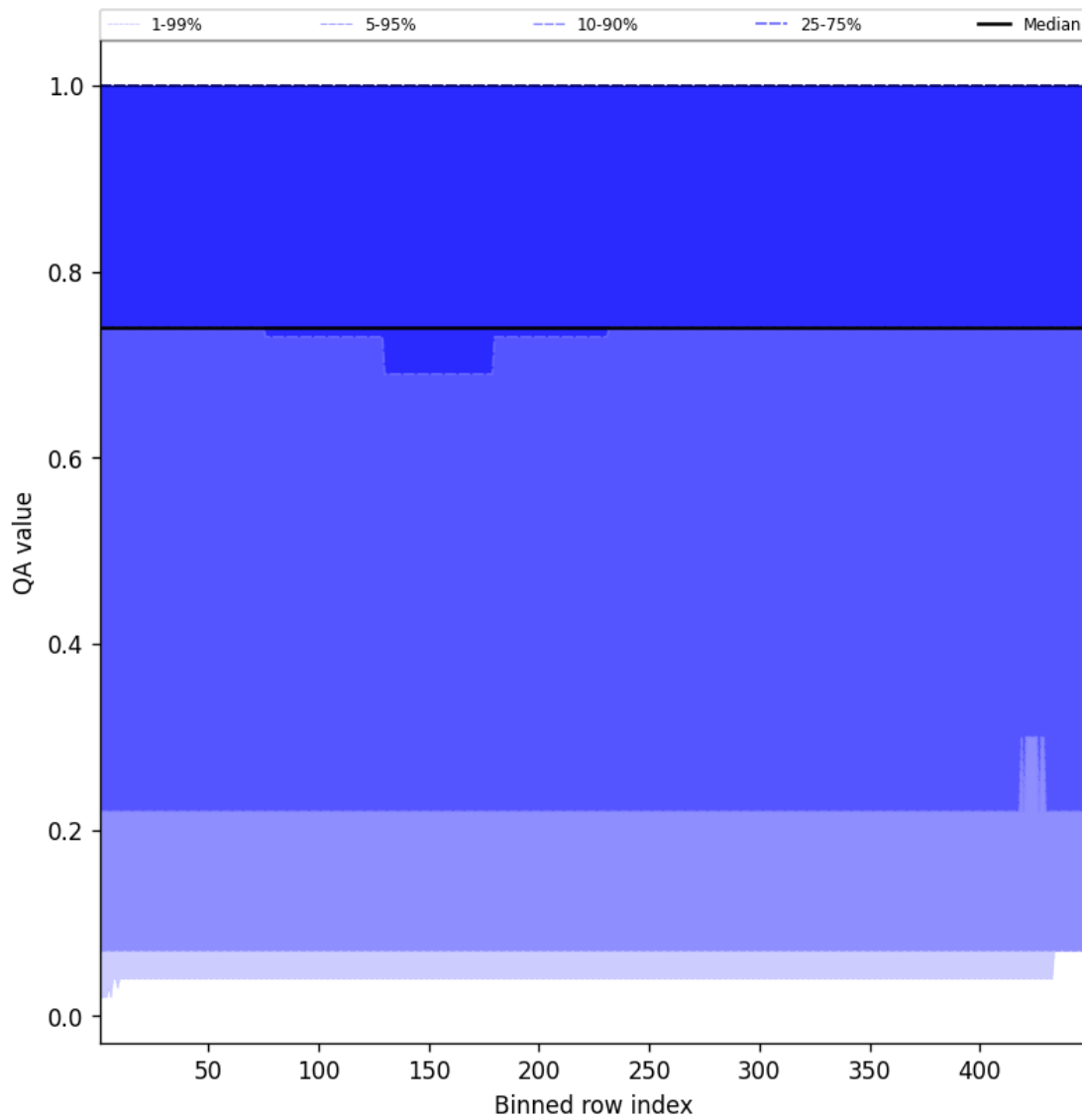
Figure 43: Along track statistics of “QA value” for 2025-08-31 to 2025-09-01
