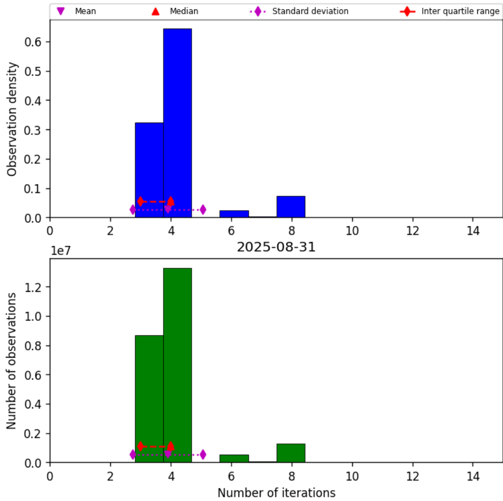
Figure 32: Histogram of “Number of iterations” for 2025-08-31 to 2025-09-01
