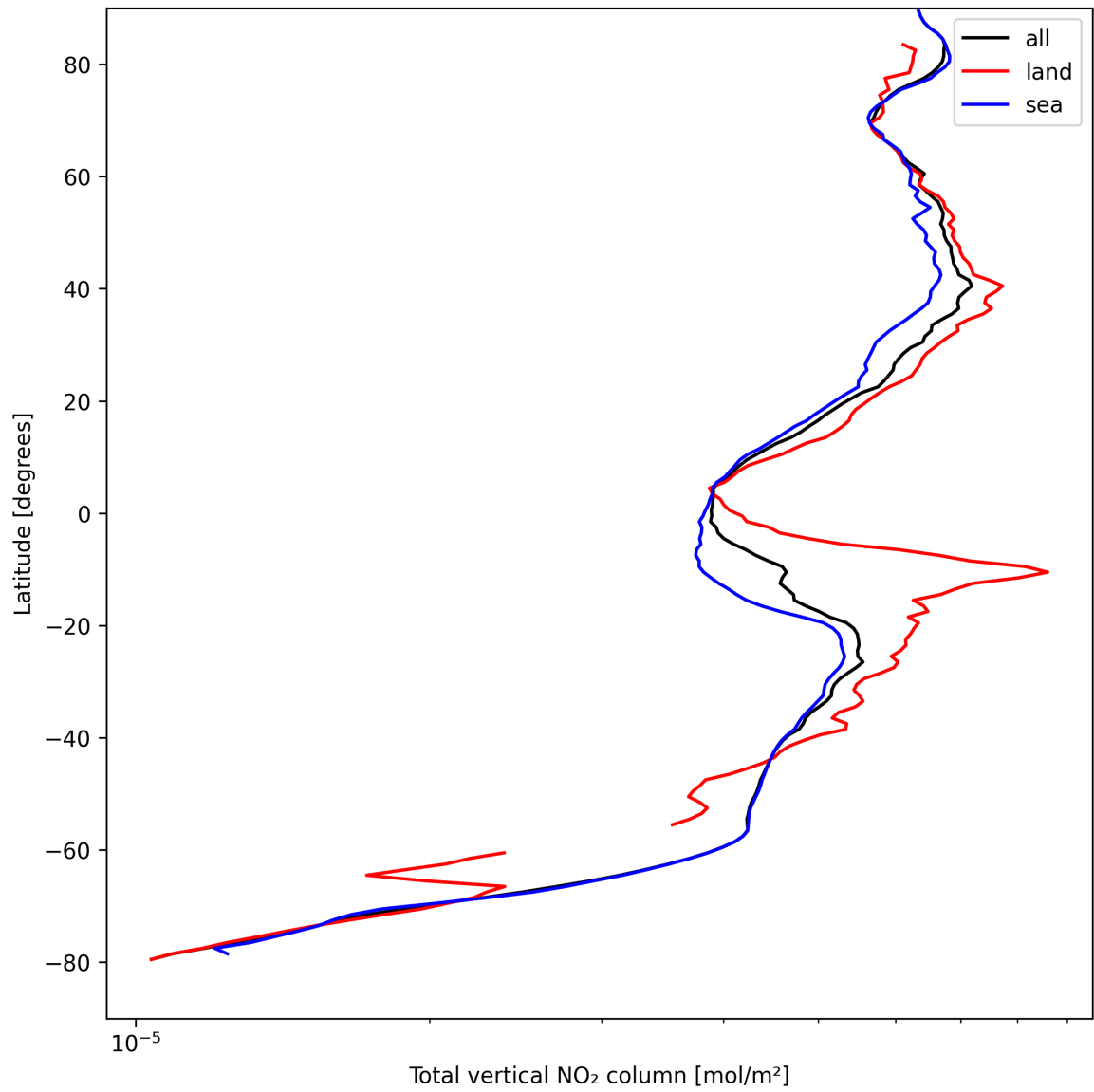
Figure 19: Zonal average of “Total vertical NO 2 column” for 2025-08-31 to 2025-09-01.
