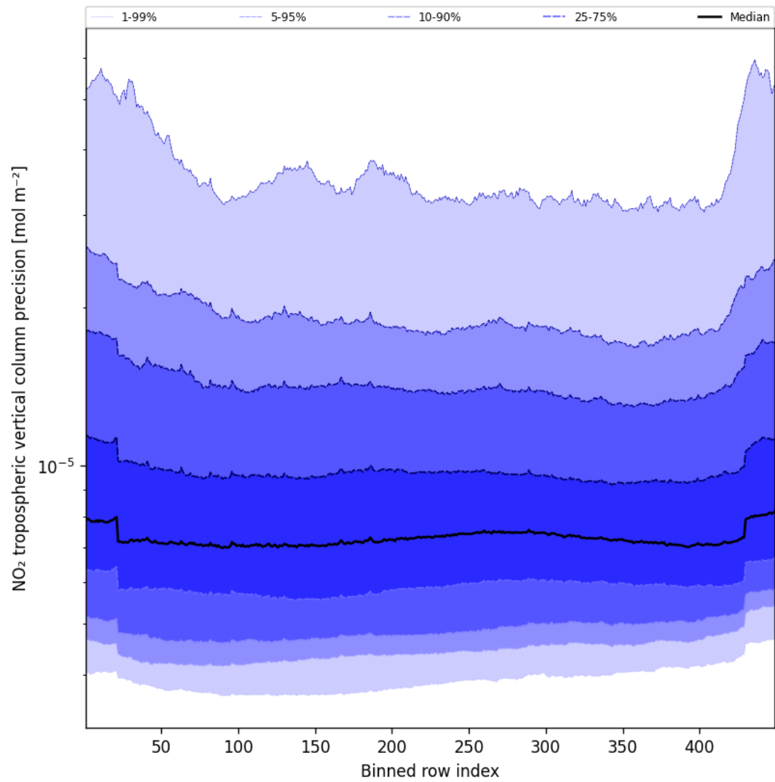
Figure 45: Along track statistics of “NO 2 tropospheric vertical column precision” for 2025-08-31 to 2025-09-01
