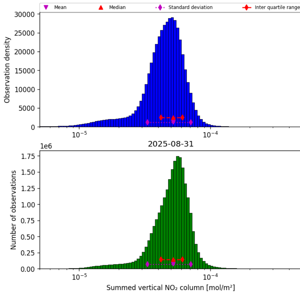
Figure 38: Histogram of “Summed vertical NO 2 column” for 2025-08-31 to 2025-09-01
