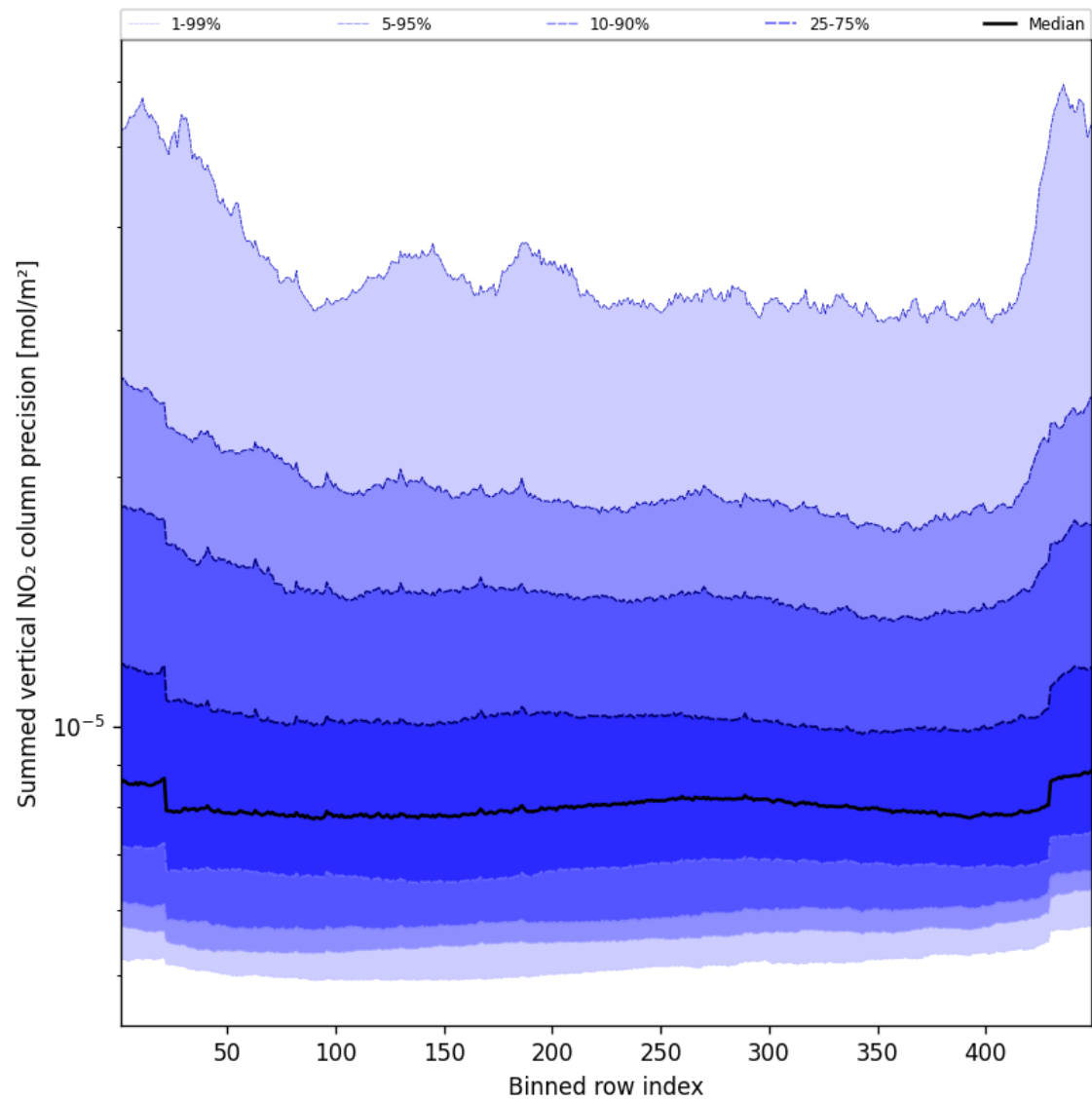
Figure 56: Along track statistics of “Summed vertical NO 2 column precision” for 2025-08-31 to 2025-09-01
