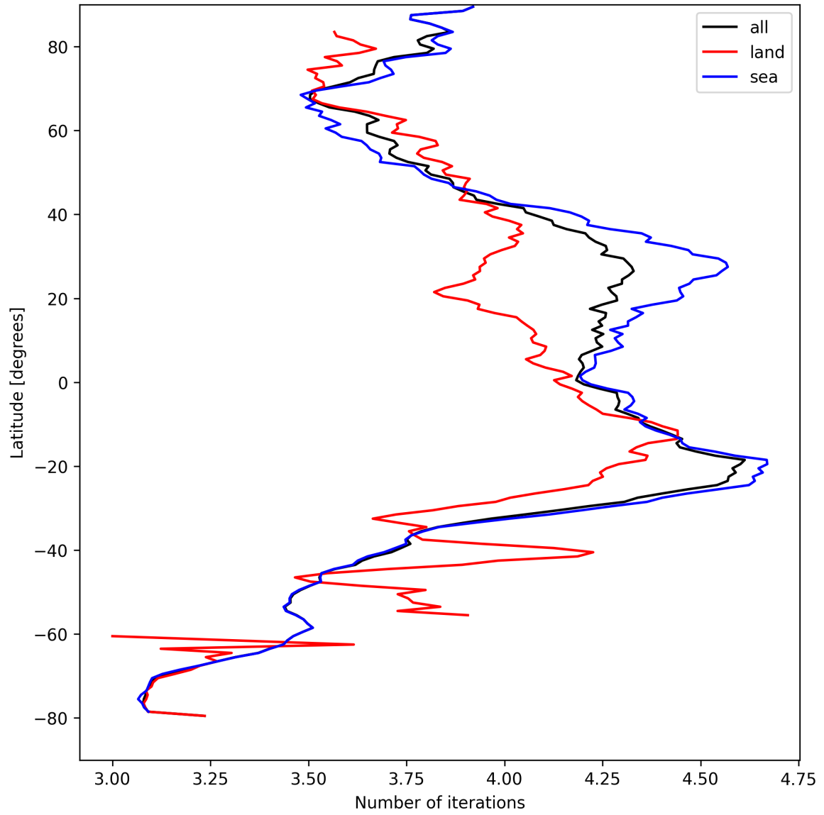
Figure 15: Zonal average of “Number of iterations” for 2025-08-31 to 2025-09-01.
