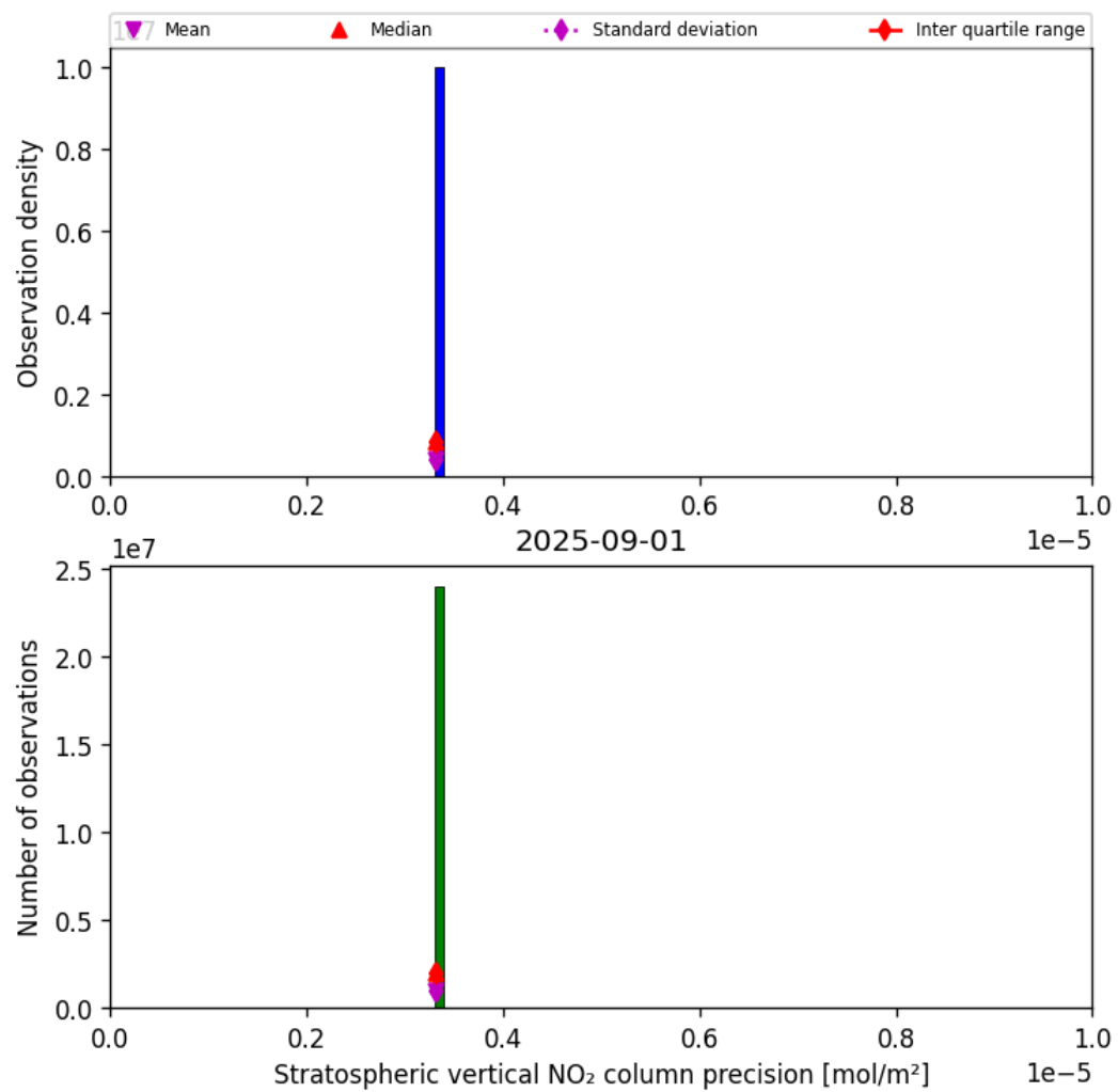
Figure 35: Histogram of “Stratospheric vertical NO 2 column precision” for 2025-09-01 to 2025-09-02
