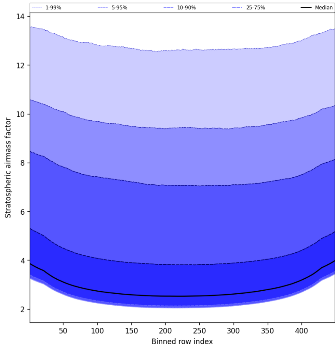
Figure 59: Along track statistics of “Stratospheric airmass factor” for 2025-09-01 to 2025-09-02
