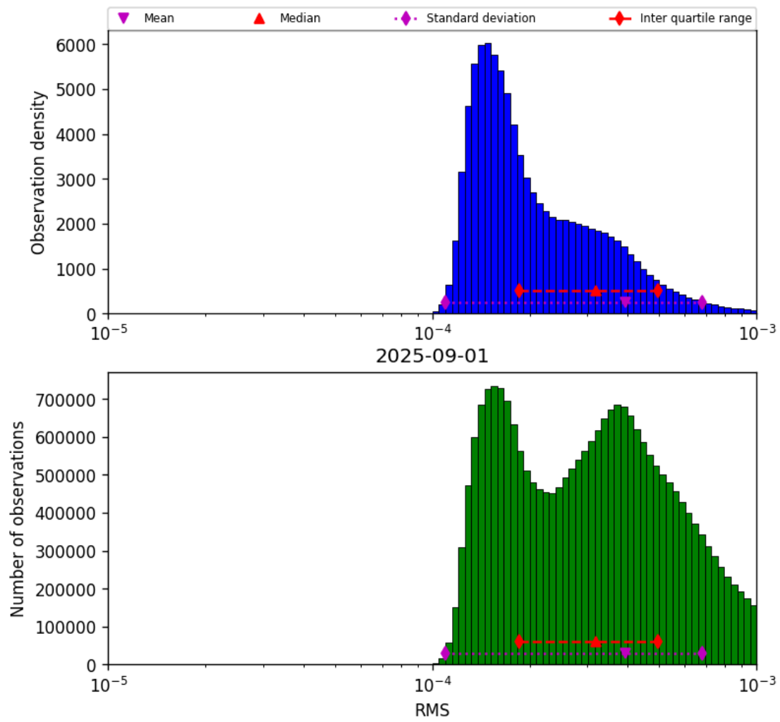
Figure 41: Histogram of “RMS” for 2025-09-01 to 2025-09-02
