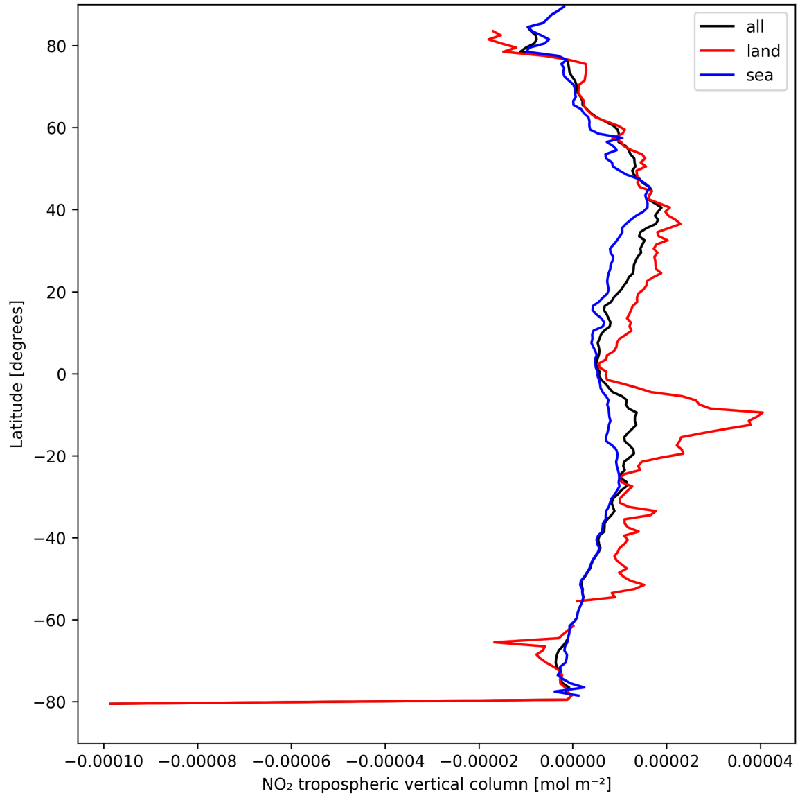
Figure 10: Zonal average of “NO 2 tropospheric vertical column” for 2025-09-01 to 2025-09-02.
