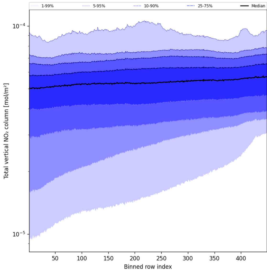
Figure 53: Along track statistics of “Total vertical NO 2 column” for 2025-09-01 to 2025-09-02
