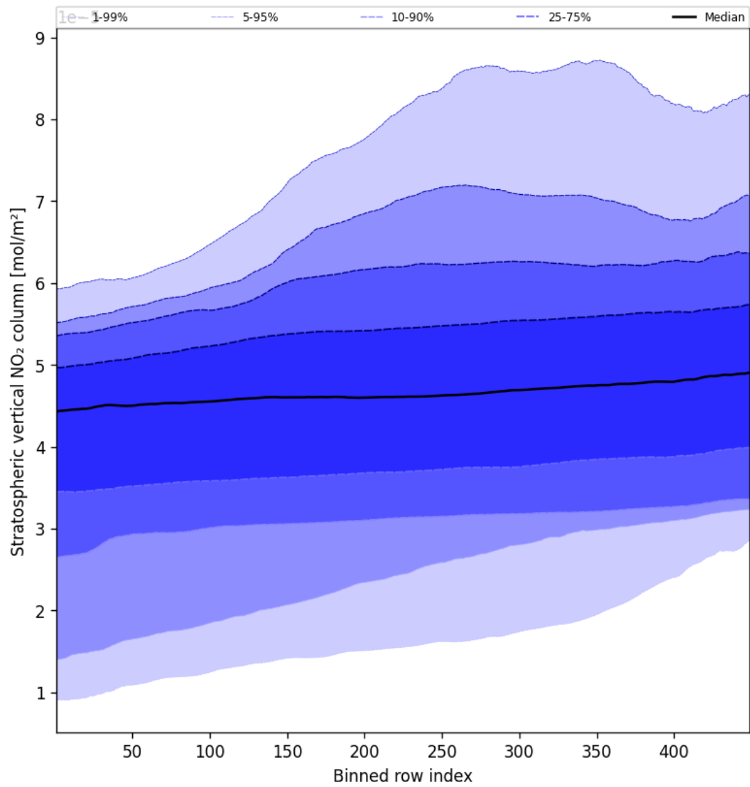
Figure 51: Along track statistics of “Stratospheric vertical NO 2 column” for 2025-09-01 to 2025-09-02
