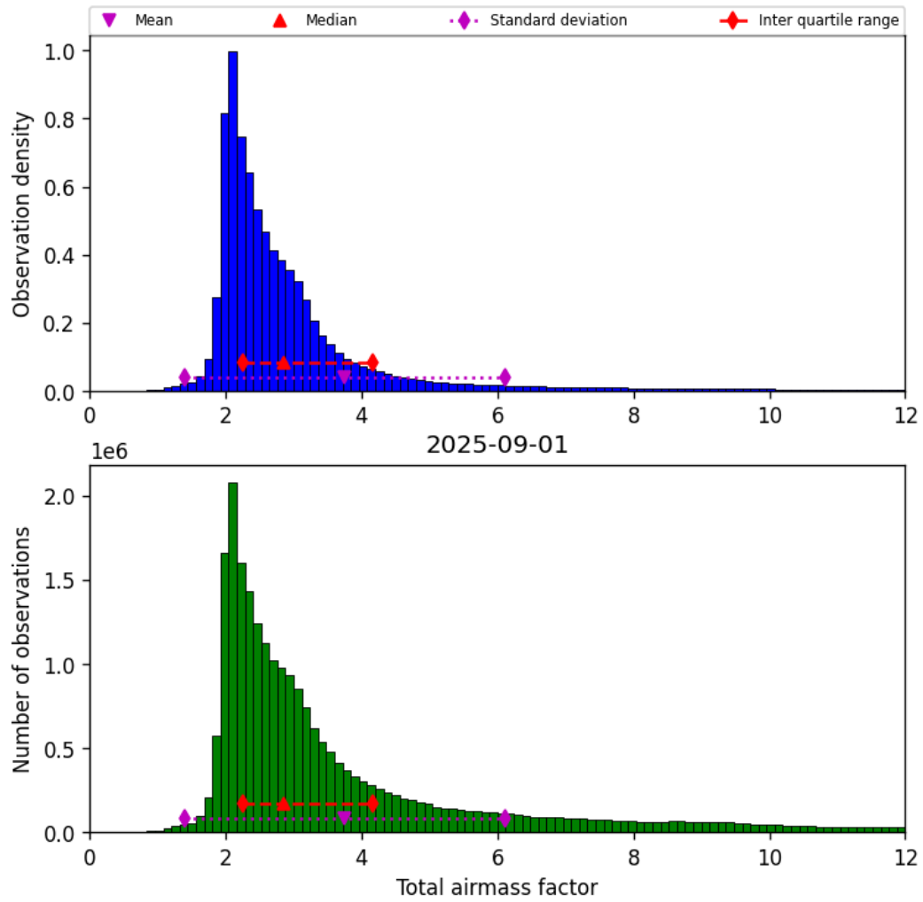
Figure 30: Histogram of “Total airmass factor” for 2025-09-01 to 2025-09-02
