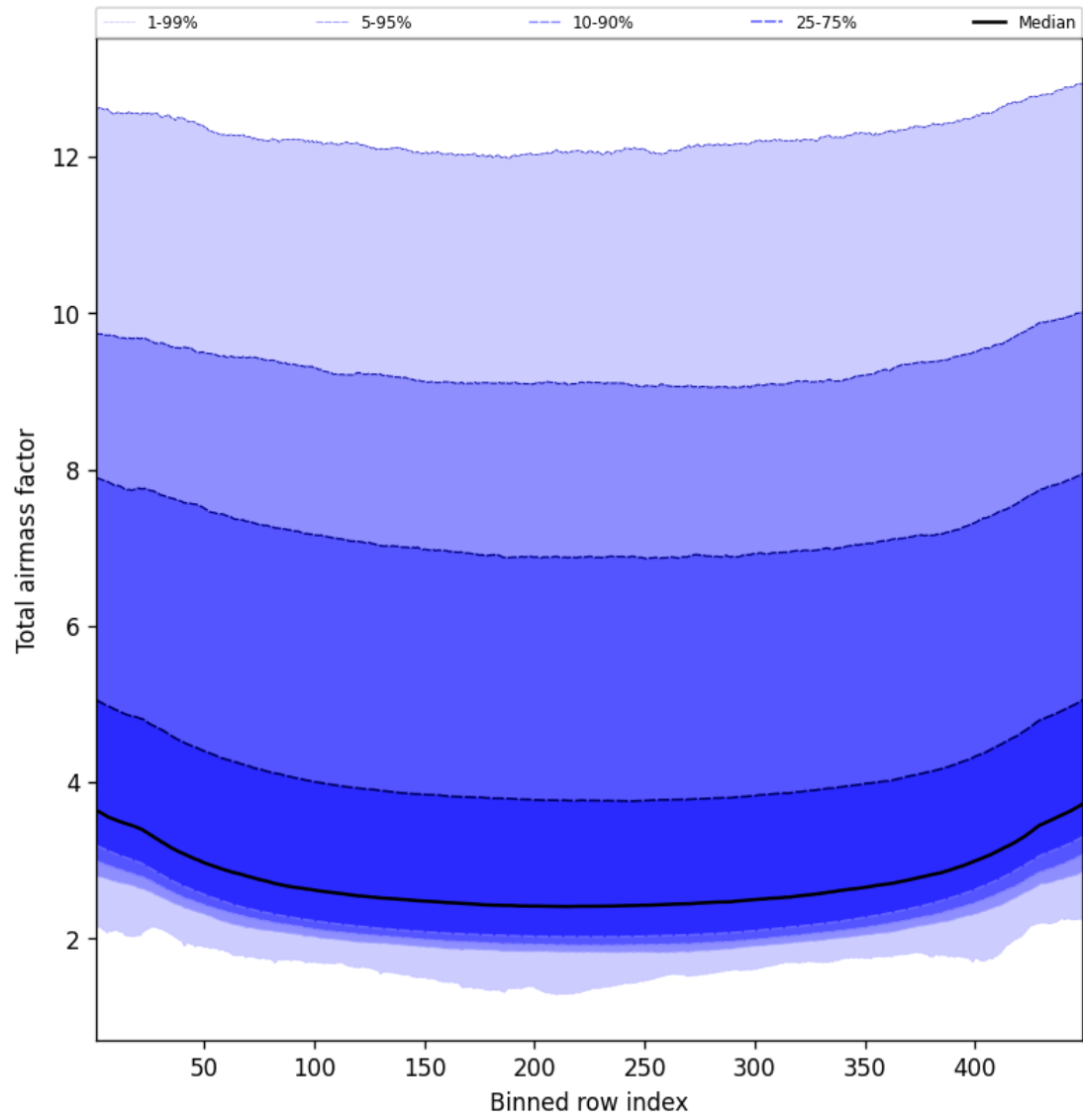
Figure 47: Along track statistics of “Total airmass factor” for 2025-09-01 to 2025-09-02
