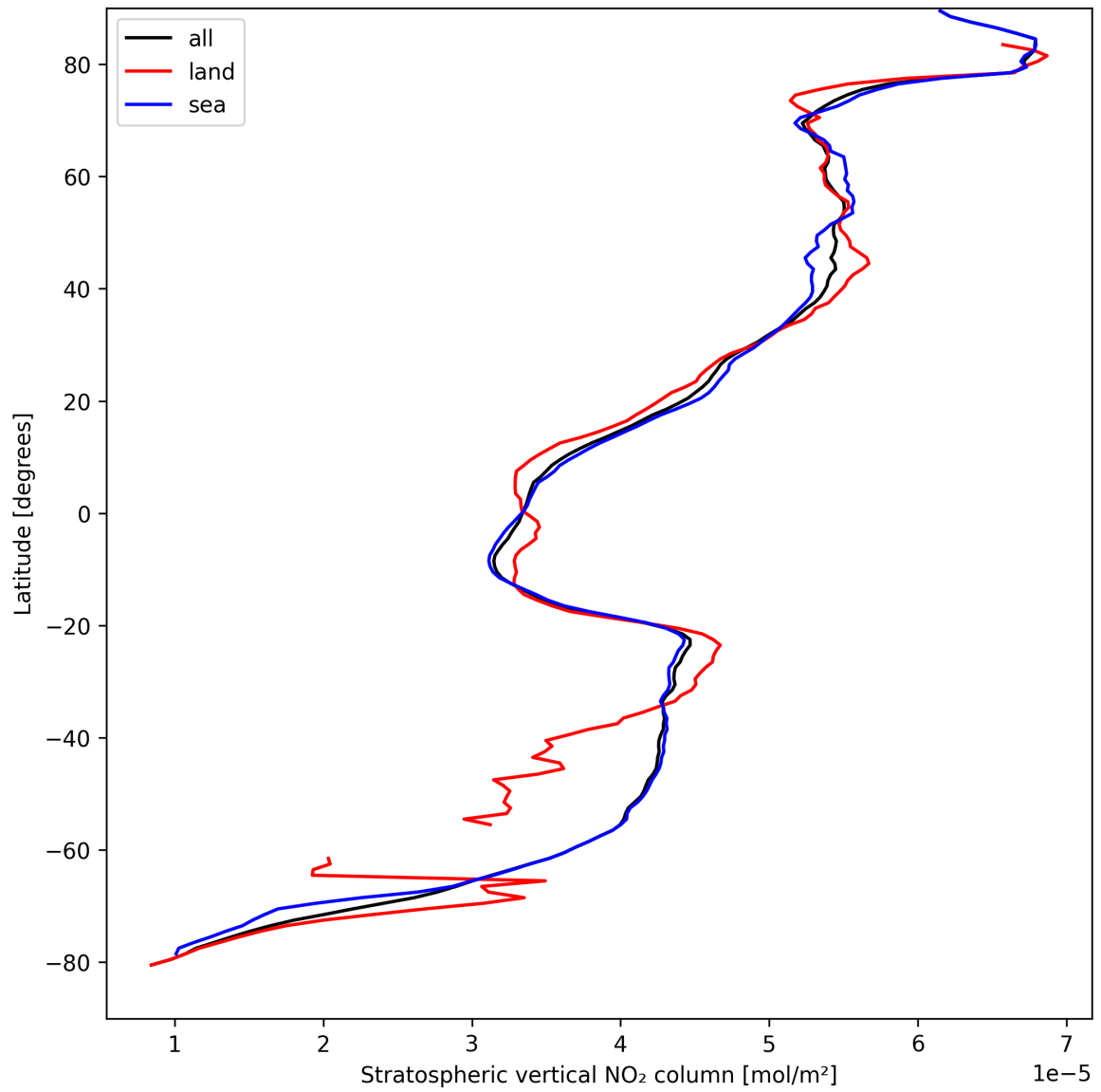
Figure 17: Zonal average of “Stratospheric vertical NO 2 column” for 2025-09-01 to 2025-09-02.
