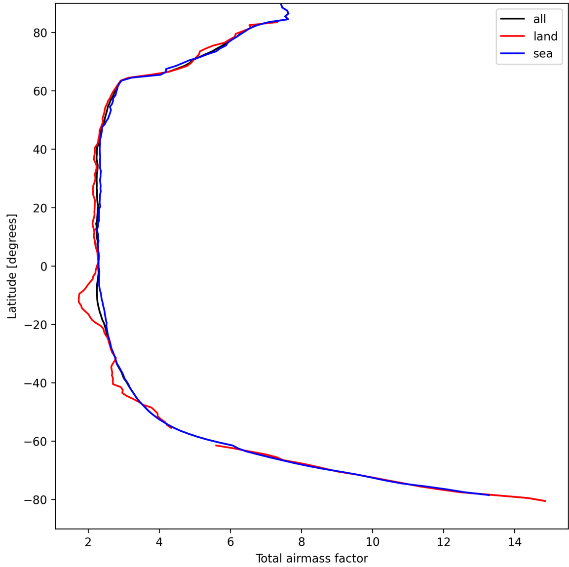
Figure 13: Zonal average of “Total airmass factor” for 2025-09-01 to 2025-09-02.
