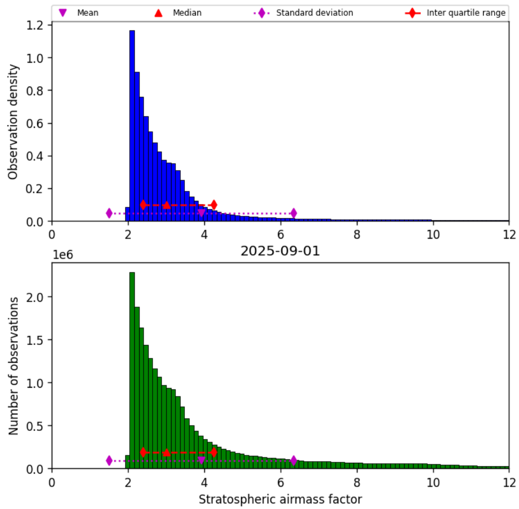
Figure 42: Histogram of “Stratospheric airmass factor” for 2025-09-01 to 2025-09-02
