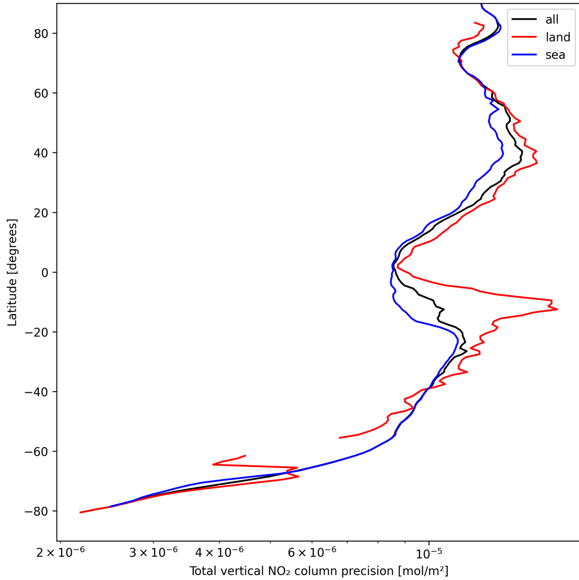
Figure 20: Zonal average of “Total vertical NO 2 column precision” for 2025-09-01 to 2025-09-02.
