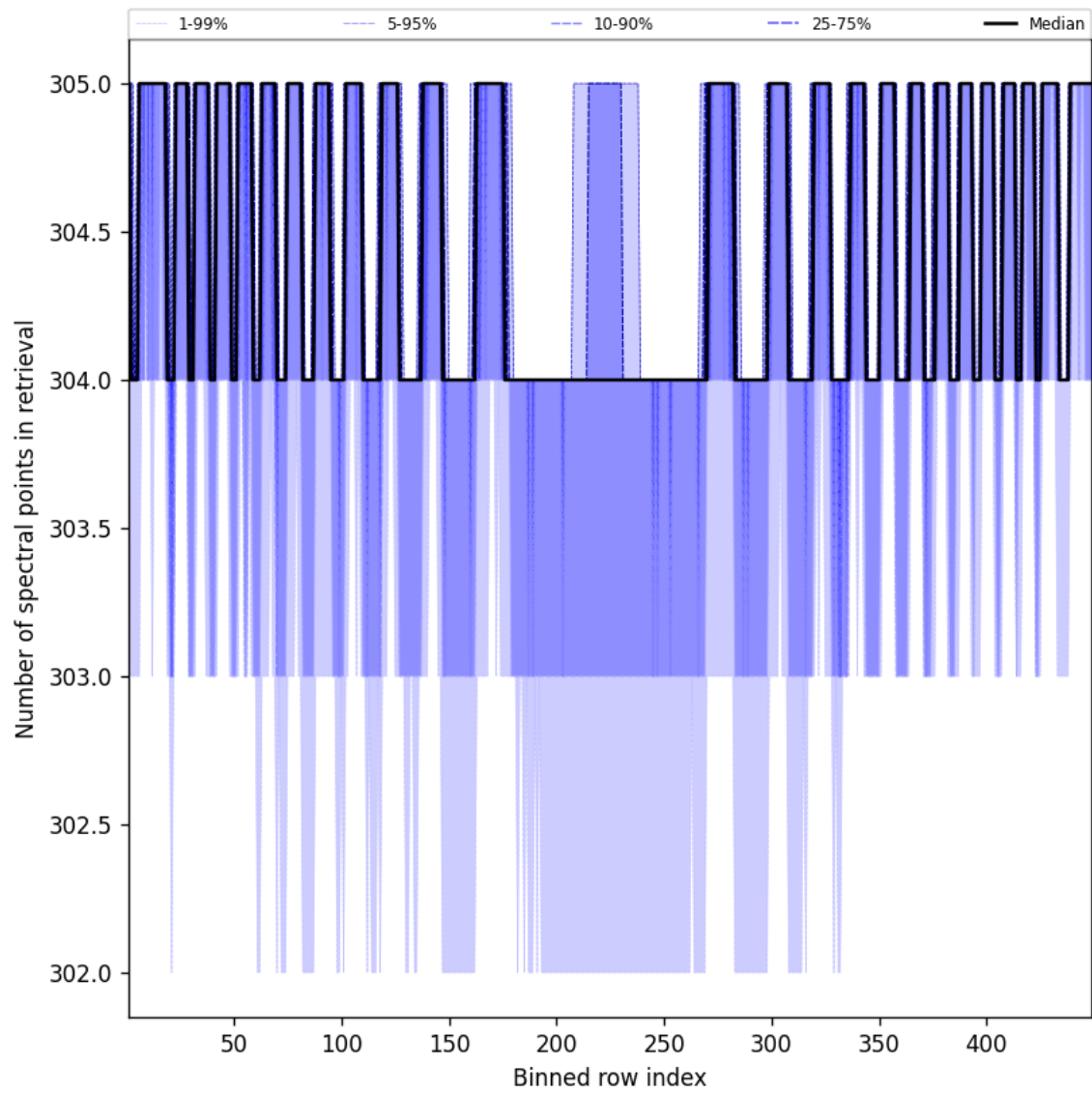
Figure 48: Along track statistics of “Number of spectral points in retrieval” for 2025-09-01 to 2025-09-02
