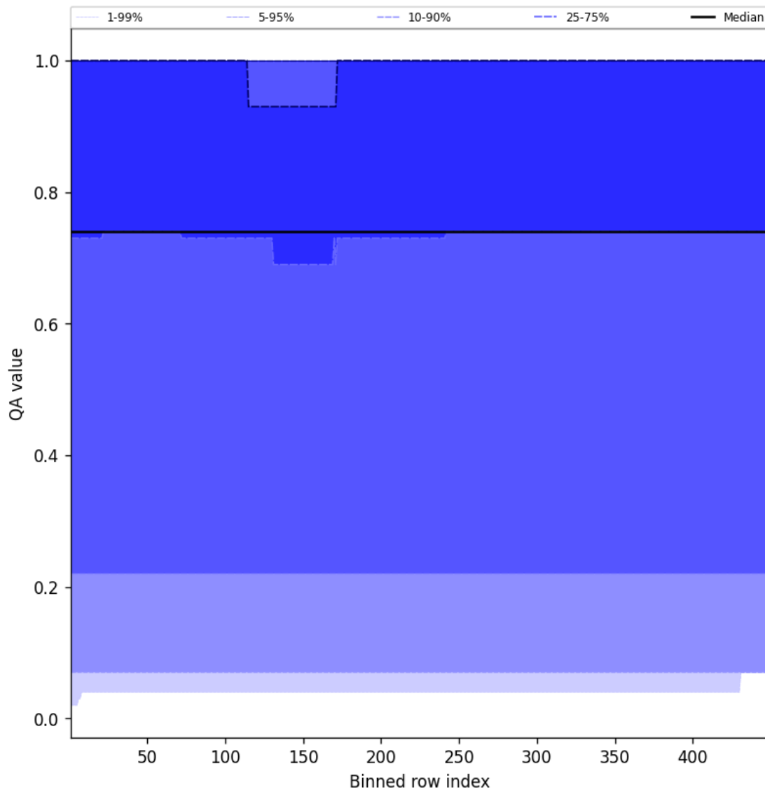
Figure 43: Along track statistics of “QA value” for 2025-09-01 to 2025-09-02
