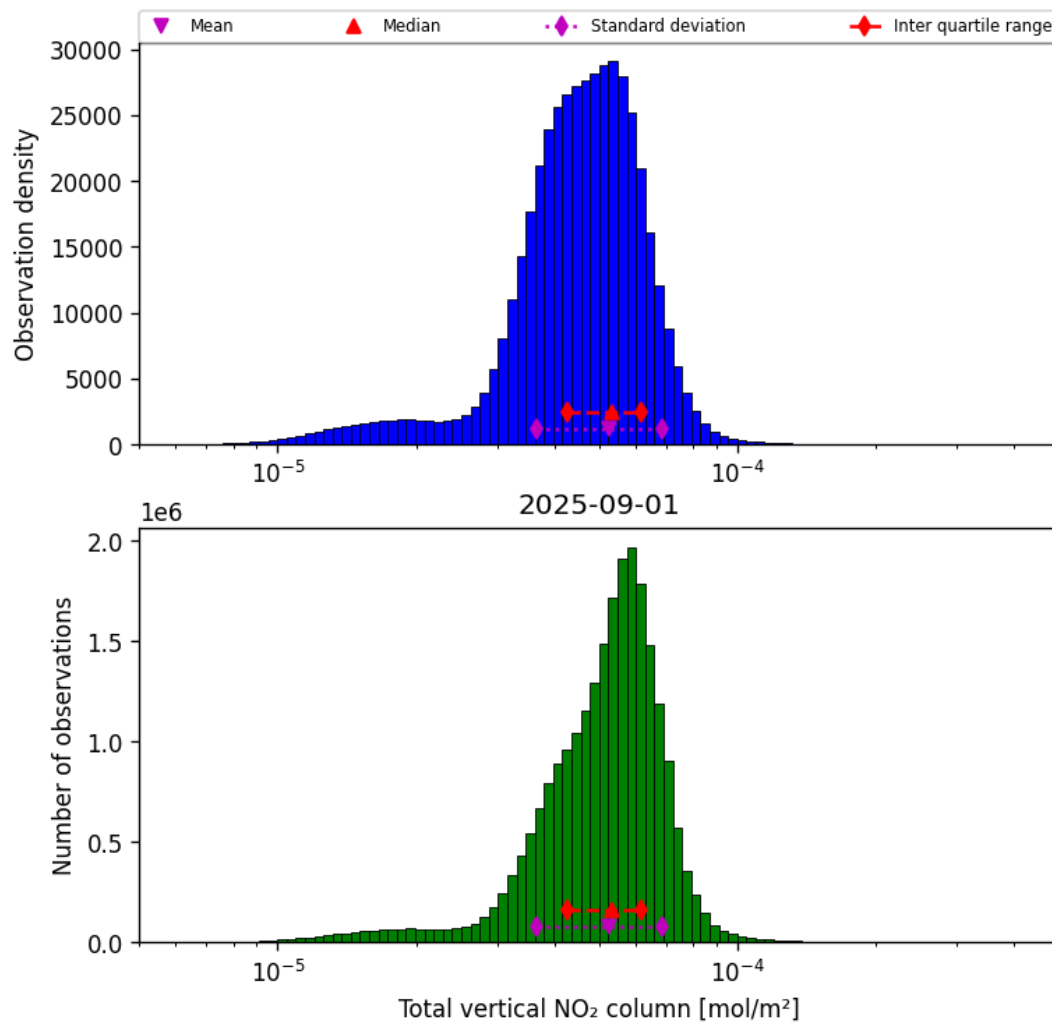
Figure 36: Histogram of “Total vertical NO 2 column” for 2025-09-01 to 2025-09-02
