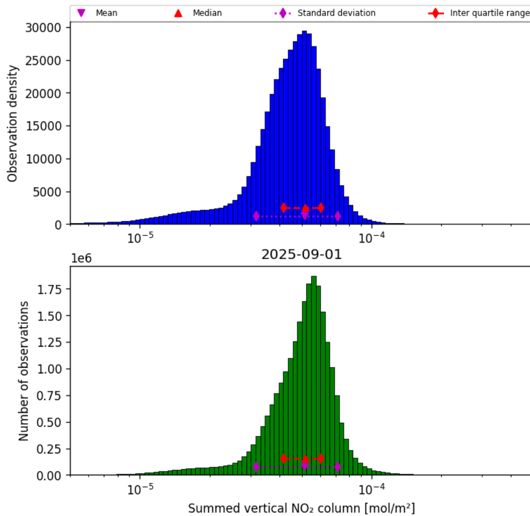
Figure 38: Histogram of “Summed vertical NO 2 column” for 2025-09-01 to 2025-09-02
