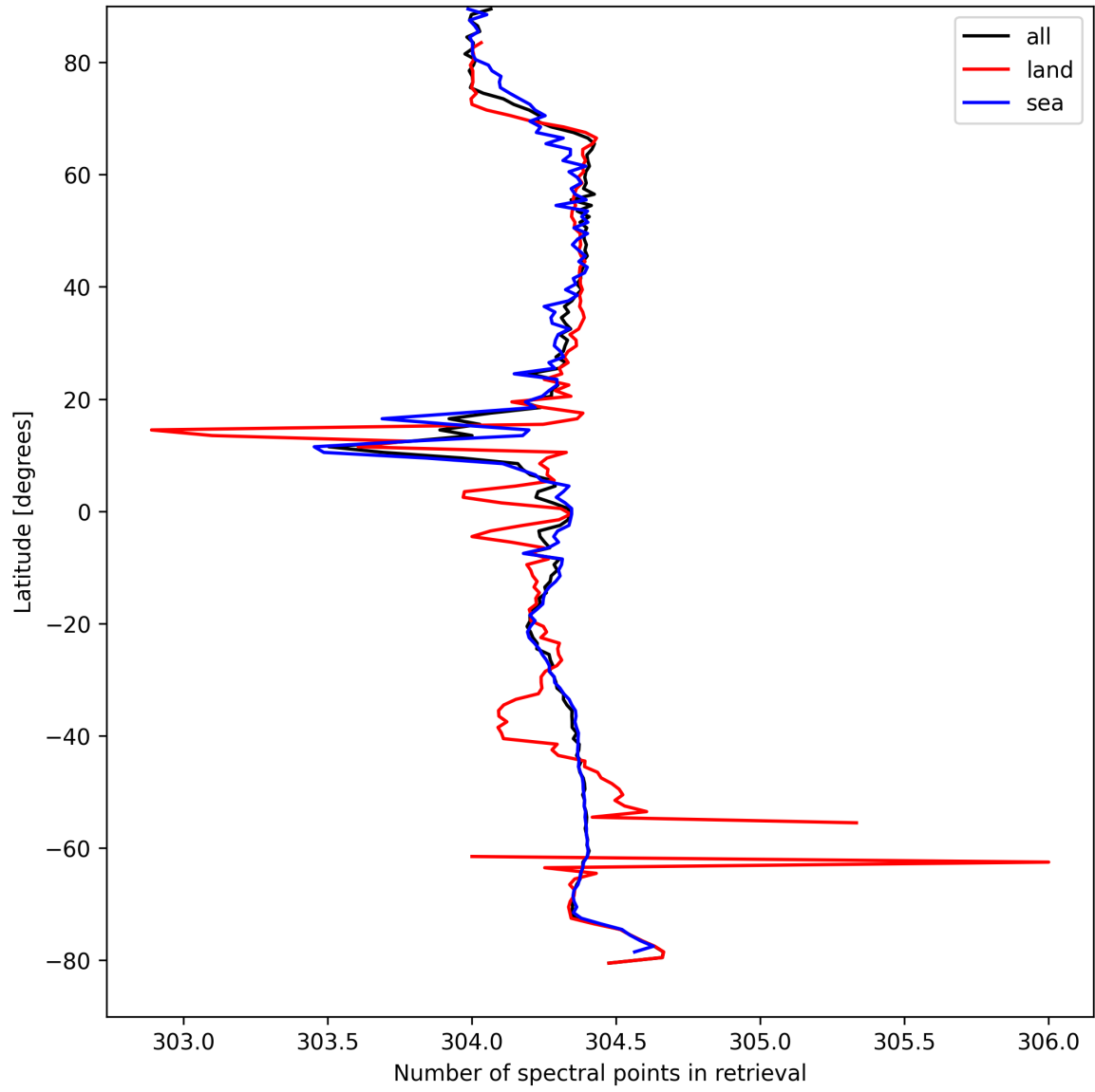
Figure 14: Zonal average of “Number of spectral points in retrieval” for 2025-09-01 to 2025-09-02.
