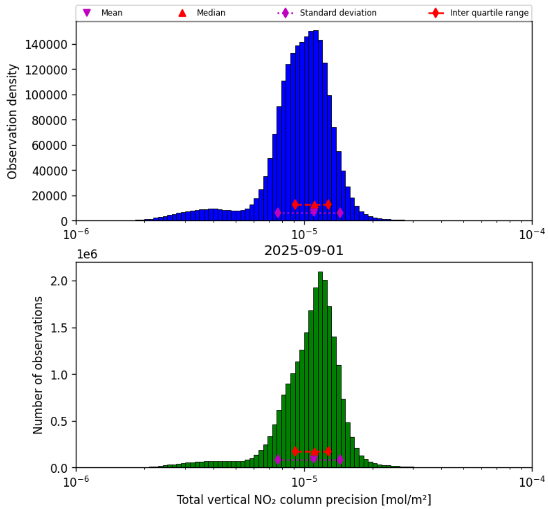
Figure 37: Histogram of “Total vertical NO 2 column precision” for 2025-09-01 to 2025-09-02
