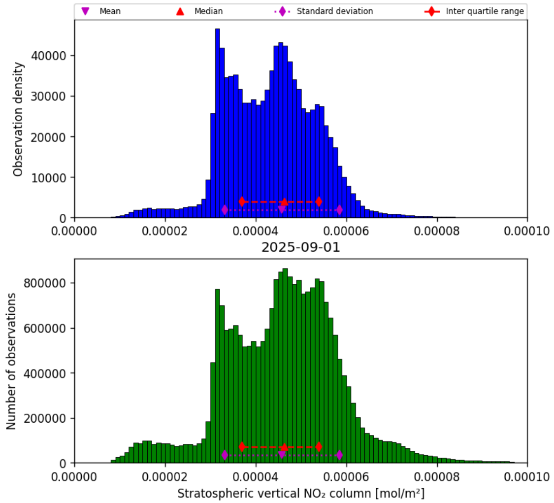
Figure 34: Histogram of “Stratospheric vertical NO 2 column” for 2025-09-01 to 2025-09-02
