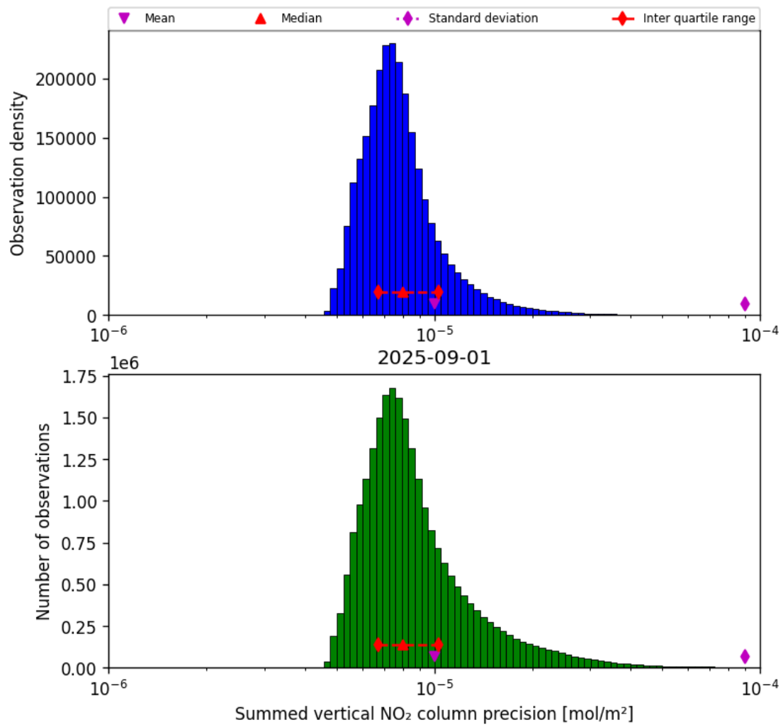
Figure 39: Histogram of "Summed vertical NO 2 column precision" for 2025-09-01 to 2025-09-02
