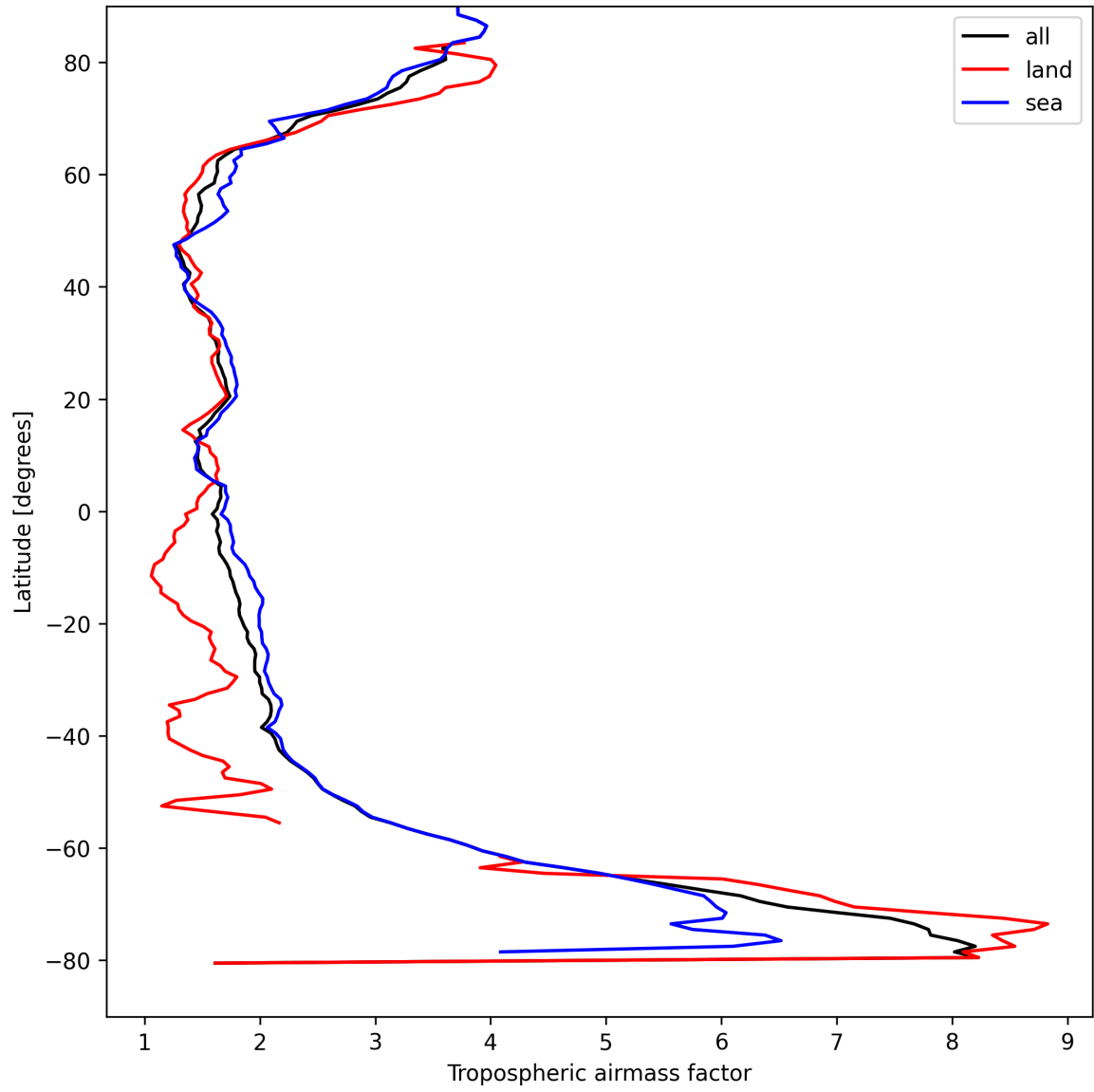
Figure 12: Zonal average of “Tropospheric airmass factor” for 2025-09-01 to 2025-09-02.
