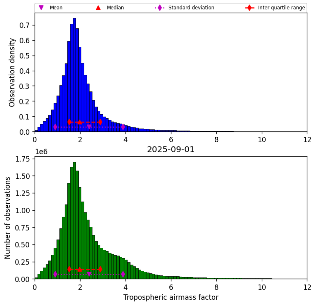
Figure 29: Histogram of “Tropospheric airmass factor” for 2025-09-01 to 2025-09-02
