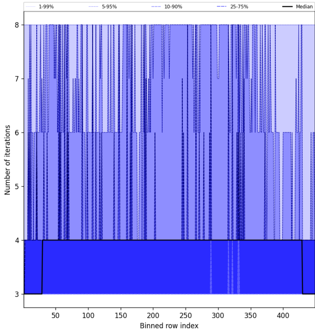
Figure 49: Along track statistics of “Number of iterations” for 2025-09-01 to 2025-09-02
