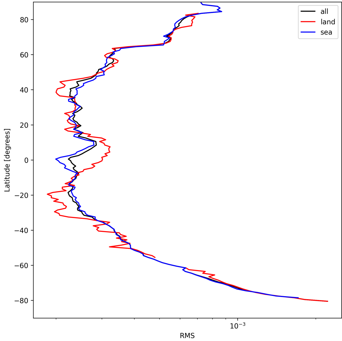
Figure 24: Zonal average of “RMS” for 2025-09-01 to 2025-09-02.
