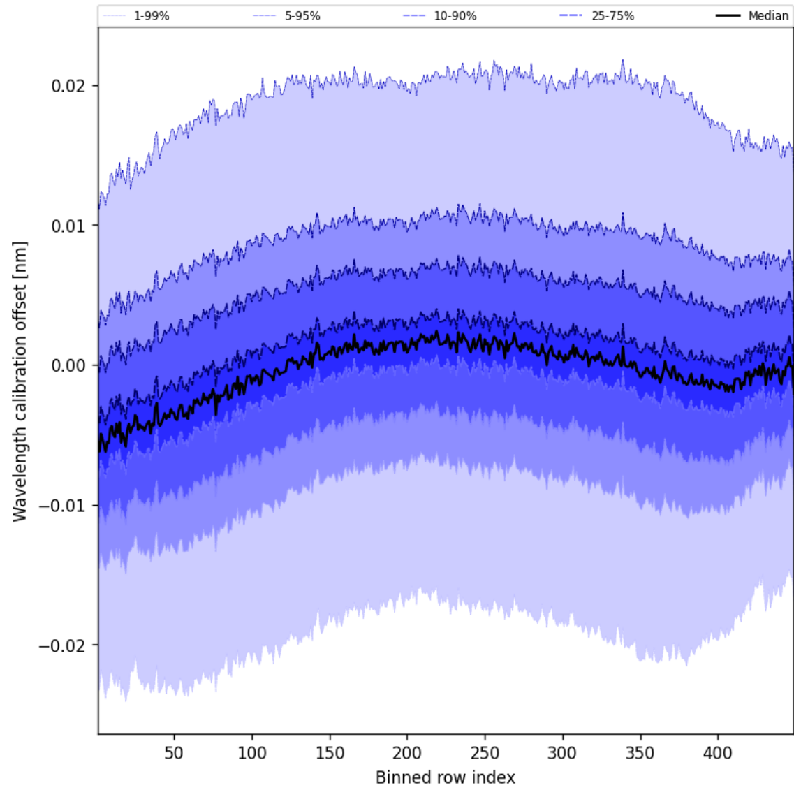
Figure 50: Along track statistics of “Wavelength calibration offset” for 2025-09-01 to 2025-09-02
