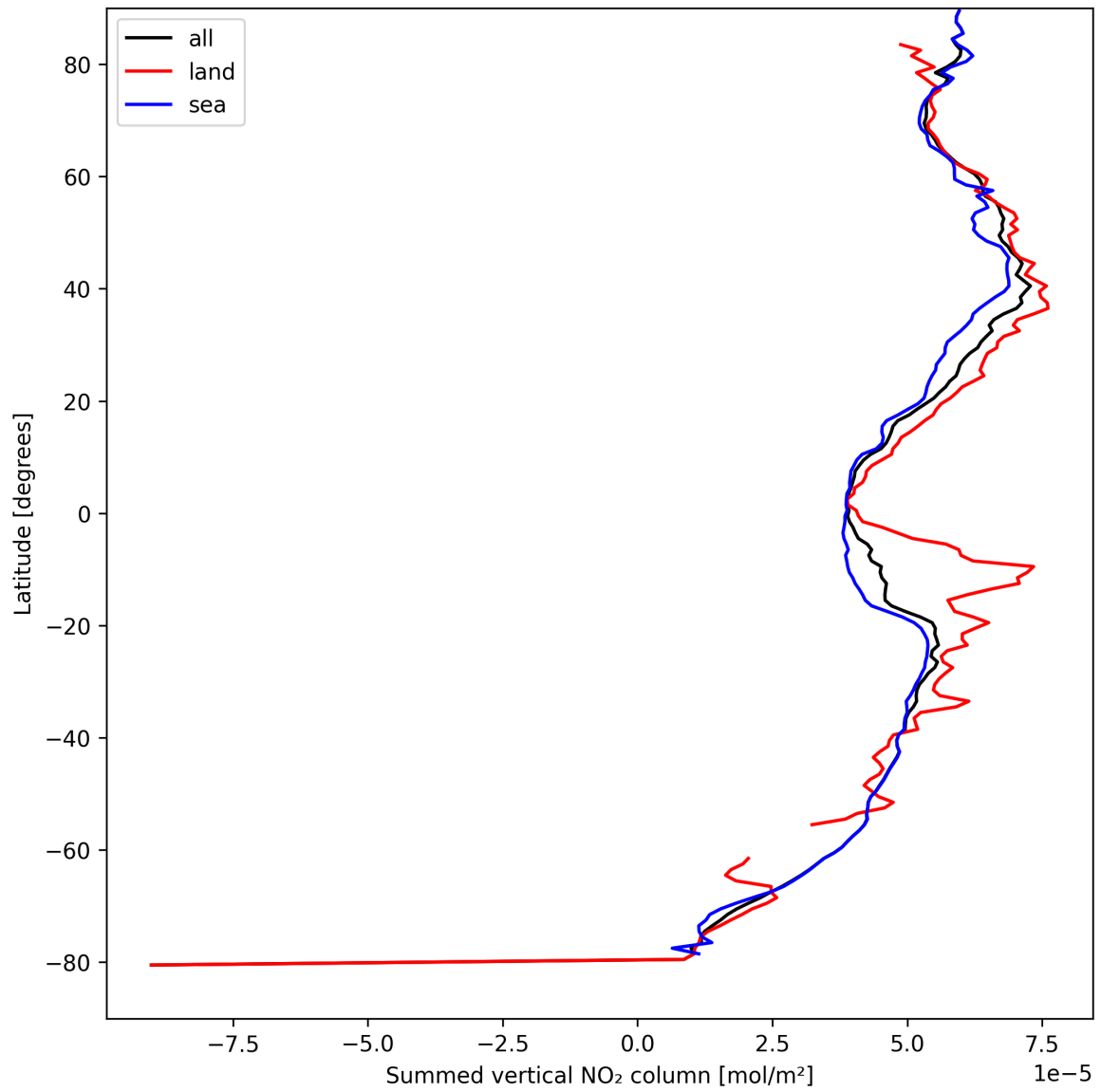
Figure 21: Zonal average of “Summed vertical NO 2 column” for 2025-09-01 to 2025-09-02.
