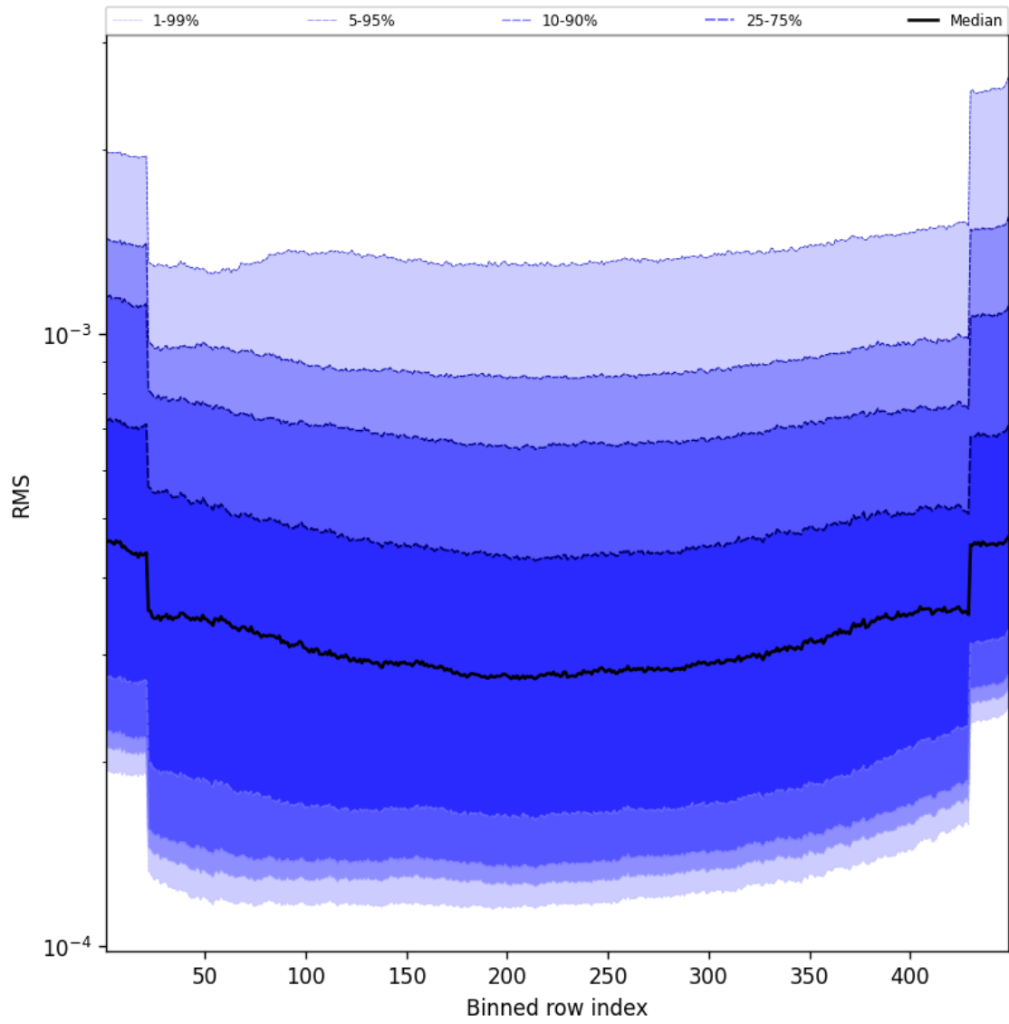
Figure 58: Along track statistics of “RMS” for 2025-09-01 to 2025-09-02
