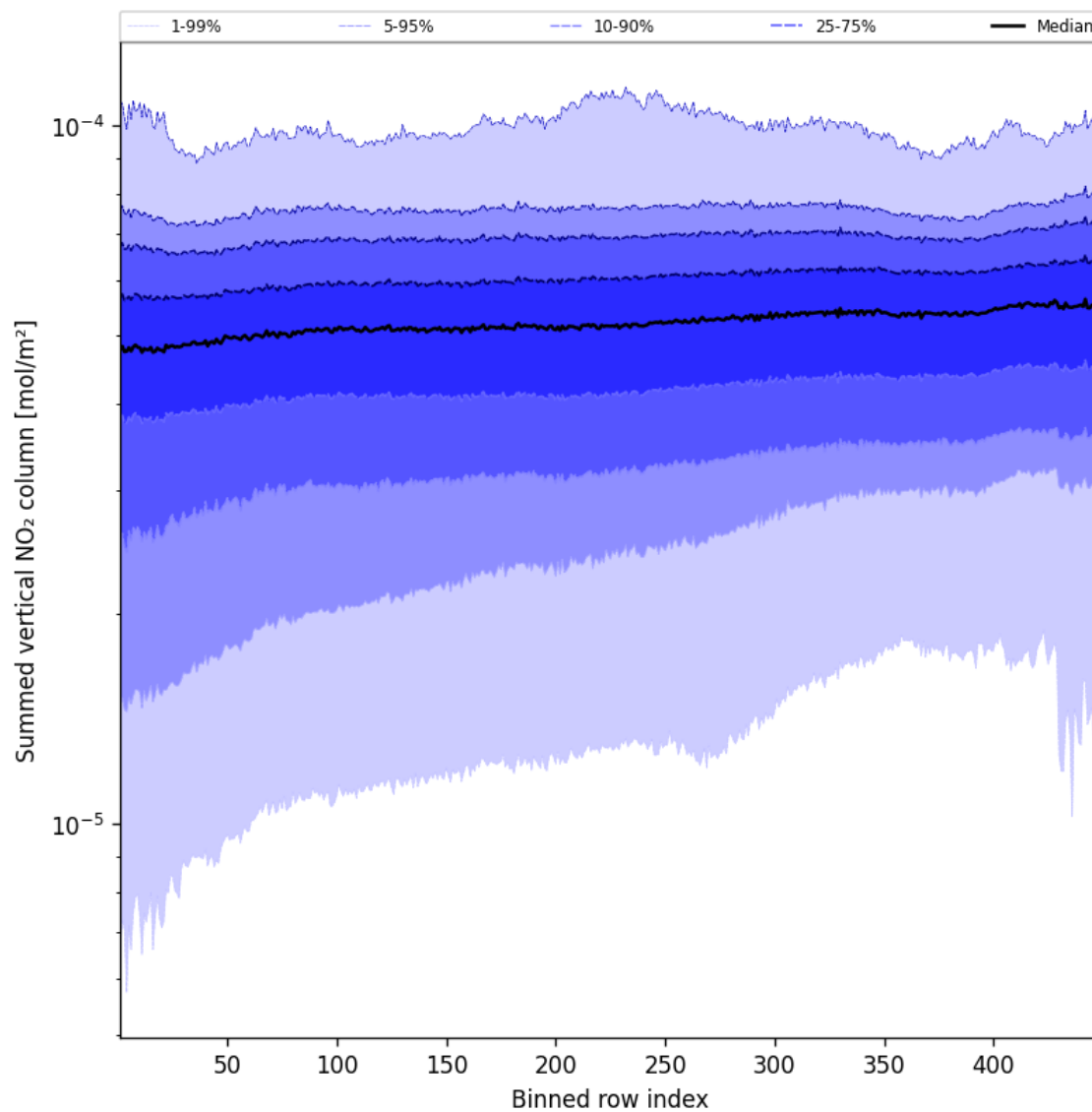
Figure 55: Along track statistics of “Summed vertical NO 2 column” for 2025-09-01 to 2025-09-02
