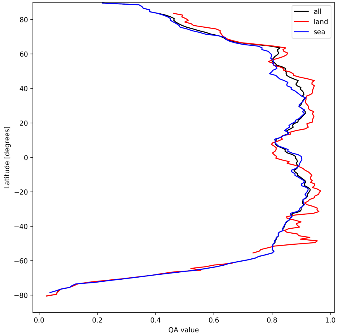
Figure 9: Zonal average of “QA value” for 2025-09-01 to 2025-09-02.
