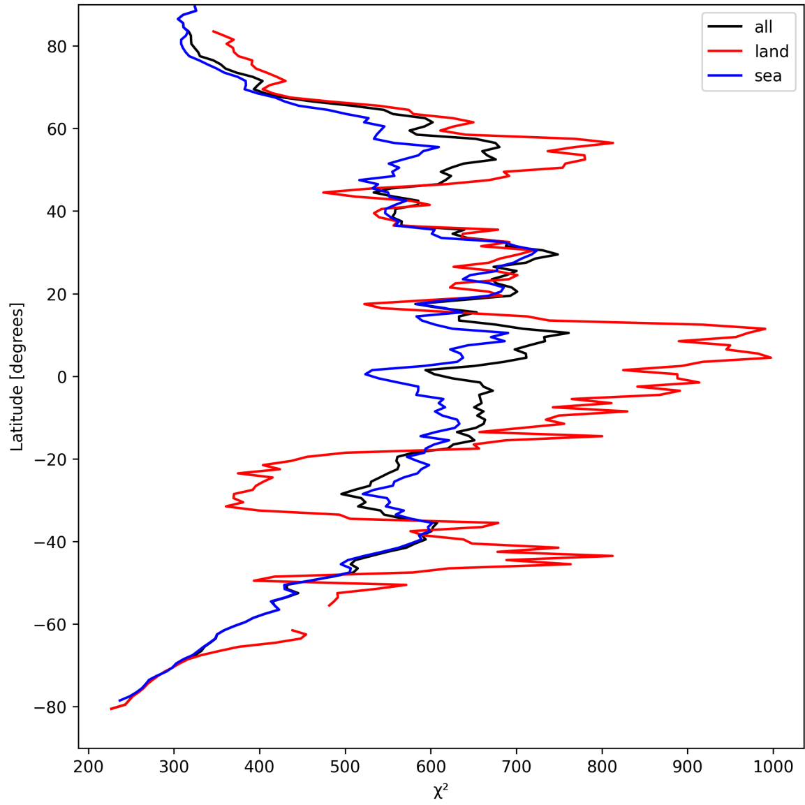
Figure 23: Zonal average of “ \chi^2 ” for 2025-09-01 to 2025-09-02.
