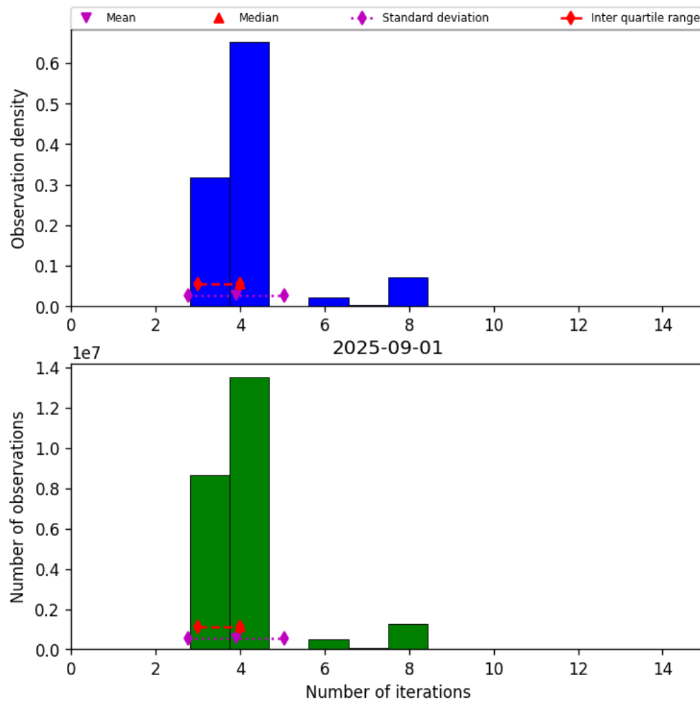
Figure 32: Histogram of “Number of iterations” for 2025-09-01 to 2025-09-02
