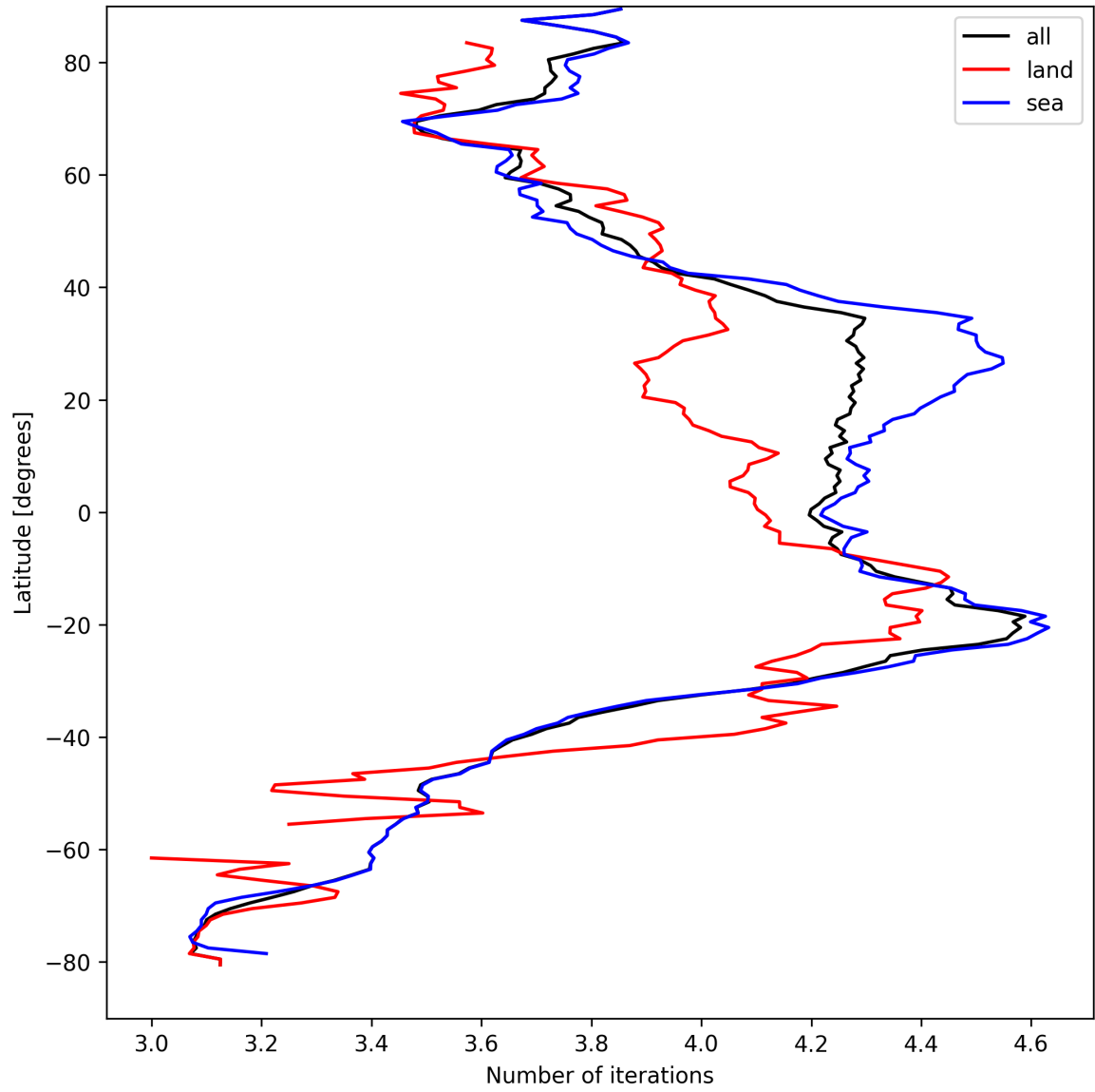
Figure 15: Zonal average of “Number of iterations” for 2025-09-01 to 2025-09-02.
