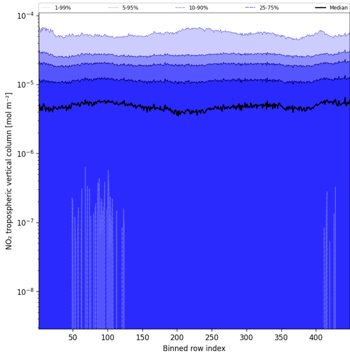
Figure 44: Along track statistics of “NO 2 tropospheric vertical column” for 2025-09-01 to 2025-09-02
