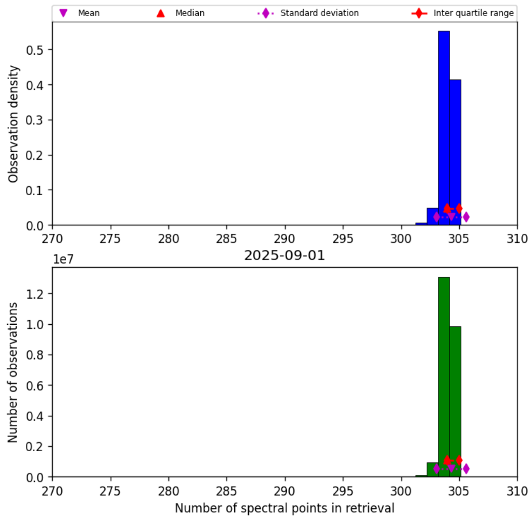
Figure 31: Histogram of “Number of spectral points in retrieval” for 2025-09-01 to 2025-09-02
