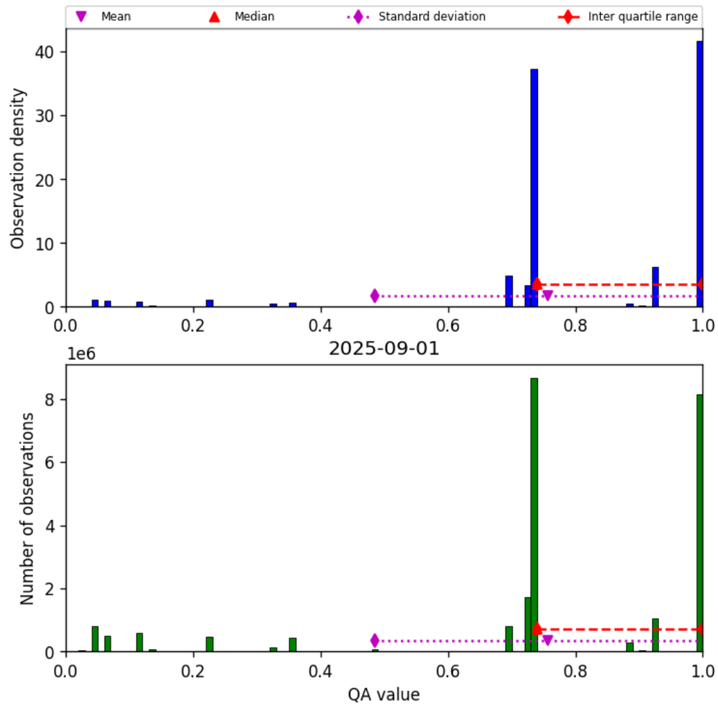
Figure 26: Histogram of “QA value” for 2025-09-01 to 2025-09-02
