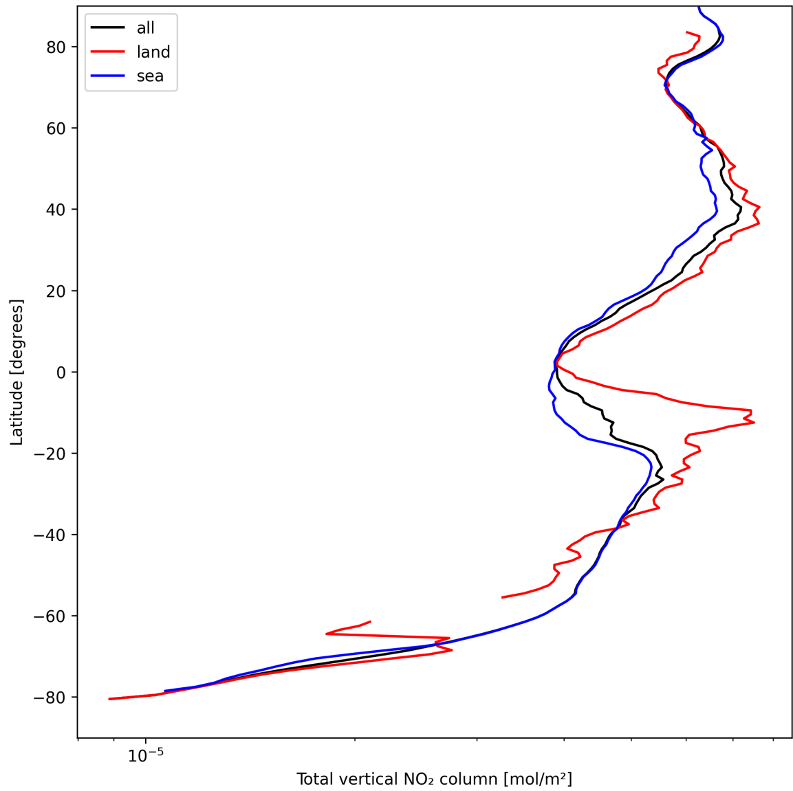
Figure 19: Zonal average of “Total vertical NO 2 column” for 2025-09-01 to 2025-09-02.
