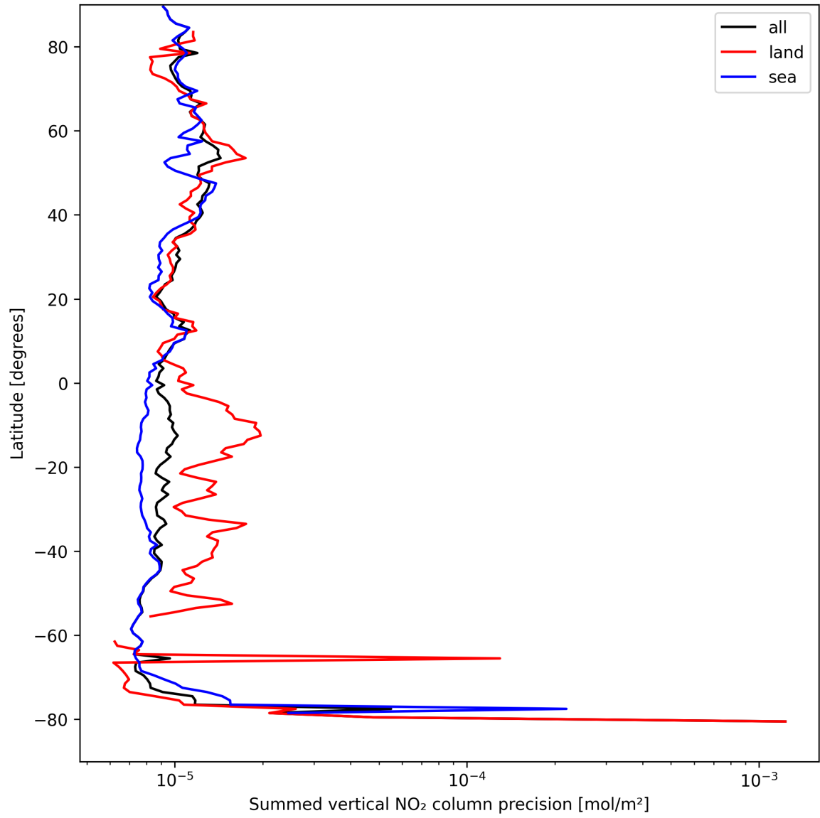
Figure 22: Zonal average of “Summed vertical NO 2 column precision” for 2025-09-01 to 2025-09-02.
