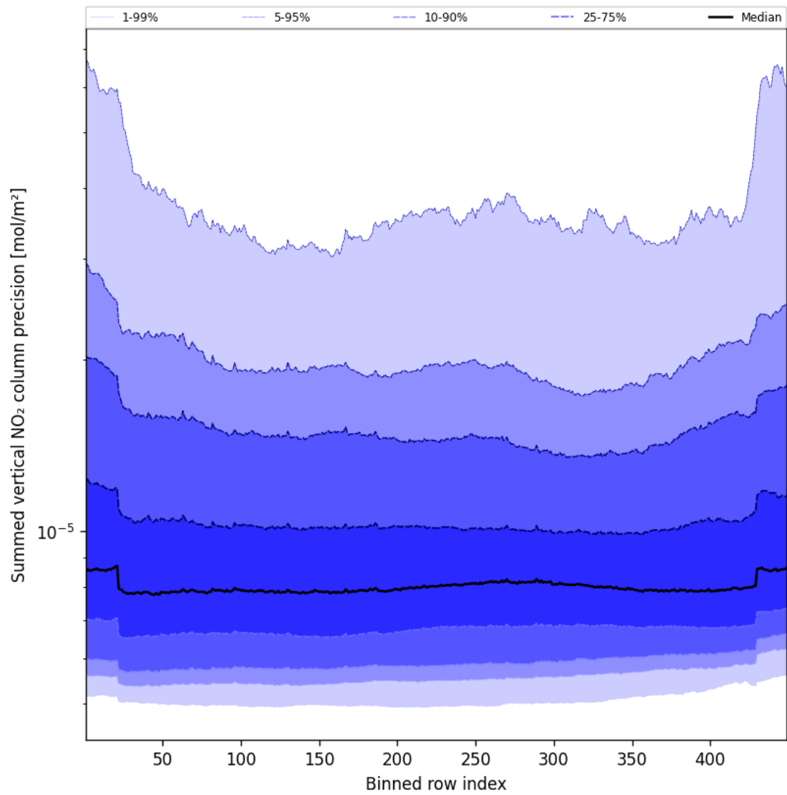
Figure 56: Along track statistics of “Summed vertical NO 2 column precision” for 2025-09-01 to 2025-09-02
