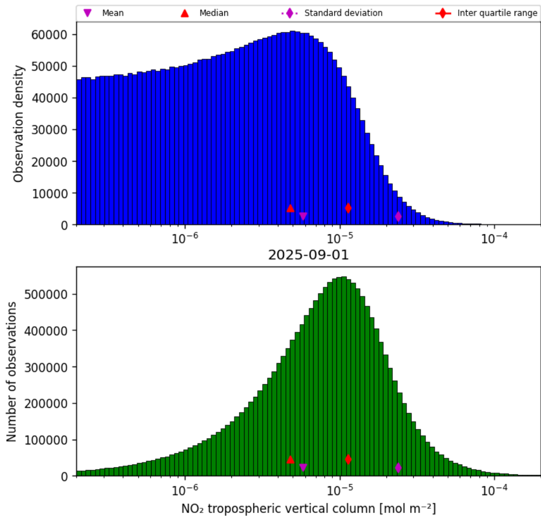
Figure 27: Histogram of “NO 2 tropospheric vertical column” for 2025-09-01 to 2025-09-02
