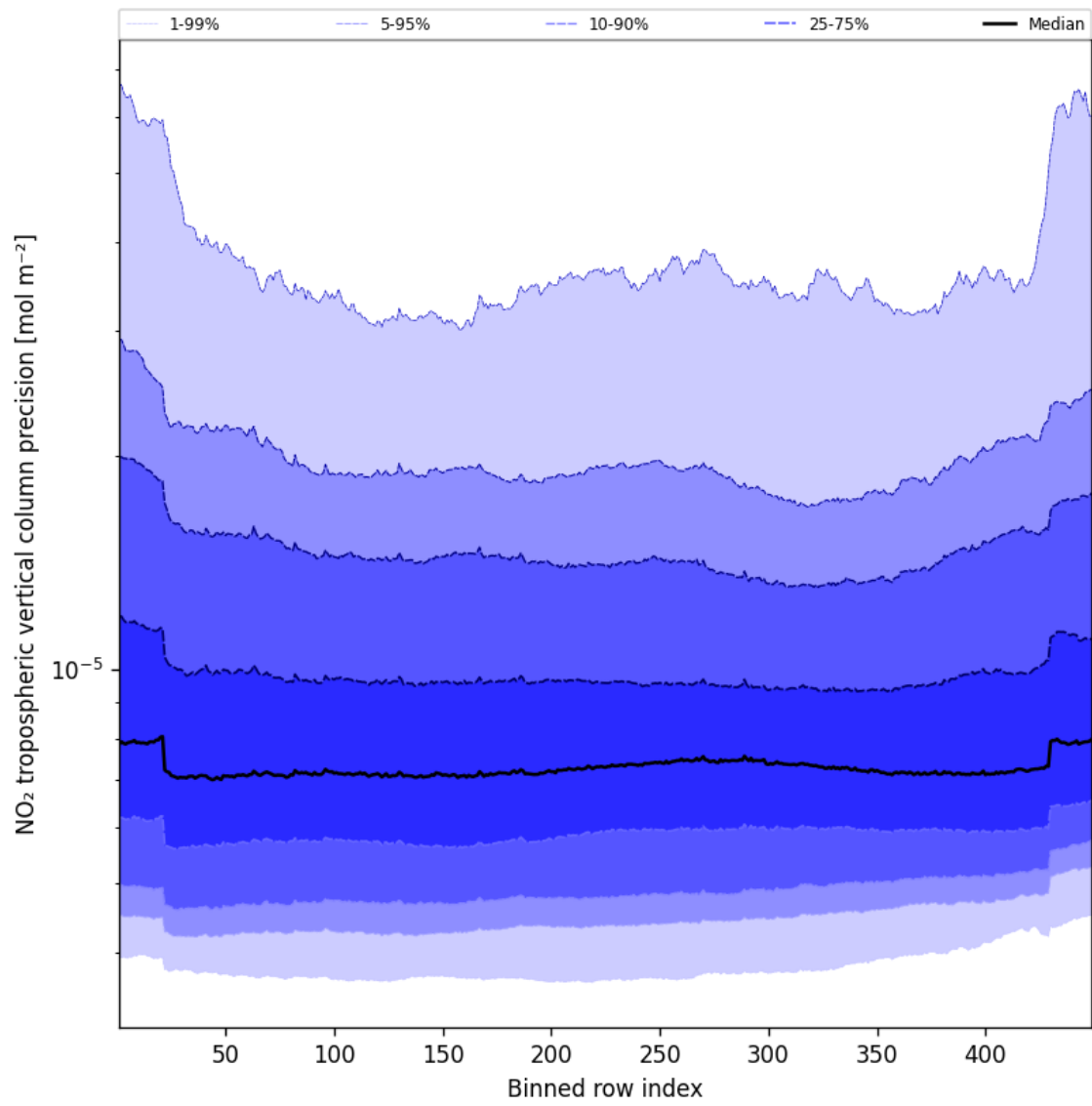
Figure 45: Along track statistics of “NO 2 tropospheric vertical column precision” for 2025-09-01 to 2025-09-02
