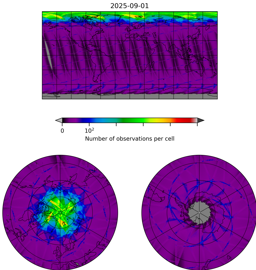
Figure 8: Map of the number of observations for 2025-09-01 to 2025-09-02
