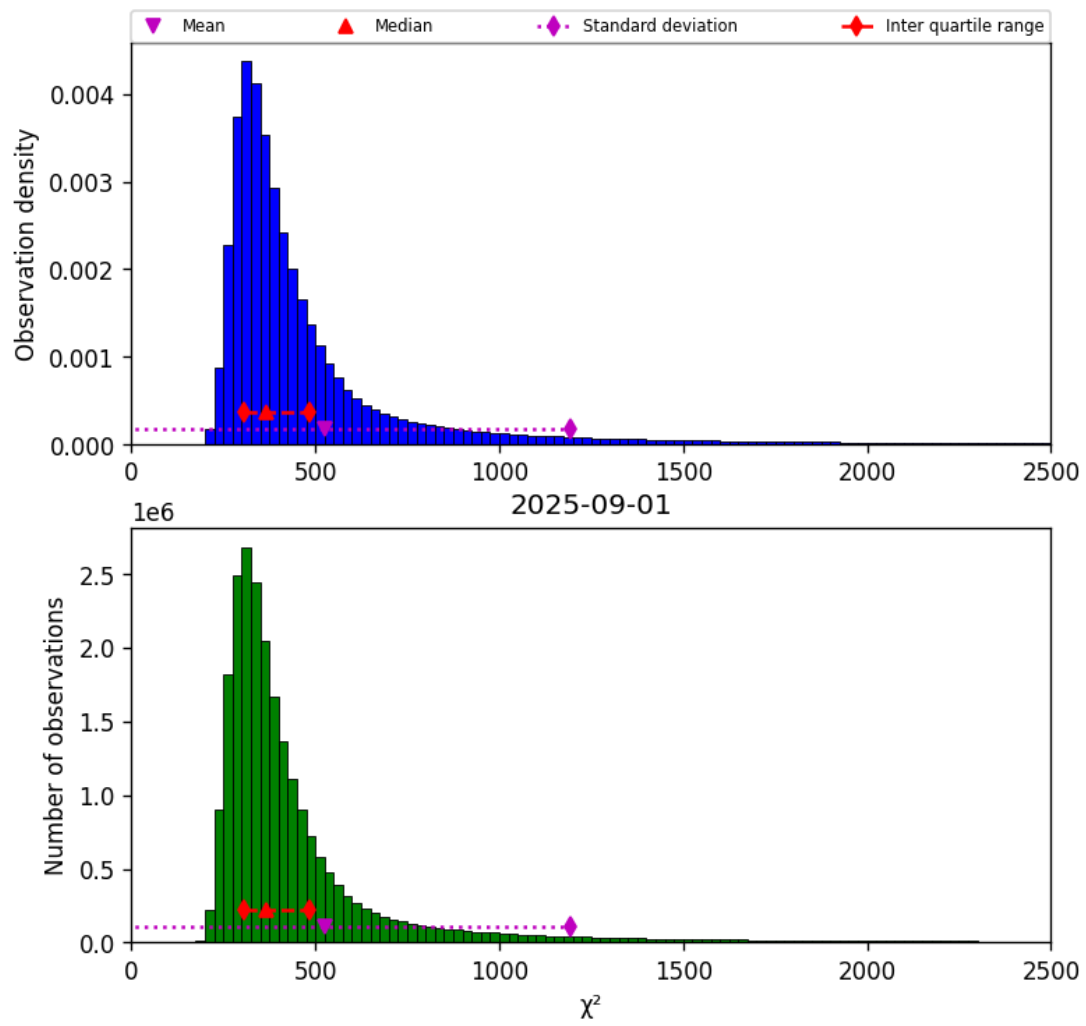
Figure 40: Histogram of “ \chi^2 ” for 2025-09-01 to 2025-09-02
