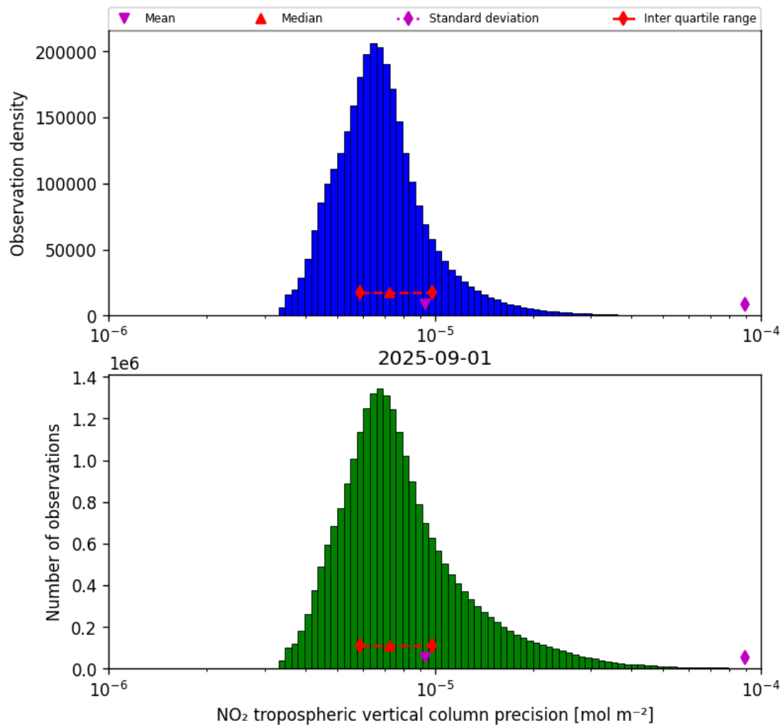
Figure 28: Histogram of “NO 2 tropospheric vertical column precision” for 2025-09-01 to 2025-09-02
