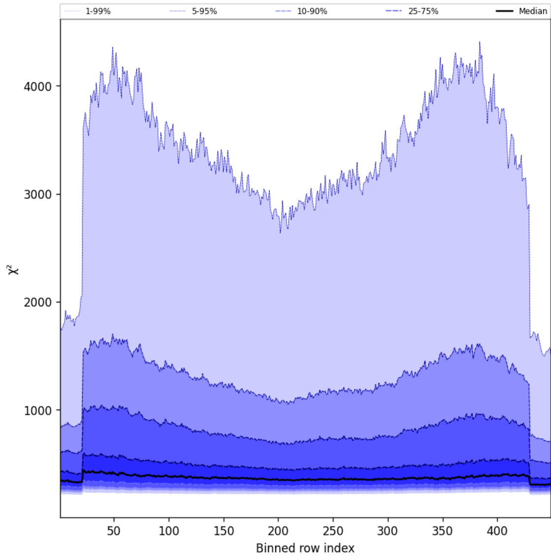
Figure 57: Along track statistics of “ \chi^2 ” for 2025-09-01 to 2025-09-02
