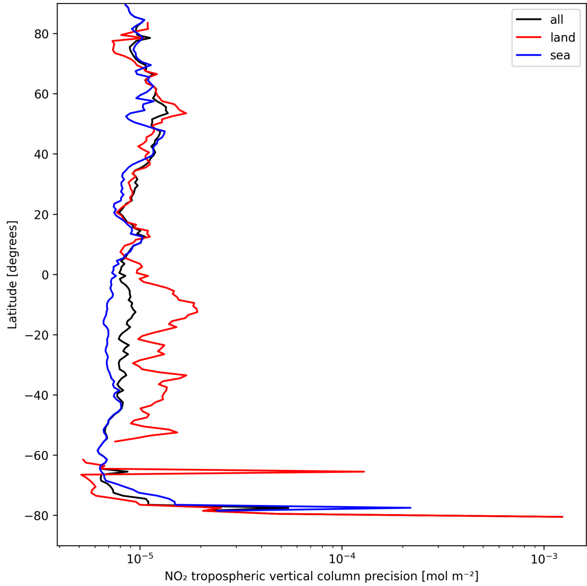
Figure 11: Zonal average of “NO 2 tropospheric vertical column precision” for 2025-09-01 to 2025-09-02.
