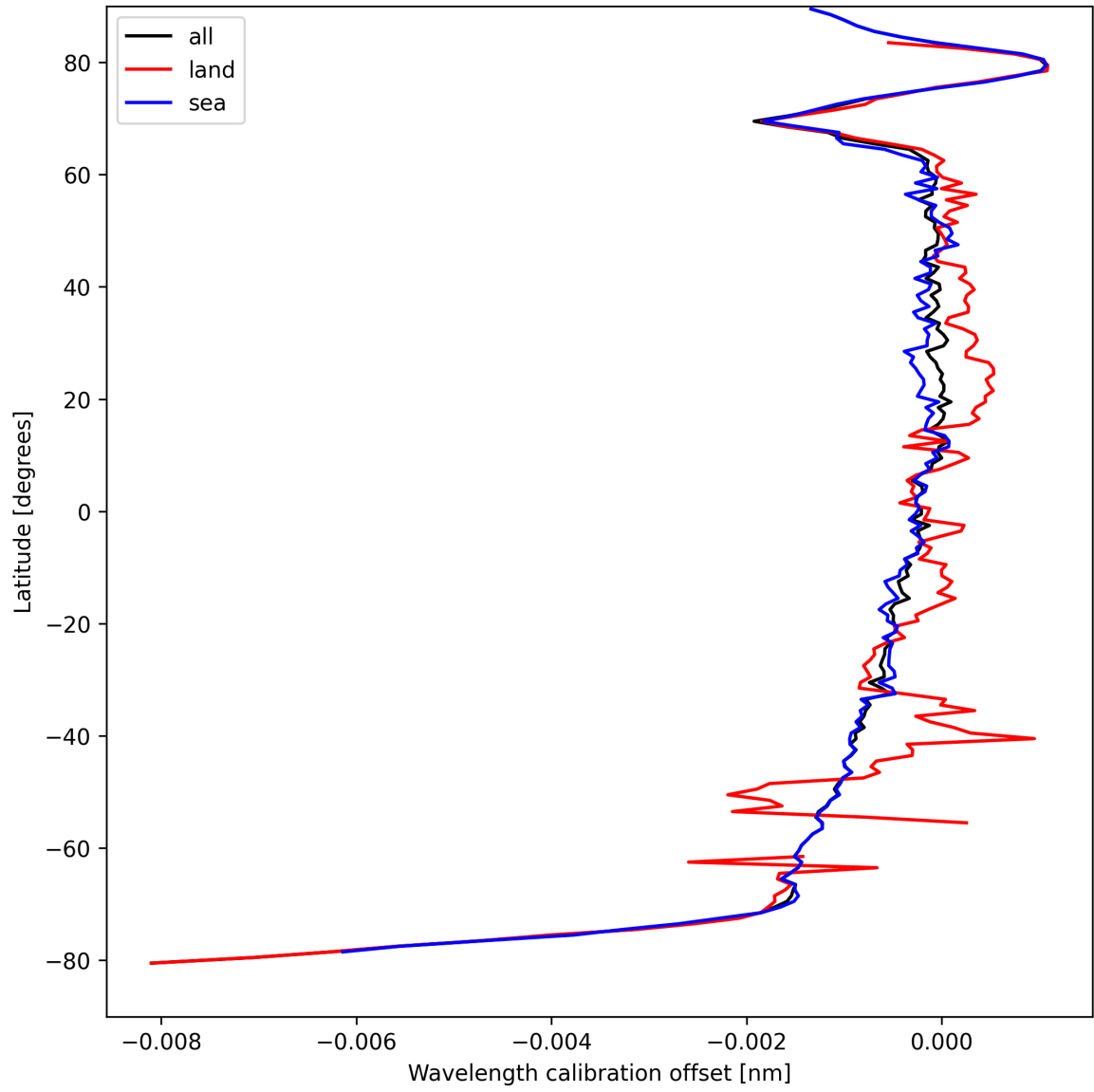
Figure 16: Zonal average of “Wavelength calibration offset” for 2025-09-01 to 2025-09-02.
