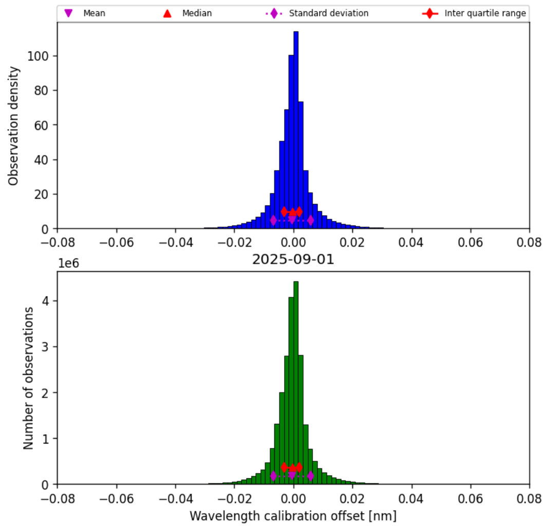
Figure 33: Histogram of “Wavelength calibration offset” for 2025-09-01 to 2025-09-02
