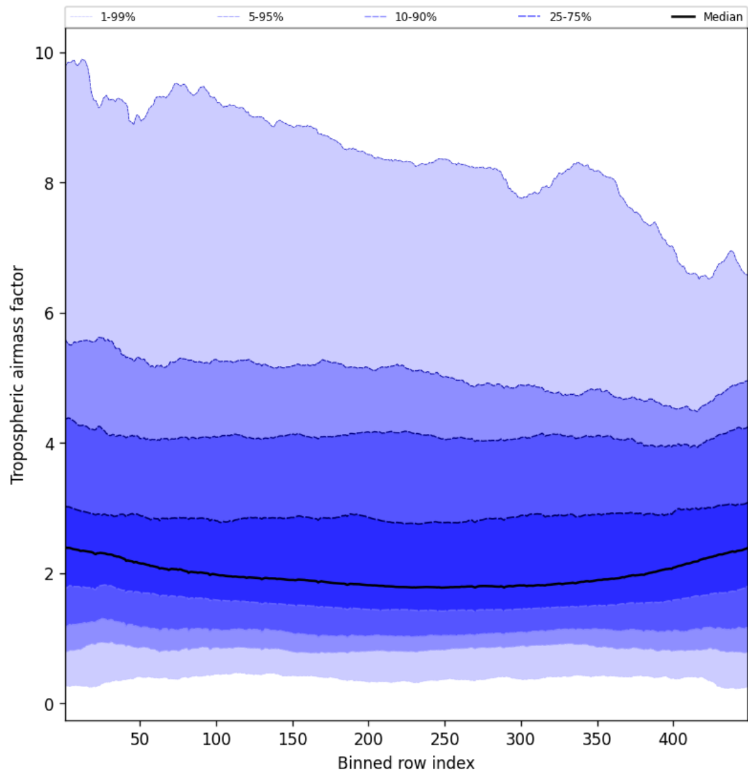
Figure 46: Along track statistics of “Tropospheric airmass factor” for 2025-09-01 to 2025-09-02
