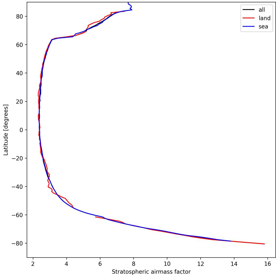
Figure 25: Zonal average of “Stratospheric air mass factor” for 2025-09-01 to 2025-09-02.
