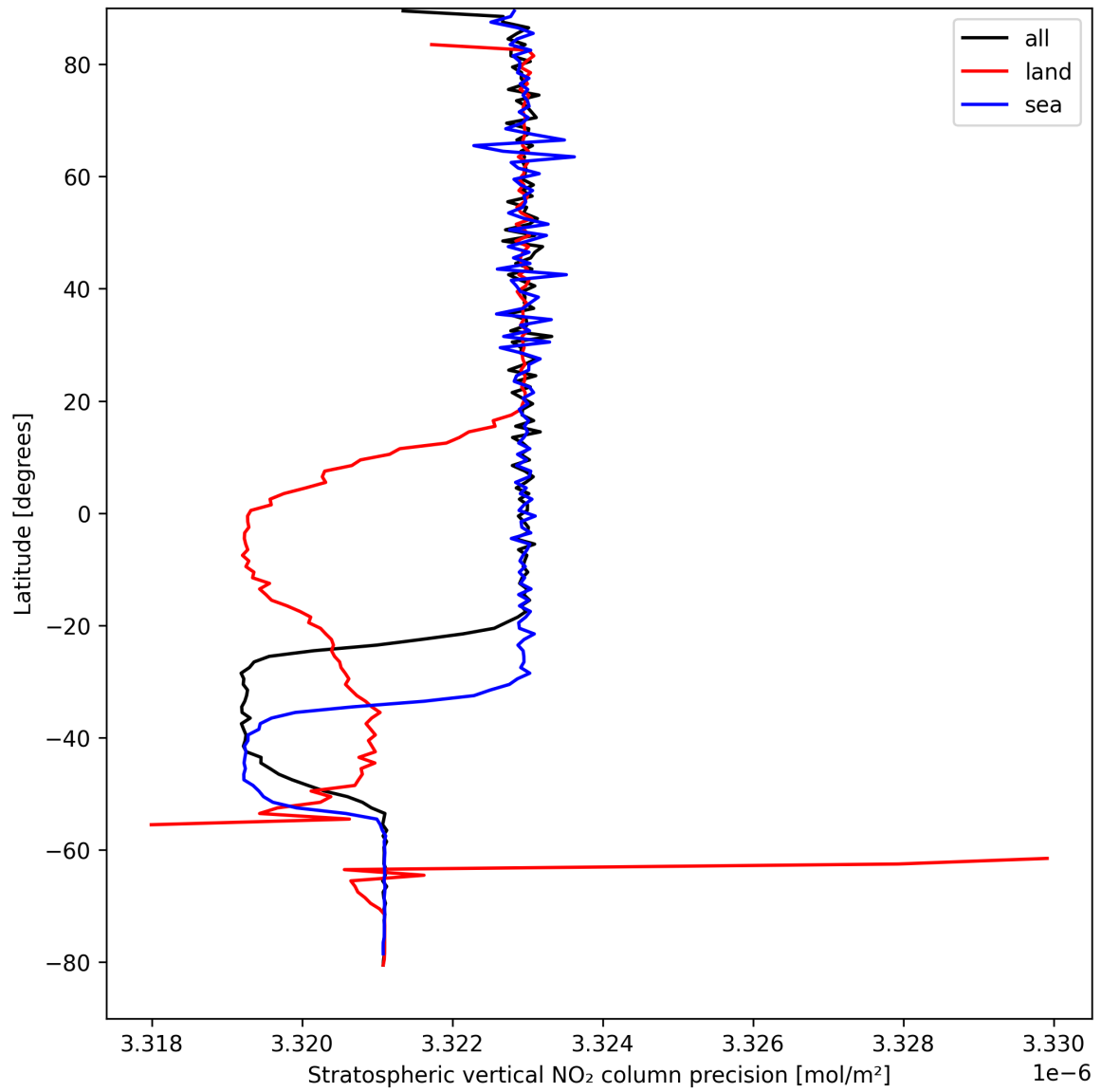
Figure 18: Zonal average of “Stratospheric vertical NO 2 column precision” for 2025-09-01 to 2025-09-02.
