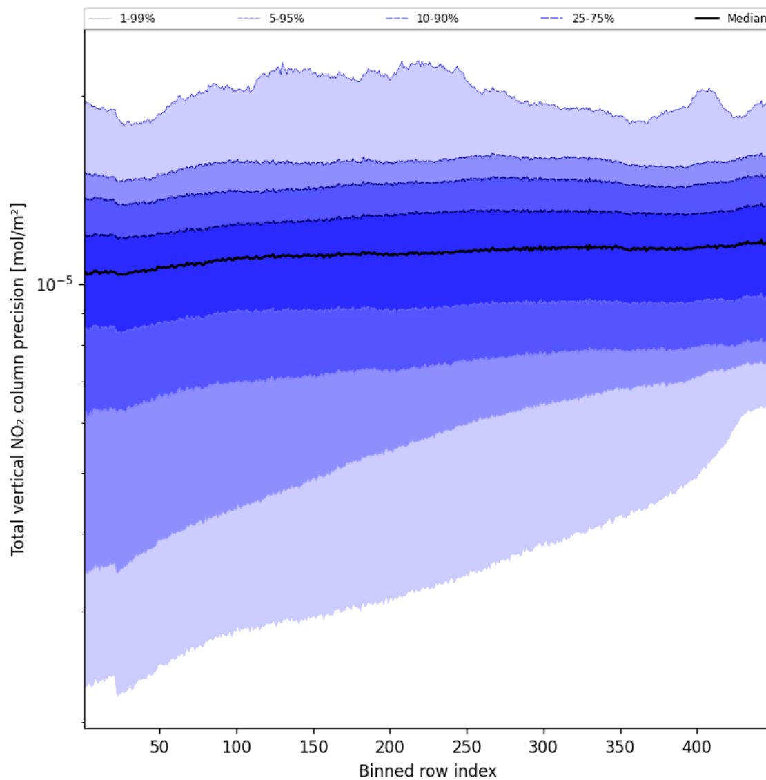
Figure 54: Along track statistics of “Total vertical NO 2 column precision” for 2025-09-01 to 2025-09-02
