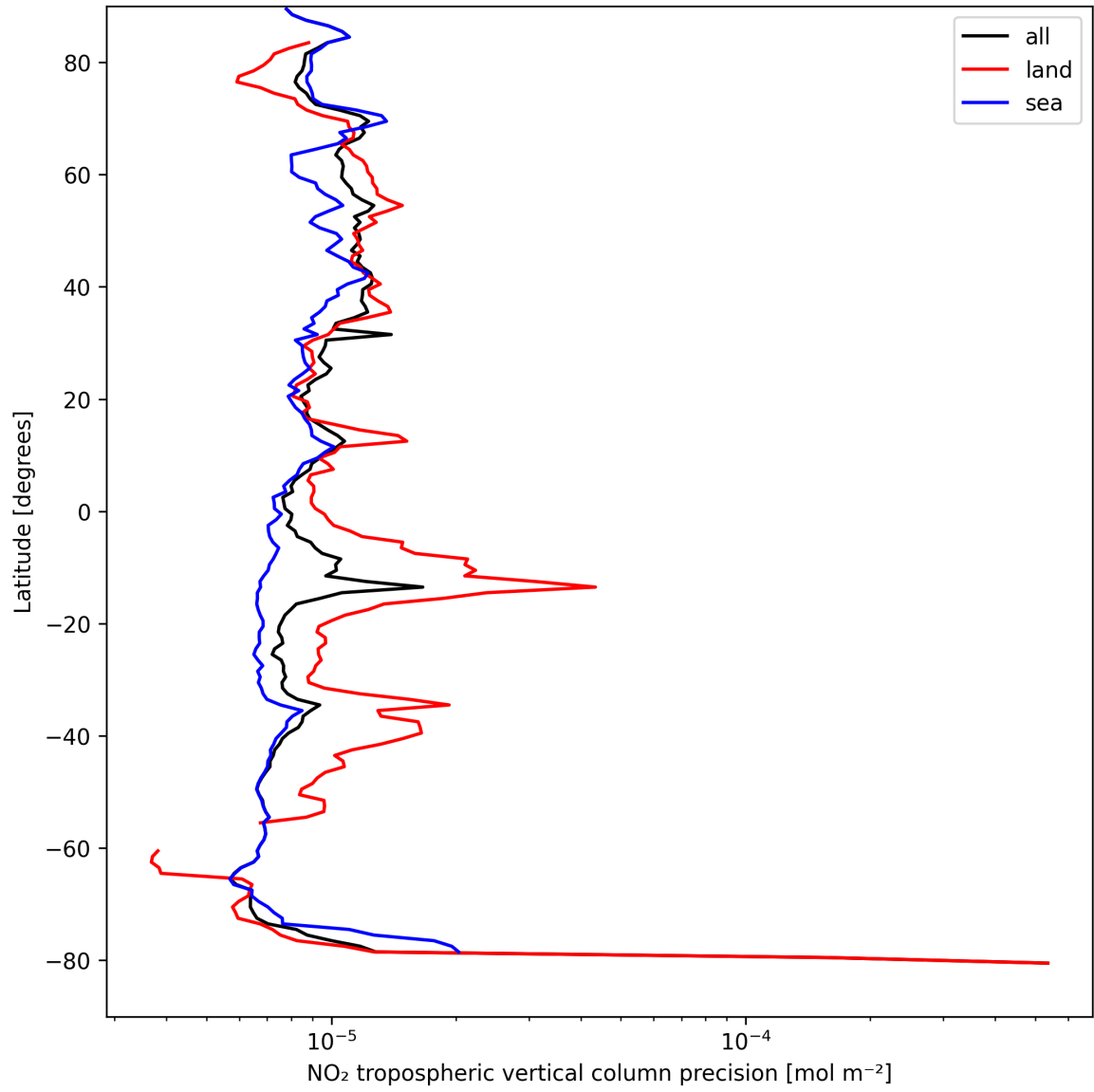
Figure 11: Zonal average of “NO 2 tropospheric vertical column precision” for 2025-09-02 to 2025-09-02.
