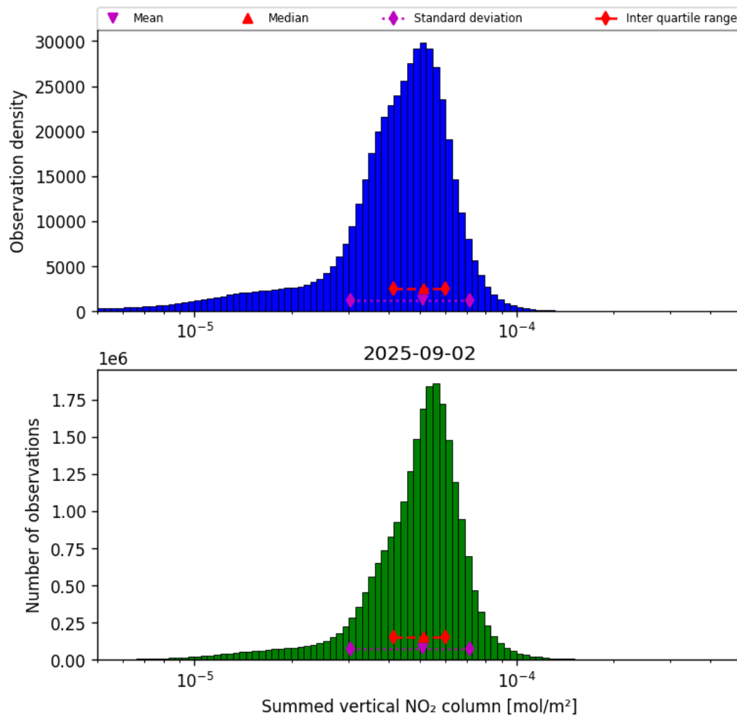
Figure 38: Histogram of "Summed vertical NO 2 column" for 2025-09-02 to 2025-09-02
