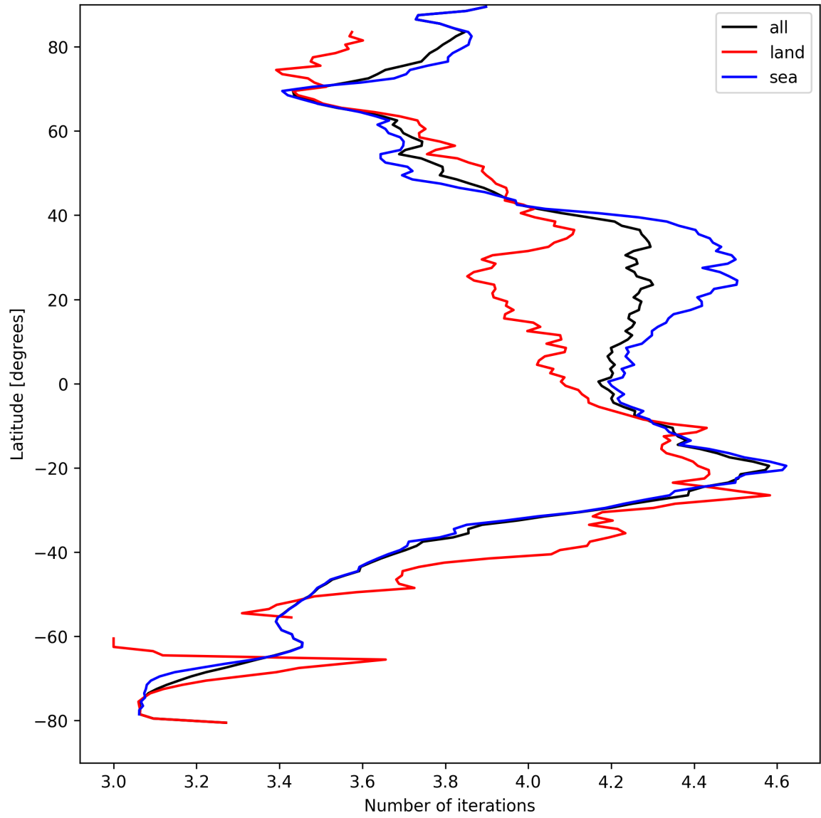
Figure 15: Zonal average of “Number of iterations” for 2025-09-02 to 2025-09-02.
