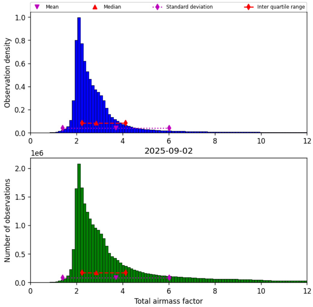
Figure 30: Histogram of “Total airmass factor” for 2025-09-02 to 2025-09-02
