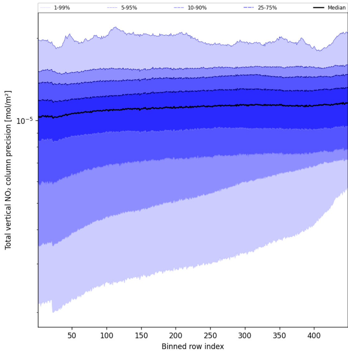
Figure 54: Along track statistics of “Total vertical NO 2 column precision” for 2025-09-02 to 2025-09-02
