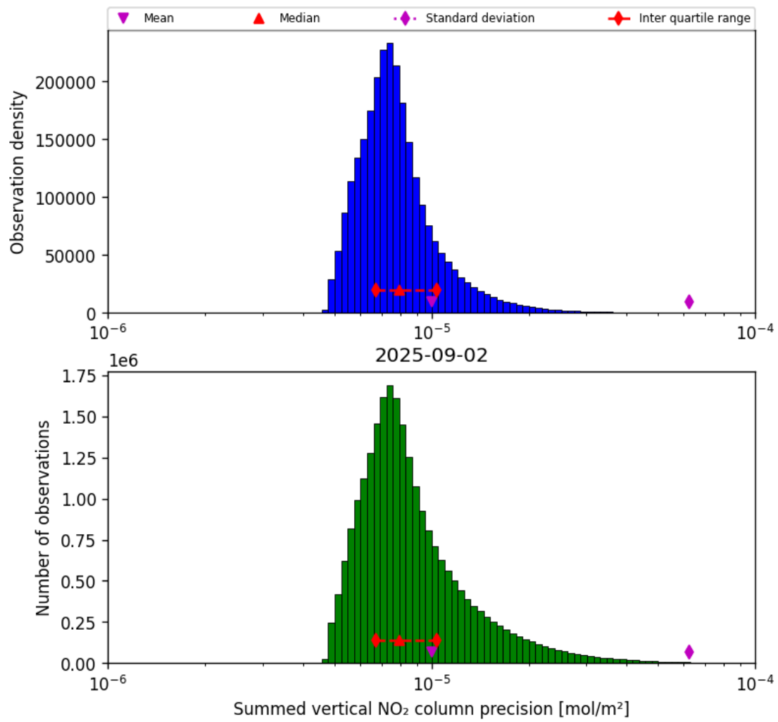
Figure 39: Histogram of "Summed vertical NO 2 column precision" for 2025-09-02 to 2025-09-02
