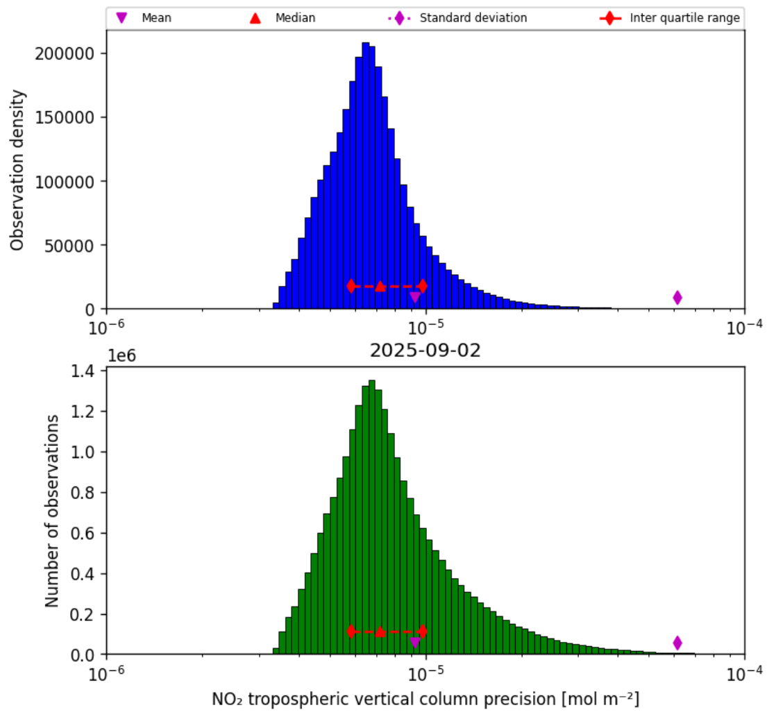
Figure 28: Histogram of “NO 2 tropospheric vertical column precision” for 2025-09-02 to 2025-09-02
