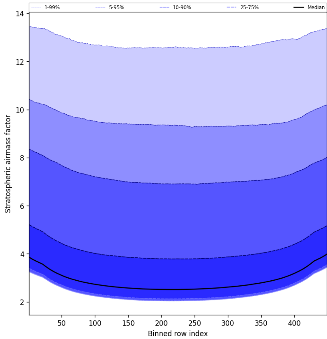
Figure 59: Along track statistics of “Stratospheric airmass factor” for 2025-09-02 to 2025-09-02
