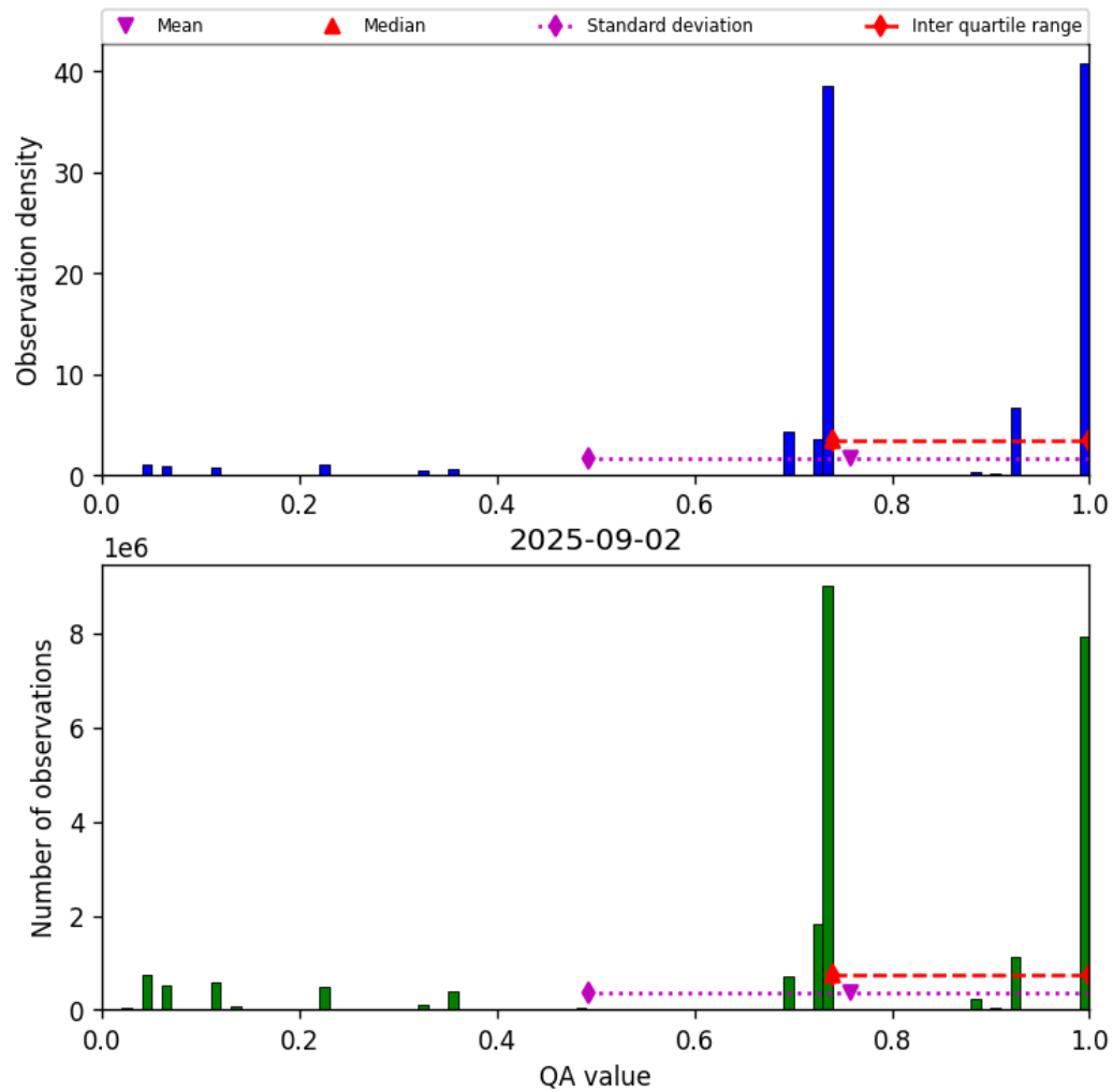
Figure 26: Histogram of “QA value” for 2025-09-02 to 2025-09-02
