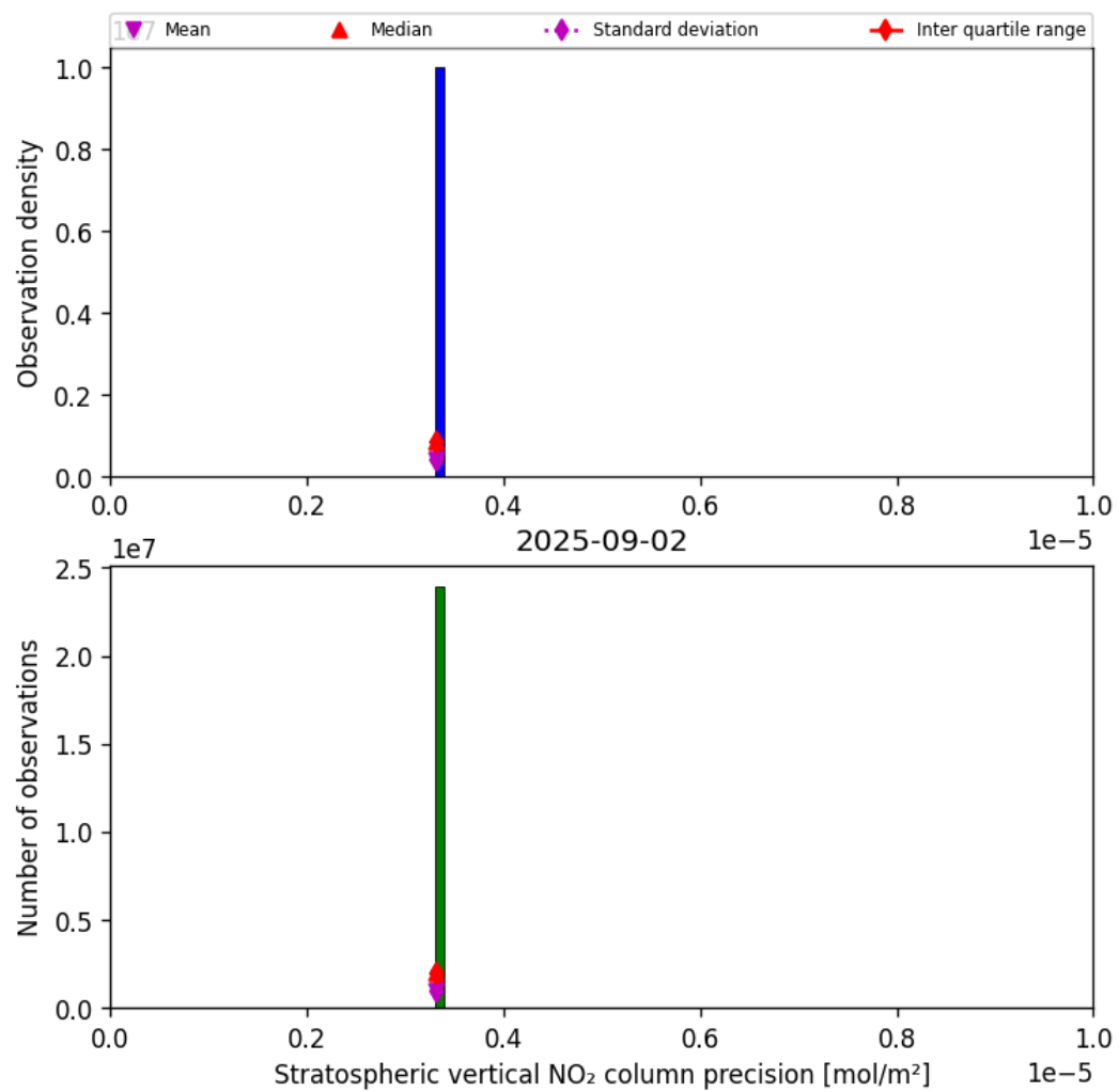
Figure 35: Histogram of “Stratospheric vertical NO 2 column precision” for 2025-09-02 to 2025-09-02
