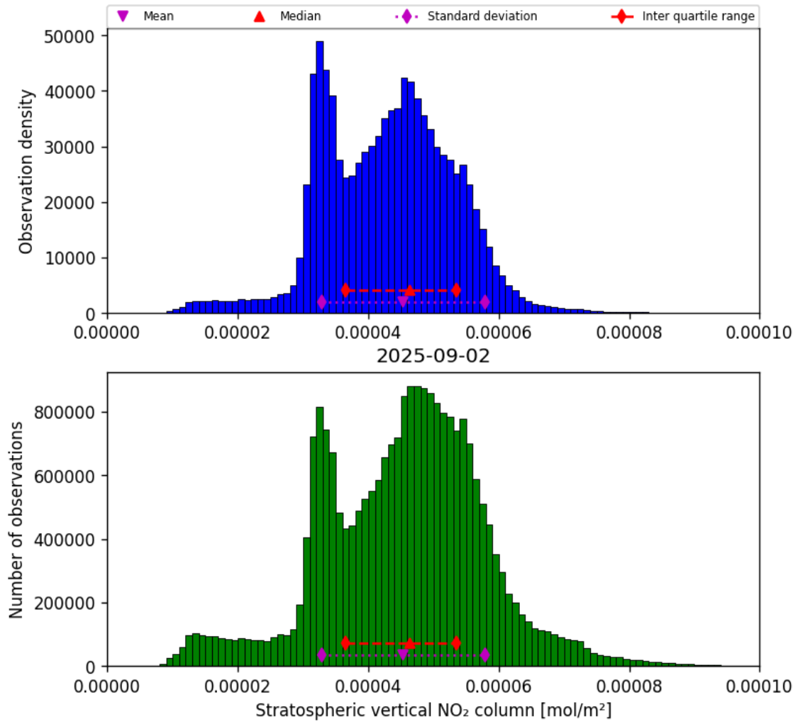
Figure 34: Histogram of “Stratospheric vertical NO 2 column” for 2025-09-02 to 2025-09-02
