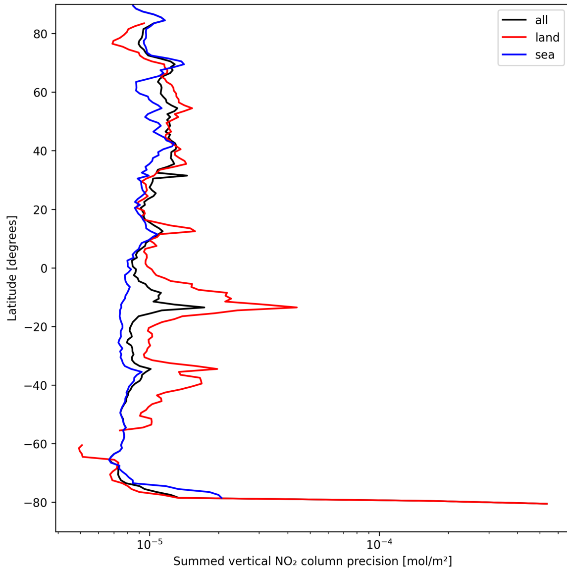
Figure 22: Zonal average of “Summed vertical NO 2 column precision” for 2025-09-02 to 2025-09-02.
