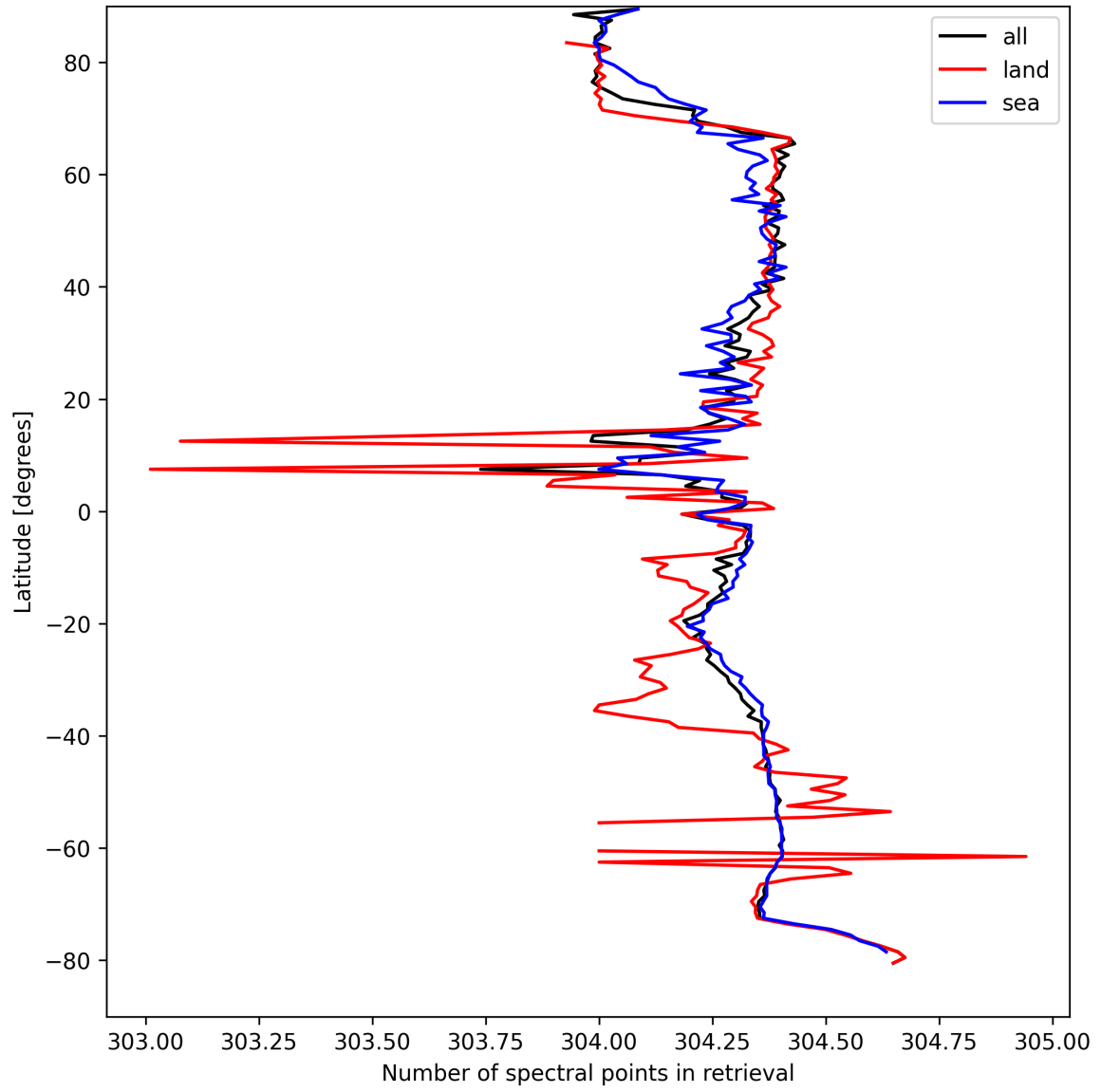
Figure 14: Zonal average of “Number of spectral points in retrieval” for 2025-09-02 to 2025-09-02.
