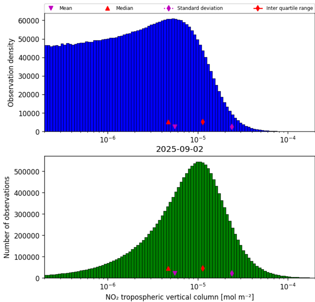
Figure 27: Histogram of “NO 2 tropospheric vertical column” for 2025-09-02 to 2025-09-02
