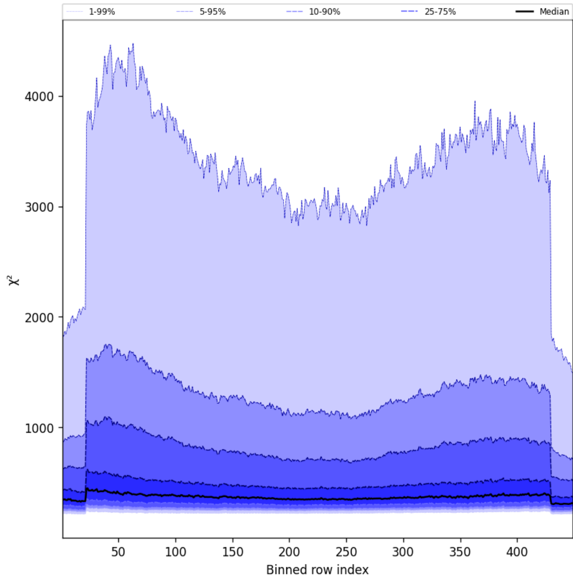
Figure 57: Along track statistics of “ \chi^2 ” for 2025-09-02 to 2025-09-02
