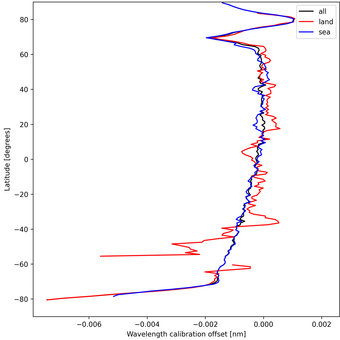
Figure 16: Zonal average of “Wavelength calibration offset” for 2025-09-02 to 2025-09-02.
