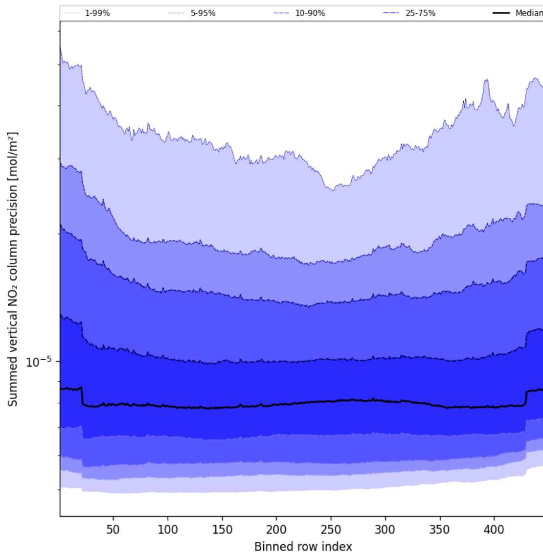
Figure 56: Along track statistics of “Summed vertical NO 2 column precision” for 2025-09-02 to 2025-09-02
