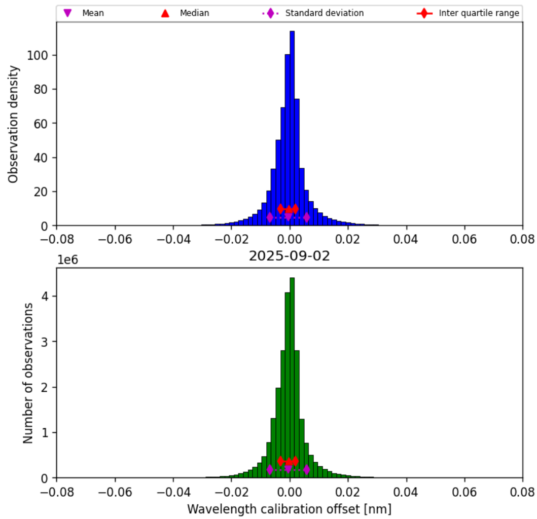
Figure 33: Histogram of “Wavelength calibration offset” for 2025-09-02 to 2025-09-02
