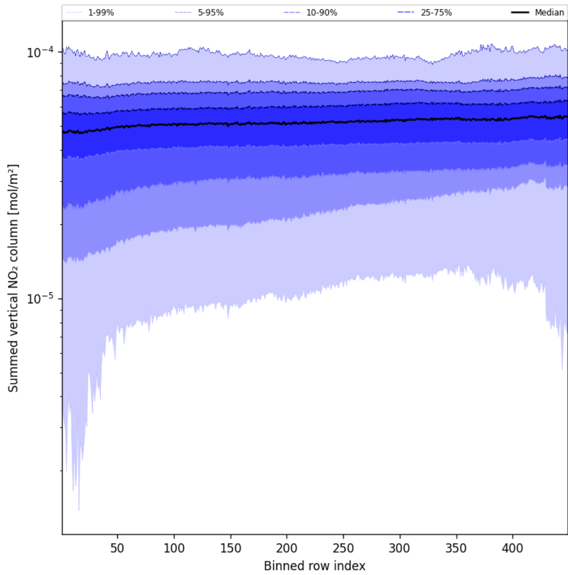
Figure 55: Along track statistics of “Summed vertical NO 2 column” for 2025-09-02 to 2025-09-02
