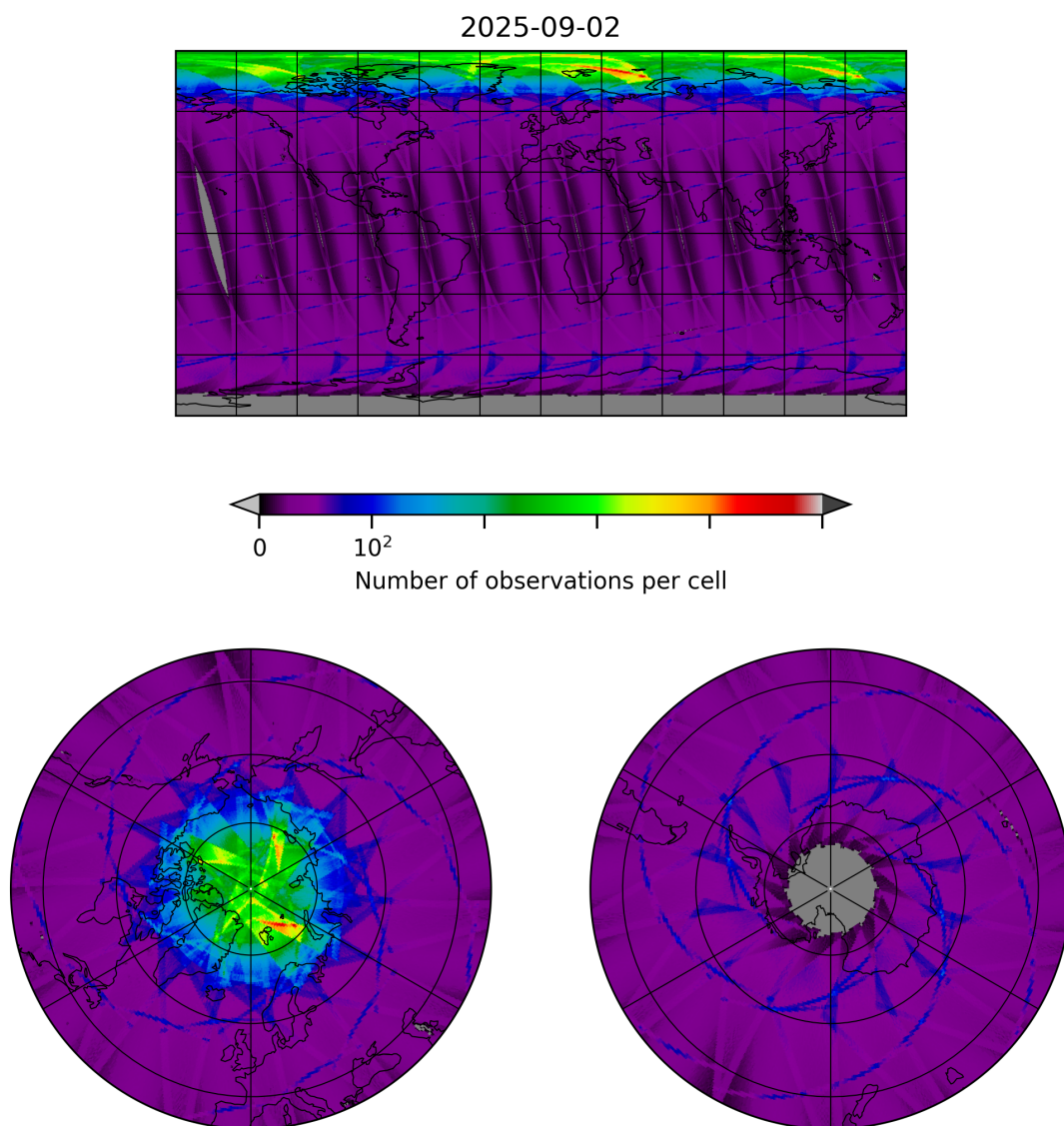
Figure 8: Map of the number of observations for 2025-09-02 to 2025-09-02
