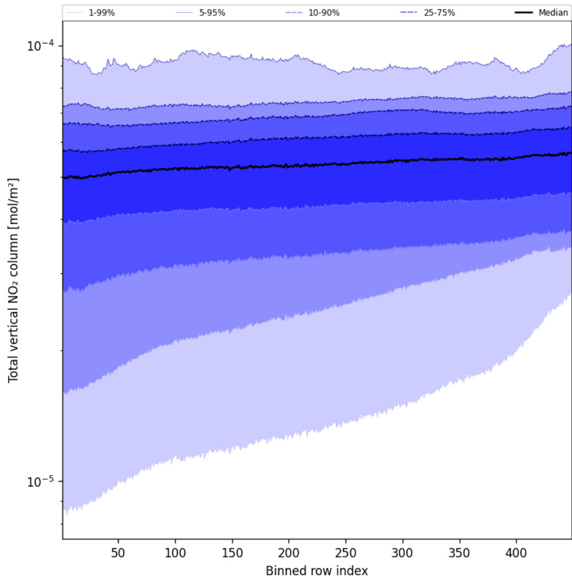
Figure 53: Along track statistics of “Total vertical NO 2 column” for 2025-09-02 to 2025-09-02
