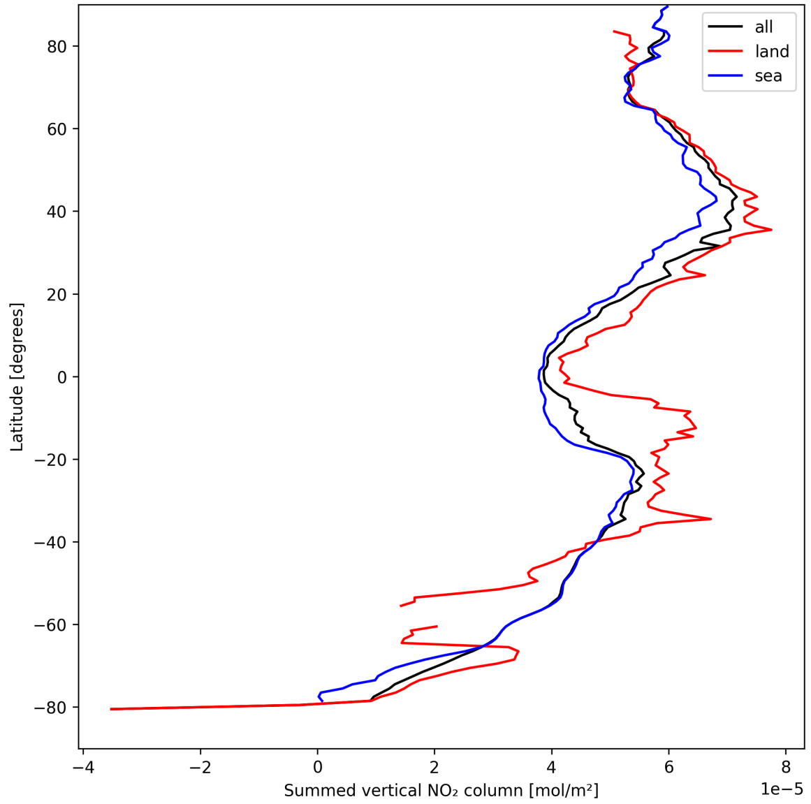
Figure 21: Zonal average of “Summed vertical NO 2 column” for 2025-09-02 to 2025-09-02.
