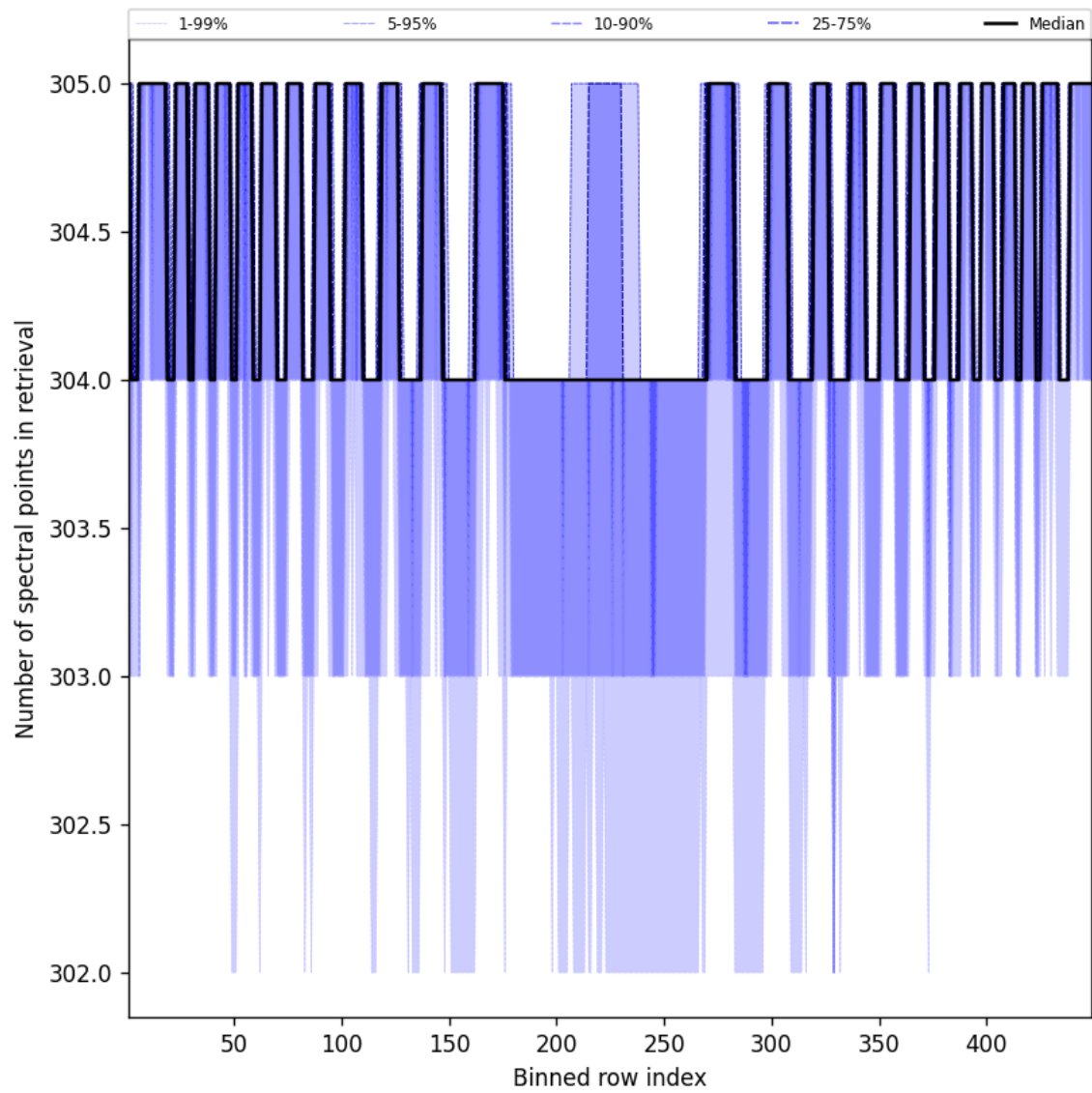
Figure 48: Along track statistics of “Number of spectral points in retrieval” for 2025-09-02 to 2025-09-02
