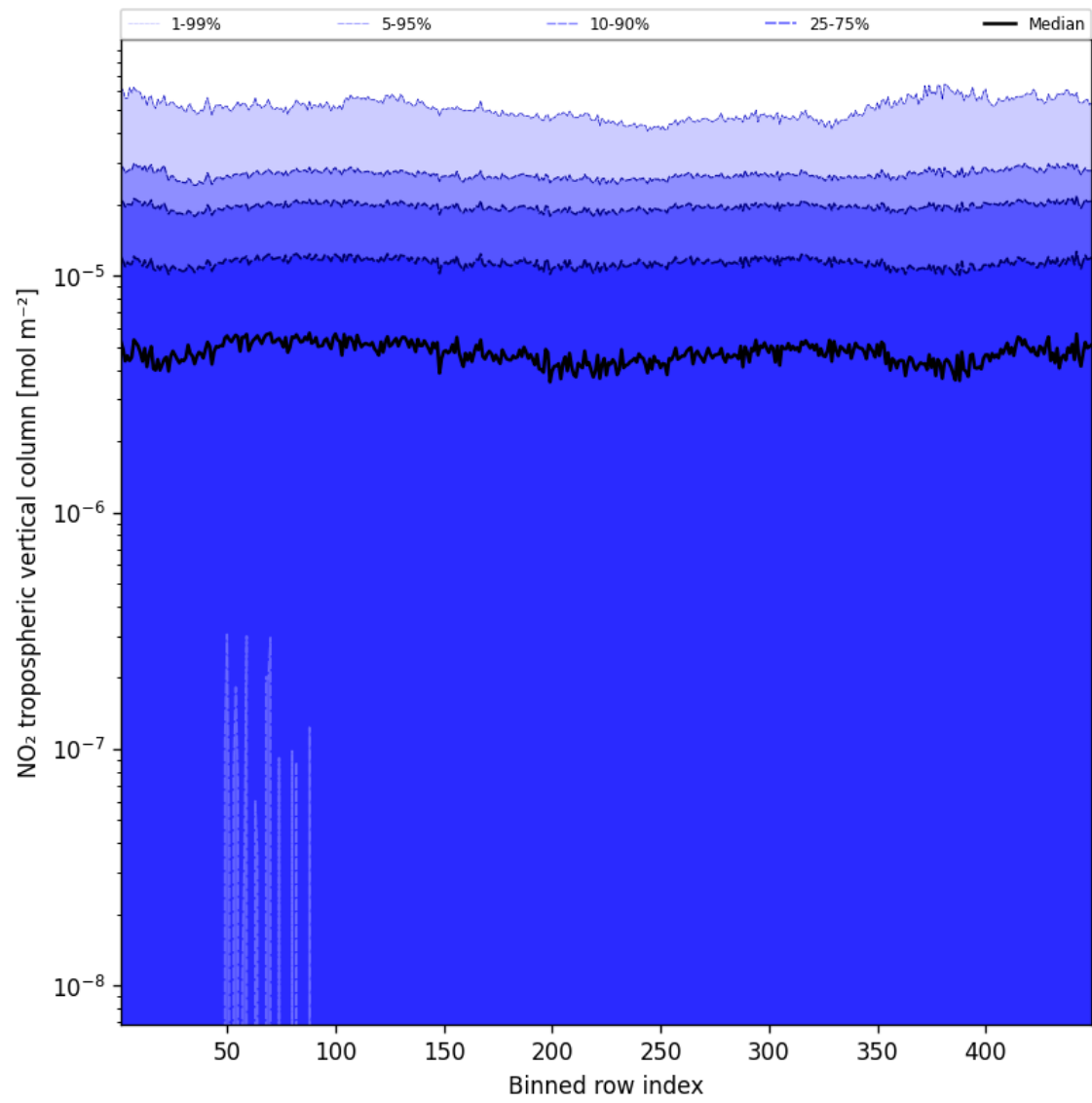
Figure 44: Along track statistics of “NO 2 tropospheric vertical column” for 2025-09-02 to 2025-09-02
