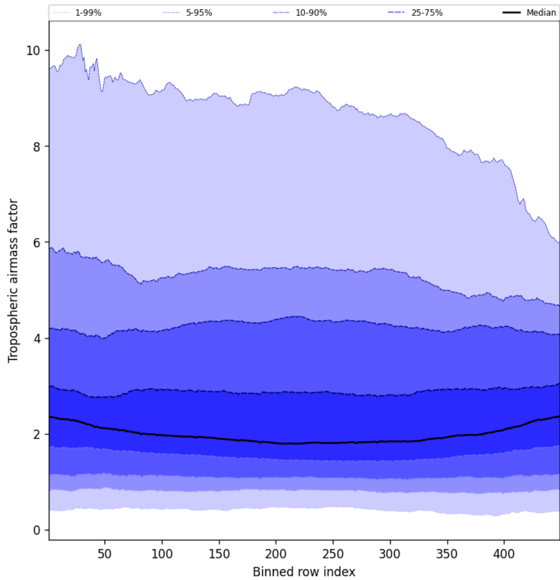
Figure 46: Along track statistics of “Tropospheric air mass factor” for 2025-09-02 to 2025-09-02
