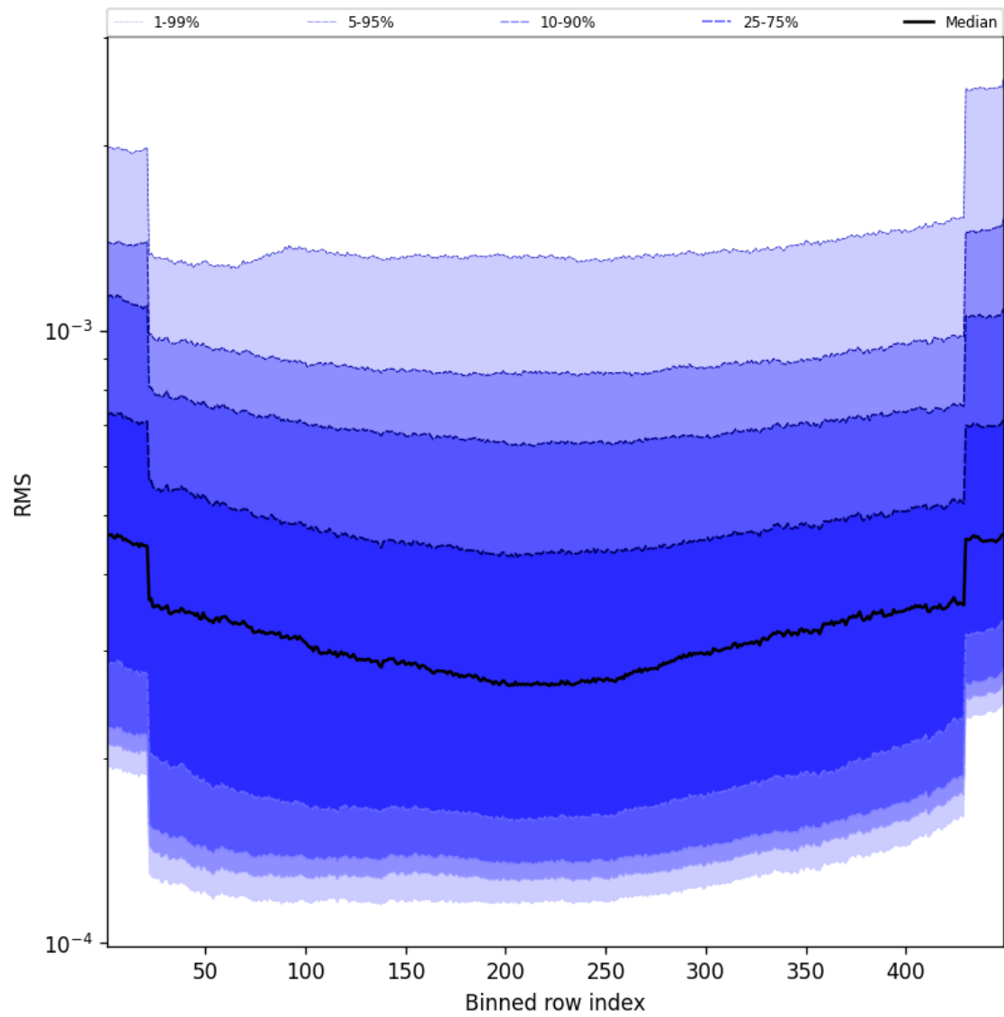
Figure 58: Along track statistics of “RMS” for 2025-09-02 to 2025-09-02
