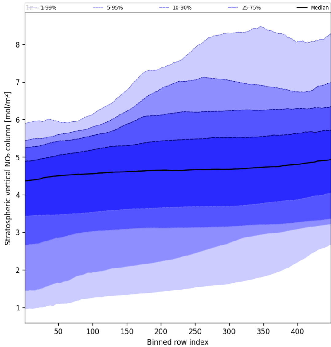
Figure 51: Along track statistics of “Stratospheric vertical NO 2 column” for 2025-09-02 to 2025-09-02
