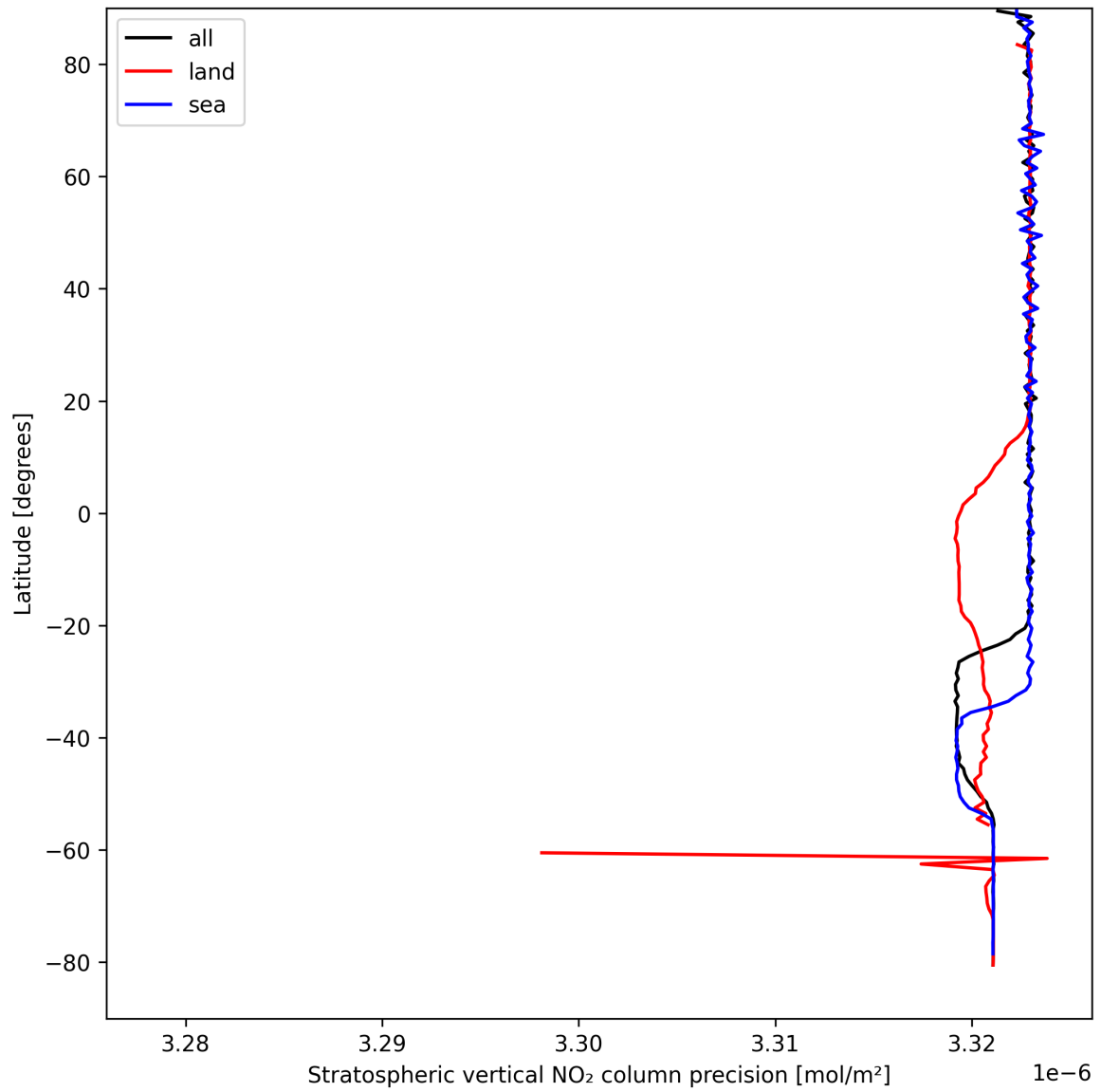
Figure 18: Zonal average of “Stratospheric vertical NO 2 column precision” for 2025-09-02 to 2025-09-02.
