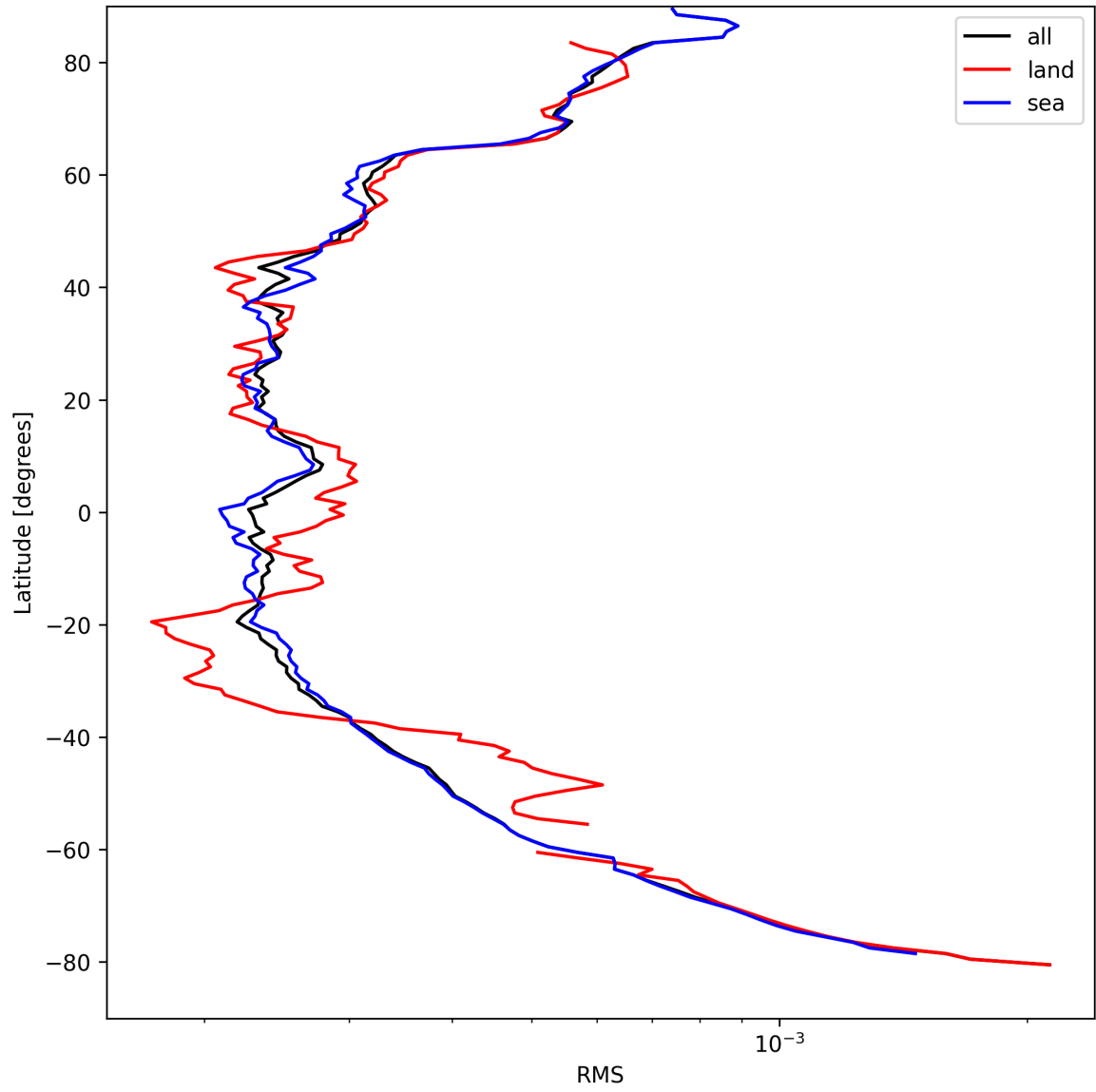
Figure 24: Zonal average of “RMS” for 2025-09-02 to 2025-09-02.
