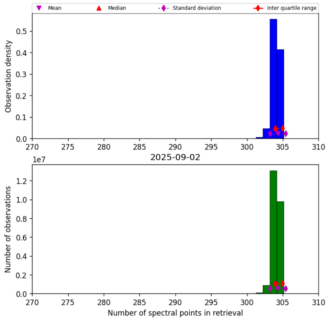
Figure 31: Histogram of “Number of spectral points in retrieval” for 2025-09-02 to 2025-09-02
