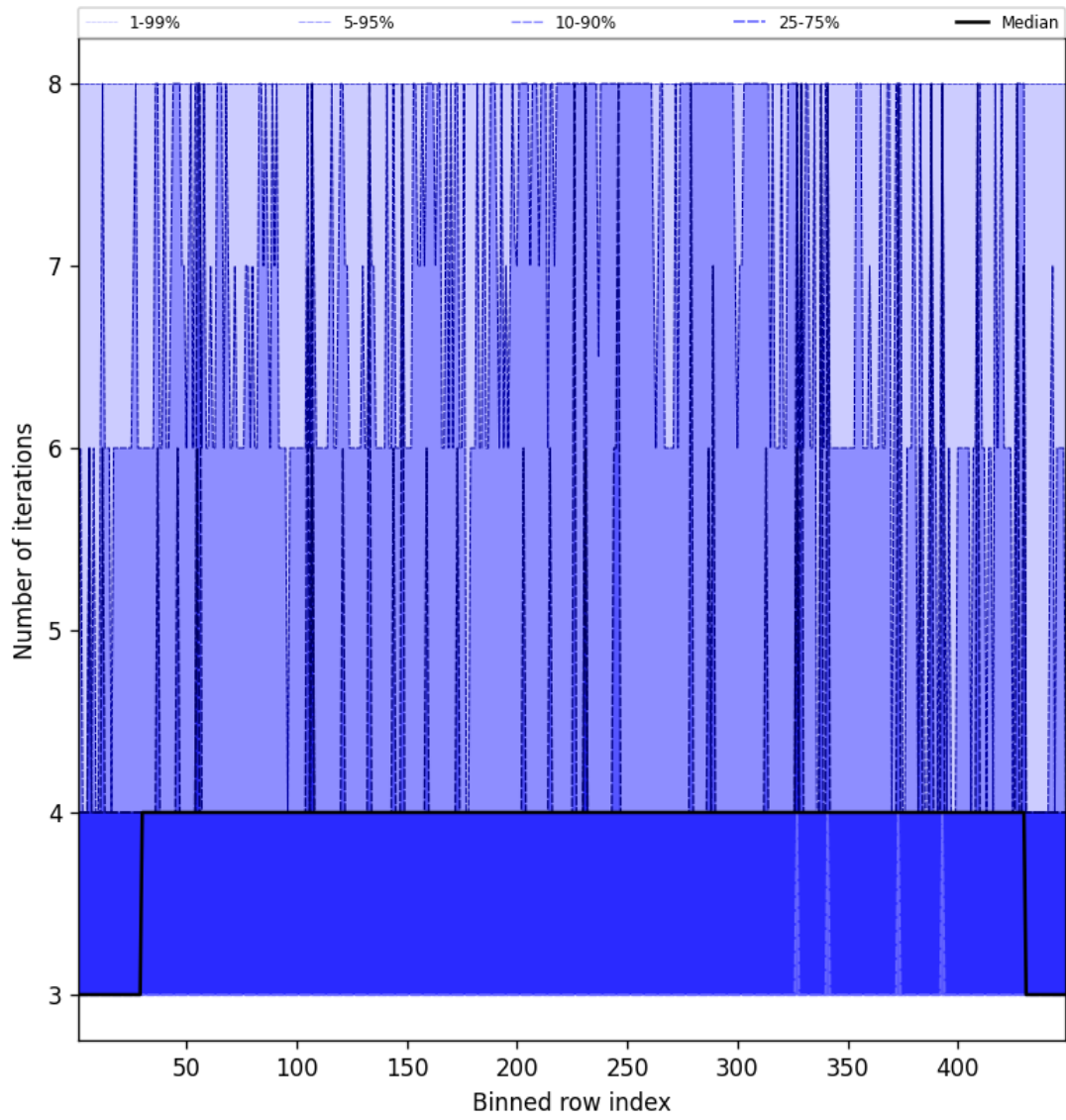
Figure 49: Along track statistics of “Number of iterations” for 2025-09-02 to 2025-09-02
