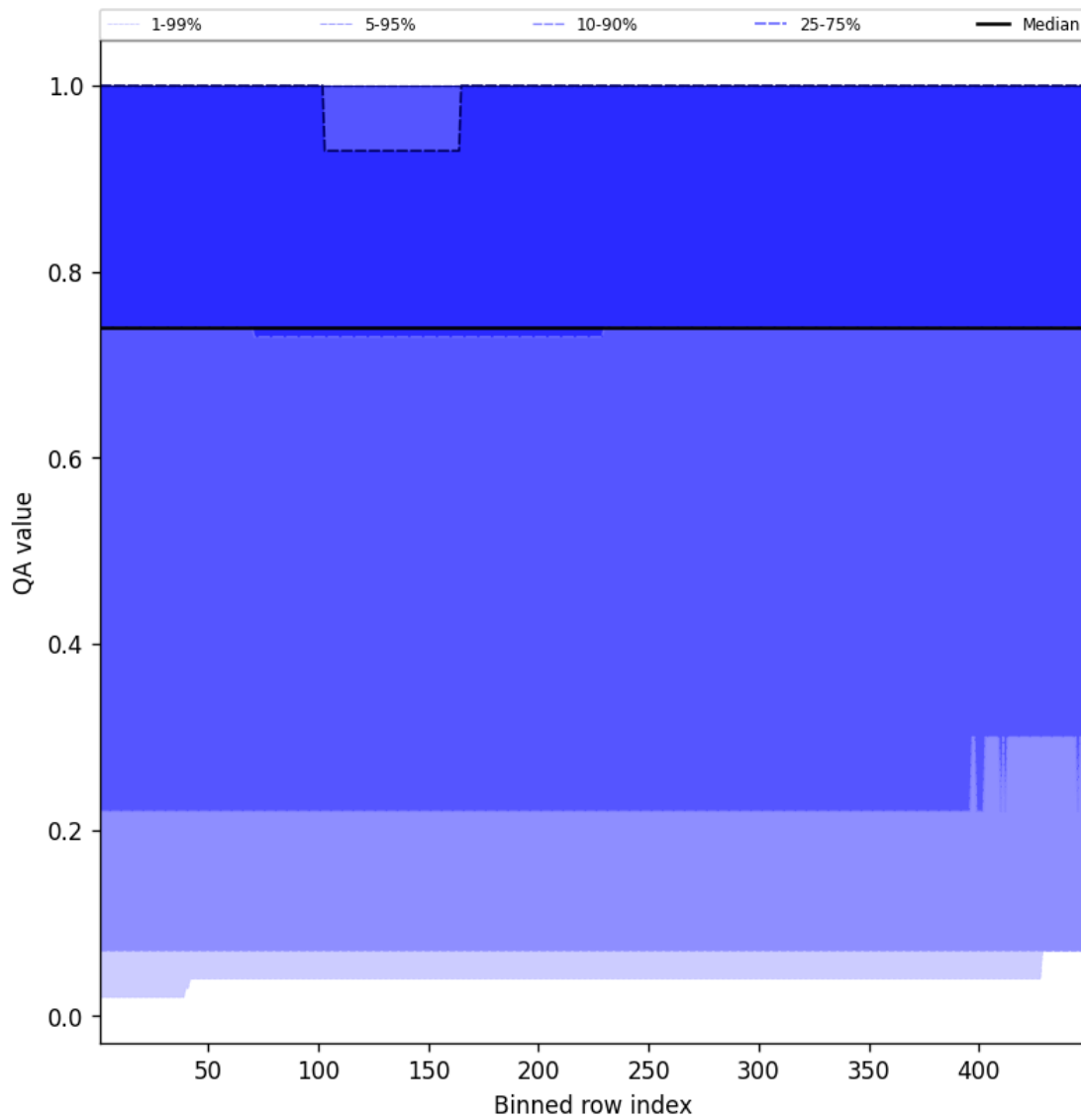
Figure 43: Along track statistics of "QA value" for 2025-09-02 to 2025-09-02
