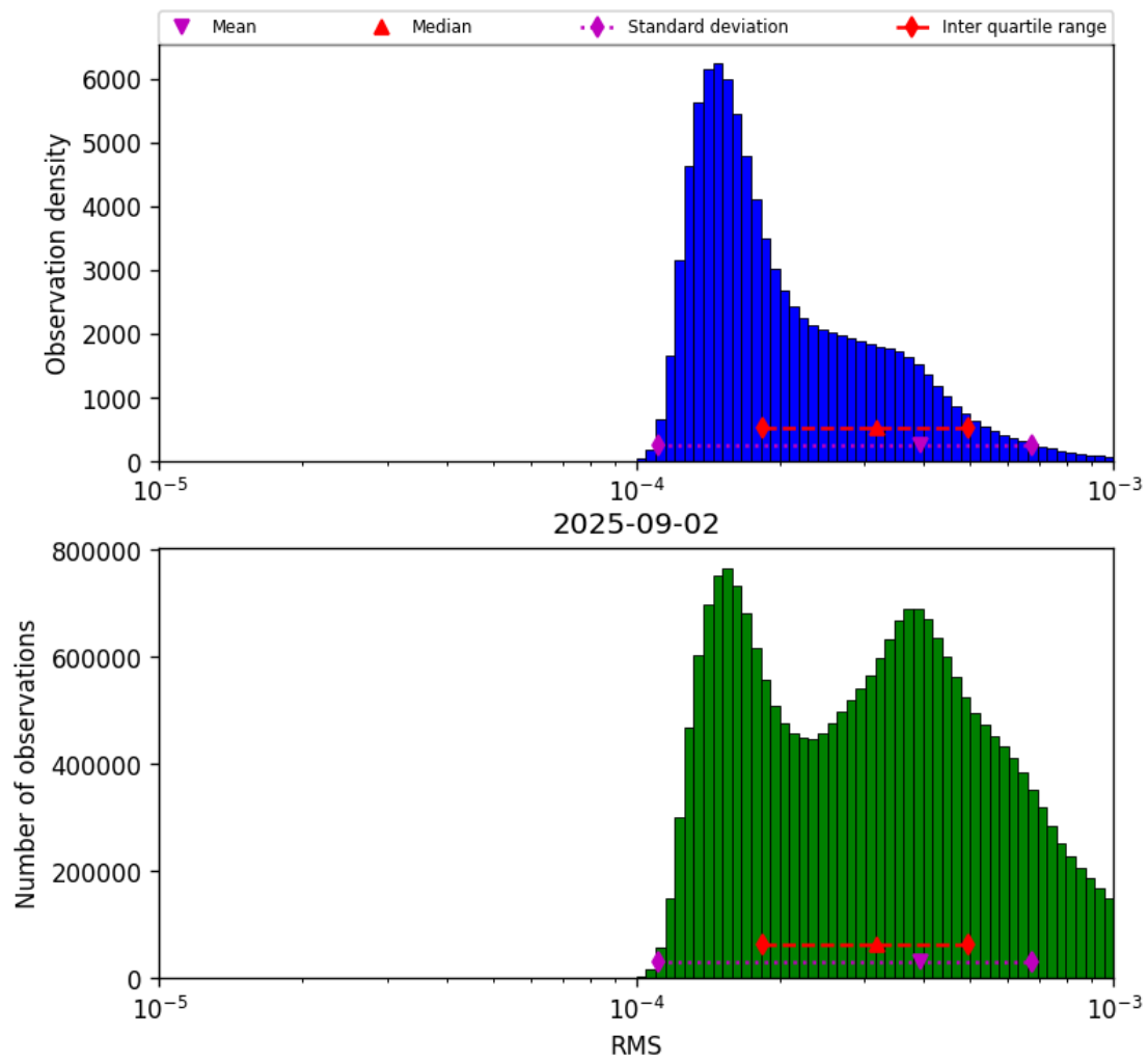
Figure 41: Histogram of “RMS” for 2025-09-02 to 2025-09-02
