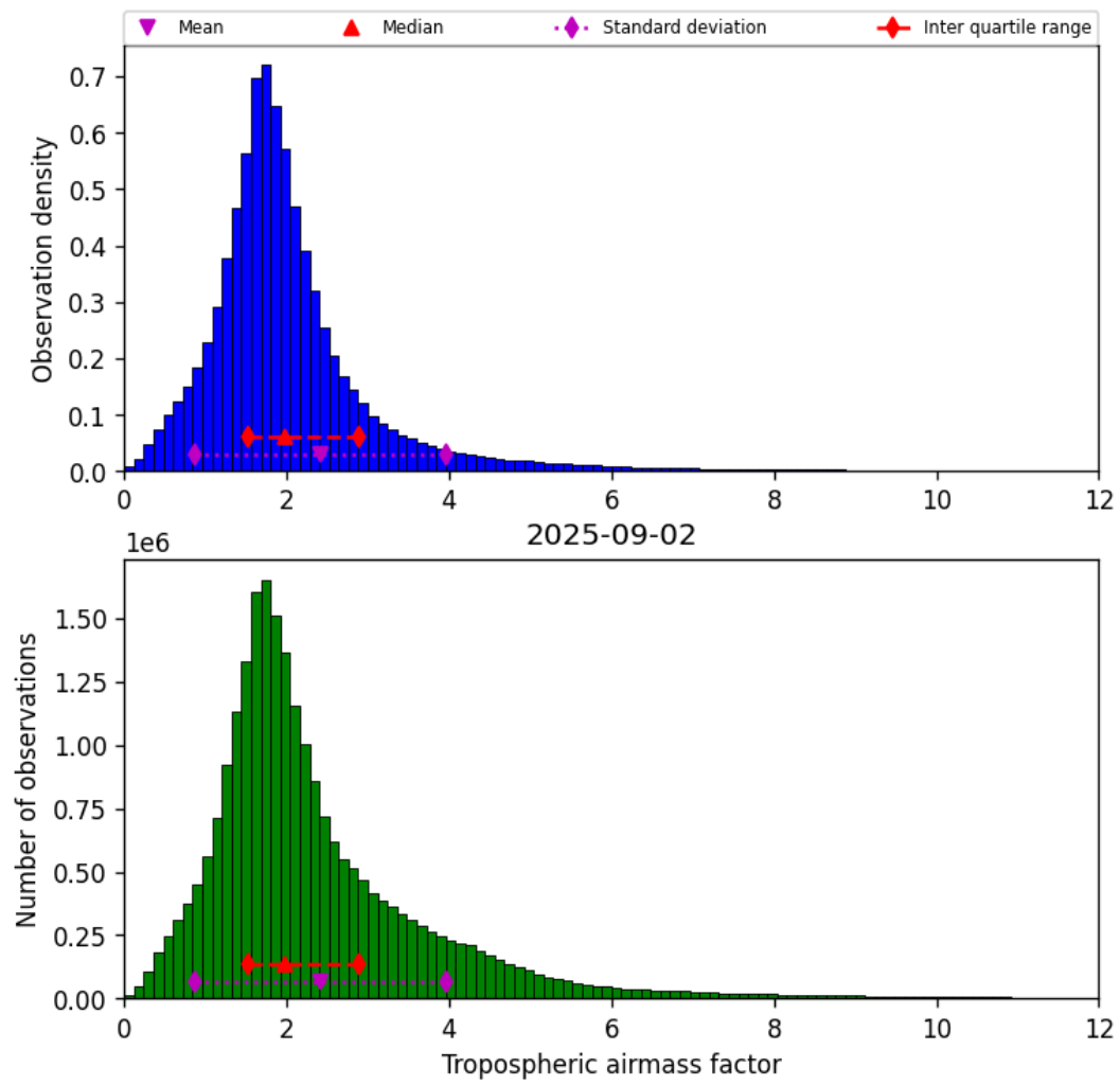
Figure 29: Histogram of “Tropospheric airmass factor” for 2025-09-02 to 2025-09-02
