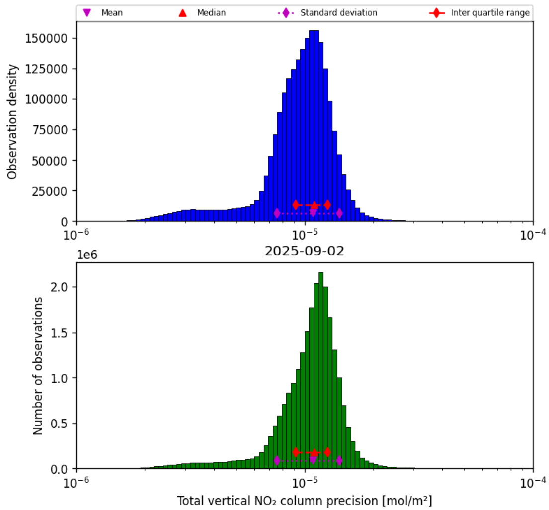
Figure 37: Histogram of "Total vertical NO 2 column precision" for 2025-09-02 to 2025-09-02
