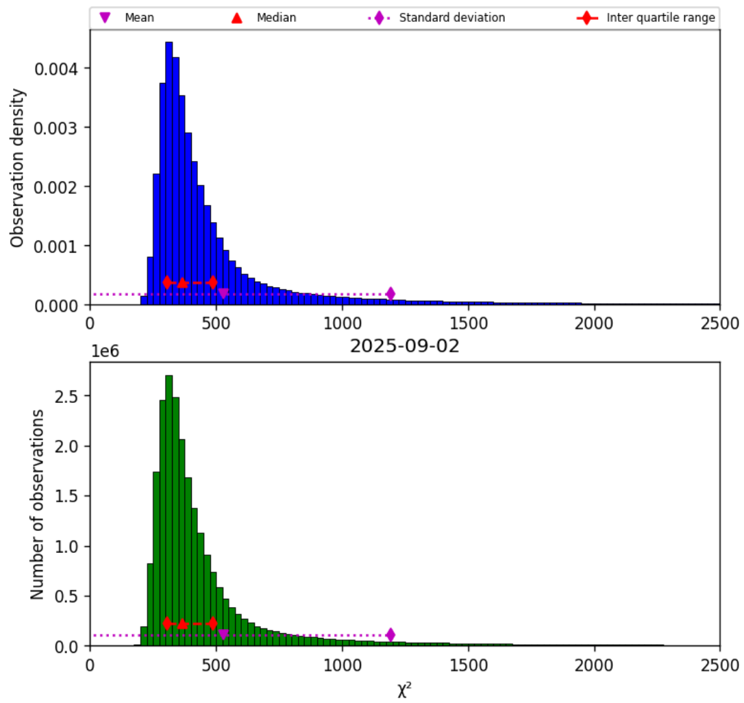
Figure 40: Histogram of “ \chi^2 ” for 2025-09-02 to 2025-09-02
