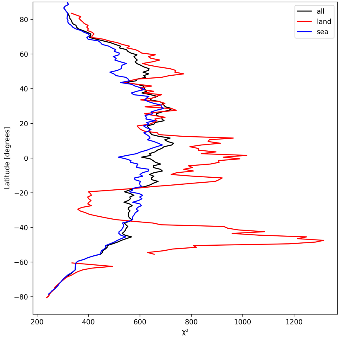
Figure 23: Zonal average of “ \chi^2 ” for 2025-09-02 to 2025-09-02.
