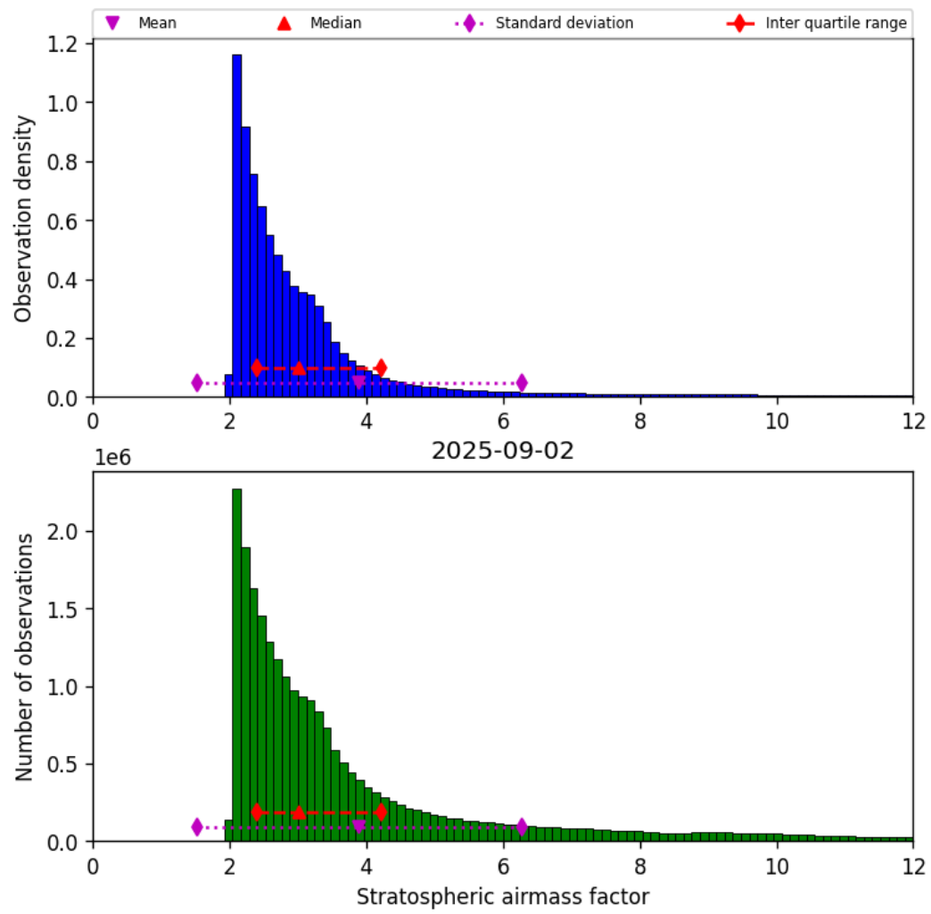
Figure 42: Histogram of “Stratospheric airmass factor” for 2025-09-02 to 2025-09-02
