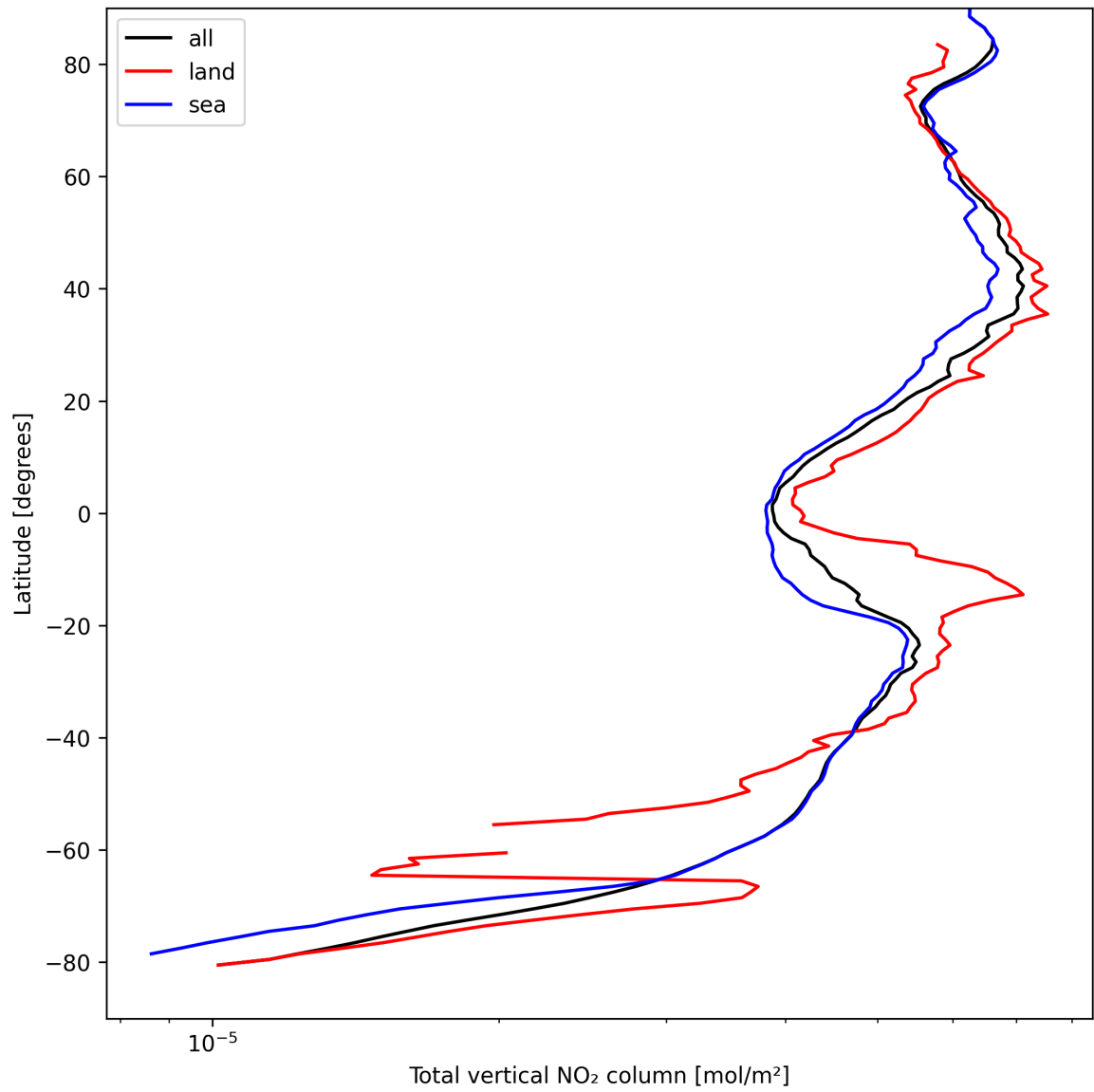
Figure 19: Zonal average of “Total vertical NO 2 column” for 2025-09-02 to 2025-09-02.
