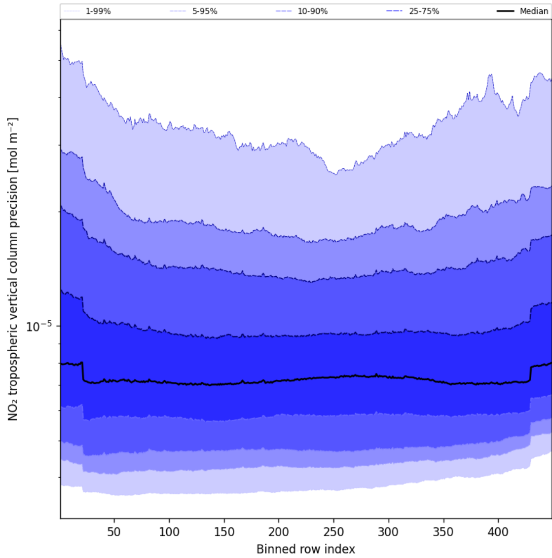
Figure 45: Along track statistics of “NO 2 tropospheric vertical column precision” for 2025-09-02 to 2025-09-02
