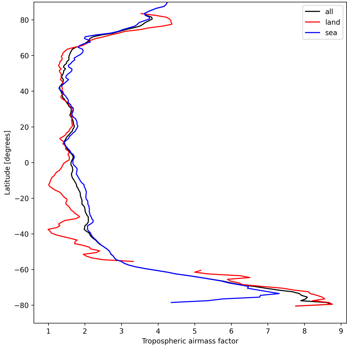
Figure 12: Zonal average of “Tropospheric air mass factor” for 2025-09-02 to 2025-09-02.
