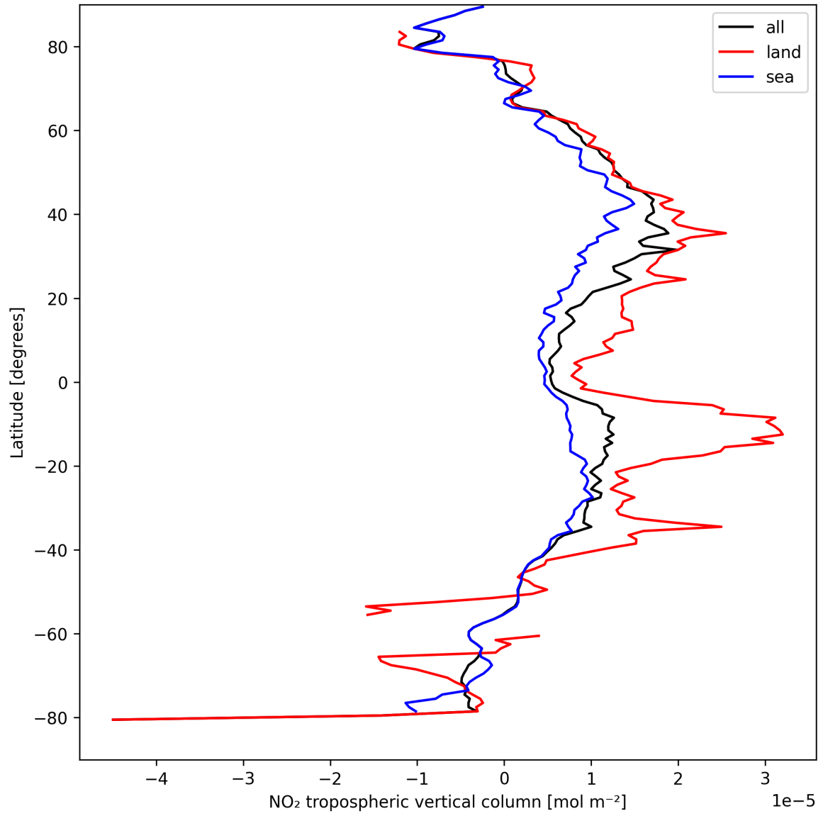
Figure 10: Zonal average of “NO 2 tropospheric vertical column” for 2025-09-02 to 2025-09-02.
