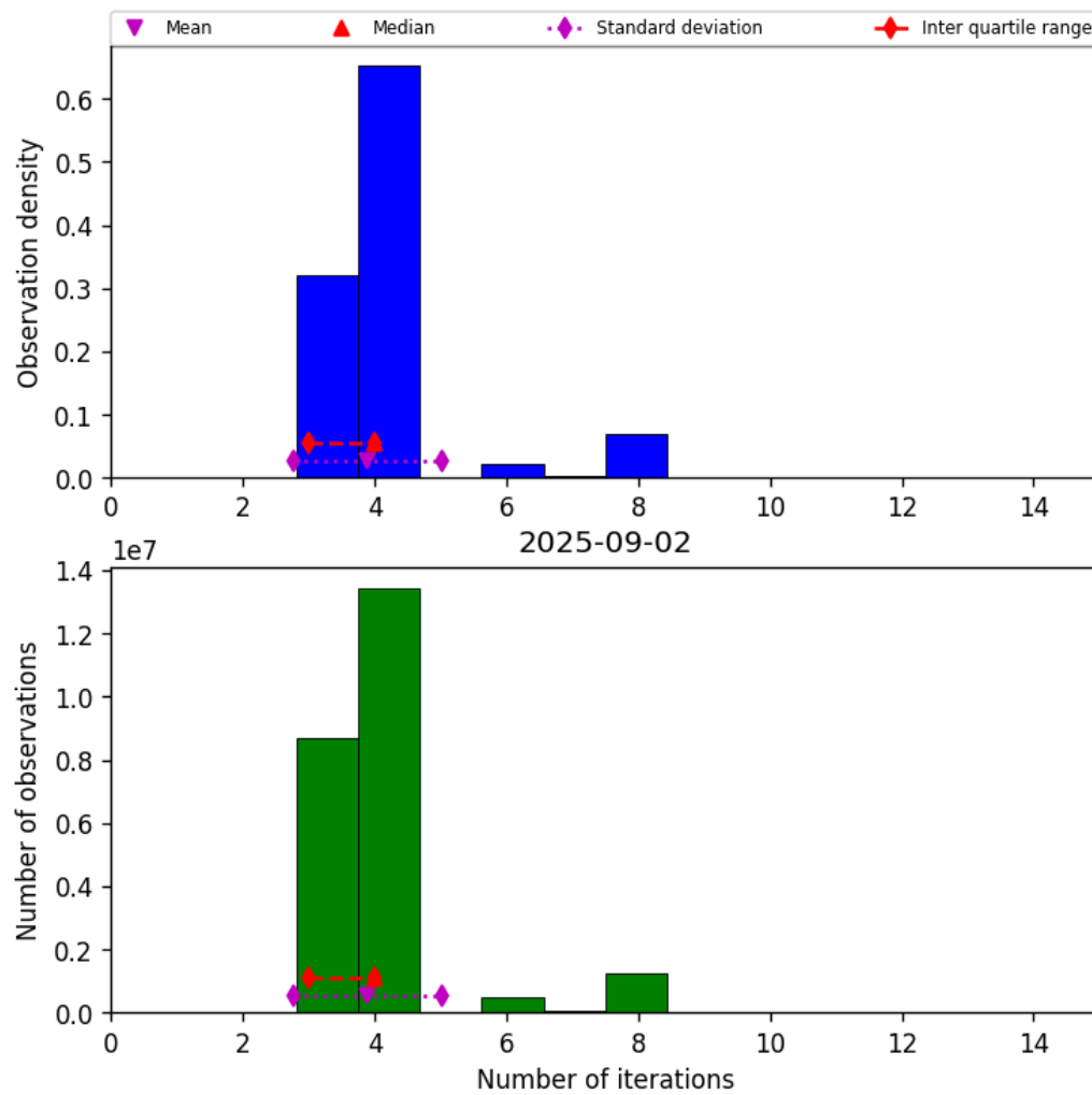
Figure 32: Histogram of “Number of iterations” for 2025-09-02 to 2025-09-02
