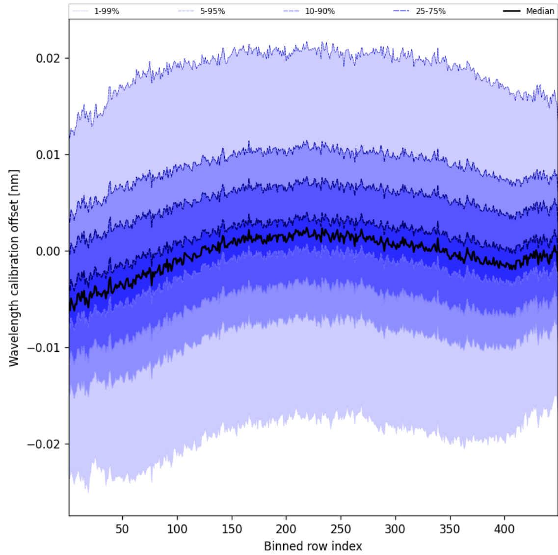
Figure 50: Along track statistics of “Wavelength calibration offset” for 2025-09-02 to 2025-09-02
