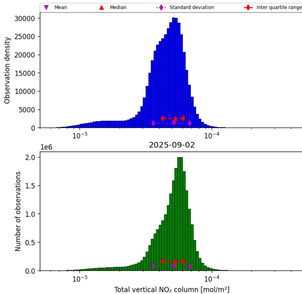
Figure 36: Histogram of "Total vertical NO 2 column" for 2025-09-02 to 2025-09-02
