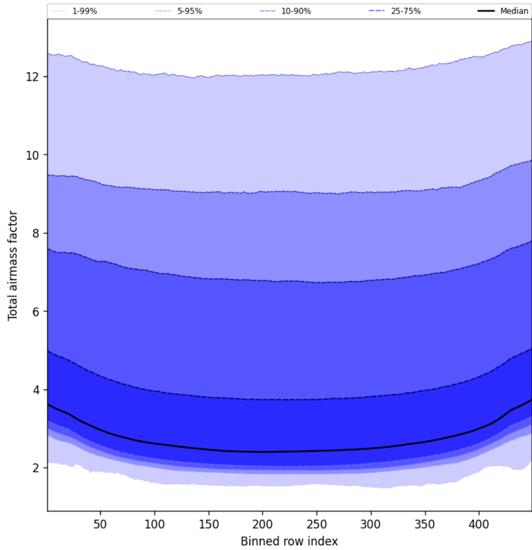
Figure 47: Along track statistics of “Total airmass factor” for 2025-09-02 to 2025-09-02
