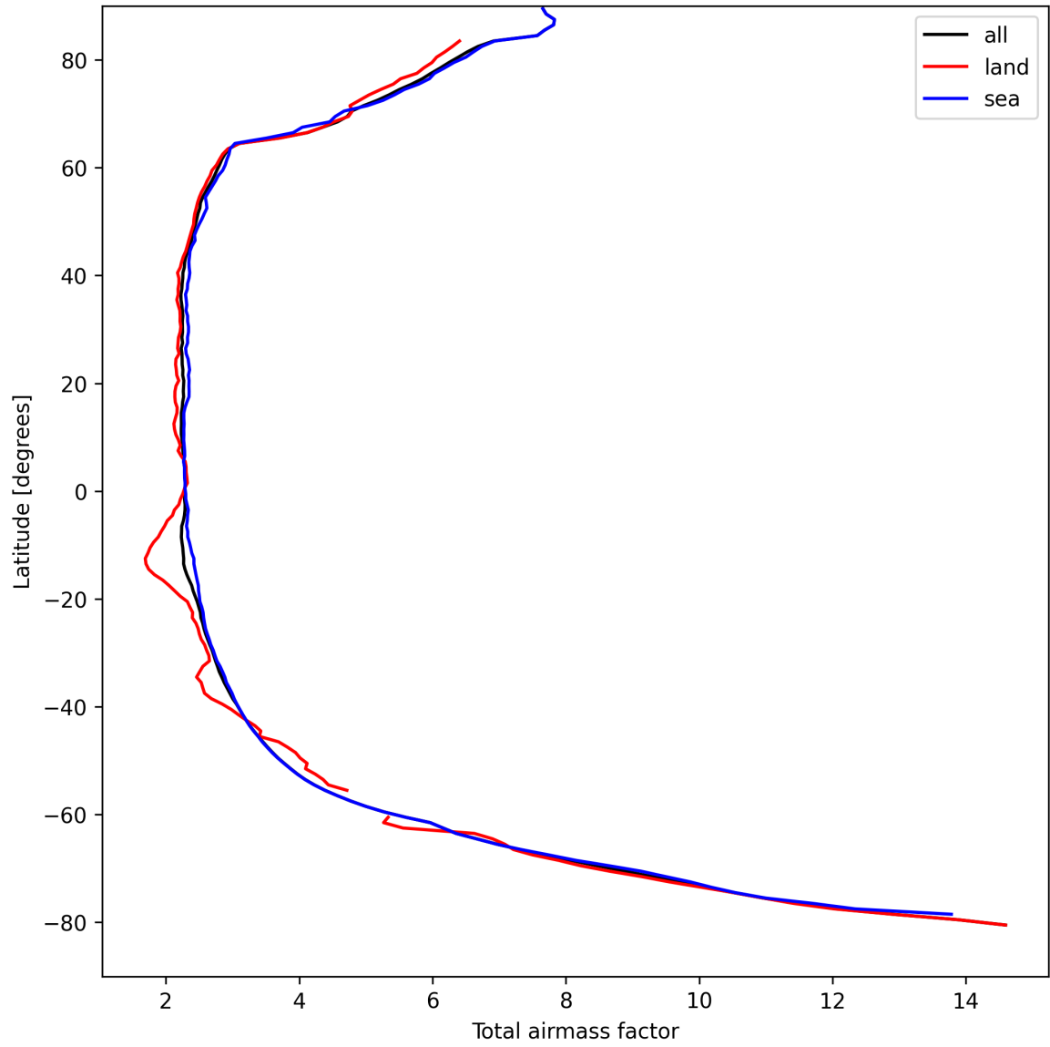
Figure 13: Zonal average of “Total airmass factor” for 2025-09-02 to 2025-09-02.
