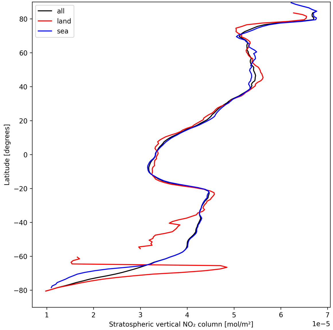
Figure 17: Zonal average of “Stratospheric vertical NO 2 column” for 2025-09-02 to 2025-09-02.
