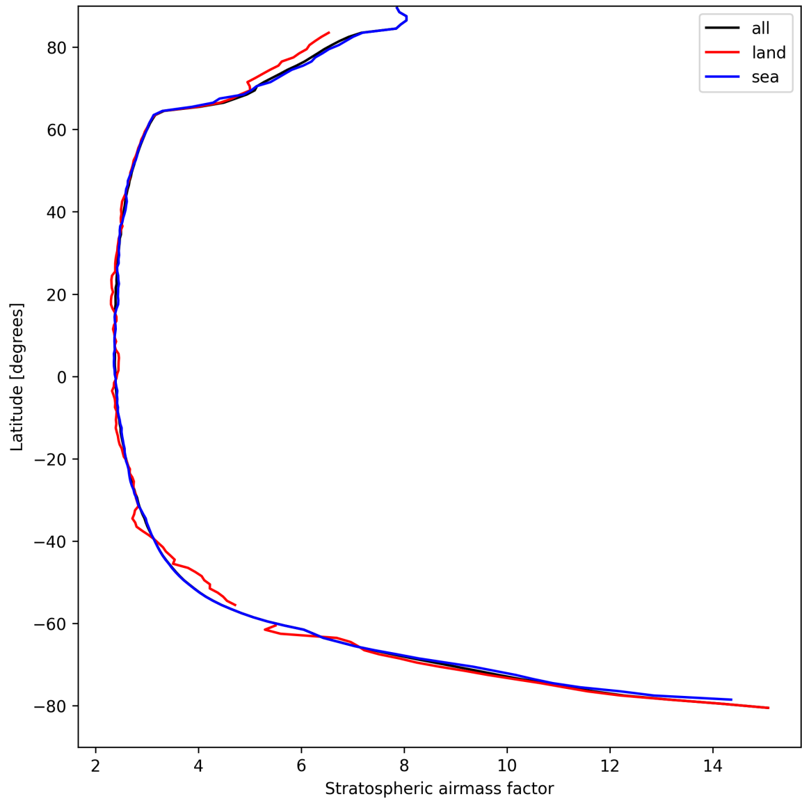
Figure 25: Zonal average of “Stratospheric air mass factor” for 2025-09-02 to 2025-09-02.
