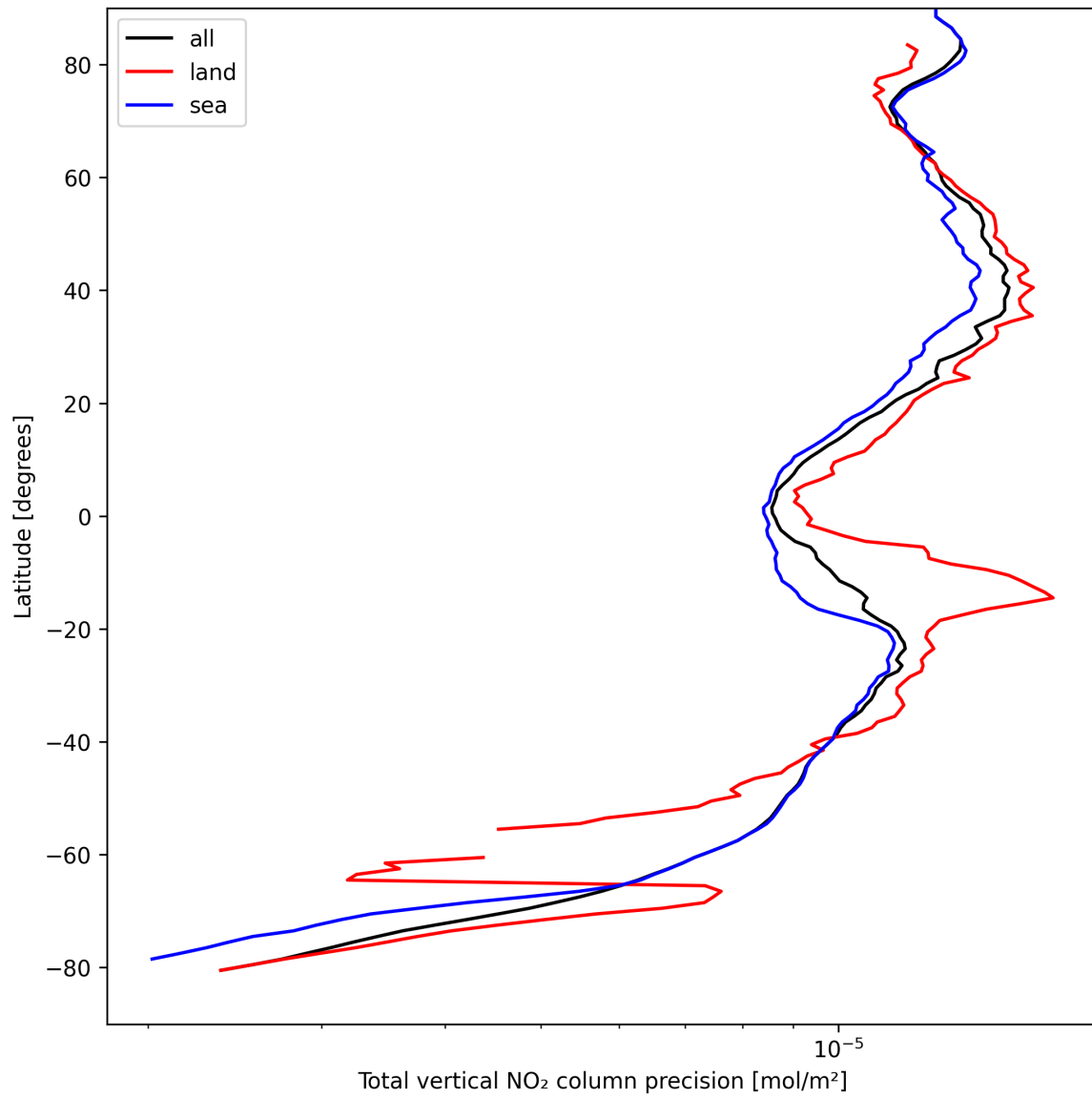
Figure 20: Zonal average of “Total vertical NO 2 column precision” for 2025-09-02 to 2025-09-02.
