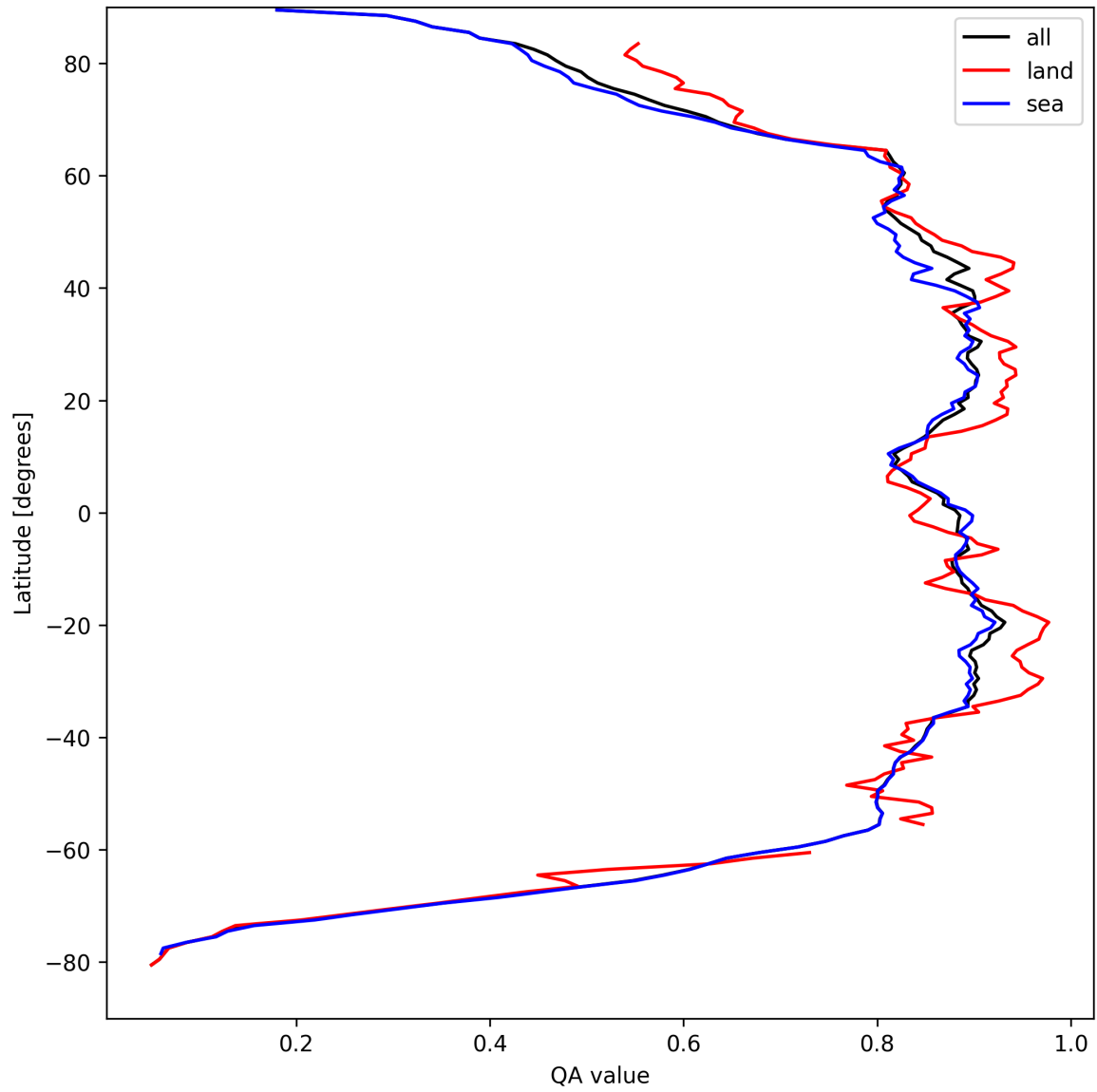
Figure 9: Zonal average of “QA value” for 2025-09-02 to 2025-09-02.
