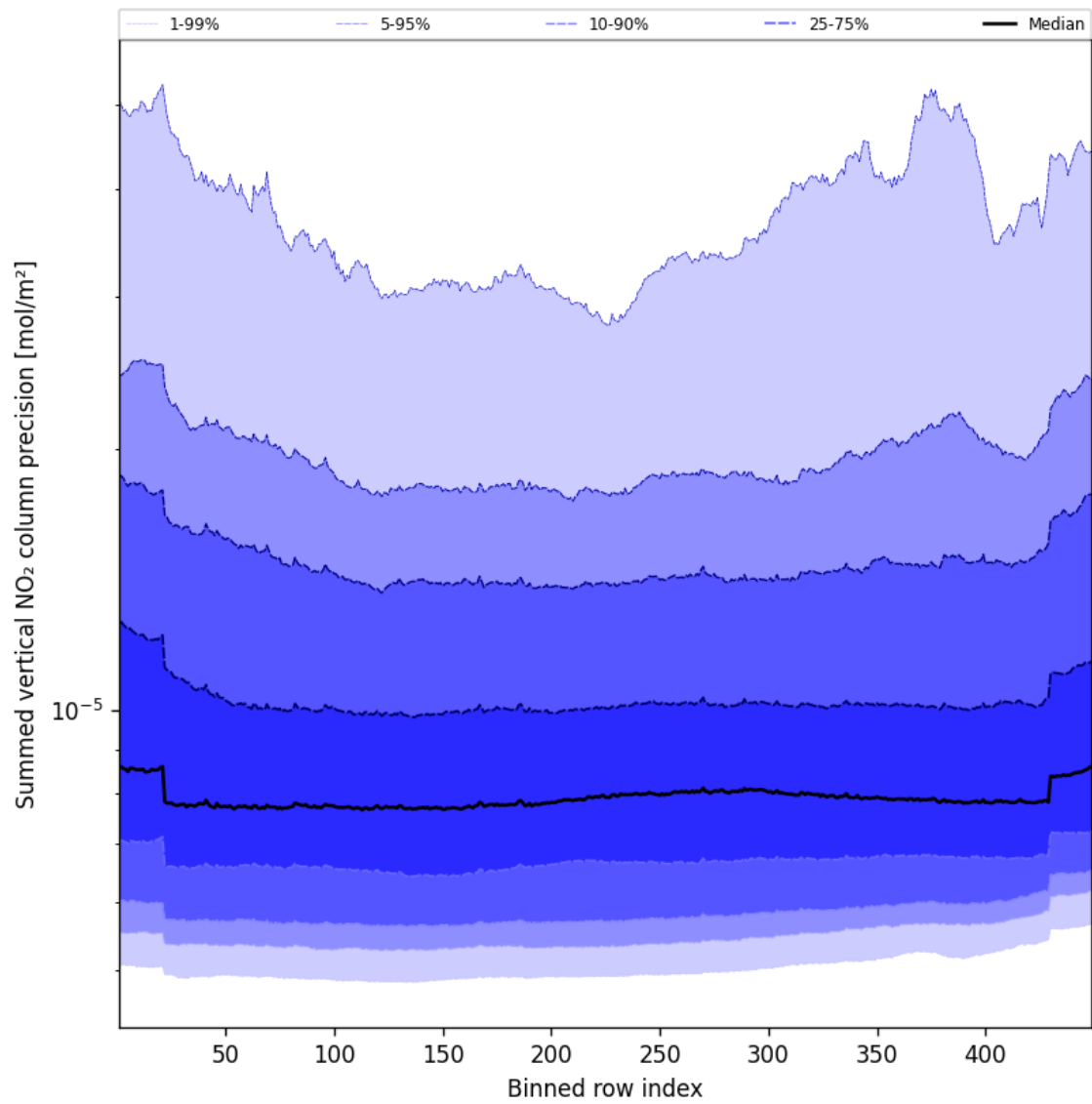
Figure 56: Along track statistics of “Summed vertical NO 2 column precision” for 2025-09-03 to 2025-09-04
