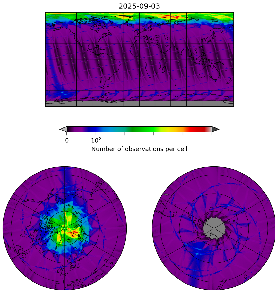
Figure 8: Map of the number of observations for 2025-09-03 to 2025-09-04
