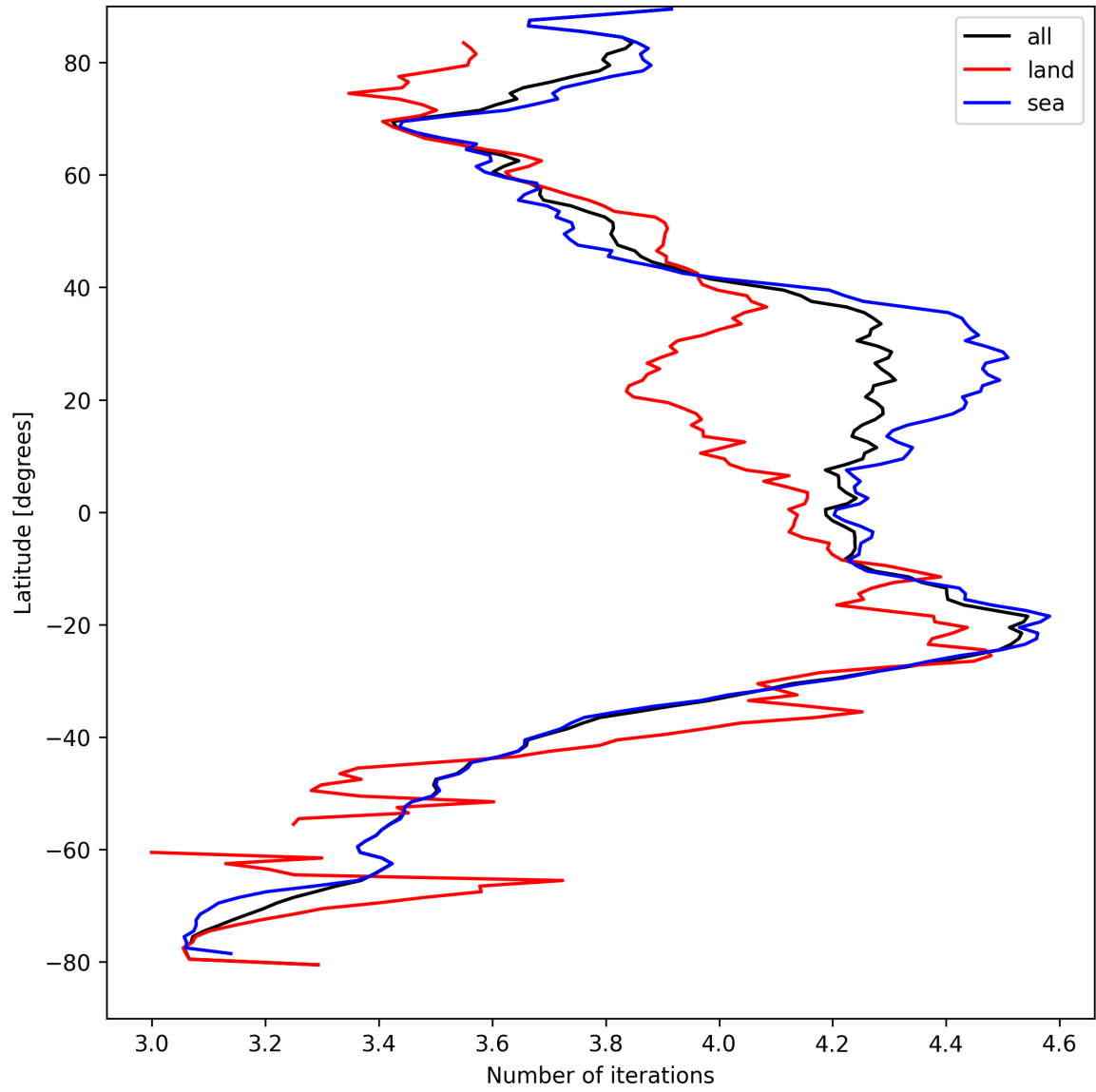
Figure 15: Zonal average of “Number of iterations” for 2025-09-03 to 2025-09-04.
