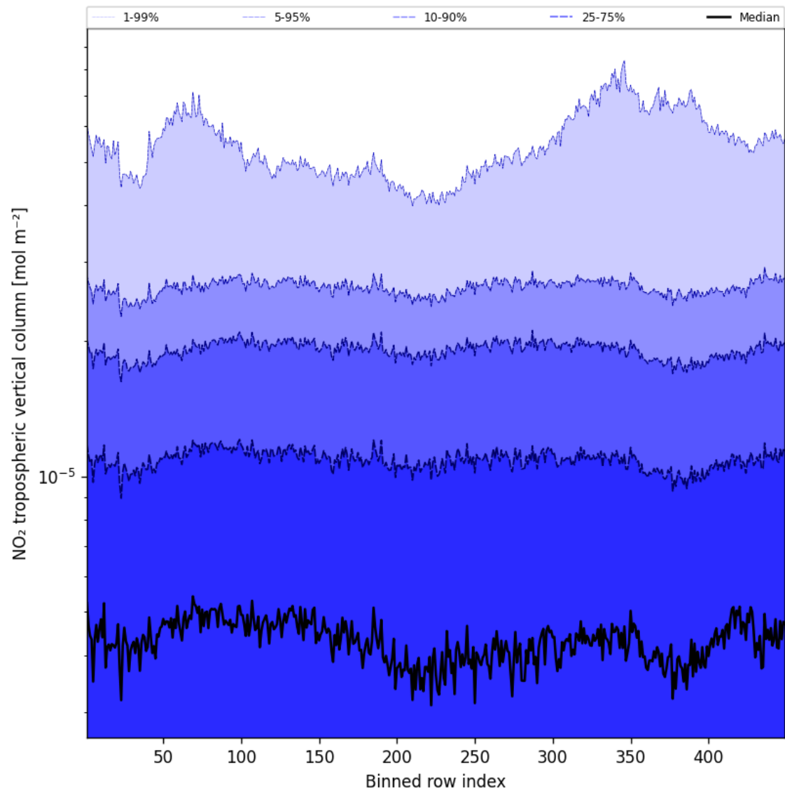
Figure 44: Along track statistics of “NO 2 tropospheric vertical column” for 2025-09-03 to 2025-09-04
