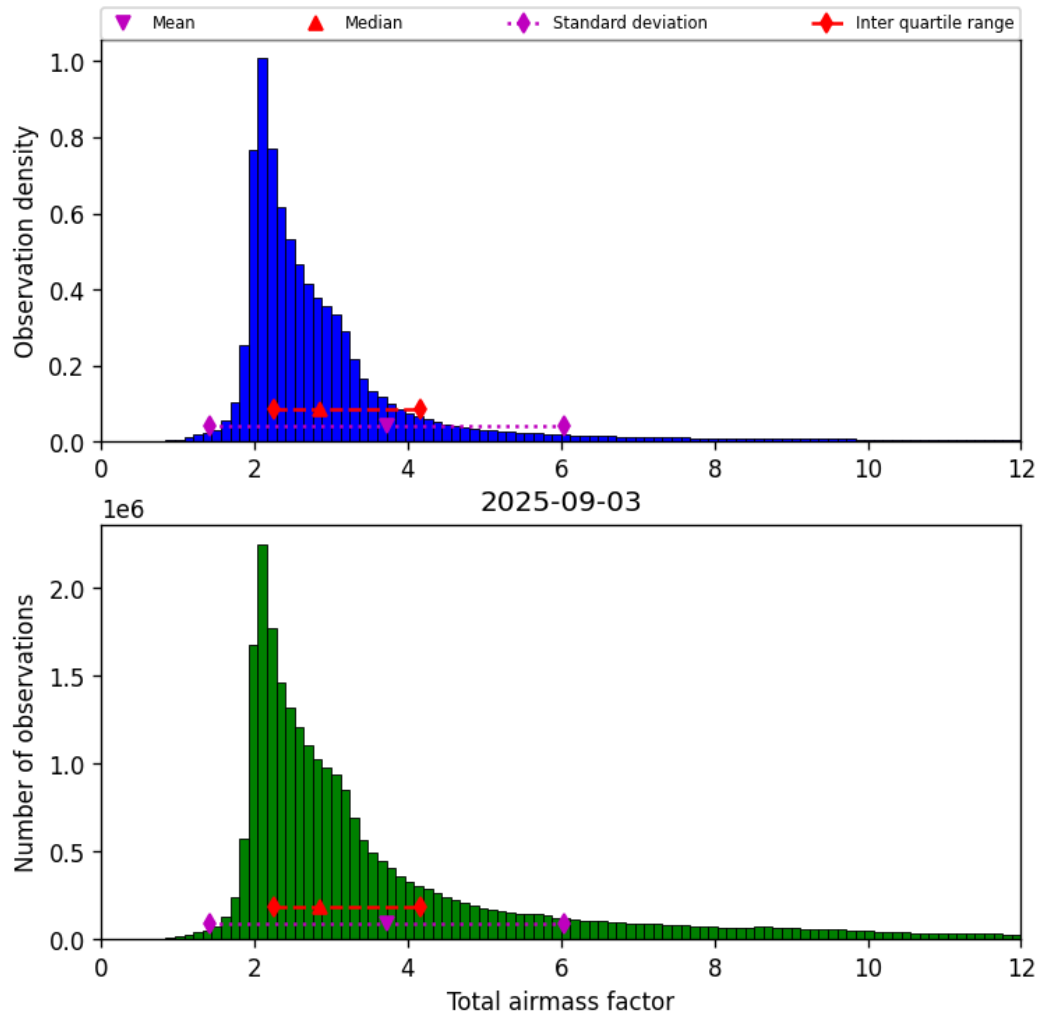
Figure 30: Histogram of “Total airmass factor” for 2025-09-03 to 2025-09-04
