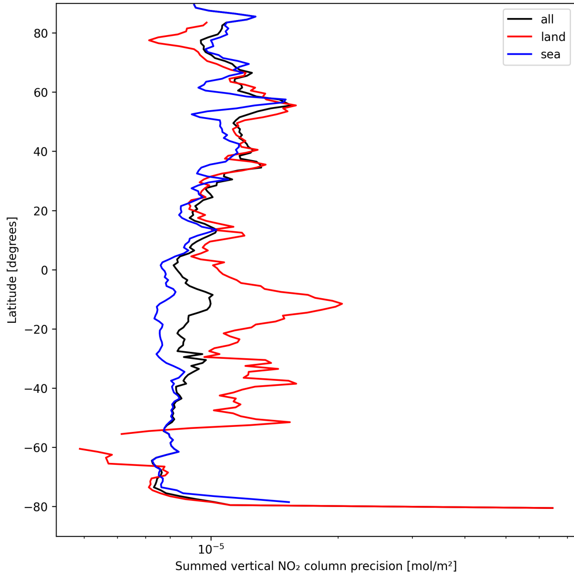
Figure 22: Zonal average of “Summed vertical NO 2 column precision” for 2025-09-03 to 2025-09-04.
