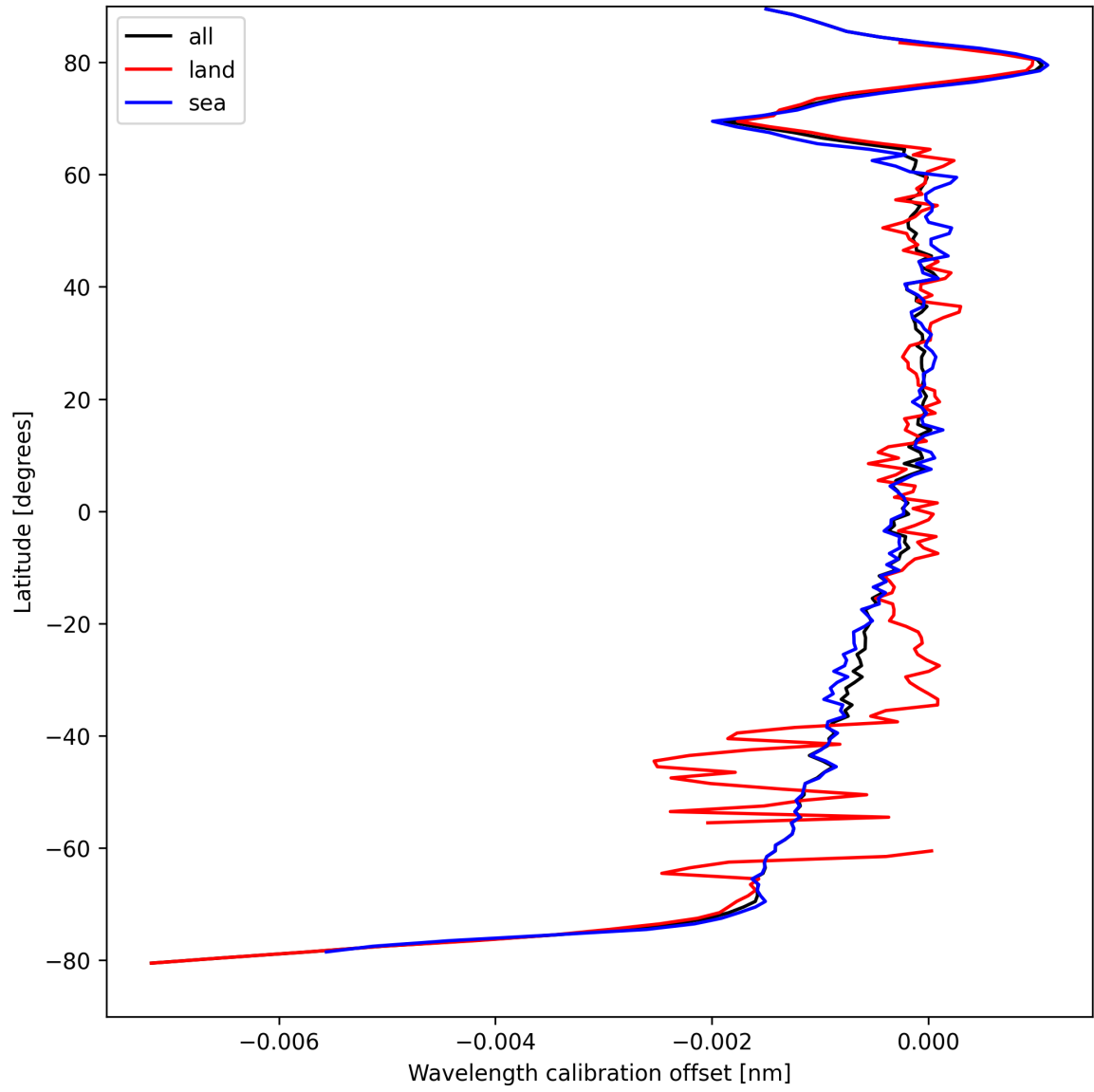
Figure 16: Zonal average of “Wavelength calibration offset” for 2025-09-03 to 2025-09-04.
