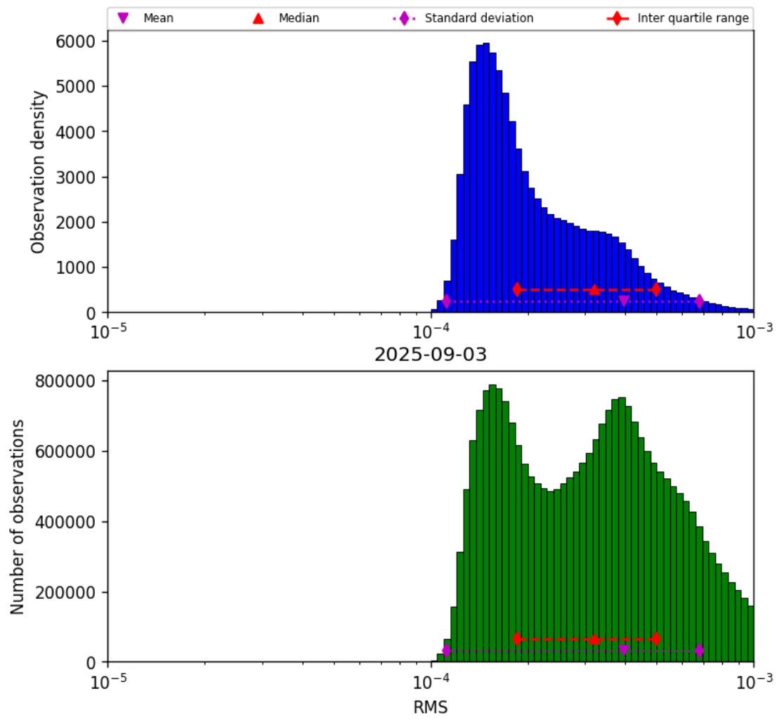
Figure 41: Histogram of “RMS” for 2025-09-03 to 2025-09-04
