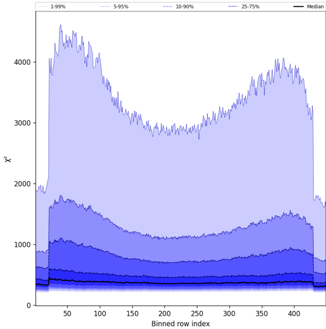
Figure 57: Along track statistics of “ \chi^2 ” for 2025-09-03 to 2025-09-04
