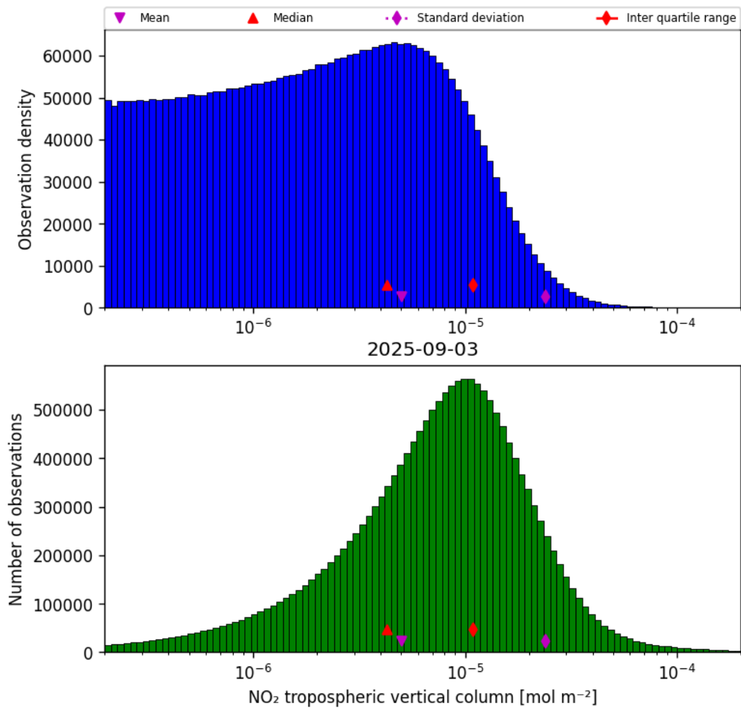
Figure 27: Histogram of “NO 2 tropospheric vertical column” for 2025-09-03 to 2025-09-04
