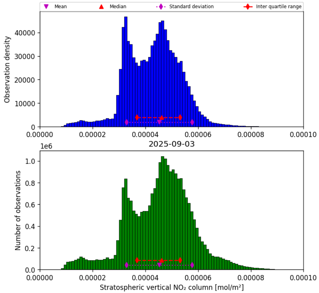
Figure 34: Histogram of “Stratospheric vertical NO 2 column” for 2025-09-03 to 2025-09-04
