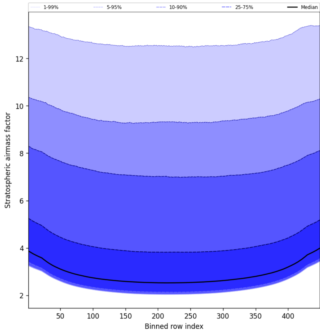
Figure 59: Along track statistics of “Stratospheric airmass factor” for 2025-09-03 to 2025-09-04
