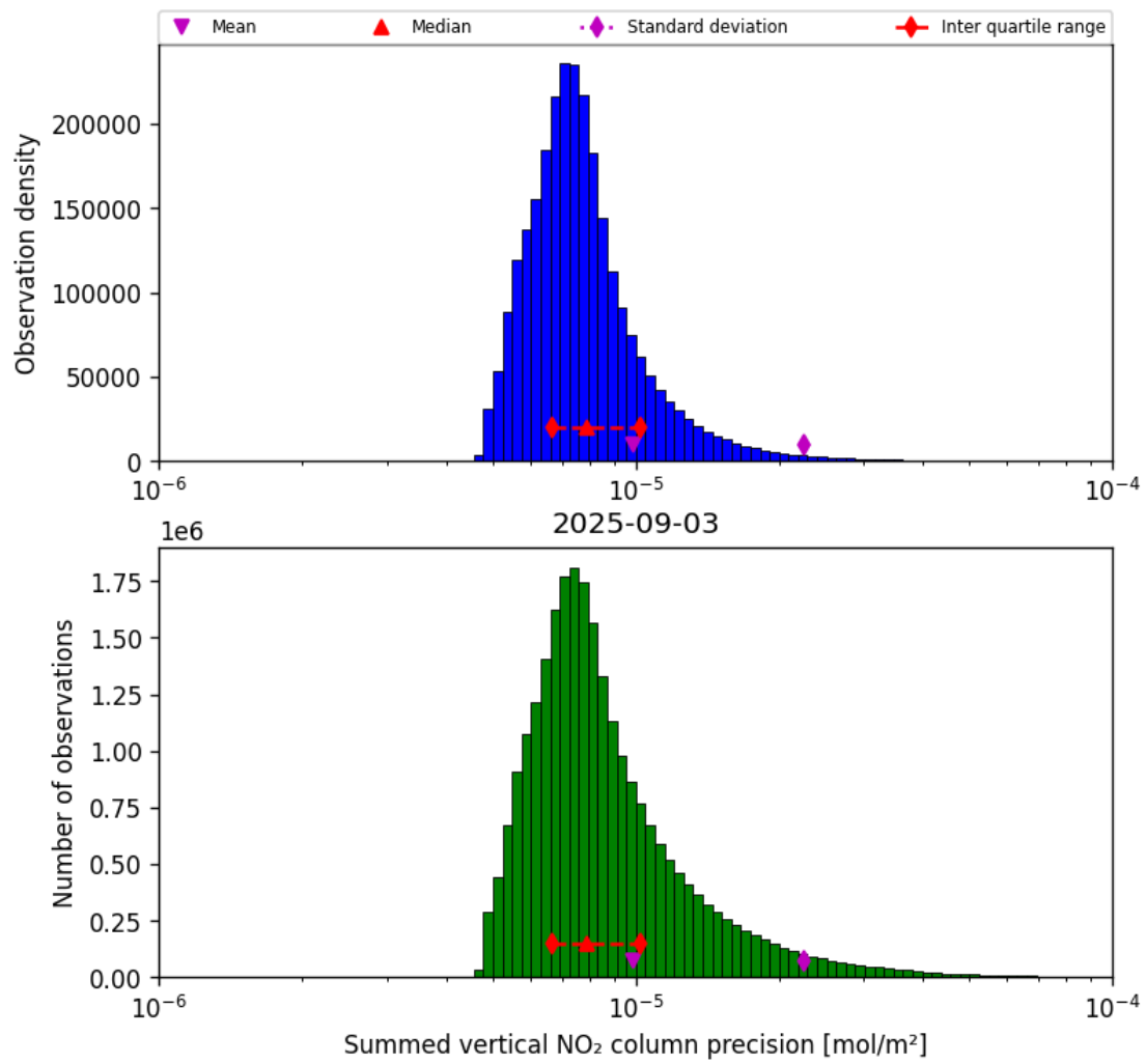
Figure 39: Histogram of “Summed vertical NO 2 column precision” for 2025-09-03 to 2025-09-04
