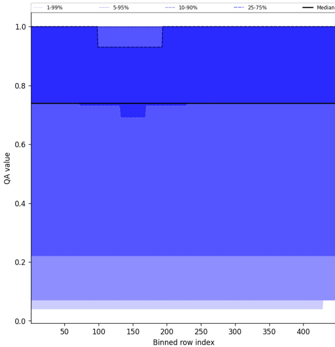
Figure 43: Along track statistics of "QA value" for 2025-09-03 to 2025-09-04
