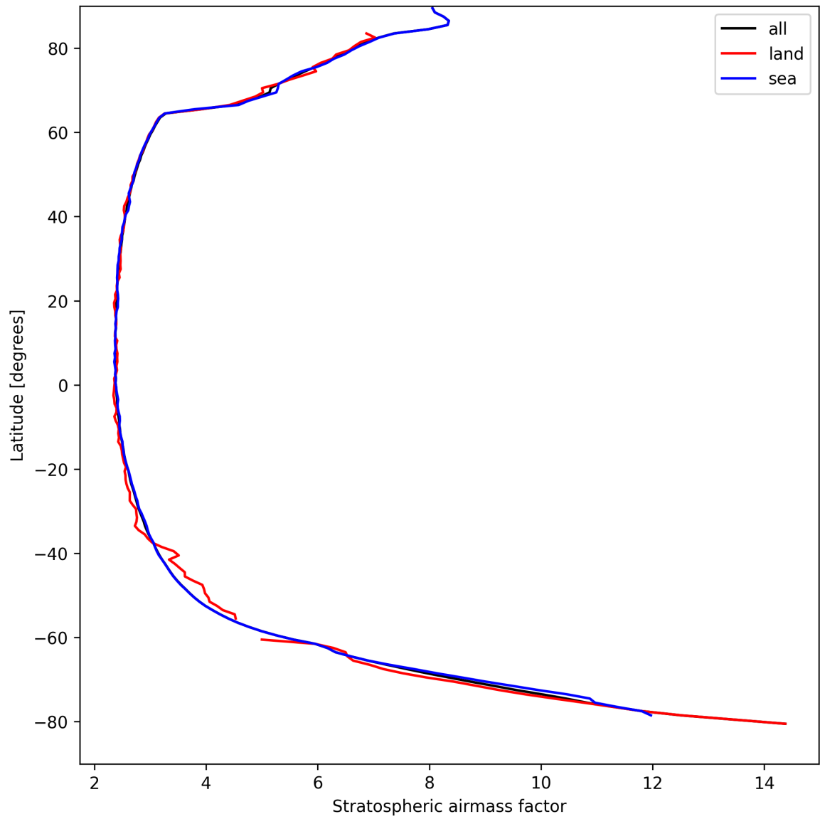
Figure 25: Zonal average of “Stratospheric air mass factor” for 2025-09-03 to 2025-09-04.
