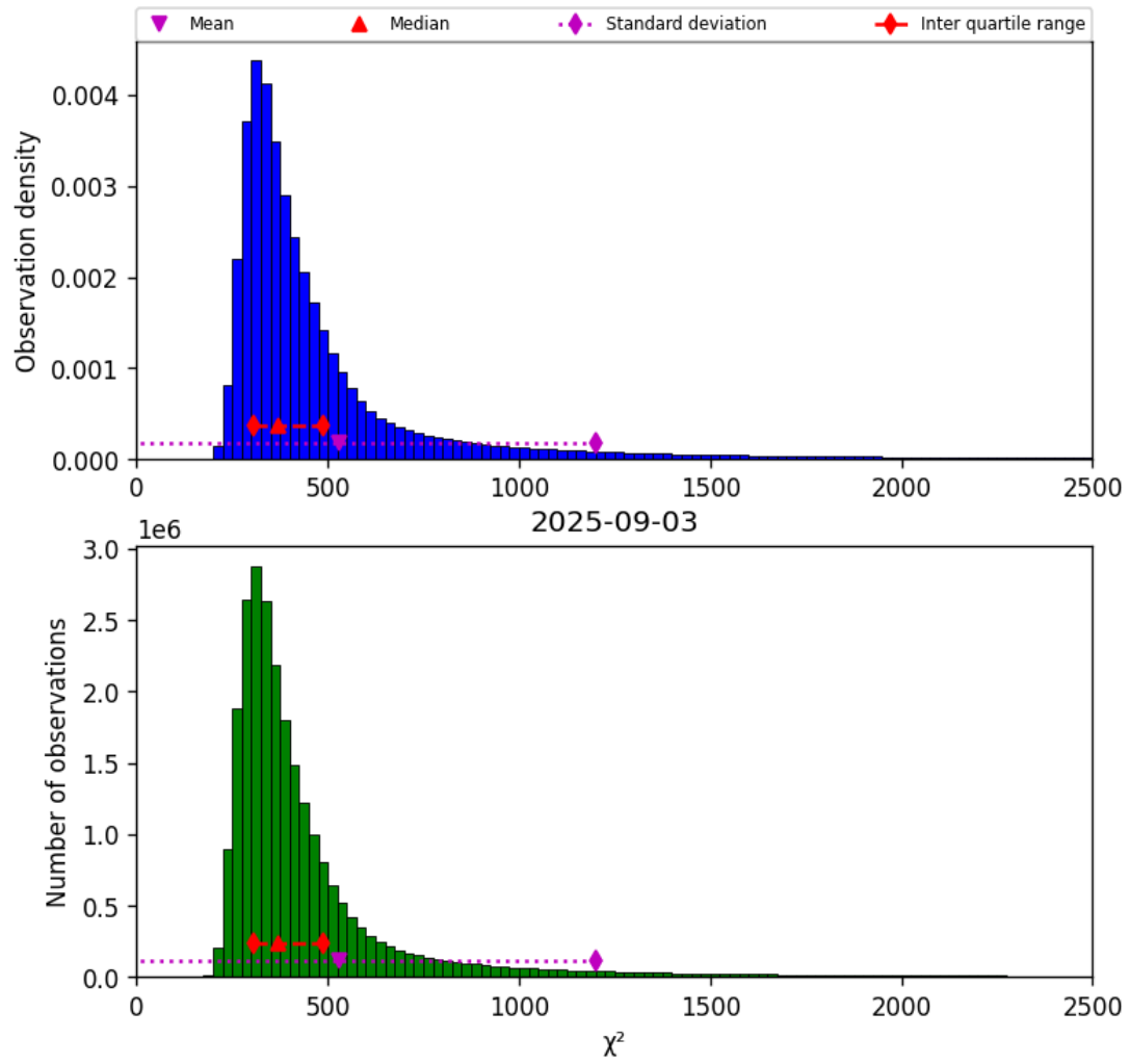
Figure 40: Histogram of “ \chi^2 ” for 2025-09-03 to 2025-09-04
