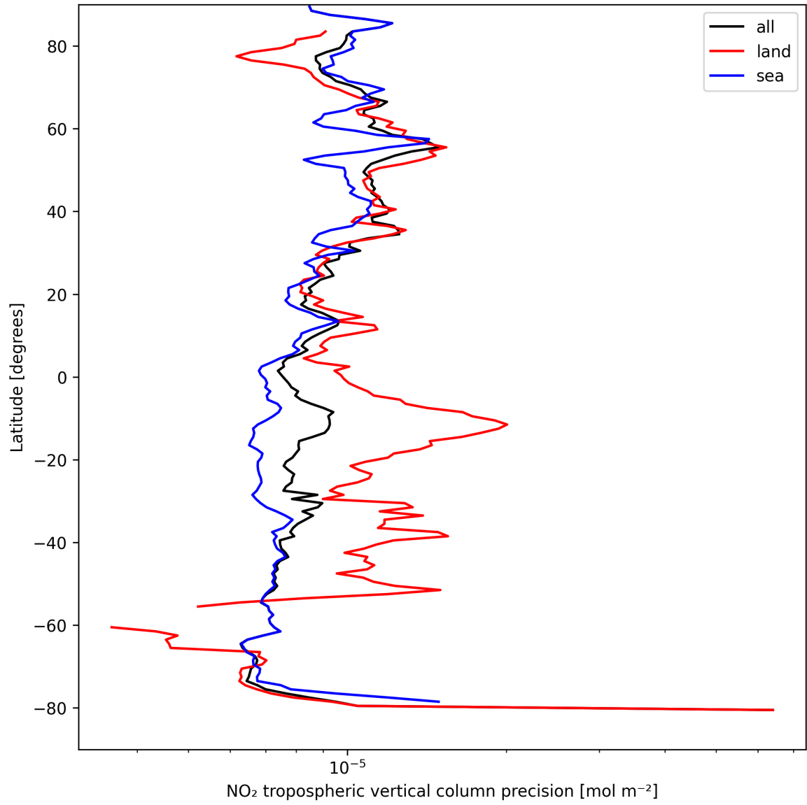
Figure 11: Zonal average of “NO 2 tropospheric vertical column precision” for 2025-09-03 to 2025-09-04.
