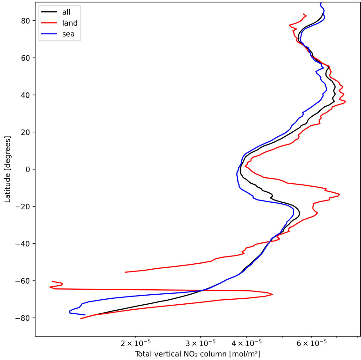
Figure 19: Zonal average of “Total vertical NO 2 column” for 2025-09-03 to 2025-09-04.
