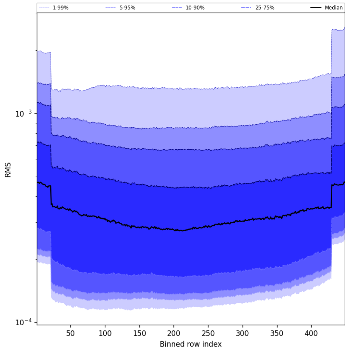
Figure 58: Along track statistics of “RMS” for 2025-09-03 to 2025-09-04
