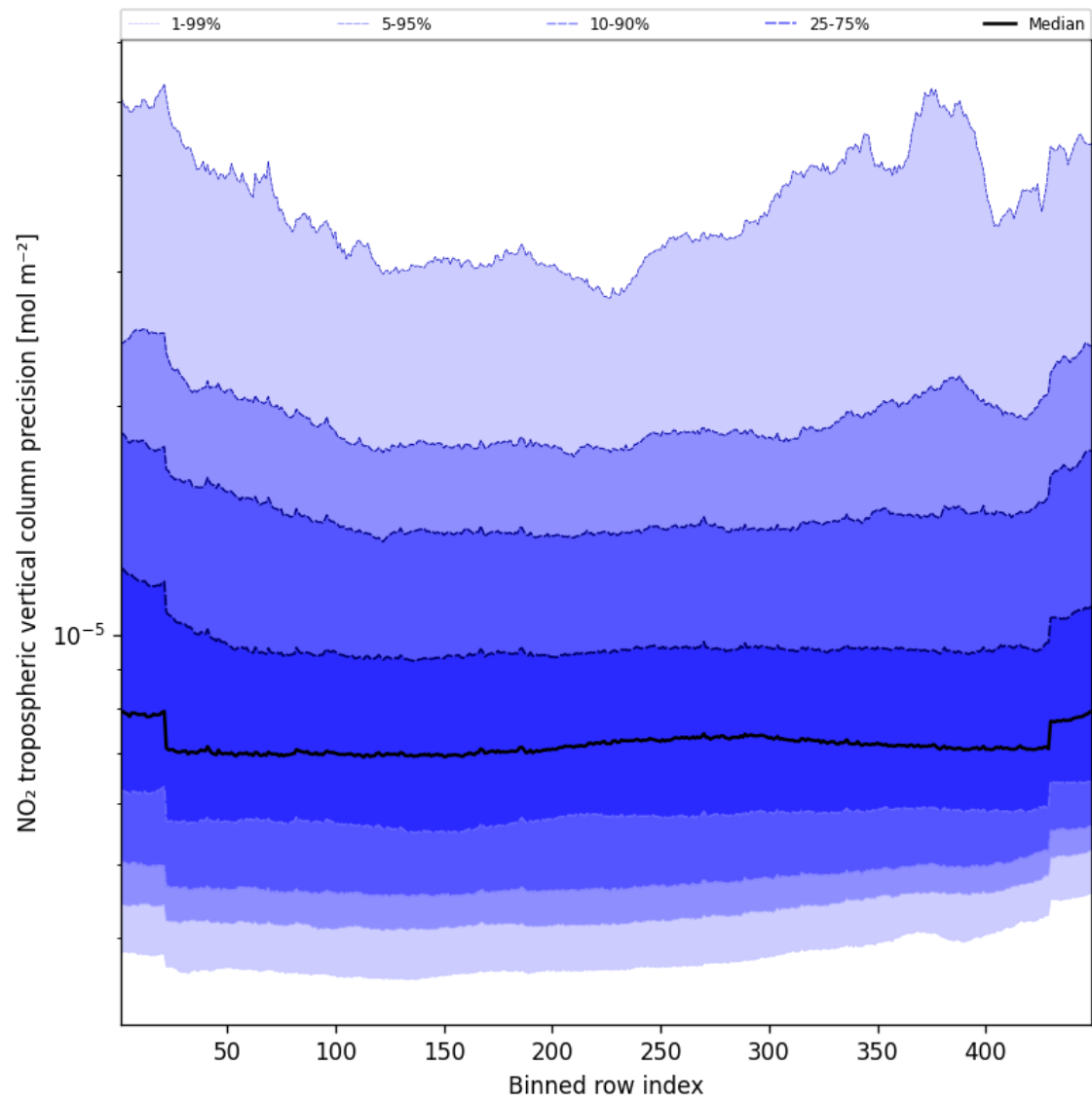
Figure 45: Along track statistics of “NO 2 tropospheric vertical column precision” for 2025-09-03 to 2025-09-04
