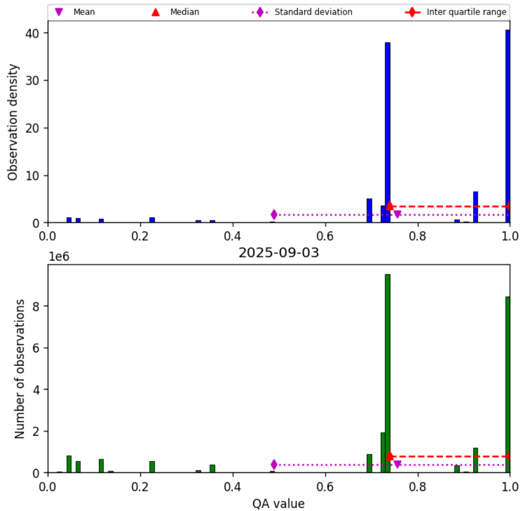
Figure 26: Histogram of “QA value” for 2025-09-03 to 2025-09-04
