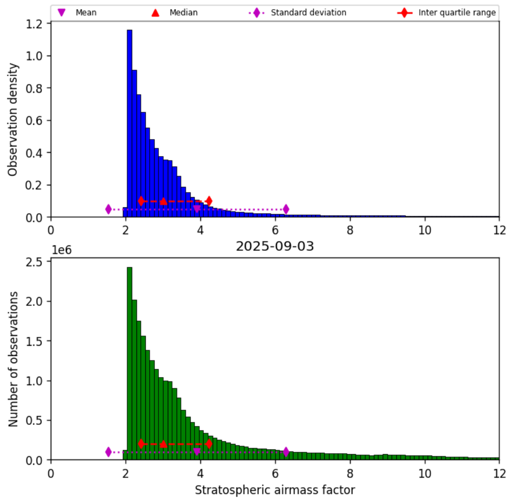
Figure 42: Histogram of “Stratospheric airmass factor” for 2025-09-03 to 2025-09-04
