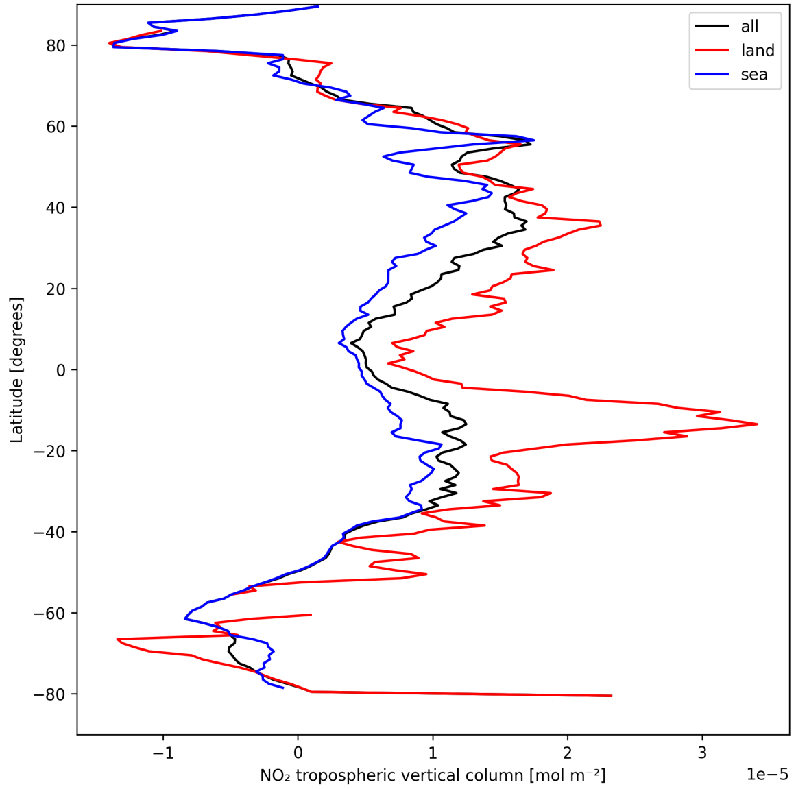
Figure 10: Zonal average of “NO 2 tropospheric vertical column” for 2025-09-03 to 2025-09-04.
