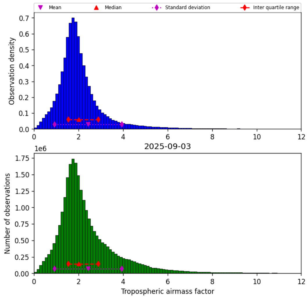
Figure 29: Histogram of “Tropospheric airmass factor” for 2025-09-03 to 2025-09-04
