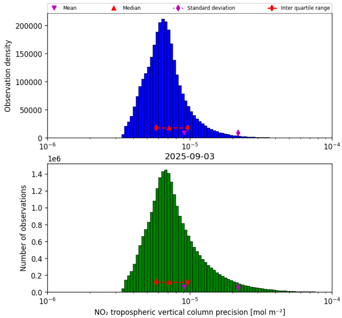
Figure 28: Histogram of “NO 2 tropospheric vertical column precision” for 2025-09-03 to 2025-09-04
