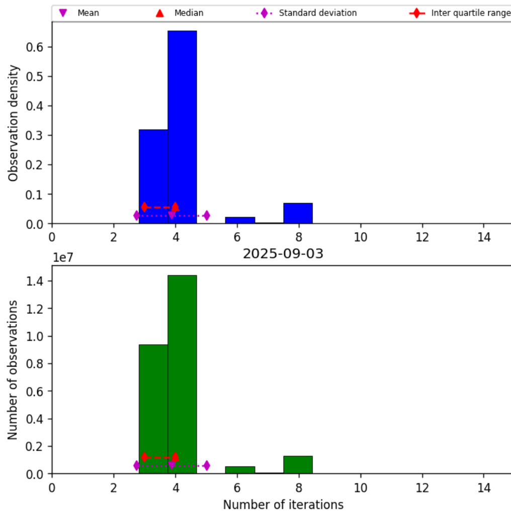
Figure 32: Histogram of “Number of iterations” for 2025-09-03 to 2025-09-04
