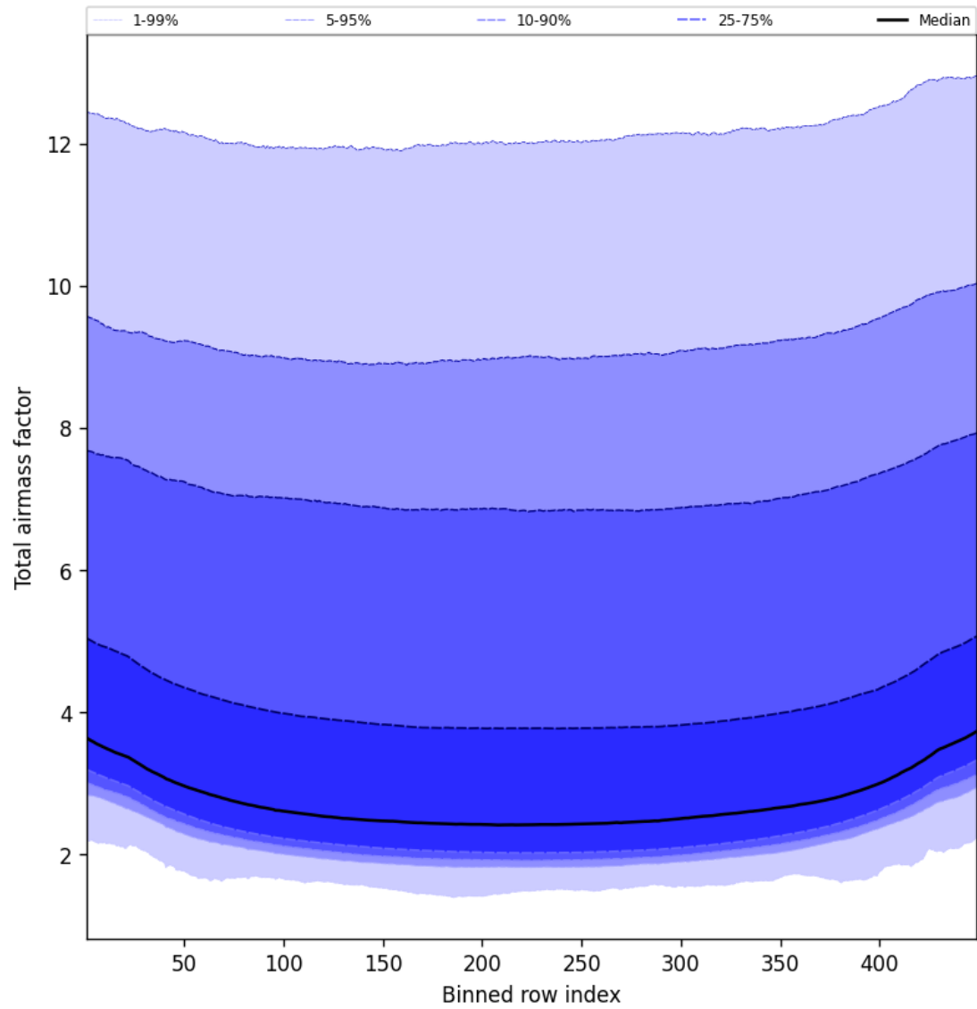
Figure 47: Along track statistics of “Total airmass factor” for 2025-09-03 to 2025-09-04
