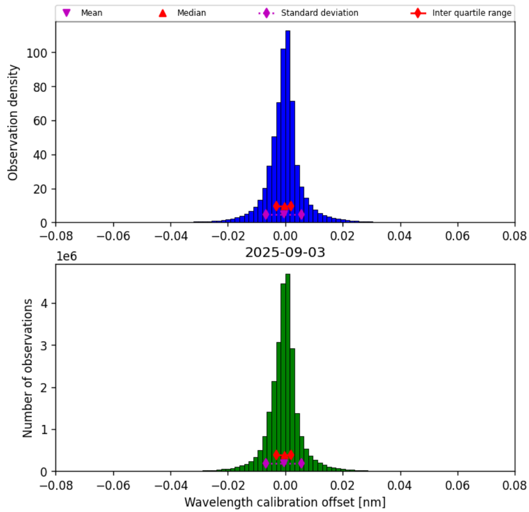
Figure 33: Histogram of “Wavelength calibration offset” for 2025-09-03 to 2025-09-04
