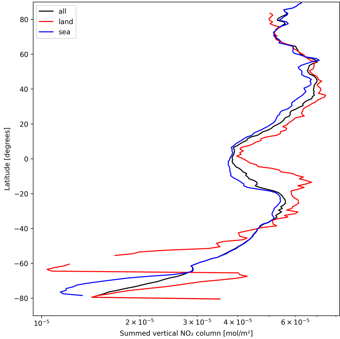
Figure 21: Zonal average of “Summed vertical NO 2 column” for 2025-09-03 to 2025-09-04.
