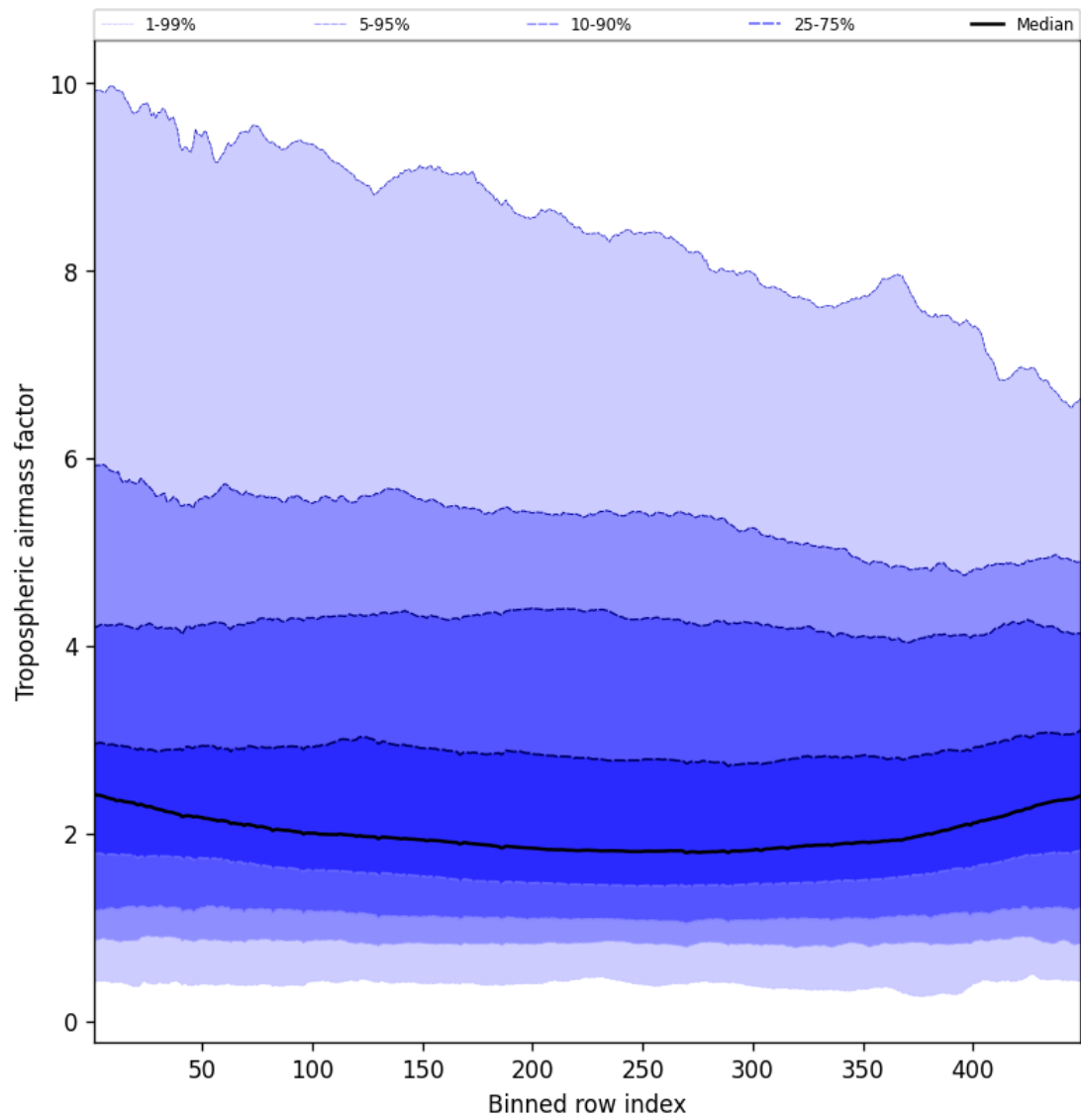
Figure 46: Along track statistics of “Tropospheric airmass factor” for 2025-09-03 to 2025-09-04
