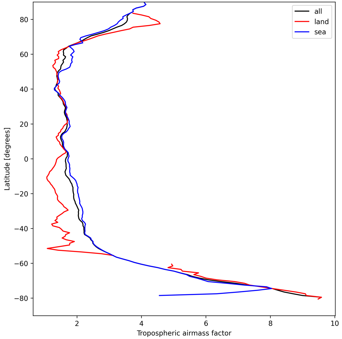
Figure 12: Zonal average of “Tropospheric airmass factor” for 2025-09-03 to 2025-09-04.
