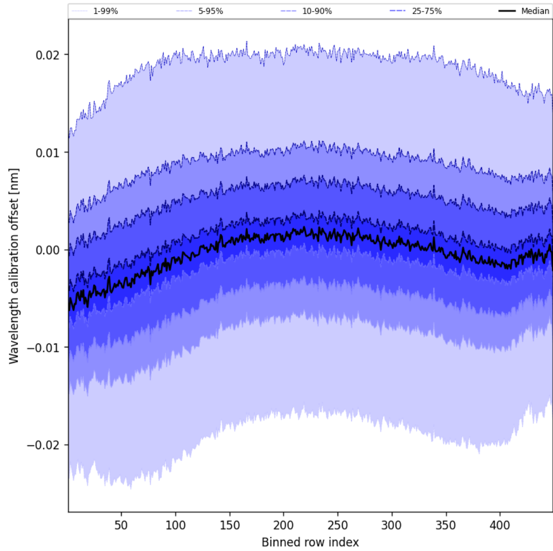
Figure 50: Along track statistics of “Wavelength calibration offset” for 2025-09-03 to 2025-09-04
