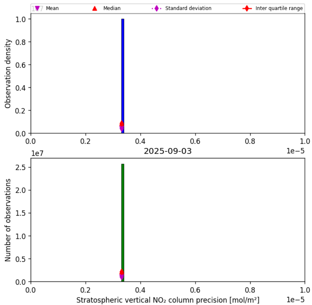
Figure 35: Histogram of “Stratospheric vertical NO 2 column precision” for 2025-09-03 to 2025-09-04
