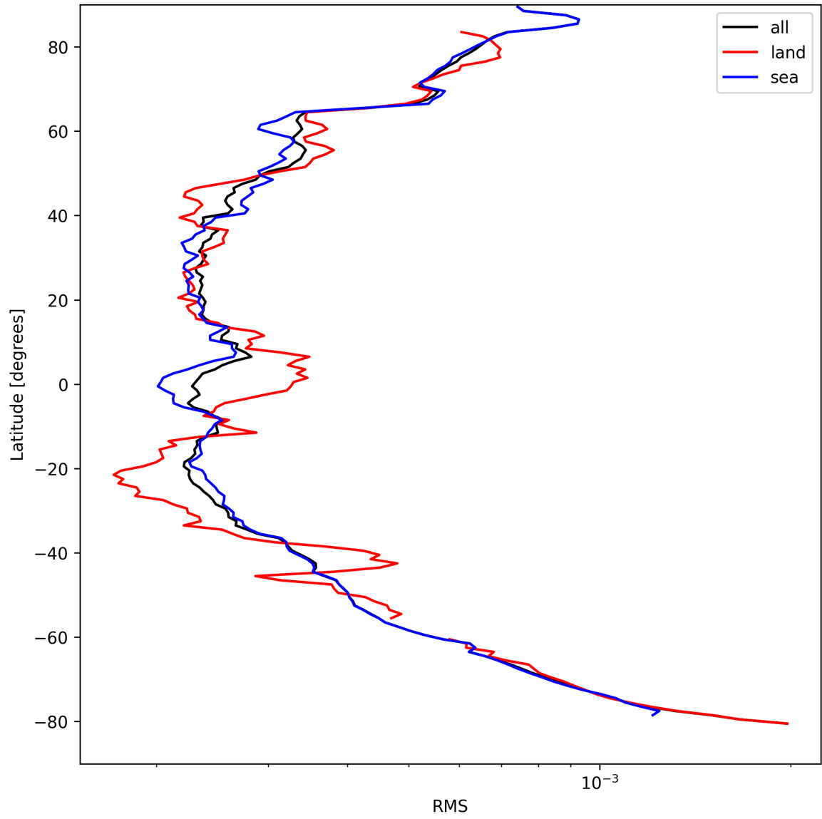
Figure 24: Zonal average of “RMS” for 2025-09-03 to 2025-09-04.
