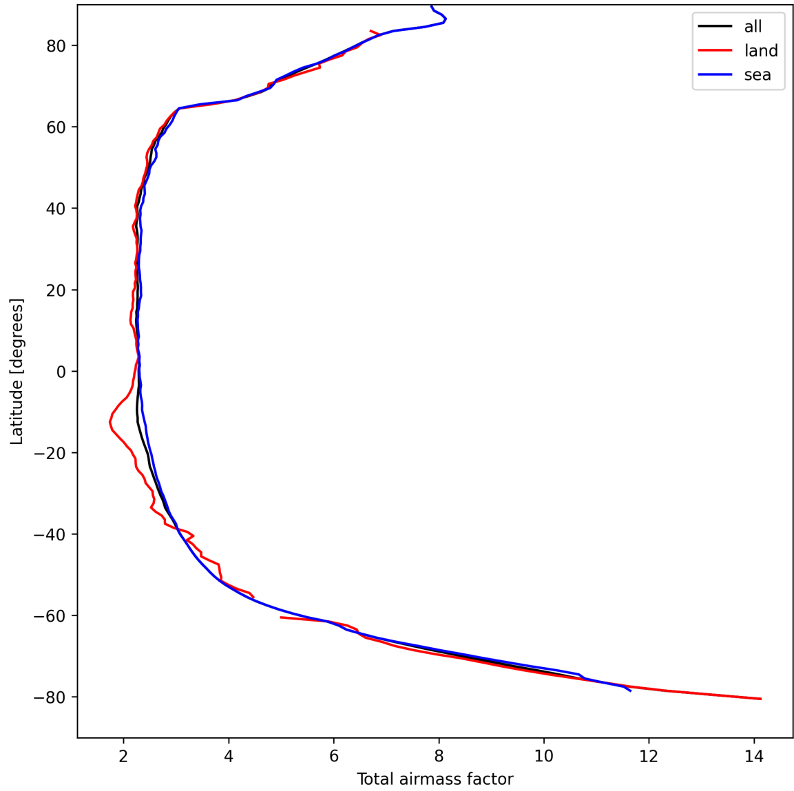
Figure 13: Zonal average of “Total airmass factor” for 2025-09-03 to 2025-09-04.
