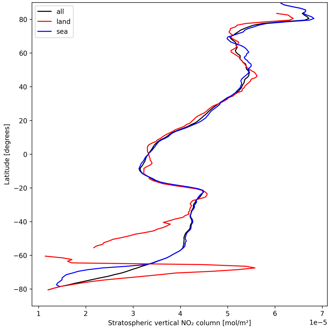
Figure 17: Zonal average of “Stratospheric vertical NO 2 column” for 2025-09-03 to 2025-09-04.
