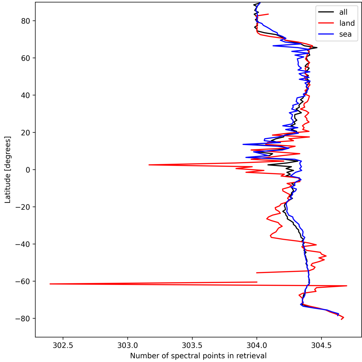
Figure 14: Zonal average of “Number of spectral points in retrieval” for 2025-09-03 to 2025-09-04.
