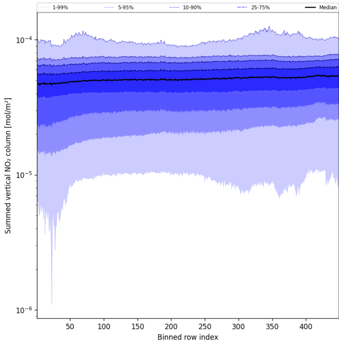
Figure 55: Along track statistics of “Summed vertical NO 2 column” for 2025-09-03 to 2025-09-04
