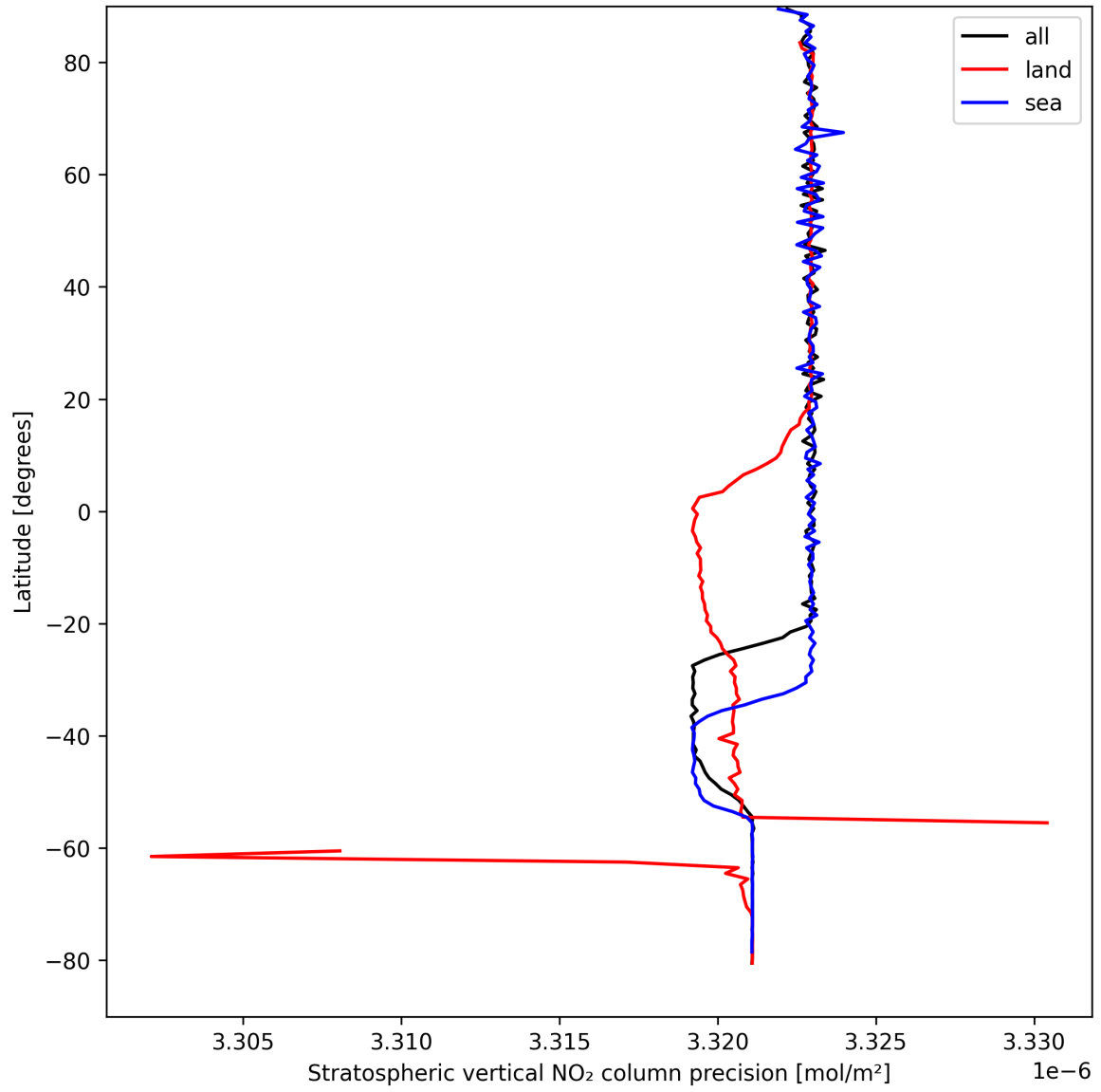
Figure 18: Zonal average of “Stratospheric vertical NO 2 column precision” for 2025-09-03 to 2025-09-04.
