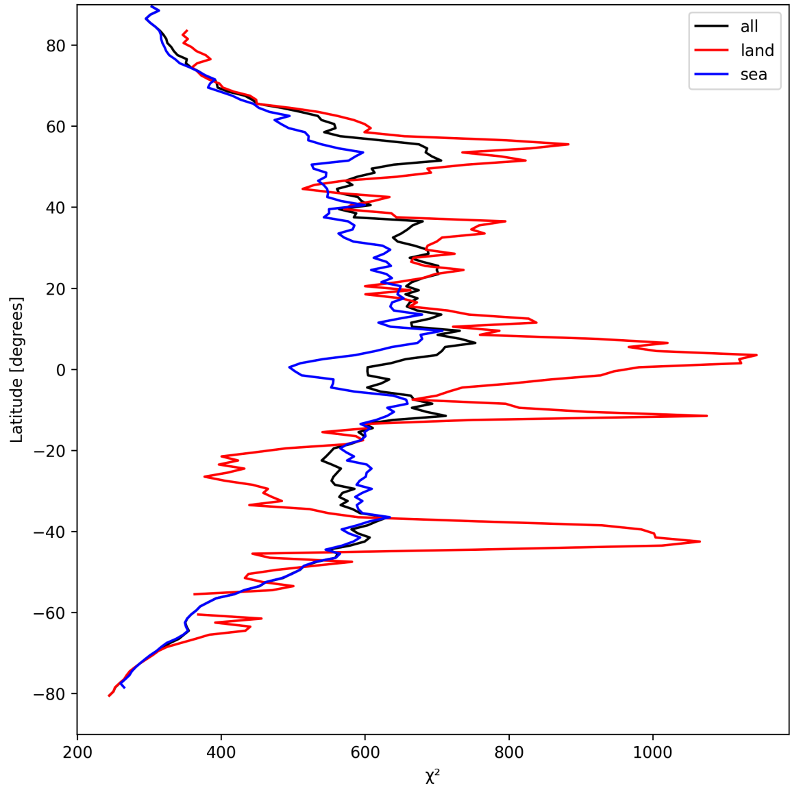
Figure 23: Zonal average of “ \chi^2 ” for 2025-09-03 to 2025-09-04.
