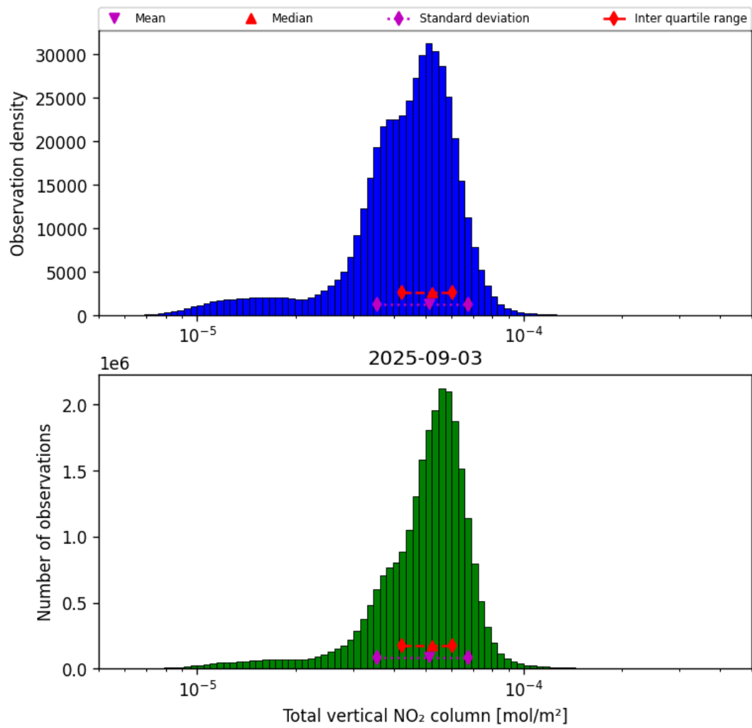
Figure 36: Histogram of “Total vertical NO 2 column” for 2025-09-03 to 2025-09-04
