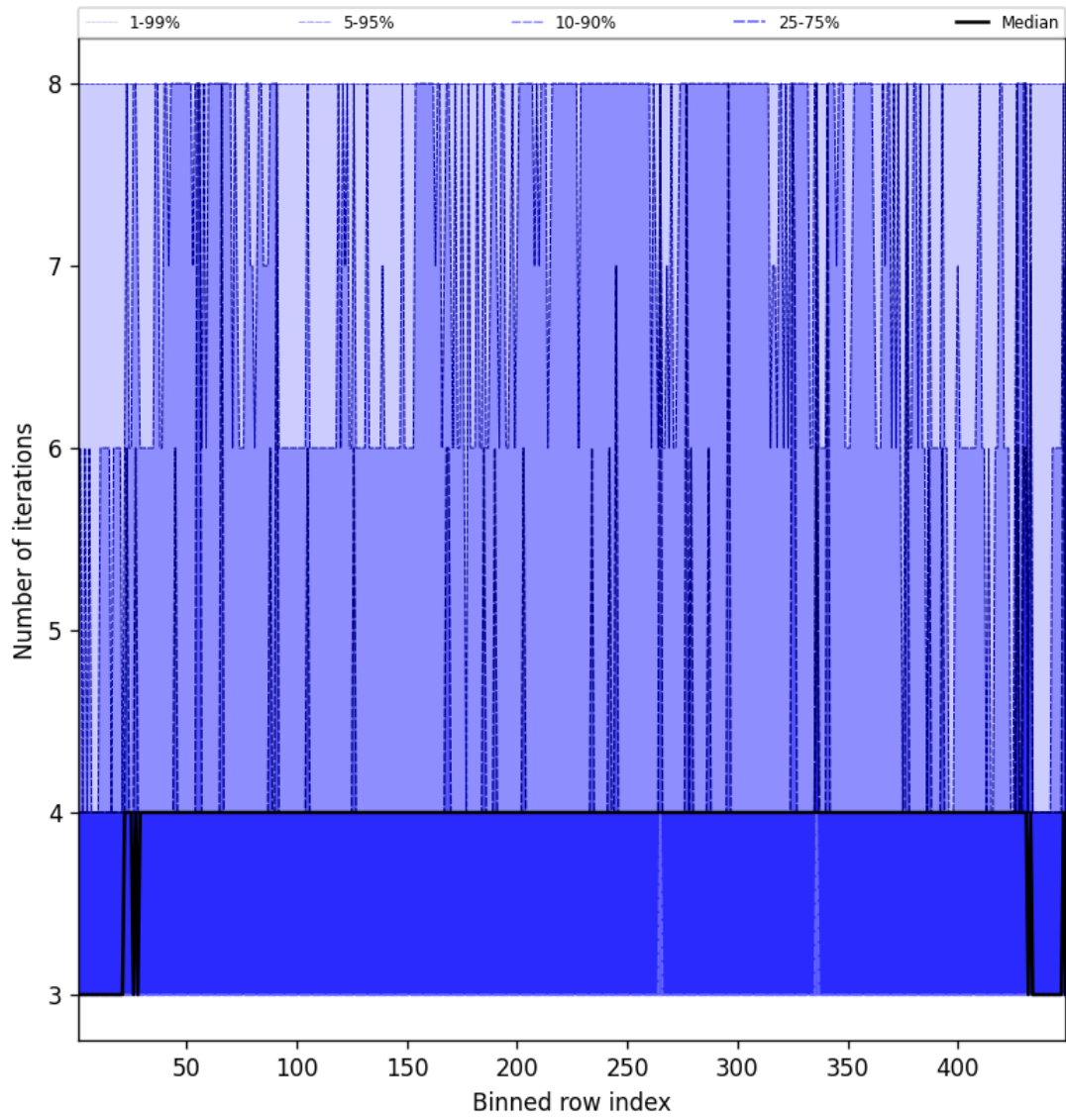
Figure 49: Along track statistics of “Number of iterations” for 2025-09-03 to 2025-09-04
