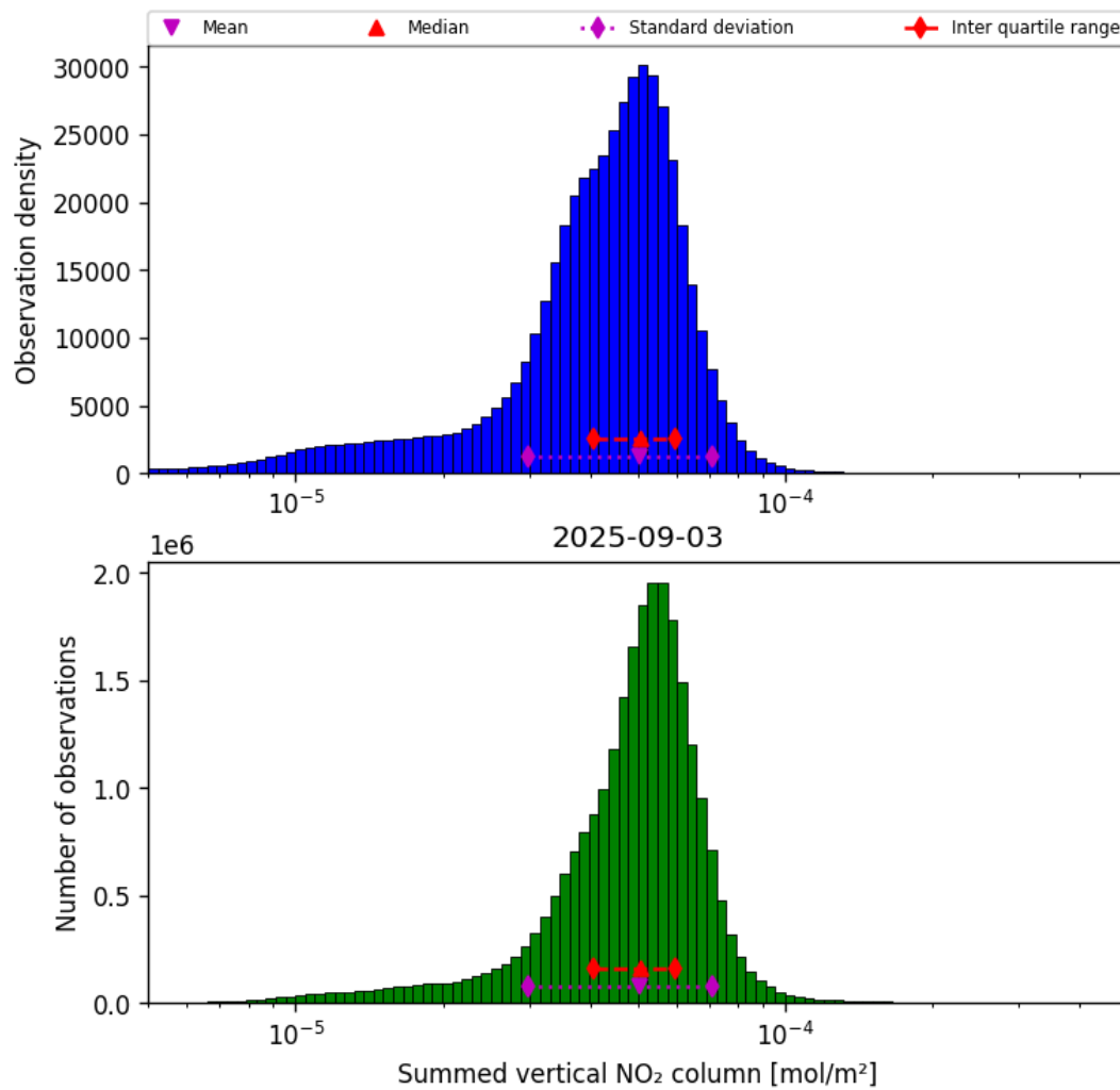
Figure 38: Histogram of “Summed vertical NO 2 column” for 2025-09-03 to 2025-09-04
