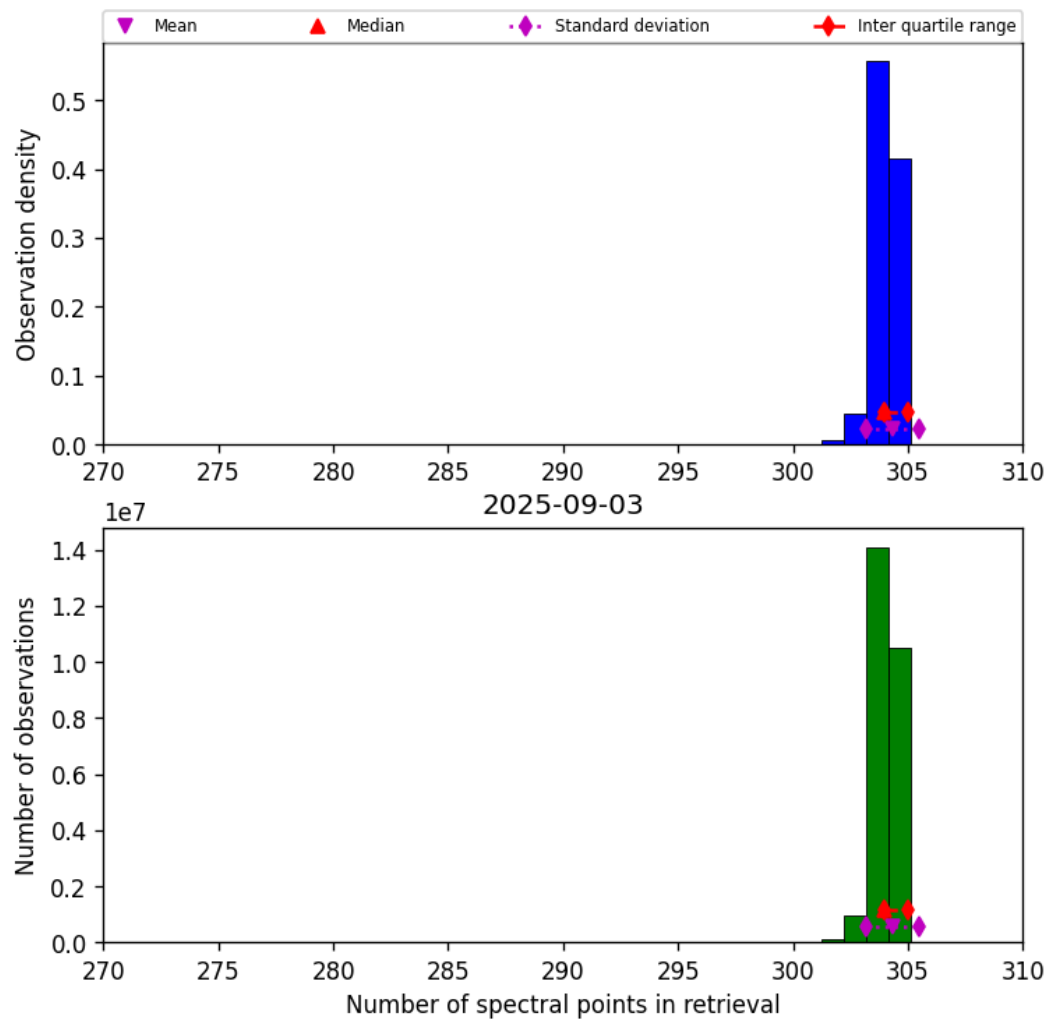
Figure 31: Histogram of “Number of spectral points in retrieval” for 2025-09-03 to 2025-09-04
