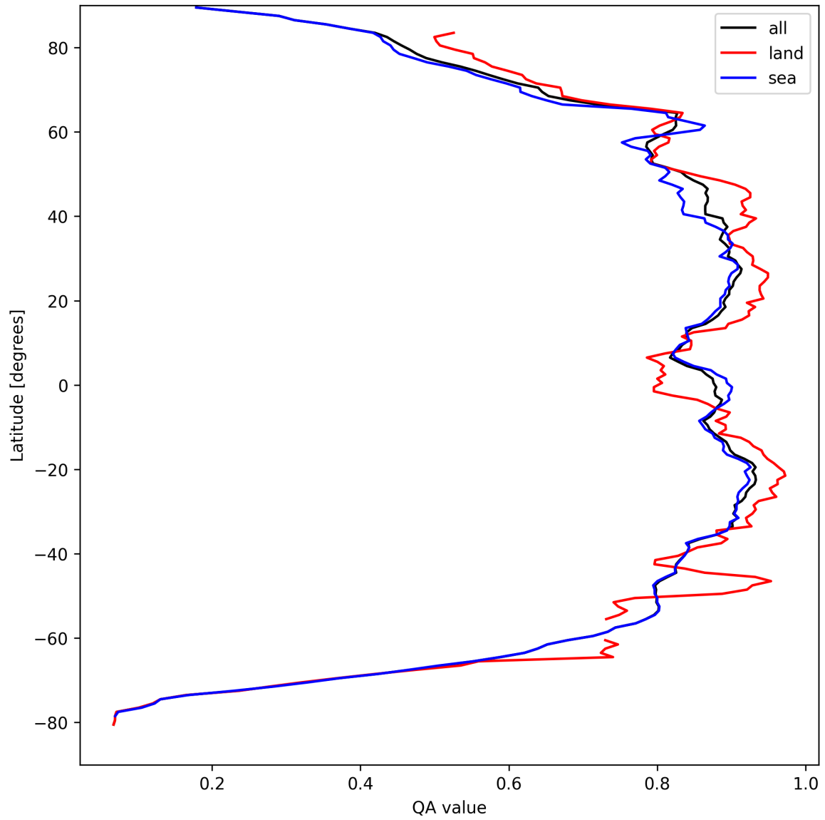
Figure 9: Zonal average of “QA value” for 2025-09-03 to 2025-09-04.
