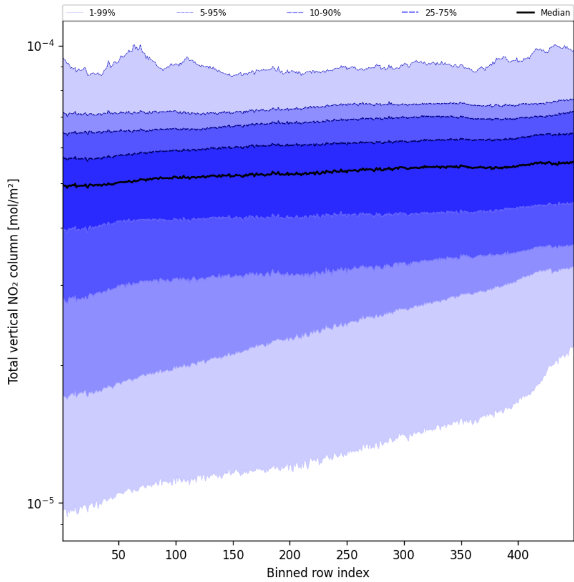
Figure 53: Along track statistics of “Total vertical NO 2 column” for 2025-09-03 to 2025-09-04
