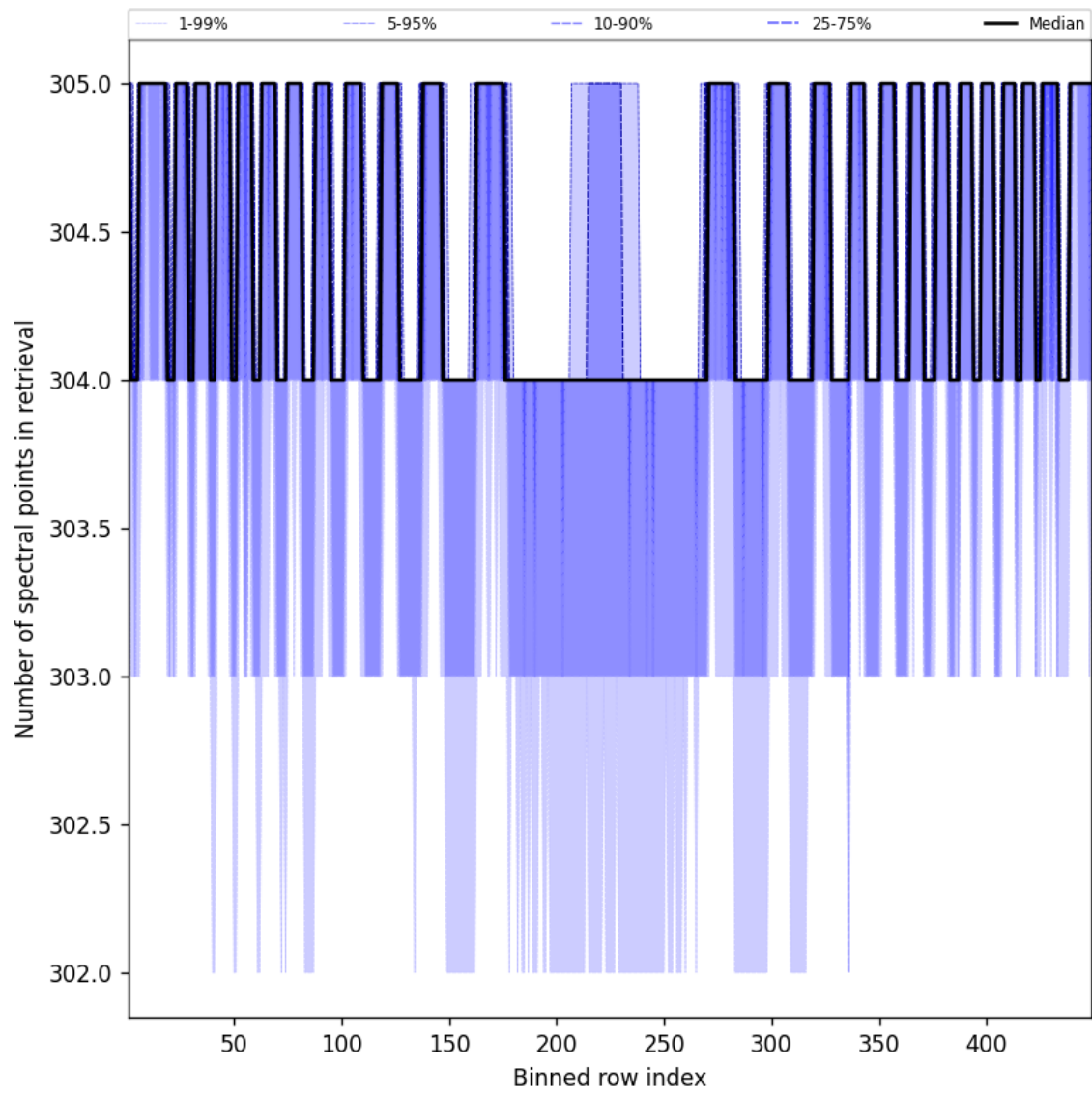
Figure 48: Along track statistics of “Number of spectral points in retrieval” for 2025-09-03 to 2025-09-04
