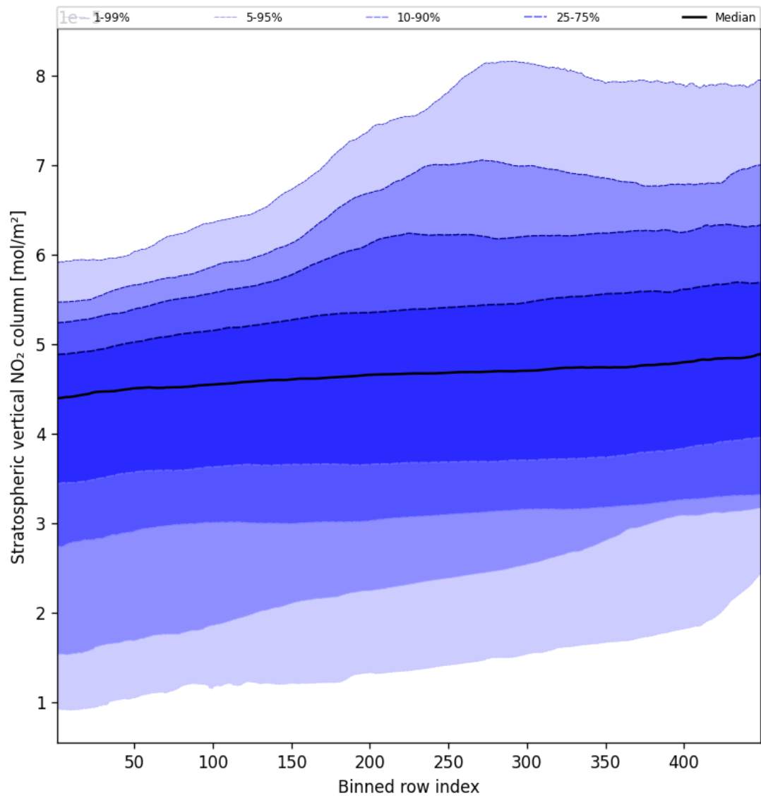
Figure 51: Along track statistics of “Stratospheric vertical NO 2 column” for 2025-09-03 to 2025-09-04
