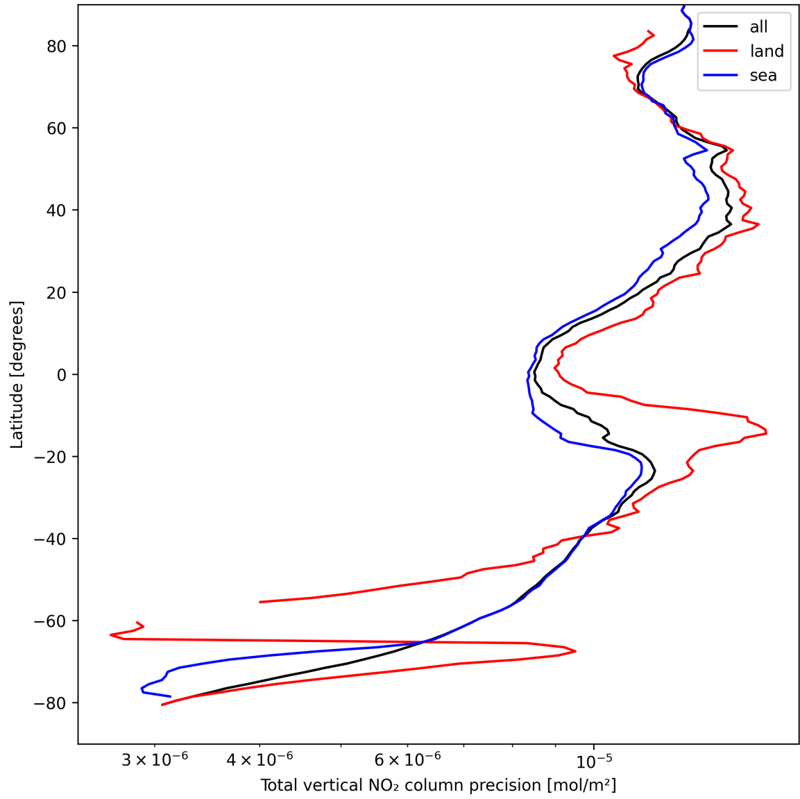
Figure 20: Zonal average of “Total vertical NO 2 column precision” for 2025-09-03 to 2025-09-04.
