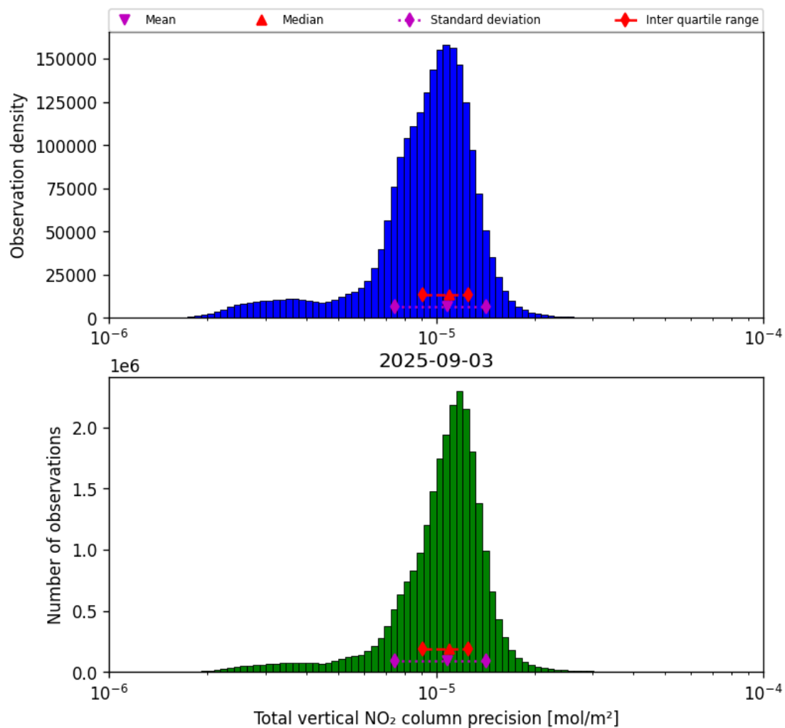
Figure 37: Histogram of "Total vertical NO 2 column precision" for 2025-09-03 to 2025-09-04
