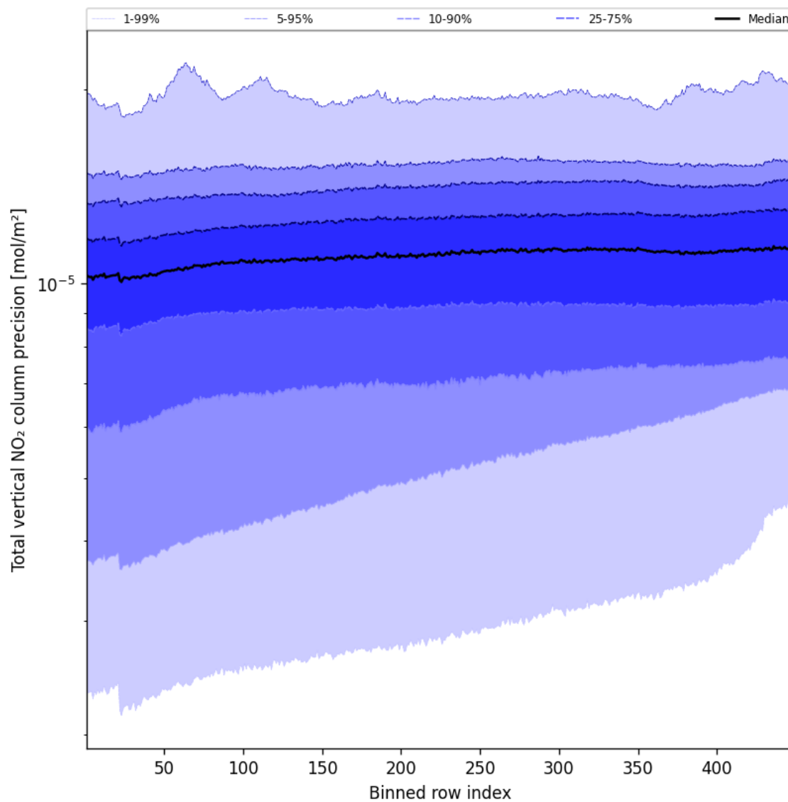
Figure 54: Along track statistics of “Total vertical NO 2 column precision” for 2025-09-03 to 2025-09-04
