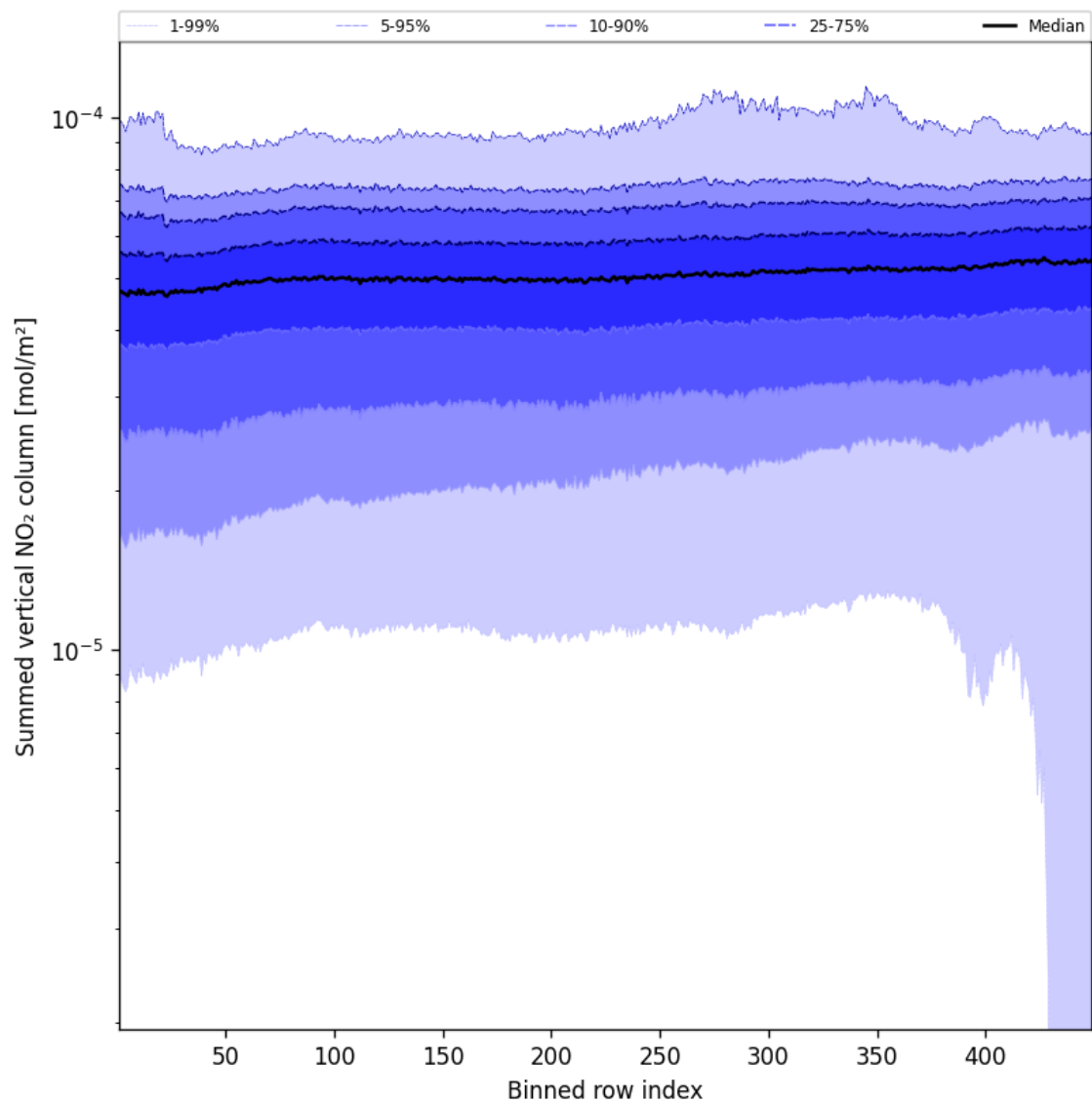
Figure 55: Along track statistics of “Summed vertical NO 2 column” for 2025-09-04 to 2025-09-05
