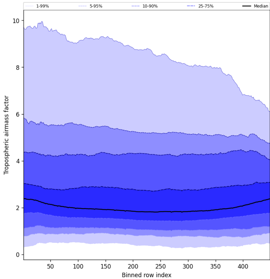
Figure 46: Along track statistics of “Tropospheric airmass factor” for 2025-09-04 to 2025-09-05
