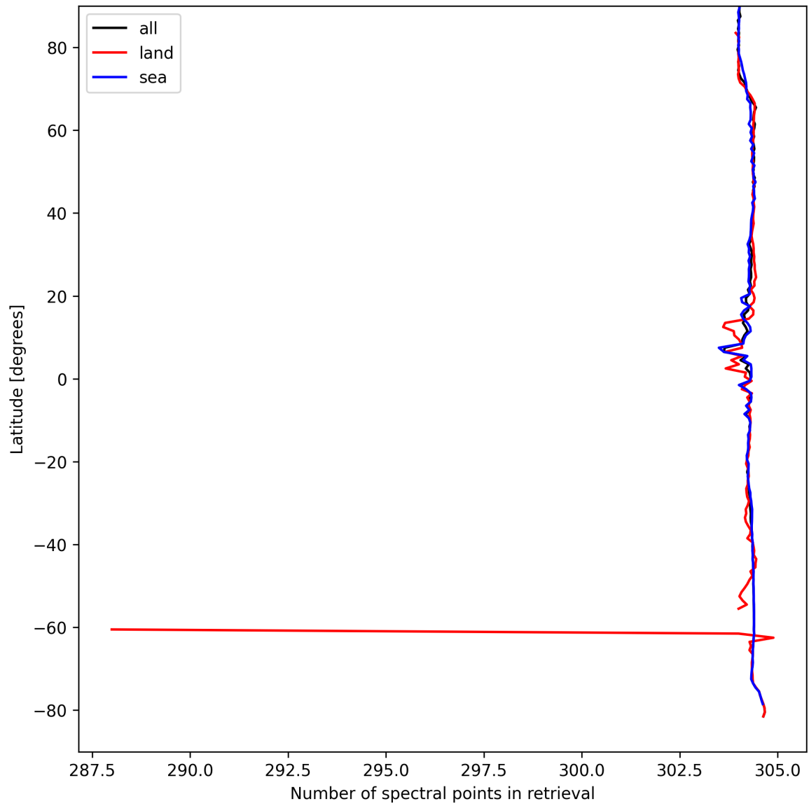
Figure 14: Zonal average of “Number of spectral points in retrieval” for 2025-09-04 to 2025-09-05.
