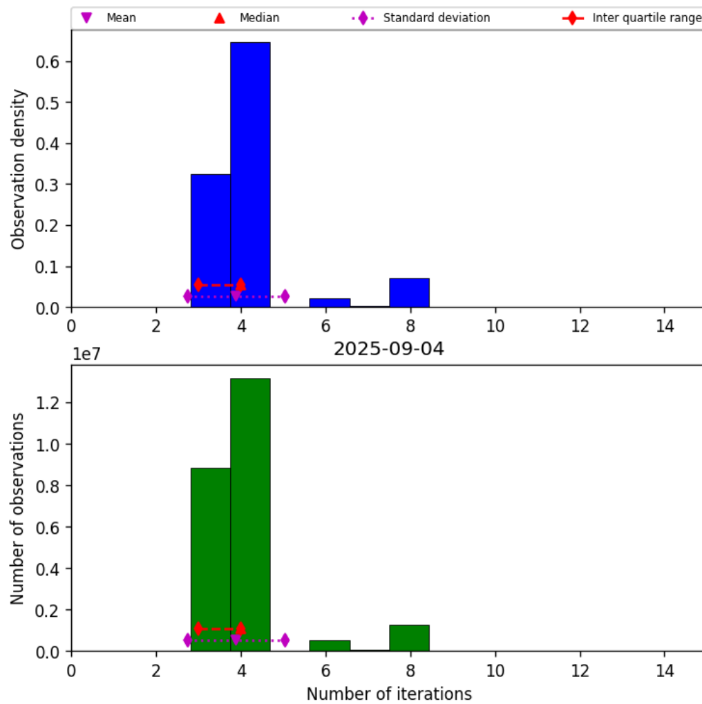
Figure 32: Histogram of “Number of iterations” for 2025-09-04 to 2025-09-05
