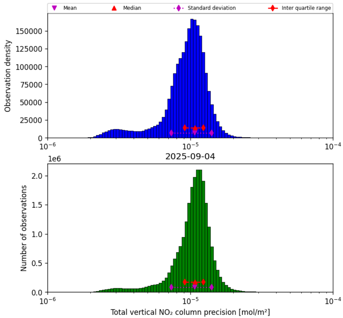
Figure 37: Histogram of “Total vertical NO 2 column precision” for 2025-09-04 to 2025-09-05
