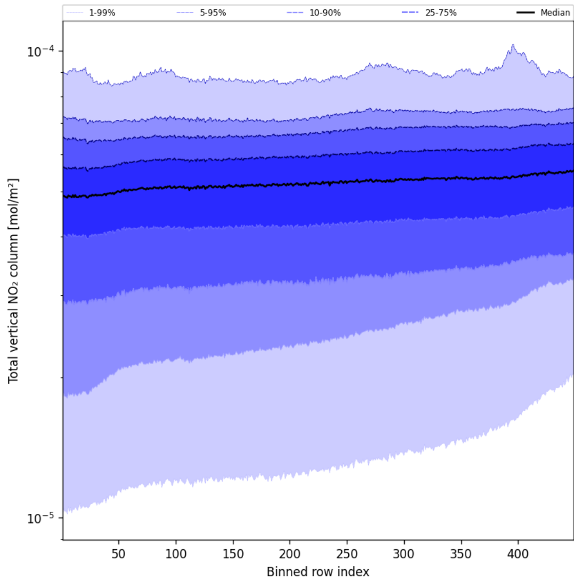
Figure 53: Along track statistics of “Total vertical NO 2 column” for 2025-09-04 to 2025-09-05
