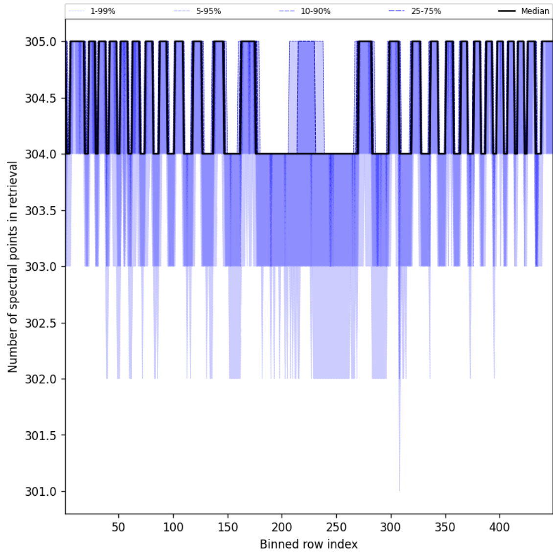
Figure 48: Along track statistics of “Number of spectral points in retrieval” for 2025-09-04 to 2025-09-05
