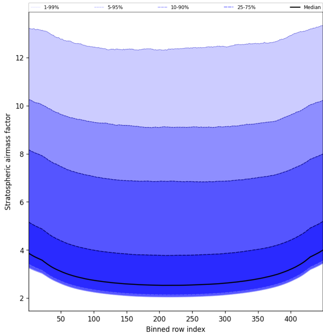
Figure 59: Along track statistics of “Stratospheric airmass factor” for 2025-09-04 to 2025-09-05
