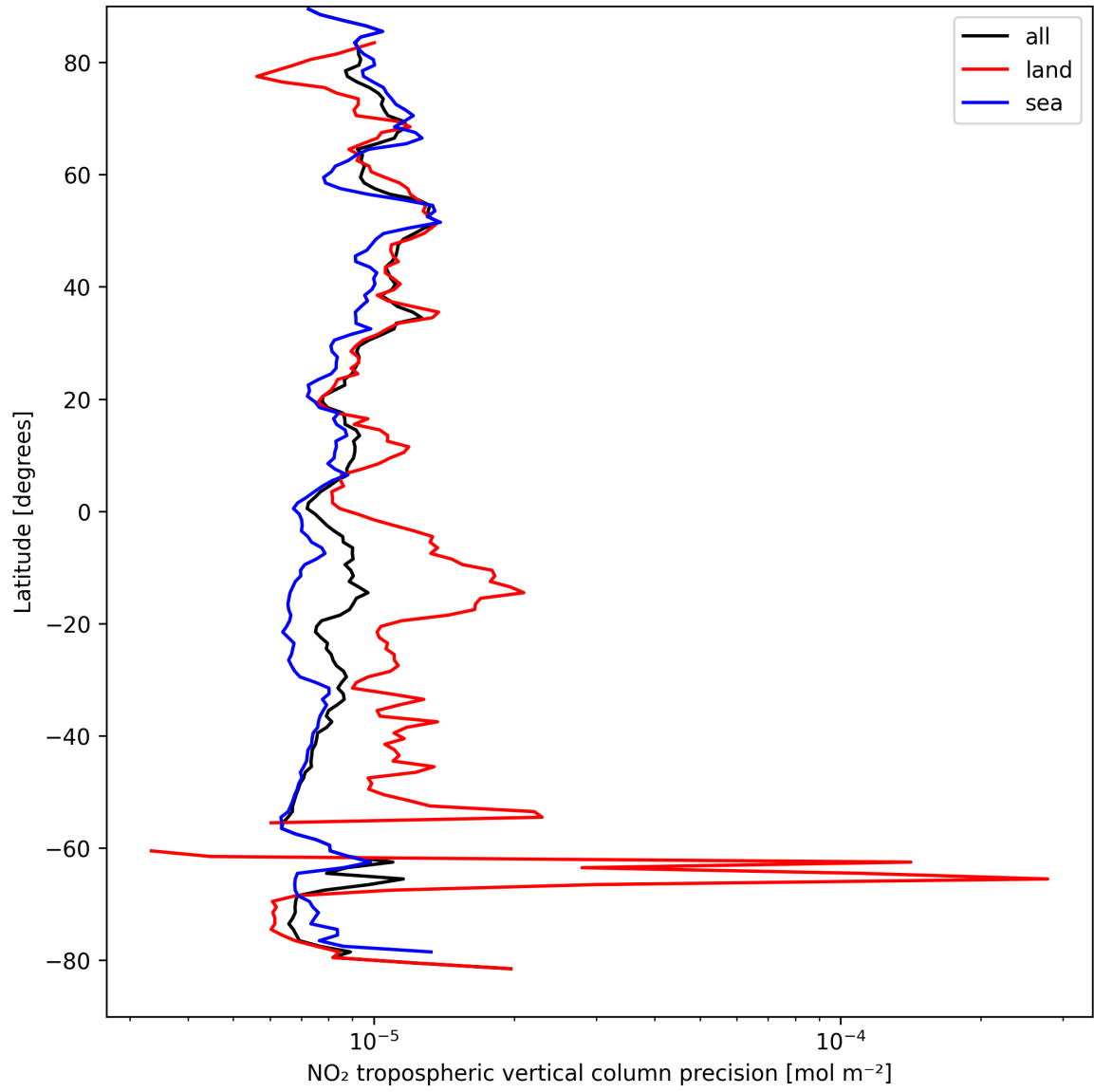
Figure 11: Zonal average of “NO 2 tropospheric vertical column precision” for 2025-09-04 to 2025-09-05.
