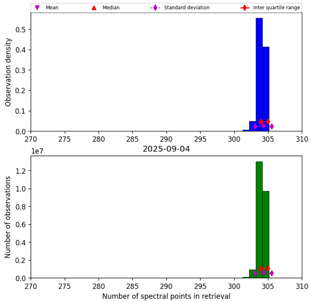
Figure 31: Histogram of “Number of spectral points in retrieval” for 2025-09-04 to 2025-09-05
