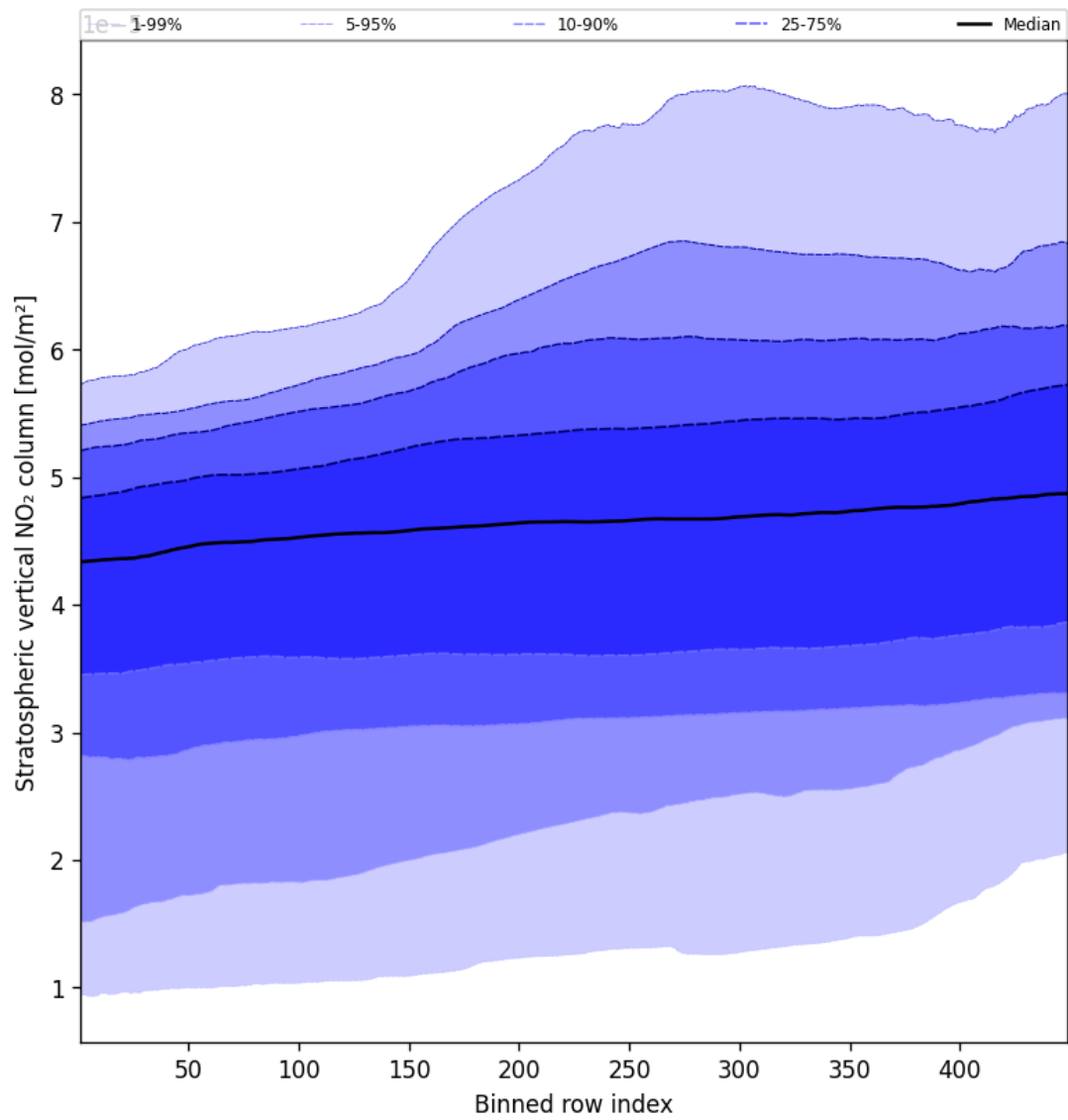
Figure 51: Along track statistics of “Stratospheric vertical NO 2 column” for 2025-09-04 to 2025-09-05
