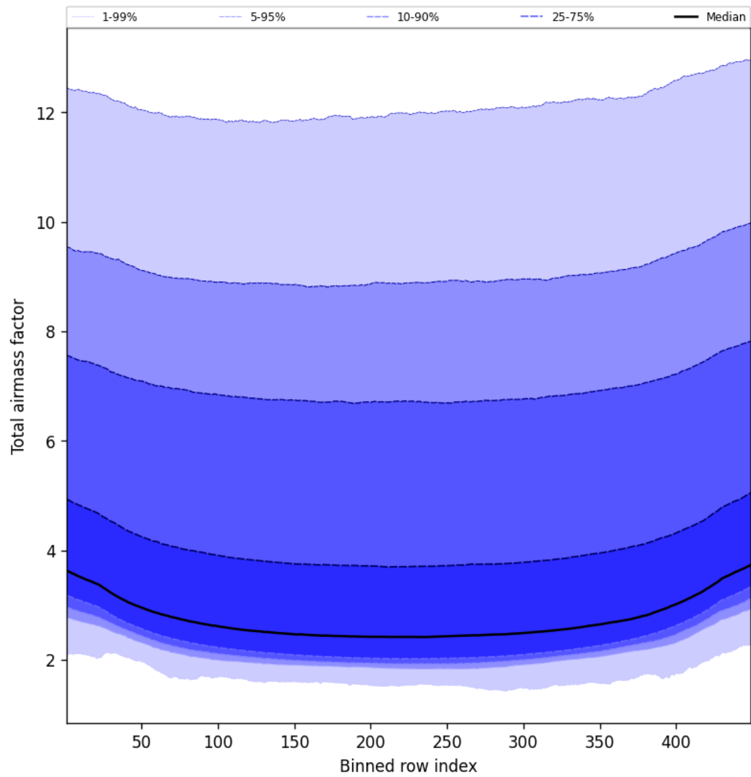
Figure 47: Along track statistics of “Total airmass factor” for 2025-09-04 to 2025-09-05
