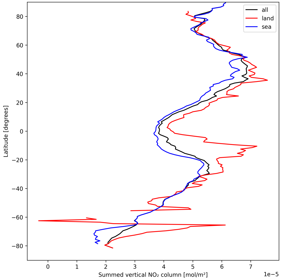
Figure 21: Zonal average of “Summed vertical NO 2 column” for 2025-09-04 to 2025-09-05.
