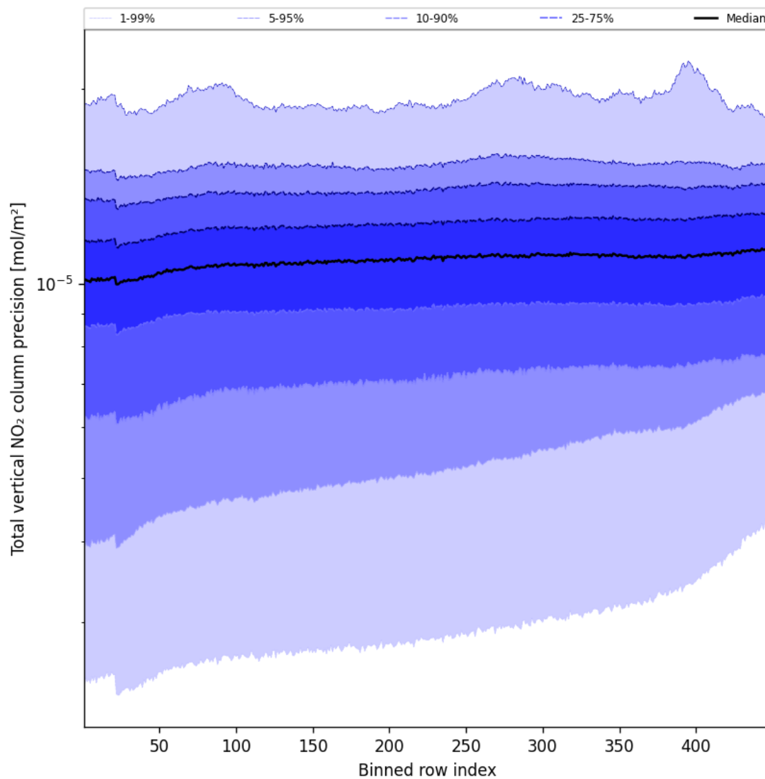
Figure 54: Along track statistics of “Total vertical NO 2 column precision” for 2025-09-04 to 2025-09-05
