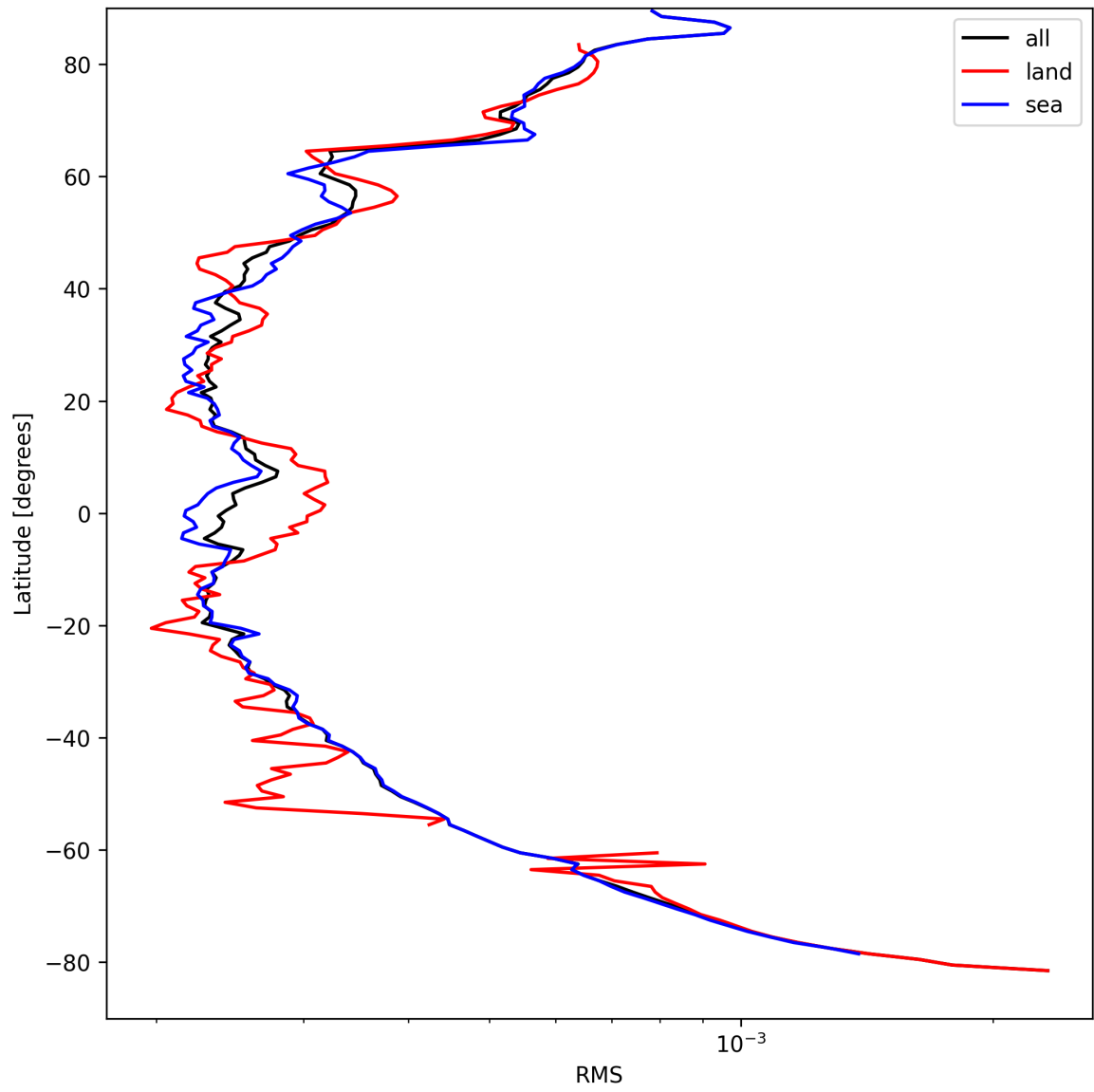
Figure 24: Zonal average of “RMS” for 2025-09-04 to 2025-09-05.
