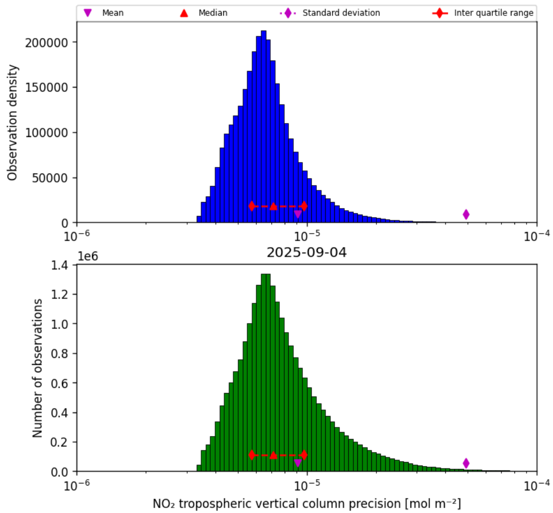
Figure 28: Histogram of “NO 2 tropospheric vertical column precision” for 2025-09-04 to 2025-09-05
