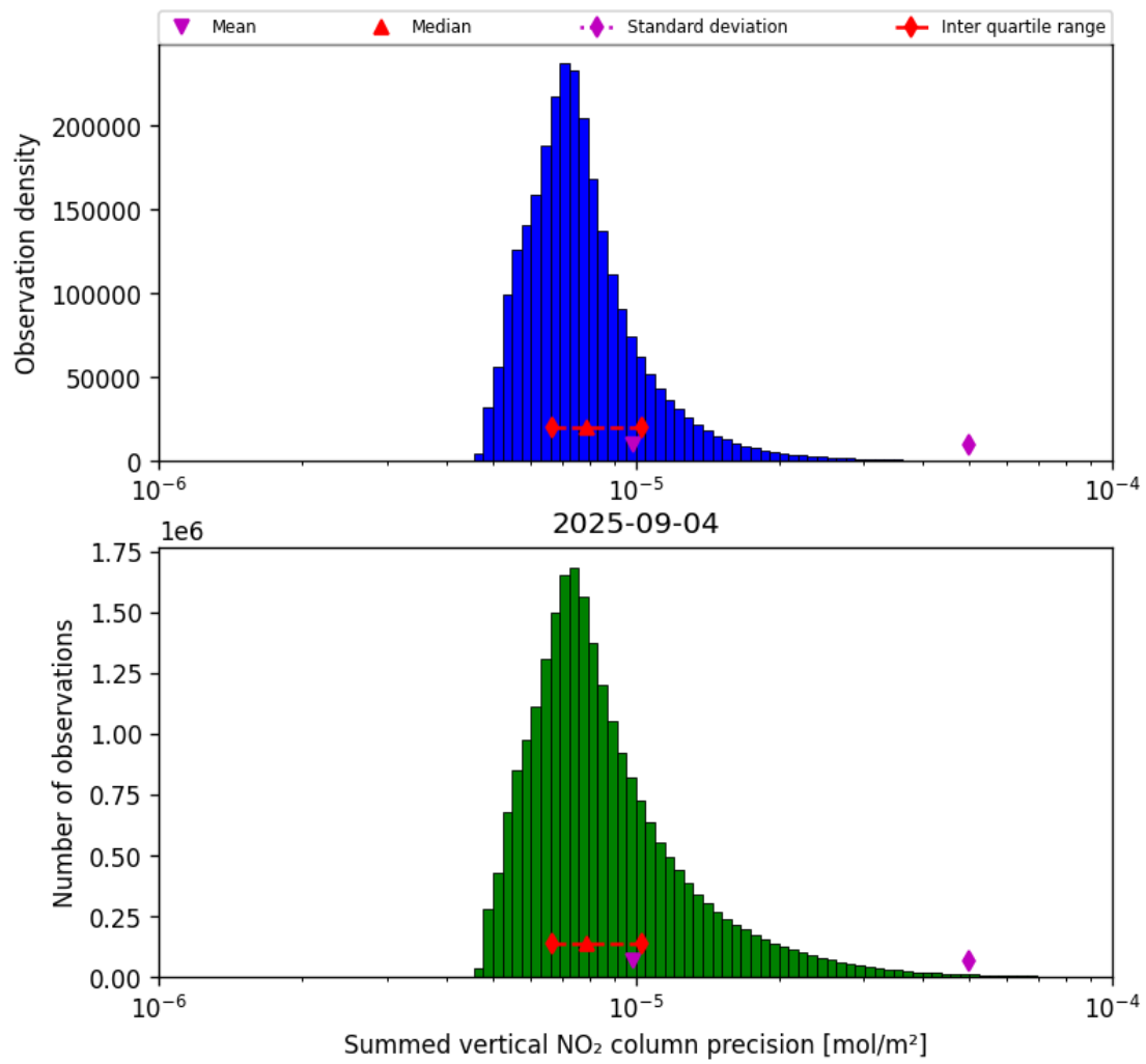
Figure 39: Histogram of “Summed vertical NO 2 column precision” for 2025-09-04 to 2025-09-05
