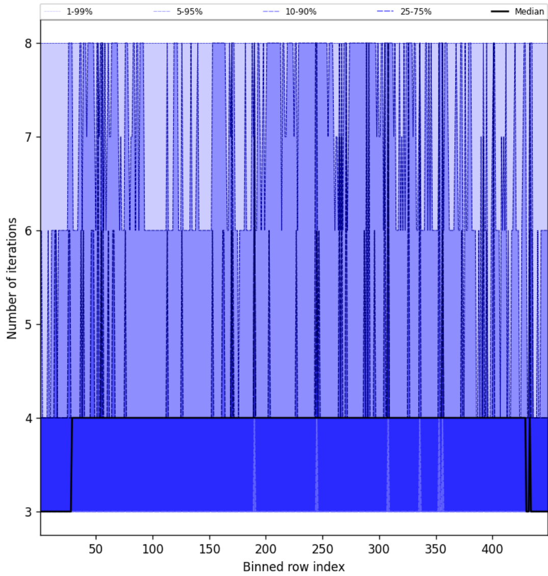
Figure 49: Along track statistics of “Number of iterations” for 2025-09-04 to 2025-09-05
