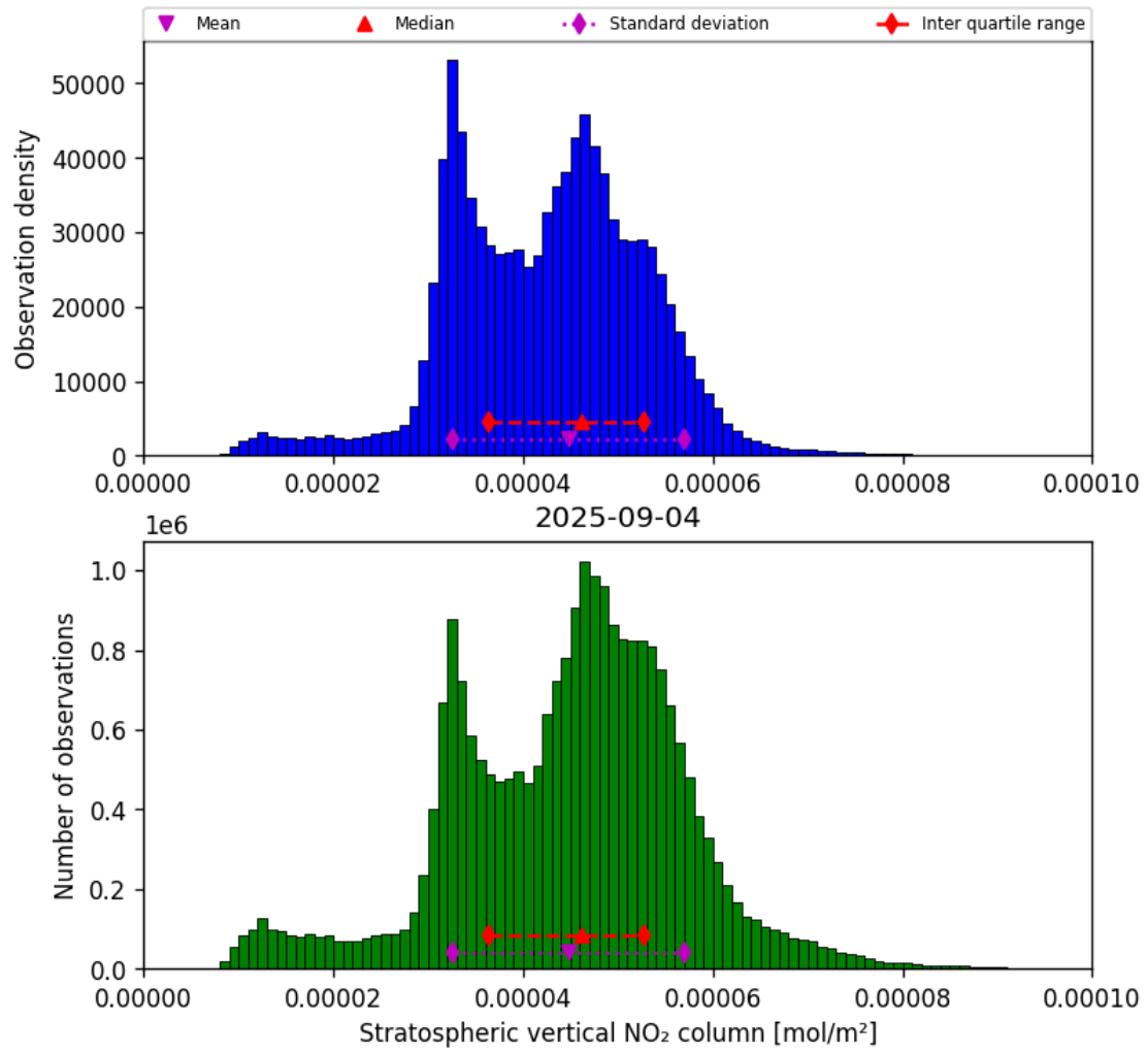
Figure 34: Histogram of “Stratospheric vertical NO 2 column” for 2025-09-04 to 2025-09-05
