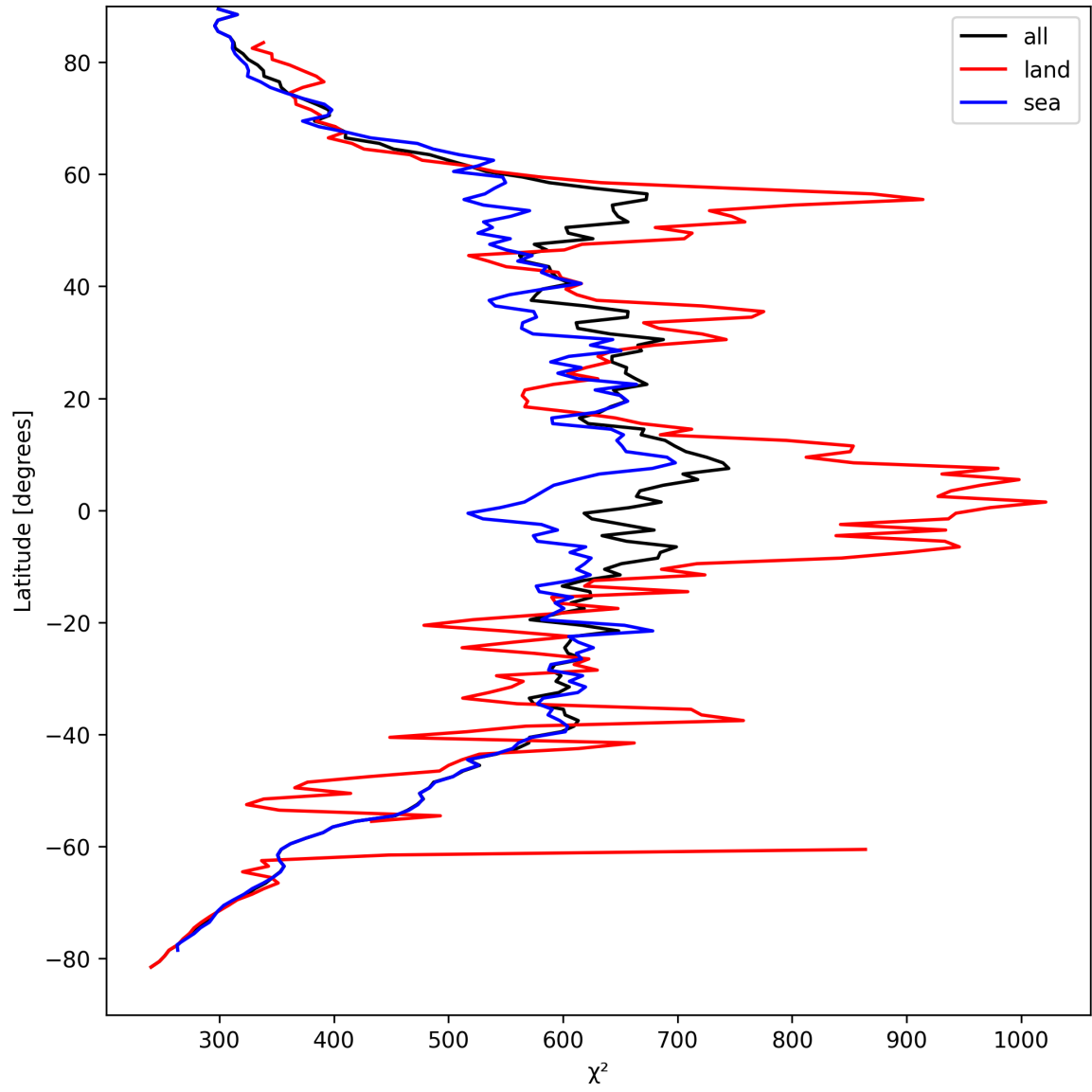
Figure 23: Zonal average of “ \chi^2 ” for 2025-09-04 to 2025-09-05.
