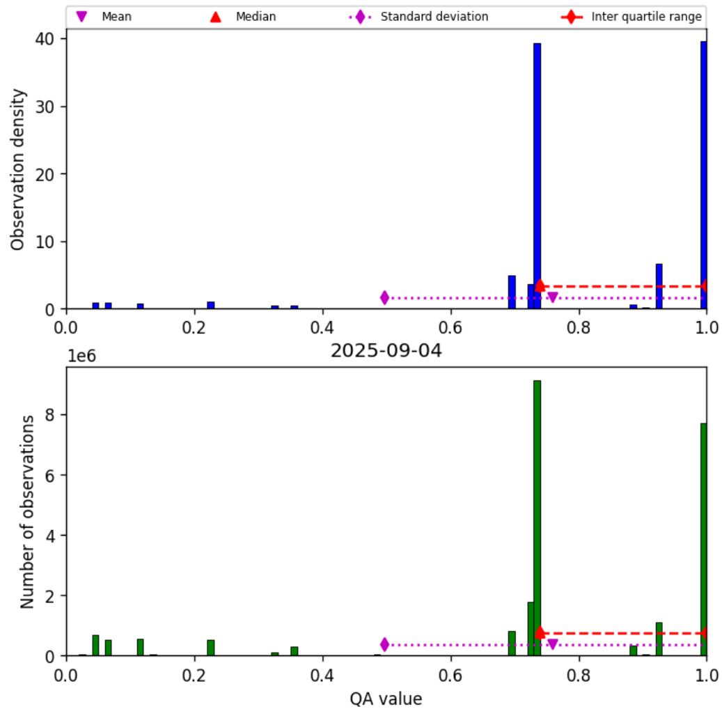
Figure 26: Histogram of “QA value” for 2025-09-04 to 2025-09-05
