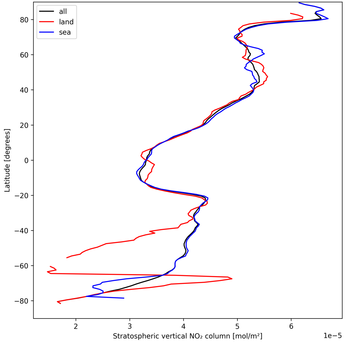
Figure 17: Zonal average of “Stratospheric vertical NO 2 column” for 2025-09-04 to 2025-09-05.
