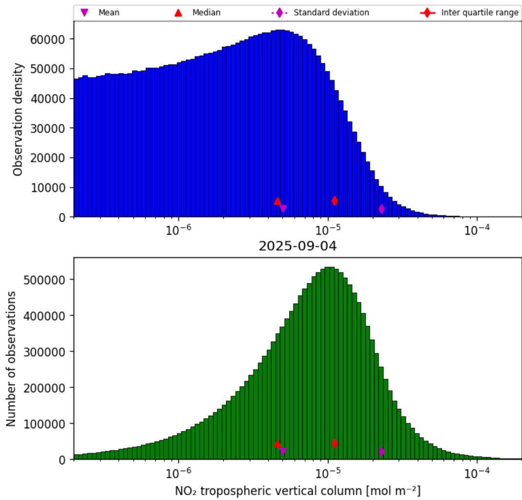
Figure 27: Histogram of “NO 2 tropospheric vertical column” for 2025-09-04 to 2025-09-05
