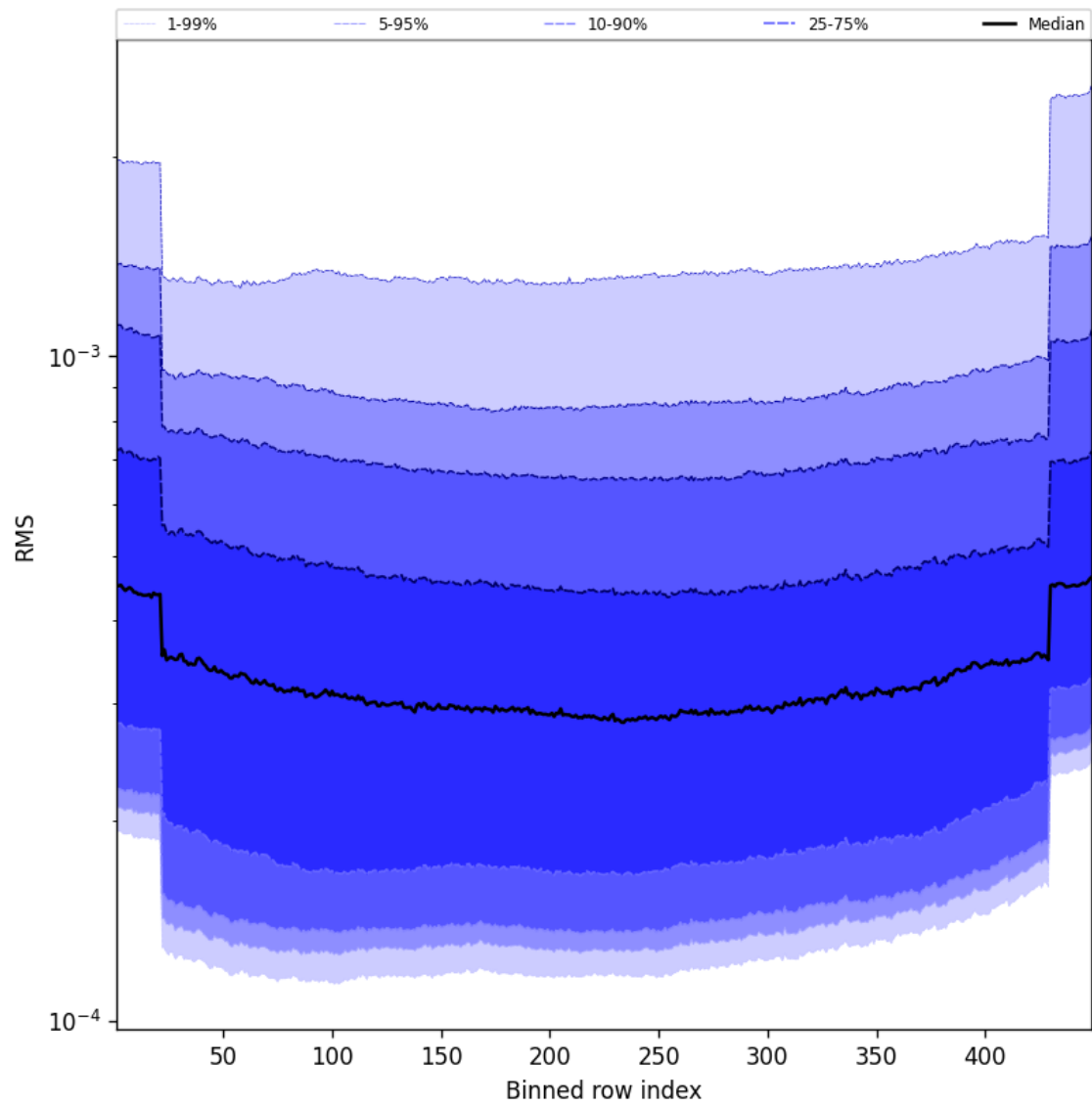
Figure 58: Along track statistics of “RMS” for 2025-09-04 to 2025-09-05
