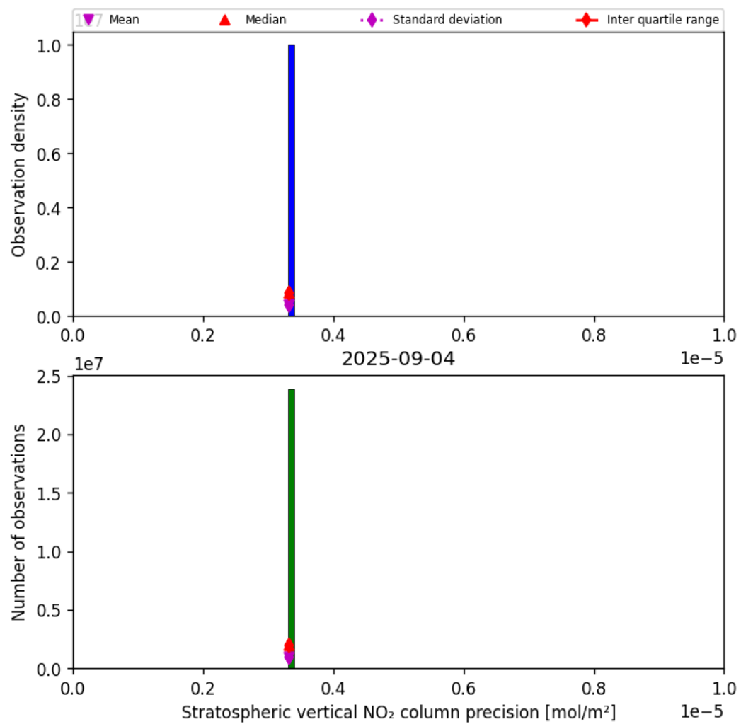
Figure 35: Histogram of “Stratospheric vertical NO 2 column precision” for 2025-09-04 to 2025-09-05
