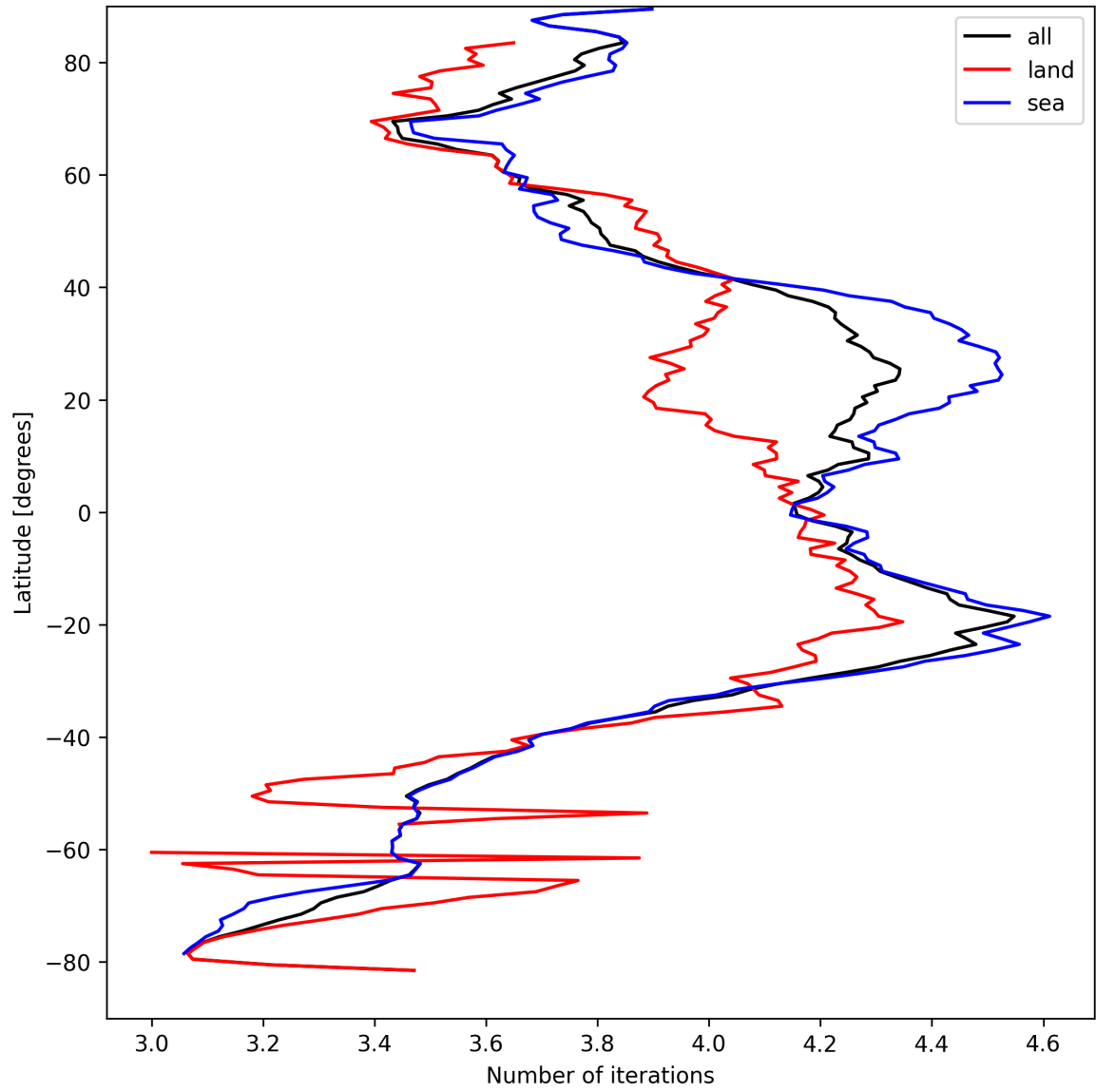
Figure 15: Zonal average of “Number of iterations” for 2025-09-04 to 2025-09-05.
