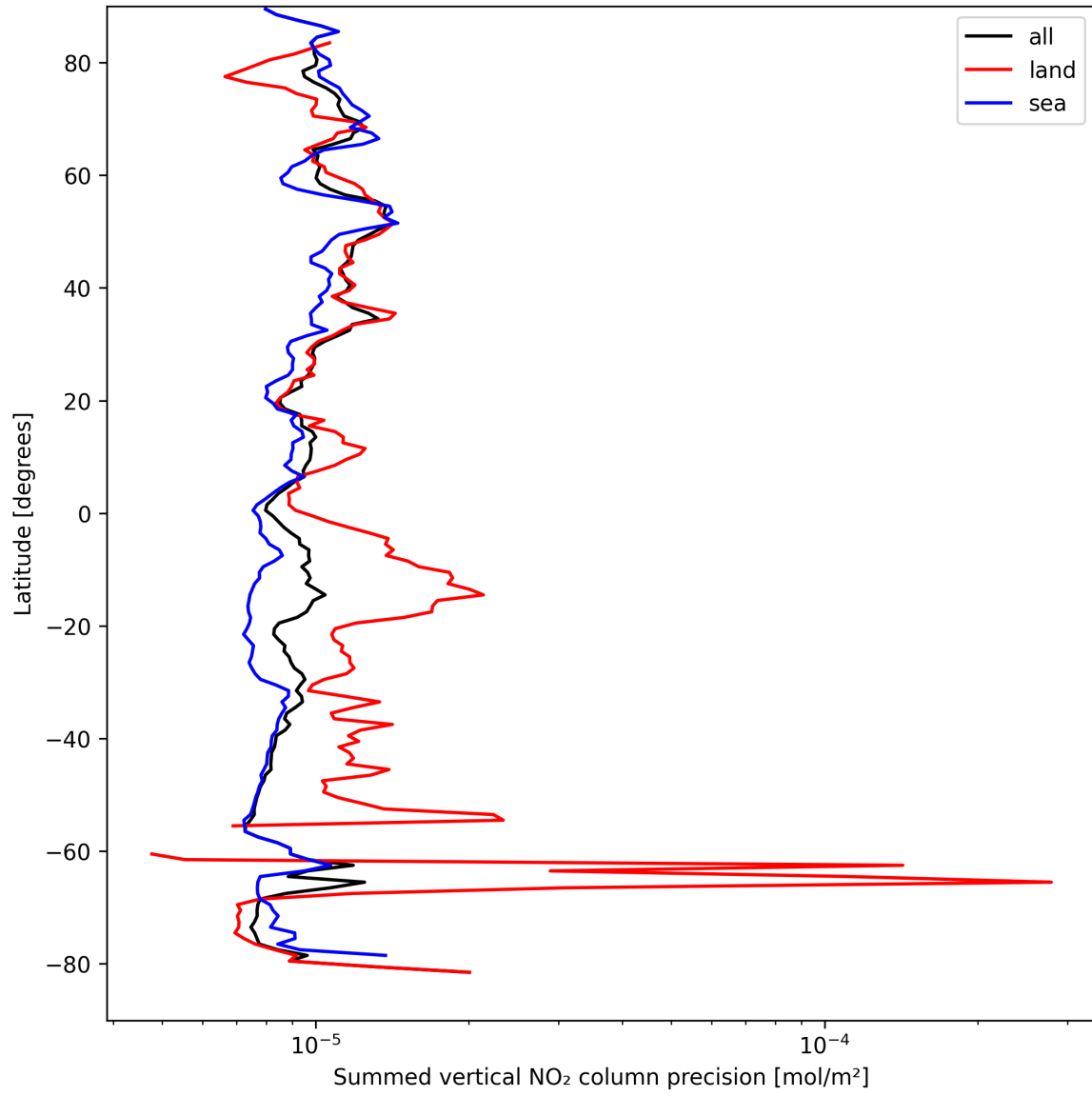
Figure 22: Zonal average of “Summed vertical NO 2 column precision” for 2025-09-04 to 2025-09-05.
