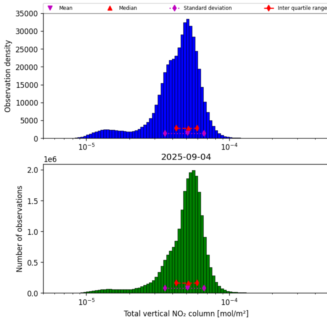
Figure 36: Histogram of “Total vertical NO 2 column” for 2025-09-04 to 2025-09-05
