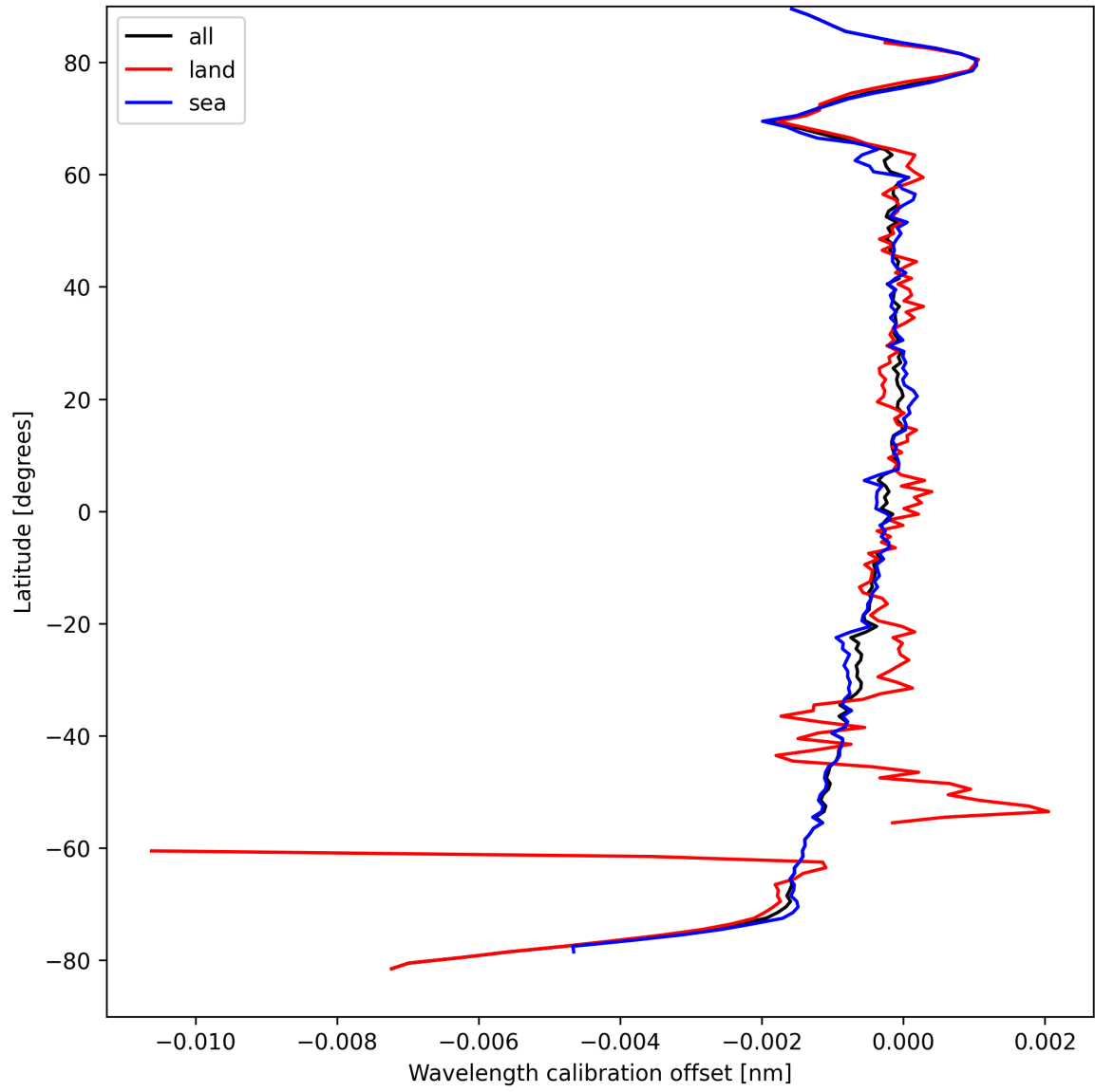
Figure 16: Zonal average of “Wavelength calibration offset” for 2025-09-04 to 2025-09-05.
