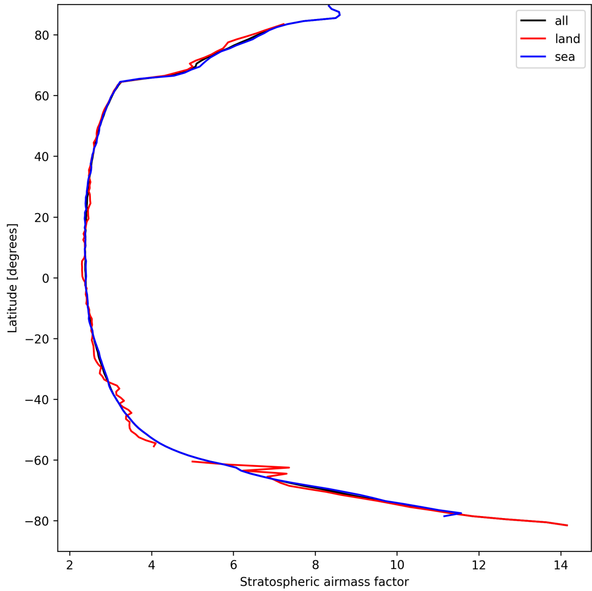
Figure 25: Zonal average of “Stratospheric air mass factor” for 2025-09-04 to 2025-09-05.
