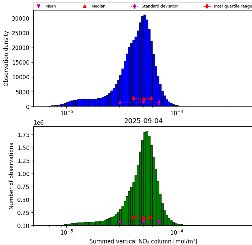
Figure 38: Histogram of “Summed vertical NO 2 column” for 2025-09-04 to 2025-09-05
