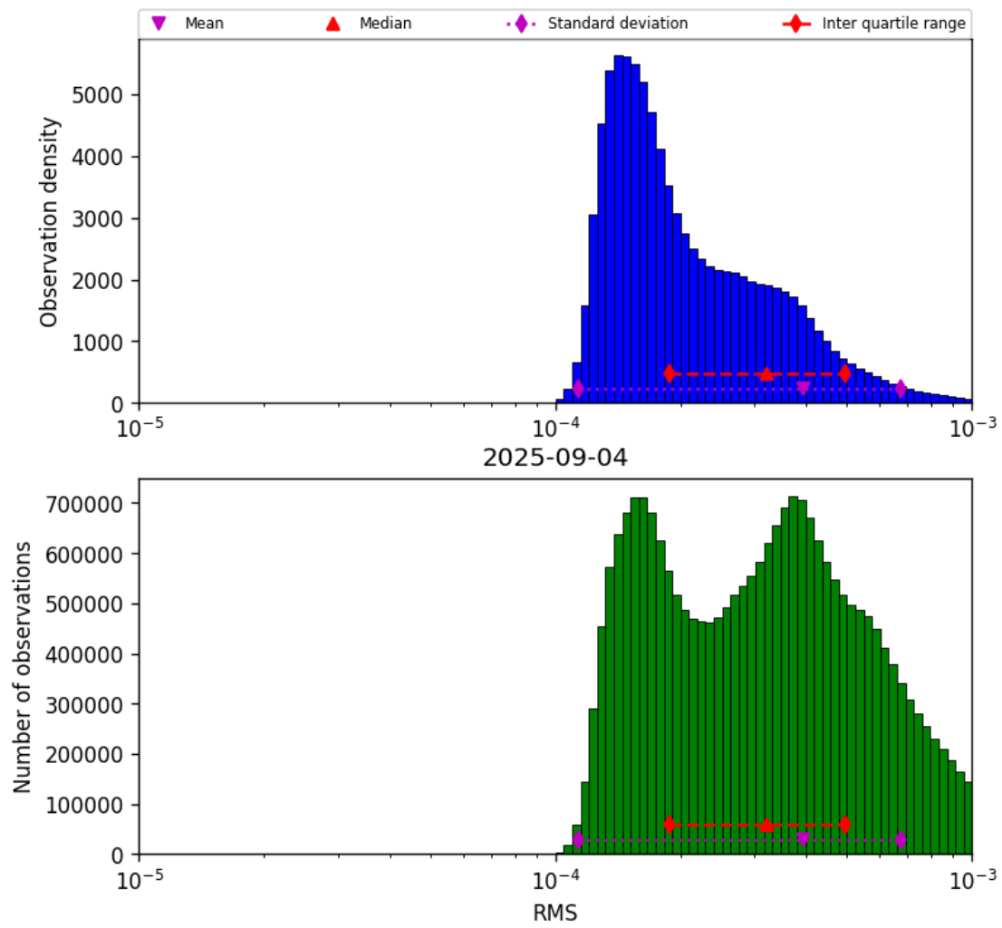
Figure 41: Histogram of “RMS” for 2025-09-04 to 2025-09-05
