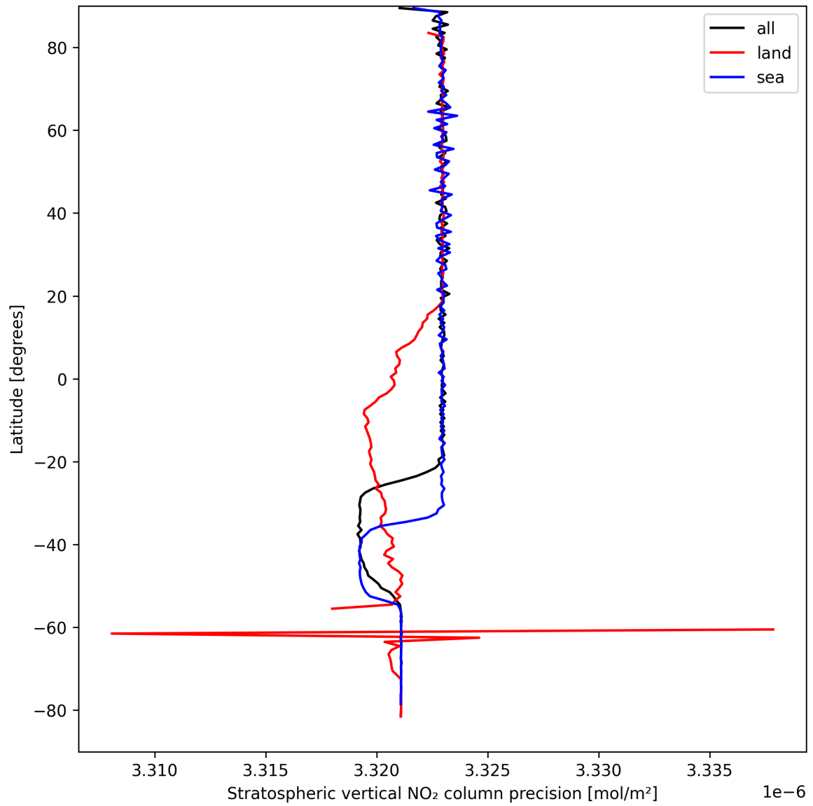
Figure 18: Zonal average of “Stratospheric vertical NO 2 column precision” for 2025-09-04 to 2025-09-05.
