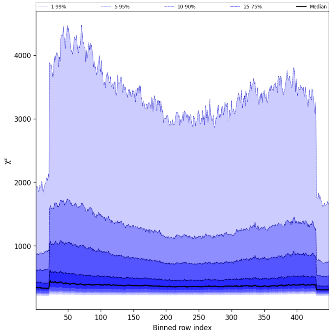
Figure 57: Along track statistics of “ \chi^2 ” for 2025-09-04 to 2025-09-05
