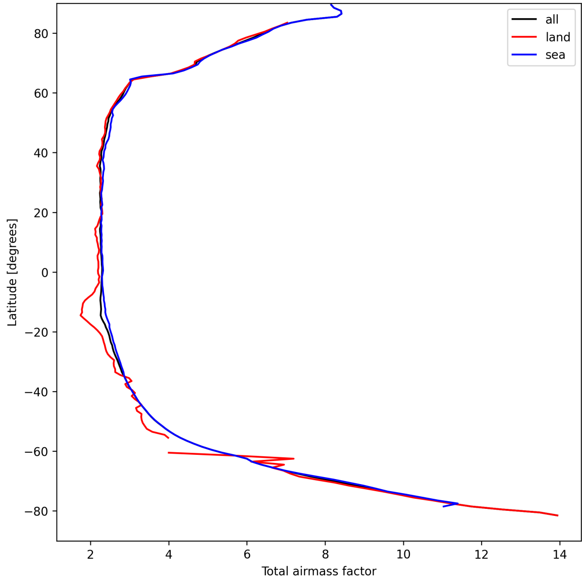
Figure 13: Zonal average of “Total airmass factor” for 2025-09-04 to 2025-09-05.
