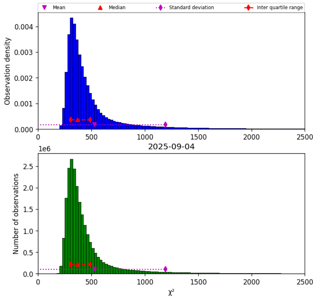
Figure 40: Histogram of “ \chi^2 ” for 2025-09-04 to 2025-09-05
