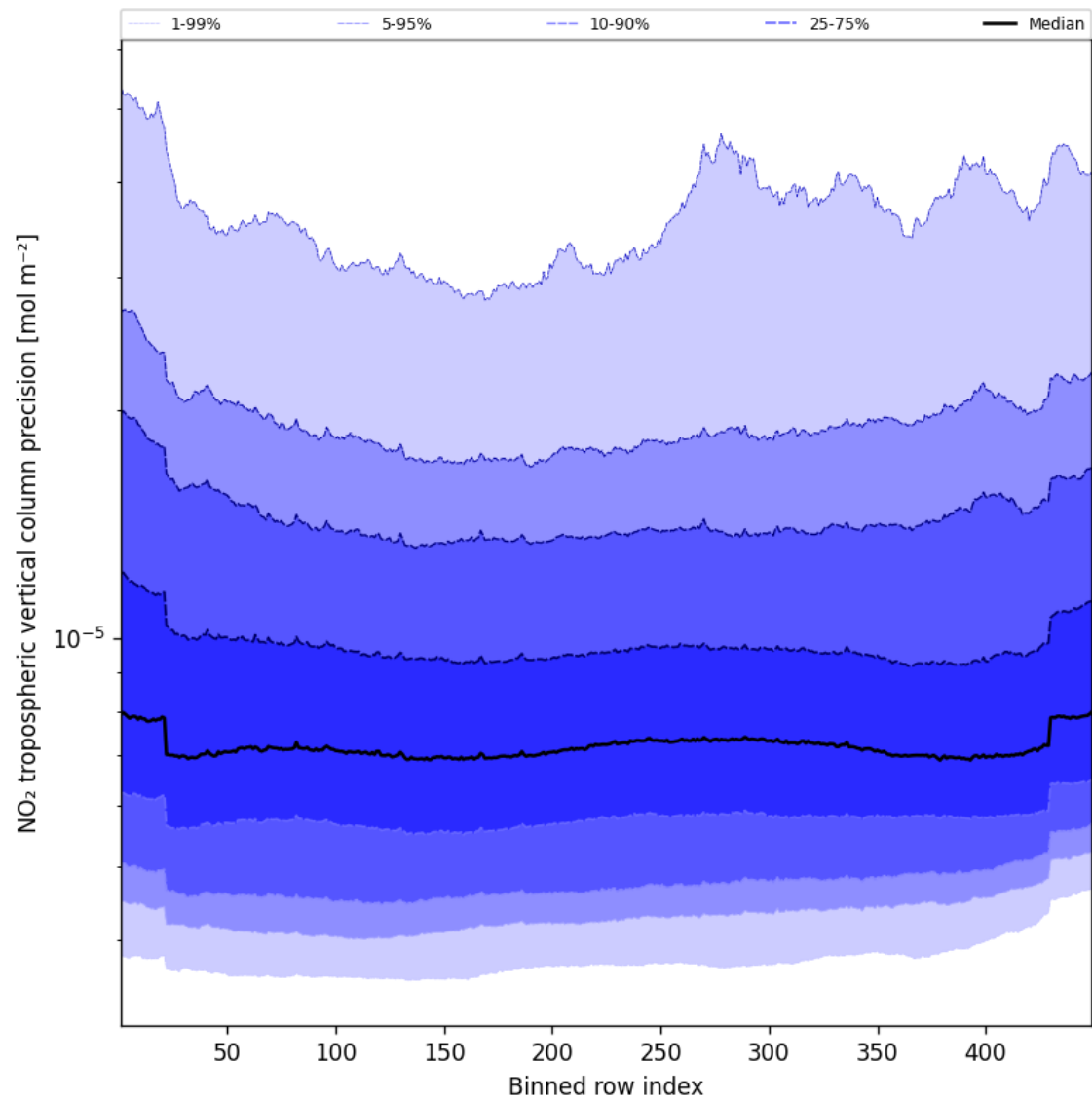
Figure 45: Along track statistics of “NO 2 tropospheric vertical column precision” for 2025-09-04 to 2025-09-05
