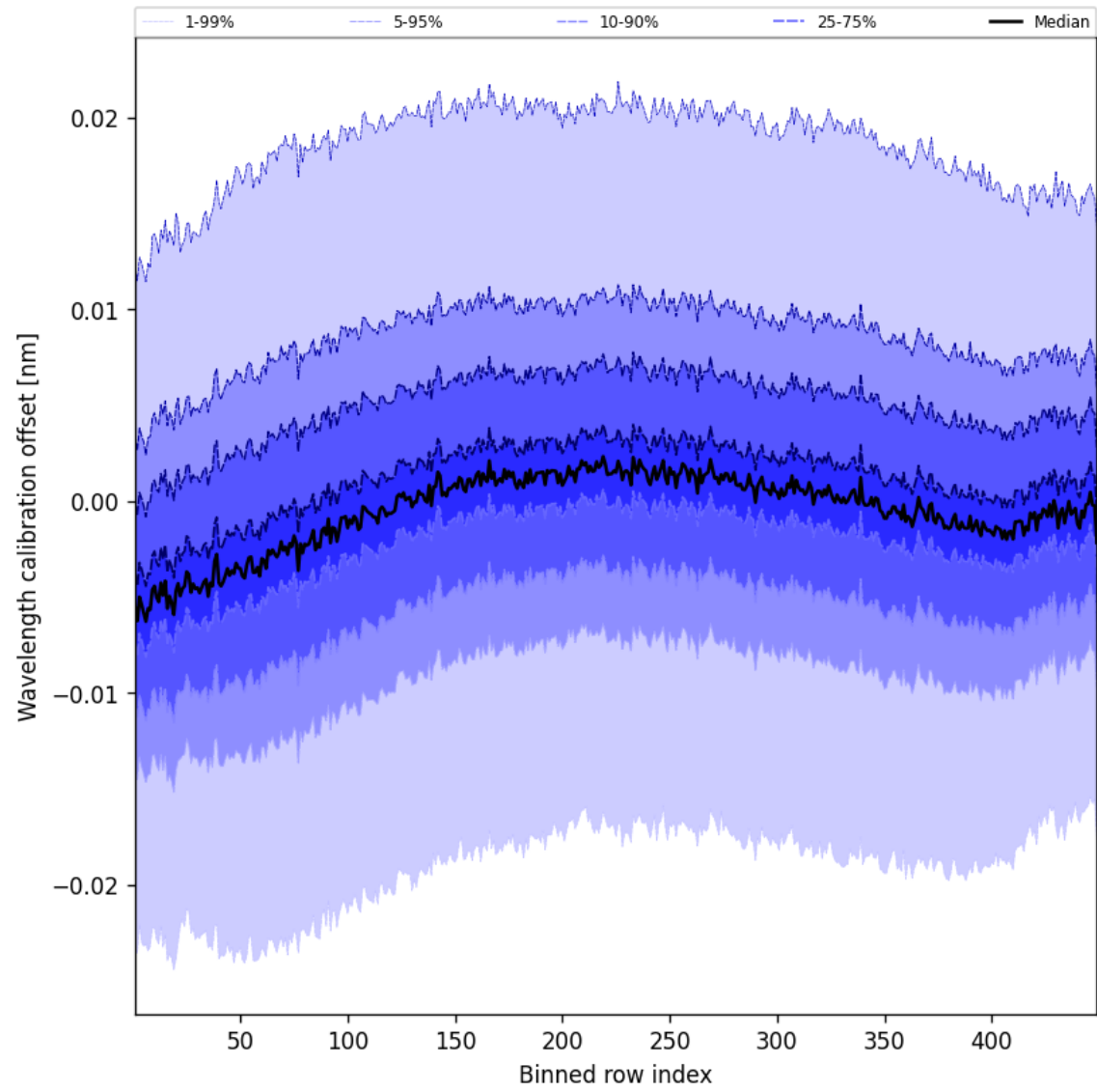
Figure 50: Along track statistics of “Wavelength calibration offset” for 2025-09-04 to 2025-09-05
