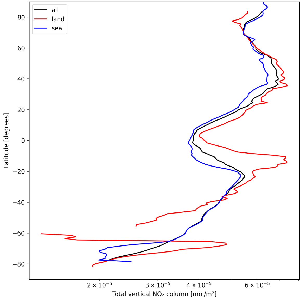
Figure 19: Zonal average of “Total vertical NO 2 column” for 2025-09-04 to 2025-09-05.
