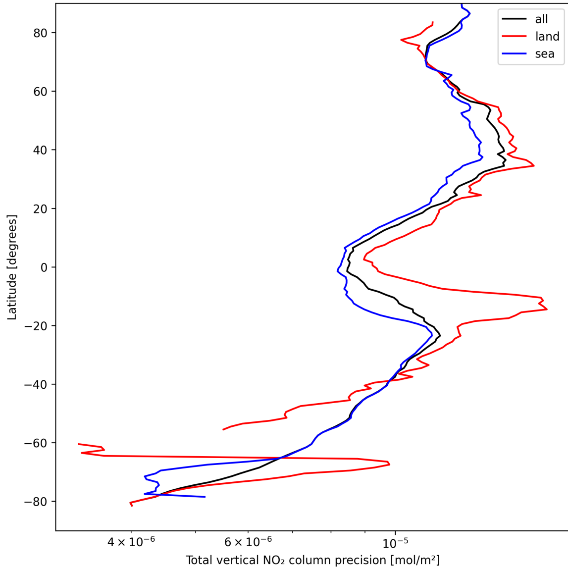
Figure 20: Zonal average of “Total vertical NO 2 column precision” for 2025-09-04 to 2025-09-05.
