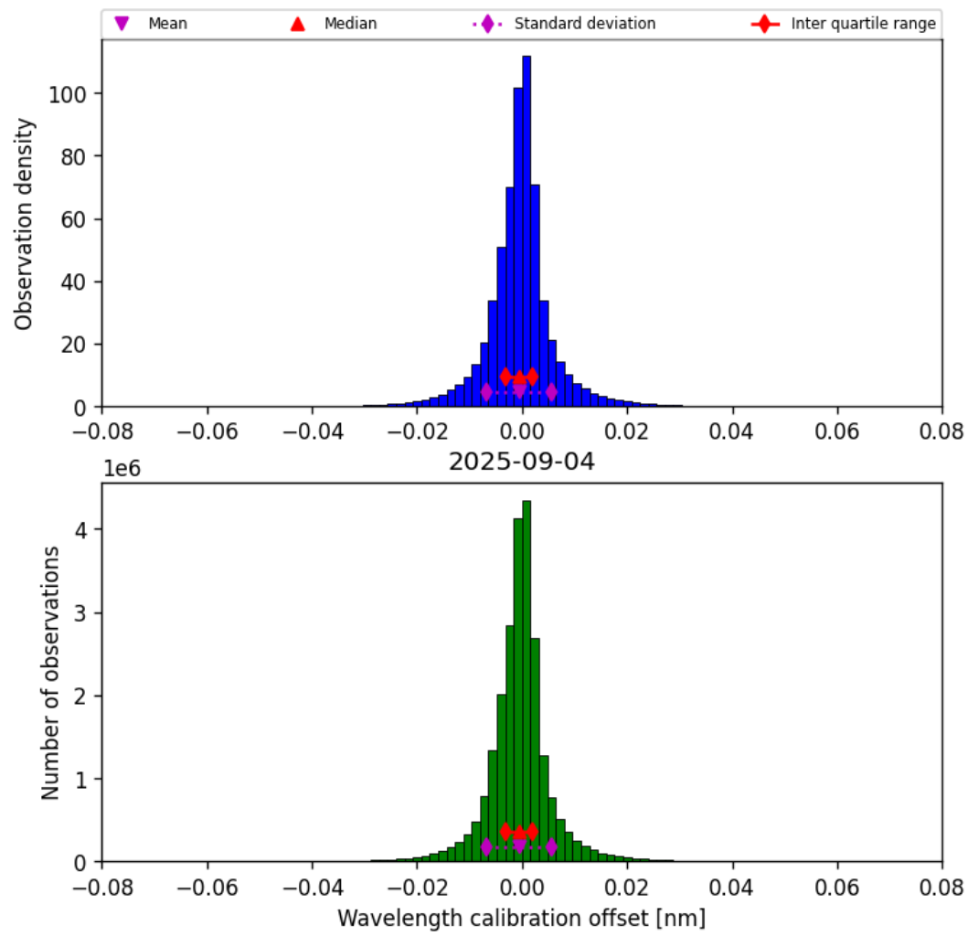
Figure 33: Histogram of “Wavelength calibration offset” for 2025-09-04 to 2025-09-05
