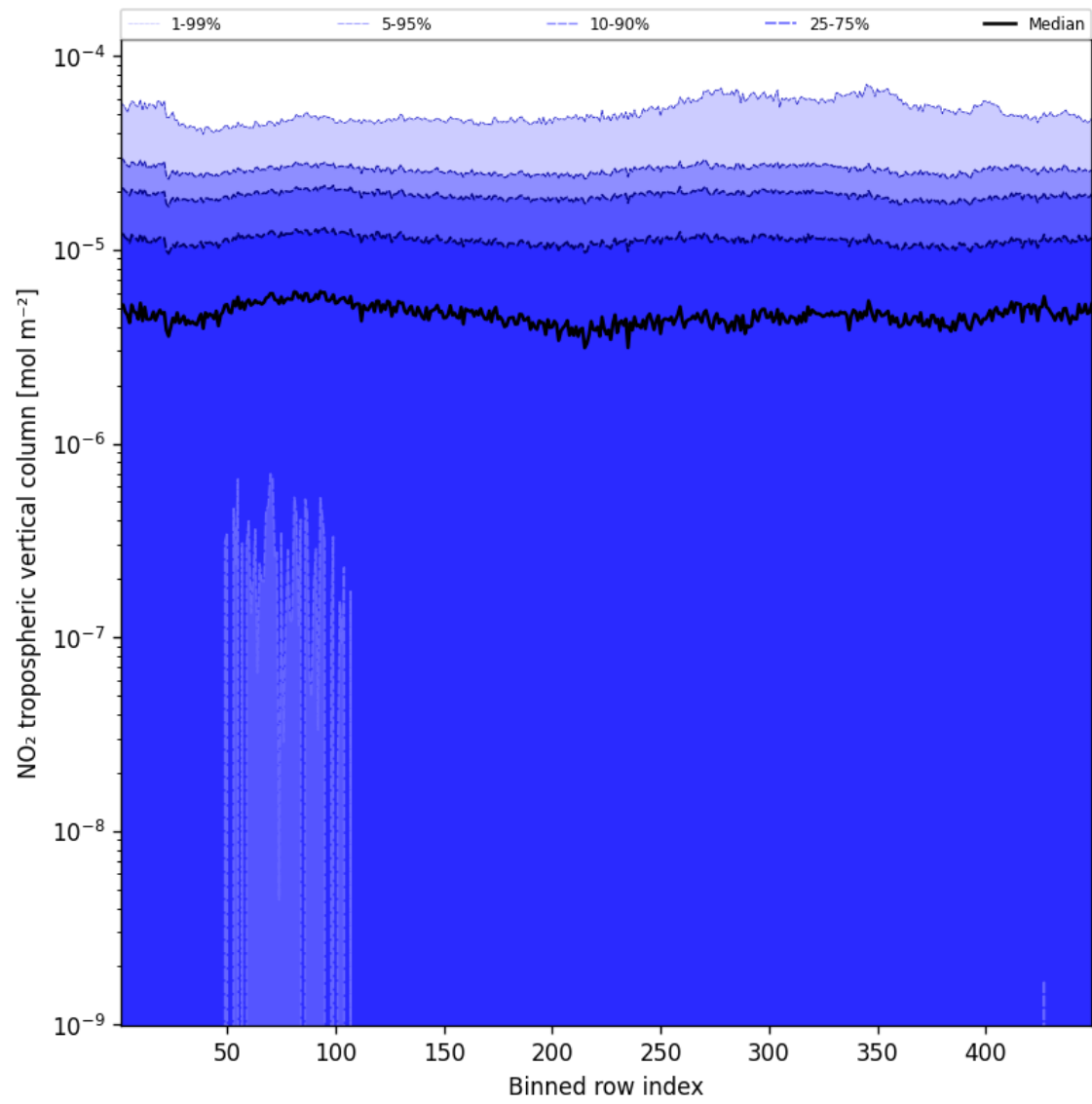
Figure 44: Along track statistics of “NO 2 tropospheric vertical column” for 2025-09-04 to 2025-09-05
