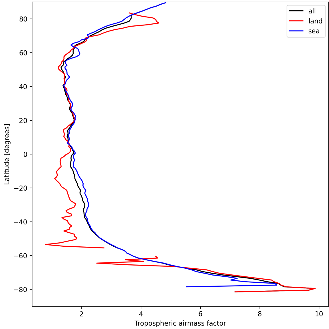
Figure 12: Zonal average of “Tropospheric airmass factor” for 2025-09-04 to 2025-09-05.
