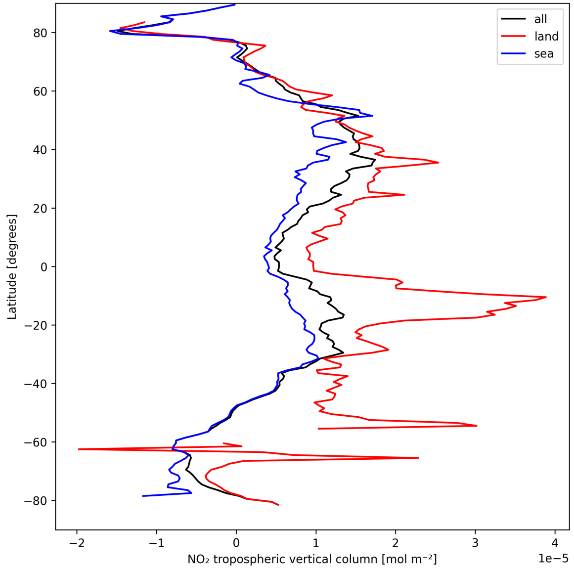
Figure 10: Zonal average of “NO 2 tropospheric vertical column” for 2025-09-04 to 2025-09-05.
