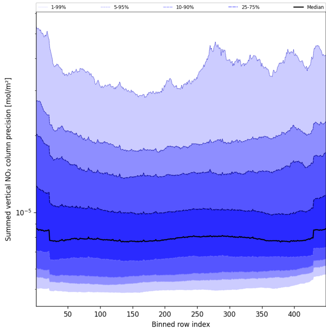
Figure 56: Along track statistics of “Summed vertical NO 2 column precision” for 2025-09-04 to 2025-09-05
