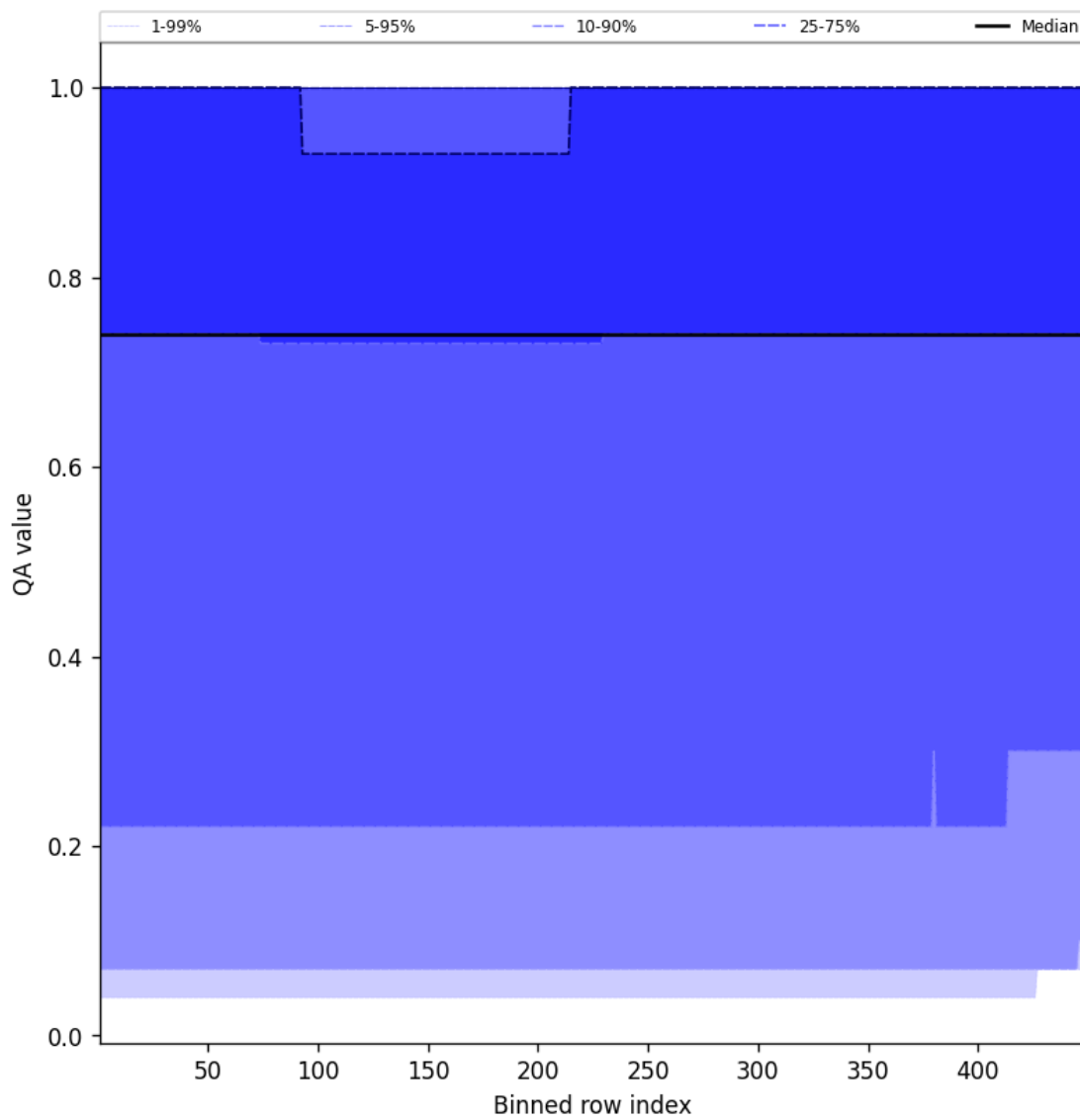
Figure 43: Along track statistics of “QA value” for 2025-09-04 to 2025-09-05
