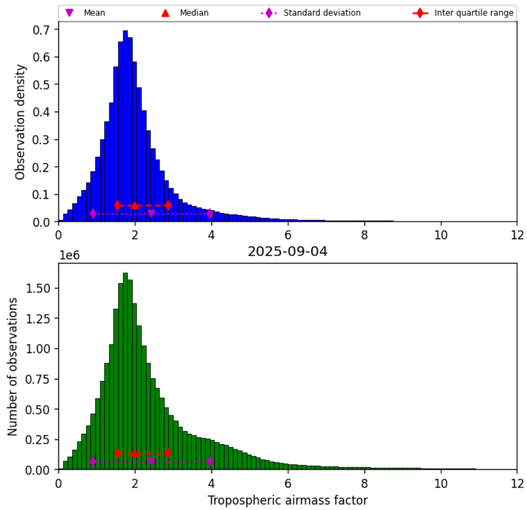
Figure 29: Histogram of “Tropospheric airmass factor” for 2025-09-04 to 2025-09-05
