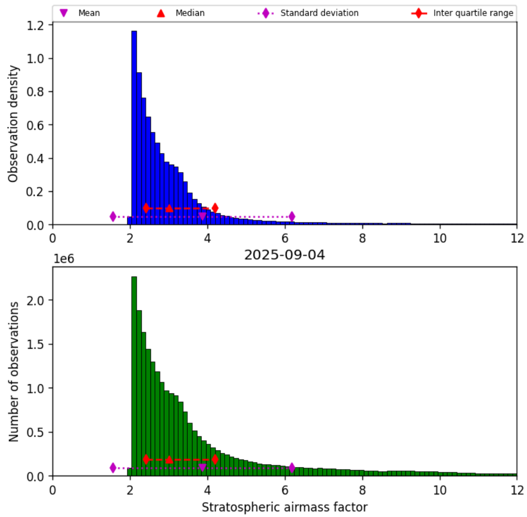
Figure 42: Histogram of “Stratospheric airmass factor” for 2025-09-04 to 2025-09-05
