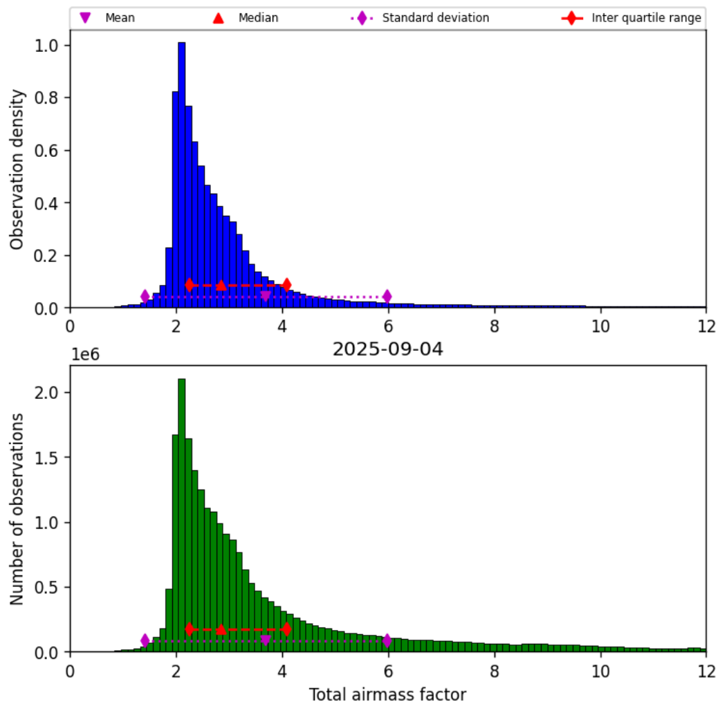
Figure 30: Histogram of “Total airmass factor” for 2025-09-04 to 2025-09-05
