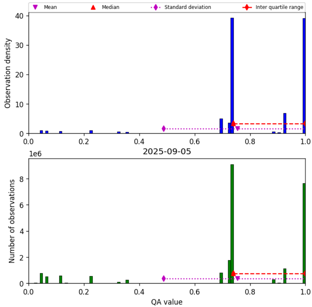
Figure 26: Histogram of “QA value” for 2025-09-05 to 2025-09-06
