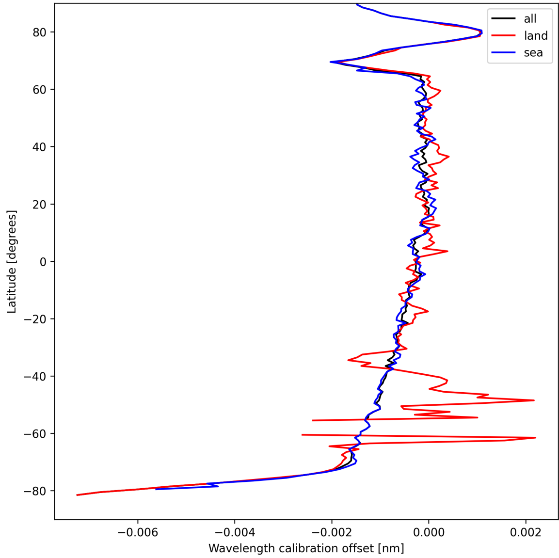
Figure 16: Zonal average of “Wavelength calibration offset” for 2025-09-05 to 2025-09-06.
