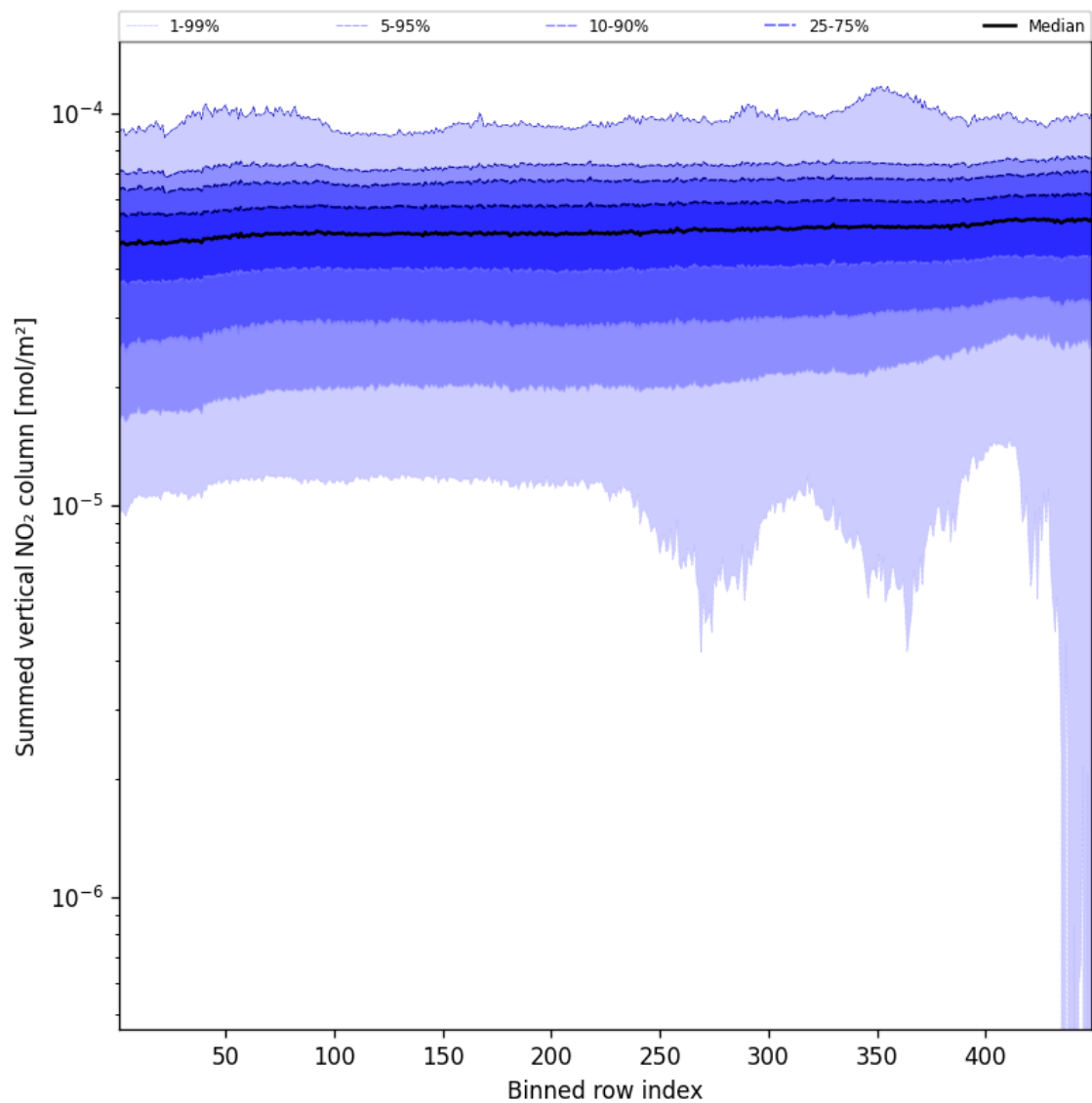
Figure 55: Along track statistics of “Summed vertical NO 2 column” for 2025-09-05 to 2025-09-06
