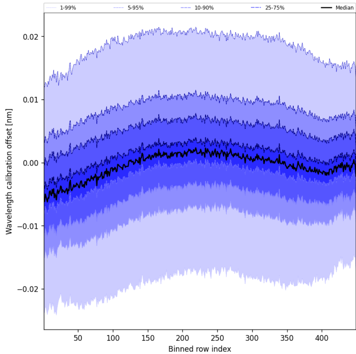
Figure 50: Along track statistics of “Wavelength calibration offset” for 2025-09-05 to 2025-09-06
