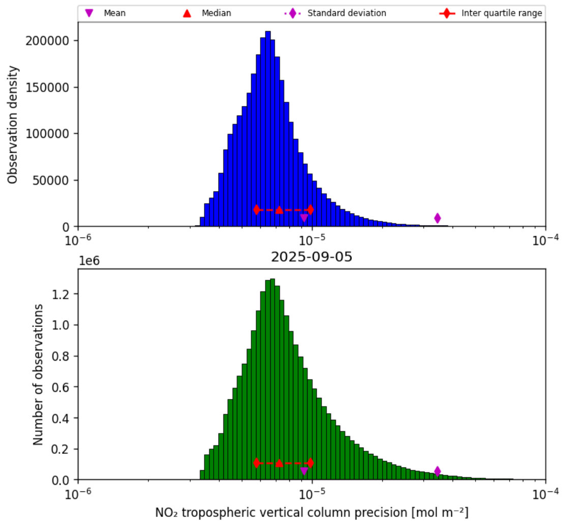
Figure 28: Histogram of “NO 2 tropospheric vertical column precision” for 2025-09-05 to 2025-09-06
