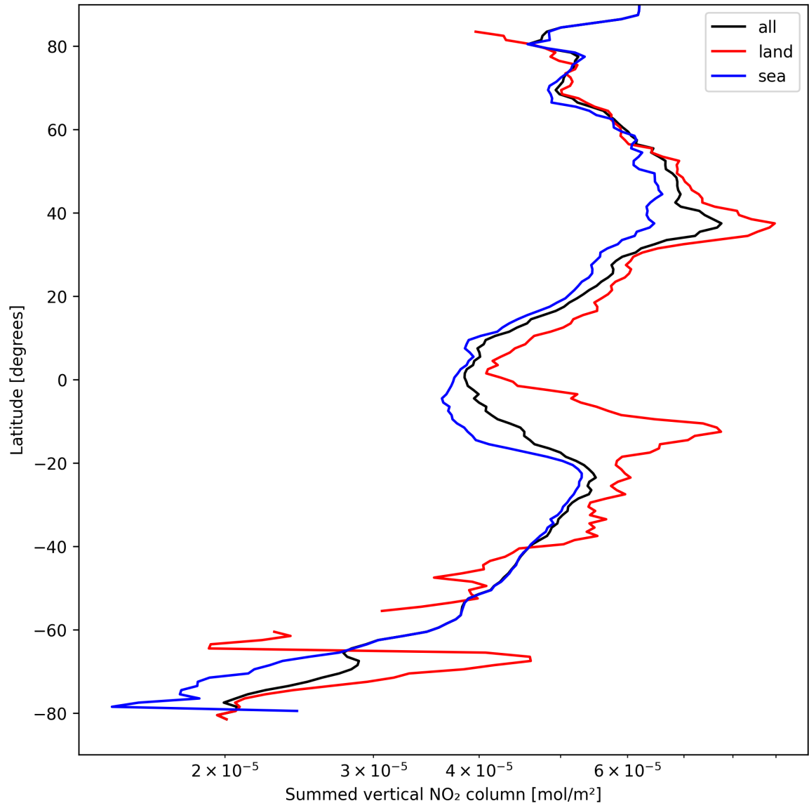
Figure 21: Zonal average of “Summed vertical NO 2 column” for 2025-09-05 to 2025-09-06.
