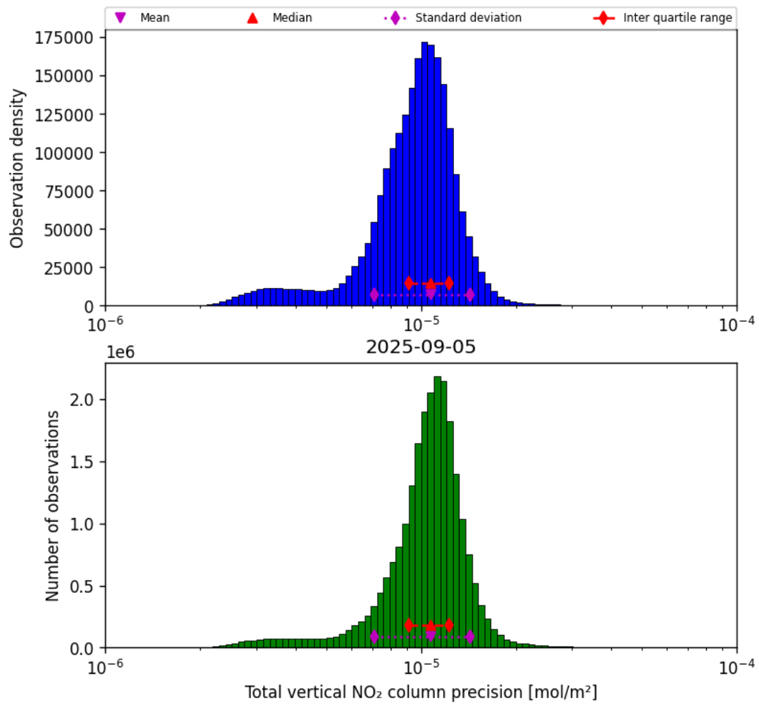
Figure 37: Histogram of "Total vertical NO 2 column precision" for 2025-09-05 to 2025-09-06
