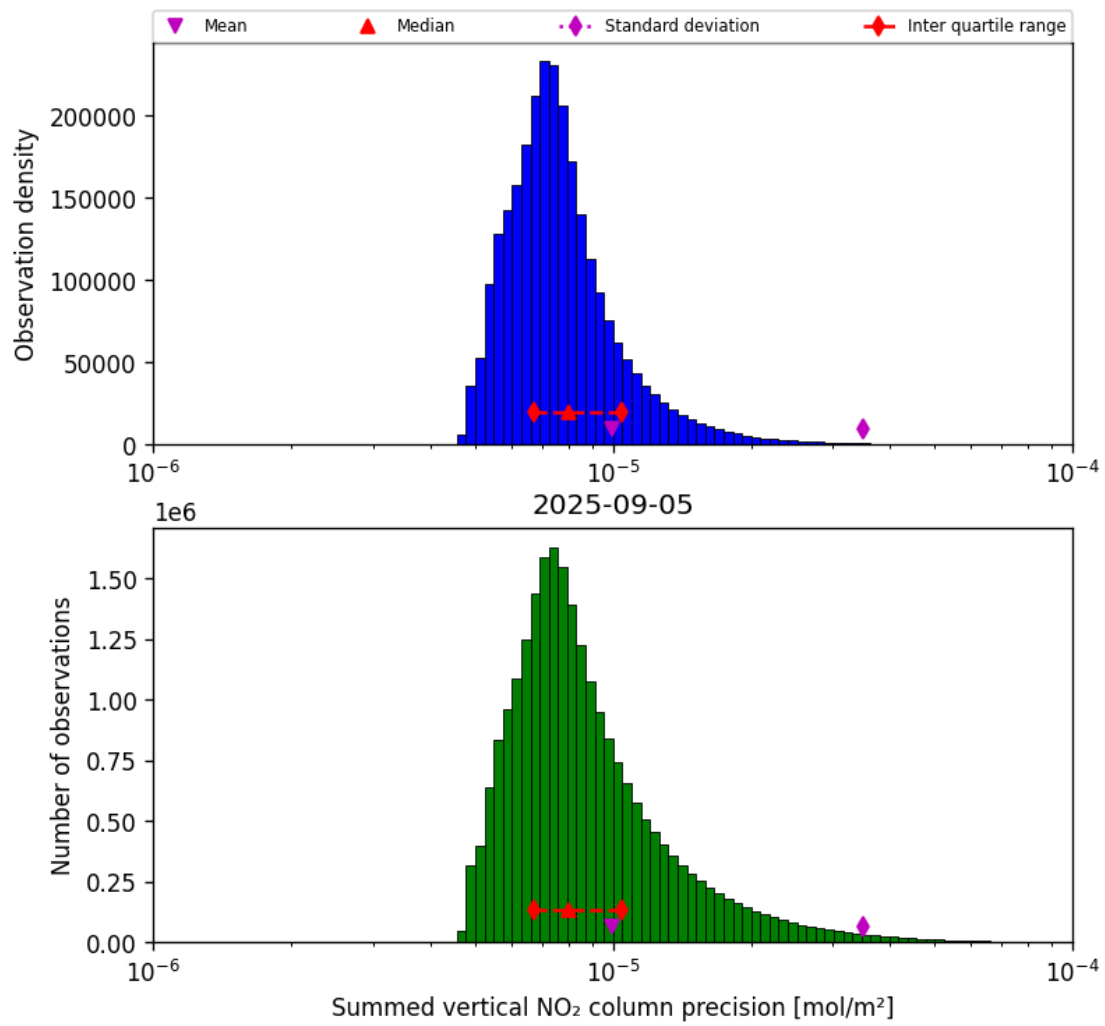
Figure 39: Histogram of "Summed vertical NO 2 column precision" for 2025-09-05 to 2025-09-06
