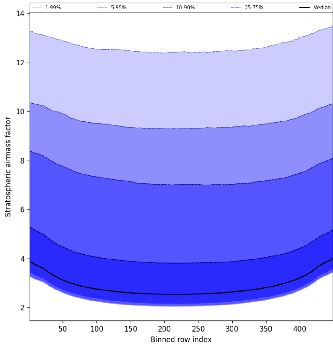
Figure 59: Along track statistics of “Stratospheric airmass factor” for 2025-09-05 to 2025-09-06
