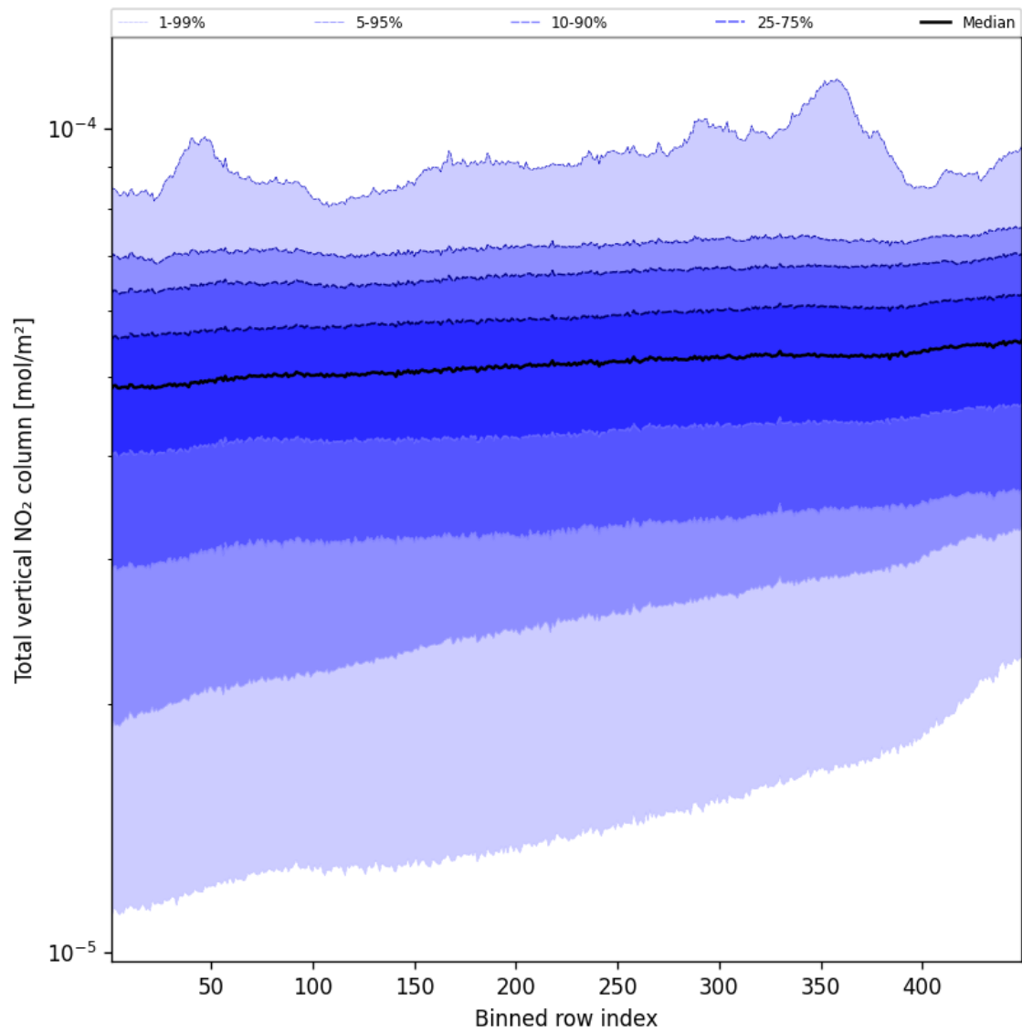
Figure 53: Along track statistics of “Total vertical NO 2 column” for 2025-09-05 to 2025-09-06
