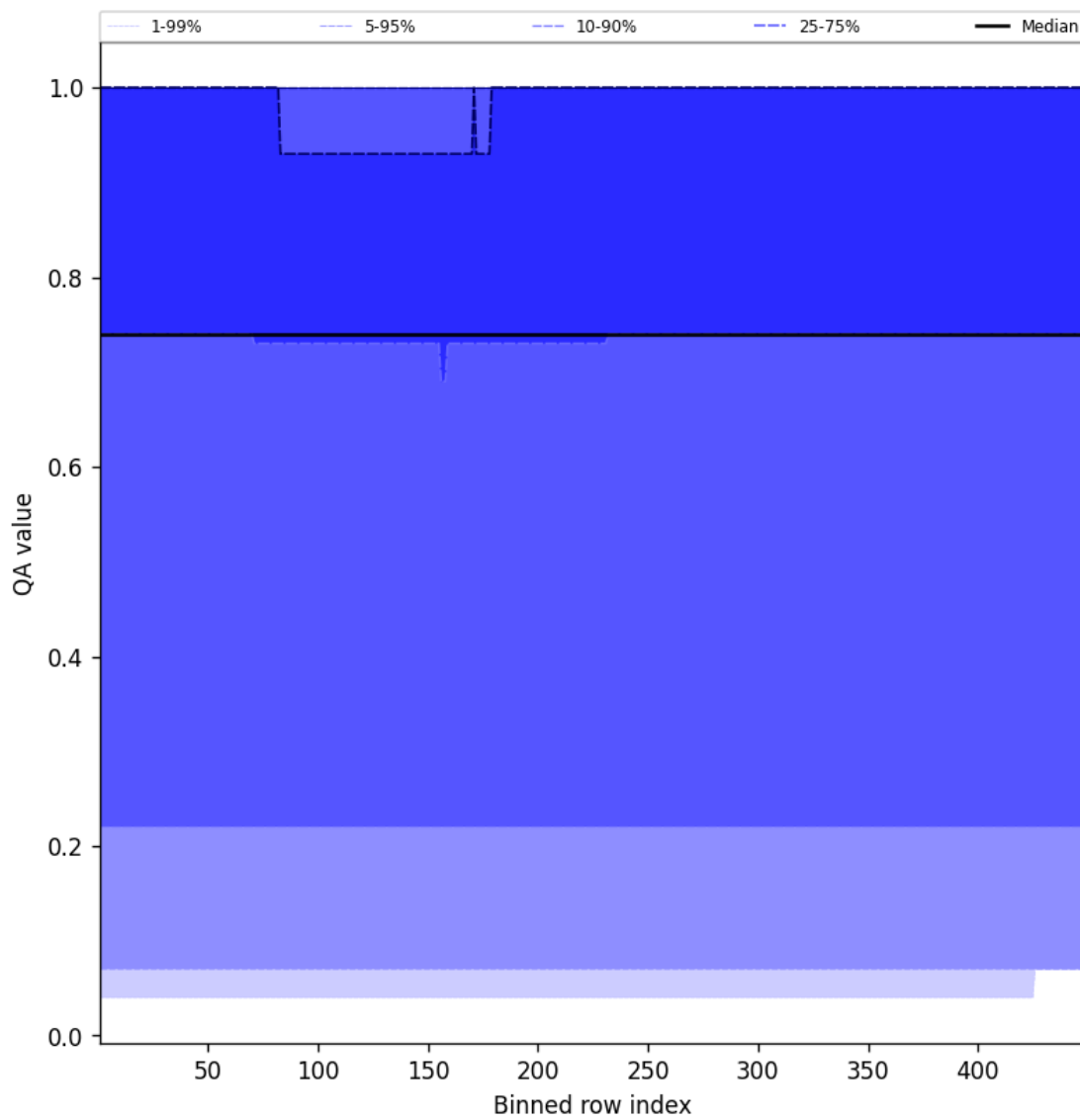
Figure 43: Along track statistics of “QA value” for 2025-09-05 to 2025-09-06
