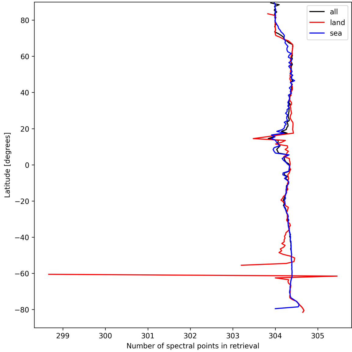
Figure 14: Zonal average of “Number of spectral points in retrieval” for 2025-09-05 to 2025-09-06.
