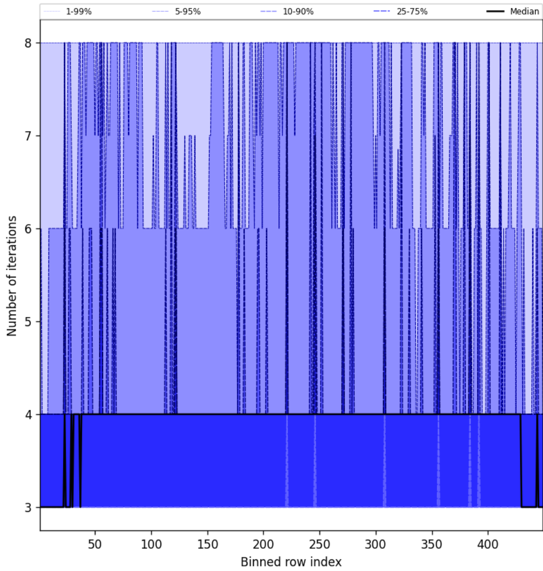
Figure 49: Along track statistics of “Number of iterations” for 2025-09-05 to 2025-09-06
