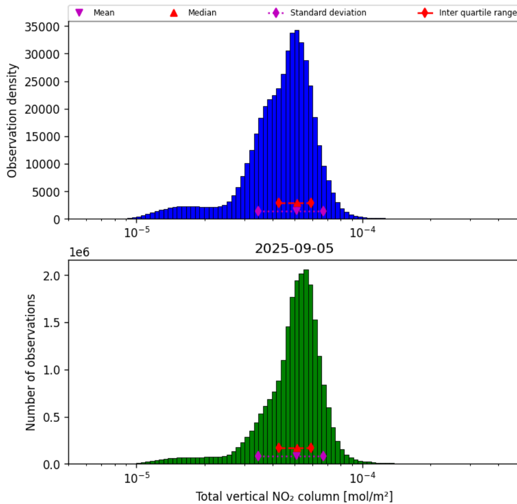
Figure 36: Histogram of “Total vertical NO 2 column” for 2025-09-05 to 2025-09-06
