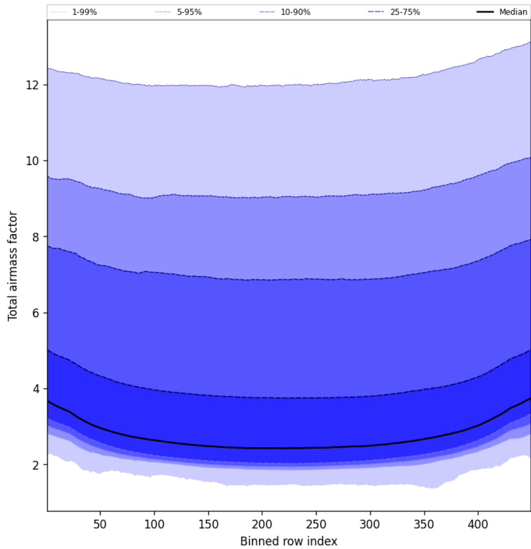
Figure 47: Along track statistics of “Total airmass factor” for 2025-09-05 to 2025-09-06
