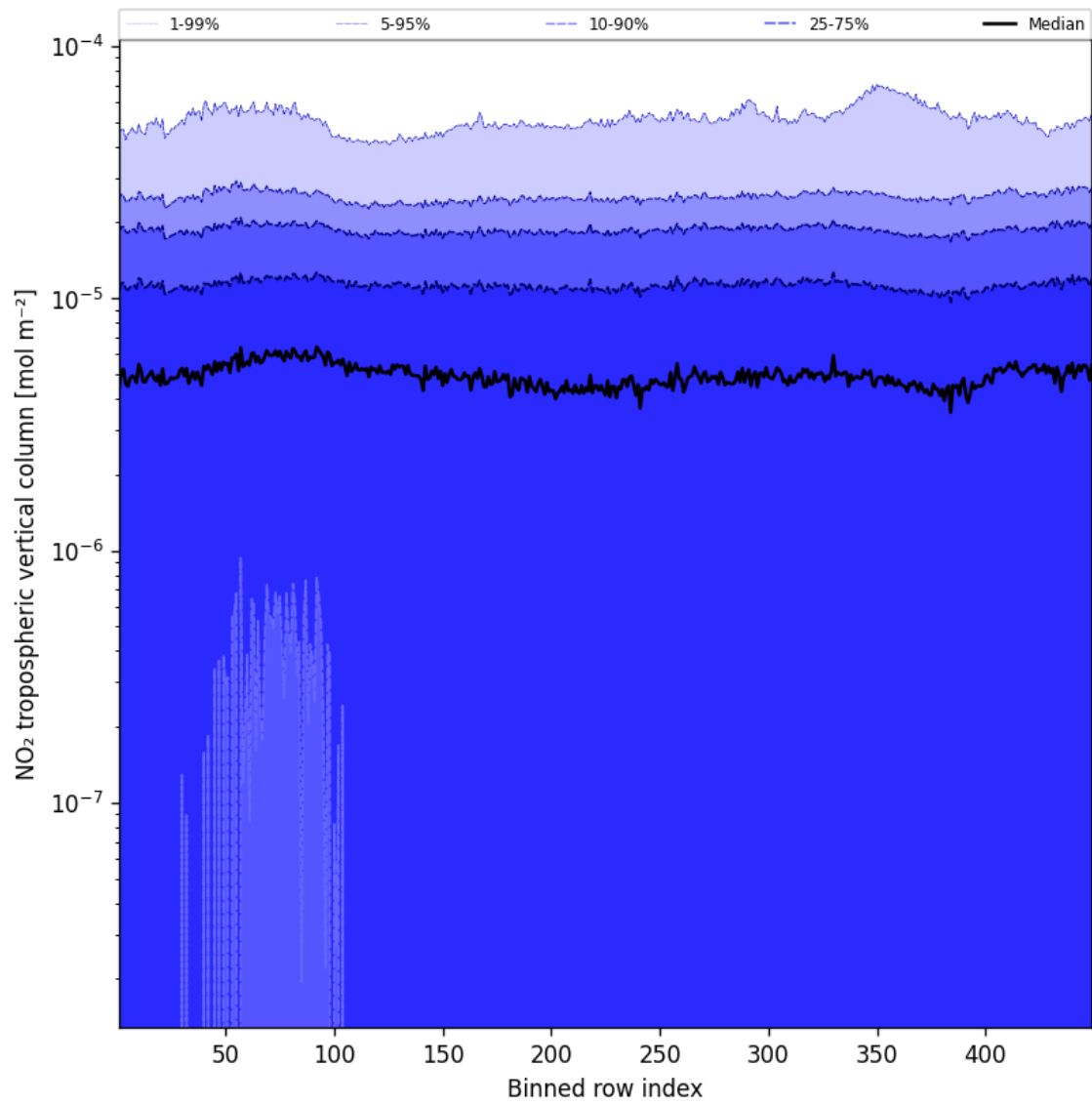
Figure 44: Along track statistics of “NO 2 tropospheric vertical column” for 2025-09-05 to 2025-09-06
