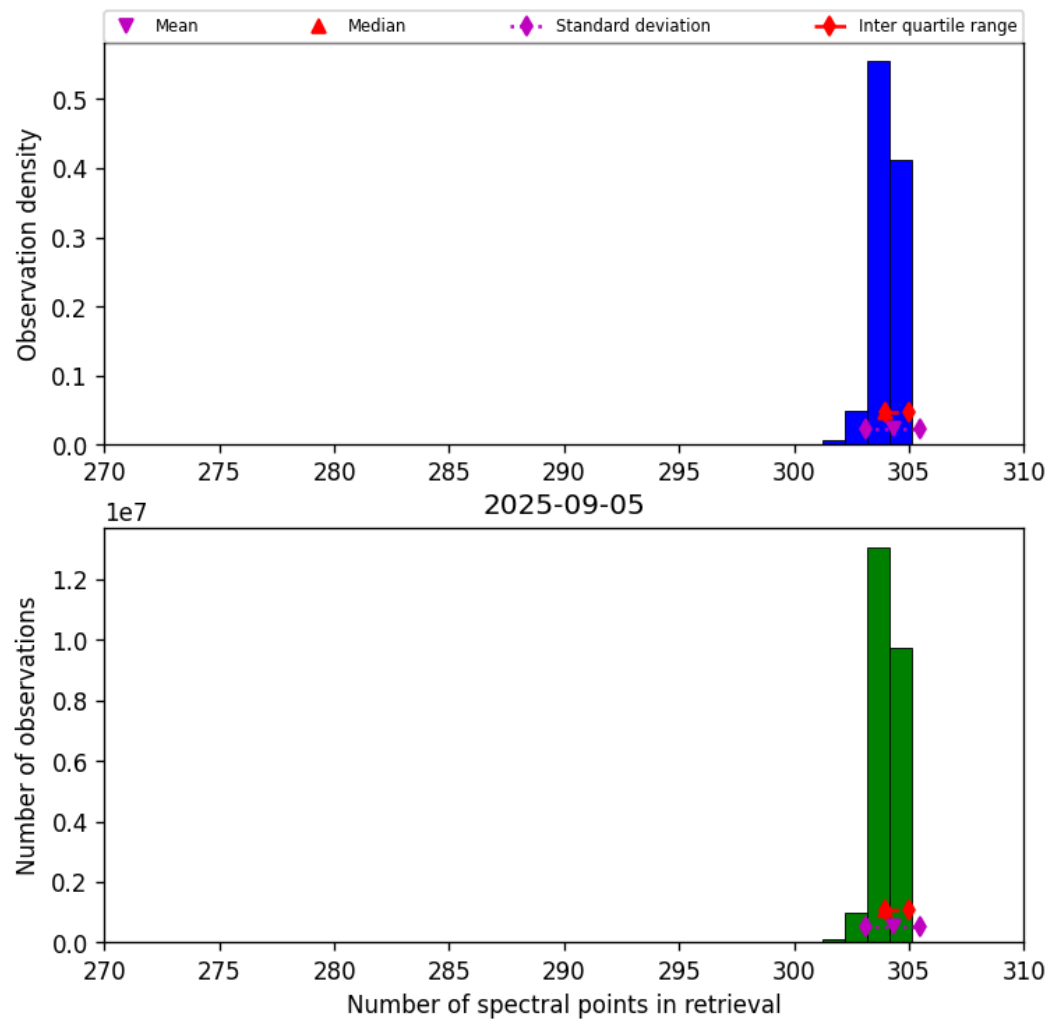
Figure 31: Histogram of “Number of spectral points in retrieval” for 2025-09-05 to 2025-09-06
