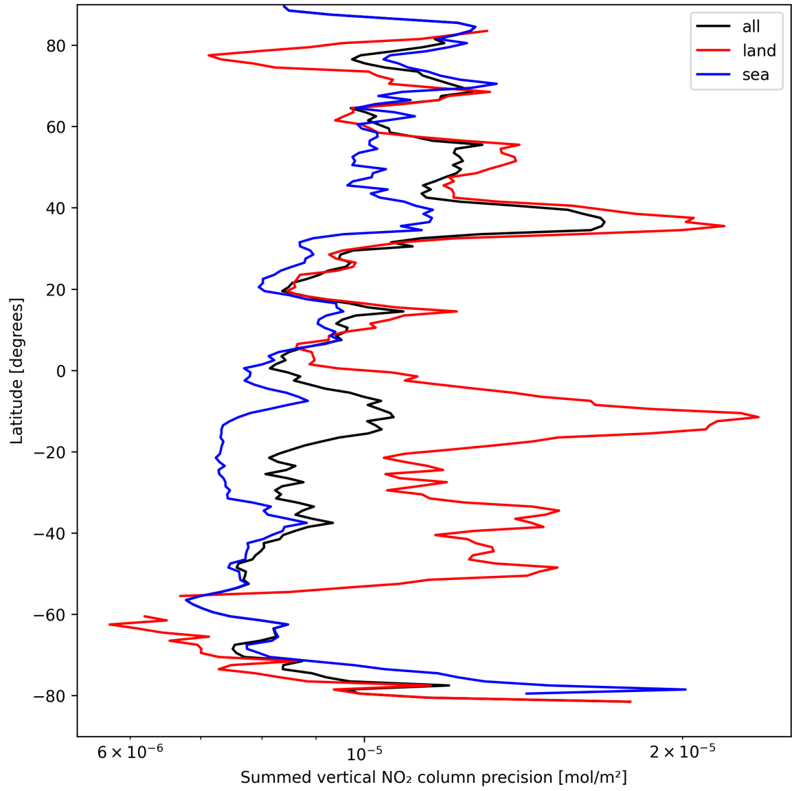
Figure 22: Zonal average of “Summed vertical NO 2 column precision” for 2025-09-05 to 2025-09-06.
