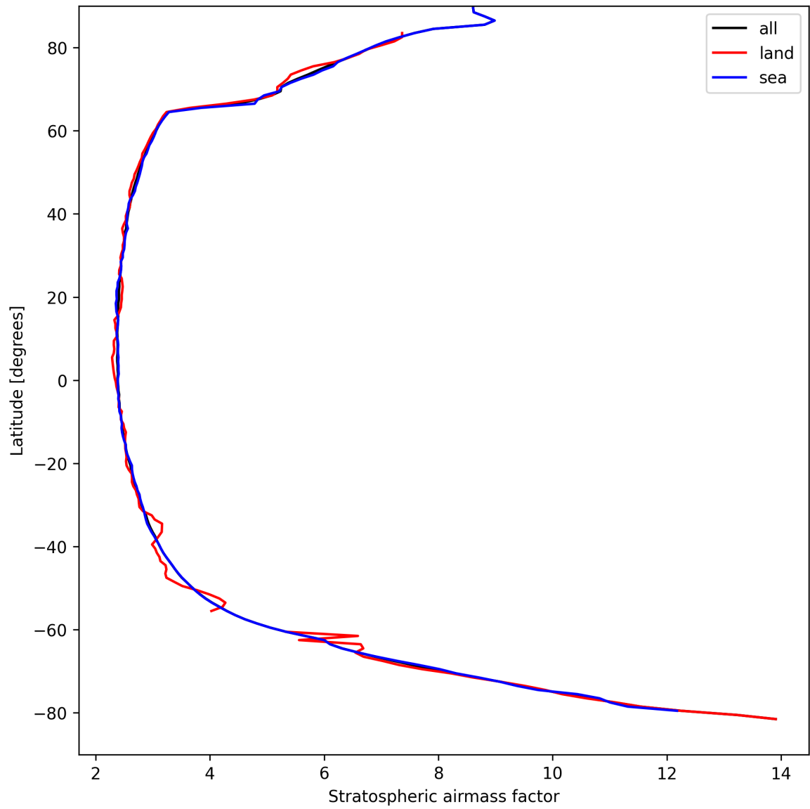
Figure 25: Zonal average of “Stratospheric air mass factor” for 2025-09-05 to 2025-09-06.
