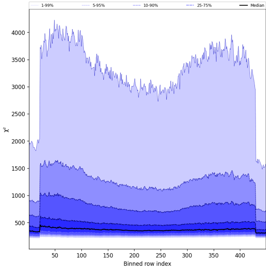
Figure 57: Along track statistics of “ \chi^2 ” for 2025-09-05 to 2025-09-06
