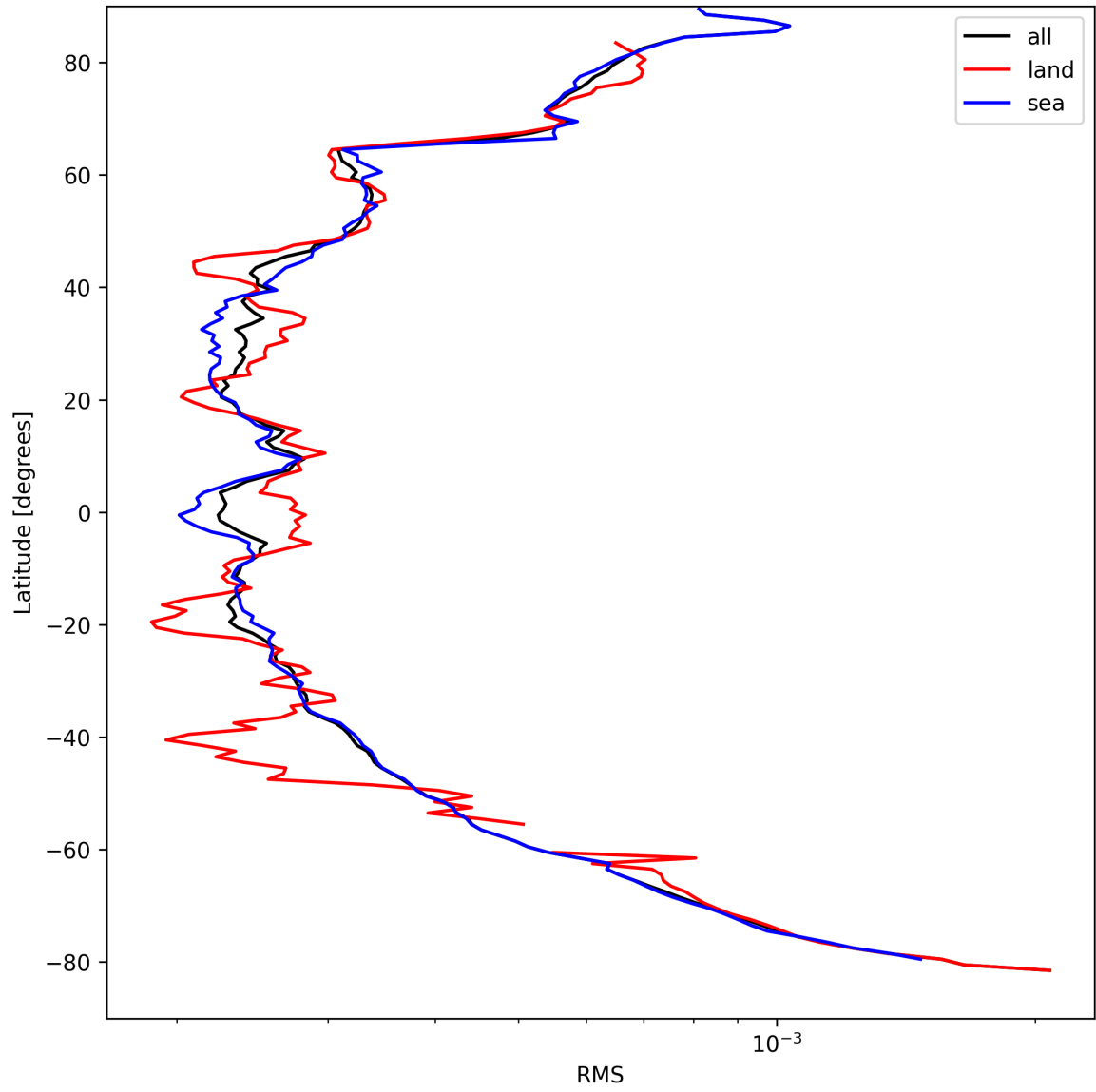
Figure 24: Zonal average of “RMS” for 2025-09-05 to 2025-09-06.
