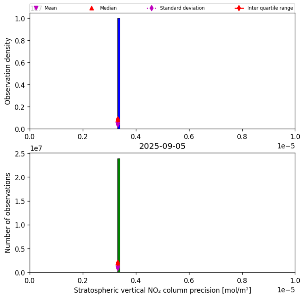
Figure 35: Histogram of “Stratospheric vertical NO 2 column precision” for 2025-09-05 to 2025-09-06
