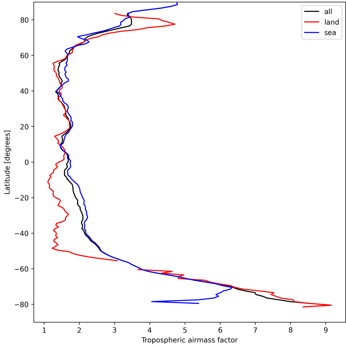
Figure 12: Zonal average of “Tropospheric airmass factor” for 2025-09-05 to 2025-09-06.
