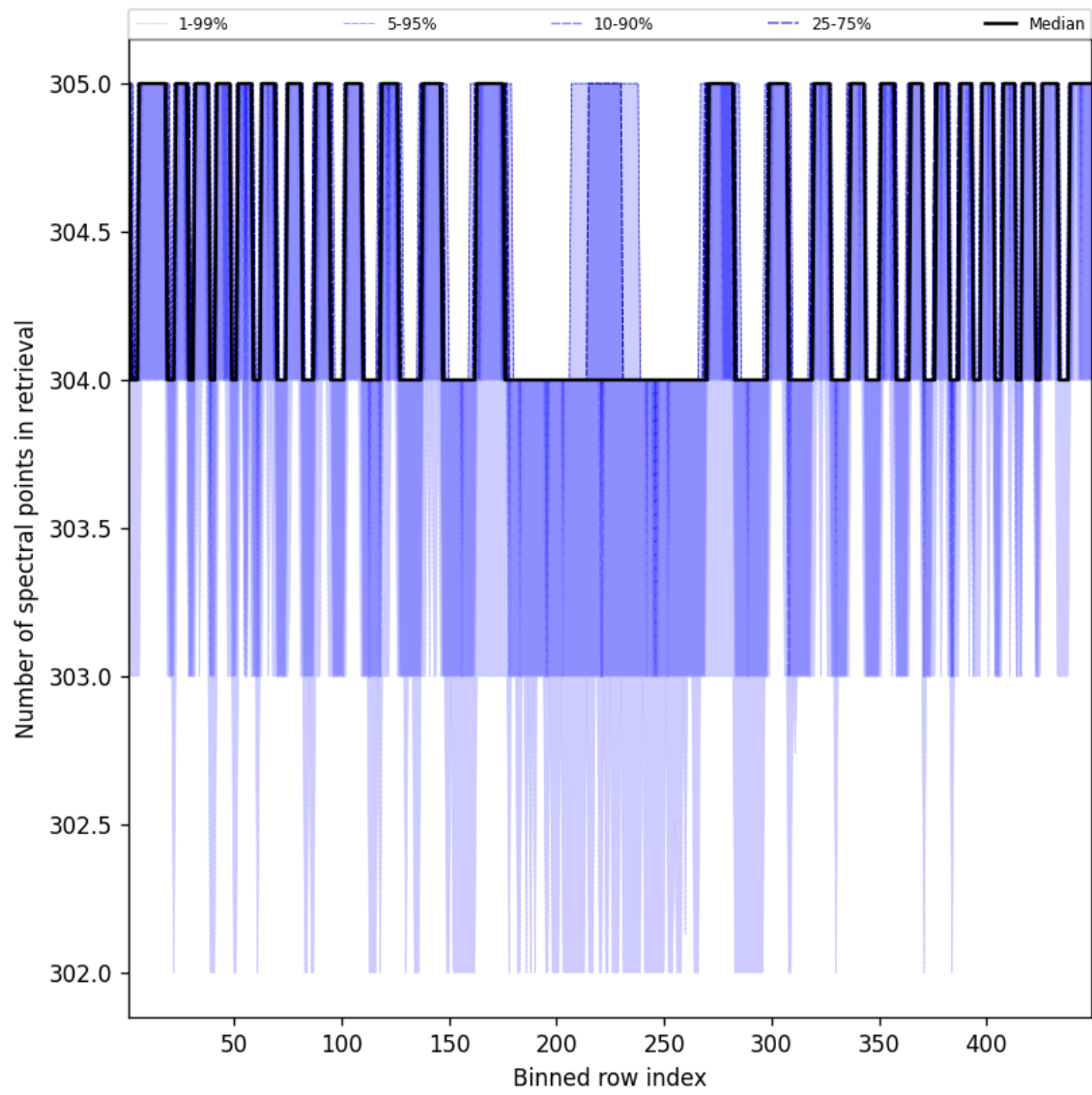
Figure 48: Along track statistics of “Number of spectral points in retrieval” for 2025-09-05 to 2025-09-06
