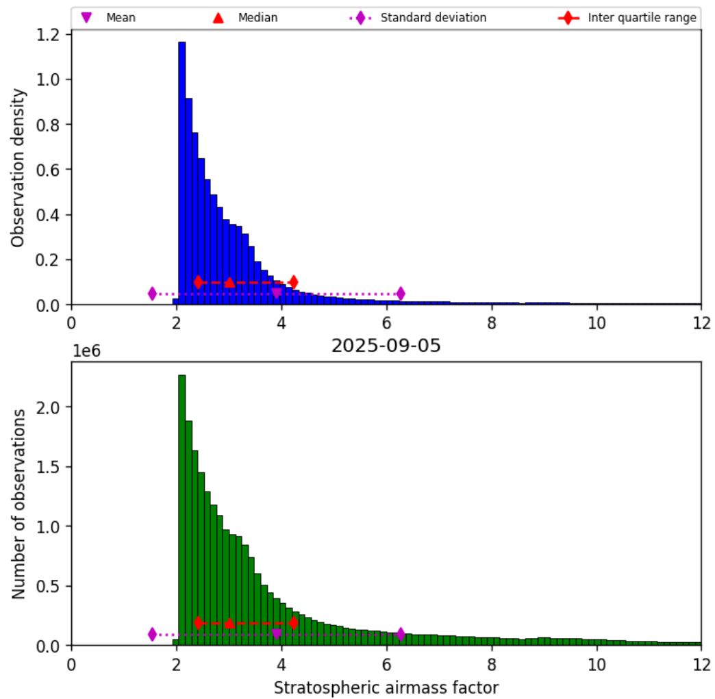
Figure 42: Histogram of “Stratospheric airmass factor” for 2025-09-05 to 2025-09-06
