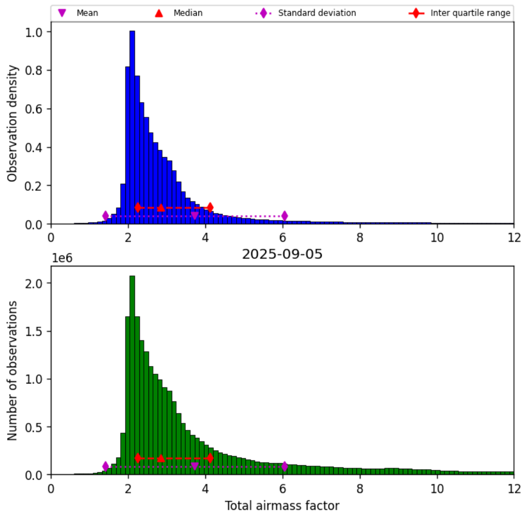
Figure 30: Histogram of “Total airmass factor” for 2025-09-05 to 2025-09-06
