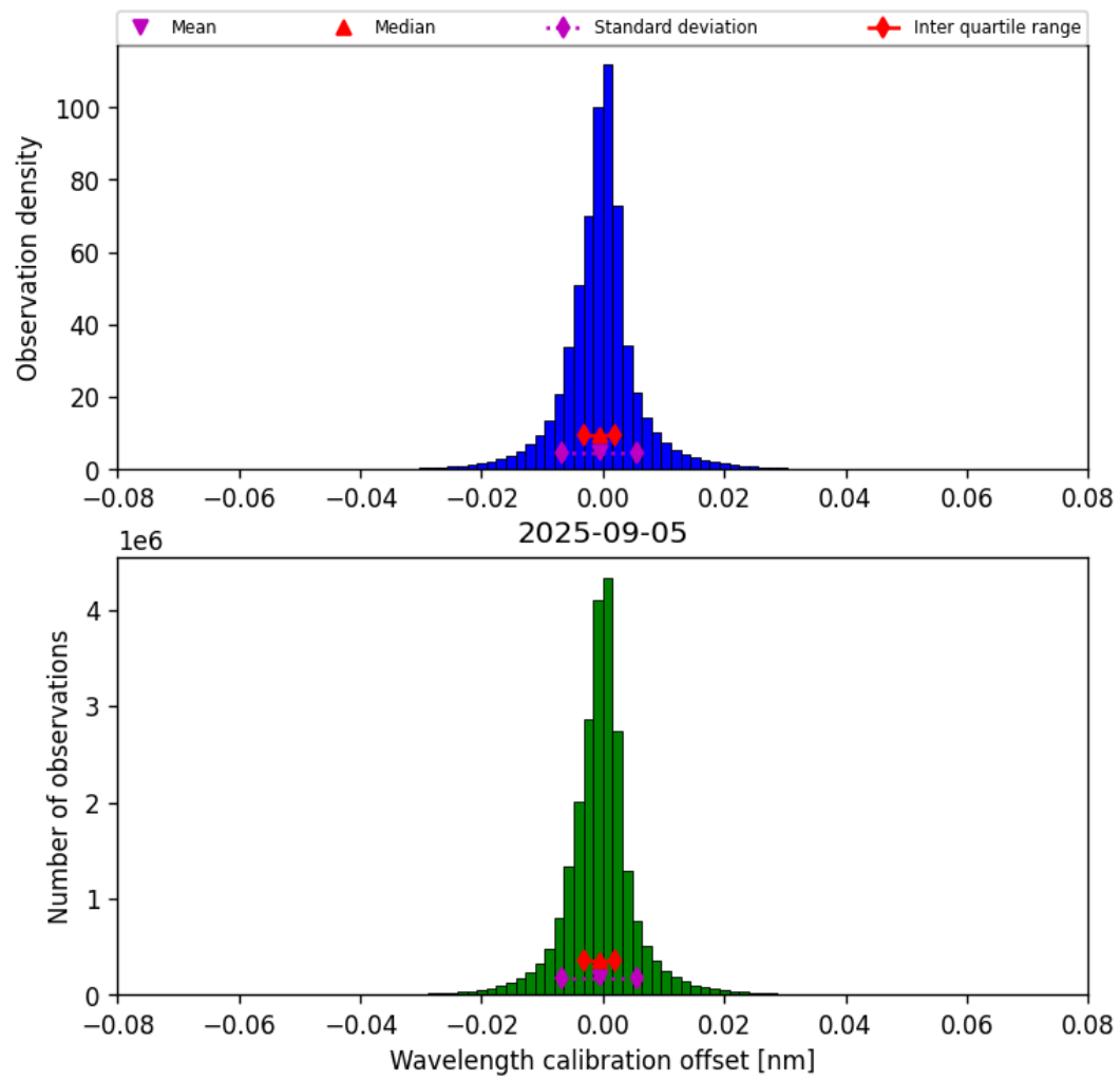
Figure 33: Histogram of “Wavelength calibration offset” for 2025-09-05 to 2025-09-06
