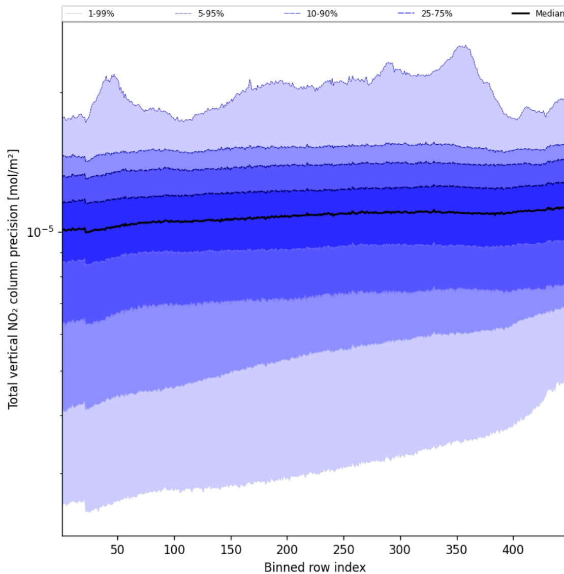
Figure 54: Along track statistics of “Total vertical NO 2 column precision” for 2025-09-05 to 2025-09-06
