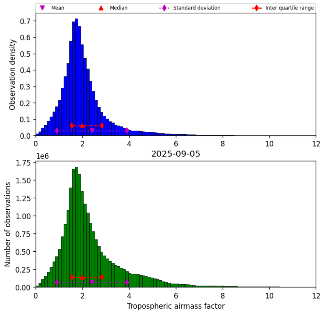
Figure 29: Histogram of “Tropospheric airmass factor” for 2025-09-05 to 2025-09-06
