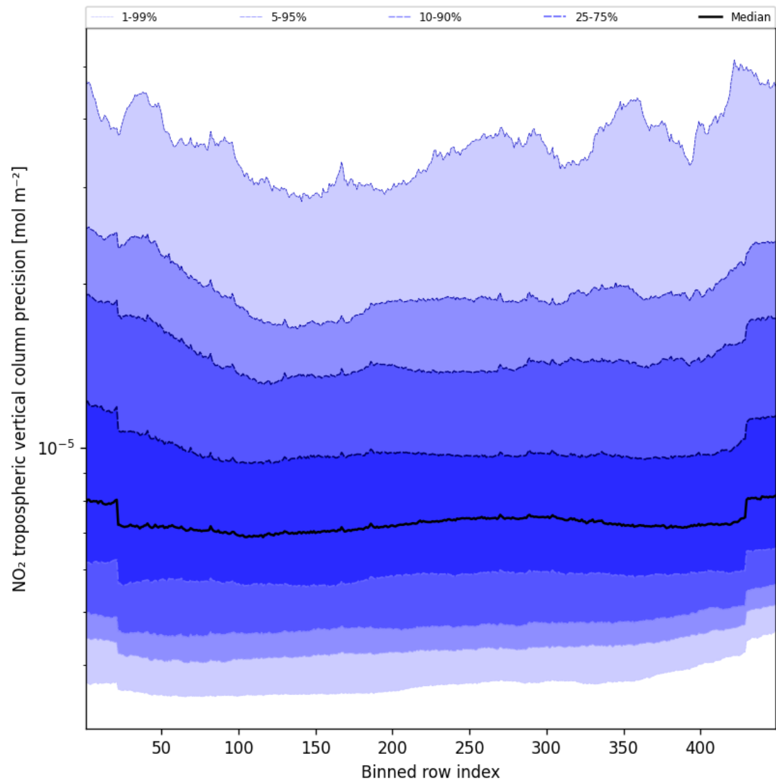
Figure 45: Along track statistics of “NO 2 tropospheric vertical column precision” for 2025-09-05 to 2025-09-06
