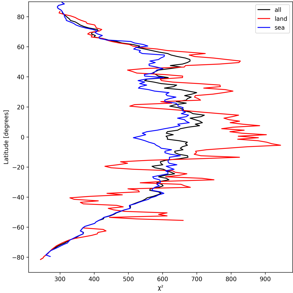
Figure 23: Zonal average of “ \chi^2 ” for 2025-09-05 to 2025-09-06.
