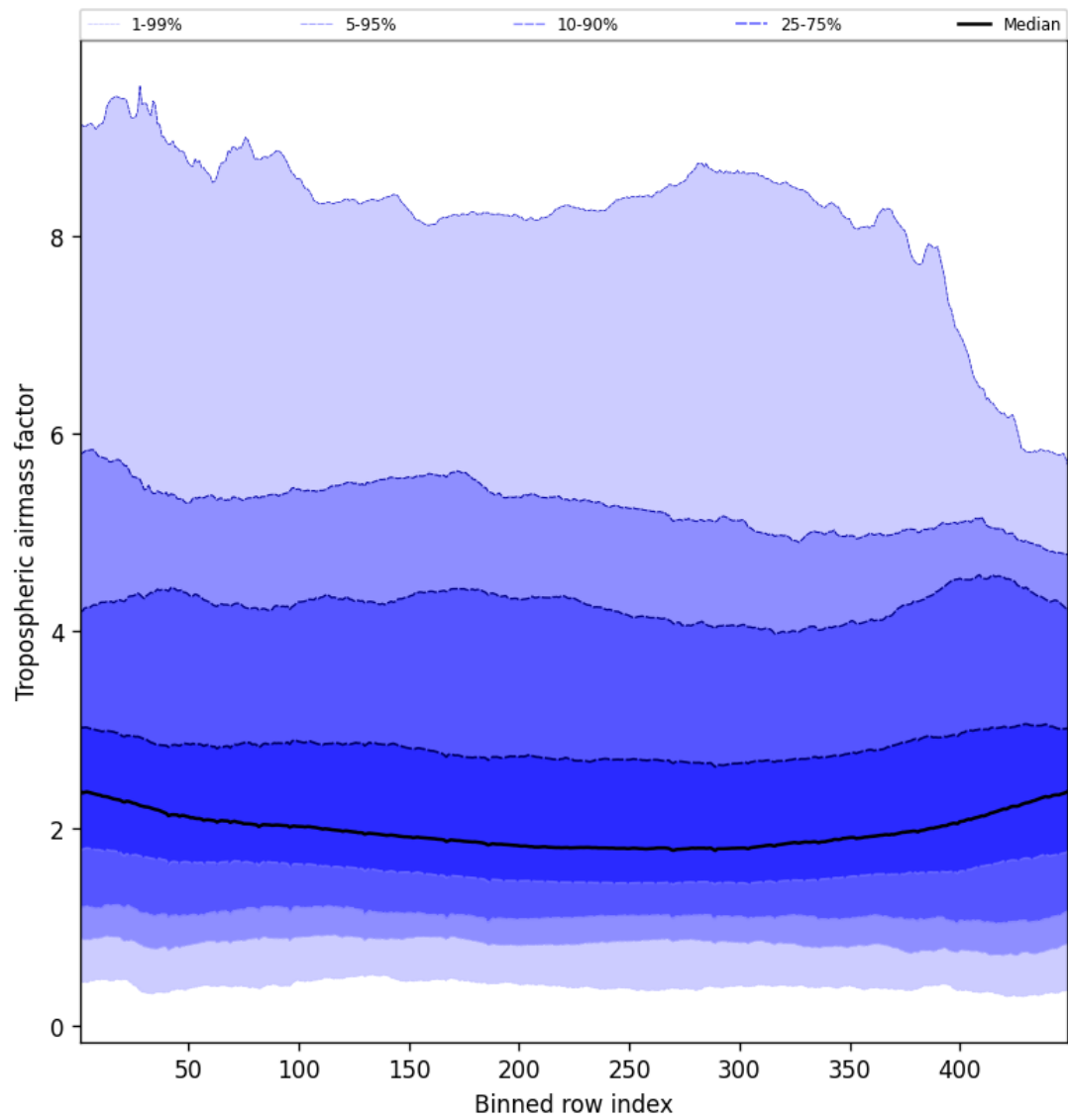
Figure 46: Along track statistics of “Tropospheric air mass factor” for 2025-09-05 to 2025-09-06
