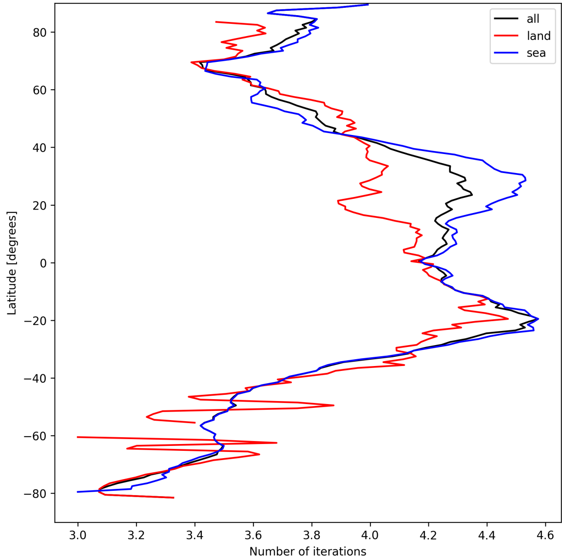
Figure 15: Zonal average of “Number of iterations” for 2025-09-05 to 2025-09-06.
