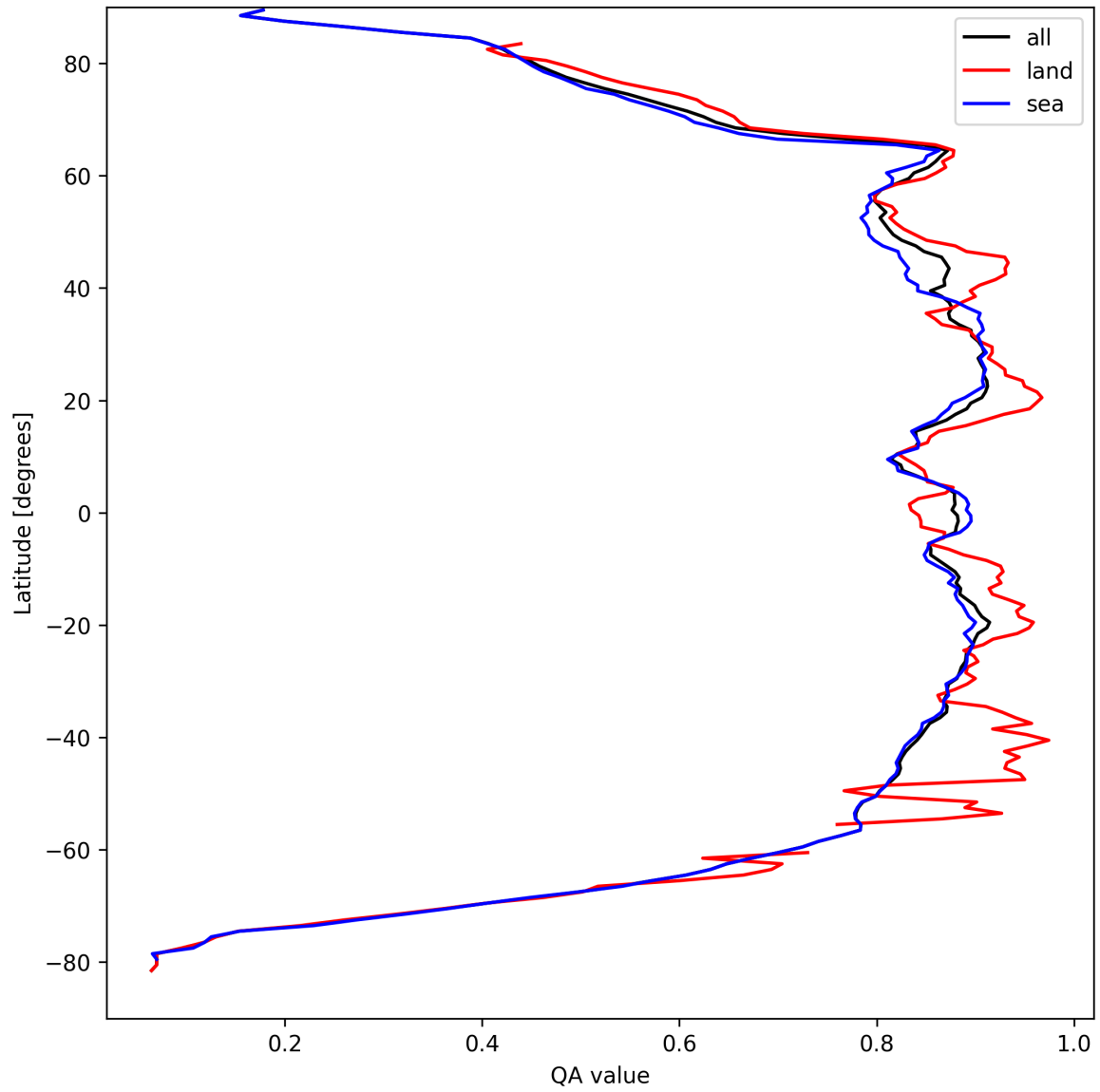
Figure 9: Zonal average of “QA value” for 2025-09-05 to 2025-09-06.
