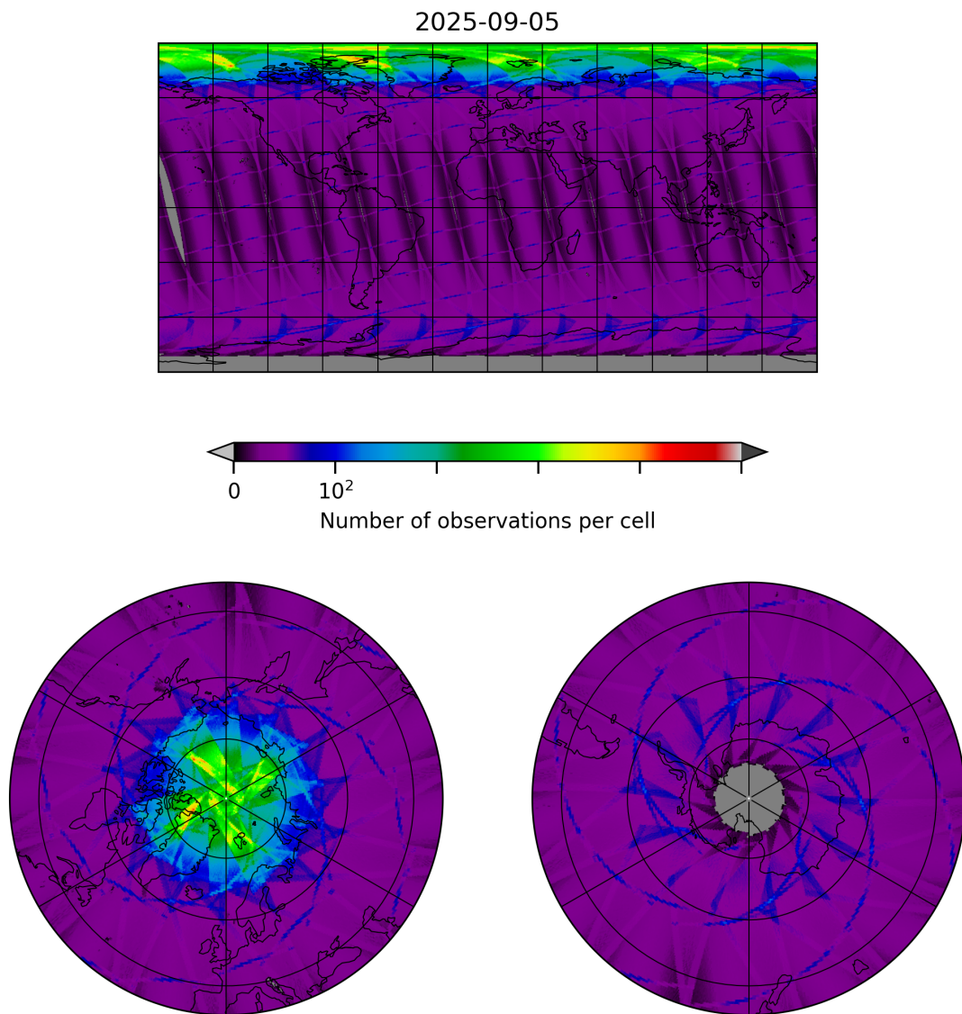
Figure 8: Map of the number of observations for 2025-09-05 to 2025-09-06
