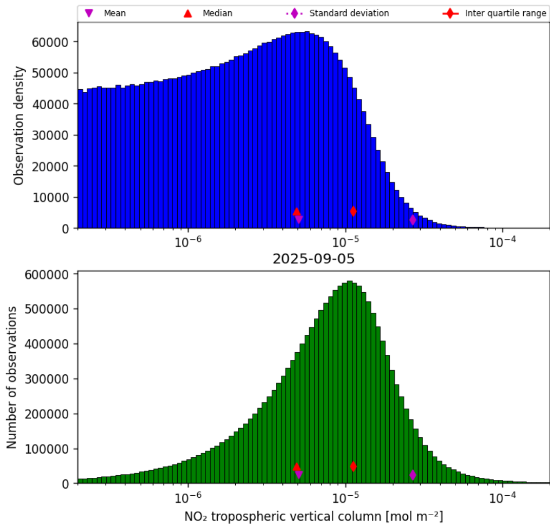
Figure 27: Histogram of “NO 2 tropospheric vertical column” for 2025-09-05 to 2025-09-06
