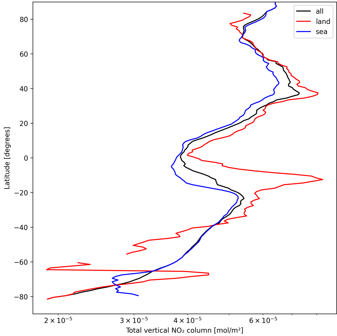
Figure 19: Zonal average of “Total vertical NO 2 column” for 2025-09-05 to 2025-09-06.
