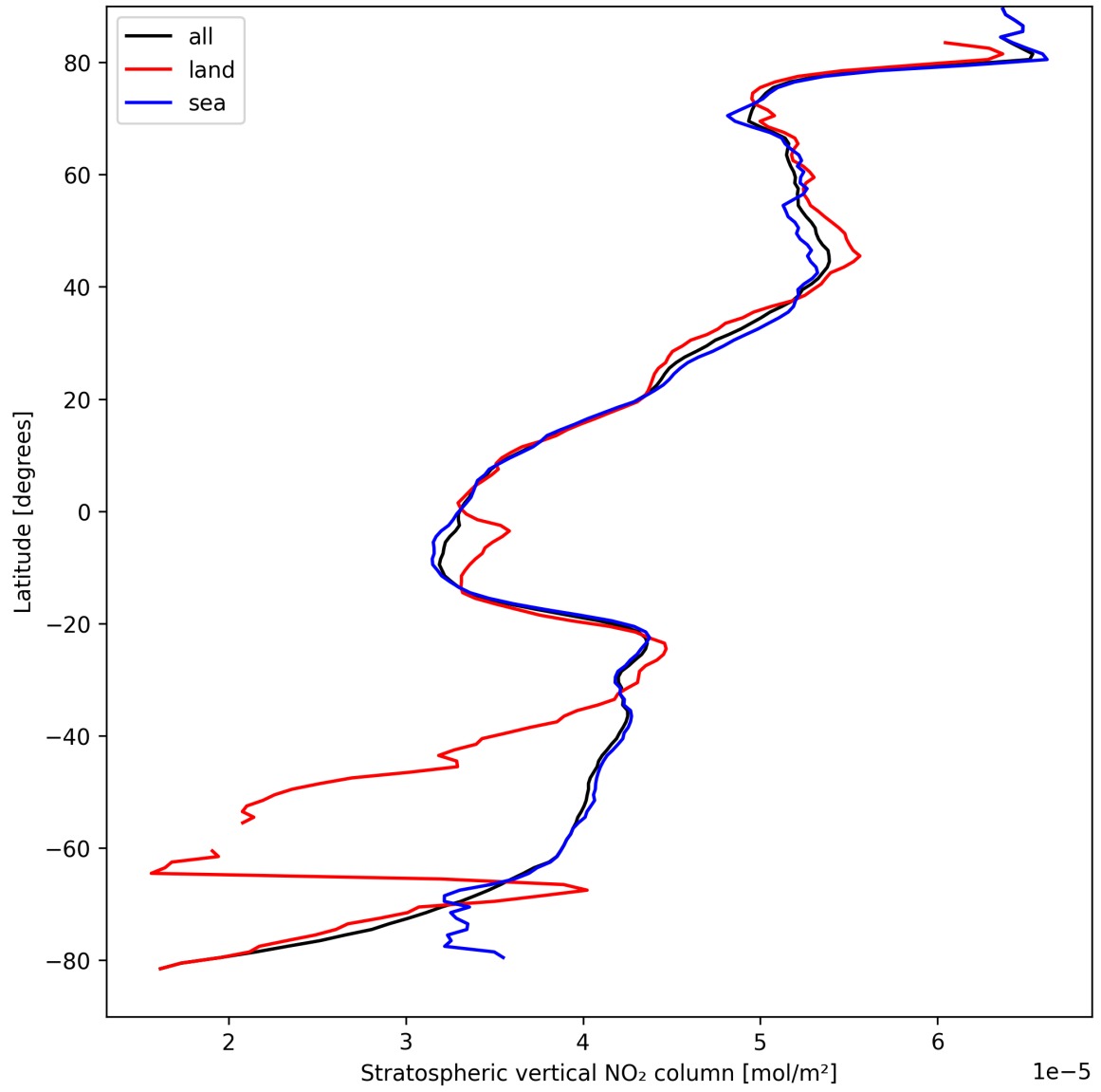
Figure 17: Zonal average of “Stratospheric vertical NO 2 column” for 2025-09-05 to 2025-09-06.
