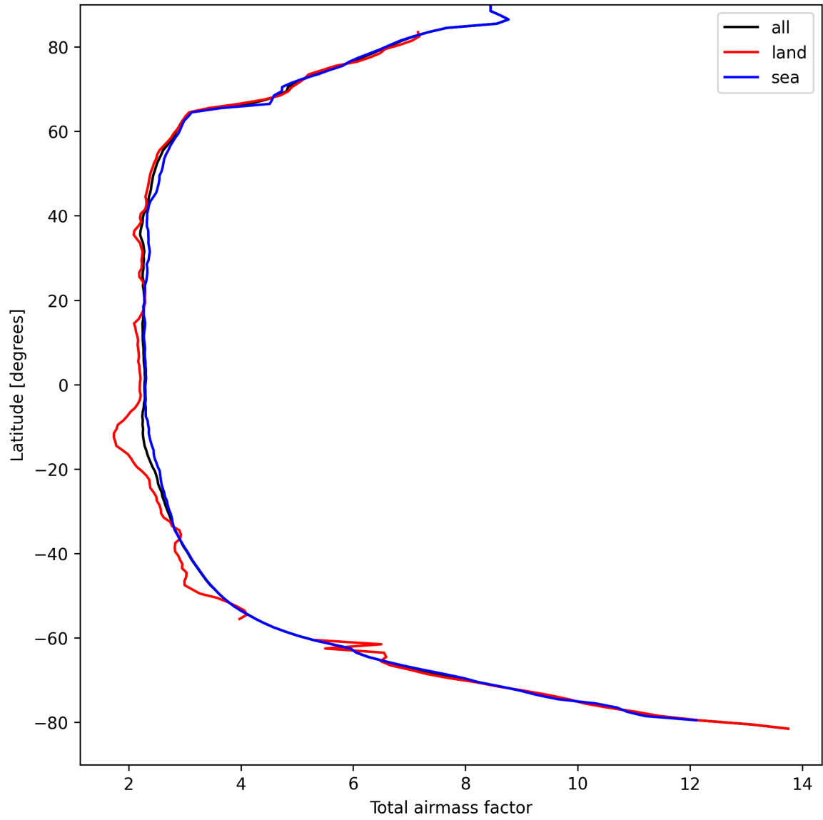
Figure 13: Zonal average of “Total airmass factor” for 2025-09-05 to 2025-09-06.
