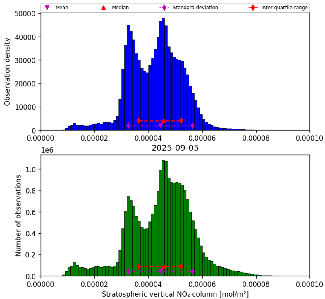
Figure 34: Histogram of “Stratospheric vertical NO 2 column” for 2025-09-05 to 2025-09-06
