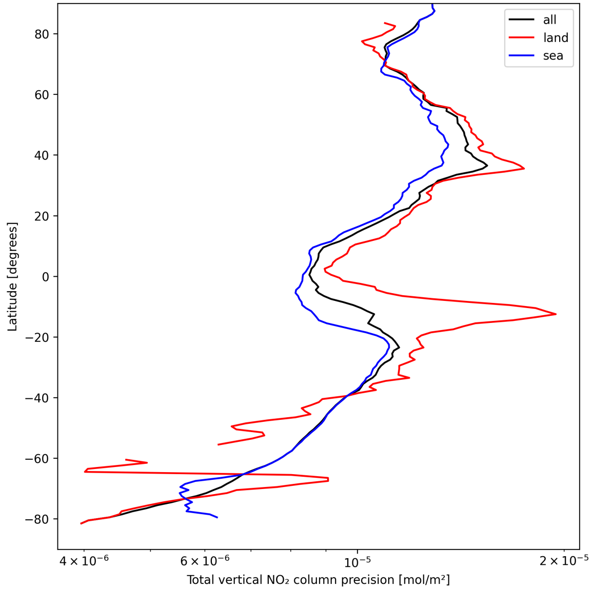
Figure 20: Zonal average of “Total vertical NO 2 column precision” for 2025-09-05 to 2025-09-06.
