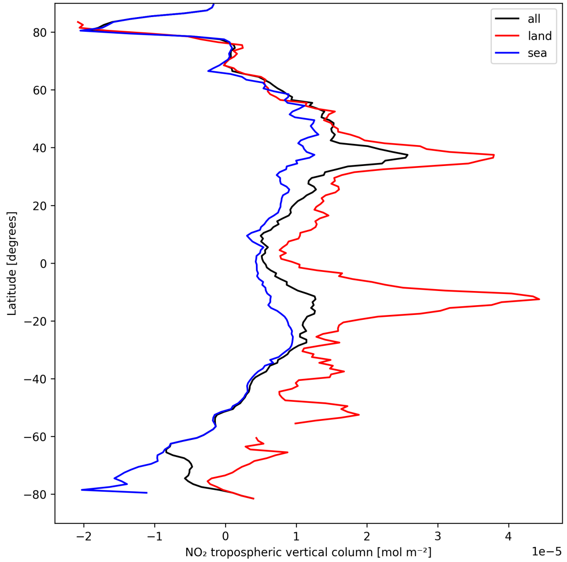
Figure 10: Zonal average of “NO 2 tropospheric vertical column” for 2025-09-05 to 2025-09-06.
