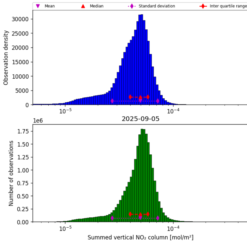
Figure 38: Histogram of “Summed vertical NO 2 column” for 2025-09-05 to 2025-09-06
