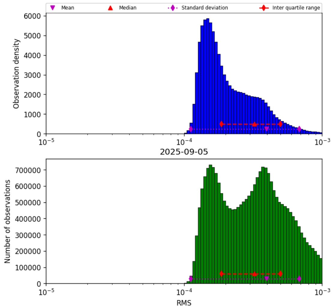
Figure 41: Histogram of “RMS” for 2025-09-05 to 2025-09-06
