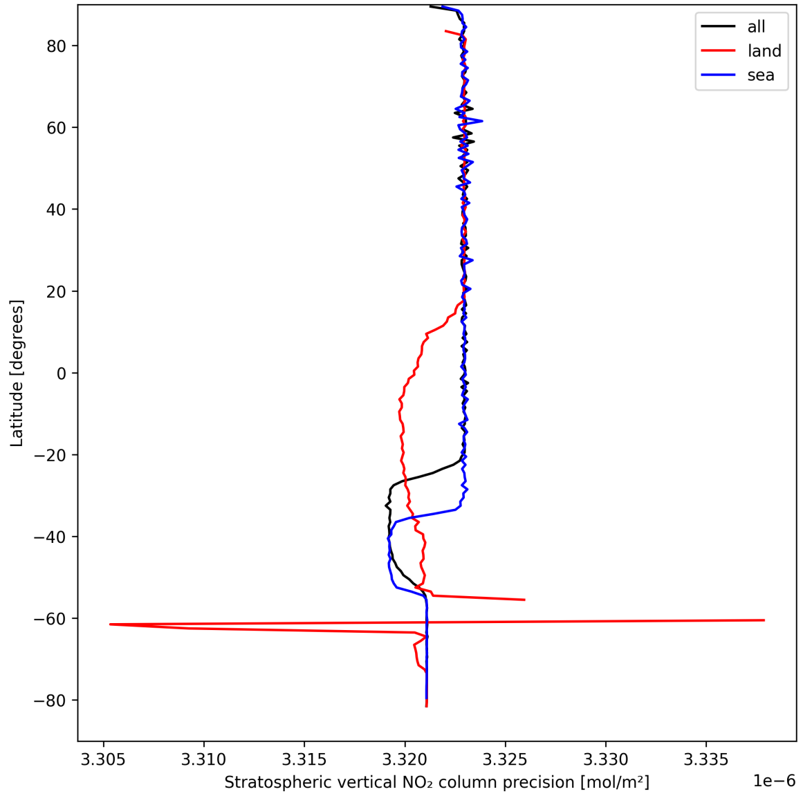
Figure 18: Zonal average of “Stratospheric vertical NO 2 column precision” for 2025-09-05 to 2025-09-06.
