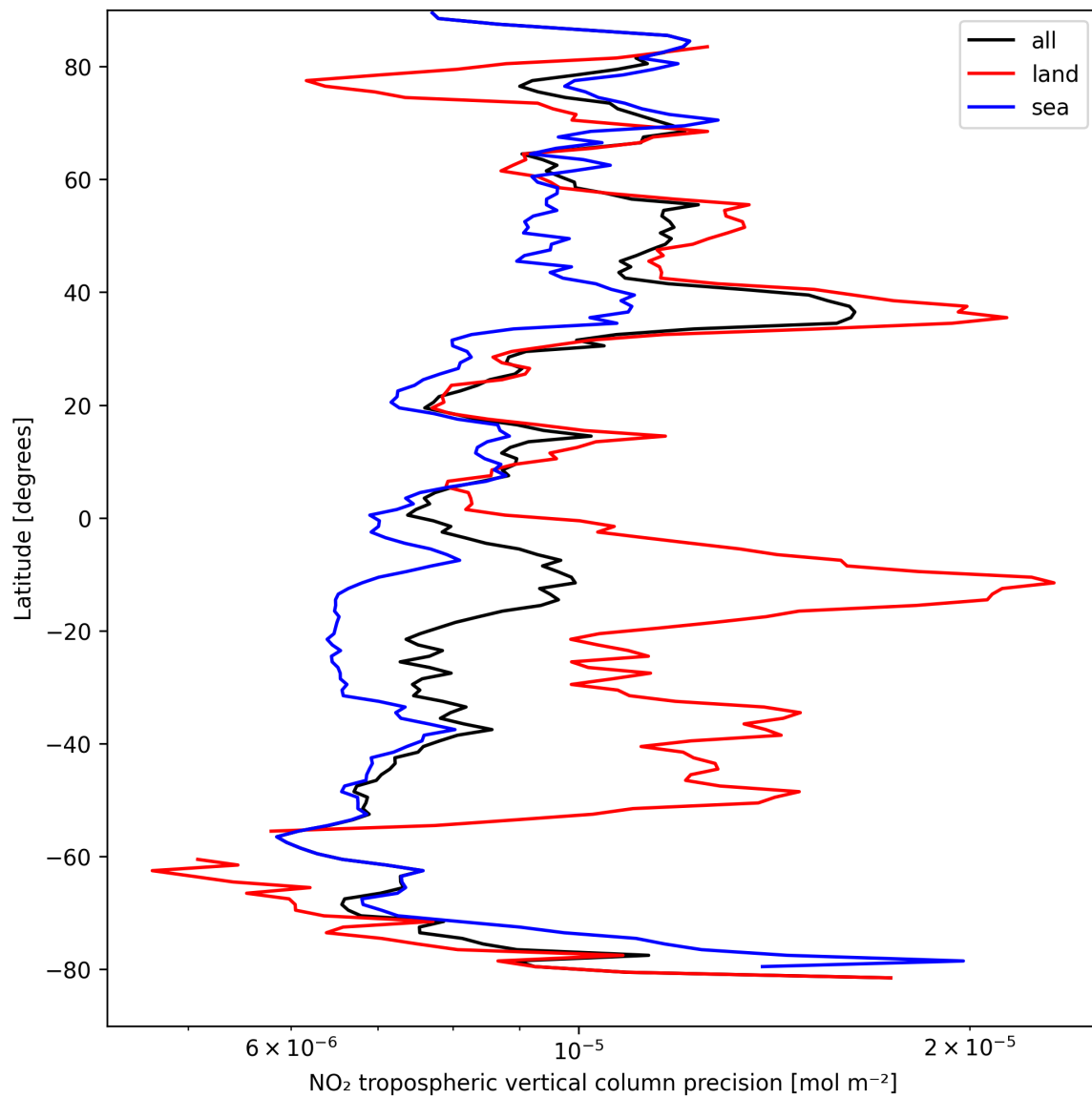
Figure 11: Zonal average of “NO 2 tropospheric vertical column precision” for 2025-09-05 to 2025-09-06.
