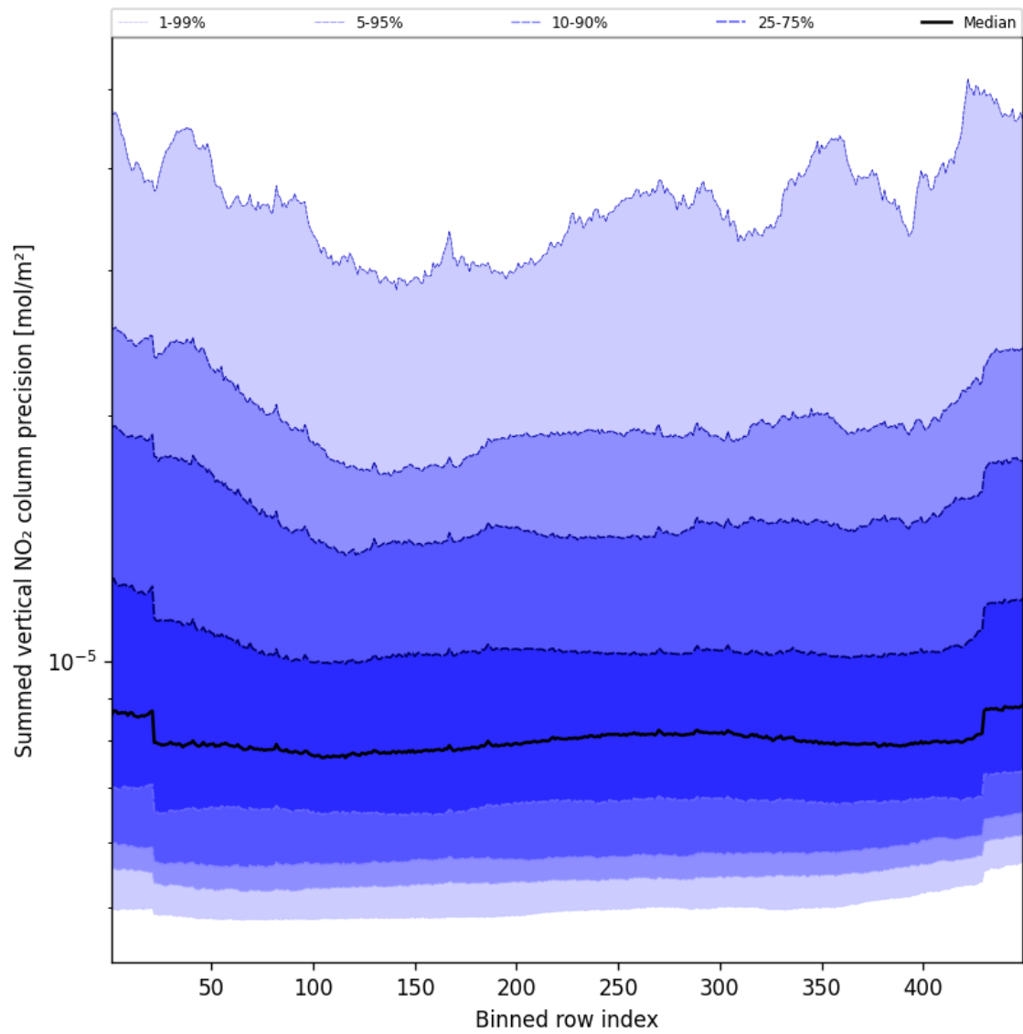
Figure 56: Along track statistics of “Summed vertical NO 2 column precision” for 2025-09-05 to 2025-09-06
