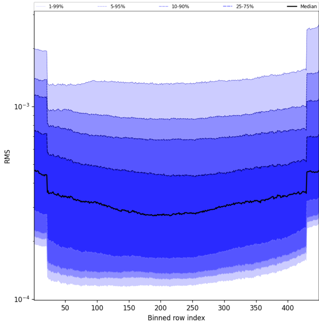
Figure 58: Along track statistics of “RMS” for 2025-09-05 to 2025-09-06
