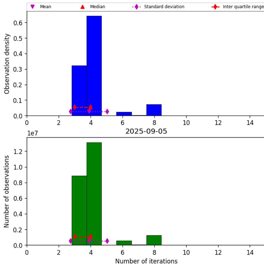
Figure 32: Histogram of “Number of iterations” for 2025-09-05 to 2025-09-06
