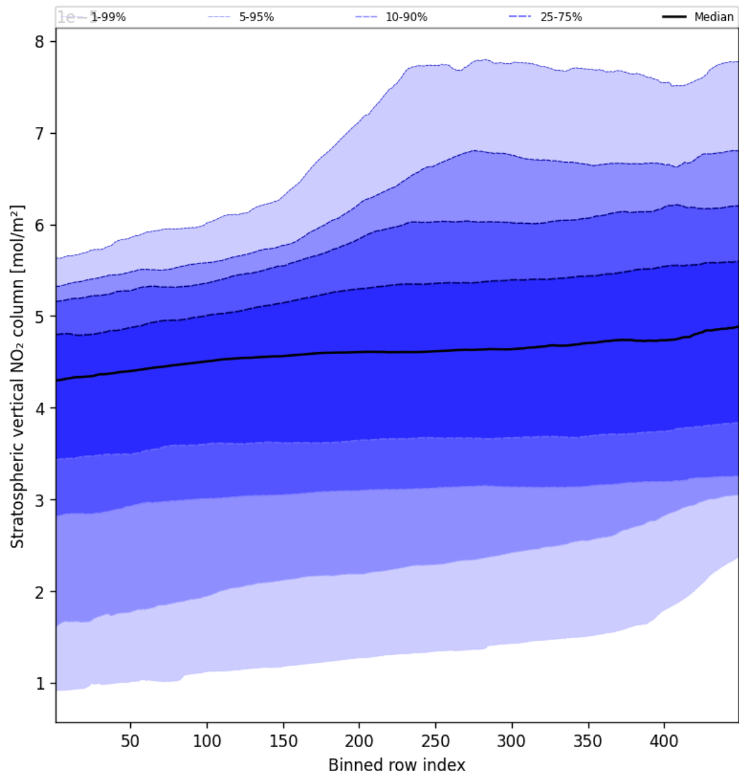
Figure 51: Along track statistics of “Stratospheric vertical NO 2 column” for 2025-09-05 to 2025-09-06
