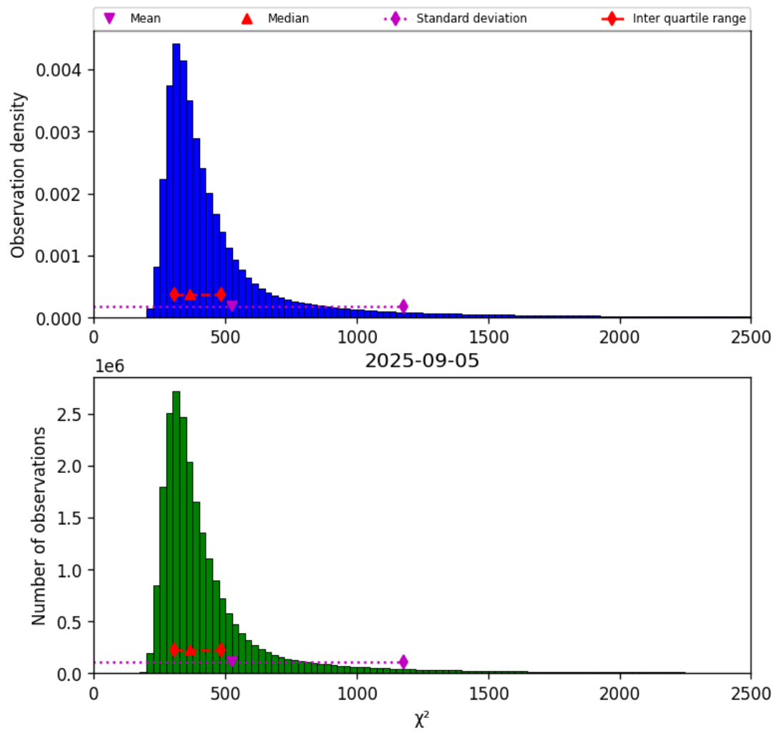
Figure 40: Histogram of “ \chi^2 ” for 2025-09-05 to 2025-09-06
