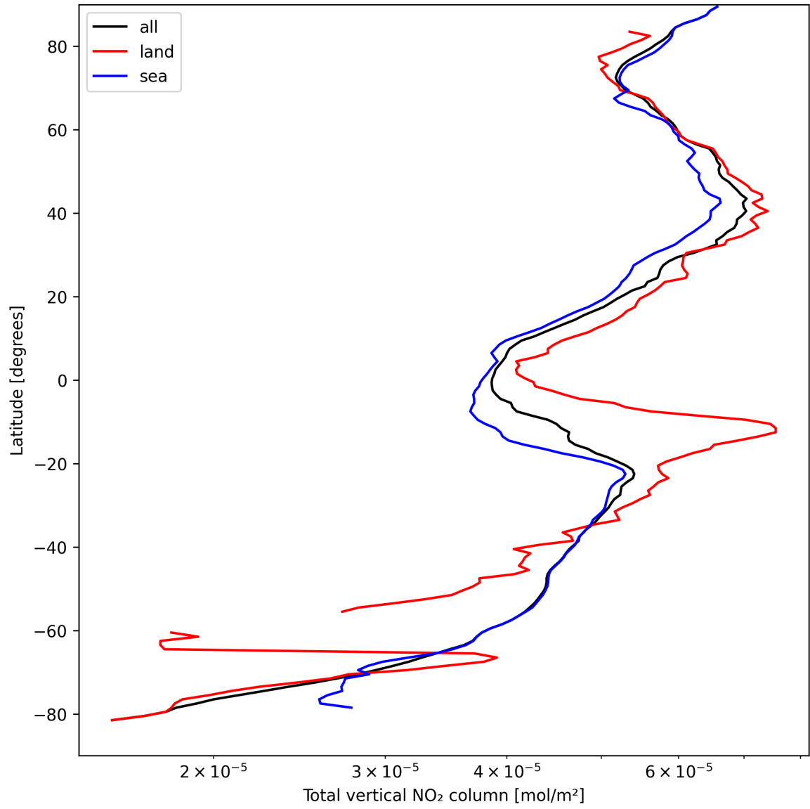
Figure 19: Zonal average of “Total vertical NO 2 column” for 2025-09-06 to 2025-09-07.
