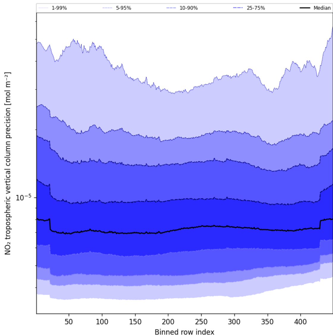
Figure 45: Along track statistics of “NO 2 tropospheric vertical column precision” for 2025-09-06 to 2025-09-07
