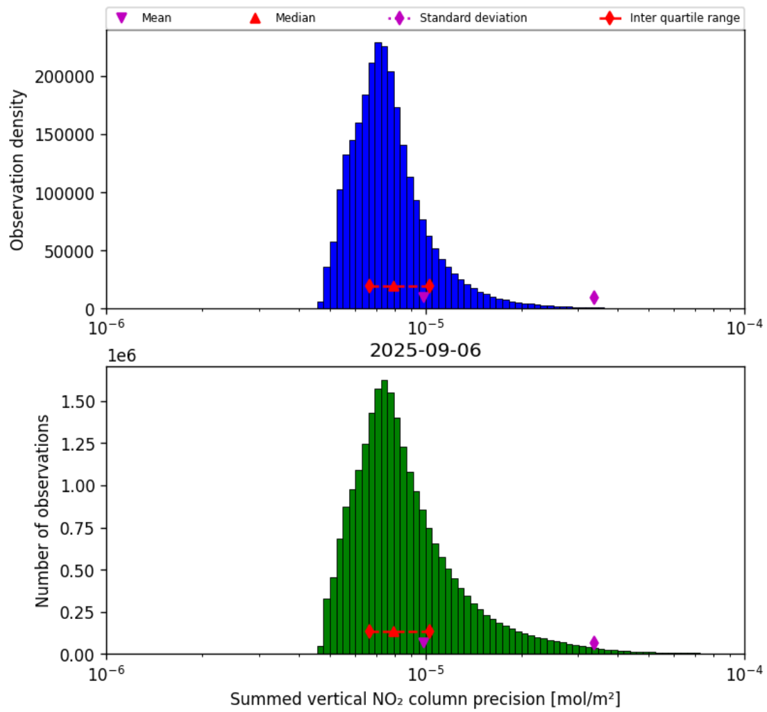
Figure 39: Histogram of "Summed vertical NO 2 column precision" for 2025-09-06 to 2025-09-07
