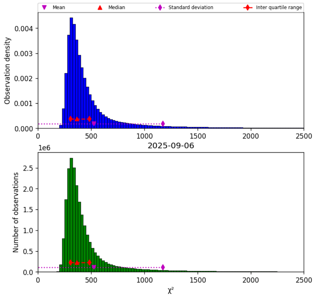
Figure 40: Histogram of “ \chi^2 ” for 2025-09-06 to 2025-09-07
