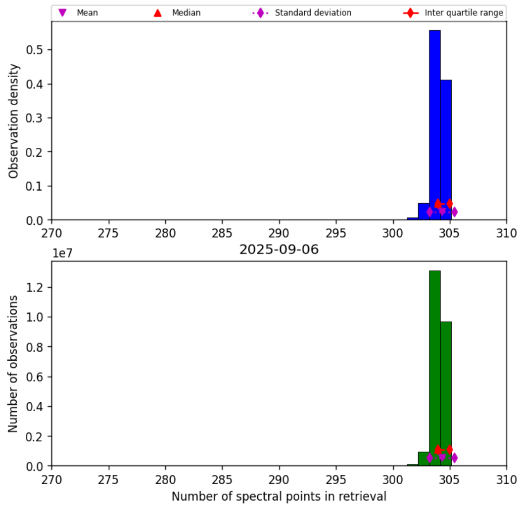
Figure 31: Histogram of “Number of spectral points in retrieval” for 2025-09-06 to 2025-09-07
