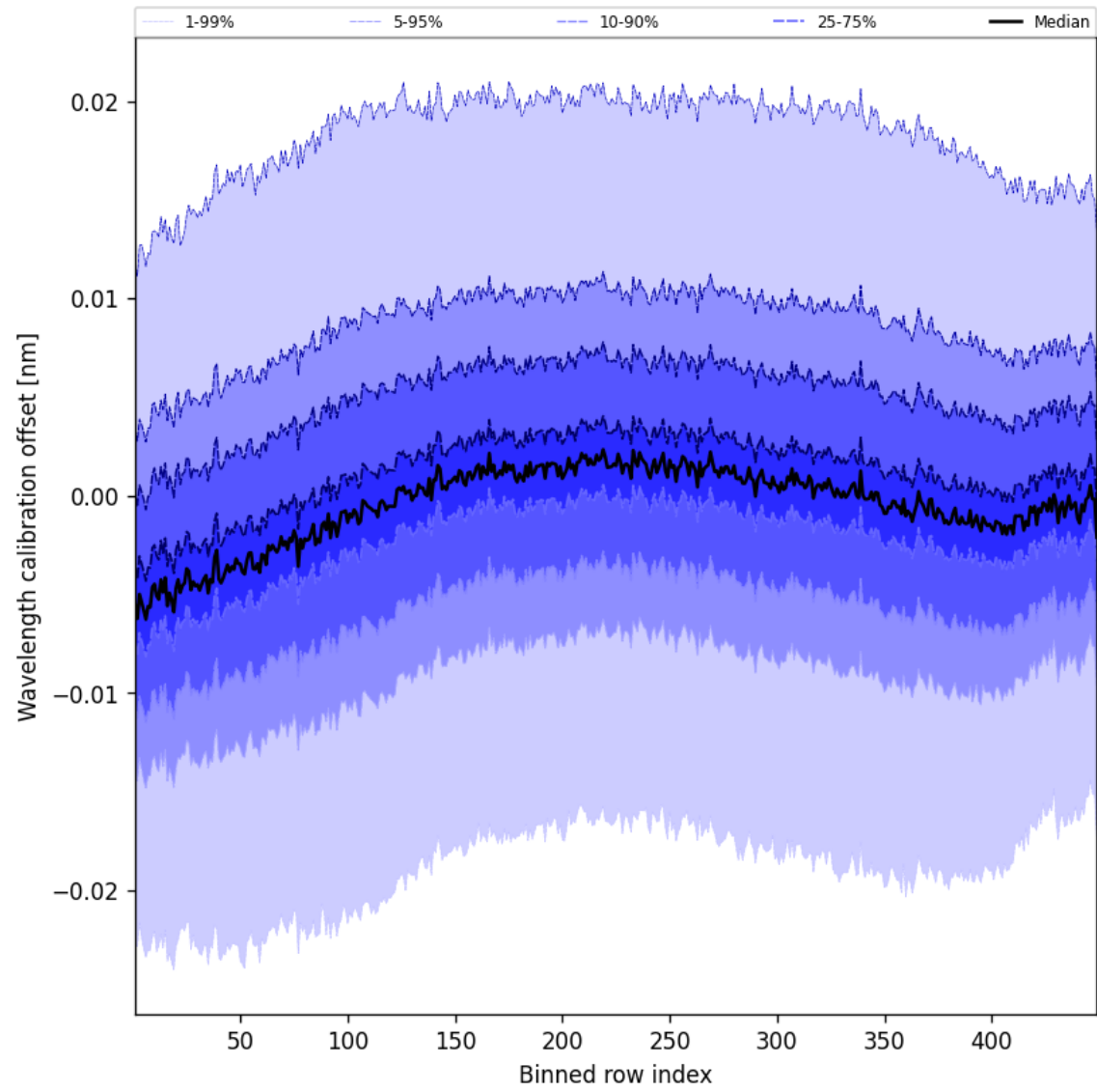
Figure 50: Along track statistics of “Wavelength calibration offset” for 2025-09-06 to 2025-09-07
