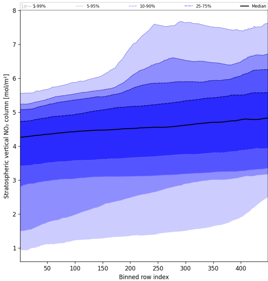
Figure 51: Along track statistics of “Stratospheric vertical NO 2 column” for 2025-09-06 to 2025-09-07
