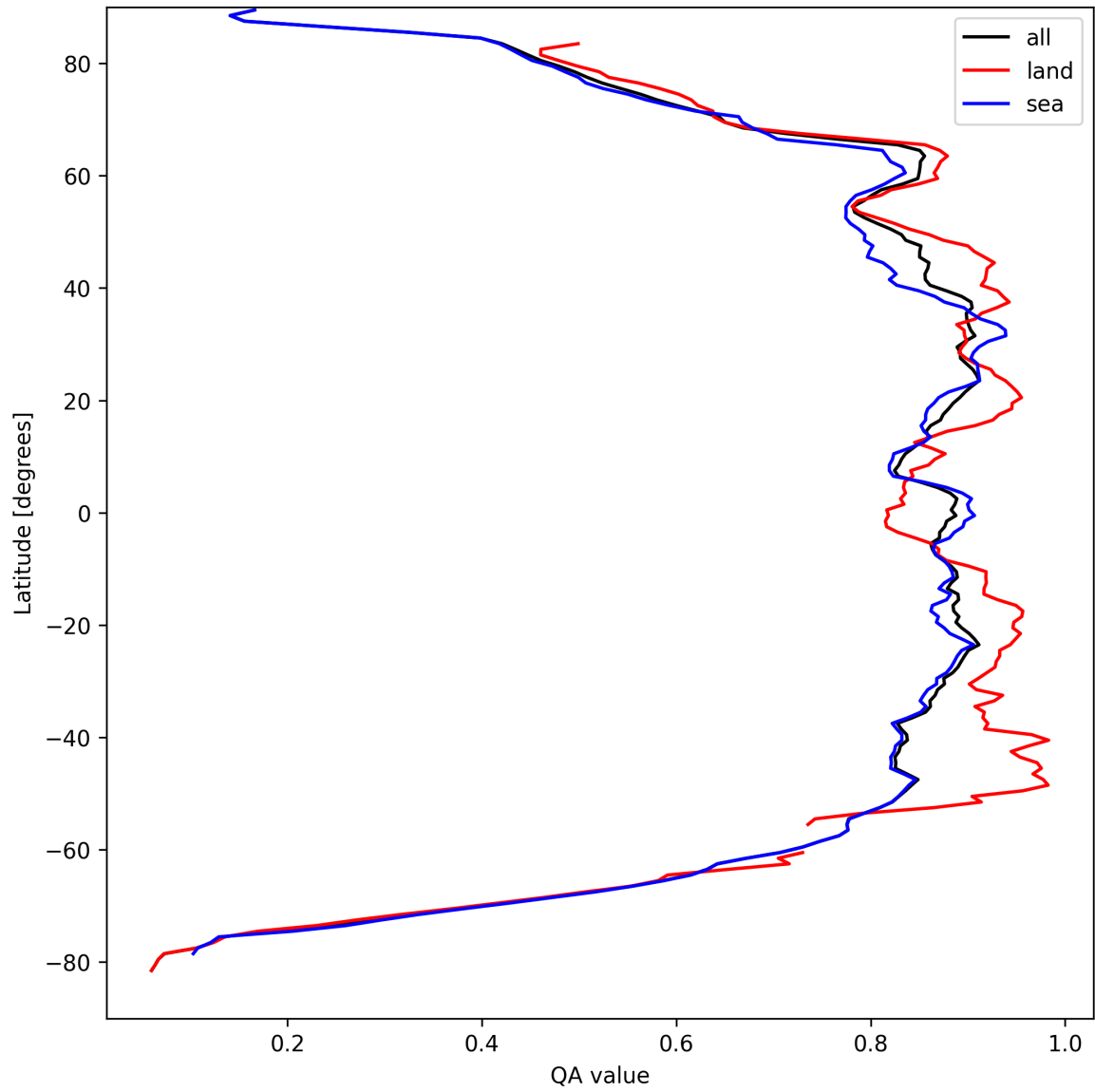
Figure 9: Zonal average of “QA value” for 2025-09-06 to 2025-09-07.
