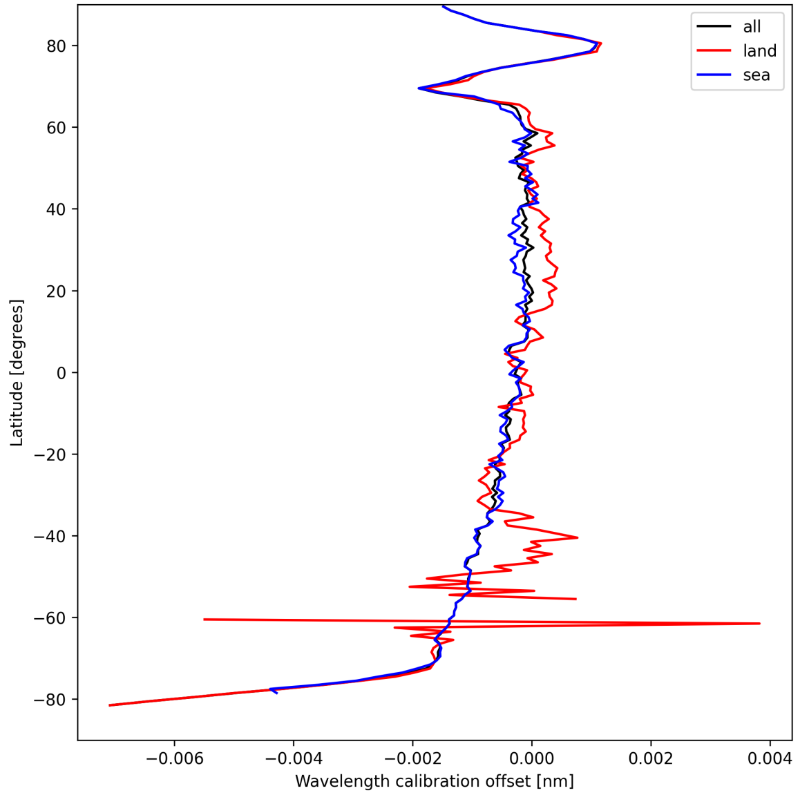
Figure 16: Zonal average of “Wavelength calibration offset” for 2025-09-06 to 2025-09-07.
