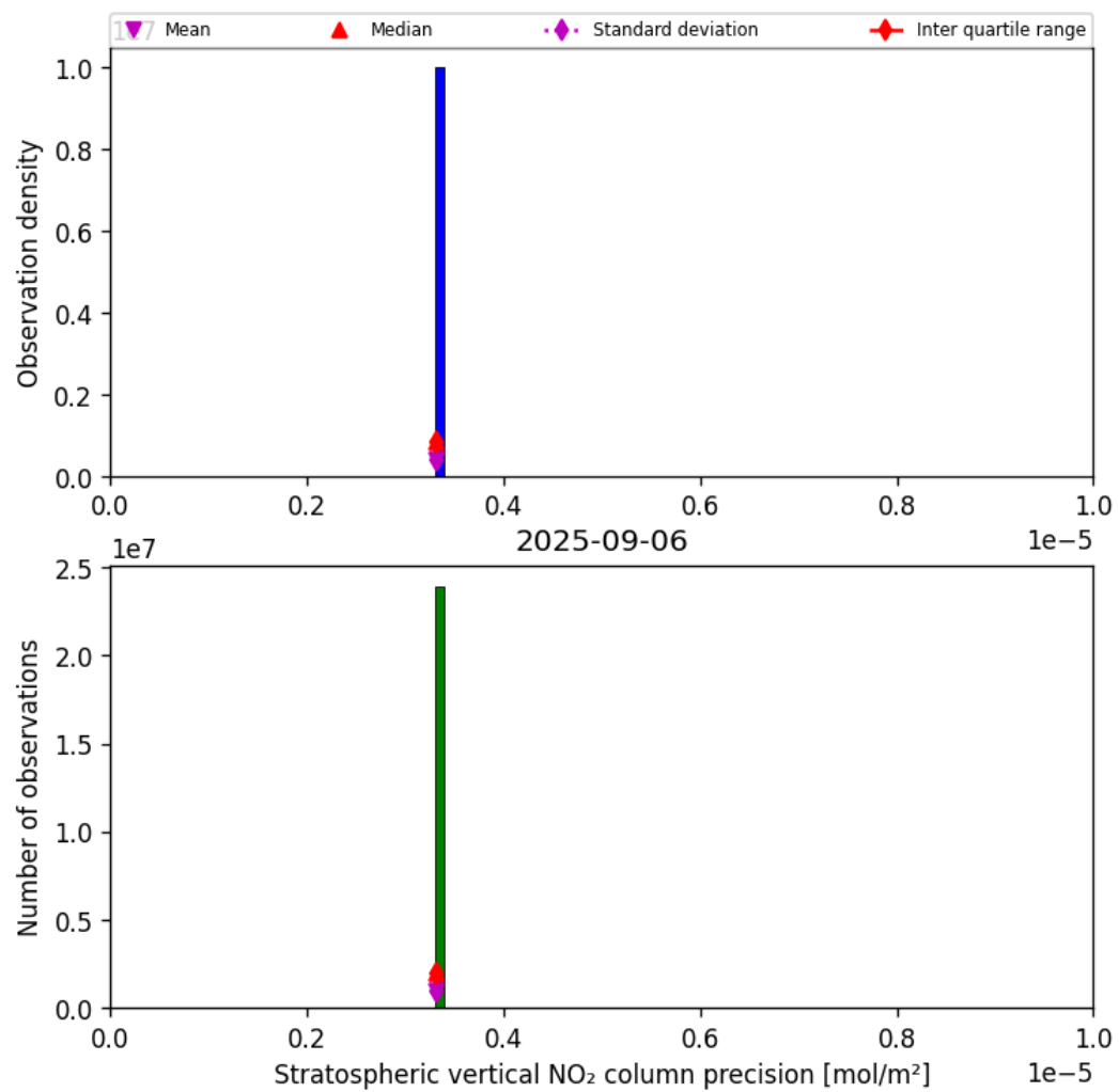
Figure 35: Histogram of “Stratospheric vertical NO 2 column precision” for 2025-09-06 to 2025-09-07
