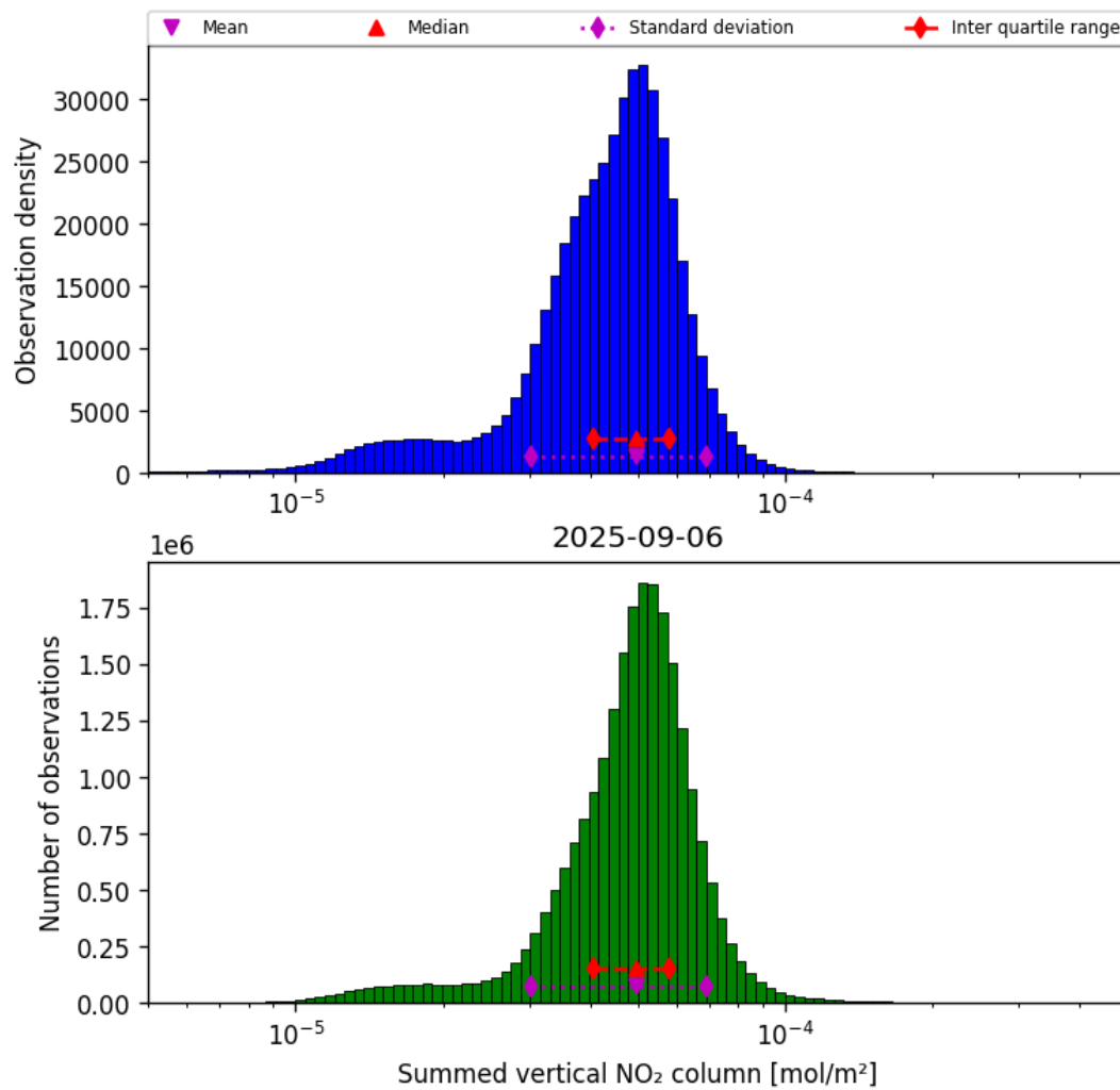
Figure 38: Histogram of “Summed vertical NO 2 column” for 2025-09-06 to 2025-09-07
