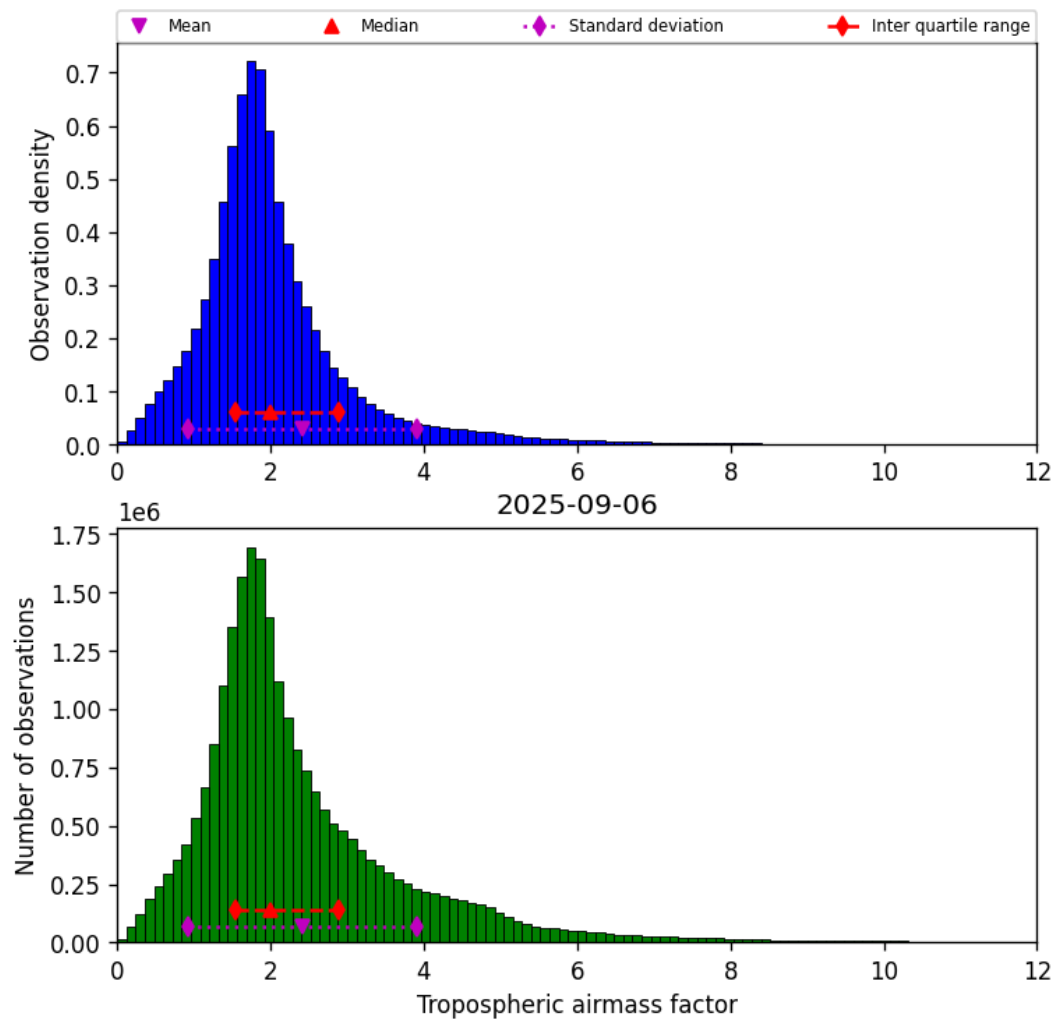
Figure 29: Histogram of “Tropospheric airmass factor” for 2025-09-06 to 2025-09-07
