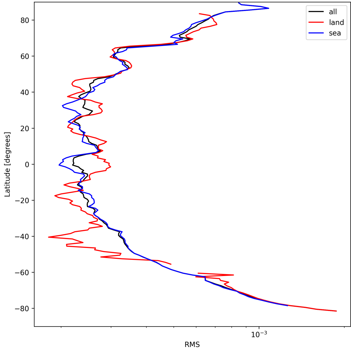
Figure 24: Zonal average of “RMS” for 2025-09-06 to 2025-09-07.
