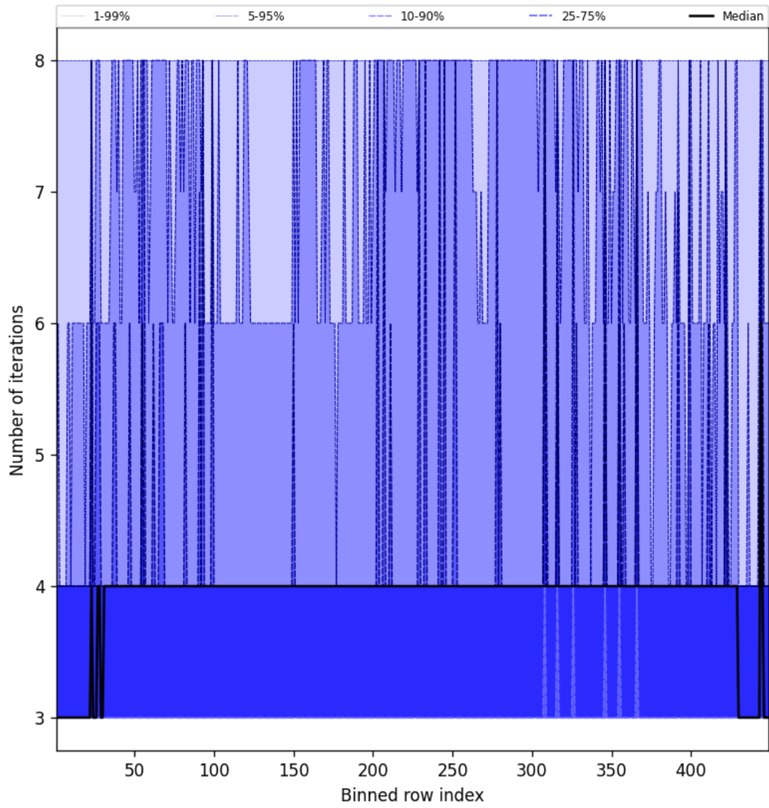
Figure 49: Along track statistics of “Number of iterations” for 2025-09-06 to 2025-09-07
