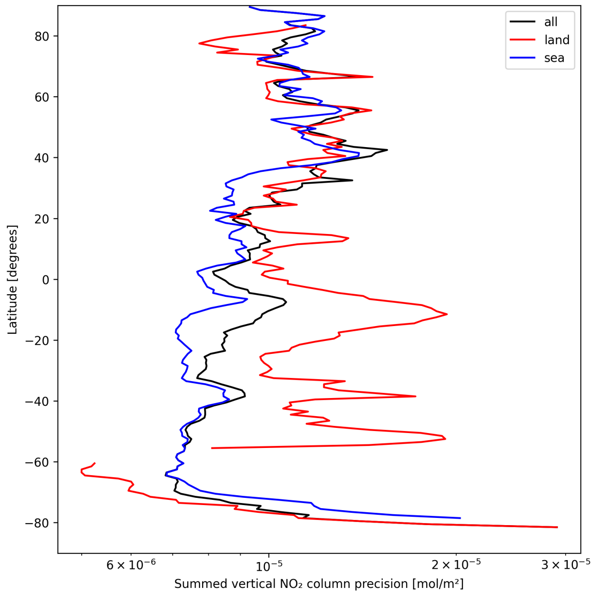
Figure 22: Zonal average of “Summed vertical NO 2 column precision” for 2025-09-06 to 2025-09-07.
