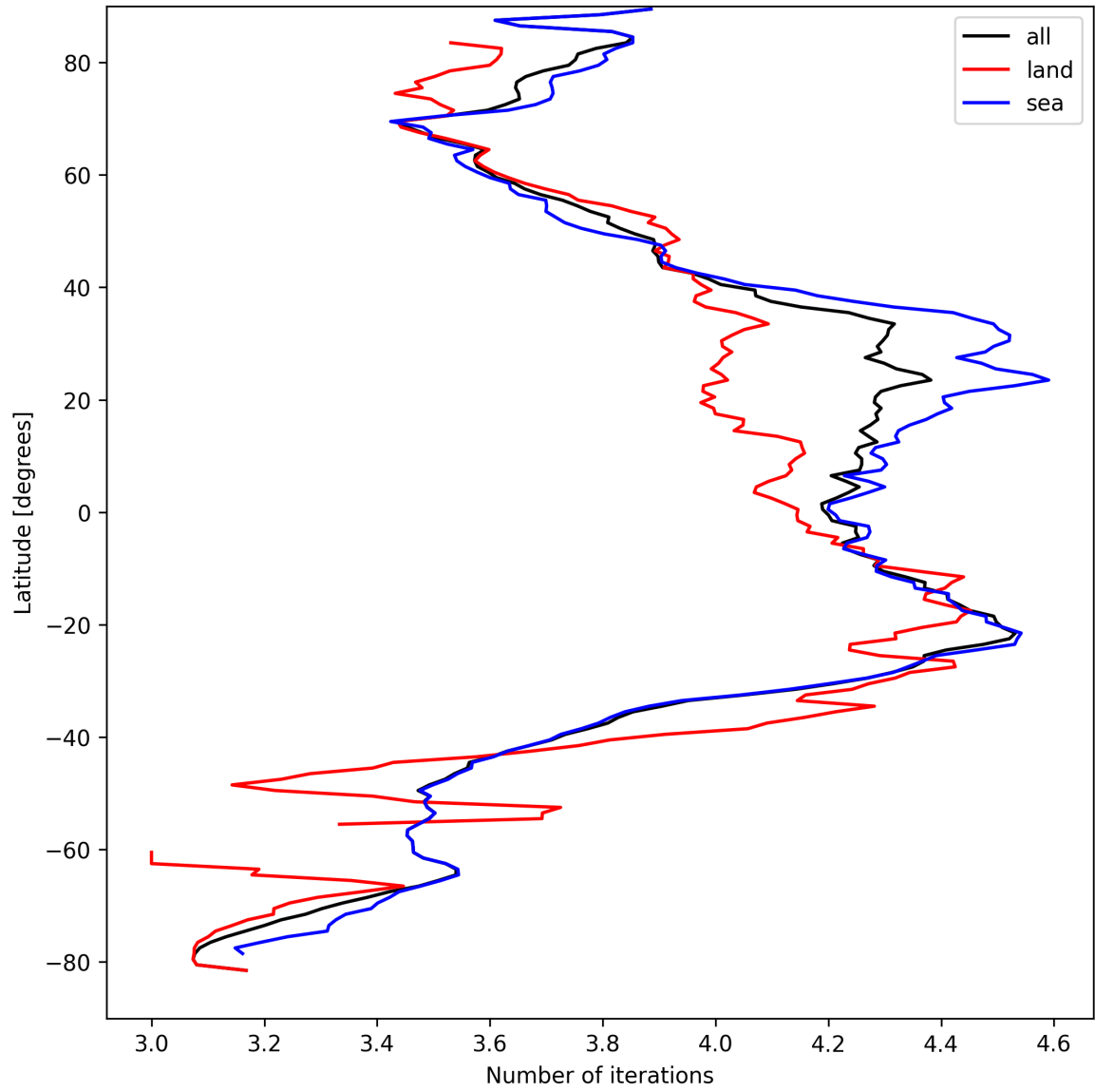
Figure 15: Zonal average of “Number of iterations” for 2025-09-06 to 2025-09-07.
