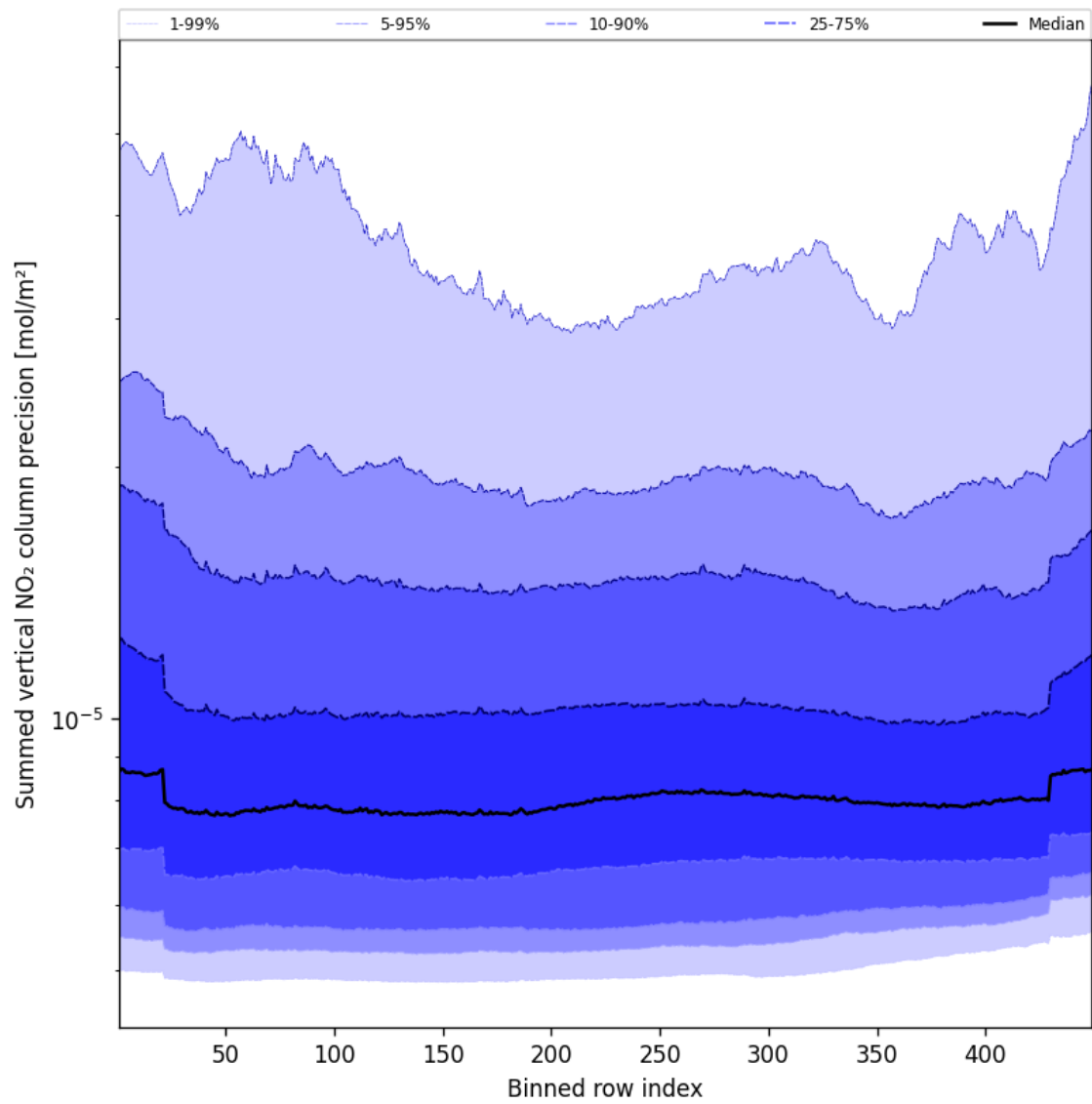
Figure 56: Along track statistics of “Summed vertical NO 2 column precision” for 2025-09-06 to 2025-09-07
