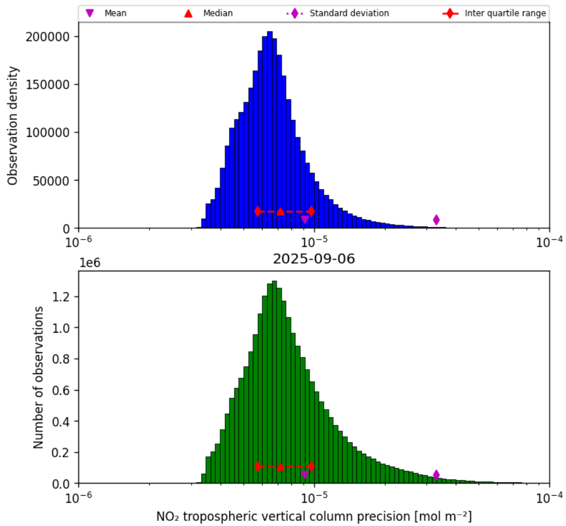
Figure 28: Histogram of “NO 2 tropospheric vertical column precision” for 2025-09-06 to 2025-09-07
