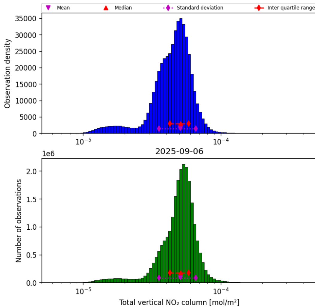
Figure 36: Histogram of “Total vertical NO 2 column” for 2025-09-06 to 2025-09-07
