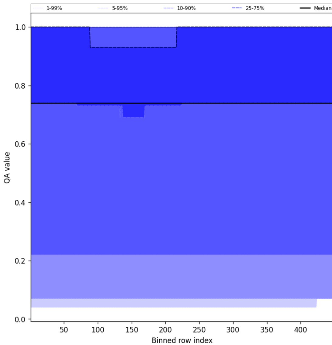
Figure 43: Along track statistics of “QA value” for 2025-09-06 to 2025-09-07
