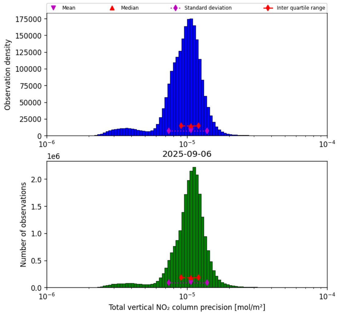
Figure 37: Histogram of “Total vertical NO 2 column precision” for 2025-09-06 to 2025-09-07
