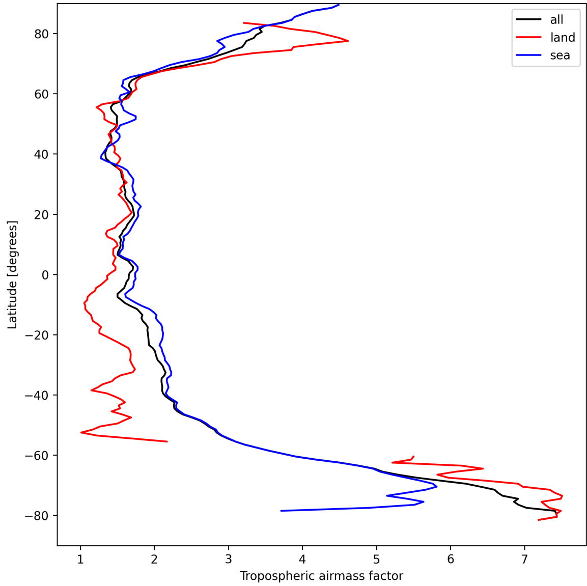
Figure 12: Zonal average of “Tropospheric air mass factor” for 2025-09-06 to 2025-09-07.
