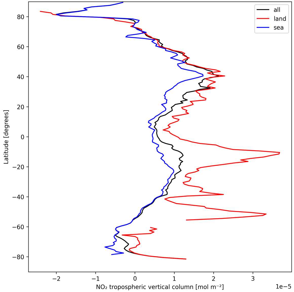
Figure 10: Zonal average of “NO 2 tropospheric vertical column” for 2025-09-06 to 2025-09-07.
