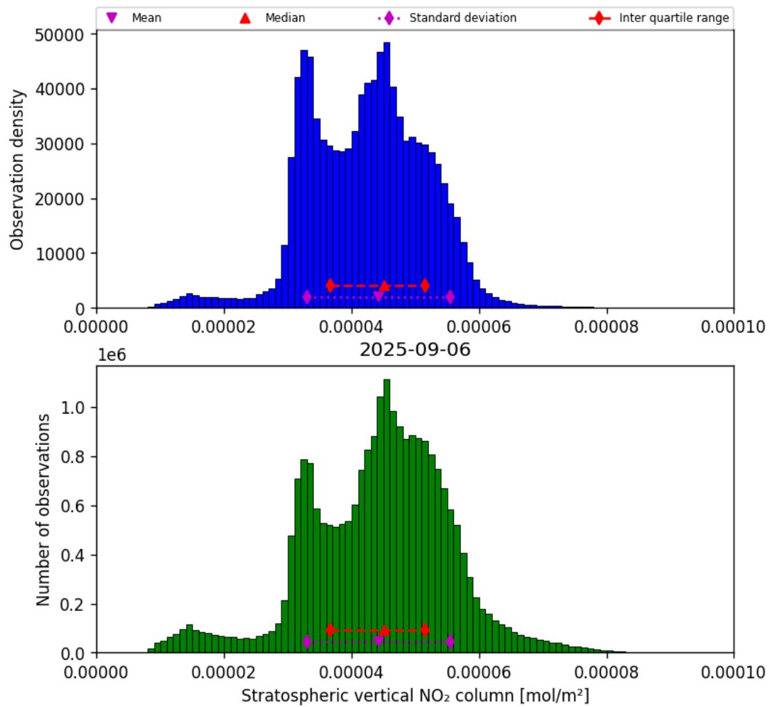
Figure 34: Histogram of “Stratospheric vertical NO 2 column” for 2025-09-06 to 2025-09-07
