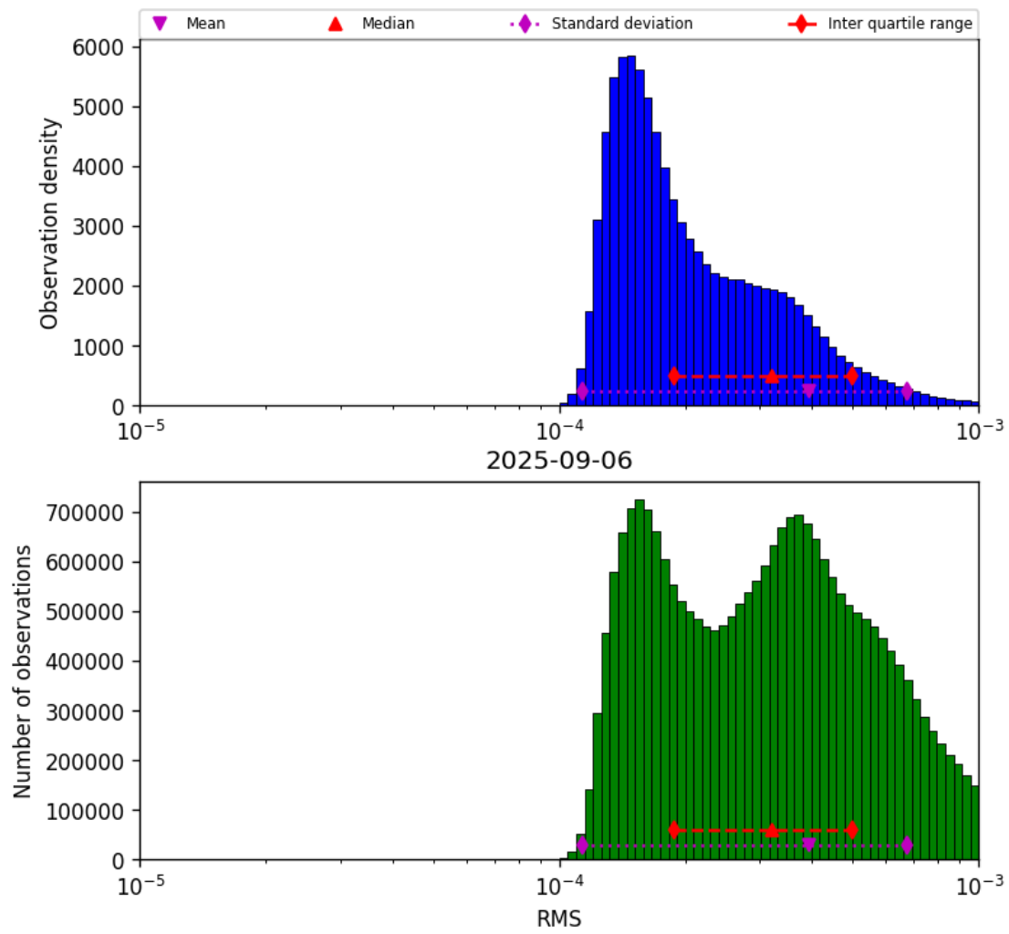
Figure 41: Histogram of “RMS” for 2025-09-06 to 2025-09-07
