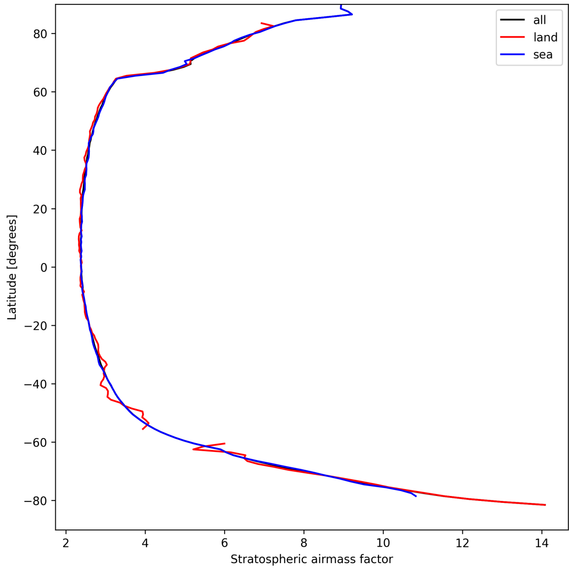
Figure 25: Zonal average of “Stratospheric airmass factor” for 2025-09-06 to 2025-09-07.
