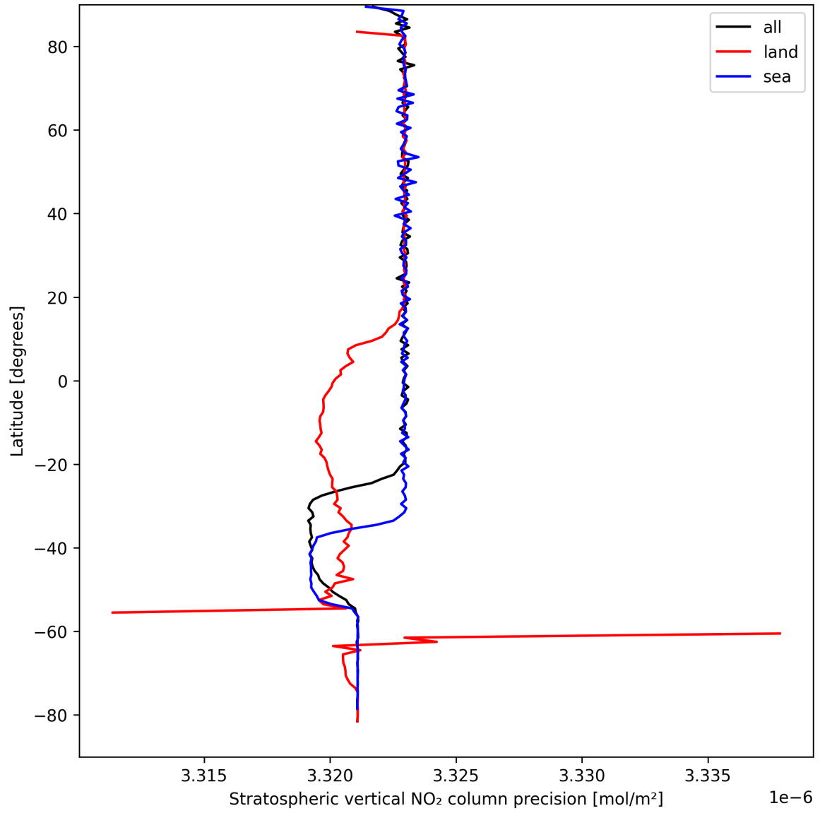
Figure 18: Zonal average of “Stratospheric vertical NO 2 column precision” for 2025-09-06 to 2025-09-07.
