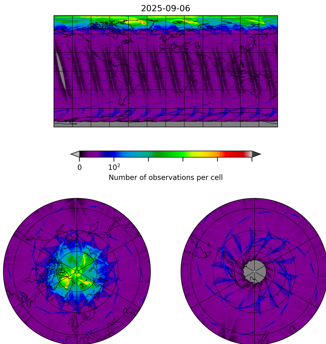
Figure 8: Map of the number of observations for 2025-09-06 to 2025-09-07
