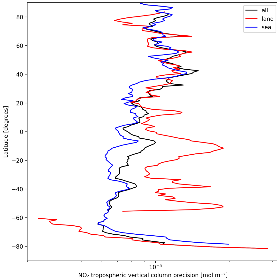
Figure 11: Zonal average of “NO 2 tropospheric vertical column precision” for 2025-09-06 to 2025-09-07.
