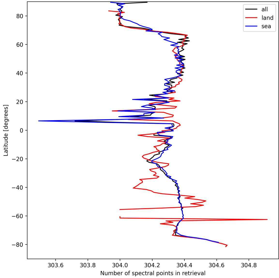
Figure 14: Zonal average of “Number of spectral points in retrieval” for 2025-09-06 to 2025-09-07.
