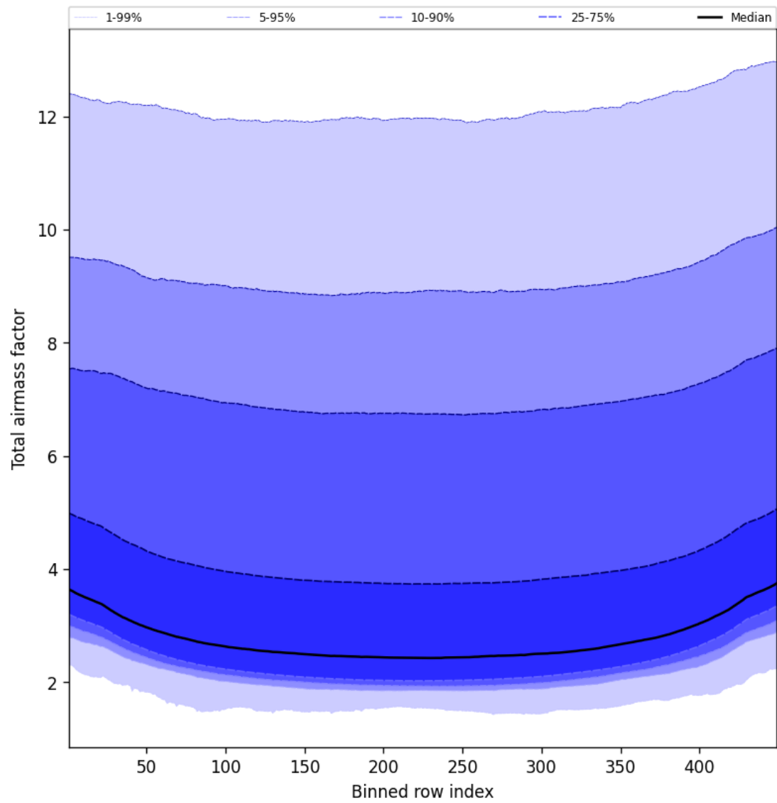
Figure 47: Along track statistics of “Total airmass factor” for 2025-09-06 to 2025-09-07
