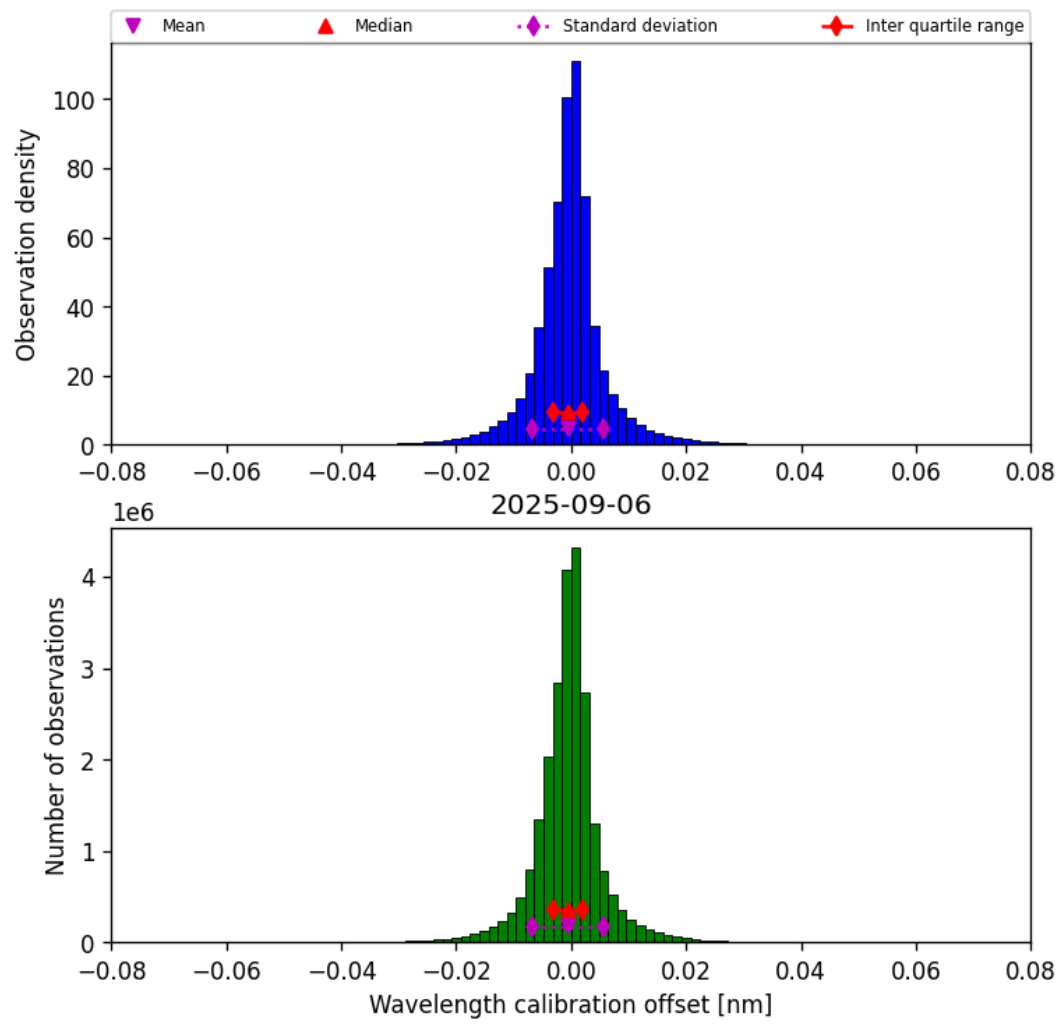
Figure 33: Histogram of “Wavelength calibration offset” for 2025-09-06 to 2025-09-07
