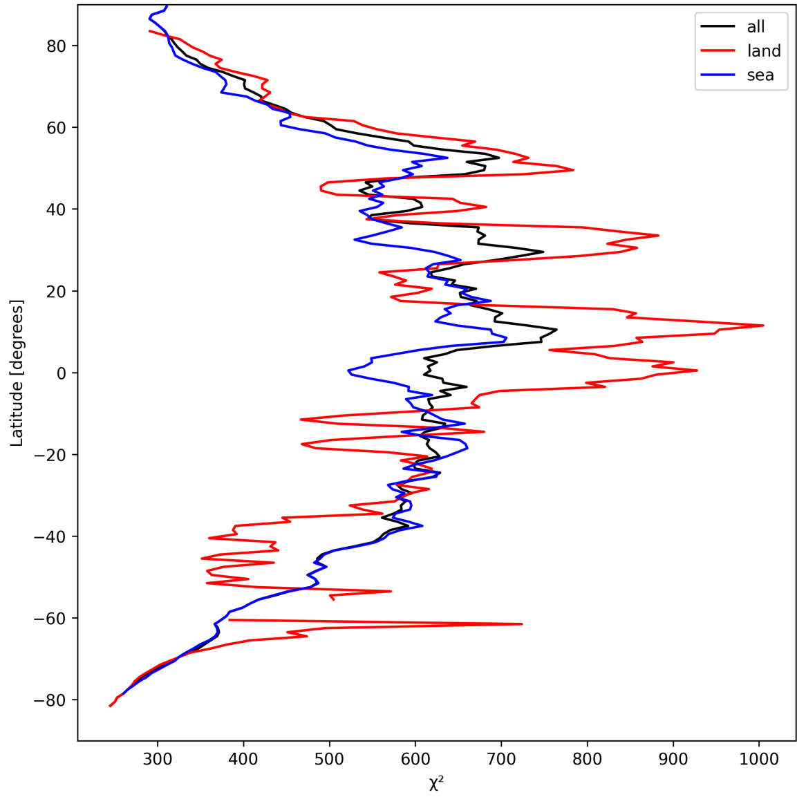
Figure 23: Zonal average of “ \chi^2 ” for 2025-09-06 to 2025-09-07.
