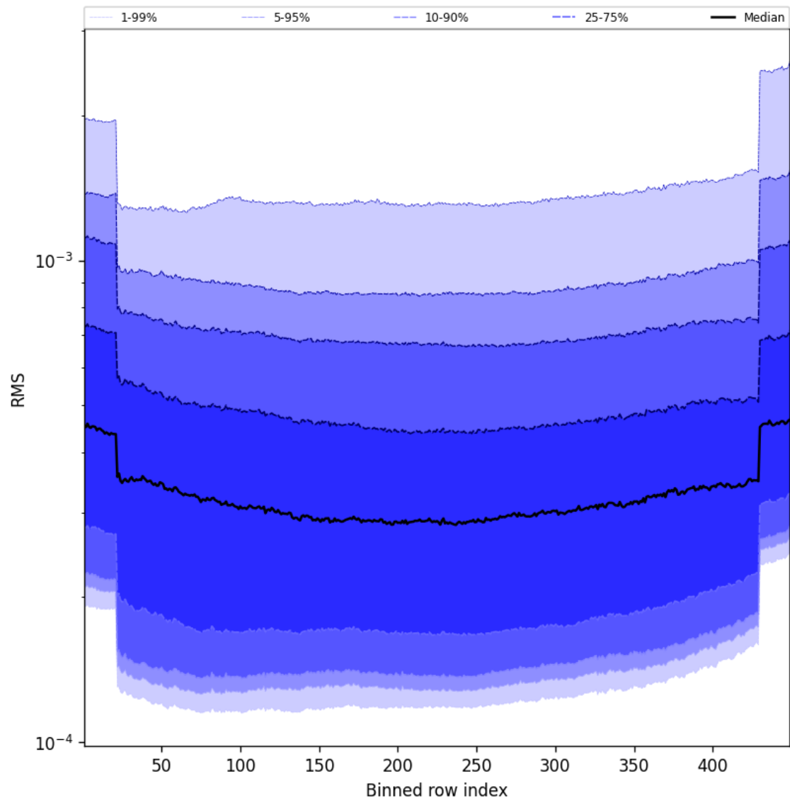
Figure 58: Along track statistics of “RMS” for 2025-09-06 to 2025-09-07
