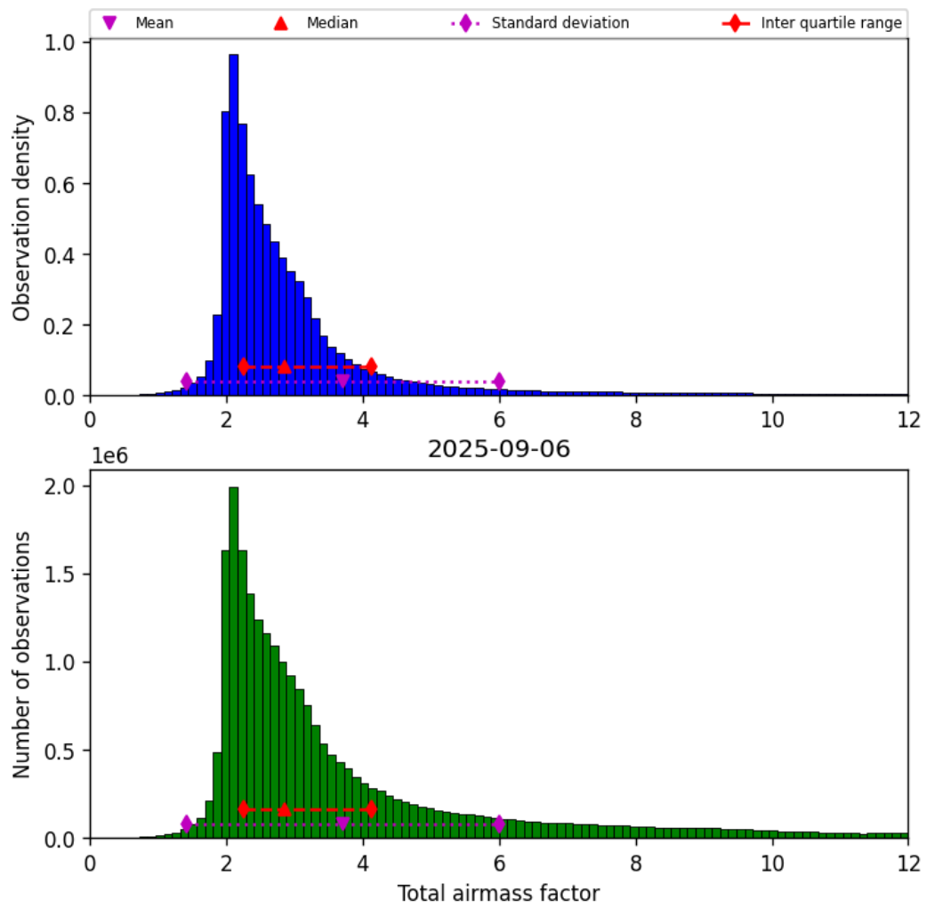
Figure 30: Histogram of “Total airmass factor” for 2025-09-06 to 2025-09-07
