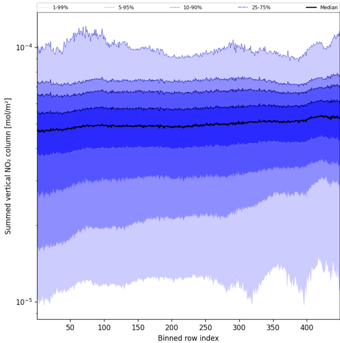
Figure 55: Along track statistics of “Summed vertical NO 2 column” for 2025-09-06 to 2025-09-07
