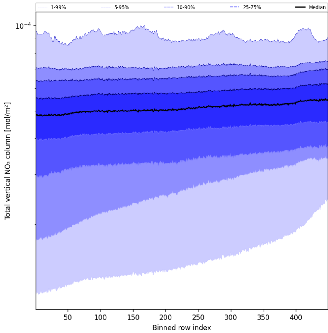
Figure 53: Along track statistics of “Total vertical NO 2 column” for 2025-09-06 to 2025-09-07
