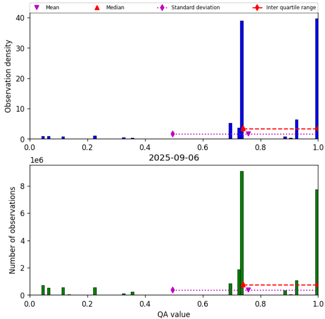
Figure 26: Histogram of “QA value” for 2025-09-06 to 2025-09-07
