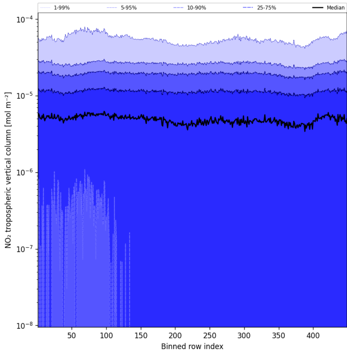
Figure 44: Along track statistics of “NO 2 tropospheric vertical column” for 2025-09-06 to 2025-09-07
