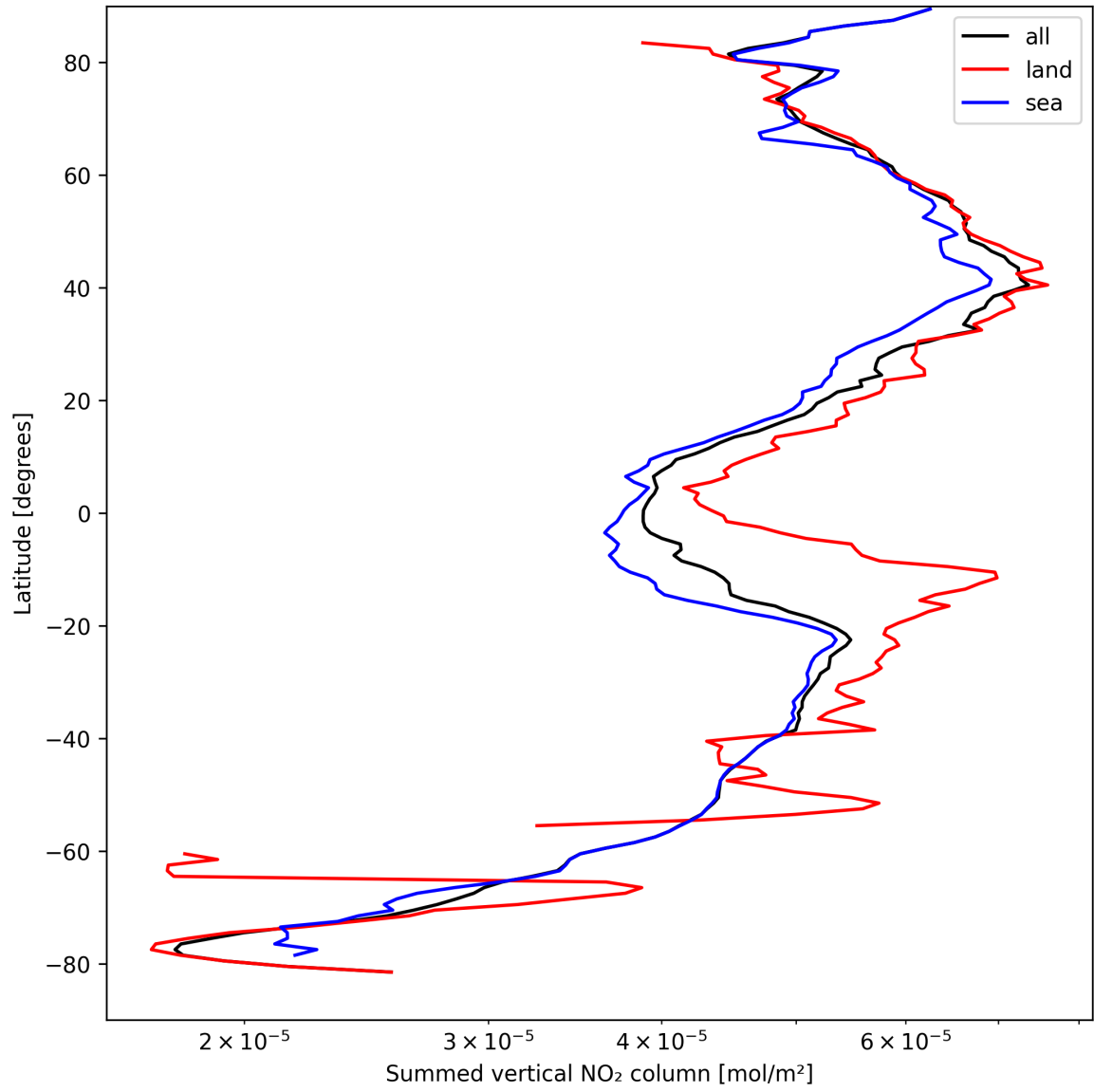
Figure 21: Zonal average of “Summed vertical NO 2 column” for 2025-09-06 to 2025-09-07.
