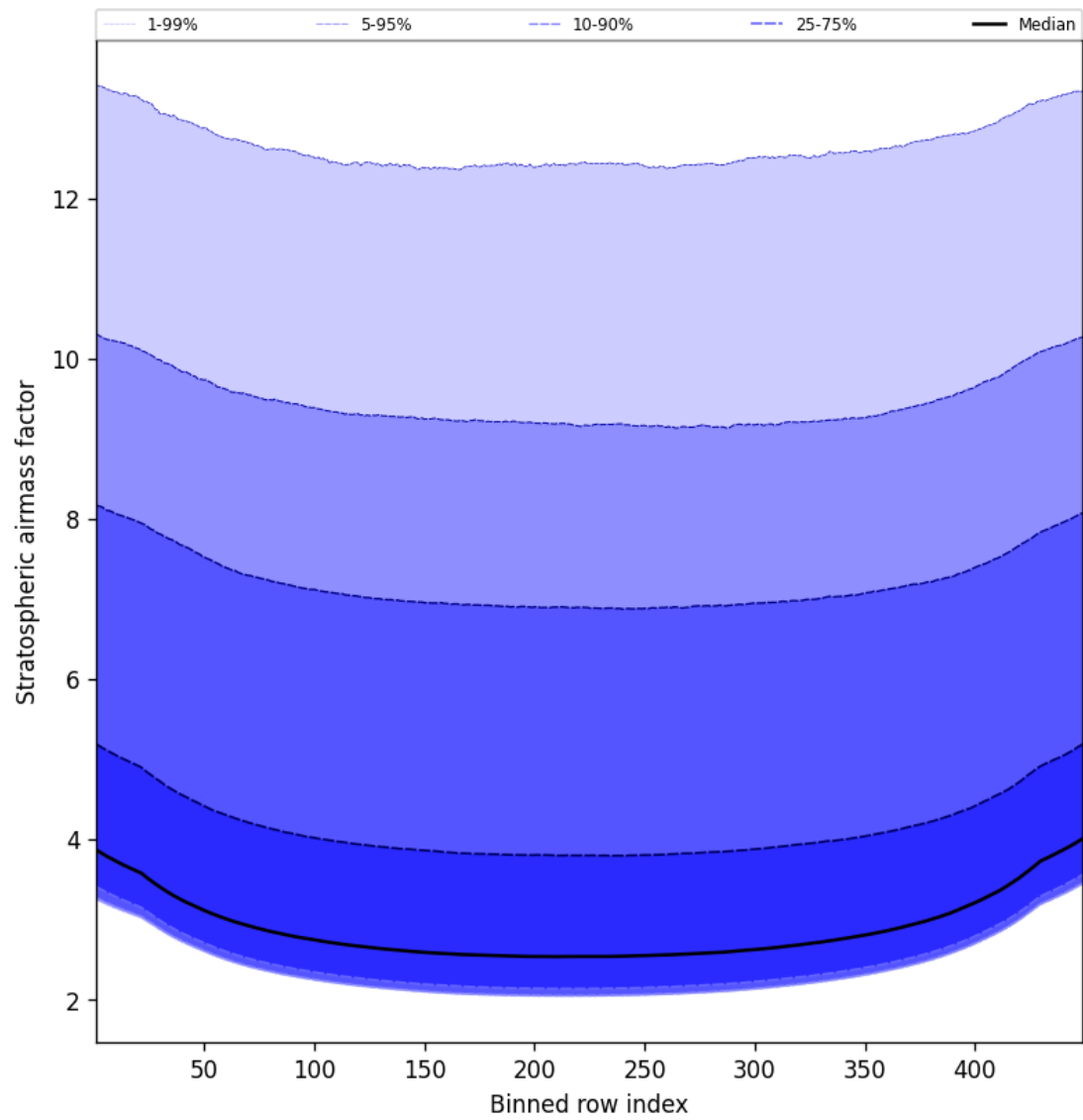
Figure 59: Along track statistics of “Stratospheric airmass factor” for 2025-09-06 to 2025-09-07
