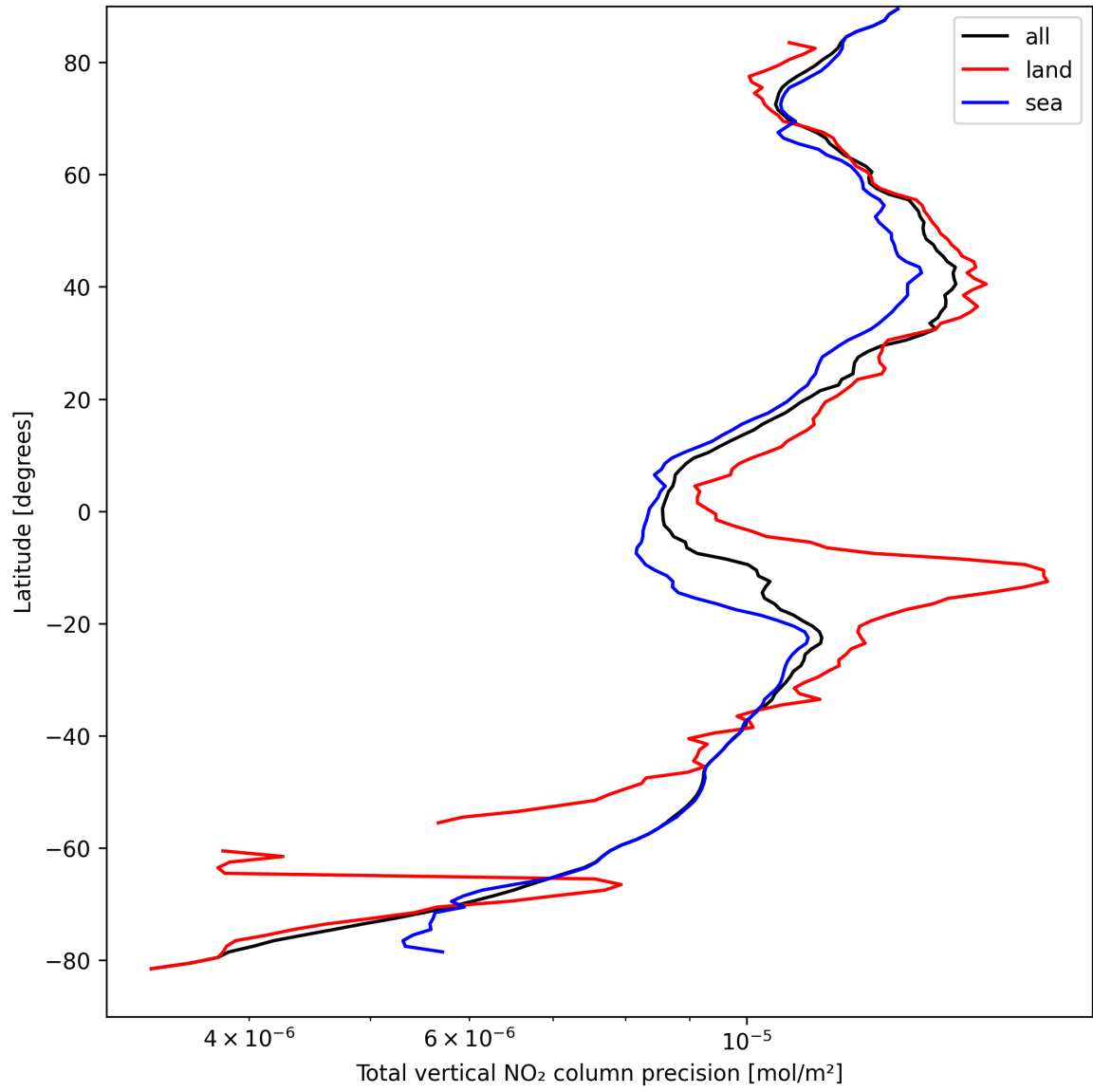
Figure 20: Zonal average of “Total vertical NO 2 column precision” for 2025-09-06 to 2025-09-07.
