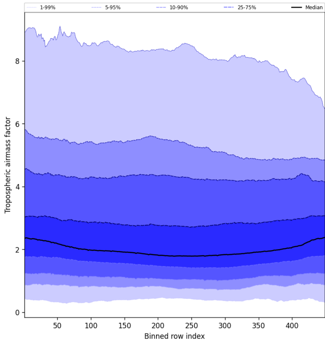
Figure 46: Along track statistics of “Tropospheric air mass factor” for 2025-09-06 to 2025-09-07
