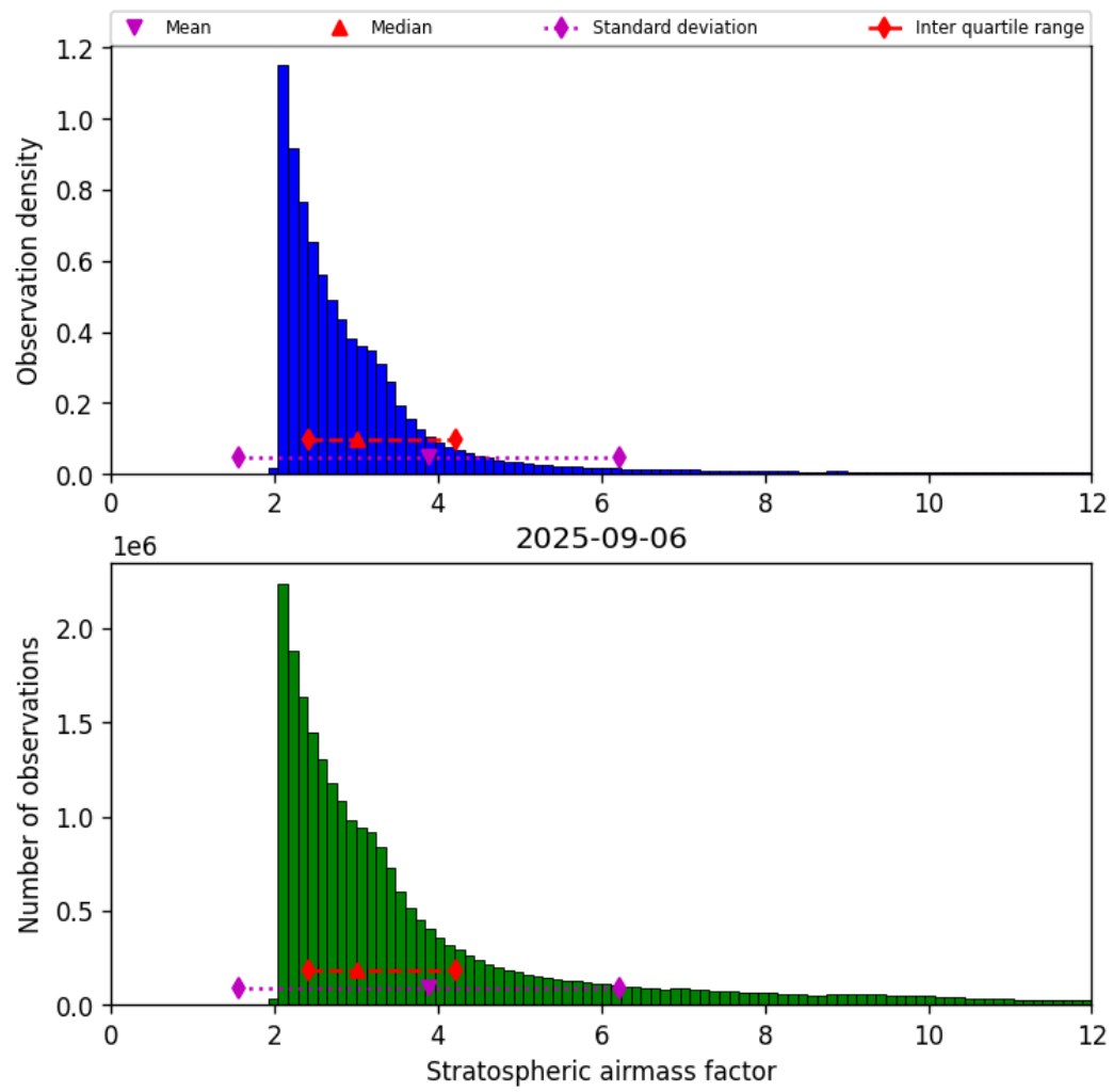
Figure 42: Histogram of “Stratospheric airmass factor” for 2025-09-06 to 2025-09-07
