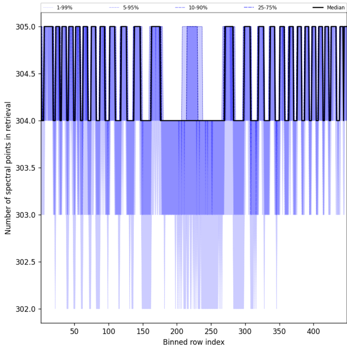
Figure 48: Along track statistics of “Number of spectral points in retrieval” for 2025-09-06 to 2025-09-07
