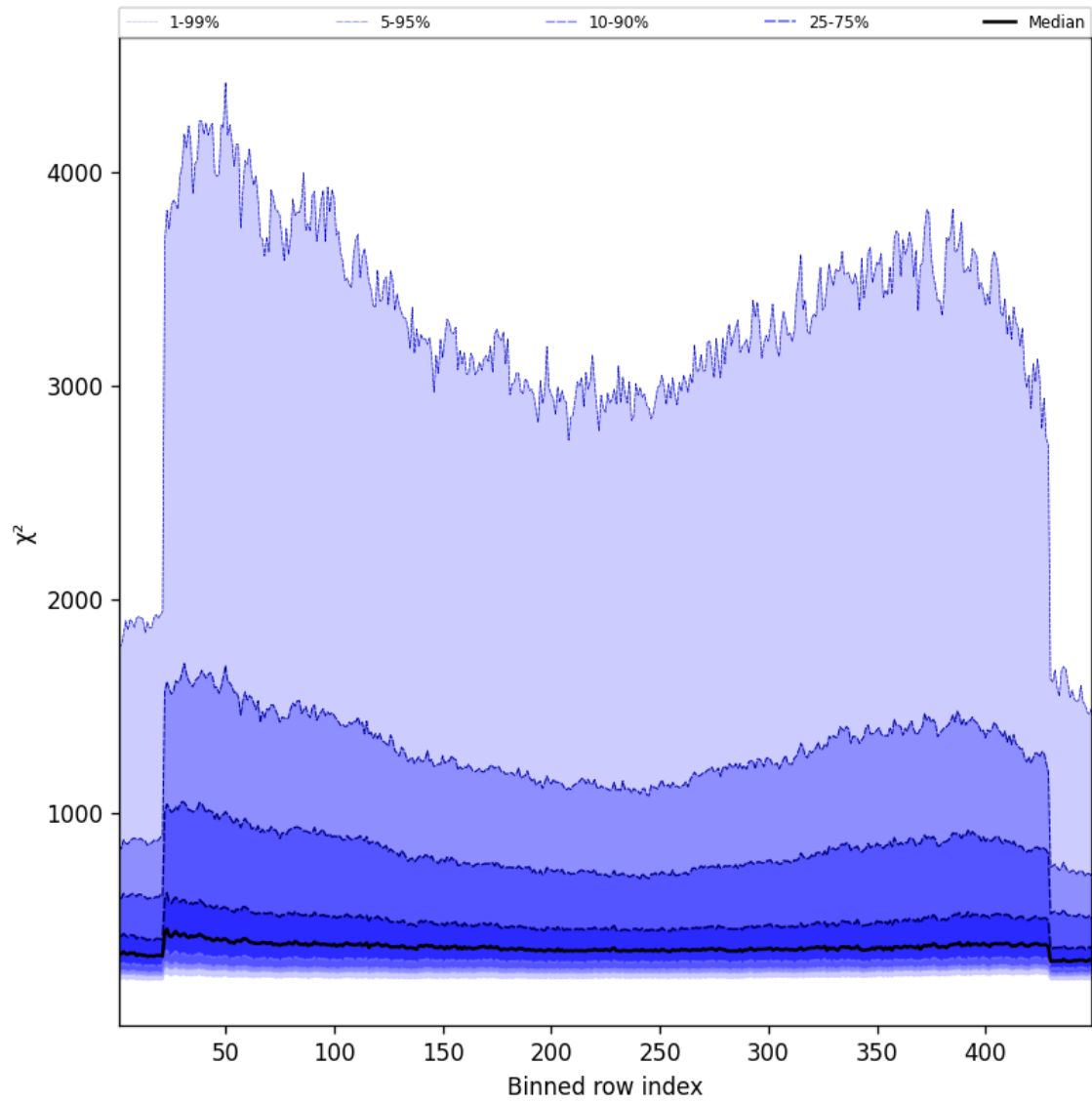
Figure 57: Along track statistics of “ \chi^2 ” for 2025-09-06 to 2025-09-07
