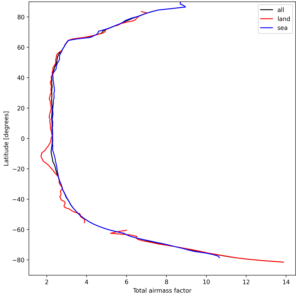
Figure 13: Zonal average of “Total airmass factor” for 2025-09-06 to 2025-09-07.
