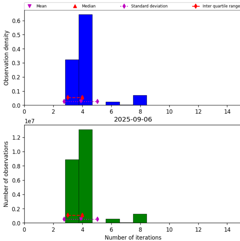
Figure 32: Histogram of “Number of iterations” for 2025-09-06 to 2025-09-07
