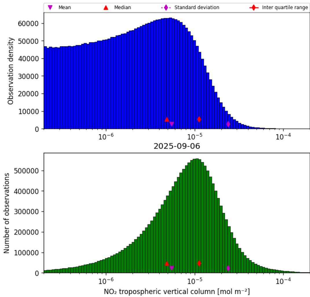
Figure 27: Histogram of “NO 2 tropospheric vertical column” for 2025-09-06 to 2025-09-07
