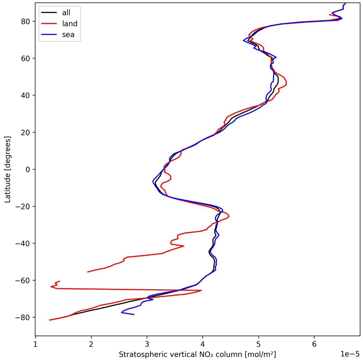
Figure 17: Zonal average of “Stratospheric vertical NO 2 column” for 2025-09-06 to 2025-09-07.
