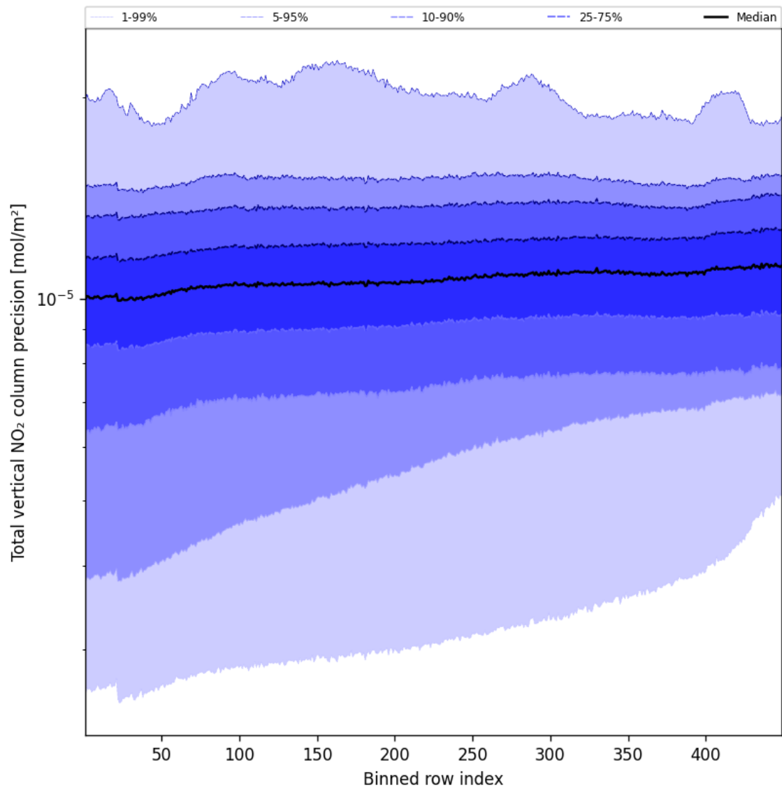
Figure 54: Along track statistics of “Total vertical NO 2 column precision” for 2025-09-06 to 2025-09-07
