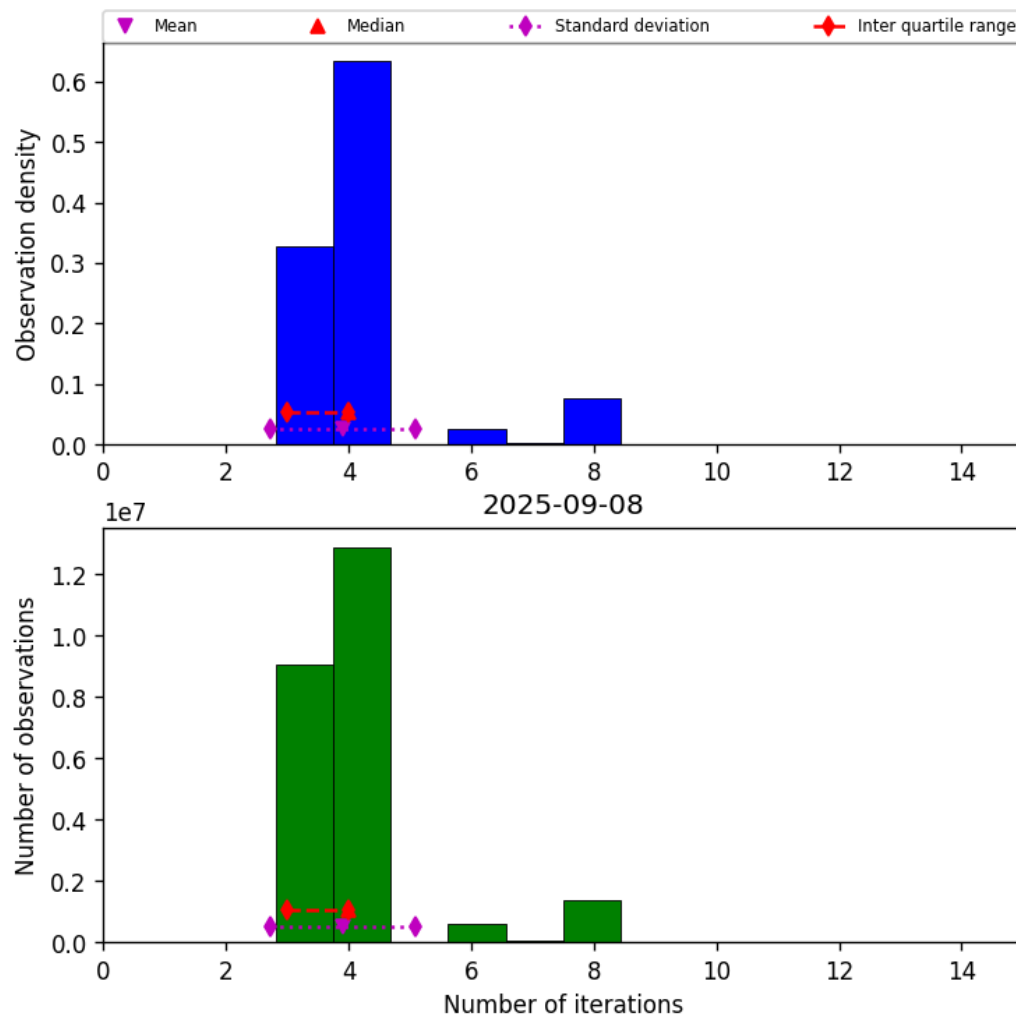
Figure 32: Histogram of “Number of iterations” for 2025-09-08 to 2025-09-08
