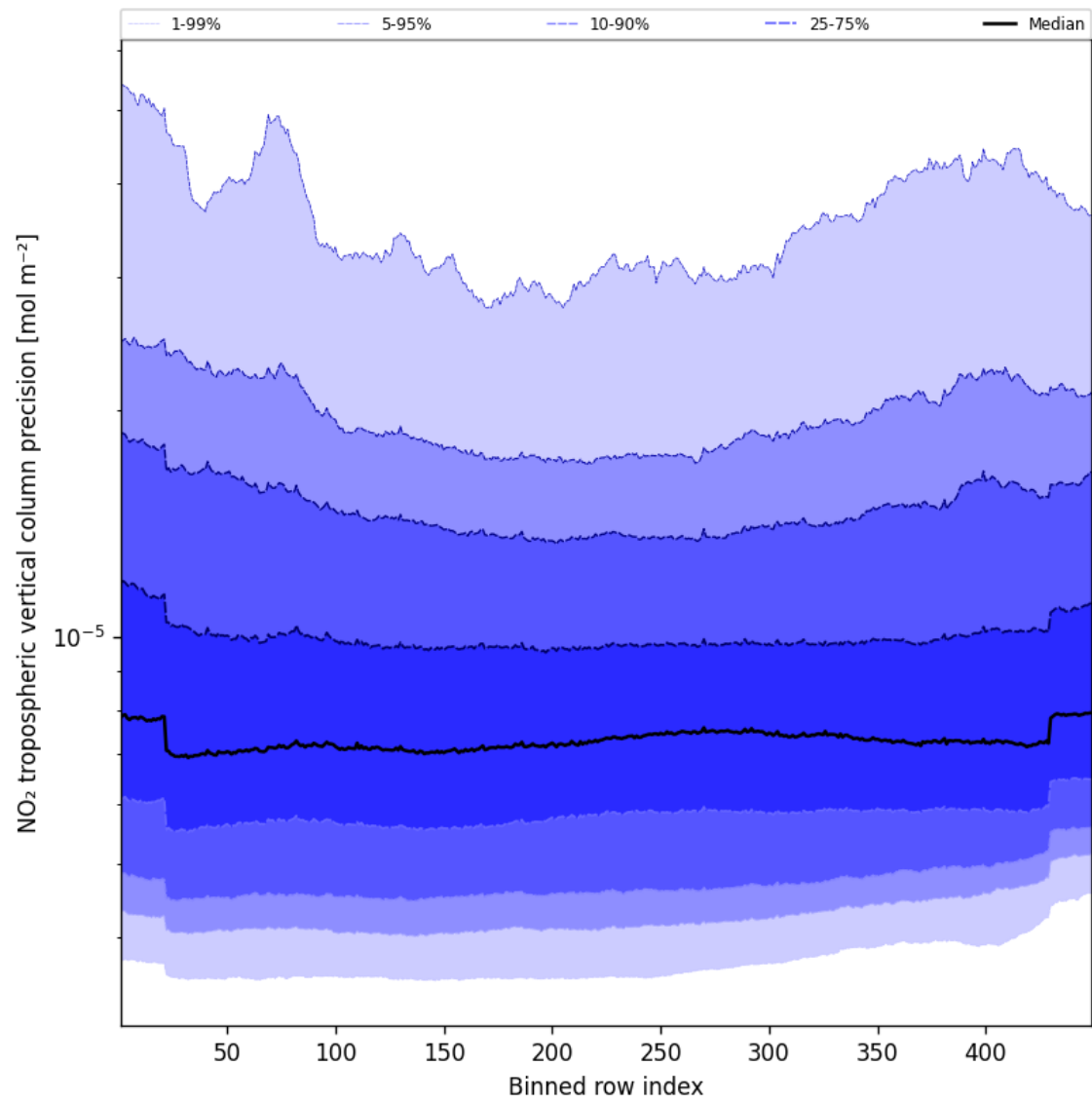
Figure 45: Along track statistics of “NO 2 tropospheric vertical column precision” for 2025-09-08 to 2025-09-08
