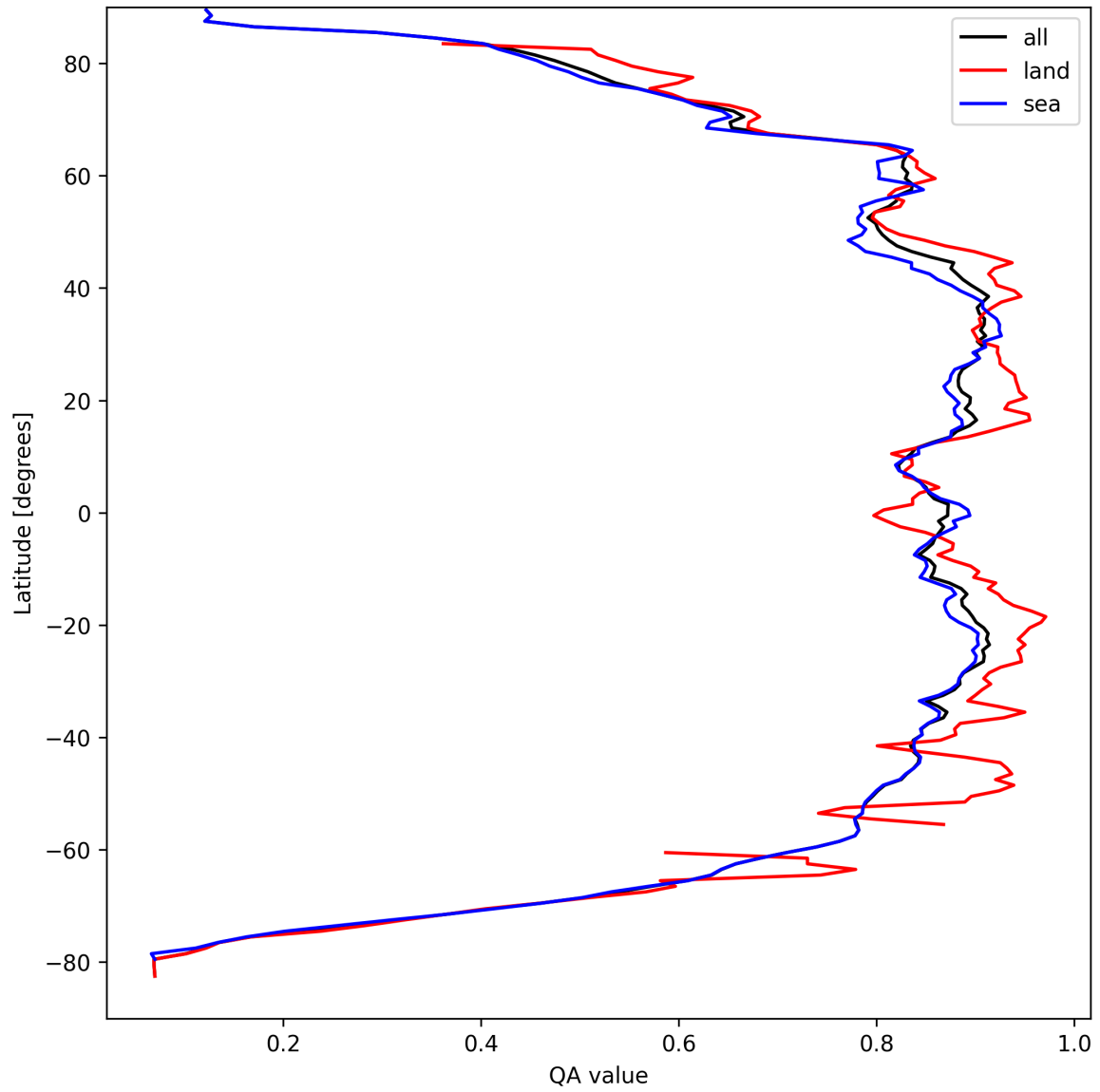
Figure 9: Zonal average of “QA value” for 2025-09-08 to 2025-09-08.
