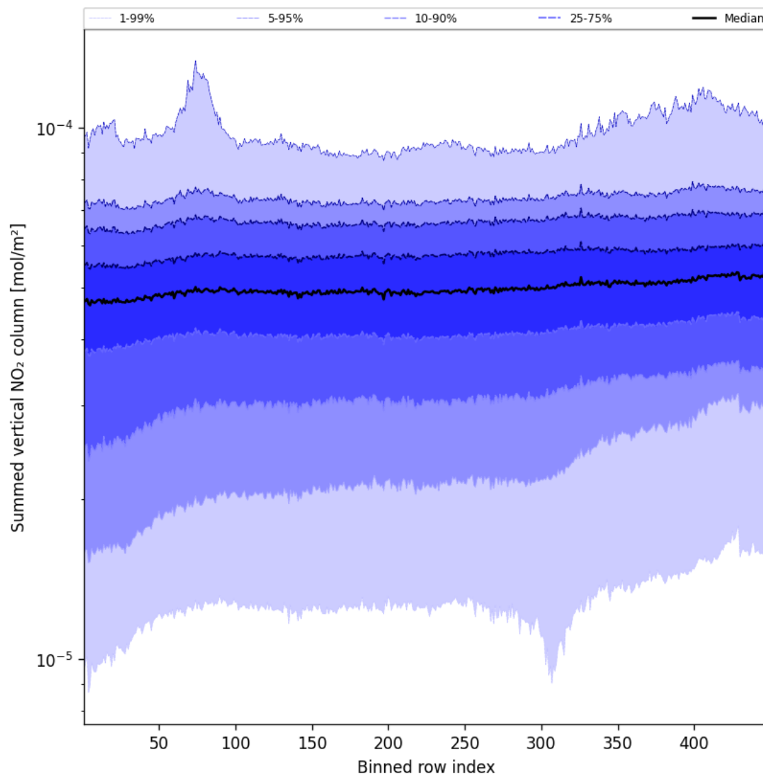
Figure 55: Along track statistics of “Summed vertical NO 2 column” for 2025-09-08 to 2025-09-08
