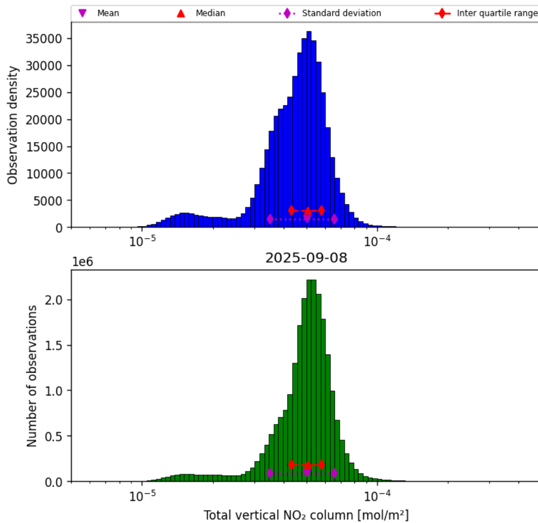
Figure 36: Histogram of "Total vertical NO 2 column" for 2025-09-08 to 2025-09-08
