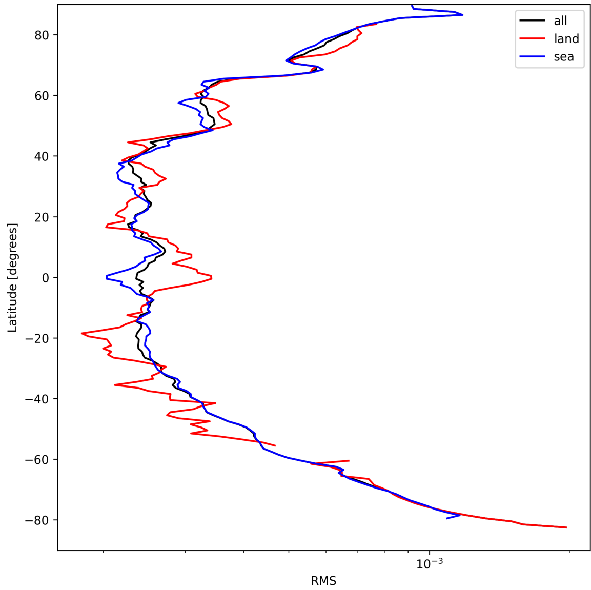
Figure 24: Zonal average of “RMS” for 2025-09-08 to 2025-09-08.
