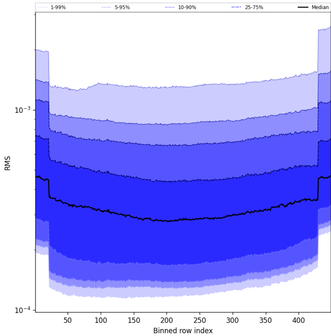
Figure 58: Along track statistics of “RMS” for 2025-09-08 to 2025-09-08
