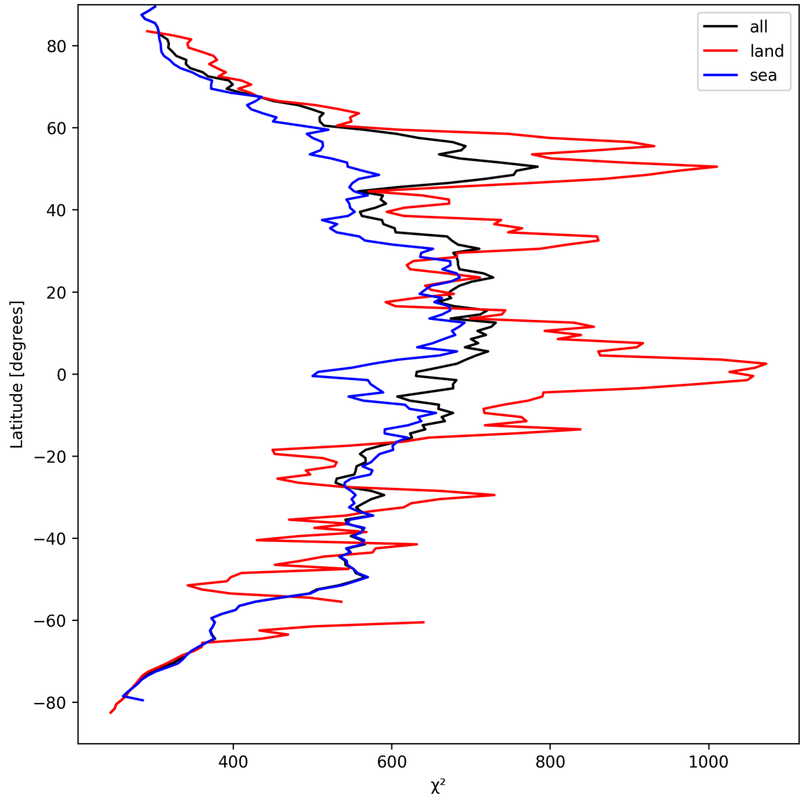
Figure 23: Zonal average of “ \chi^2 ” for 2025-09-08 to 2025-09-08.
