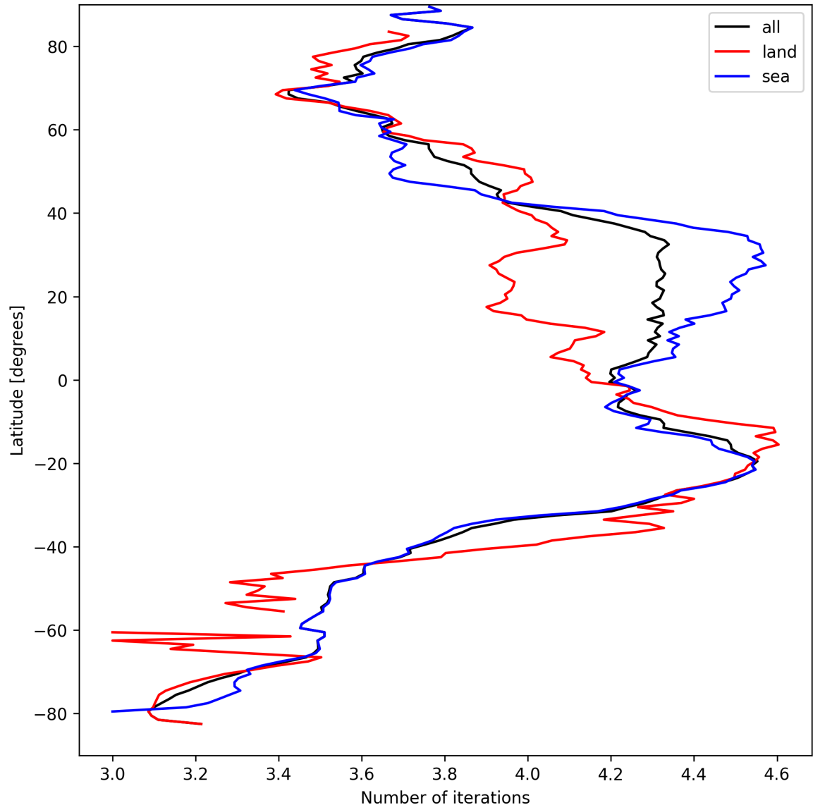
Figure 15: Zonal average of “Number of iterations” for 2025-09-08 to 2025-09-08.
