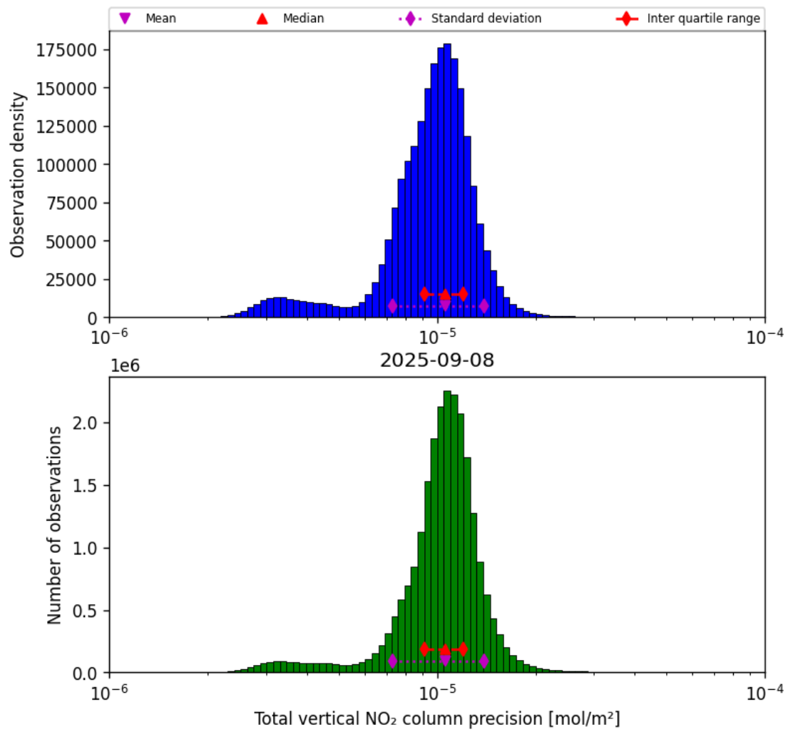
Figure 37: Histogram of “Total vertical NO 2 column precision” for 2025-09-08 to 2025-09-08
