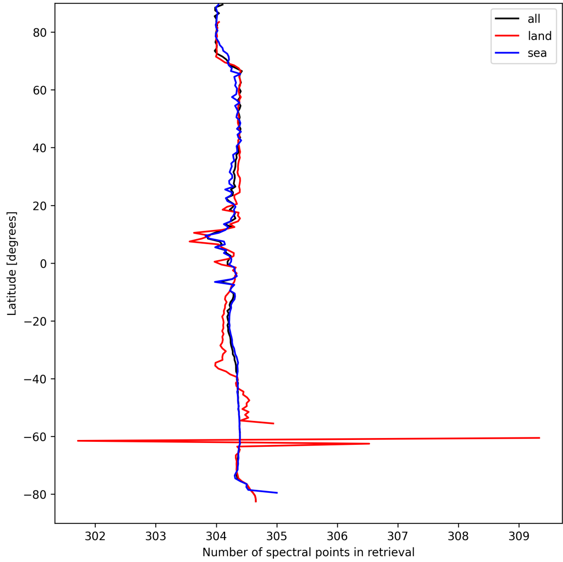
Figure 14: Zonal average of “Number of spectral points in retrieval” for 2025-09-08 to 2025-09-08.
