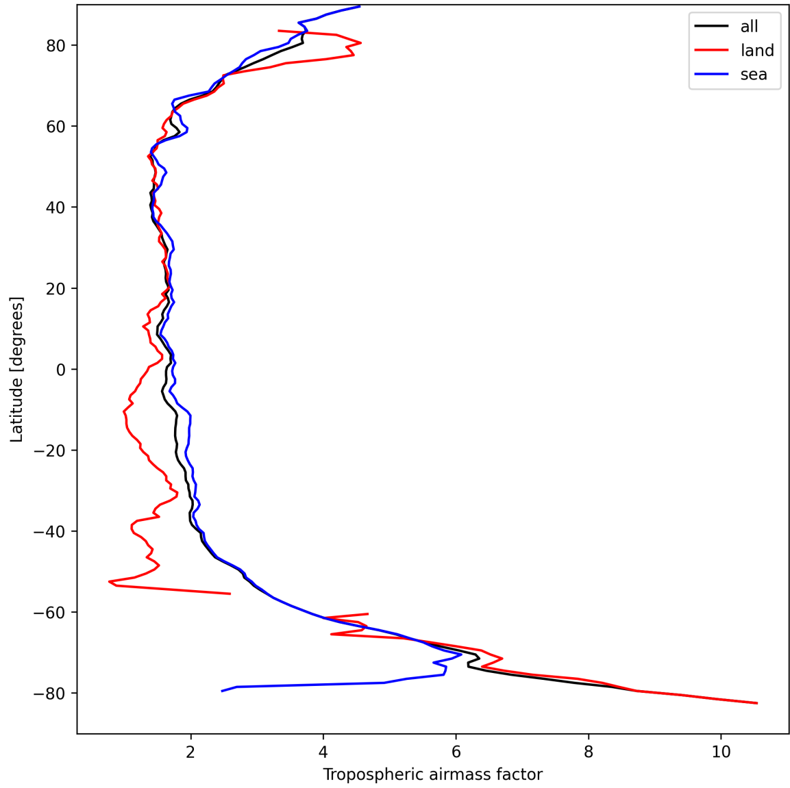
Figure 12: Zonal average of “Tropospheric airmass factor” for 2025-09-08 to 2025-09-08.
