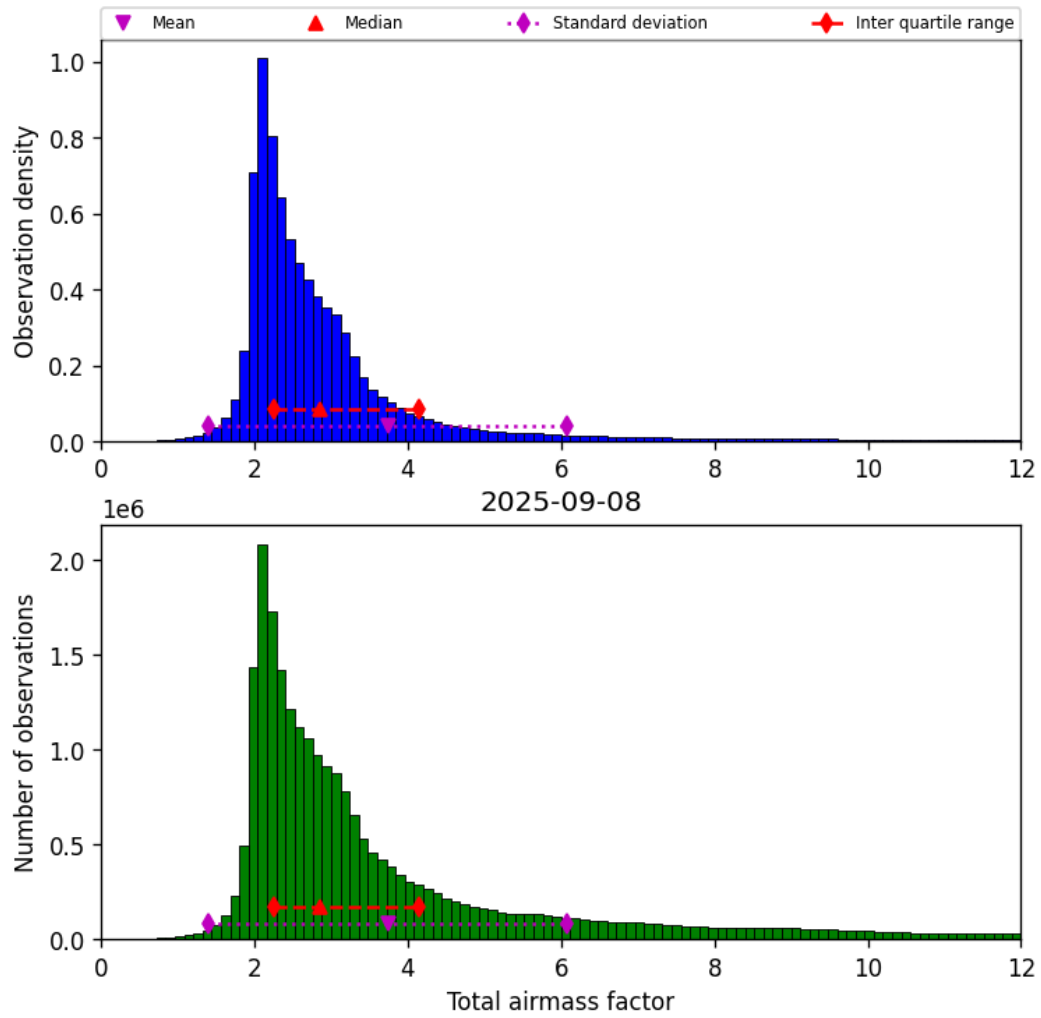
Figure 30: Histogram of “Total airmass factor” for 2025-09-08 to 2025-09-08
