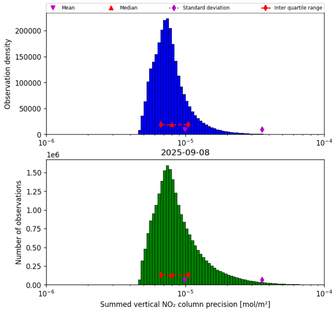
Figure 39: Histogram of "Summed vertical NO 2 column precision" for 2025-09-08 to 2025-09-08
