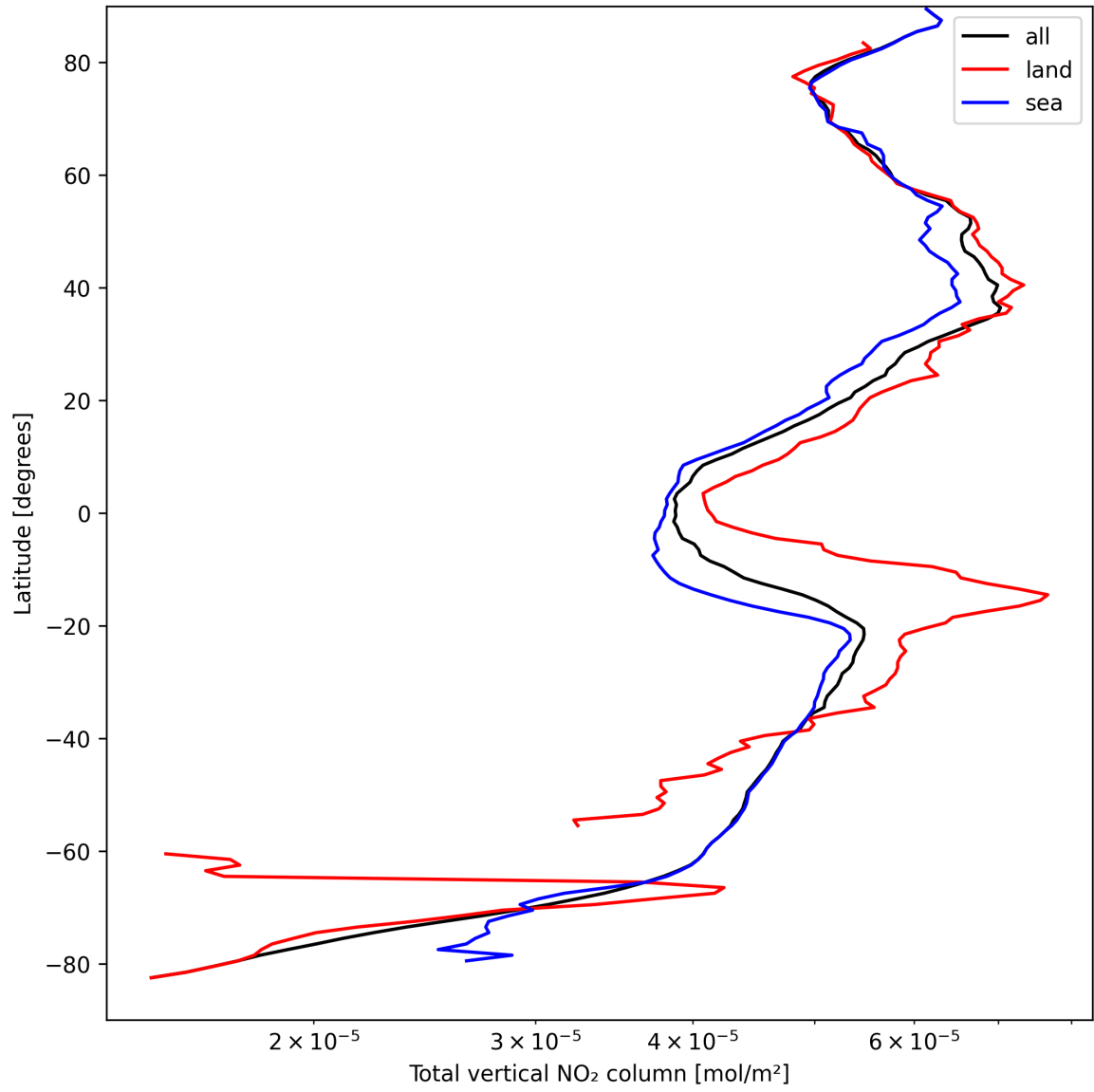
Figure 19: Zonal average of “Total vertical NO 2 column” for 2025-09-08 to 2025-09-08.
