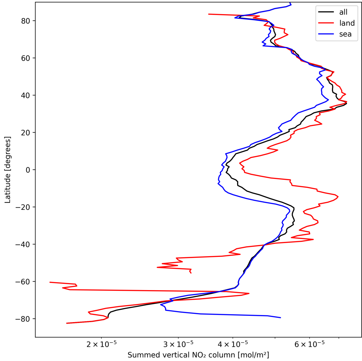
Figure 21: Zonal average of “Summed vertical NO 2 column” for 2025-09-08 to 2025-09-08.
