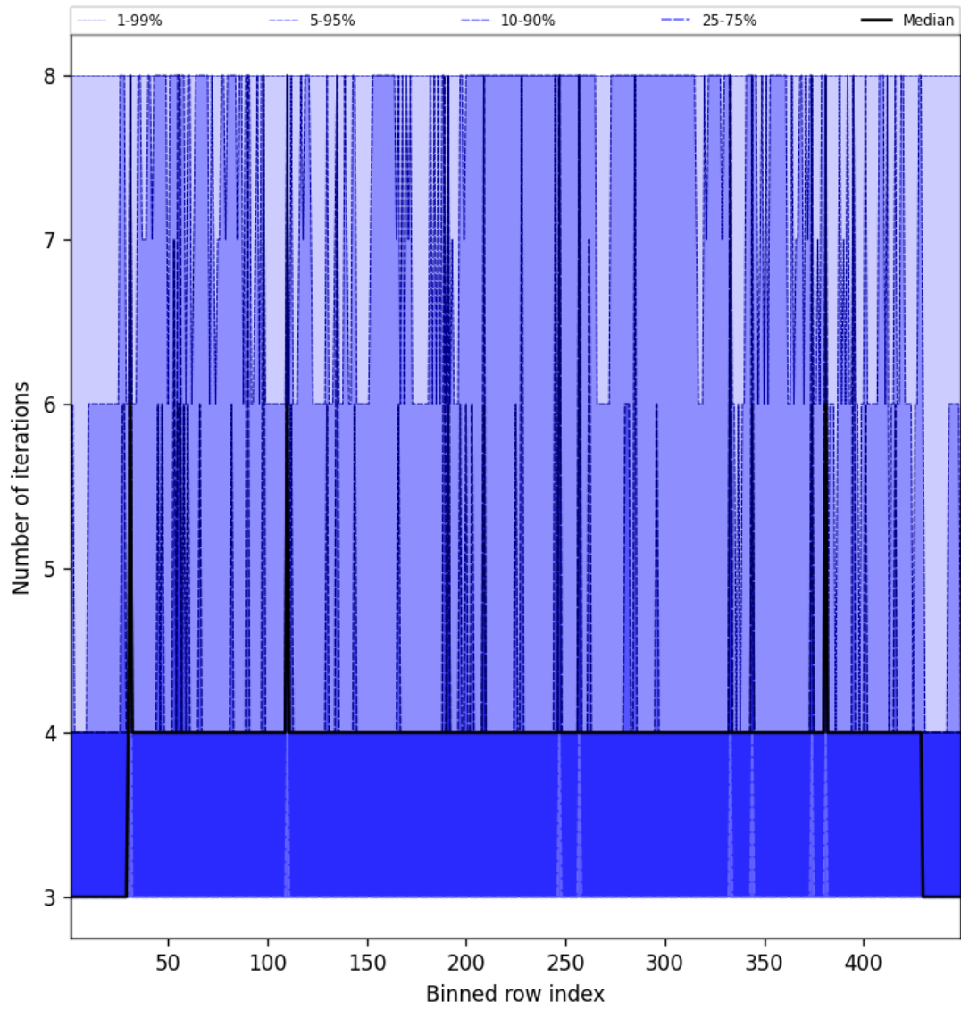
Figure 49: Along track statistics of “Number of iterations” for 2025-09-08 to 2025-09-08
