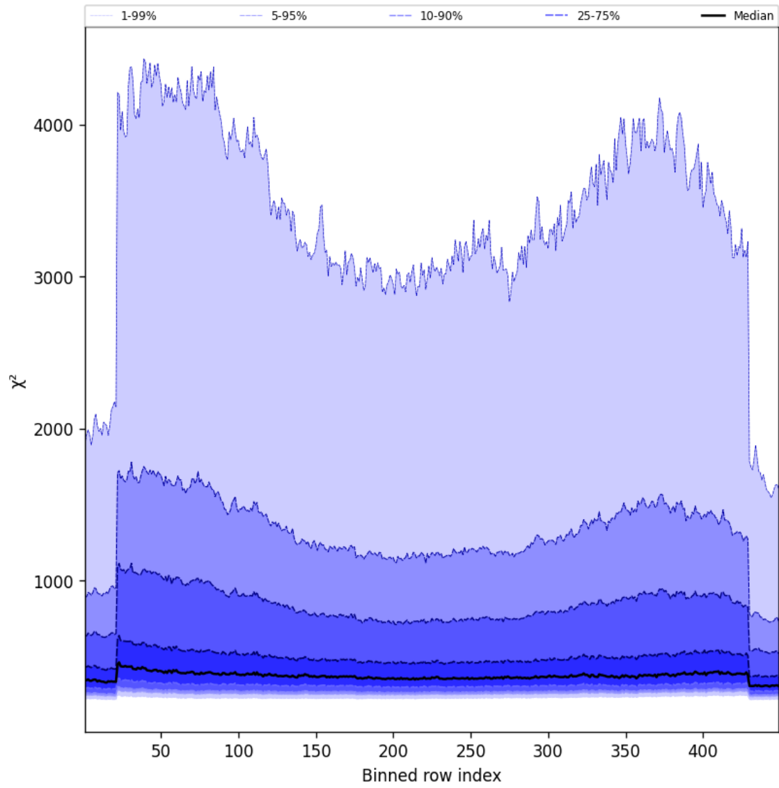
Figure 57: Along track statistics of “ \chi^2 ” for 2025-09-08 to 2025-09-08
