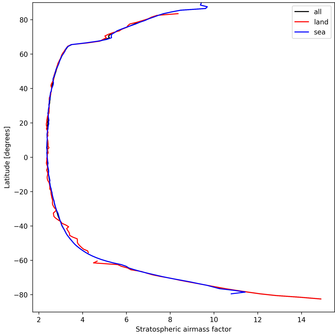
Figure 25: Zonal average of “Stratospheric airmass factor” for 2025-09-08 to 2025-09-08.
