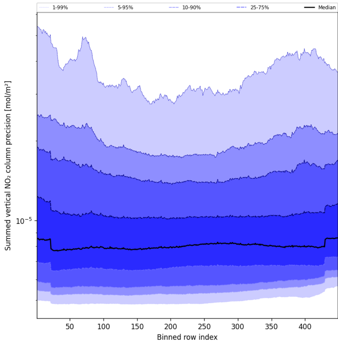
Figure 56: Along track statistics of “Summed vertical NO 2 column precision” for 2025-09-08 to 2025-09-08
