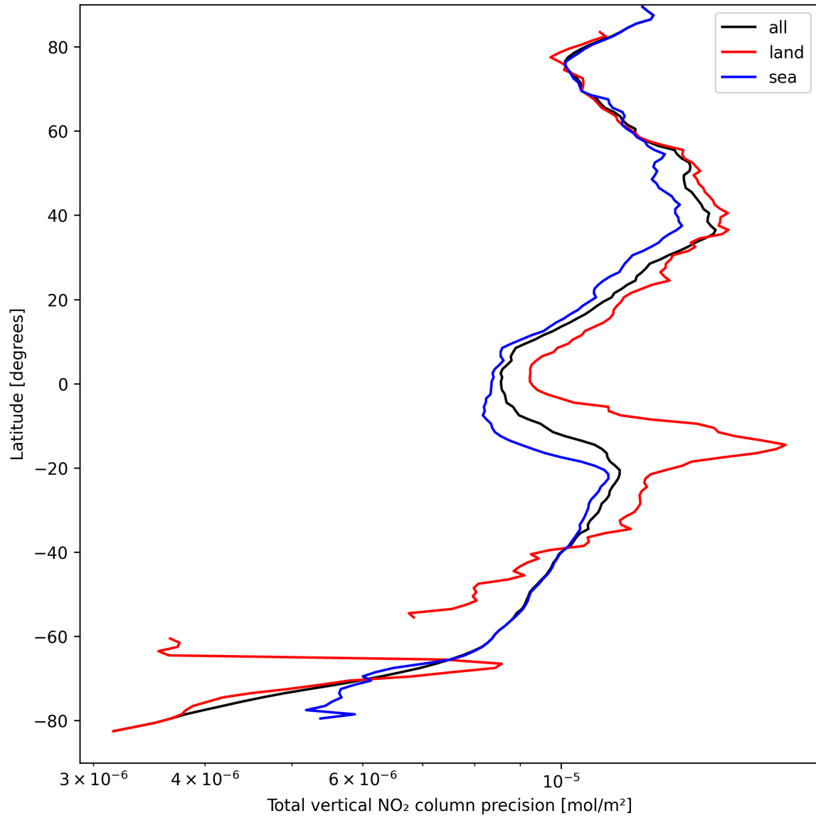
Figure 20: Zonal average of “Total vertical NO 2 column precision” for 2025-09-08 to 2025-09-08.
