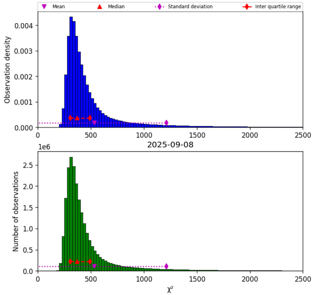
Figure 40: Histogram of “ \chi^2 ” for 2025-09-08 to 2025-09-08
