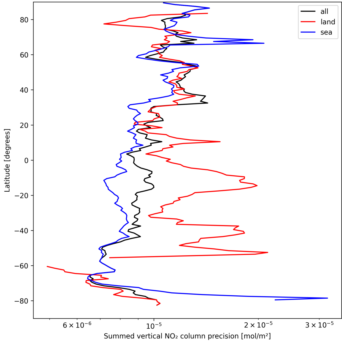
Figure 22: Zonal average of “Summed vertical NO 2 column precision” for 2025-09-08 to 2025-09-08.
