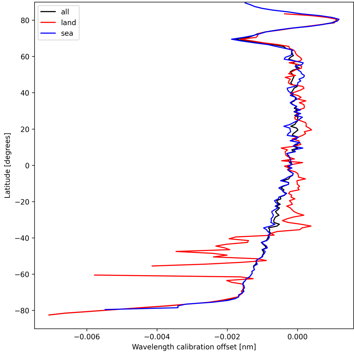
Figure 16: Zonal average of “Wavelength calibration offset” for 2025-09-08 to 2025-09-08.
