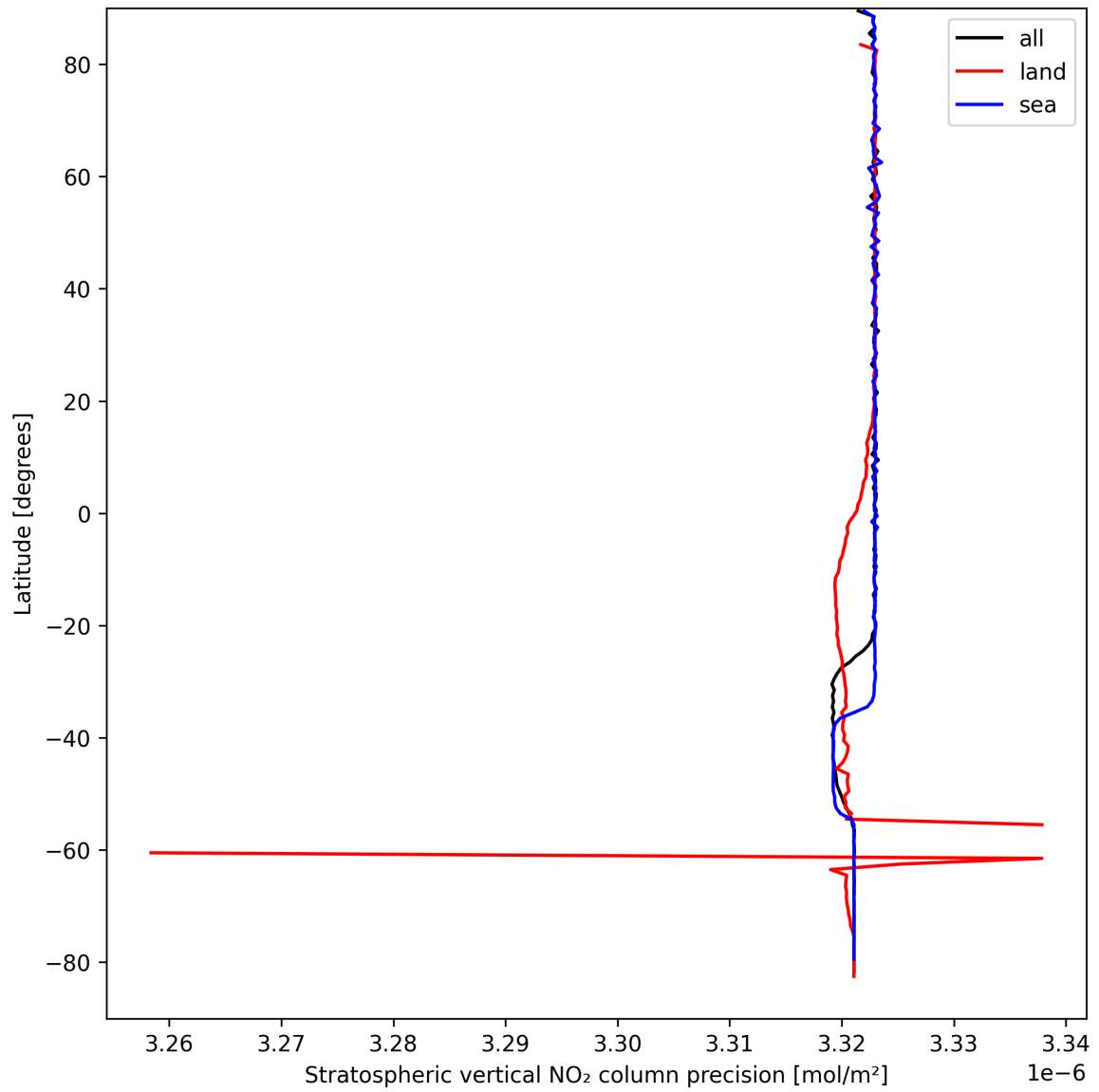
Figure 18: Zonal average of “Stratospheric vertical NO 2 column precision” for 2025-09-08 to 2025-09-08.
