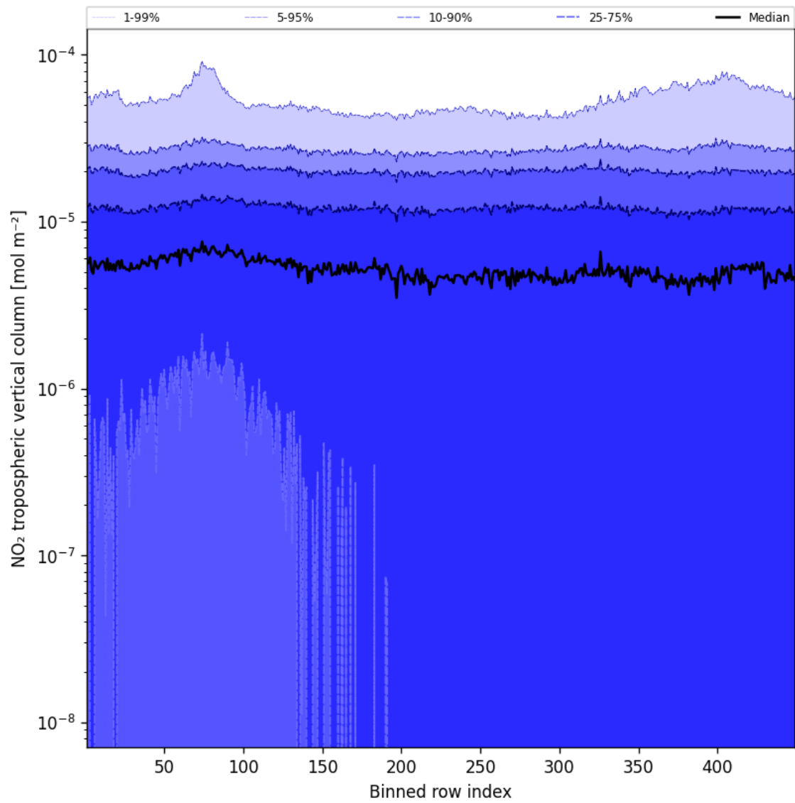
Figure 44: Along track statistics of “NO 2 tropospheric vertical column” for 2025-09-08 to 2025-09-08
