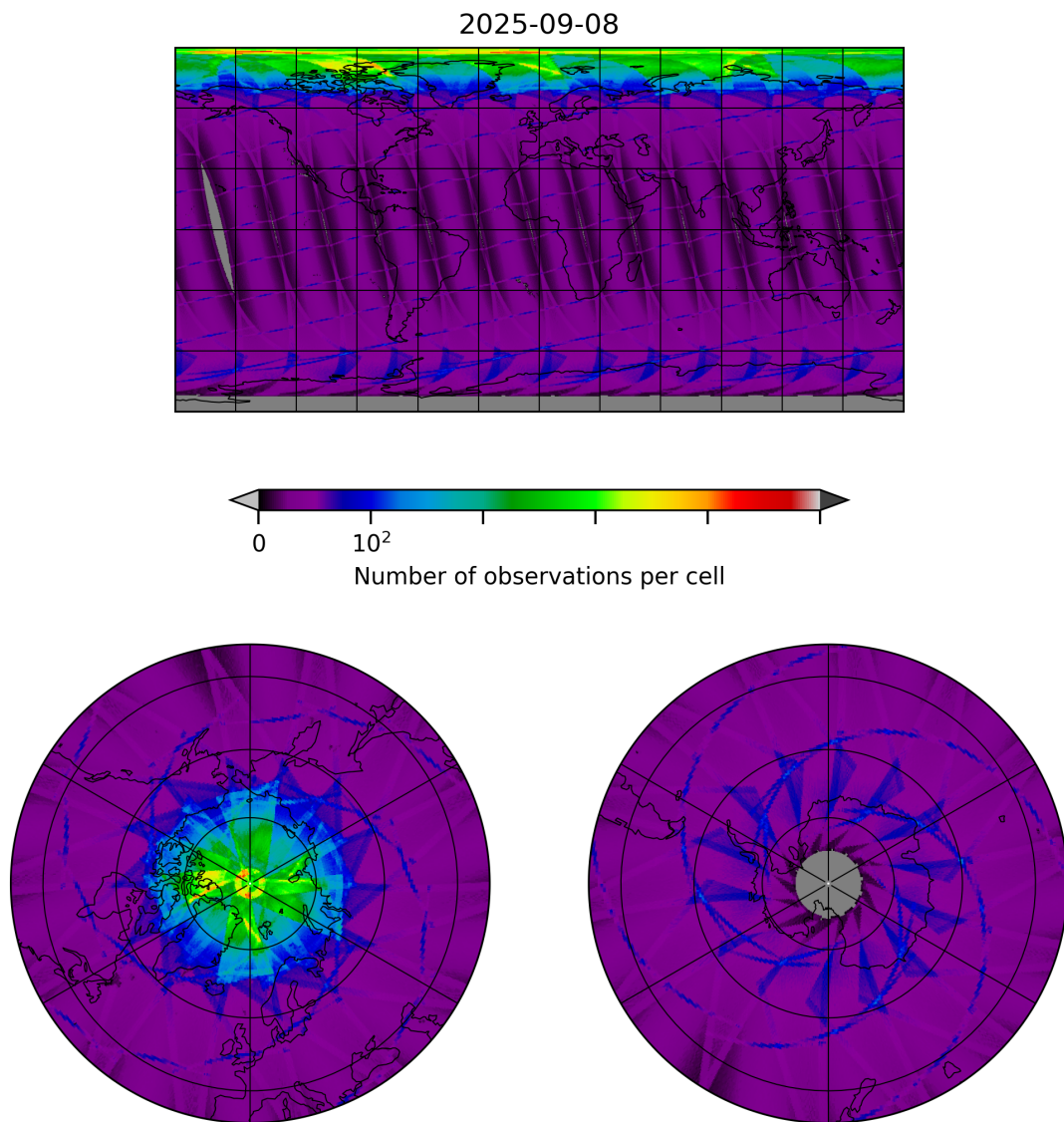
Figure 8: Map of the number of observations for 2025-09-08 to 2025-09-08
