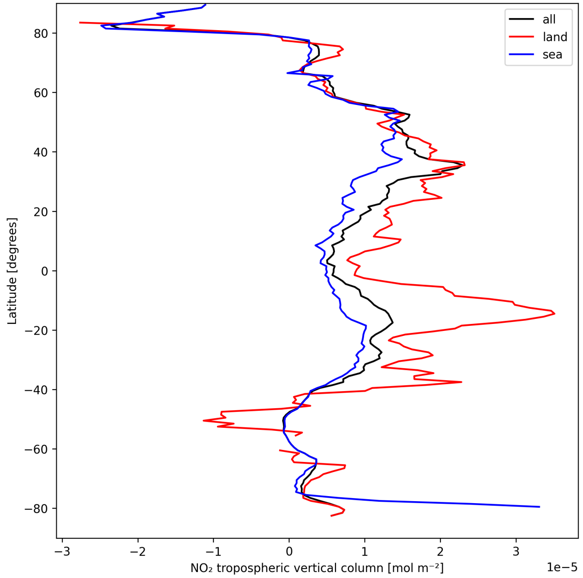
Figure 10: Zonal average of “NO 2 tropospheric vertical column” for 2025-09-08 to 2025-09-08.
