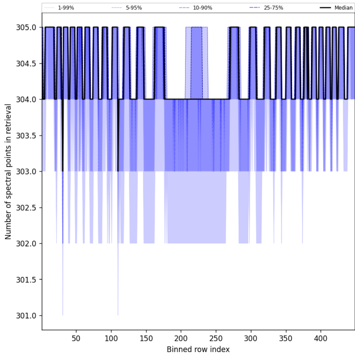
Figure 48: Along track statistics of “Number of spectral points in retrieval” for 2025-09-08 to 2025-09-08
