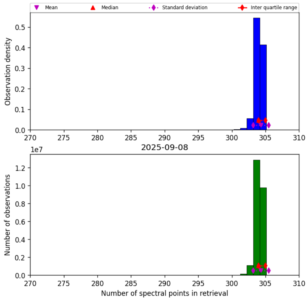
Figure 31: Histogram of “Number of spectral points in retrieval” for 2025-09-08 to 2025-09-08
