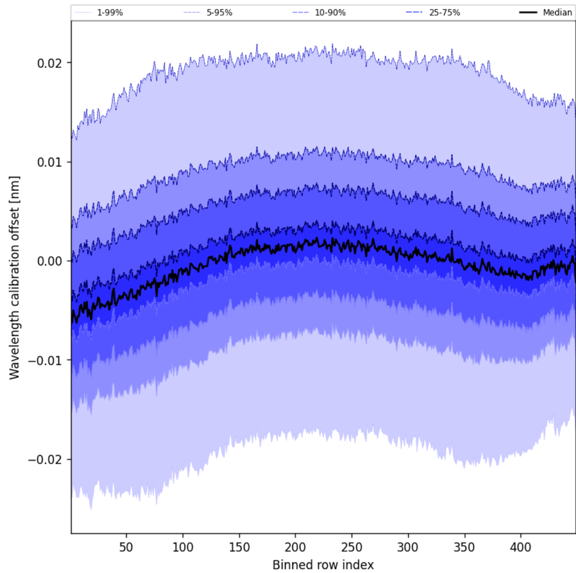
Figure 50: Along track statistics of “Wavelength calibration offset” for 2025-09-08 to 2025-09-08
