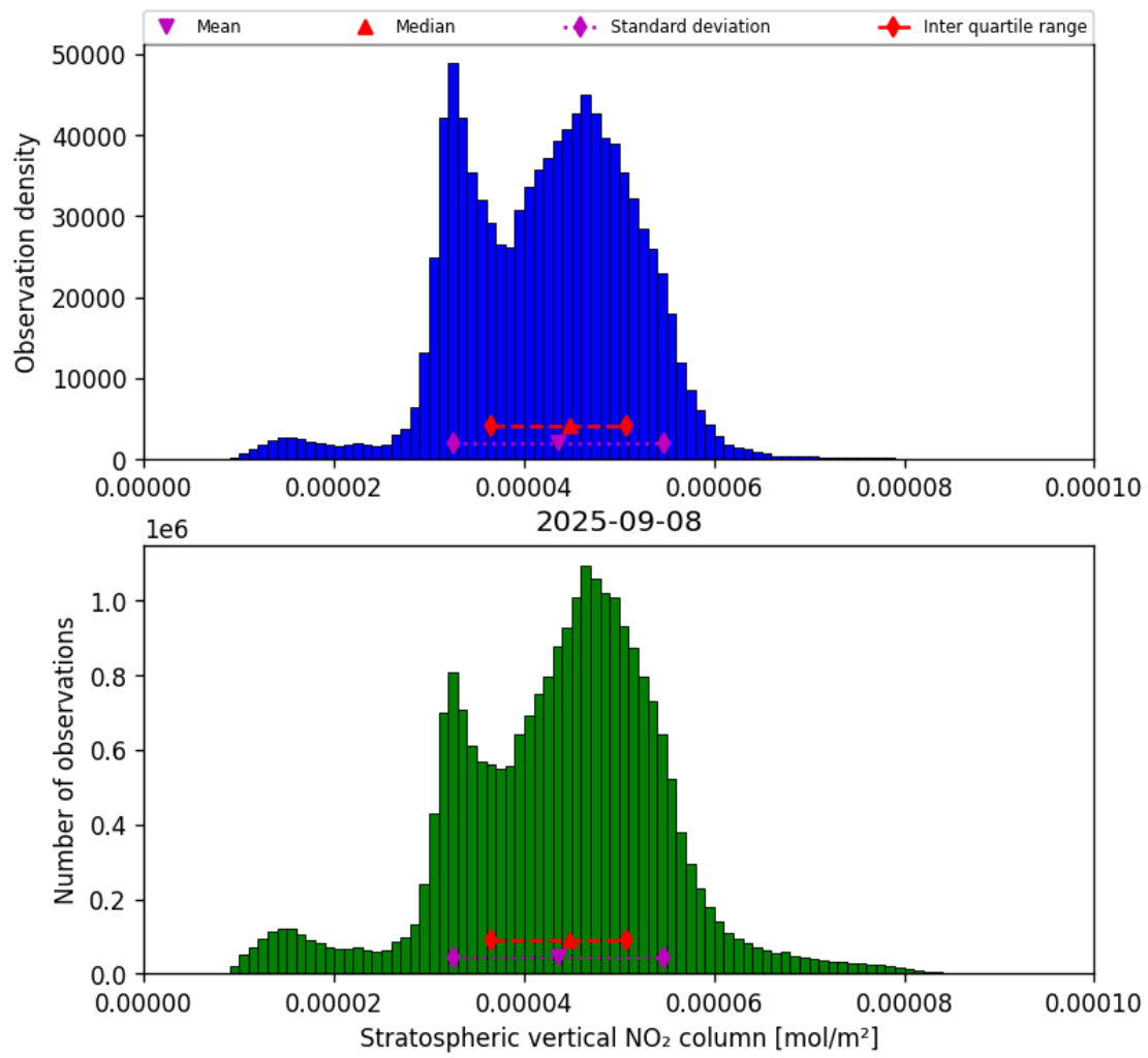
Figure 34: Histogram of “Stratospheric vertical NO 2 column” for 2025-09-08 to 2025-09-08
