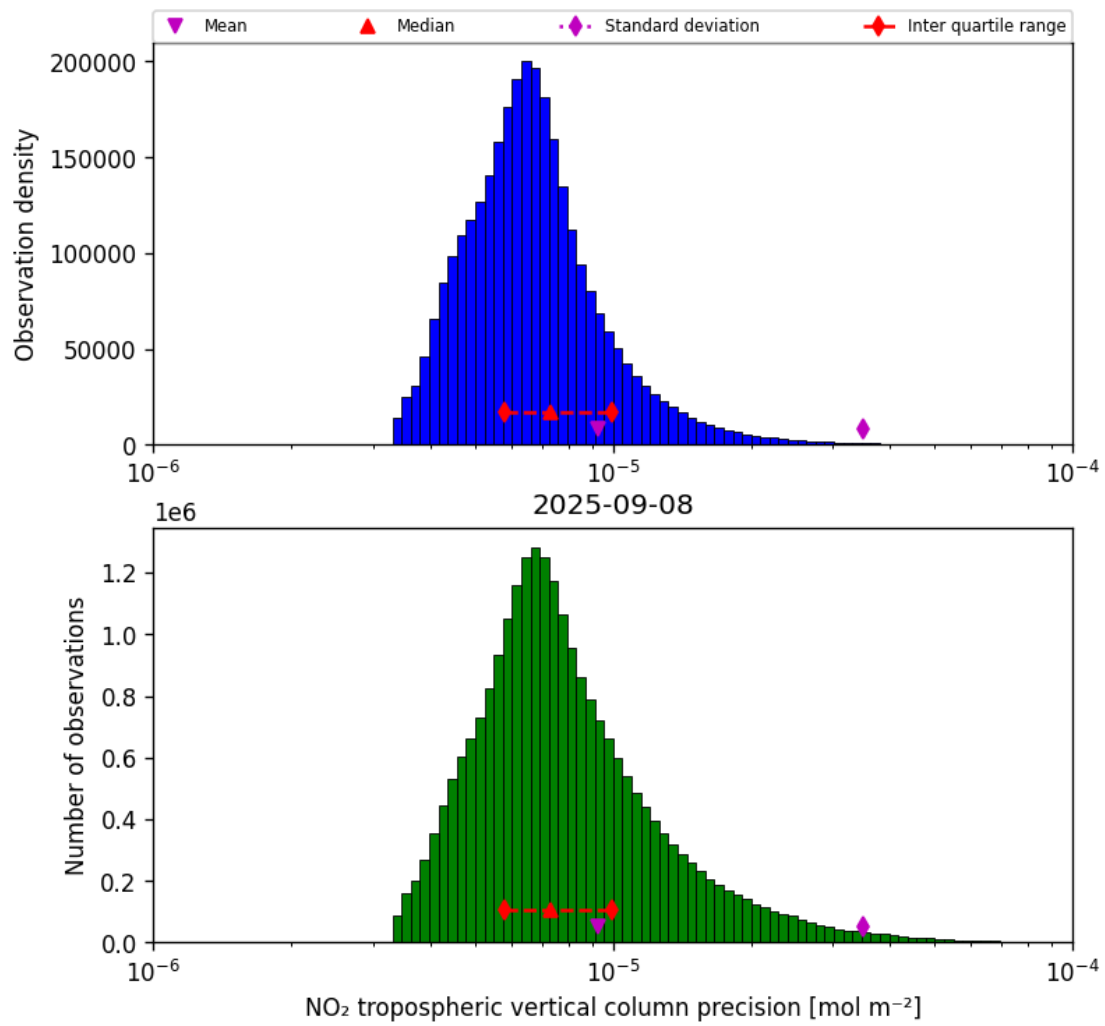
Figure 28: Histogram of “NO 2 tropospheric vertical column precision” for 2025-09-08 to 2025-09-08
