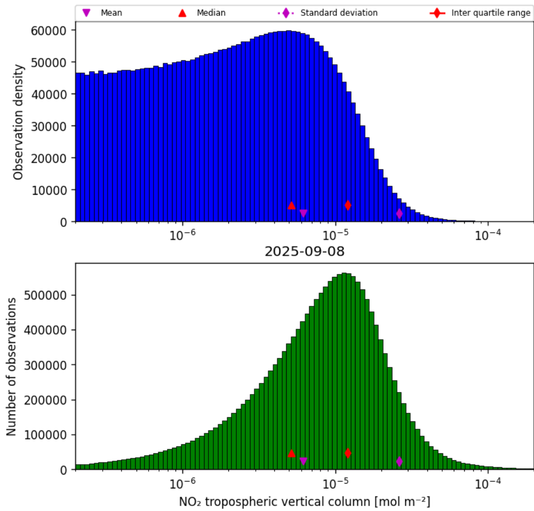
Figure 27: Histogram of “NO 2 tropospheric vertical column” for 2025-09-08 to 2025-09-08
