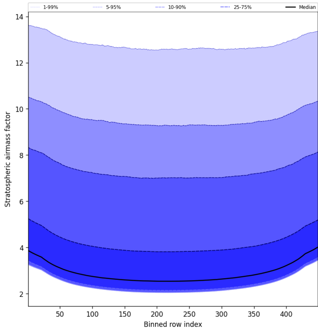
Figure 59: Along track statistics of “Stratospheric airmass factor” for 2025-09-08 to 2025-09-08
