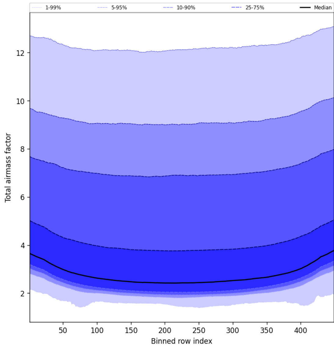
Figure 47: Along track statistics of “Total airmass factor” for 2025-09-08 to 2025-09-08
