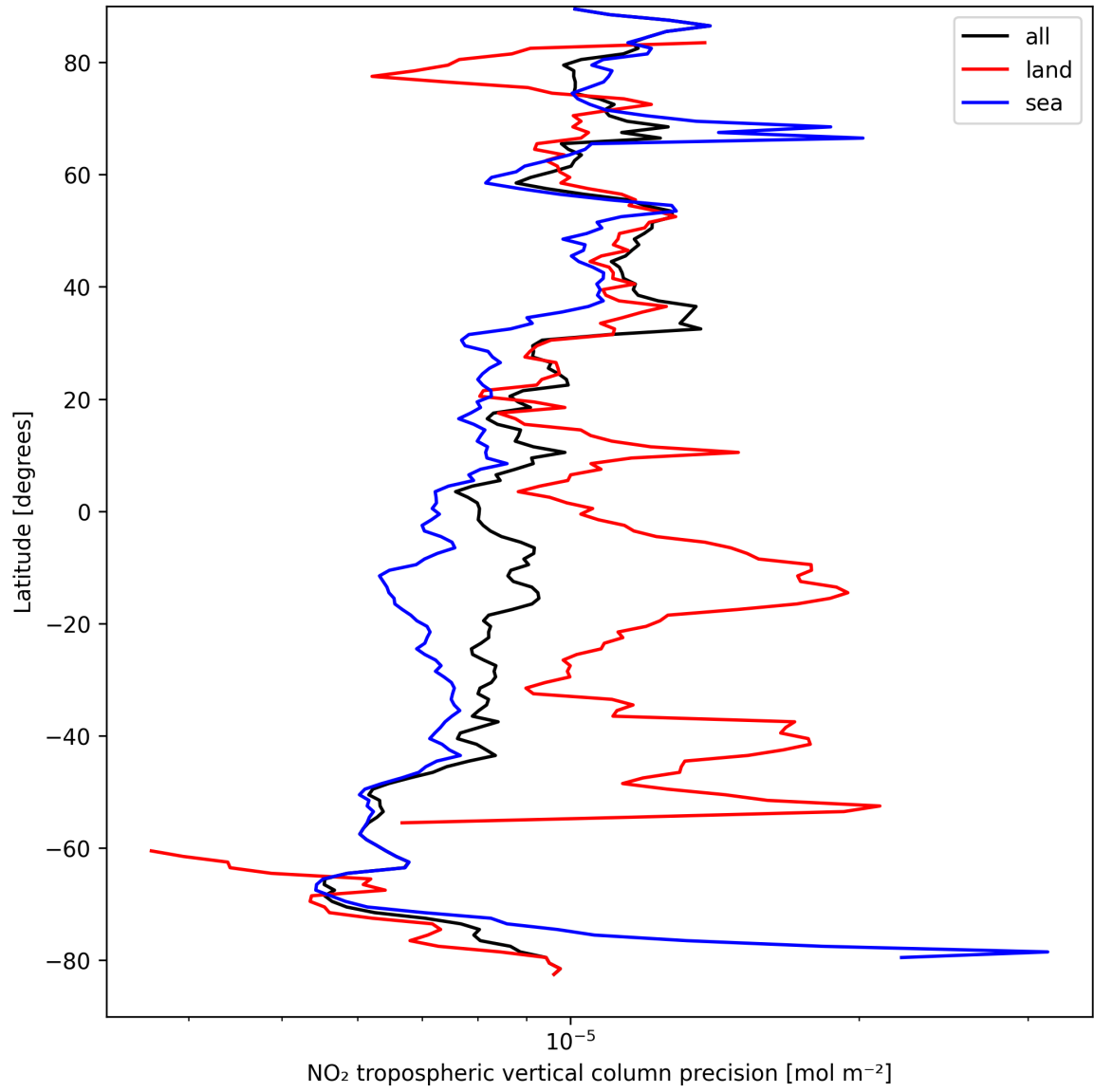
Figure 11: Zonal average of “NO 2 tropospheric vertical column precision” for 2025-09-08 to 2025-09-08.
