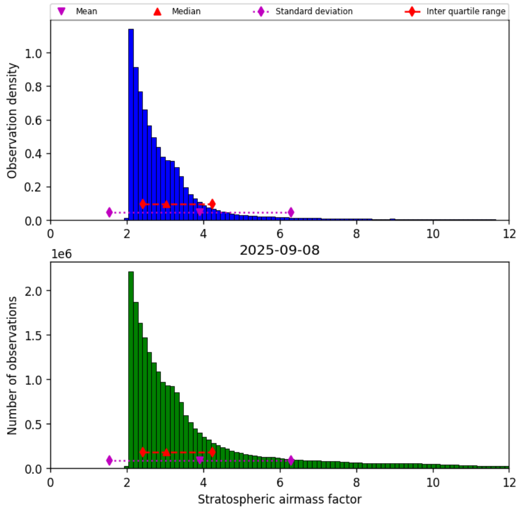
Figure 42: Histogram of “Stratospheric airmass factor” for 2025-09-08 to 2025-09-08
