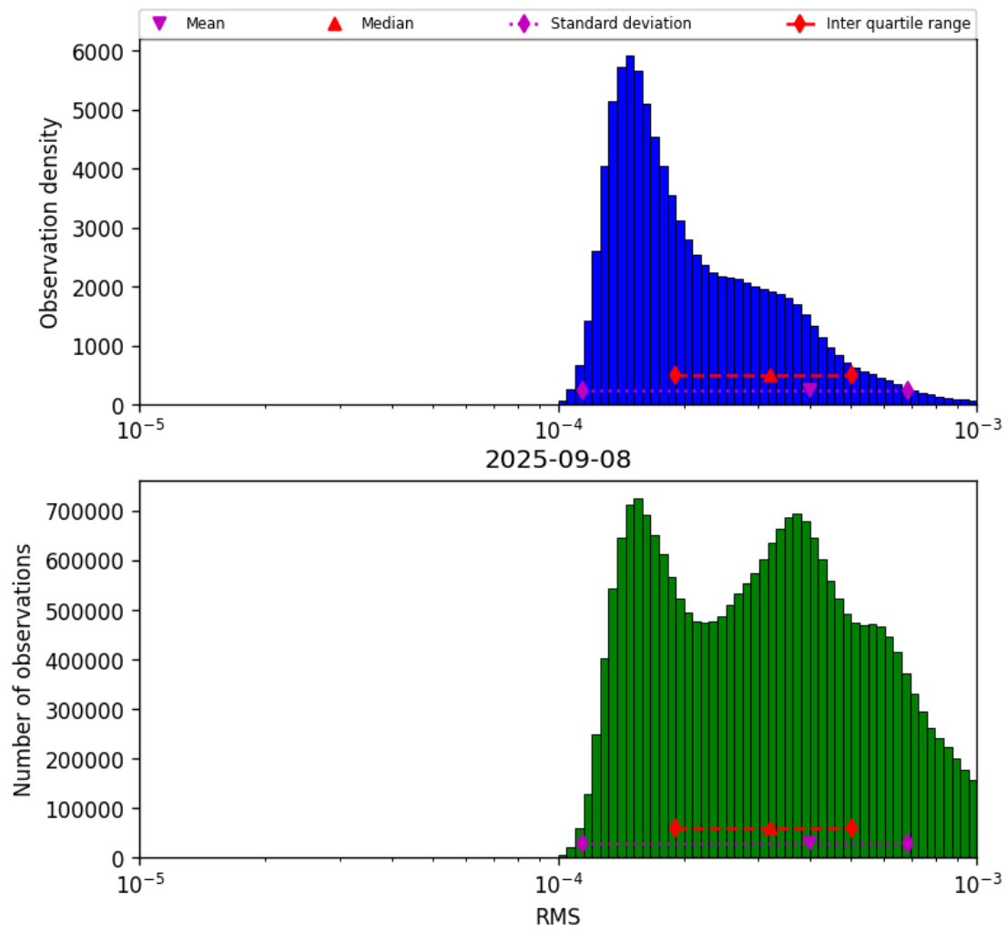
Figure 41: Histogram of “RMS” for 2025-09-08 to 2025-09-08
