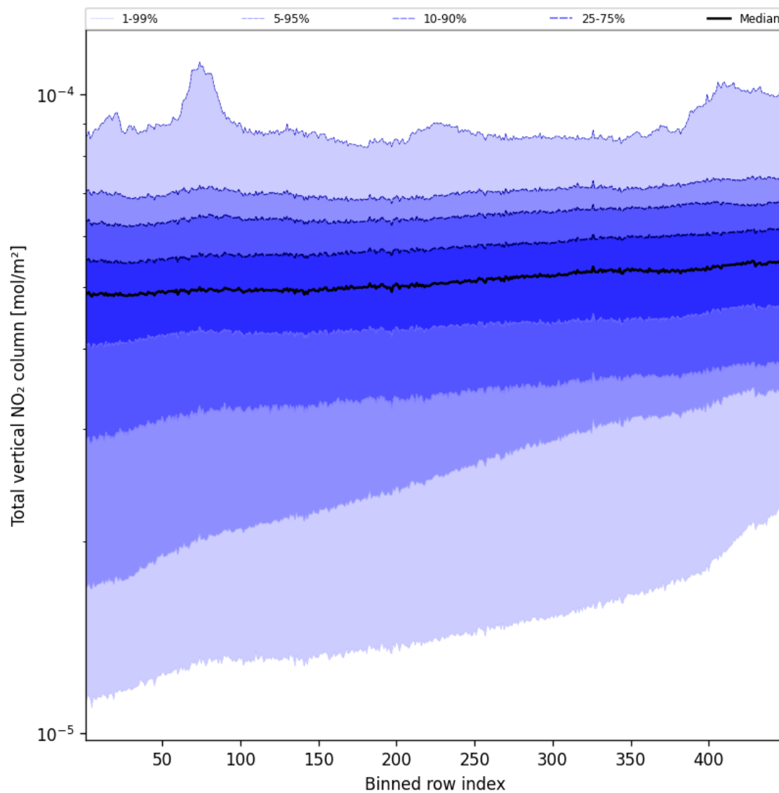
Figure 53: Along track statistics of “Total vertical NO 2 column” for 2025-09-08 to 2025-09-08
