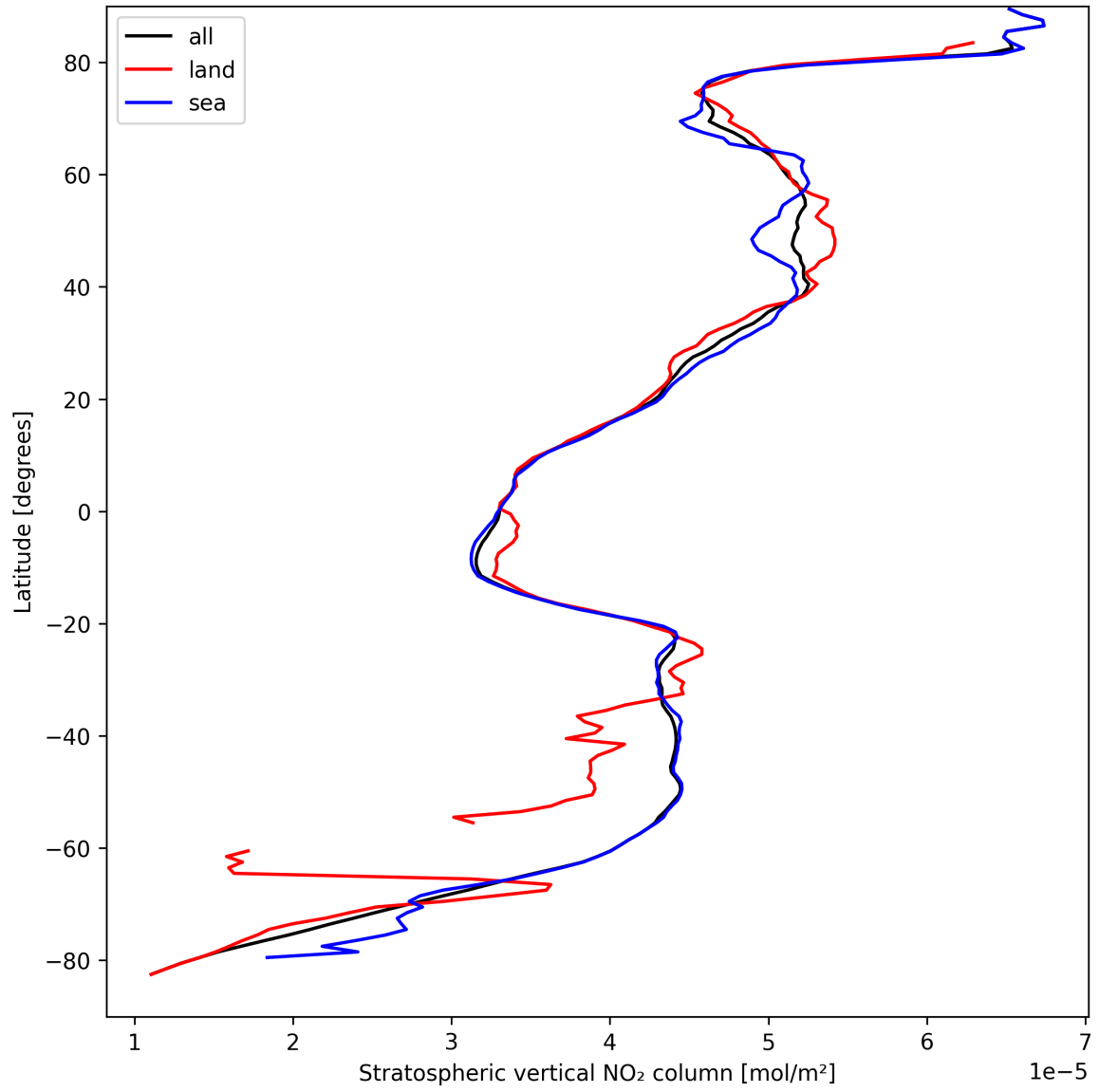
Figure 17: Zonal average of “Stratospheric vertical NO 2 column” for 2025-09-08 to 2025-09-08.
