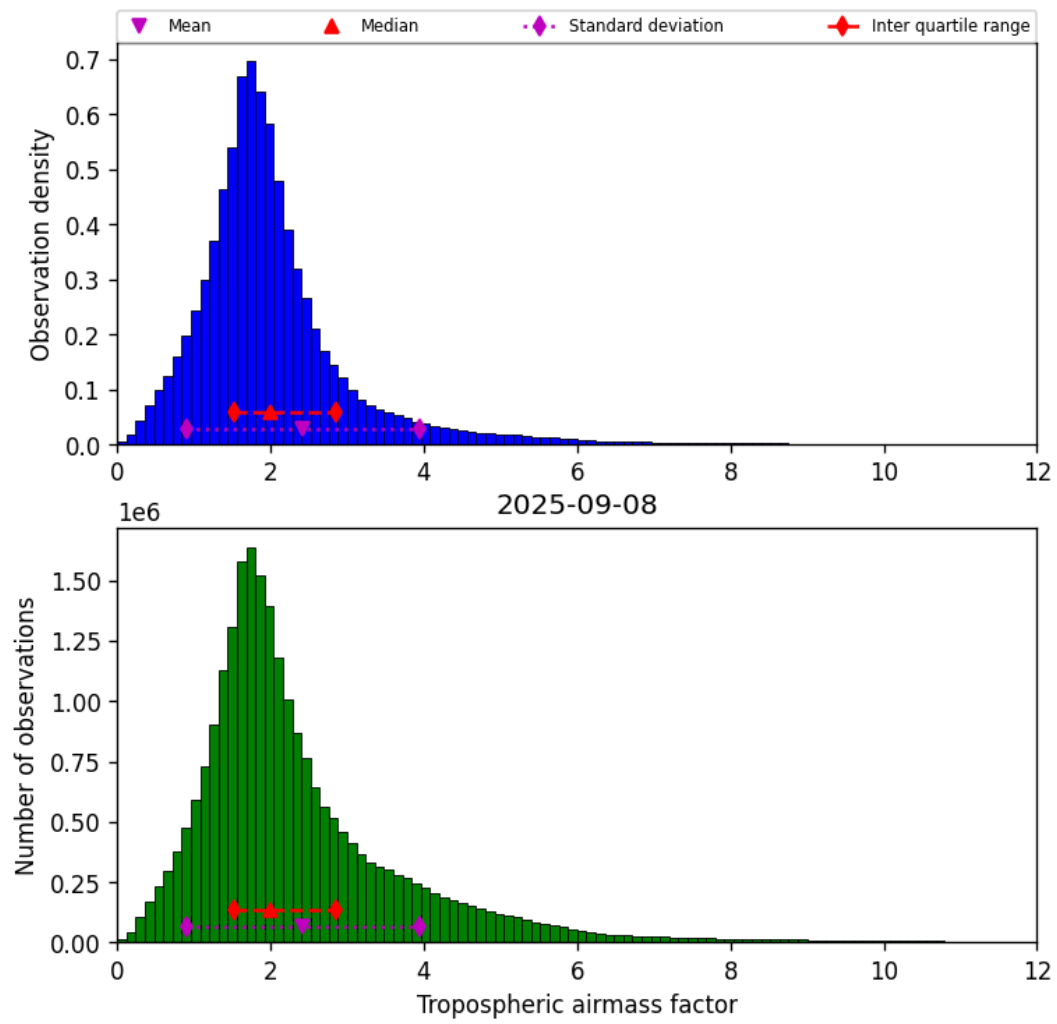
Figure 29: Histogram of “Tropospheric airmass factor” for 2025-09-08 to 2025-09-08
