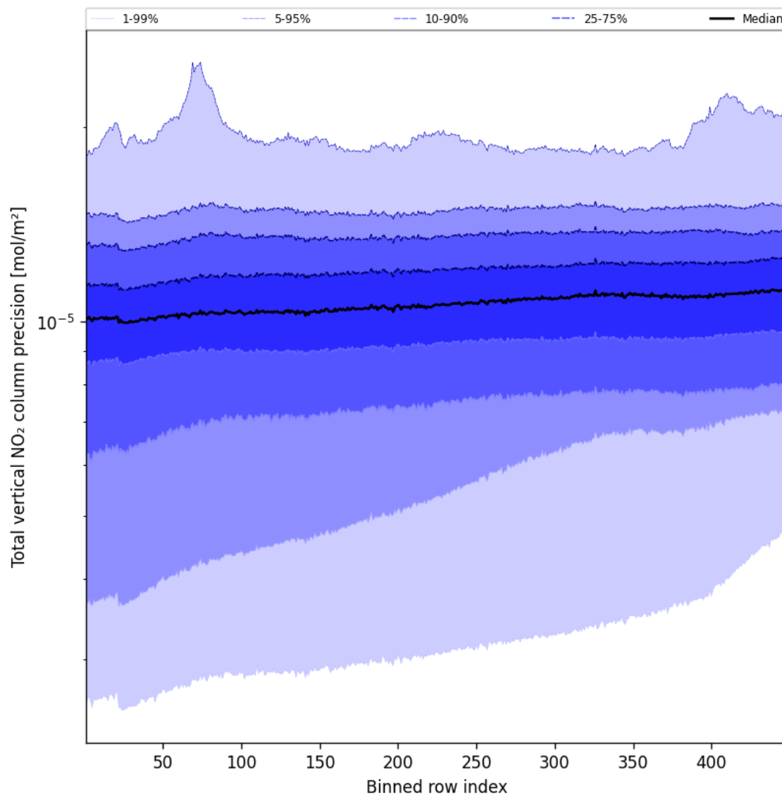
Figure 54: Along track statistics of “Total vertical NO 2 column precision” for 2025-09-08 to 2025-09-08
