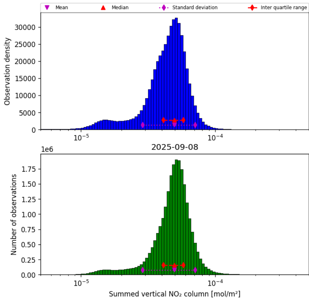
Figure 38: Histogram of "Summed vertical NO 2 column" for 2025-09-08 to 2025-09-08
