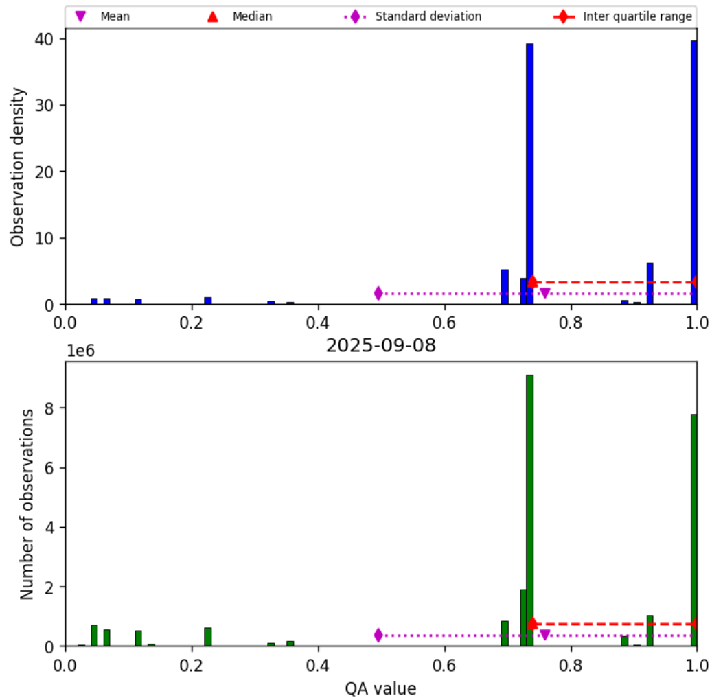
Figure 26: Histogram of “QA value” for 2025-09-08 to 2025-09-08
