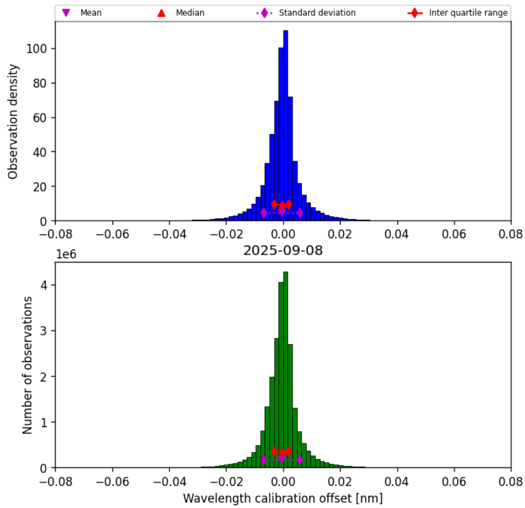
Figure 33: Histogram of “Wavelength calibration offset” for 2025-09-08 to 2025-09-08
