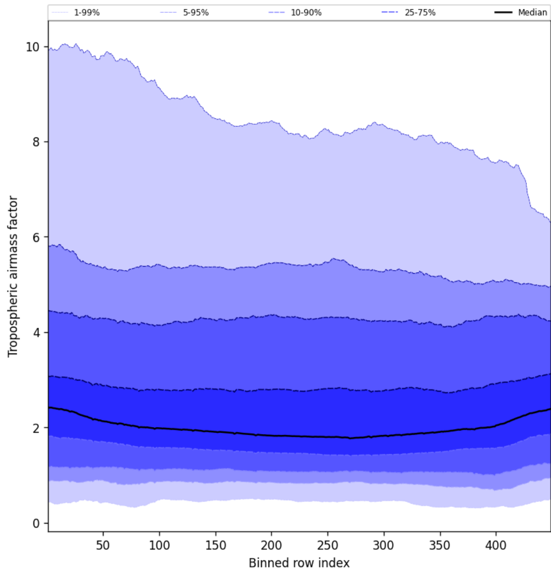
Figure 46: Along track statistics of “Tropospheric air mass factor” for 2025-09-08 to 2025-09-08
