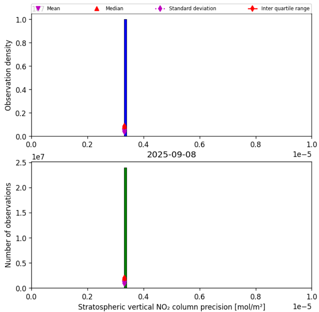
Figure 35: Histogram of “Stratospheric vertical NO 2 column precision” for 2025-09-08 to 2025-09-08
