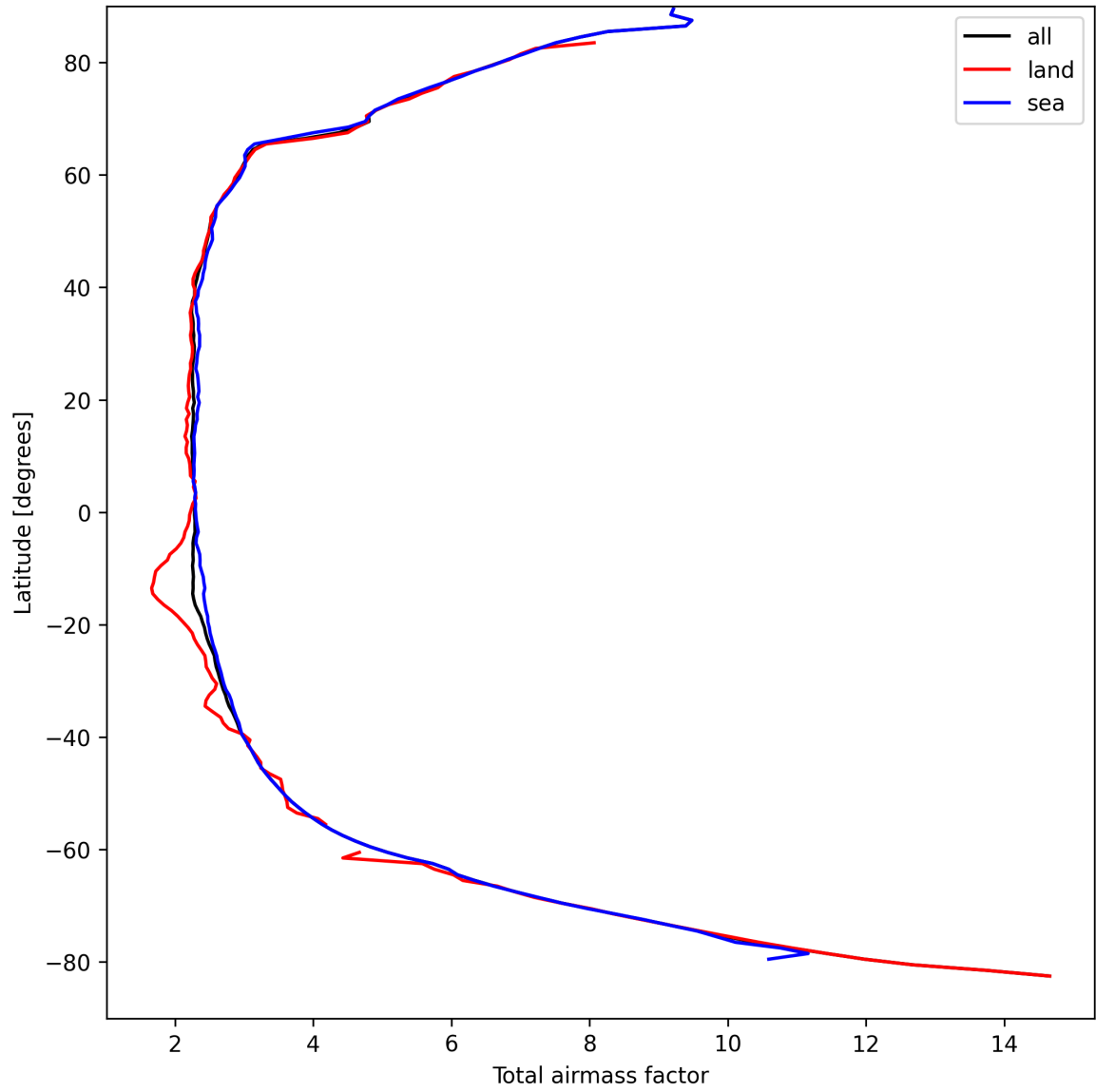
Figure 13: Zonal average of “Total airmass factor” for 2025-09-08 to 2025-09-08.
