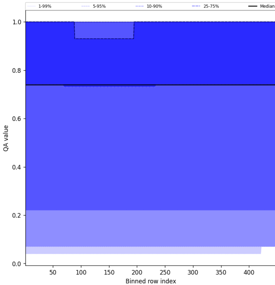
Figure 43: Along track statistics of “QA value” for 2025-09-08 to 2025-09-08
