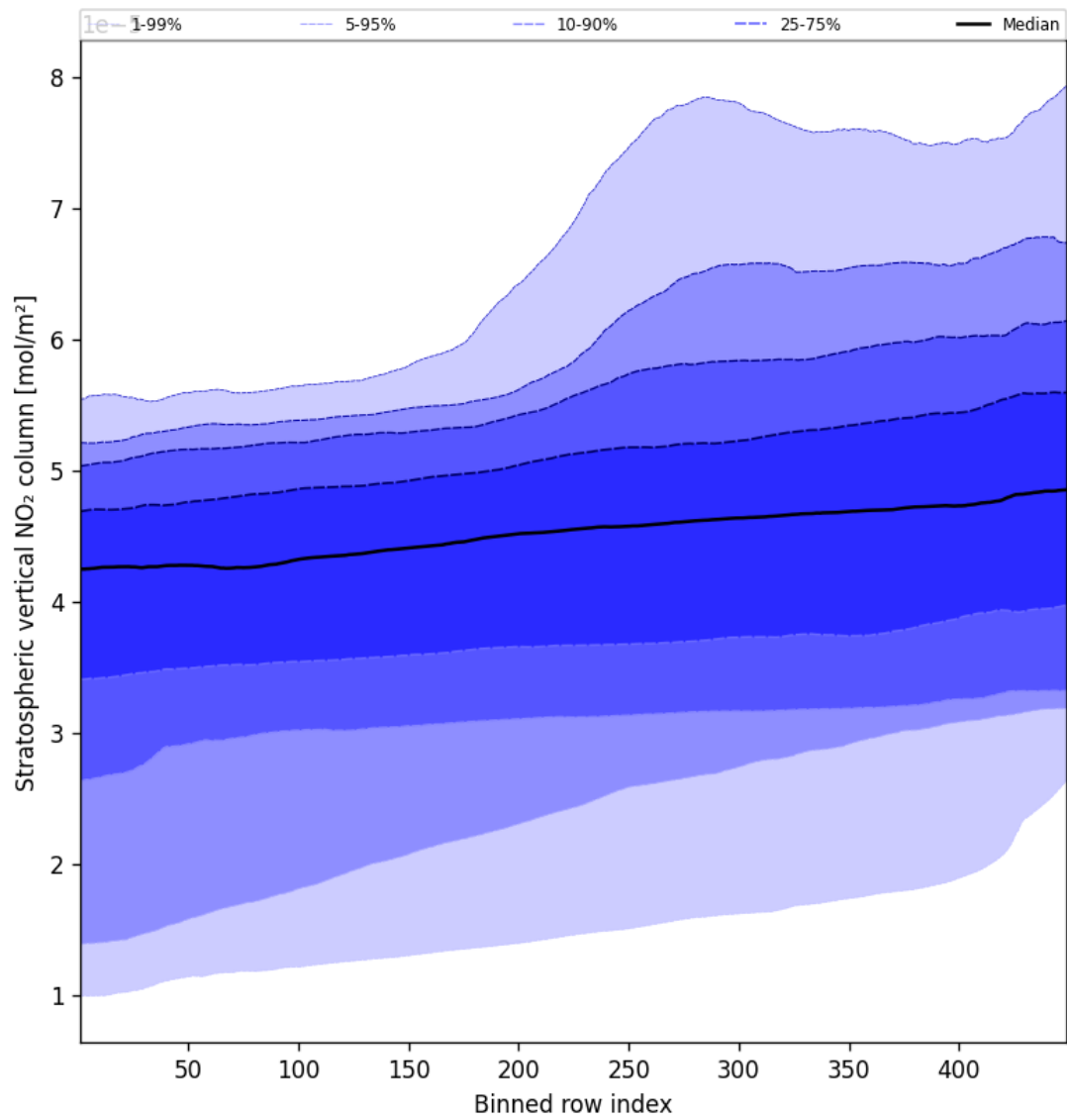
Figure 51: Along track statistics of “Stratospheric vertical NO 2 column” for 2025-09-08 to 2025-09-08
