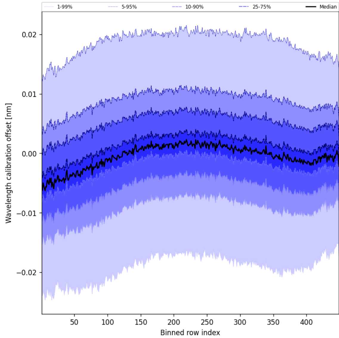
Figure 50: Along track statistics of “Wavelength calibration offset” for 2025-09-10 to 2025-09-11
