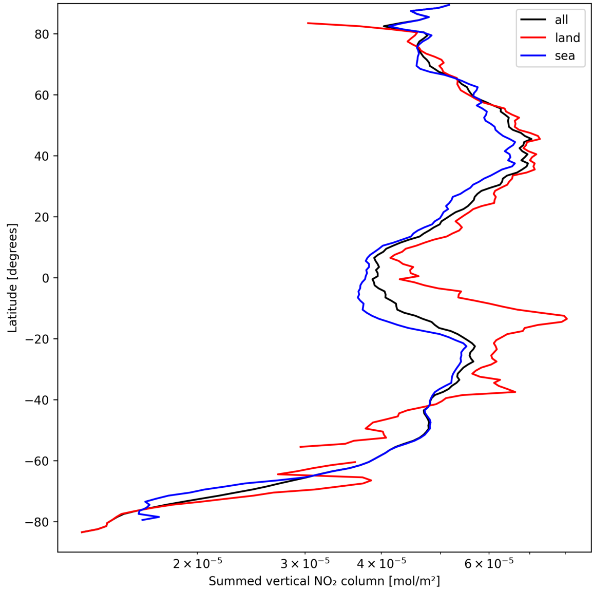
Figure 21: Zonal average of “Summed vertical NO 2 column” for 2025-09-10 to 2025-09-11.
