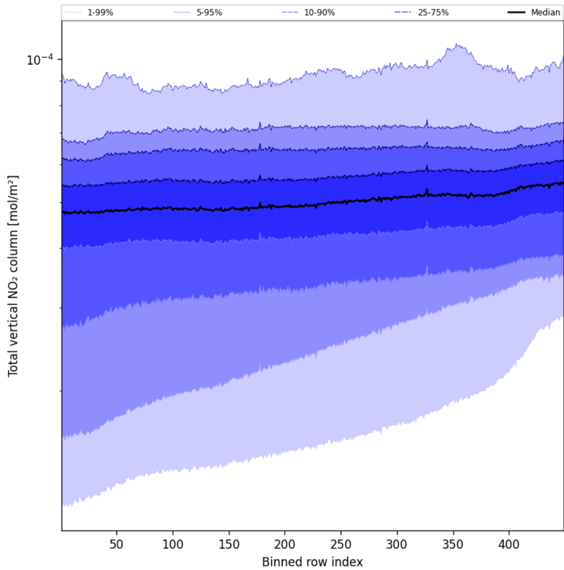
Figure 53: Along track statistics of “Total vertical NO 2 column” for 2025-09-10 to 2025-09-11
