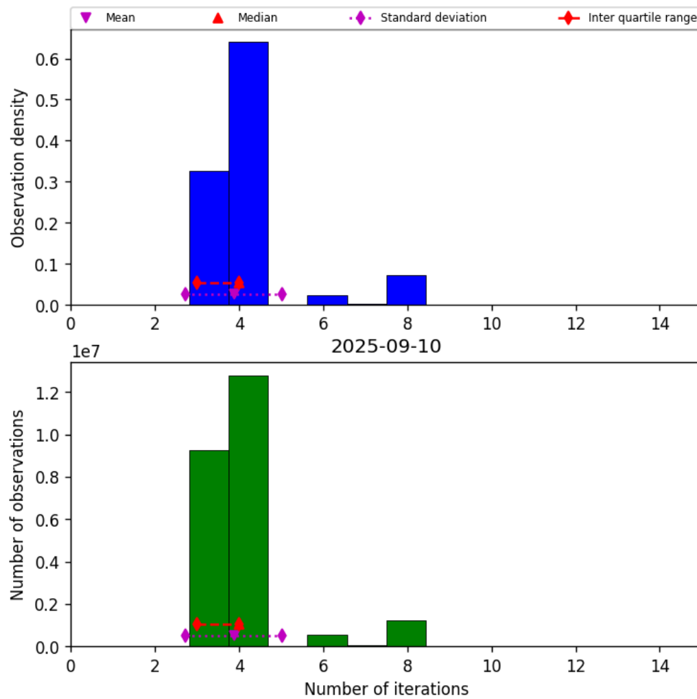
Figure 32: Histogram of “Number of iterations” for 2025-09-10 to 2025-09-11
