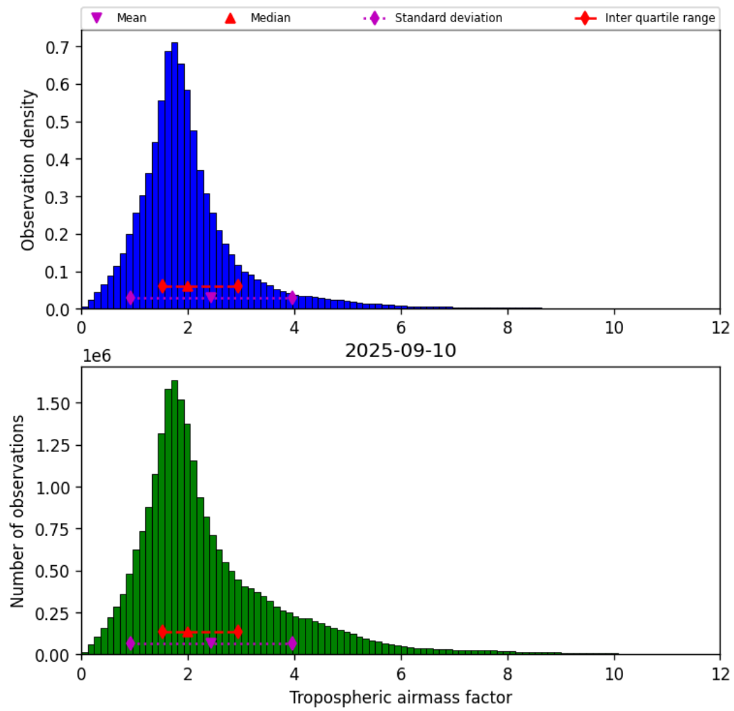
Figure 29: Histogram of “Tropospheric airmass factor” for 2025-09-10 to 2025-09-11
