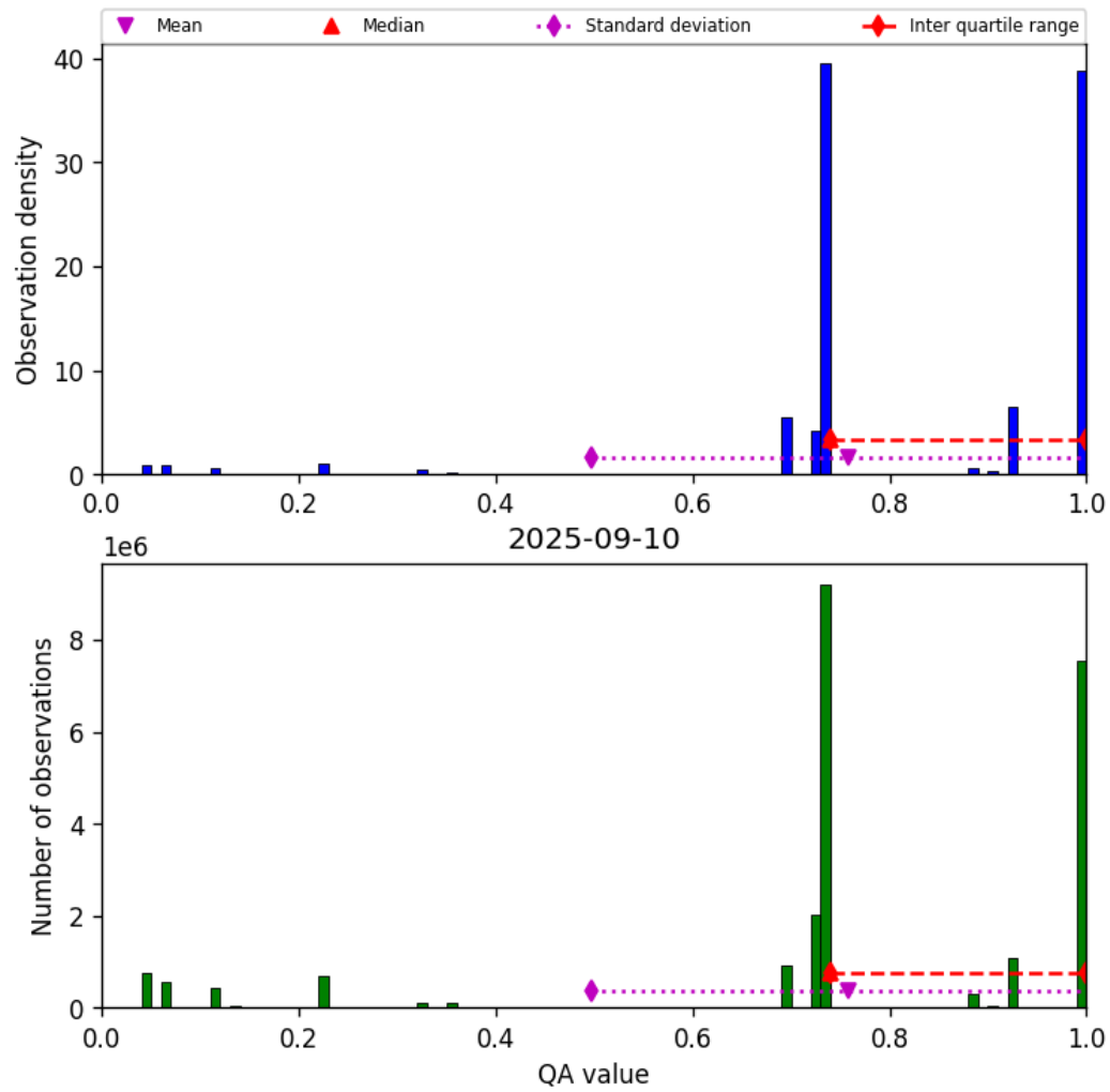
Figure 26: Histogram of “QA value” for 2025-09-10 to 2025-09-11
