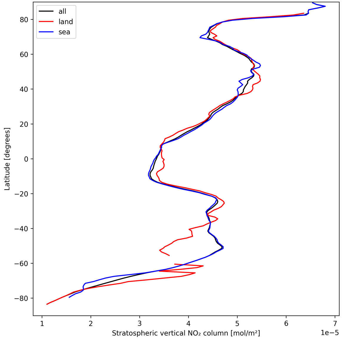
Figure 17: Zonal average of “Stratospheric vertical NO 2 column” for 2025-09-10 to 2025-09-11.
