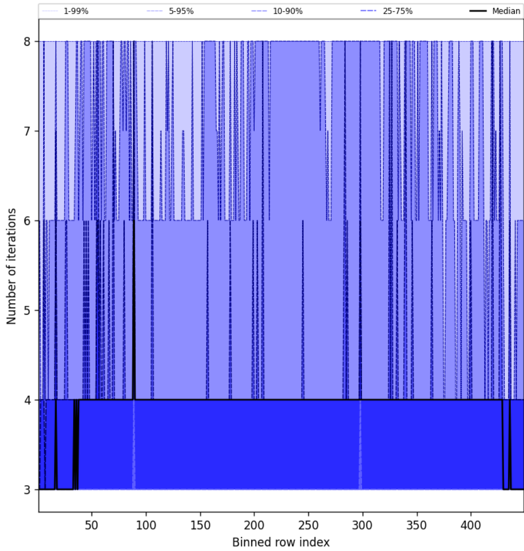
Figure 49: Along track statistics of “Number of iterations” for 2025-09-10 to 2025-09-11
