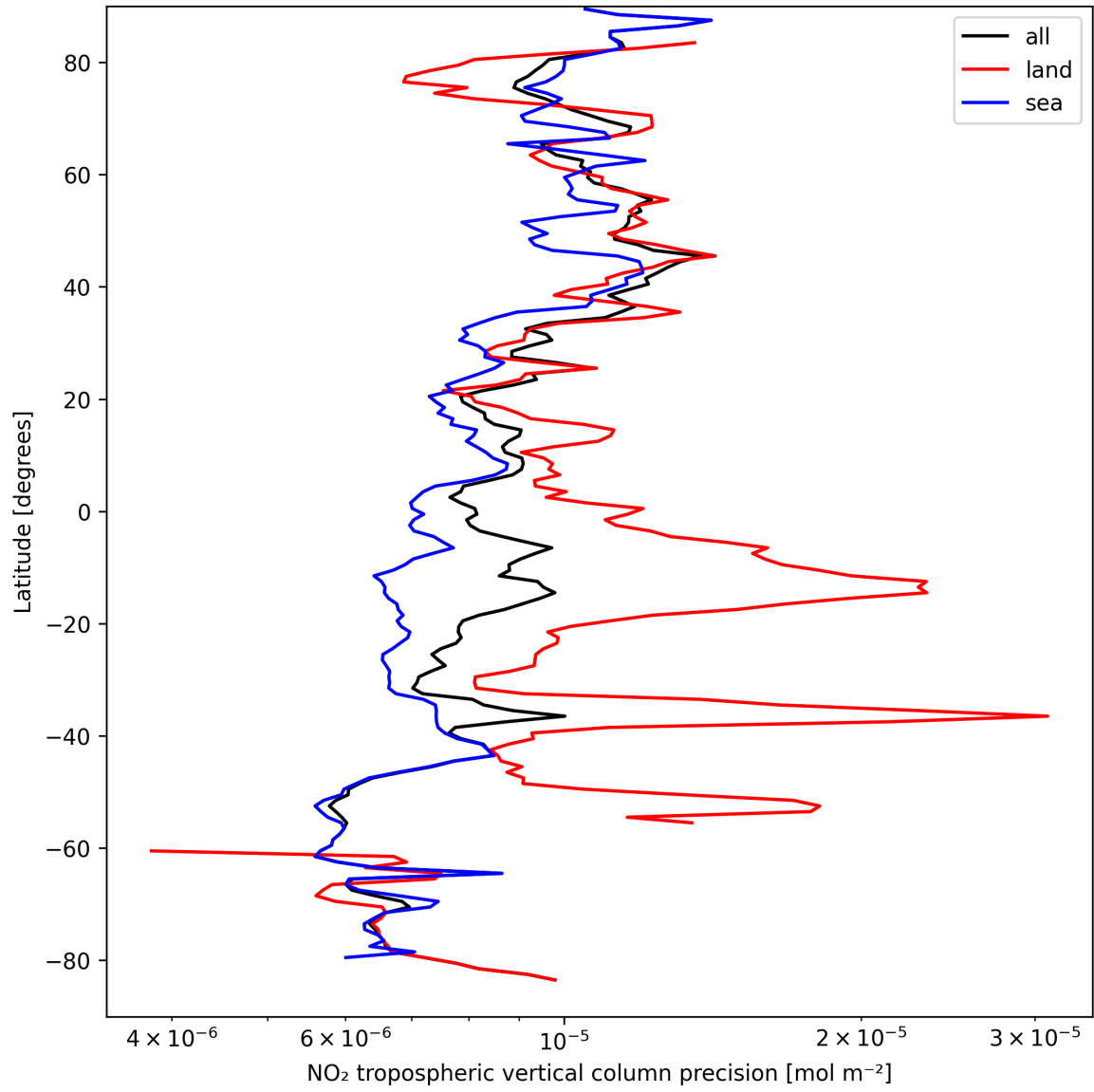
Figure 11: Zonal average of “NO 2 tropospheric vertical column precision” for 2025-09-10 to 2025-09-11.
