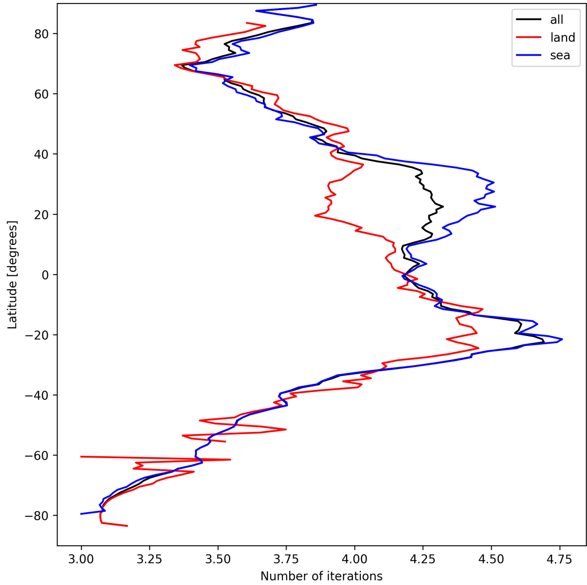
Figure 15: Zonal average of “Number of iterations” for 2025-09-10 to 2025-09-11.
