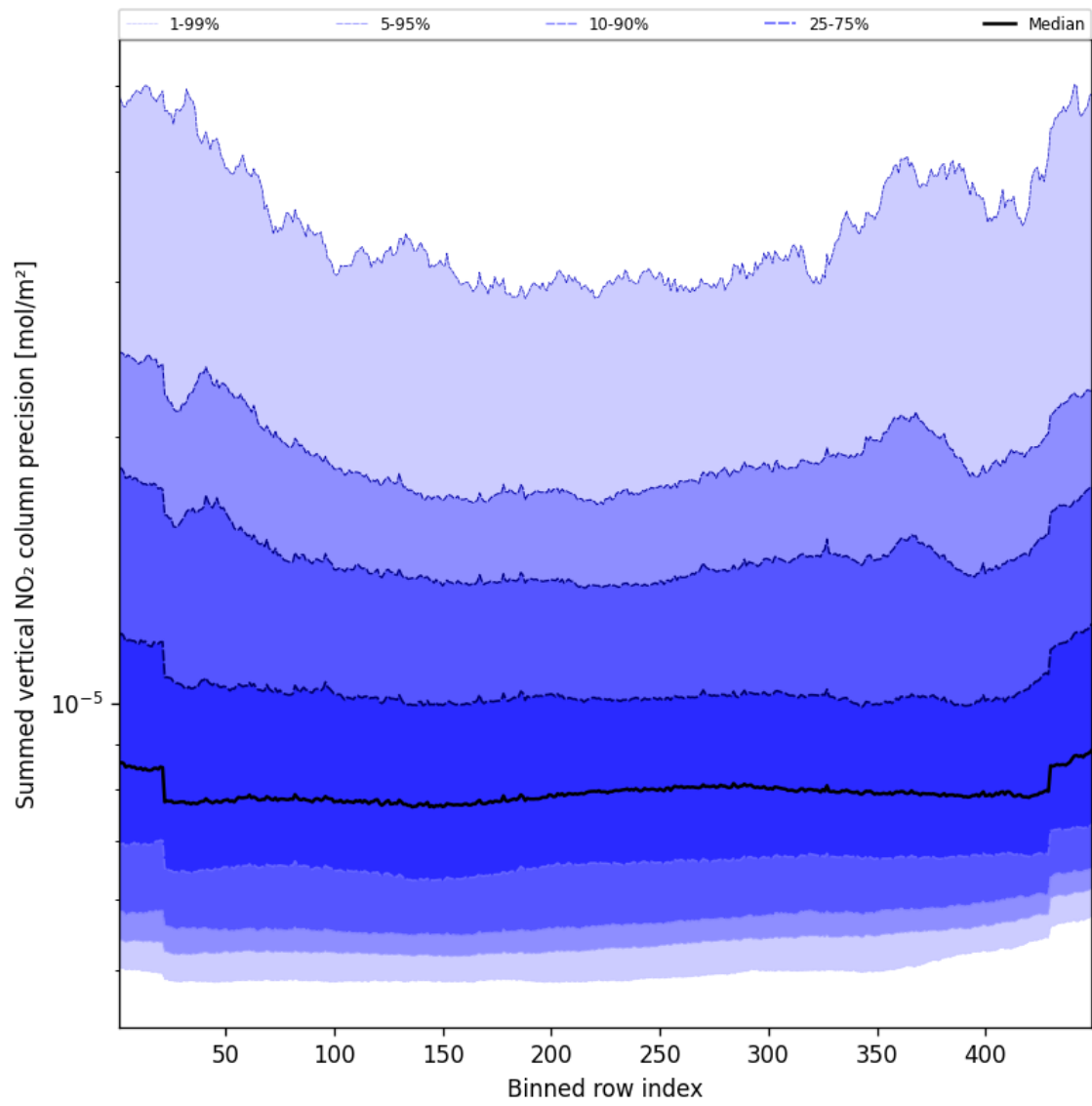
Figure 56: Along track statistics of “Summed vertical NO 2 column precision” for 2025-09-10 to 2025-09-11
