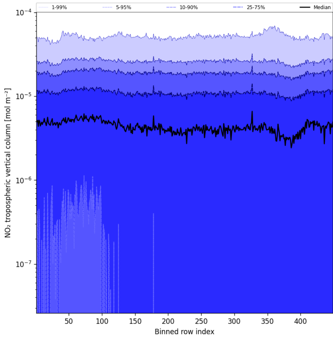
Figure 44: Along track statistics of “NO 2 tropospheric vertical column” for 2025-09-10 to 2025-09-11
