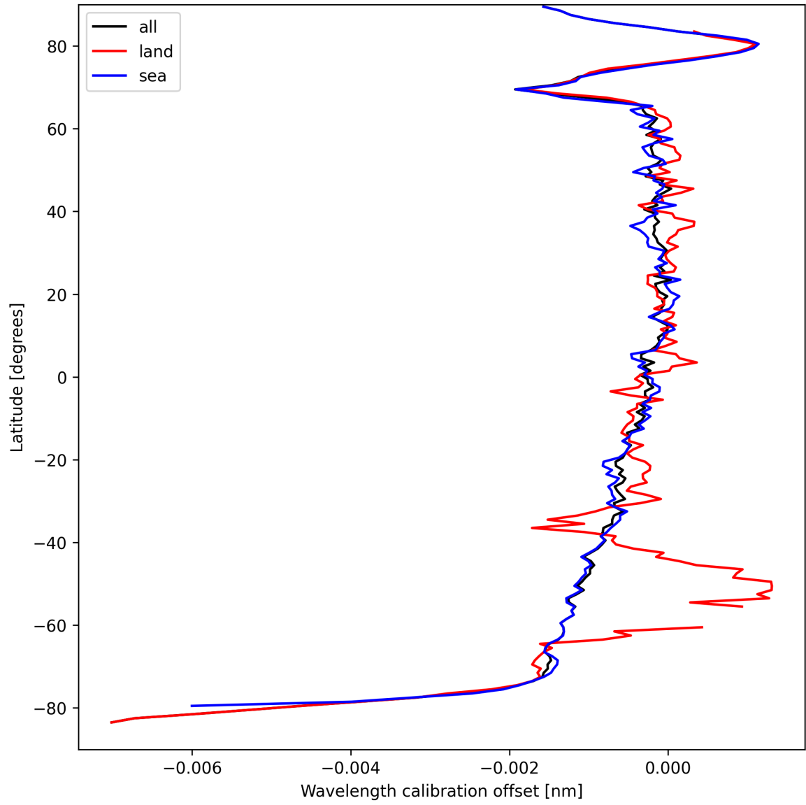
Figure 16: Zonal average of “Wavelength calibration offset” for 2025-09-10 to 2025-09-11.
