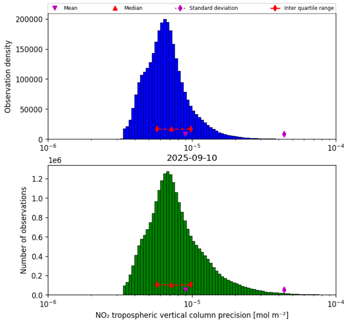
Figure 28: Histogram of “NO 2 tropospheric vertical column precision” for 2025-09-10 to 2025-09-11
