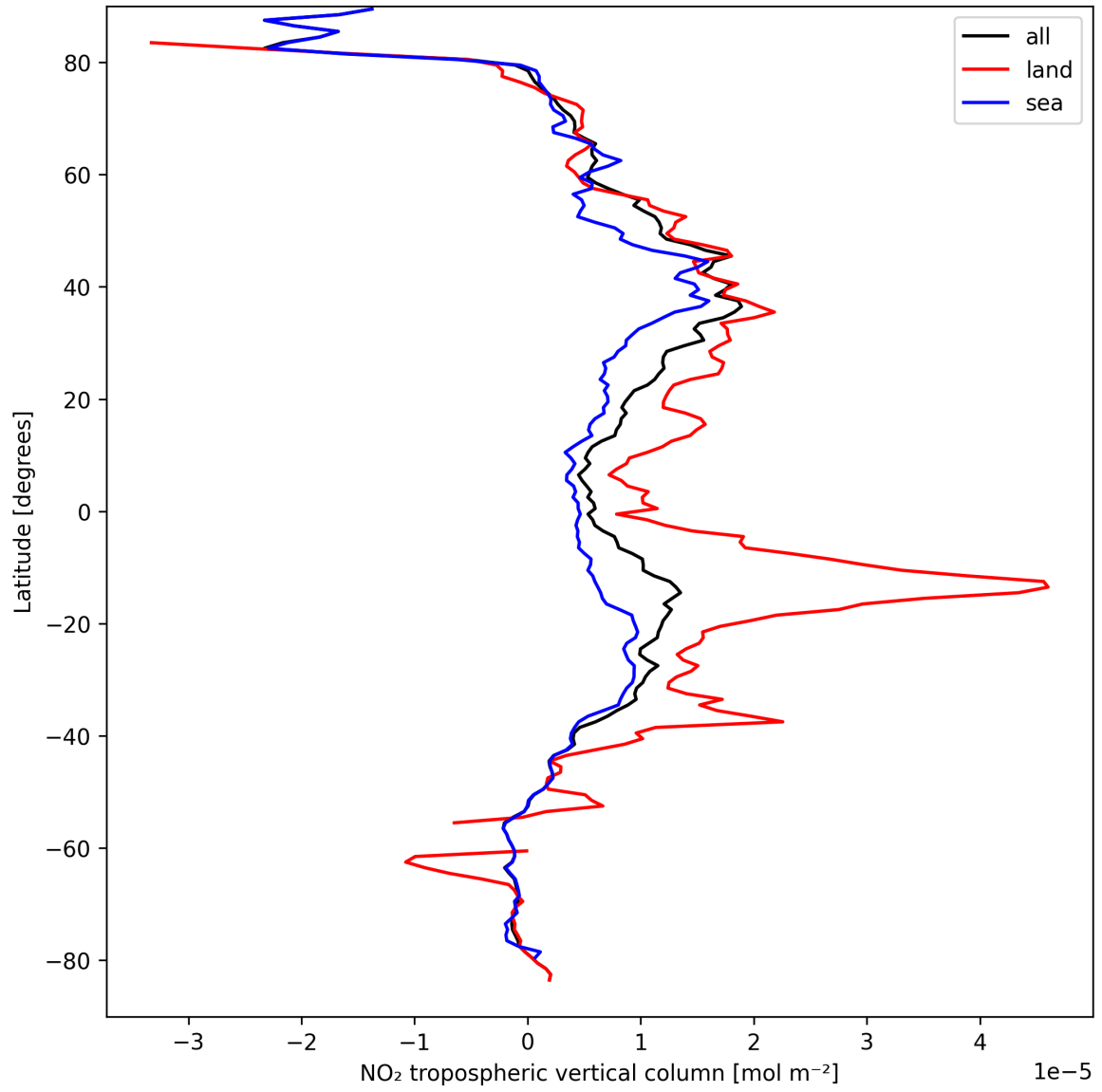
Figure 10: Zonal average of “NO 2 tropospheric vertical column” for 2025-09-10 to 2025-09-11.
