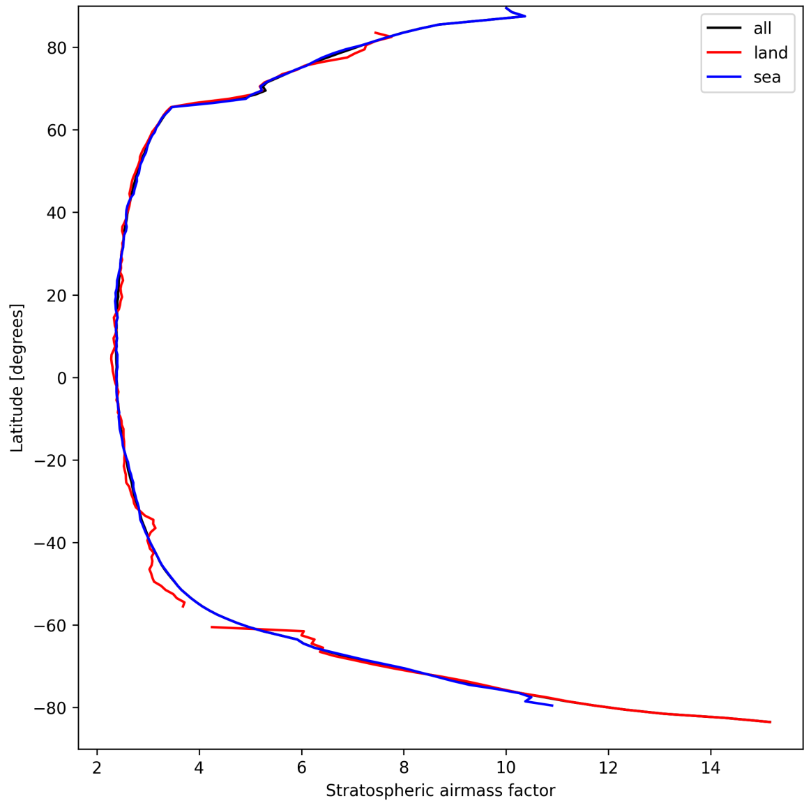
Figure 25: Zonal average of “Stratospheric airmass factor” for 2025-09-10 to 2025-09-11.
