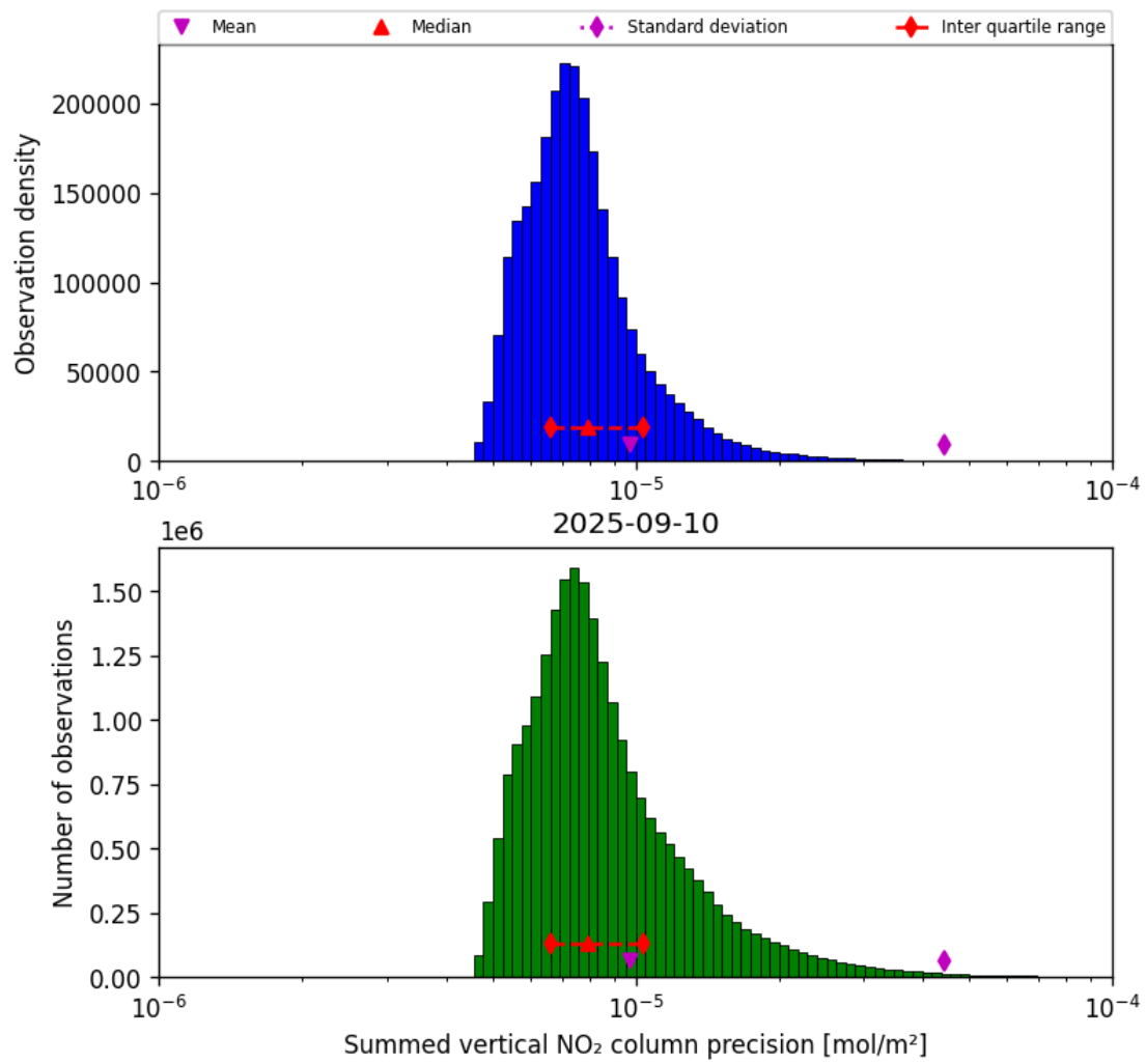
Figure 39: Histogram of “Summed vertical NO 2 column precision” for 2025-09-10 to 2025-09-11
