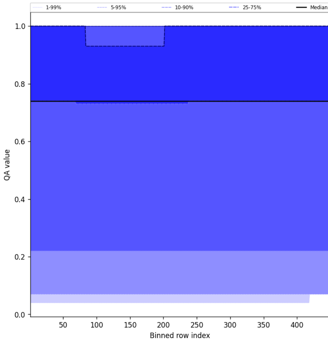
Figure 43: Along track statistics of “QA value” for 2025-09-10 to 2025-09-11
