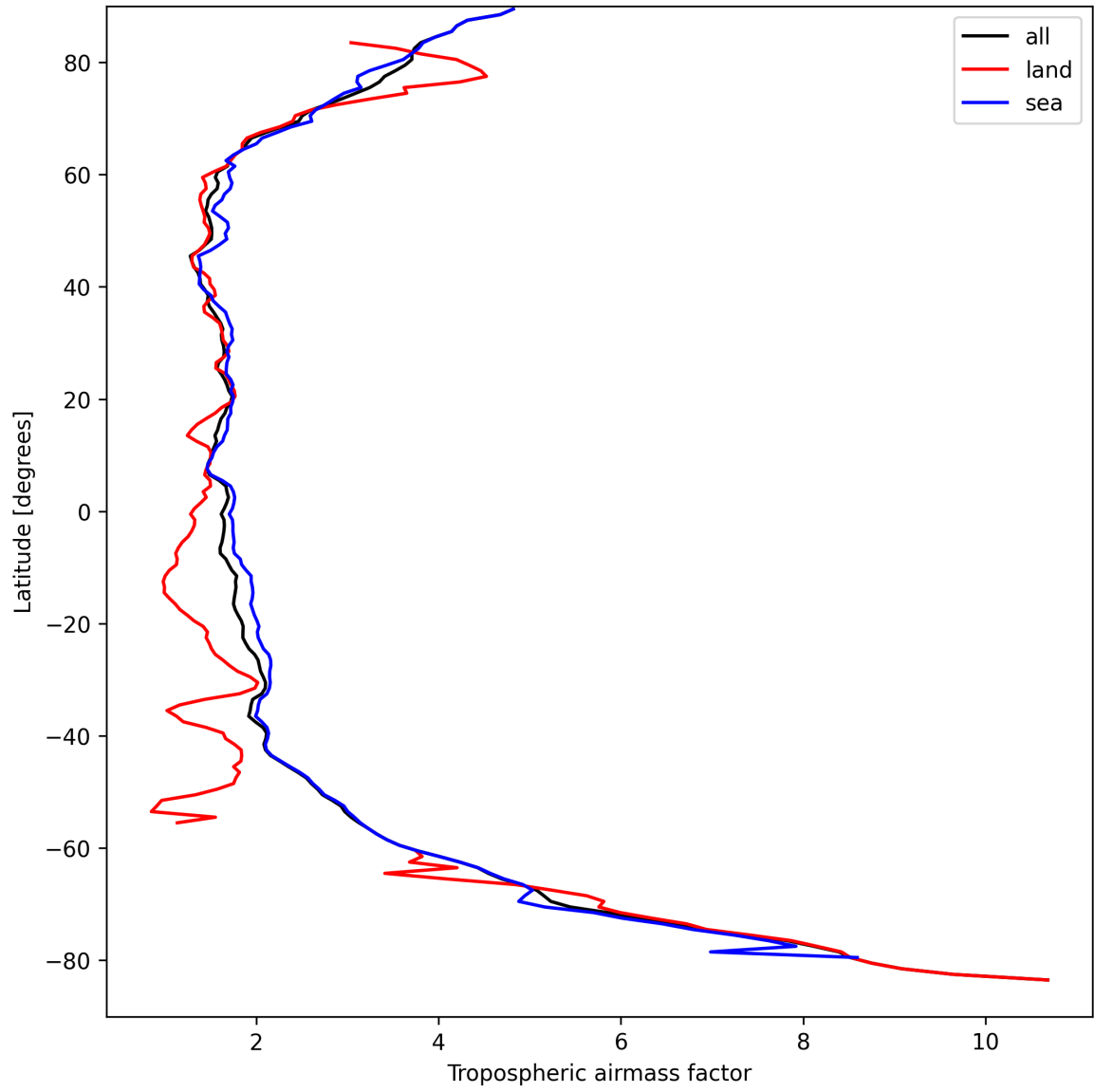
Figure 12: Zonal average of “Tropospheric airmass factor” for 2025-09-10 to 2025-09-11.
