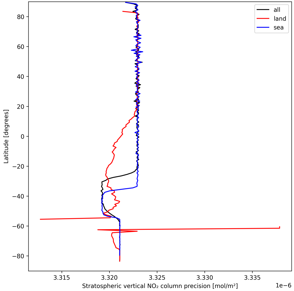
Figure 18: Zonal average of “Stratospheric vertical NO 2 column precision” for 2025-09-10 to 2025-09-11.
