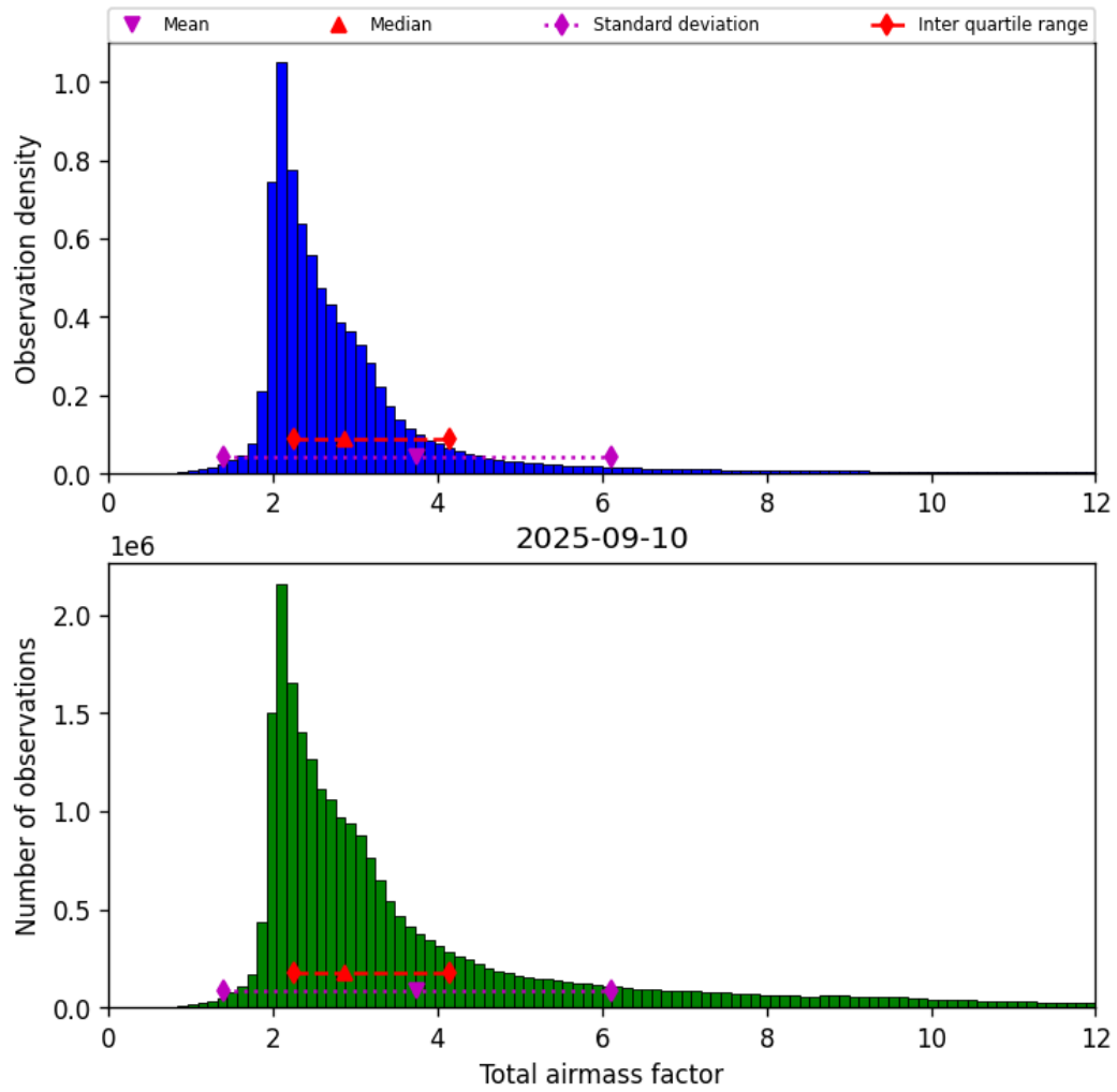
Figure 30: Histogram of “Total airmass factor” for 2025-09-10 to 2025-09-11
