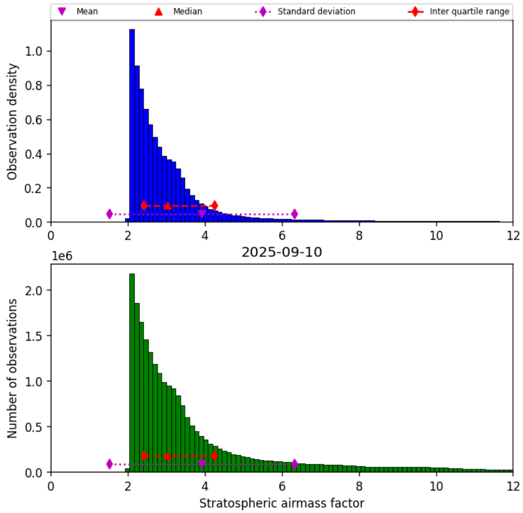
Figure 42: Histogram of “Stratospheric airmass factor” for 2025-09-10 to 2025-09-11
