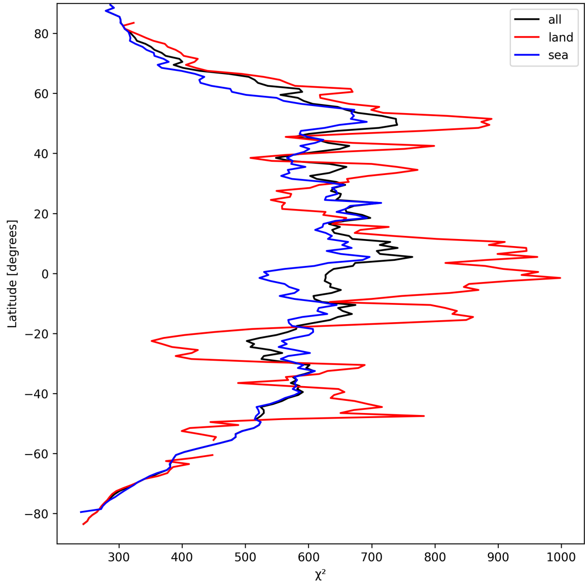
Figure 23: Zonal average of “ \chi^2 ” for 2025-09-10 to 2025-09-11.
