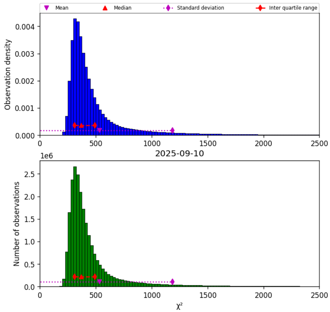
Figure 40: Histogram of “ \chi^2 ” for 2025-09-10 to 2025-09-11
