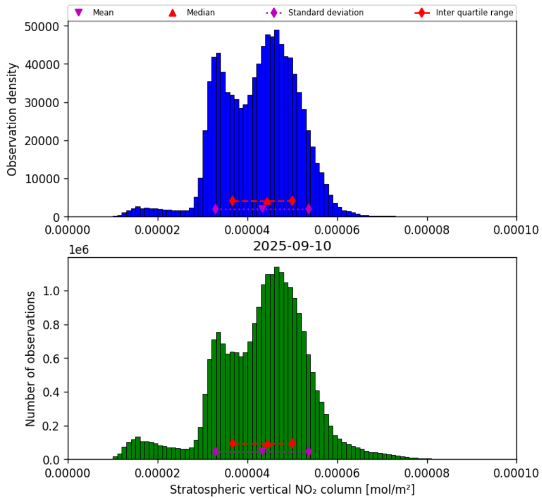
Figure 34: Histogram of “Stratospheric vertical NO 2 column” for 2025-09-10 to 2025-09-11
