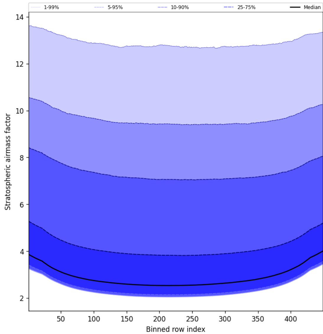
Figure 59: Along track statistics of “Stratospheric airmass factor” for 2025-09-10 to 2025-09-11
