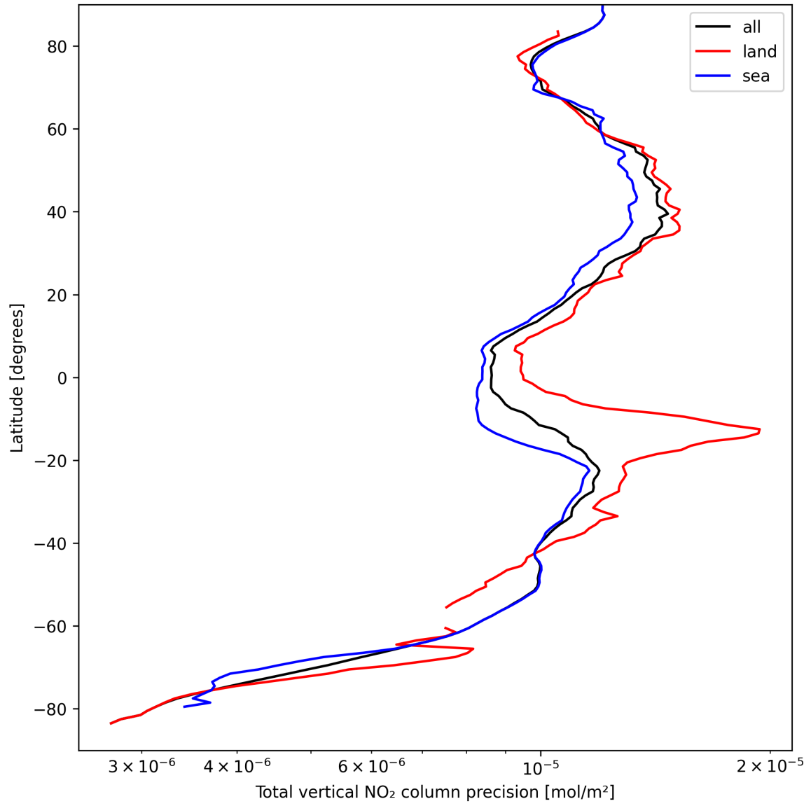
Figure 20: Zonal average of “Total vertical NO 2 column precision” for 2025-09-10 to 2025-09-11.
