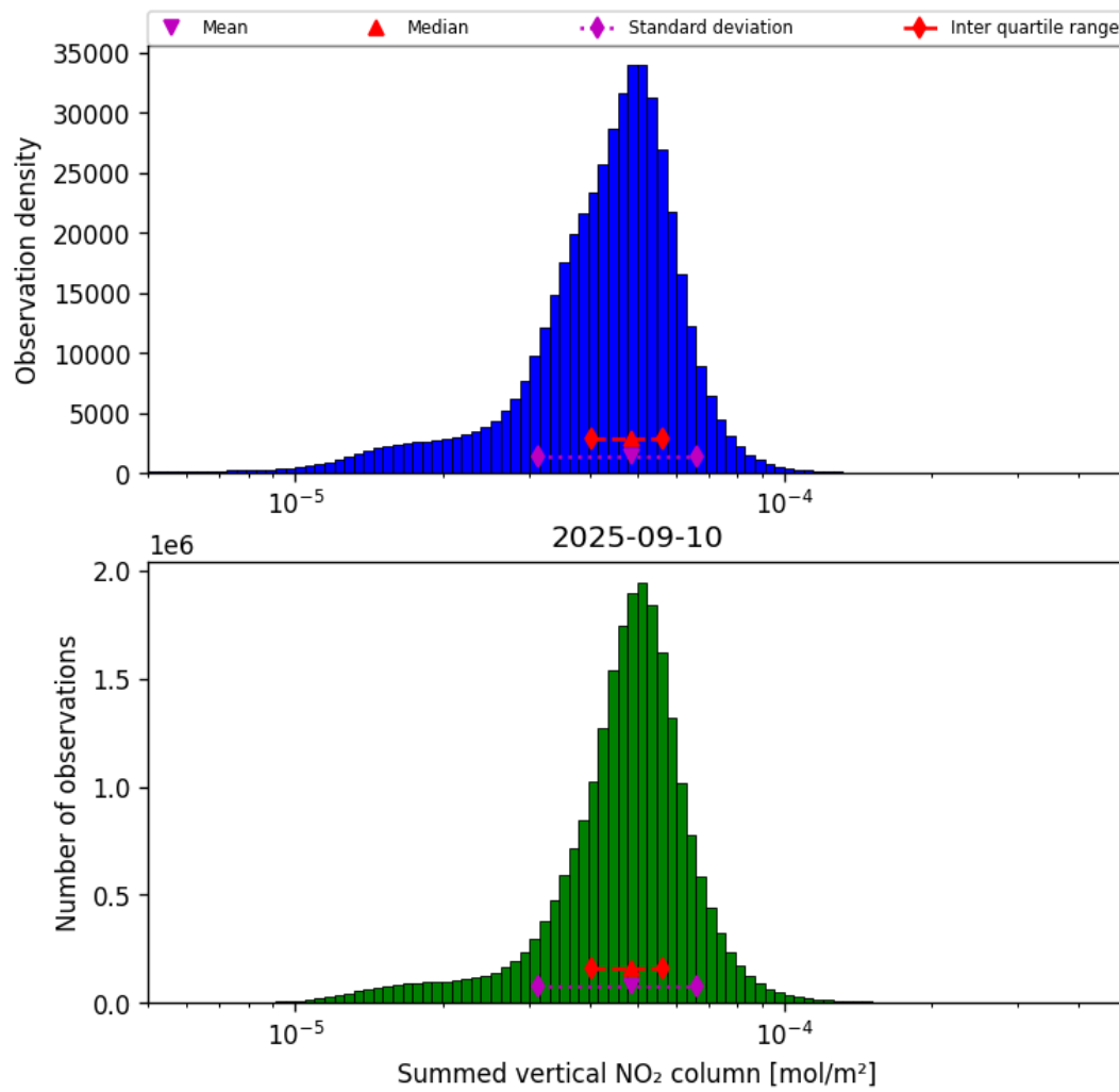
Figure 38: Histogram of “Summed vertical NO 2 column” for 2025-09-10 to 2025-09-11
