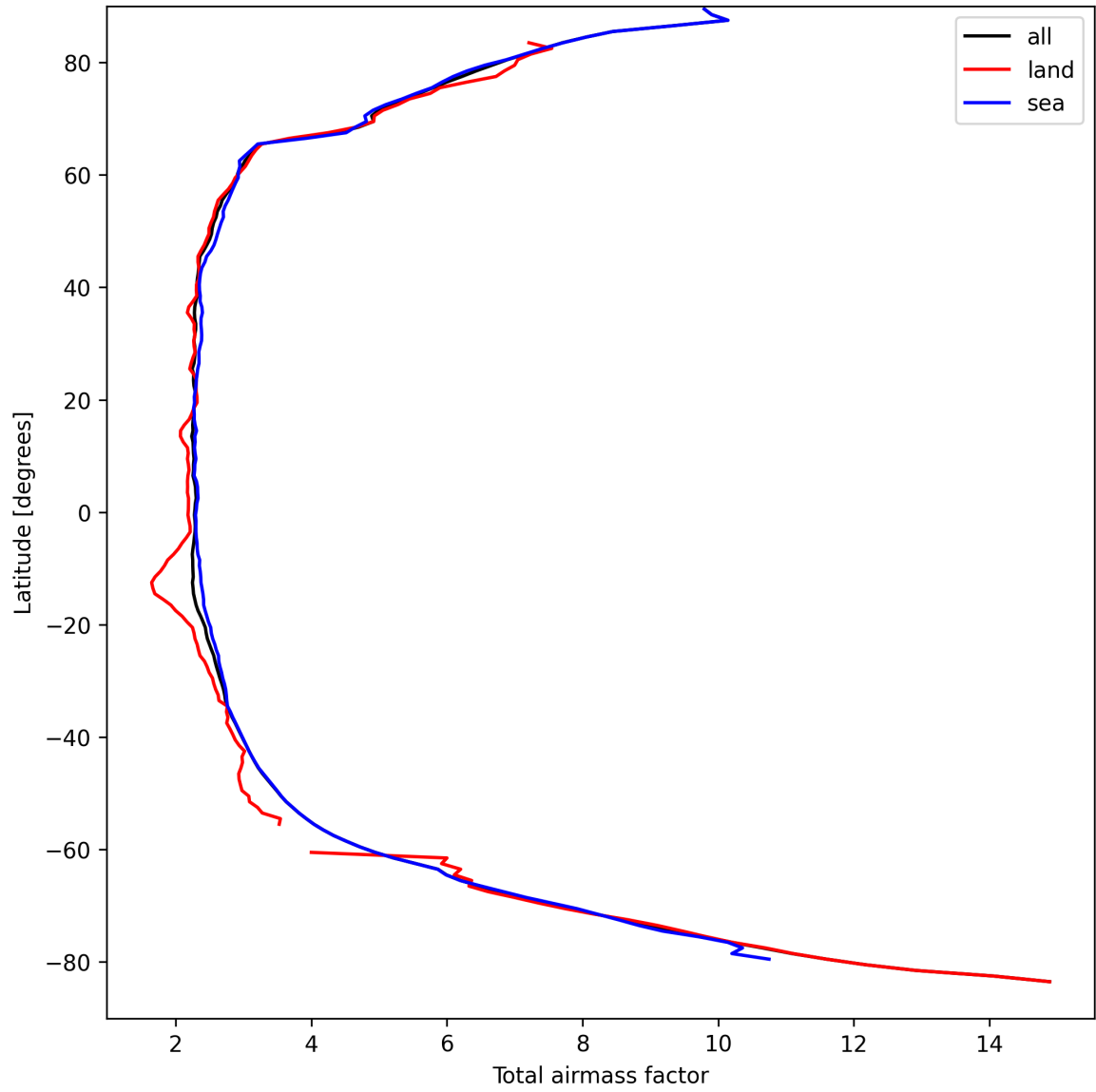
Figure 13: Zonal average of “Total airmass factor” for 2025-09-10 to 2025-09-11.
