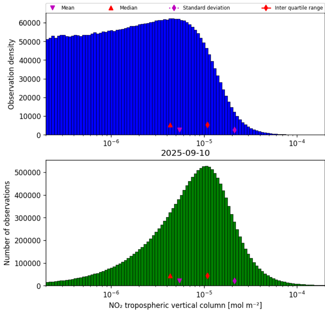
Figure 27: Histogram of “NO 2 tropospheric vertical column” for 2025-09-10 to 2025-09-11
