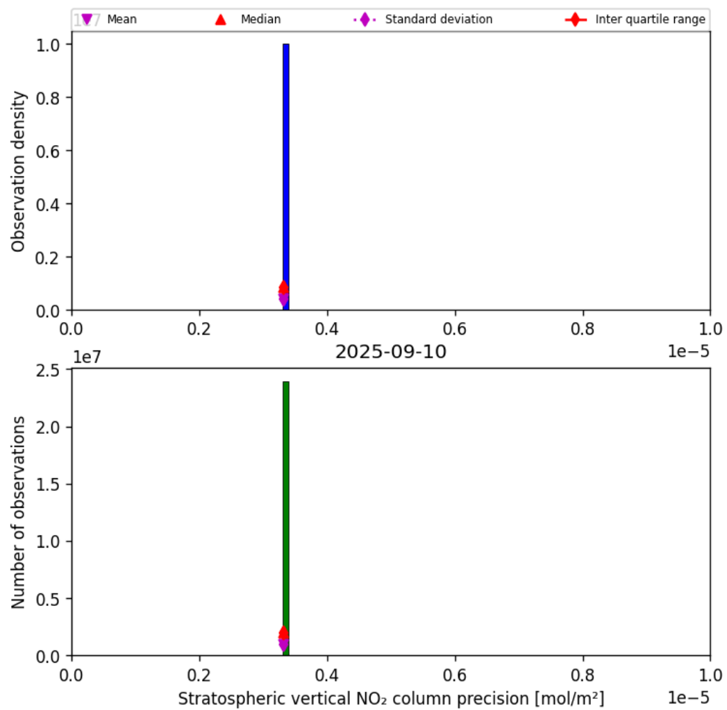
Figure 35: Histogram of “Stratospheric vertical NO 2 column precision” for 2025-09-10 to 2025-09-11
