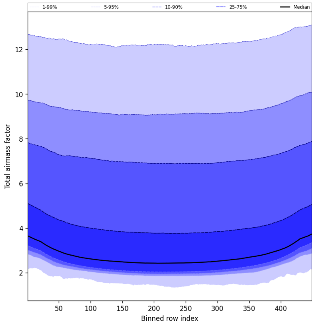
Figure 47: Along track statistics of “Total airmass factor” for 2025-09-10 to 2025-09-11
