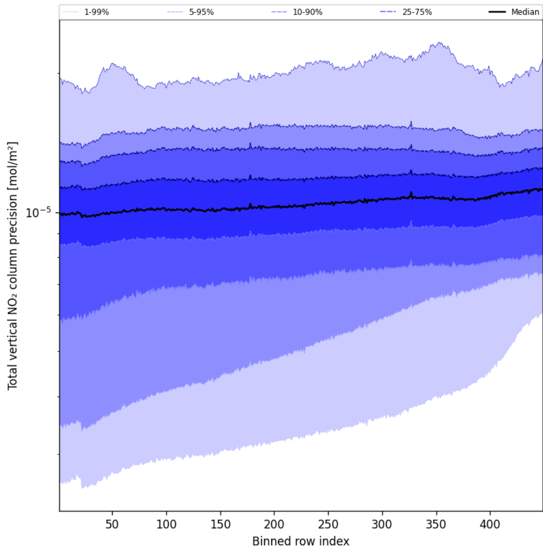
Figure 54: Along track statistics of “Total vertical NO 2 column precision” for 2025-09-10 to 2025-09-11
