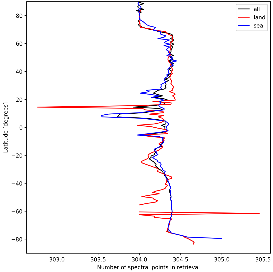
Figure 14: Zonal average of “Number of spectral points in retrieval” for 2025-09-10 to 2025-09-11.
