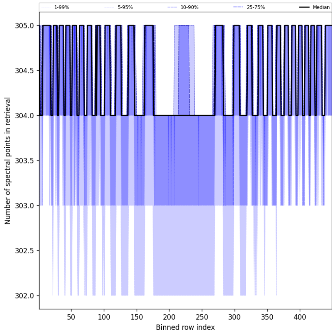
Figure 48: Along track statistics of “Number of spectral points in retrieval” for 2025-09-10 to 2025-09-11
