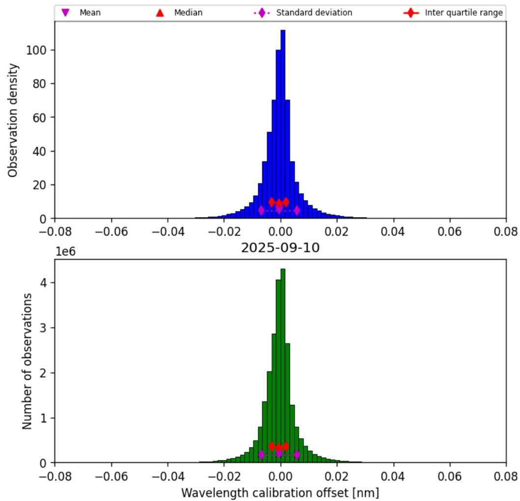
Figure 33: Histogram of “Wavelength calibration offset” for 2025-09-10 to 2025-09-11
