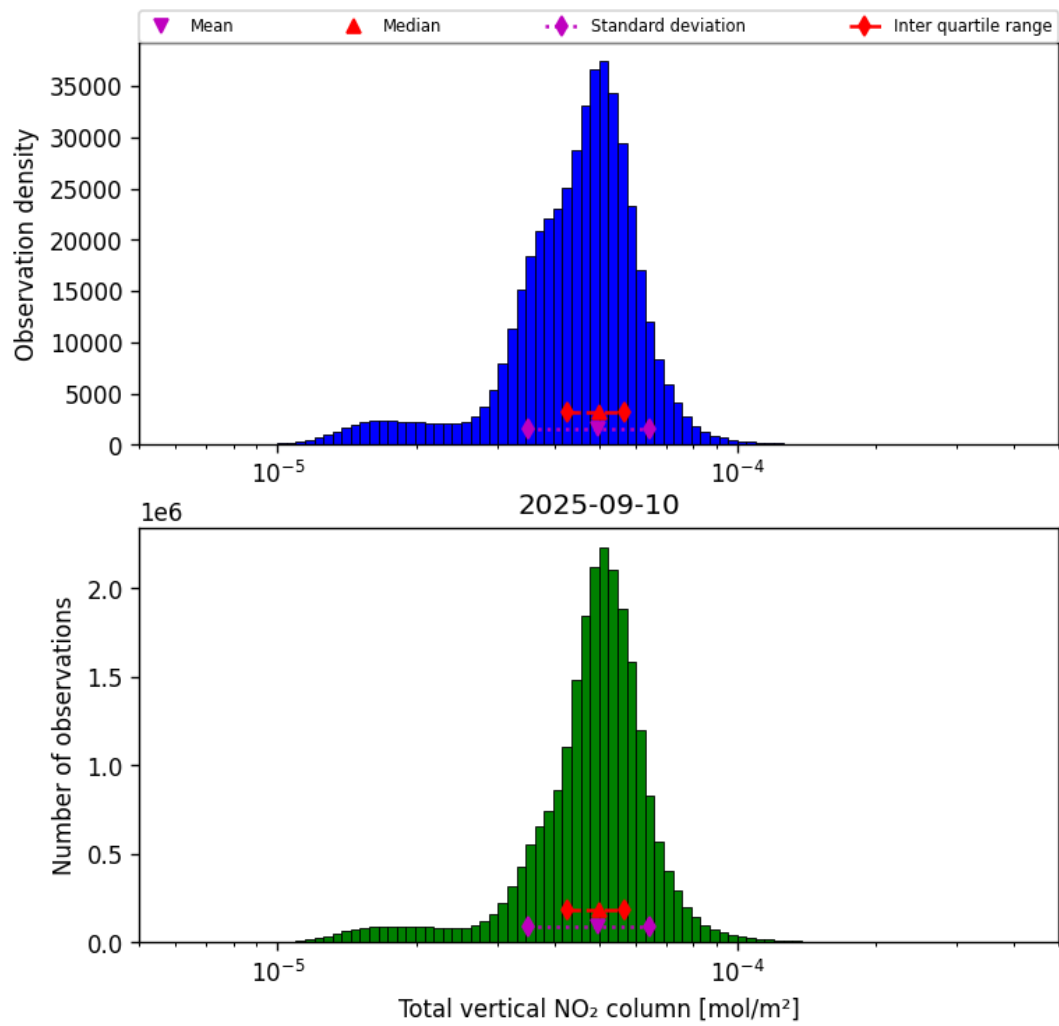
Figure 36: Histogram of “Total vertical NO 2 column” for 2025-09-10 to 2025-09-11
