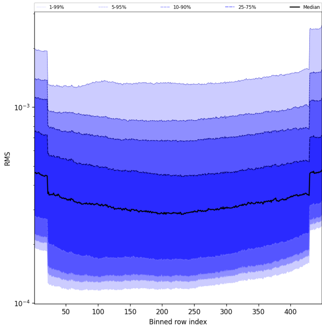
Figure 58: Along track statistics of “RMS” for 2025-09-10 to 2025-09-11
