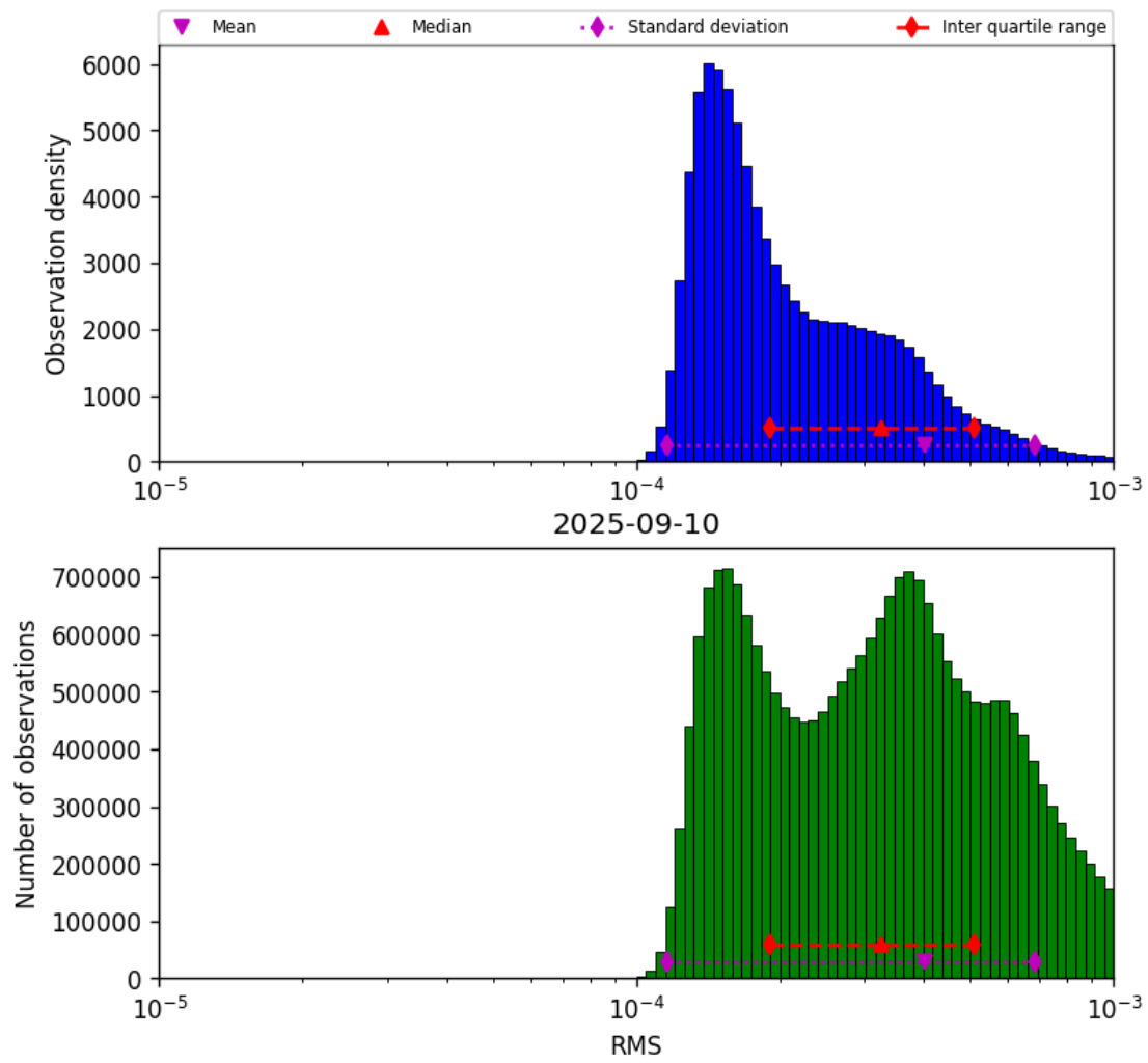
Figure 41: Histogram of “RMS” for 2025-09-10 to 2025-09-11
