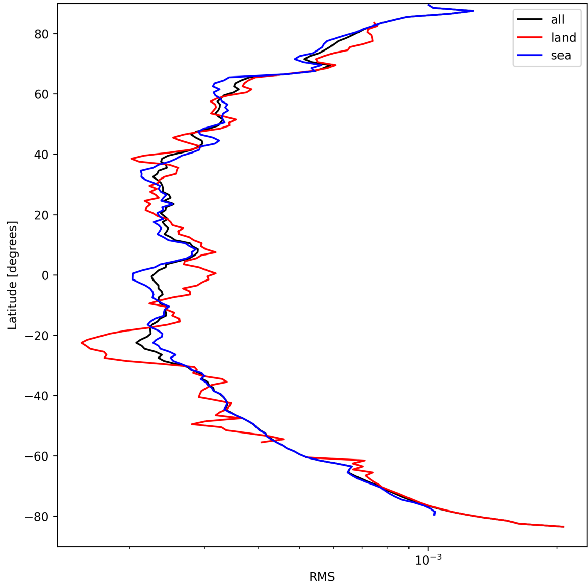
Figure 24: Zonal average of “RMS” for 2025-09-10 to 2025-09-11.
