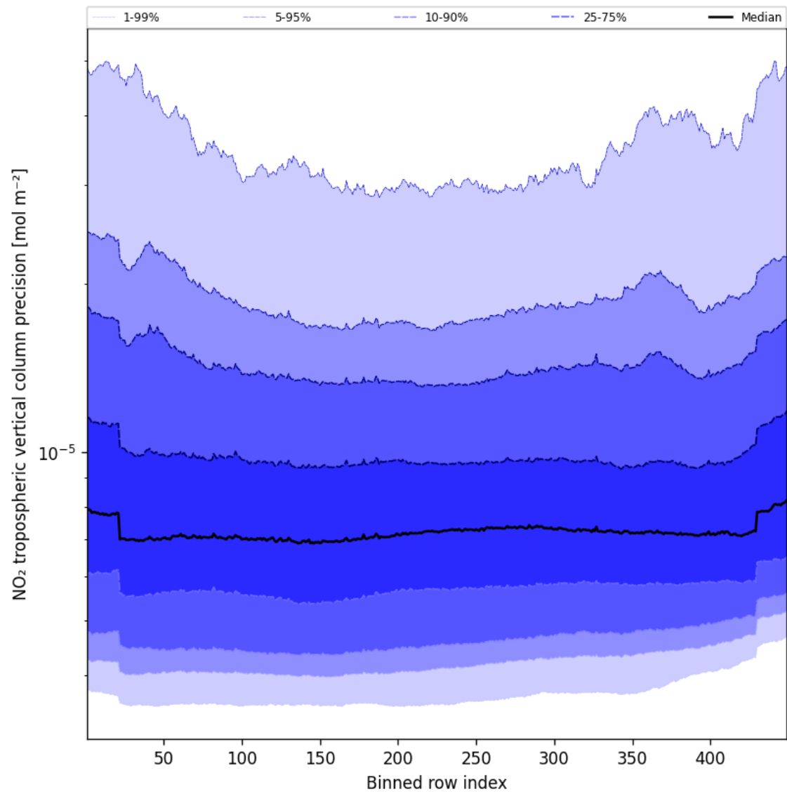
Figure 45: Along track statistics of “NO 2 tropospheric vertical column precision” for 2025-09-10 to 2025-09-11
