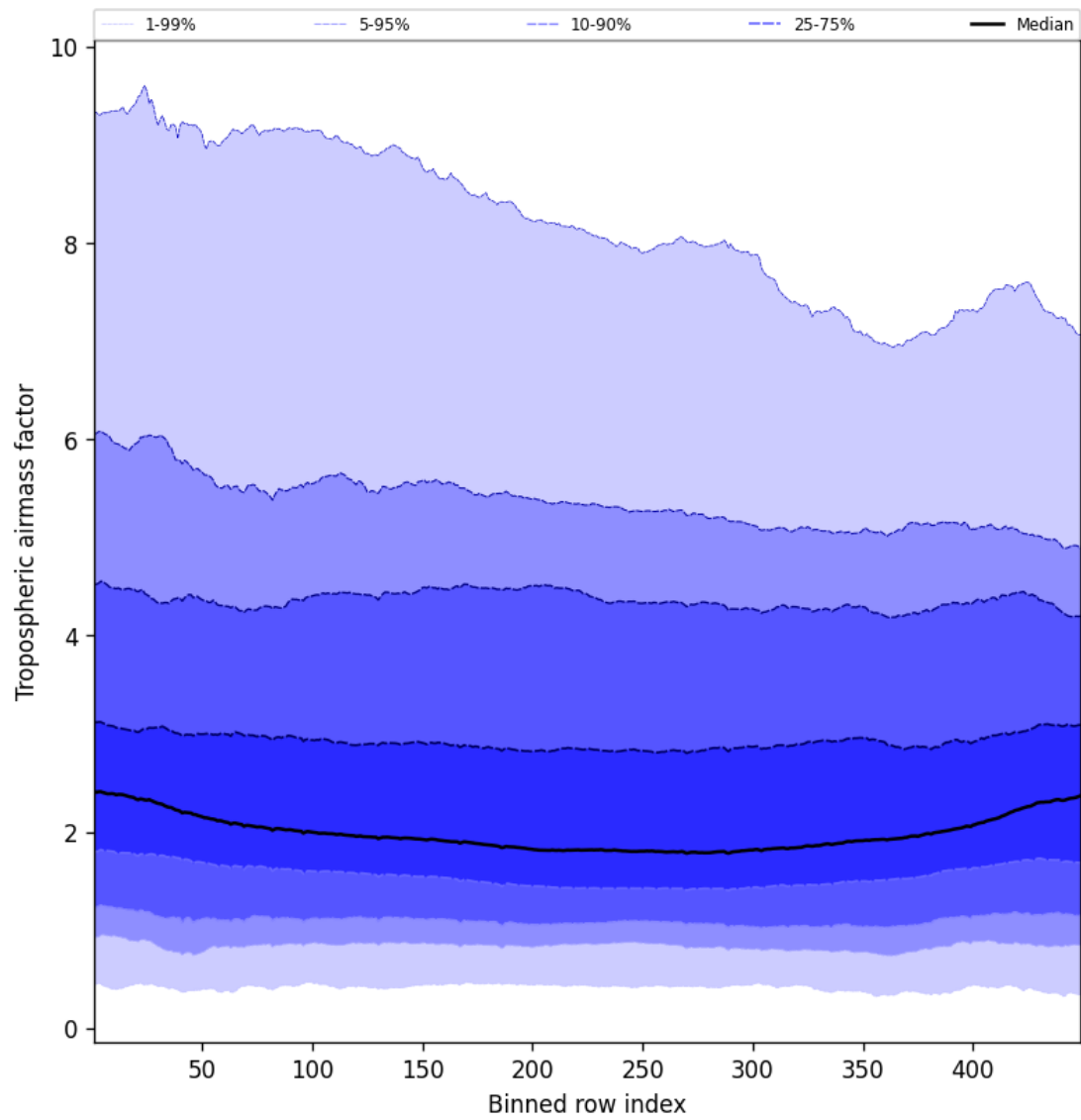
Figure 46: Along track statistics of “Tropospheric air mass factor” for 2025-09-10 to 2025-09-11
