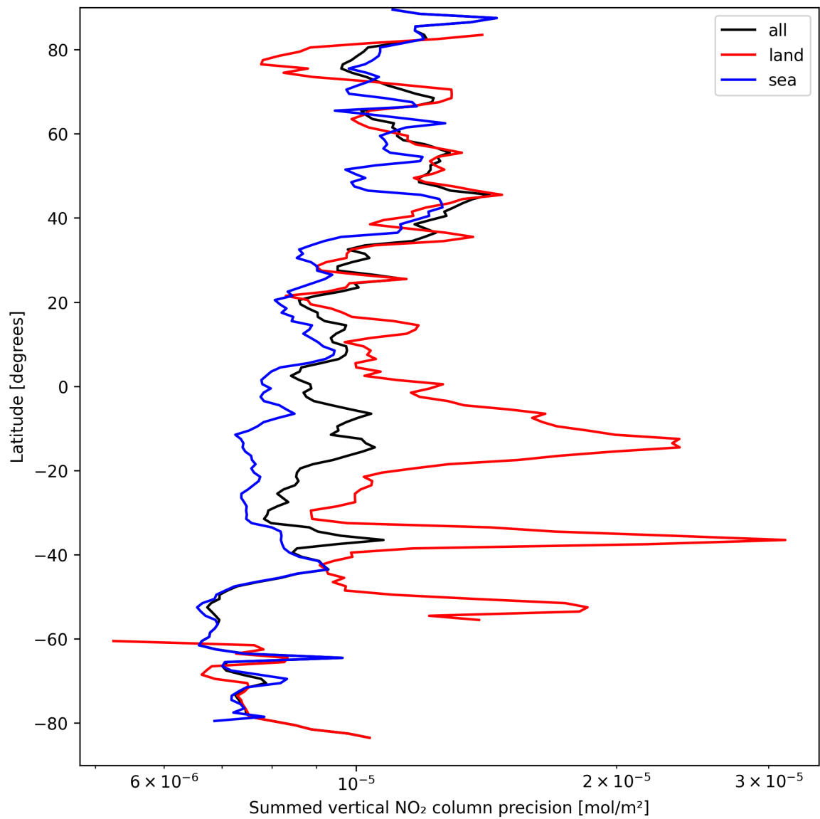
Figure 22: Zonal average of “Summed vertical NO 2 column precision” for 2025-09-10 to 2025-09-11.
