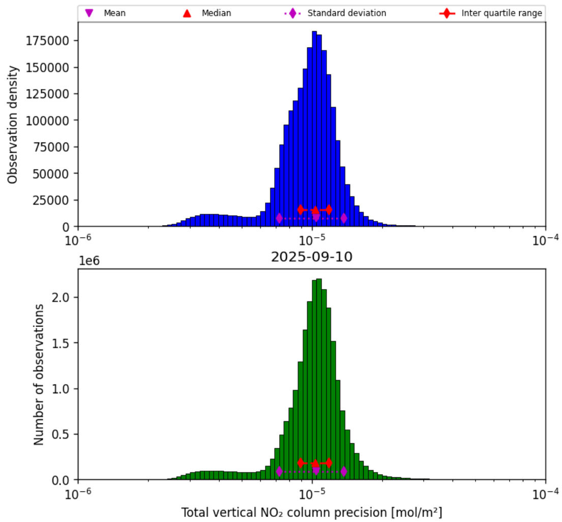
Figure 37: Histogram of “Total vertical NO 2 column precision” for 2025-09-10 to 2025-09-11
