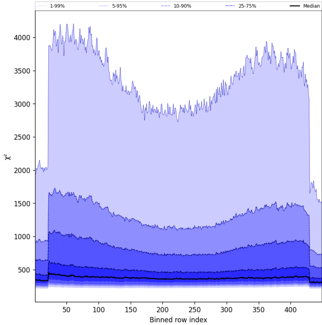
Figure 57: Along track statistics of “ \chi^2 ” for 2025-09-10 to 2025-09-11
