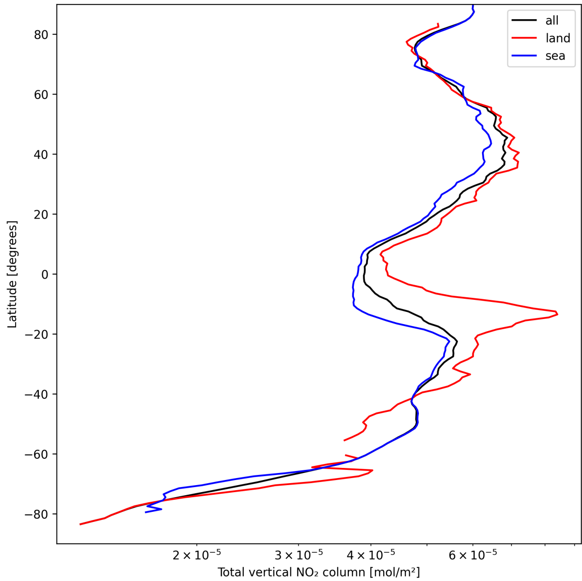
Figure 19: Zonal average of “Total vertical NO 2 column” for 2025-09-10 to 2025-09-11.
