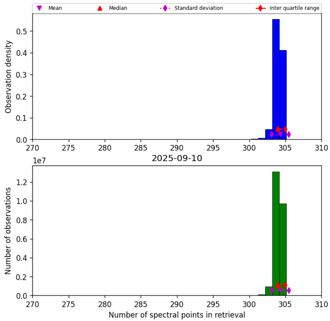
Figure 31: Histogram of “Number of spectral points in retrieval” for 2025-09-10 to 2025-09-11
