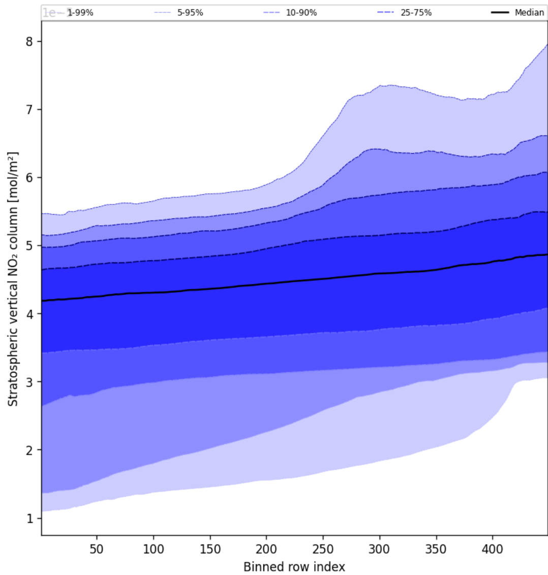
Figure 51: Along track statistics of “Stratospheric vertical NO 2 column” for 2025-09-10 to 2025-09-11
