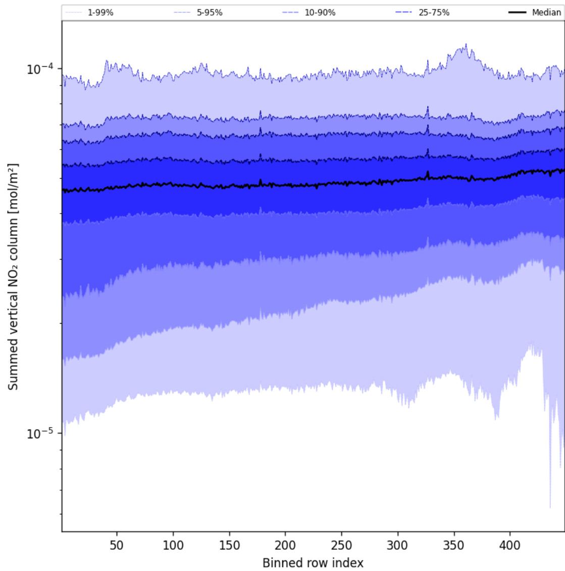
Figure 55: Along track statistics of “Summed vertical NO 2 column” for 2025-09-10 to 2025-09-11
