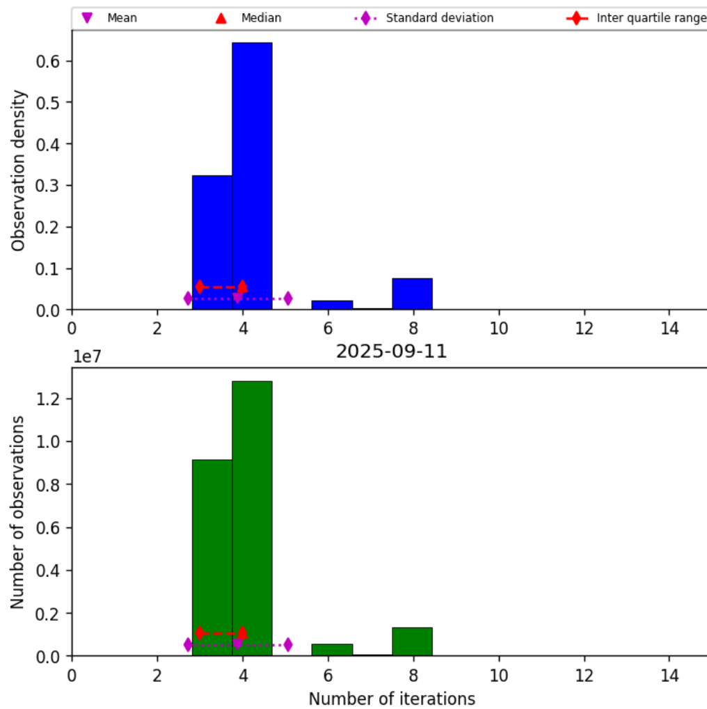
Figure 32: Histogram of “Number of iterations” for 2025-09-11 to 2025-09-12
