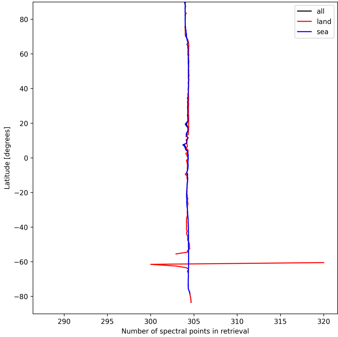
Figure 14: Zonal average of “Number of spectral points in retrieval” for 2025-09-11 to 2025-09-12.
