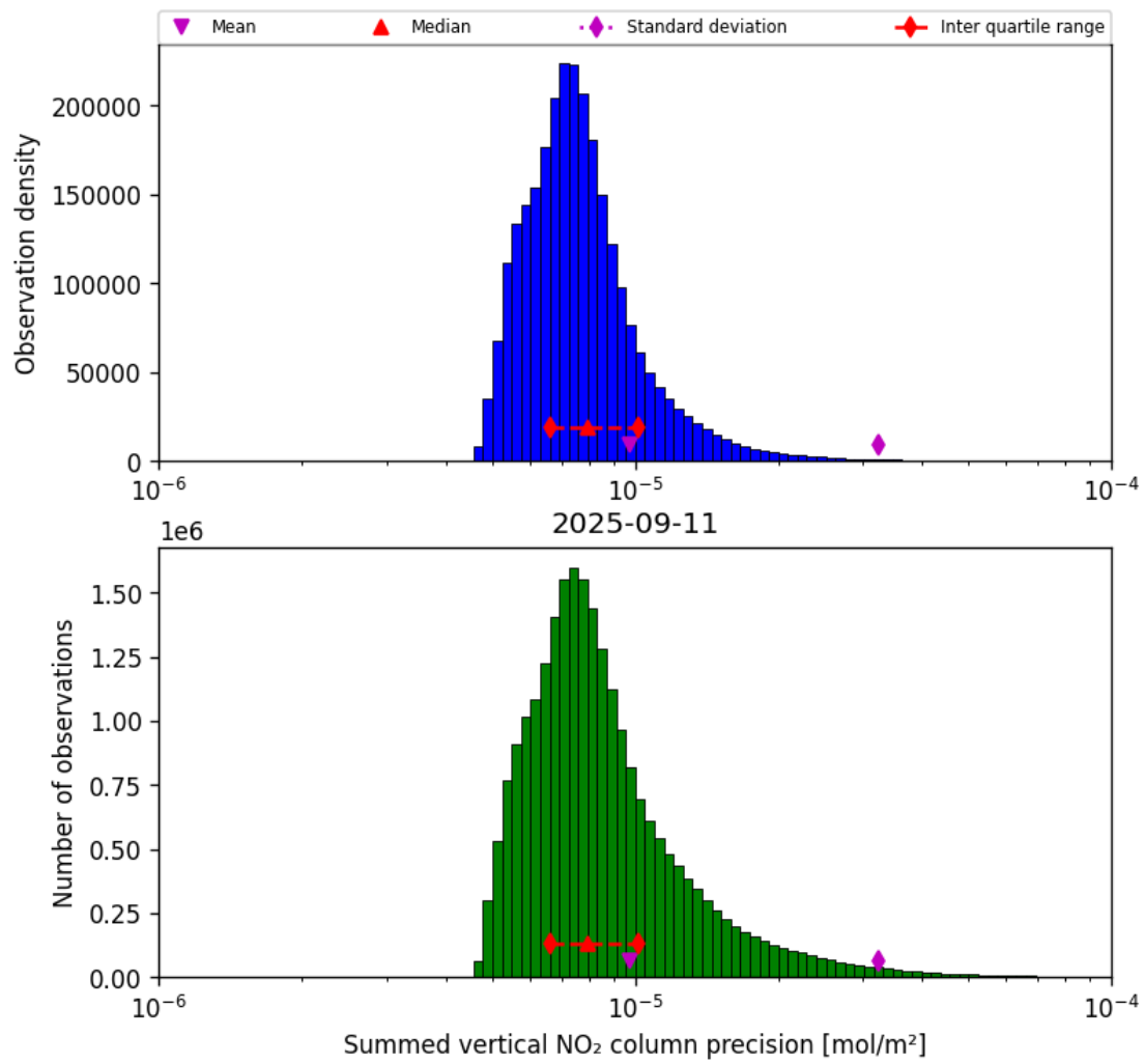
Figure 39: Histogram of “Summed vertical NO 2 column precision” for 2025-09-11 to 2025-09-12
