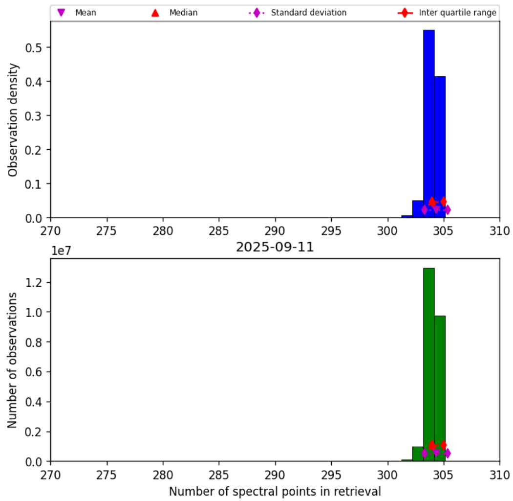
Figure 31: Histogram of “Number of spectral points in retrieval” for 2025-09-11 to 2025-09-12
