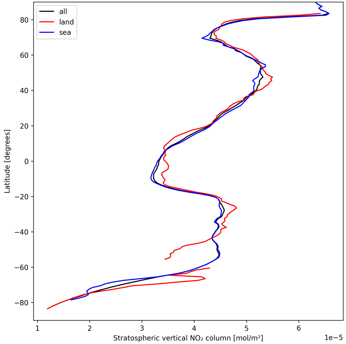
Figure 17: Zonal average of “Stratospheric vertical NO 2 column” for 2025-09-11 to 2025-09-12.
