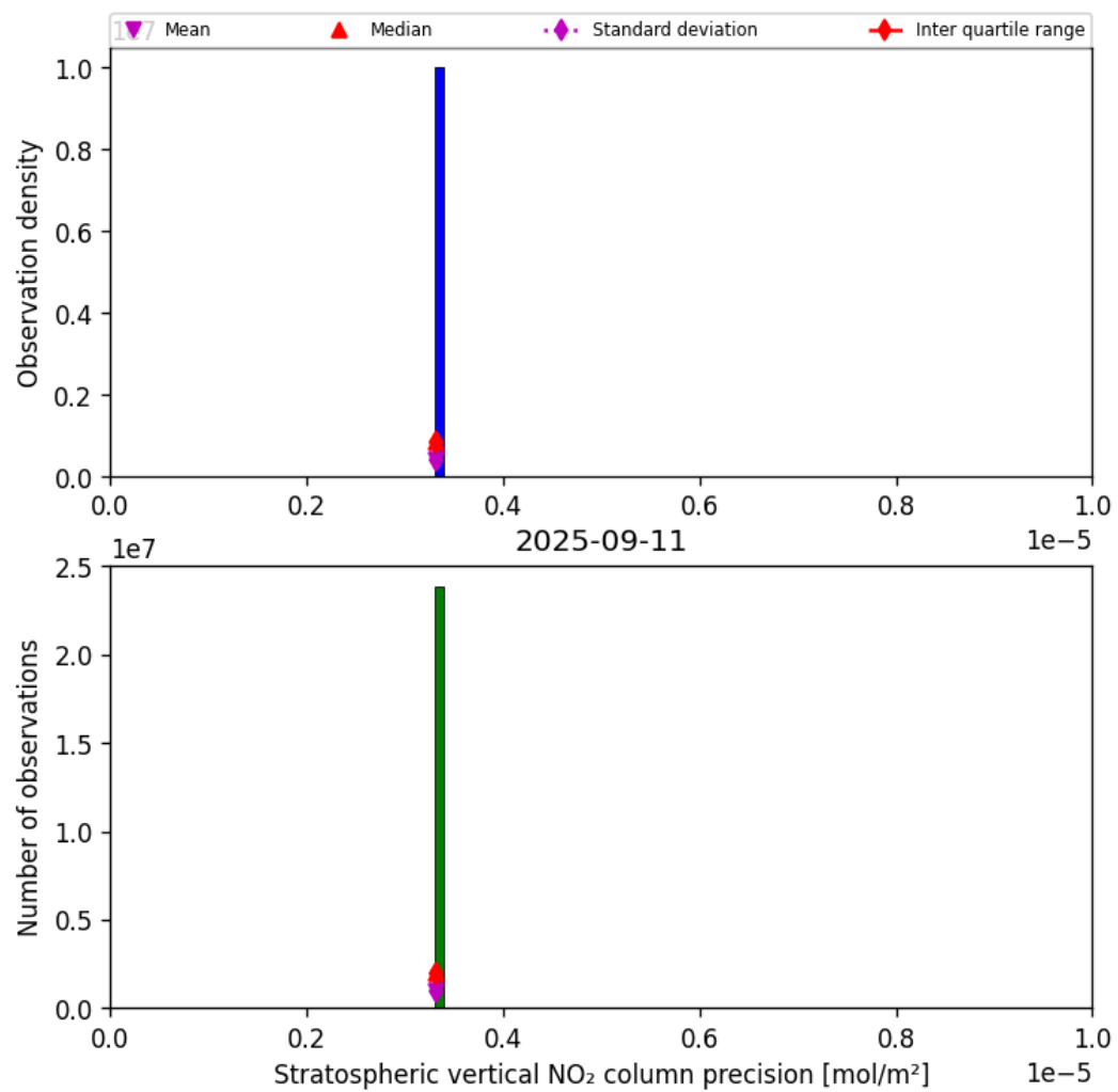
Figure 35: Histogram of “Stratospheric vertical NO 2 column precision” for 2025-09-11 to 2025-09-12
