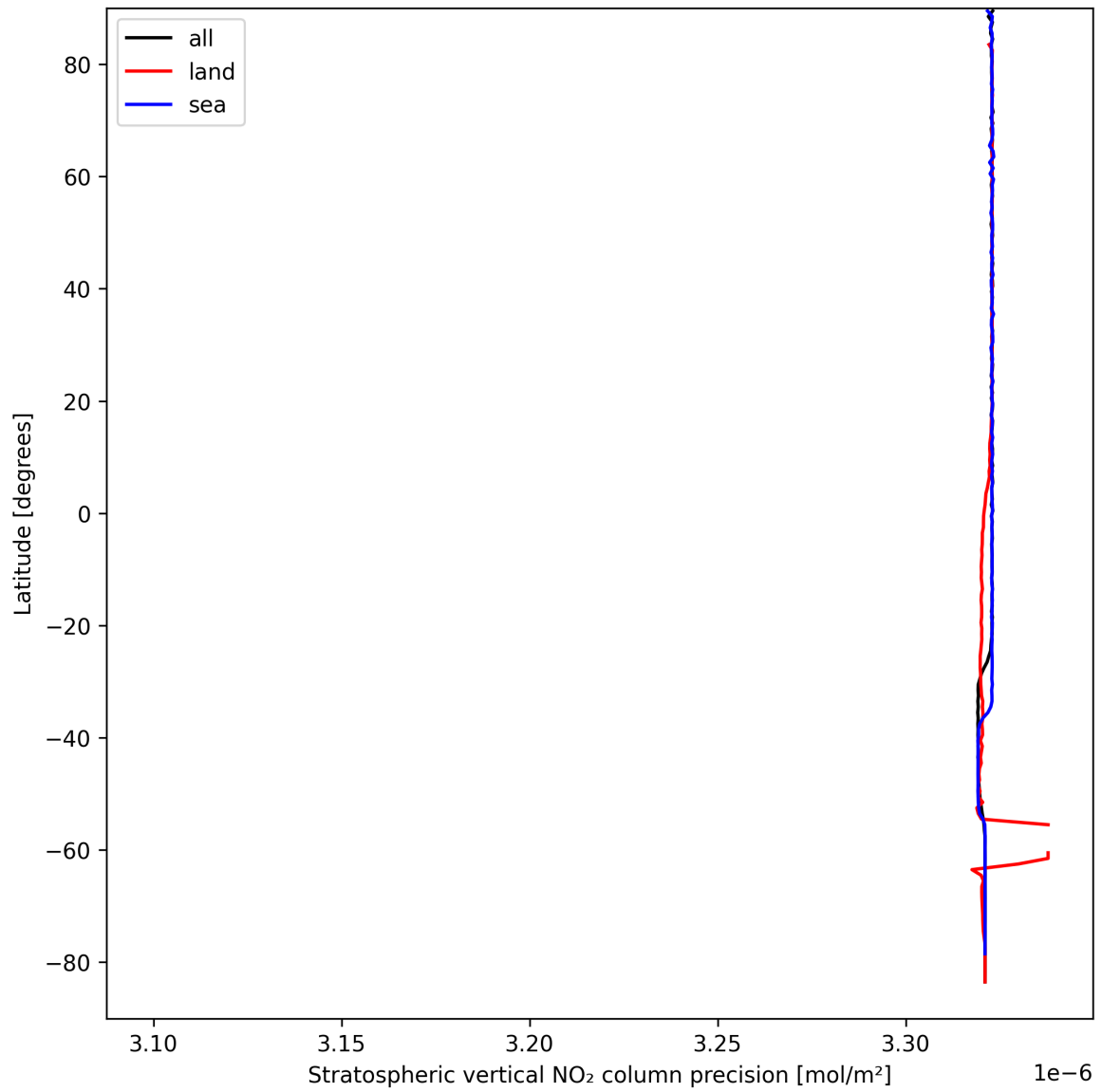
Figure 18: Zonal average of “Stratospheric vertical NO 2 column precision” for 2025-09-11 to 2025-09-12.
