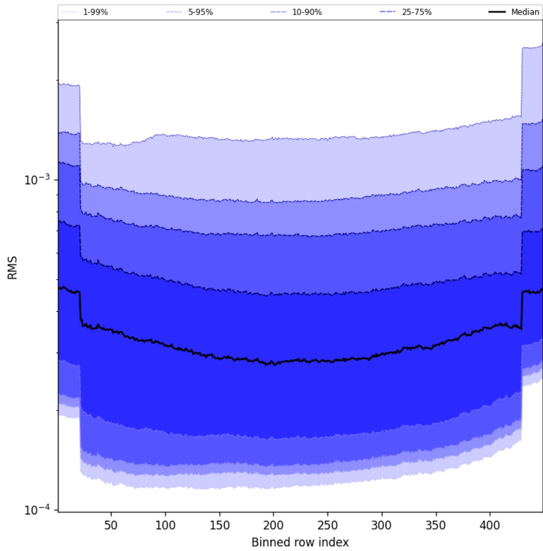
Figure 58: Along track statistics of “RMS” for 2025-09-11 to 2025-09-12
