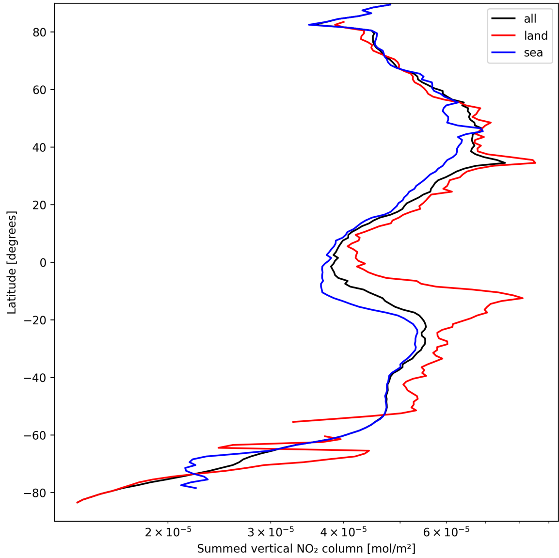
Figure 21: Zonal average of “Summed vertical NO 2 column” for 2025-09-11 to 2025-09-12.
