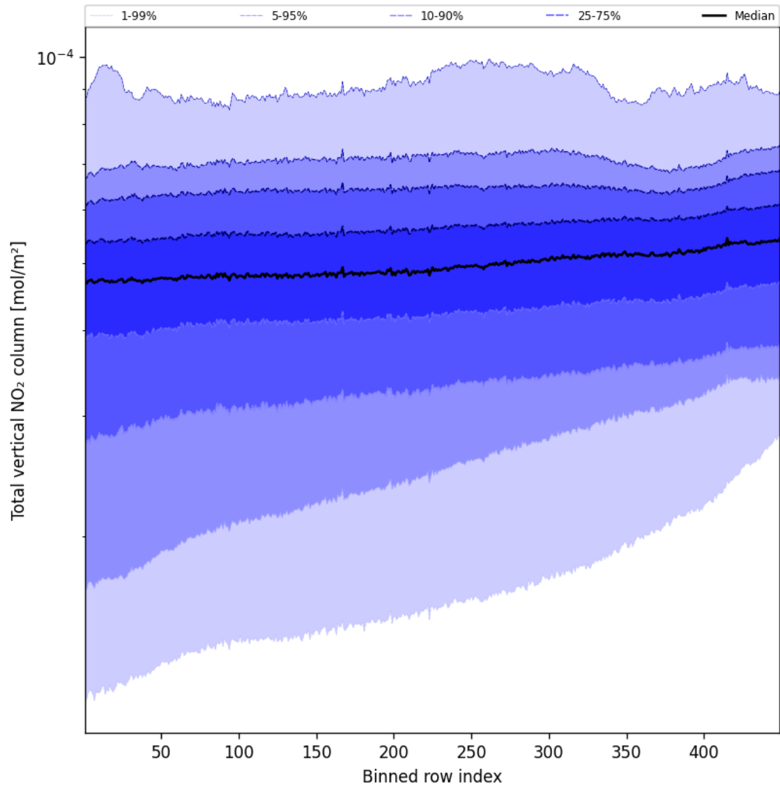
Figure 53: Along track statistics of “Total vertical NO 2 column” for 2025-09-11 to 2025-09-12
