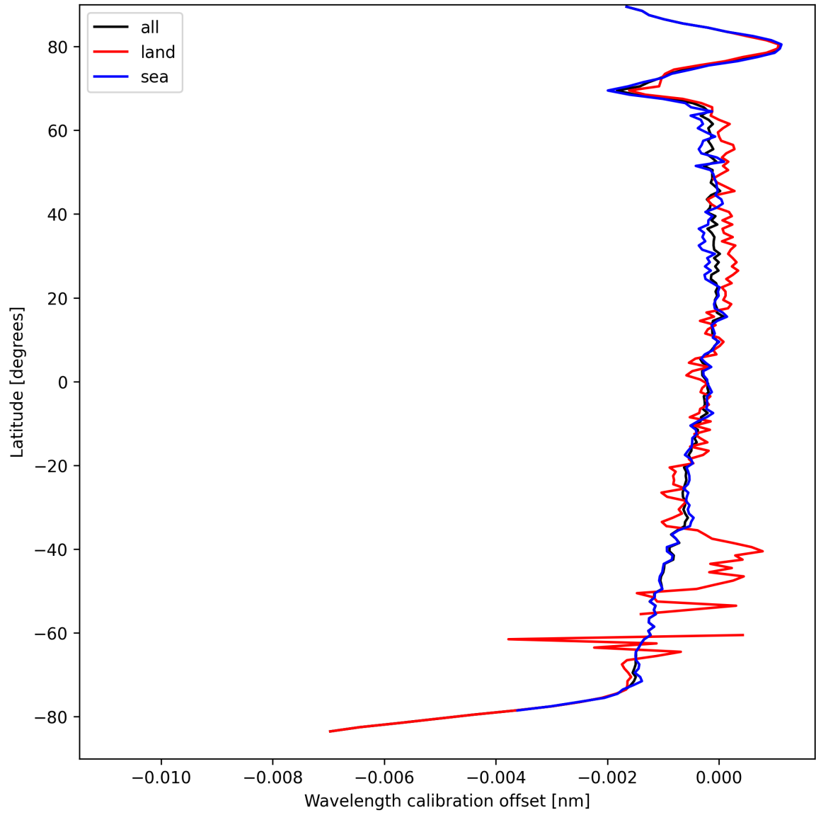
Figure 16: Zonal average of “Wavelength calibration offset” for 2025-09-11 to 2025-09-12.
