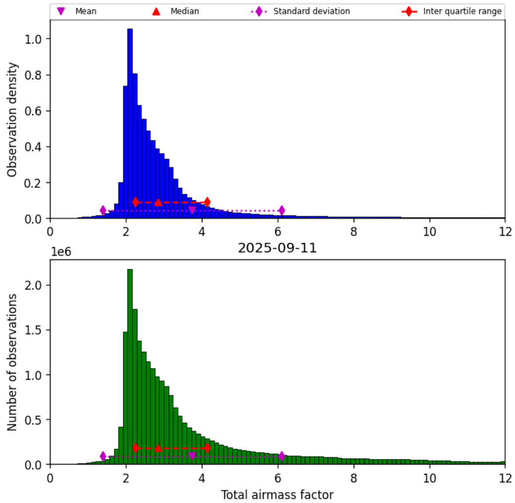
Figure 30: Histogram of “Total airmass factor” for 2025-09-11 to 2025-09-12
