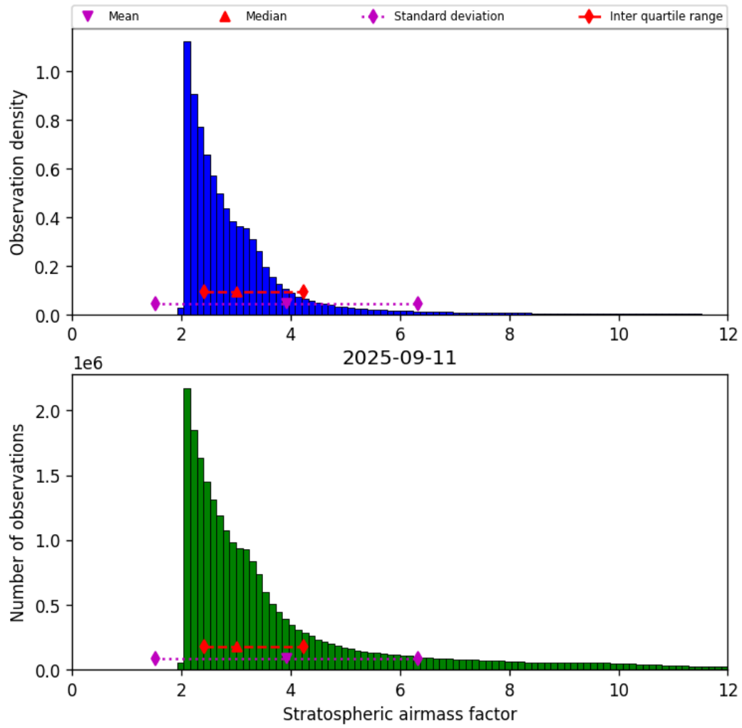
Figure 42: Histogram of “Stratospheric airmass factor” for 2025-09-11 to 2025-09-12
