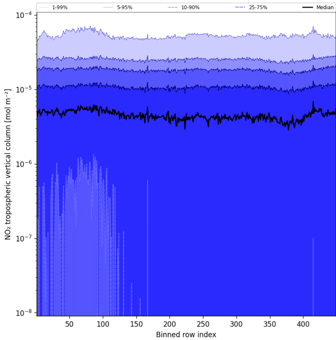
Figure 44: Along track statistics of “NO 2 tropospheric vertical column” for 2025-09-11 to 2025-09-12
