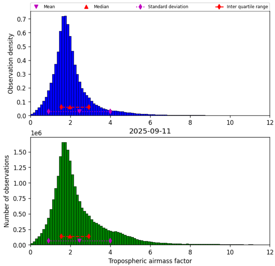
Figure 29: Histogram of “Tropospheric airmass factor” for 2025-09-11 to 2025-09-12
