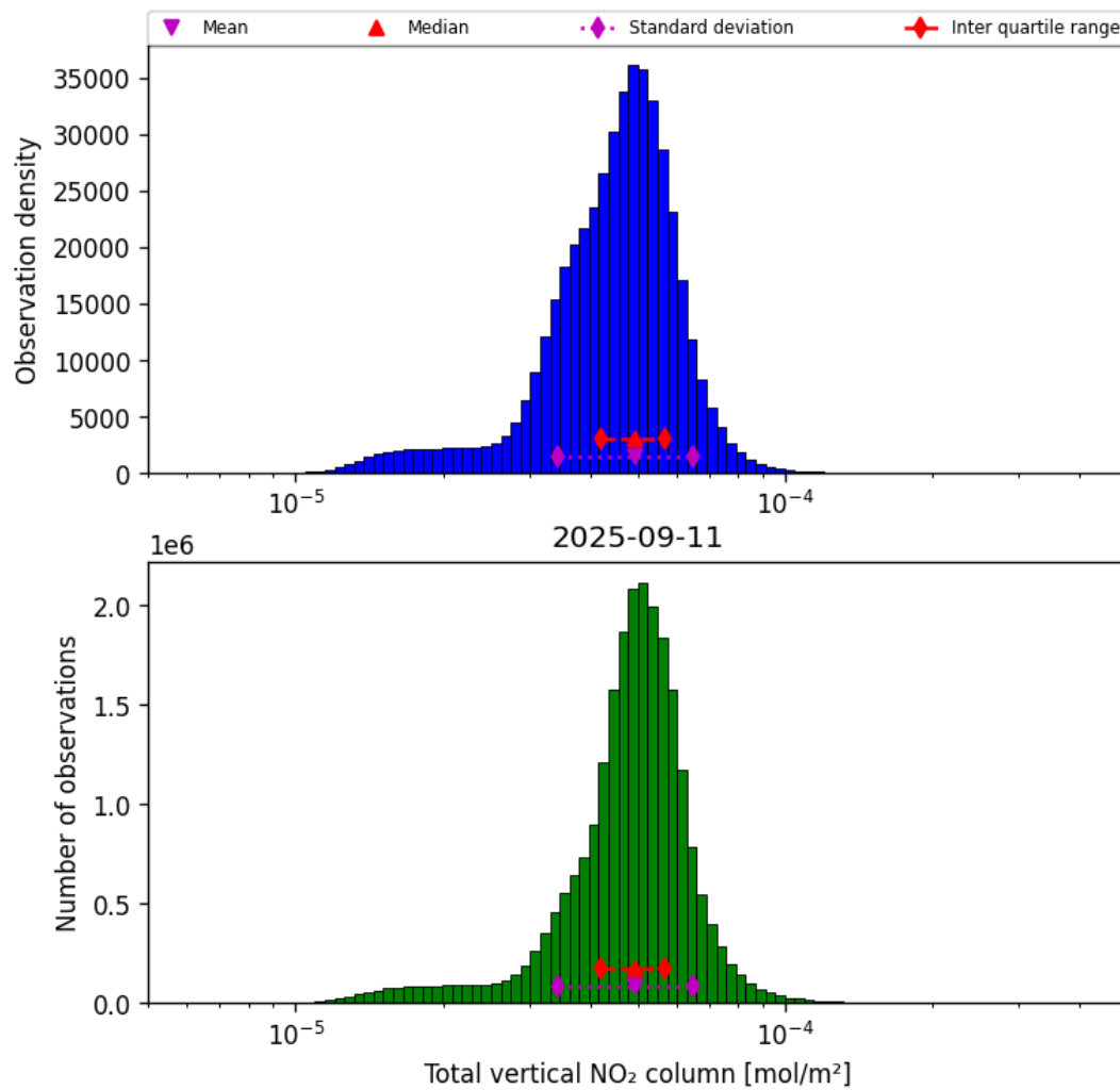
Figure 36: Histogram of “Total vertical NO 2 column” for 2025-09-11 to 2025-09-12
