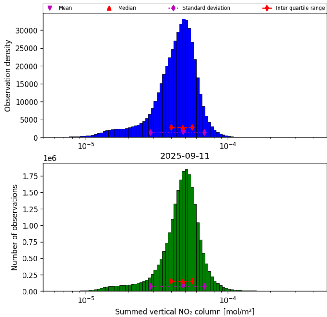
Figure 38: Histogram of “Summed vertical NO 2 column” for 2025-09-11 to 2025-09-12
