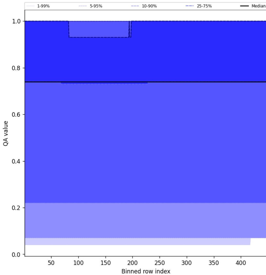
Figure 43: Along track statistics of “QA value” for 2025-09-11 to 2025-09-12
