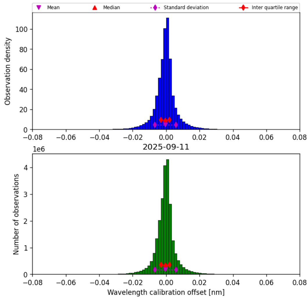
Figure 33: Histogram of “Wavelength calibration offset” for 2025-09-11 to 2025-09-12
