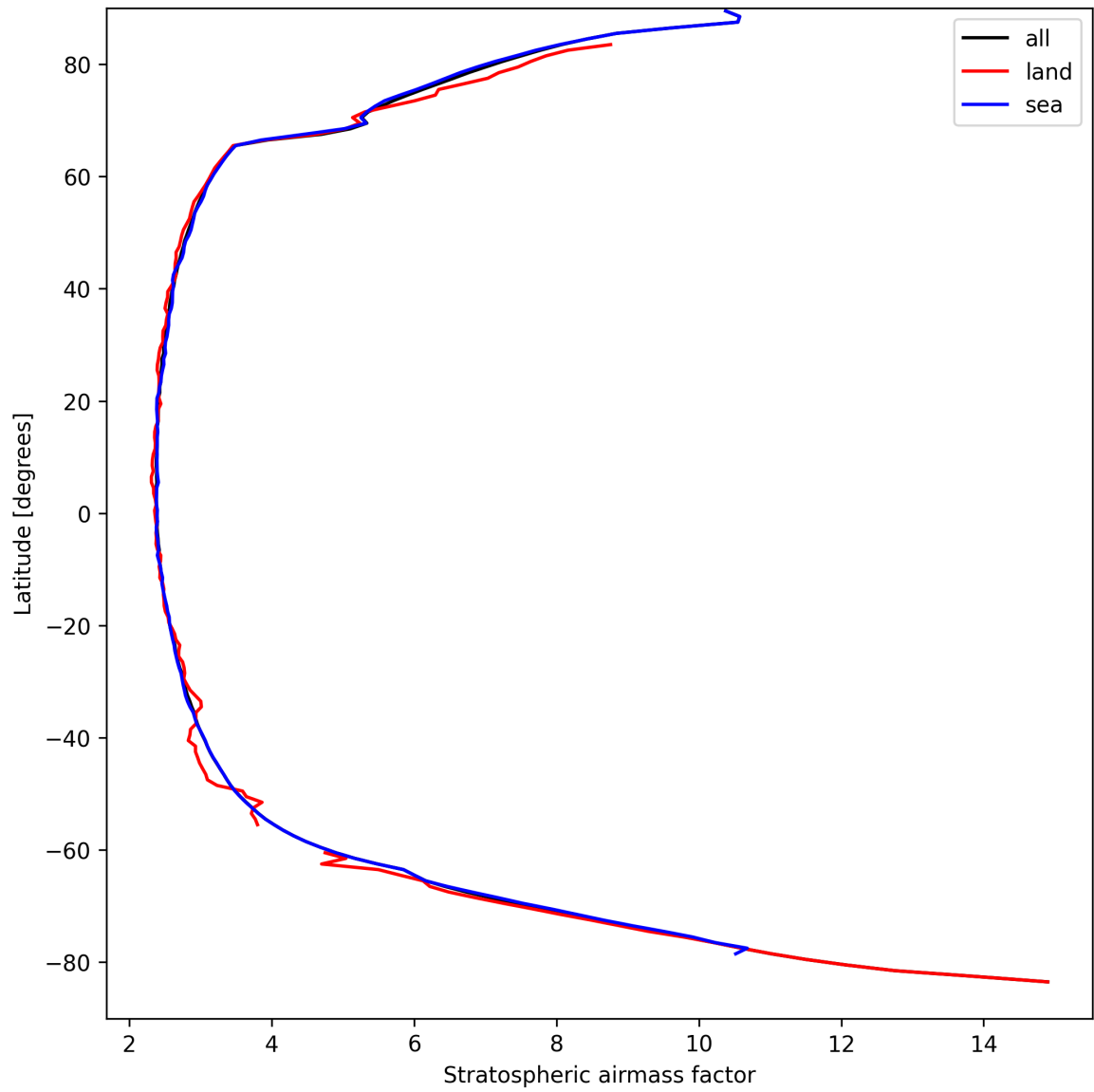
Figure 25: Zonal average of “Stratospheric air mass factor” for 2025-09-11 to 2025-09-12.
