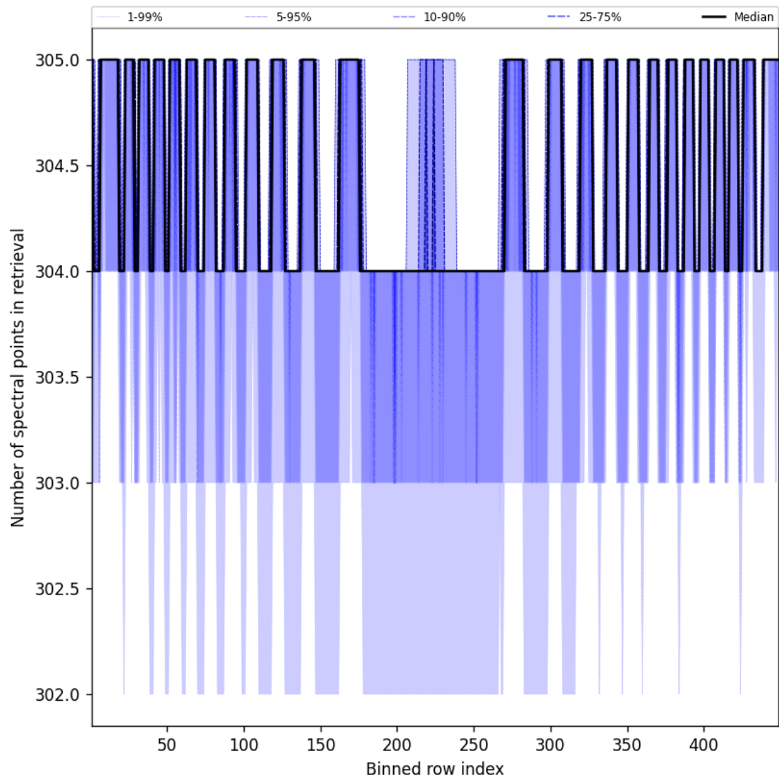
Figure 48: Along track statistics of “Number of spectral points in retrieval” for 2025-09-11 to 2025-09-12
