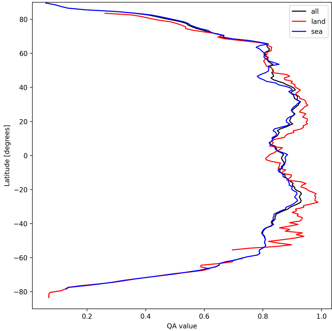
Figure 9: Zonal average of “QA value” for 2025-09-11 to 2025-09-12.
