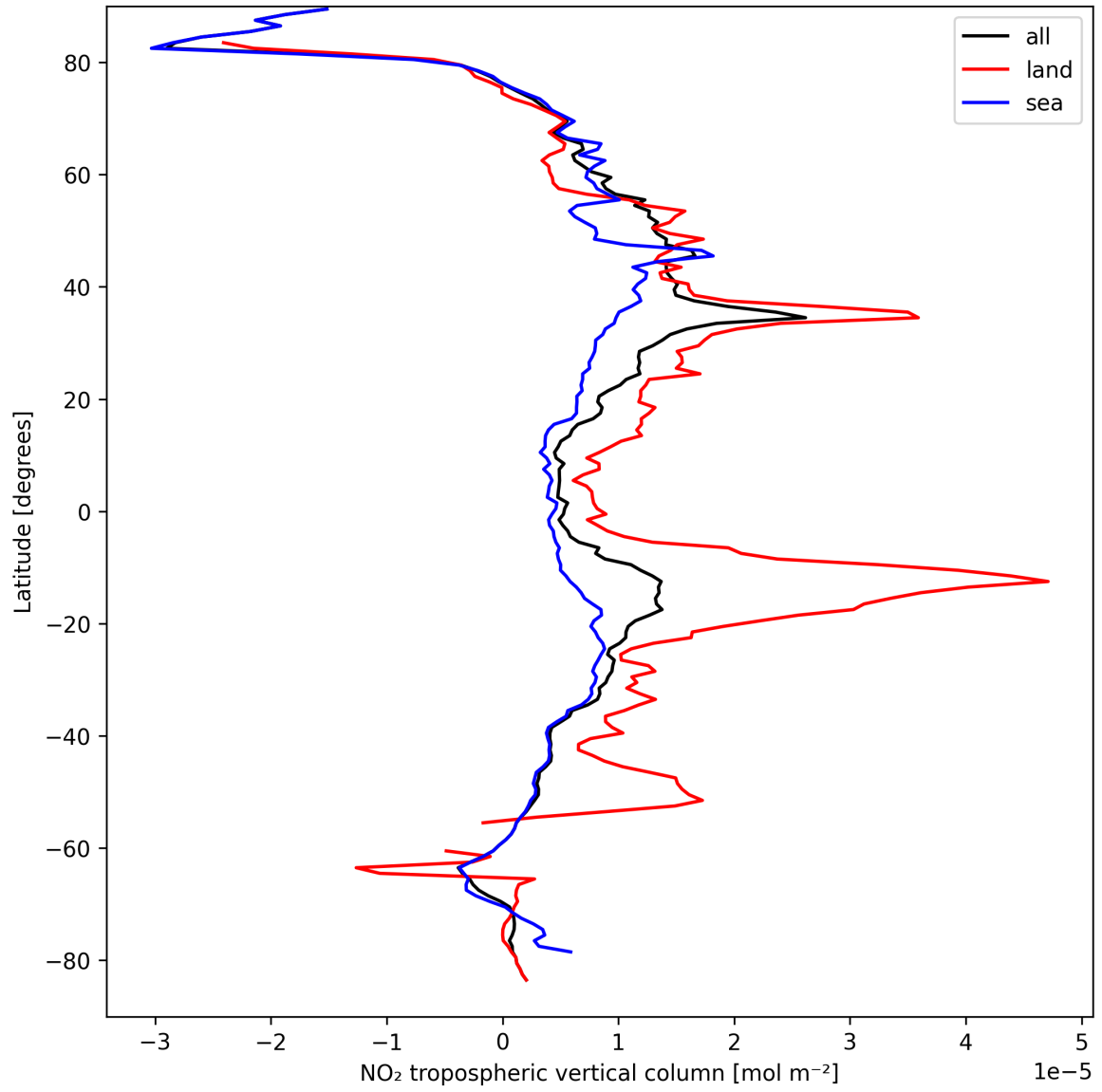
Figure 10: Zonal average of “NO 2 tropospheric vertical column” for 2025-09-11 to 2025-09-12.
