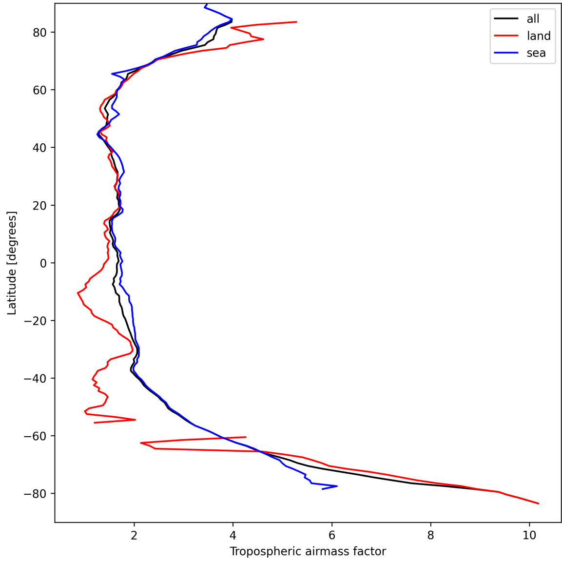
Figure 12: Zonal average of “Tropospheric airmass factor” for 2025-09-11 to 2025-09-12.
