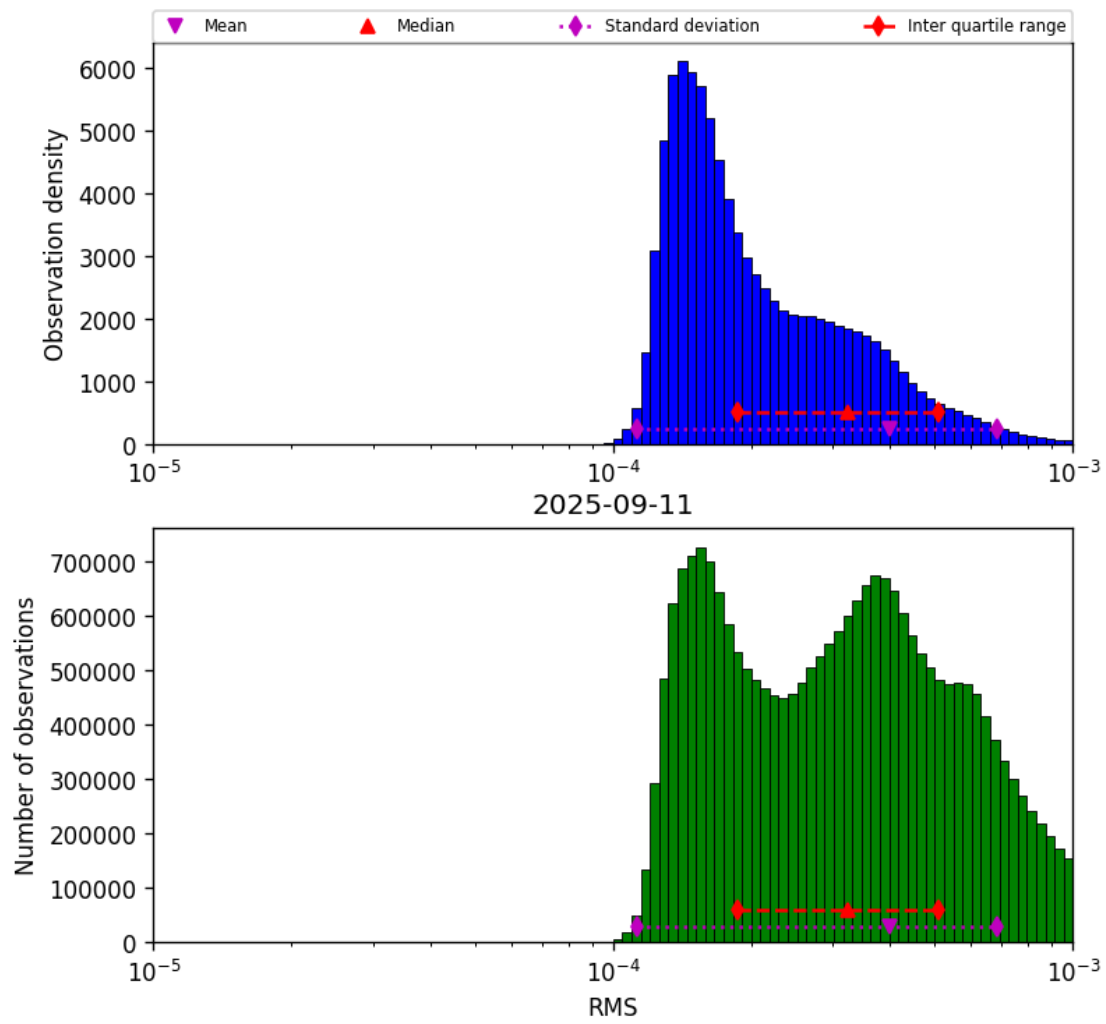
Figure 41: Histogram of “RMS” for 2025-09-11 to 2025-09-12
