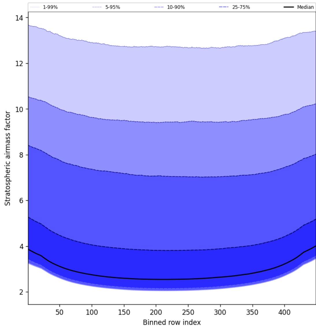
Figure 59: Along track statistics of “Stratospheric air mass factor” for 2025-09-11 to 2025-09-12
