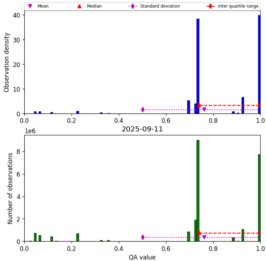
Figure 26: Histogram of “QA value” for 2025-09-11 to 2025-09-12
