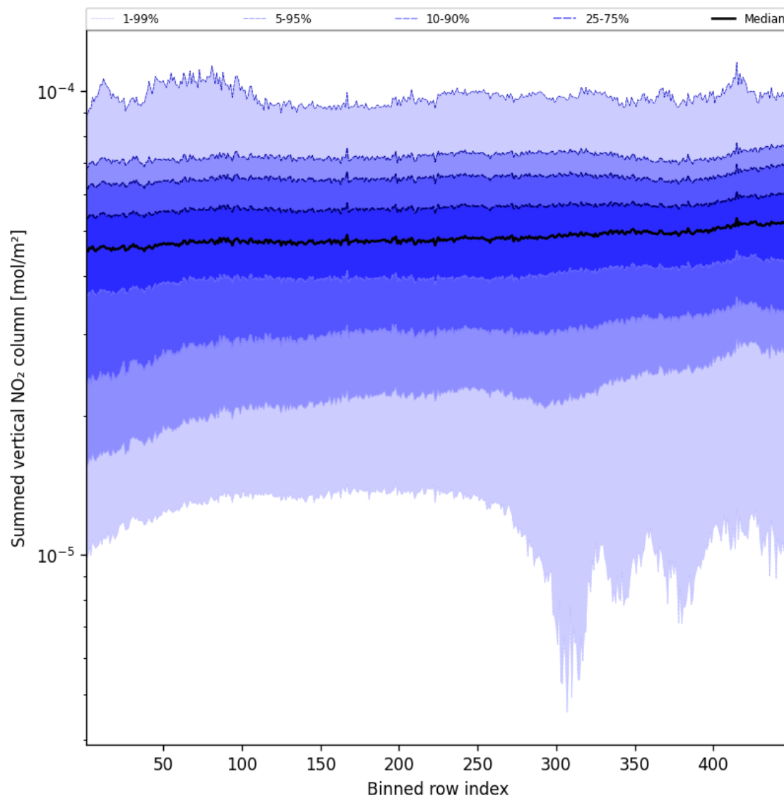
Figure 55: Along track statistics of “Summed vertical NO 2 column” for 2025-09-11 to 2025-09-12
