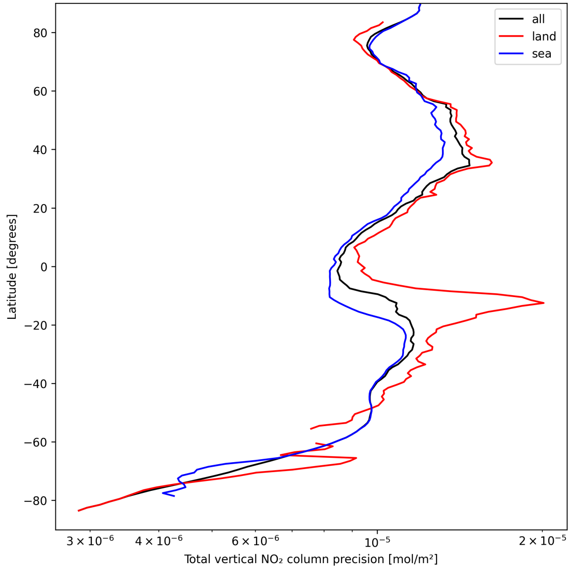
Figure 20: Zonal average of “Total vertical NO 2 column precision” for 2025-09-11 to 2025-09-12.
