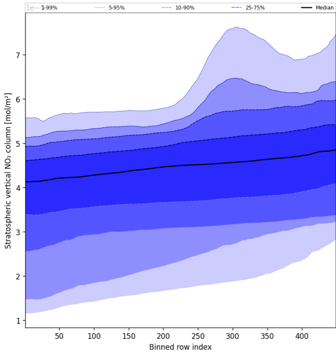
Figure 51: Along track statistics of “Stratospheric vertical NO 2 column” for 2025-09-11 to 2025-09-12
