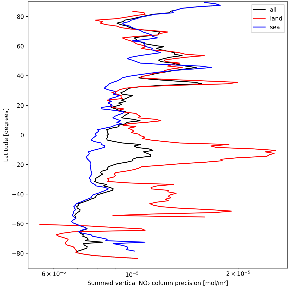
Figure 22: Zonal average of “Summed vertical NO 2 column precision” for 2025-09-11 to 2025-09-12.
