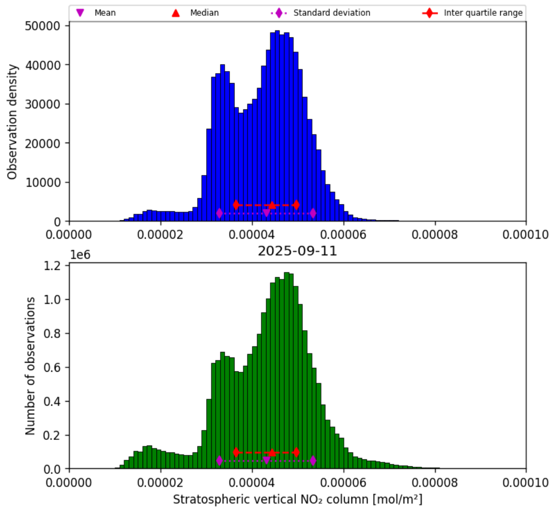
Figure 34: Histogram of “Stratospheric vertical NO 2 column” for 2025-09-11 to 2025-09-12
