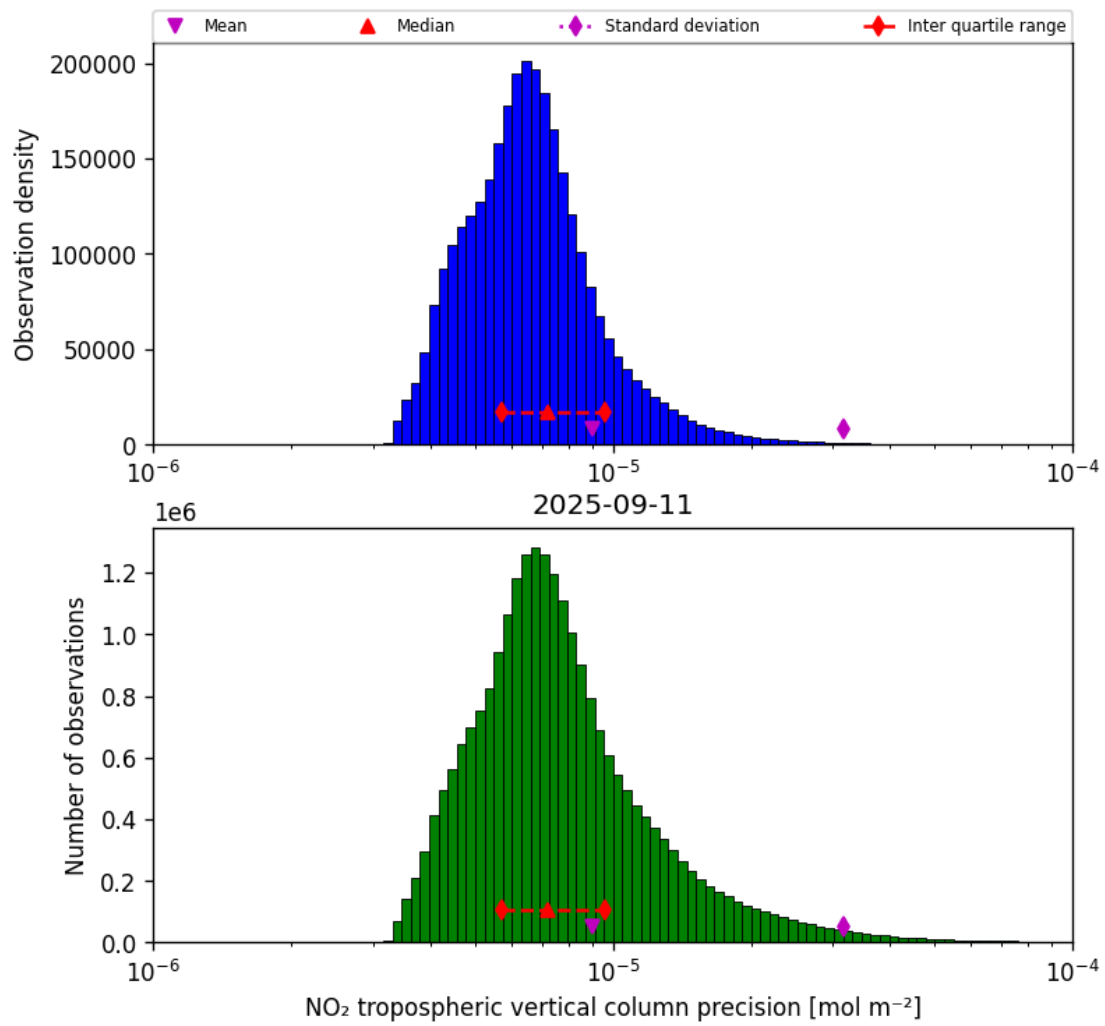
Figure 28: Histogram of “NO 2 tropospheric vertical column precision” for 2025-09-11 to 2025-09-12
