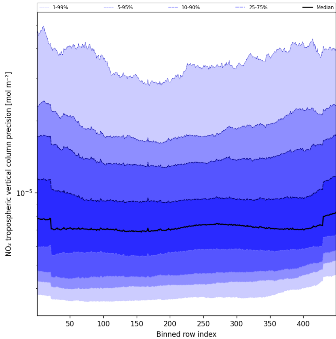
Figure 45: Along track statistics of “NO 2 tropospheric vertical column precision” for 2025-09-11 to 2025-09-12
