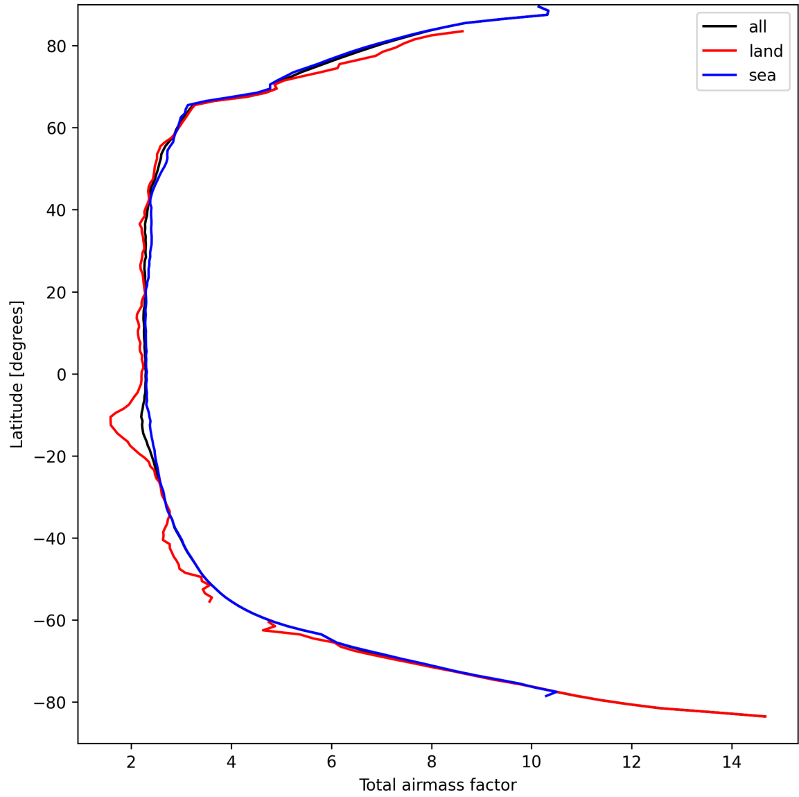
Figure 13: Zonal average of “Total airmass factor” for 2025-09-11 to 2025-09-12.
