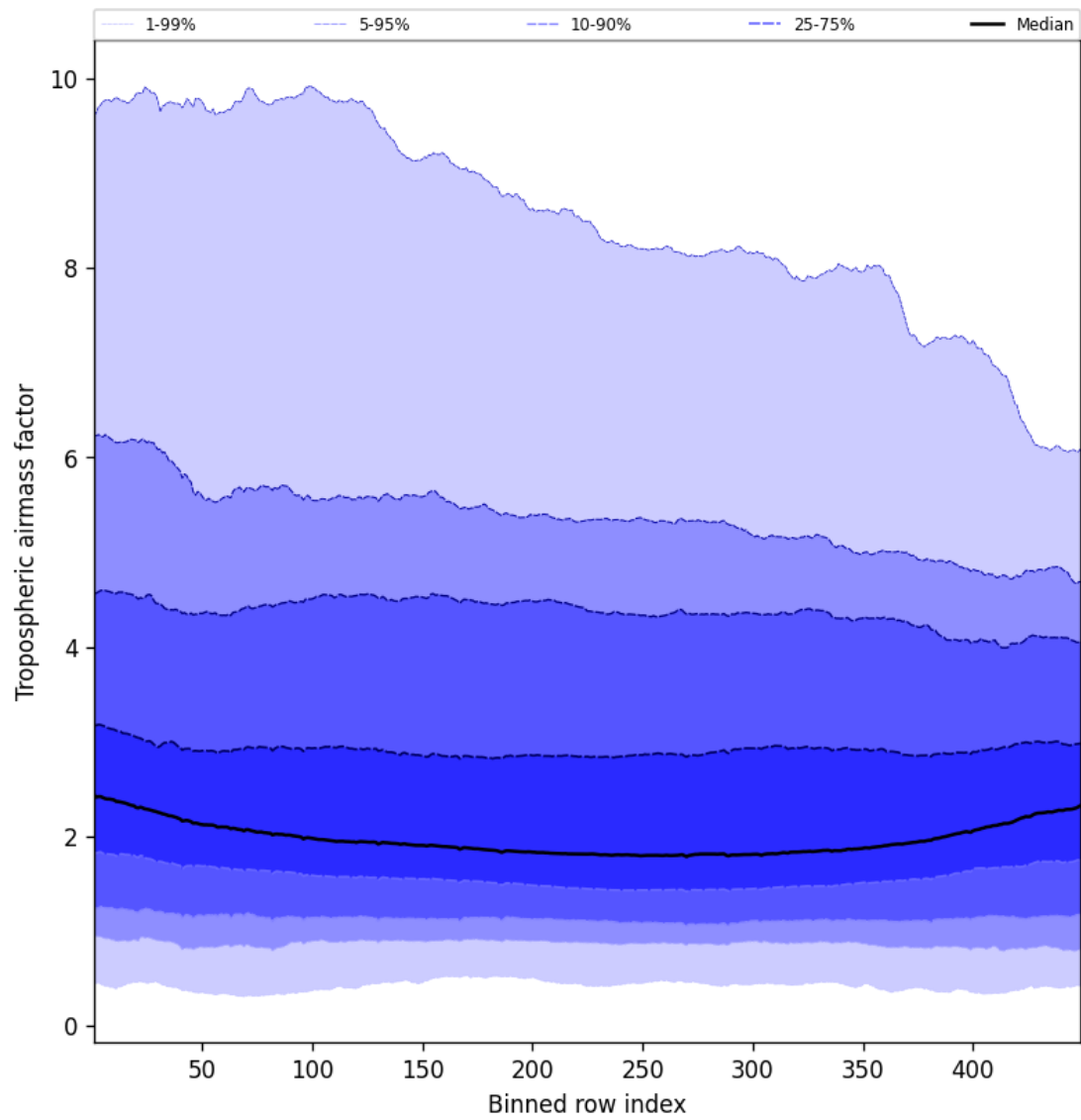
Figure 46: Along track statistics of “Tropospheric airmass factor” for 2025-09-11 to 2025-09-12
