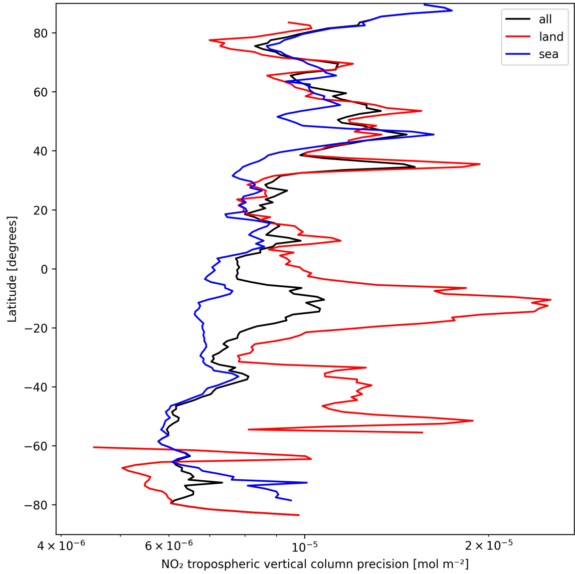
Figure 11: Zonal average of “NO 2 tropospheric vertical column precision” for 2025-09-11 to 2025-09-12.
