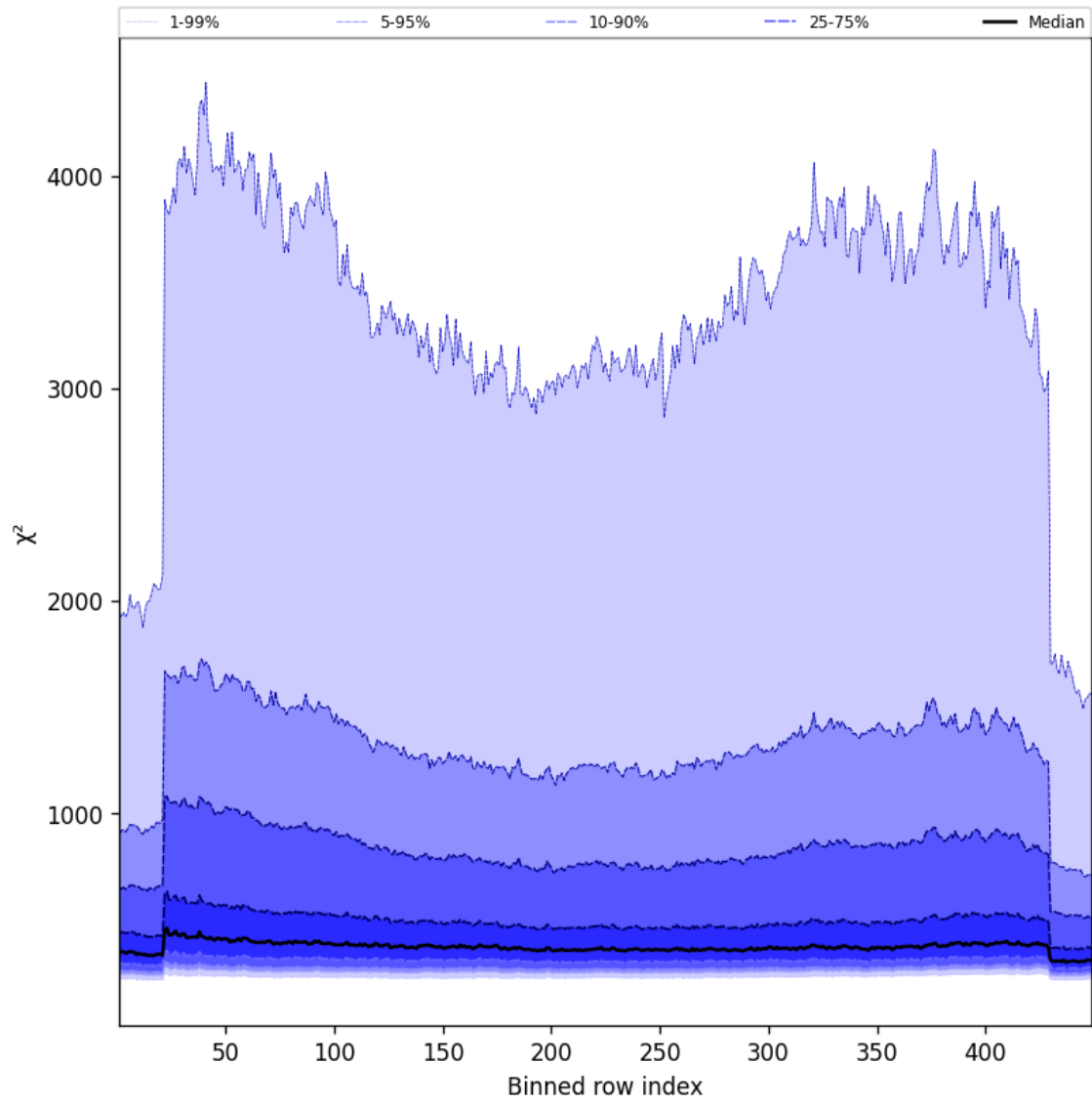
Figure 57: Along track statistics of “ \chi^2 ” for 2025-09-11 to 2025-09-12
