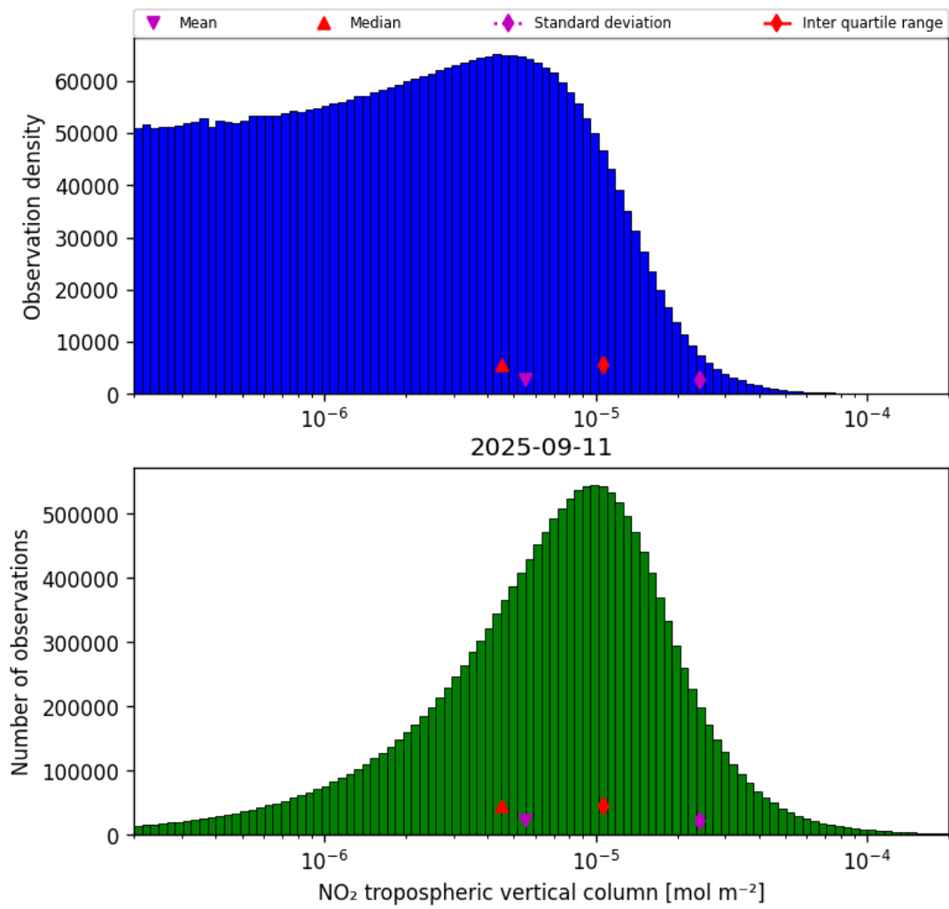
Figure 27: Histogram of “NO 2 tropospheric vertical column” for 2025-09-11 to 2025-09-12
