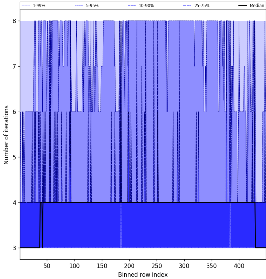
Figure 49: Along track statistics of “Number of iterations” for 2025-09-11 to 2025-09-12
