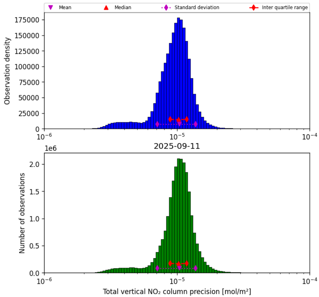
Figure 37: Histogram of “Total vertical NO 2 column precision” for 2025-09-11 to 2025-09-12
