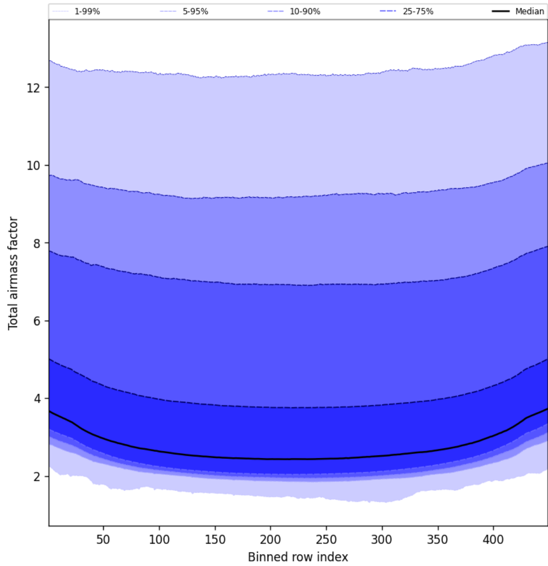
Figure 47: Along track statistics of “Total airmass factor” for 2025-09-11 to 2025-09-12
