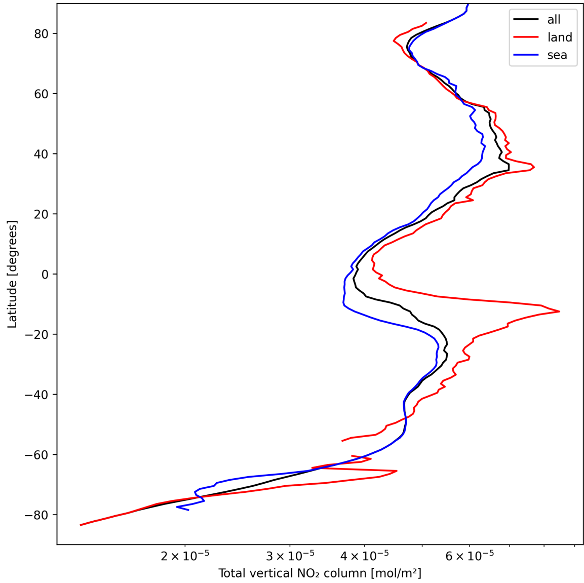
Figure 19: Zonal average of “Total vertical NO 2 column” for 2025-09-11 to 2025-09-12.
