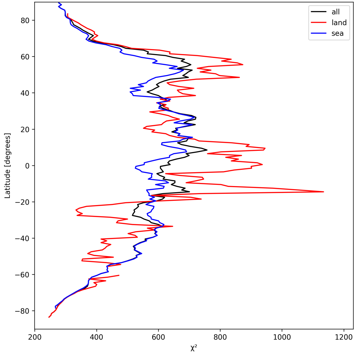
Figure 23: Zonal average of “ \chi^2 ” for 2025-09-11 to 2025-09-12.
