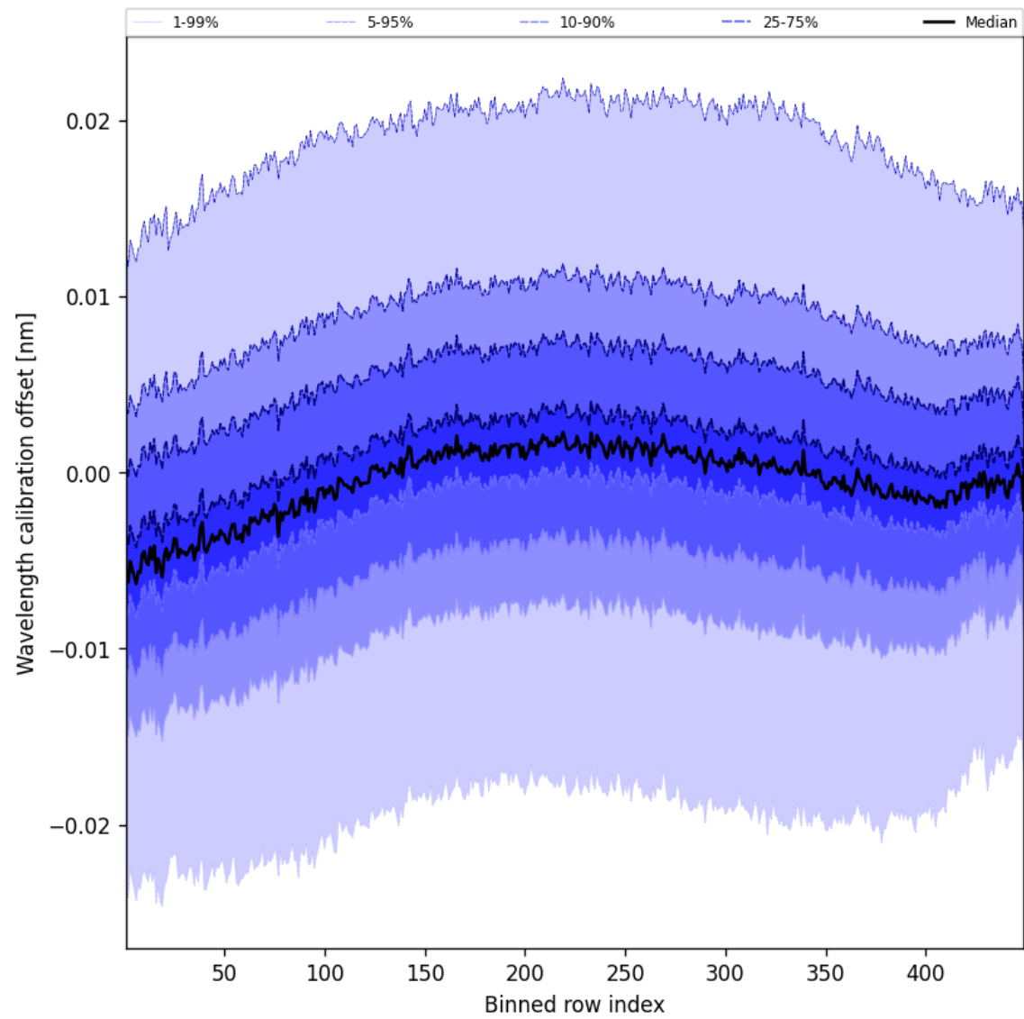
Figure 50: Along track statistics of “Wavelength calibration offset” for 2025-09-11 to 2025-09-12
