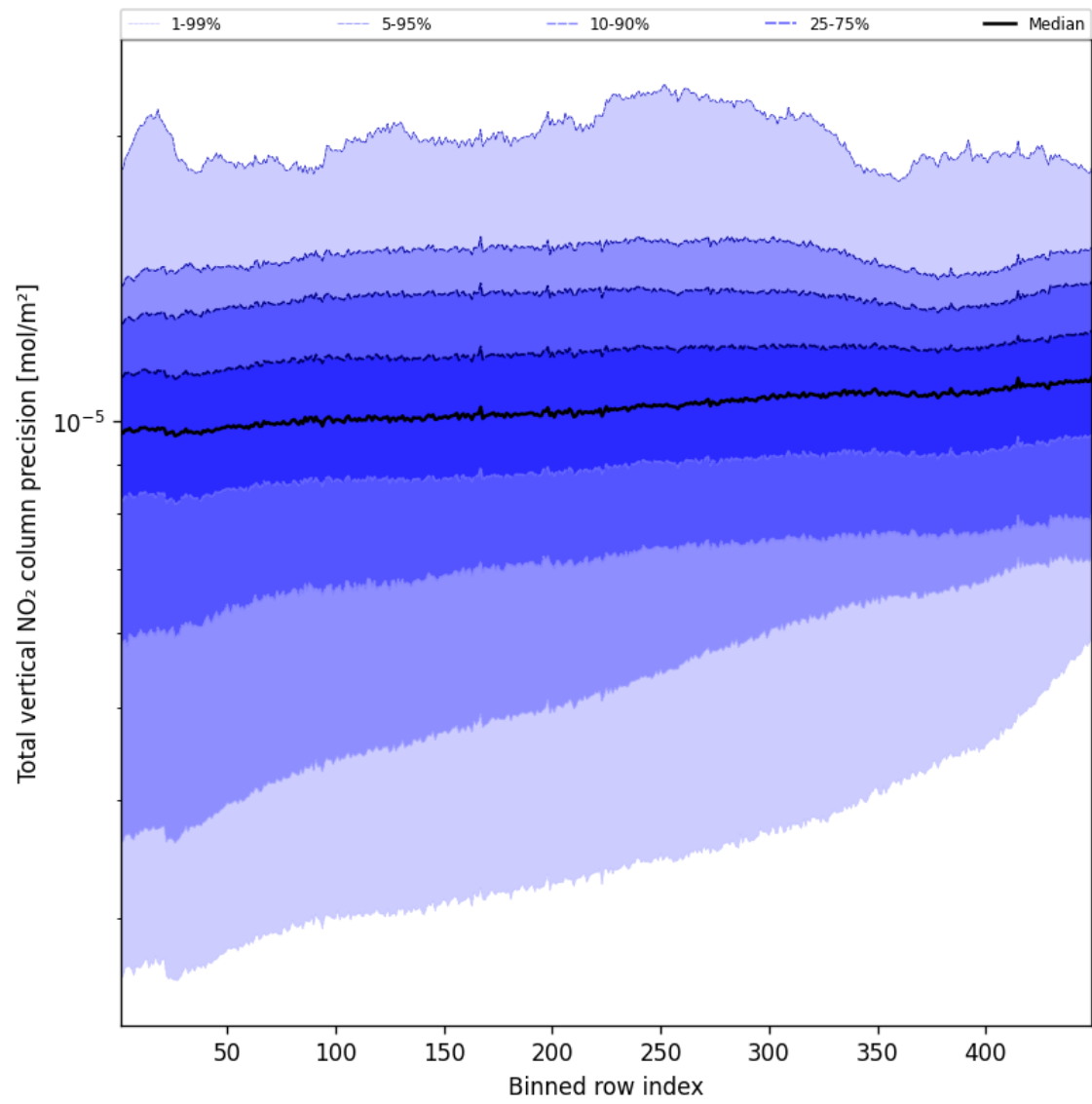
Figure 54: Along track statistics of “Total vertical NO 2 column precision” for 2025-09-11 to 2025-09-12
