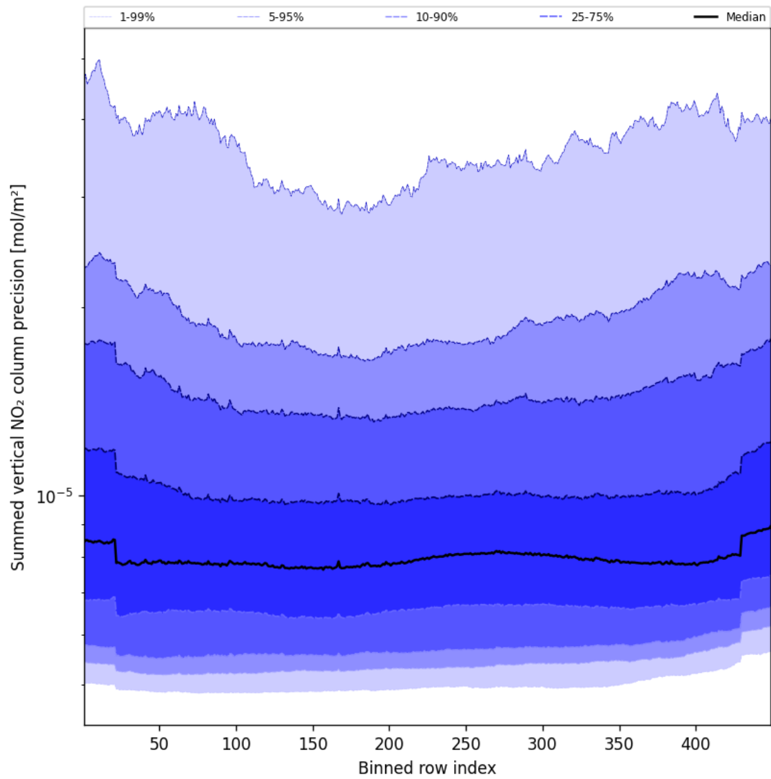
Figure 56: Along track statistics of “Summed vertical NO 2 column precision” for 2025-09-11 to 2025-09-12
