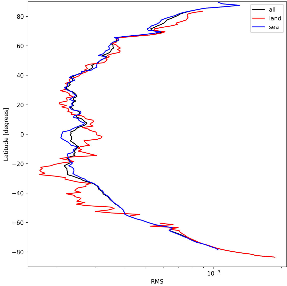
Figure 24: Zonal average of “RMS” for 2025-09-11 to 2025-09-12.
