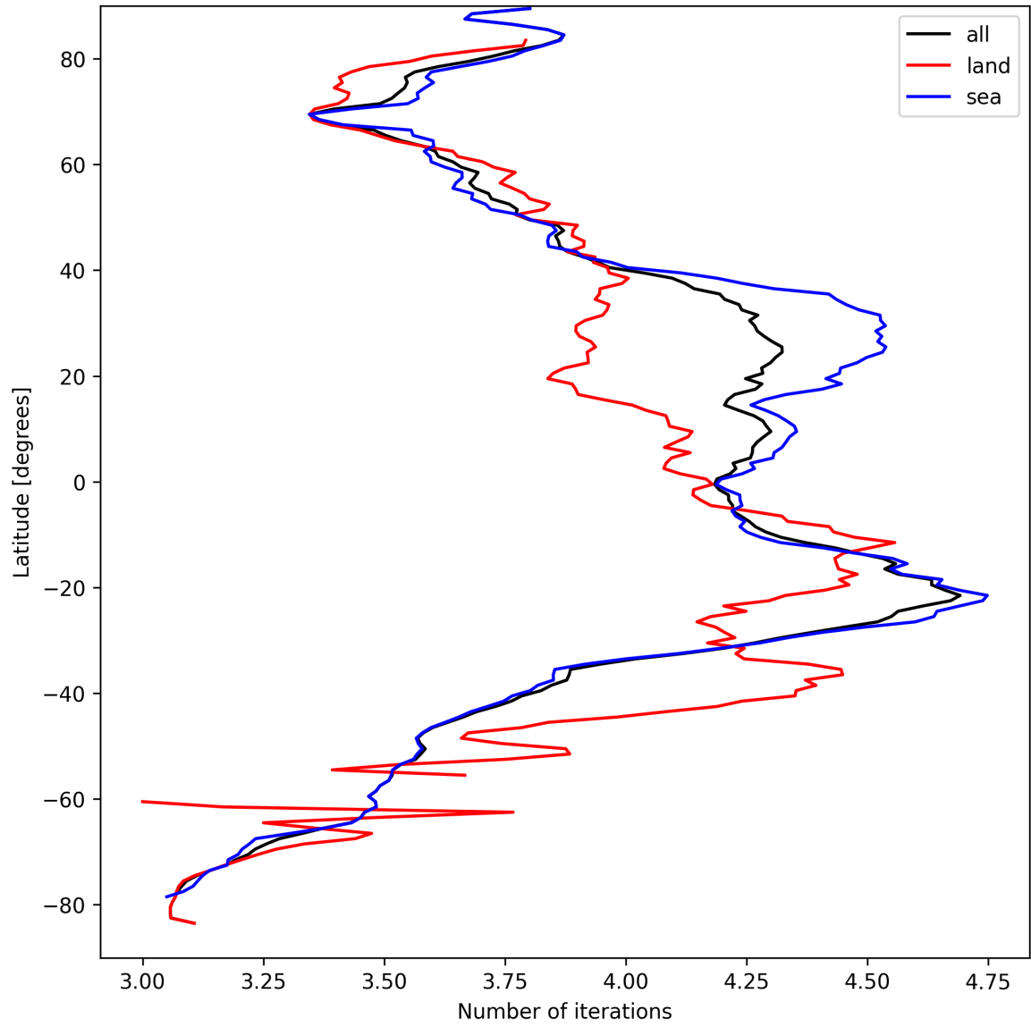
Figure 15: Zonal average of “Number of iterations” for 2025-09-11 to 2025-09-12.
