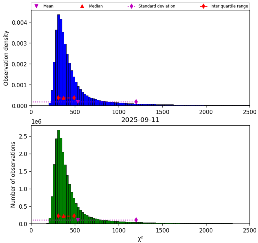
Figure 40: Histogram of “ \chi^2 ” for 2025-09-11 to 2025-09-12
