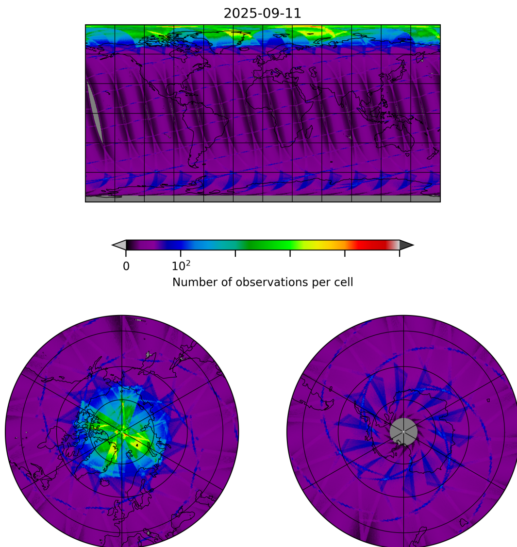
Figure 8: Map of the number of observations for 2025-09-11 to 2025-09-12
