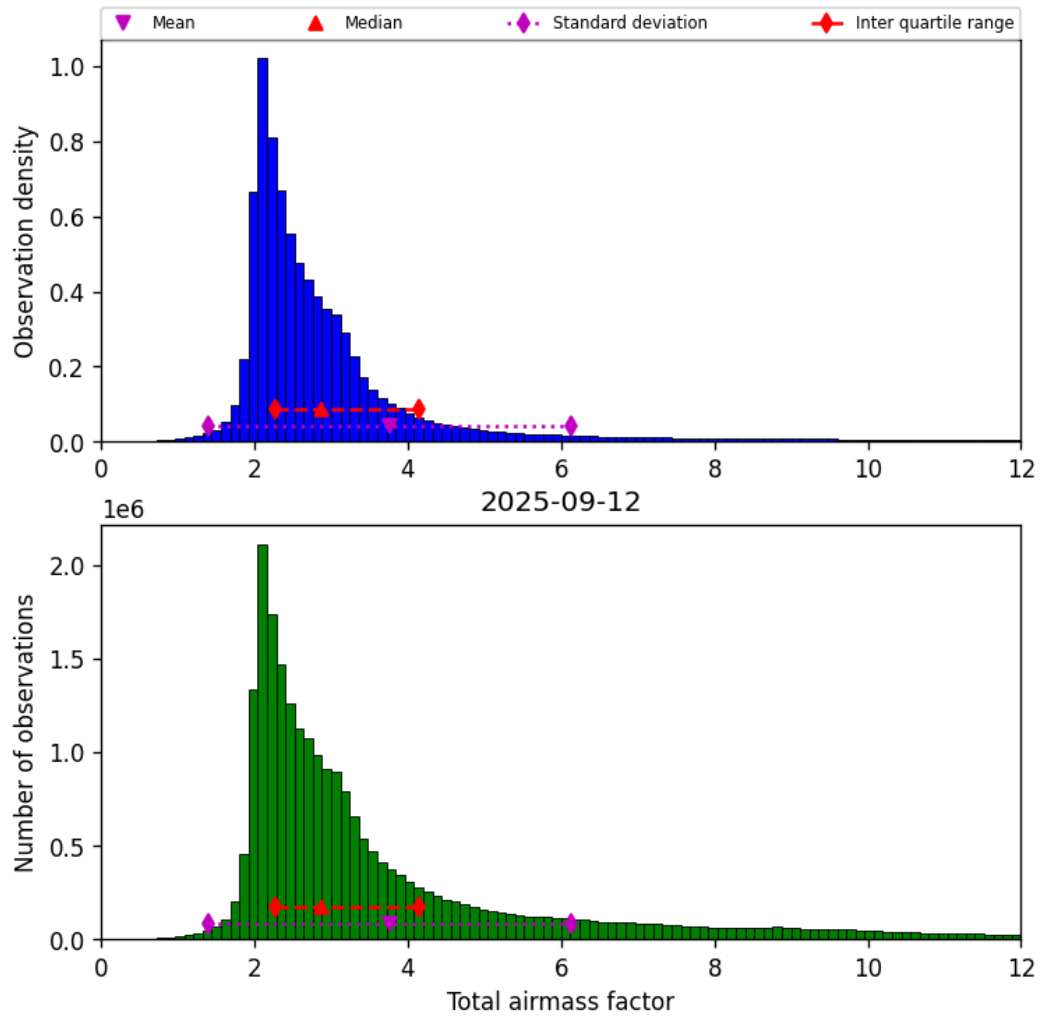
Figure 30: Histogram of “Total airmass factor” for 2025-09-12 to 2025-09-13
