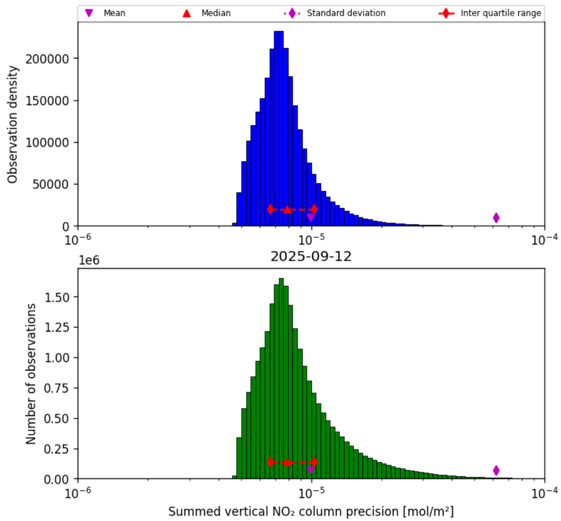
Figure 39: Histogram of “Summed vertical NO 2 column precision” for 2025-09-12 to 2025-09-13
