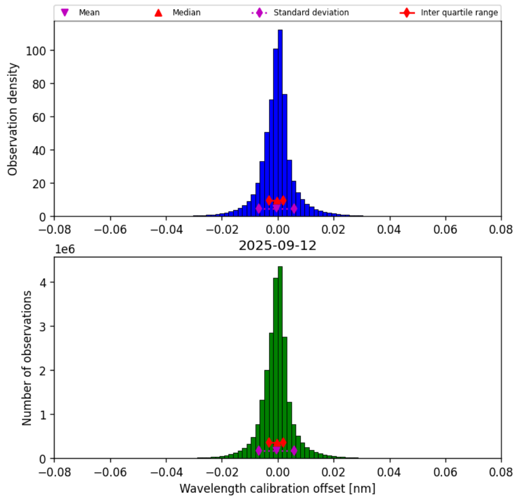
Figure 33: Histogram of “Wavelength calibration offset” for 2025-09-12 to 2025-09-13
