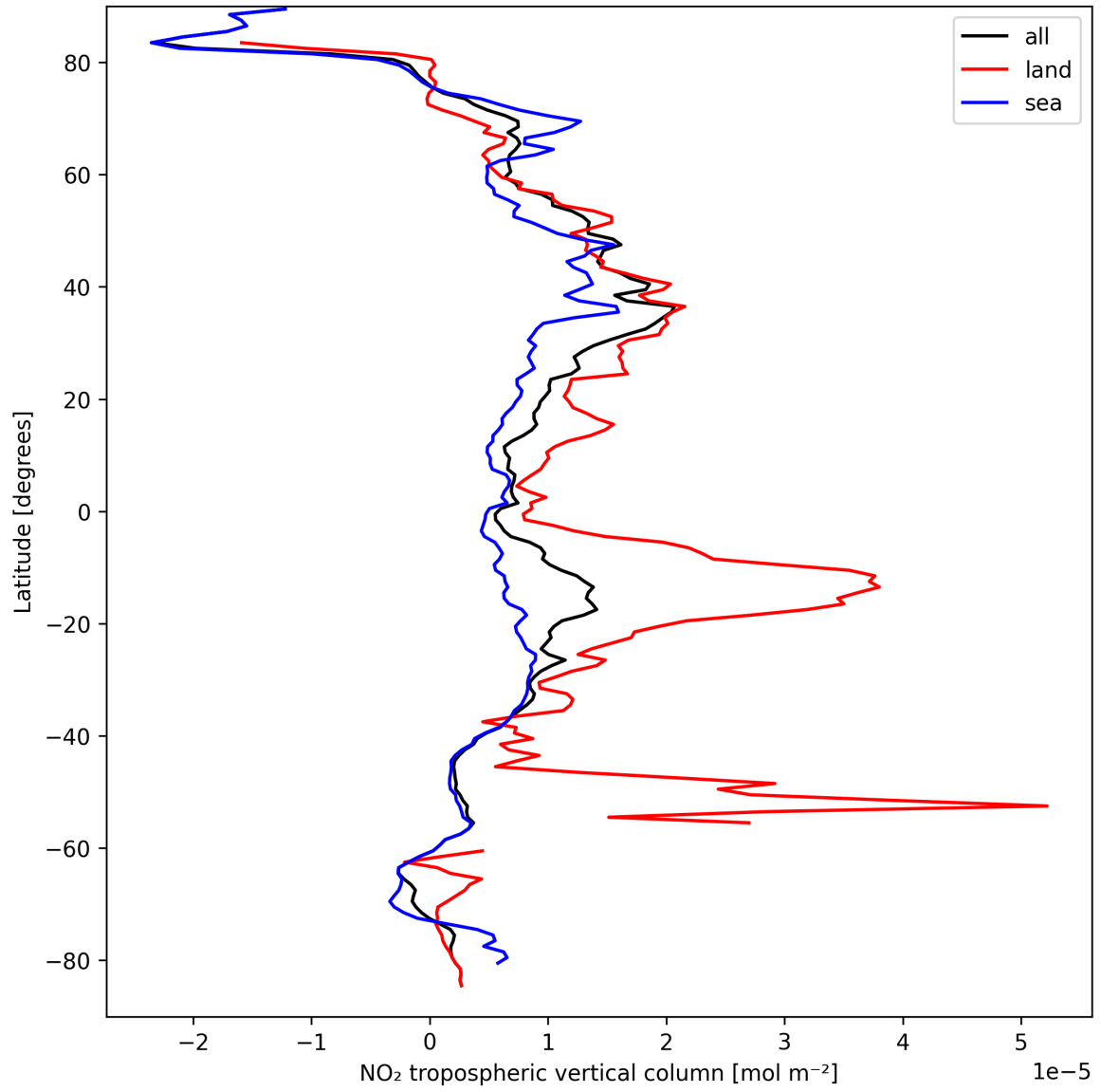
Figure 10: Zonal average of “NO 2 tropospheric vertical column” for 2025-09-12 to 2025-09-13.
