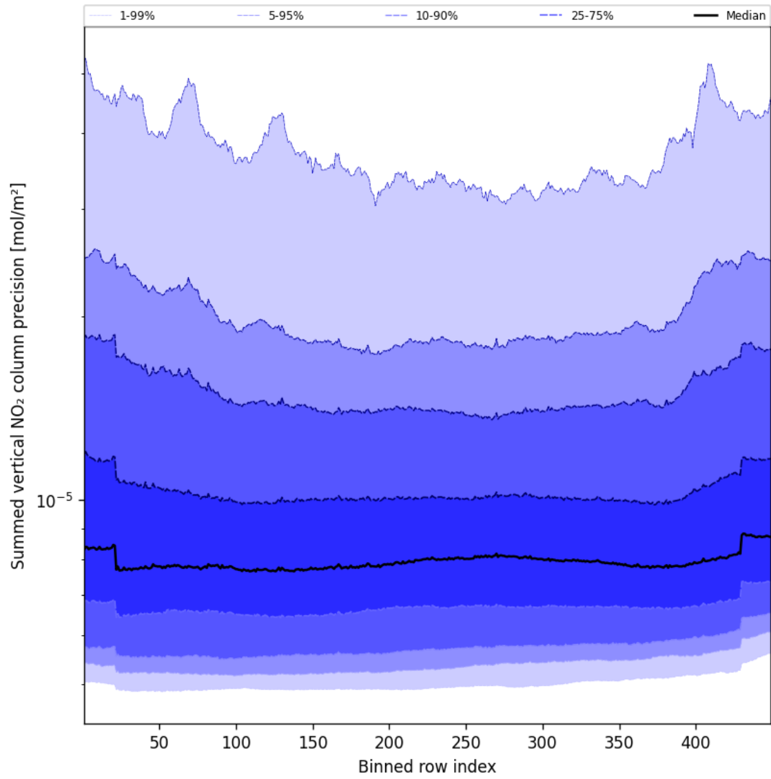
Figure 56: Along track statistics of “Summed vertical NO 2 column precision” for 2025-09-12 to 2025-09-13
