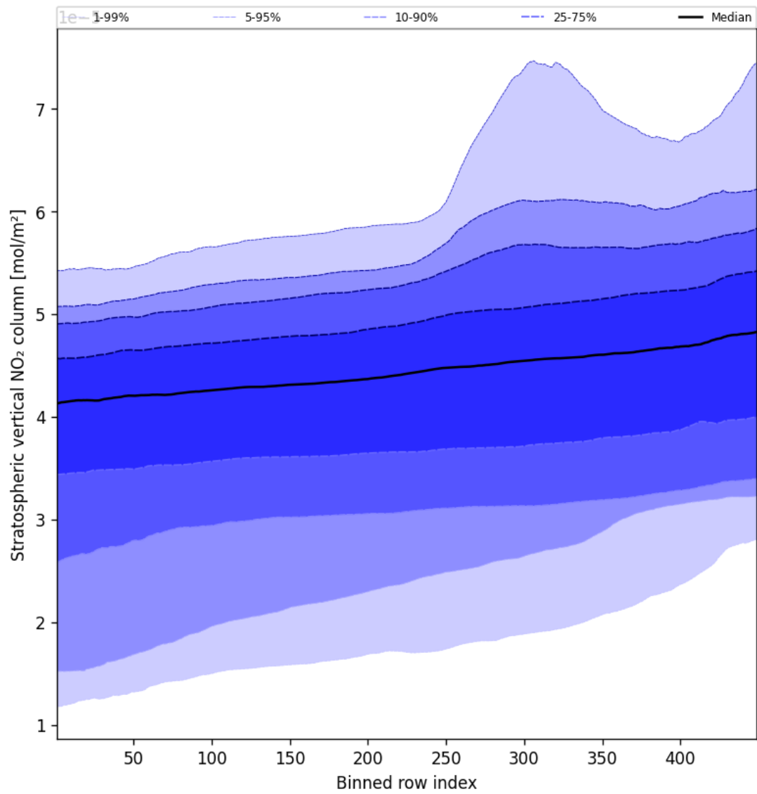
Figure 51: Along track statistics of “Stratospheric vertical NO 2 column” for 2025-09-12 to 2025-09-13
