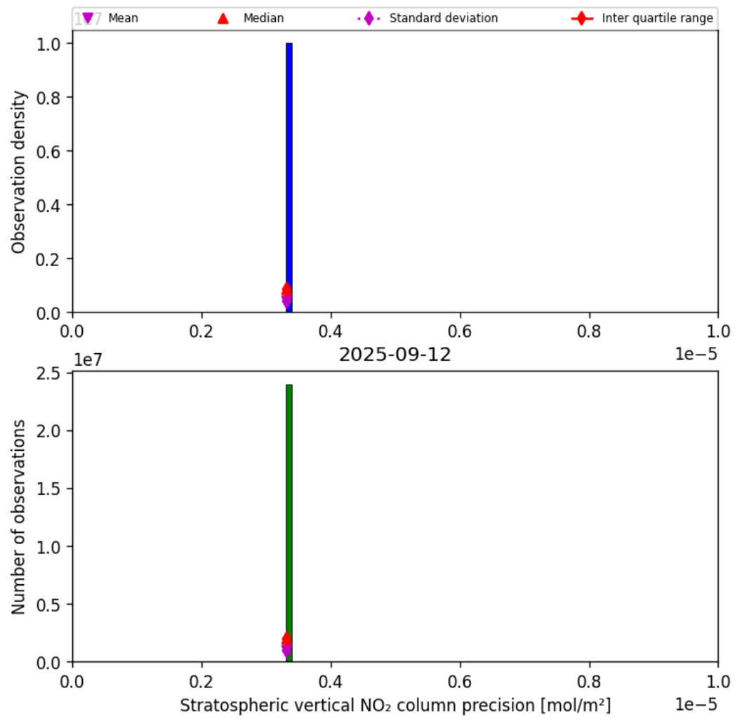
Figure 35: Histogram of “Stratospheric vertical NO 2 column precision” for 2025-09-12 to 2025-09-13
