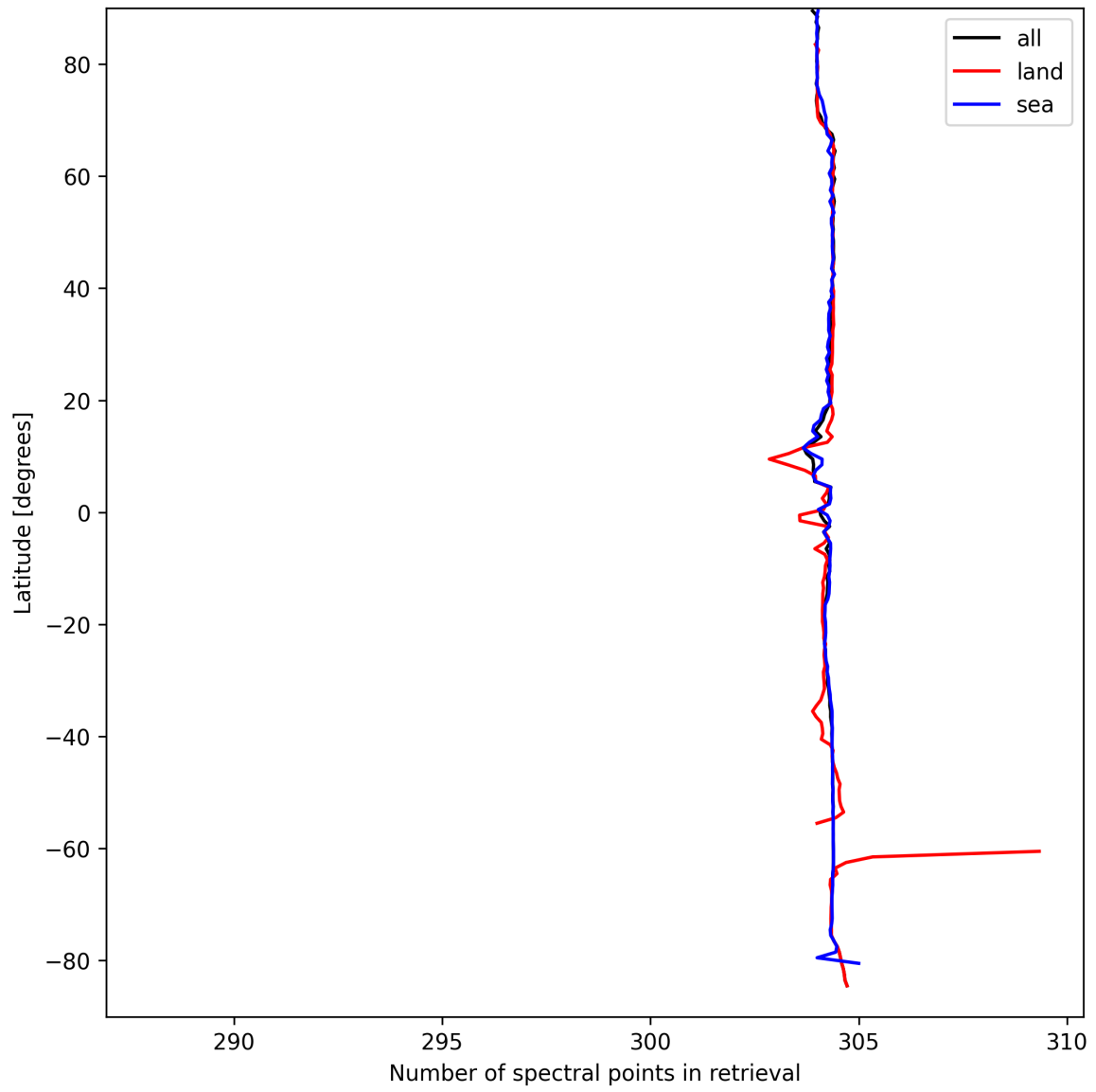
Figure 14: Zonal average of “Number of spectral points in retrieval” for 2025-09-12 to 2025-09-13.
