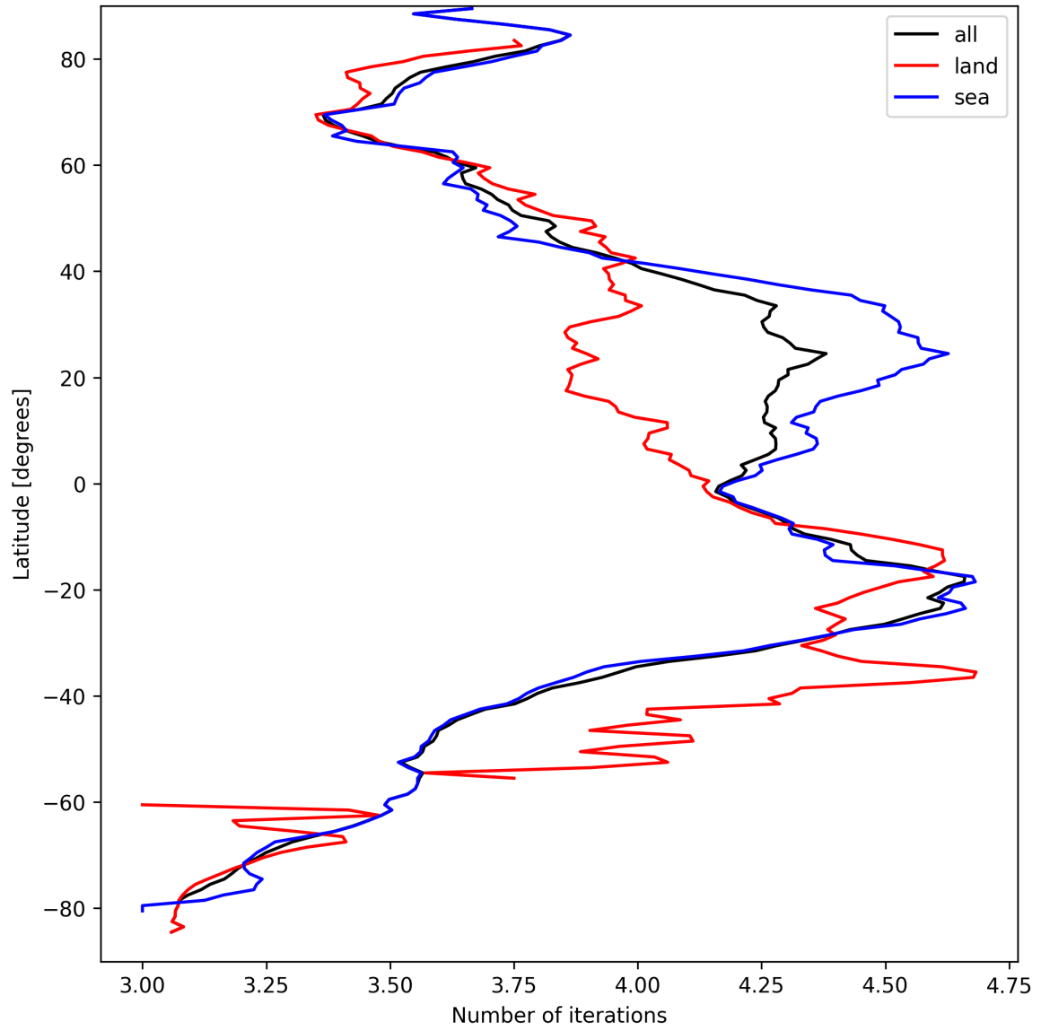
Figure 15: Zonal average of “Number of iterations” for 2025-09-12 to 2025-09-13.
