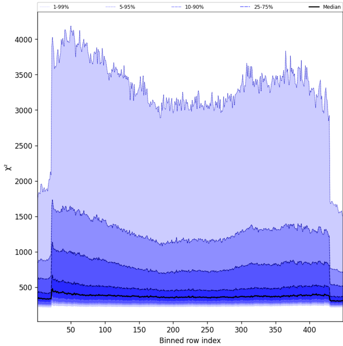
Figure 57: Along track statistics of “ \chi^2 ” for 2025-09-12 to 2025-09-13
