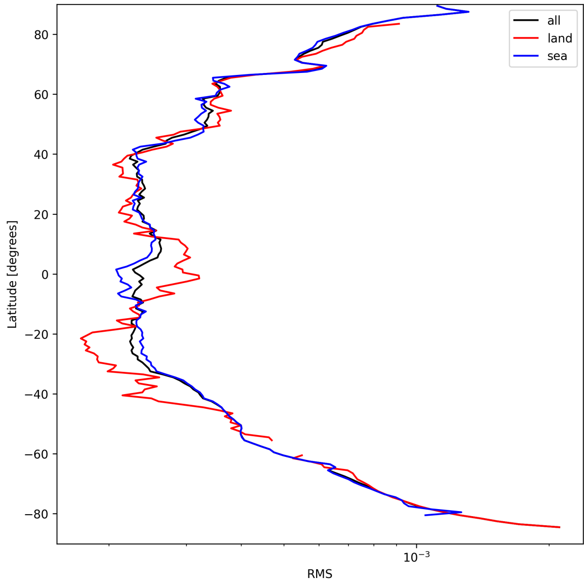
Figure 24: Zonal average of “RMS” for 2025-09-12 to 2025-09-13.
