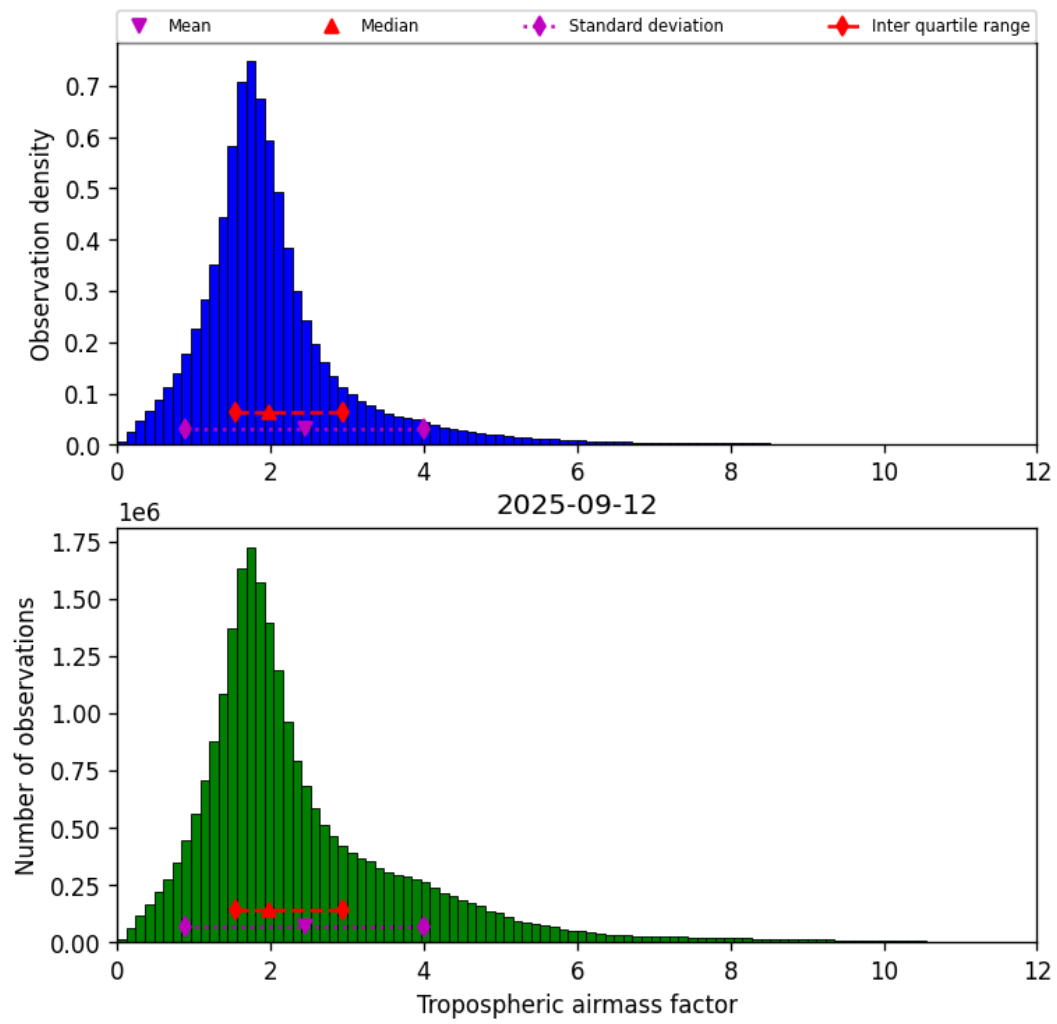
Figure 29: Histogram of “Tropospheric airmass factor” for 2025-09-12 to 2025-09-13
