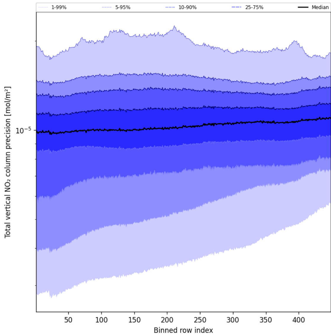
Figure 54: Along track statistics of “Total vertical NO 2 column precision” for 2025-09-12 to 2025-09-13
