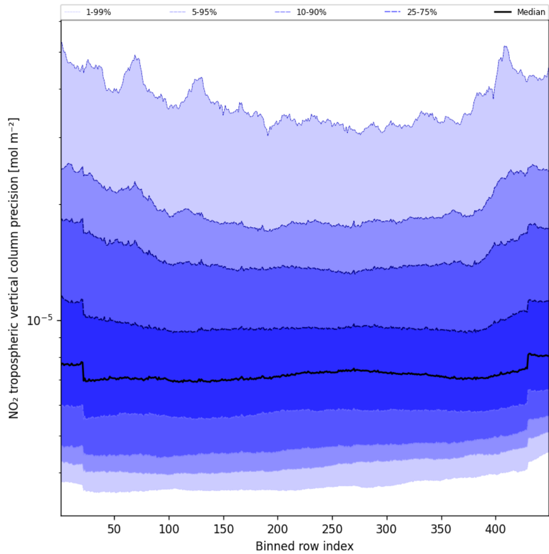
Figure 45: Along track statistics of “NO 2 tropospheric vertical column precision” for 2025-09-12 to 2025-09-13
