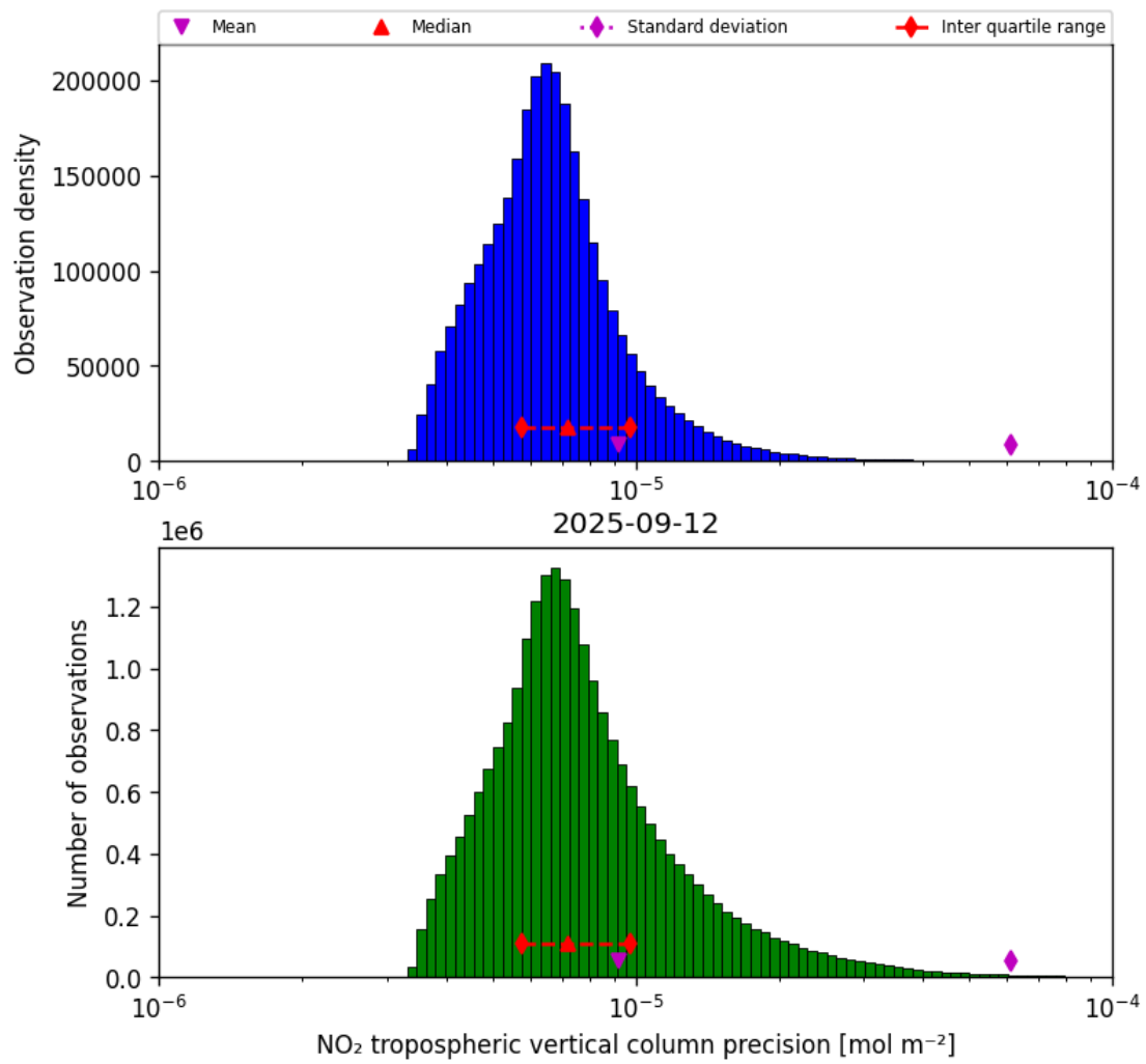
Figure 28: Histogram of “NO 2 tropospheric vertical column precision” for 2025-09-12 to 2025-09-13
