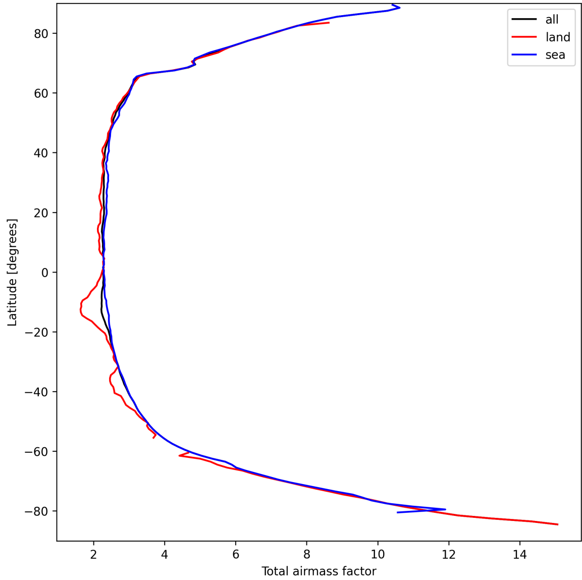
Figure 13: Zonal average of “Total airmass factor” for 2025-09-12 to 2025-09-13.
