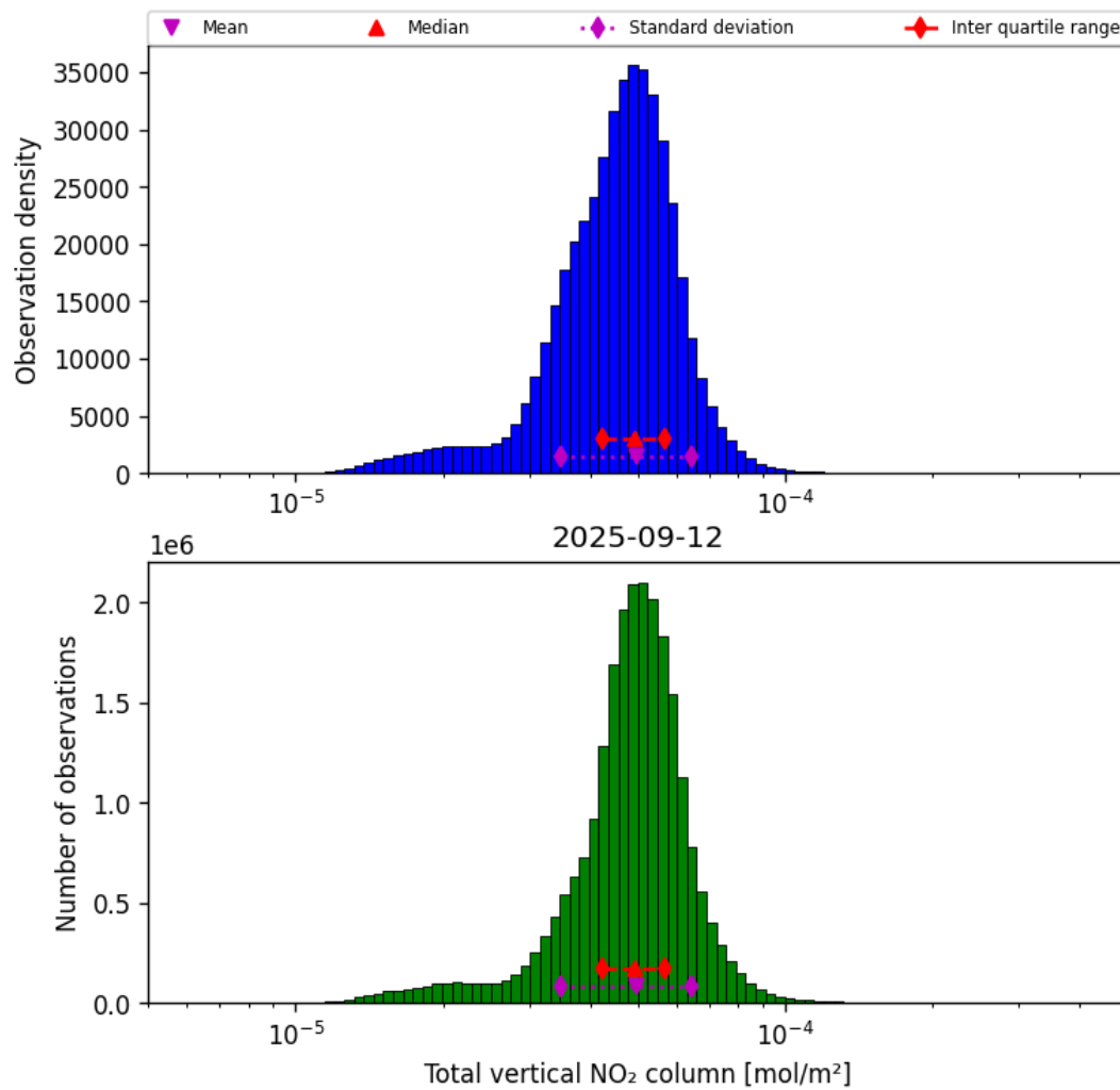
Figure 36: Histogram of “Total vertical NO 2 column” for 2025-09-12 to 2025-09-13
