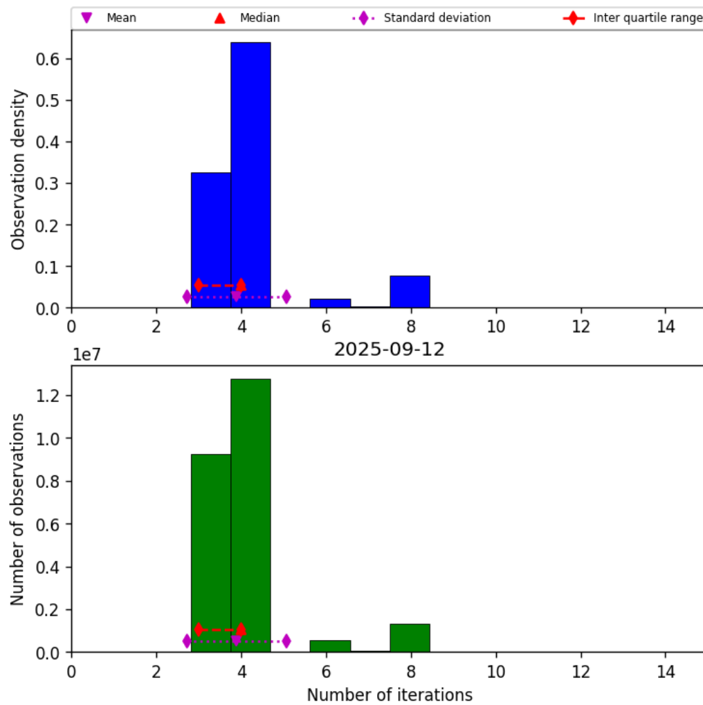
Figure 32: Histogram of “Number of iterations” for 2025-09-12 to 2025-09-13
