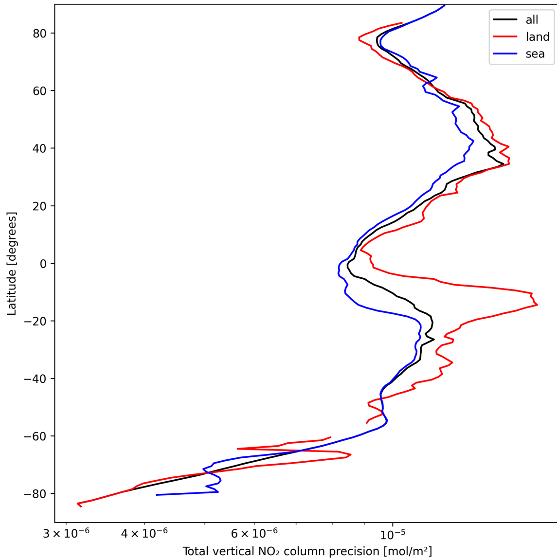
Figure 20: Zonal average of “Total vertical NO 2 column precision” for 2025-09-12 to 2025-09-13.
