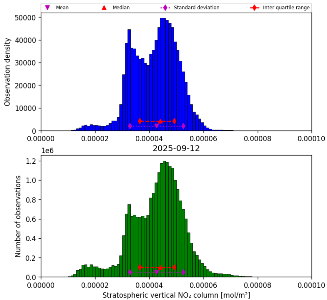
Figure 34: Histogram of “Stratospheric vertical NO 2 column” for 2025-09-12 to 2025-09-13
