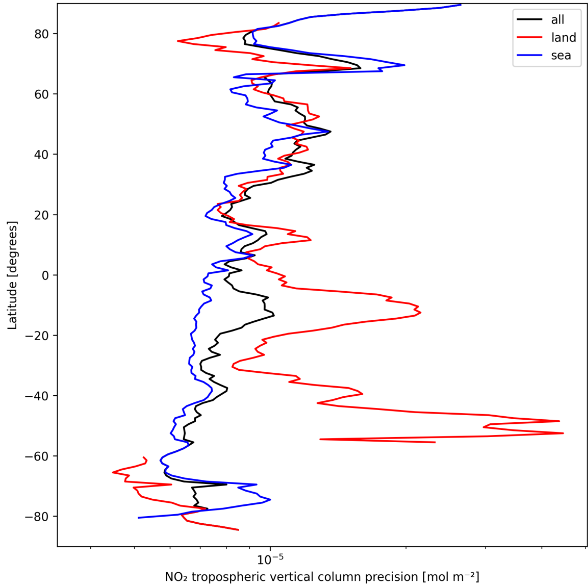
Figure 11: Zonal average of “NO 2 tropospheric vertical column precision” for 2025-09-12 to 2025-09-13.
