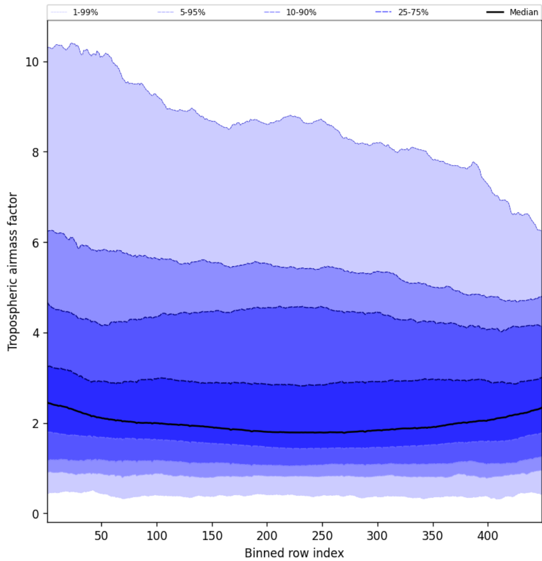
Figure 46: Along track statistics of “Tropospheric air mass factor” for 2025-09-12 to 2025-09-13
