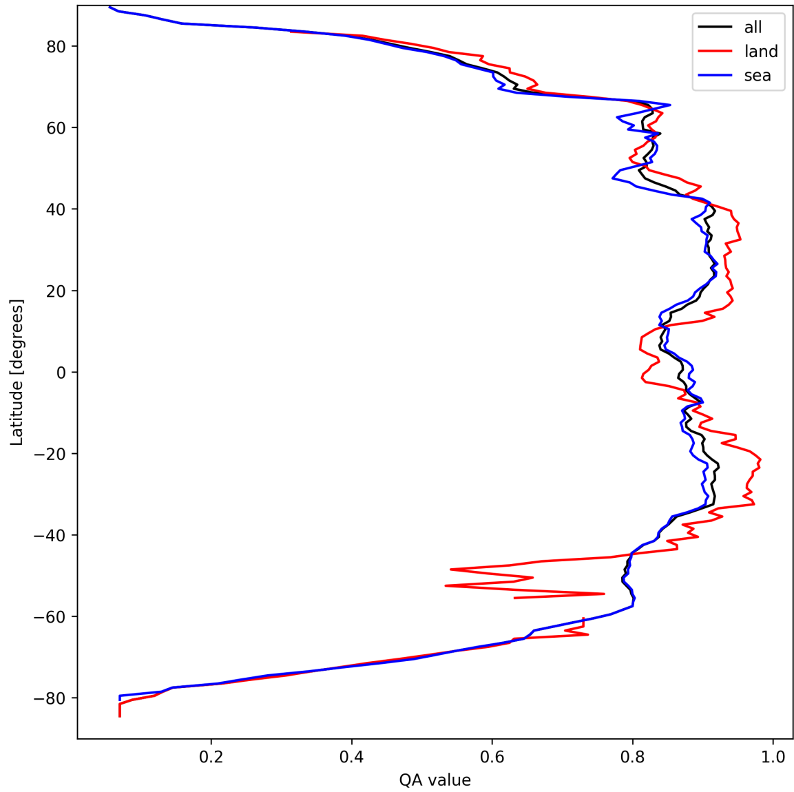
Figure 9: Zonal average of “QA value” for 2025-09-12 to 2025-09-13.
