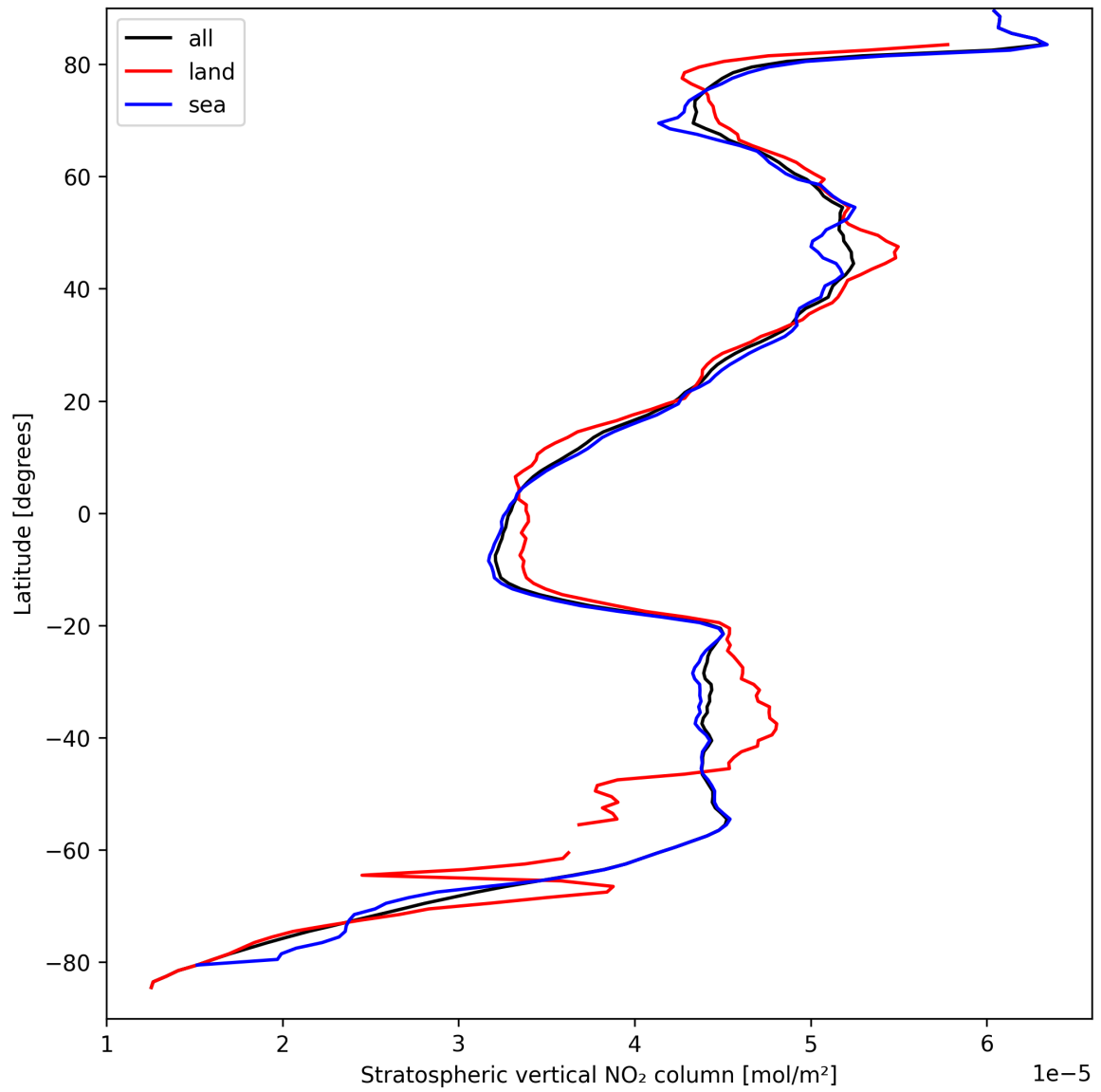
Figure 17: Zonal average of “Stratospheric vertical NO 2 column” for 2025-09-12 to 2025-09-13.
