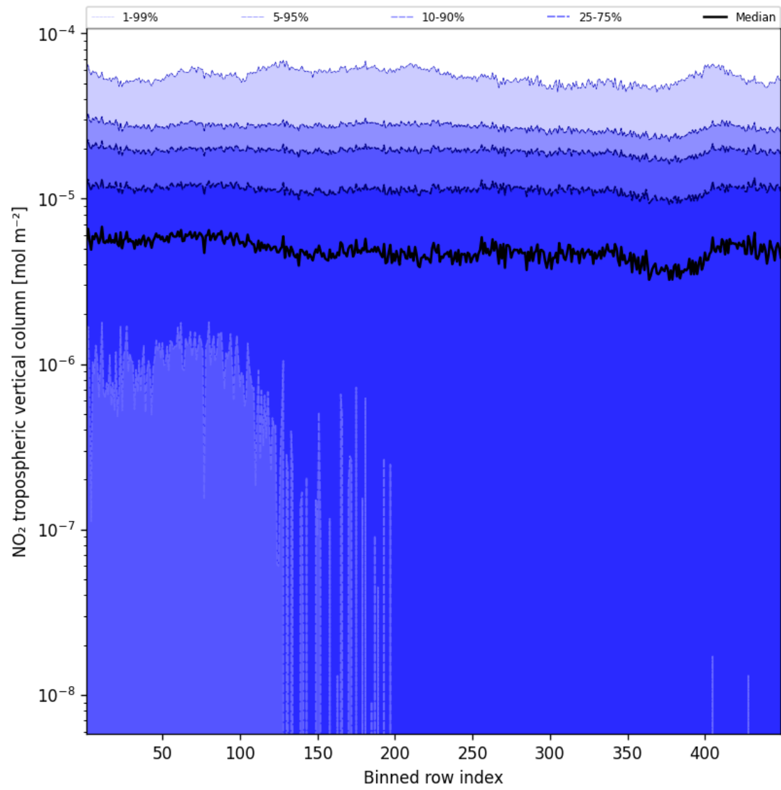
Figure 44: Along track statistics of “NO 2 tropospheric vertical column” for 2025-09-12 to 2025-09-13
