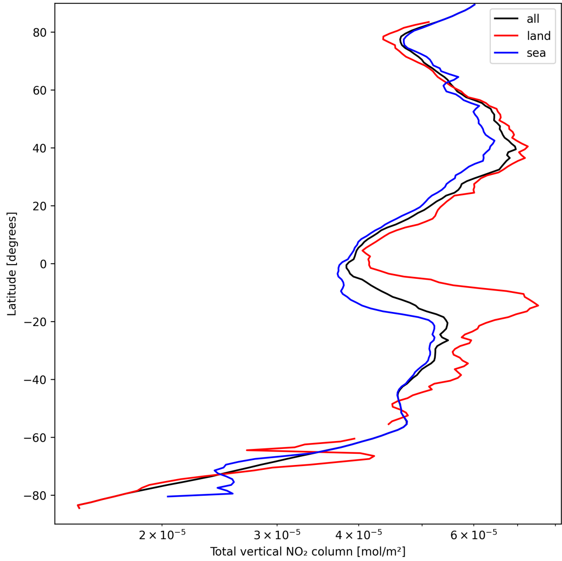
Figure 19: Zonal average of “Total vertical NO 2 column” for 2025-09-12 to 2025-09-13.
