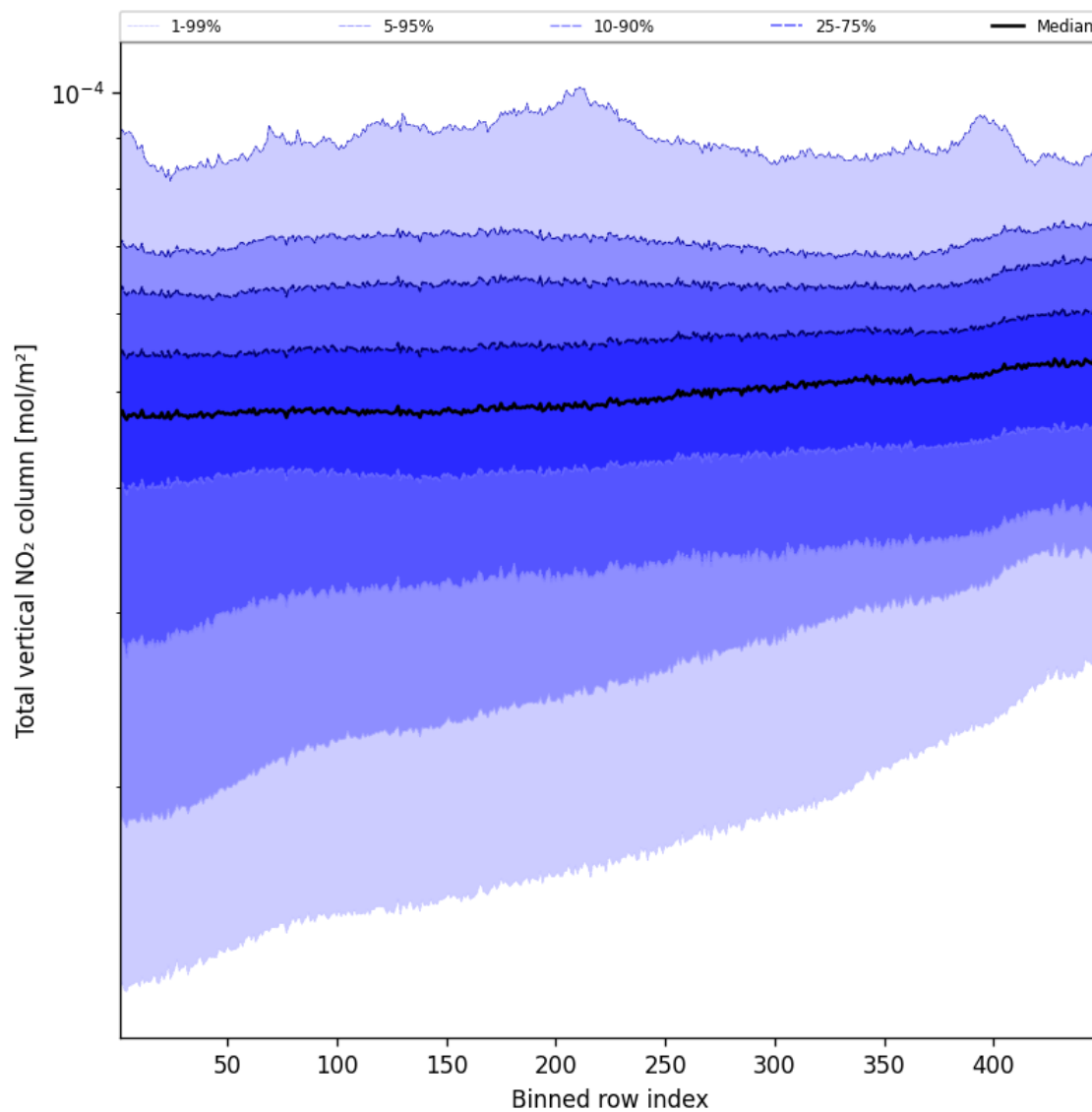
Figure 53: Along track statistics of “Total vertical NO 2 column” for 2025-09-12 to 2025-09-13
