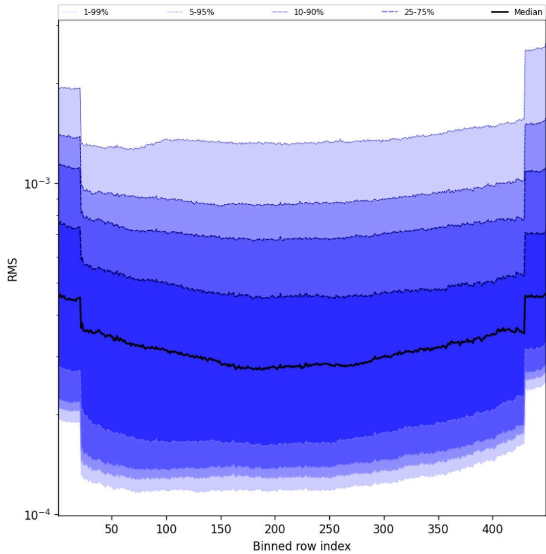
Figure 58: Along track statistics of “RMS” for 2025-09-12 to 2025-09-13
