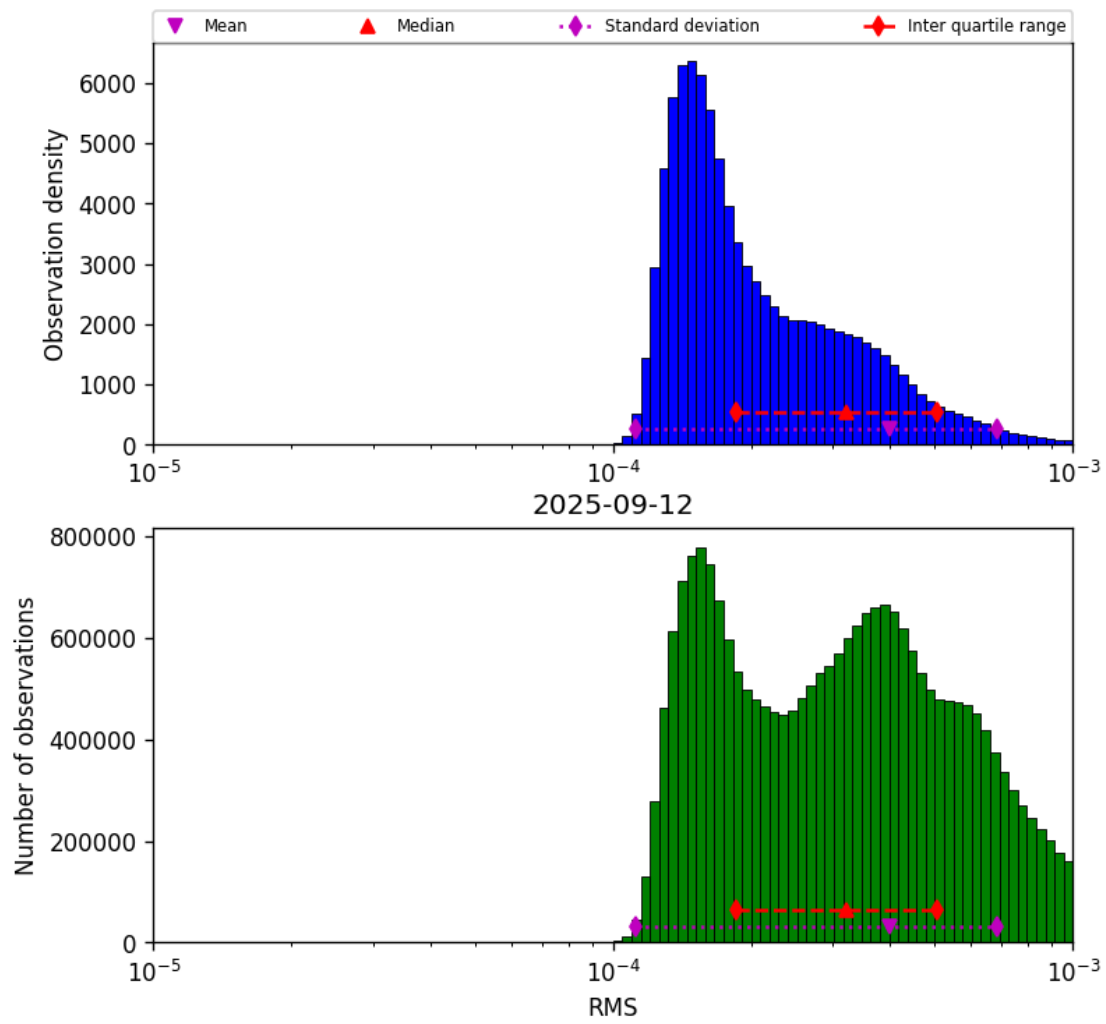
Figure 41: Histogram of “RMS” for 2025-09-12 to 2025-09-13
