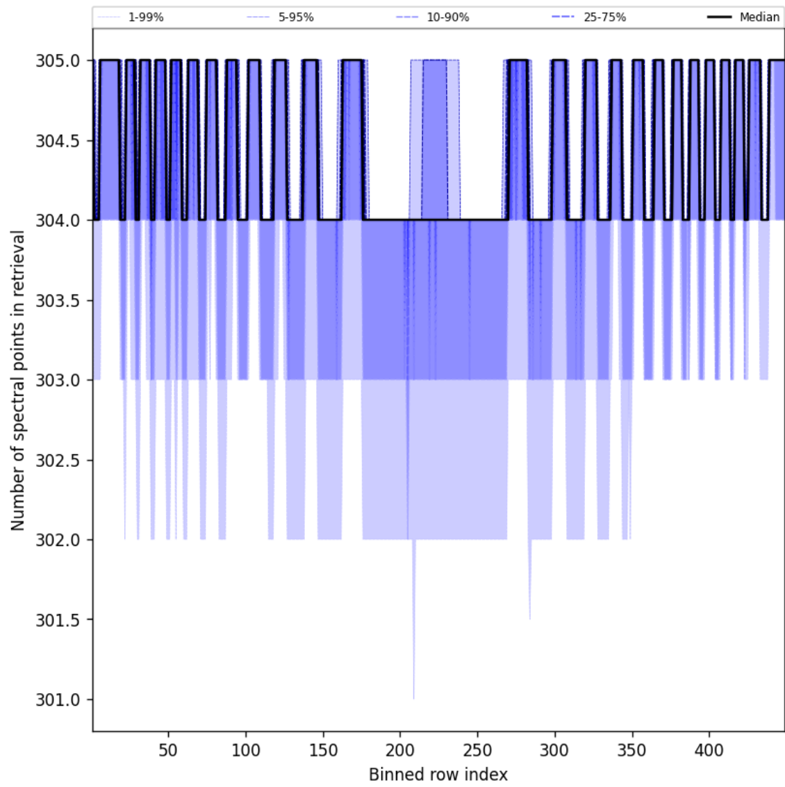
Figure 48: Along track statistics of “Number of spectral points in retrieval” for 2025-09-12 to 2025-09-13
