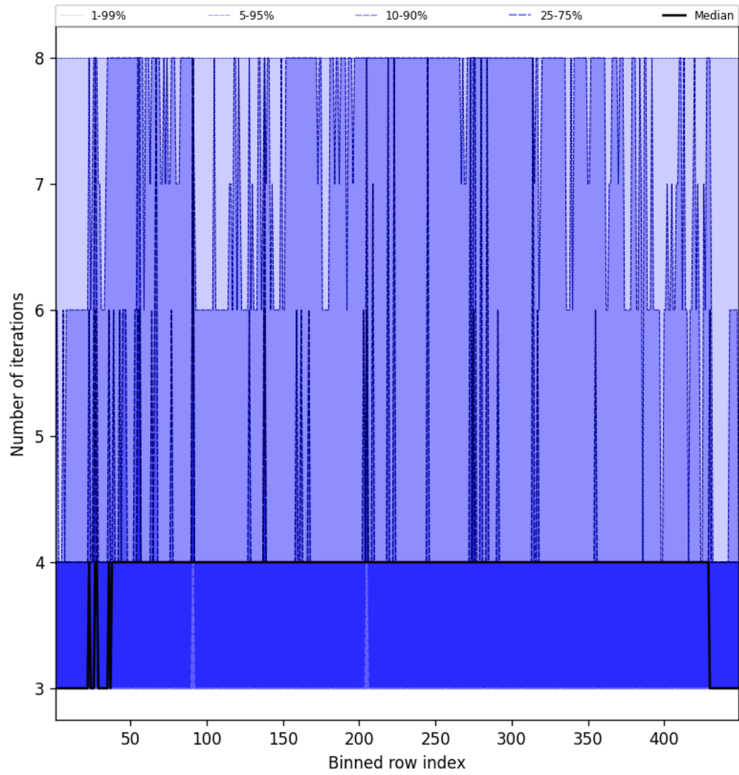
Figure 49: Along track statistics of “Number of iterations” for 2025-09-12 to 2025-09-13
