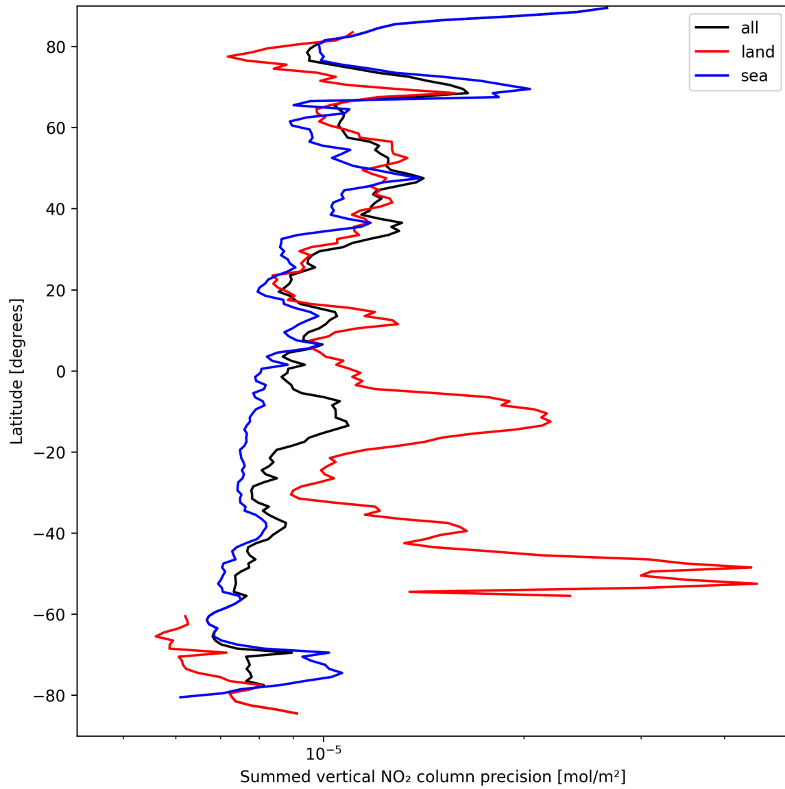
Figure 22: Zonal average of “Summed vertical NO 2 column precision” for 2025-09-12 to 2025-09-13.
