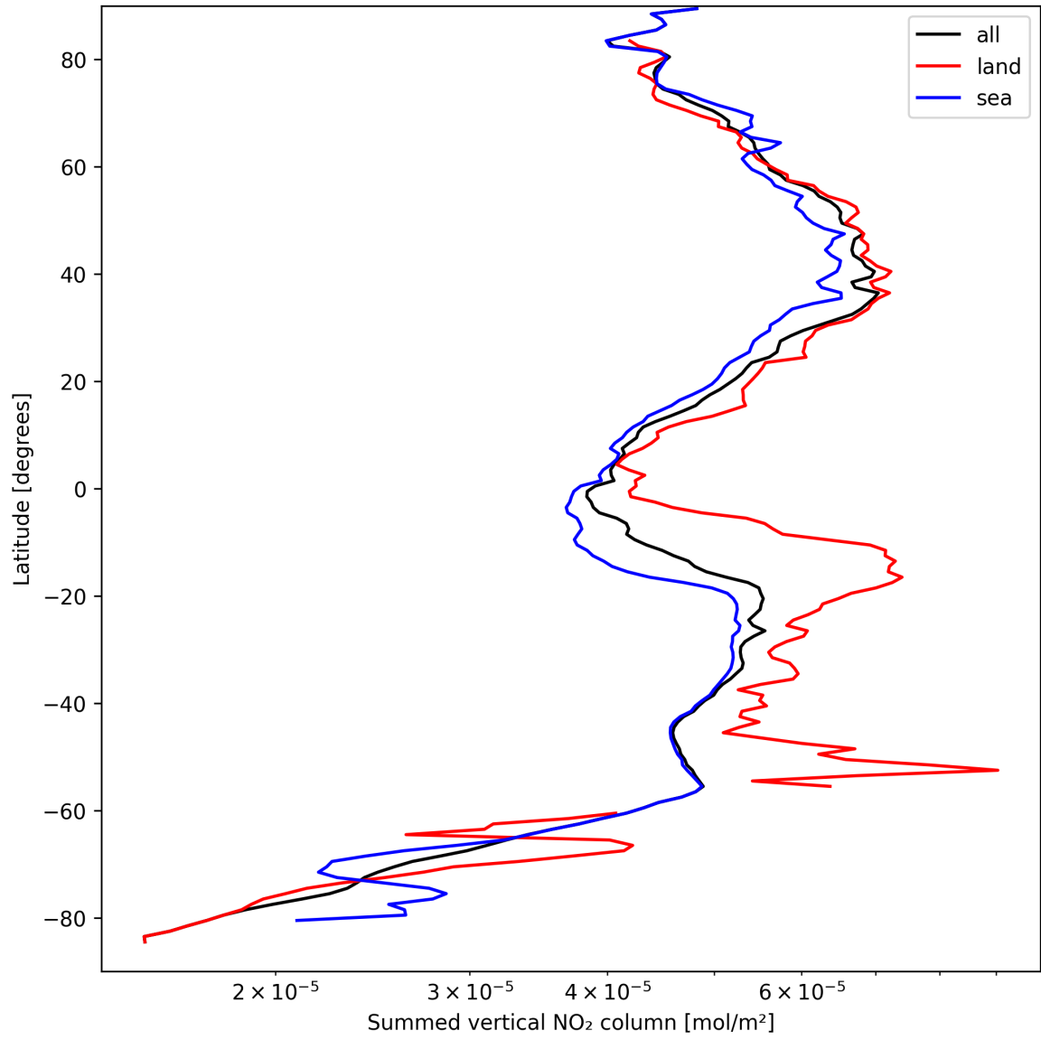
Figure 21: Zonal average of “Summed vertical NO 2 column” for 2025-09-12 to 2025-09-13.
