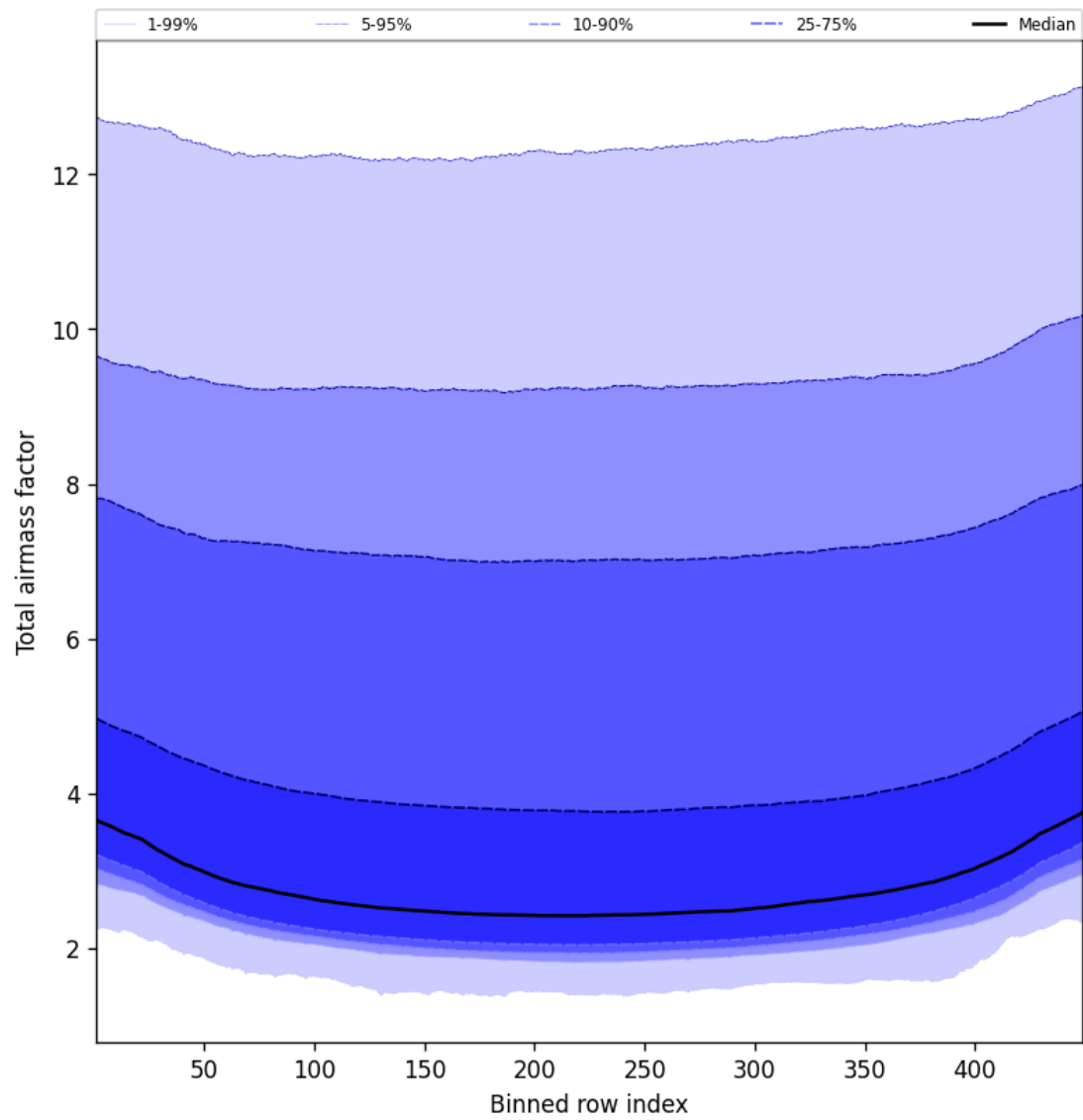
Figure 47: Along track statistics of “Total airmass factor” for 2025-09-12 to 2025-09-13
