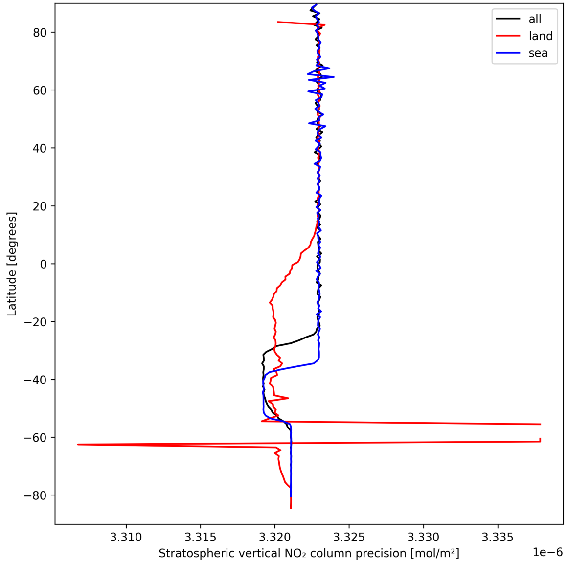
Figure 18: Zonal average of “Stratospheric vertical NO 2 column precision” for 2025-09-12 to 2025-09-13.
