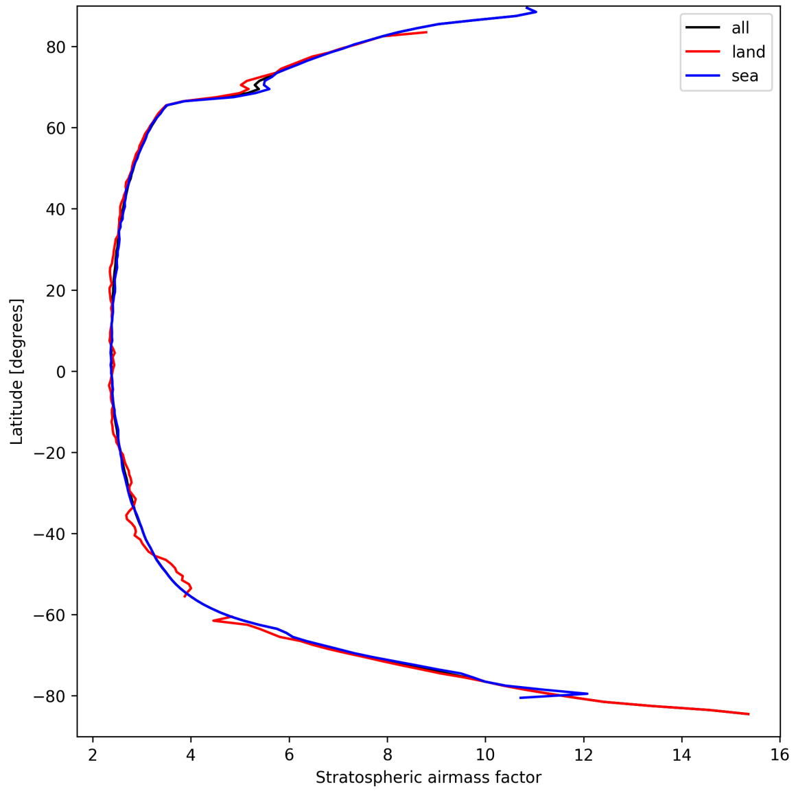
Figure 25: Zonal average of “Stratospheric airmass factor” for 2025-09-12 to 2025-09-13.
