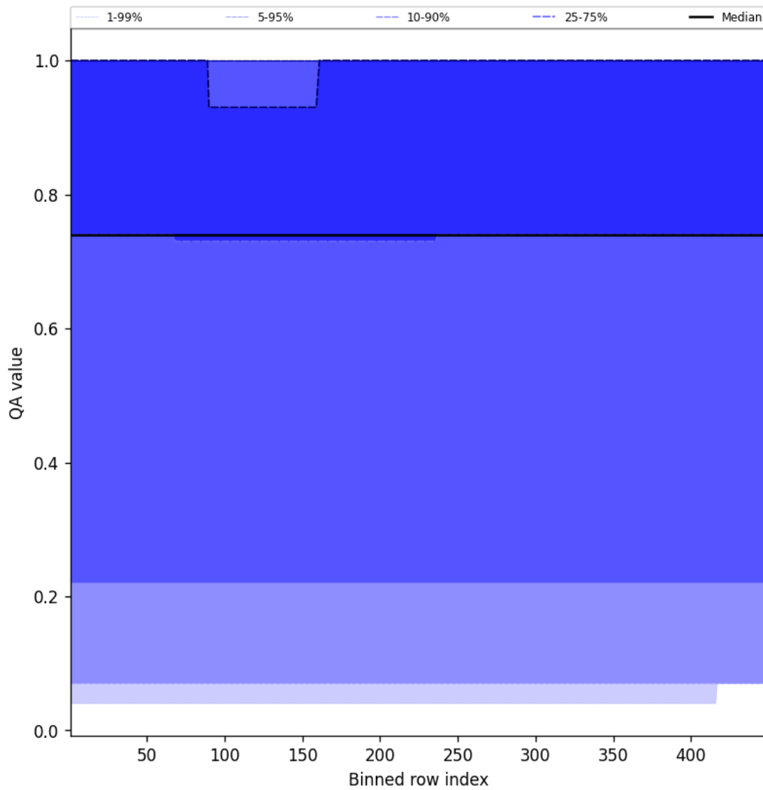
Figure 43: Along track statistics of “QA value” for 2025-09-12 to 2025-09-13
