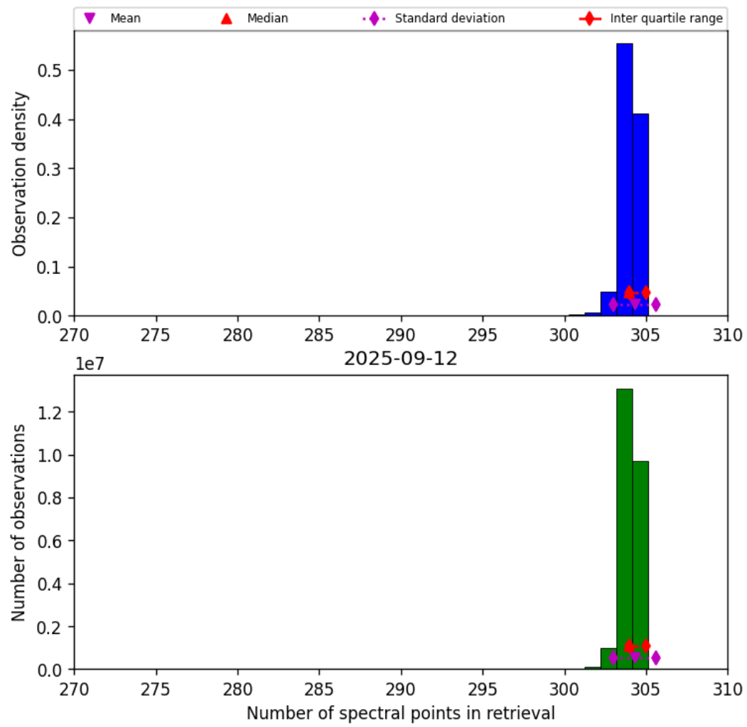
Figure 31: Histogram of “Number of spectral points in retrieval” for 2025-09-12 to 2025-09-13
