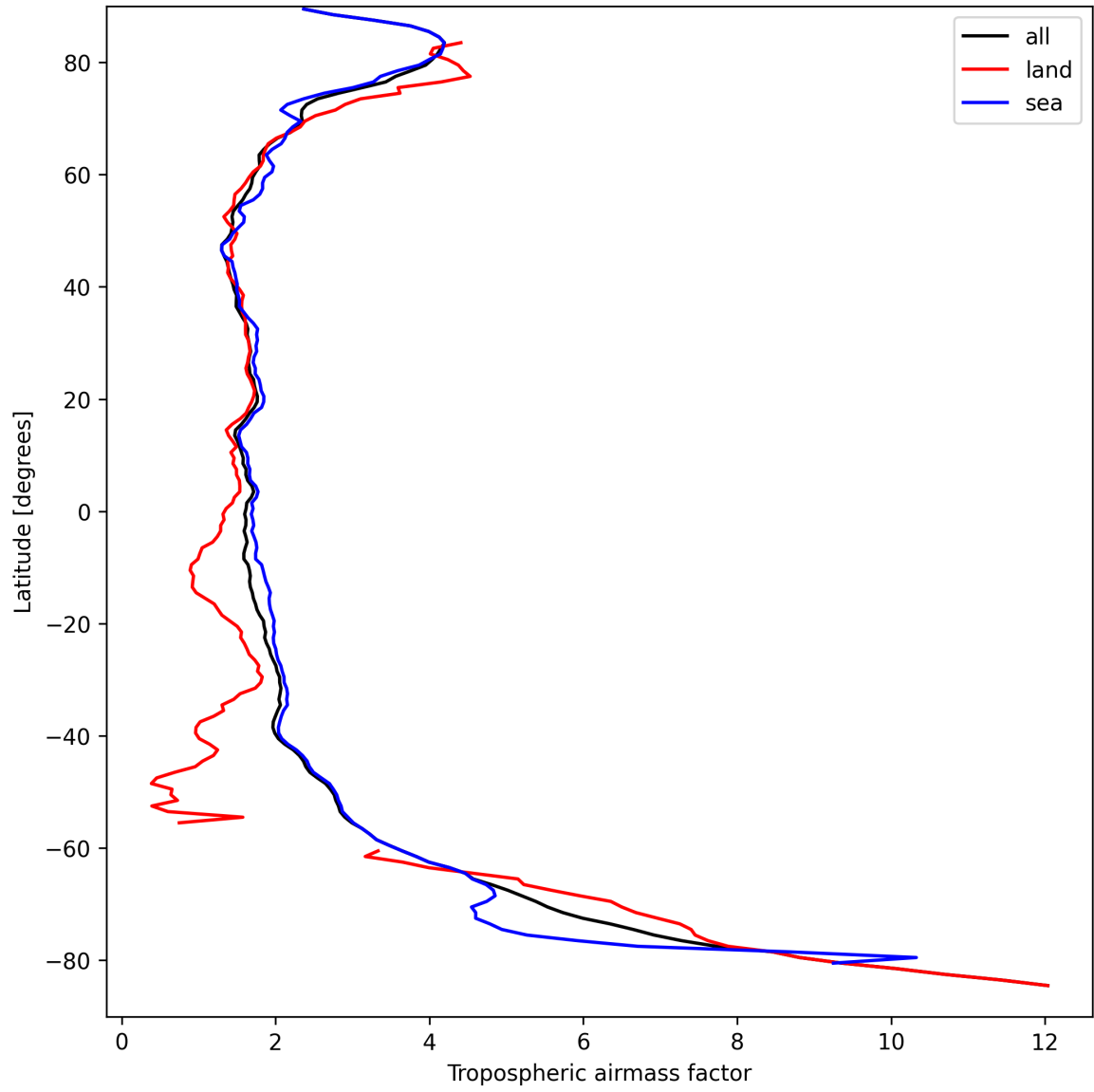
Figure 12: Zonal average of “Tropospheric airmass factor” for 2025-09-12 to 2025-09-13.
