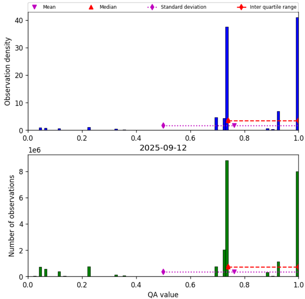
Figure 26: Histogram of “QA value” for 2025-09-12 to 2025-09-13
