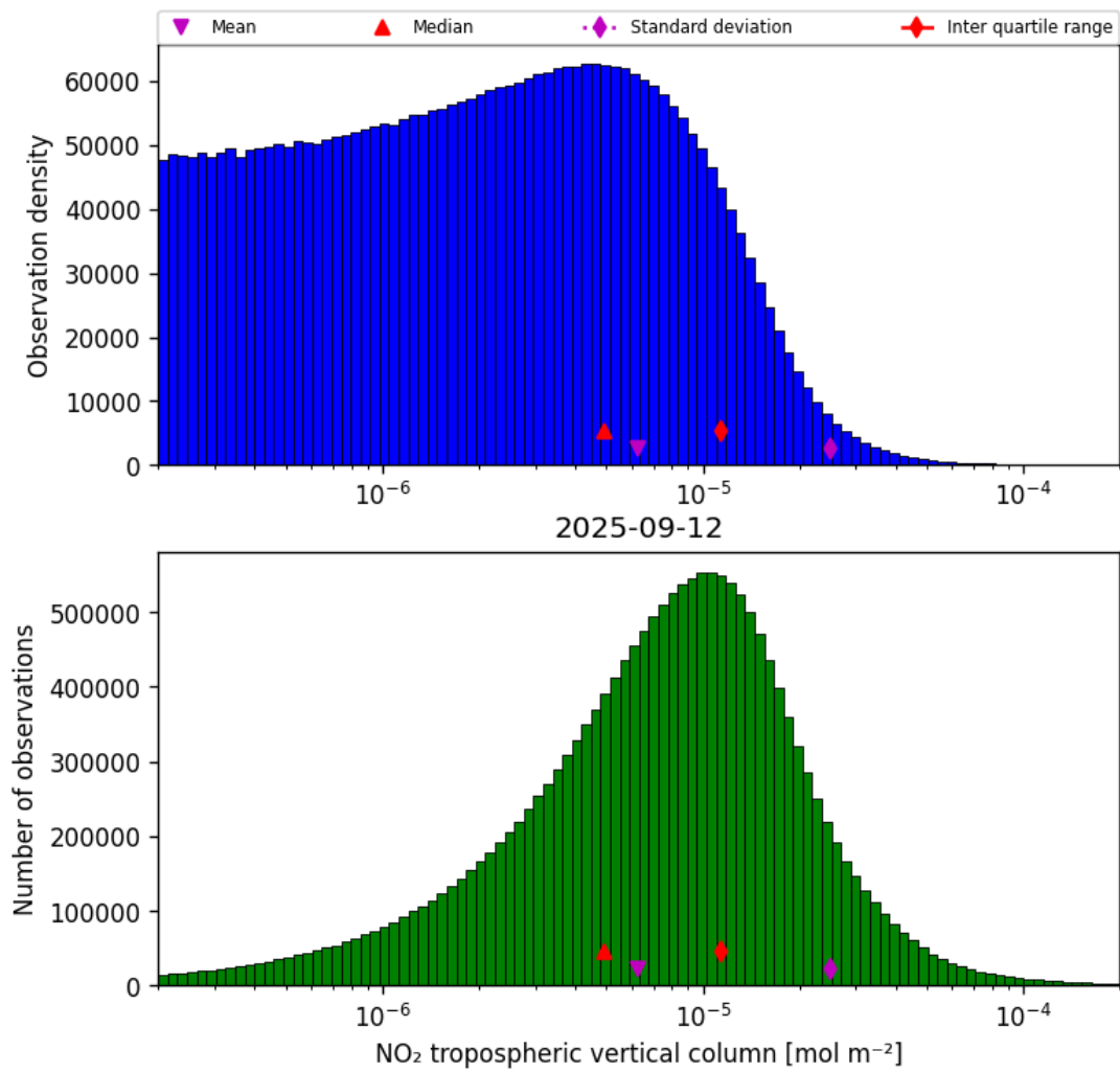
Figure 27: Histogram of “NO 2 tropospheric vertical column” for 2025-09-12 to 2025-09-13
