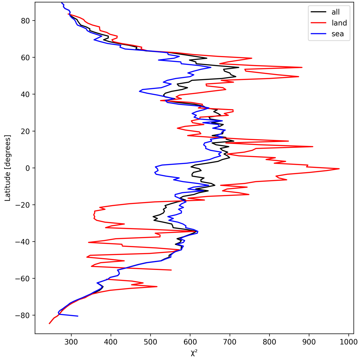
Figure 23: Zonal average of “ \chi^2 ” for 2025-09-12 to 2025-09-13.
