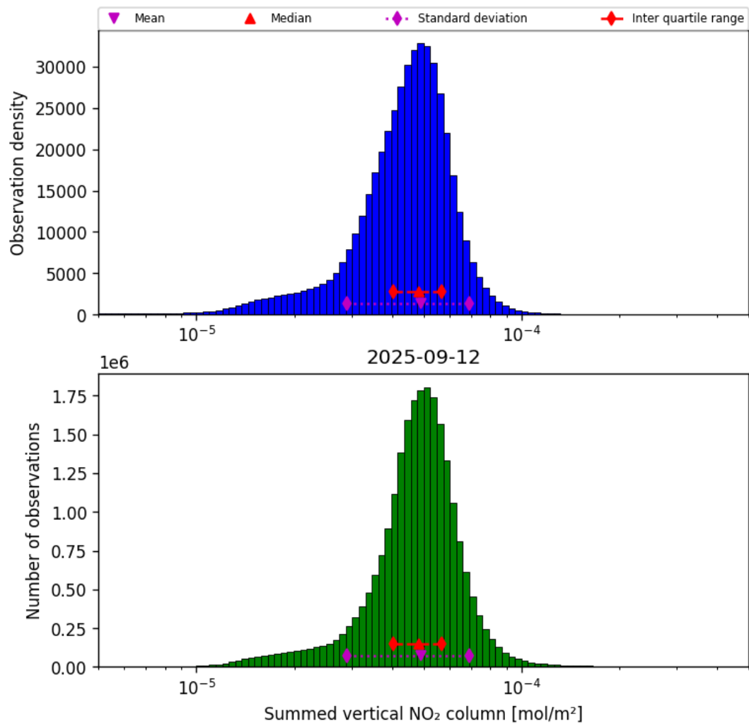
Figure 38: Histogram of “Summed vertical NO 2 column” for 2025-09-12 to 2025-09-13
