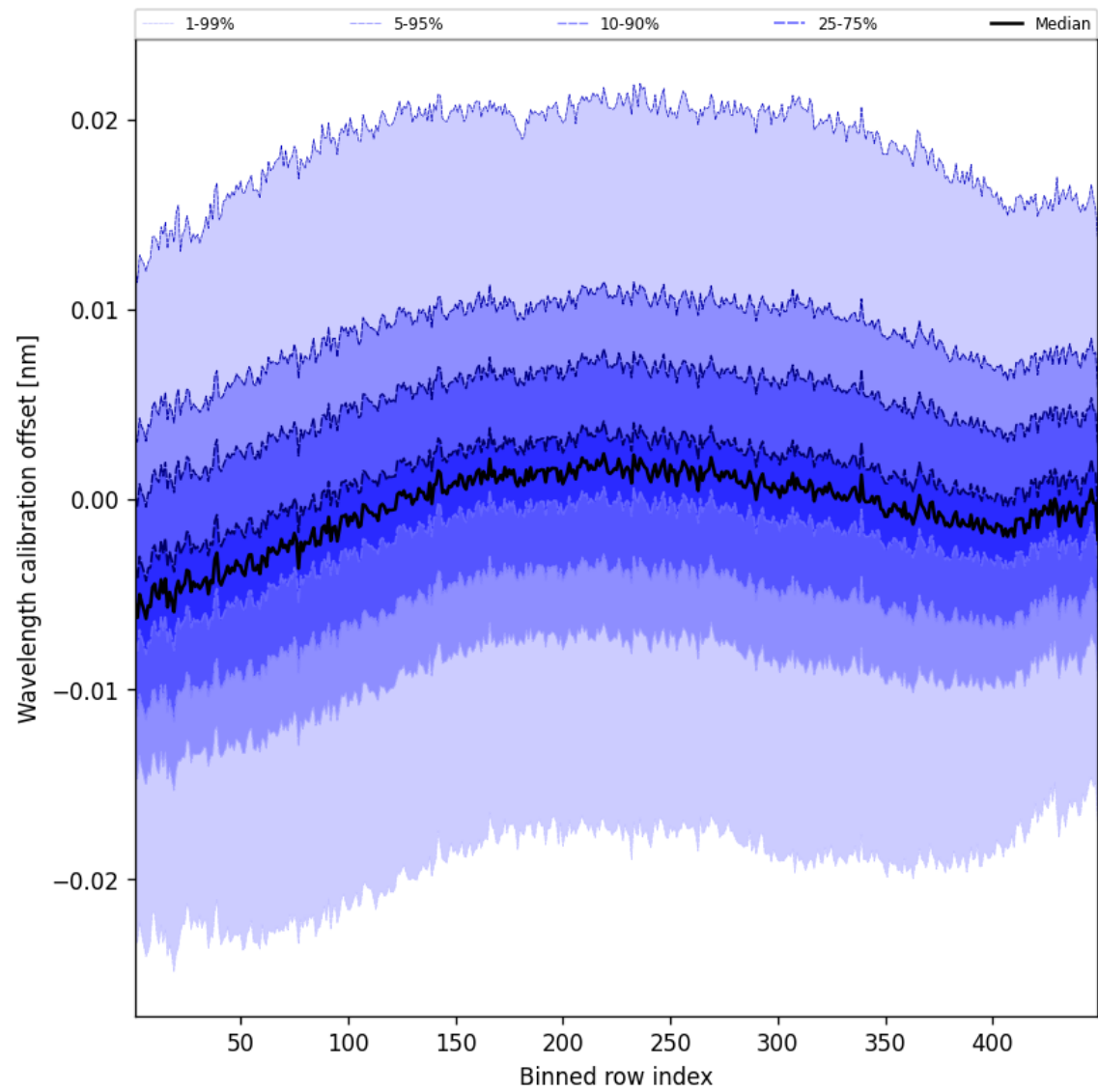
Figure 50: Along track statistics of “Wavelength calibration offset” for 2025-09-12 to 2025-09-13
