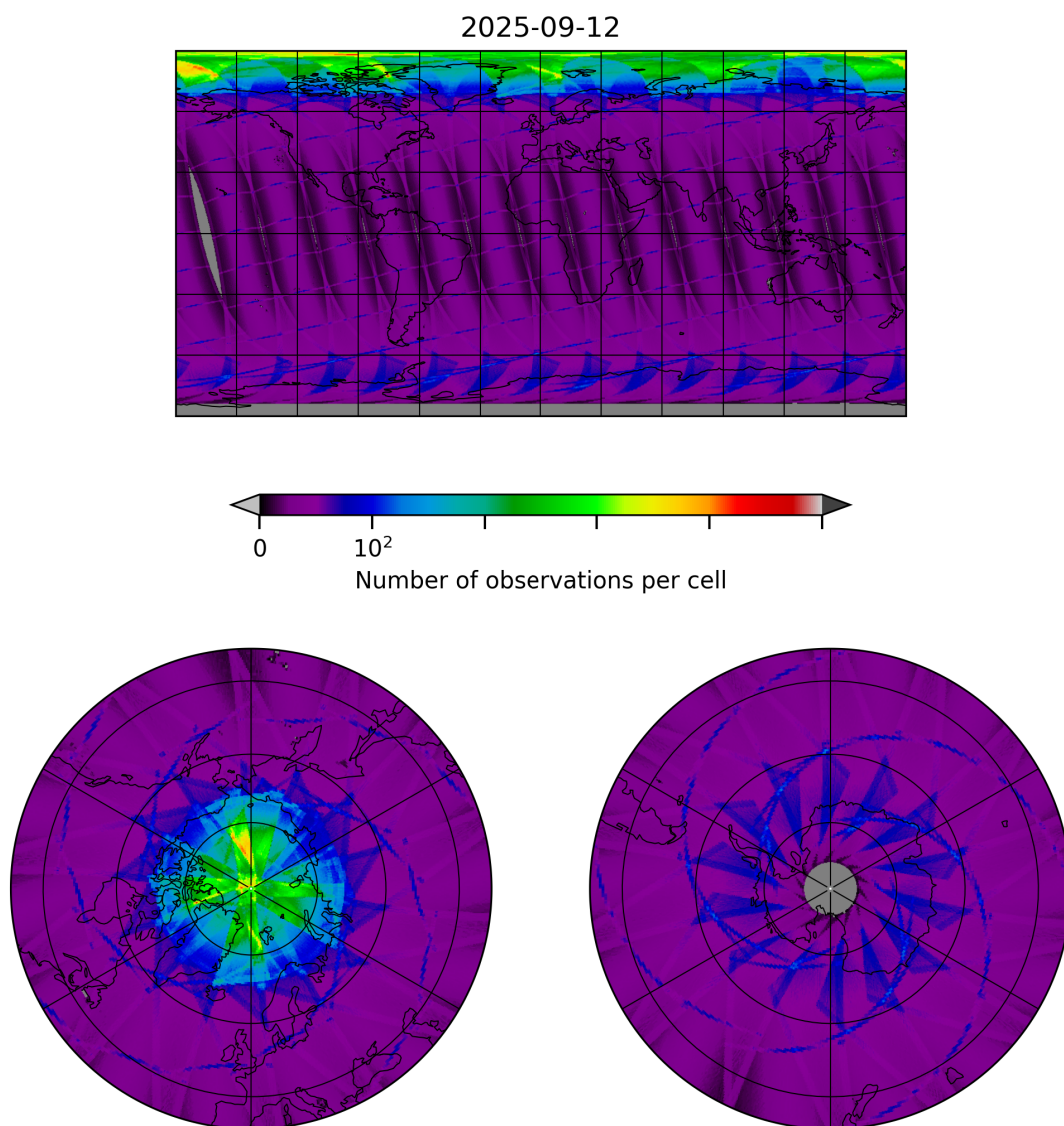
Figure 8: Map of the number of observations for 2025-09-12 to 2025-09-13
