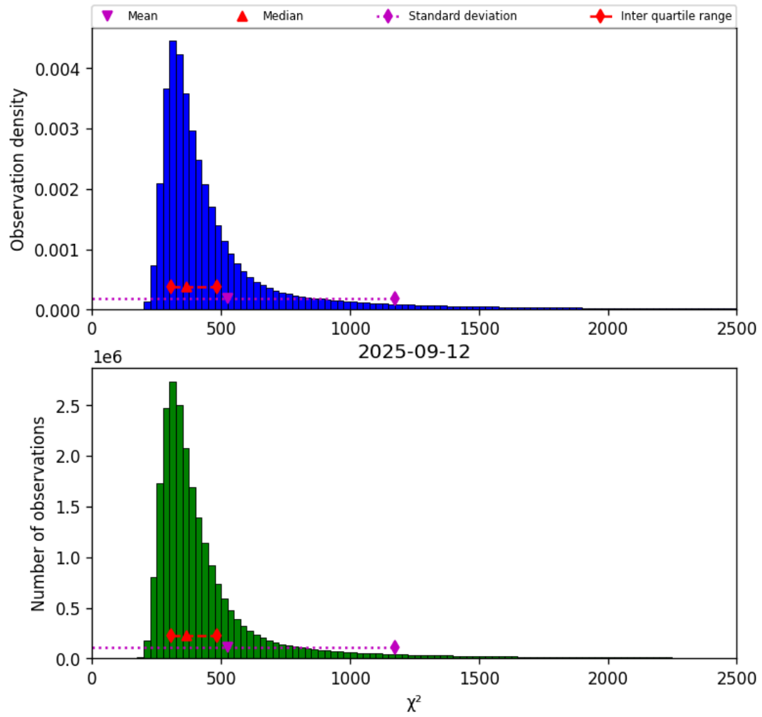
Figure 40: Histogram of “ \chi^2 ” for 2025-09-12 to 2025-09-13
