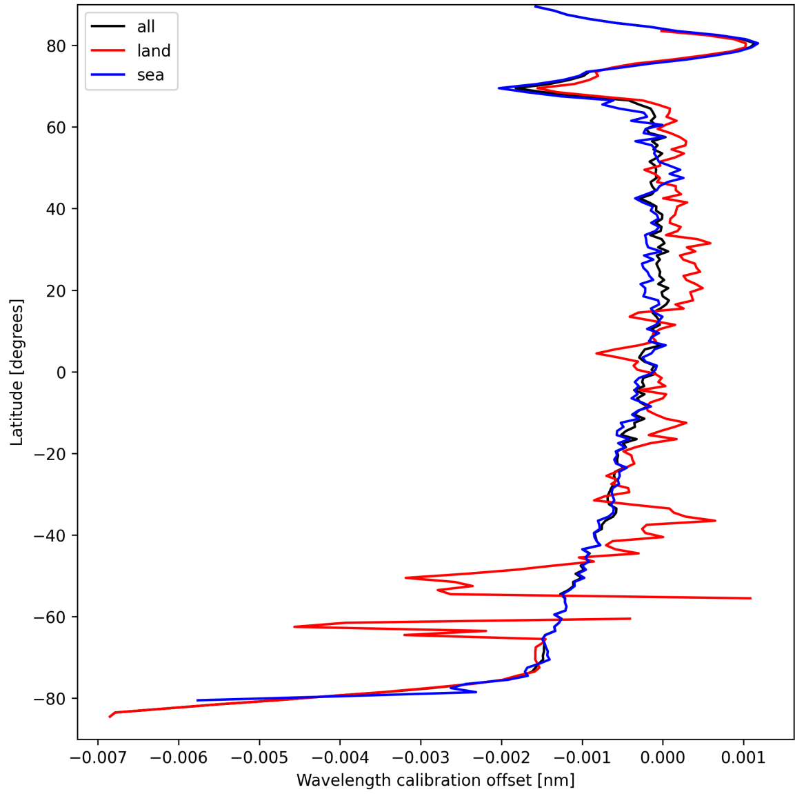
Figure 16: Zonal average of “Wavelength calibration offset” for 2025-09-12 to 2025-09-13.
