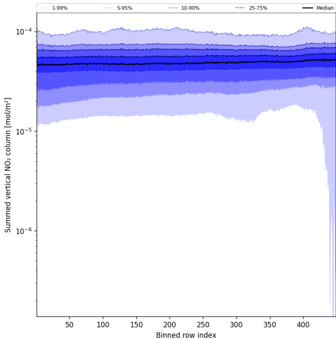
Figure 55: Along track statistics of “Summed vertical NO 2 column” for 2025-09-12 to 2025-09-13
