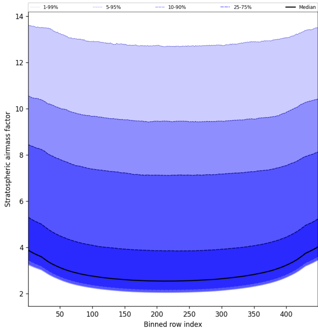
Figure 59: Along track statistics of “Stratospheric airmass factor” for 2025-09-12 to 2025-09-13
