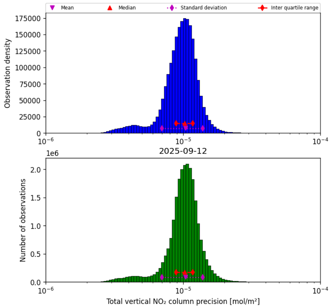
Figure 37: Histogram of “Total vertical NO 2 column precision” for 2025-09-12 to 2025-09-13
