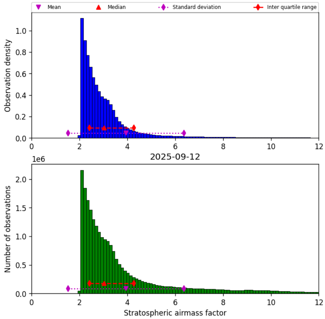
Figure 42: Histogram of “Stratospheric airmass factor” for 2025-09-12 to 2025-09-13
