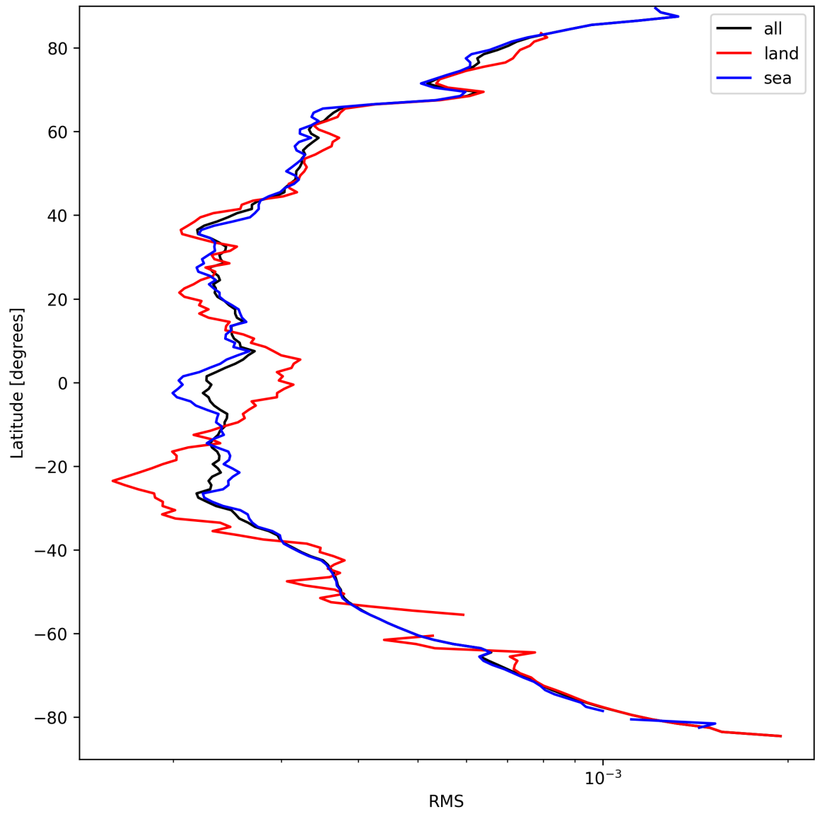
Figure 24: Zonal average of “RMS” for 2025-09-13 to 2025-09-13.
