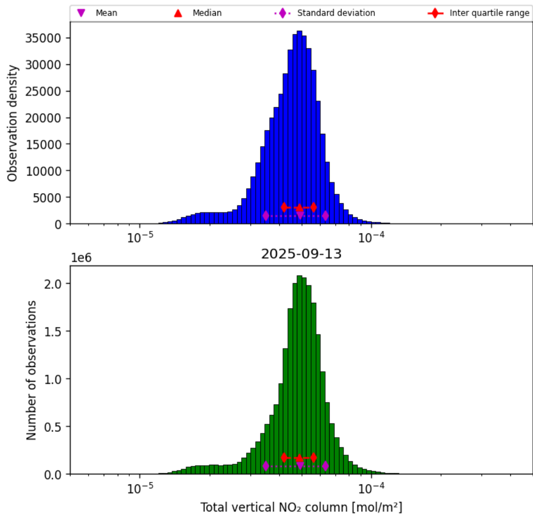
Figure 36: Histogram of "Total vertical NO 2 column" for 2025-09-13 to 2025-09-13
