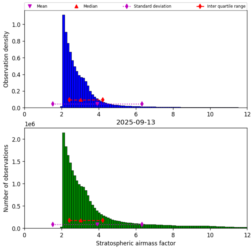
Figure 42: Histogram of “Stratospheric airmass factor” for 2025-09-13 to 2025-09-13
