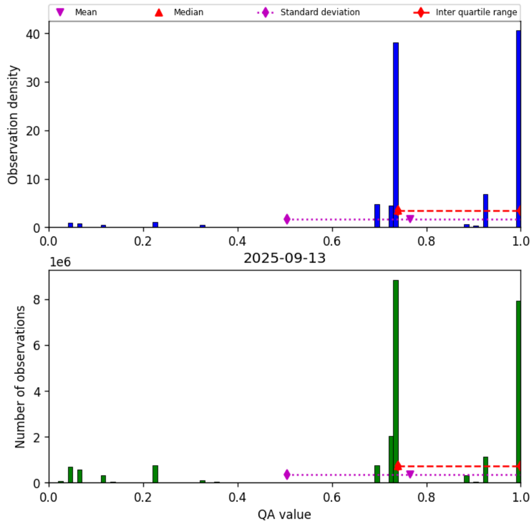
Figure 26: Histogram of “QA value” for 2025-09-13 to 2025-09-13
