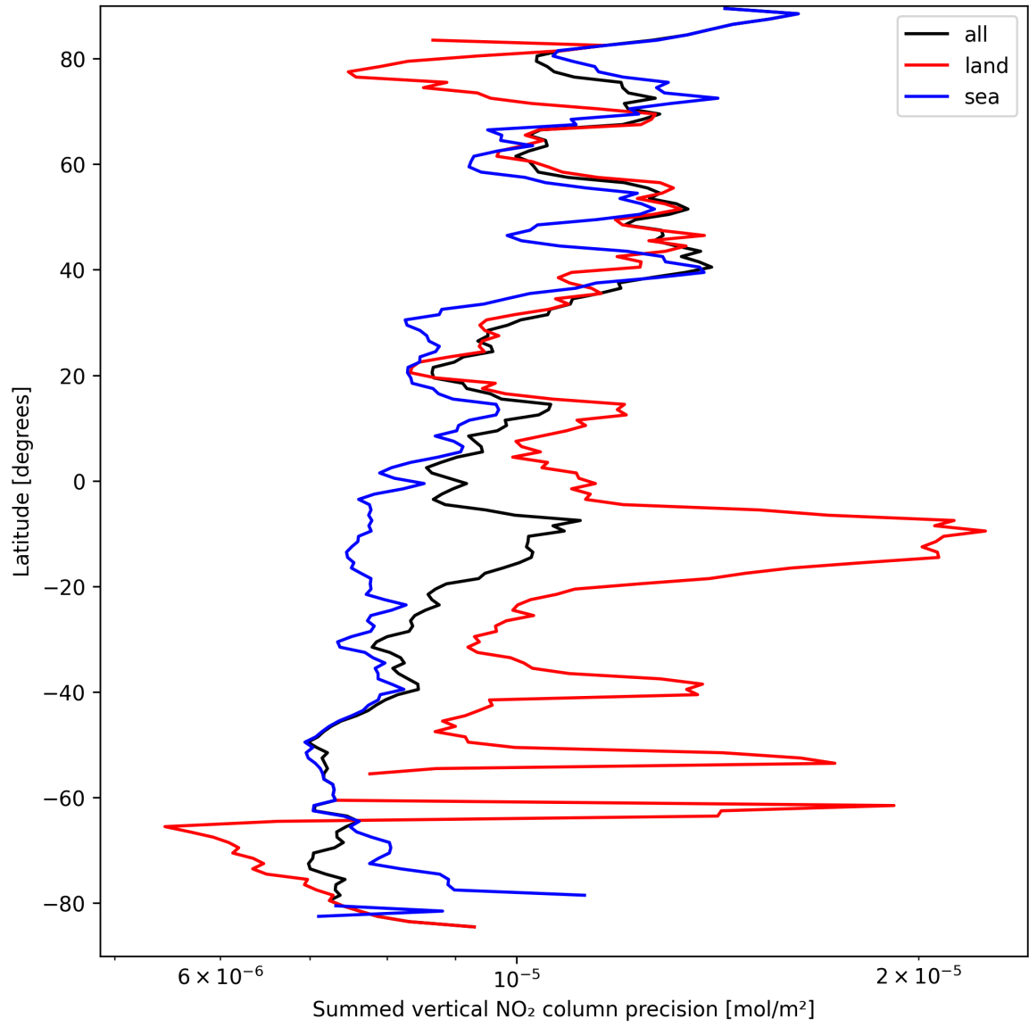
Figure 22: Zonal average of “Summed vertical NO 2 column precision” for 2025-09-13 to 2025-09-13.
