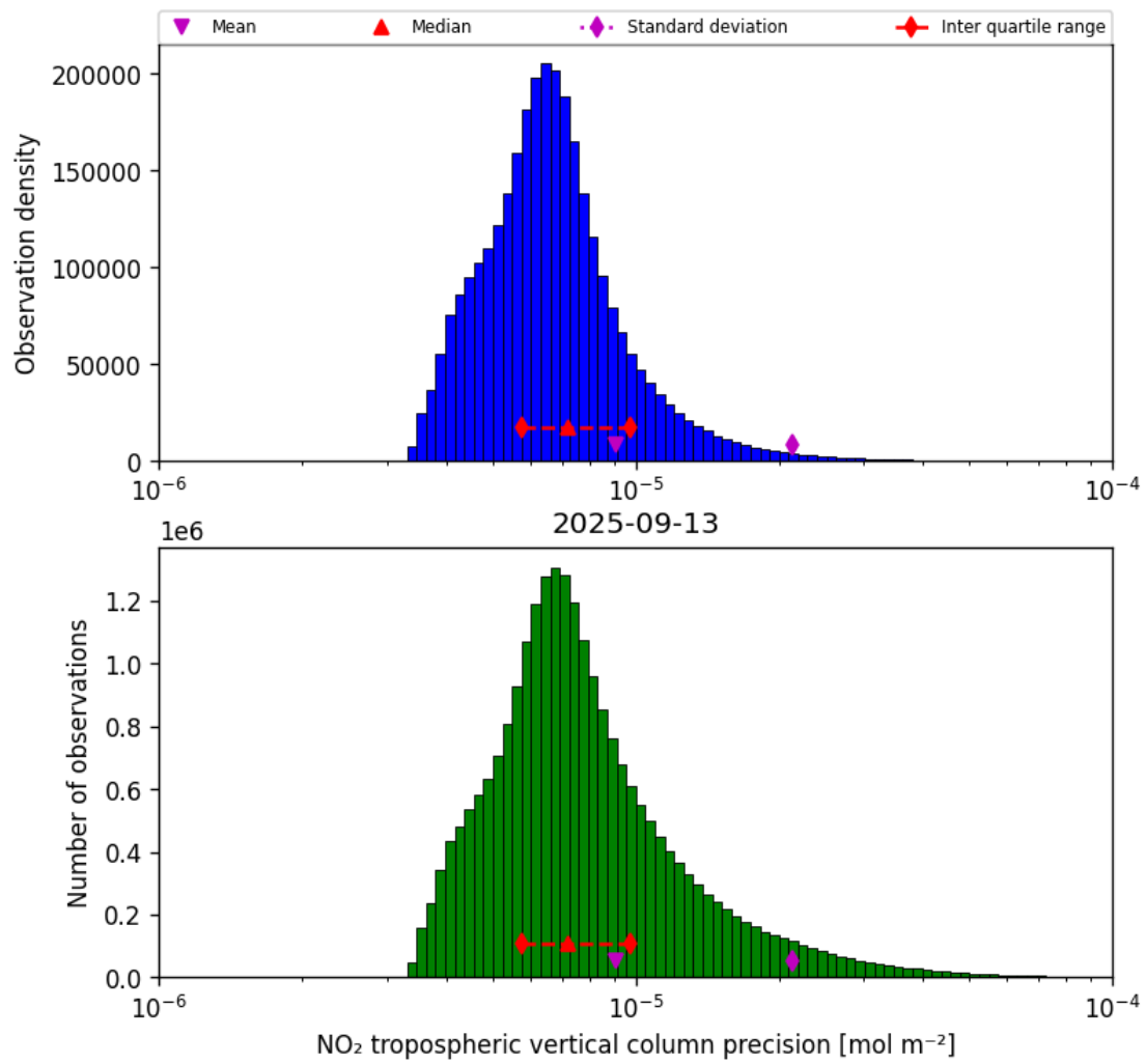
Figure 28: Histogram of “NO 2 tropospheric vertical column precision” for 2025-09-13 to 2025-09-13
