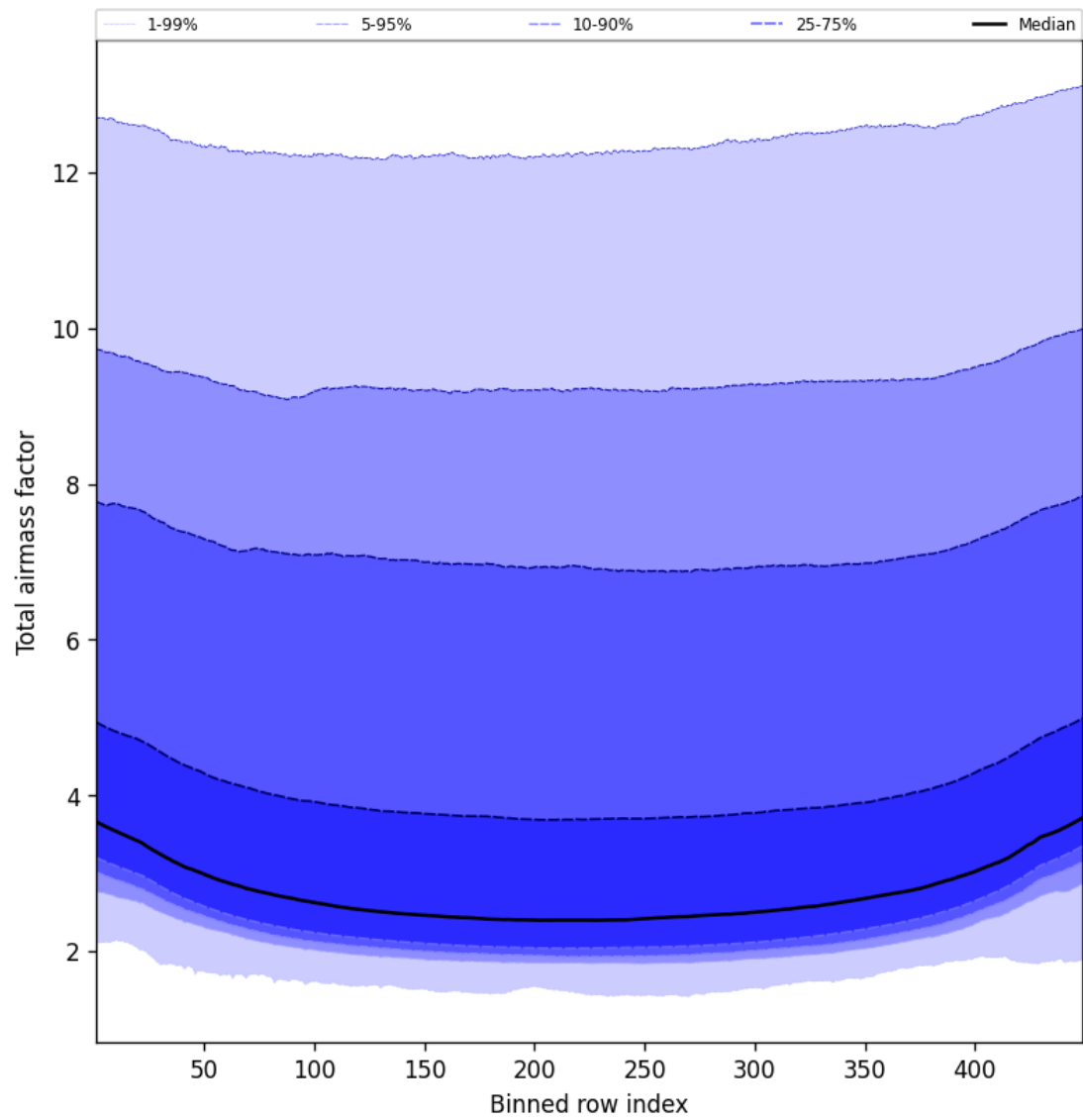
Figure 47: Along track statistics of “Total airmass factor” for 2025-09-13 to 2025-09-13
