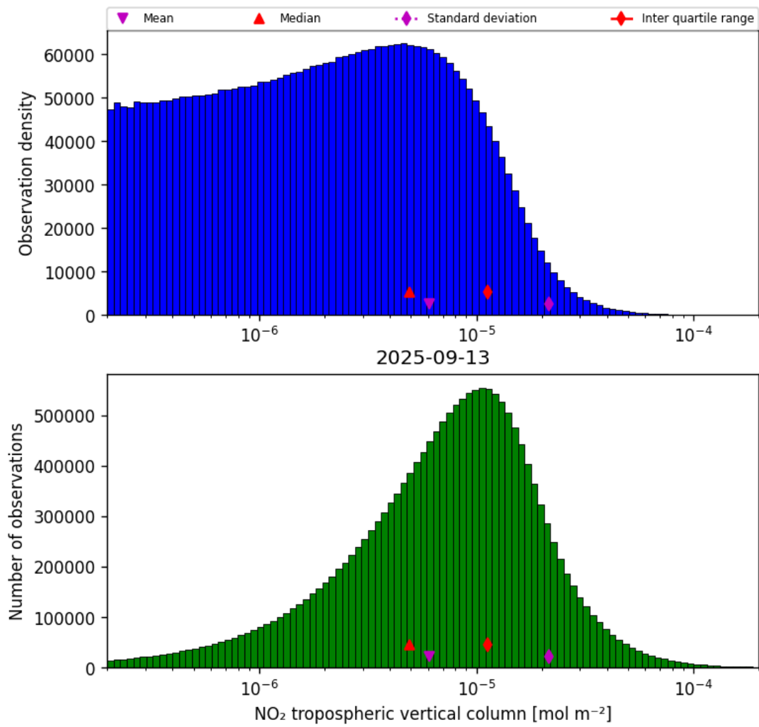
Figure 27: Histogram of “NO 2 tropospheric vertical column” for 2025-09-13 to 2025-09-13
