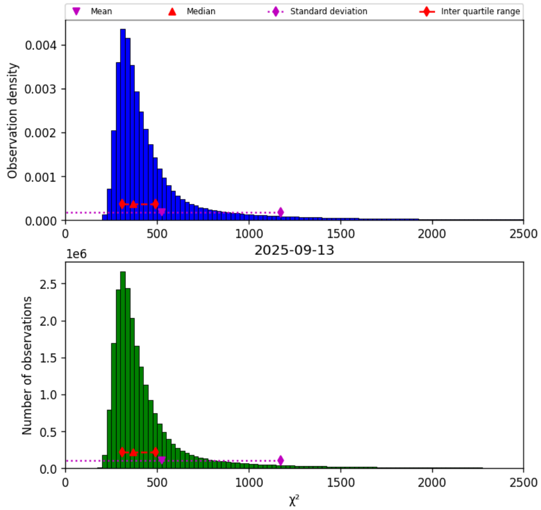
Figure 40: Histogram of “ \chi^2 ” for 2025-09-13 to 2025-09-13
