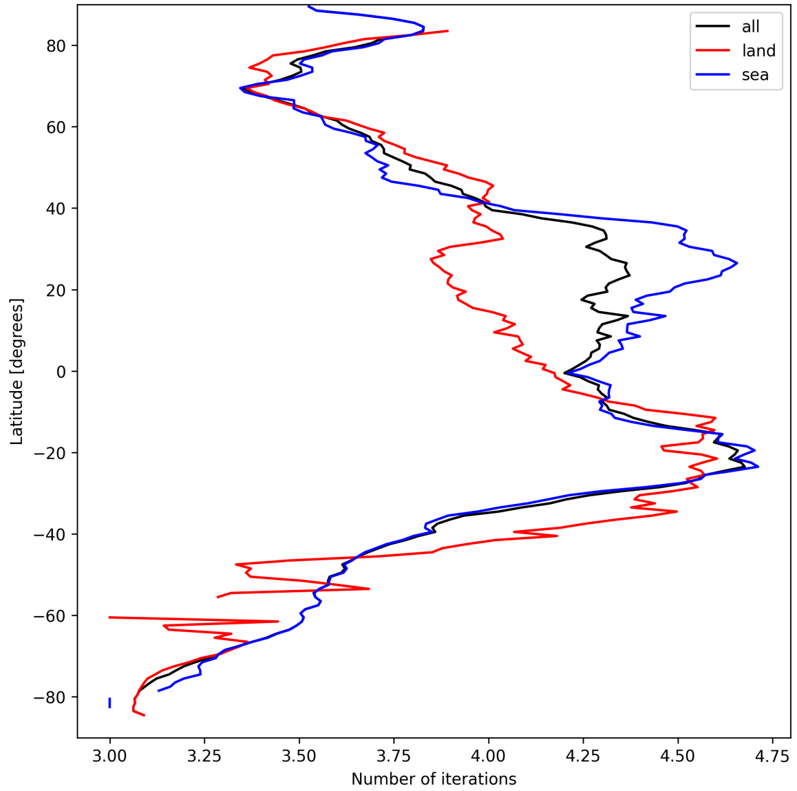
Figure 15: Zonal average of “Number of iterations” for 2025-09-13 to 2025-09-13.
