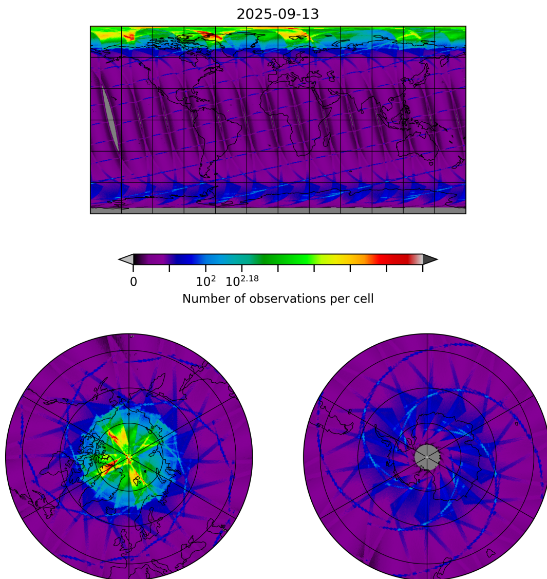
Figure 8: Map of the number of observations for 2025-09-13 to 2025-09-13
