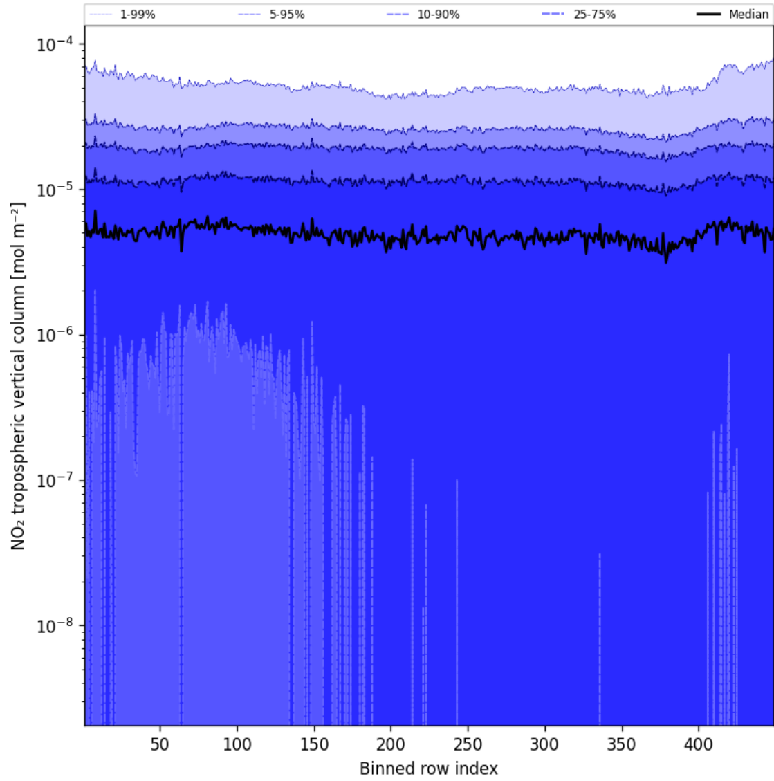
Figure 44: Along track statistics of “NO 2 tropospheric vertical column” for 2025-09-13 to 2025-09-13
