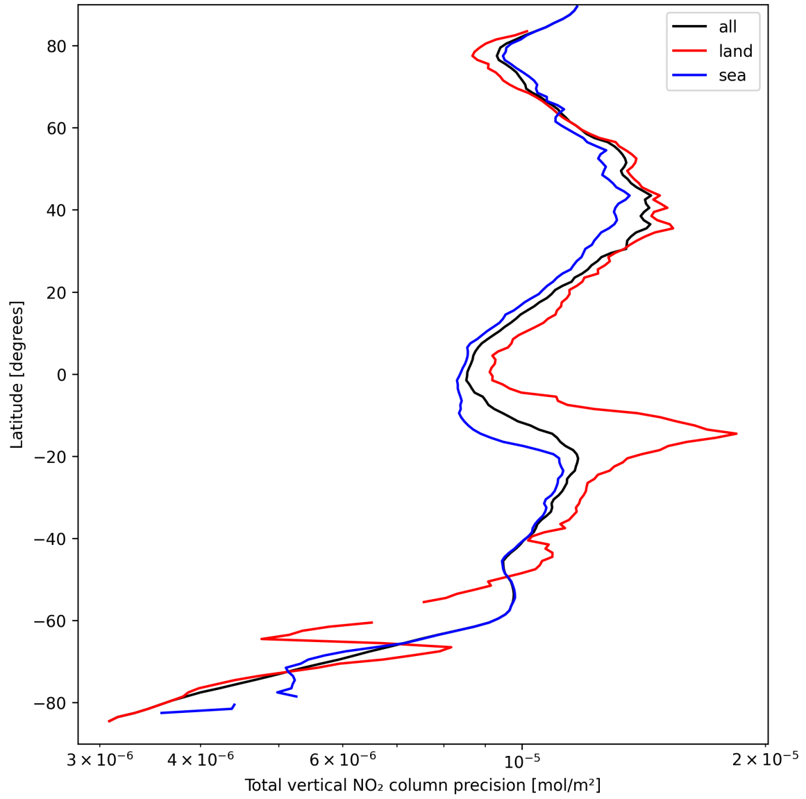
Figure 20: Zonal average of “Total vertical NO 2 column precision” for 2025-09-13 to 2025-09-13.
