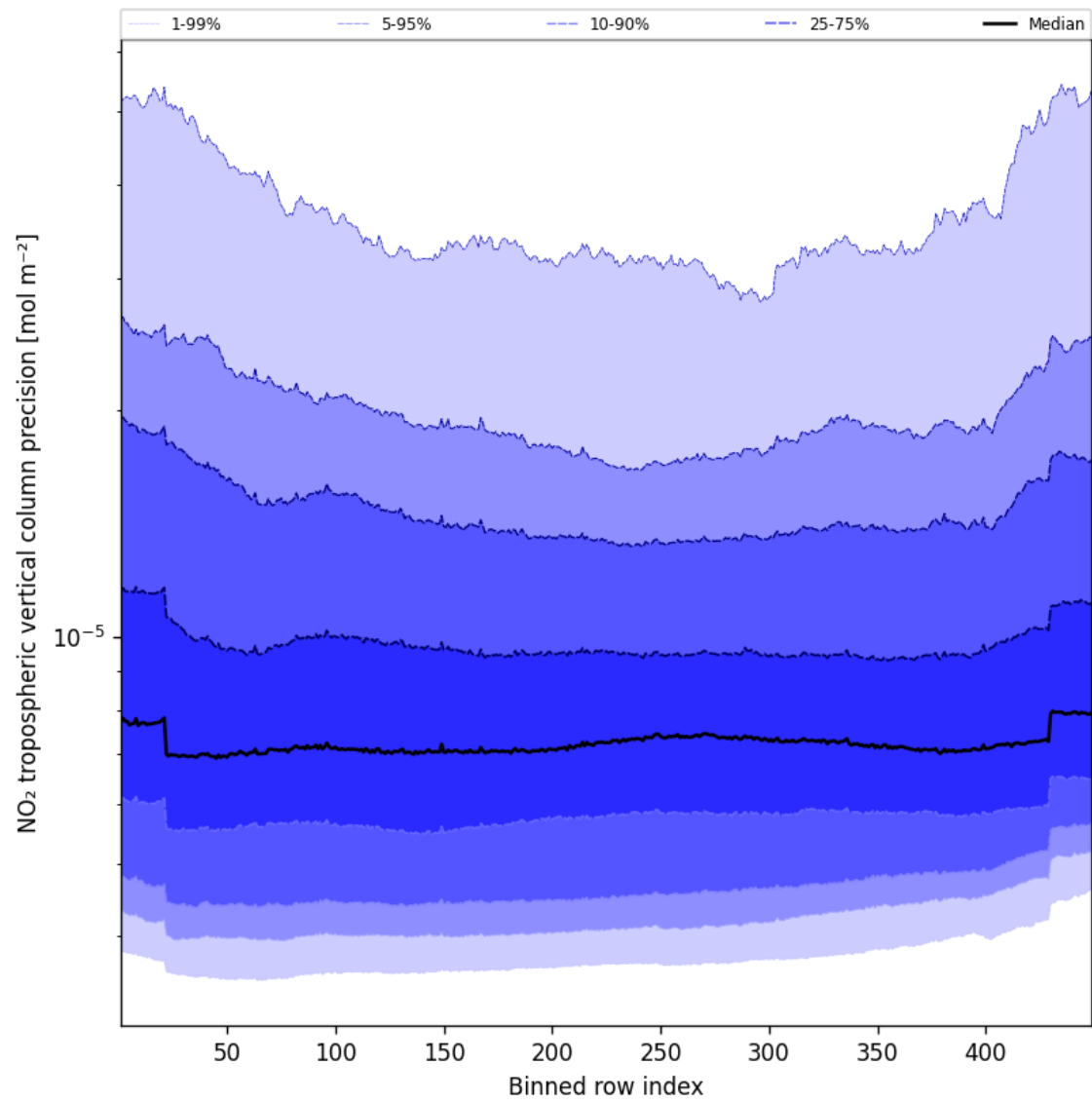
Figure 45: Along track statistics of “NO 2 tropospheric vertical column precision” for 2025-09-13 to 2025-09-13
