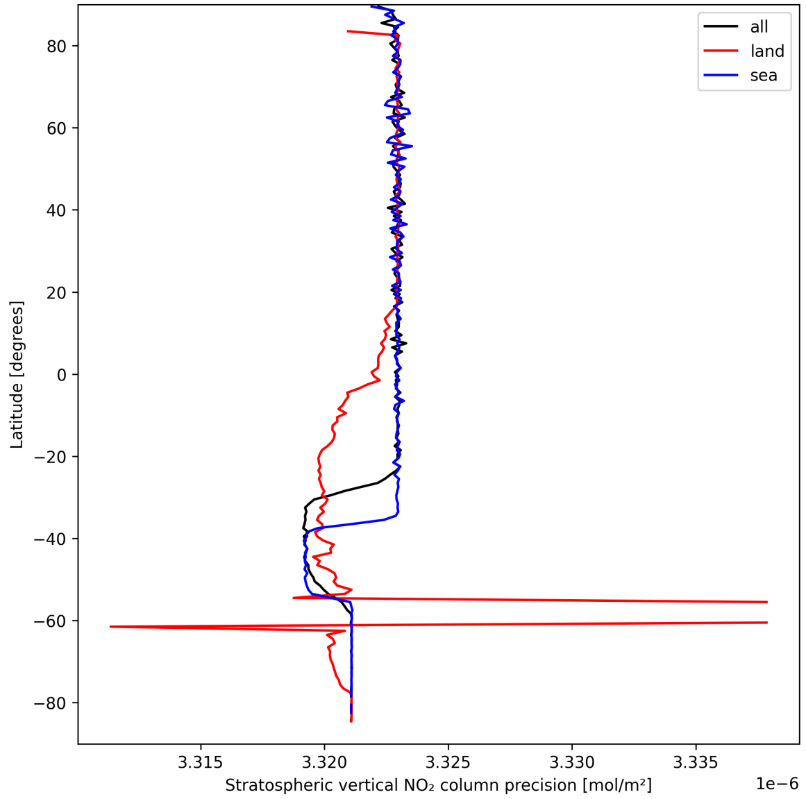
Figure 18: Zonal average of “Stratospheric vertical NO 2 column precision” for 2025-09-13 to 2025-09-13.
