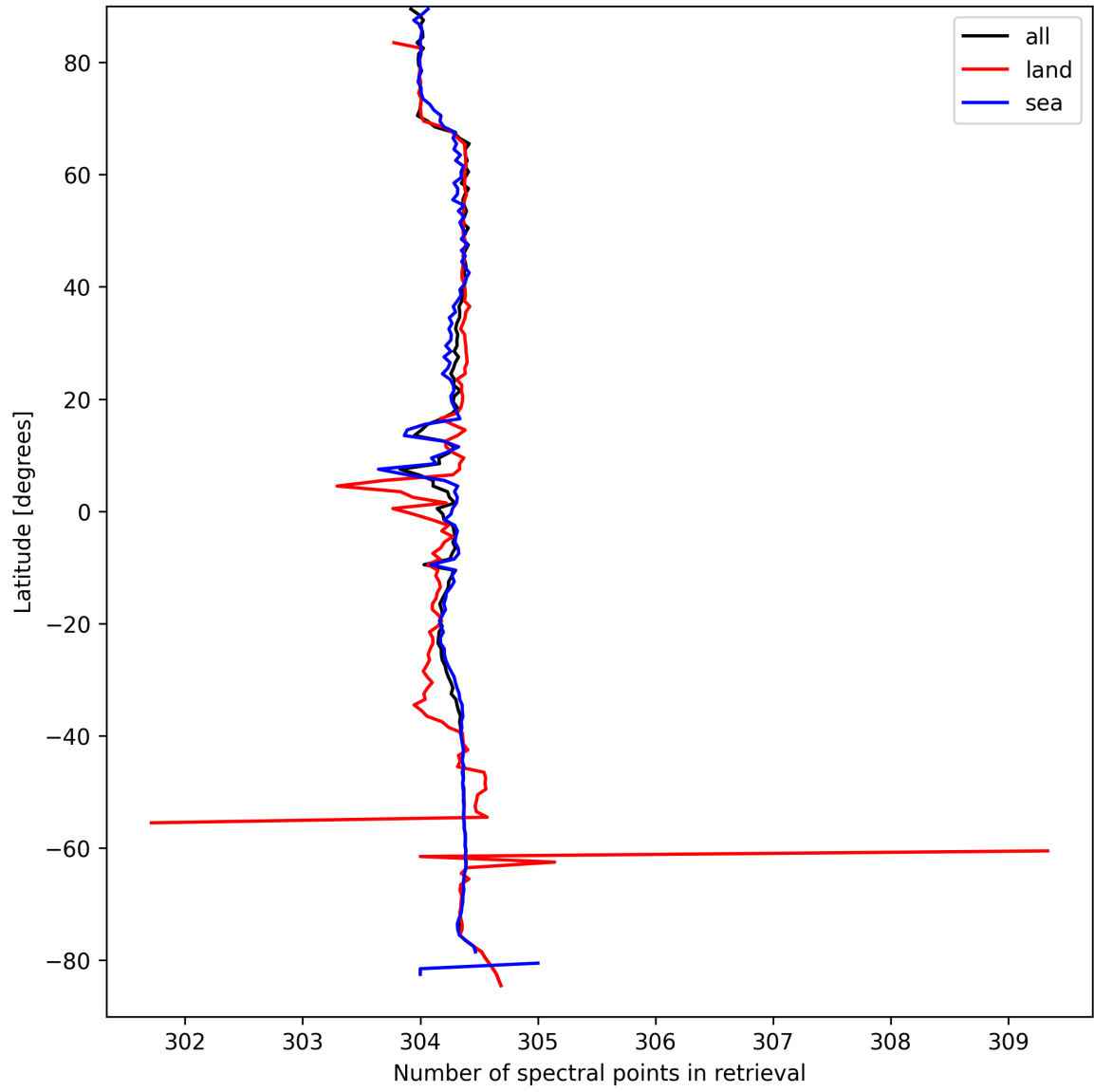
Figure 14: Zonal average of “Number of spectral points in retrieval” for 2025-09-13 to 2025-09-13.
