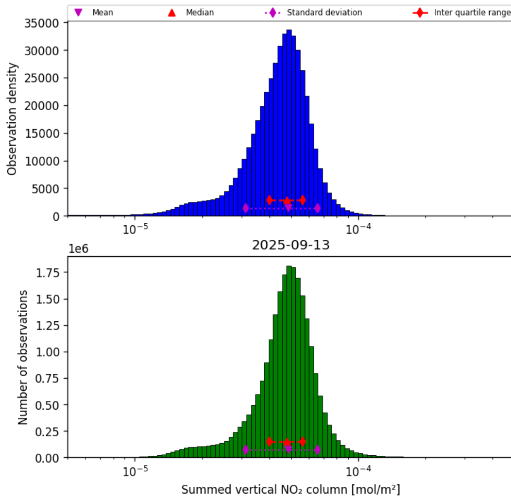
Figure 38: Histogram of “Summed vertical NO 2 column” for 2025-09-13 to 2025-09-13
