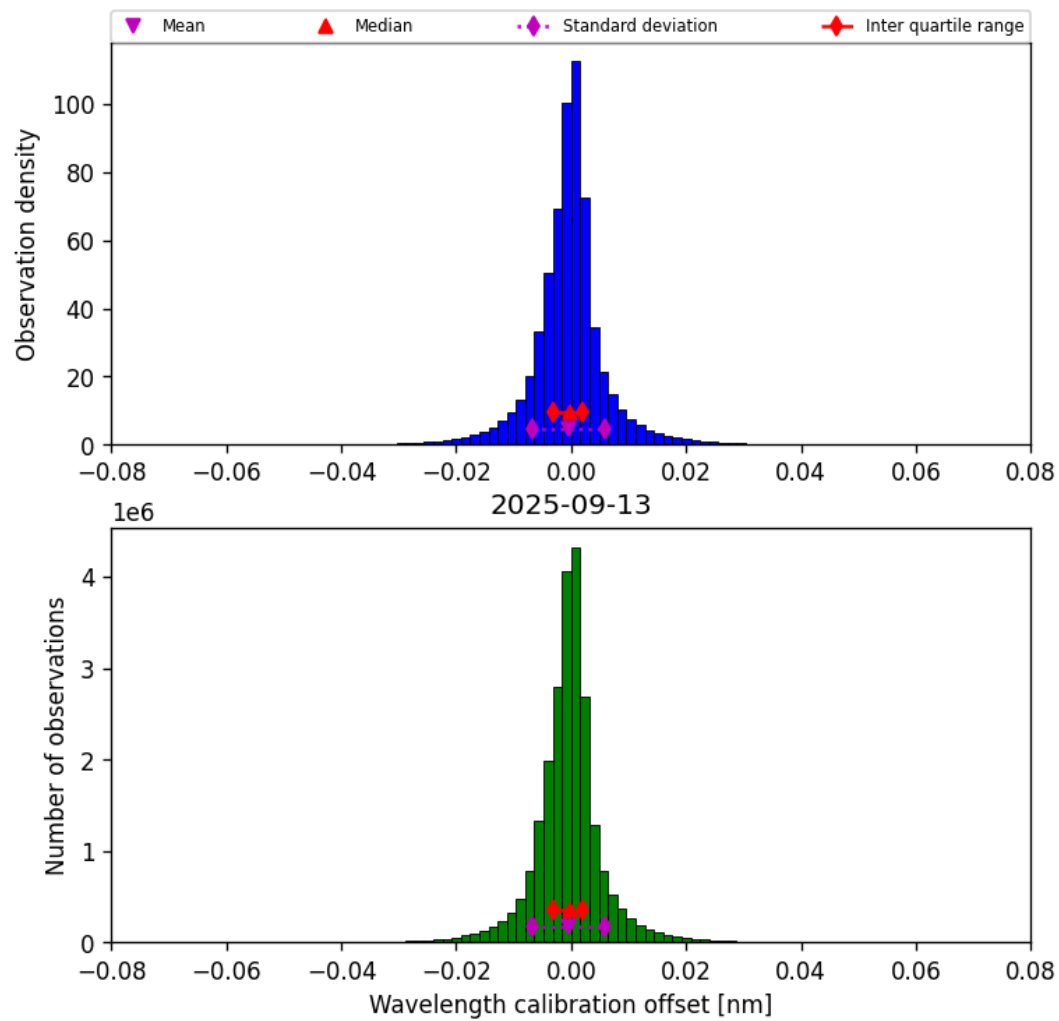
Figure 33: Histogram of “Wavelength calibration offset” for 2025-09-13 to 2025-09-13
