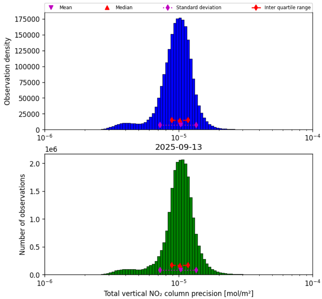
Figure 37: Histogram of “Total vertical NO 2 column precision” for 2025-09-13 to 2025-09-13
