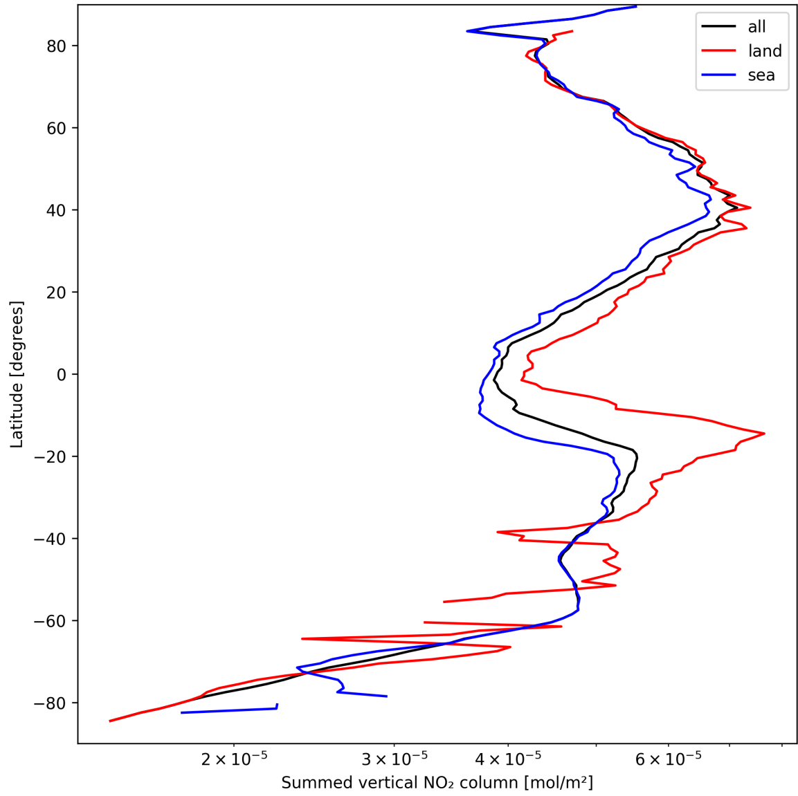
Figure 21: Zonal average of “Summed vertical NO 2 column” for 2025-09-13 to 2025-09-13.
