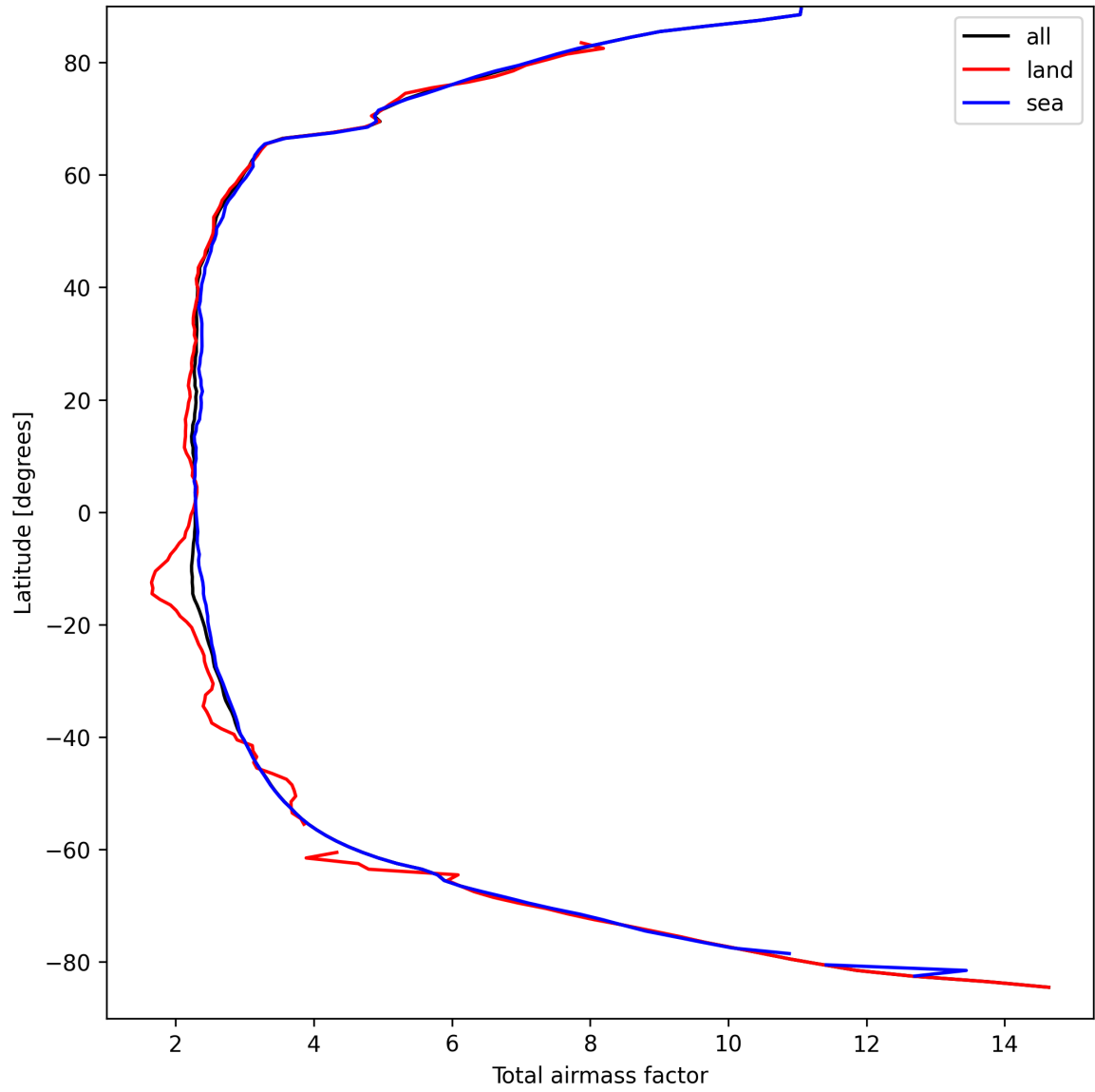
Figure 13: Zonal average of “Total airmass factor” for 2025-09-13 to 2025-09-13.
