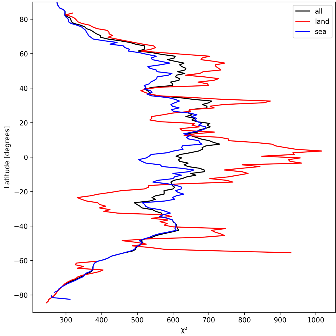
Figure 23: Zonal average of “ \chi^2 ” for 2025-09-13 to 2025-09-13.
