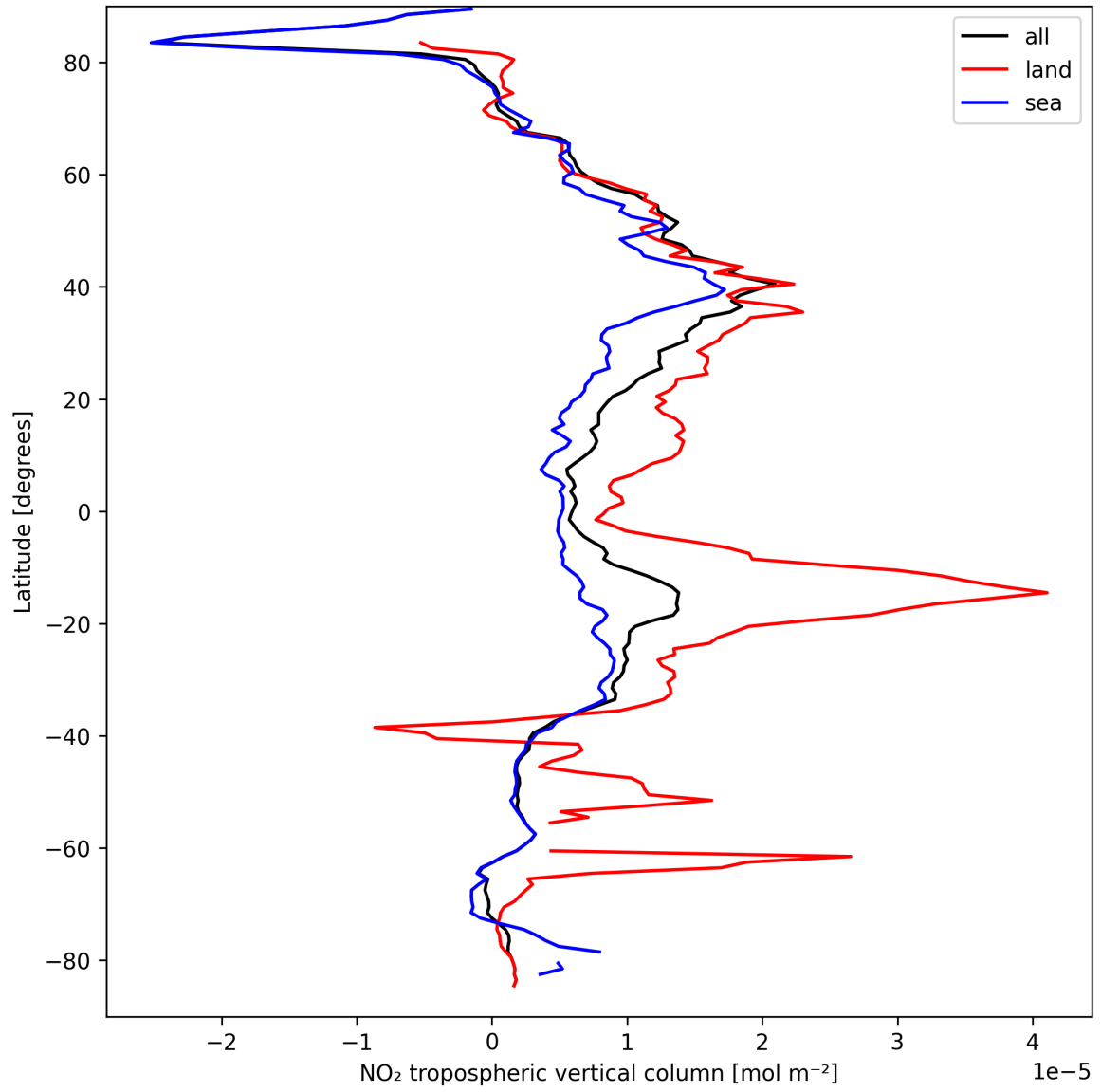
Figure 10: Zonal average of “NO 2 tropospheric vertical column” for 2025-09-13 to 2025-09-13.
