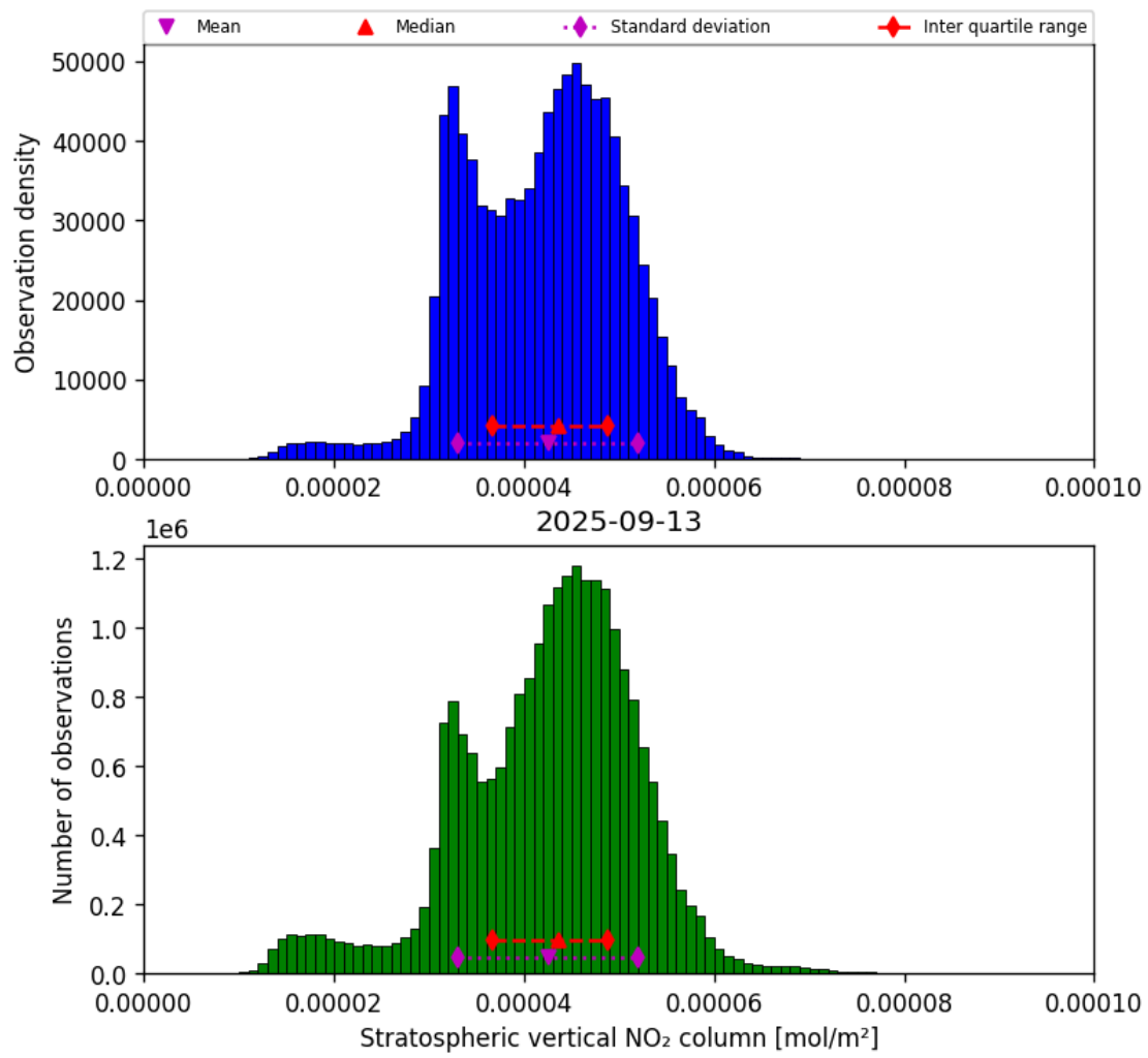
Figure 34: Histogram of “Stratospheric vertical NO 2 column” for 2025-09-13 to 2025-09-13
