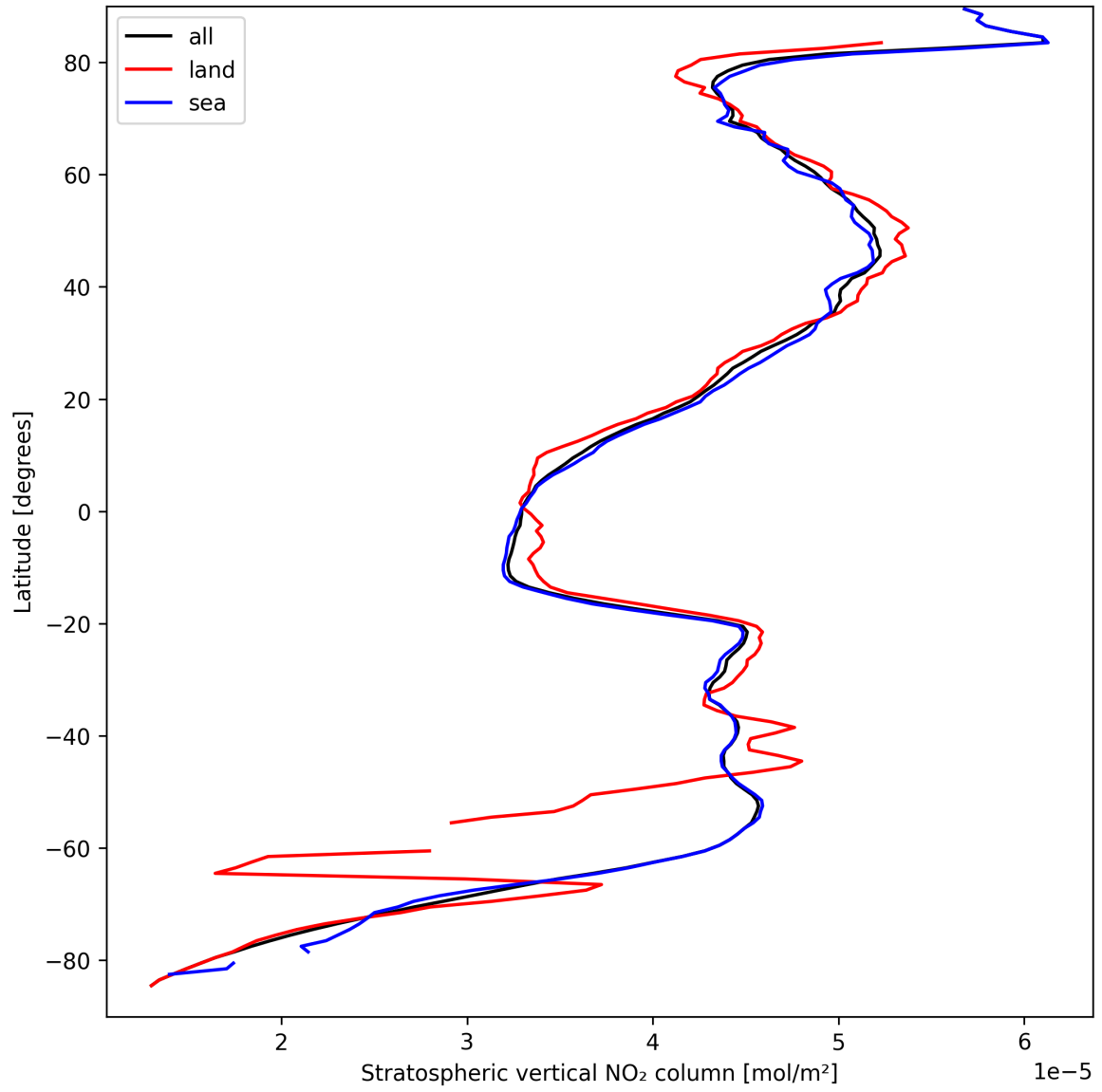
Figure 17: Zonal average of “Stratospheric vertical NO 2 column” for 2025-09-13 to 2025-09-13.
