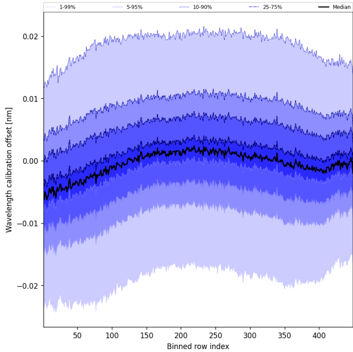
Figure 50: Along track statistics of “Wavelength calibration offset” for 2025-09-13 to 2025-09-13
