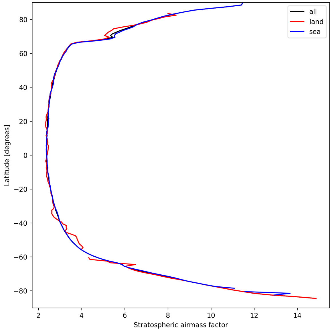
Figure 25: Zonal average of “Stratospheric airmass factor” for 2025-09-13 to 2025-09-13.
