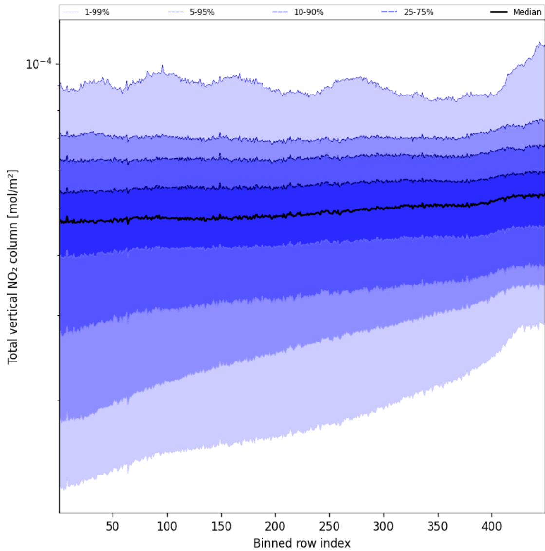
Figure 53: Along track statistics of “Total vertical NO 2 column” for 2025-09-13 to 2025-09-13
