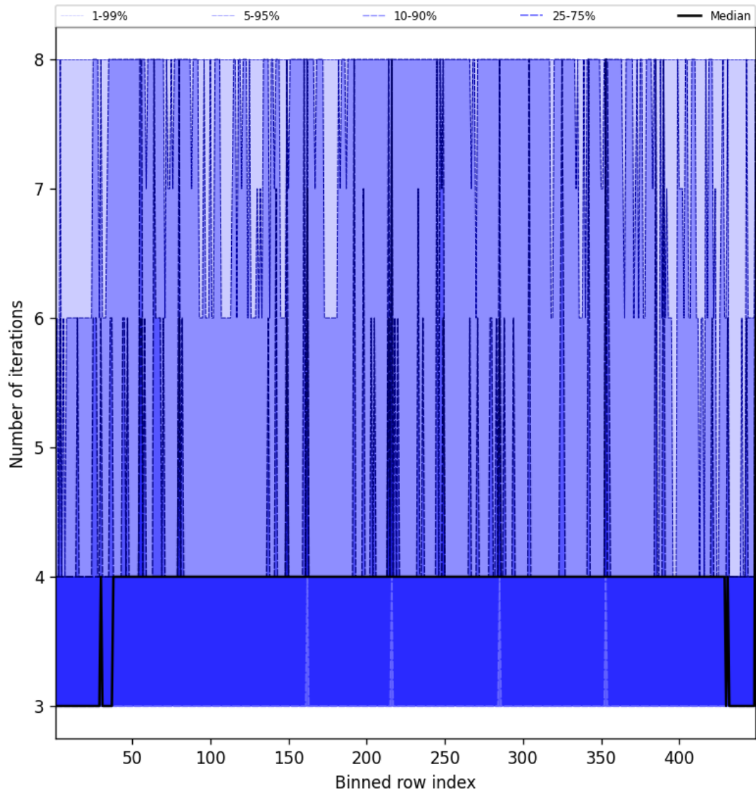
Figure 49: Along track statistics of “Number of iterations” for 2025-09-13 to 2025-09-13
