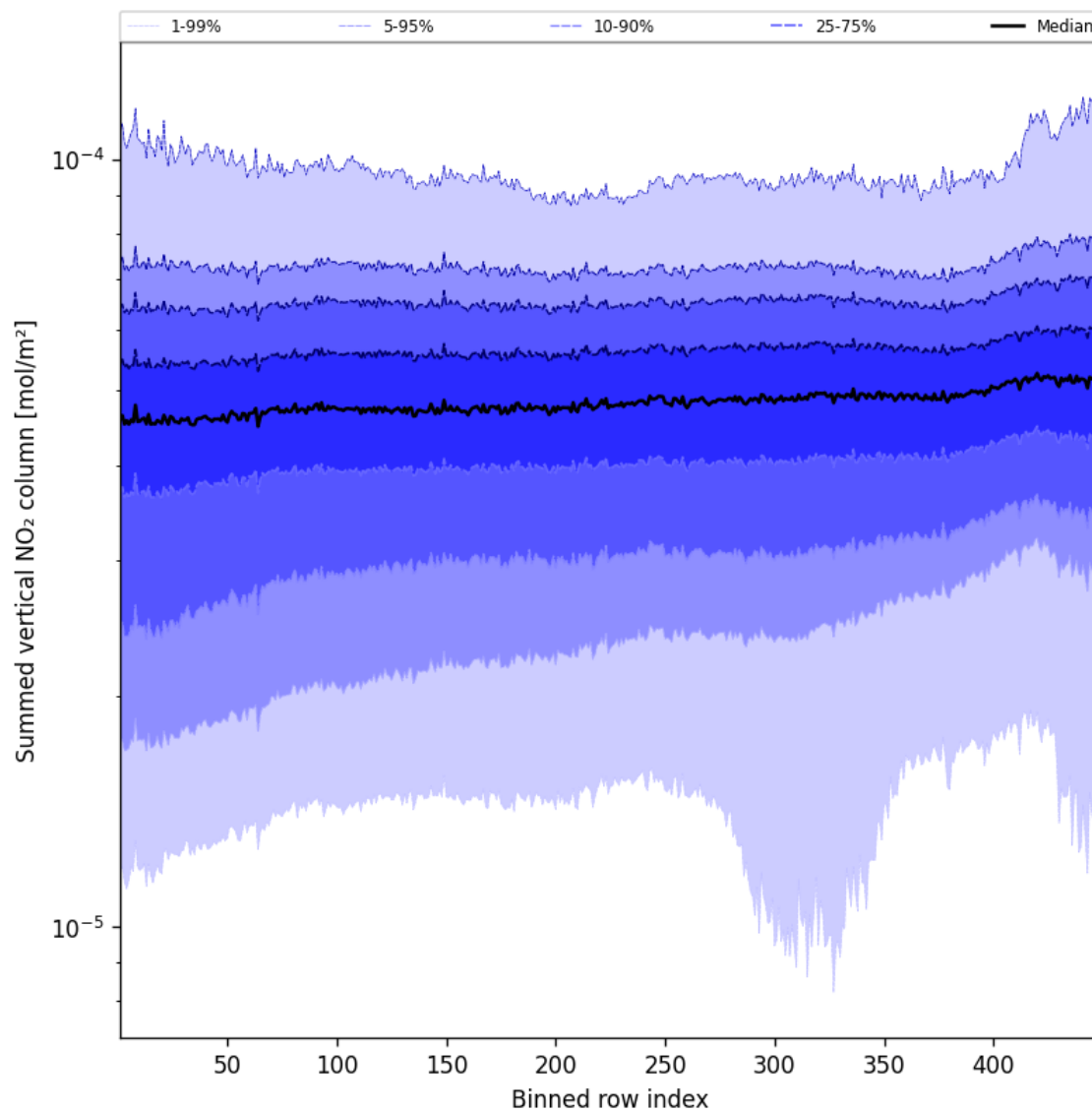
Figure 55: Along track statistics of “Summed vertical NO 2 column” for 2025-09-13 to 2025-09-13
