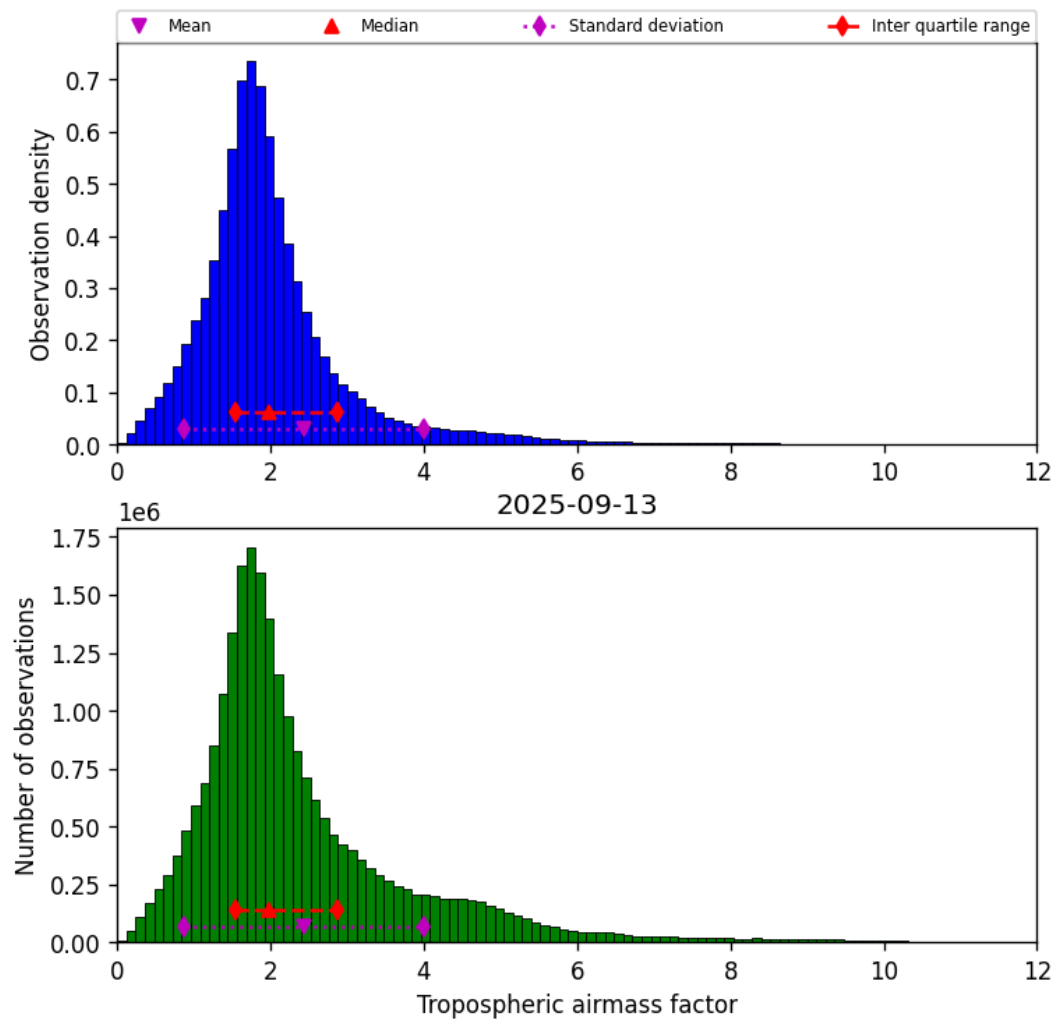
Figure 29: Histogram of “Tropospheric airmass factor” for 2025-09-13 to 2025-09-13
