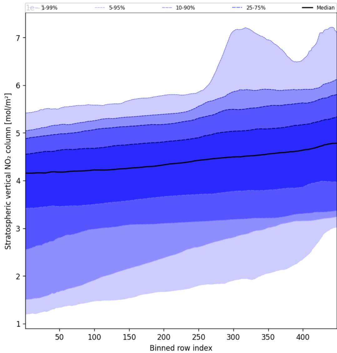
Figure 51: Along track statistics of “Stratospheric vertical NO 2 column” for 2025-09-13 to 2025-09-13
