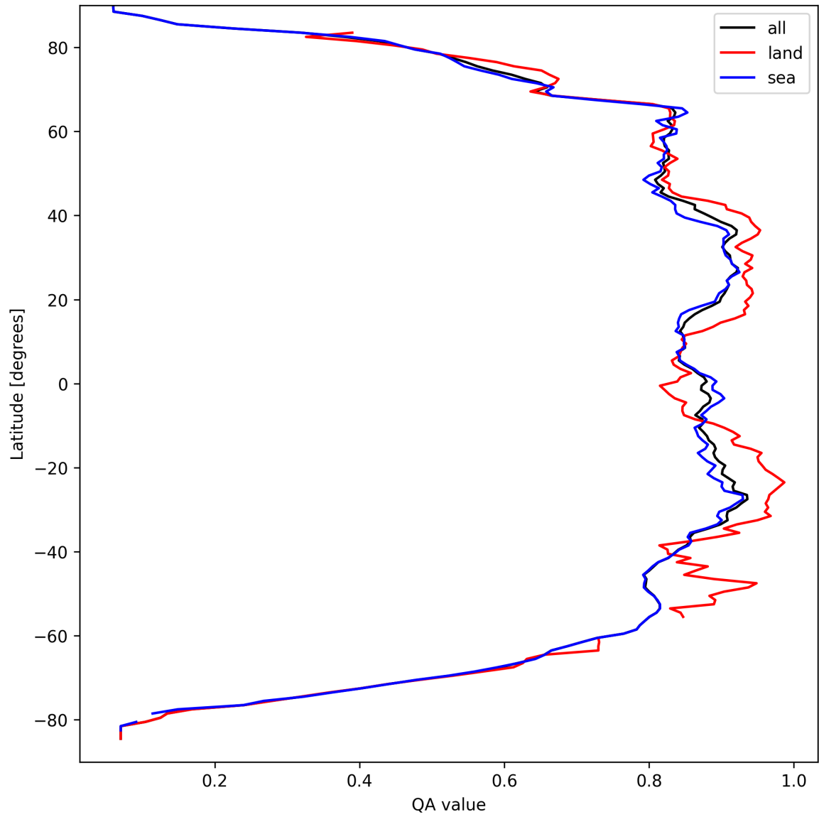
Figure 9: Zonal average of “QA value” for 2025-09-13 to 2025-09-13.
