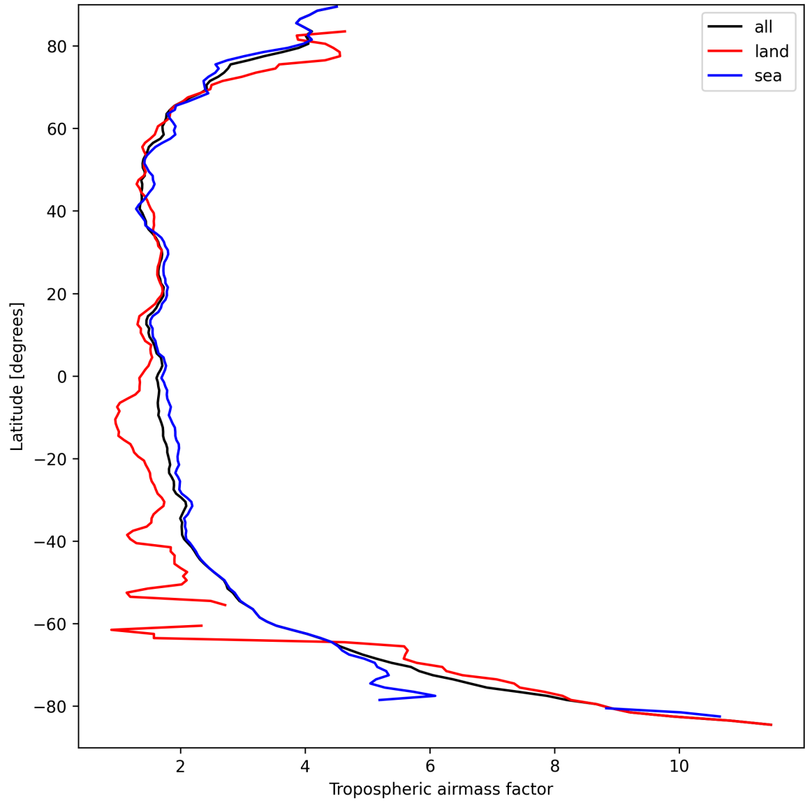
Figure 12: Zonal average of “Tropospheric airmass factor” for 2025-09-13 to 2025-09-13.
