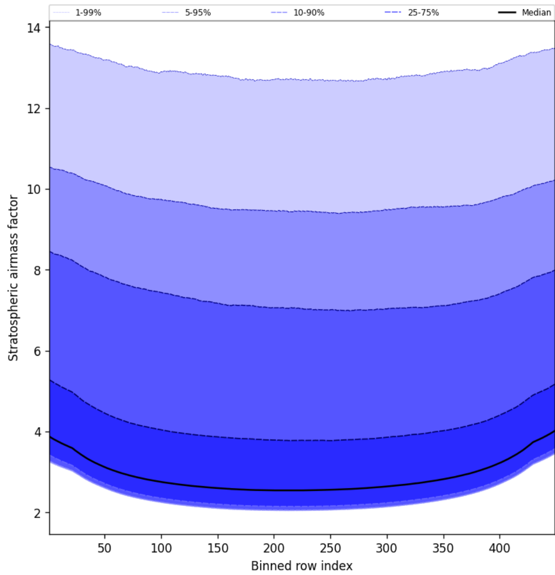
Figure 59: Along track statistics of “Stratospheric airmass factor” for 2025-09-13 to 2025-09-13
