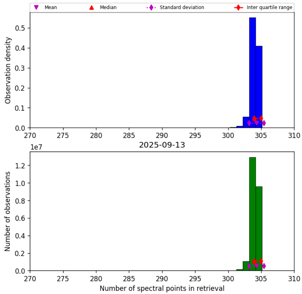
Figure 31: Histogram of “Number of spectral points in retrieval” for 2025-09-13 to 2025-09-13
