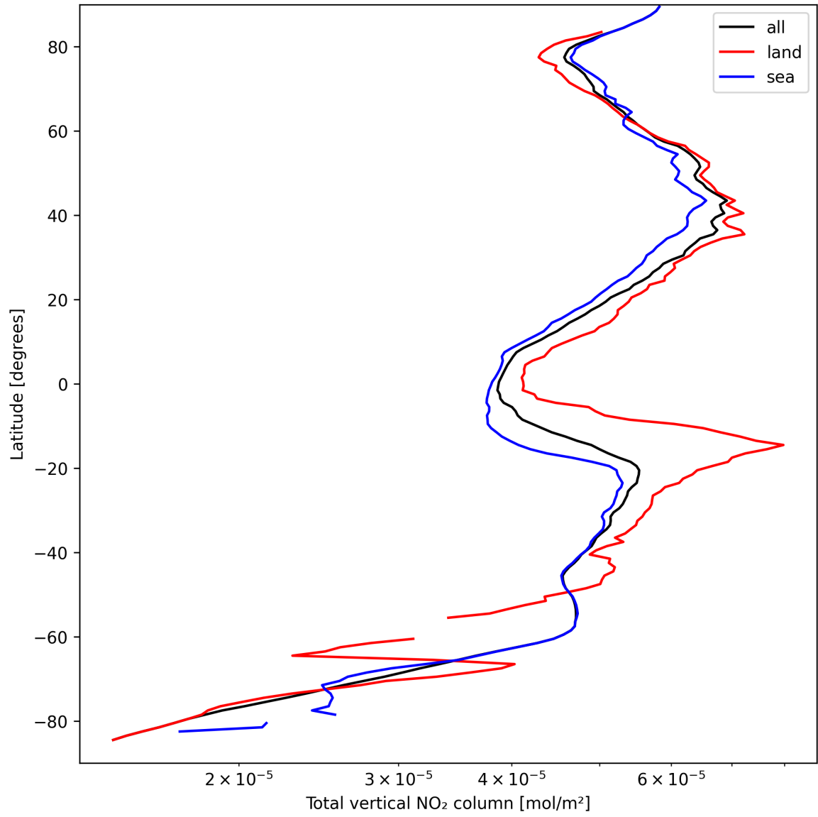
Figure 19: Zonal average of “Total vertical NO 2 column” for 2025-09-13 to 2025-09-13.
