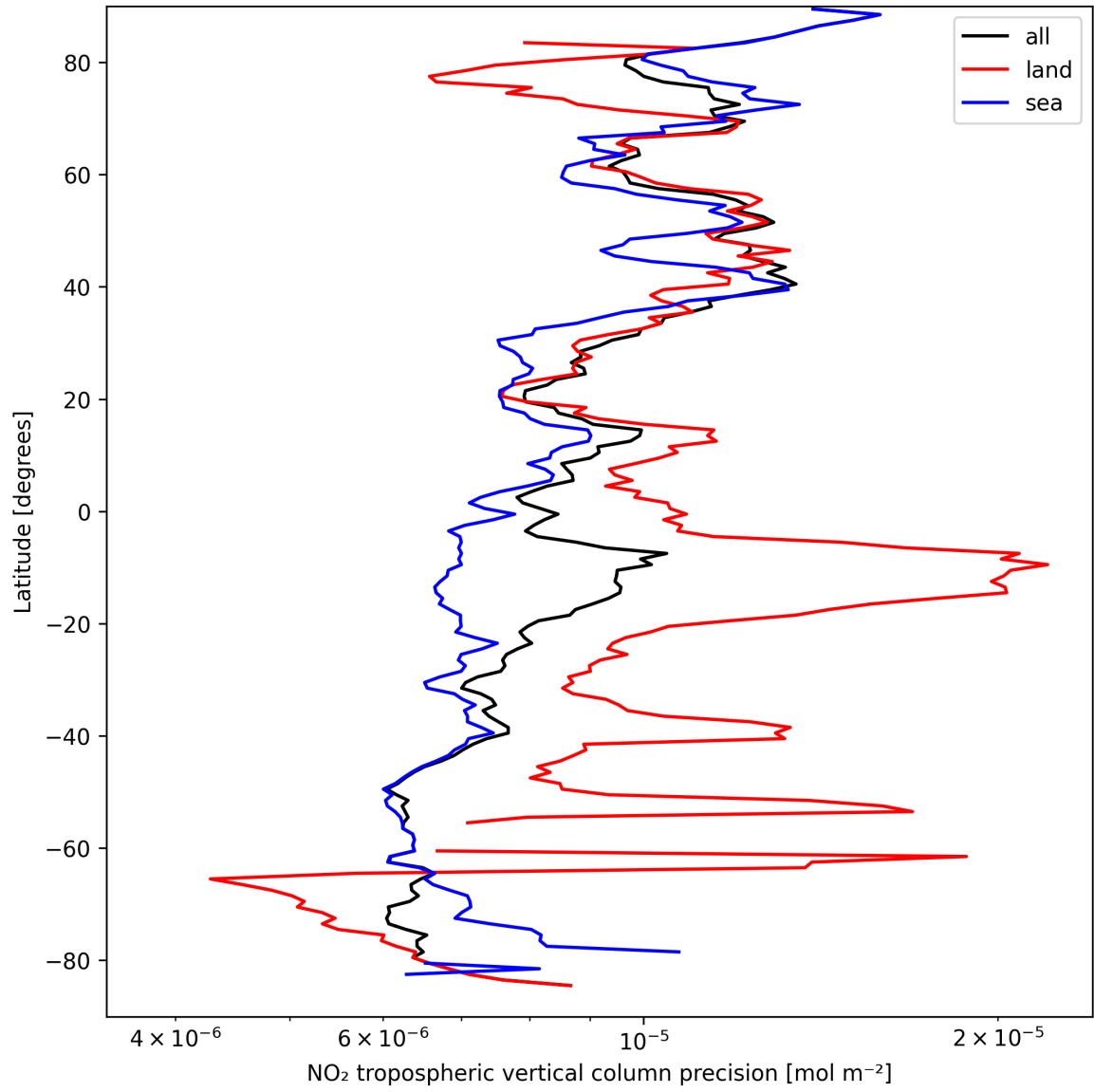
Figure 11: Zonal average of “NO 2 tropospheric vertical column precision” for 2025-09-13 to 2025-09-13.
