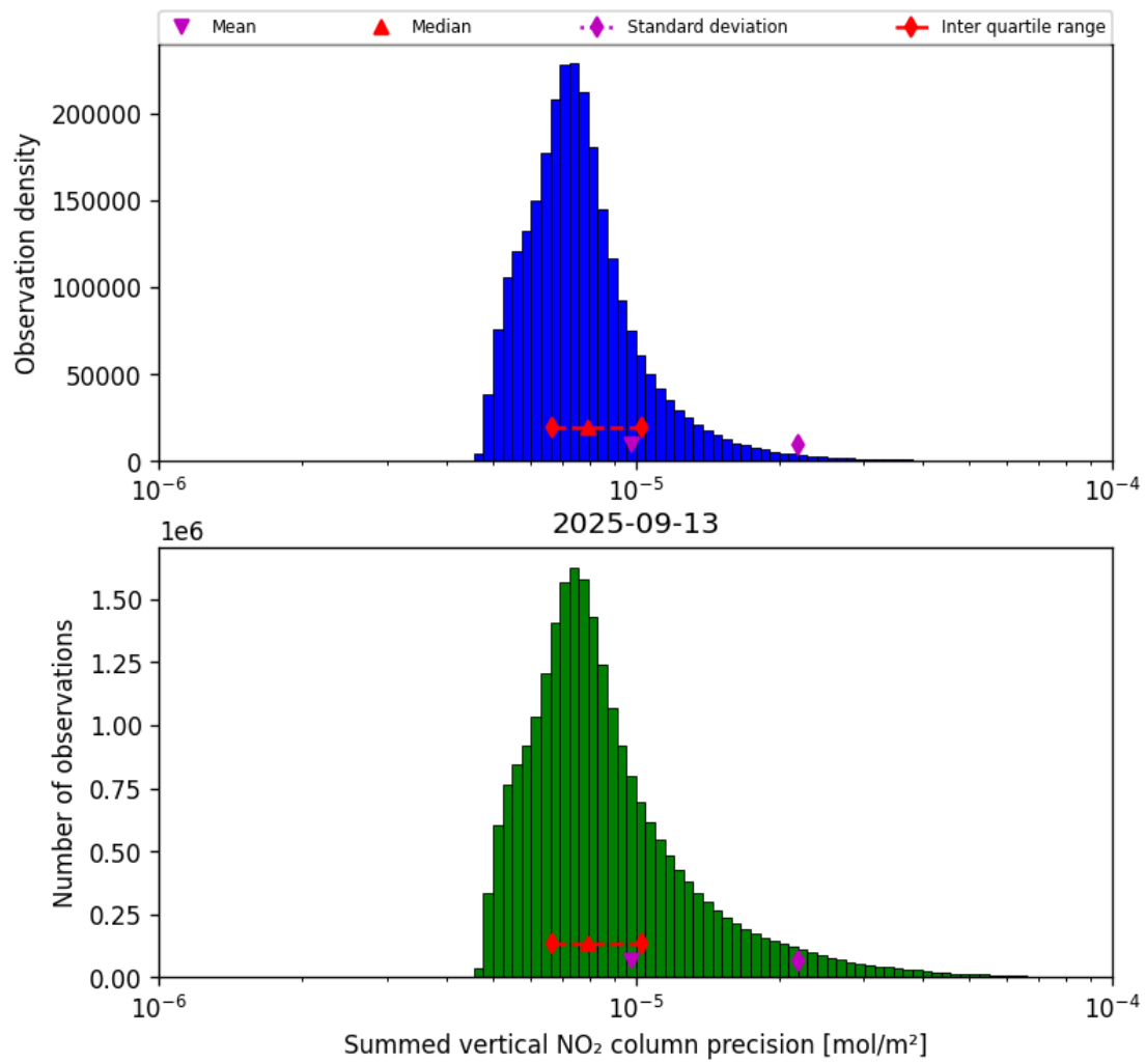
Figure 39: Histogram of "Summed vertical NO 2 column precision" for 2025-09-13 to 2025-09-13
