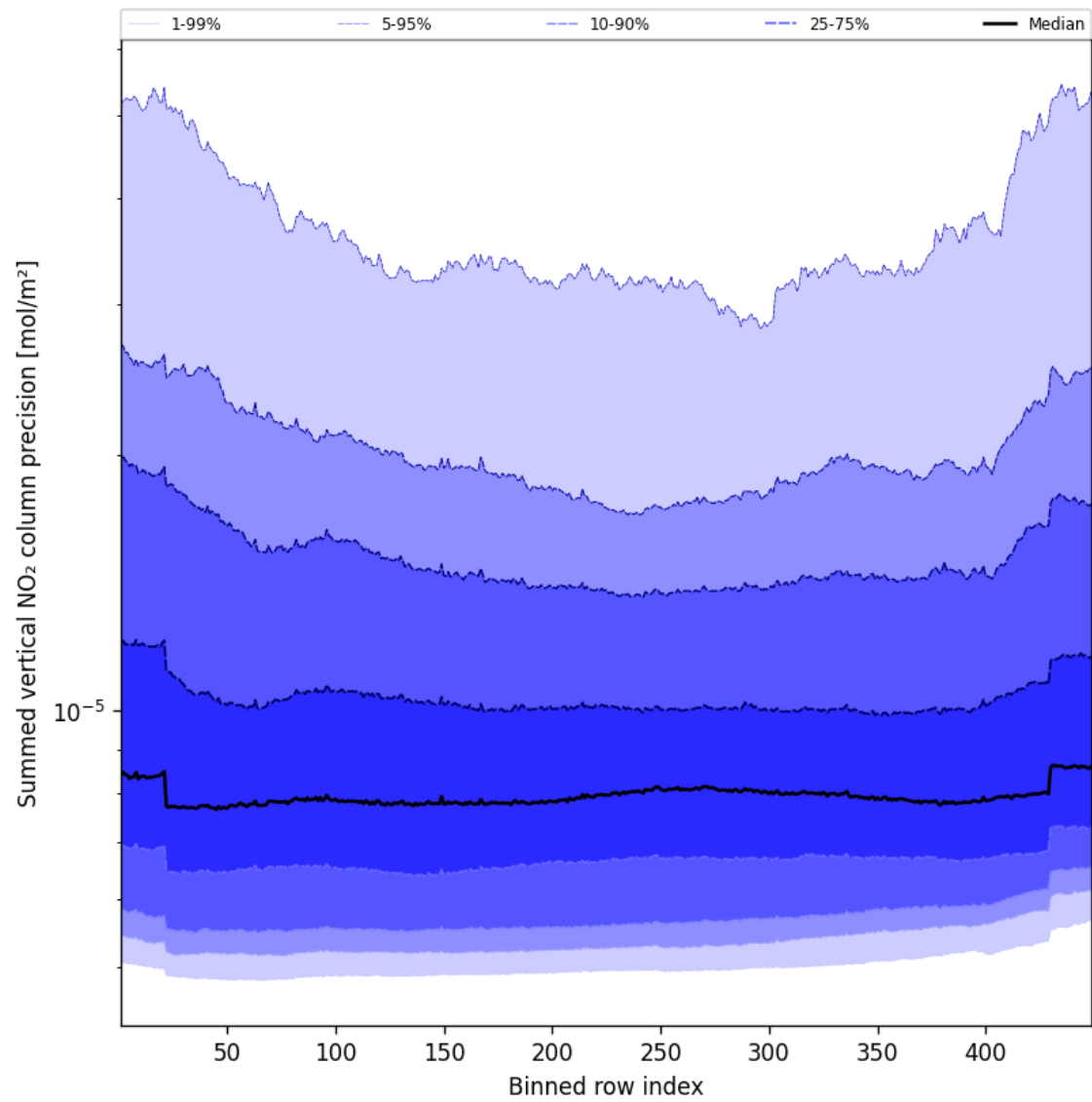
Figure 56: Along track statistics of “Summed vertical NO 2 column precision” for 2025-09-13 to 2025-09-13
