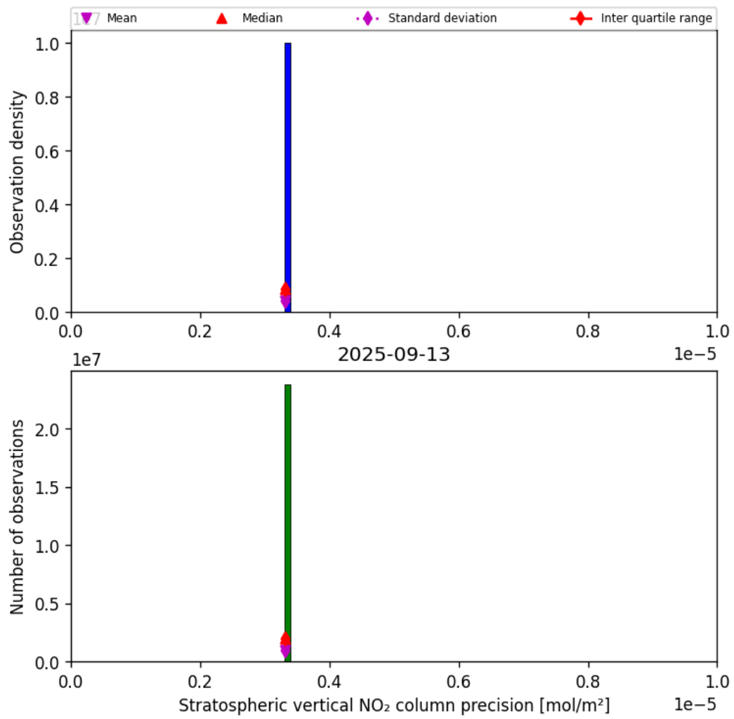
Figure 35: Histogram of “Stratospheric vertical NO 2 column precision” for 2025-09-13 to 2025-09-13
