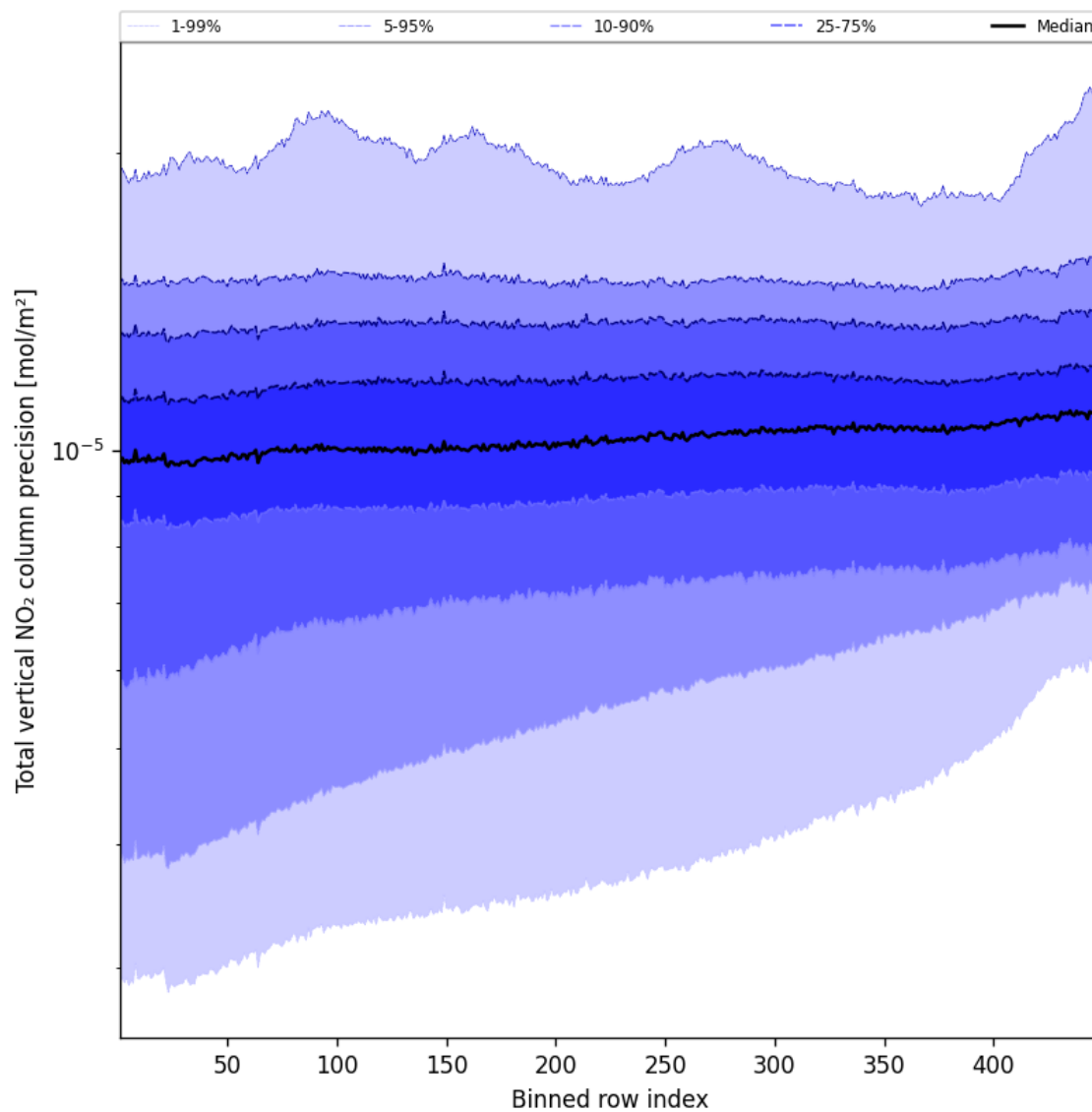
Figure 54: Along track statistics of “Total vertical NO 2 column precision” for 2025-09-13 to 2025-09-13
