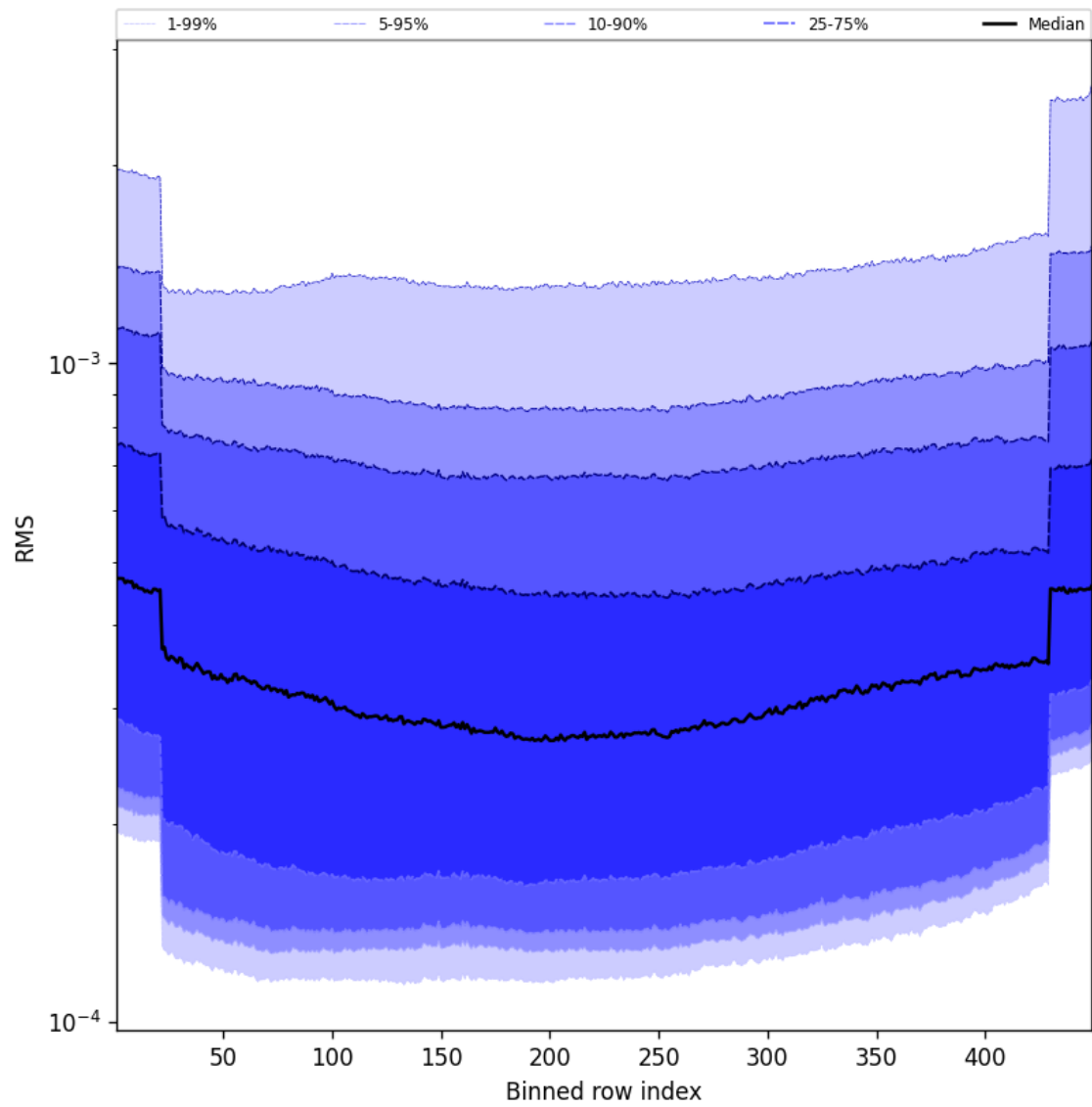
Figure 58: Along track statistics of “RMS” for 2025-09-13 to 2025-09-13
