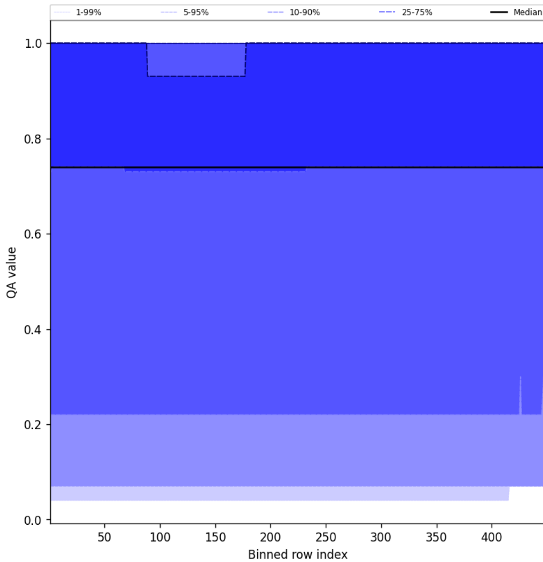
Figure 43: Along track statistics of “QA value” for 2025-09-13 to 2025-09-13
