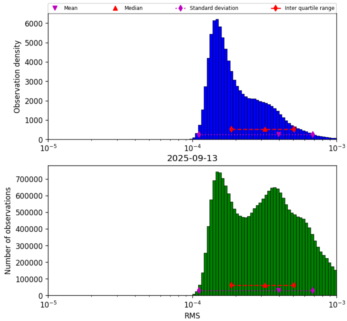
Figure 41: Histogram of “RMS” for 2025-09-13 to 2025-09-13
