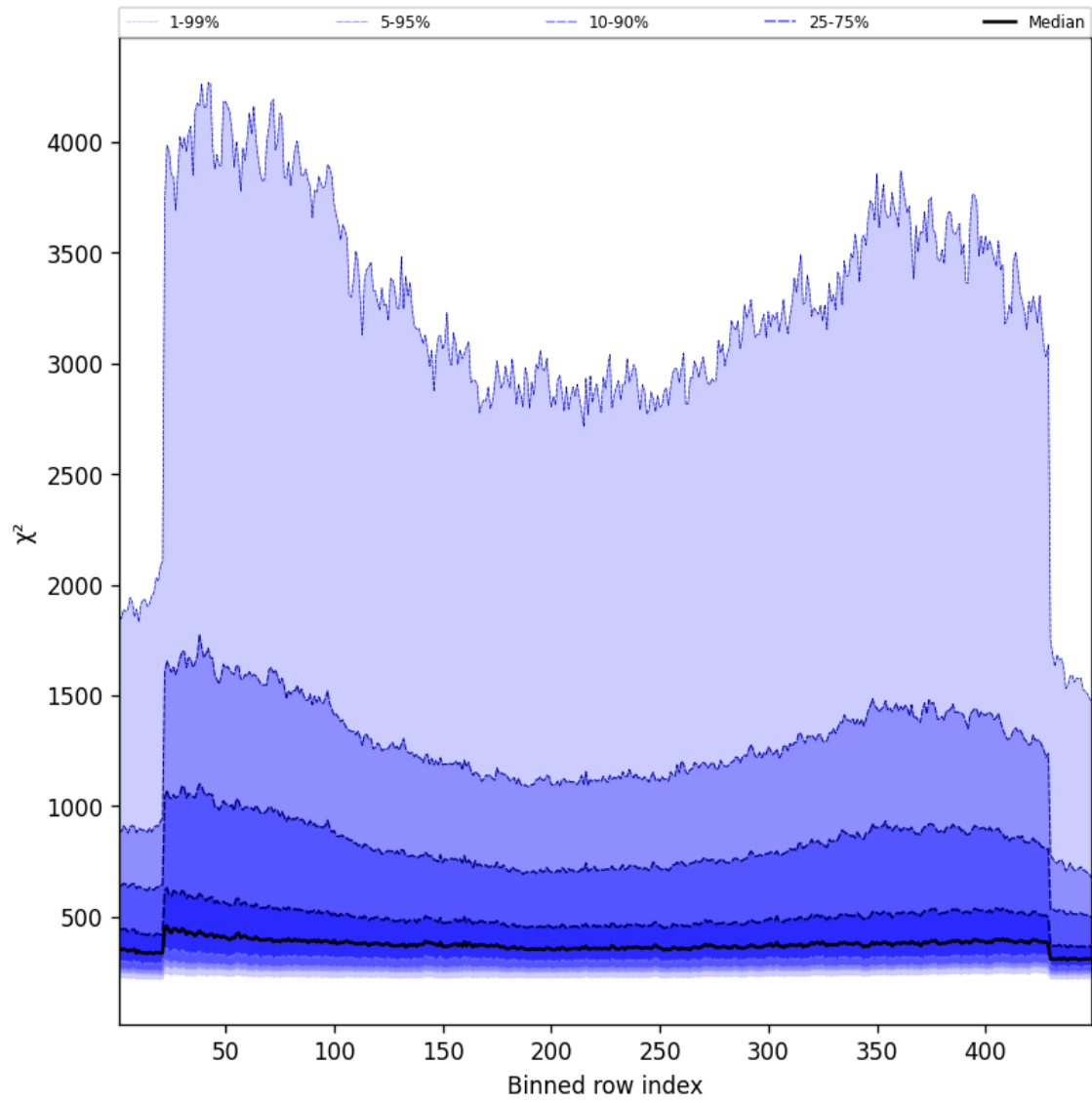
Figure 57: Along track statistics of “ \chi^2 ” for 2025-09-13 to 2025-09-13
