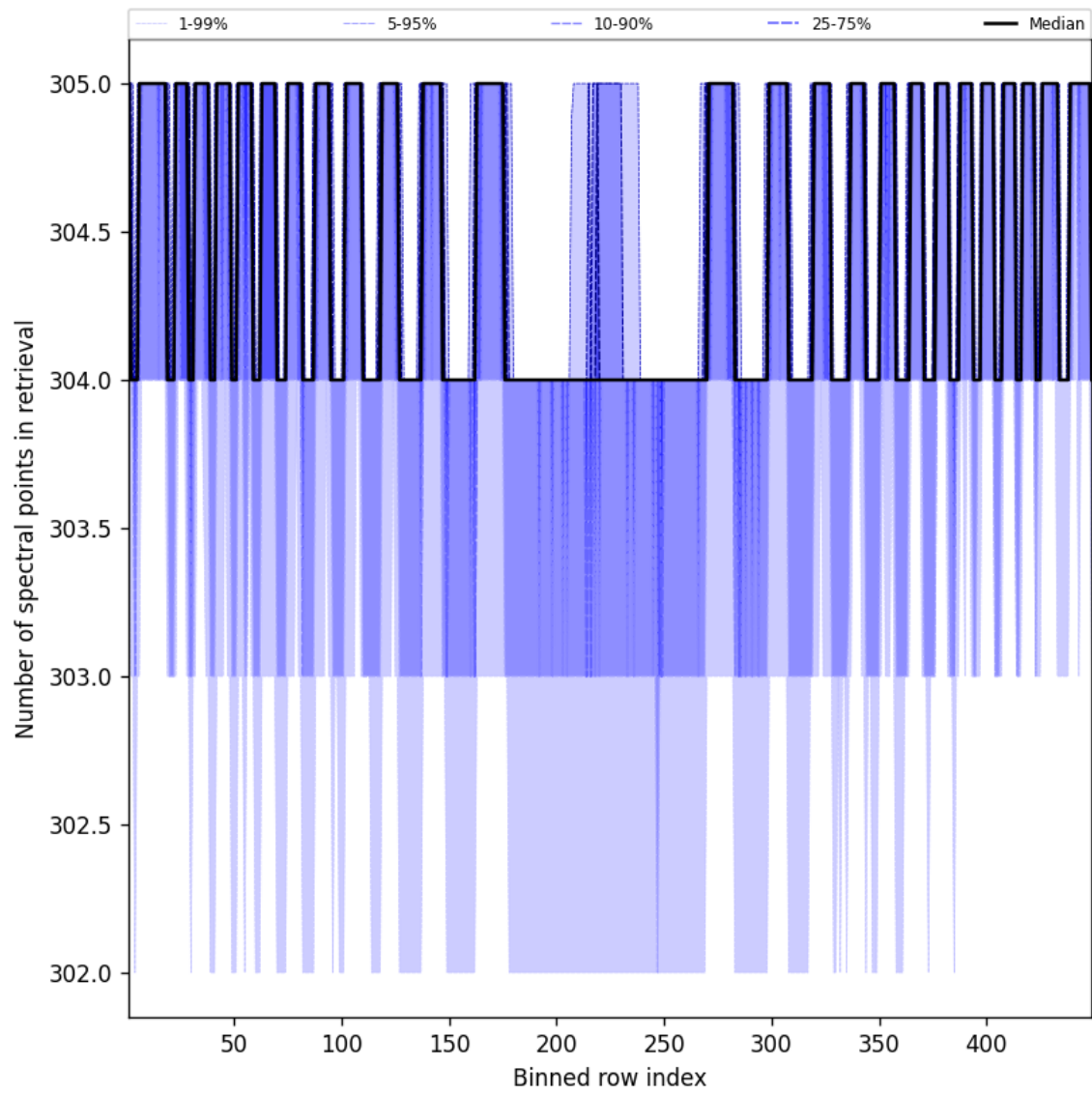
Figure 48: Along track statistics of “Number of spectral points in retrieval” for 2025-09-13 to 2025-09-13
