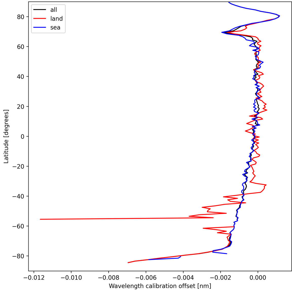
Figure 16: Zonal average of “Wavelength calibration offset” for 2025-09-13 to 2025-09-13.
