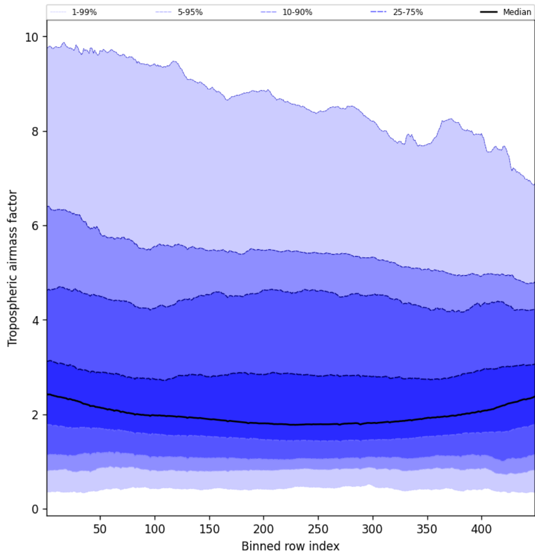
Figure 46: Along track statistics of “Tropospheric air mass factor” for 2025-09-13 to 2025-09-13
