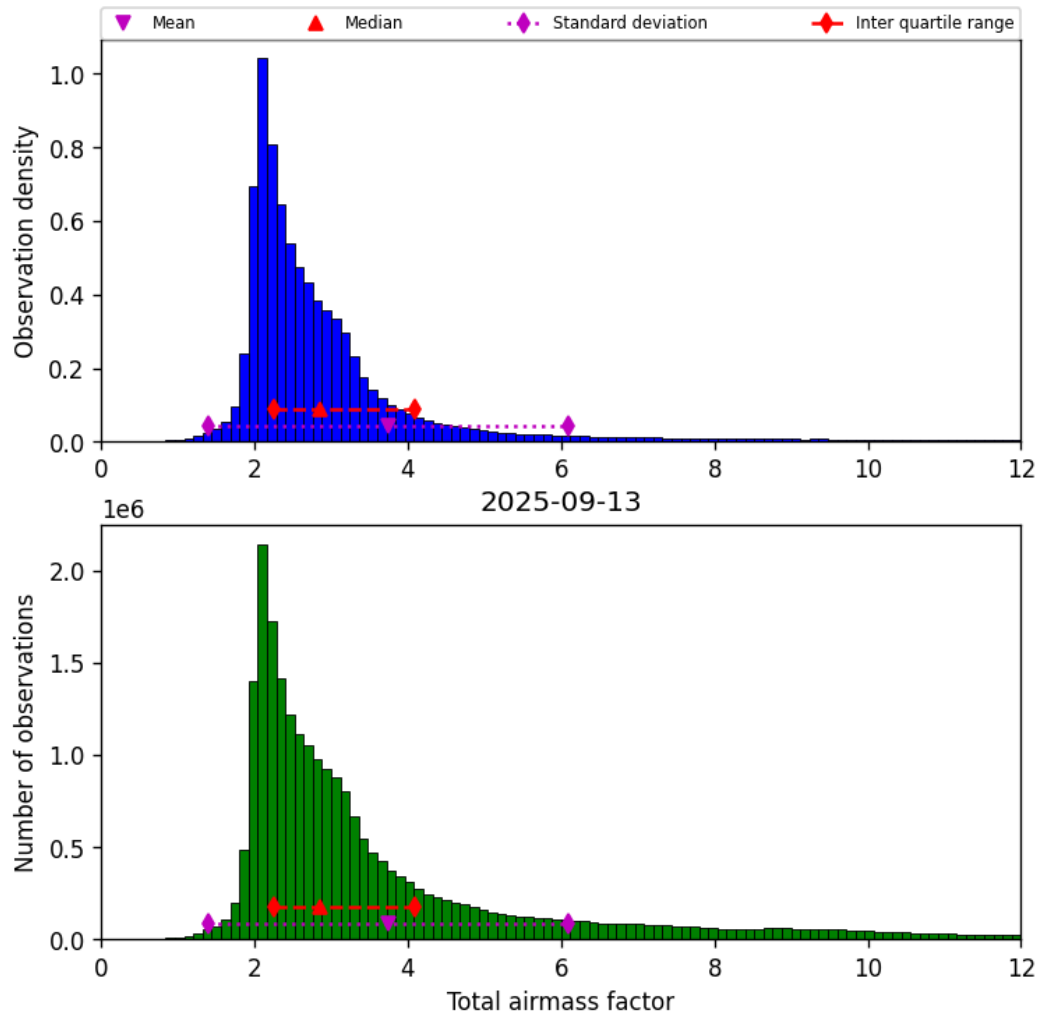
Figure 30: Histogram of “Total airmass factor” for 2025-09-13 to 2025-09-13
