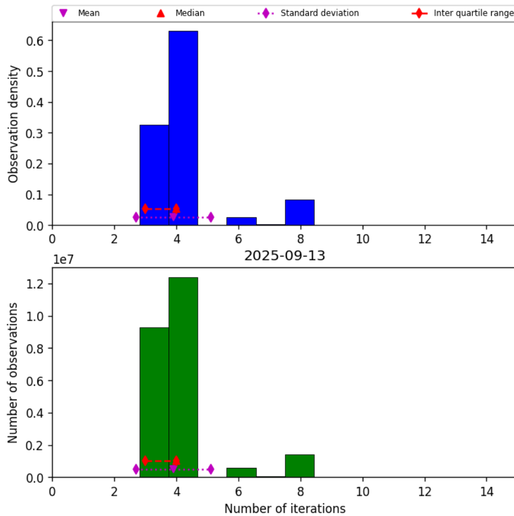
Figure 32: Histogram of “Number of iterations” for 2025-09-13 to 2025-09-13
