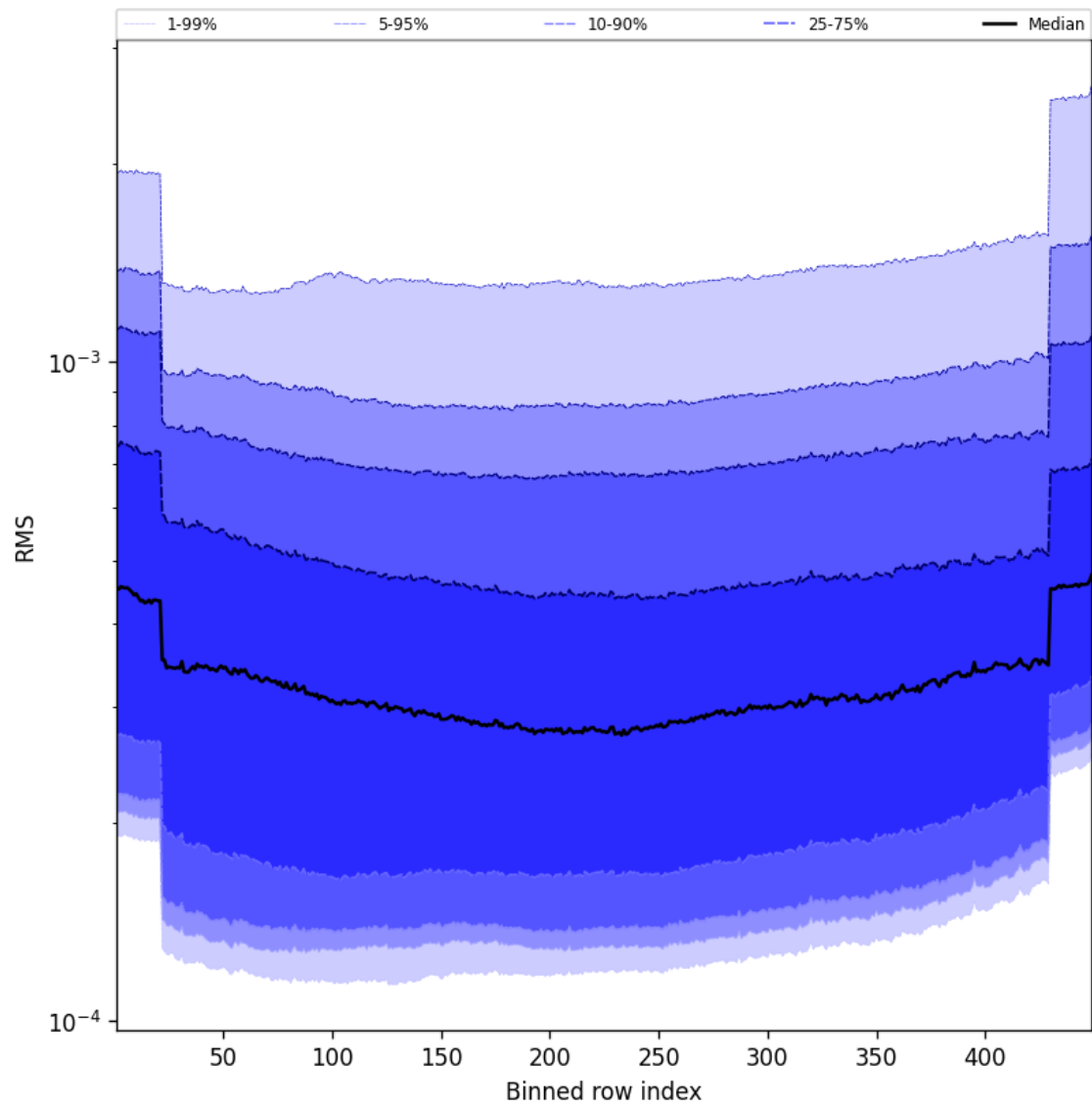
Figure 58: Along track statistics of “RMS” for 2025-09-14 to 2025-09-15
