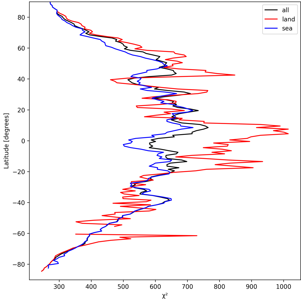
Figure 23: Zonal average of “ \chi^2 ” for 2025-09-14 to 2025-09-15.
