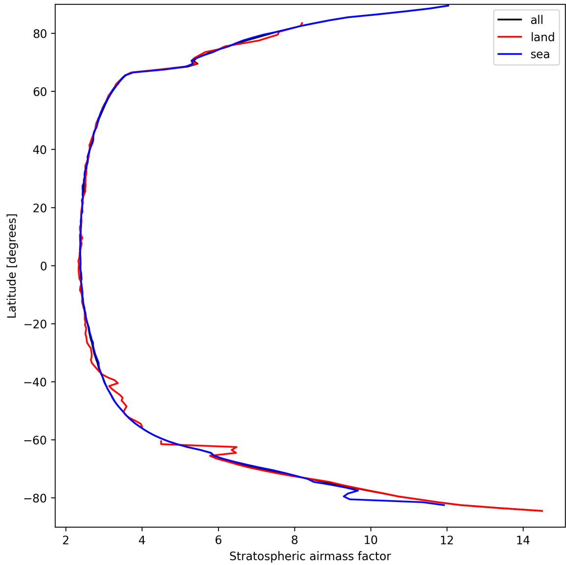
Figure 25: Zonal average of “Stratospheric airmass factor” for 2025-09-14 to 2025-09-15.
