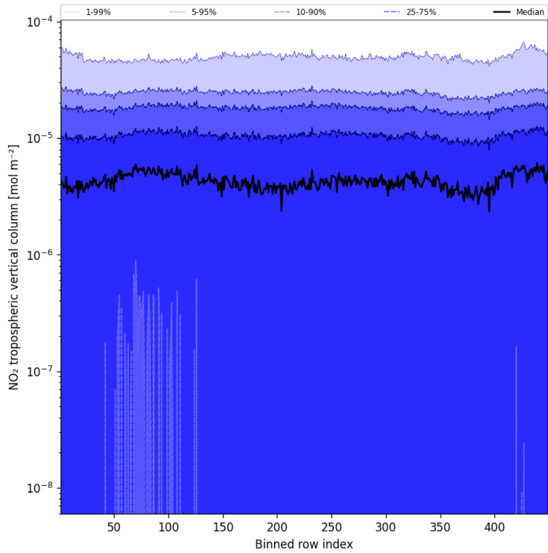
Figure 44: Along track statistics of “NO 2 tropospheric vertical column” for 2025-09-14 to 2025-09-15
