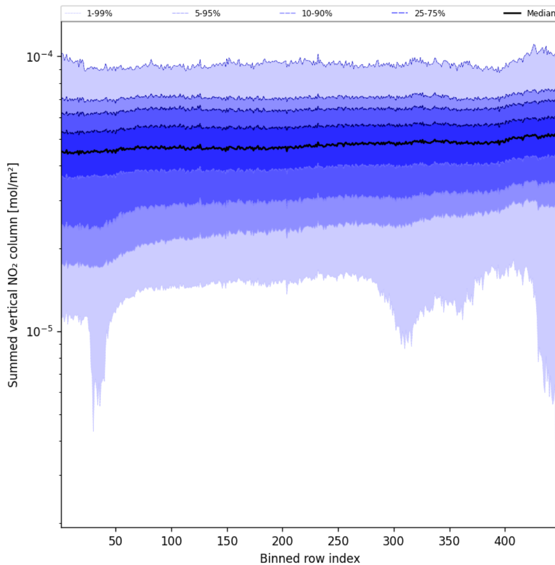
Figure 55: Along track statistics of “Summed vertical NO 2 column” for 2025-09-14 to 2025-09-15
