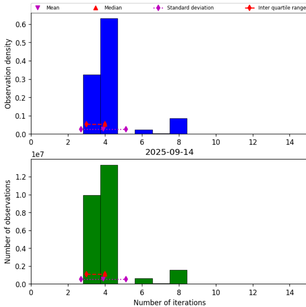
Figure 32: Histogram of “Number of iterations” for 2025-09-14 to 2025-09-15
