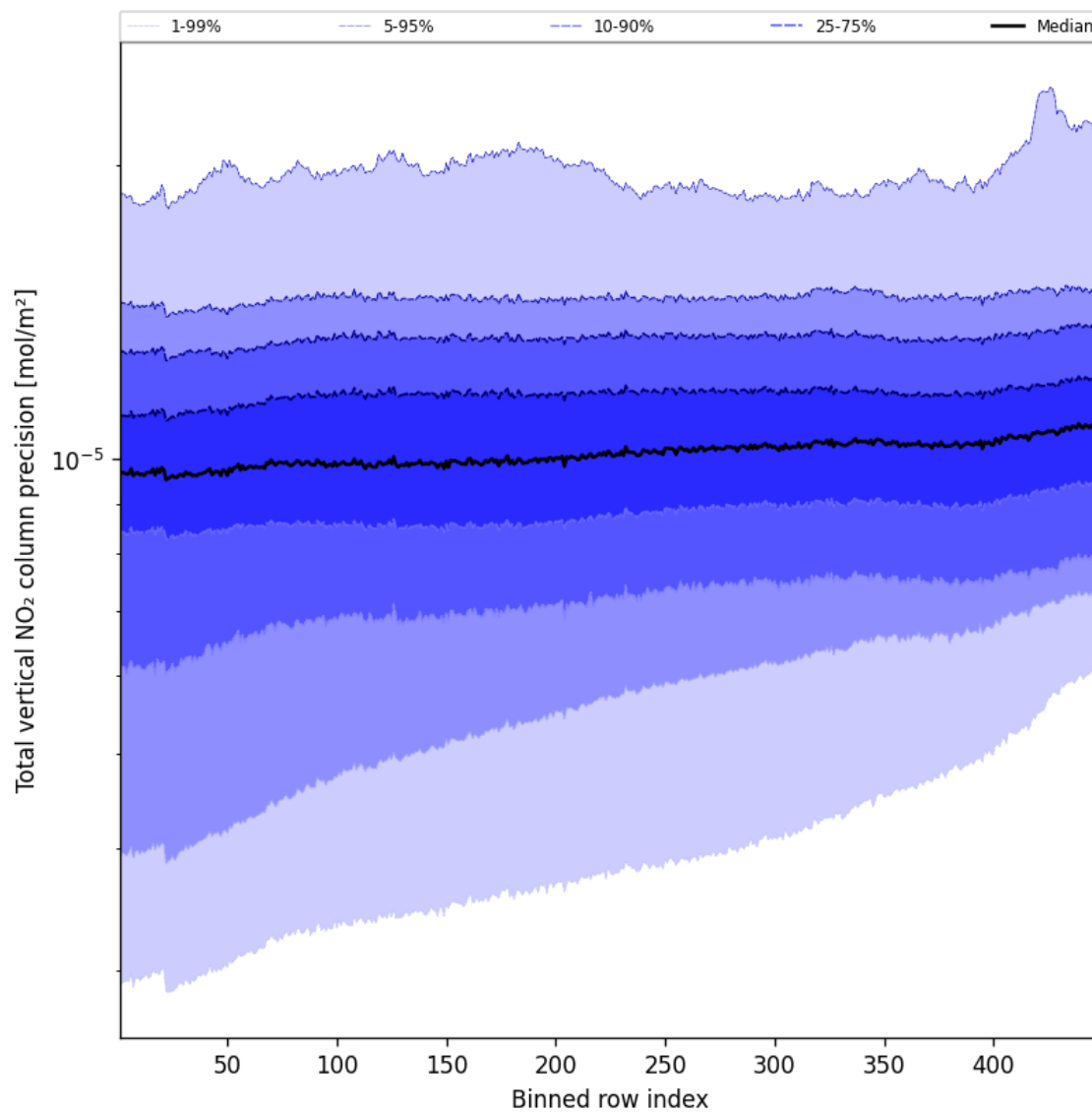
Figure 54: Along track statistics of “Total vertical NO 2 column precision” for 2025-09-14 to 2025-09-15
