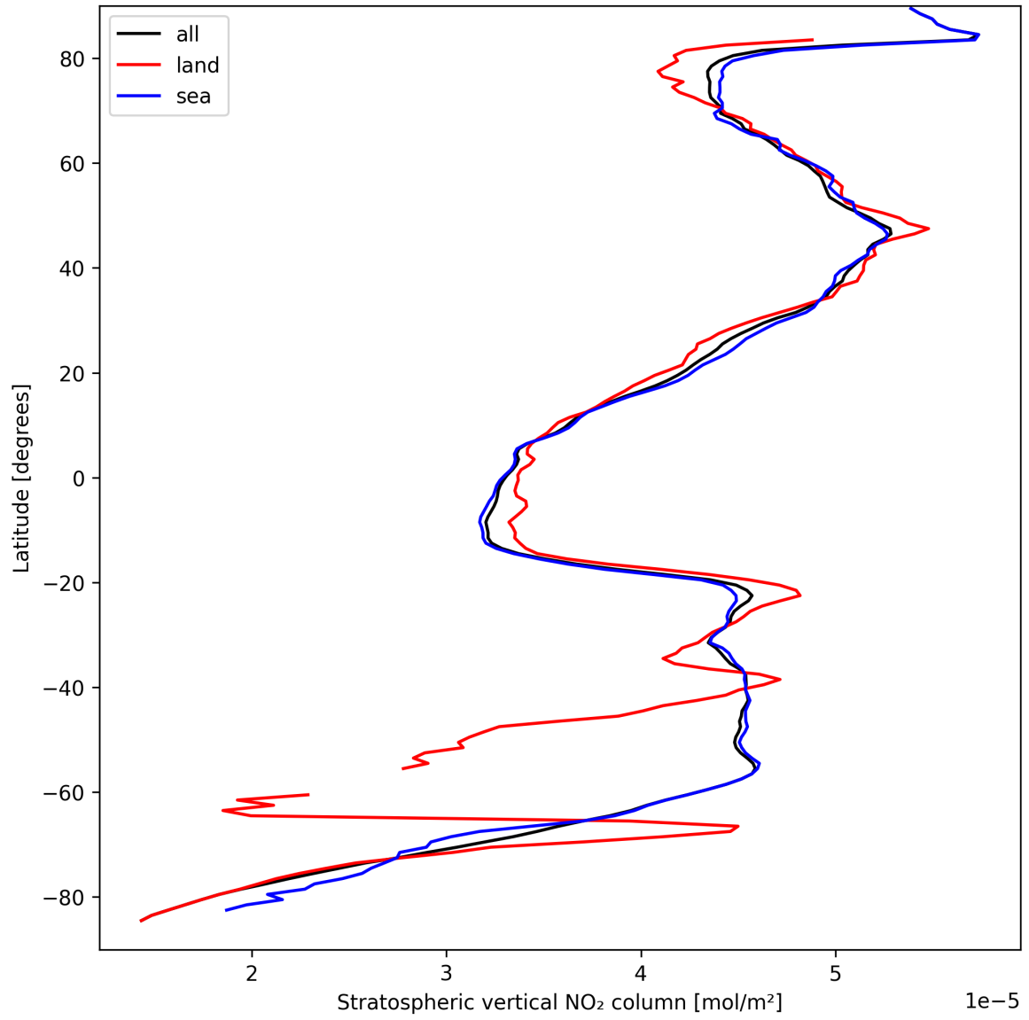
Figure 17: Zonal average of “Stratospheric vertical NO 2 column” for 2025-09-14 to 2025-09-15.
