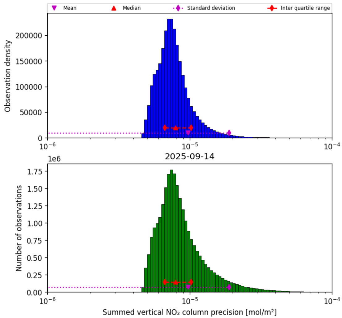
Figure 39: Histogram of “Summed vertical NO 2 column precision” for 2025-09-14 to 2025-09-15
