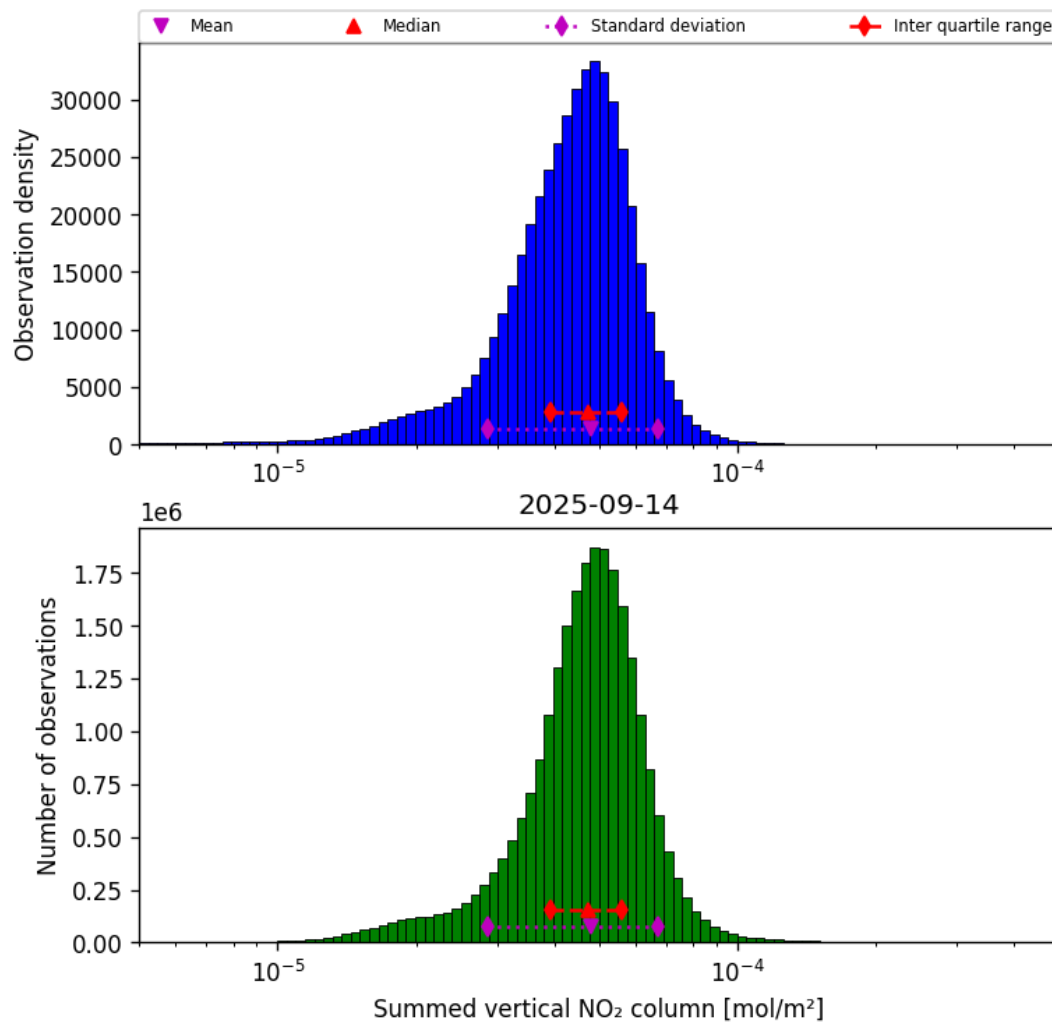
Figure 38: Histogram of “Summed vertical NO 2 column” for 2025-09-14 to 2025-09-15
