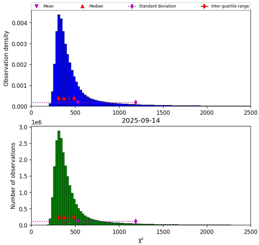
Figure 40: Histogram of “ \chi^2 ” for 2025-09-14 to 2025-09-15
