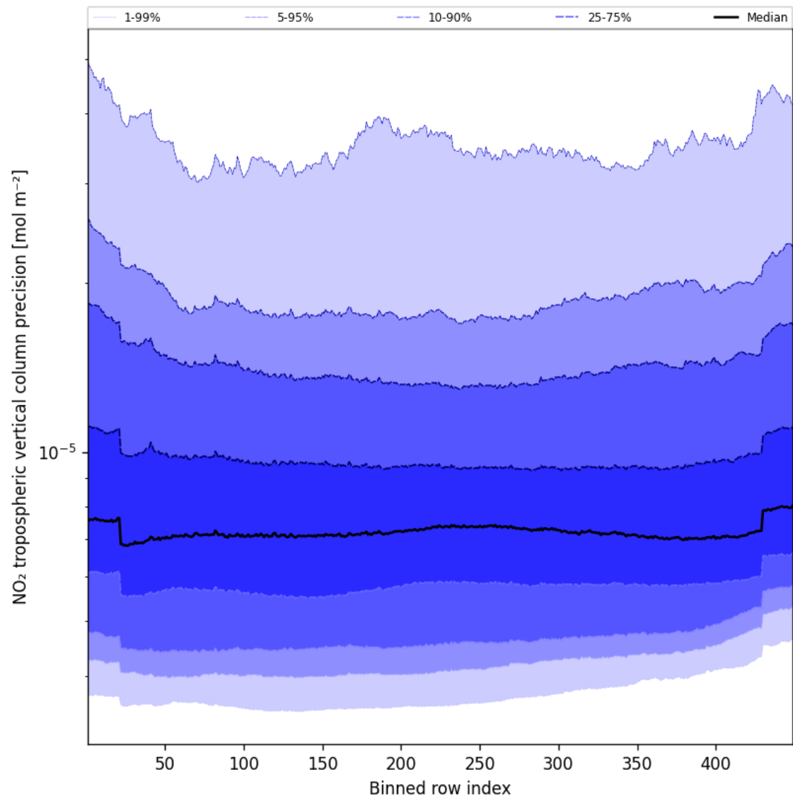
Figure 45: Along track statistics of “NO 2 tropospheric vertical column precision” for 2025-09-14 to 2025-09-15
