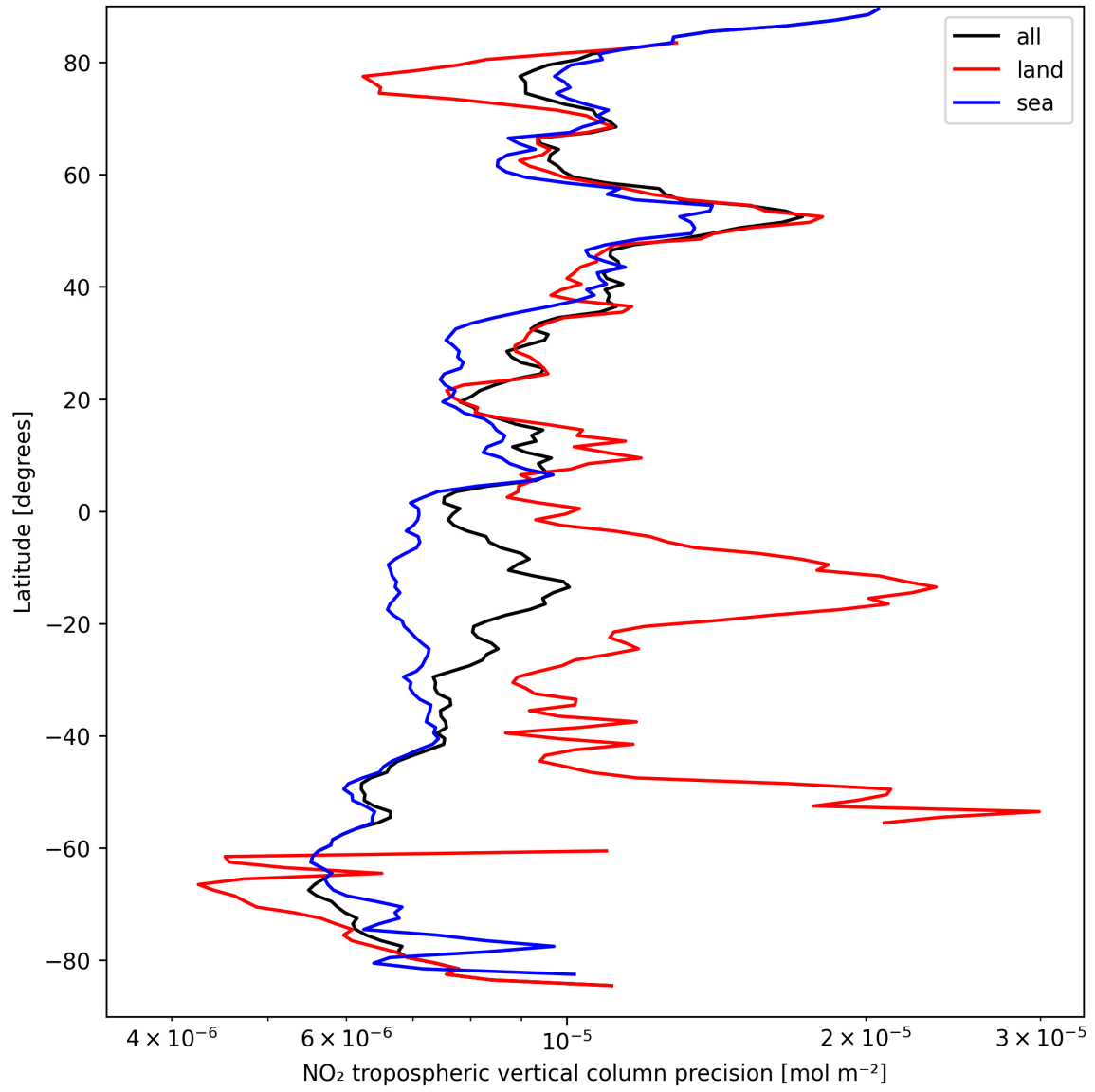
Figure 11: Zonal average of “NO 2 tropospheric vertical column precision” for 2025-09-14 to 2025-09-15.
