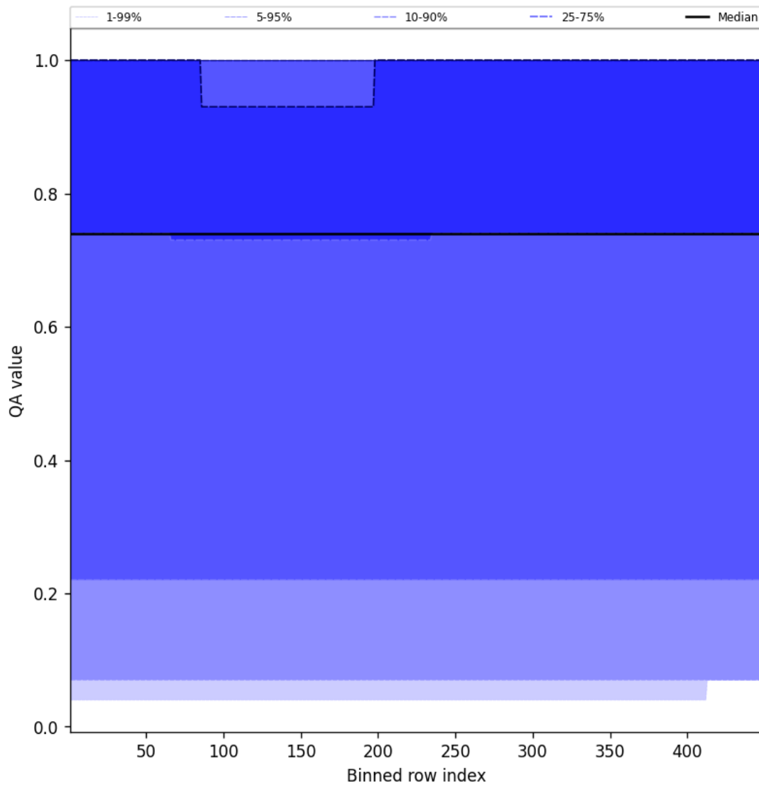
Figure 43: Along track statistics of “QA value” for 2025-09-14 to 2025-09-15
