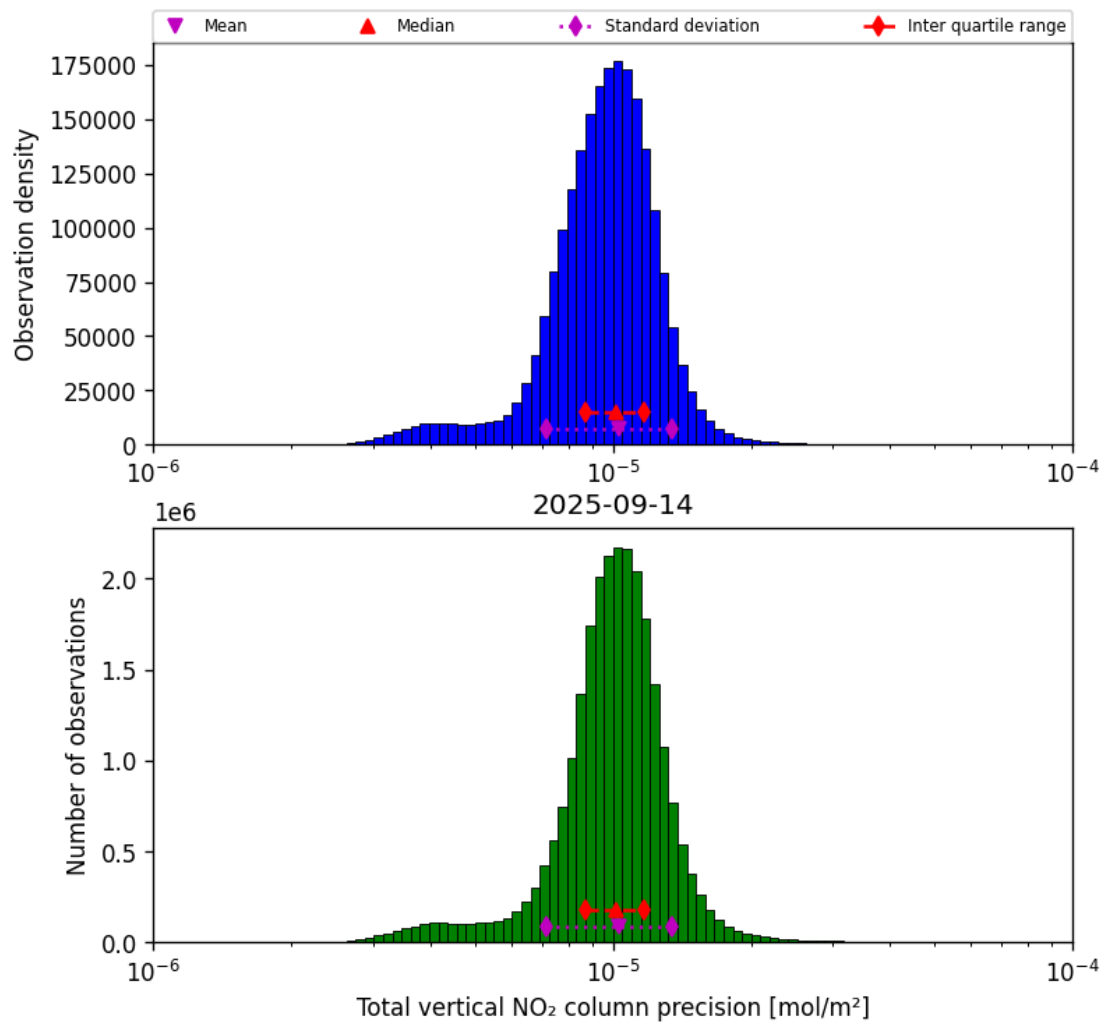
Figure 37: Histogram of “Total vertical NO 2 column precision” for 2025-09-14 to 2025-09-15
