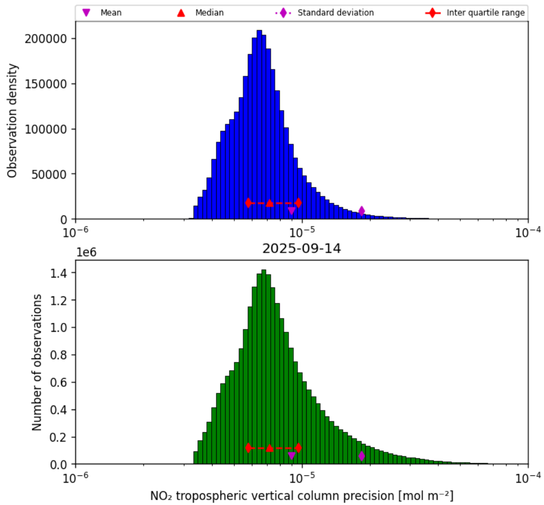
Figure 28: Histogram of “NO 2 tropospheric vertical column precision” for 2025-09-14 to 2025-09-15
