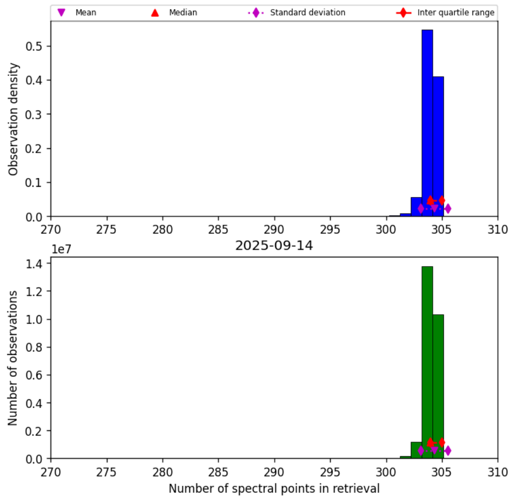
Figure 31: Histogram of “Number of spectral points in retrieval” for 2025-09-14 to 2025-09-15
