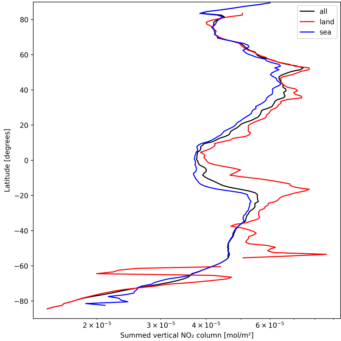
Figure 21: Zonal average of “Summed vertical NO 2 column” for 2025-09-14 to 2025-09-15.
