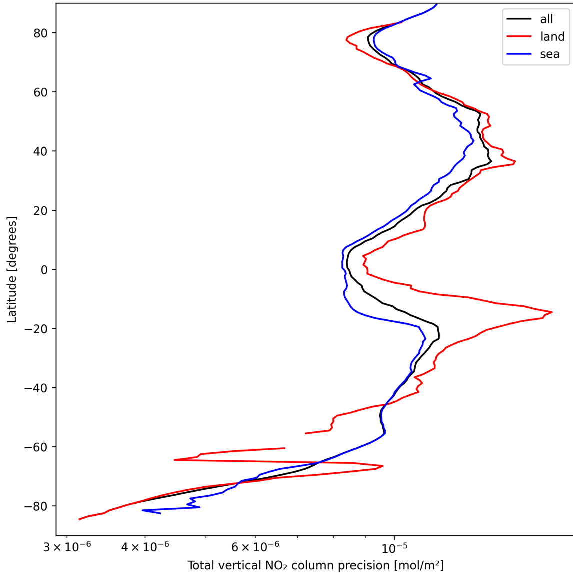
Figure 20: Zonal average of “Total vertical NO 2 column precision” for 2025-09-14 to 2025-09-15.
