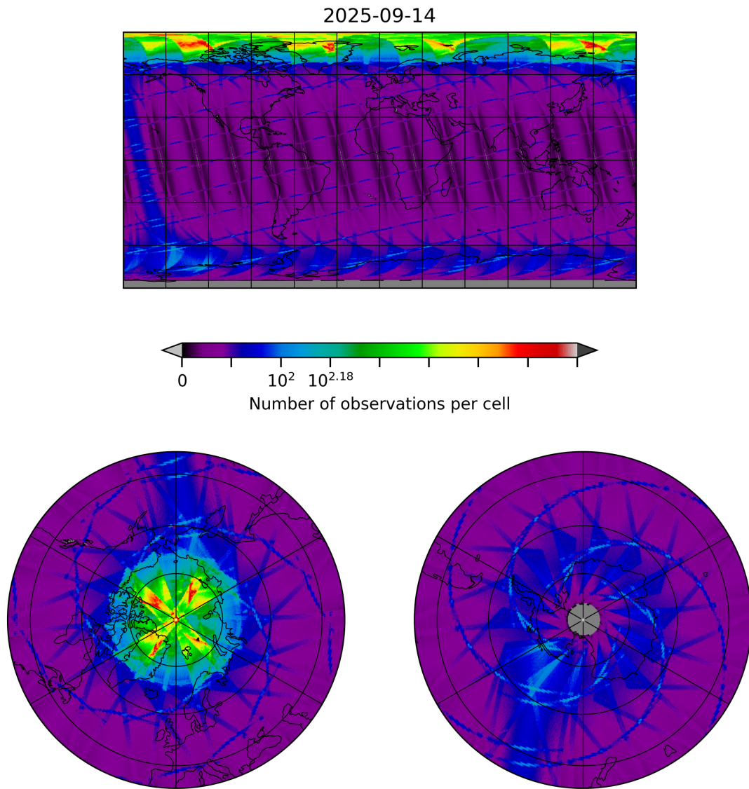
Figure 8: Map of the number of observations for 2025-09-14 to 2025-09-15
