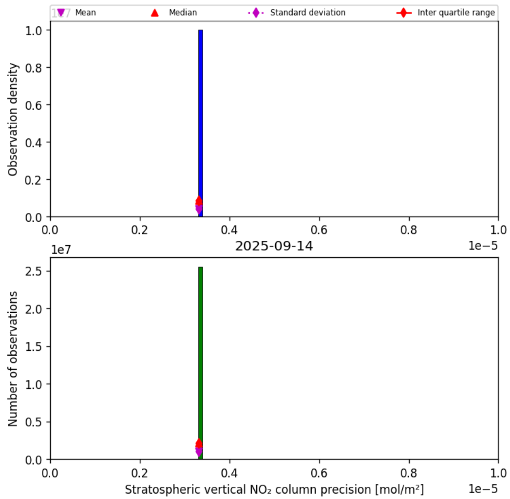
Figure 35: Histogram of “Stratospheric vertical NO 2 column precision” for 2025-09-14 to 2025-09-15
