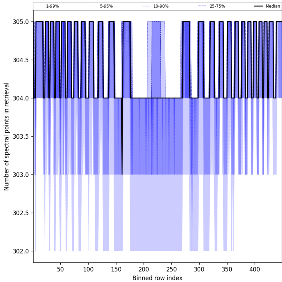
Figure 48: Along track statistics of “Number of spectral points in retrieval” for 2025-09-14 to 2025-09-15
