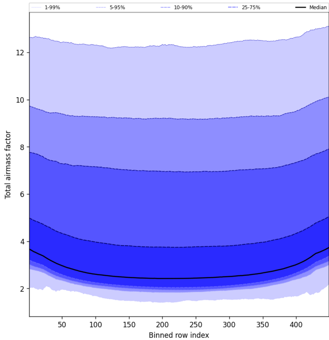
Figure 47: Along track statistics of “Total airmass factor” for 2025-09-14 to 2025-09-15
