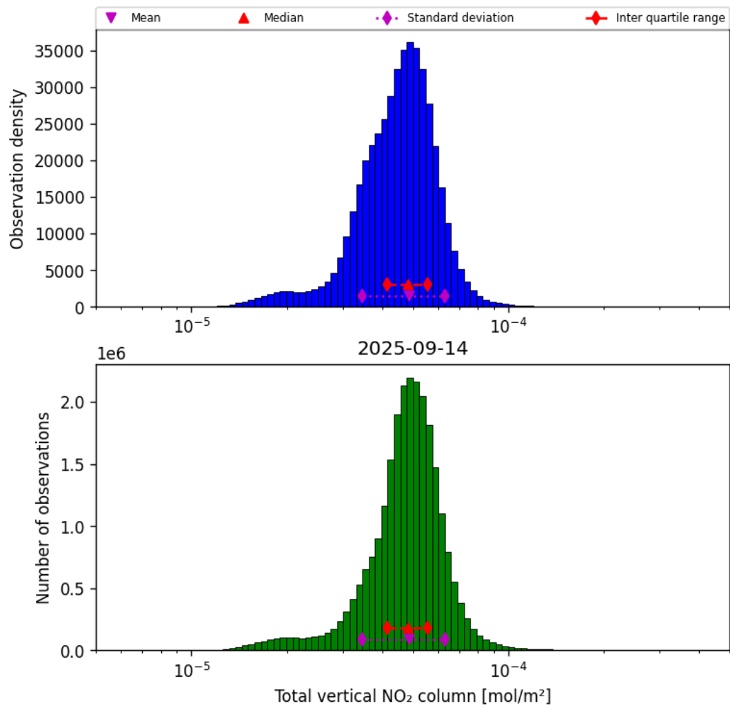
Figure 36: Histogram of “Total vertical NO 2 column” for 2025-09-14 to 2025-09-15
