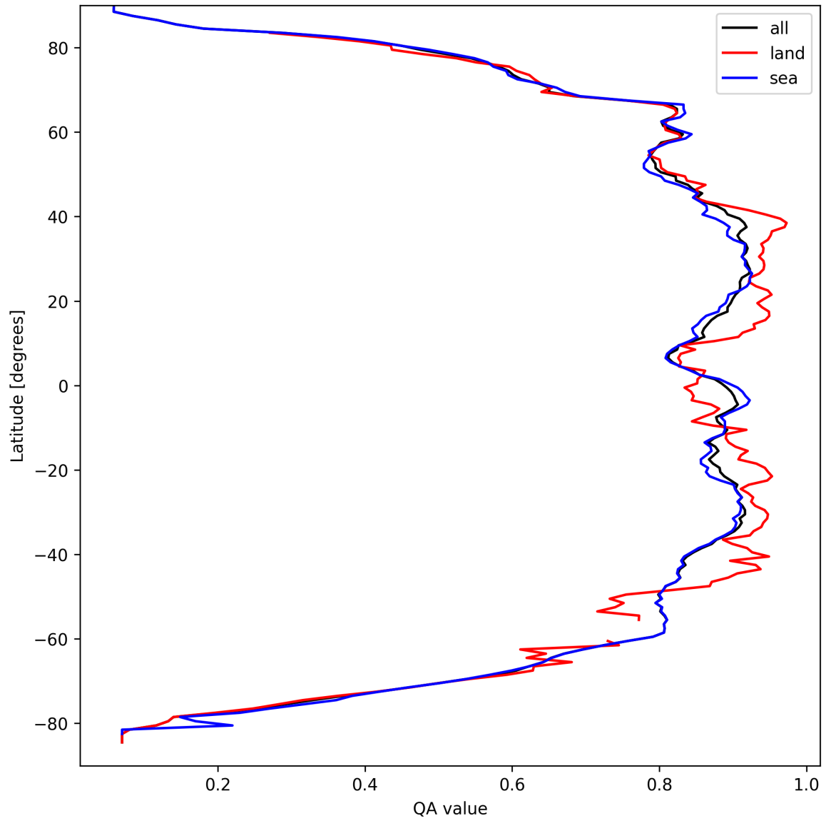
Figure 9: Zonal average of “QA value” for 2025-09-14 to 2025-09-15.
