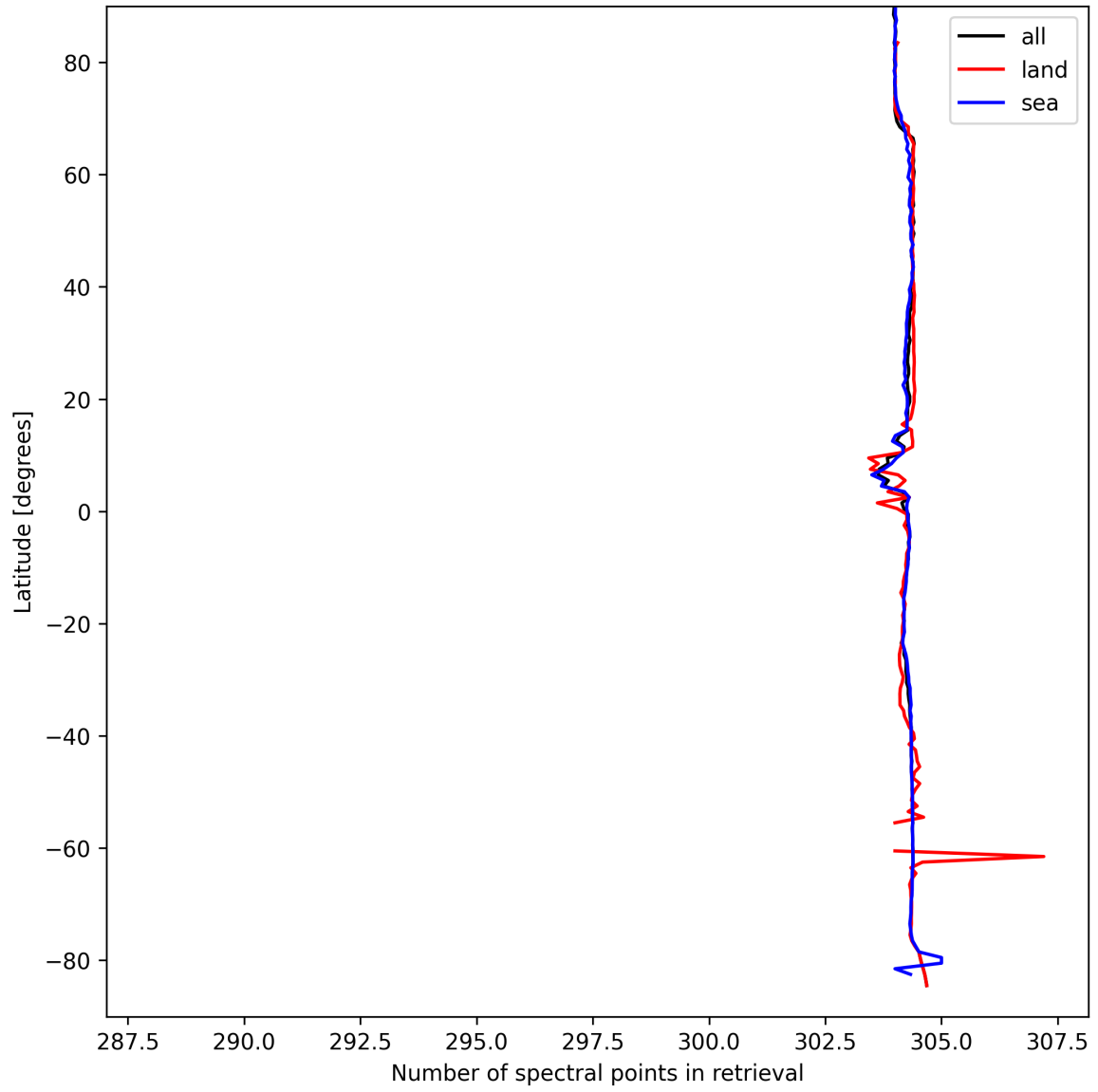
Figure 14: Zonal average of “Number of spectral points in retrieval” for 2025-09-14 to 2025-09-15.
