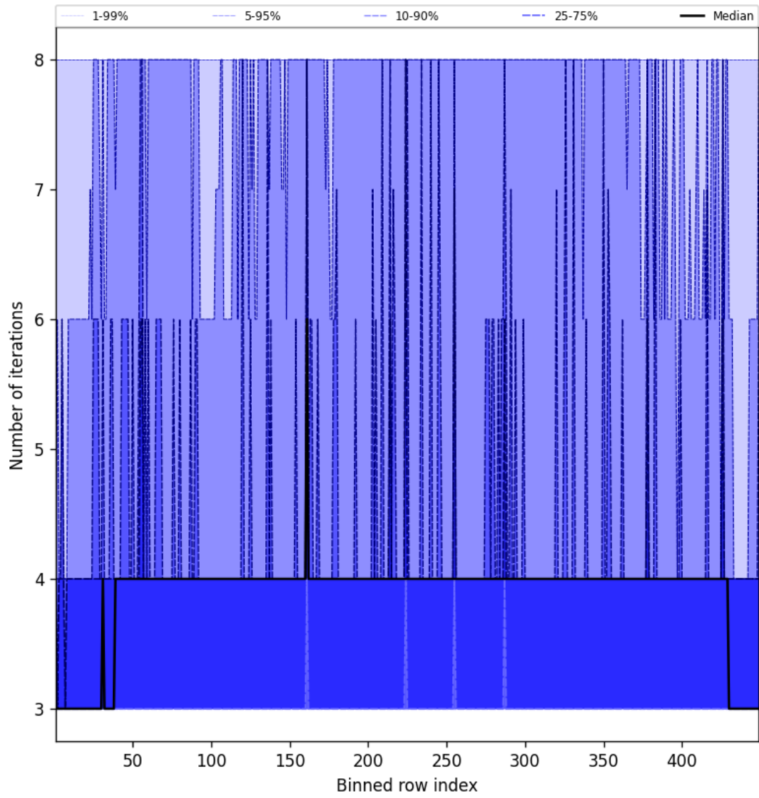
Figure 49: Along track statistics of “Number of iterations” for 2025-09-14 to 2025-09-15
