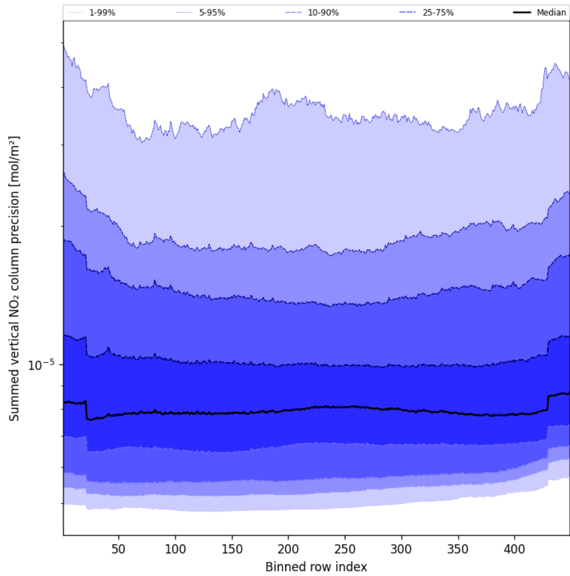
Figure 56: Along track statistics of “Summed vertical NO 2 column precision” for 2025-09-14 to 2025-09-15
