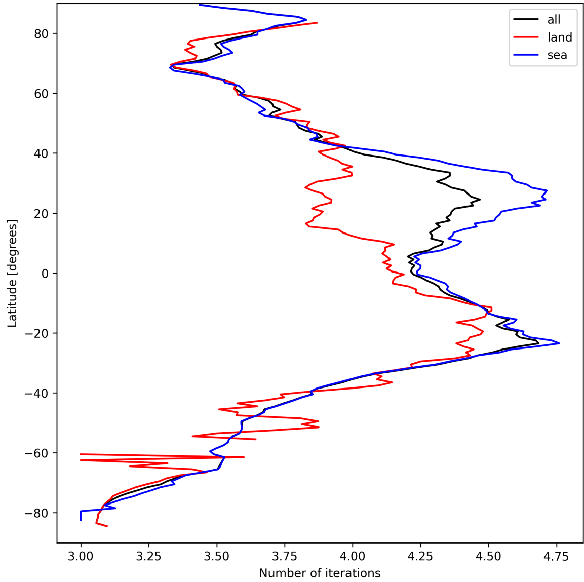
Figure 15: Zonal average of “Number of iterations” for 2025-09-14 to 2025-09-15.
