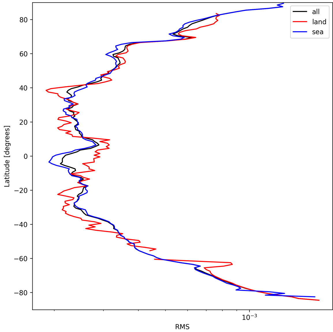
Figure 24: Zonal average of “RMS” for 2025-09-14 to 2025-09-15.
