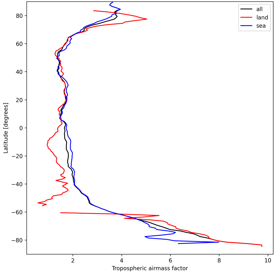
Figure 12: Zonal average of “Tropospheric airmass factor” for 2025-09-14 to 2025-09-15.
