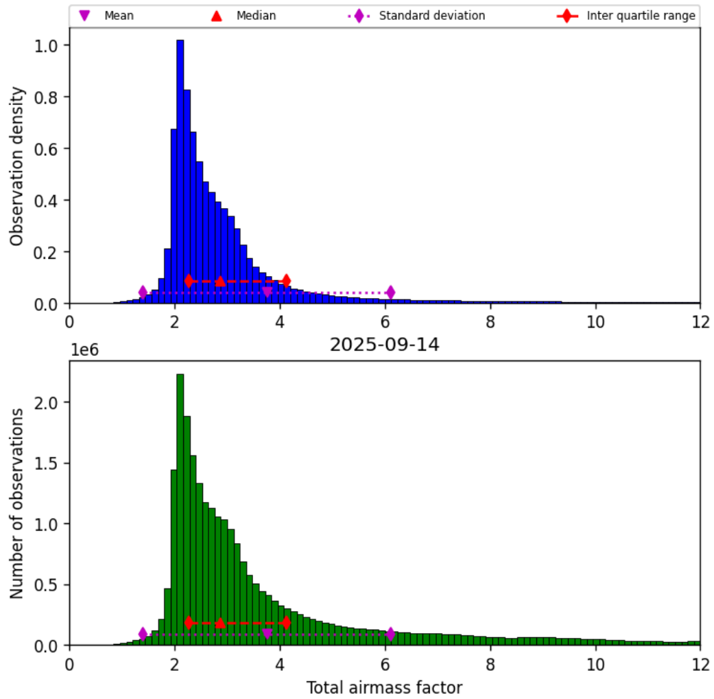
Figure 30: Histogram of “Total airmass factor” for 2025-09-14 to 2025-09-15
