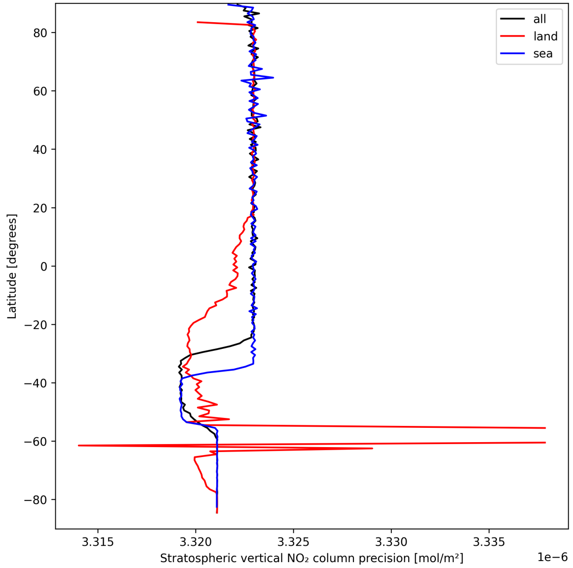
Figure 18: Zonal average of “Stratospheric vertical NO 2 column precision” for 2025-09-14 to 2025-09-15.
