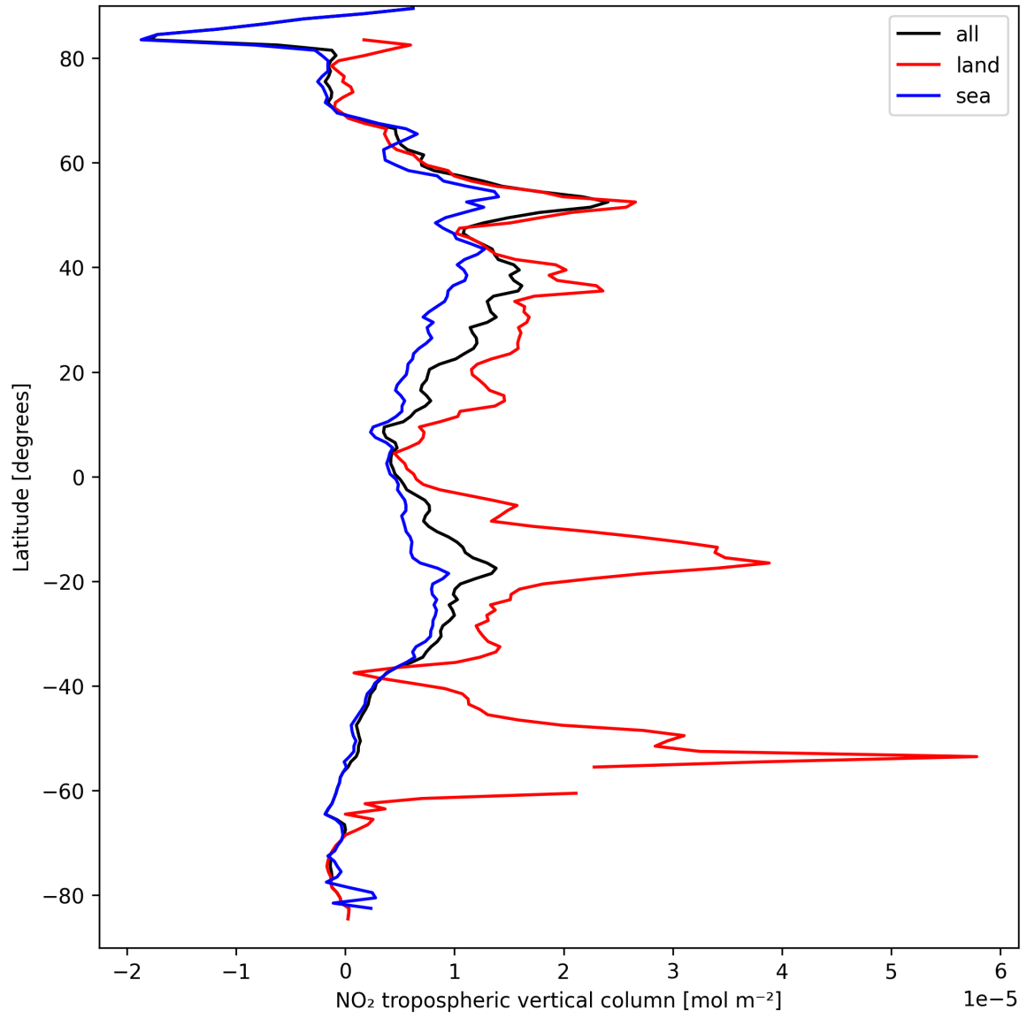
Figure 10: Zonal average of “NO 2 tropospheric vertical column” for 2025-09-14 to 2025-09-15.
