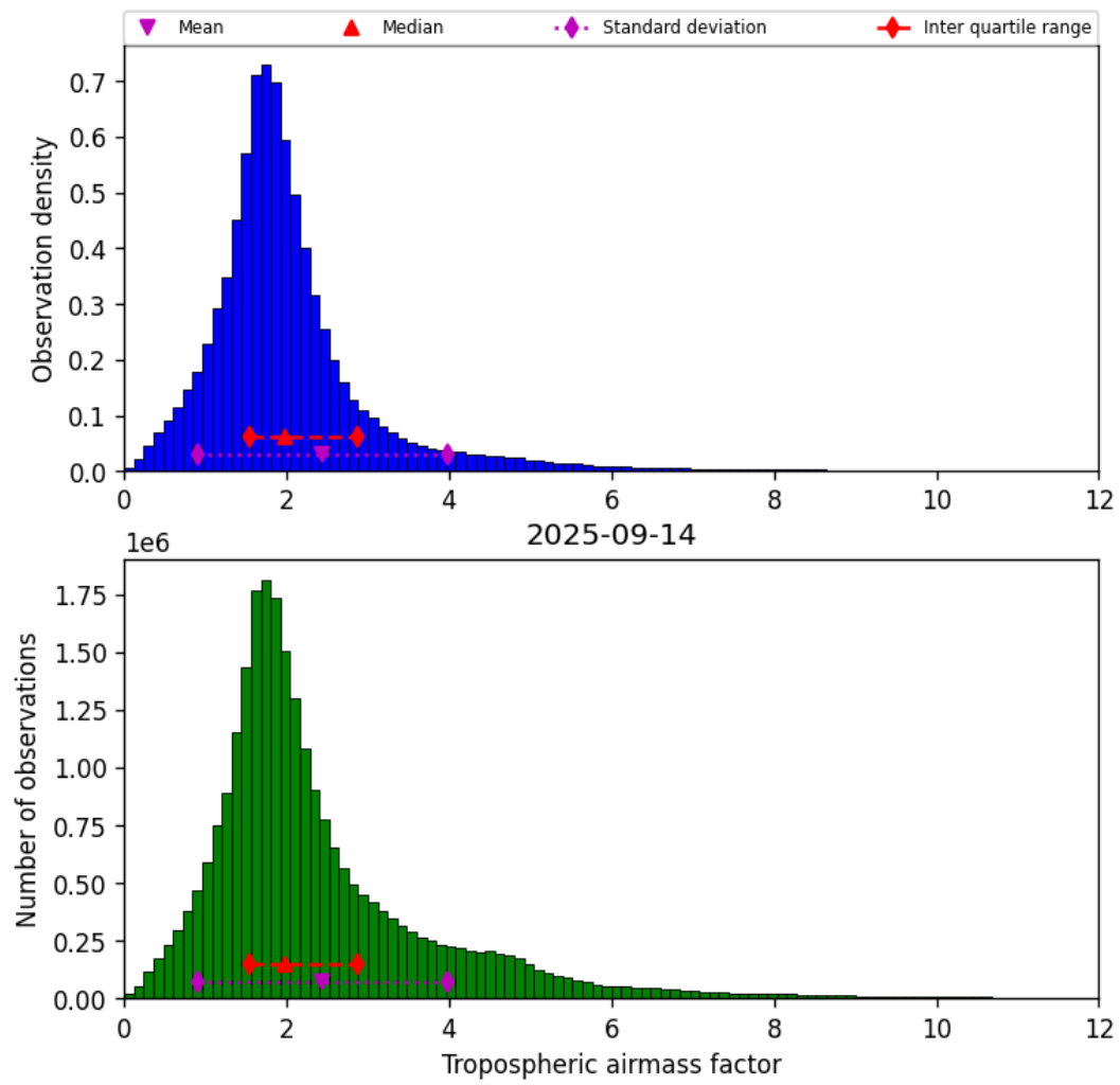
Figure 29: Histogram of “Tropospheric airmass factor” for 2025-09-14 to 2025-09-15
