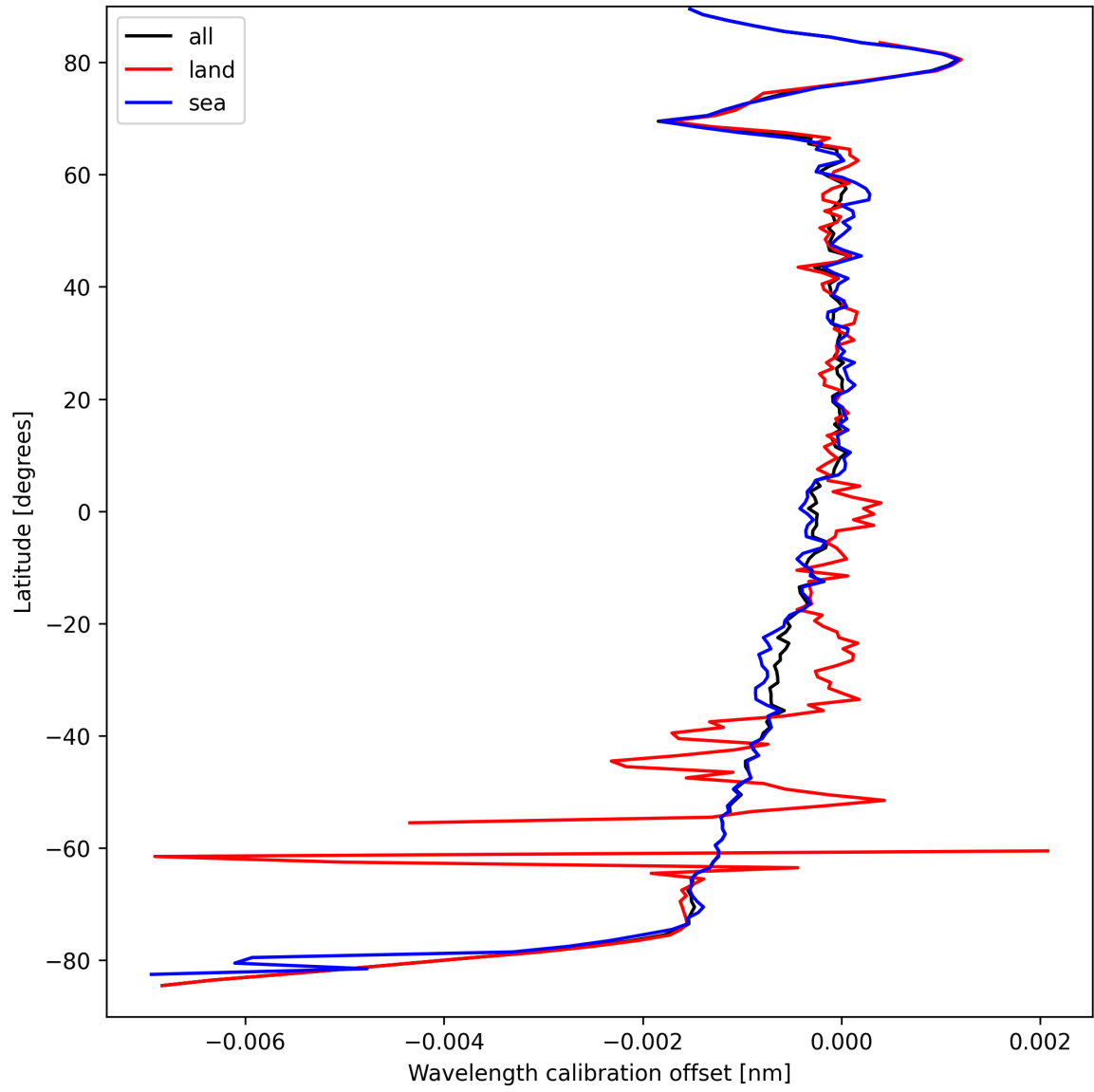
Figure 16: Zonal average of “Wavelength calibration offset” for 2025-09-14 to 2025-09-15.
