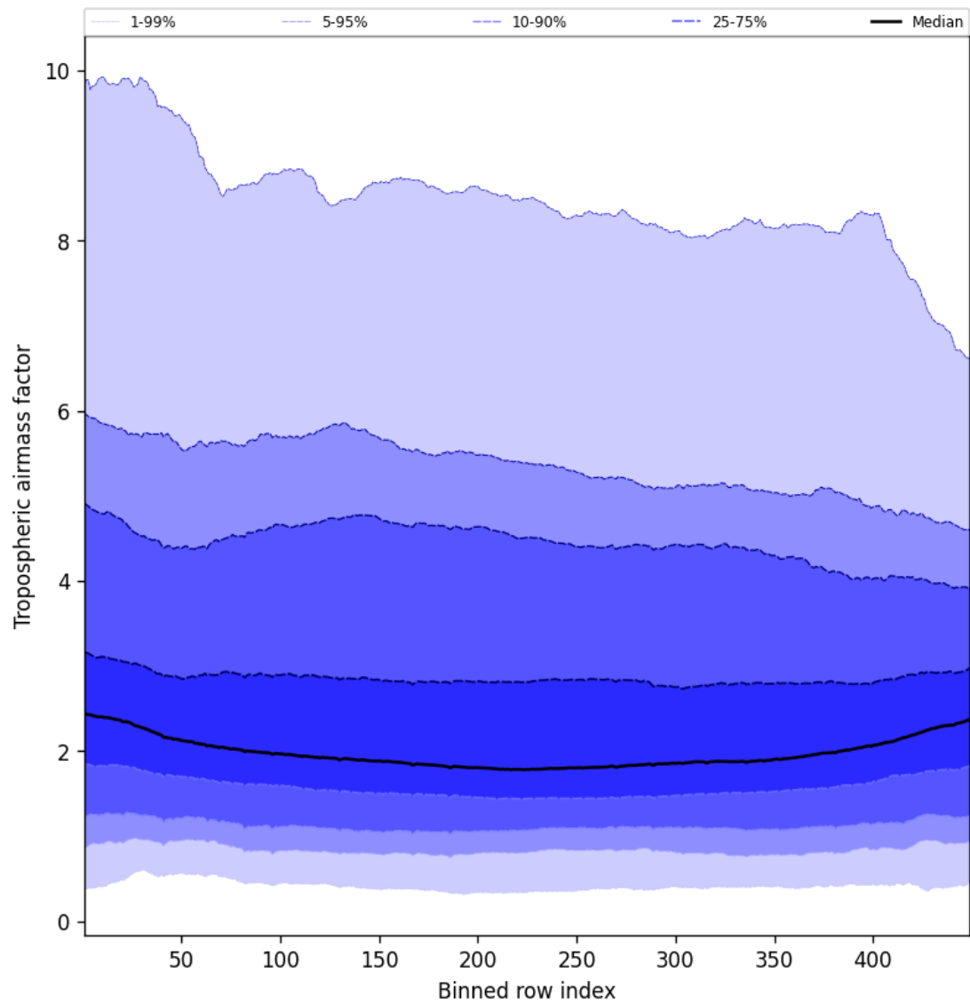
Figure 46: Along track statistics of “Tropospheric air mass factor” for 2025-09-14 to 2025-09-15
