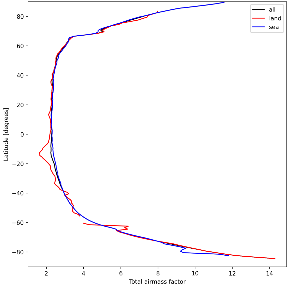
Figure 13: Zonal average of “Total airmass factor” for 2025-09-14 to 2025-09-15.
