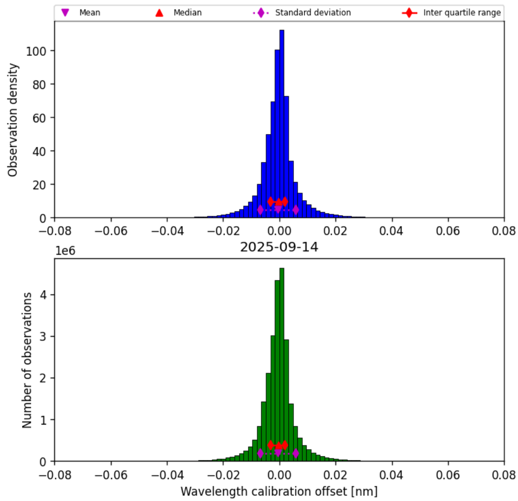
Figure 33: Histogram of “Wavelength calibration offset” for 2025-09-14 to 2025-09-15
