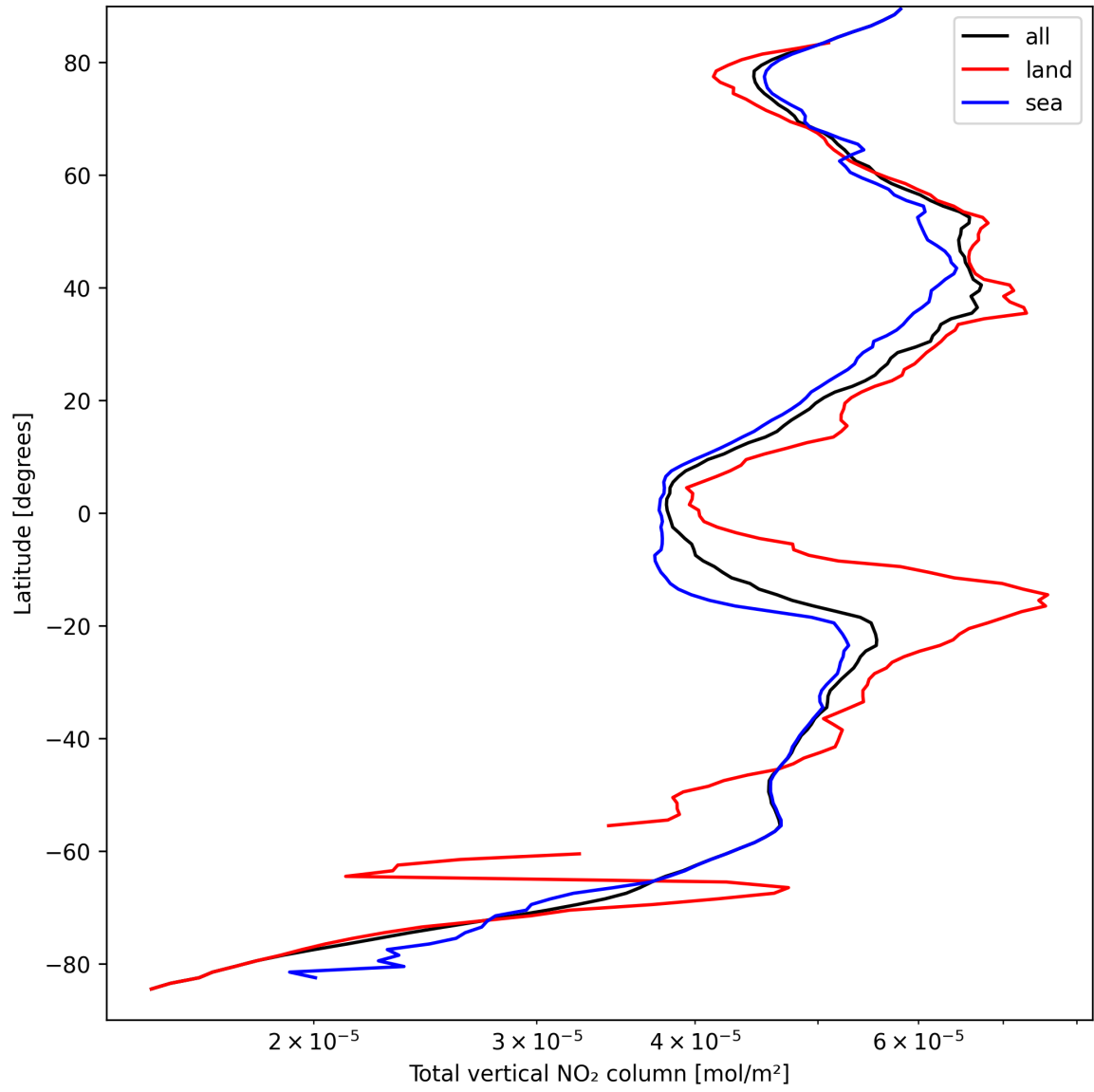
Figure 19: Zonal average of “Total vertical NO 2 column” for 2025-09-14 to 2025-09-15.
