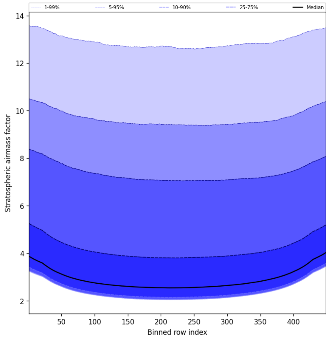
Figure 59: Along track statistics of “Stratospheric airmass factor” for 2025-09-14 to 2025-09-15
