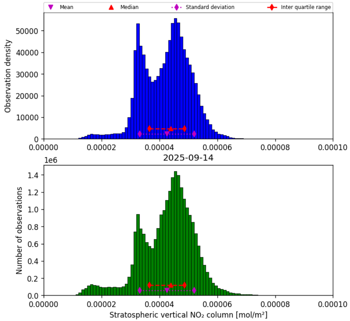
Figure 34: Histogram of “Stratospheric vertical NO 2 column” for 2025-09-14 to 2025-09-15
