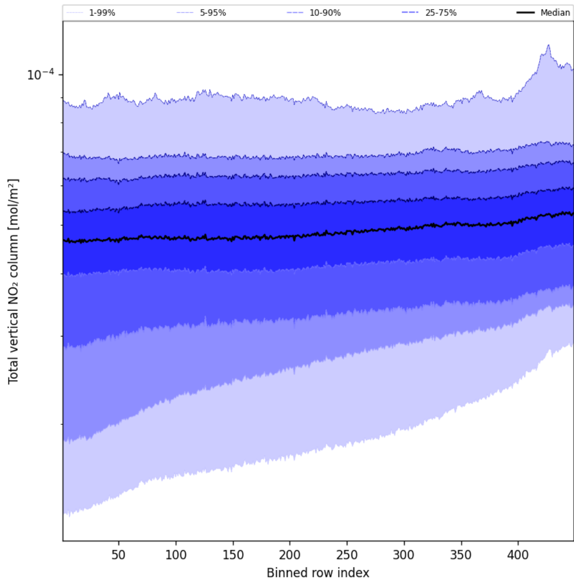
Figure 53: Along track statistics of “Total vertical NO 2 column” for 2025-09-14 to 2025-09-15
