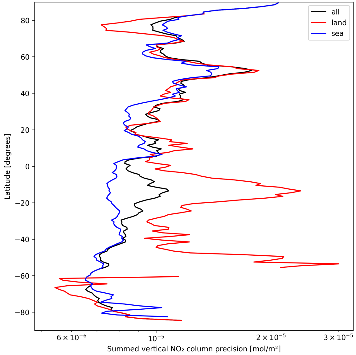
Figure 22: Zonal average of “Summed vertical NO 2 column precision” for 2025-09-14 to 2025-09-15.
