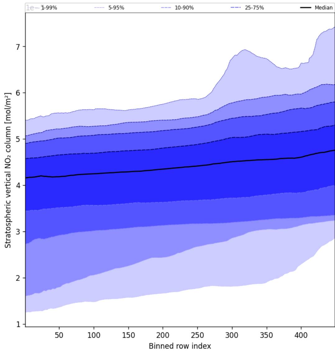
Figure 51: Along track statistics of “Stratospheric vertical NO 2 column” for 2025-09-14 to 2025-09-15
