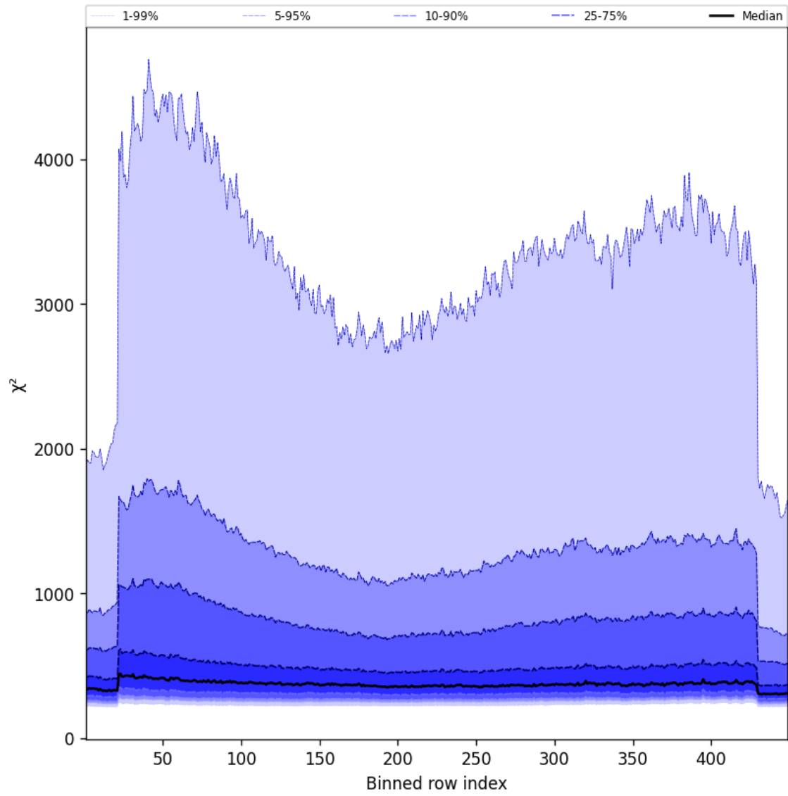
Figure 57: Along track statistics of “ \chi^2 ” for 2025-09-14 to 2025-09-15
