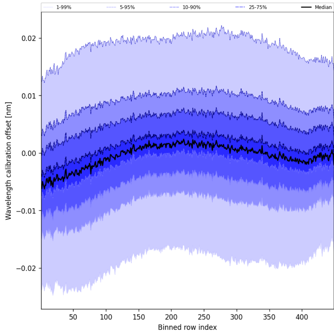
Figure 50: Along track statistics of “Wavelength calibration offset” for 2025-09-14 to 2025-09-15
