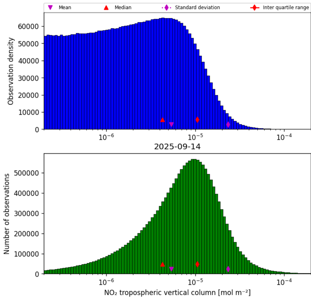
Figure 27: Histogram of “NO 2 tropospheric vertical column” for 2025-09-14 to 2025-09-15
