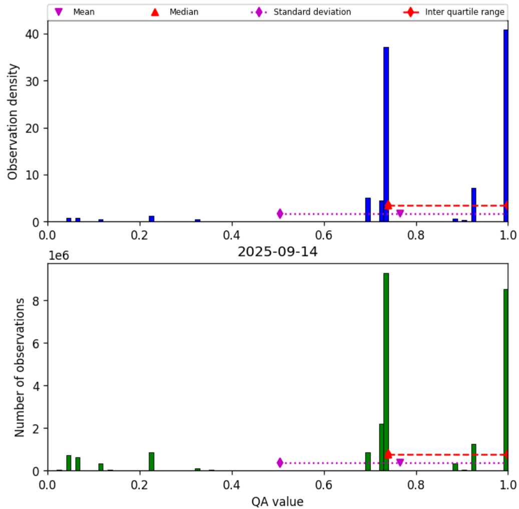
Figure 26: Histogram of “QA value” for 2025-09-14 to 2025-09-15
