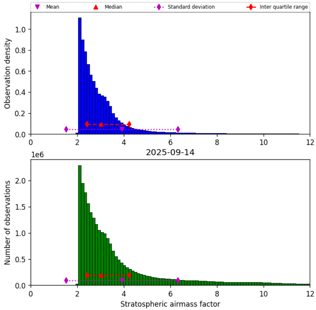
Figure 42: Histogram of “Stratospheric airmass factor” for 2025-09-14 to 2025-09-15
