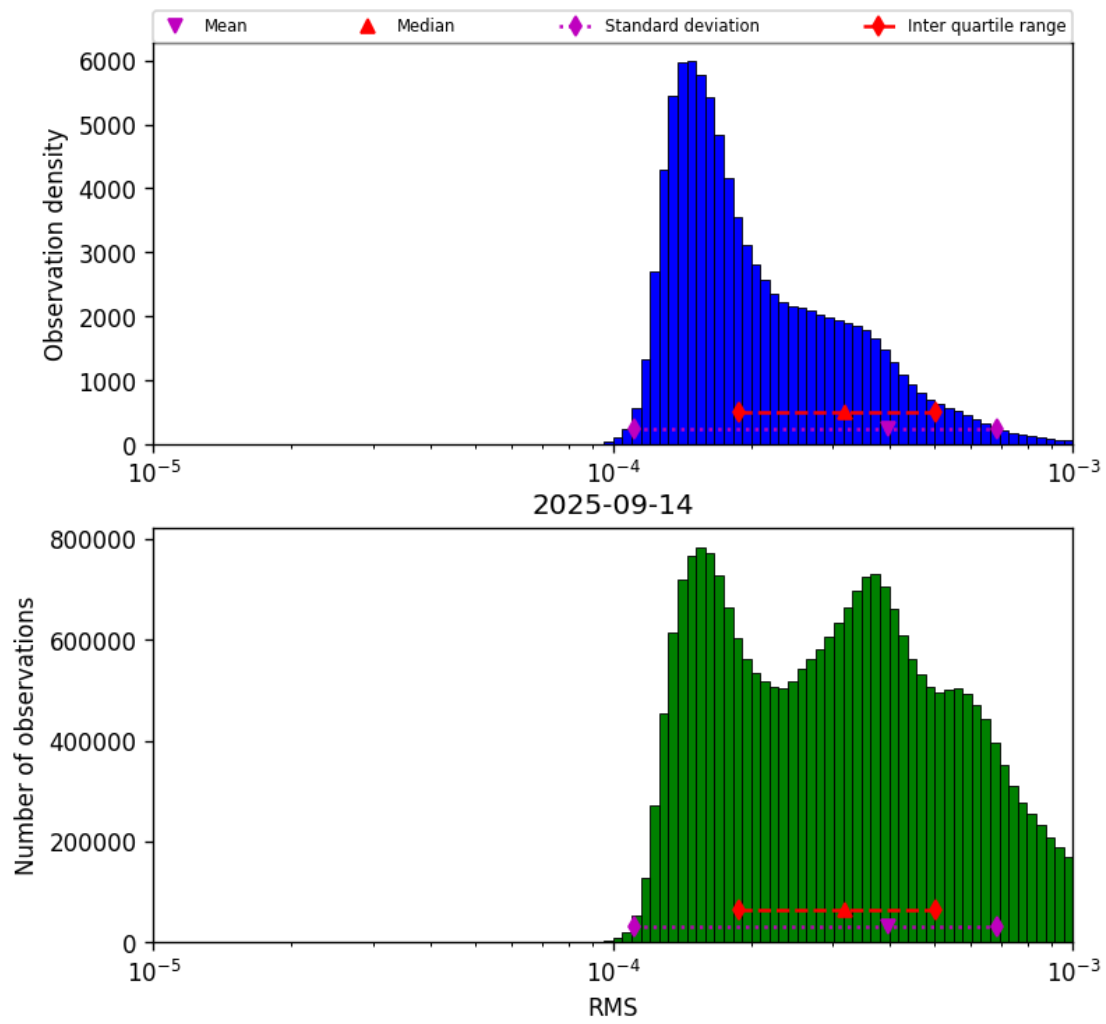
Figure 41: Histogram of “RMS” for 2025-09-14 to 2025-09-15
