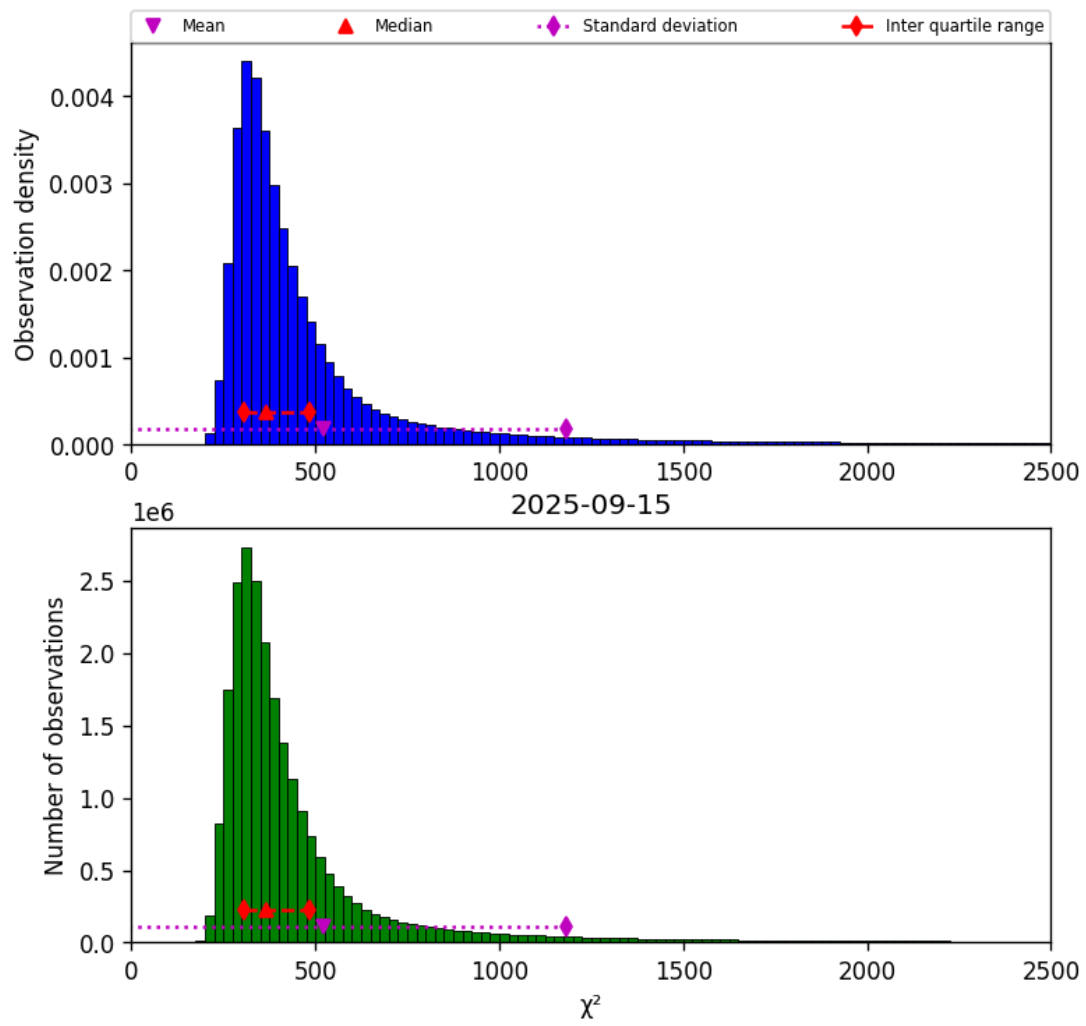
Figure 40: Histogram of “ \chi^2 ” for 2025-09-15 to 2025-09-16
