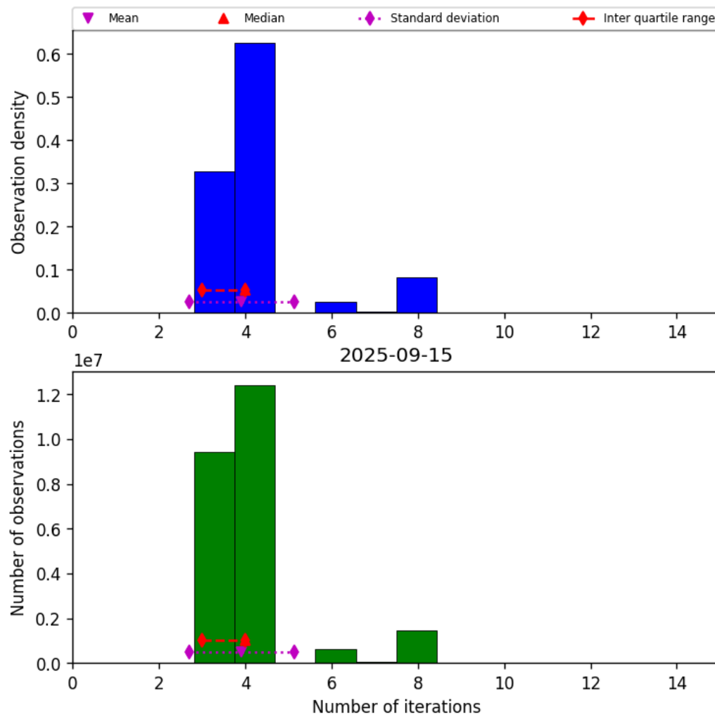
Figure 32: Histogram of “Number of iterations” for 2025-09-15 to 2025-09-16
