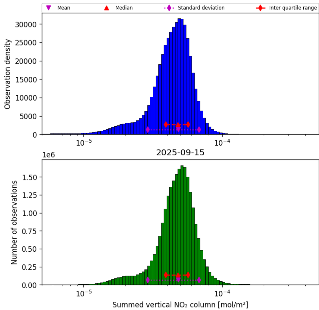
Figure 38: Histogram of “Summed vertical NO 2 column” for 2025-09-15 to 2025-09-16
