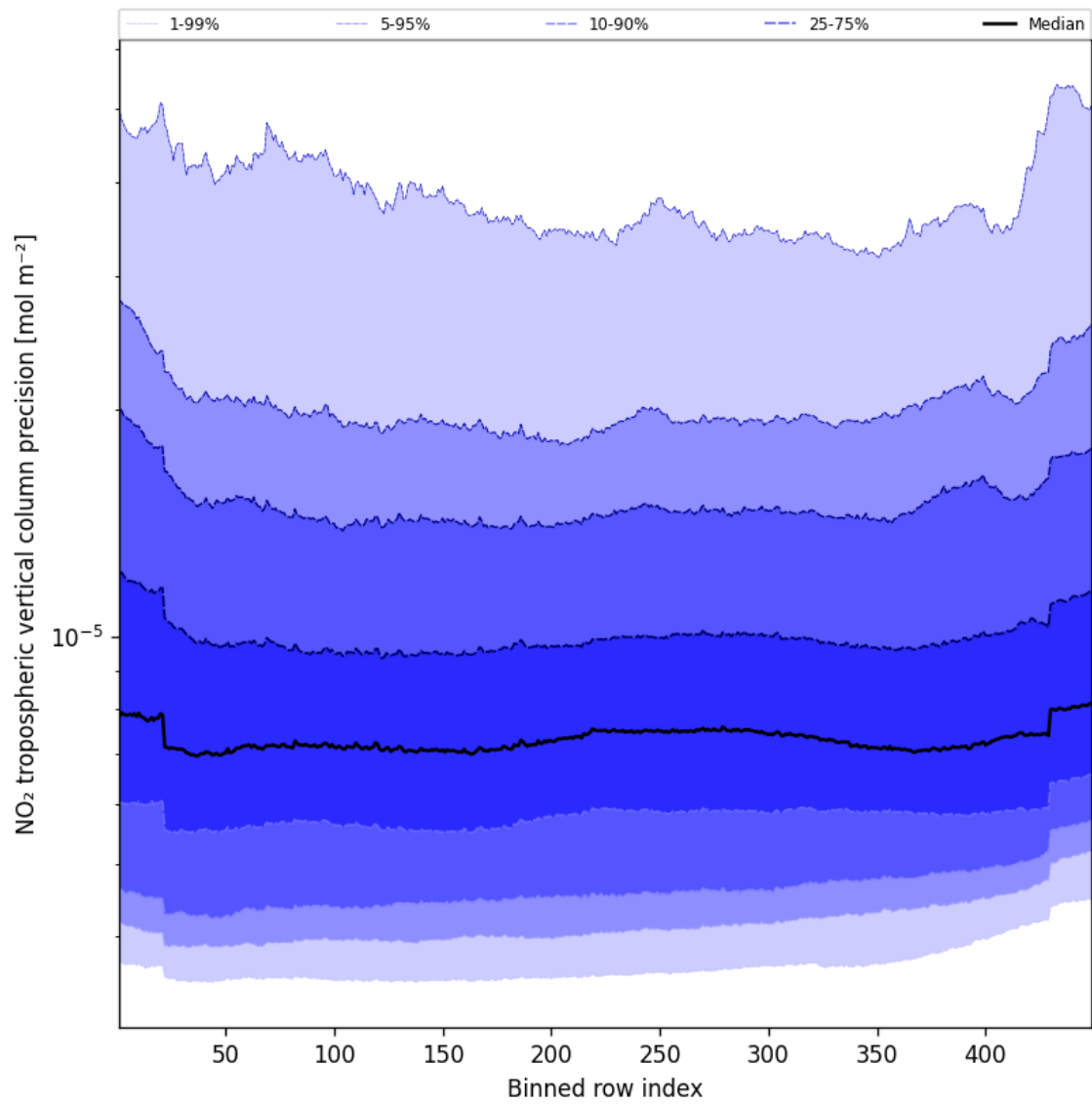
Figure 45: Along track statistics of “NO 2 tropospheric vertical column precision” for 2025-09-15 to 2025-09-16
