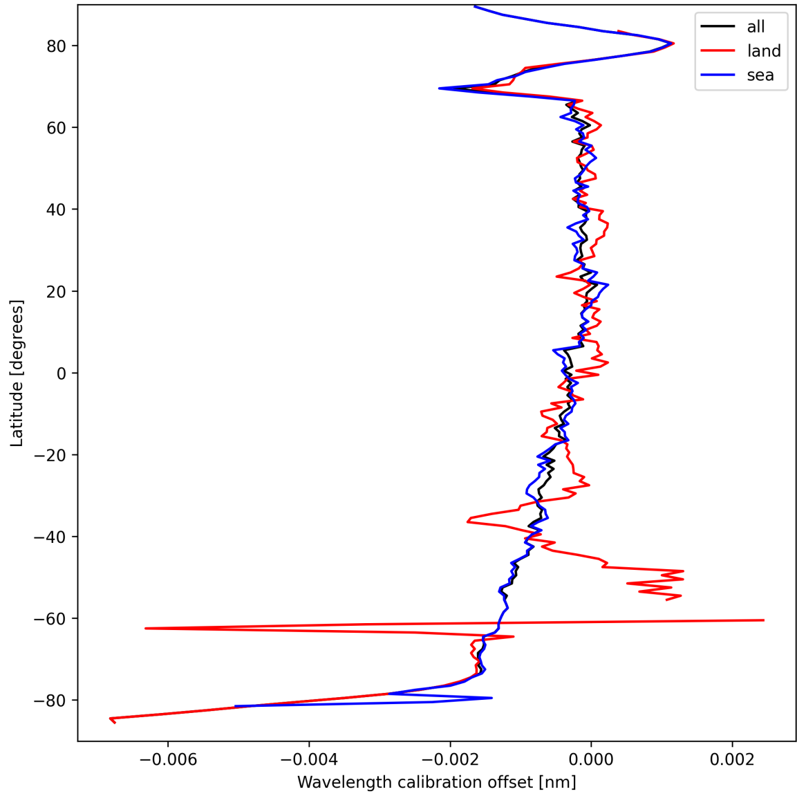
Figure 16: Zonal average of “Wavelength calibration offset” for 2025-09-15 to 2025-09-16.
