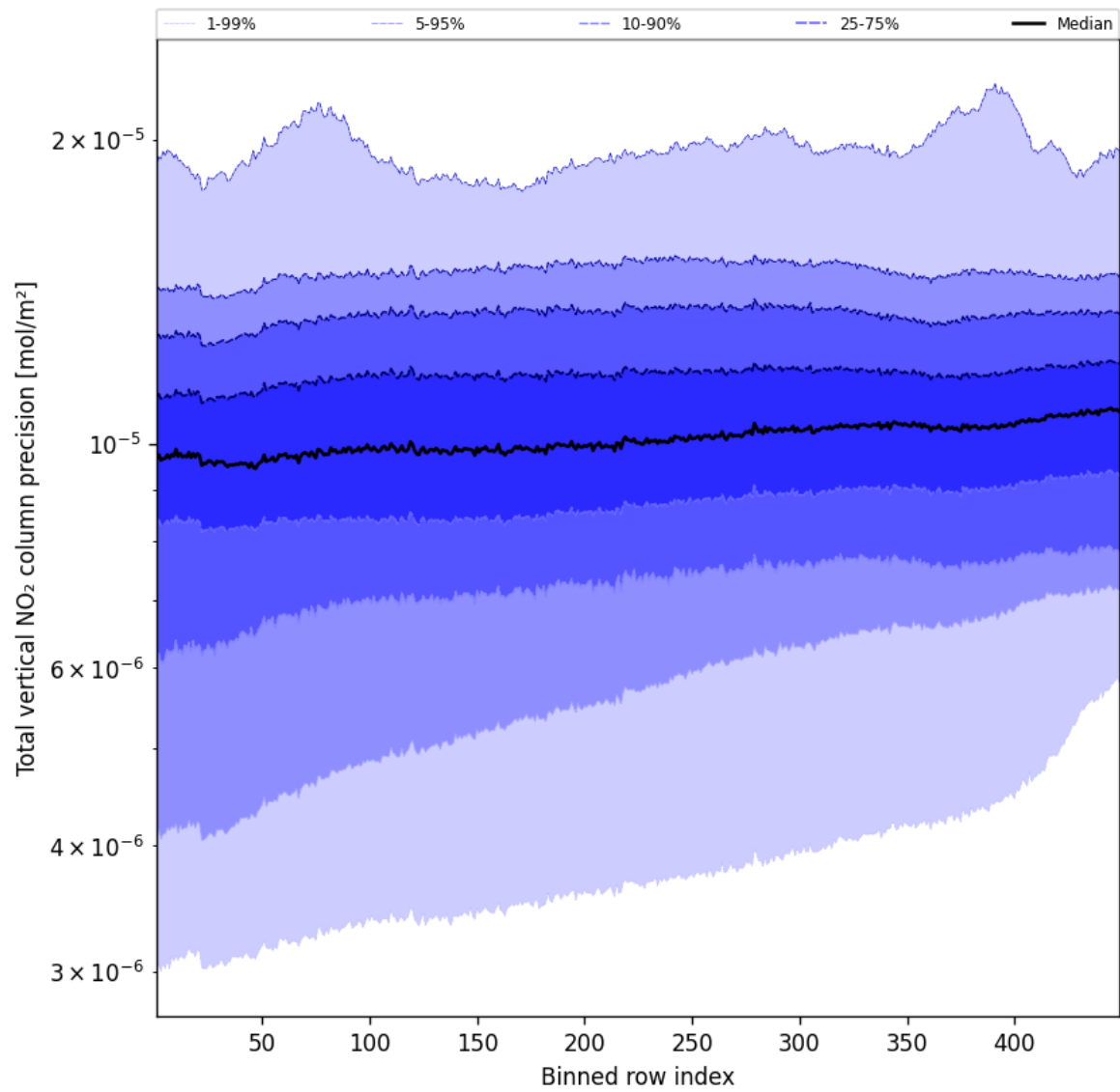
Figure 54: Along track statistics of “Total vertical NO 2 column precision” for 2025-09-15 to 2025-09-16
