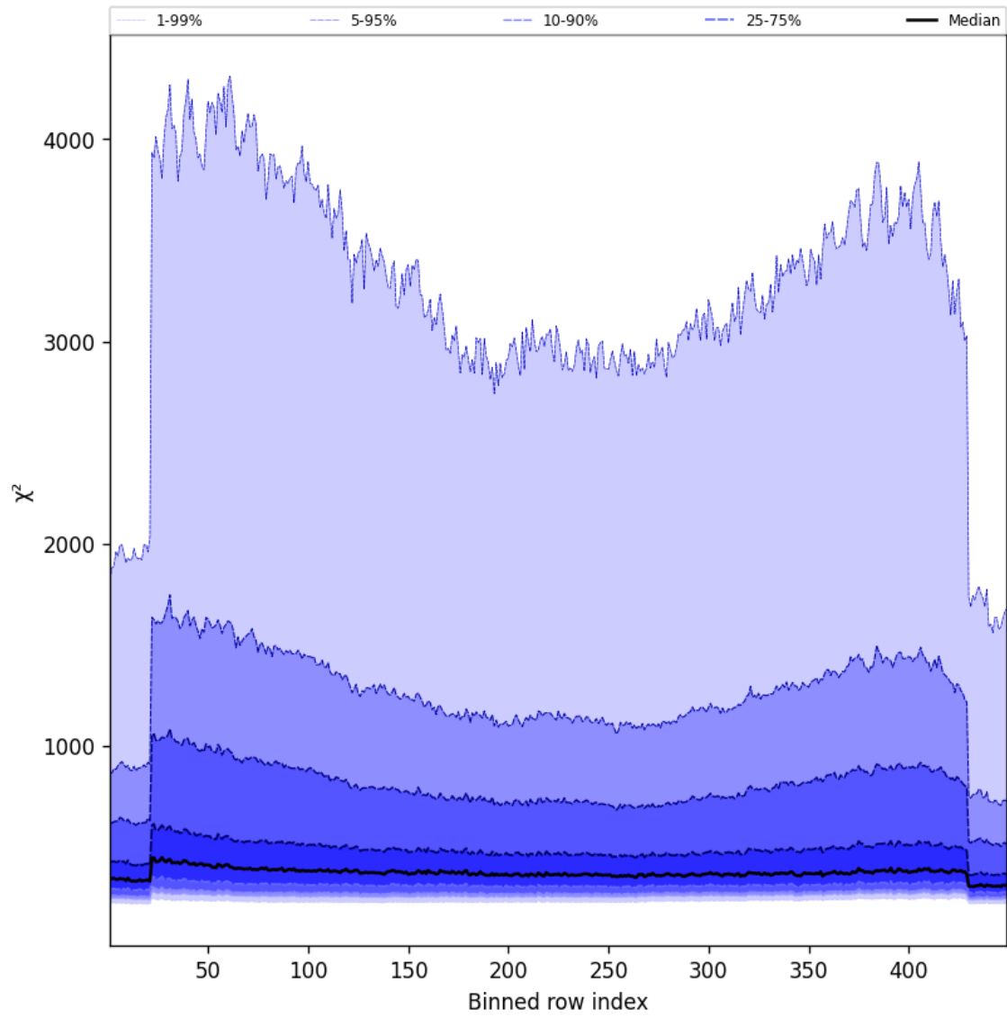
Figure 57: Along track statistics of “ \chi^2 ” for 2025-09-15 to 2025-09-16
