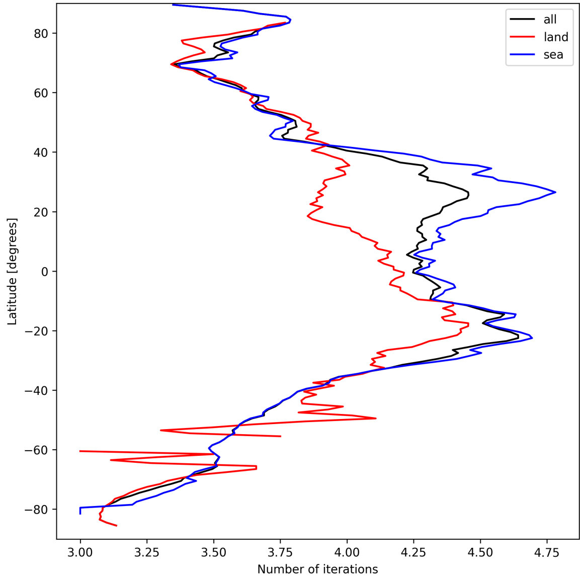
Figure 15: Zonal average of “Number of iterations” for 2025-09-15 to 2025-09-16.
