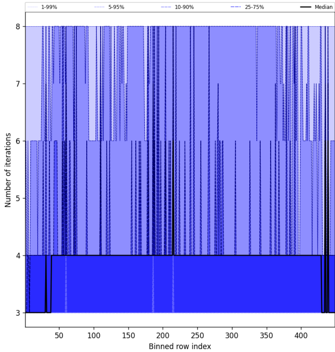
Figure 49: Along track statistics of “Number of iterations” for 2025-09-15 to 2025-09-16
