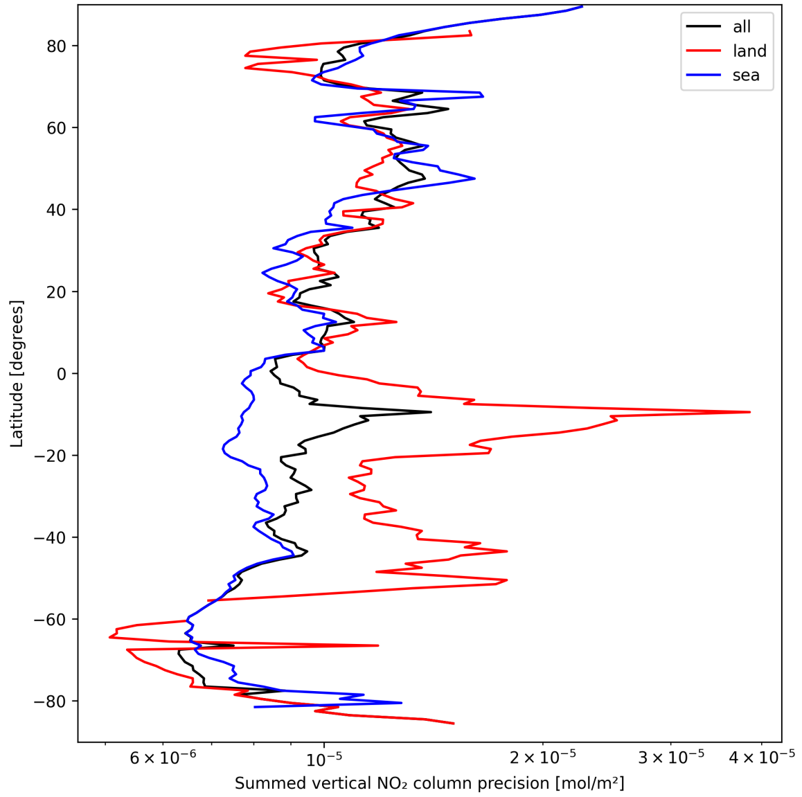
Figure 22: Zonal average of “Summed vertical NO 2 column precision” for 2025-09-15 to 2025-09-16.
