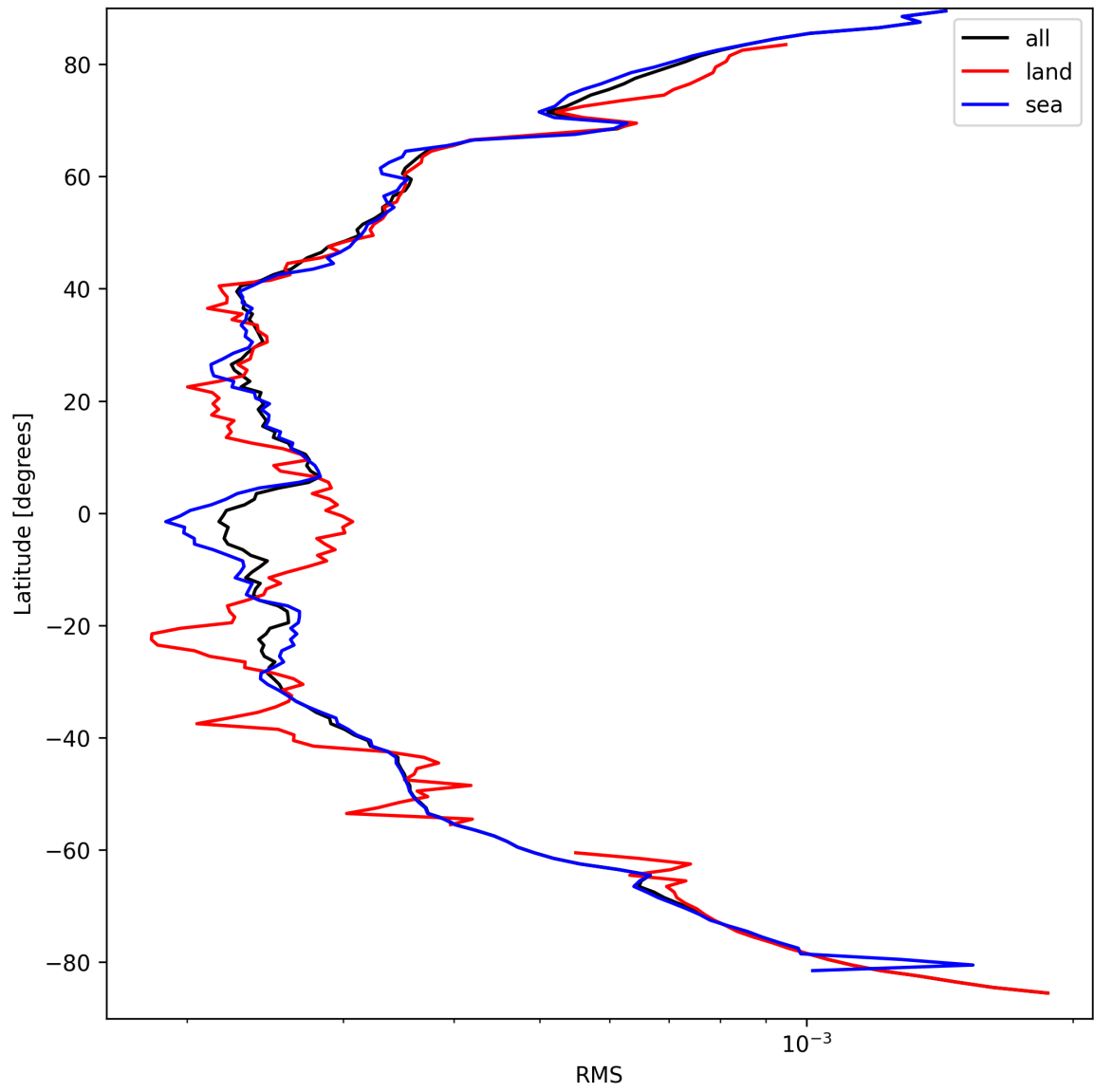
Figure 24: Zonal average of “RMS” for 2025-09-15 to 2025-09-16.
