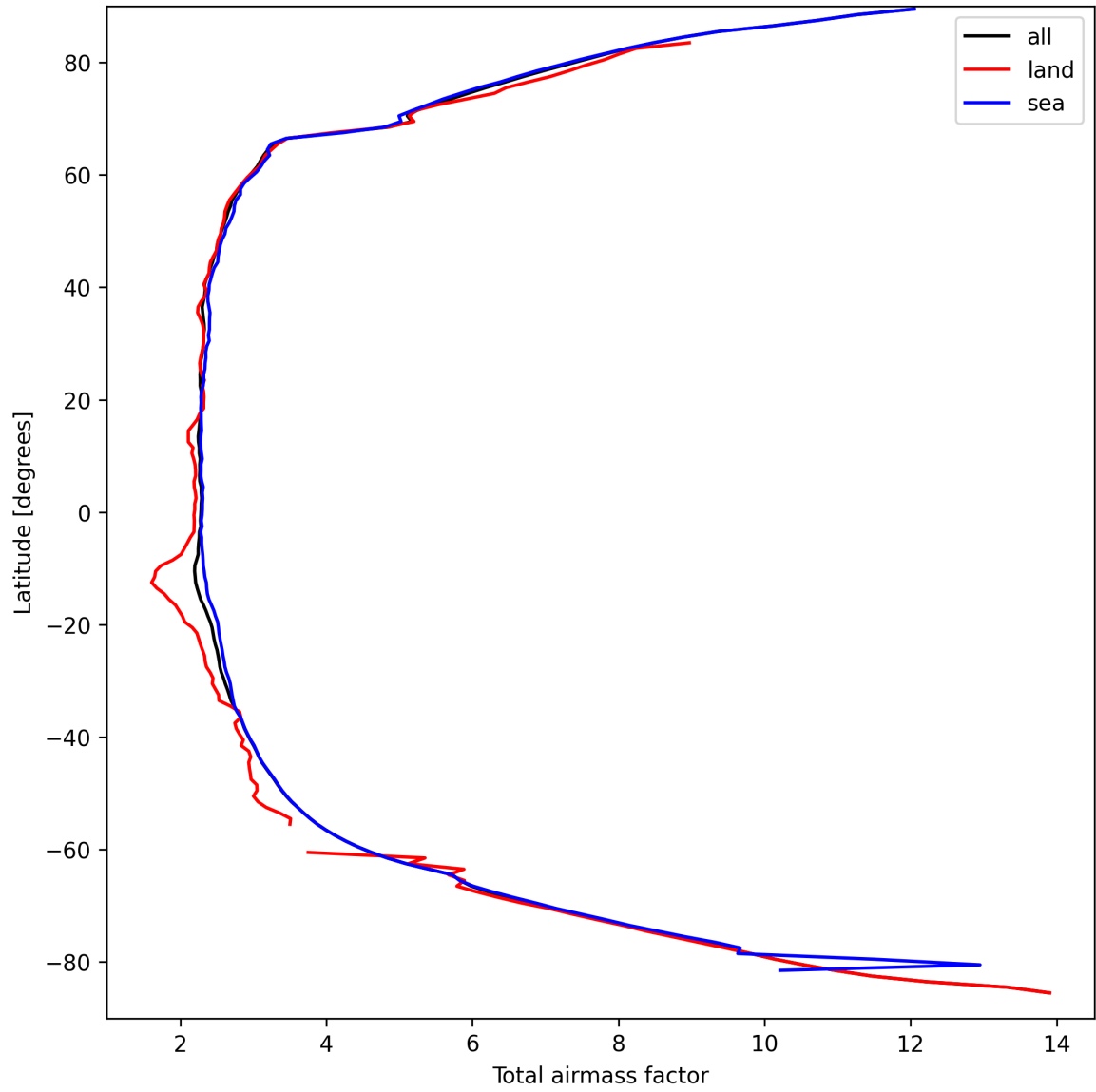
Figure 13: Zonal average of “Total airmass factor” for 2025-09-15 to 2025-09-16.
