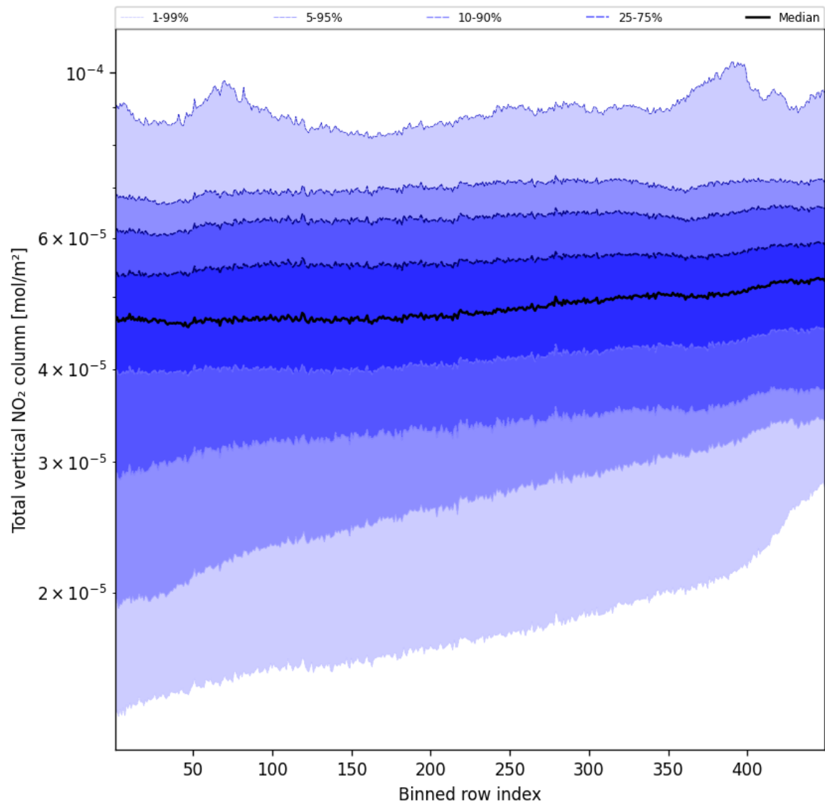
Figure 53: Along track statistics of “Total vertical NO 2 column” for 2025-09-15 to 2025-09-16
