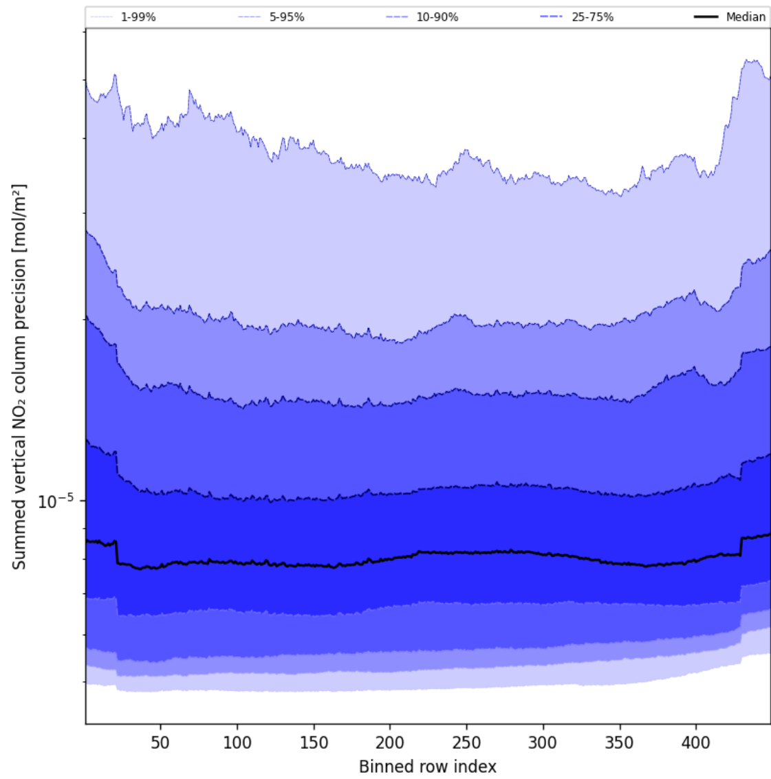
Figure 56: Along track statistics of “Summed vertical NO 2 column precision” for 2025-09-15 to 2025-09-16
