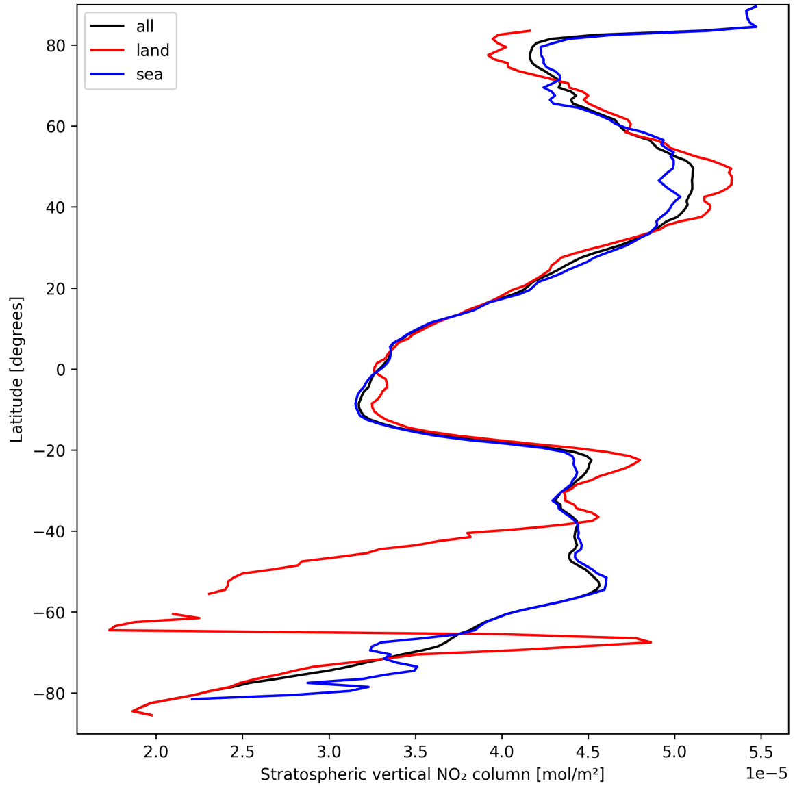
Figure 17: Zonal average of “Stratospheric vertical NO 2 column” for 2025-09-15 to 2025-09-16.
