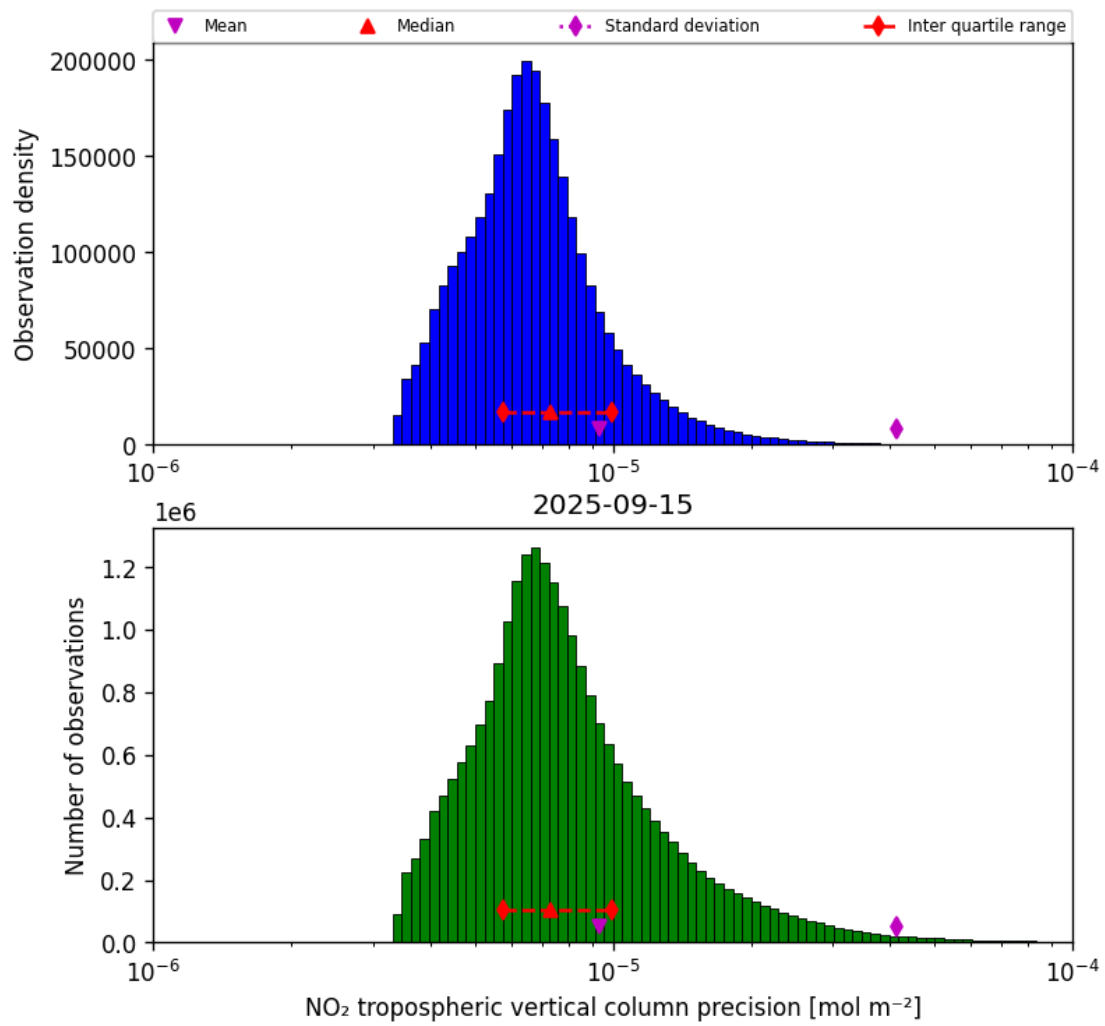
Figure 28: Histogram of “NO 2 tropospheric vertical column precision” for 2025-09-15 to 2025-09-16
