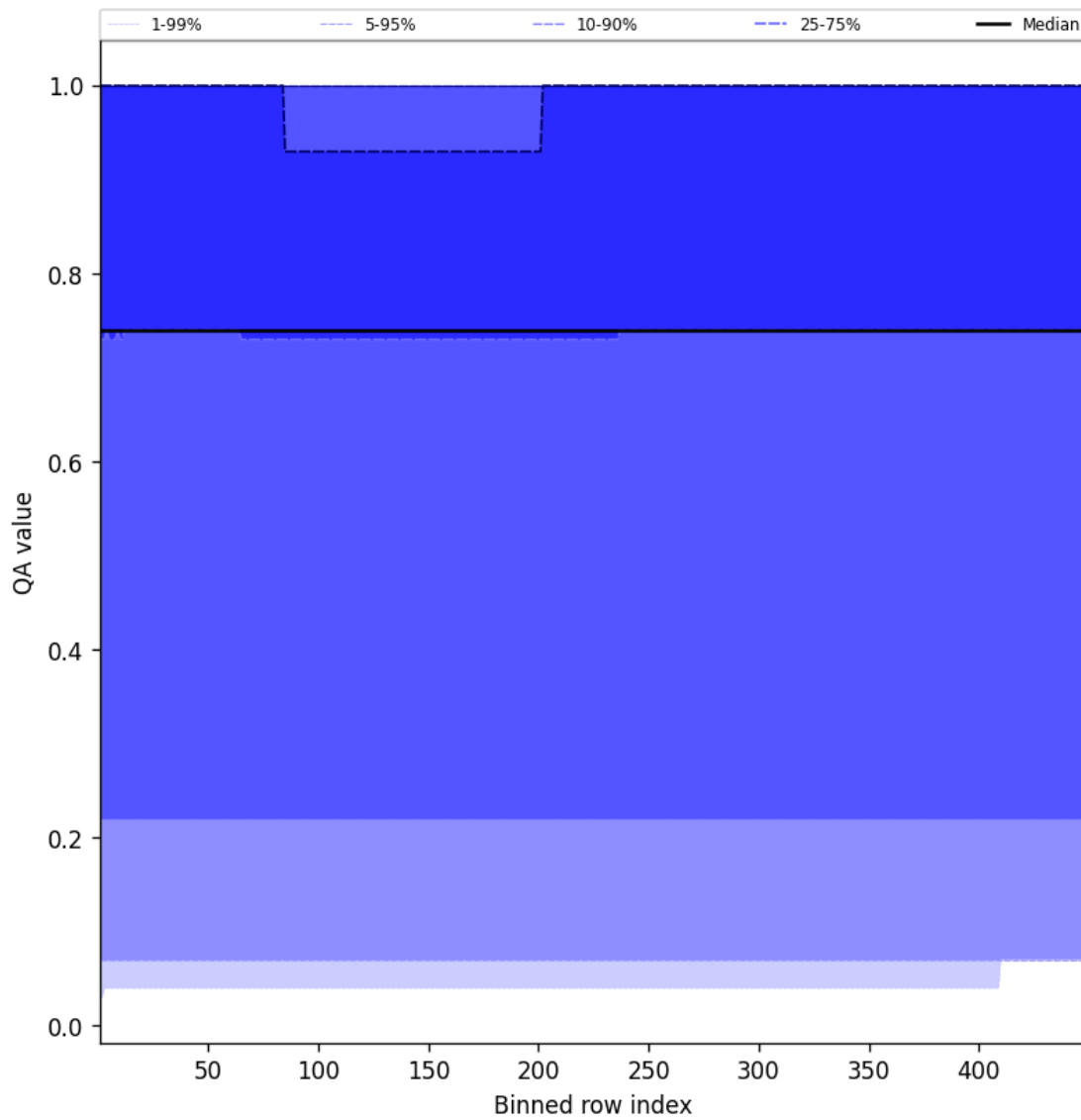
Figure 43: Along track statistics of “QA value” for 2025-09-15 to 2025-09-16
