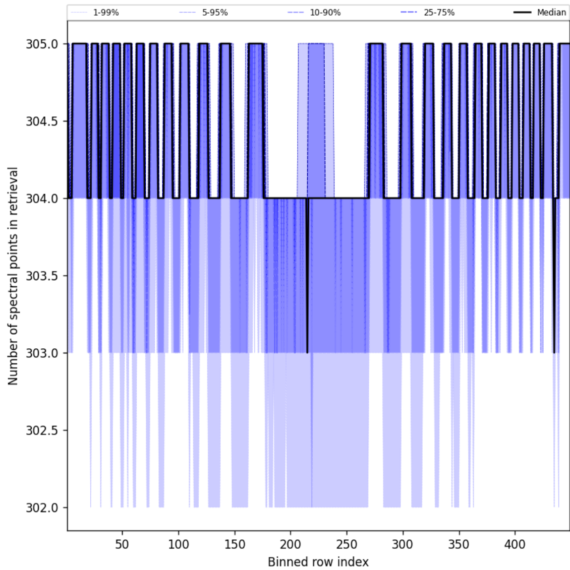
Figure 48: Along track statistics of “Number of spectral points in retrieval” for 2025-09-15 to 2025-09-16
