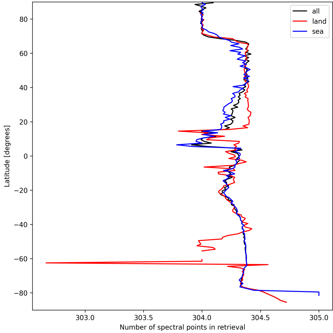
Figure 14: Zonal average of “Number of spectral points in retrieval” for 2025-09-15 to 2025-09-16.
