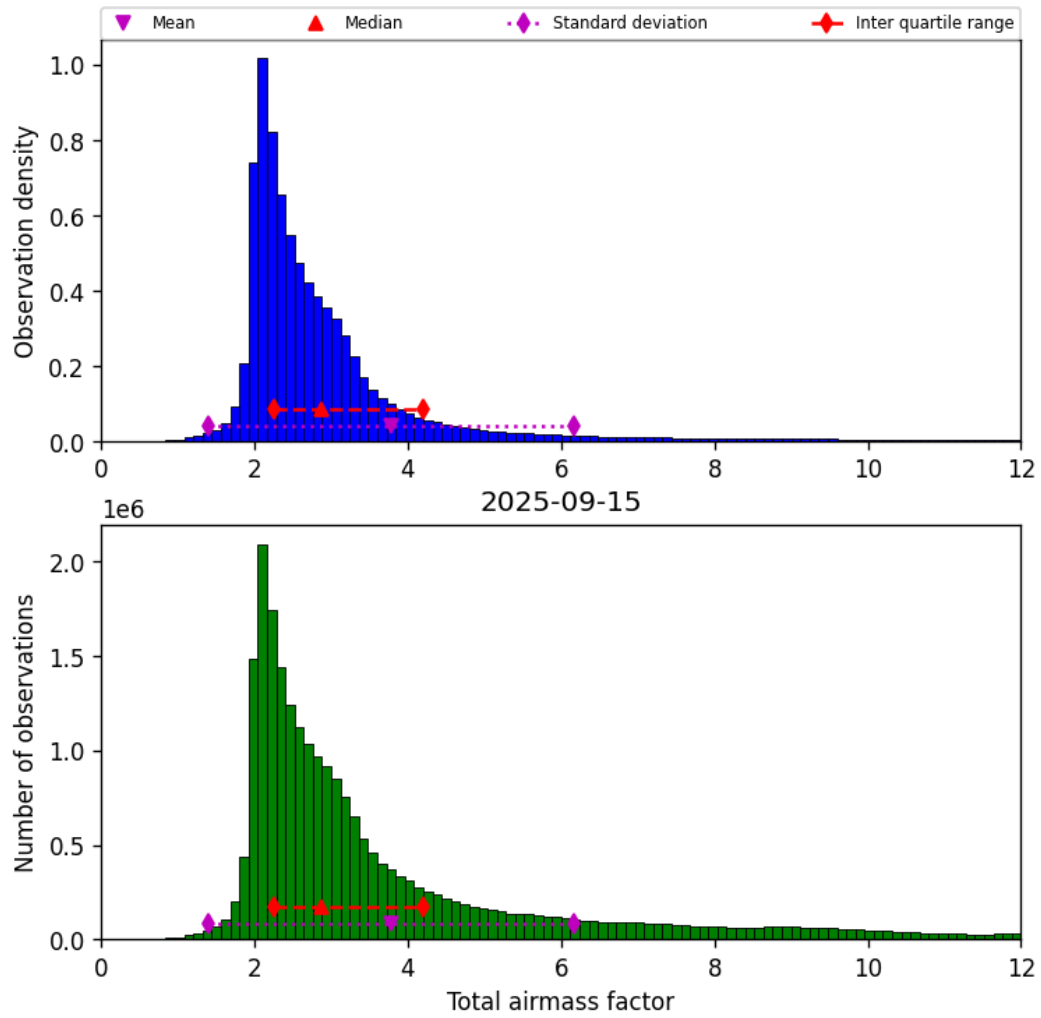
Figure 30: Histogram of “Total airmass factor” for 2025-09-15 to 2025-09-16
