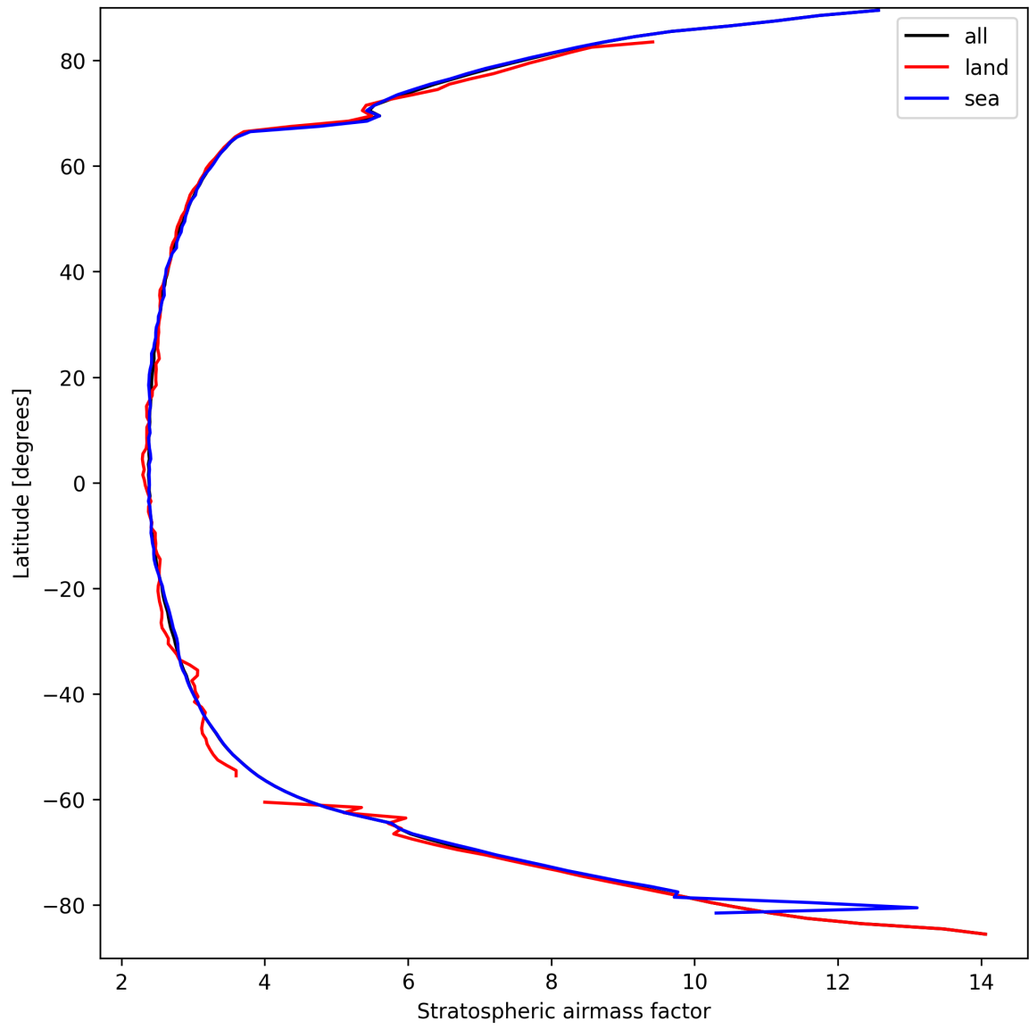
Figure 25: Zonal average of “Stratospheric airmass factor” for 2025-09-15 to 2025-09-16.
