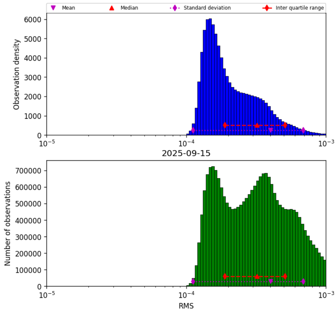
Figure 41: Histogram of “RMS” for 2025-09-15 to 2025-09-16
