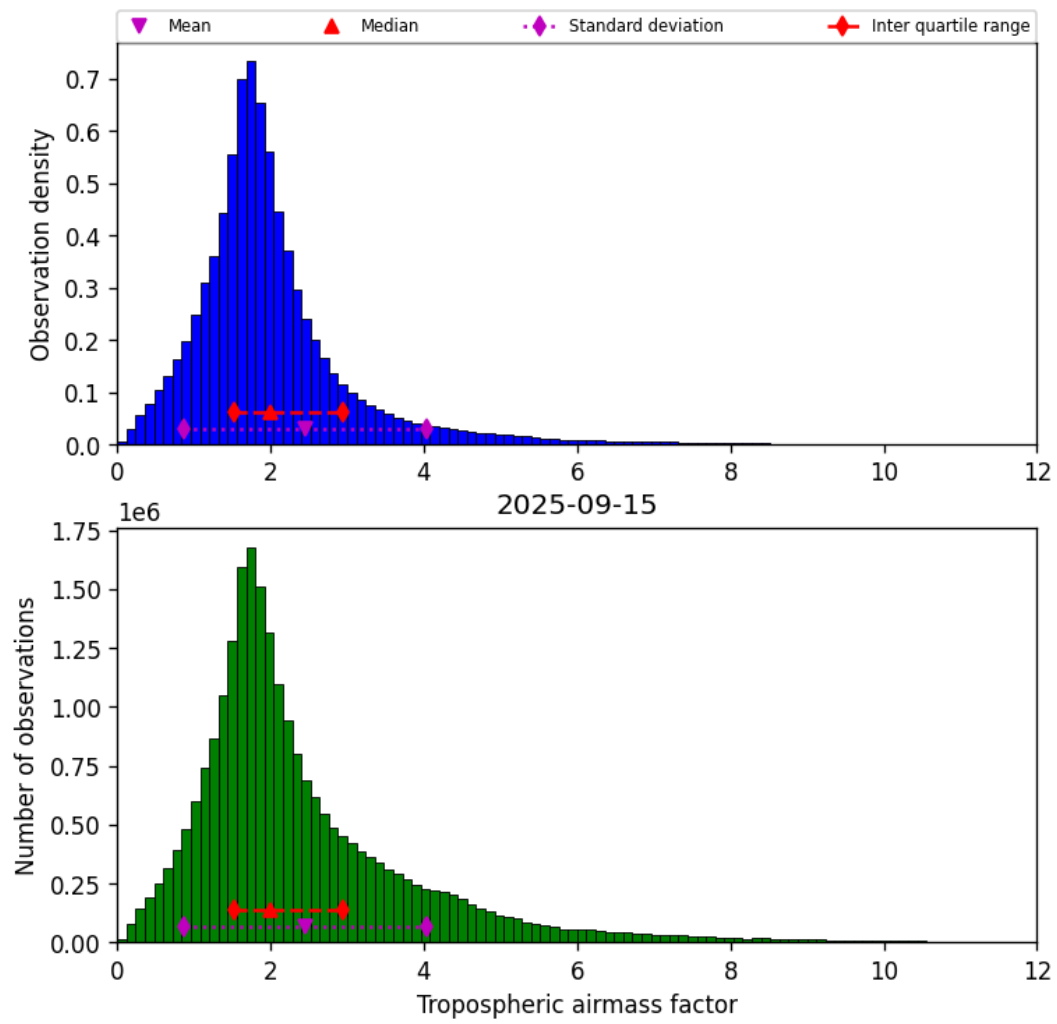
Figure 29: Histogram of “Tropospheric airmass factor” for 2025-09-15 to 2025-09-16
