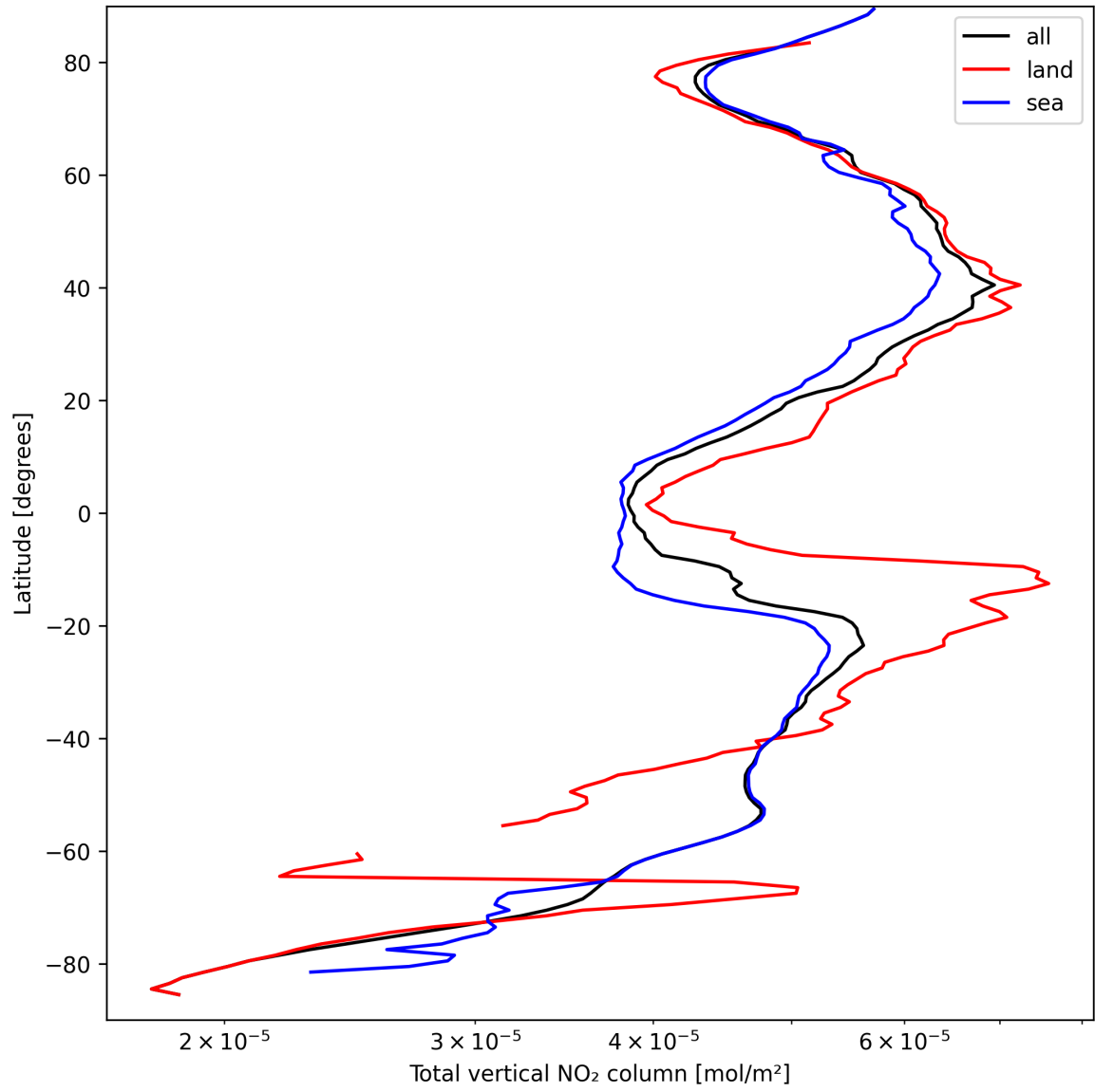
Figure 19: Zonal average of “Total vertical NO 2 column” for 2025-09-15 to 2025-09-16.
