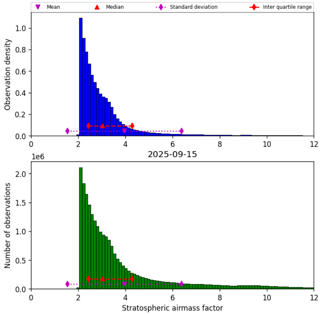
Figure 42: Histogram of “Stratospheric airmass factor” for 2025-09-15 to 2025-09-16
