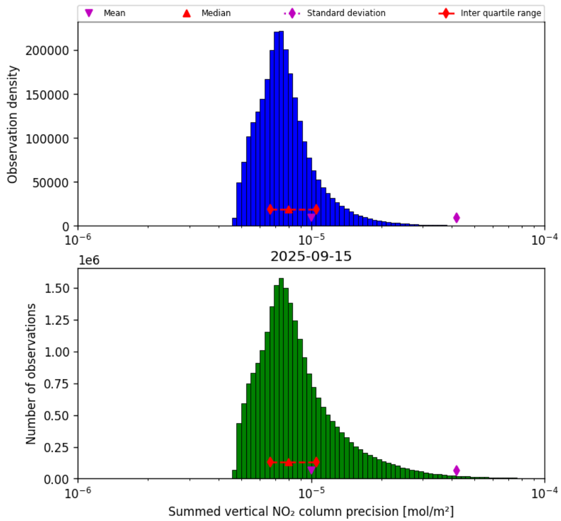
Figure 39: Histogram of “Summed vertical NO 2 column precision” for 2025-09-15 to 2025-09-16
