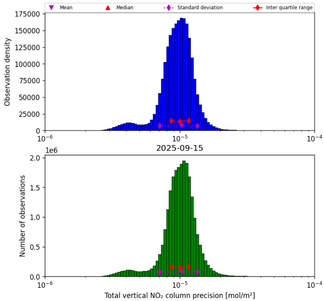
Figure 37: Histogram of “Total vertical NO 2 column precision” for 2025-09-15 to 2025-09-16
