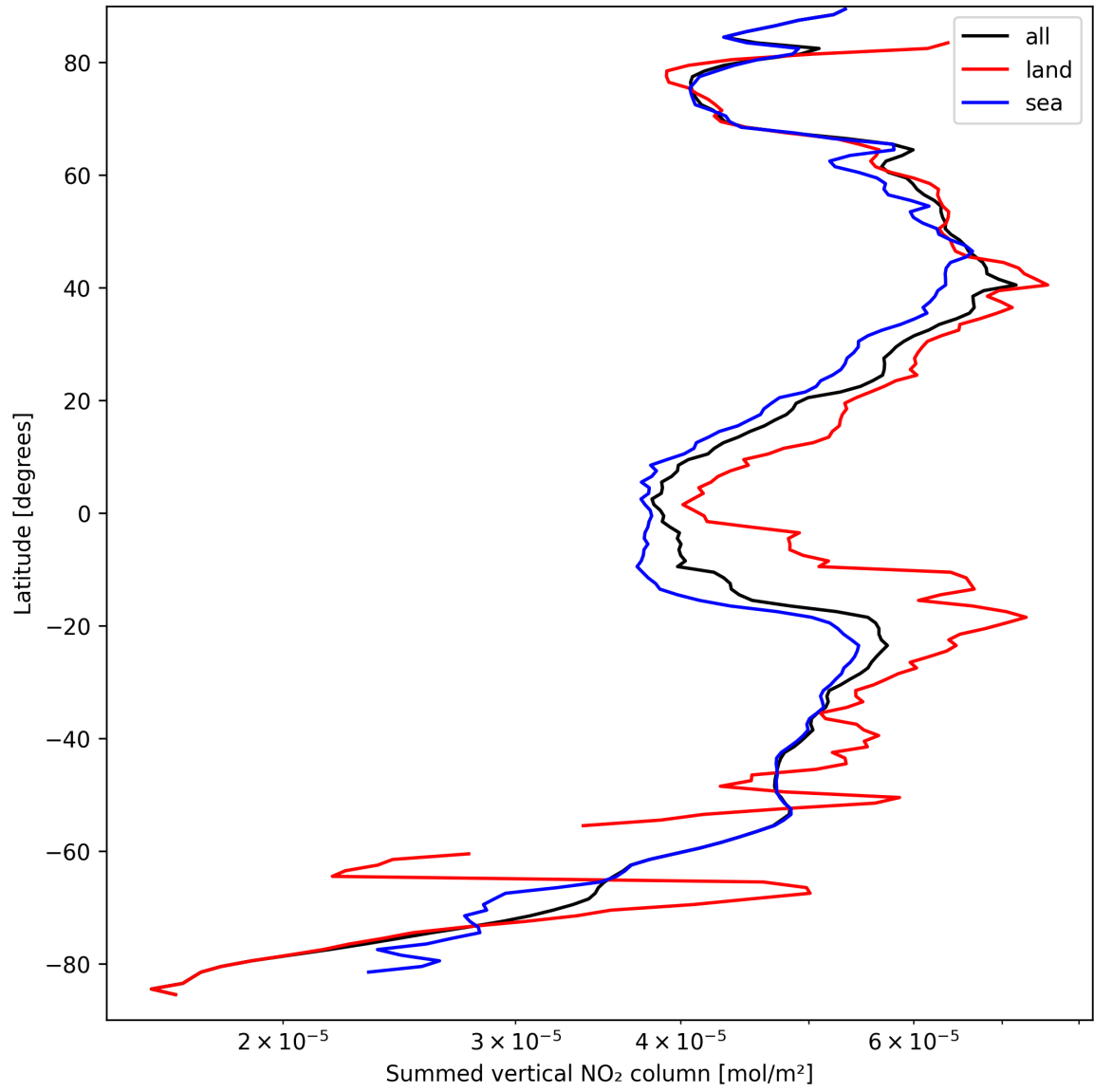
Figure 21: Zonal average of “Summed vertical NO 2 column” for 2025-09-15 to 2025-09-16.
