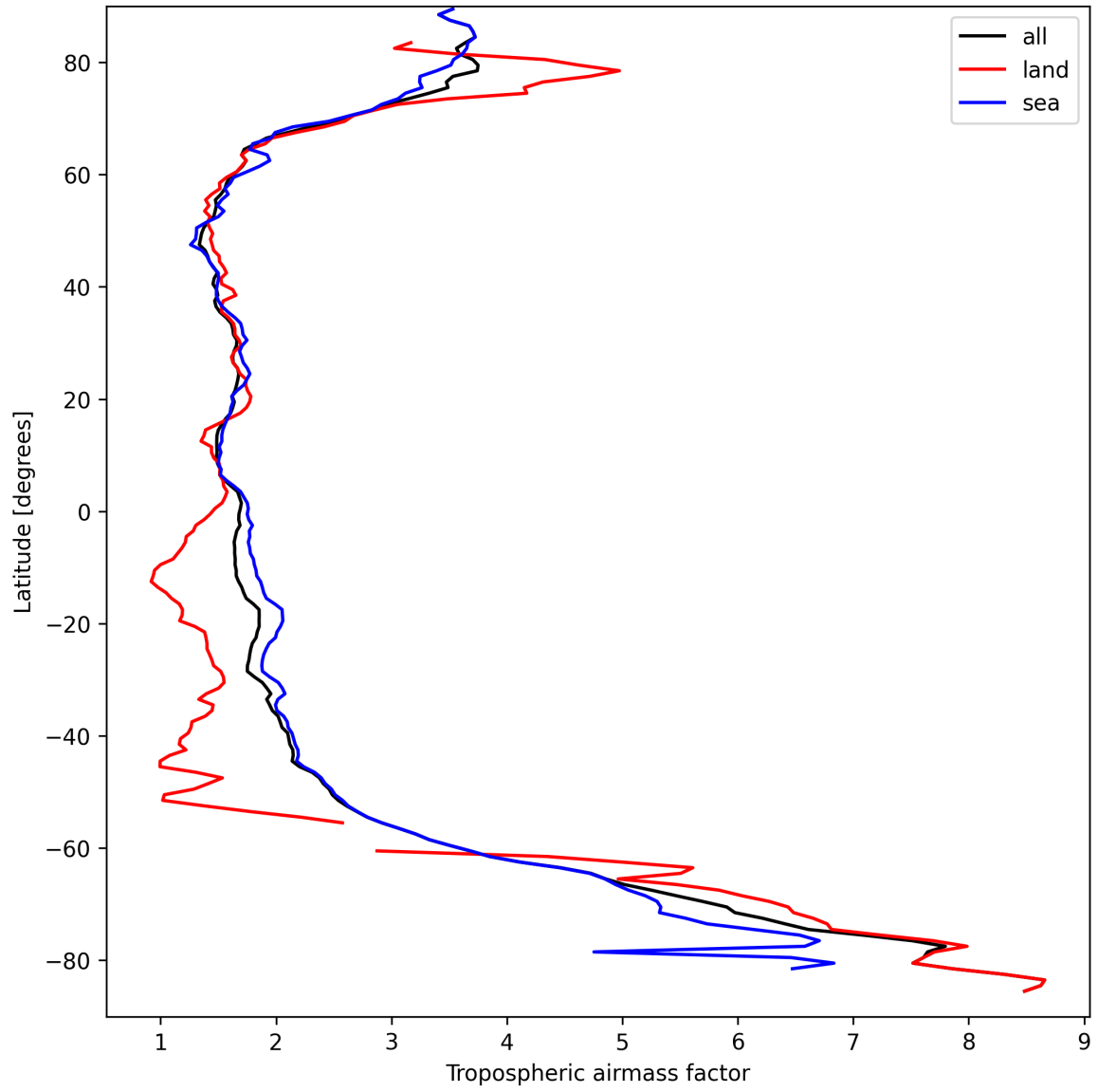
Figure 12: Zonal average of “Tropospheric air mass factor” for 2025-09-15 to 2025-09-16.
