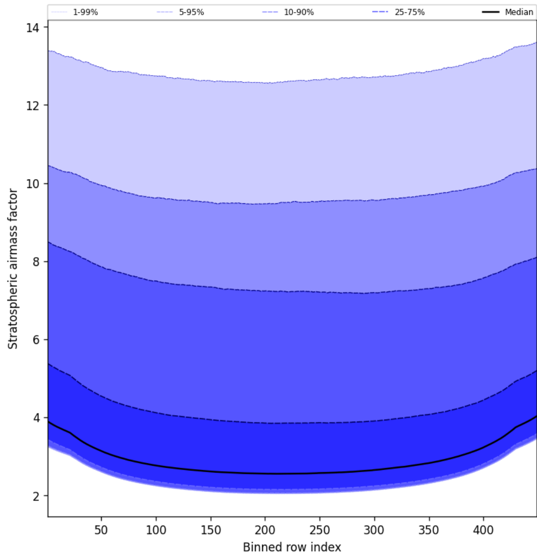
Figure 59: Along track statistics of “Stratospheric airmass factor” for 2025-09-15 to 2025-09-16
