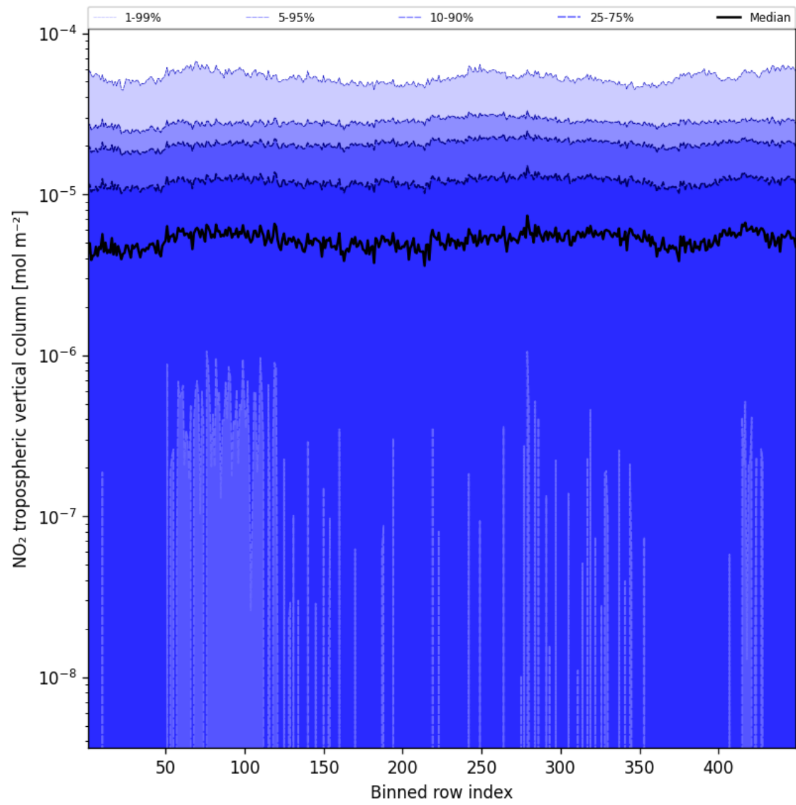
Figure 44: Along track statistics of “NO 2 tropospheric vertical column” for 2025-09-15 to 2025-09-16
