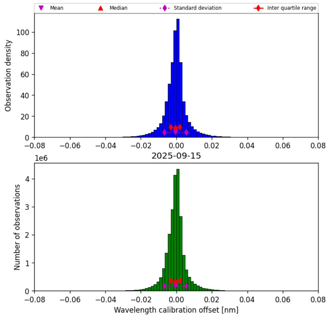
Figure 33: Histogram of “Wavelength calibration offset” for 2025-09-15 to 2025-09-16
