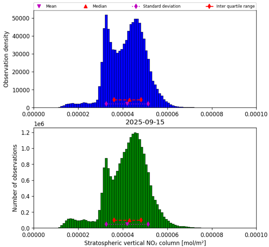
Figure 34: Histogram of “Stratospheric vertical NO 2 column” for 2025-09-15 to 2025-09-16
