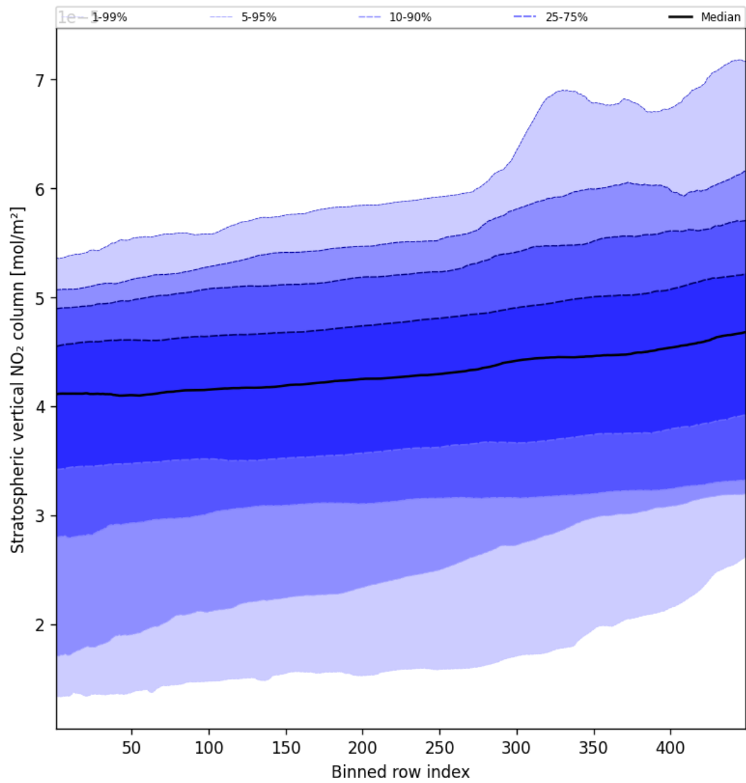
Figure 51: Along track statistics of “Stratospheric vertical NO 2 column” for 2025-09-15 to 2025-09-16
