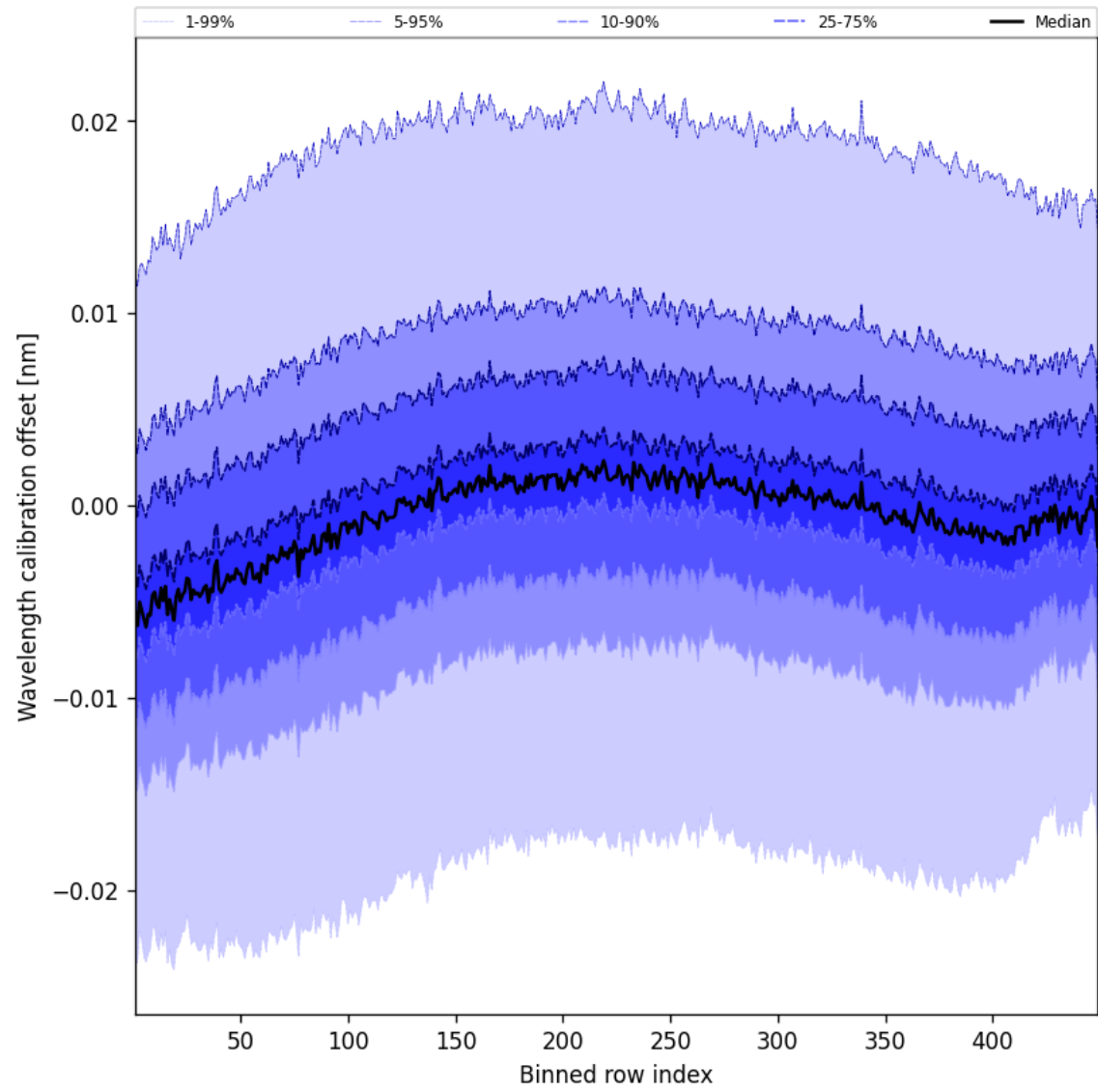
Figure 50: Along track statistics of “Wavelength calibration offset” for 2025-09-15 to 2025-09-16
