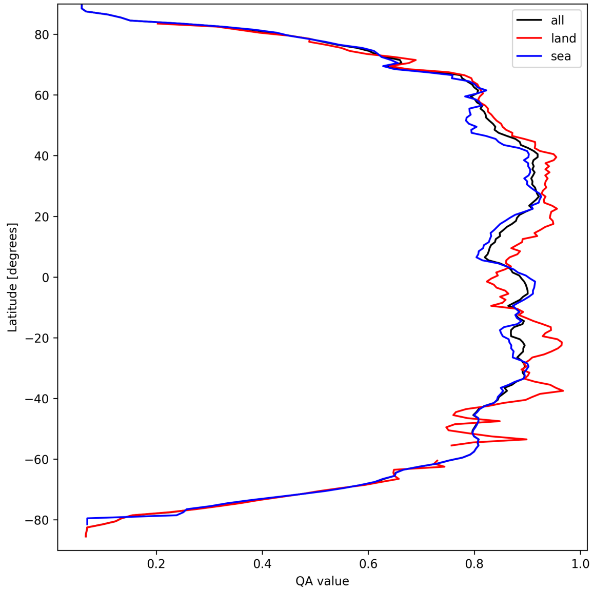
Figure 9: Zonal average of “QA value” for 2025-09-15 to 2025-09-16.
