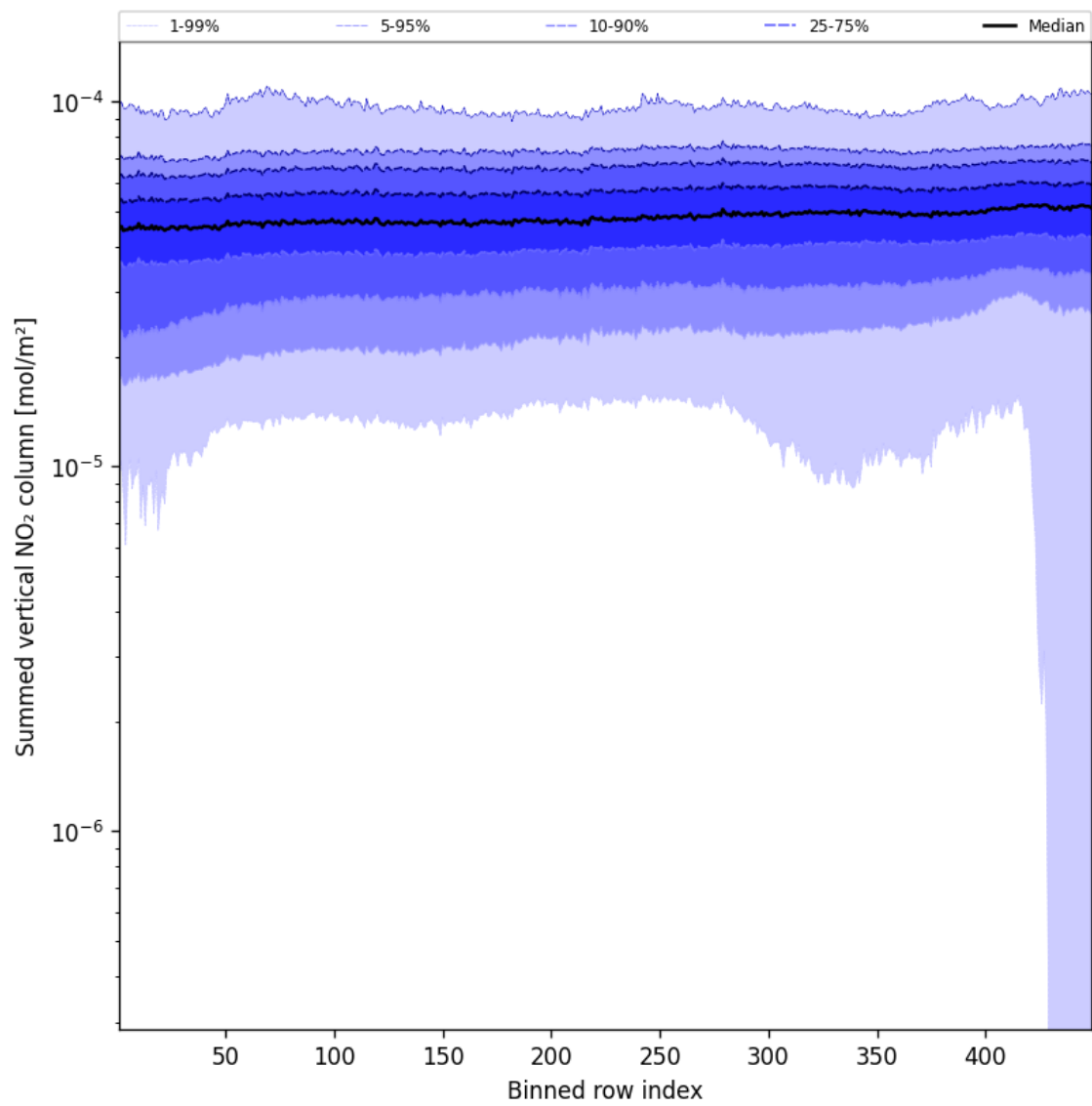
Figure 55: Along track statistics of “Summed vertical NO 2 column” for 2025-09-15 to 2025-09-16
