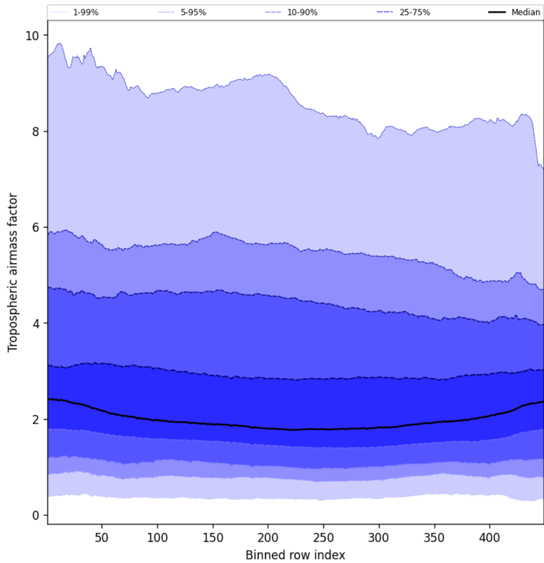
Figure 46: Along track statistics of “Tropospheric airmass factor” for 2025-09-15 to 2025-09-16
