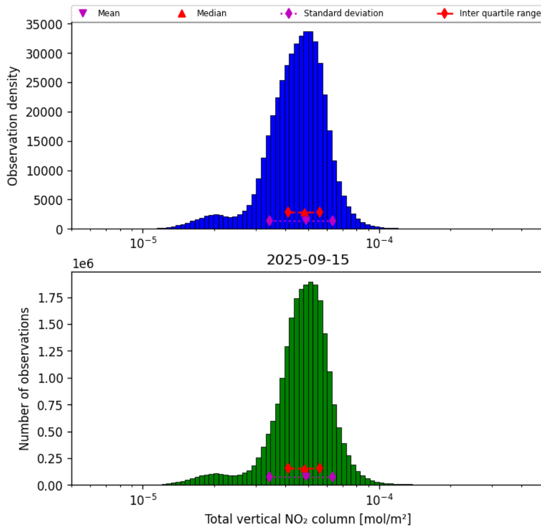
Figure 36: Histogram of “Total vertical NO 2 column” for 2025-09-15 to 2025-09-16
