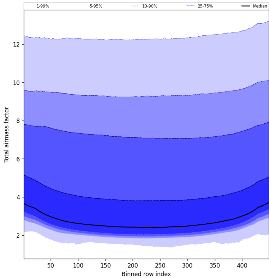
Figure 47: Along track statistics of “Total airmass factor” for 2025-09-15 to 2025-09-16
