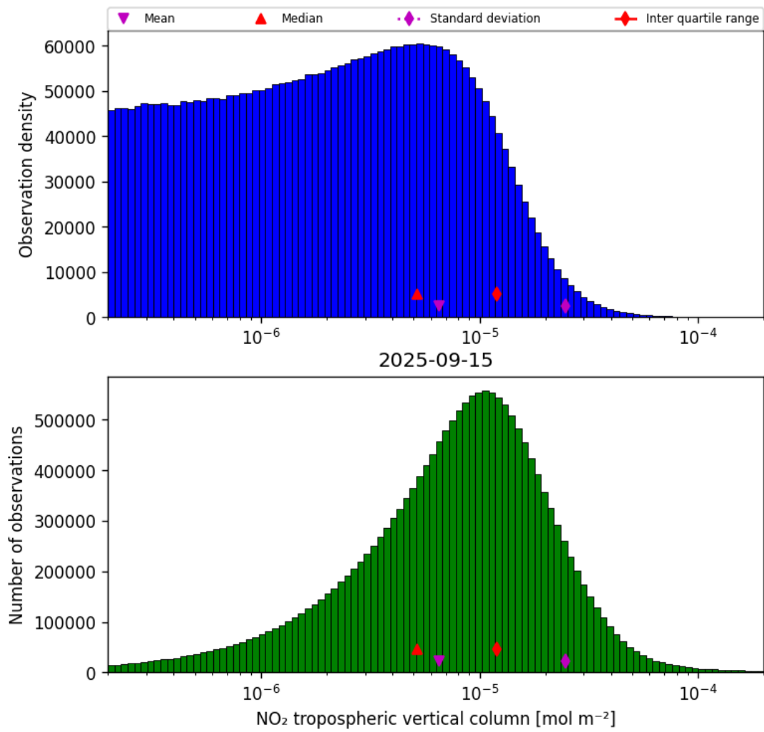
Figure 27: Histogram of “NO 2 tropospheric vertical column” for 2025-09-15 to 2025-09-16
