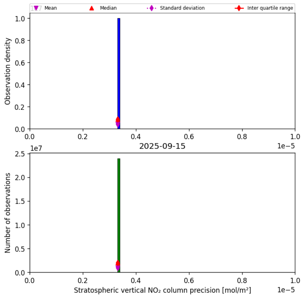
Figure 35: Histogram of “Stratospheric vertical NO 2 column precision” for 2025-09-15 to 2025-09-16
