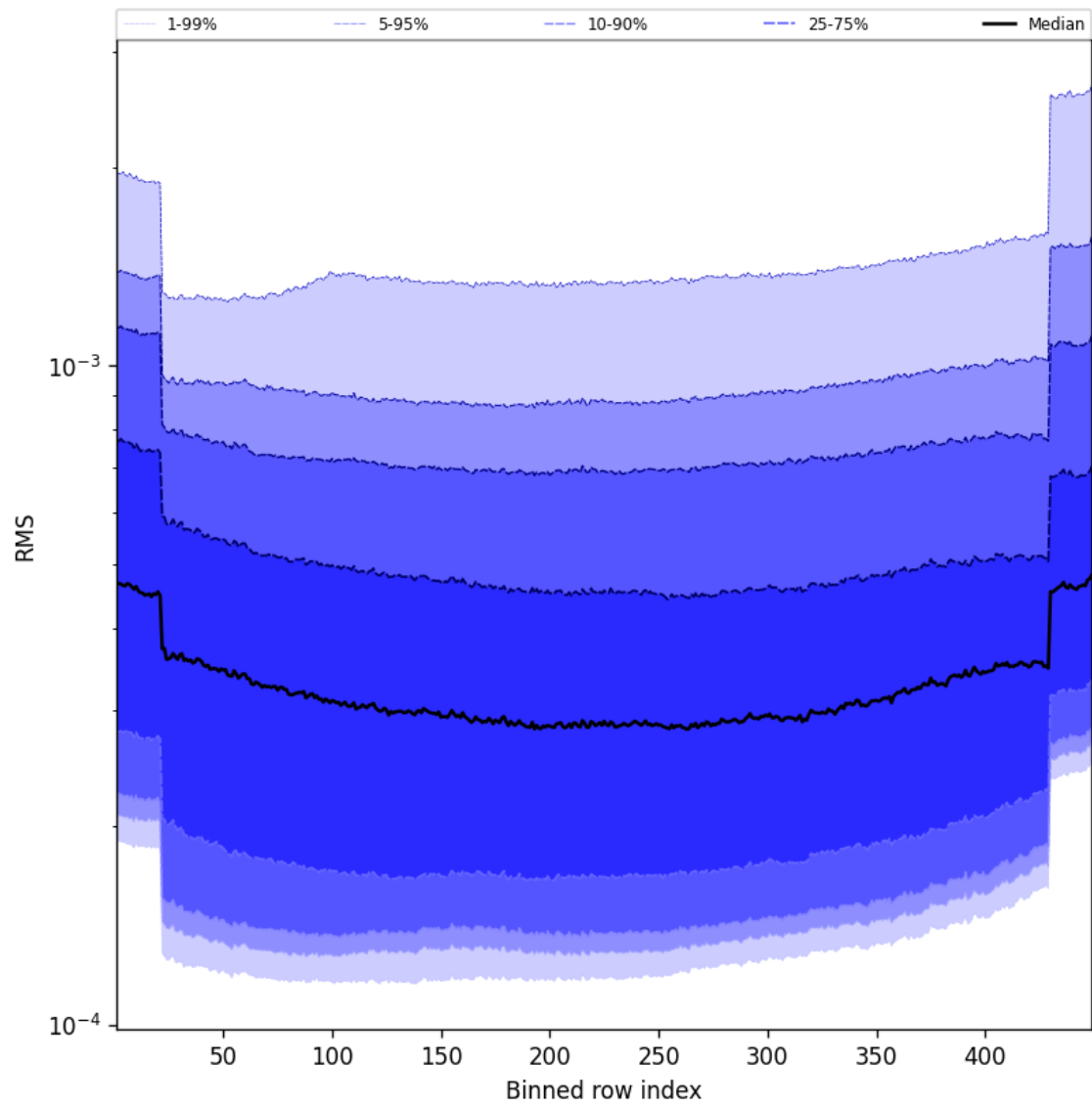
Figure 58: Along track statistics of “RMS” for 2025-09-15 to 2025-09-16
