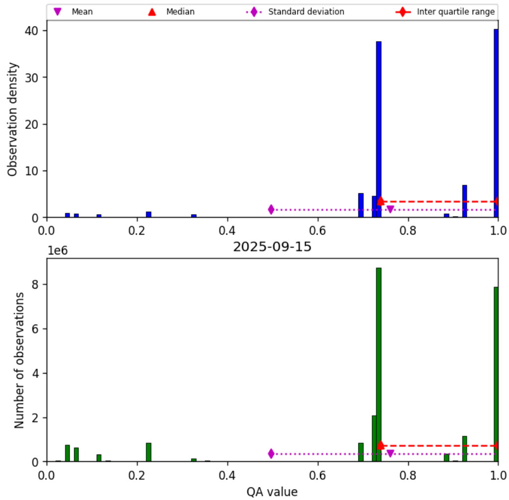
Figure 26: Histogram of “QA value” for 2025-09-15 to 2025-09-16
