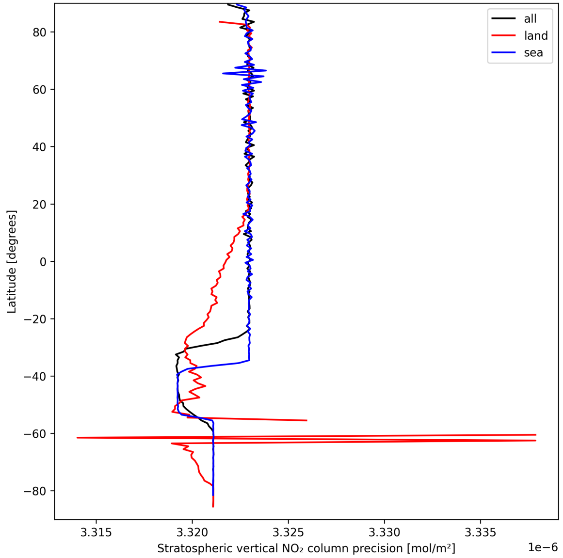
Figure 18: Zonal average of “Stratospheric vertical NO 2 column precision” for 2025-09-15 to 2025-09-16.
