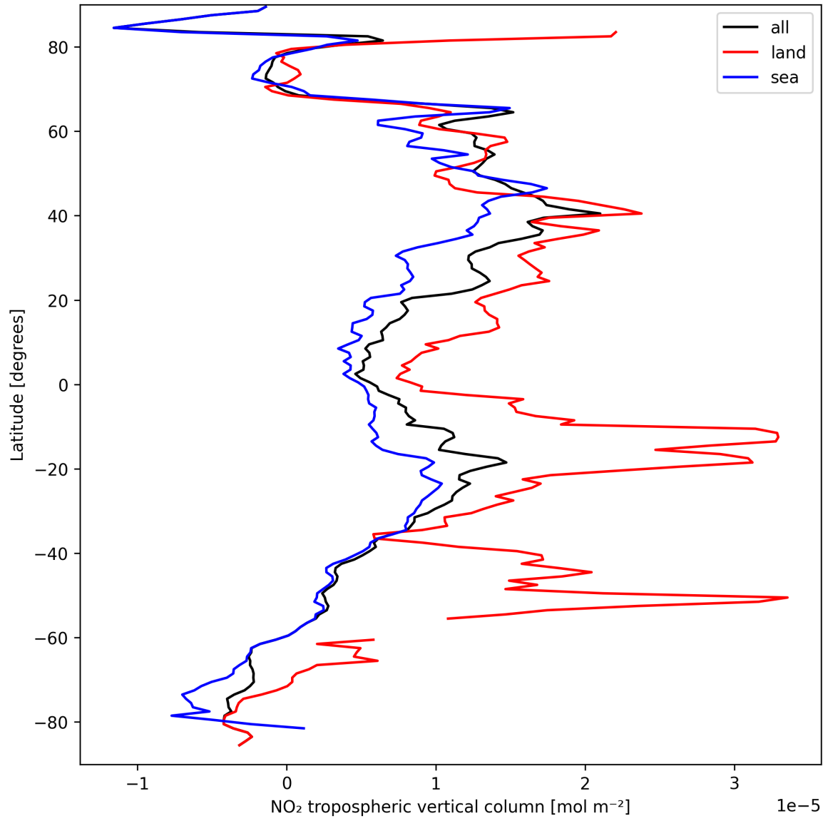
Figure 10: Zonal average of “NO 2 tropospheric vertical column” for 2025-09-15 to 2025-09-16.
