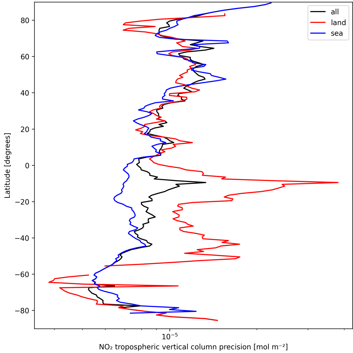
Figure 11: Zonal average of “NO 2 tropospheric vertical column precision” for 2025-09-15 to 2025-09-16.
