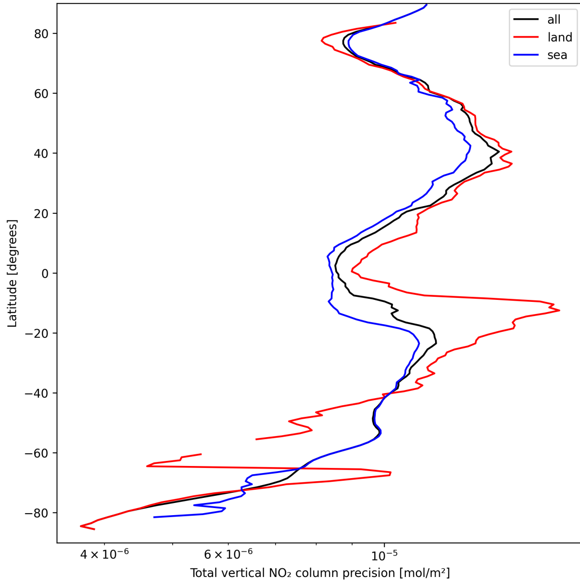
Figure 20: Zonal average of “Total vertical NO 2 column precision” for 2025-09-15 to 2025-09-16.
