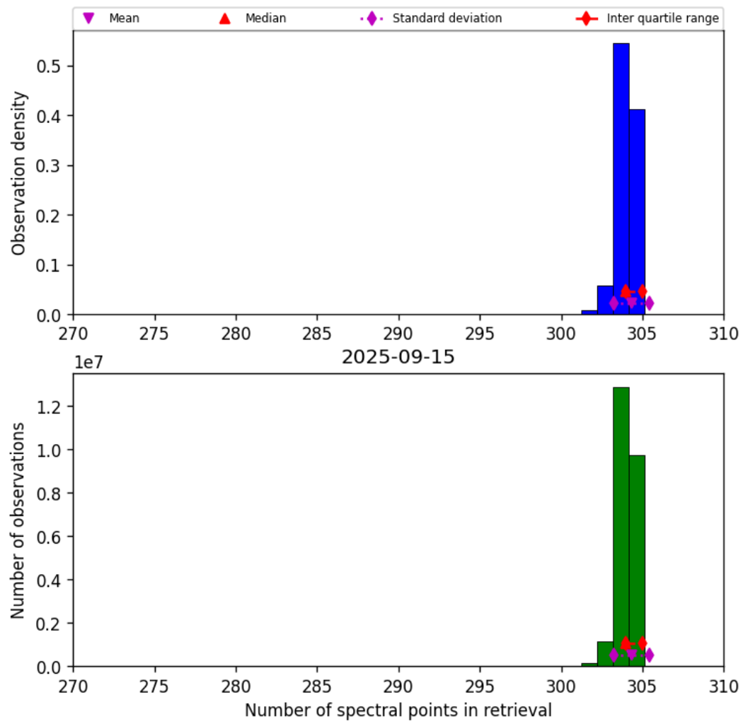
Figure 31: Histogram of “Number of spectral points in retrieval” for 2025-09-15 to 2025-09-16
