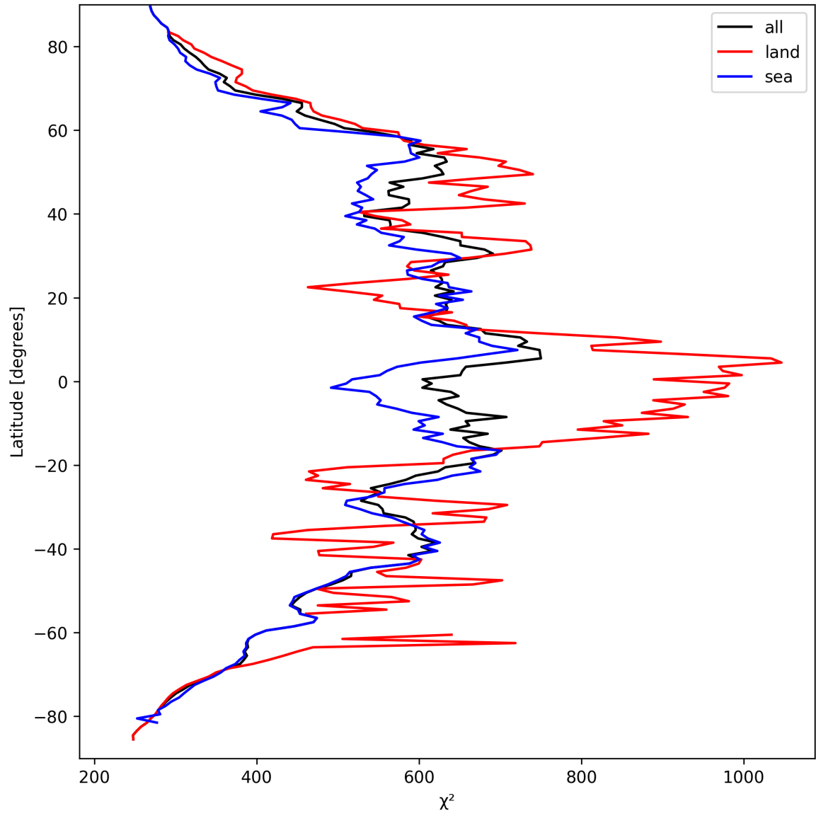
Figure 23: Zonal average of “ \chi^2 ” for 2025-09-15 to 2025-09-16.
