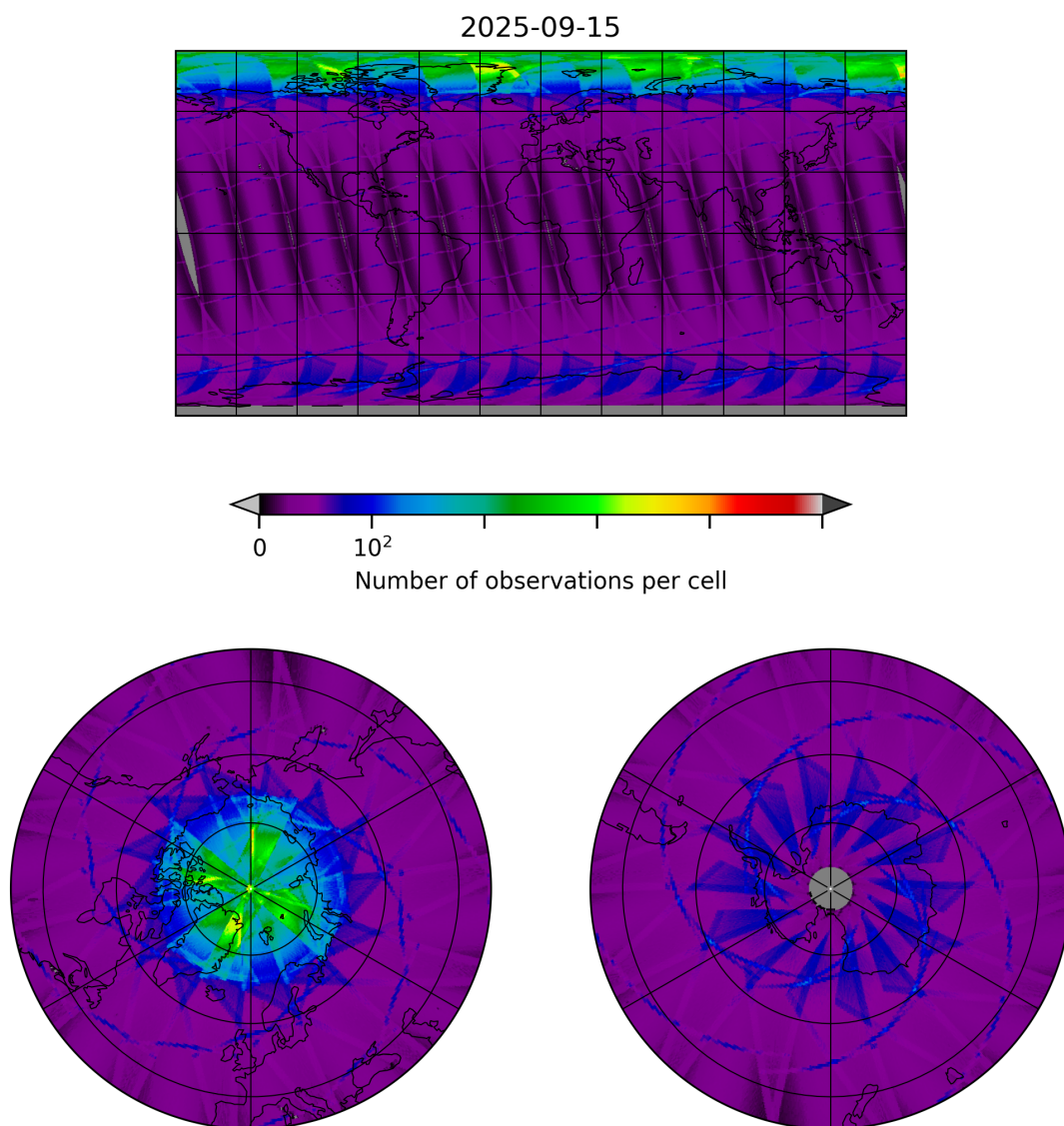
Figure 8: Map of the number of observations for 2025-09-15 to 2025-09-16
