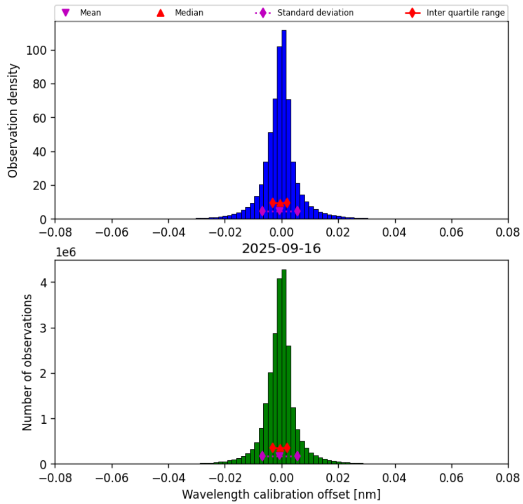
Figure 33: Histogram of “Wavelength calibration offset” for 2025-09-16 to 2025-09-17
