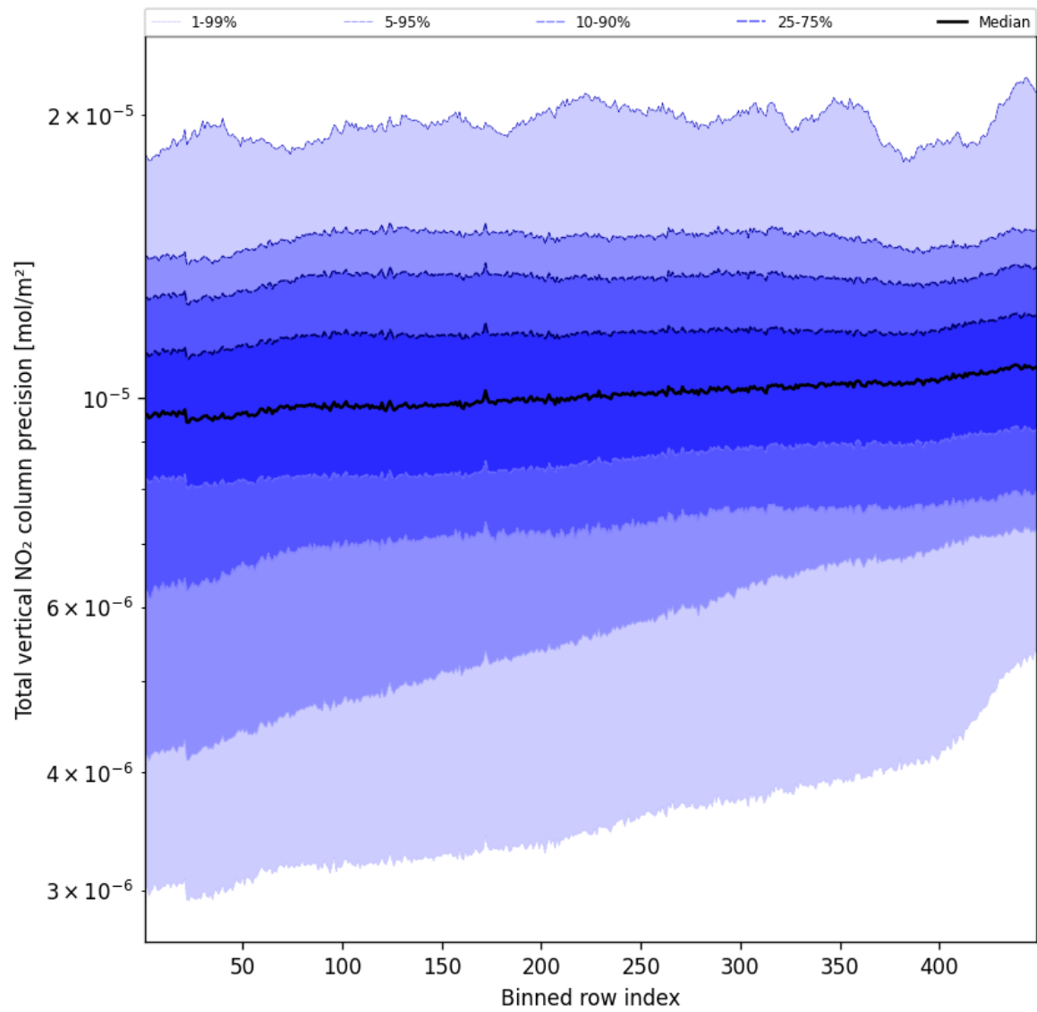
Figure 54: Along track statistics of "Total vertical NO 2 column precision" for 2025-09-16 to 2025-09-17
