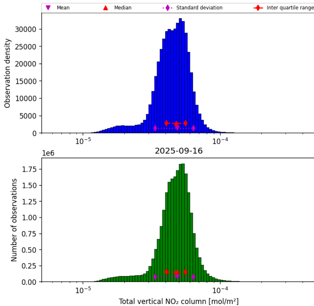
Figure 36: Histogram of “Total vertical NO 2 column” for 2025-09-16 to 2025-09-17
