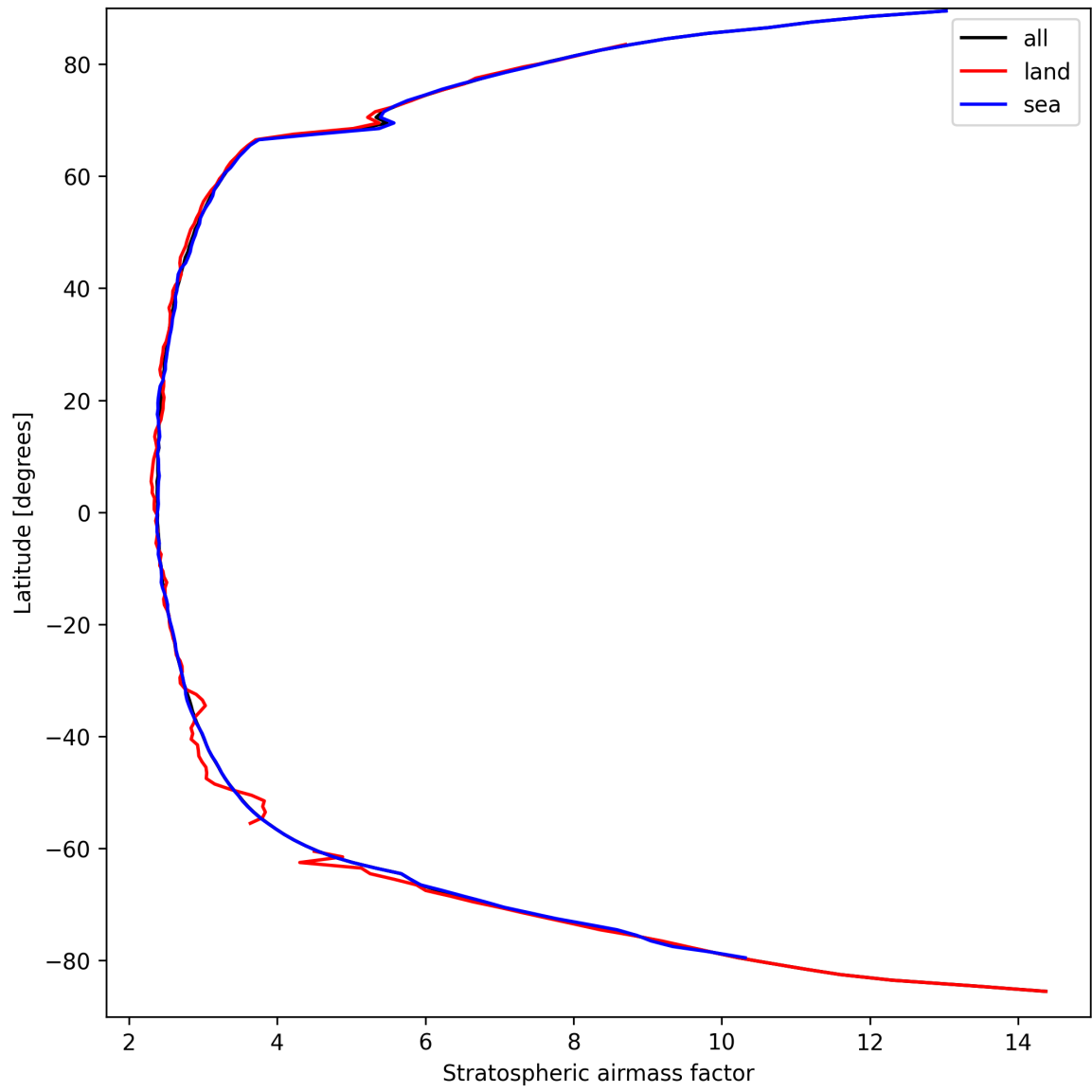
Figure 25: Zonal average of “Stratospheric airmass factor” for 2025-09-16 to 2025-09-17.
