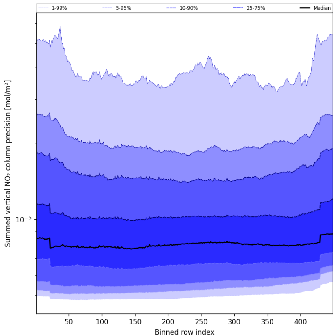
Figure 56: Along track statistics of “Summed vertical NO 2 column precision” for 2025-09-16 to 2025-09-17
