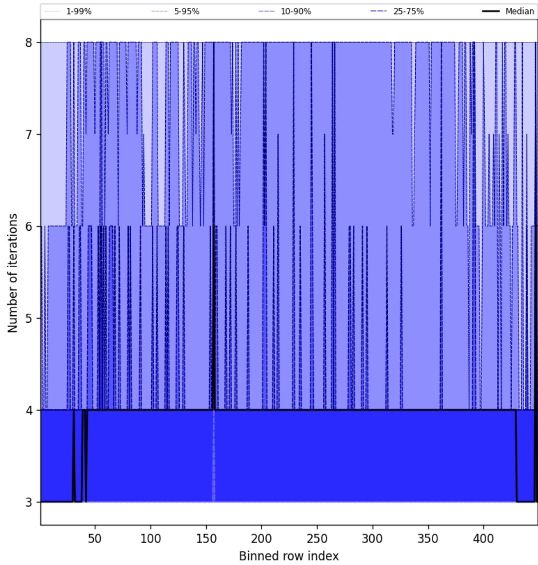
Figure 49: Along track statistics of “Number of iterations” for 2025-09-16 to 2025-09-17
