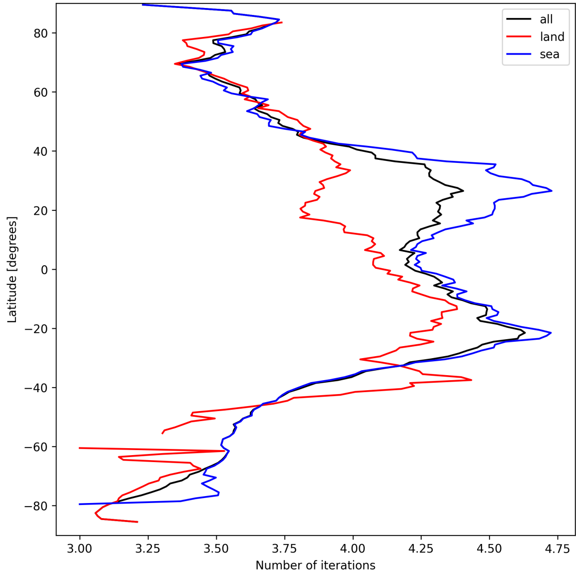
Figure 15: Zonal average of “Number of iterations” for 2025-09-16 to 2025-09-17.
