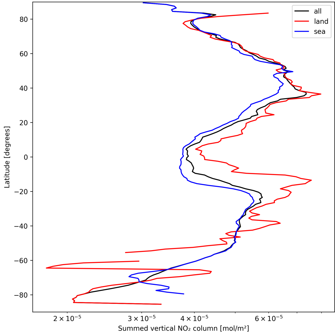
Figure 21: Zonal average of “Summed vertical NO 2 column” for 2025-09-16 to 2025-09-17.
