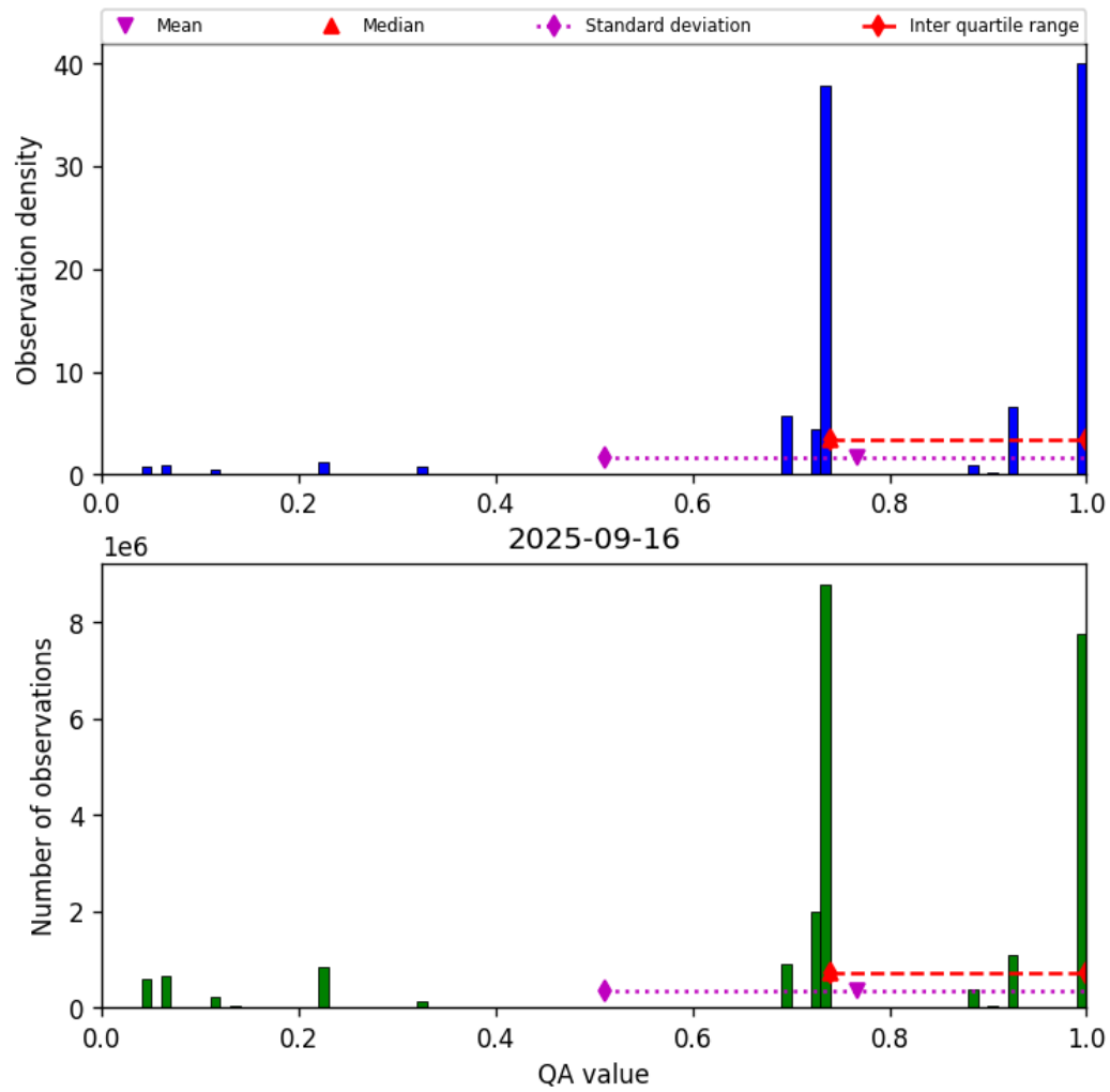
Figure 26: Histogram of “QA value” for 2025-09-16 to 2025-09-17
