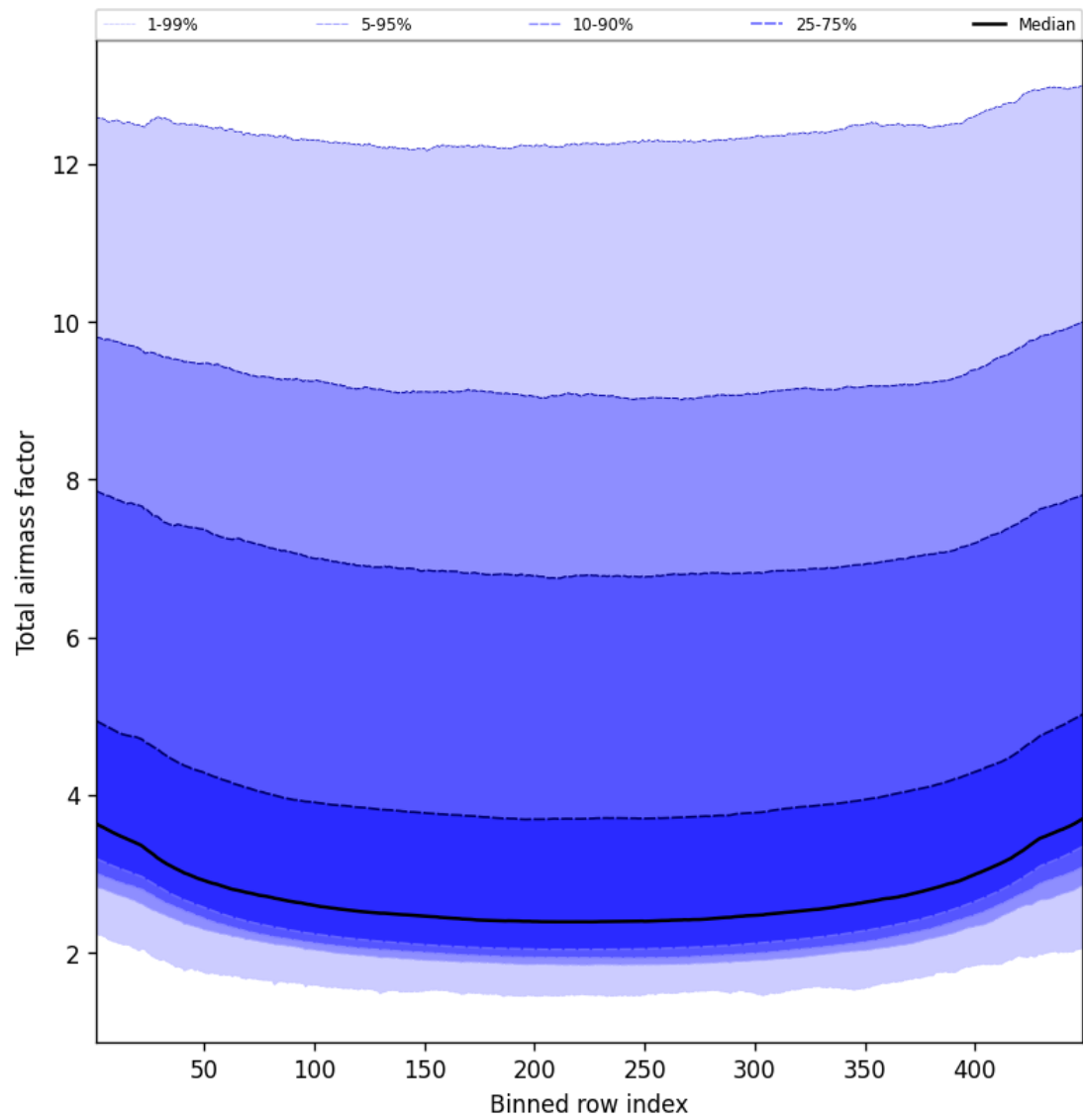
Figure 47: Along track statistics of “Total airmass factor” for 2025-09-16 to 2025-09-17
