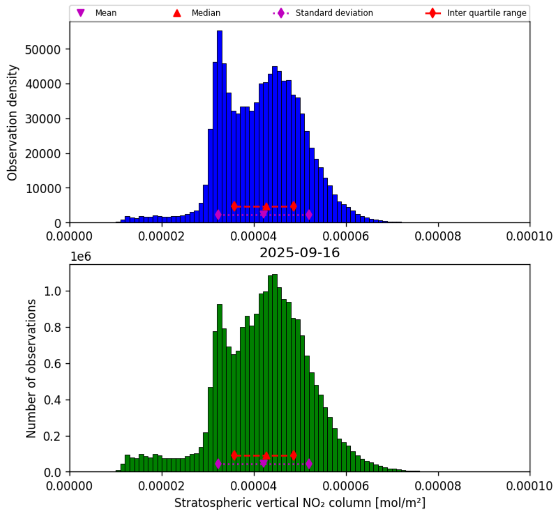
Figure 34: Histogram of “Stratospheric vertical NO 2 column” for 2025-09-16 to 2025-09-17
