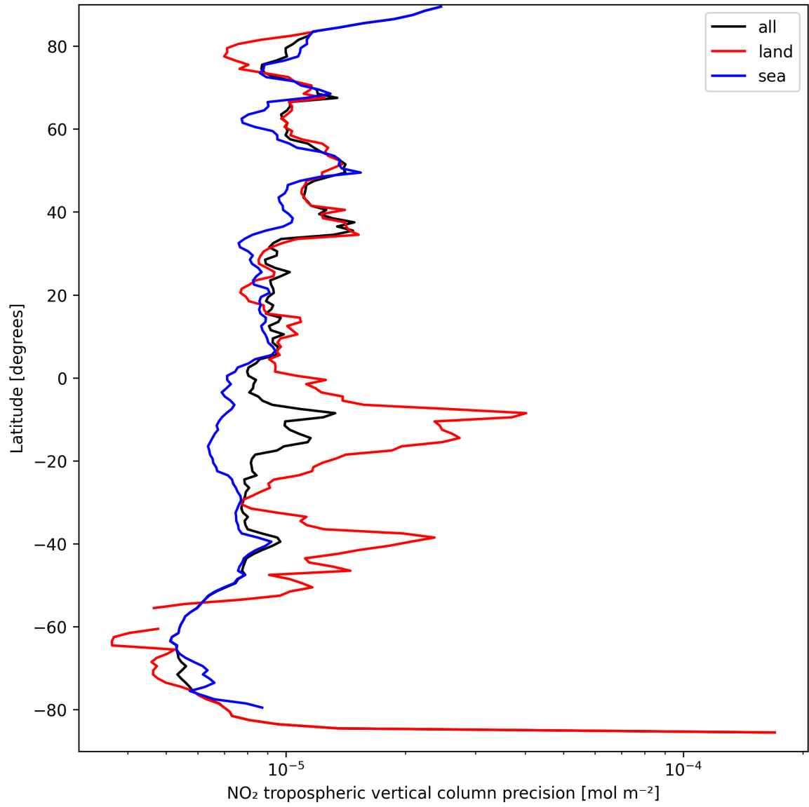
Figure 11: Zonal average of “NO 2 tropospheric vertical column precision” for 2025-09-16 to 2025-09-17.
