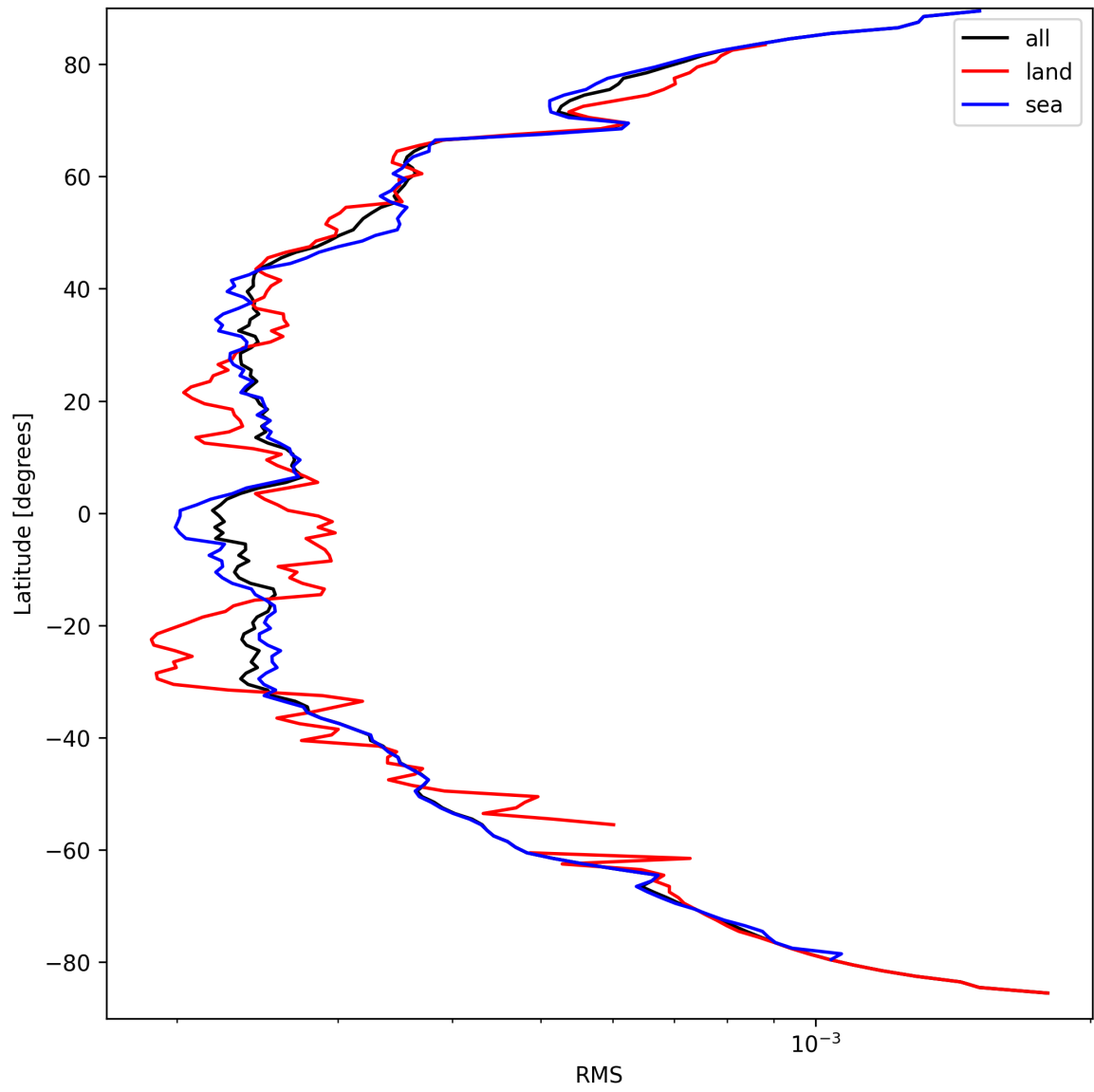
Figure 24: Zonal average of “RMS” for 2025-09-16 to 2025-09-17.
