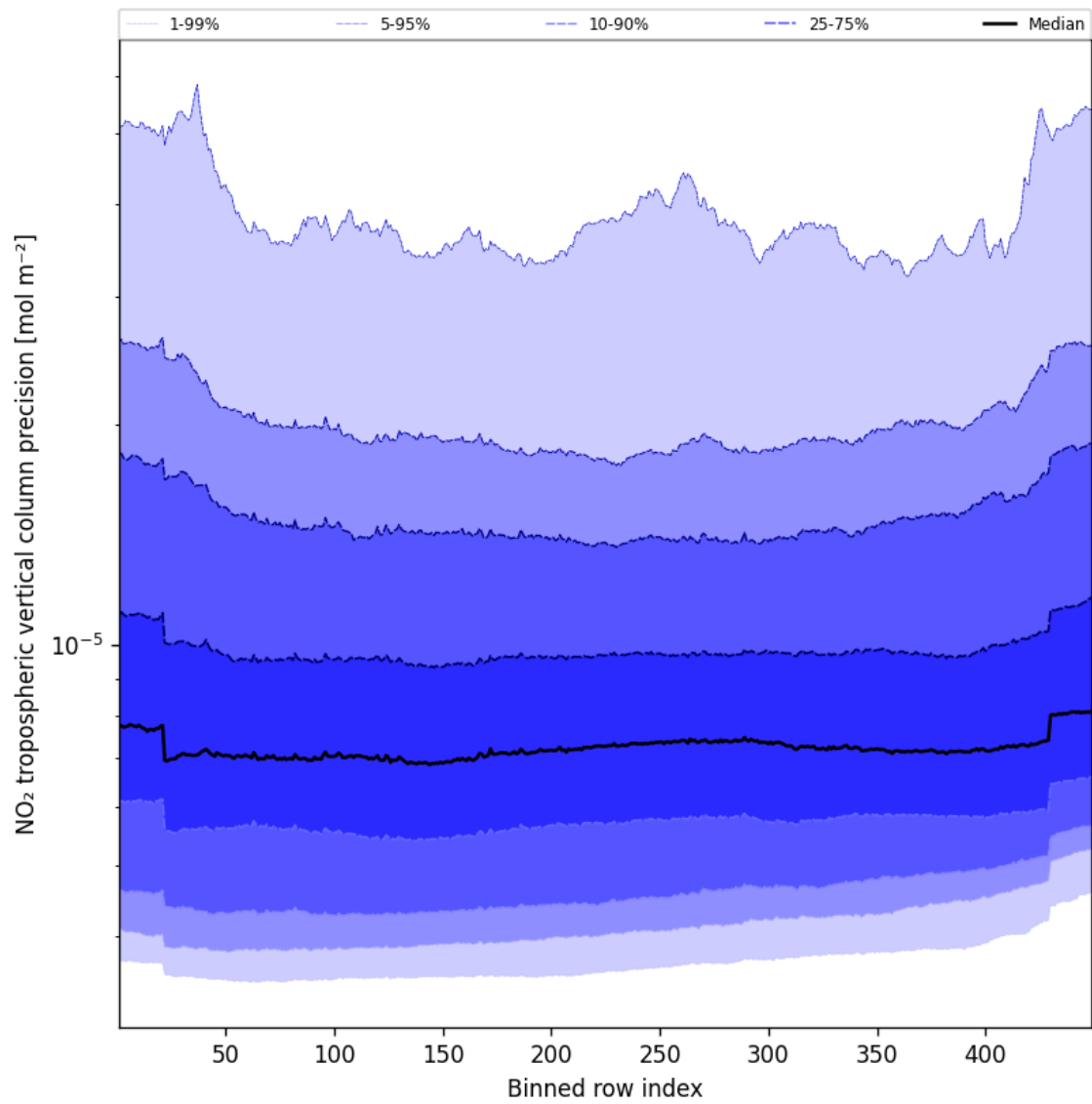
Figure 45: Along track statistics of “NO 2 tropospheric vertical column precision” for 2025-09-16 to 2025-09-17
