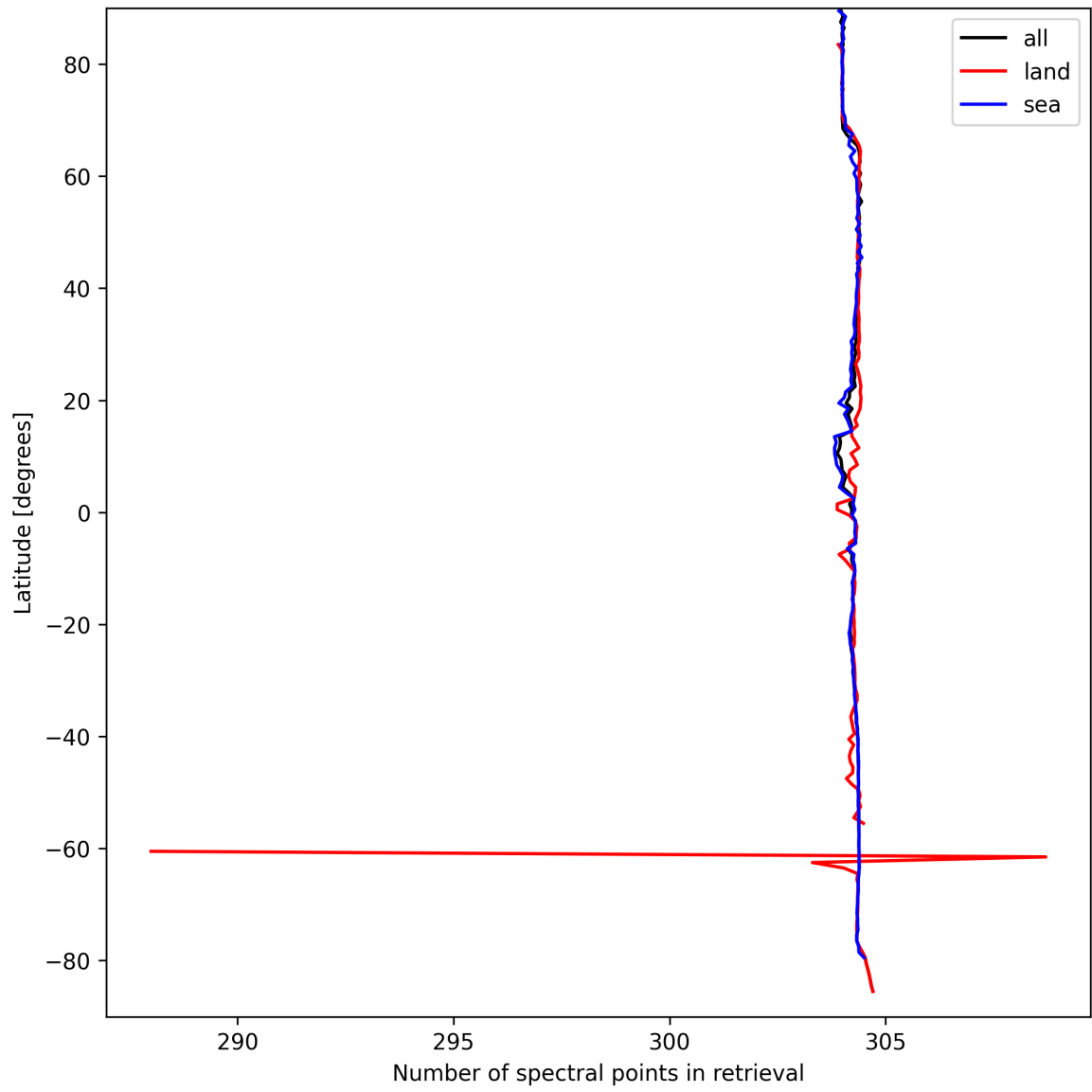
Figure 14: Zonal average of “Number of spectral points in retrieval” for 2025-09-16 to 2025-09-17.
