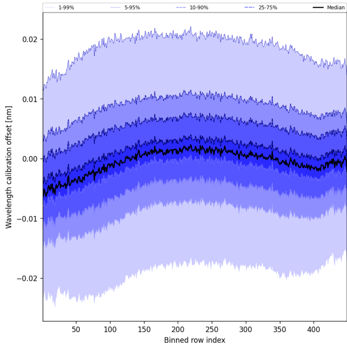
Figure 50: Along track statistics of “Wavelength calibration offset” for 2025-09-16 to 2025-09-17
