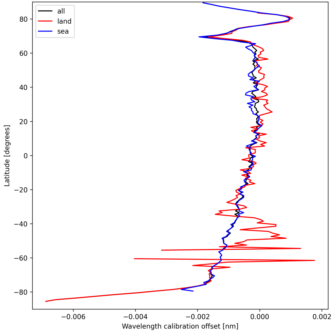
Figure 16: Zonal average of “Wavelength calibration offset” for 2025-09-16 to 2025-09-17.
