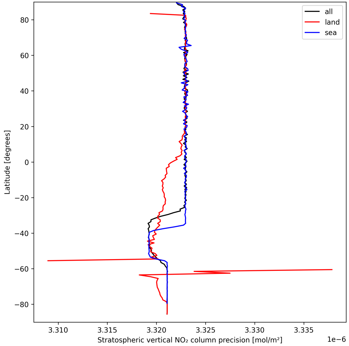
Figure 18: Zonal average of “Stratospheric vertical NO 2 column precision” for 2025-09-16 to 2025-09-17.
