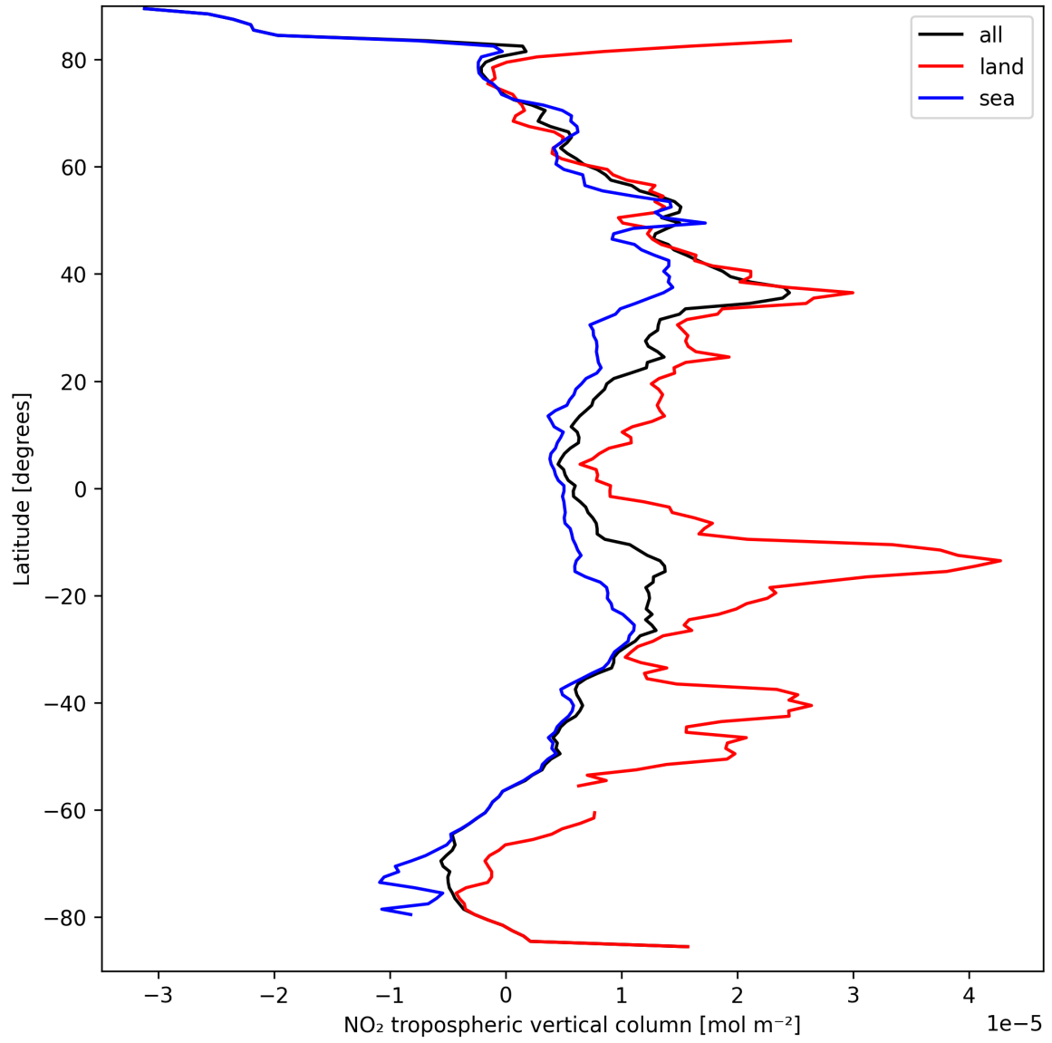
Figure 10: Zonal average of “NO 2 tropospheric vertical column” for 2025-09-16 to 2025-09-17.
