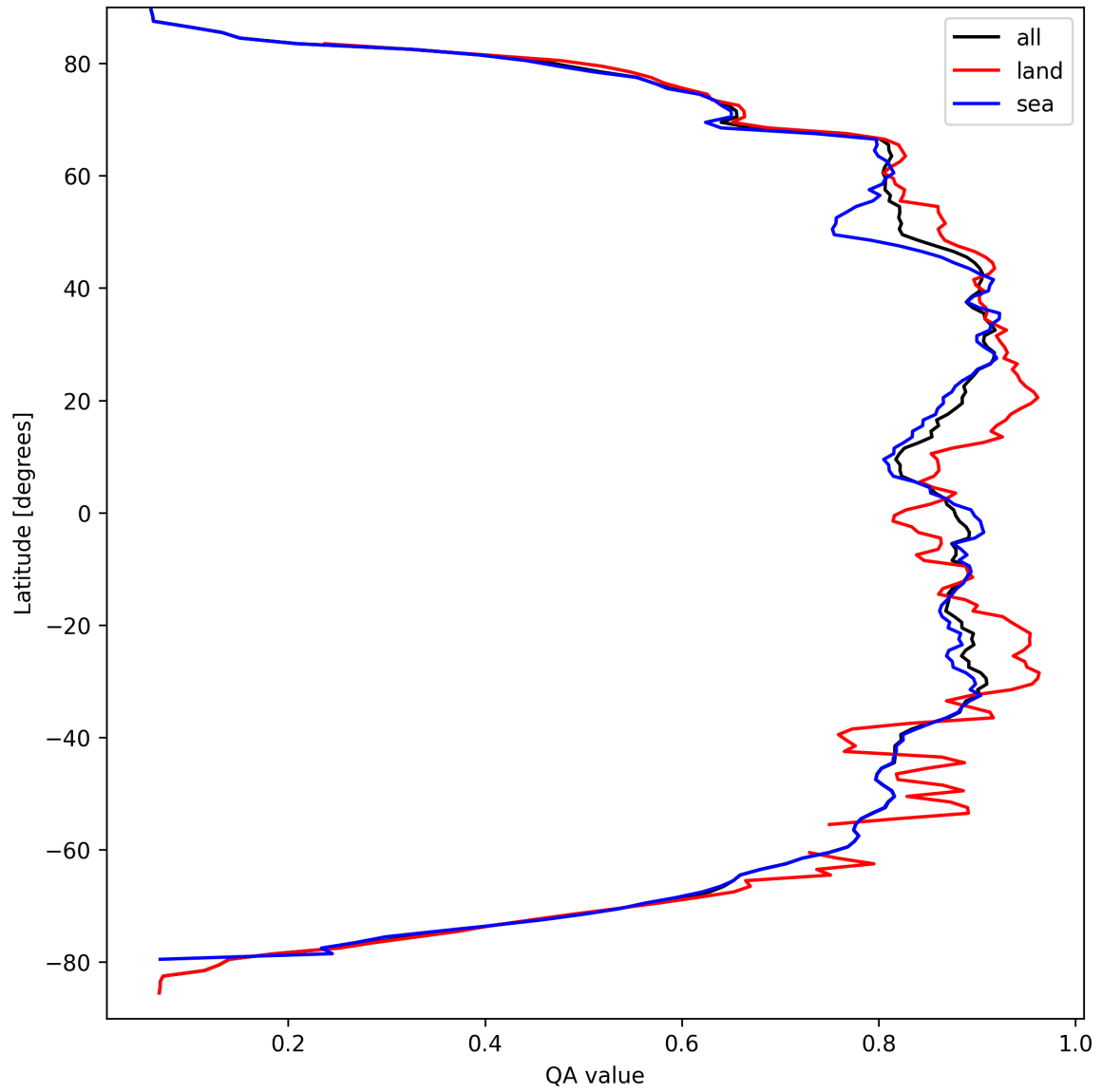
Figure 9: Zonal average of “QA value” for 2025-09-16 to 2025-09-17.
