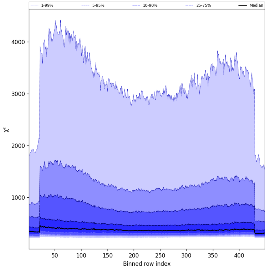
Figure 57: Along track statistics of “ \chi^2 ” for 2025-09-16 to 2025-09-17
