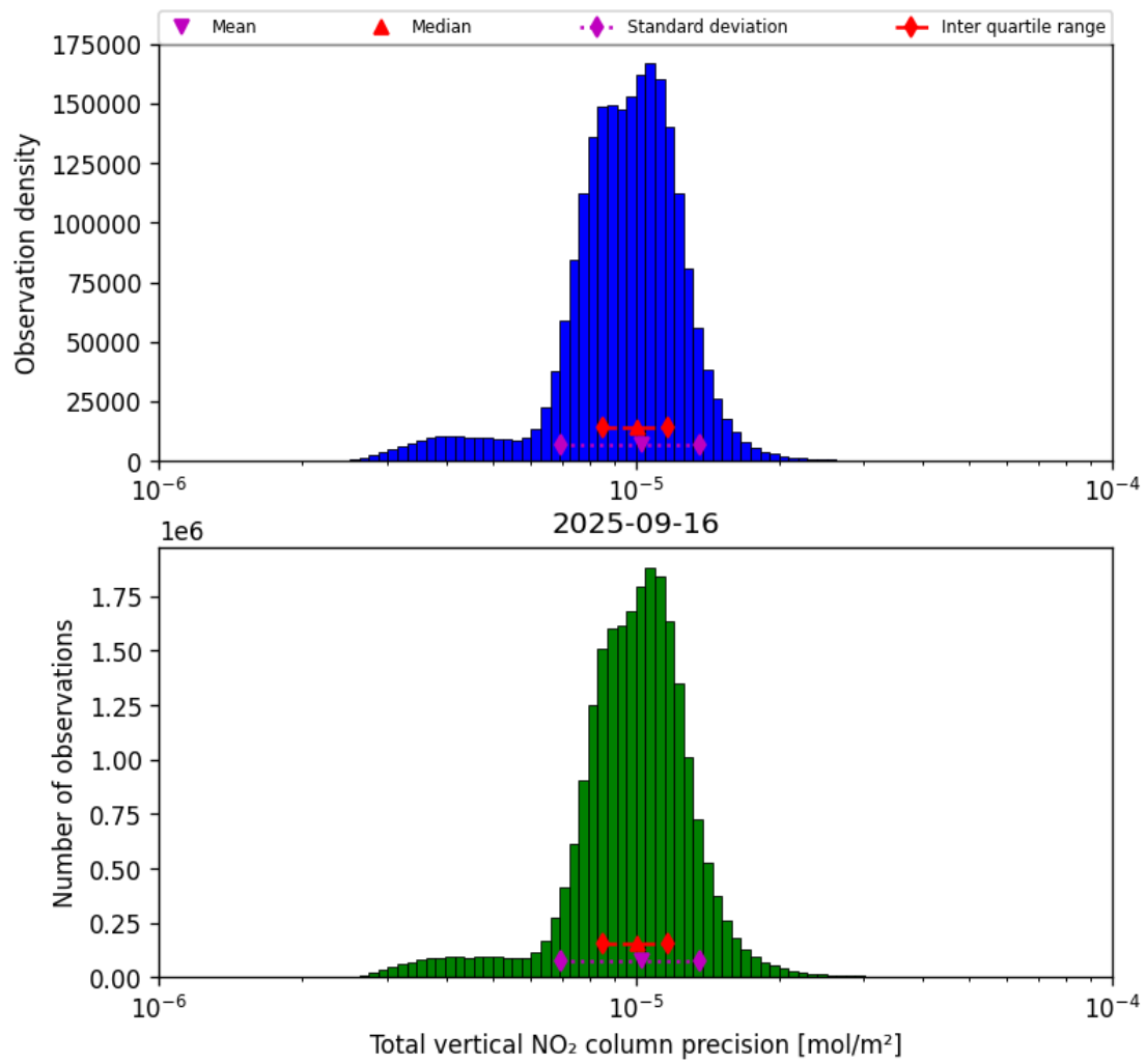
Figure 37: Histogram of “Total vertical NO 2 column precision” for 2025-09-16 to 2025-09-17
