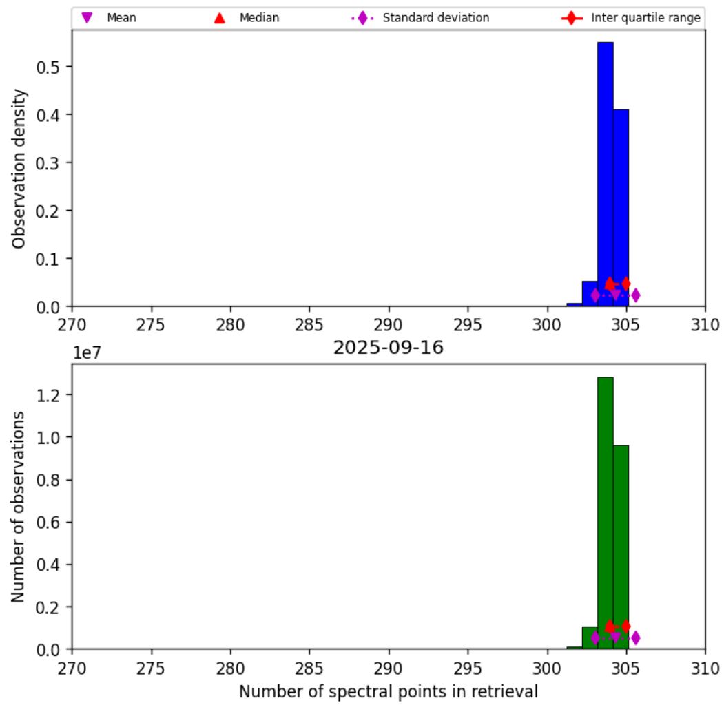
Figure 31: Histogram of “Number of spectral points in retrieval” for 2025-09-16 to 2025-09-17
