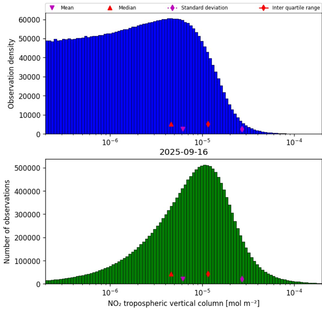
Figure 27: Histogram of “NO 2 tropospheric vertical column” for 2025-09-16 to 2025-09-17
