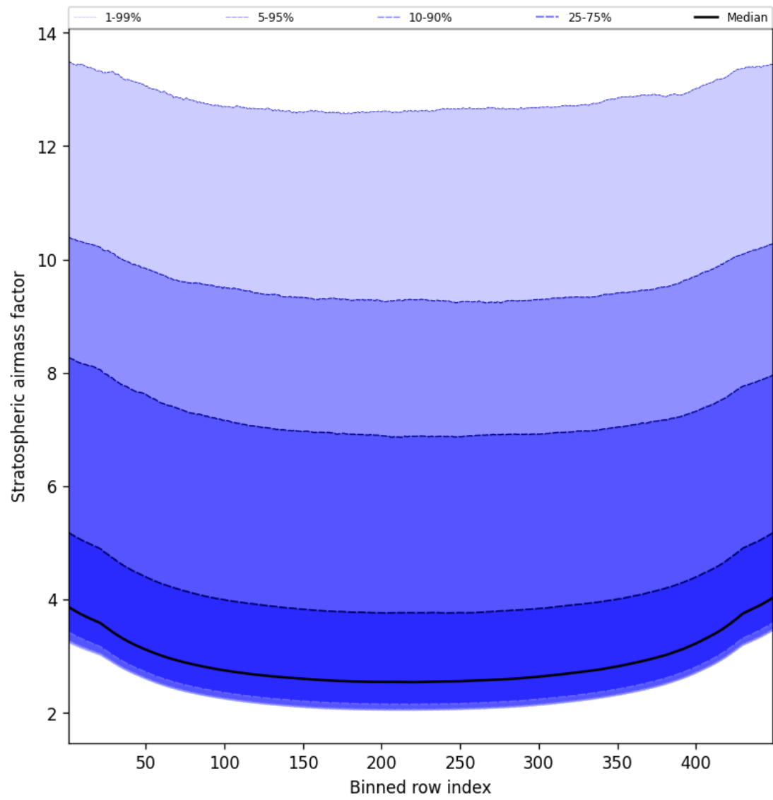
Figure 59: Along track statistics of “Stratospheric airmass factor” for 2025-09-16 to 2025-09-17
