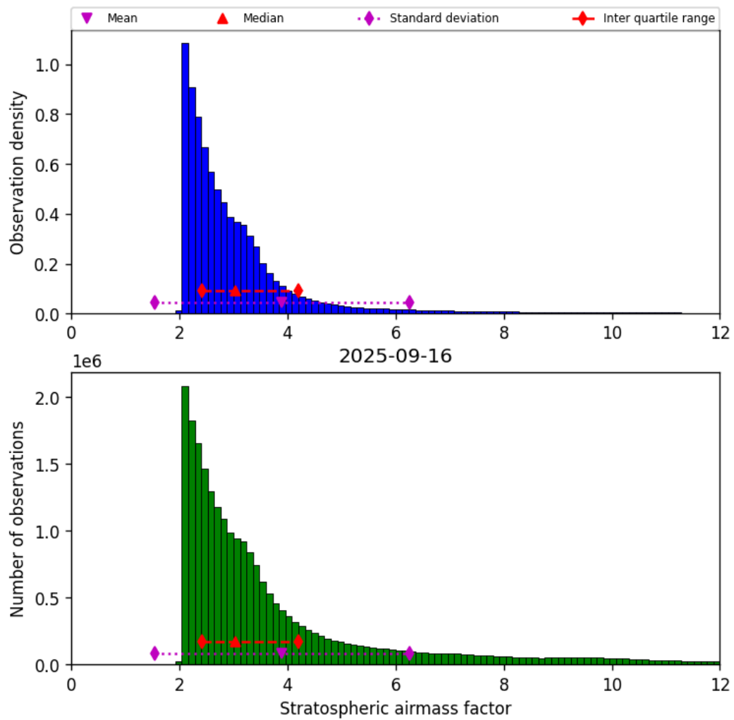
Figure 42: Histogram of “Stratospheric airmass factor” for 2025-09-16 to 2025-09-17
