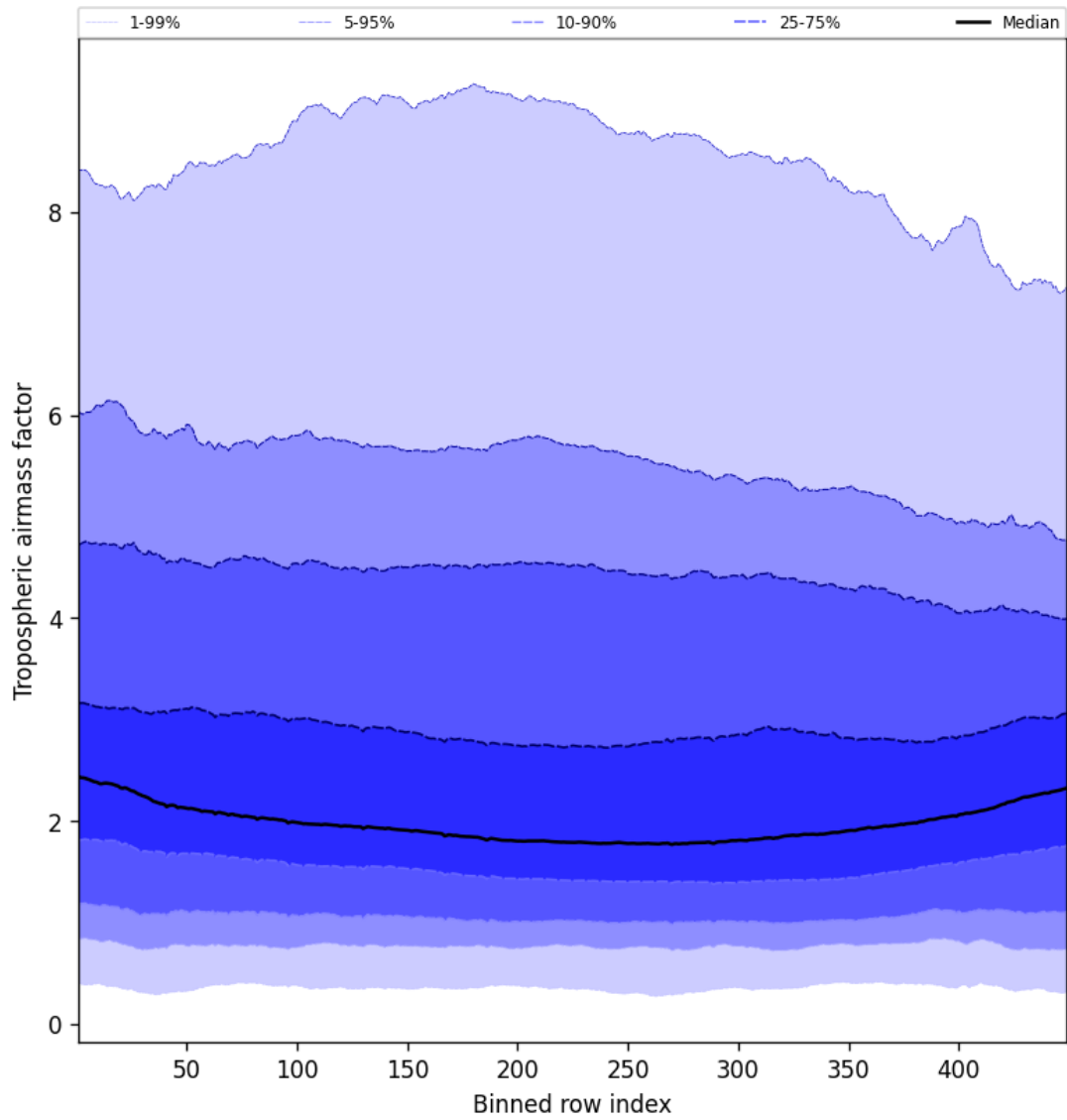
Figure 46: Along track statistics of “Tropospheric air mass factor” for 2025-09-16 to 2025-09-17
