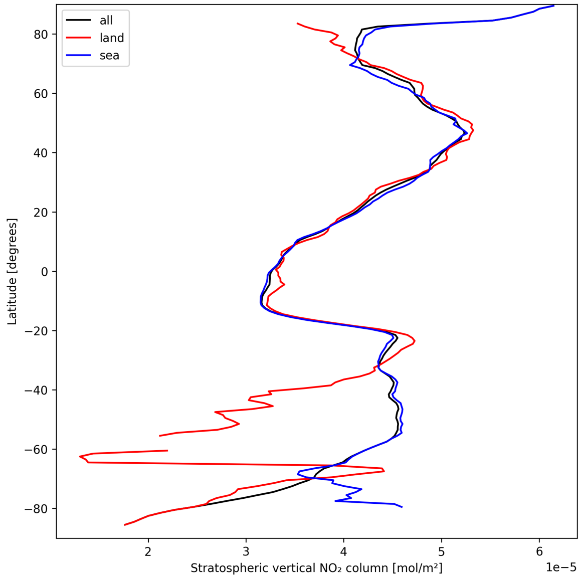
Figure 17: Zonal average of “Stratospheric vertical NO 2 column” for 2025-09-16 to 2025-09-17.
