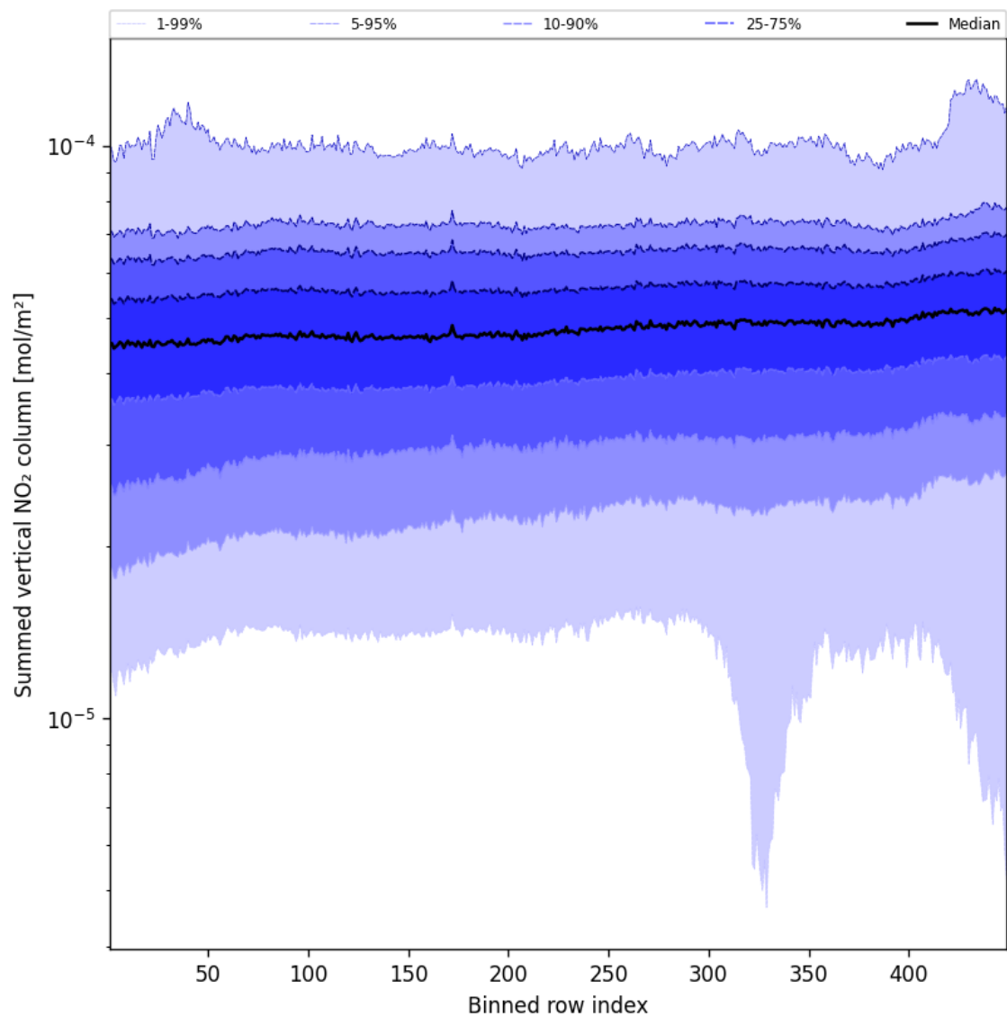
Figure 55: Along track statistics of “Summed vertical NO 2 column” for 2025-09-16 to 2025-09-17
