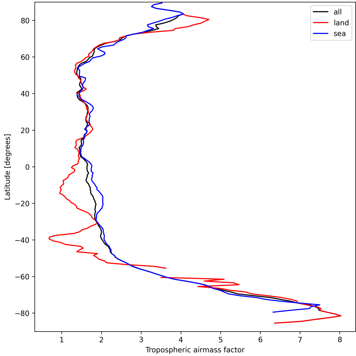
Figure 12: Zonal average of “Tropospheric airmass factor” for 2025-09-16 to 2025-09-17.
