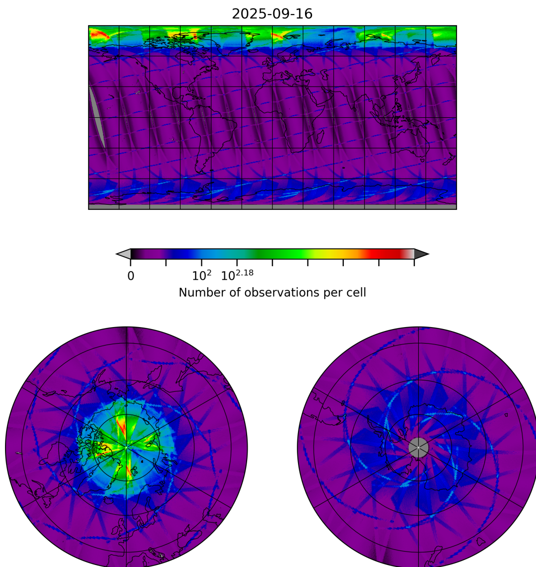
Figure 8: Map of the number of observations for 2025-09-16 to 2025-09-17
