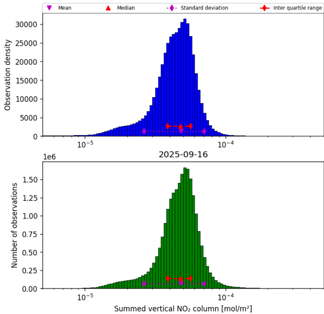
Figure 38: Histogram of “Summed vertical NO 2 column” for 2025-09-16 to 2025-09-17
