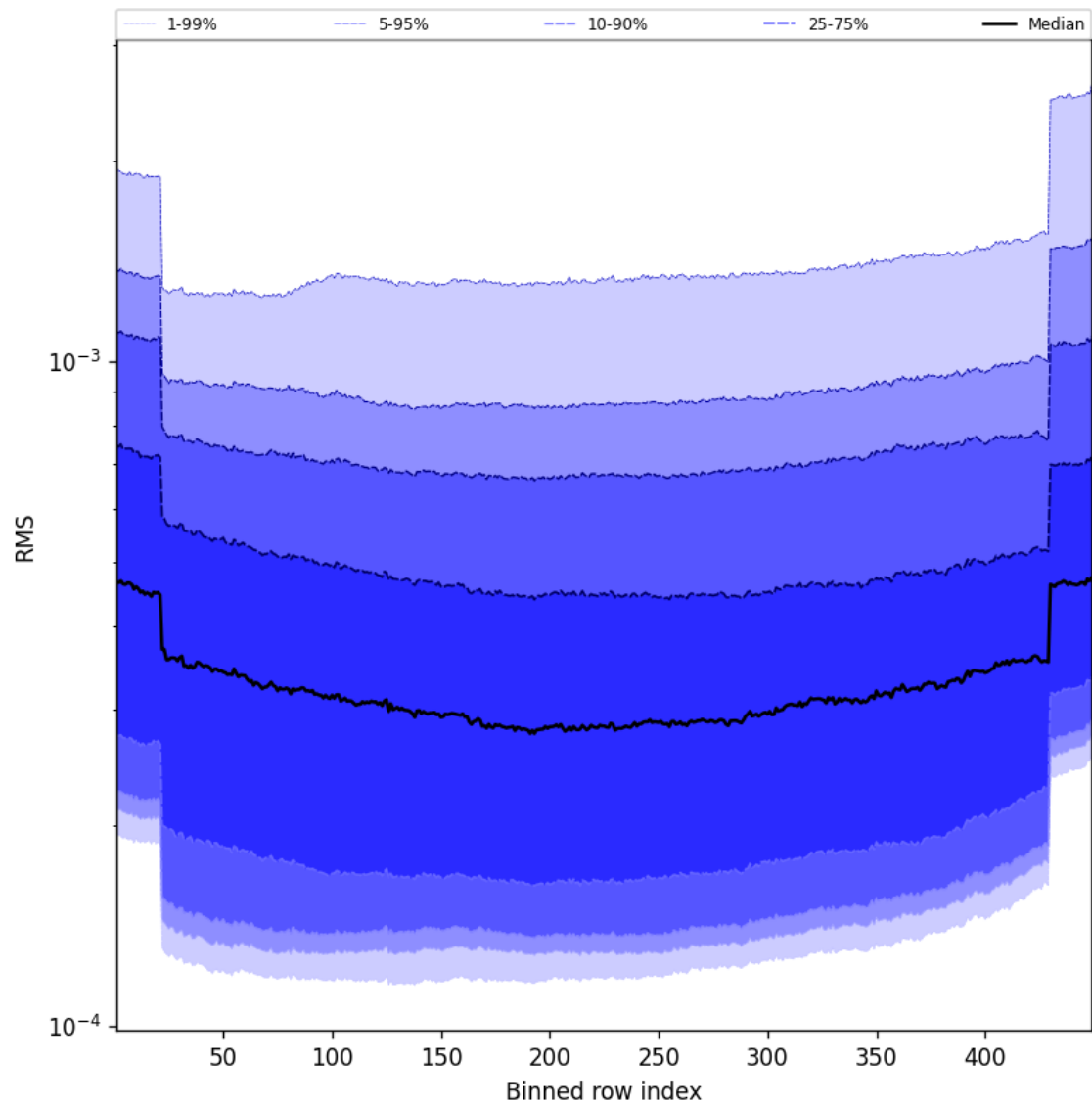
Figure 58: Along track statistics of “RMS” for 2025-09-16 to 2025-09-17
