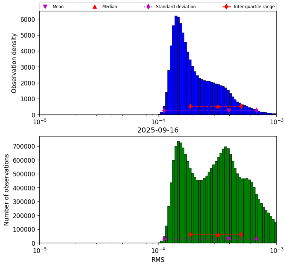
Figure 41: Histogram of “RMS” for 2025-09-16 to 2025-09-17
