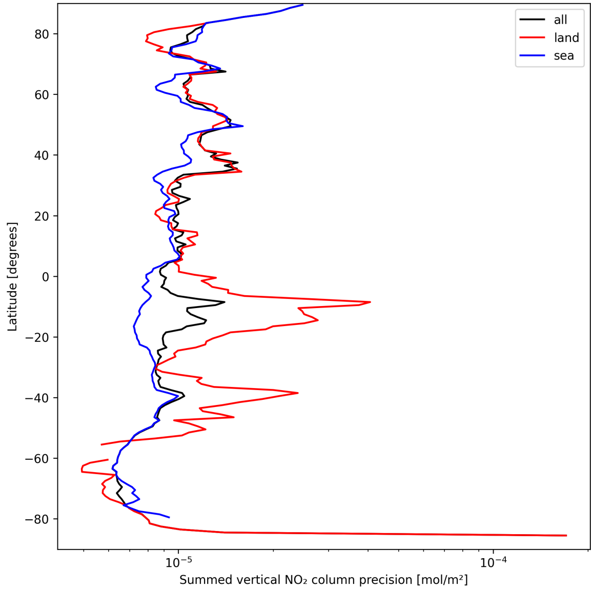
Figure 22: Zonal average of “Summed vertical NO 2 column precision” for 2025-09-16 to 2025-09-17.
