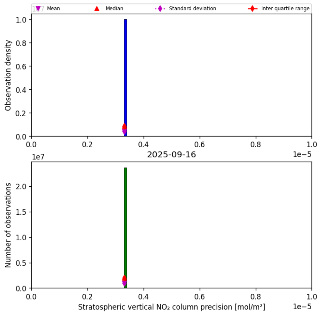
Figure 35: Histogram of “Stratospheric vertical NO 2 column precision” for 2025-09-16 to 2025-09-17
