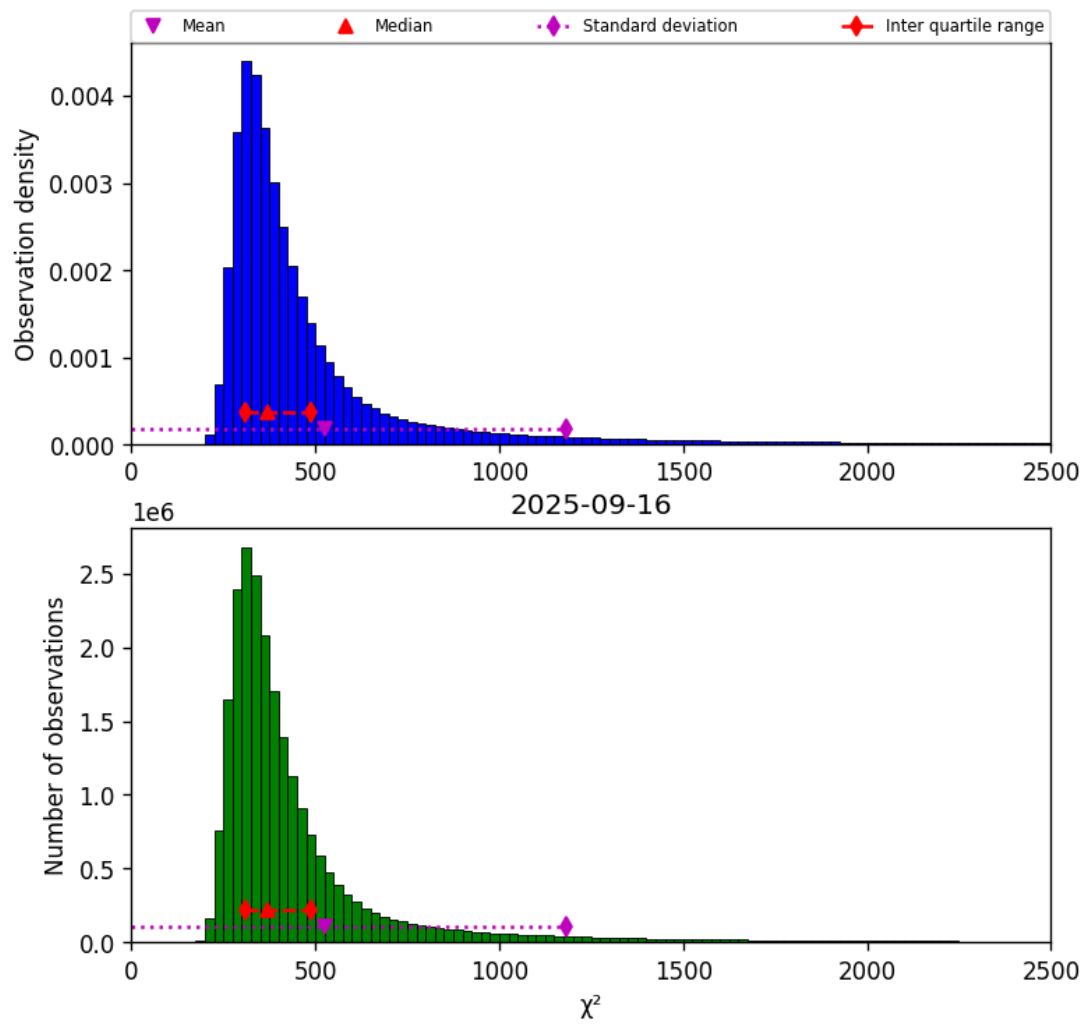
Figure 40: Histogram of “ \chi^2 ” for 2025-09-16 to 2025-09-17
