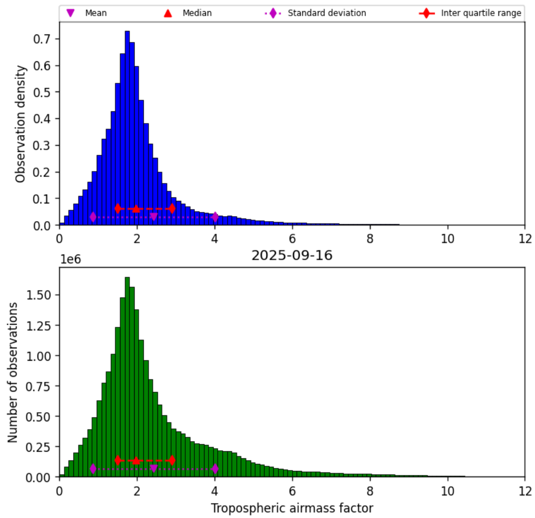
Figure 29: Histogram of “Tropospheric airmass factor” for 2025-09-16 to 2025-09-17
