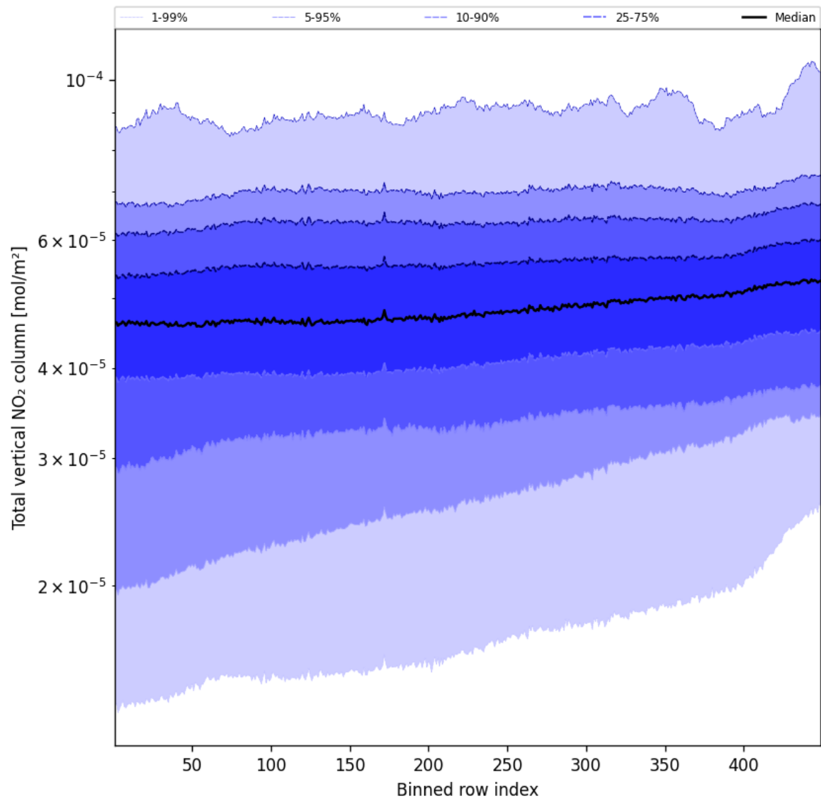
Figure 53: Along track statistics of “Total vertical NO 2 column” for 2025-09-16 to 2025-09-17
