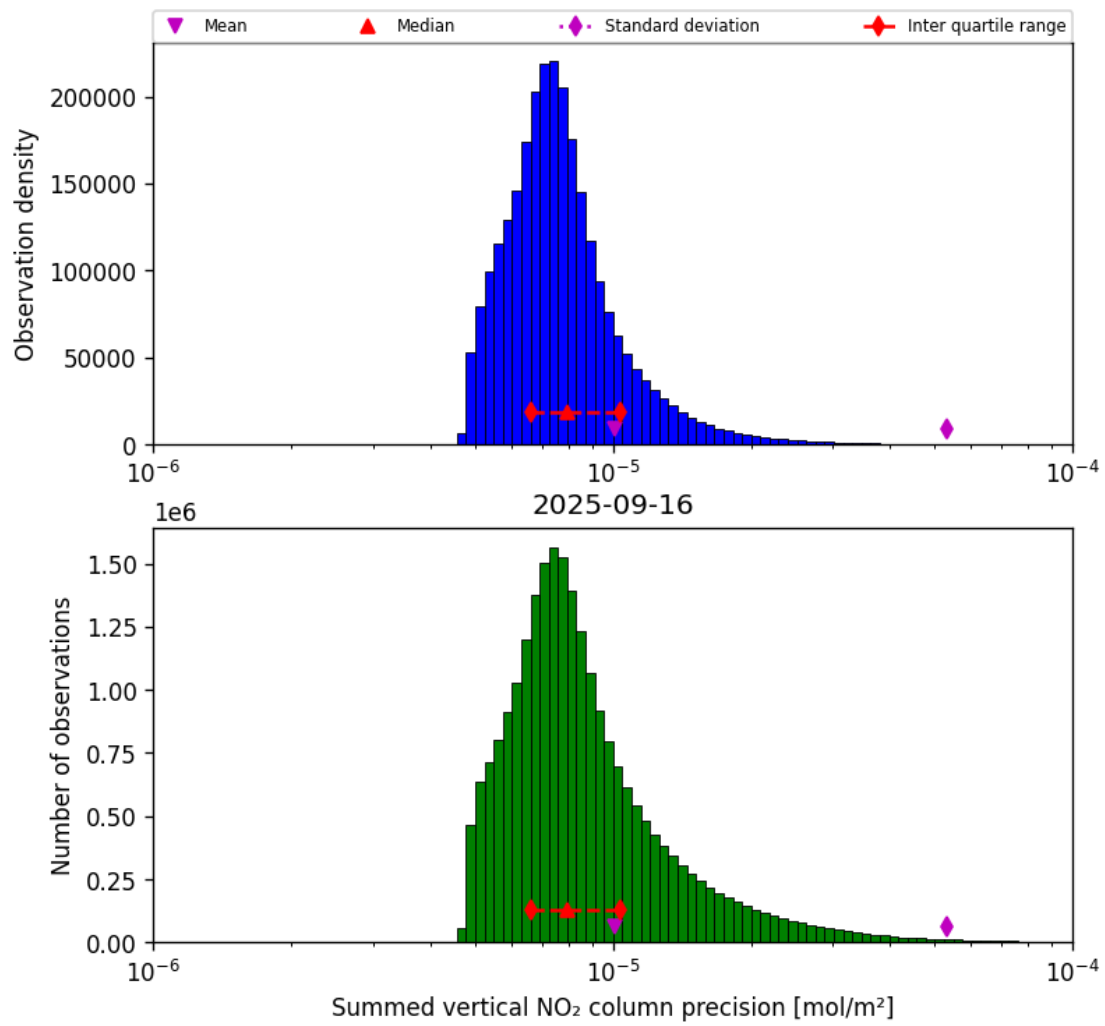
Figure 39: Histogram of “Summed vertical NO 2 column precision” for 2025-09-16 to 2025-09-17
