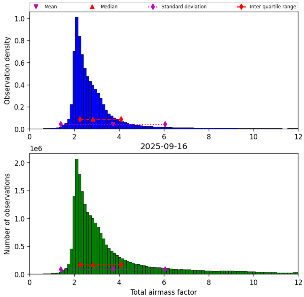
Figure 30: Histogram of “Total airmass factor” for 2025-09-16 to 2025-09-17
