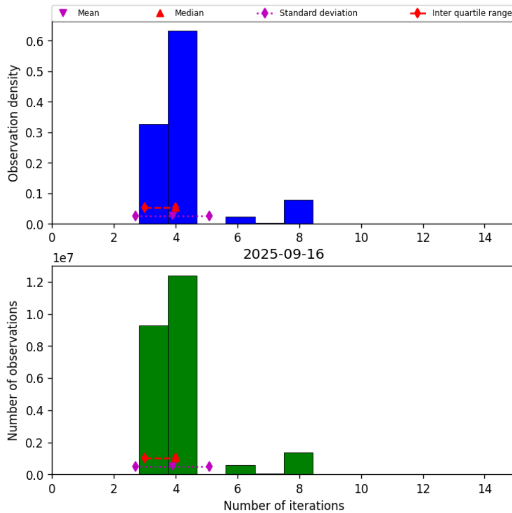
Figure 32: Histogram of “Number of iterations” for 2025-09-16 to 2025-09-17
