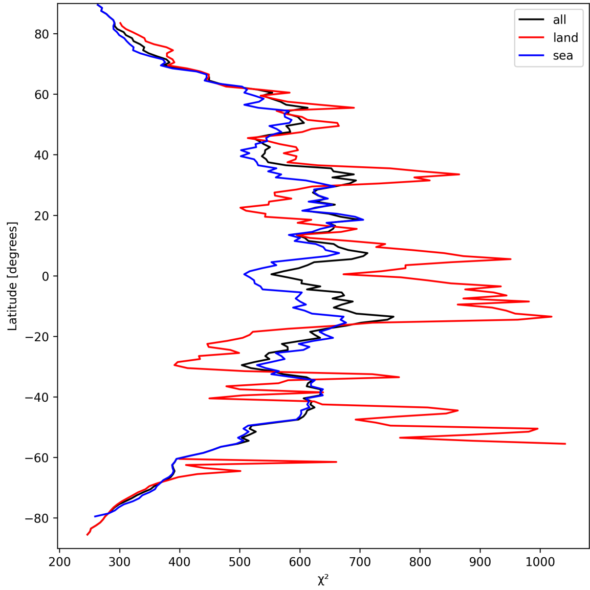
Figure 23: Zonal average of “ \chi^2 ” for 2025-09-16 to 2025-09-17.
