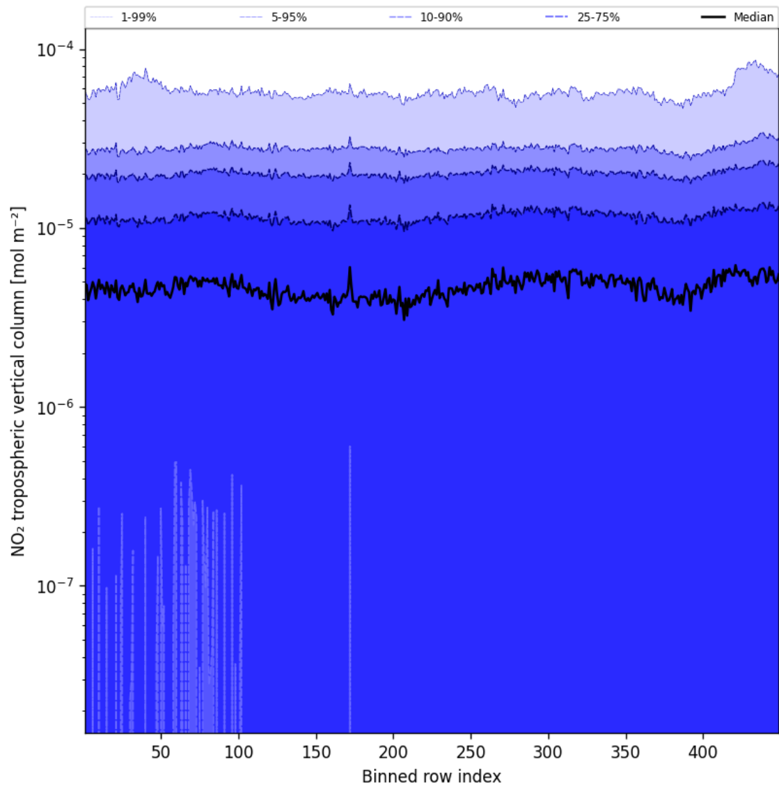
Figure 44: Along track statistics of “NO 2 tropospheric vertical column” for 2025-09-16 to 2025-09-17
