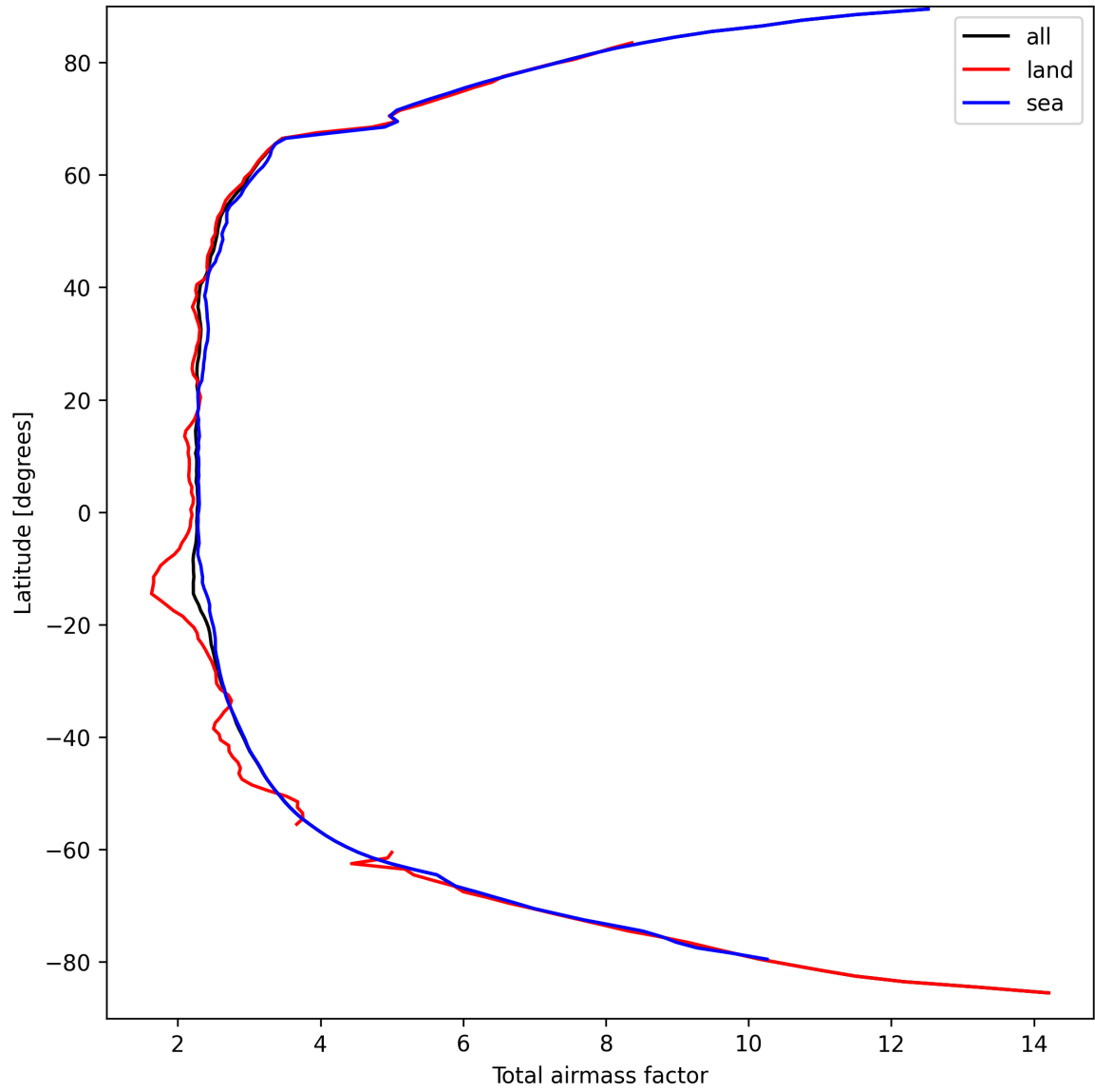
Figure 13: Zonal average of “Total airmass factor” for 2025-09-16 to 2025-09-17.
