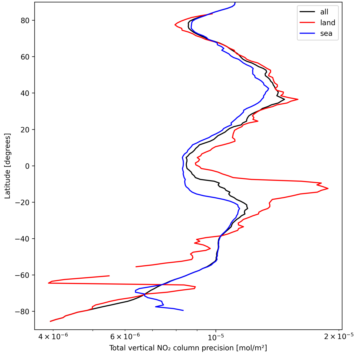
Figure 20: Zonal average of “Total vertical NO 2 column precision” for 2025-09-16 to 2025-09-17.
