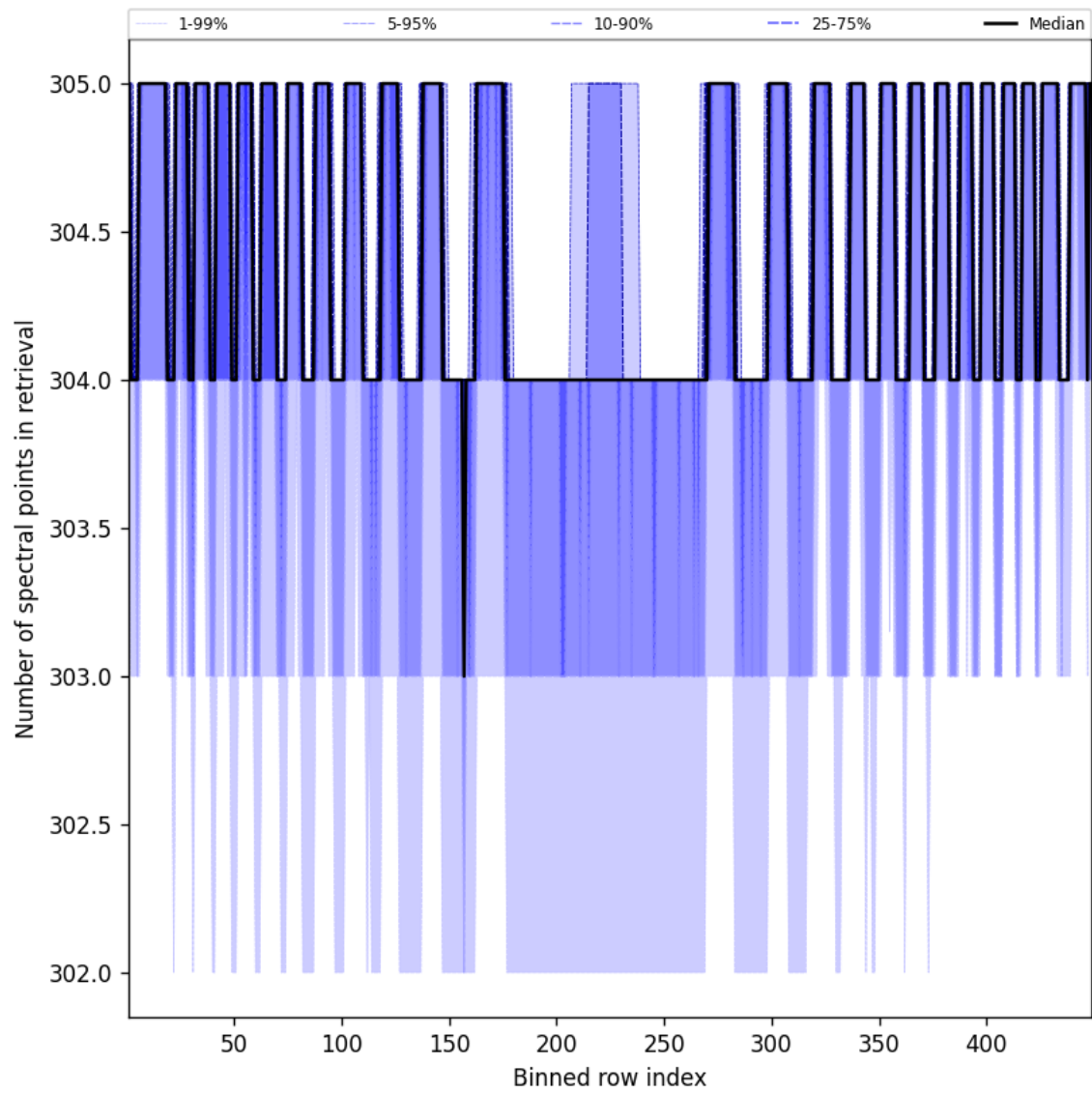
Figure 48: Along track statistics of “Number of spectral points in retrieval” for 2025-09-16 to 2025-09-17
