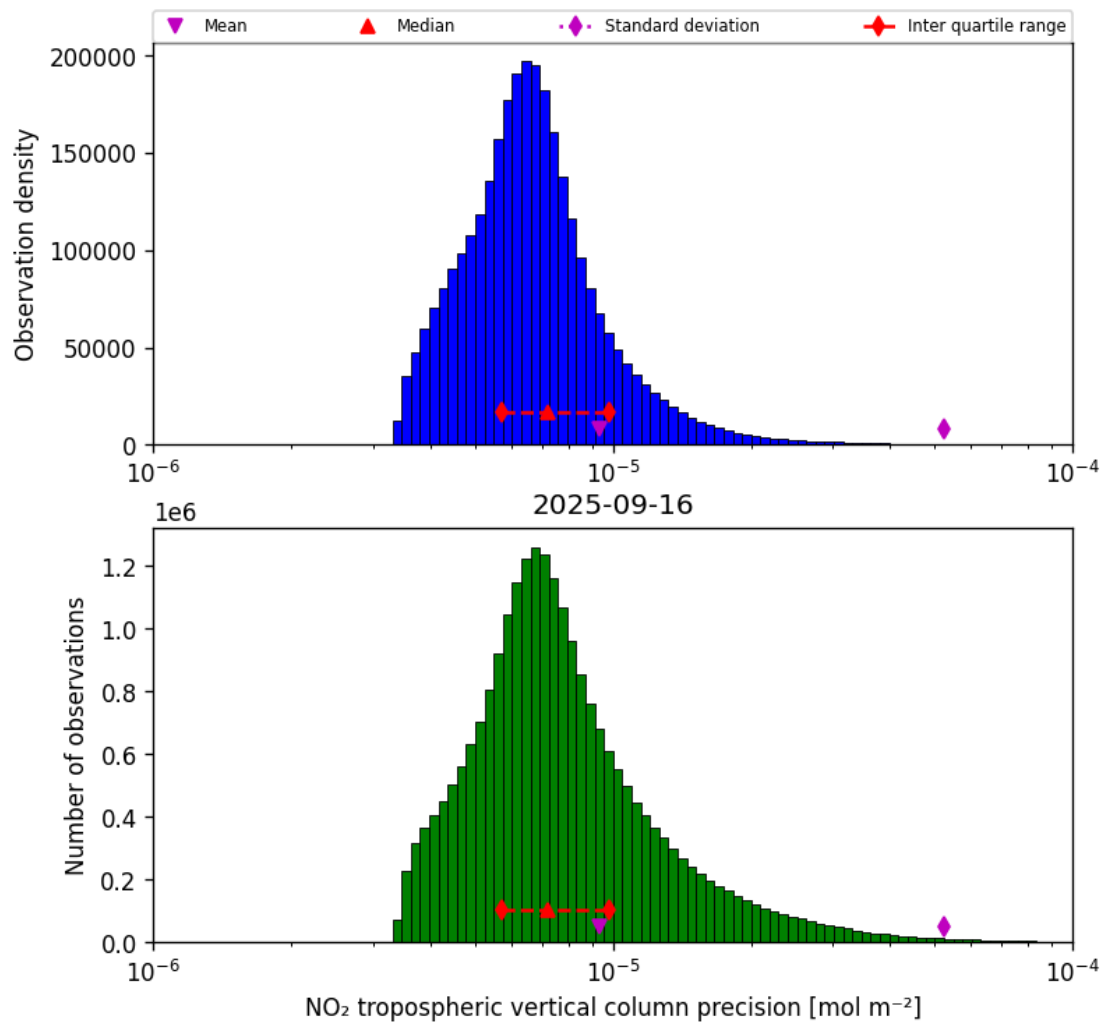
Figure 28: Histogram of “NO 2 tropospheric vertical column precision” for 2025-09-16 to 2025-09-17
