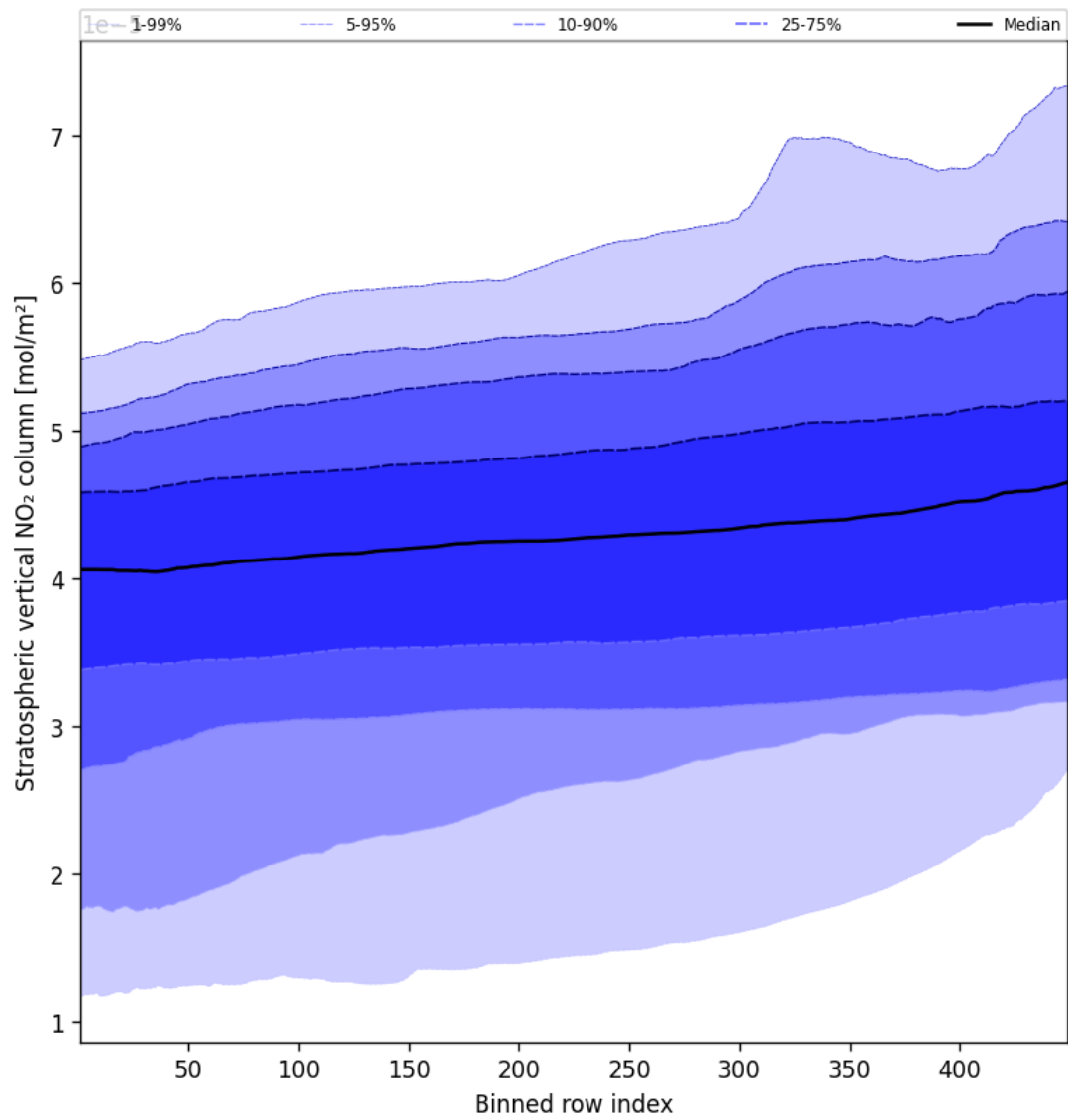
Figure 51: Along track statistics of “Stratospheric vertical NO 2 column” for 2025-09-16 to 2025-09-17
