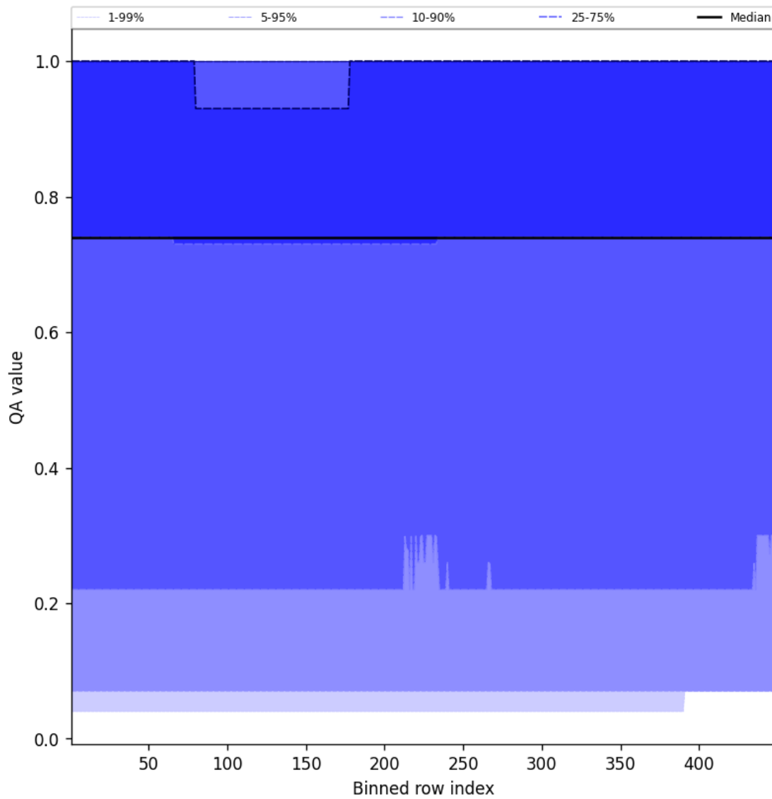
Figure 43: Along track statistics of “QA value” for 2025-09-16 to 2025-09-17
