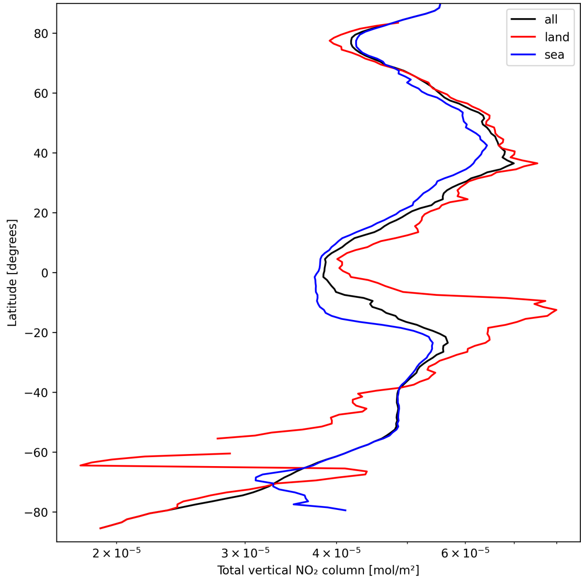
Figure 19: Zonal average of “Total vertical NO 2 column” for 2025-09-16 to 2025-09-17.
