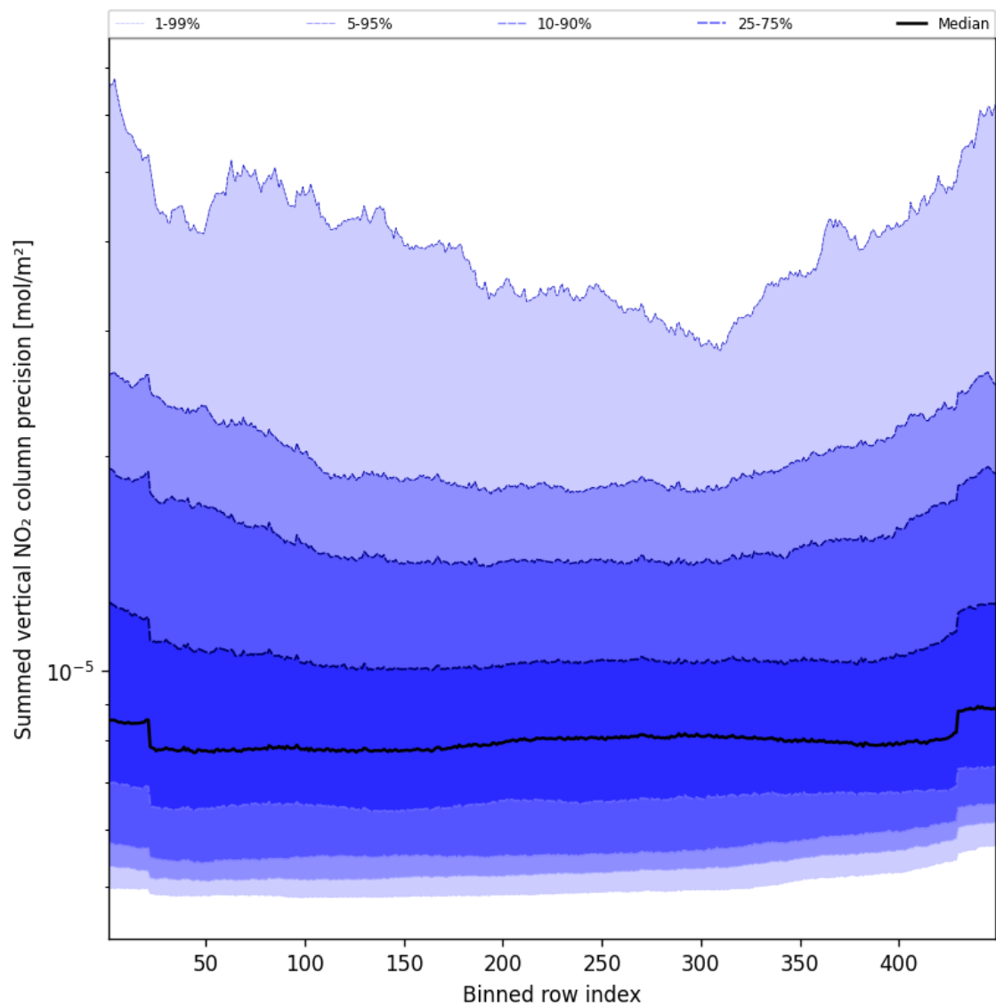
Figure 56: Along track statistics of “Summed vertical NO 2 column precision” for 2025-09-17 to 2025-09-18
