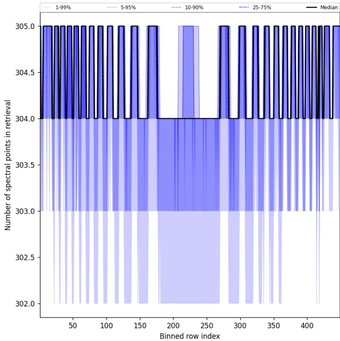
Figure 48: Along track statistics of “Number of spectral points in retrieval” for 2025-09-17 to 2025-09-18
