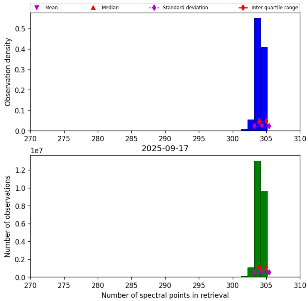
Figure 31: Histogram of “Number of spectral points in retrieval” for 2025-09-17 to 2025-09-18
