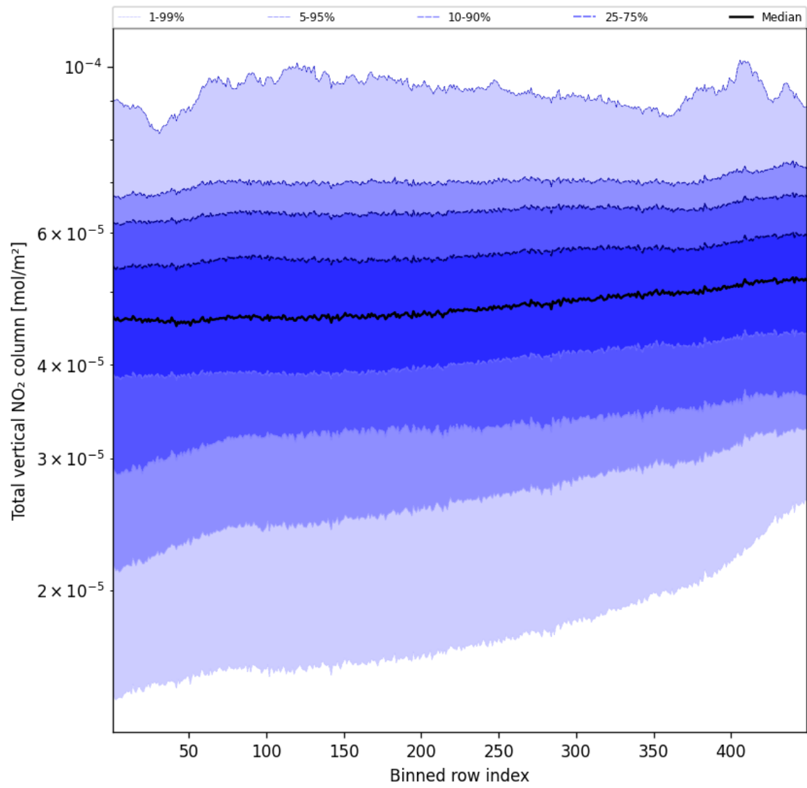
Figure 53: Along track statistics of “Total vertical NO 2 column” for 2025-09-17 to 2025-09-18
