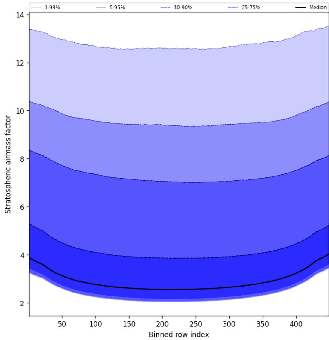
Figure 59: Along track statistics of “Stratospheric airmass factor” for 2025-09-17 to 2025-09-18
