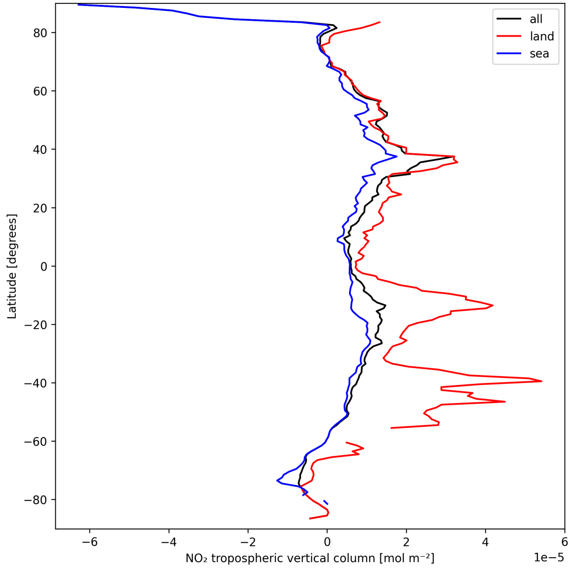
Figure 10: Zonal average of “NO 2 tropospheric vertical column” for 2025-09-17 to 2025-09-18.
