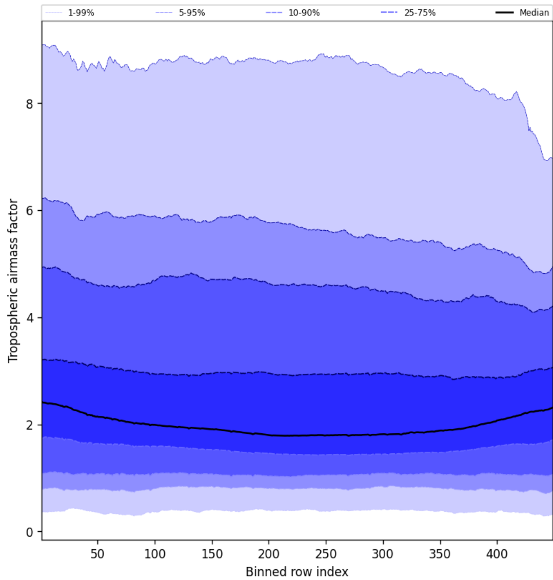
Figure 46: Along track statistics of “Tropospheric air mass factor” for 2025-09-17 to 2025-09-18
