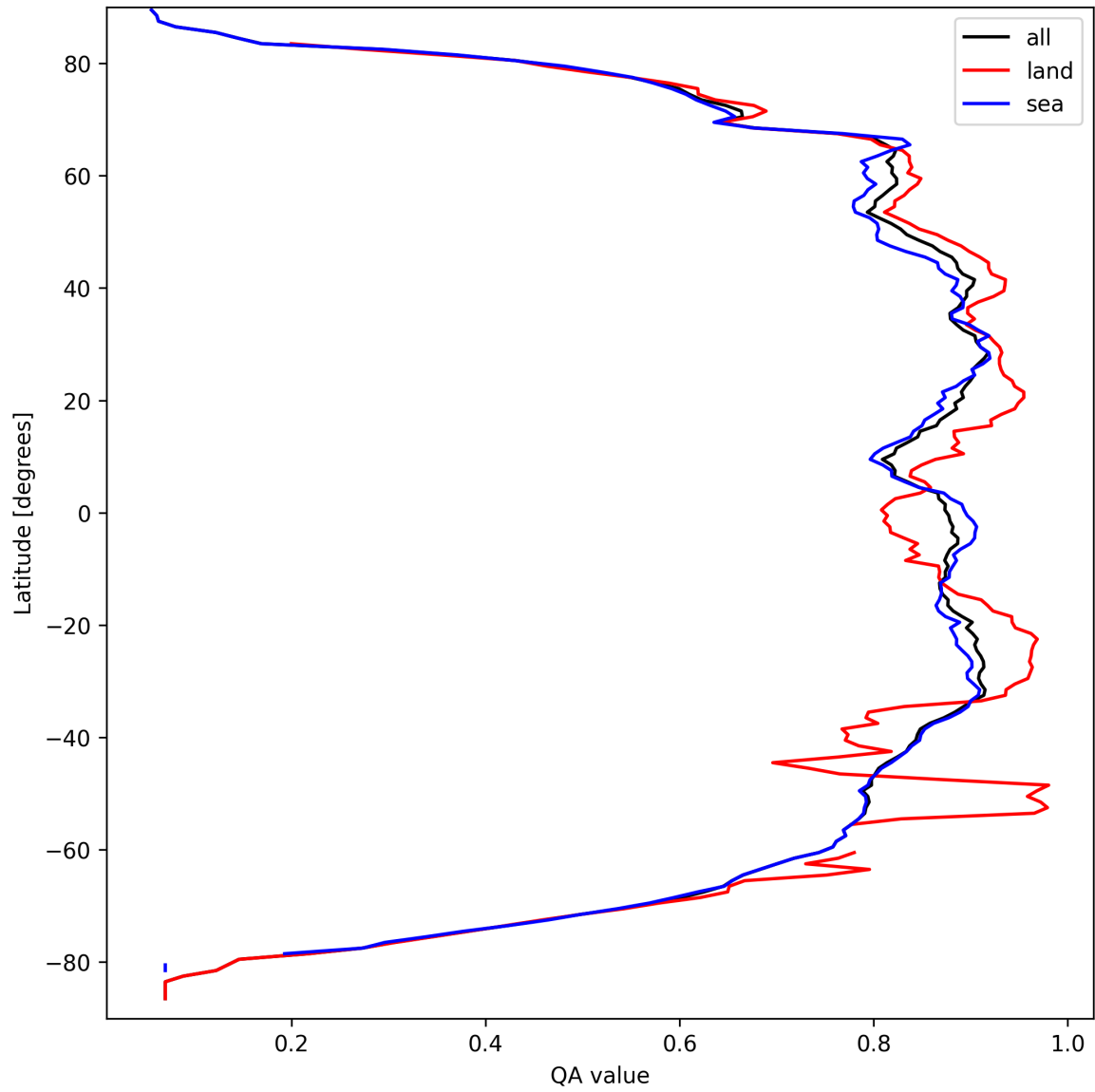
Figure 9: Zonal average of “QA value” for 2025-09-17 to 2025-09-18.
