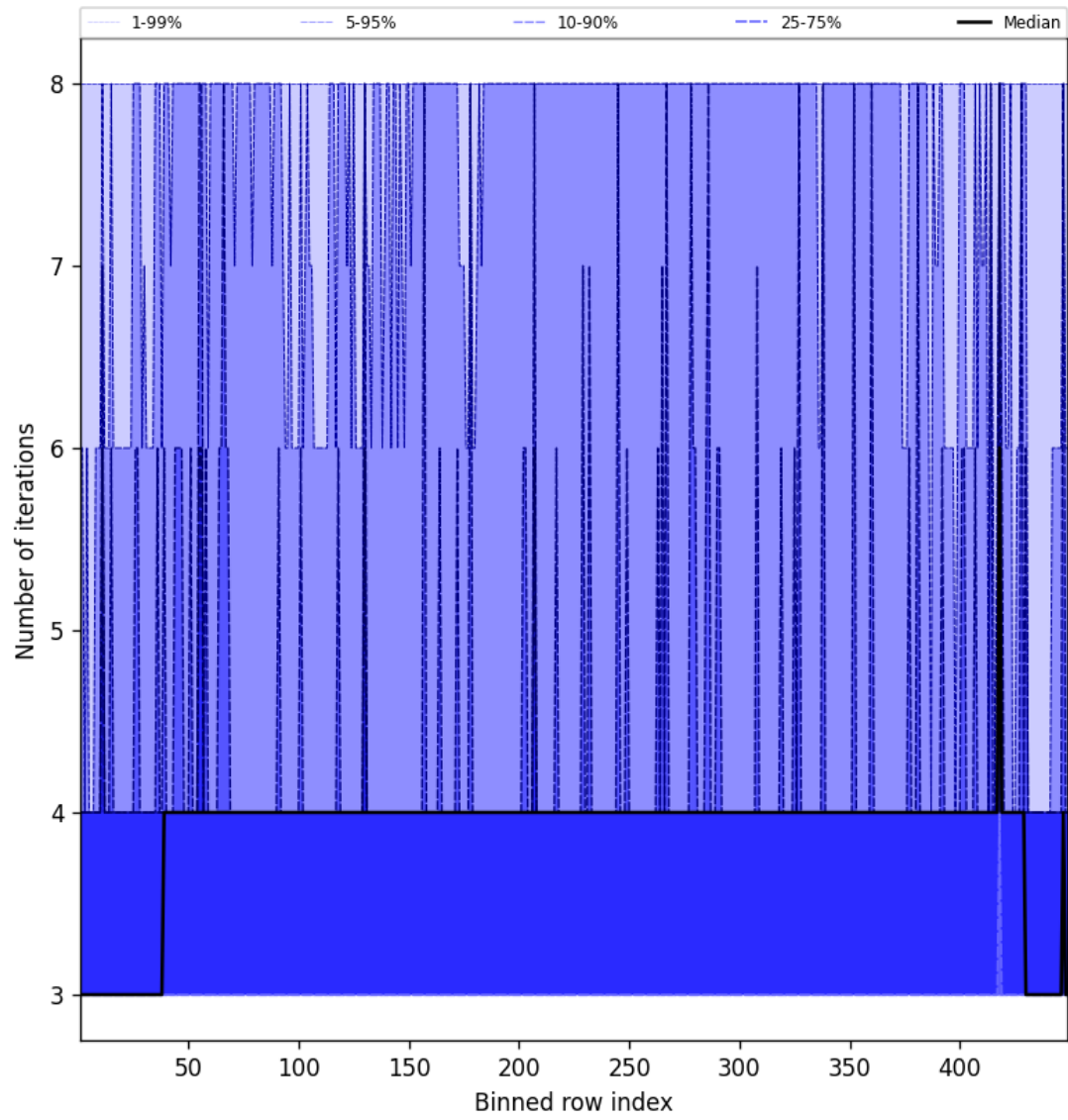
Figure 49: Along track statistics of “Number of iterations” for 2025-09-17 to 2025-09-18
