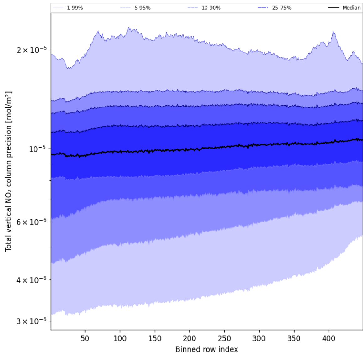
Figure 54: Along track statistics of “Total vertical NO 2 column precision” for 2025-09-17 to 2025-09-18
