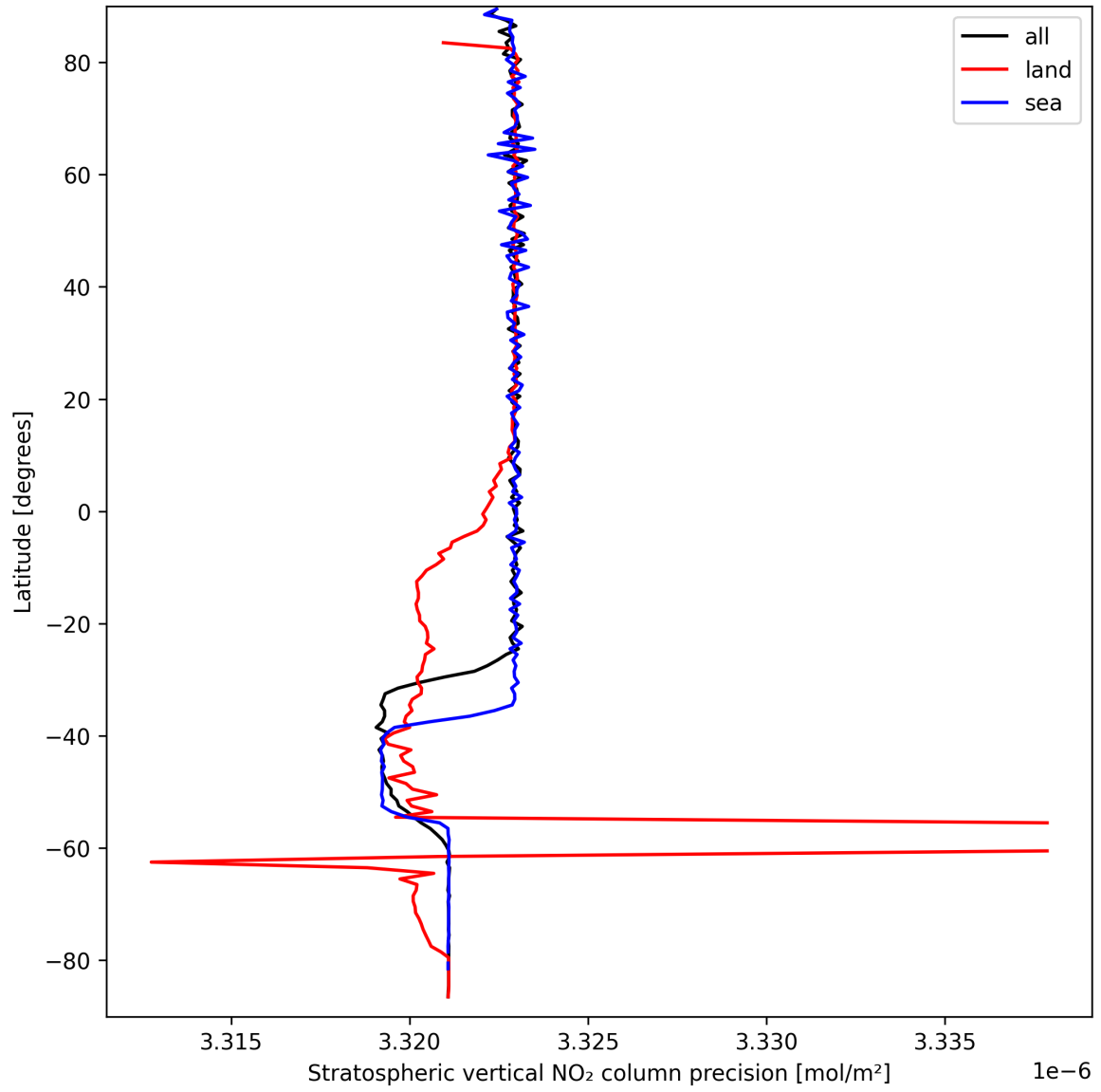
Figure 18: Zonal average of “Stratospheric vertical NO 2 column precision” for 2025-09-17 to 2025-09-18.
