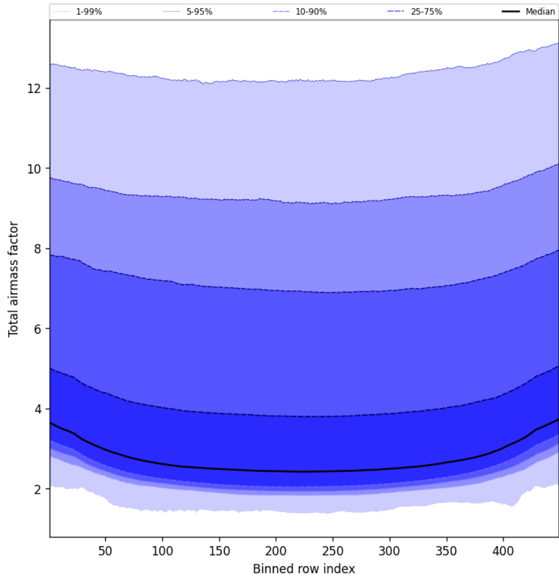
Figure 47: Along track statistics of “Total airmass factor” for 2025-09-17 to 2025-09-18
