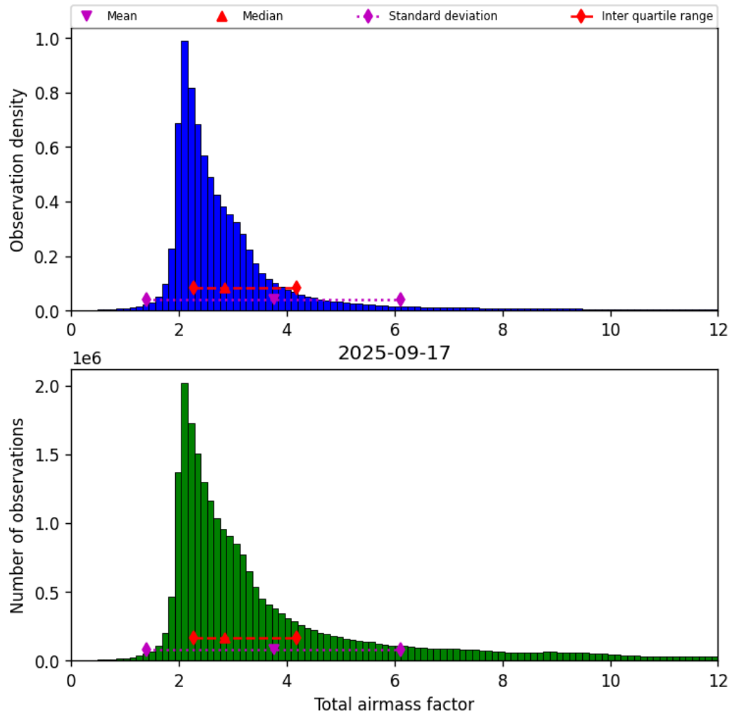
Figure 30: Histogram of “Total airmass factor” for 2025-09-17 to 2025-09-18
