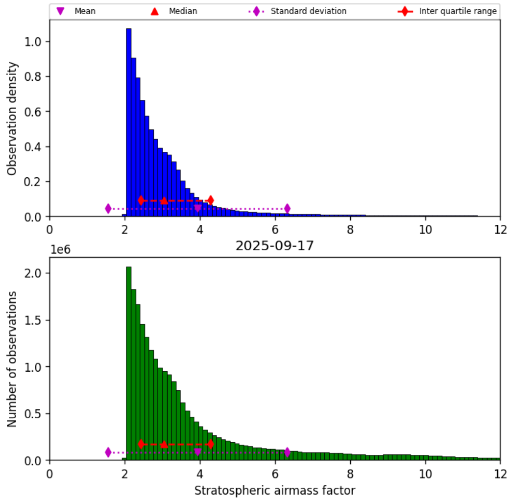
Figure 42: Histogram of “Stratospheric airmass factor” for 2025-09-17 to 2025-09-18
