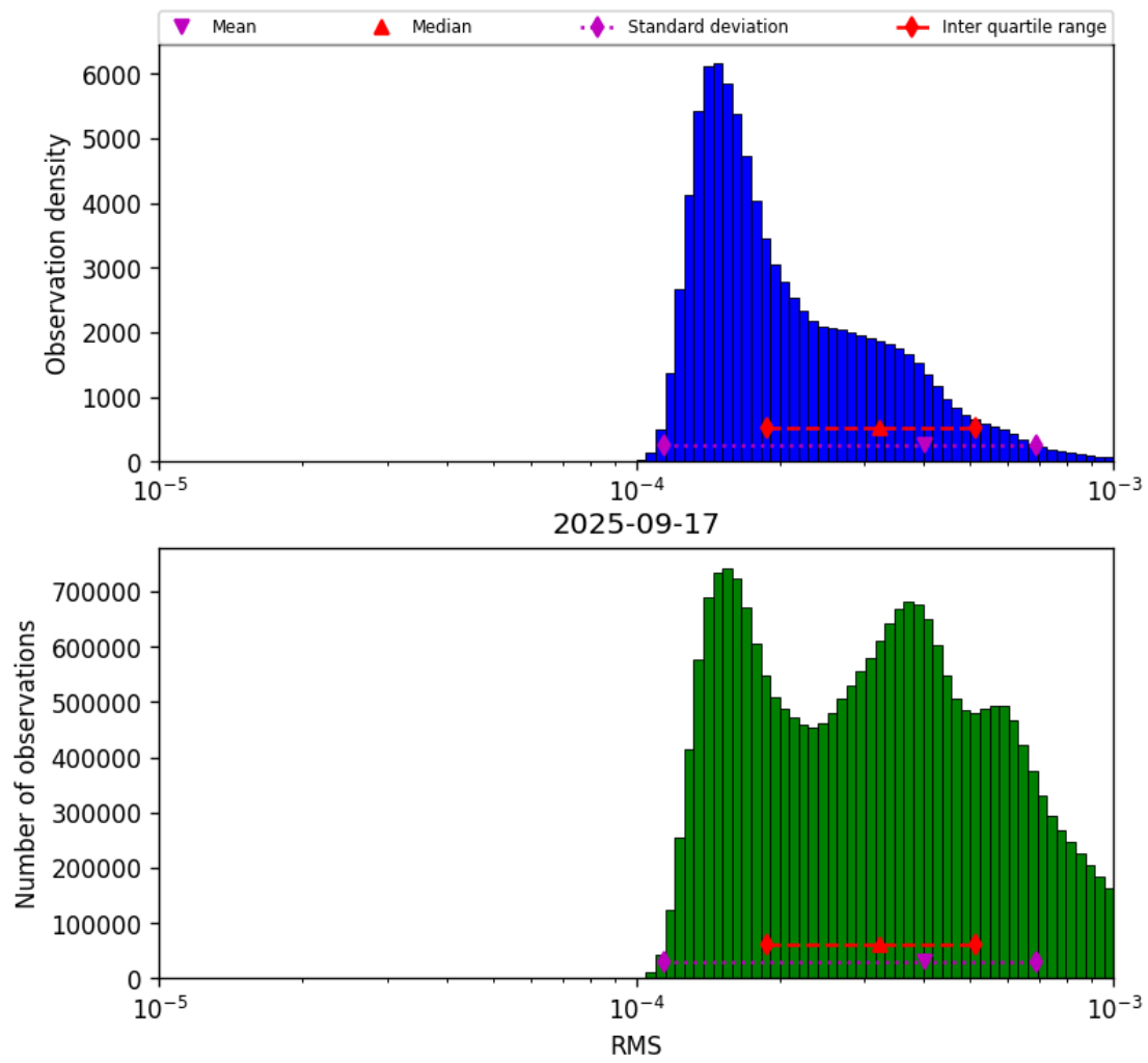
Figure 41: Histogram of “RMS” for 2025-09-17 to 2025-09-18
