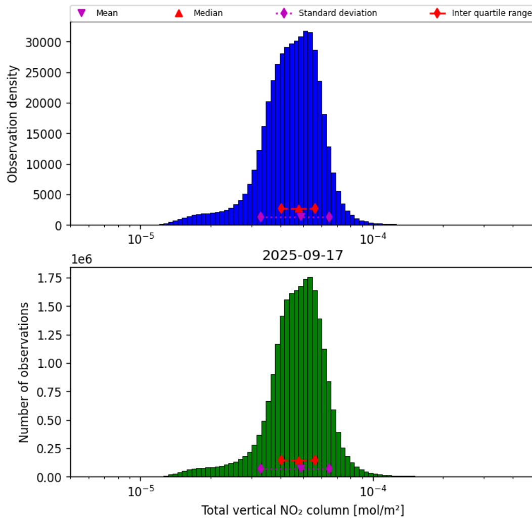
Figure 36: Histogram of "Total vertical NO 2 column" for 2025-09-17 to 2025-09-18
