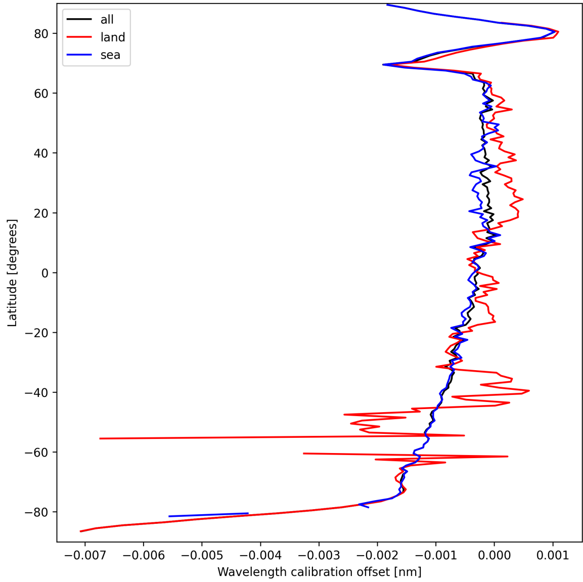
Figure 16: Zonal average of “Wavelength calibration offset” for 2025-09-17 to 2025-09-18.
