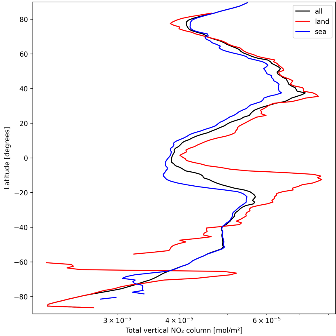
Figure 19: Zonal average of “Total vertical NO 2 column” for 2025-09-17 to 2025-09-18.
