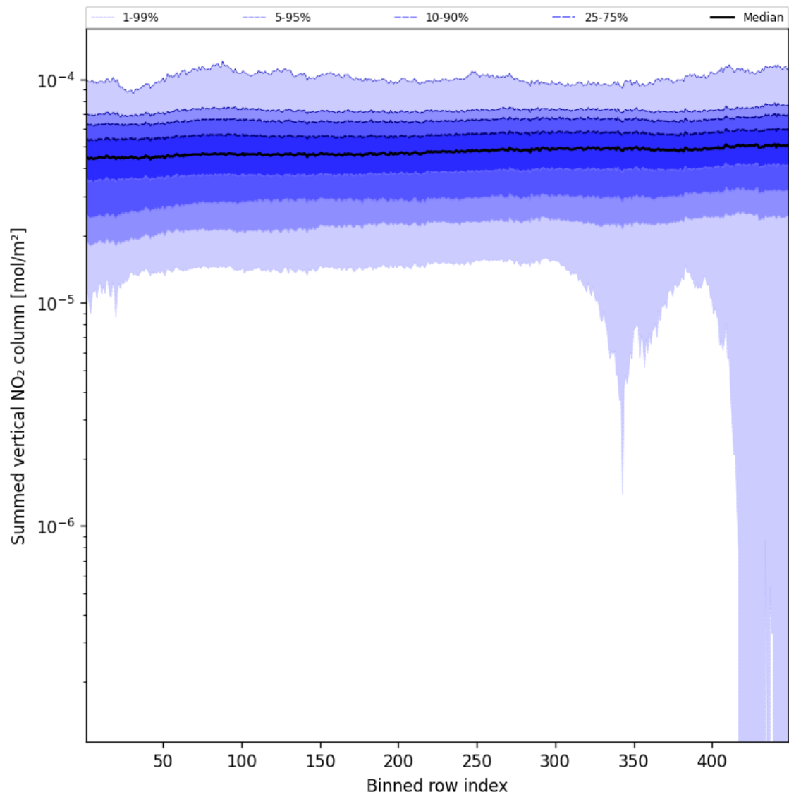
Figure 55: Along track statistics of “Summed vertical NO 2 column” for 2025-09-17 to 2025-09-18
