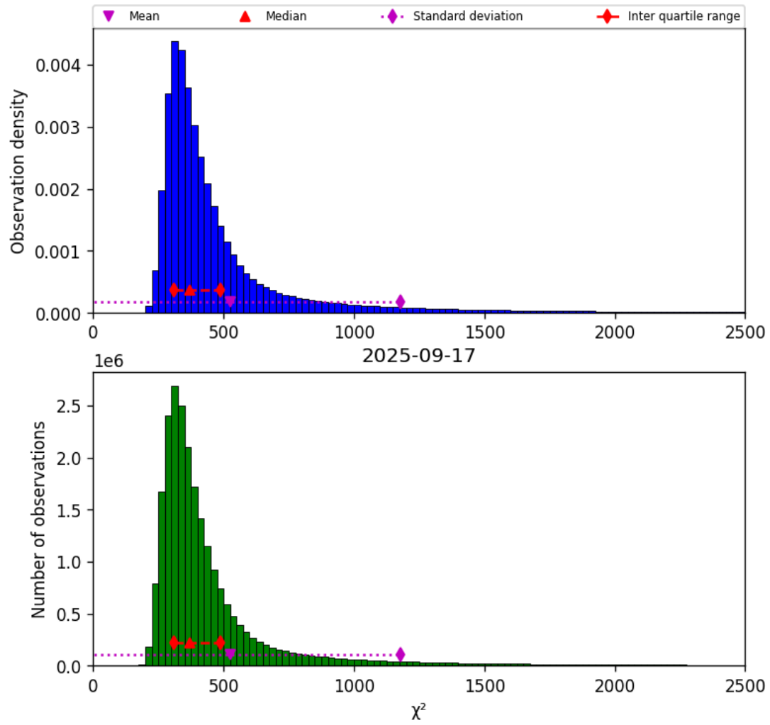
Figure 40: Histogram of “ \chi^2 ” for 2025-09-17 to 2025-09-18
