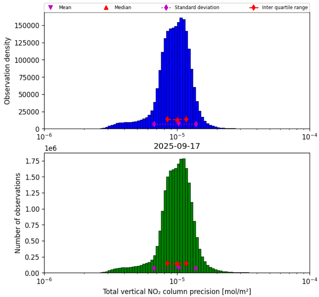
Figure 37: Histogram of “Total vertical NO 2 column precision” for 2025-09-17 to 2025-09-18
