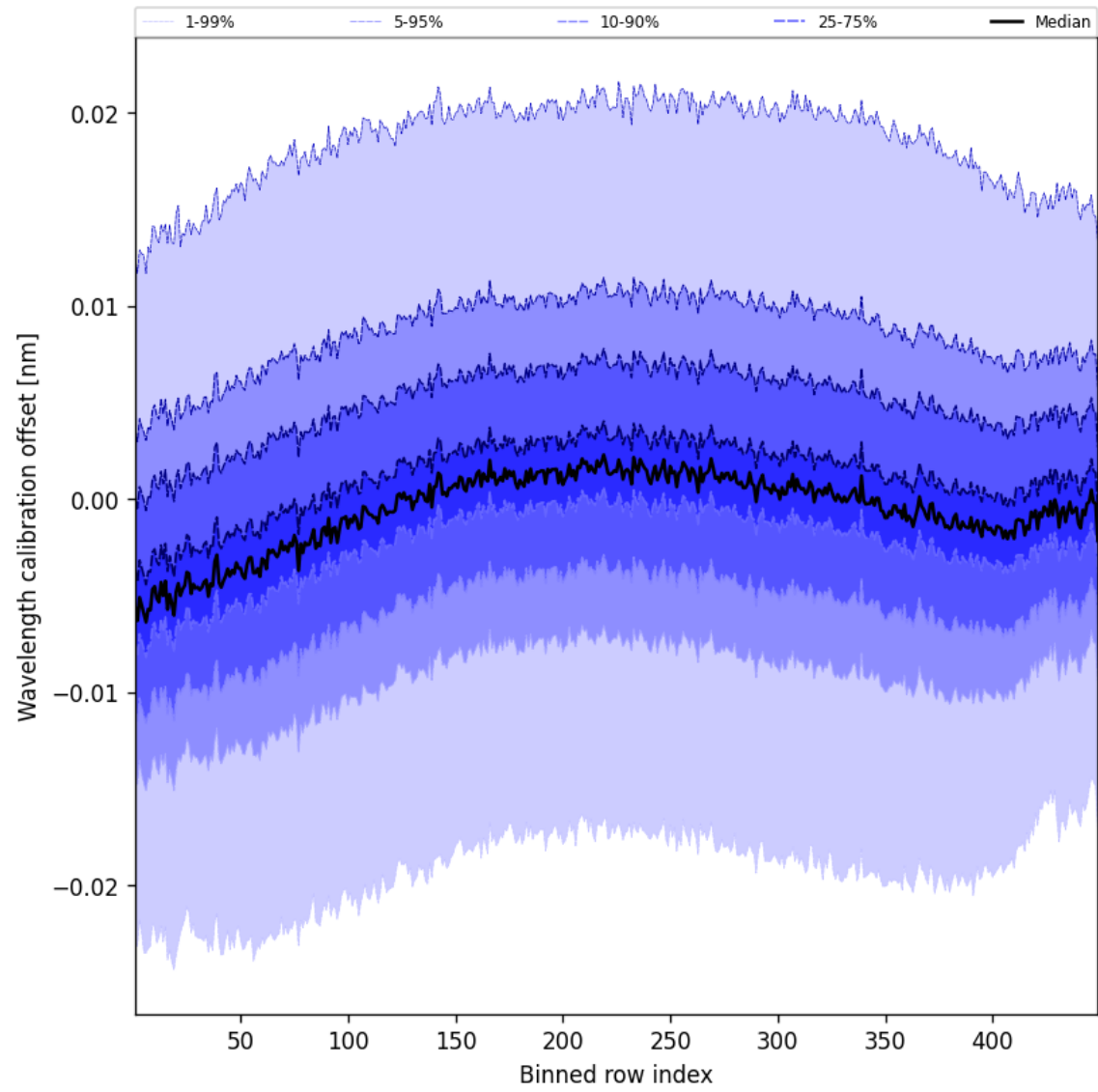
Figure 50: Along track statistics of “Wavelength calibration offset” for 2025-09-17 to 2025-09-18
