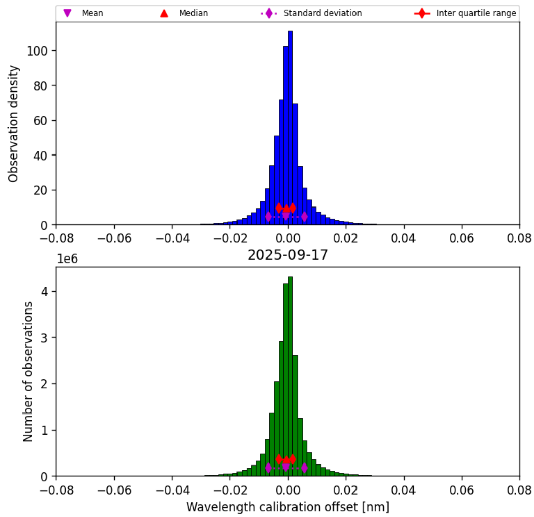
Figure 33: Histogram of “Wavelength calibration offset” for 2025-09-17 to 2025-09-18
