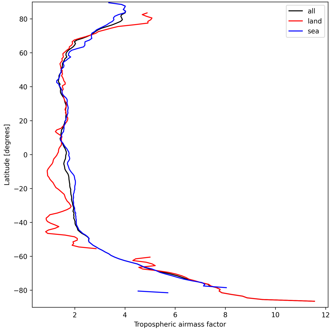
Figure 12: Zonal average of “Tropospheric airmass factor” for 2025-09-17 to 2025-09-18.
