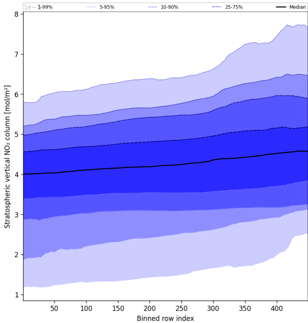
Figure 51: Along track statistics of “Stratospheric vertical NO 2 column” for 2025-09-17 to 2025-09-18
