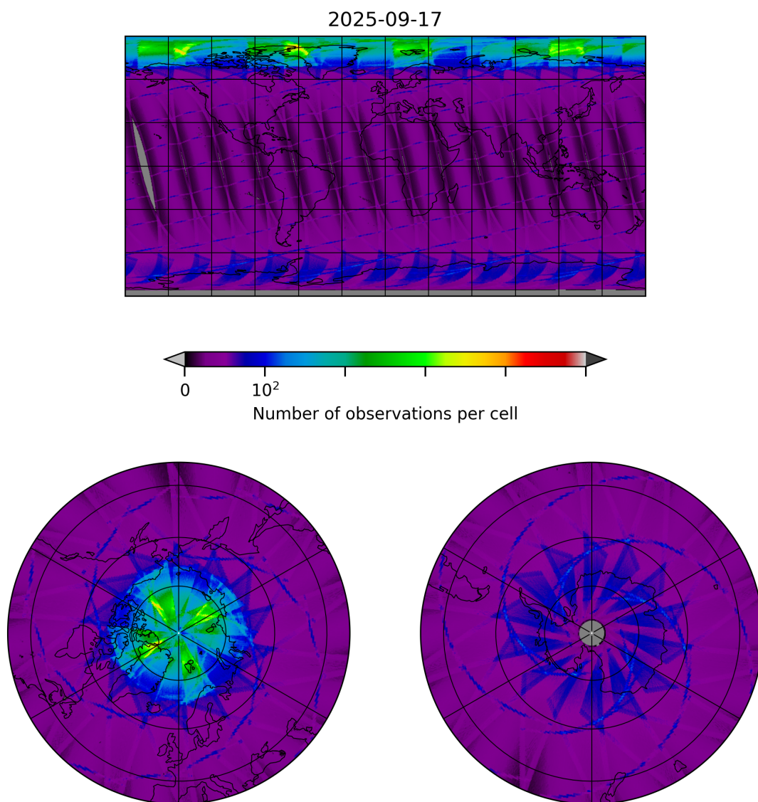
Figure 8: Map of the number of observations for 2025-09-17 to 2025-09-18
