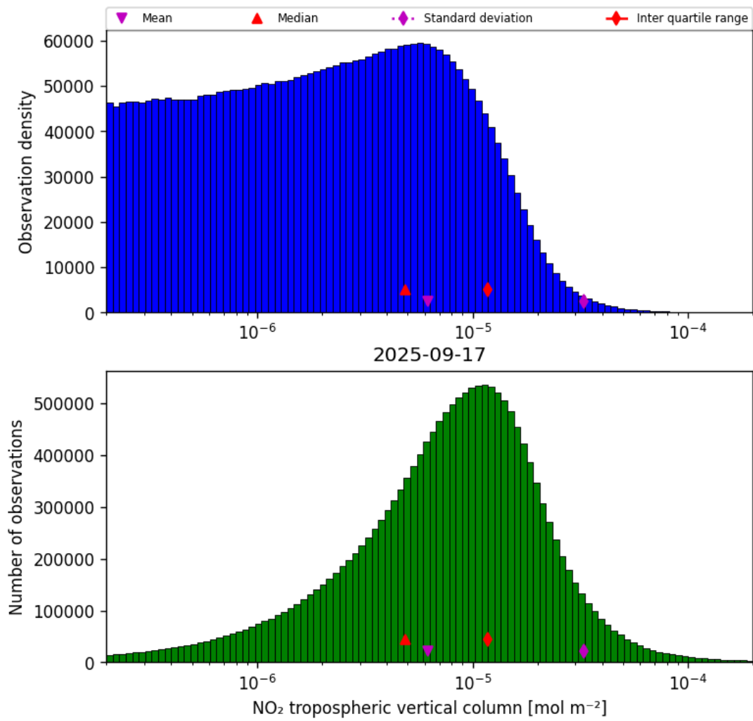
Figure 27: Histogram of “NO 2 tropospheric vertical column” for 2025-09-17 to 2025-09-18
