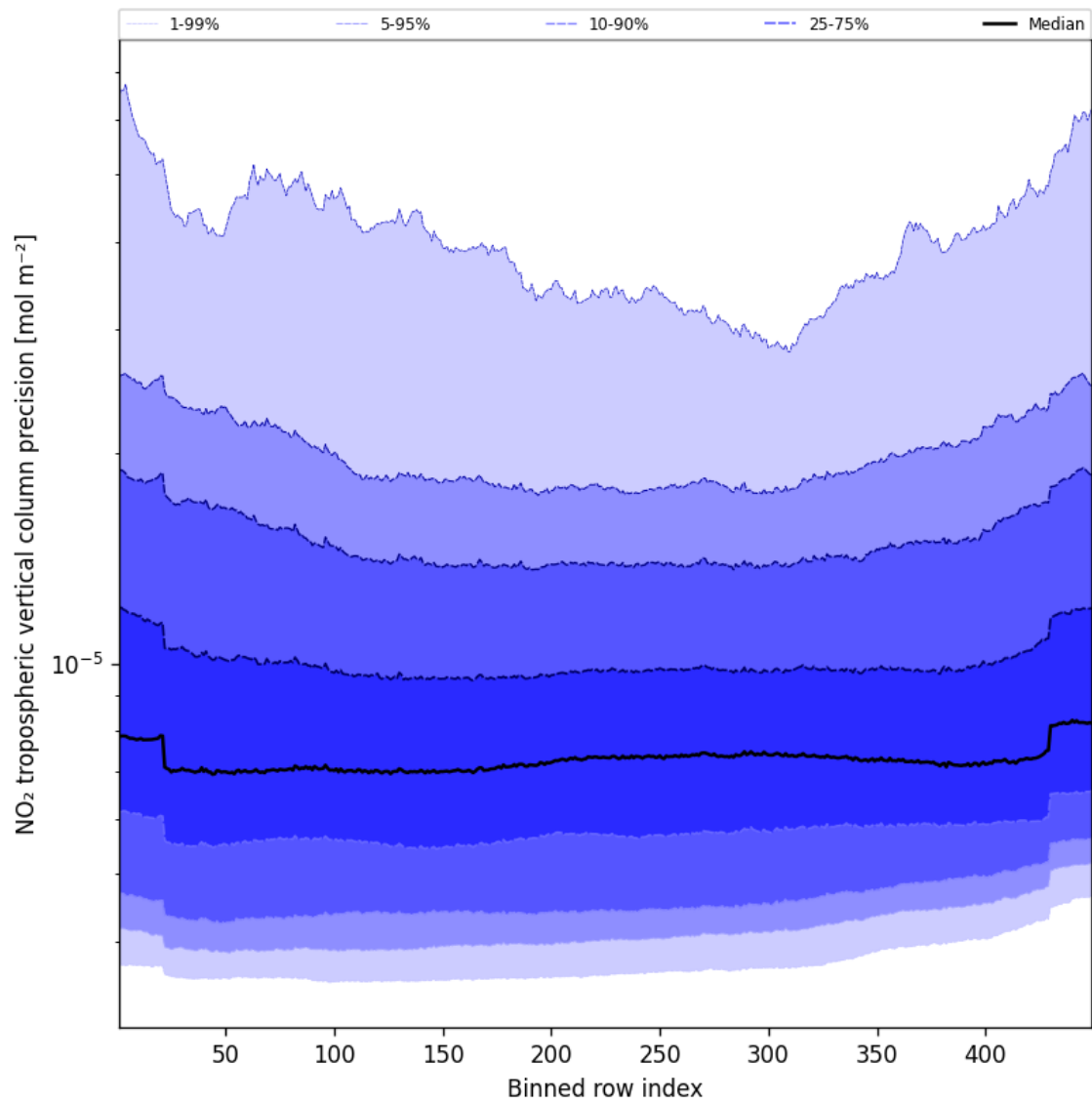
Figure 45: Along track statistics of “NO 2 tropospheric vertical column precision” for 2025-09-17 to 2025-09-18
