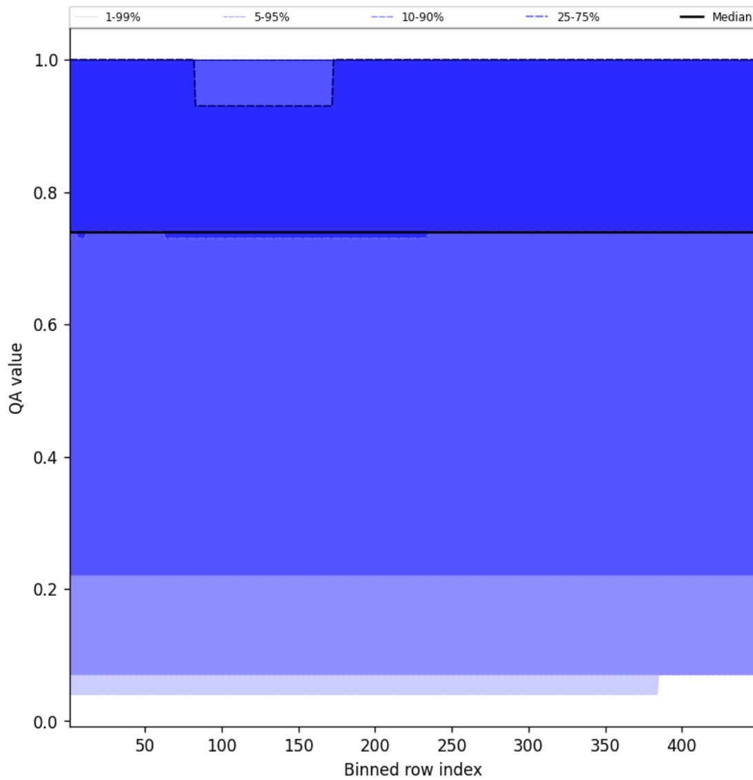
Figure 43: Along track statistics of “QA value” for 2025-09-17 to 2025-09-18
