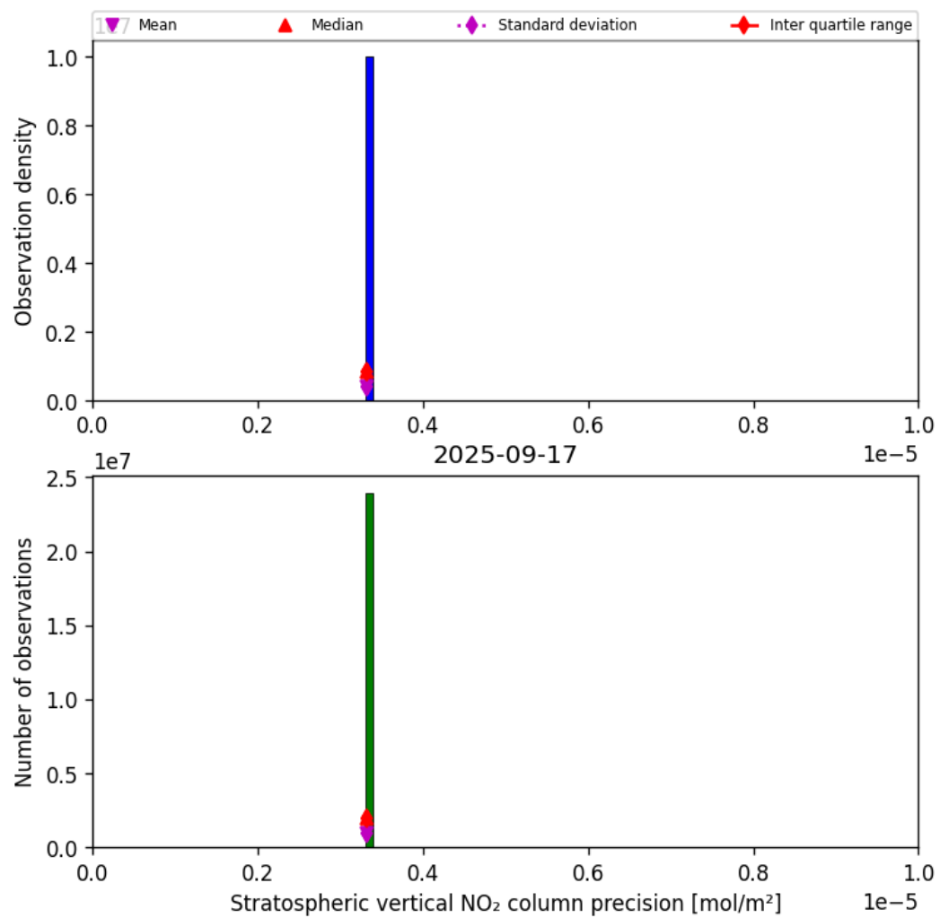
Figure 35: Histogram of “Stratospheric vertical NO 2 column precision” for 2025-09-17 to 2025-09-18
