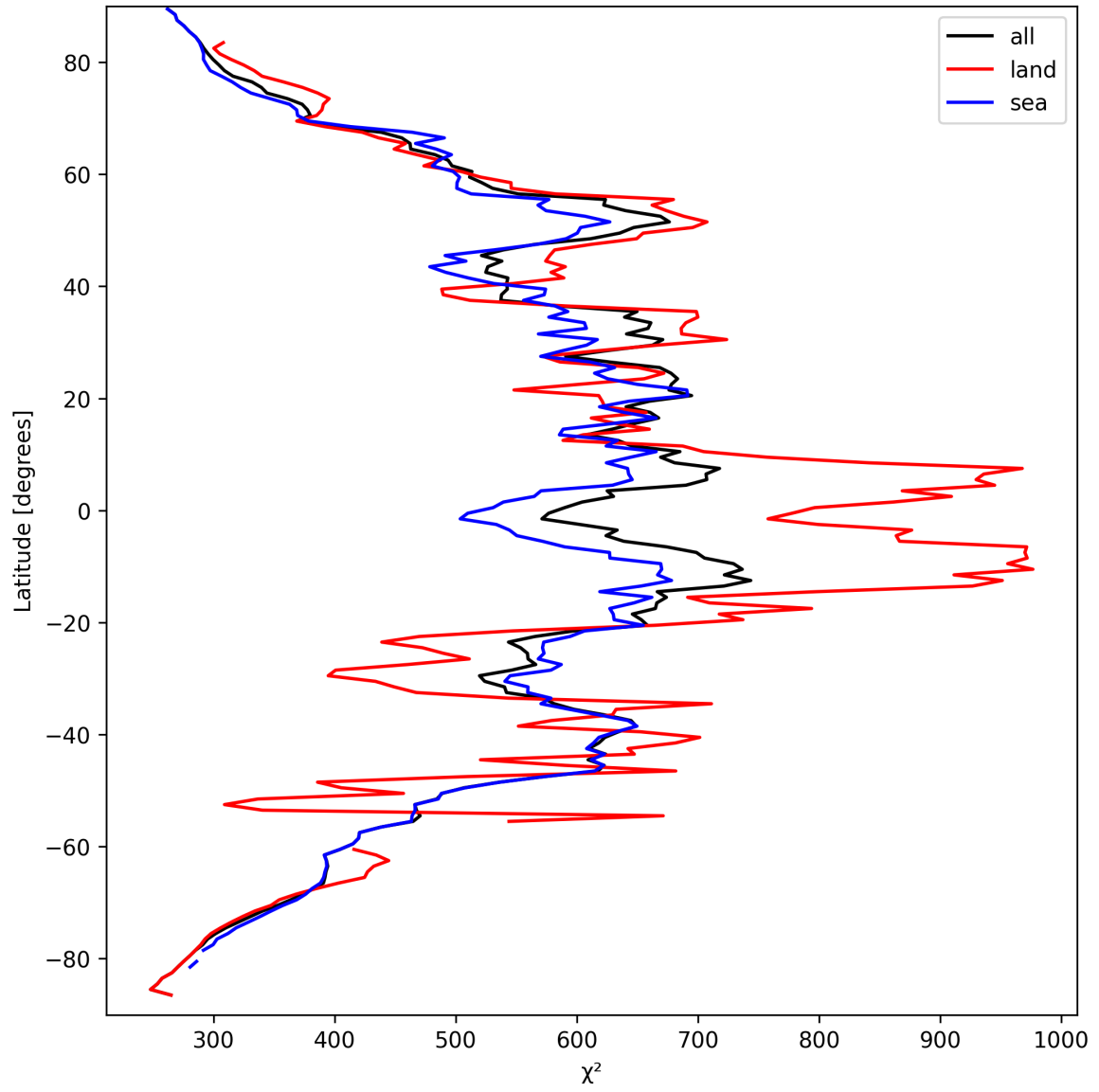
Figure 23: Zonal average of “ \chi^2 ” for 2025-09-17 to 2025-09-18.
