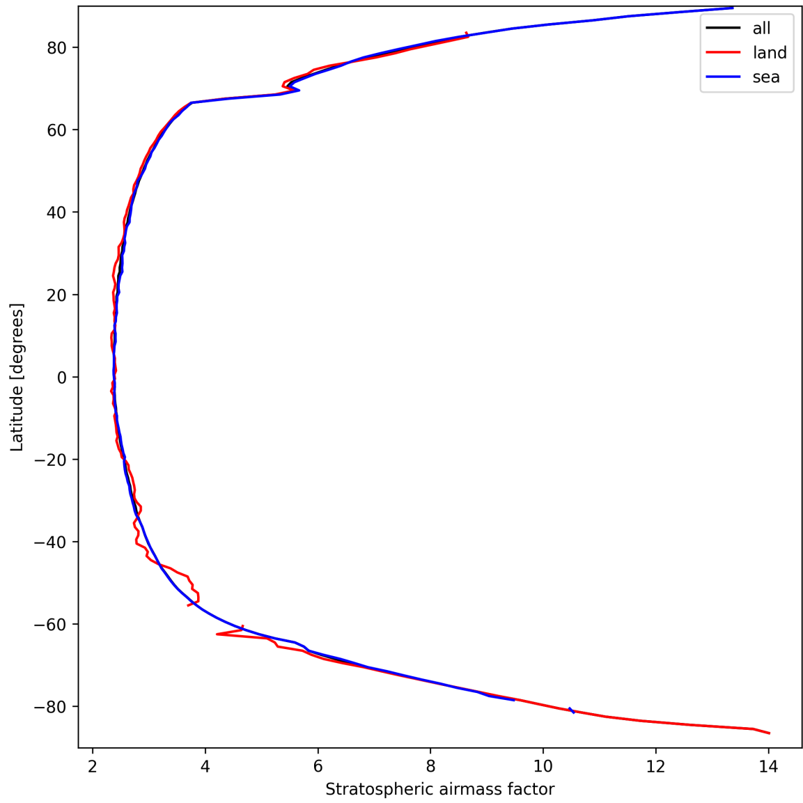
Figure 25: Zonal average of “Stratospheric airmass factor” for 2025-09-17 to 2025-09-18.
