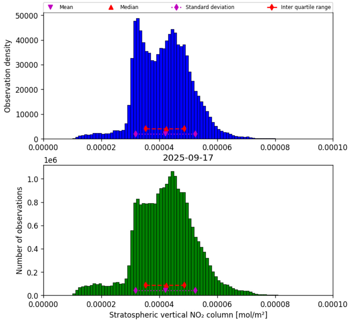
Figure 34: Histogram of “Stratospheric vertical NO 2 column” for 2025-09-17 to 2025-09-18
