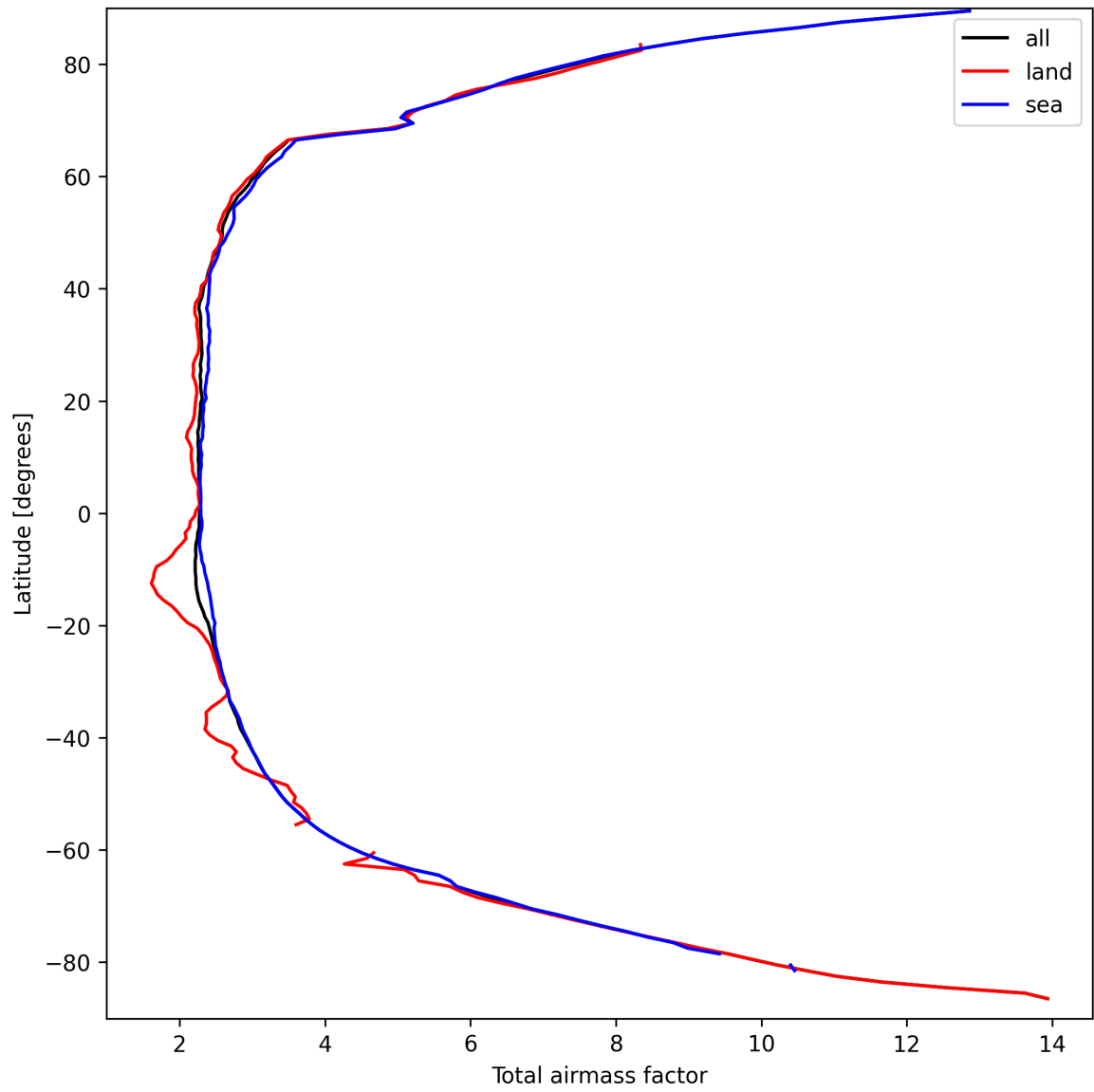
Figure 13: Zonal average of “Total airmass factor” for 2025-09-17 to 2025-09-18.
