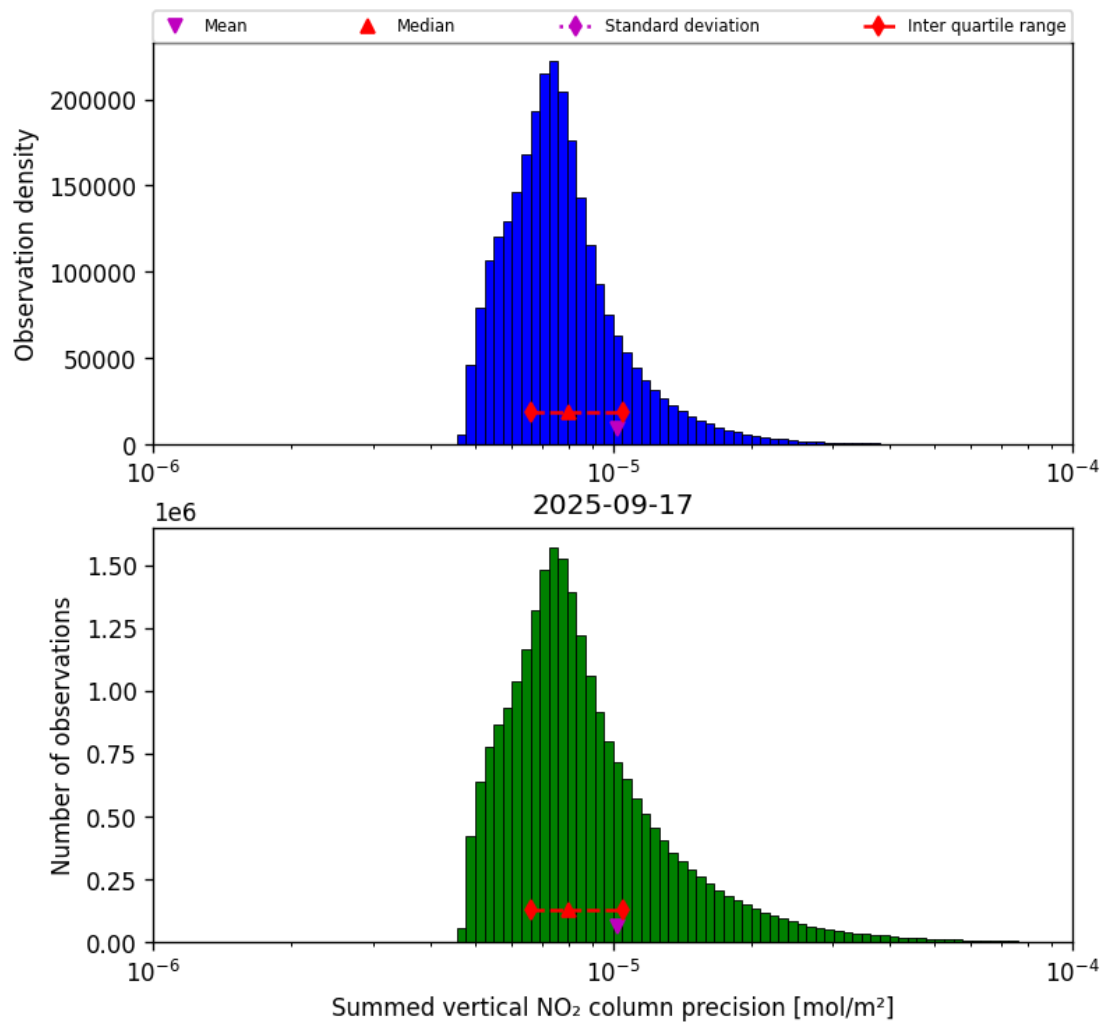
Figure 39: Histogram of “Summed vertical NO 2 column precision” for 2025-09-17 to 2025-09-18
