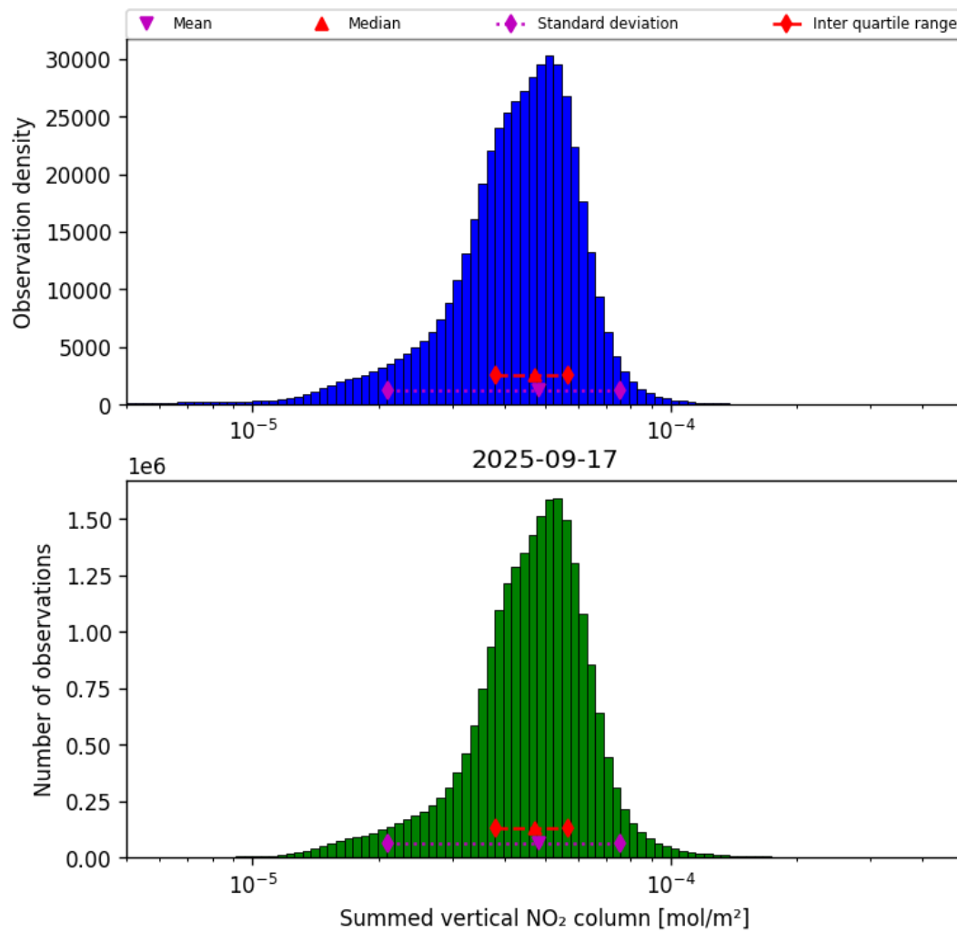
Figure 38: Histogram of “Summed vertical NO 2 column” for 2025-09-17 to 2025-09-18
