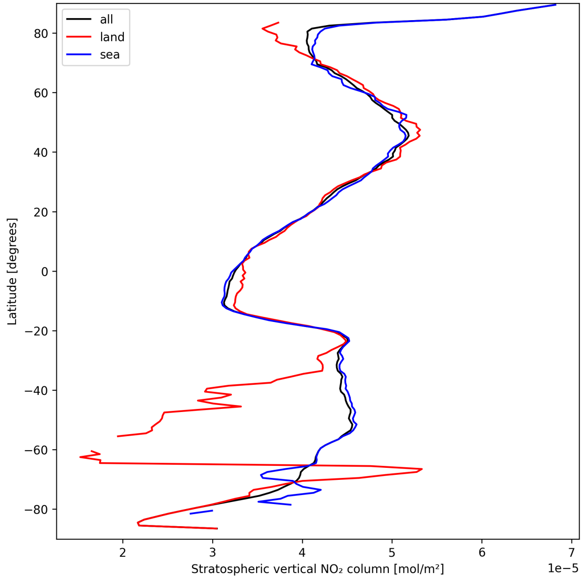
Figure 17: Zonal average of “Stratospheric vertical NO 2 column” for 2025-09-17 to 2025-09-18.
