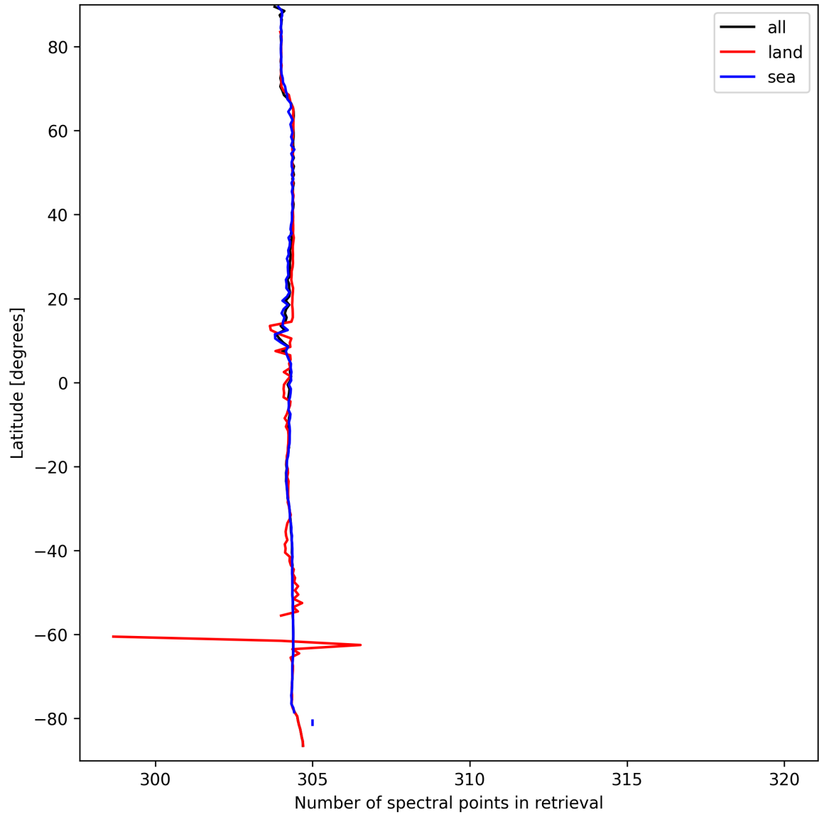
Figure 14: Zonal average of “Number of spectral points in retrieval” for 2025-09-17 to 2025-09-18.
