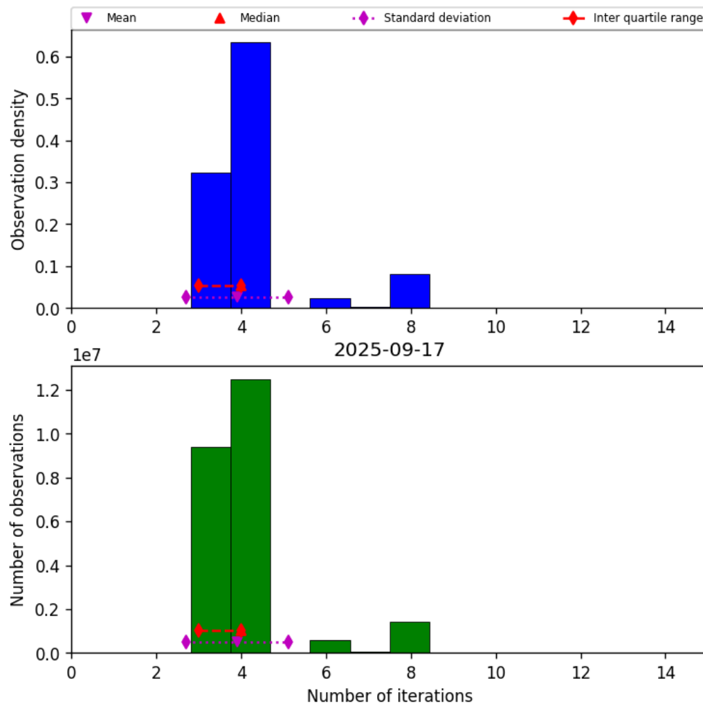
Figure 32: Histogram of “Number of iterations” for 2025-09-17 to 2025-09-18
