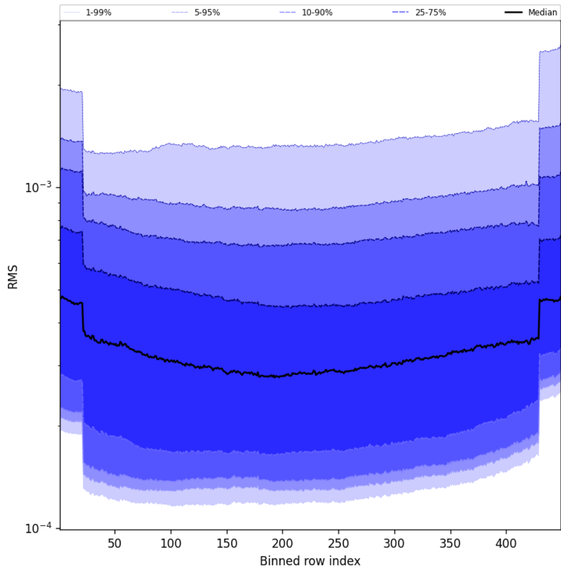
Figure 58: Along track statistics of “RMS” for 2025-09-17 to 2025-09-18
