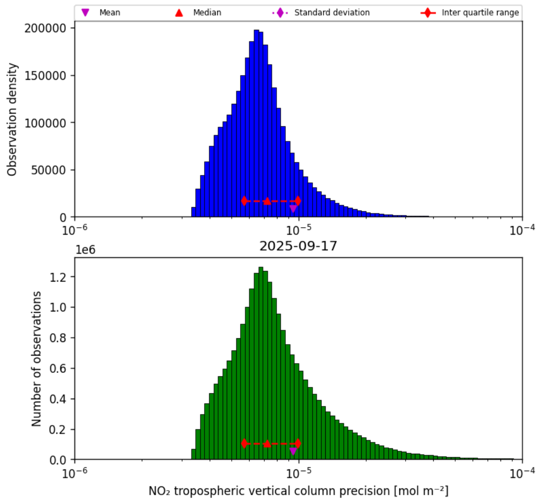
Figure 28: Histogram of “NO 2 tropospheric vertical column precision” for 2025-09-17 to 2025-09-18
