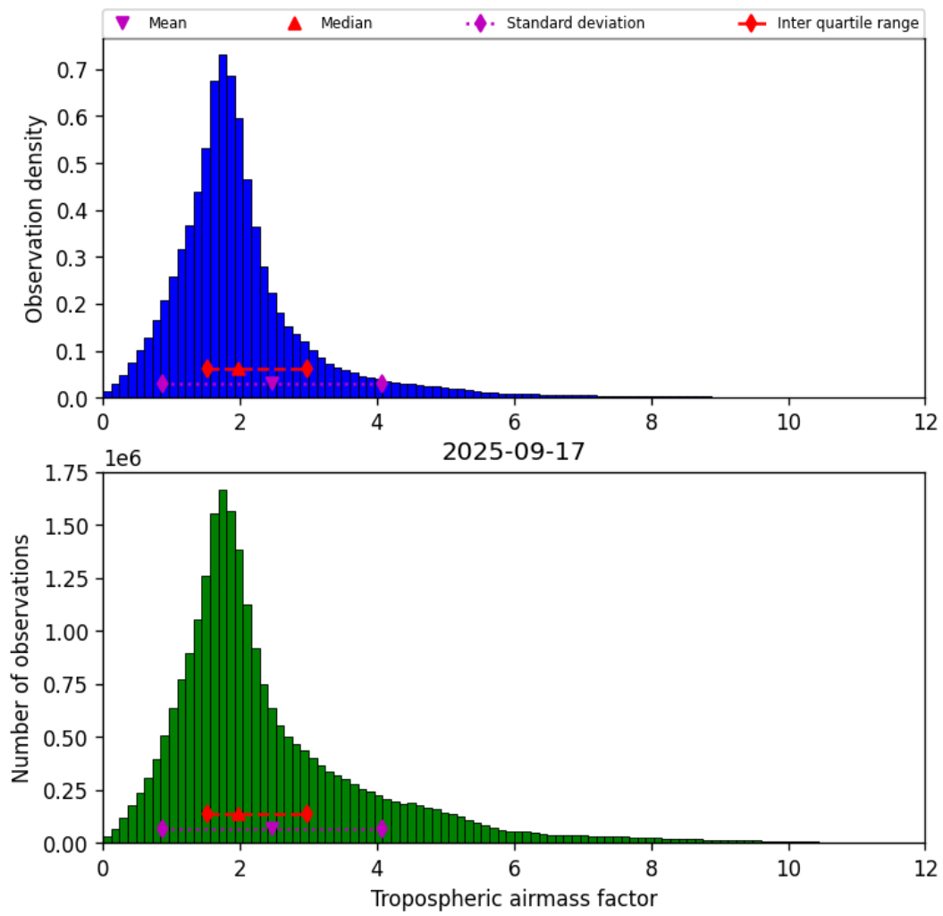
Figure 29: Histogram of “Tropospheric airmass factor” for 2025-09-17 to 2025-09-18
