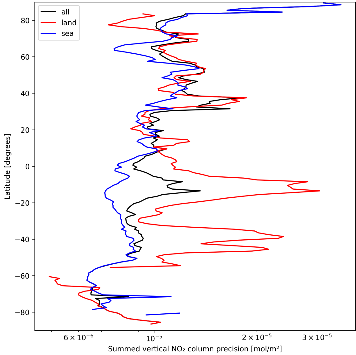
Figure 22: Zonal average of “Summed vertical NO 2 column precision” for 2025-09-17 to 2025-09-18.
