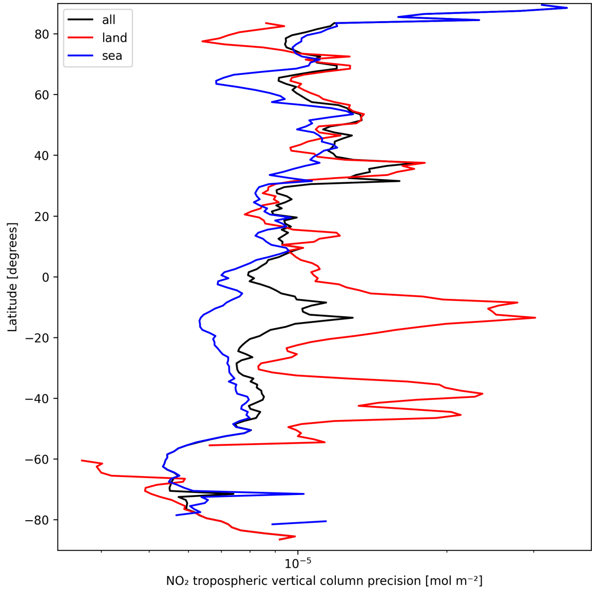
Figure 11: Zonal average of “NO 2 tropospheric vertical column precision” for 2025-09-17 to 2025-09-18.
