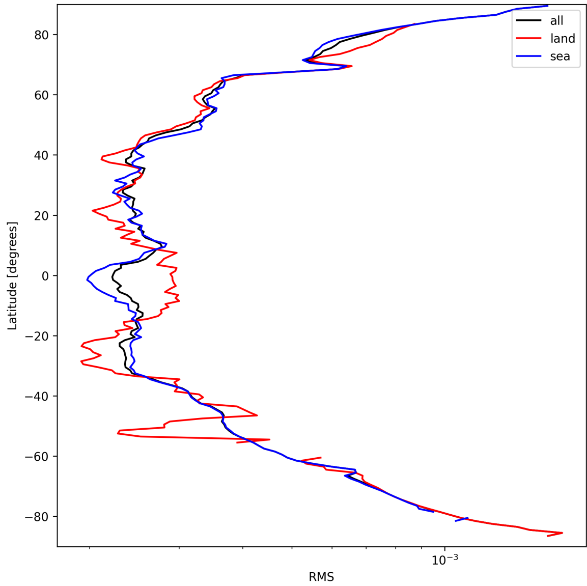
Figure 24: Zonal average of “RMS” for 2025-09-17 to 2025-09-18.
