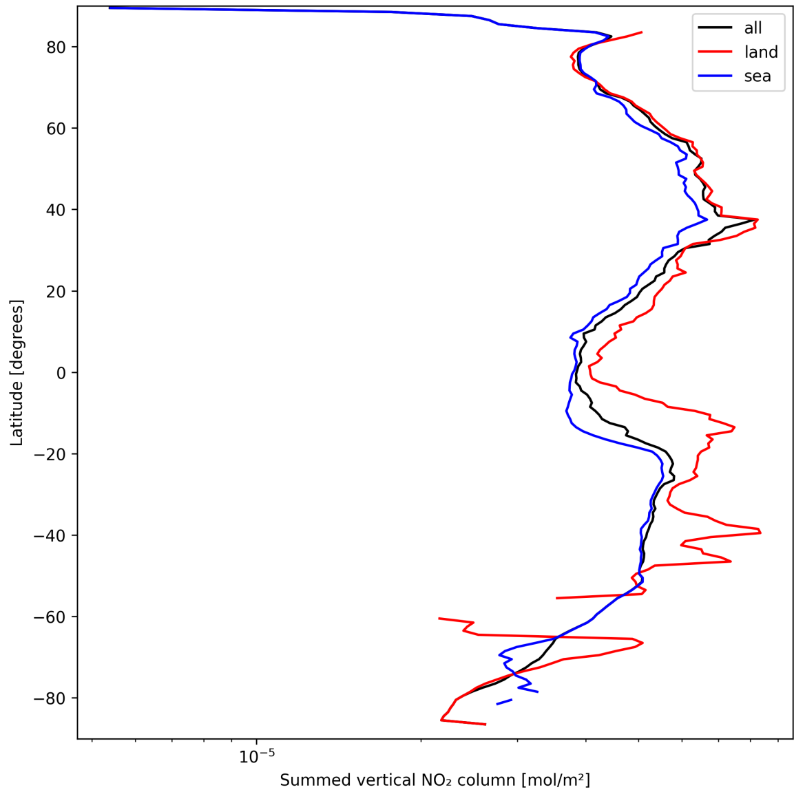
Figure 21: Zonal average of “Summed vertical NO 2 column” for 2025-09-17 to 2025-09-18.
