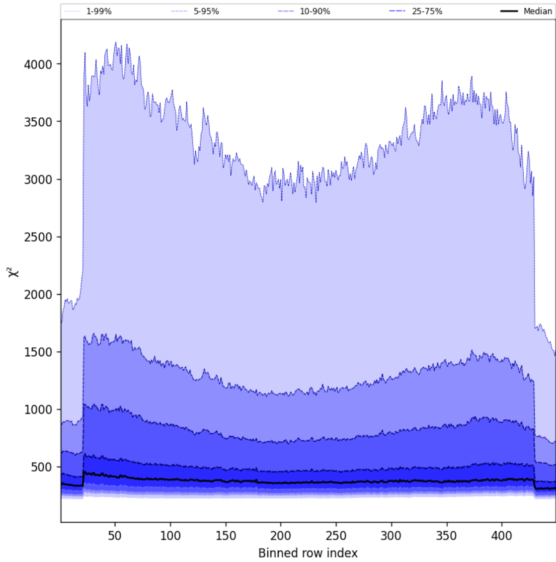
Figure 57: Along track statistics of “ \chi^2 ” for 2025-09-17 to 2025-09-18
