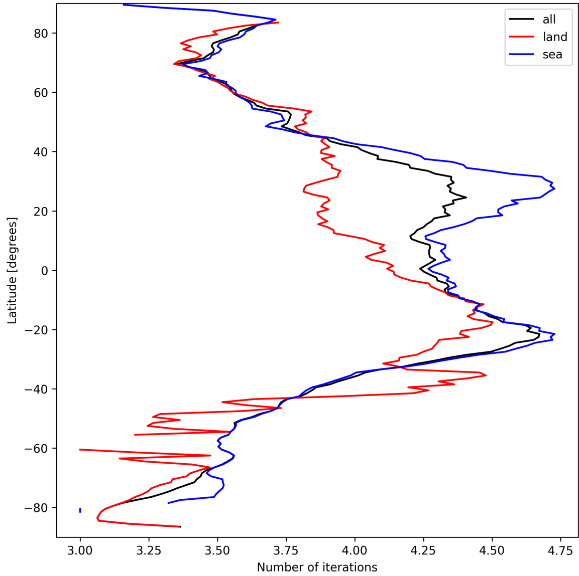
Figure 15: Zonal average of “Number of iterations” for 2025-09-17 to 2025-09-18.
