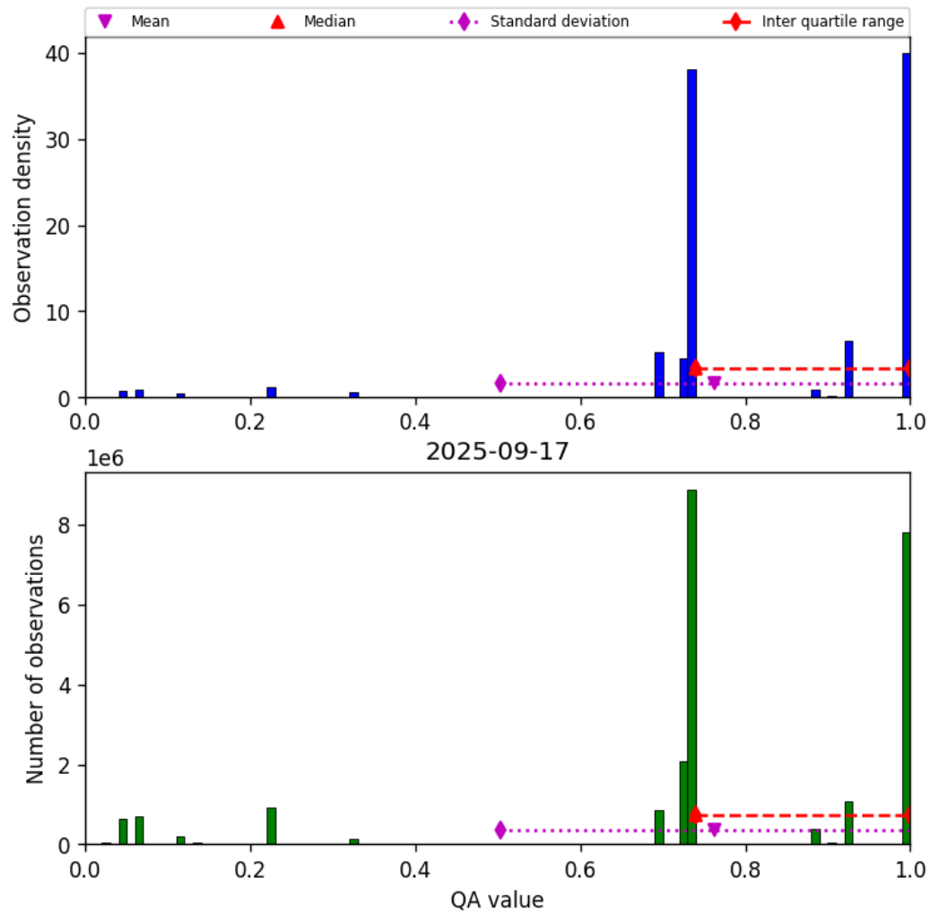
Figure 26: Histogram of “QA value” for 2025-09-17 to 2025-09-18
