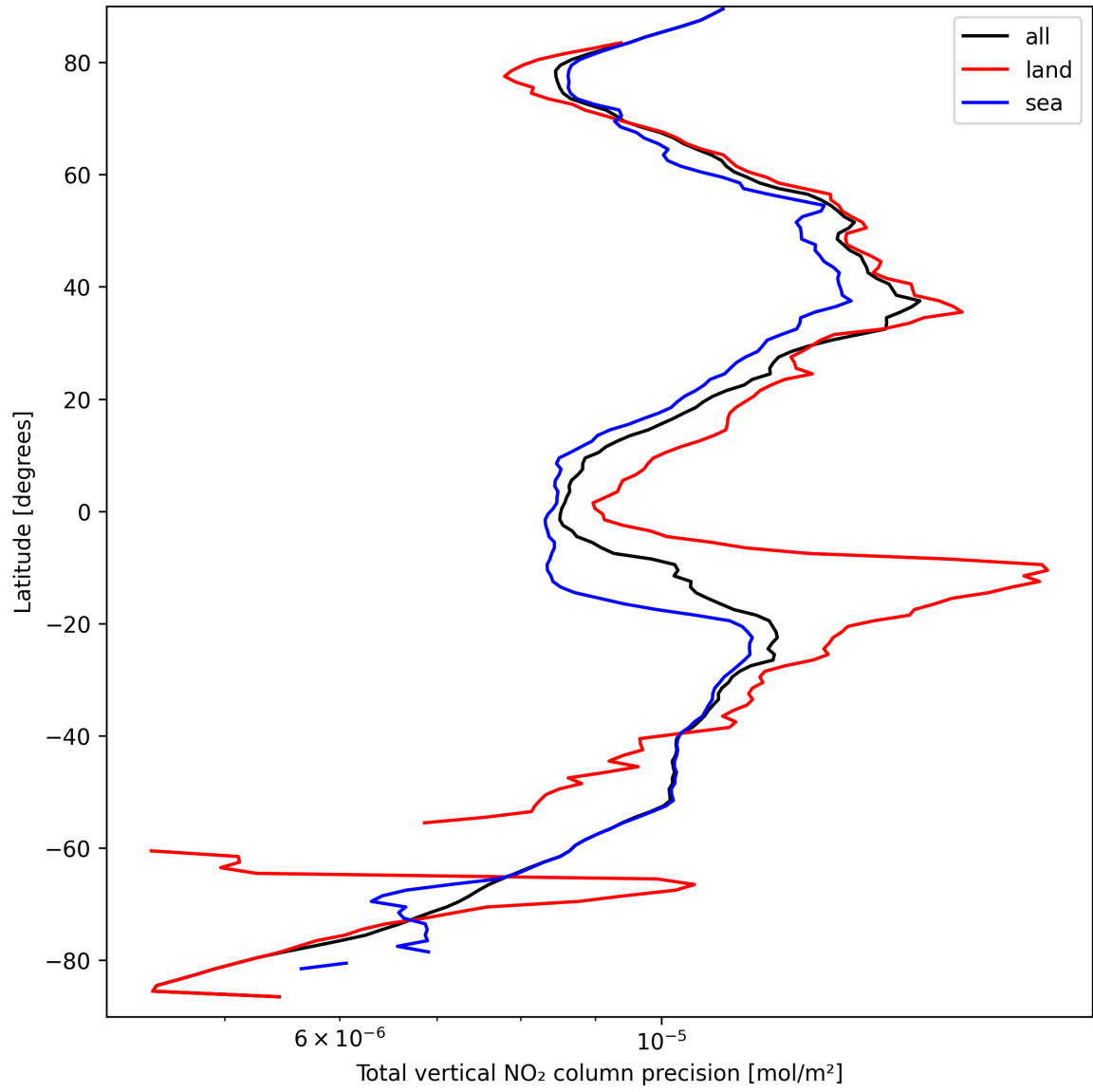
Figure 20: Zonal average of “Total vertical NO 2 column precision” for 2025-09-17 to 2025-09-18.
