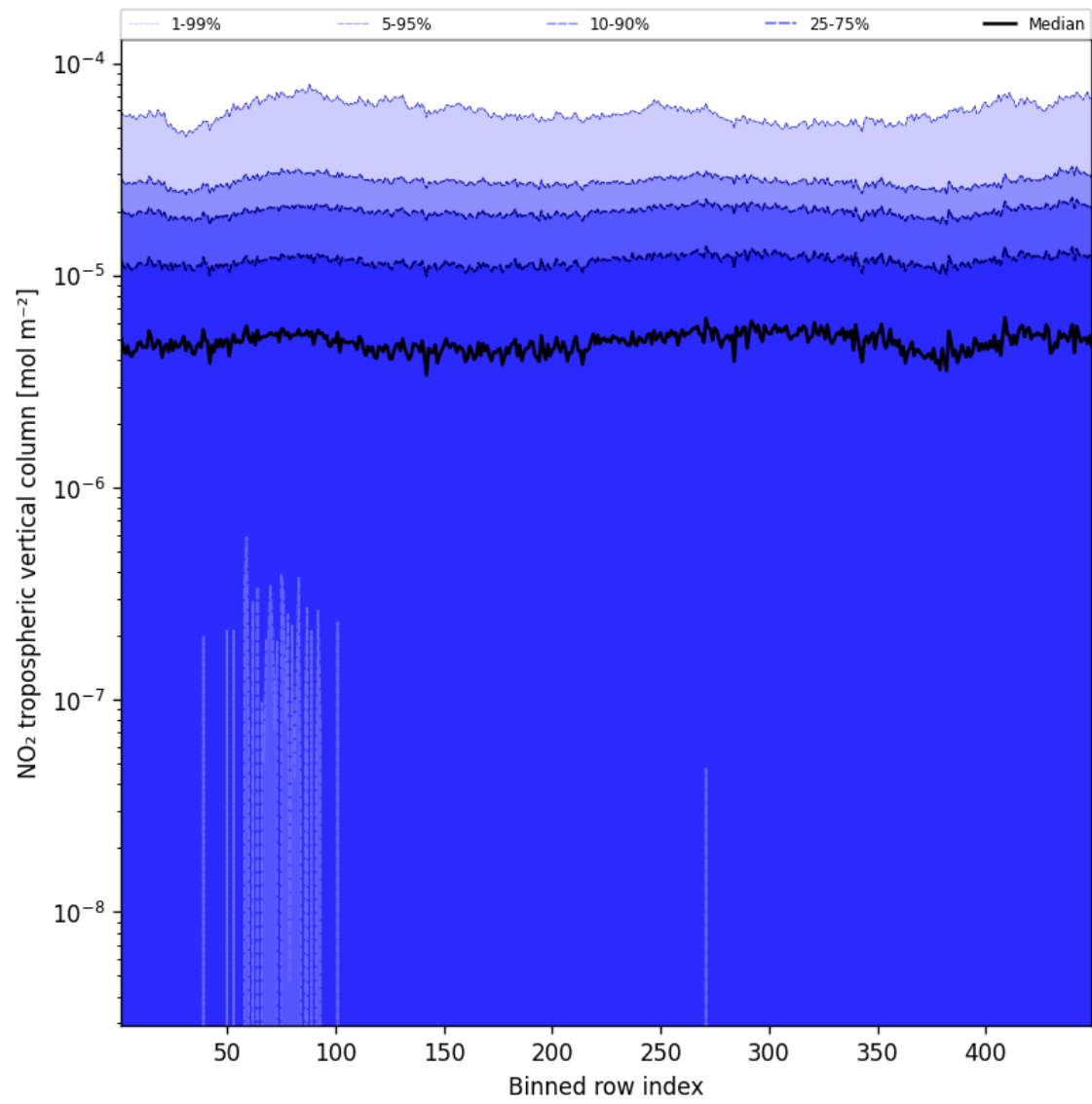
Figure 44: Along track statistics of “NO 2 tropospheric vertical column” for 2025-09-17 to 2025-09-18
