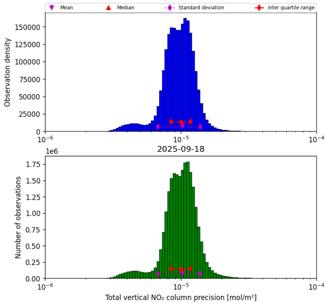
Figure 37: Histogram of "Total vertical NO 2 column precision" for 2025-09-18 to 2025-09-18
