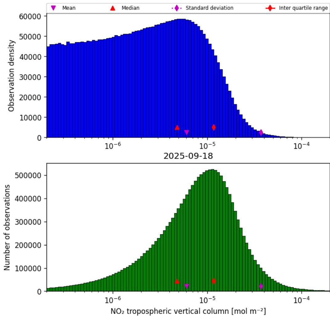
Figure 27: Histogram of “NO 2 tropospheric vertical column” for 2025-09-18 to 2025-09-18
