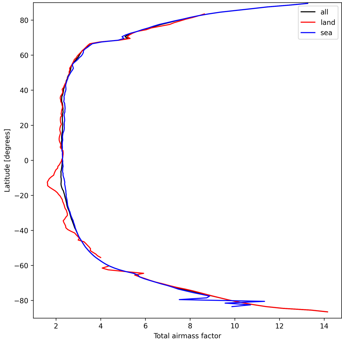
Figure 13: Zonal average of “Total airmass factor” for 2025-09-18 to 2025-09-18.
