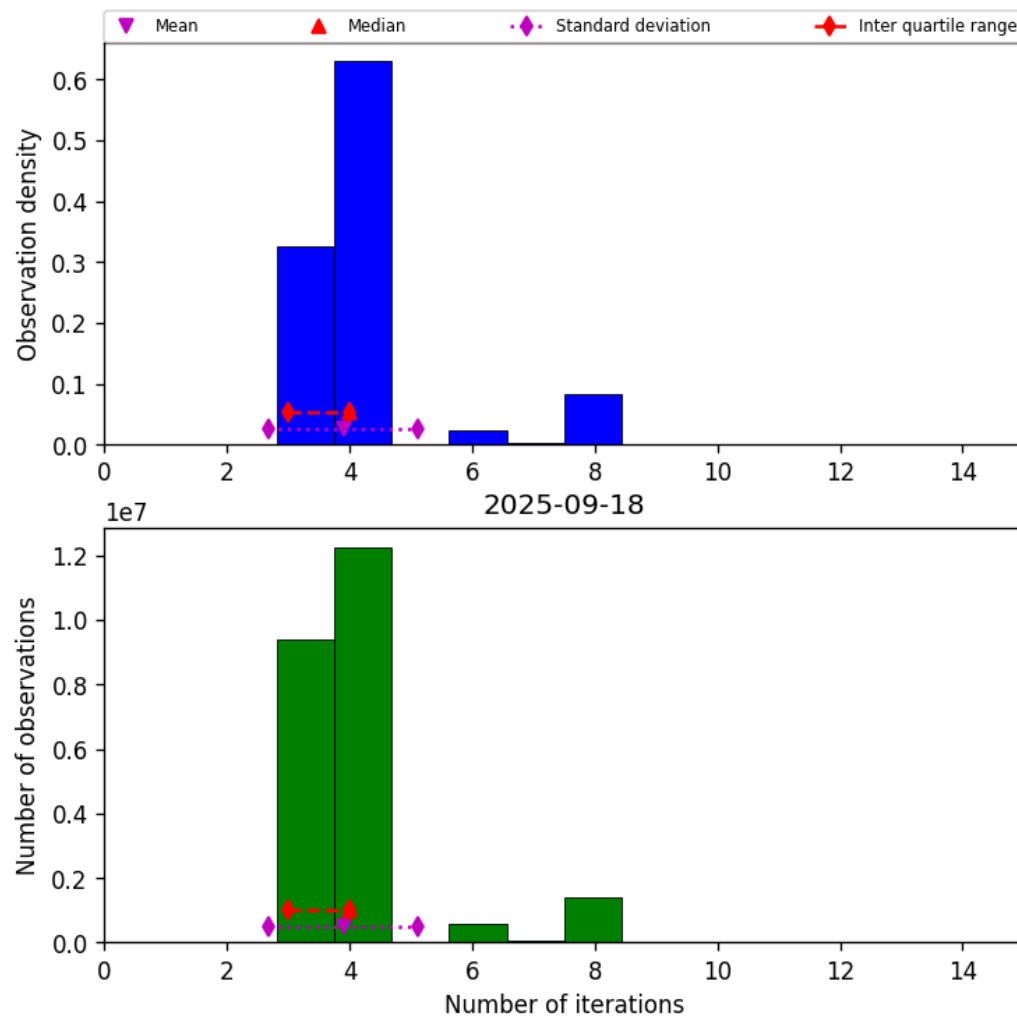
Figure 32: Histogram of “Number of iterations” for 2025-09-18 to 2025-09-18
