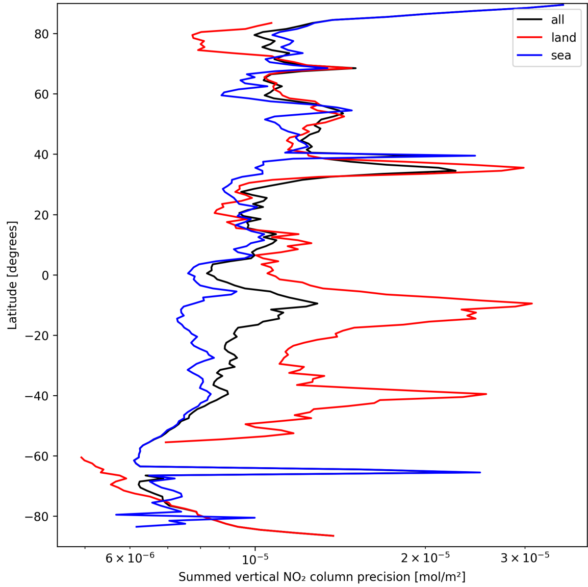
Figure 22: Zonal average of “Summed vertical NO 2 column precision” for 2025-09-18 to 2025-09-18.
