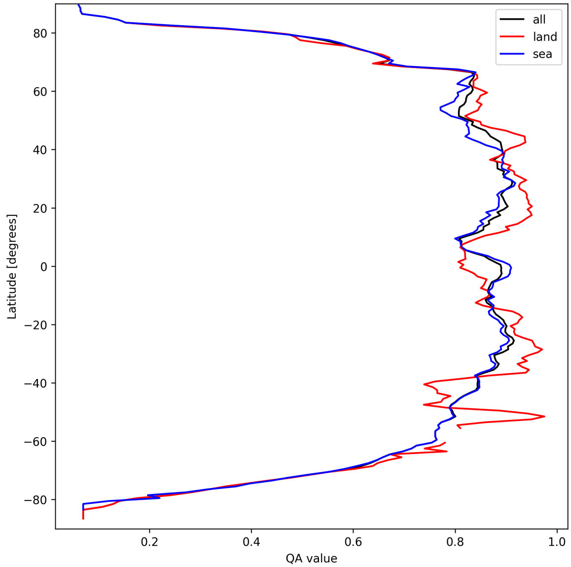
Figure 9: Zonal average of “QA value” for 2025-09-18 to 2025-09-18.
