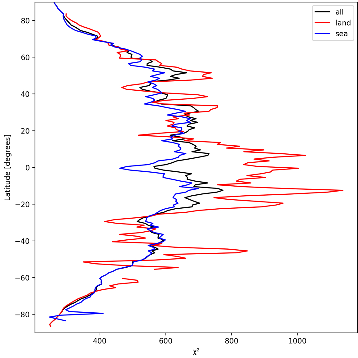
Figure 23: Zonal average of “ \chi^2 ” for 2025-09-18 to 2025-09-18.
