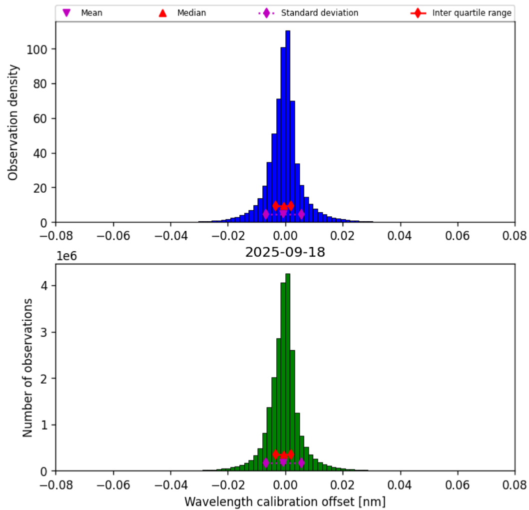
Figure 33: Histogram of “Wavelength calibration offset” for 2025-09-18 to 2025-09-18
