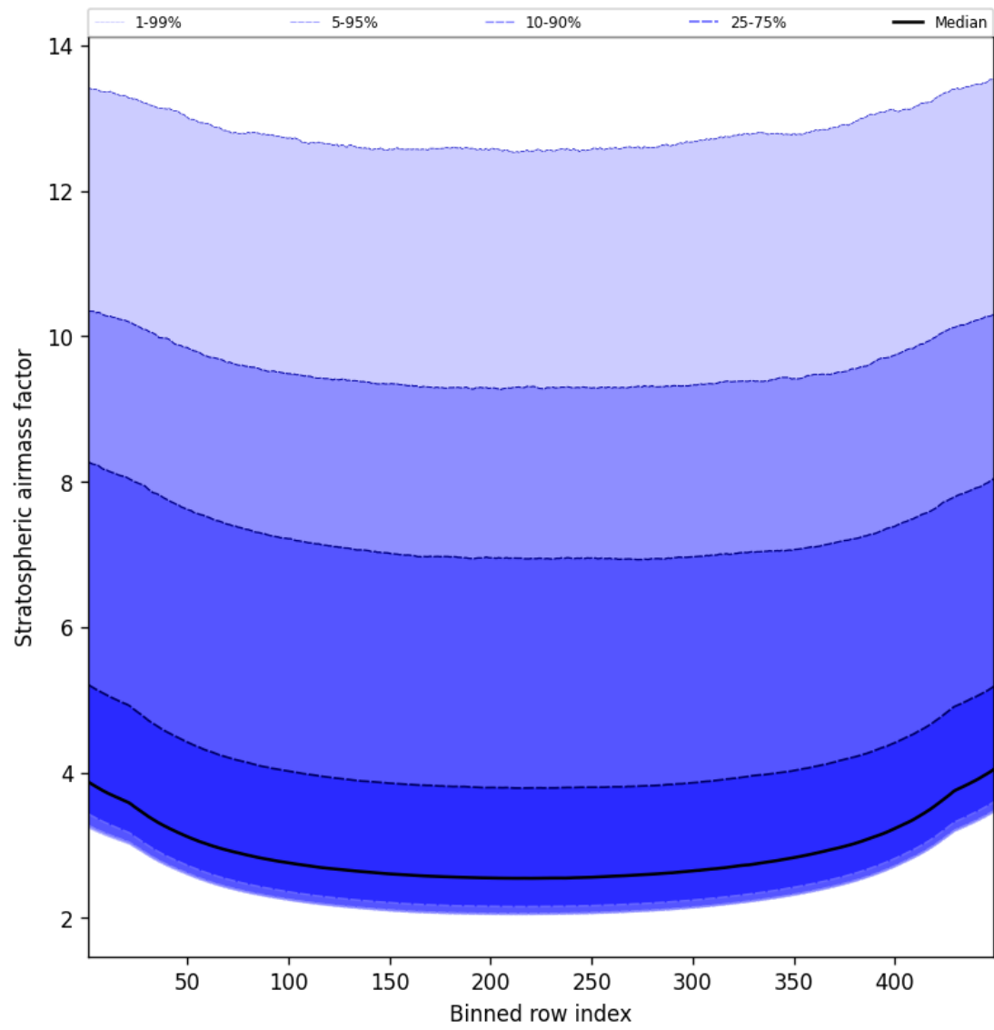
Figure 59: Along track statistics of “Stratospheric airmass factor” for 2025-09-18 to 2025-09-18
