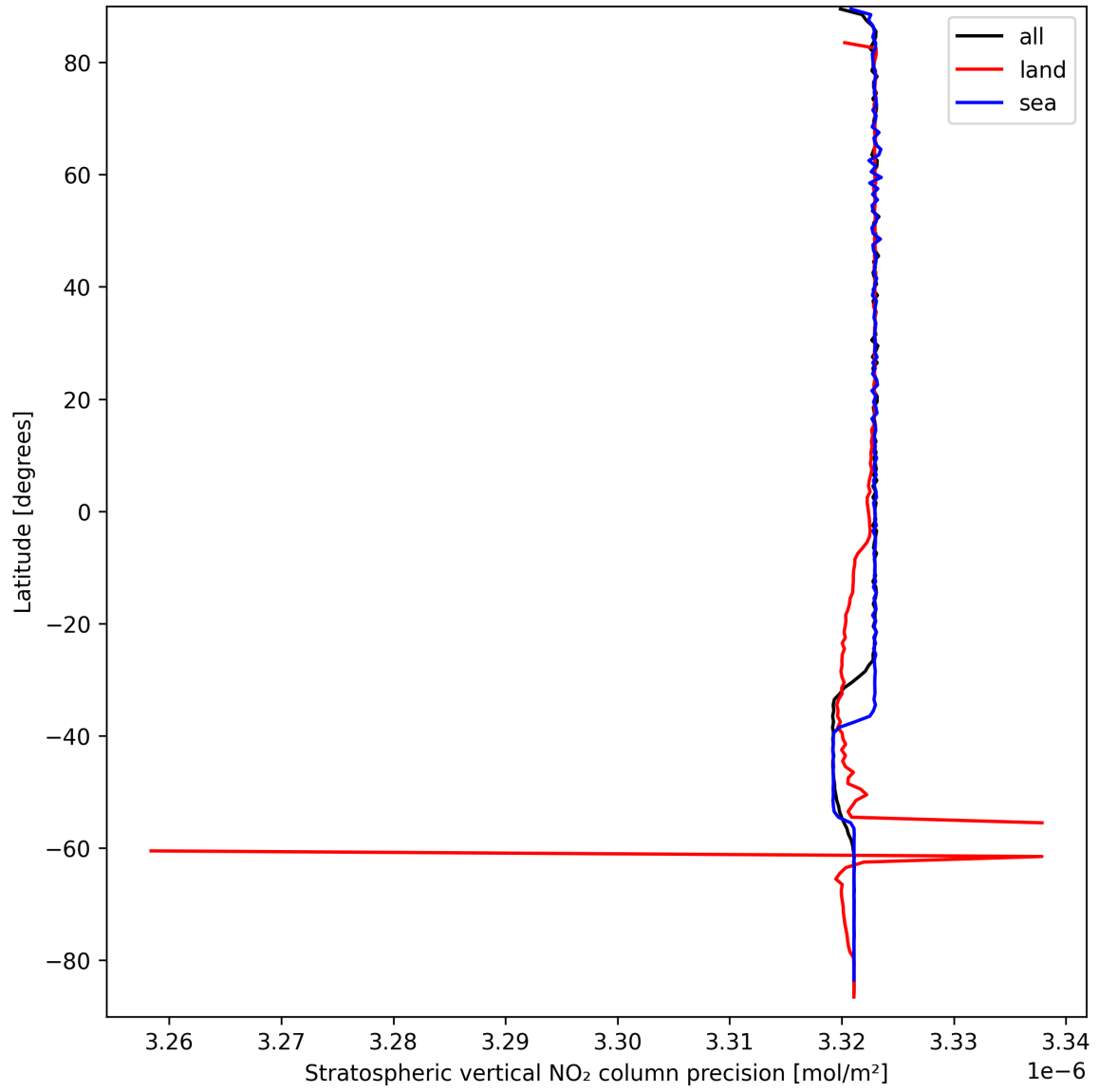
Figure 18: Zonal average of “Stratospheric vertical NO 2 column precision” for 2025-09-18 to 2025-09-18.
