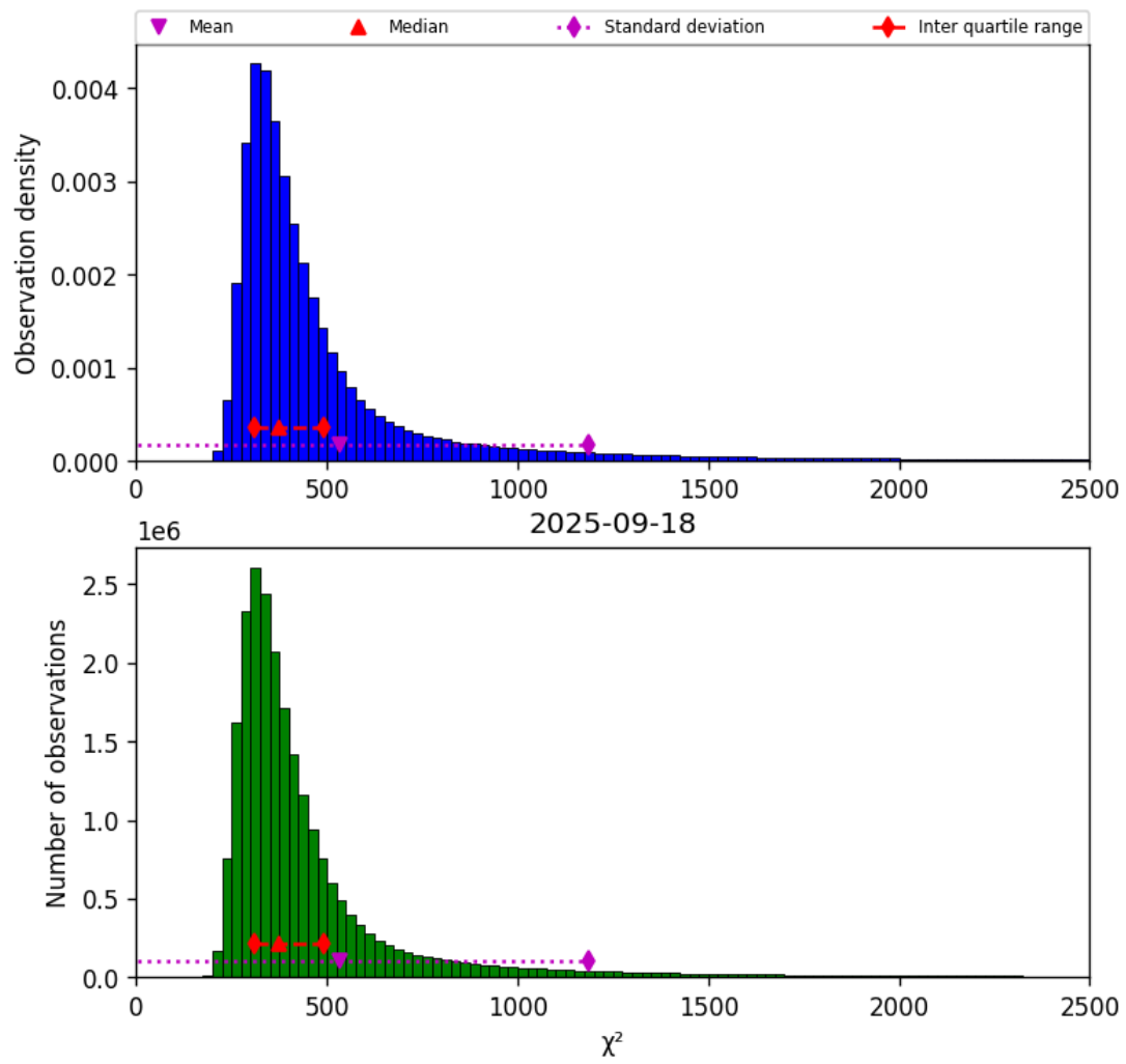
Figure 40: Histogram of “ \chi^2 ” for 2025-09-18 to 2025-09-18
