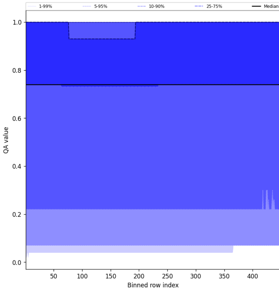
Figure 43: Along track statistics of "QA value" for 2025-09-18 to 2025-09-18
