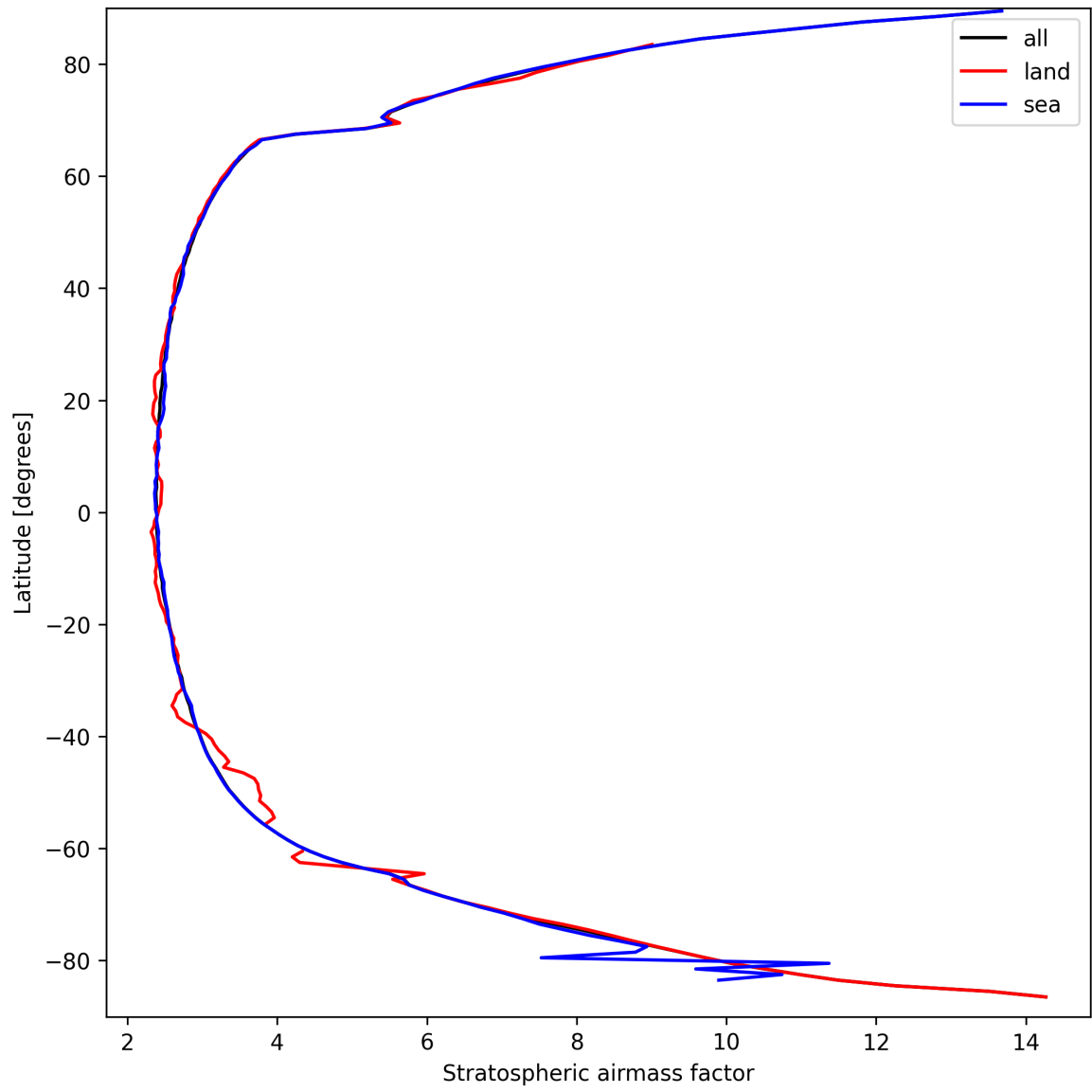
Figure 25: Zonal average of “Stratospheric air mass factor” for 2025-09-18 to 2025-09-18.
