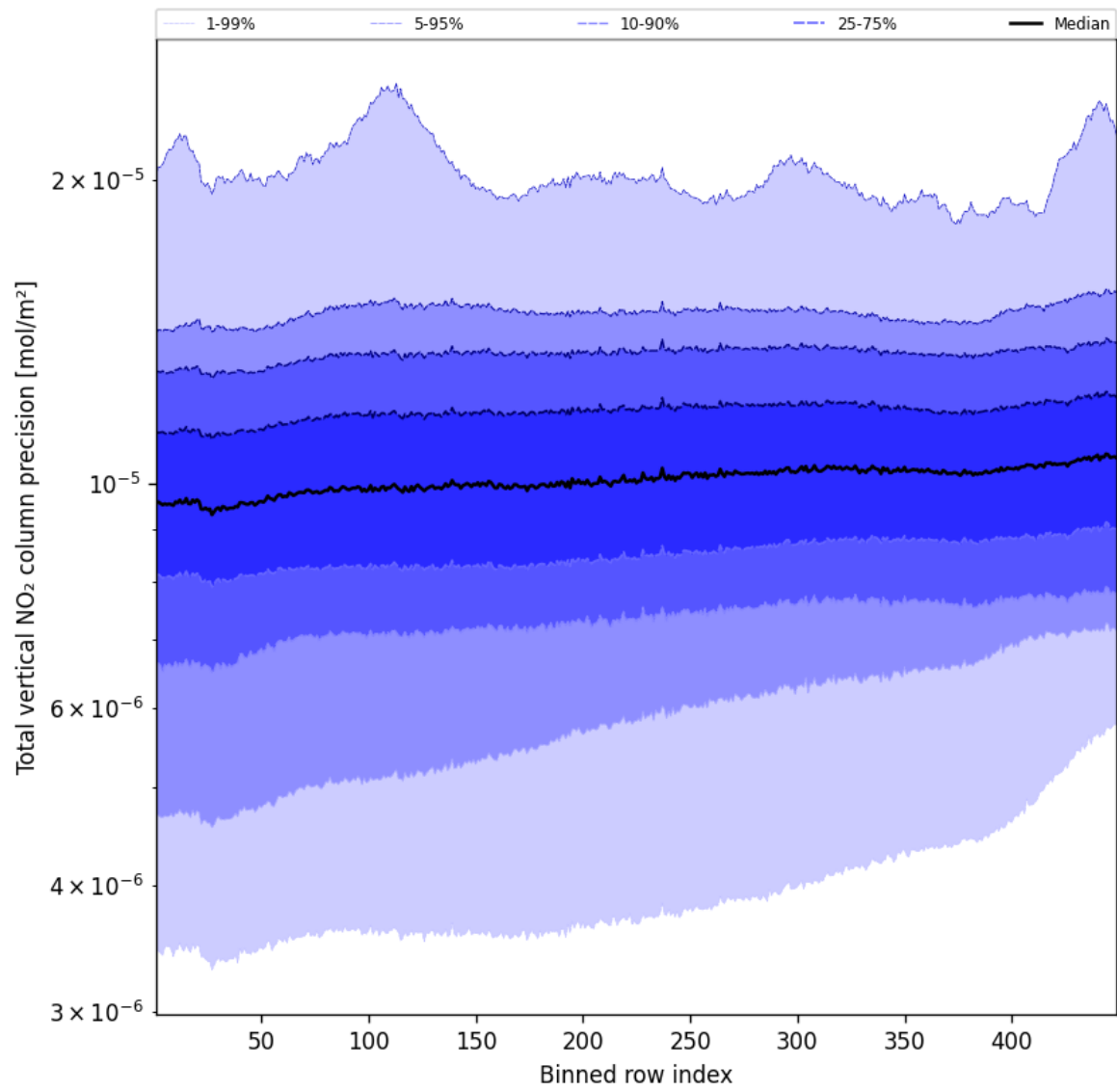
Figure 54: Along track statistics of “Total vertical NO 2 column precision” for 2025-09-18 to 2025-09-18
