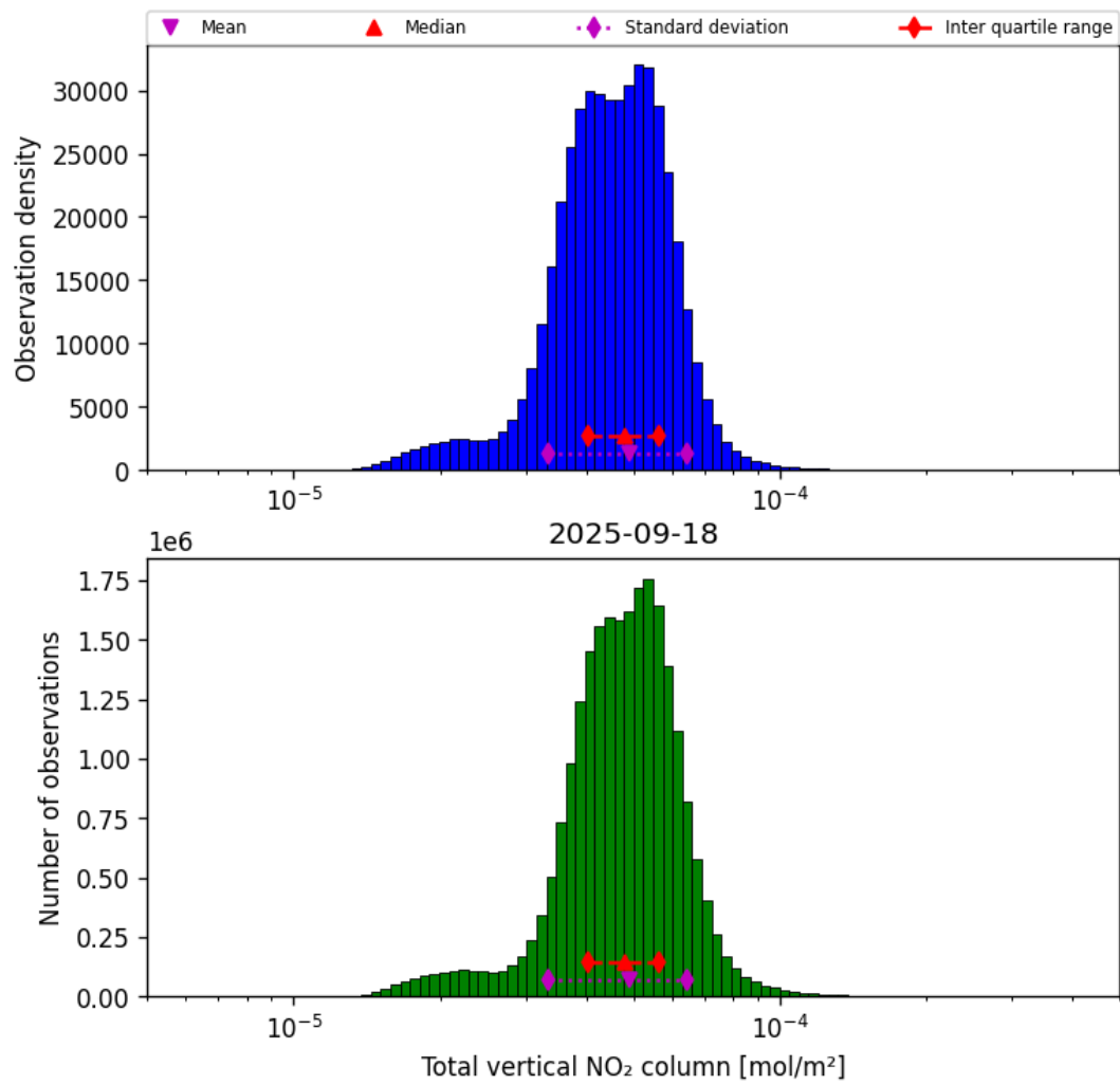
Figure 36: Histogram of "Total vertical NO 2 column" for 2025-09-18 to 2025-09-18
