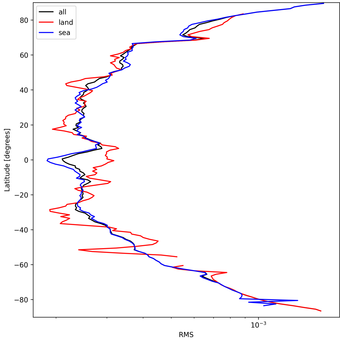
Figure 24: Zonal average of “RMS” for 2025-09-18 to 2025-09-18.
