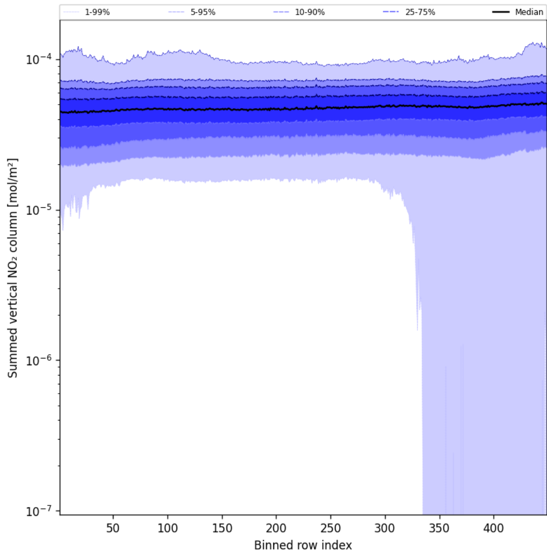
Figure 55: Along track statistics of “Summed vertical NO 2 column” for 2025-09-18 to 2025-09-18
