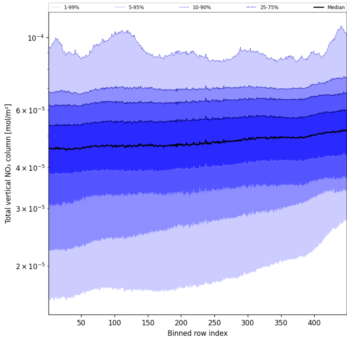
Figure 53: Along track statistics of “Total vertical NO 2 column” for 2025-09-18 to 2025-09-18
