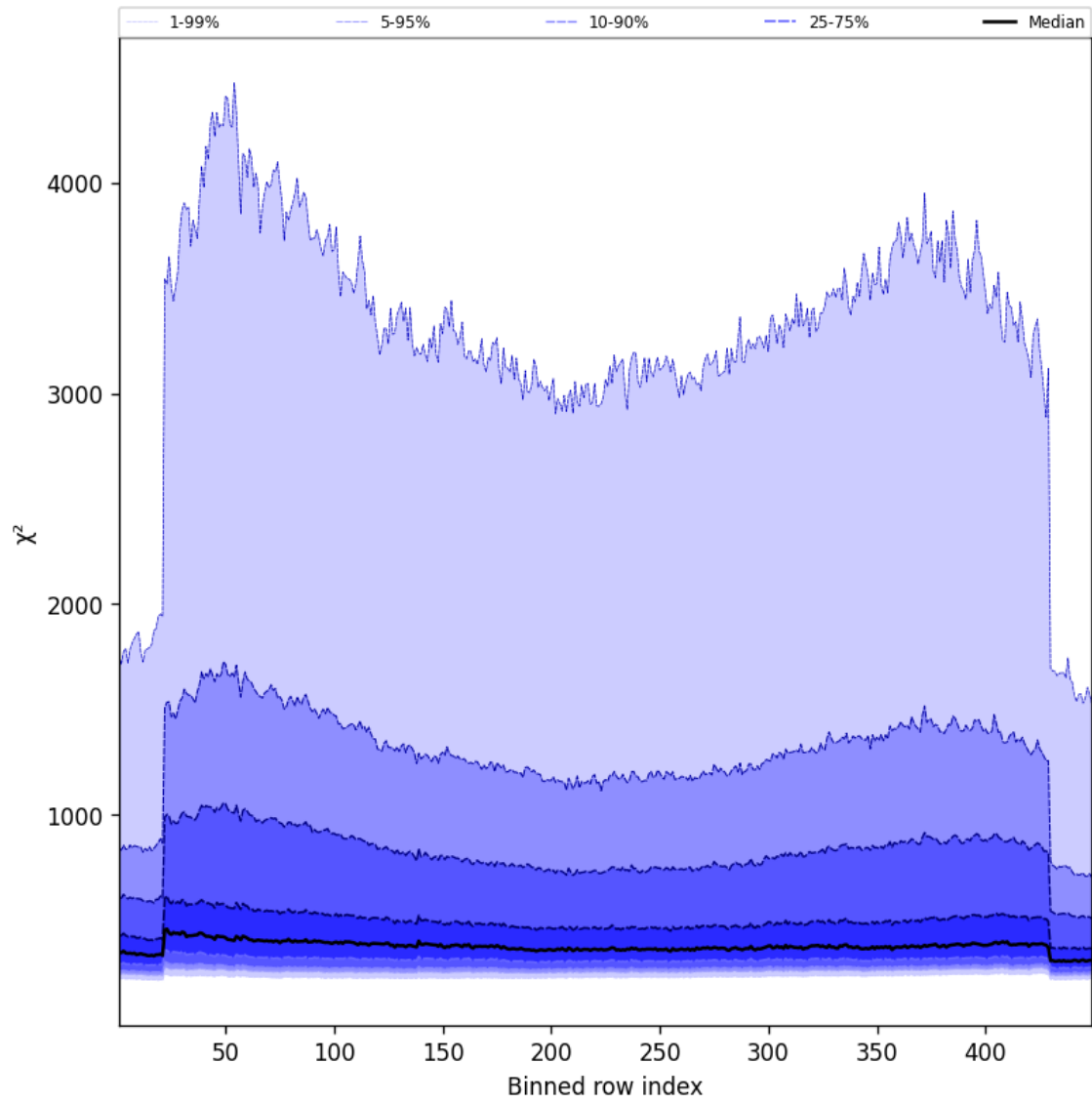
Figure 57: Along track statistics of “ \chi^2 ” for 2025-09-18 to 2025-09-18
