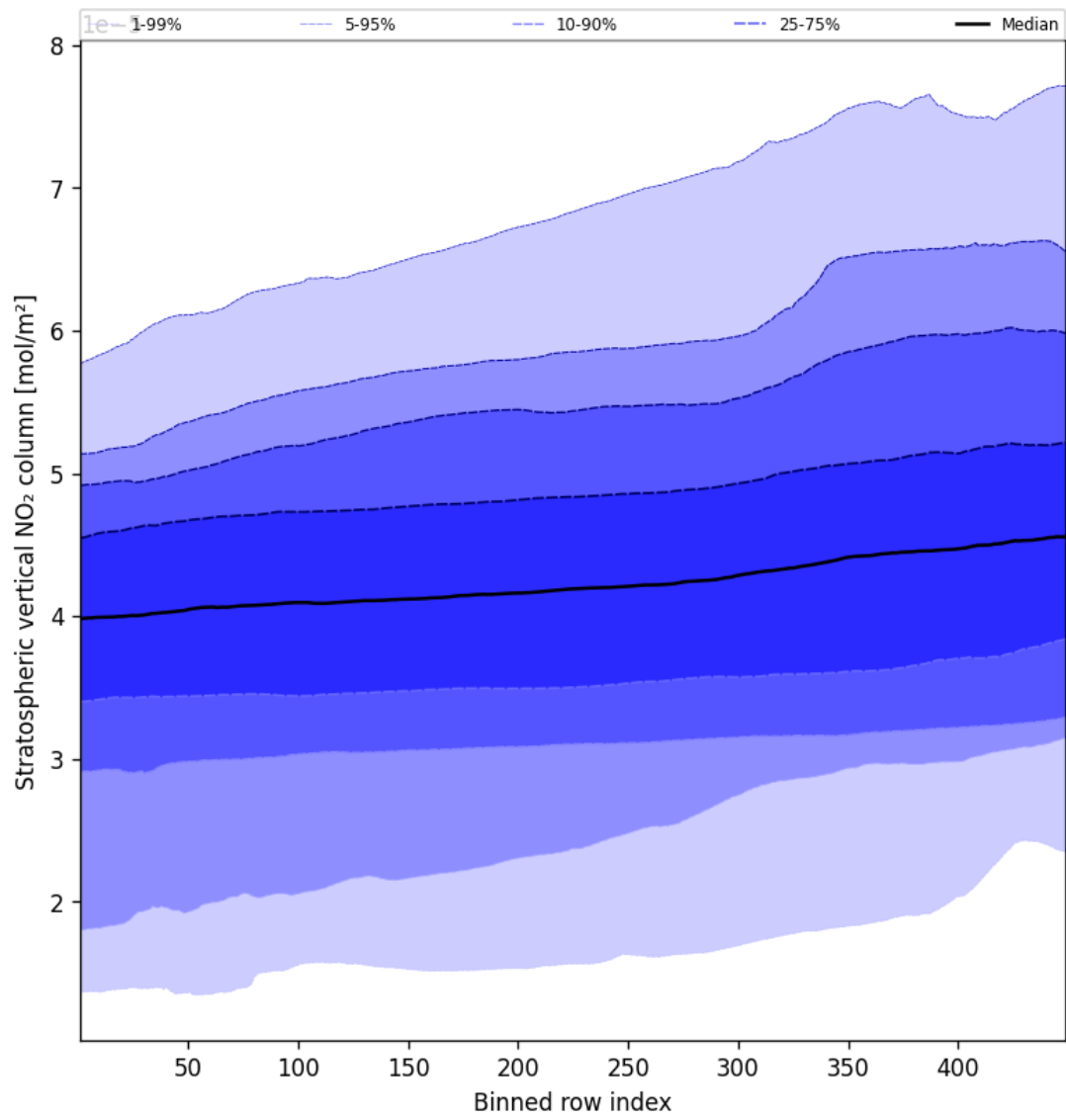
Figure 51: Along track statistics of “Stratospheric vertical NO 2 column” for 2025-09-18 to 2025-09-18
