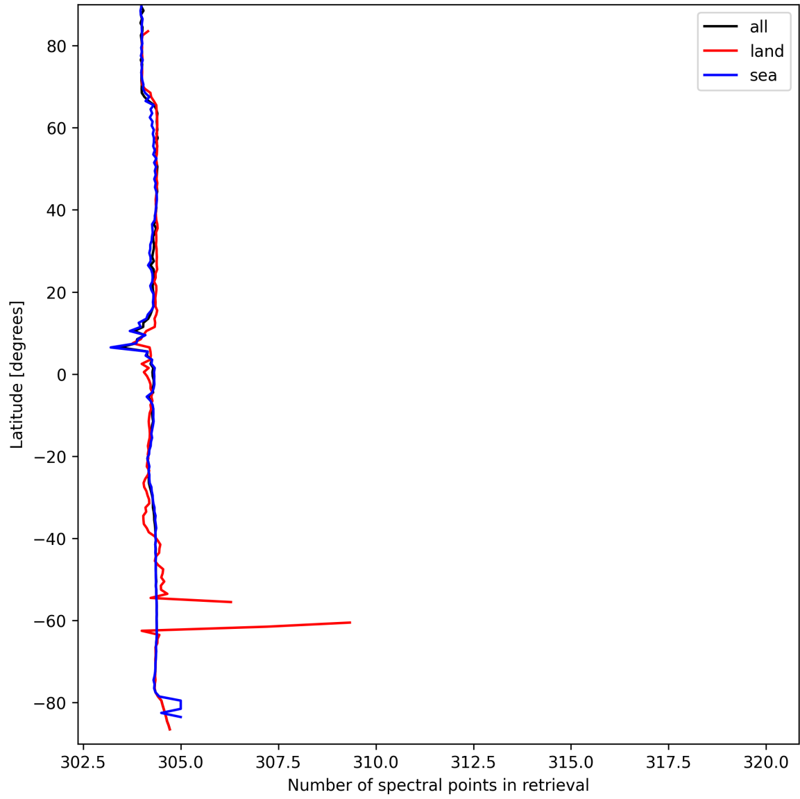
Figure 14: Zonal average of “Number of spectral points in retrieval” for 2025-09-18 to 2025-09-18.
