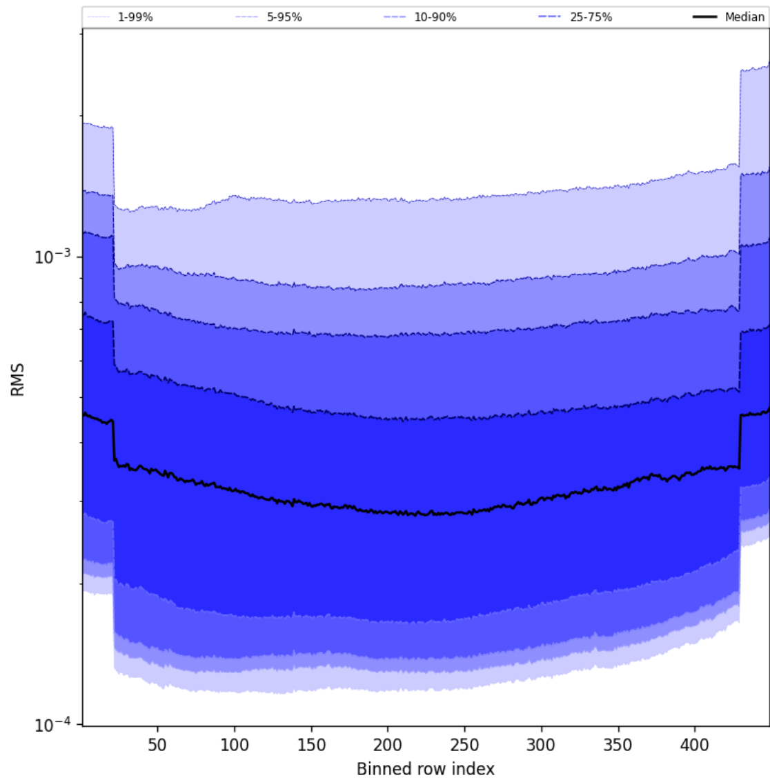
Figure 58: Along track statistics of “RMS” for 2025-09-18 to 2025-09-18
