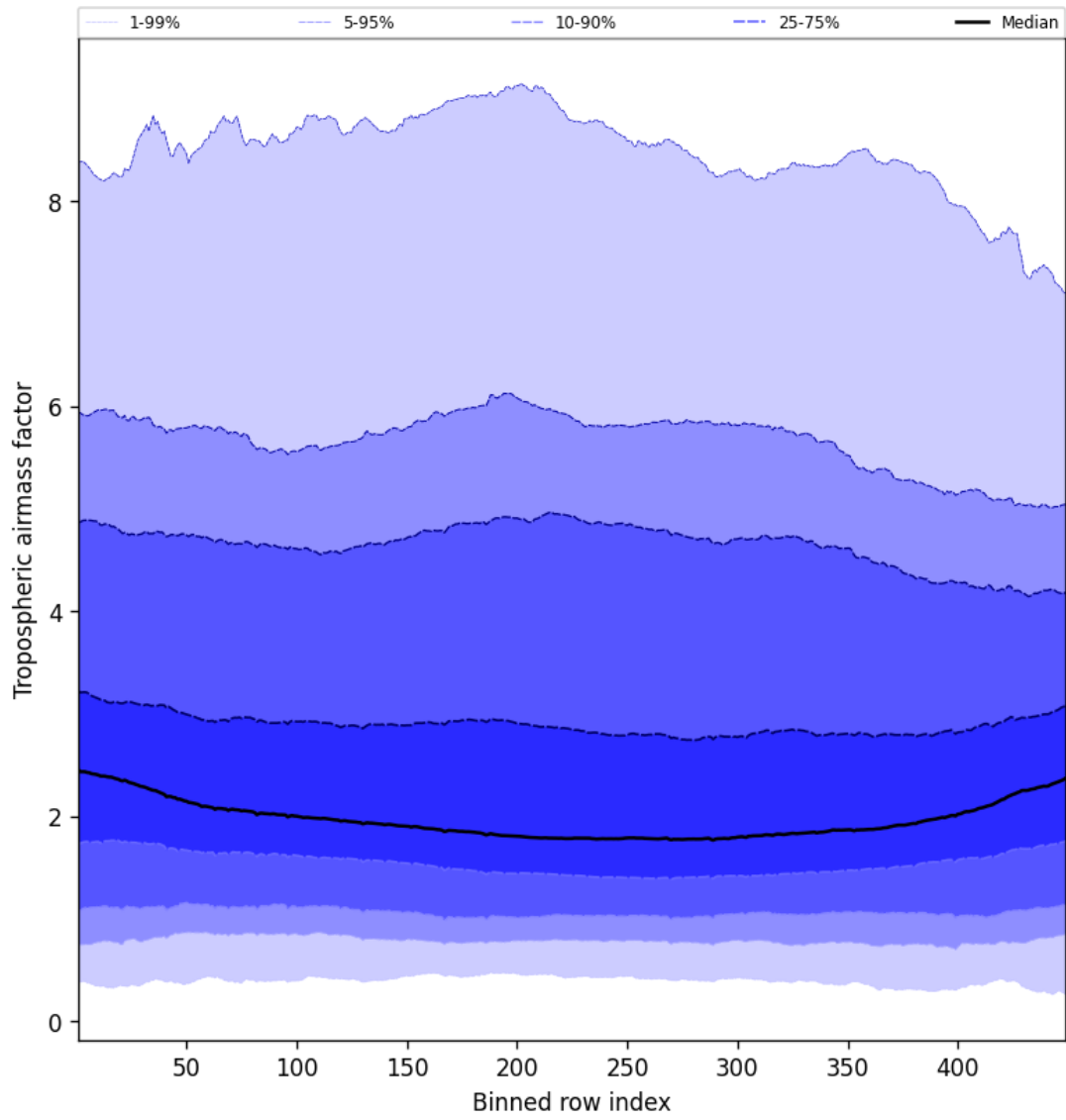
Figure 46: Along track statistics of “Tropospheric air mass factor” for 2025-09-18 to 2025-09-18
