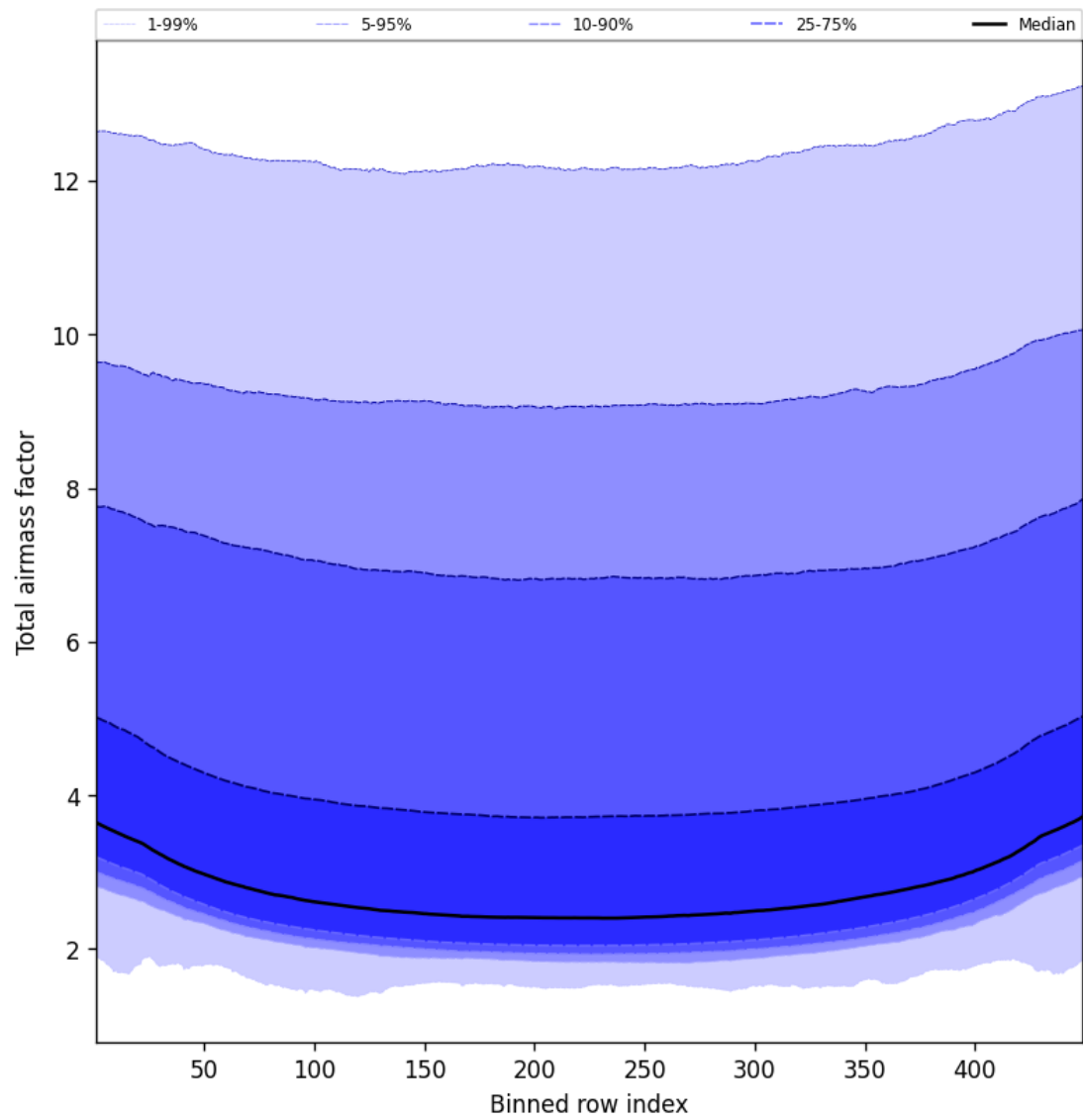
Figure 47: Along track statistics of “Total airmass factor” for 2025-09-18 to 2025-09-18
