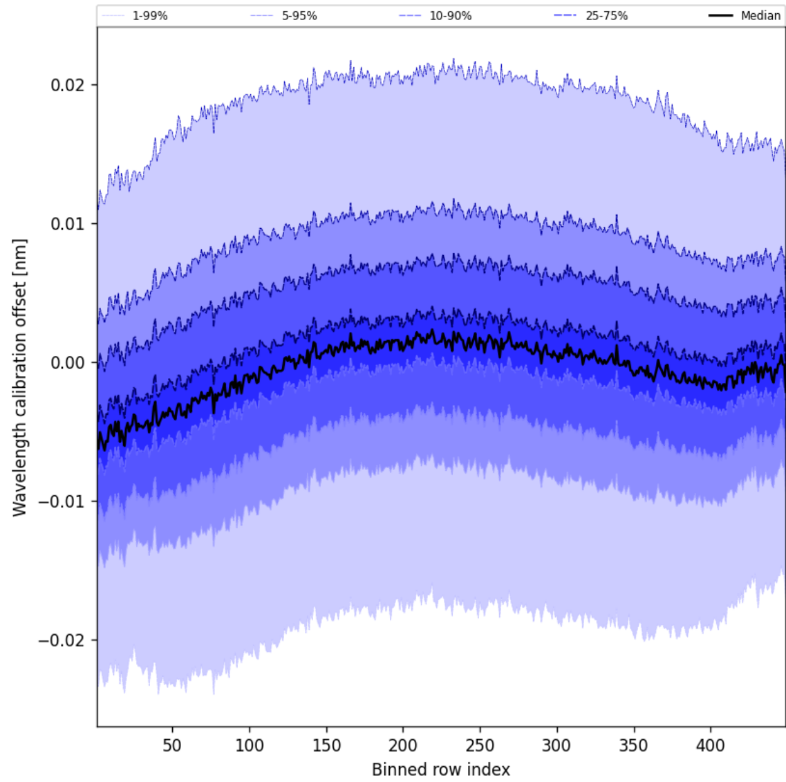
Figure 50: Along track statistics of “Wavelength calibration offset” for 2025-09-18 to 2025-09-18
