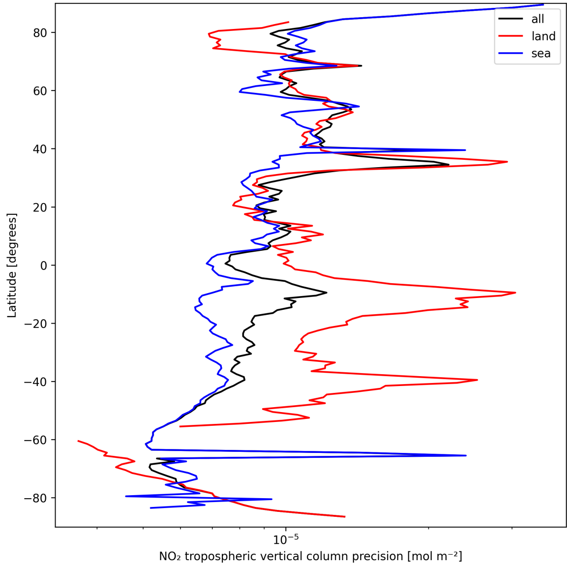
Figure 11: Zonal average of “NO 2 tropospheric vertical column precision” for 2025-09-18 to 2025-09-18.
