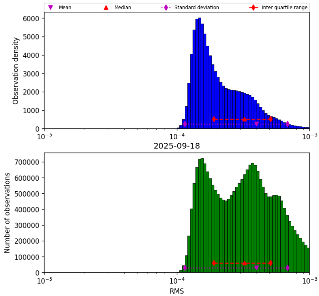
Figure 41: Histogram of “RMS” for 2025-09-18 to 2025-09-18
