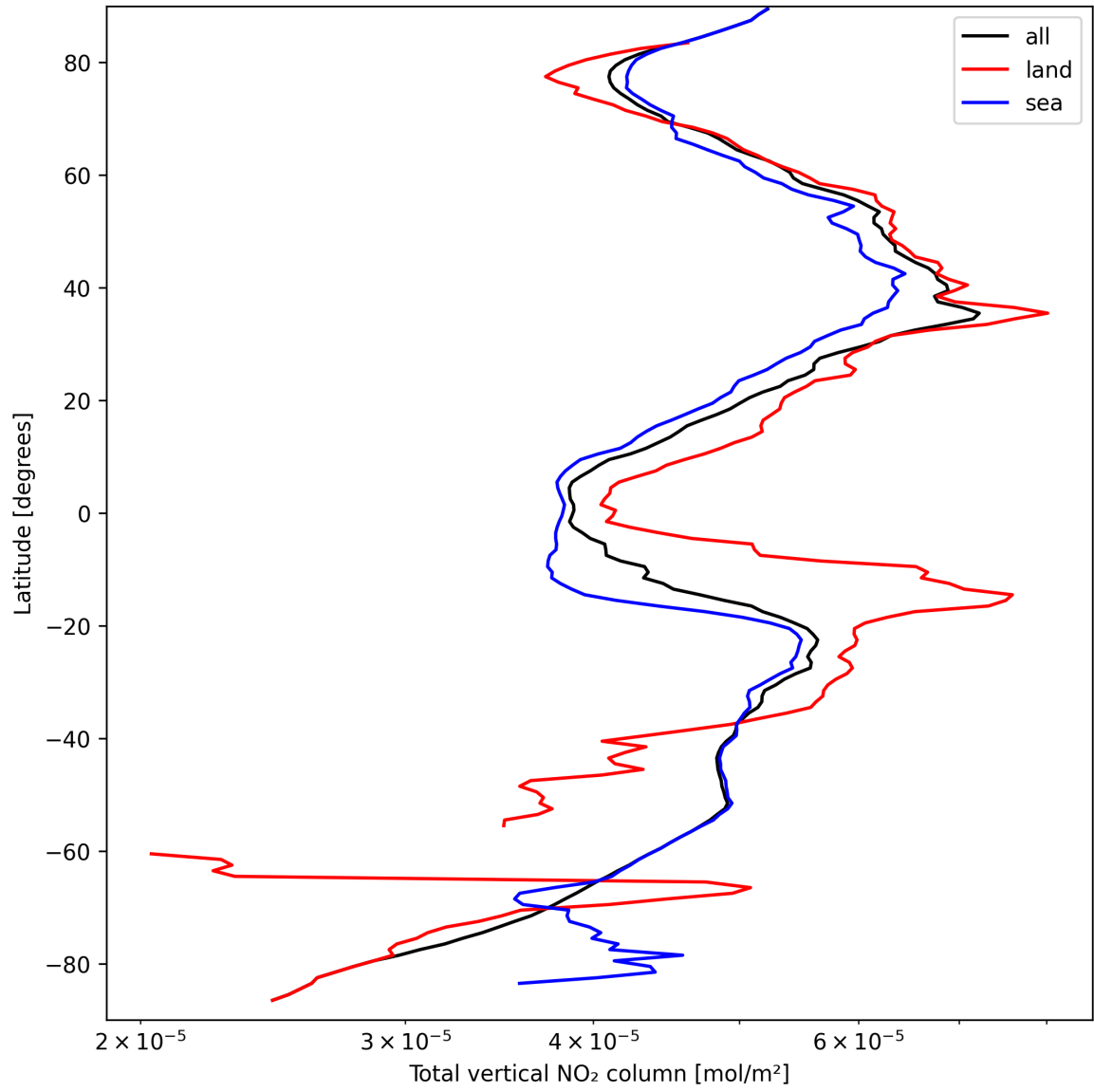
Figure 19: Zonal average of “Total vertical NO 2 column” for 2025-09-18 to 2025-09-18.
