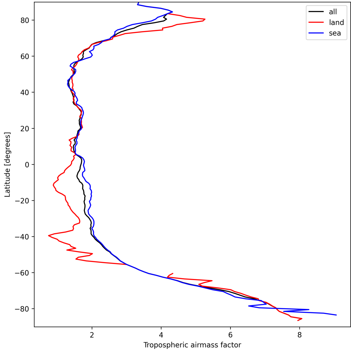
Figure 12: Zonal average of “Tropospheric airmass factor” for 2025-09-18 to 2025-09-18.
