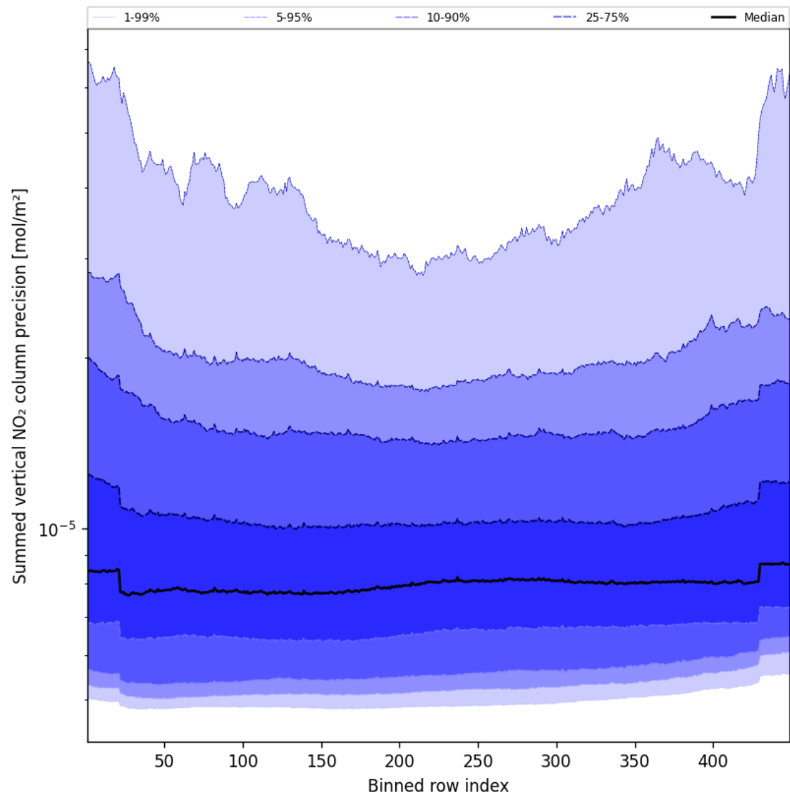
Figure 56: Along track statistics of “Summed vertical NO 2 column precision” for 2025-09-18 to 2025-09-18
