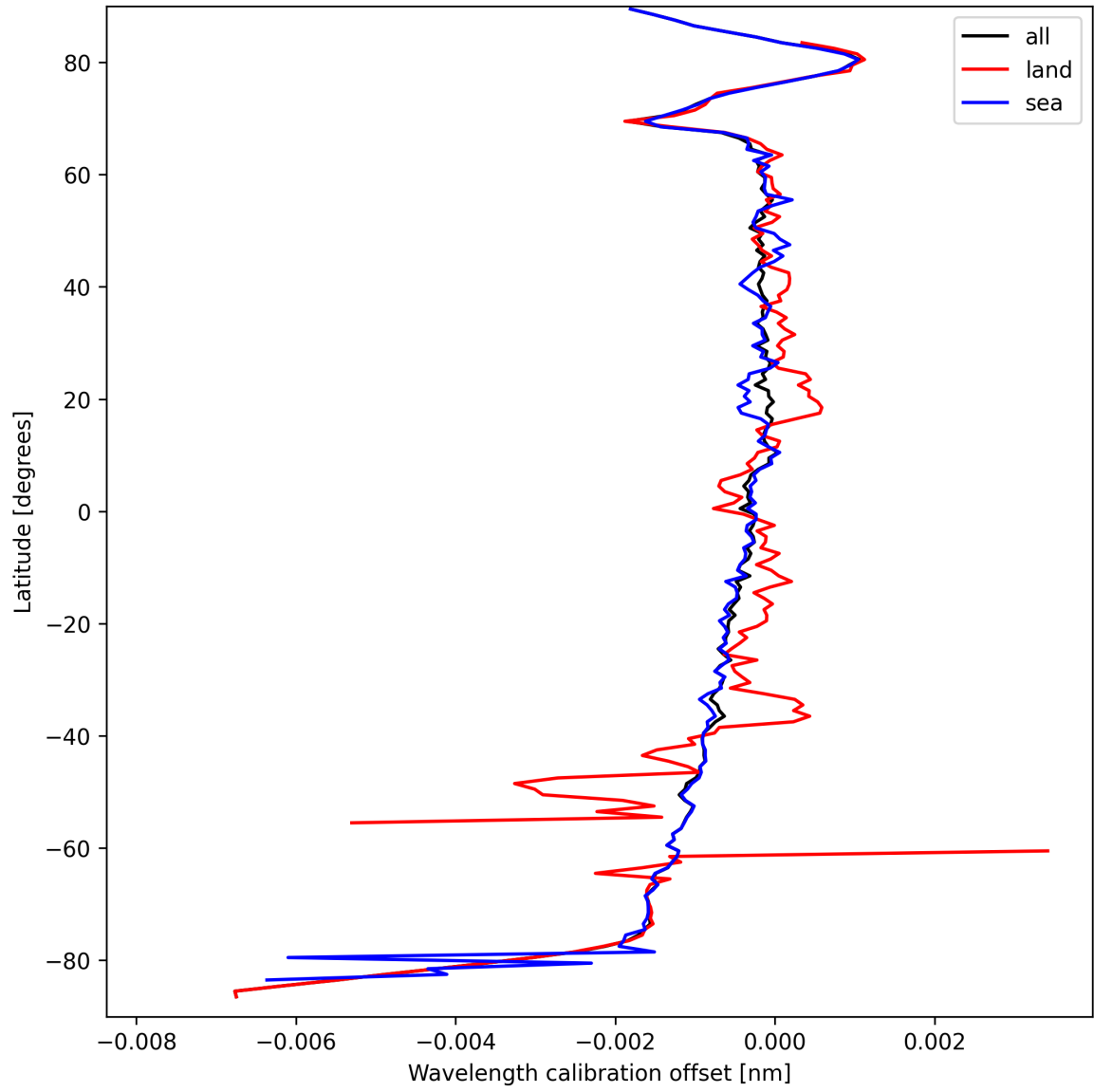
Figure 16: Zonal average of “Wavelength calibration offset” for 2025-09-18 to 2025-09-18.
