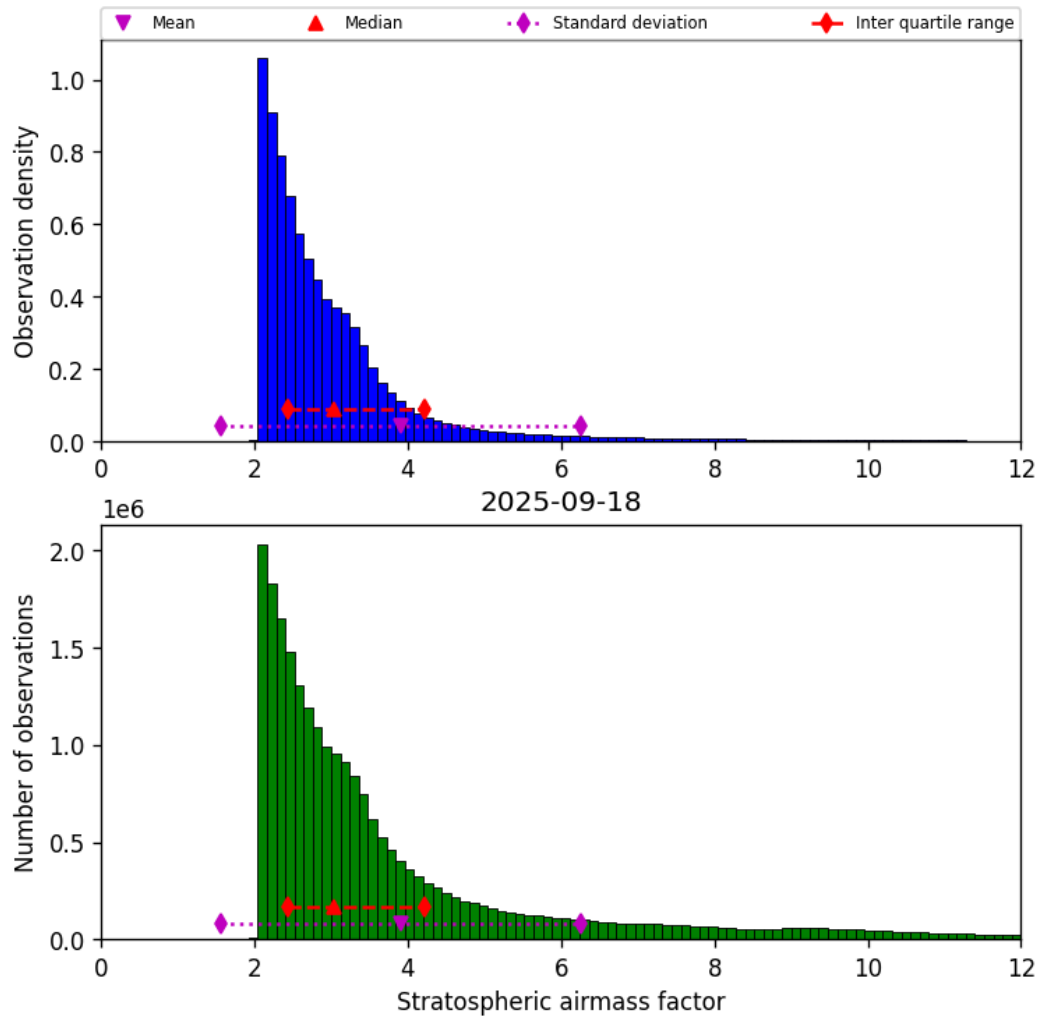
Figure 42: Histogram of “Stratospheric airmass factor” for 2025-09-18 to 2025-09-18
