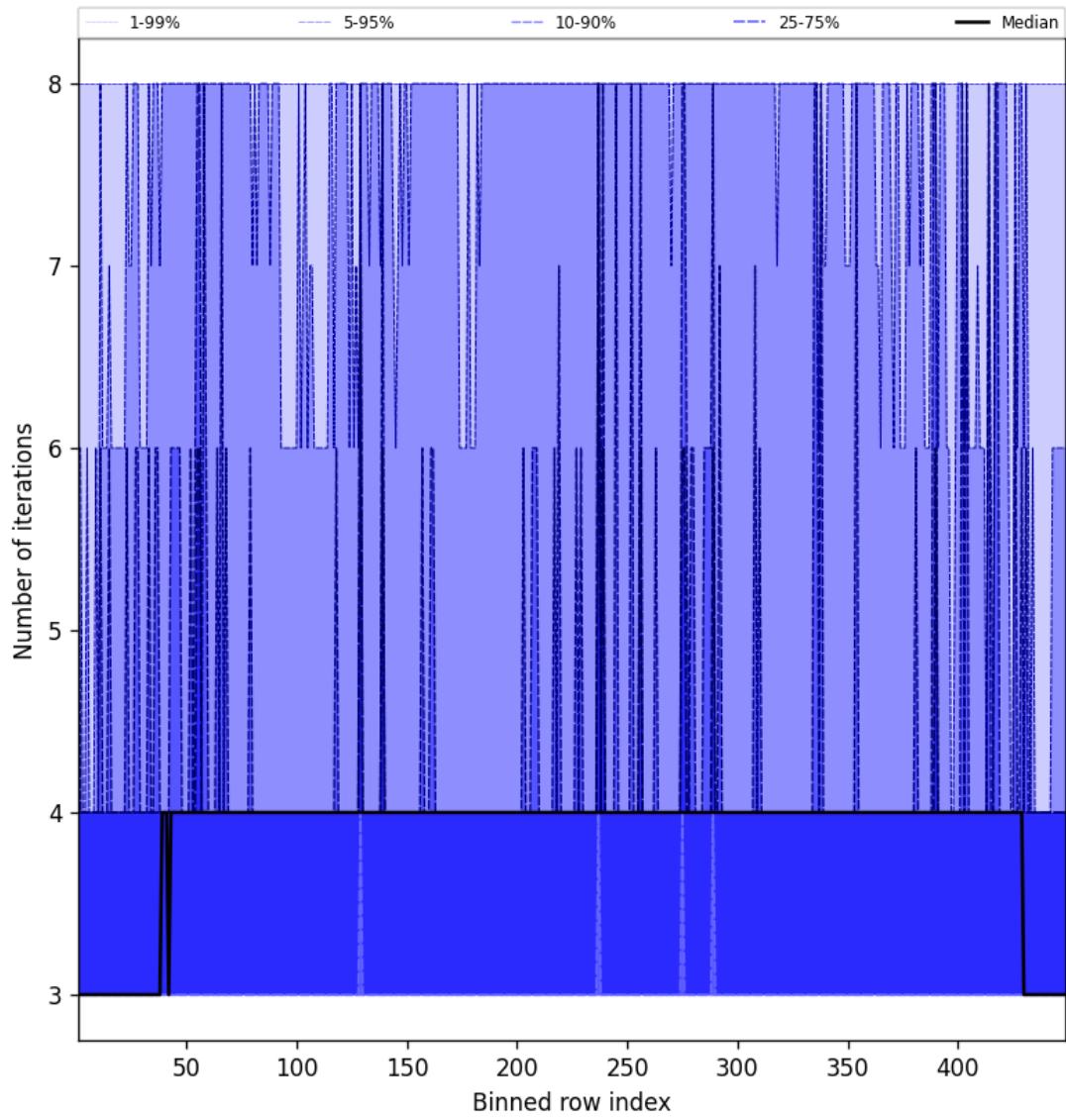
Figure 49: Along track statistics of "Number of iterations" for 2025-09-18 to 2025-09-18
