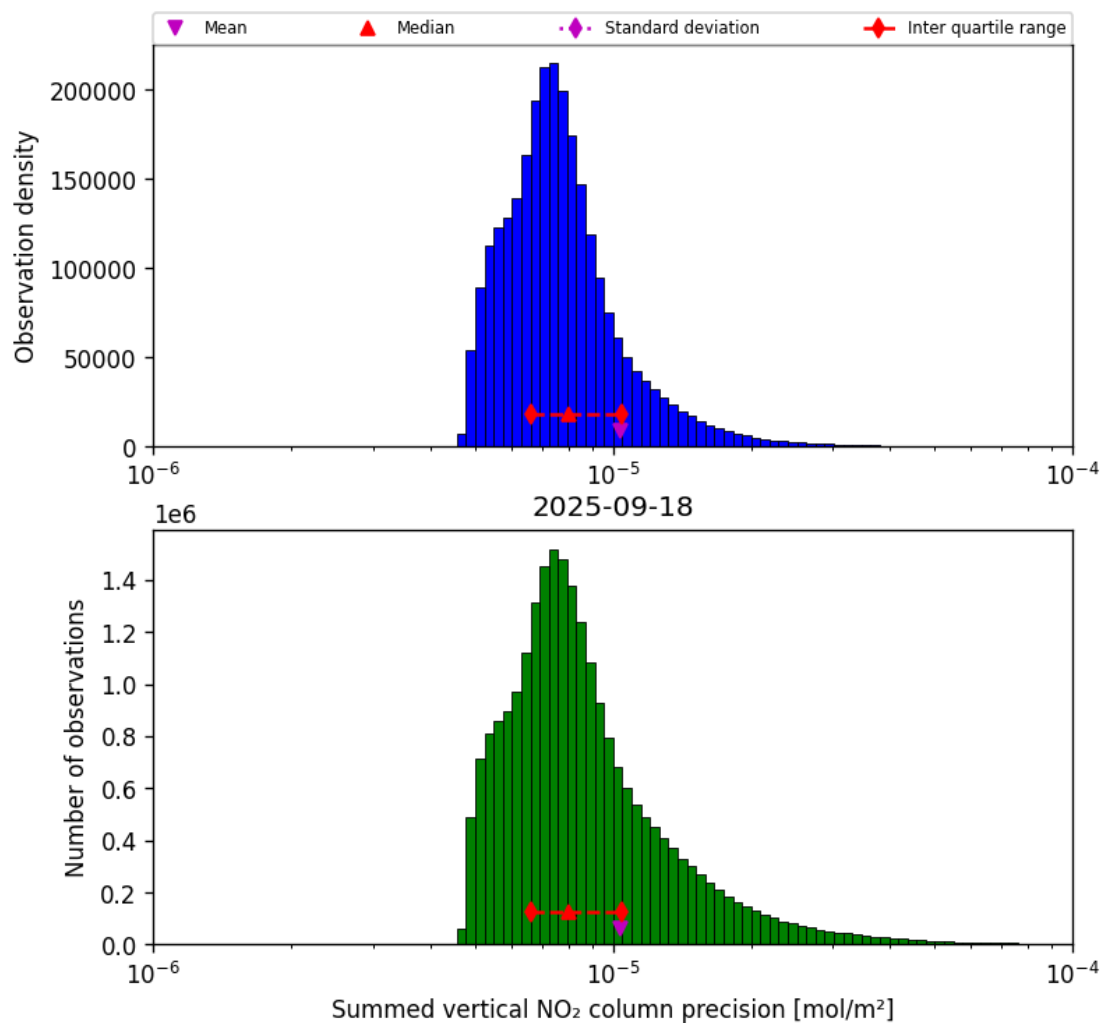
Figure 39: Histogram of "Summed vertical NO 2 column precision" for 2025-09-18 to 2025-09-18
