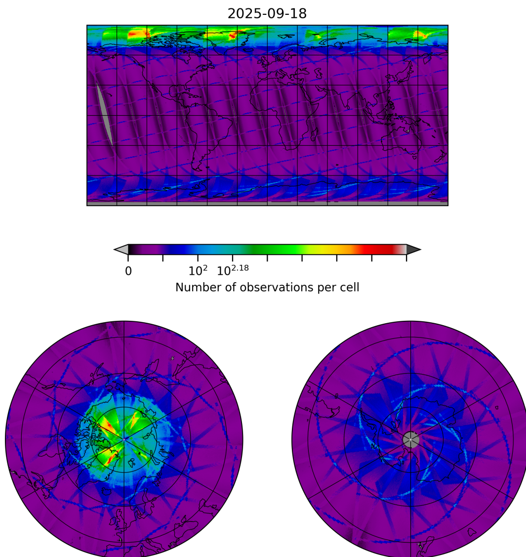
Figure 8: Map of the number of observations for 2025-09-18 to 2025-09-18
