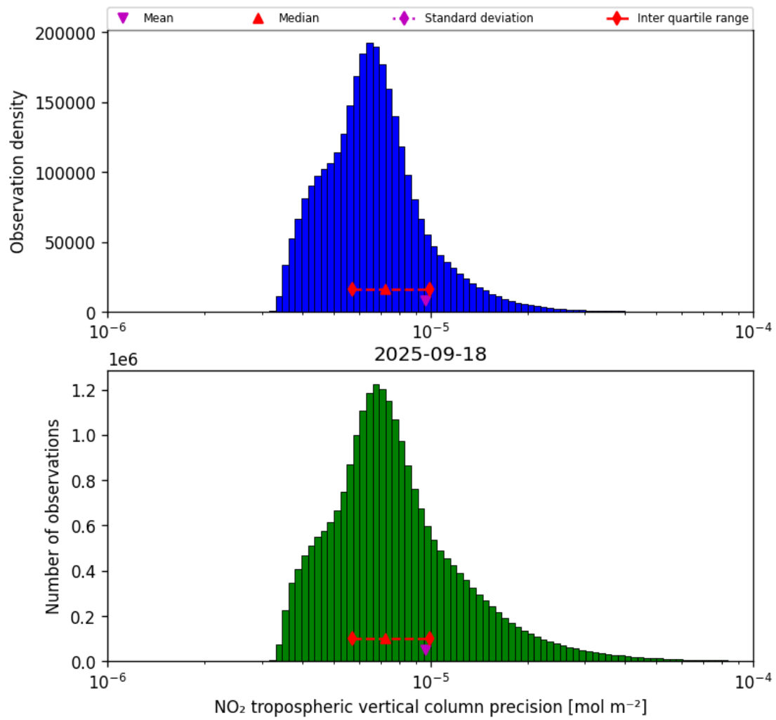
Figure 28: Histogram of “NO 2 tropospheric vertical column precision” for 2025-09-18 to 2025-09-18
