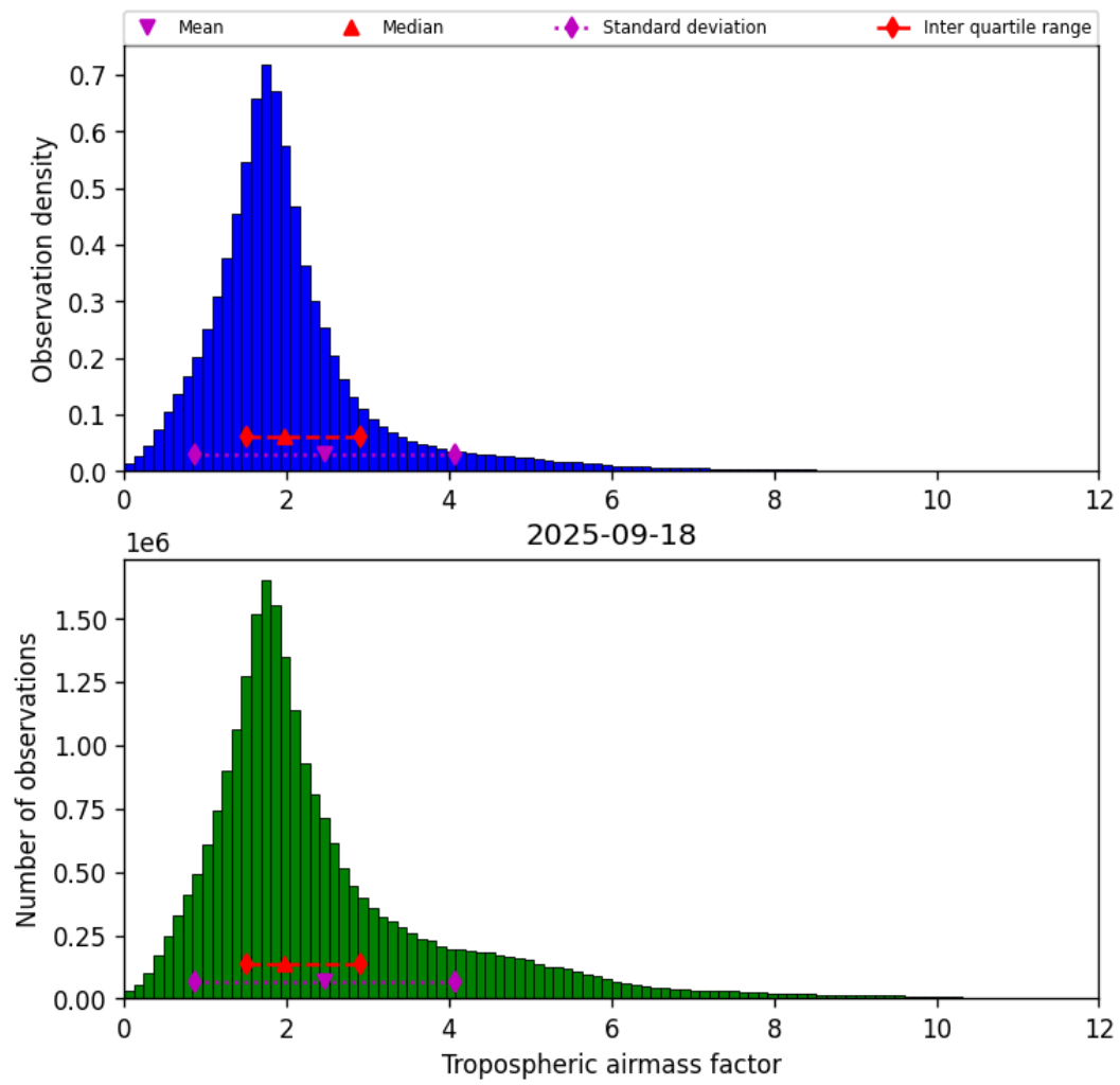
Figure 29: Histogram of “Tropospheric airmass factor” for 2025-09-18 to 2025-09-18
