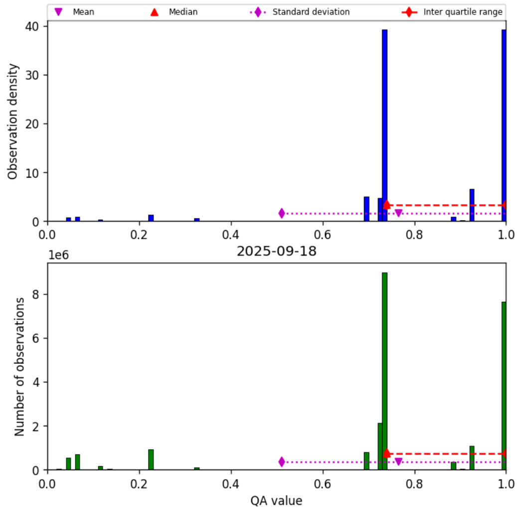
Figure 26: Histogram of “QA value” for 2025-09-18 to 2025-09-18
