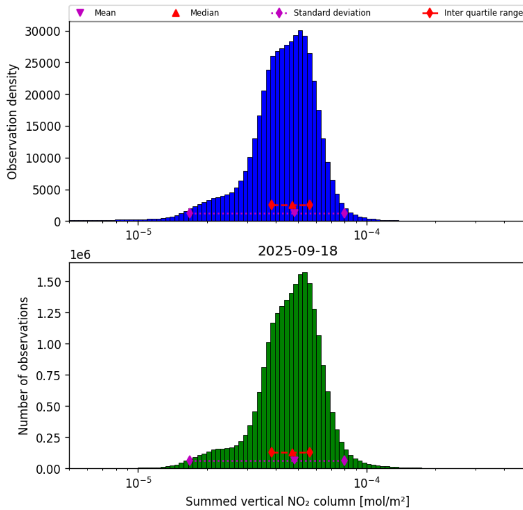
Figure 38: Histogram of “Summed vertical NO 2 column” for 2025-09-18 to 2025-09-18
