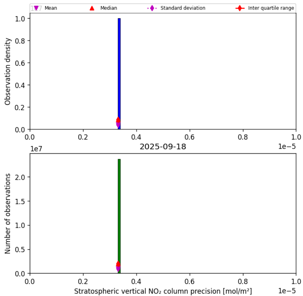
Figure 35: Histogram of “Stratospheric vertical NO 2 column precision” for 2025-09-18 to 2025-09-18
