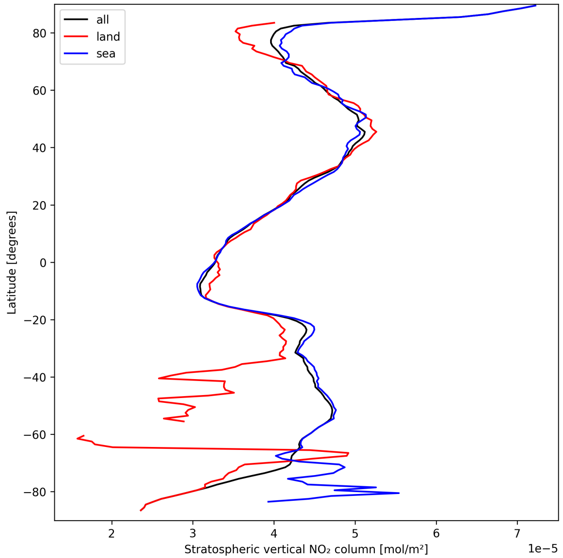
Figure 17: Zonal average of “Stratospheric vertical NO 2 column” for 2025-09-18 to 2025-09-18.
