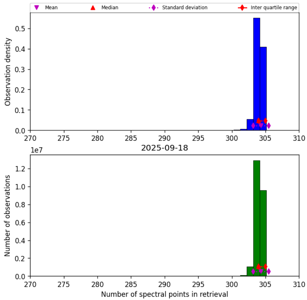
Figure 31: Histogram of “Number of spectral points in retrieval” for 2025-09-18 to 2025-09-18
