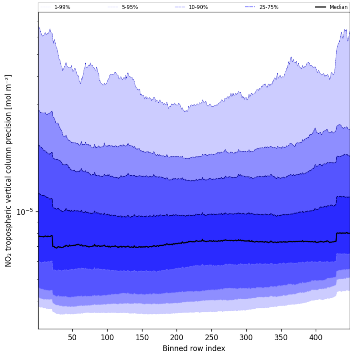
Figure 45: Along track statistics of “NO 2 tropospheric vertical column precision” for 2025-09-18 to 2025-09-18
