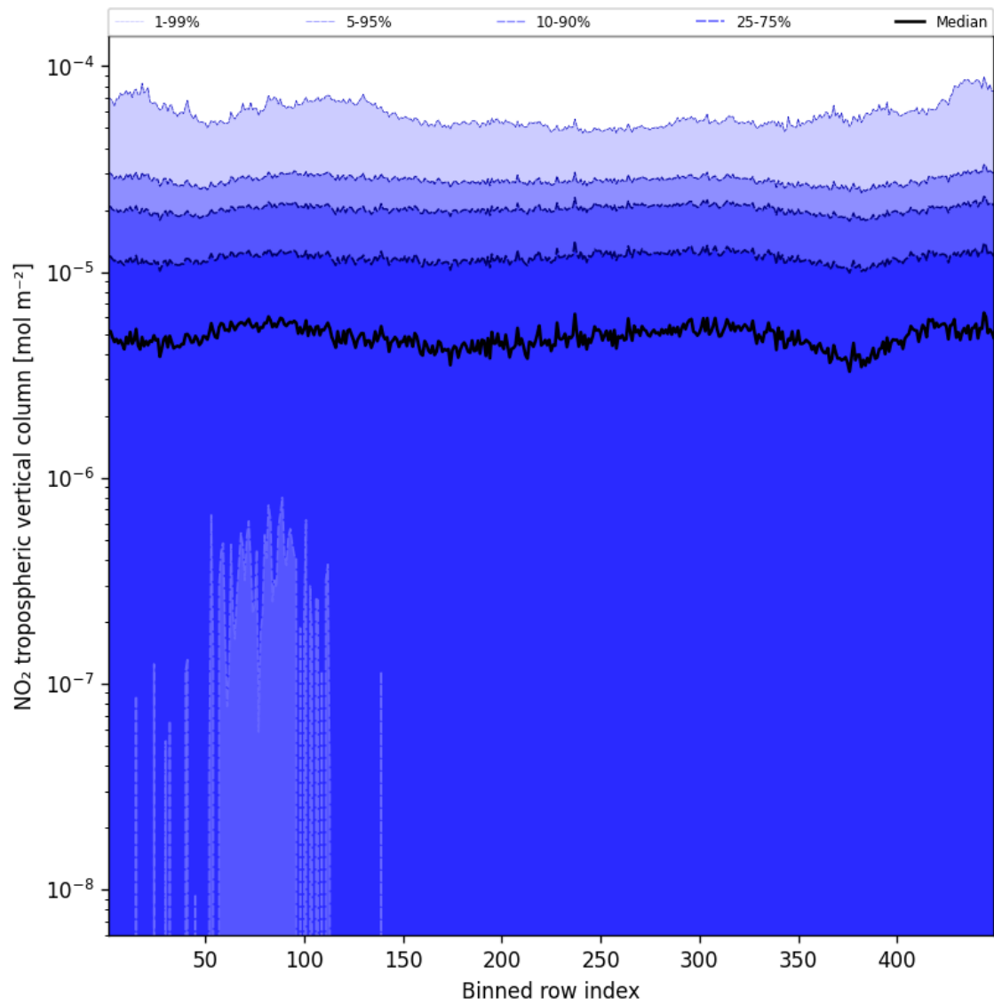
Figure 44: Along track statistics of “NO 2 tropospheric vertical column” for 2025-09-18 to 2025-09-18
