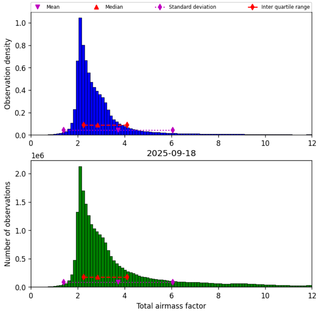
Figure 30: Histogram of “Total airmass factor” for 2025-09-18 to 2025-09-18
