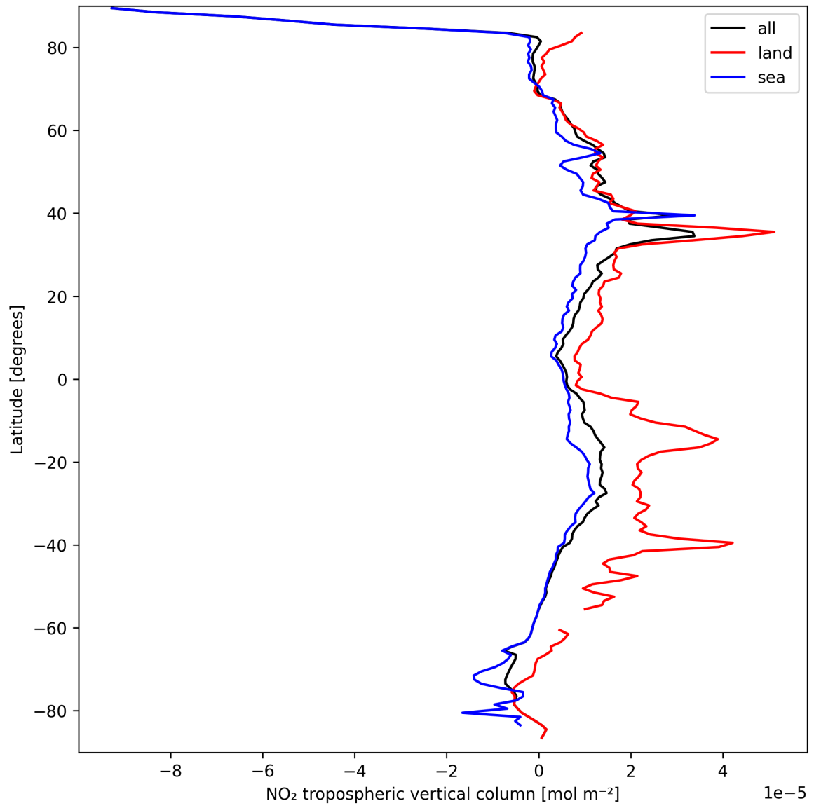
Figure 10: Zonal average of “NO 2 tropospheric vertical column” for 2025-09-18 to 2025-09-18.
