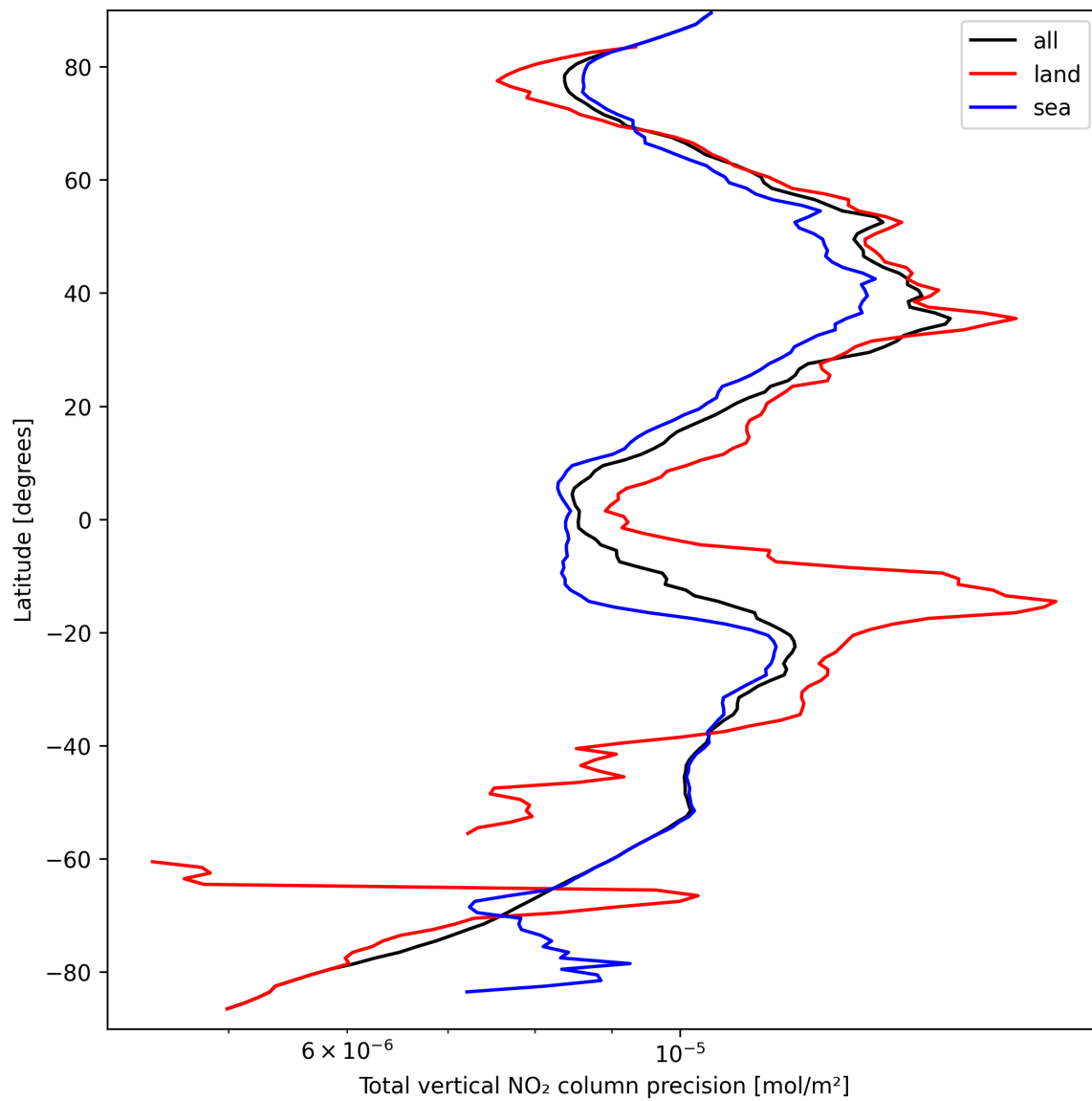
Figure 20: Zonal average of “Total vertical NO 2 column precision” for 2025-09-18 to 2025-09-18.
