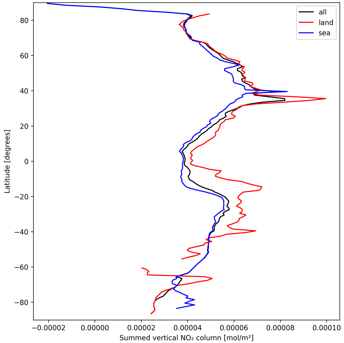
Figure 21: Zonal average of “Summed vertical NO 2 column” for 2025-09-18 to 2025-09-18.
