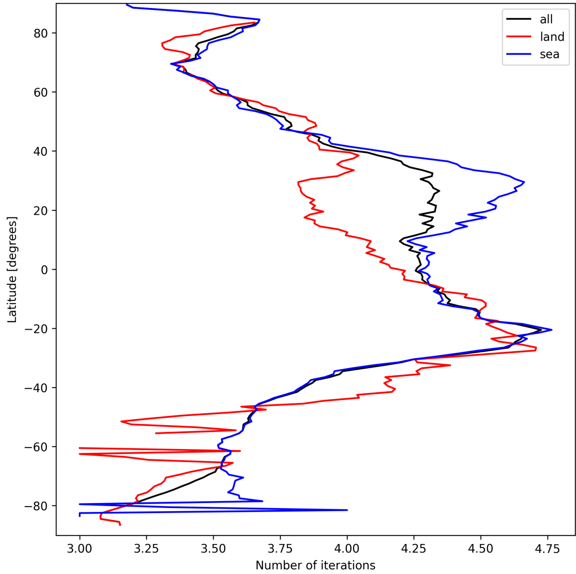
Figure 15: Zonal average of “Number of iterations” for 2025-09-18 to 2025-09-18.
