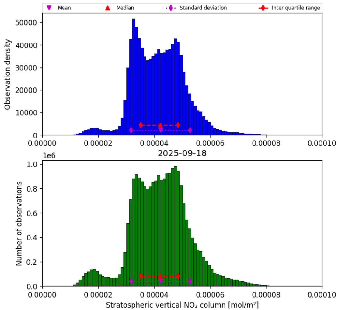
Figure 34: Histogram of “Stratospheric vertical NO 2 column” for 2025-09-18 to 2025-09-18
