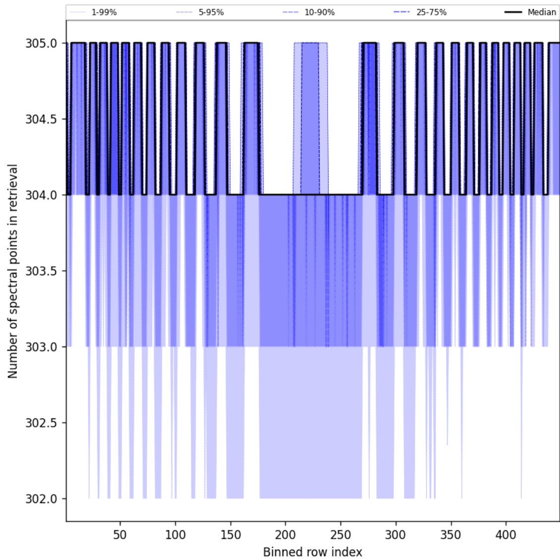
Figure 48: Along track statistics of “Number of spectral points in retrieval” for 2025-09-18 to 2025-09-18
