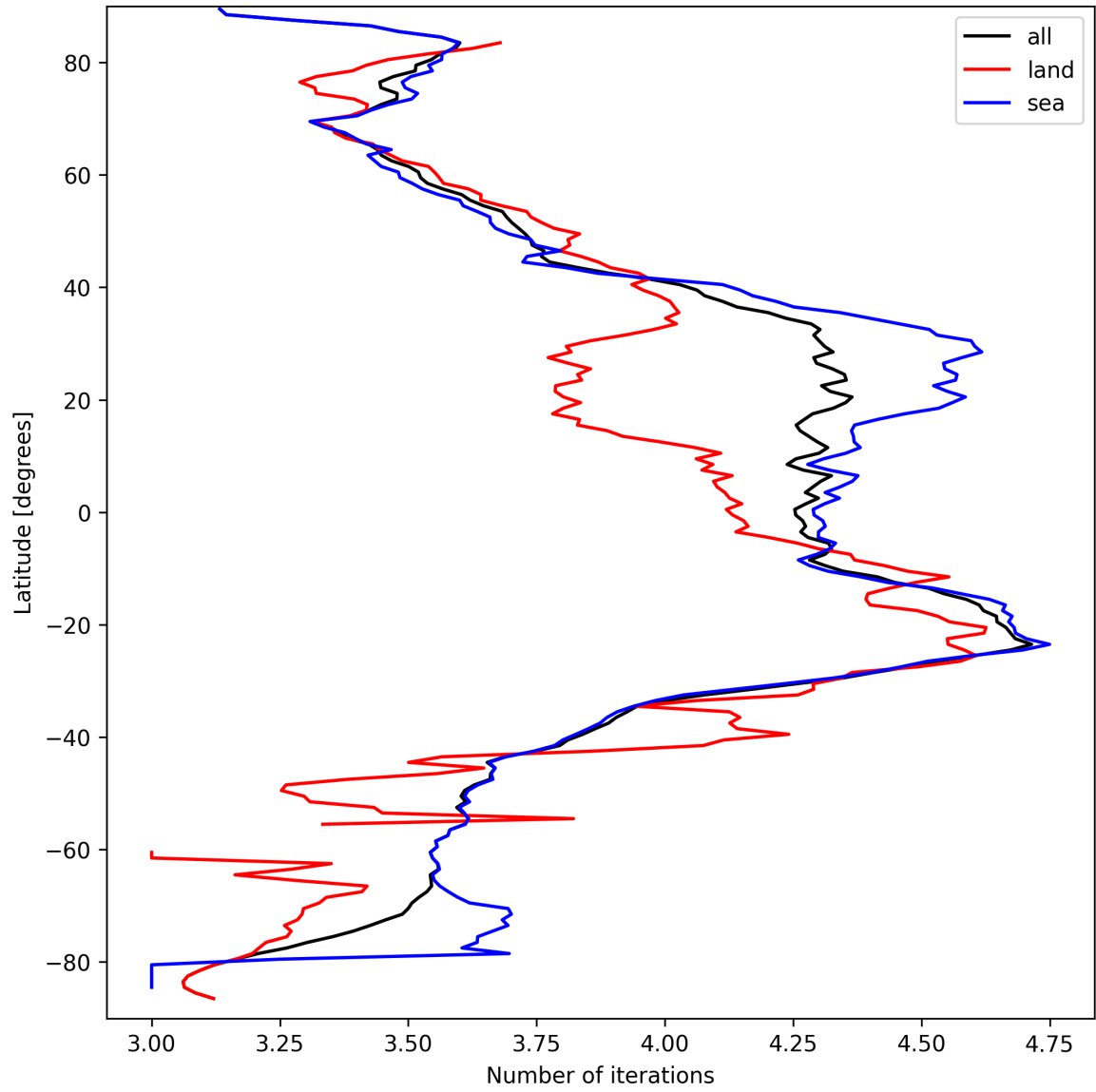
Figure 15: Zonal average of “Number of iterations” for 2025-09-19 to 2025-09-20.
