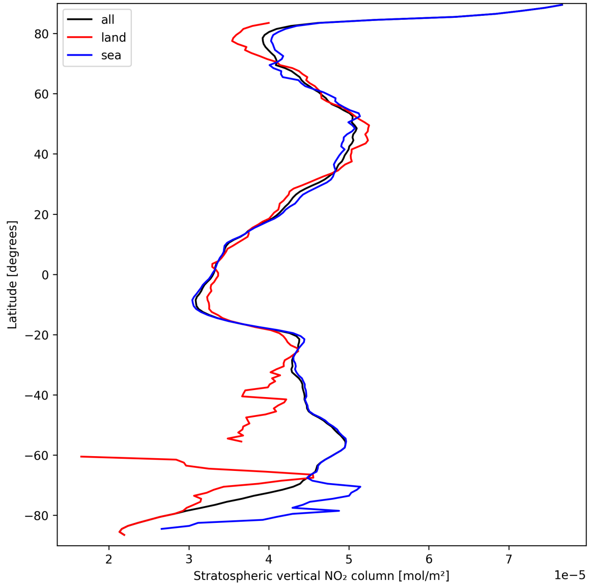
Figure 17: Zonal average of “Stratospheric vertical NO 2 column” for 2025-09-19 to 2025-09-20.
