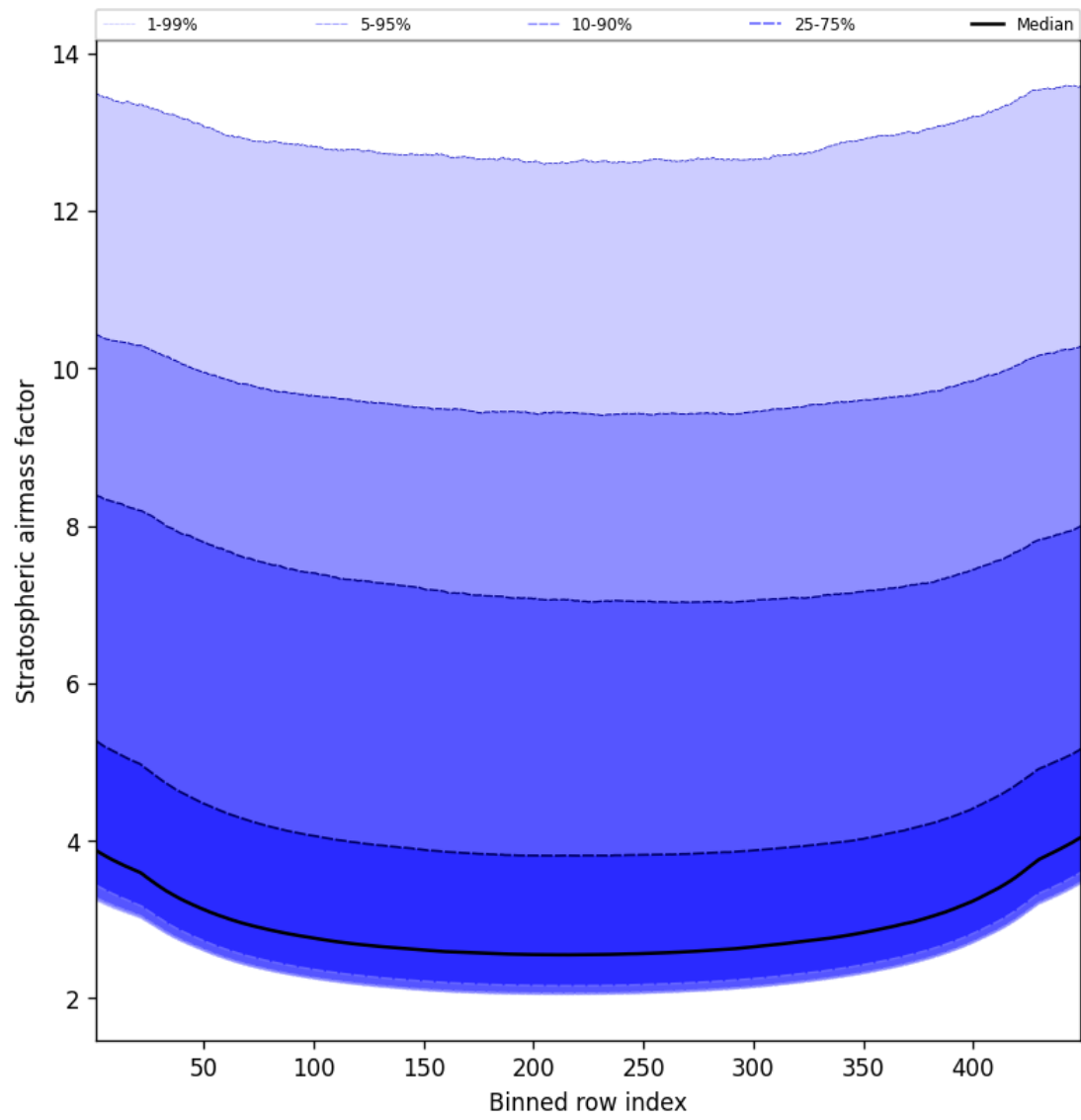
Figure 59: Along track statistics of “Stratospheric airmass factor” for 2025-09-19 to 2025-09-20
