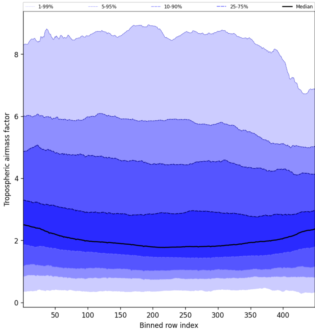
Figure 46: Along track statistics of “Tropospheric airmass factor” for 2025-09-19 to 2025-09-20
