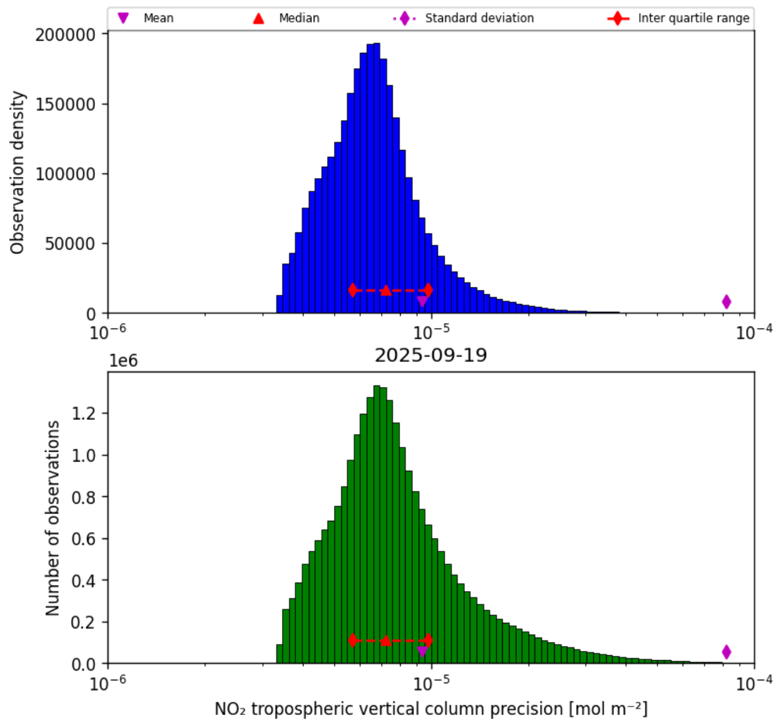
Figure 28: Histogram of “NO 2 tropospheric vertical column precision” for 2025-09-19 to 2025-09-20
