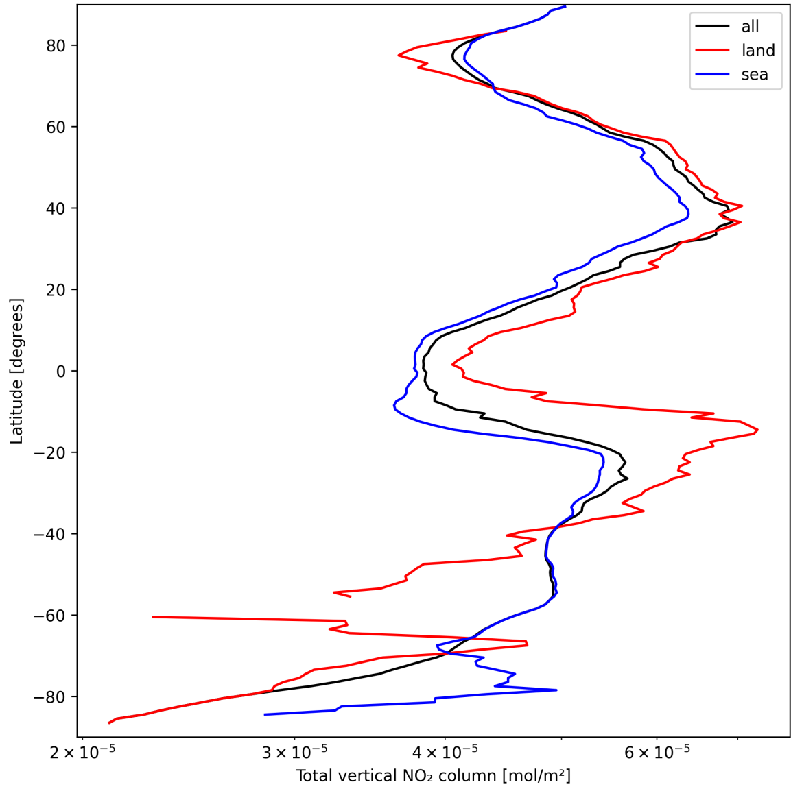
Figure 19: Zonal average of “Total vertical NO 2 column” for 2025-09-19 to 2025-09-20.
