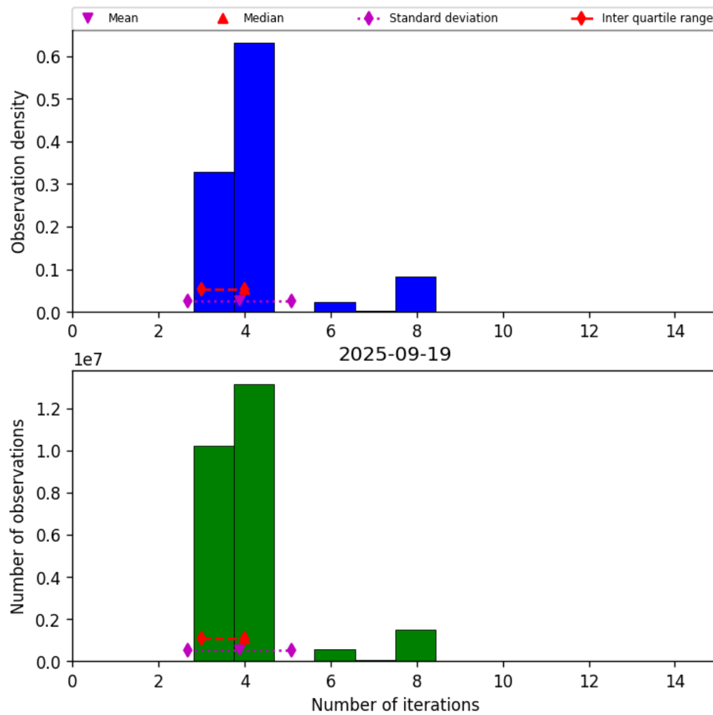
Figure 32: Histogram of “Number of iterations” for 2025-09-19 to 2025-09-20
