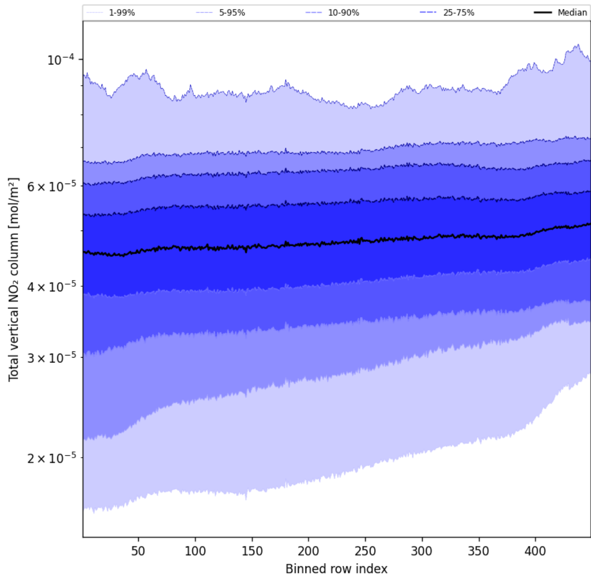
Figure 53: Along track statistics of “Total vertical NO 2 column” for 2025-09-19 to 2025-09-20
