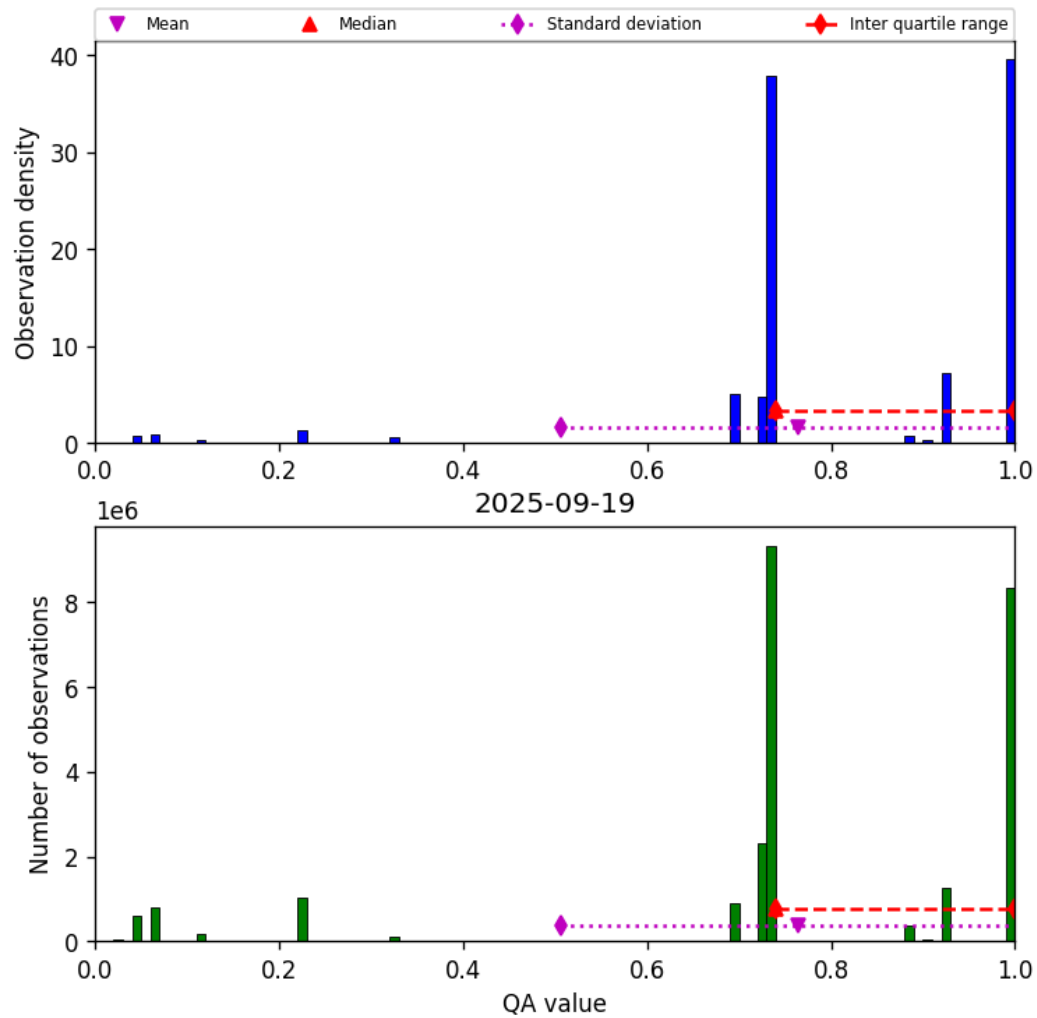
Figure 26: Histogram of “QA value” for 2025-09-19 to 2025-09-20
