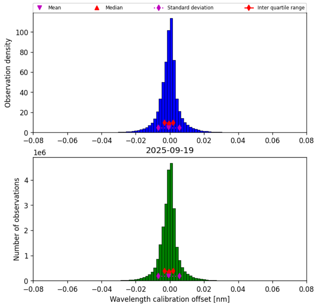
Figure 33: Histogram of “Wavelength calibration offset” for 2025-09-19 to 2025-09-20
