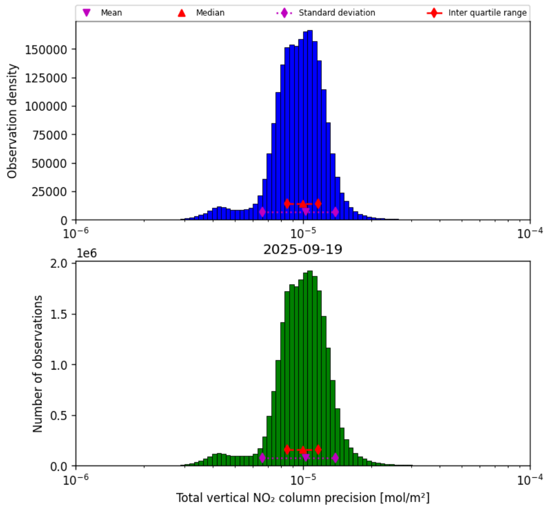
Figure 37: Histogram of “Total vertical NO 2 column precision” for 2025-09-19 to 2025-09-20
