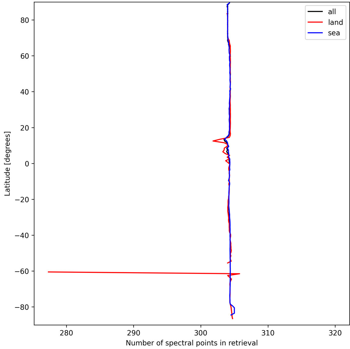
Figure 14: Zonal average of “Number of spectral points in retrieval” for 2025-09-19 to 2025-09-20.
