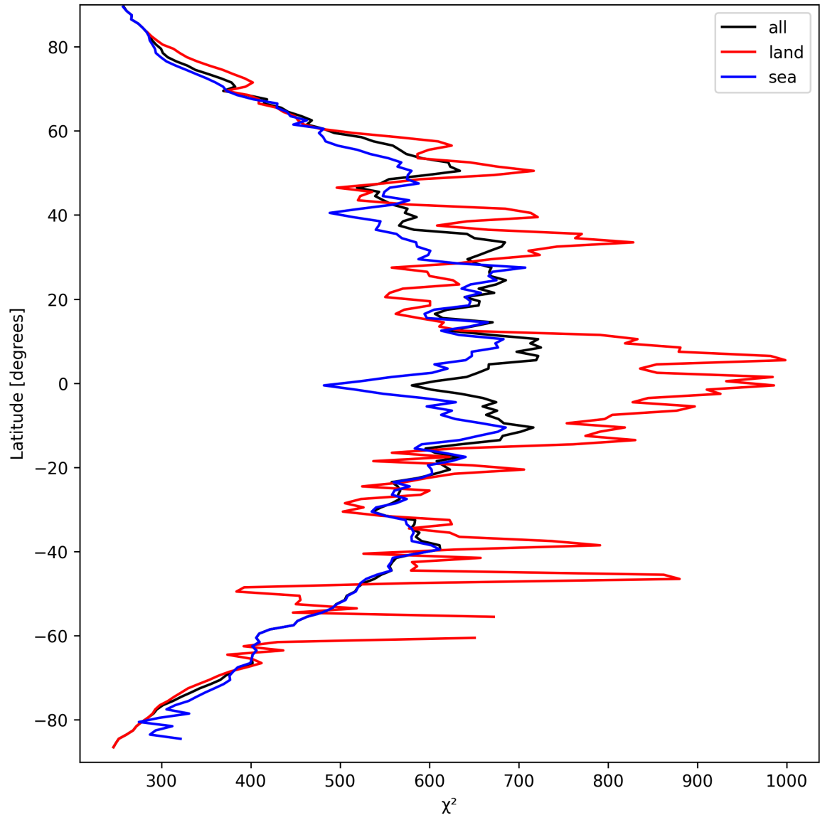
Figure 23: Zonal average of “ \chi^2 ” for 2025-09-19 to 2025-09-20.
