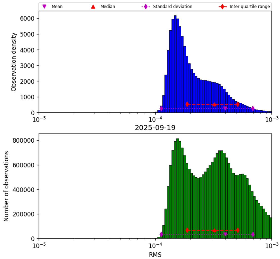
Figure 41: Histogram of “RMS” for 2025-09-19 to 2025-09-20
