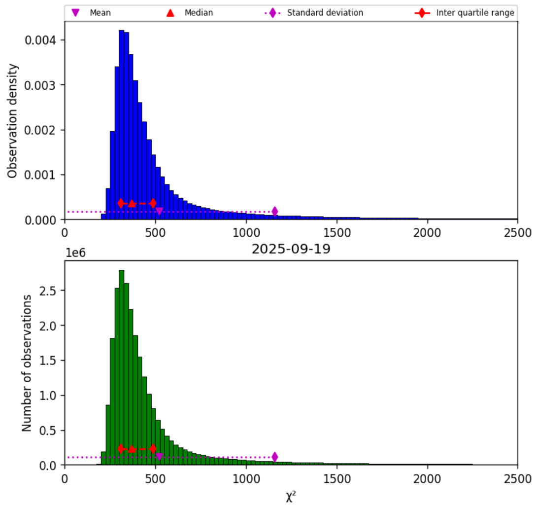
Figure 40: Histogram of “ \chi^2 ” for 2025-09-19 to 2025-09-20
