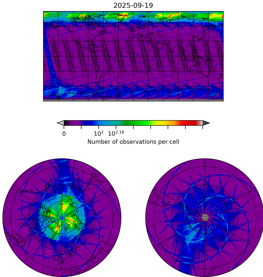
Figure 8: Map of the number of observations for 2025-09-19 to 2025-09-20
