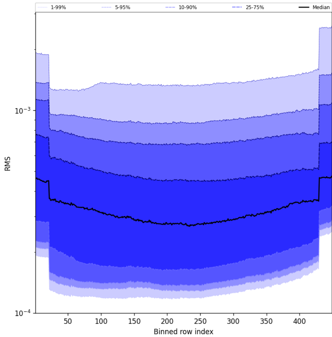
Figure 58: Along track statistics of “RMS” for 2025-09-19 to 2025-09-20
