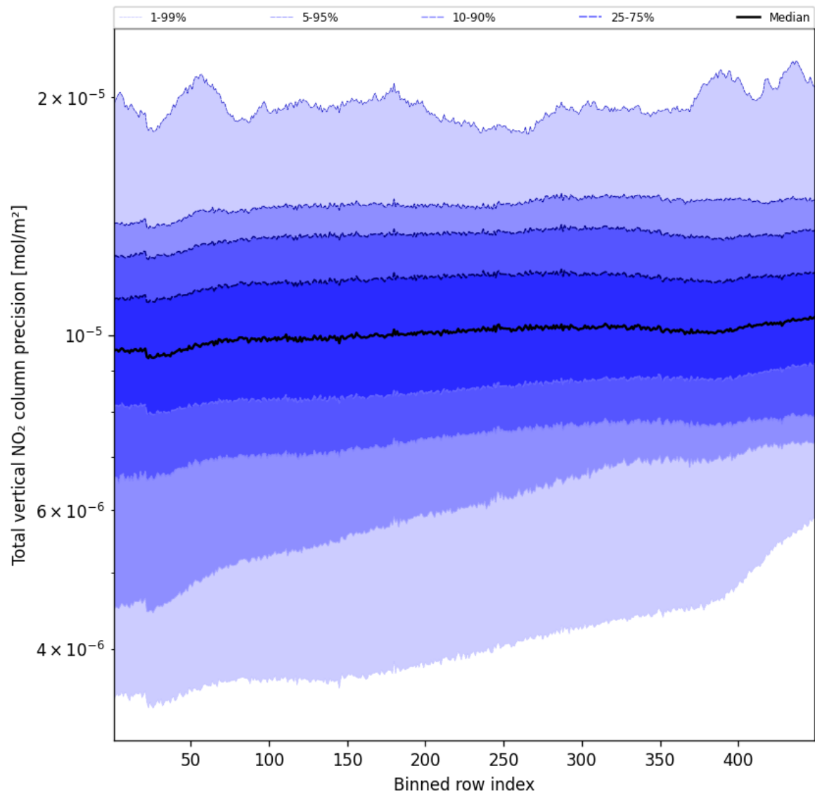
Figure 54: Along track statistics of "Total vertical NO 2 column precision" for 2025-09-19 to 2025-09-20
