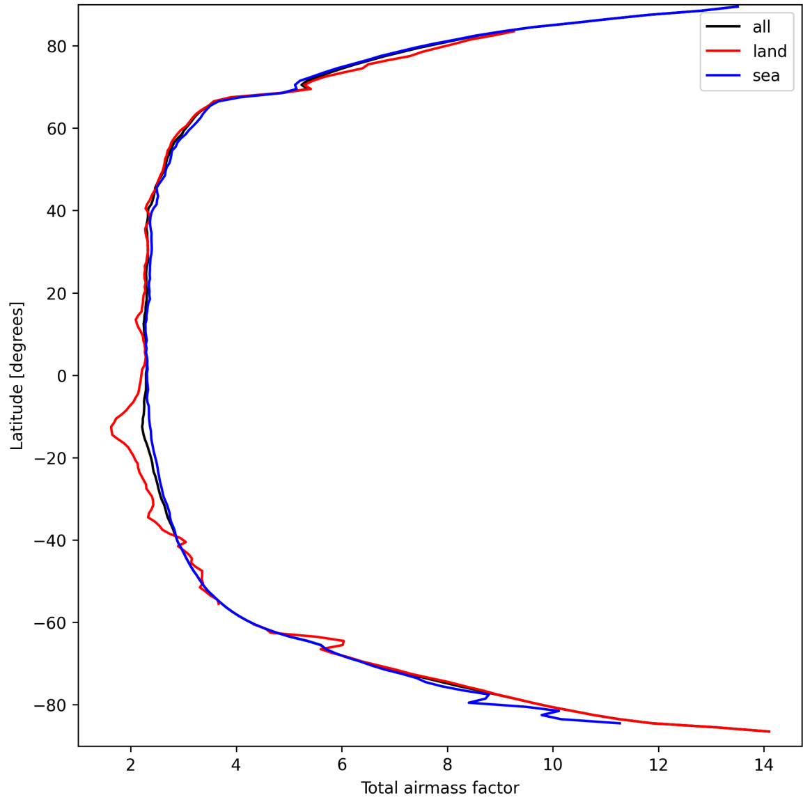
Figure 13: Zonal average of “Total airmass factor” for 2025-09-19 to 2025-09-20.
