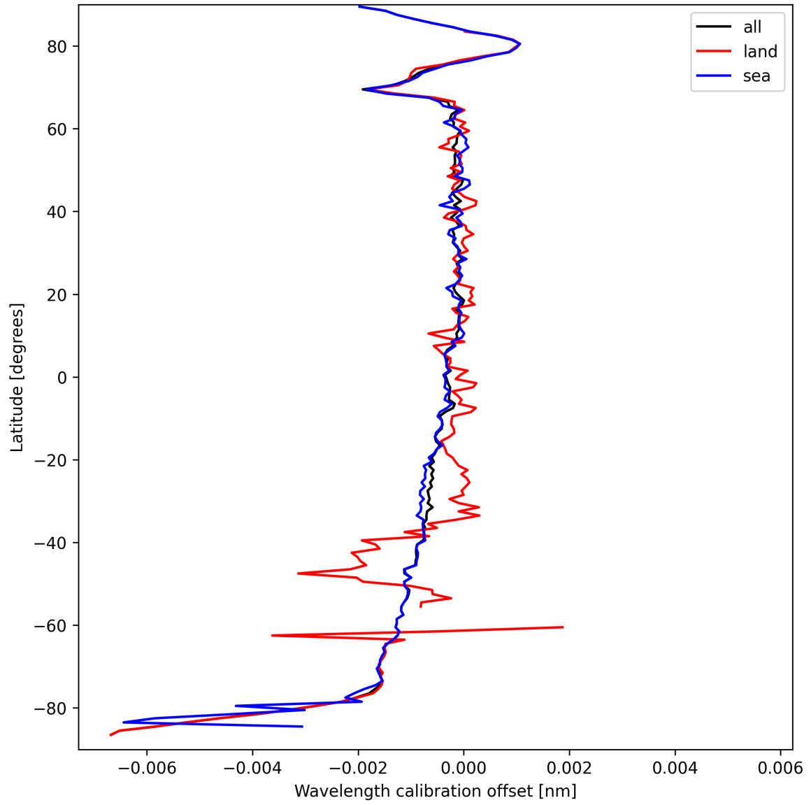
Figure 16: Zonal average of “Wavelength calibration offset” for 2025-09-19 to 2025-09-20.
