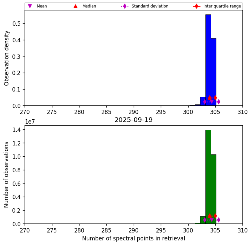
Figure 31: Histogram of “Number of spectral points in retrieval” for 2025-09-19 to 2025-09-20
