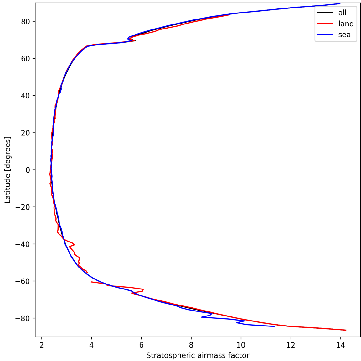
Figure 25: Zonal average of “Stratospheric airmass factor” for 2025-09-19 to 2025-09-20.
