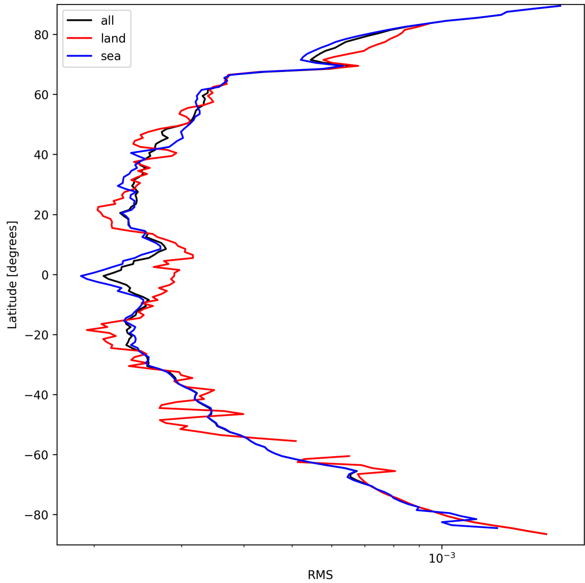
Figure 24: Zonal average of “RMS” for 2025-09-19 to 2025-09-20.
