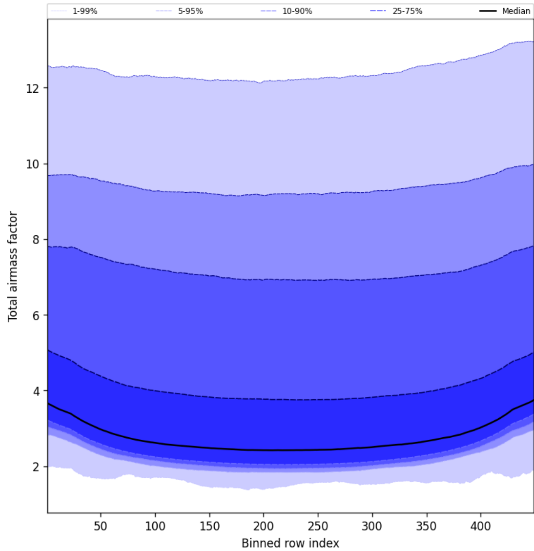
Figure 47: Along track statistics of “Total airmass factor” for 2025-09-19 to 2025-09-20
