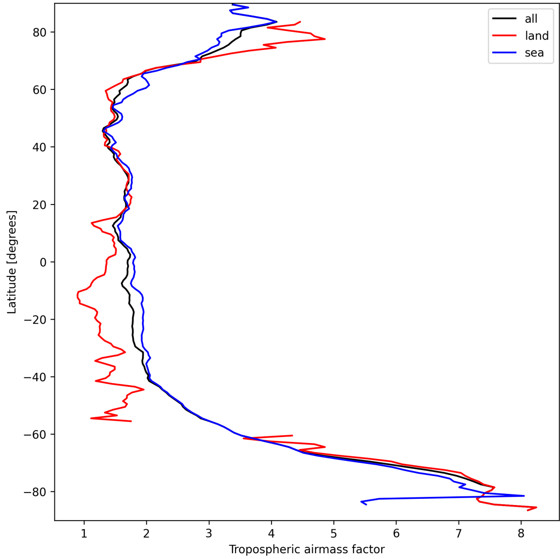
Figure 12: Zonal average of “Tropospheric airmass factor” for 2025-09-19 to 2025-09-20.
