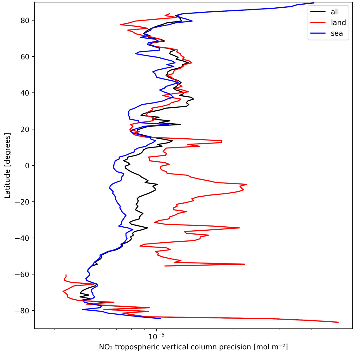
Figure 11: Zonal average of “NO 2 tropospheric vertical column precision” for 2025-09-19 to 2025-09-20.
