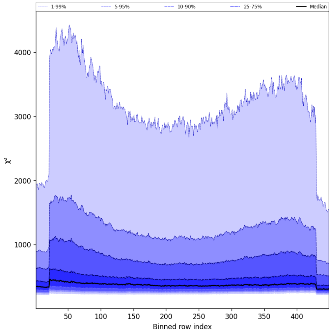
Figure 57: Along track statistics of “ \chi^2 ” for 2025-09-19 to 2025-09-20
