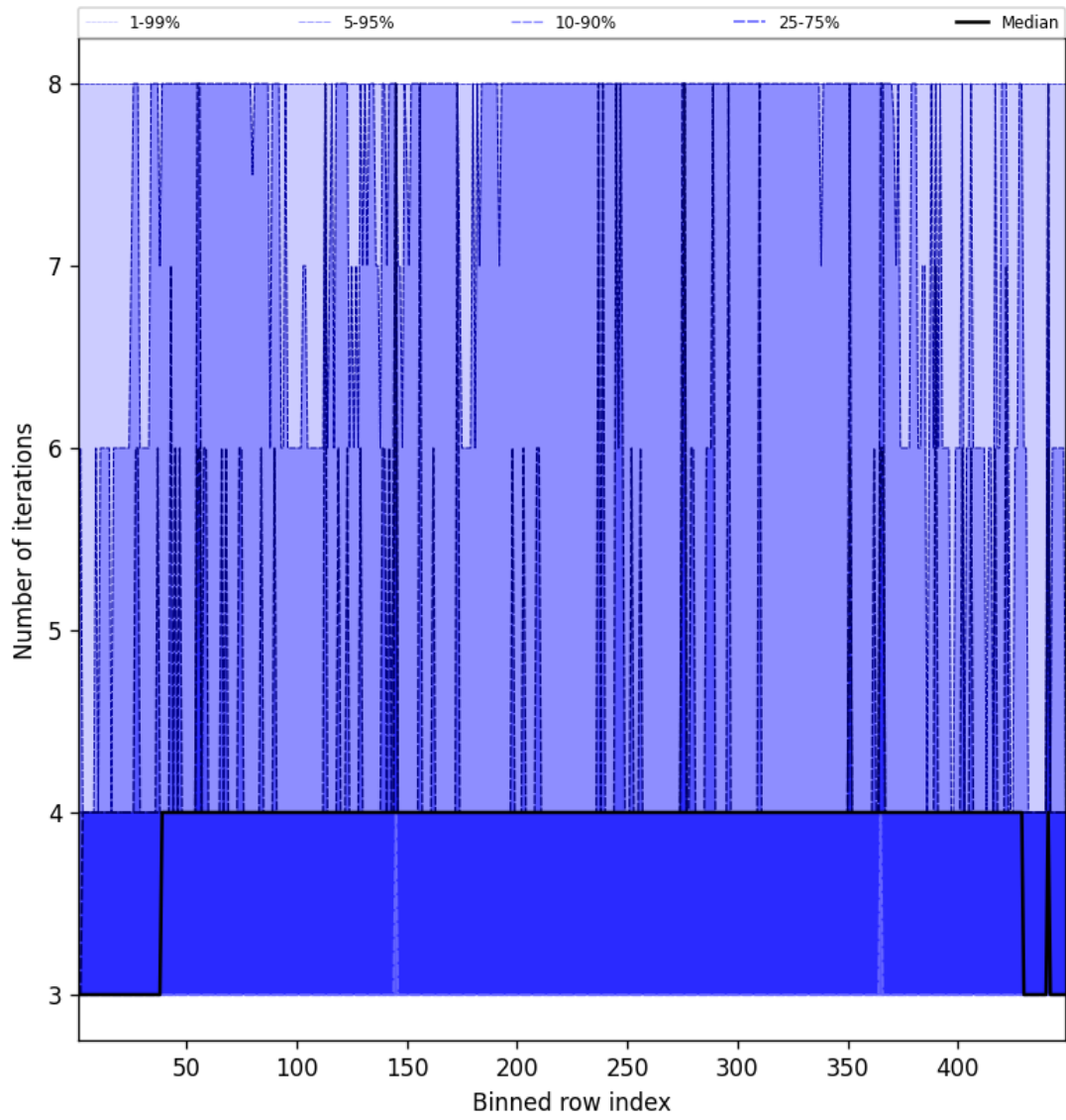
Figure 49: Along track statistics of “Number of iterations” for 2025-09-19 to 2025-09-20
