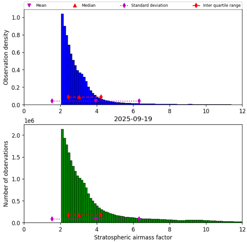
Figure 42: Histogram of “Stratospheric airmass factor” for 2025-09-19 to 2025-09-20
