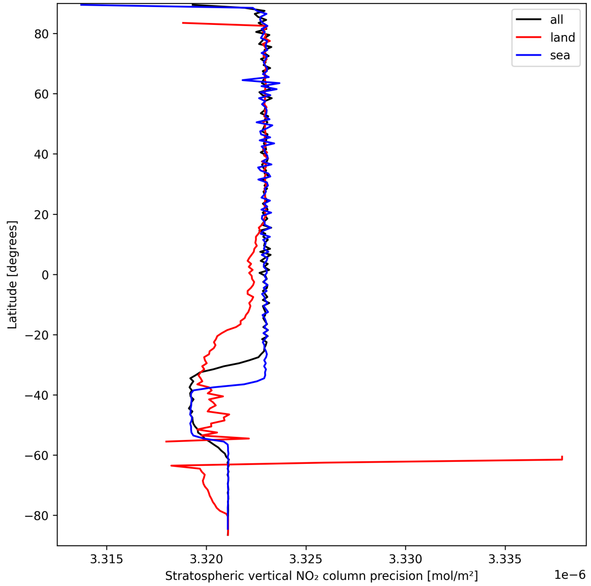
Figure 18: Zonal average of “Stratospheric vertical NO 2 column precision” for 2025-09-19 to 2025-09-20.
