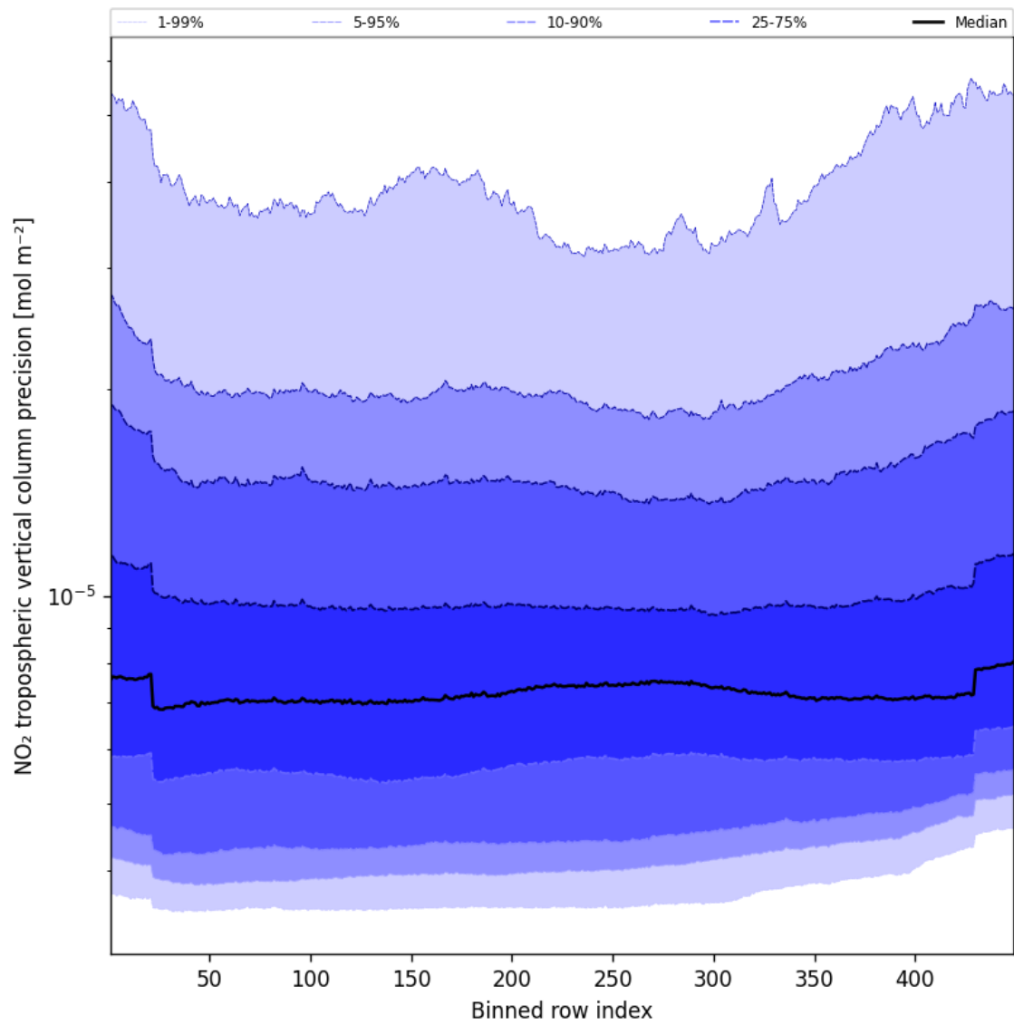
Figure 45: Along track statistics of “NO 2 tropospheric vertical column precision” for 2025-09-19 to 2025-09-20
