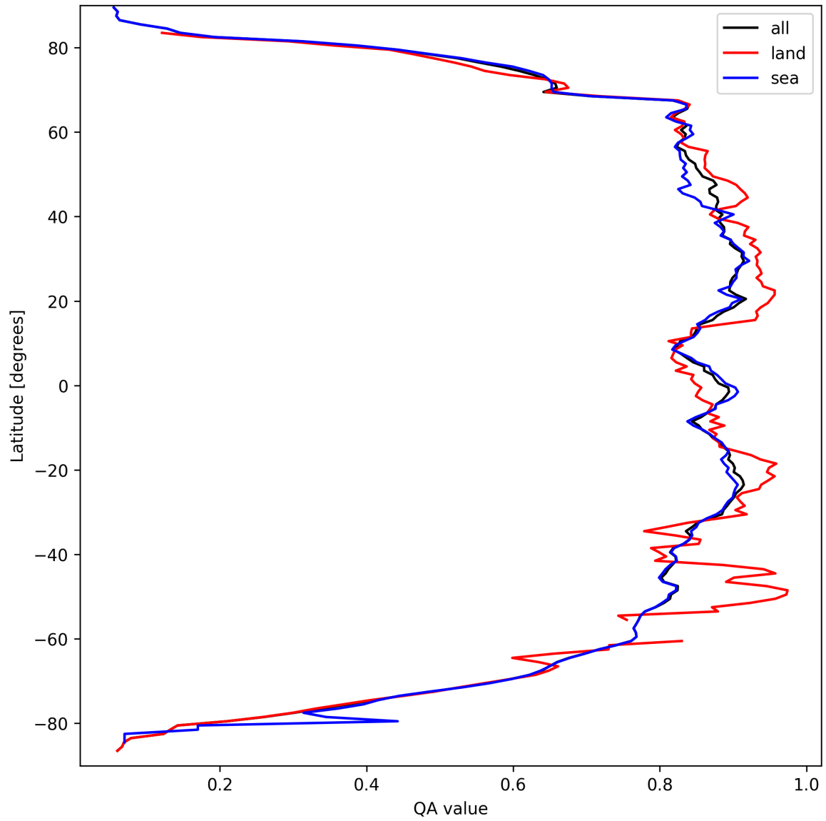
Figure 9: Zonal average of “QA value” for 2025-09-19 to 2025-09-20.
