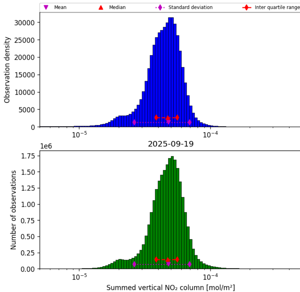
Figure 38: Histogram of “Summed vertical NO 2 column” for 2025-09-19 to 2025-09-20
