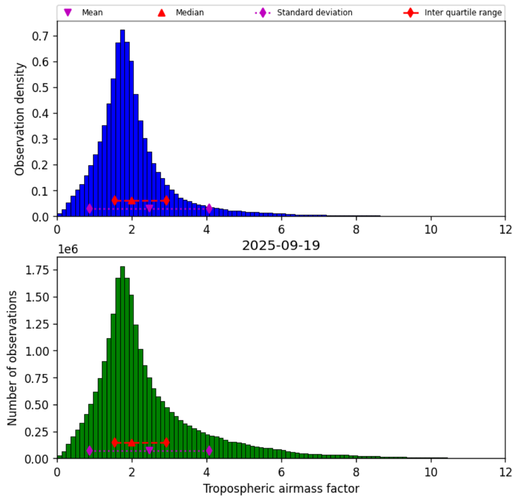
Figure 29: Histogram of “Tropospheric airmass factor” for 2025-09-19 to 2025-09-20
