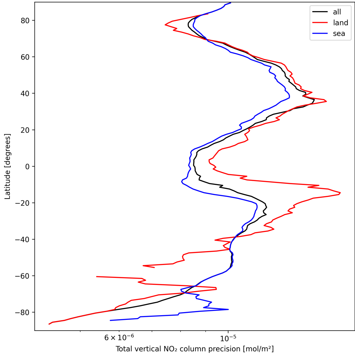
Figure 20: Zonal average of “Total vertical NO 2 column precision” for 2025-09-19 to 2025-09-20.
