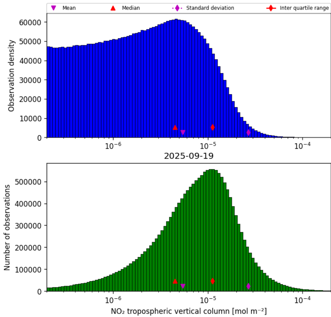
Figure 27: Histogram of “NO 2 tropospheric vertical column” for 2025-09-19 to 2025-09-20
