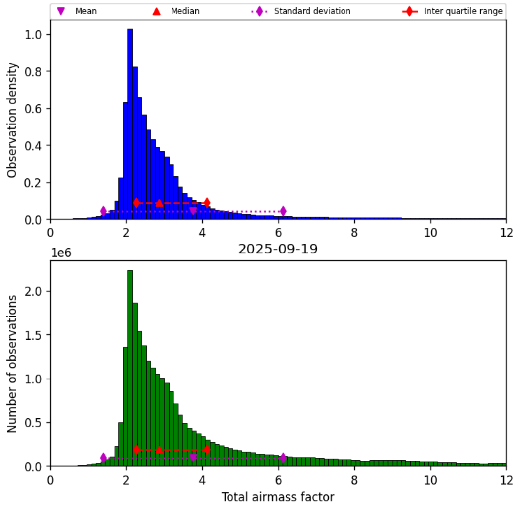
Figure 30: Histogram of “Total airmass factor” for 2025-09-19 to 2025-09-20
