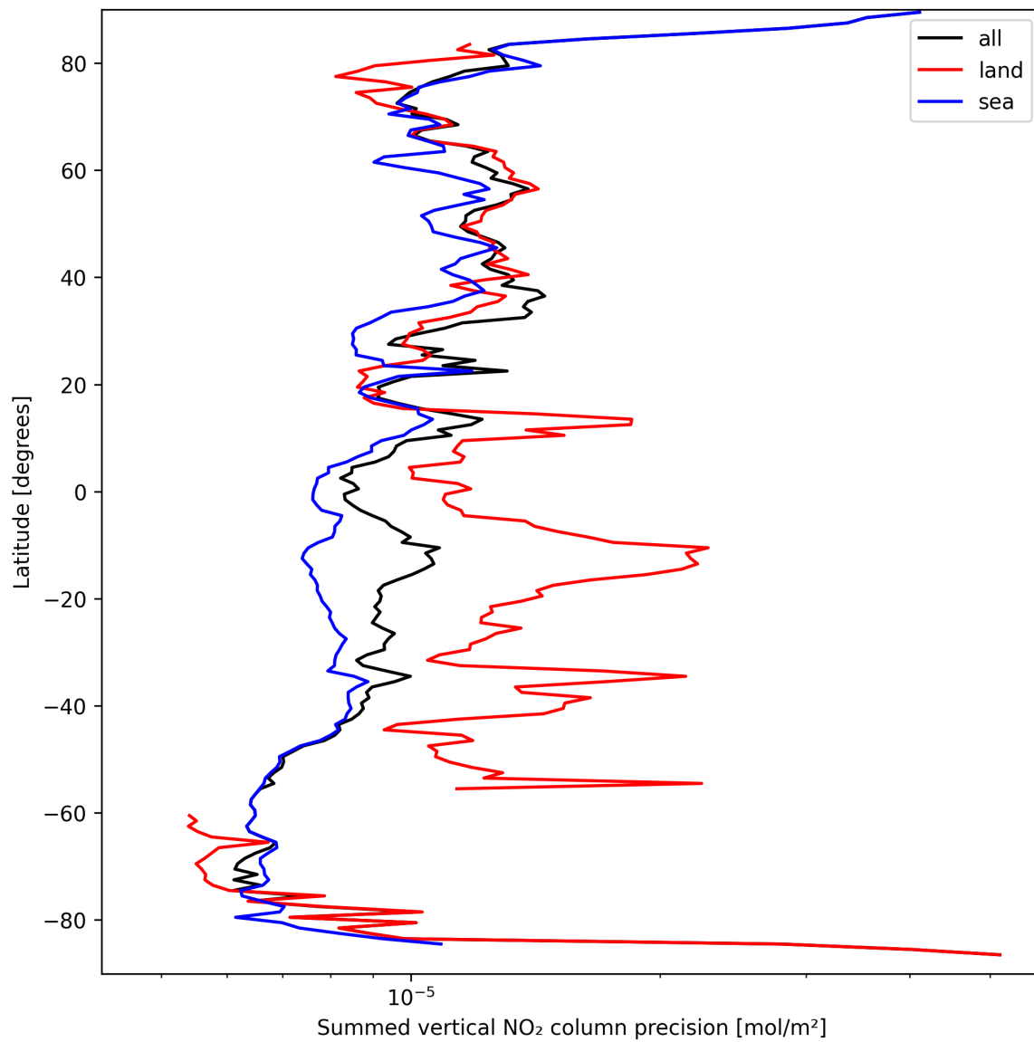
Figure 22: Zonal average of “Summed vertical NO 2 column precision” for 2025-09-19 to 2025-09-20.
