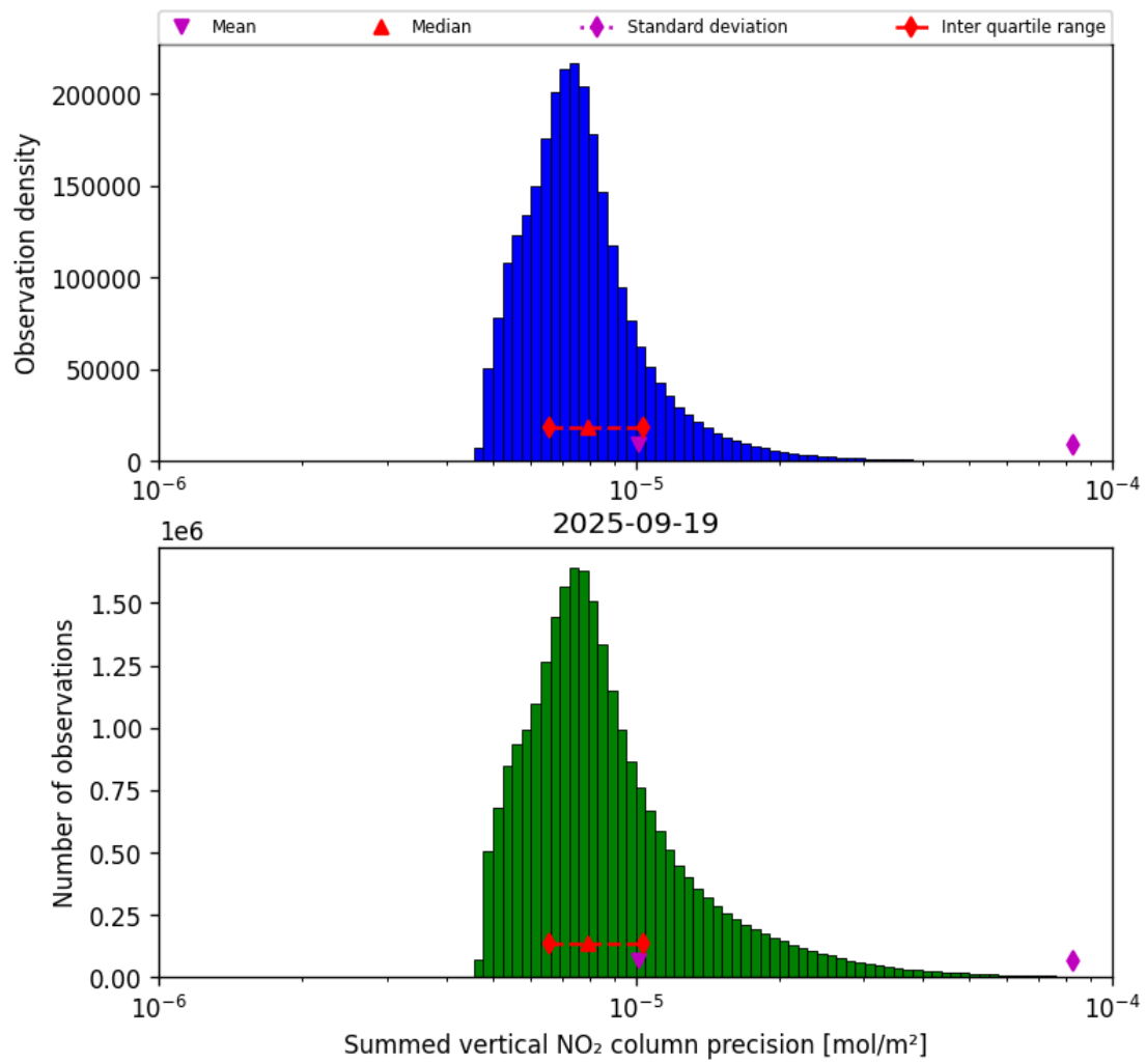
Figure 39: Histogram of "Summed vertical NO 2 column precision" for 2025-09-19 to 2025-09-20
