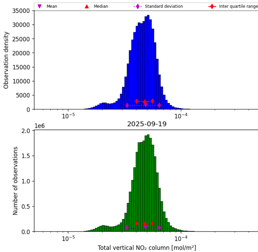
Figure 36: Histogram of “Total vertical NO 2 column” for 2025-09-19 to 2025-09-20
