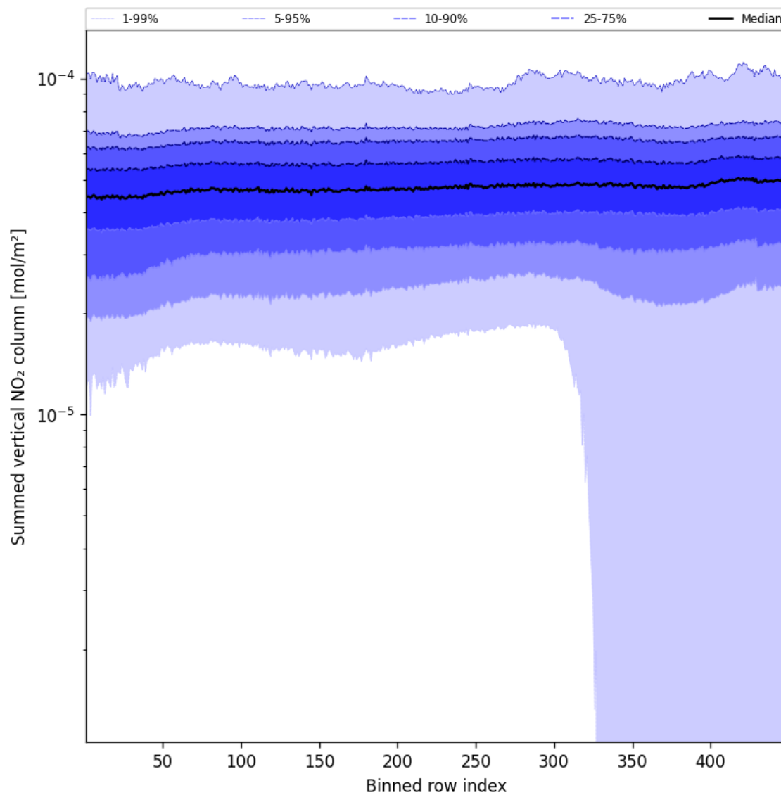
Figure 55: Along track statistics of “Summed vertical NO 2 column” for 2025-09-19 to 2025-09-20
