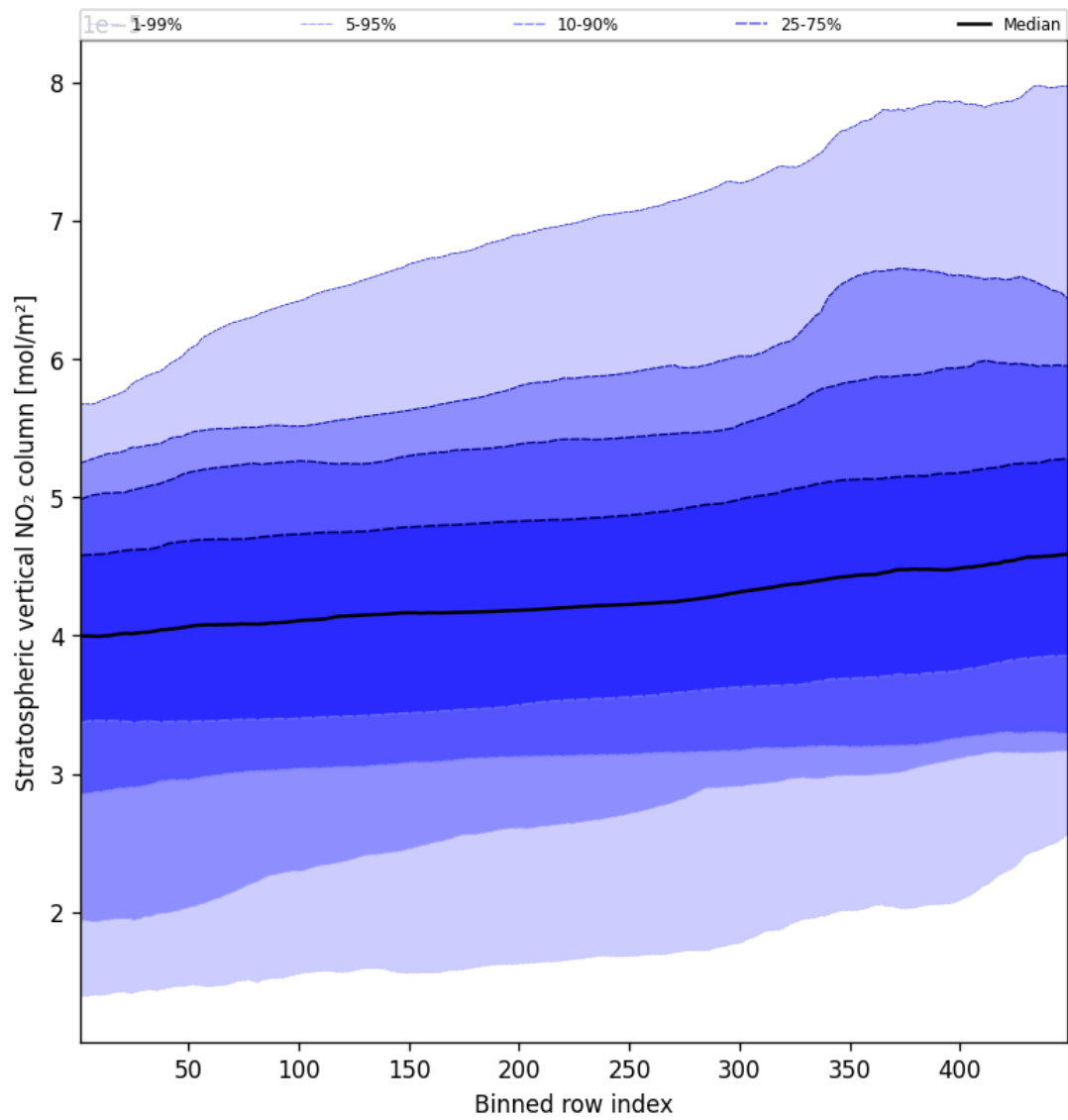
Figure 51: Along track statistics of “Stratospheric vertical NO 2 column” for 2025-09-19 to 2025-09-20
