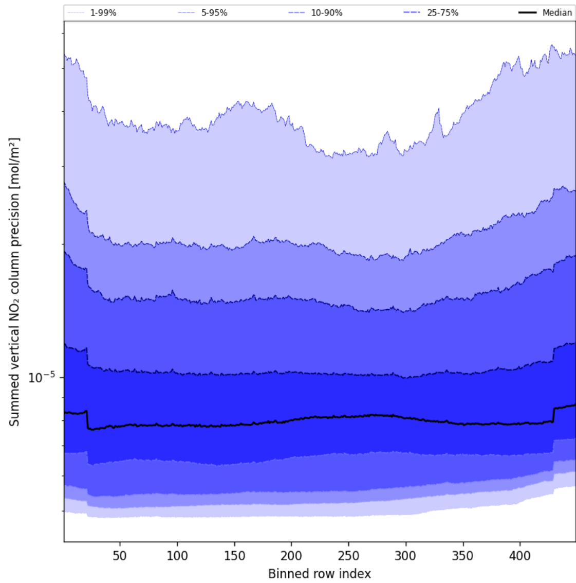
Figure 56: Along track statistics of “Summed vertical NO 2 column precision” for 2025-09-19 to 2025-09-20
