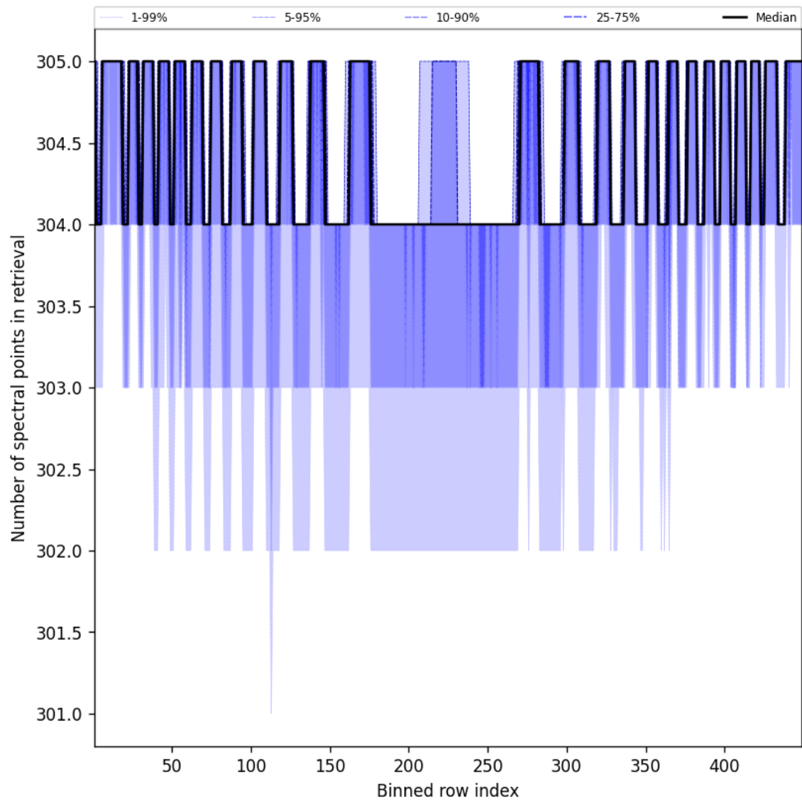
Figure 48: Along track statistics of “Number of spectral points in retrieval” for 2025-09-19 to 2025-09-20
