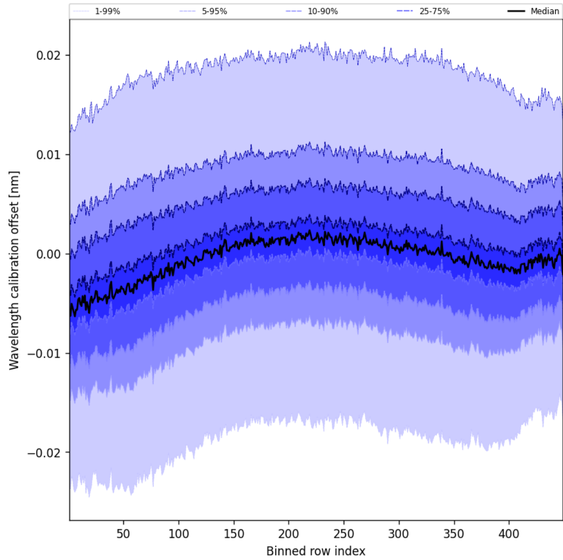
Figure 50: Along track statistics of “Wavelength calibration offset” for 2025-09-19 to 2025-09-20
