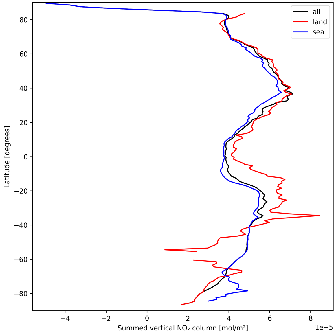
Figure 21: Zonal average of “Summed vertical NO 2 column” for 2025-09-19 to 2025-09-20.
