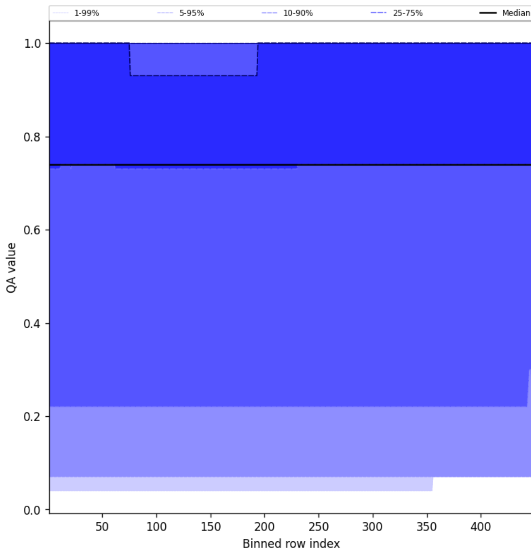
Figure 43: Along track statistics of “QA value” for 2025-09-19 to 2025-09-20
