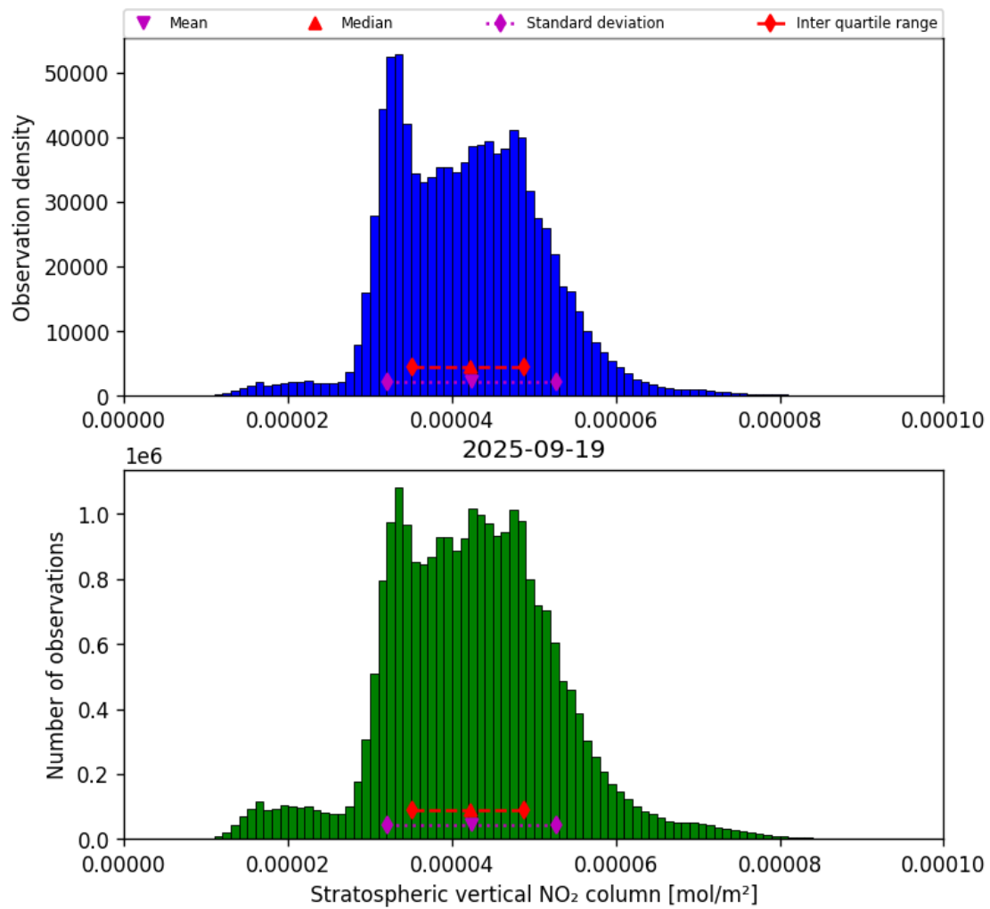
Figure 34: Histogram of “Stratospheric vertical NO 2 column” for 2025-09-19 to 2025-09-20
