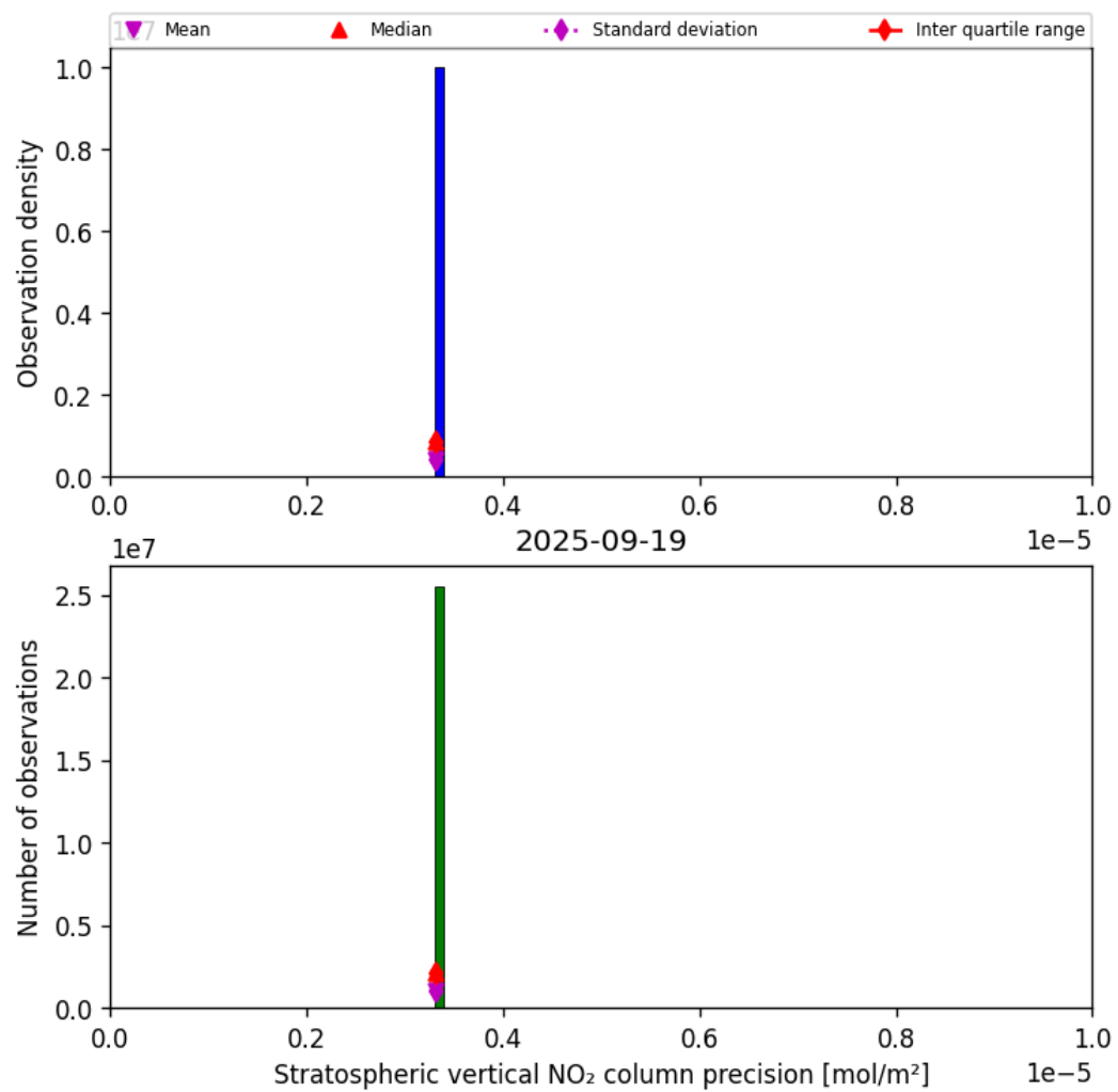
Figure 35: Histogram of “Stratospheric vertical NO 2 column precision” for 2025-09-19 to 2025-09-20
