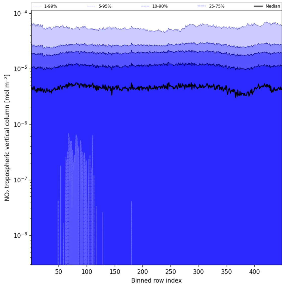
Figure 44: Along track statistics of “NO 2 tropospheric vertical column” for 2025-09-19 to 2025-09-20
