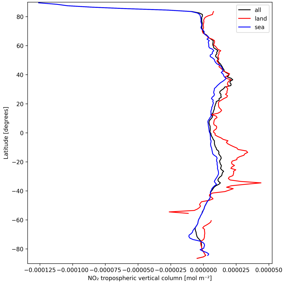
Figure 10: Zonal average of “NO 2 tropospheric vertical column” for 2025-09-19 to 2025-09-20.
